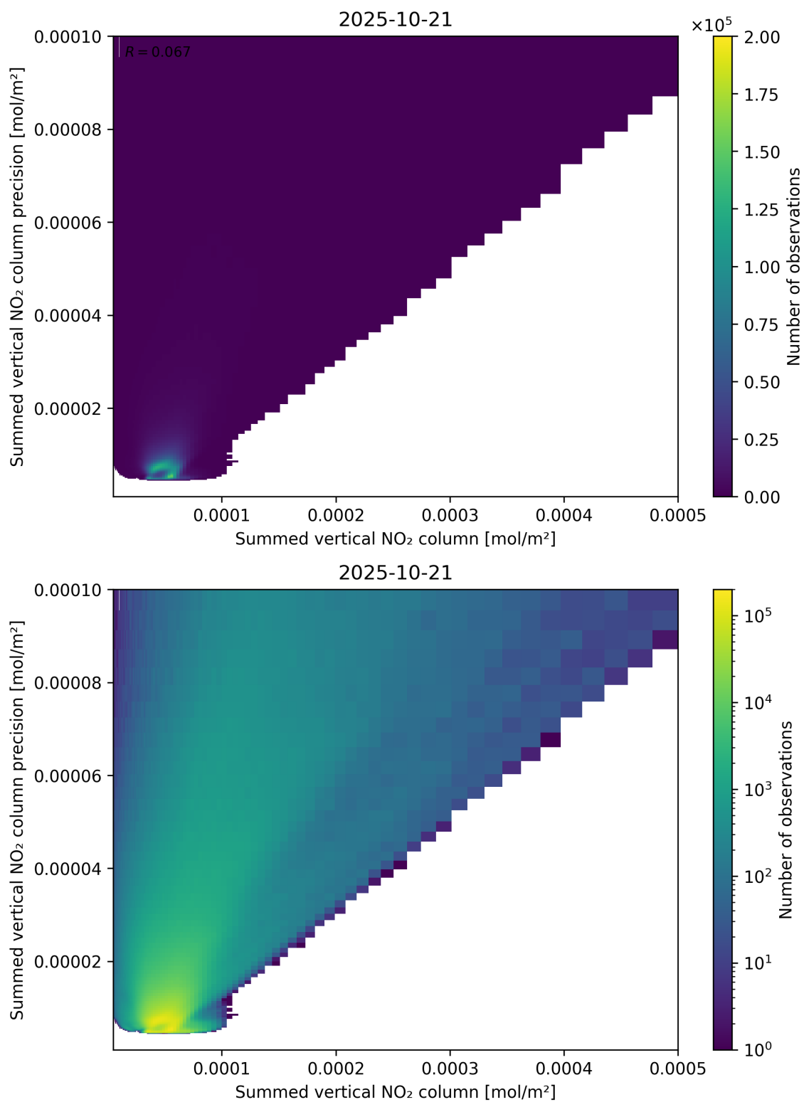
Figure 105: Scatter density plot of “Summed vertical NO 2 column” against “Summed vertical NO 2 column precision” for 2025-10-20 to 2025-10-22.
