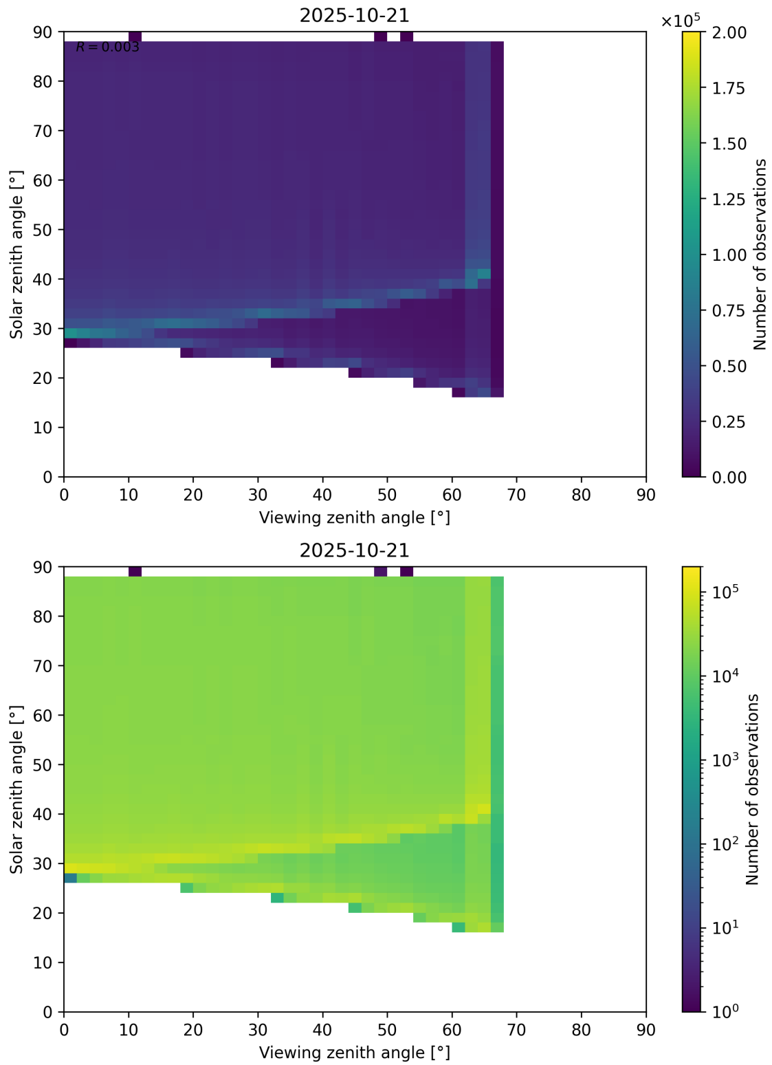
Figure 172: Scatter density plot of “Viewing zenith angle” against “Solar zenith angle” for 2025-10-20 to 2025-10-22.
