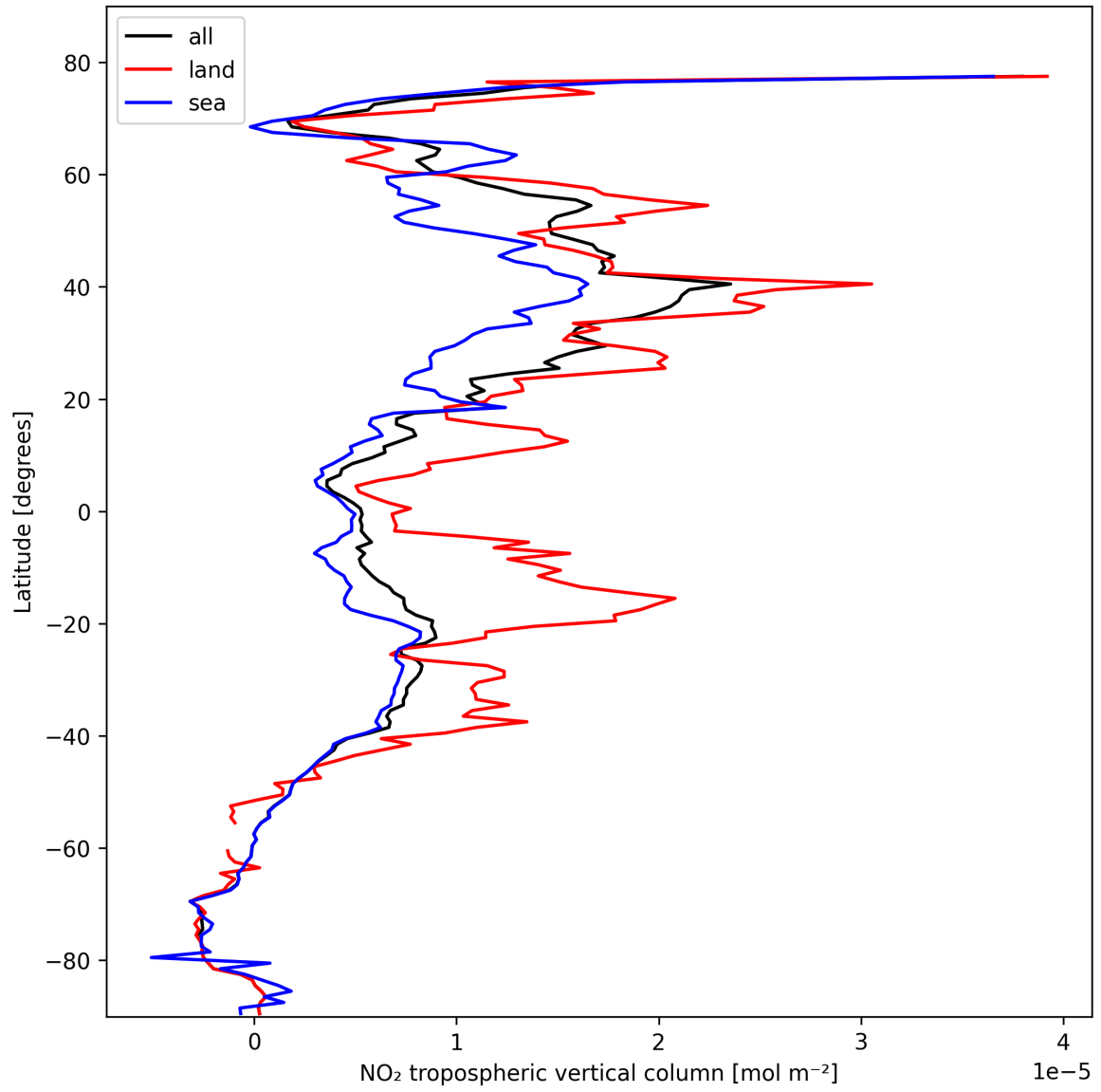
Figure 12: Zonal average of “NO 2 tropospheric vertical column” for 2025-10-20 to 2025-10-22.
