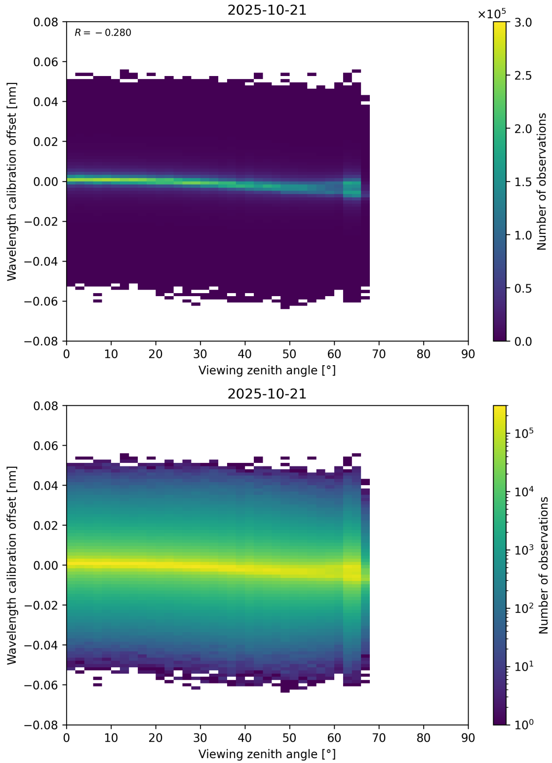
Figure 173: Scatter density plot of “Viewing zenith angle” against “Wavelength calibration offset” for 2025-10-20 to 2025-10-22.
