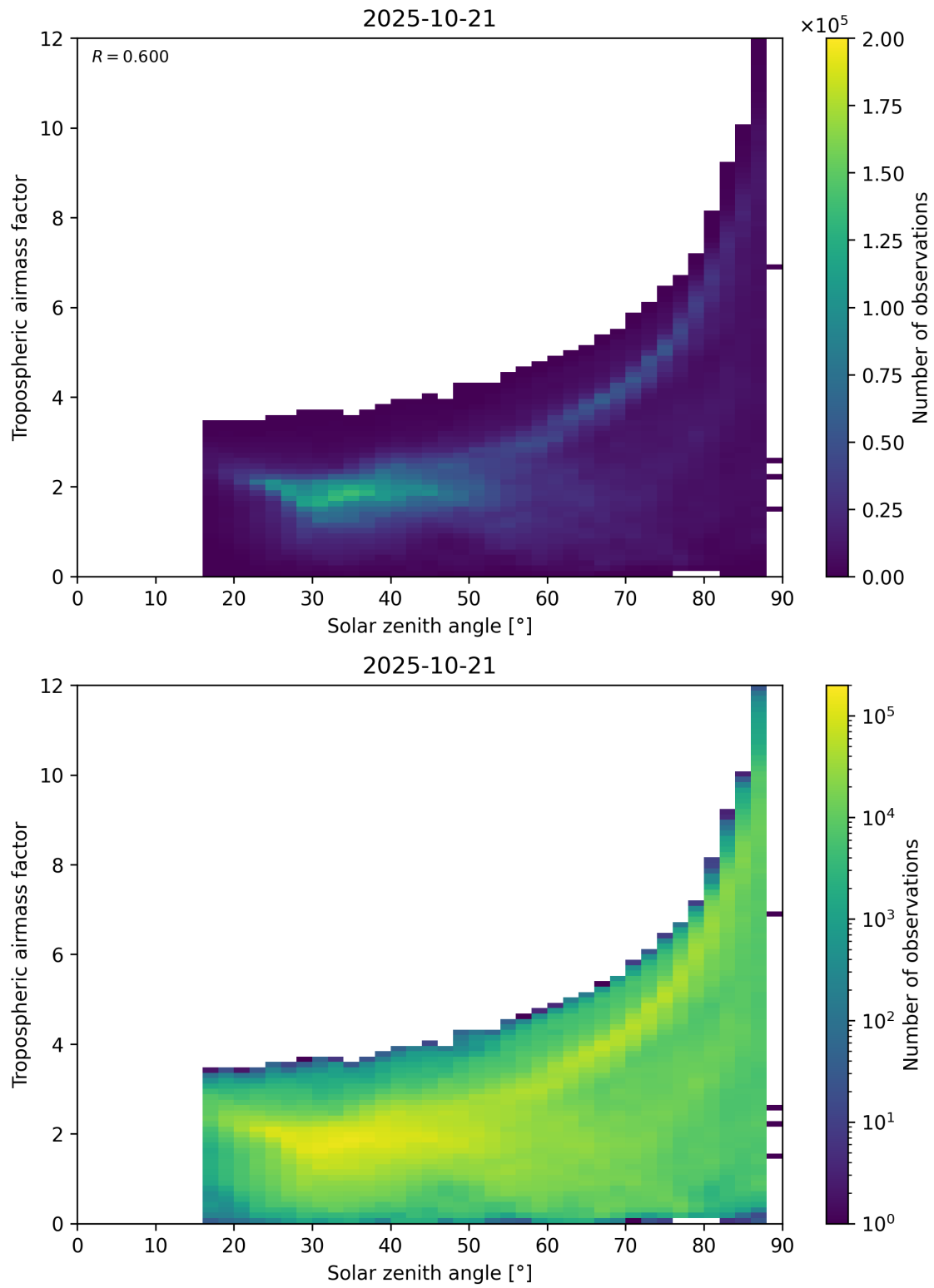
Figure 147: Scatter density plot of “Solar zenith angle” against “Tropospheric airmass factor” for 2025-10-20 to 2025-10-22.
