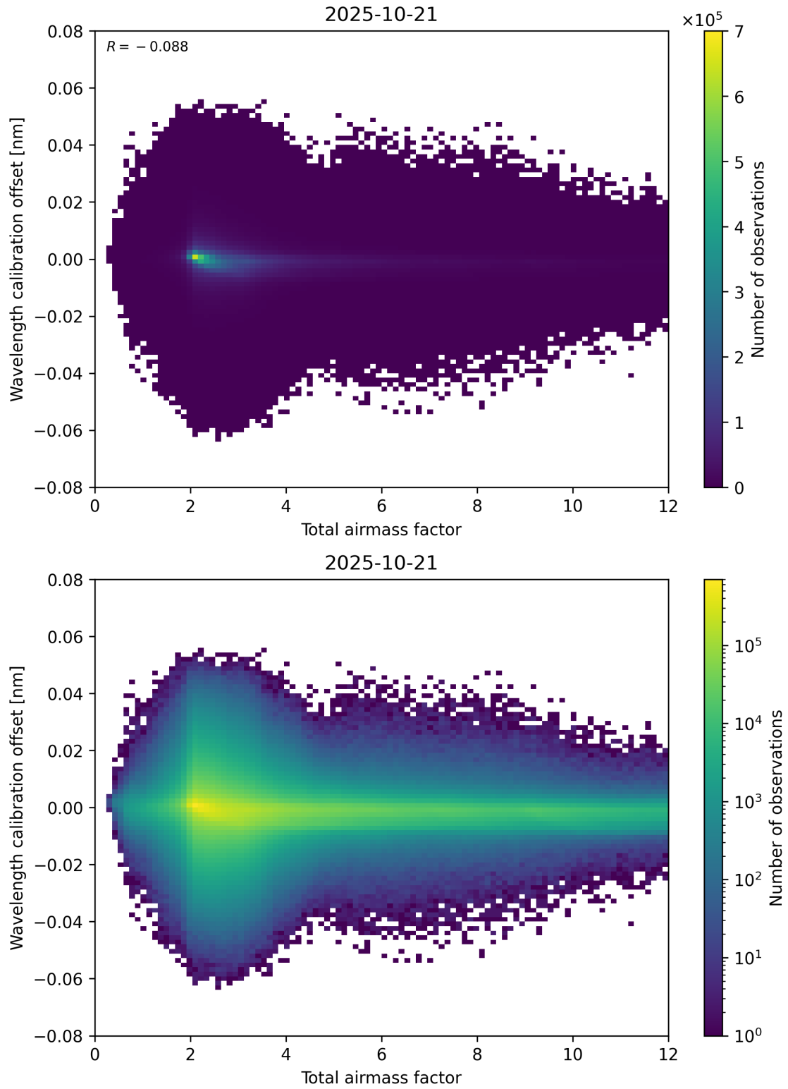
Figure 70: Scatter density plot of “Total airmass factor” against “Wavelength calibration offset” for 2025-10-20 to 2025-10-22.
