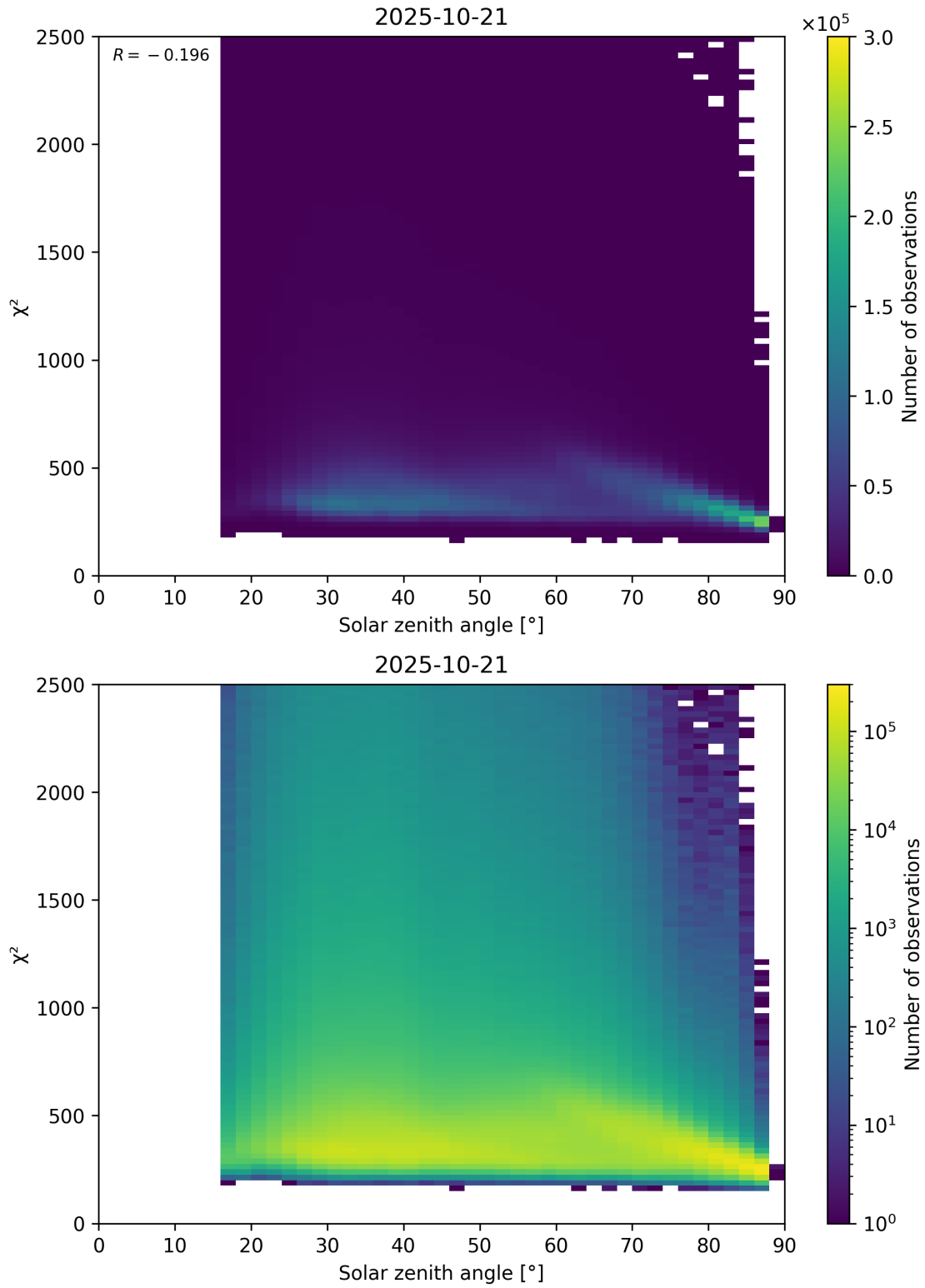
Figure 148: Scatter density plot of “Solar zenith angle” against “ \chi^2 ” for 2025-10-20 to 2025-10-22.
