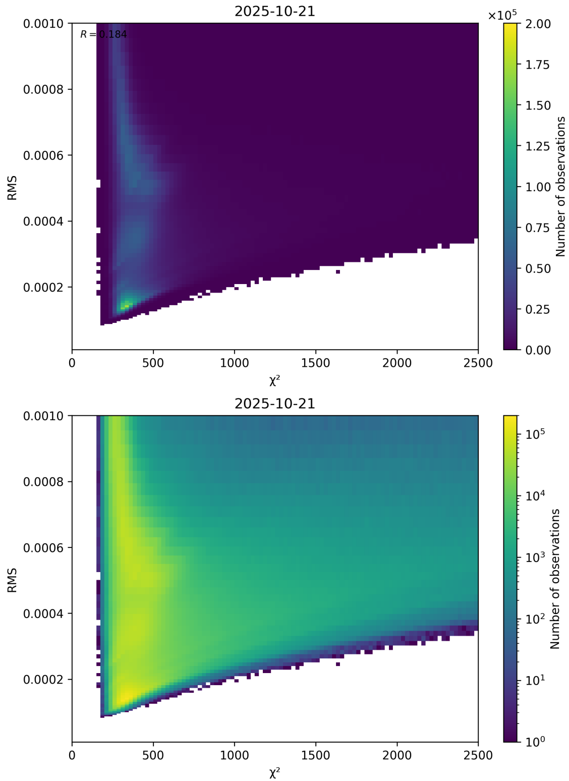
Figure 82: Scatter density plot of “ \chi^2 ” against “RMS” for 2025-10-20 to 2025-10-22.
