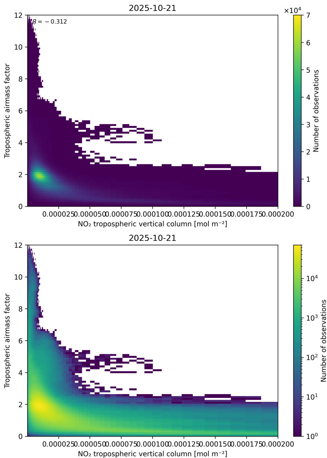
Figure 123: Scatter density plot of “NO 2 tropospheric vertical column” against “Tropospheric air mass factor” for 2025-10-20 to 2025-10-22.
