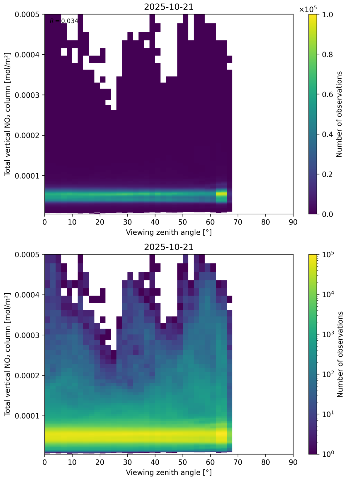
Figure 167: Scatter density plot of “Viewing zenith angle” against “Total vertical NO 2 column” for 2025-10-20 to 2025-10-22.
