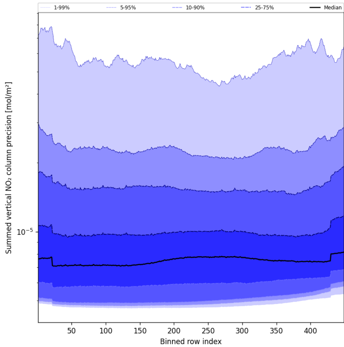
Figure 58: Along track statistics of “Summed vertical NO 2 column precision” for 2025-10-20 to 2025-10-22
