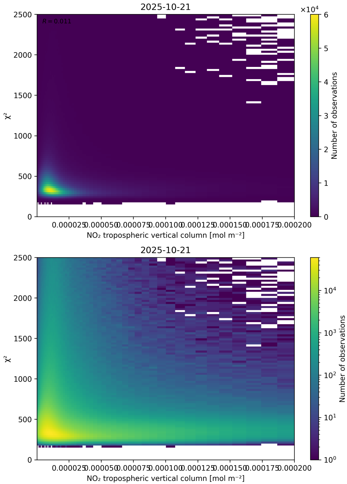
Figure 124: Scatter density plot of “NO 2 tropospheric vertical column” against “ \chi^2 ” for 2025-10-20 to 2025-10-22.
