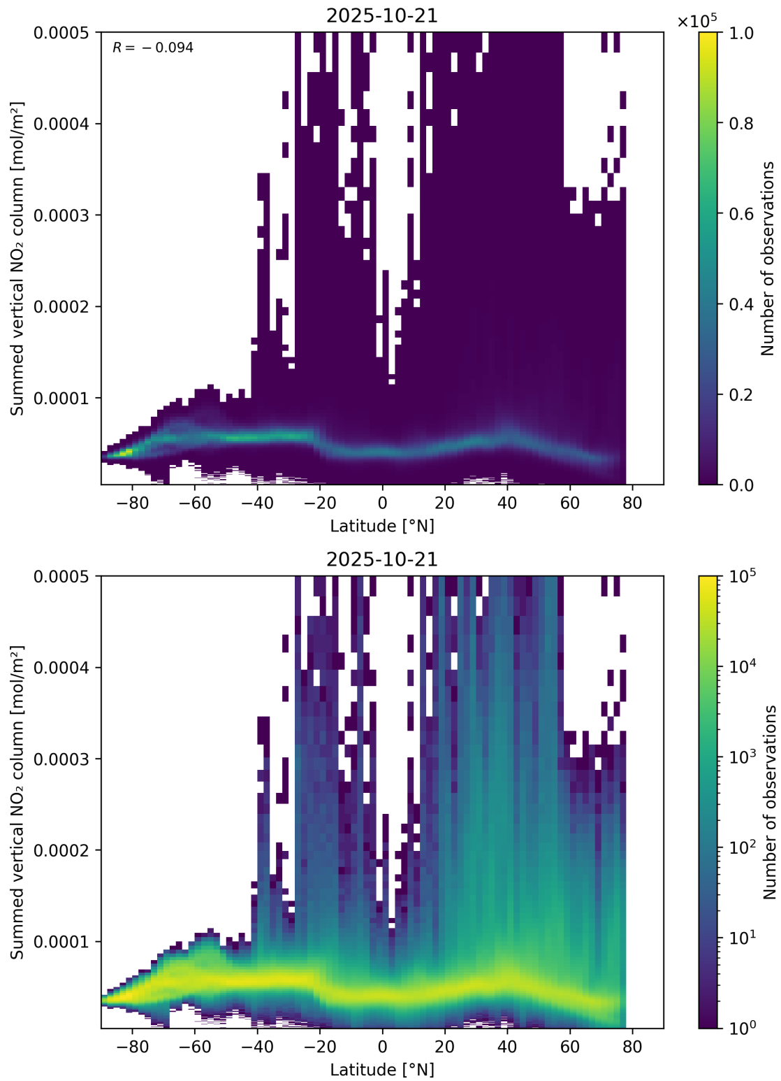
Figure 88: Scatter density plot of “Latitude” against “Summed vertical NO 2 column” for 2025-10-20 to 2025-10-22.
