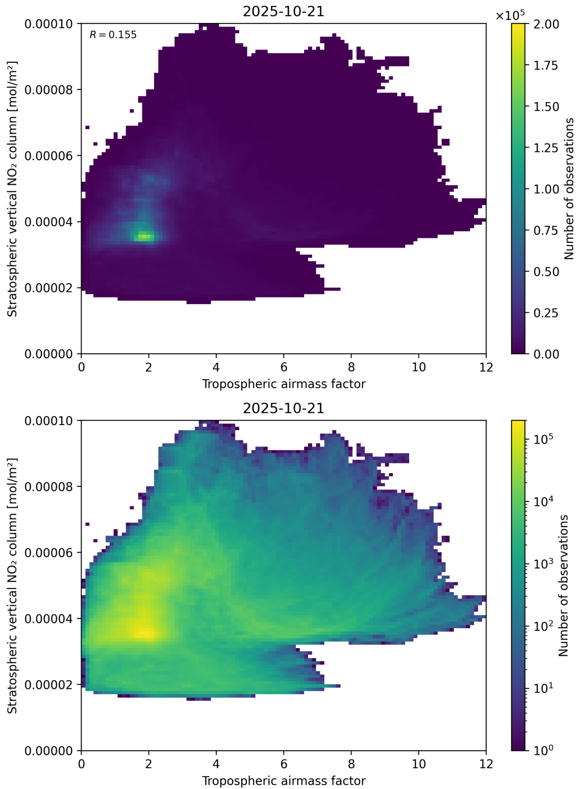
Figure 74: Scatter density plot of “Tropospheric air mass factor” against “Stratospheric vertical NO 2 column” for 2025-10-20 to 2025-10-22.
