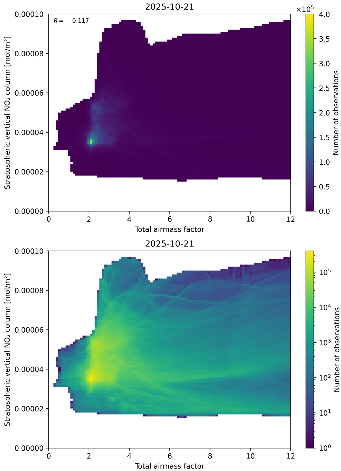
Figure 64: Scatter density plot of “Total airmass factor” against “Stratospheric vertical NO 2 column” for 2025-10-20 to 2025-10-22.
