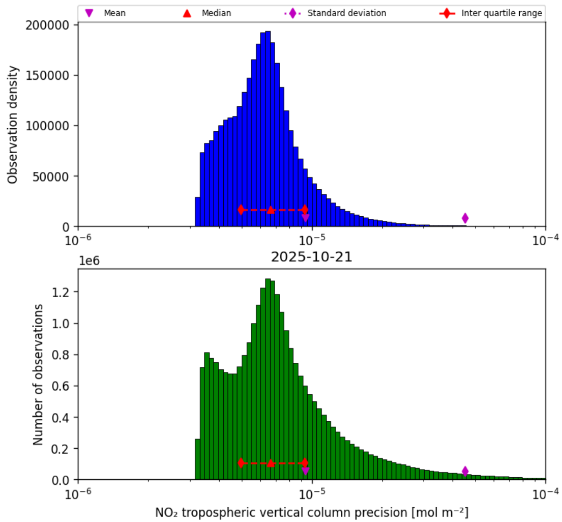
Figure 30: Histogram of “NO 2 tropospheric vertical column precision” for 2025-10-20 to 2025-10-22
