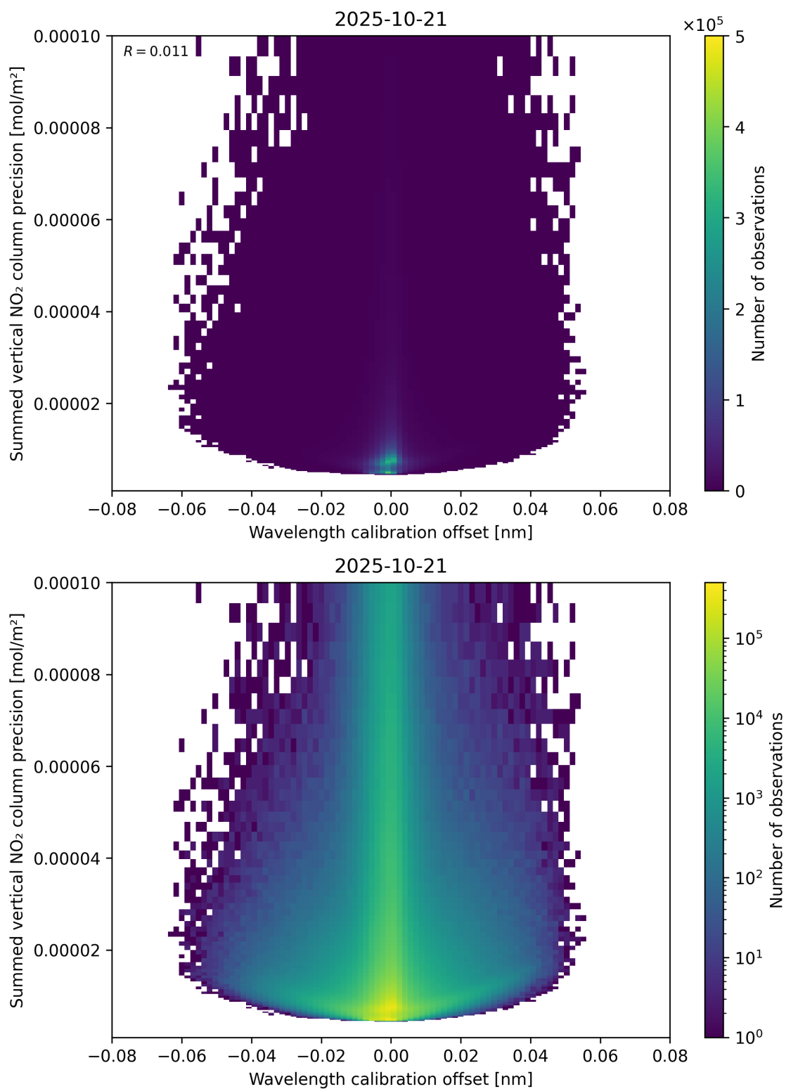
Figure 178: Scatter density plot of “Wavelength calibration offset” against “Summed vertical NO 2 column precision” for 2025-10-20 to 2025-10-22.
