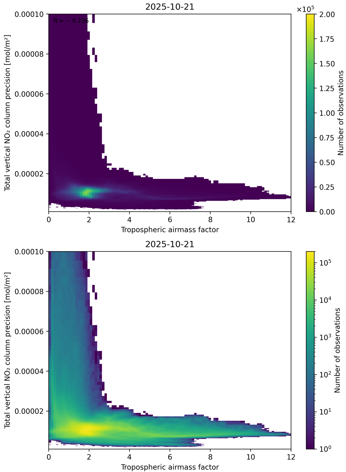
Figure 78: Scatter density plot of “Tropospheric airmass factor” against “Total vertical NO 2 column precision” for 2025-10-20 to 2025-10-22.
