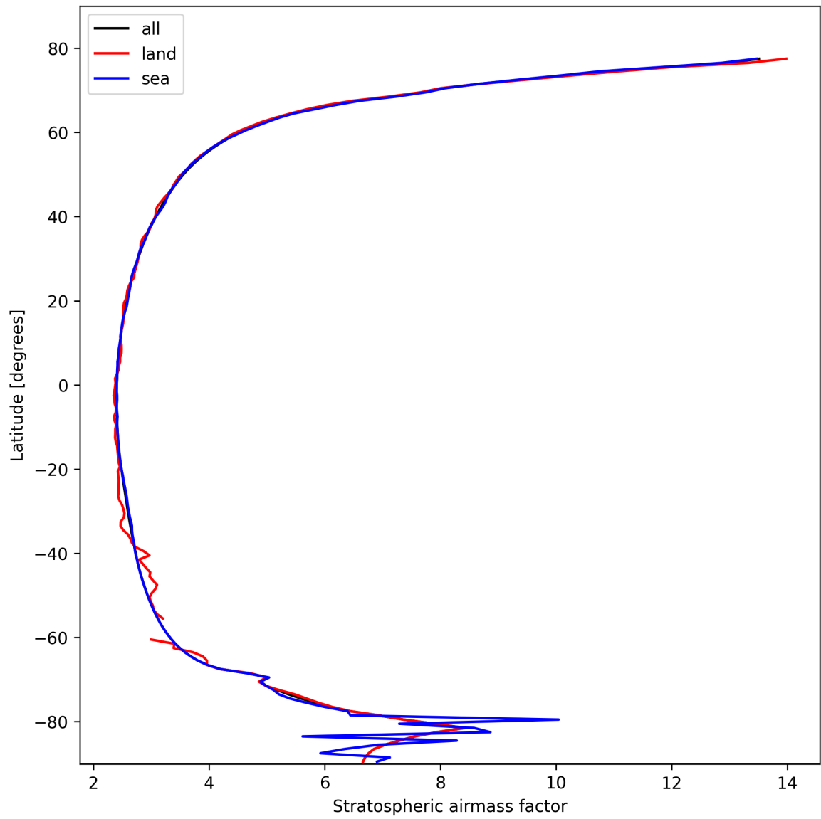
Figure 27: Zonal average of “Stratospheric airmass factor” for 2025-10-20 to 2025-10-22.
