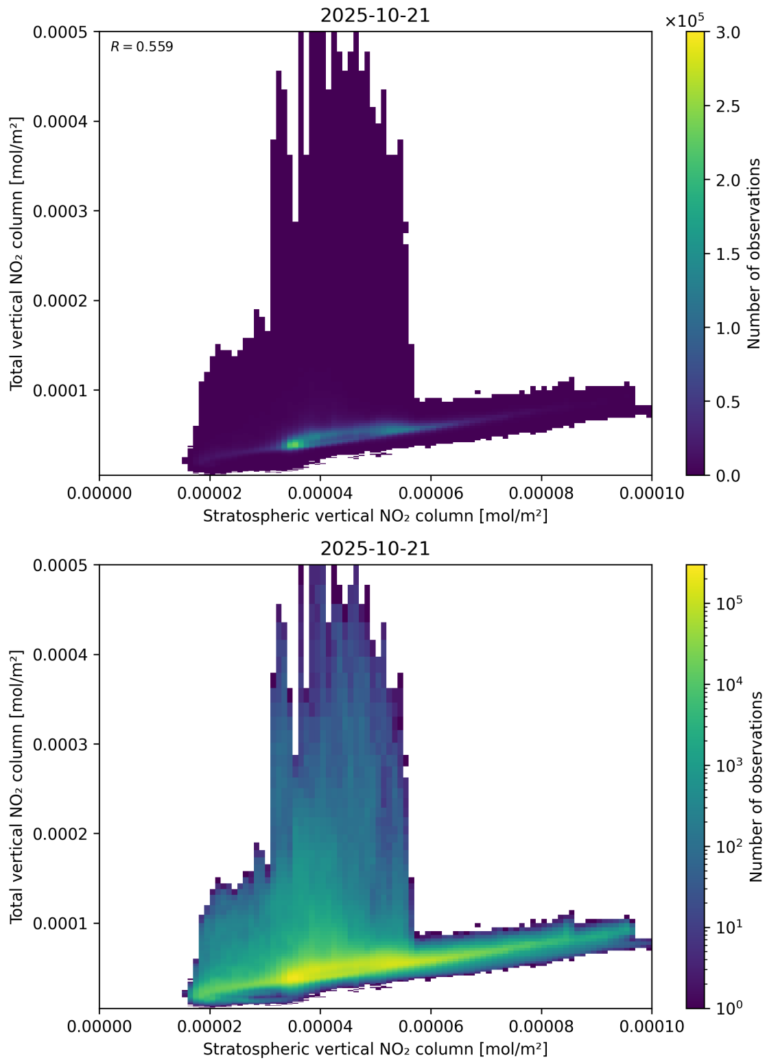
Figure 100: Scatter density plot of “Stratospheric vertical NO 2 column” against “Total vertical NO 2 column” for 2025-10-20 to 2025-10-22.
