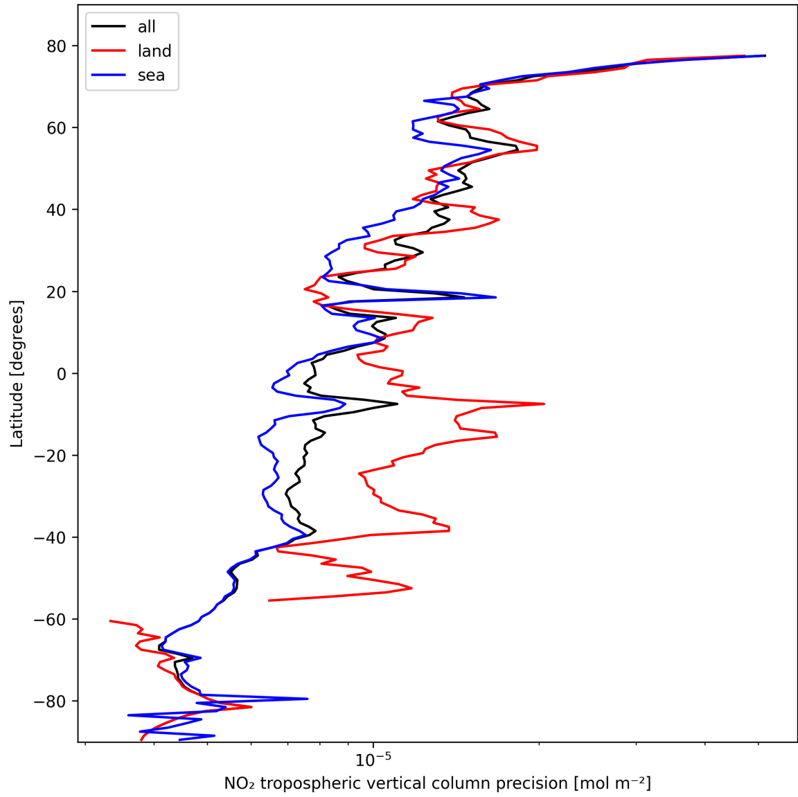
Figure 13: Zonal average of “NO 2 tropospheric vertical column precision” for 2025-10-20 to 2025-10-22.
