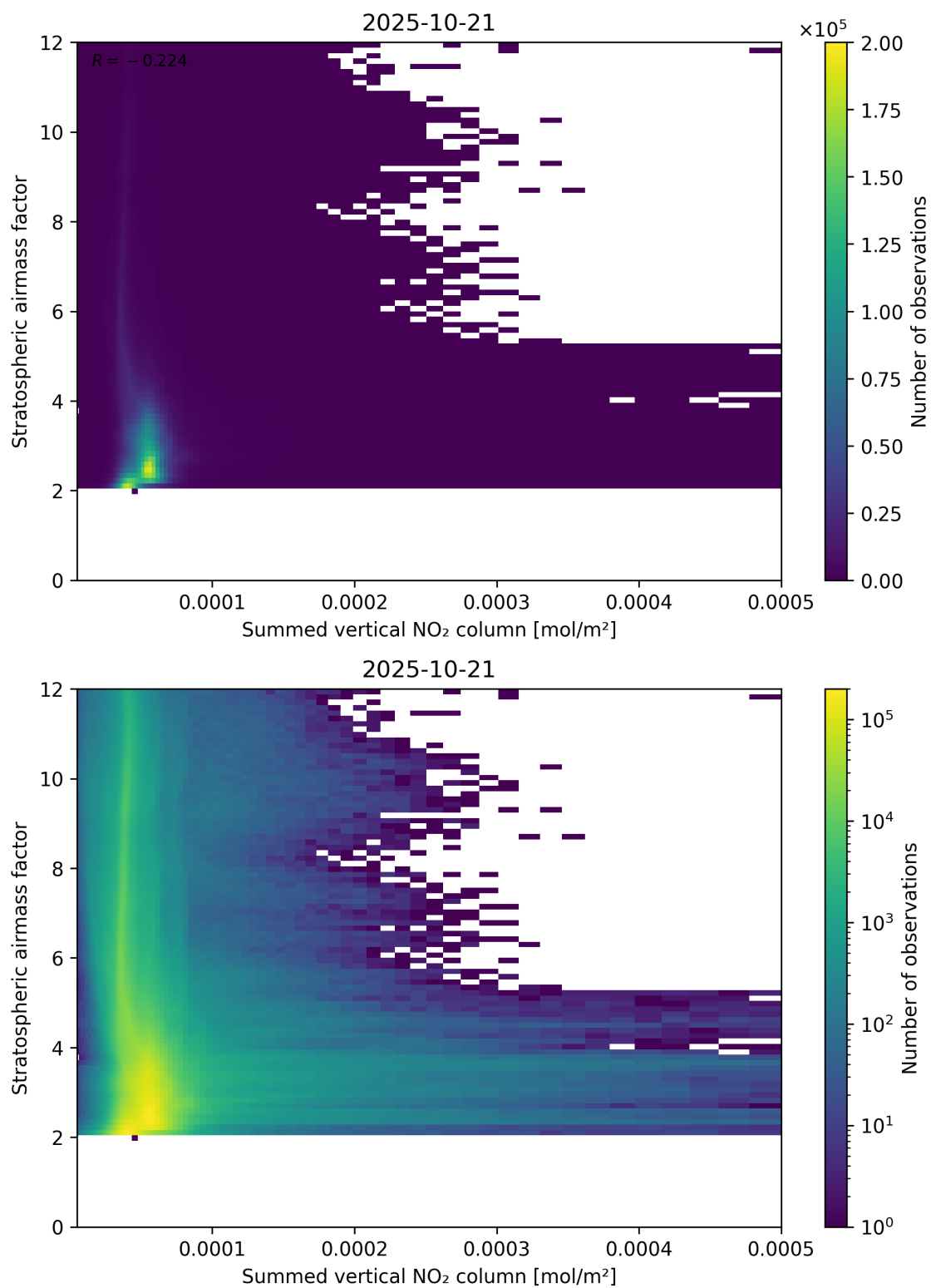
Figure 103: Scatter density plot of “Summed vertical NO 2 column” against “Stratospheric air mass factor” for 2025-10-20 to 2025-10-22.
