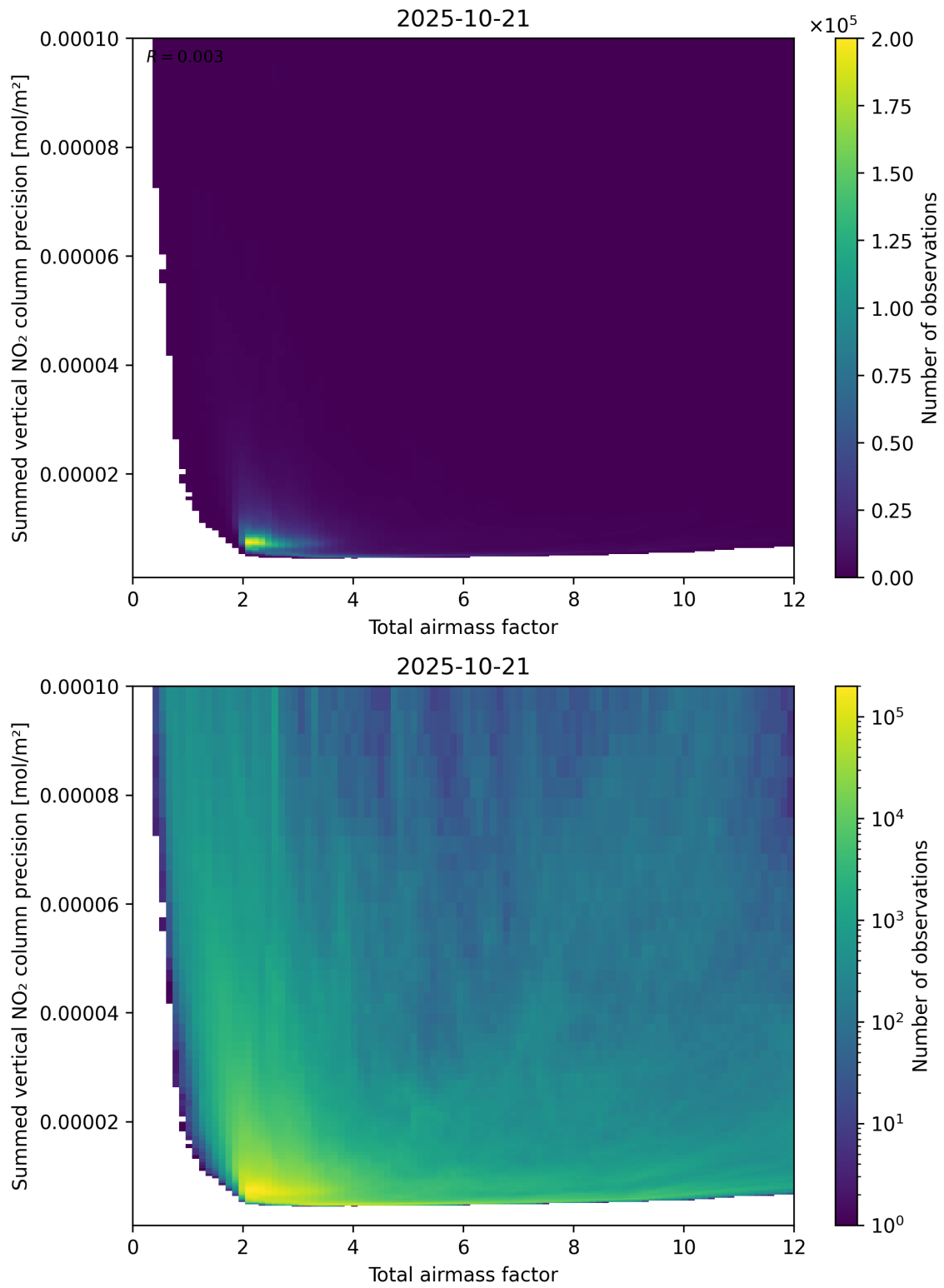
Figure 66: Scatter density plot of “Total airmass factor” against “Summed vertical NO 2 column precision” for 2025-10-20 to 2025-10-22.
