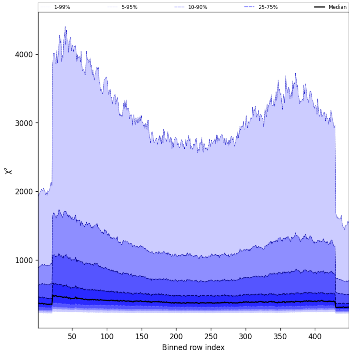
Figure 59: Along track statistics of “ \chi^2 ” for 2025-10-20 to 2025-10-22
