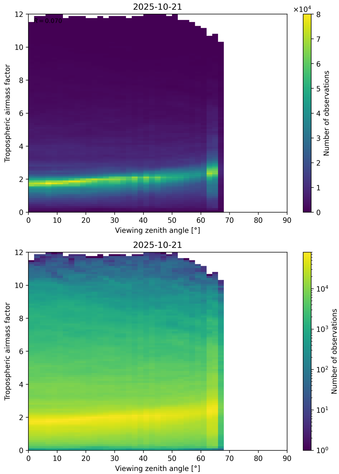
Figure 161: Scatter density plot of “Viewing zenith angle” against “Tropospheric airmass factor” for 2025-10-20 to 2025-10-22.
