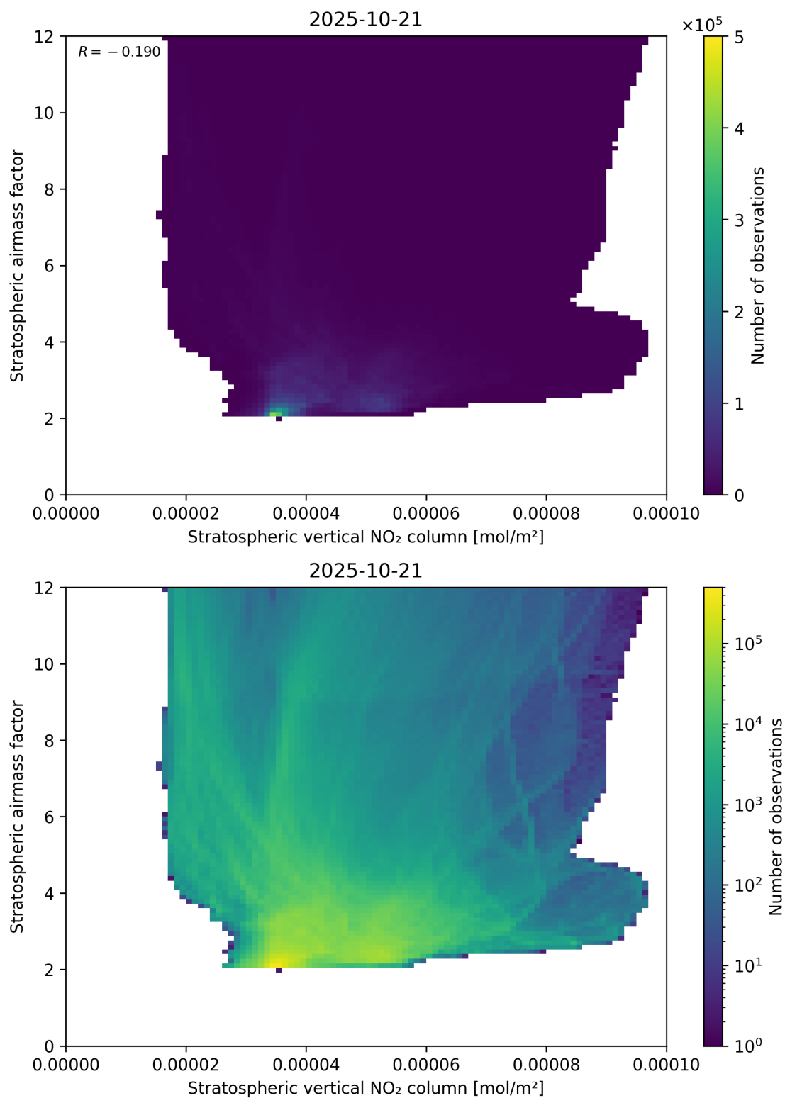
Figure 96: Scatter density plot of “Stratospheric vertical NO 2 column” against “Stratospheric airmass factor” for 2025-10-20 to 2025-10-22.
