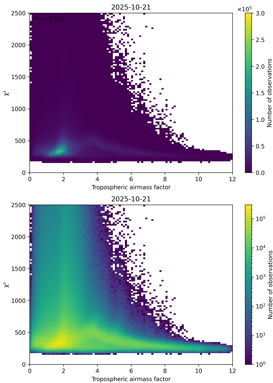
Figure 73: Scatter density plot of “Tropospheric airmass factor” against “ \chi^2 ” for 2025-10-20 to 2025-10-22.
