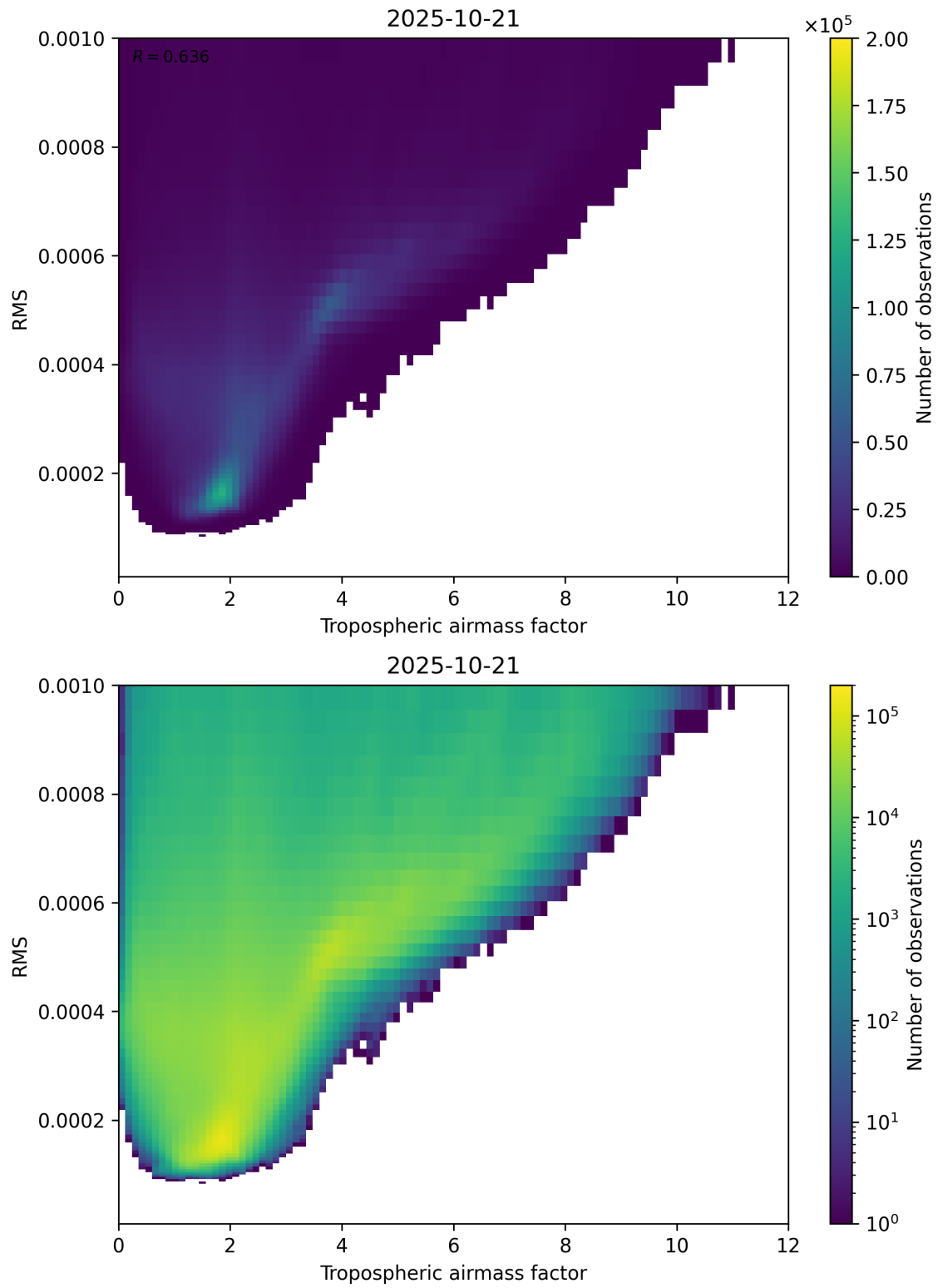
Figure 79: Scatter density plot of “Tropospheric airmass factor” against “RMS” for 2025-10-20 to 2025-10-22.
