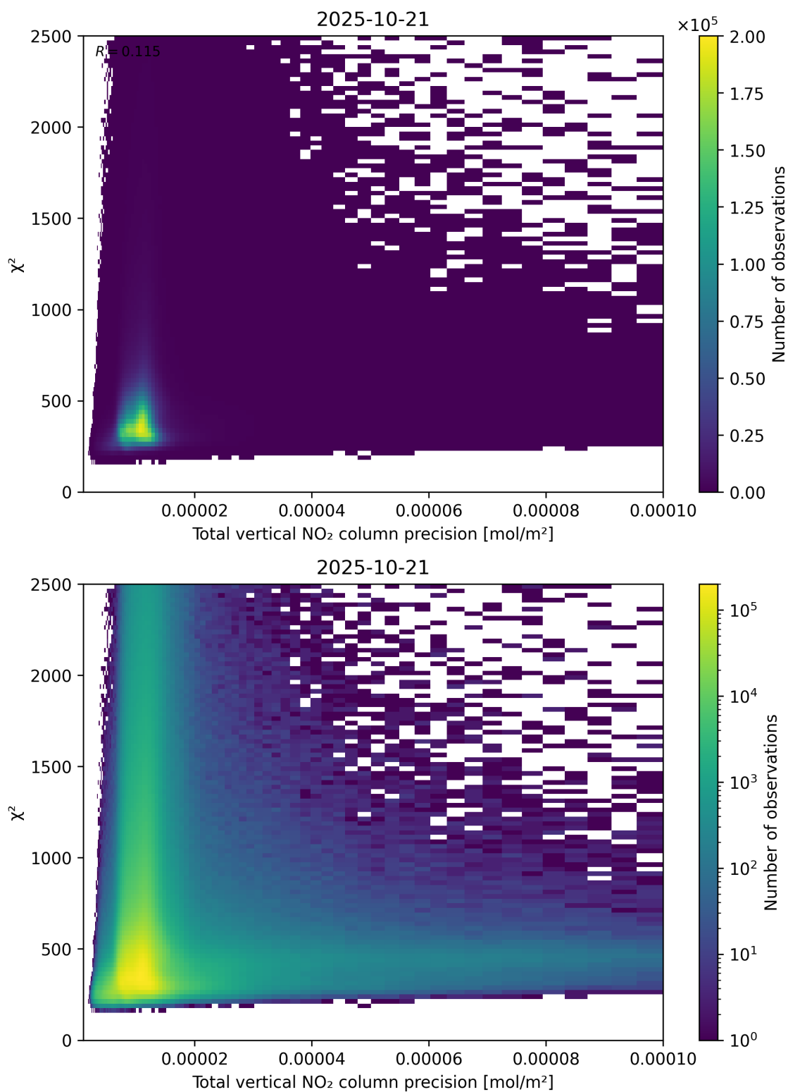
Figure 116: Scatter density plot of “Total vertical NO 2 column precision” against “ \chi^2 ” for 2025-10-20 to 2025-10-22.
