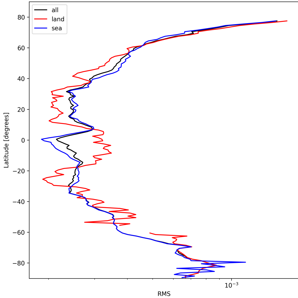
Figure 26: Zonal average of “RMS” for 2025-10-20 to 2025-10-22.
