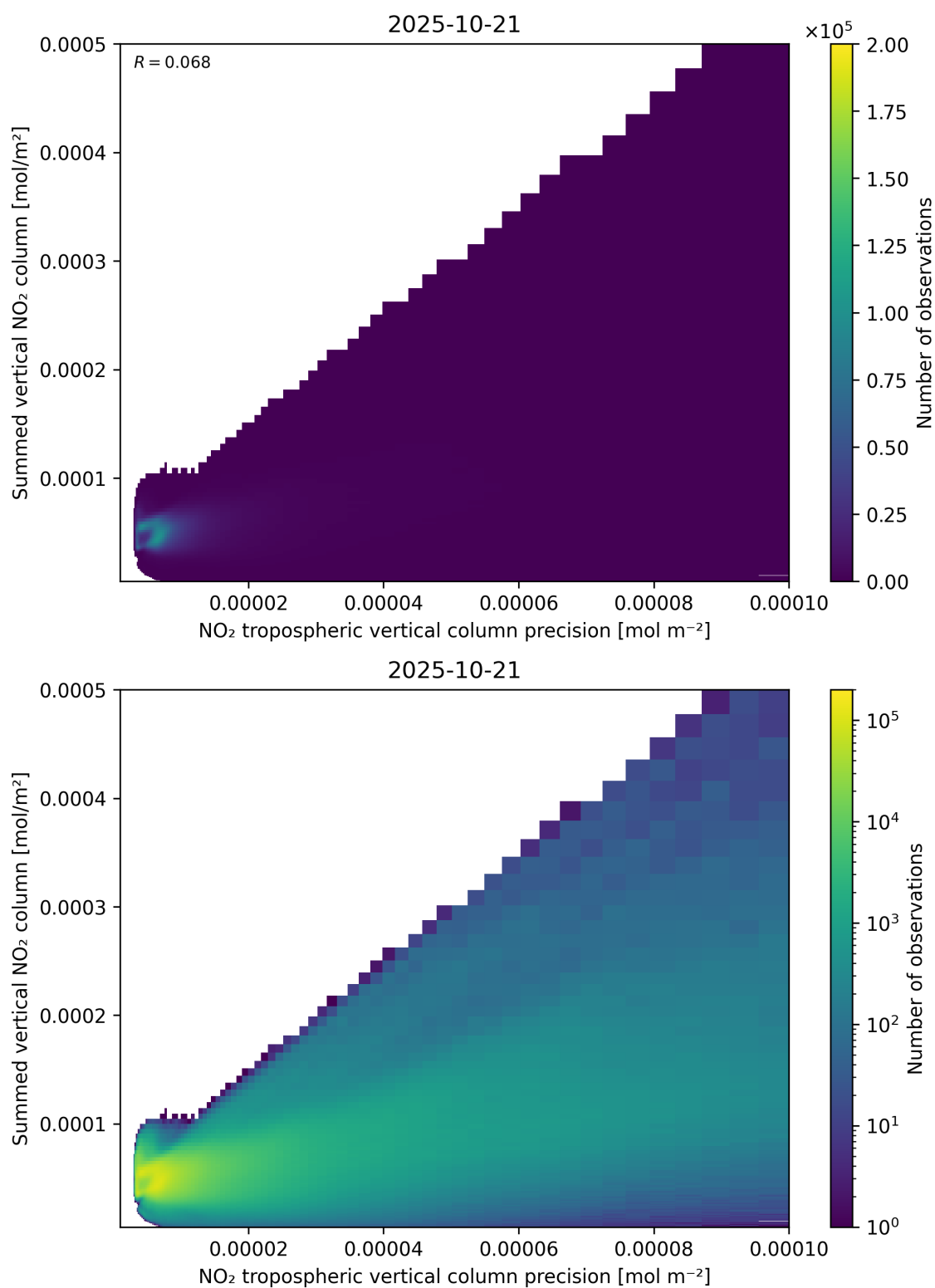
Figure 136: Scatter density plot of “NO 2 tropospheric vertical column precision” against “Summed vertical NO 2 column” for 2025-10-20 to 2025-10-22.
