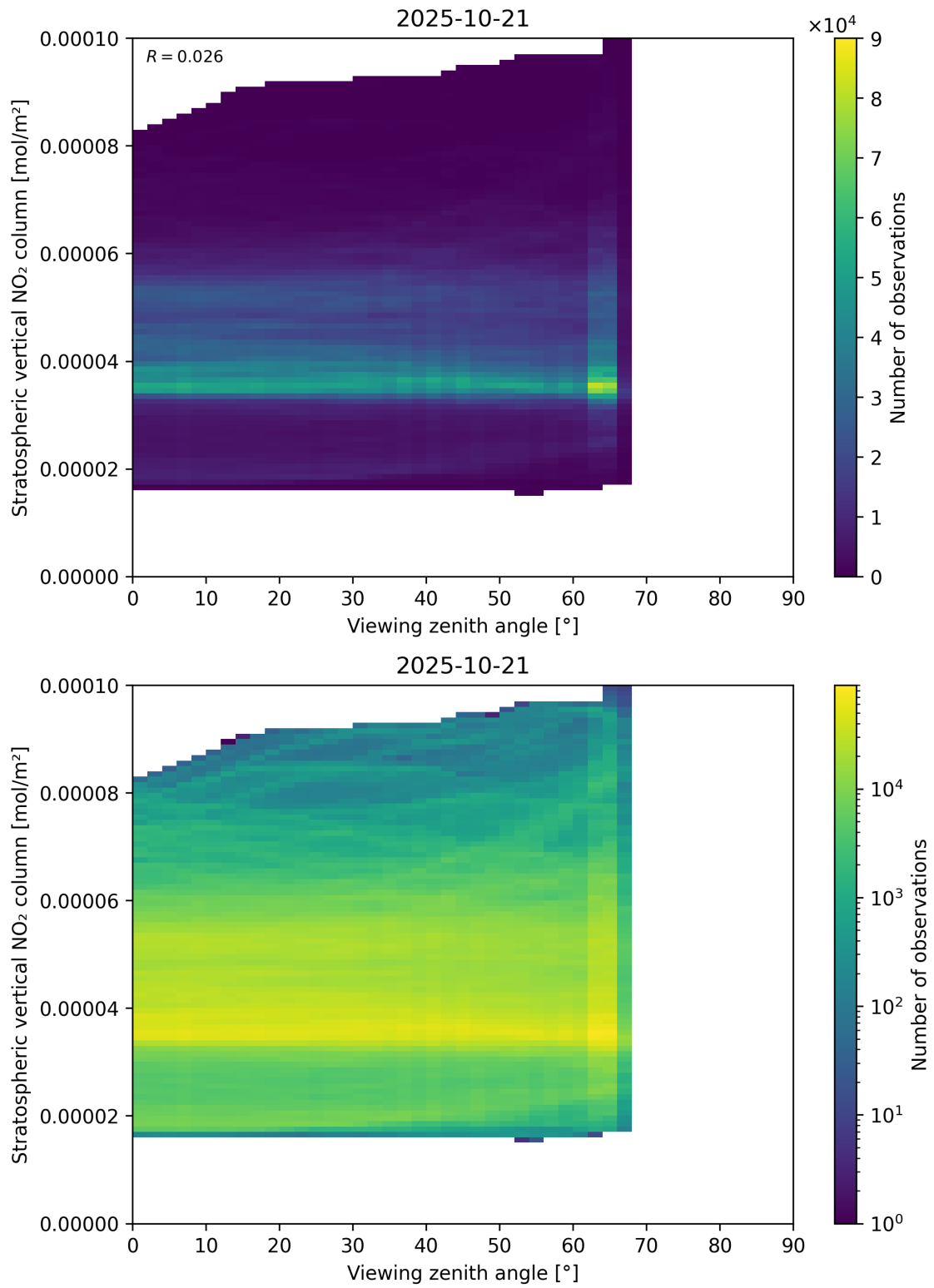
Figure 164: Scatter density plot of “Viewing zenith angle” against “Stratospheric vertical NO 2 column” for 2025-10-20 to 2025-10-22.
