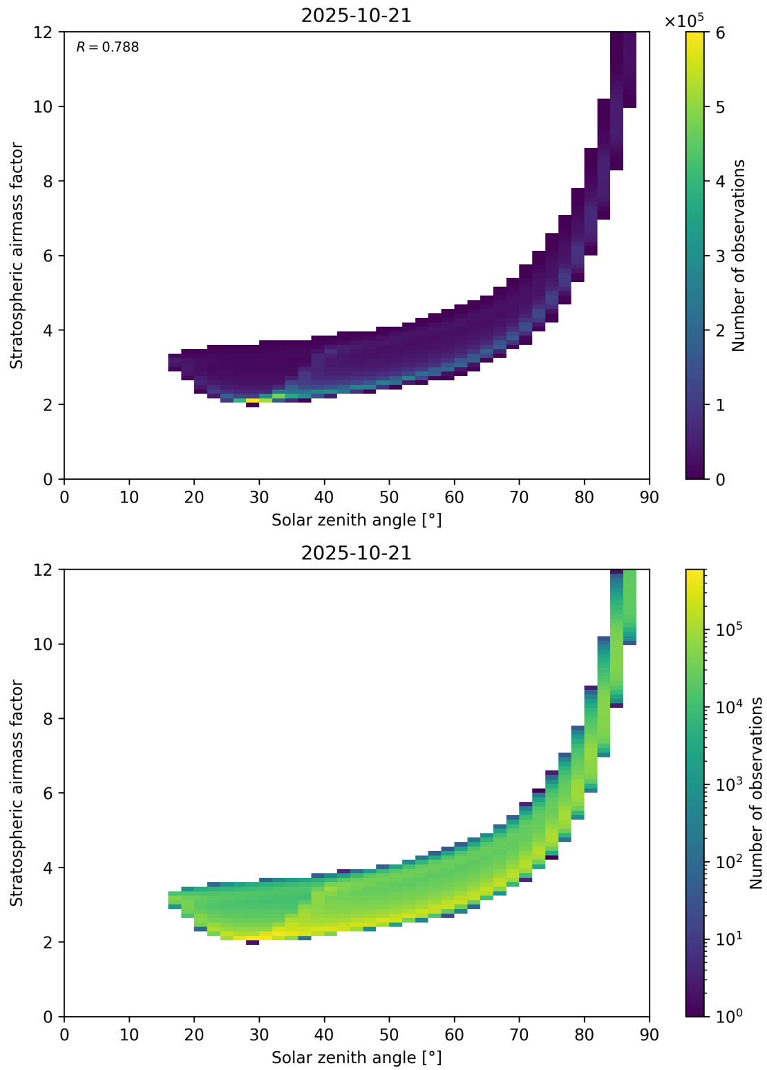
Figure 145: Scatter density plot of “Solar zenith angle” against “Stratospheric airmass factor” for 2025-10-20 to 2025-10-22.
