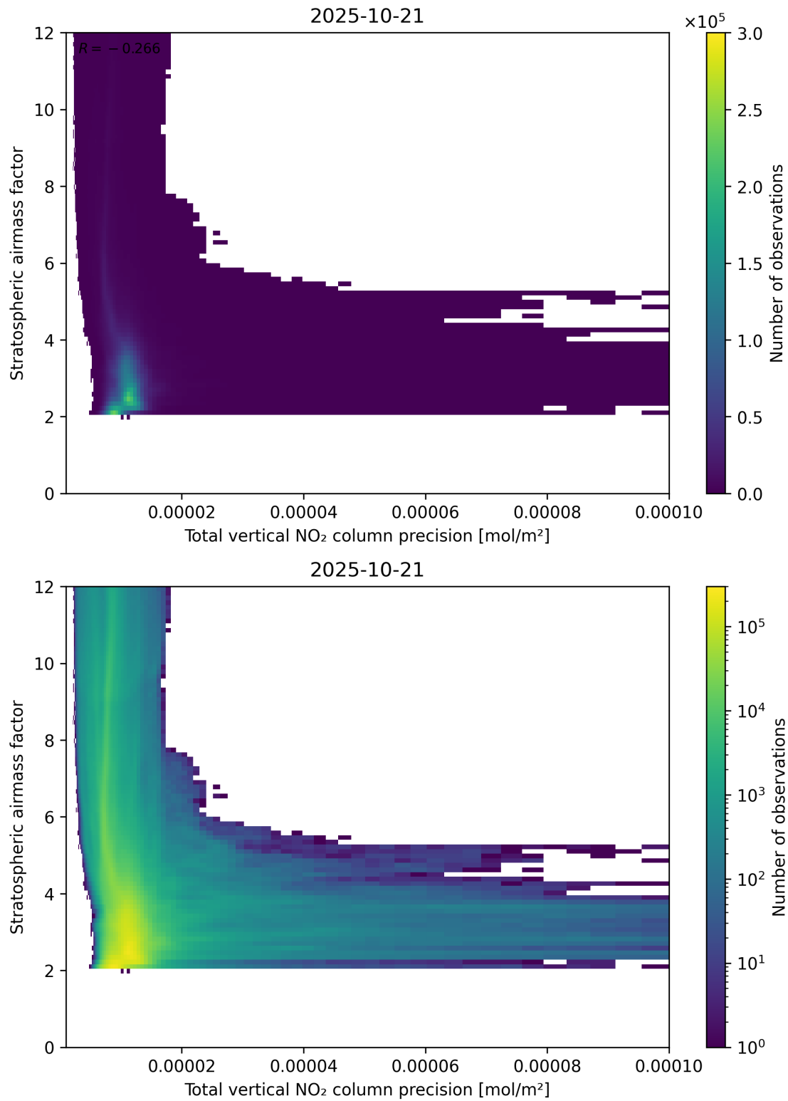
Figure 115: Scatter density plot of “Total vertical NO 2 column precision” against “Stratospheric air mass factor” for 2025-10-20 to 2025-10-22.
