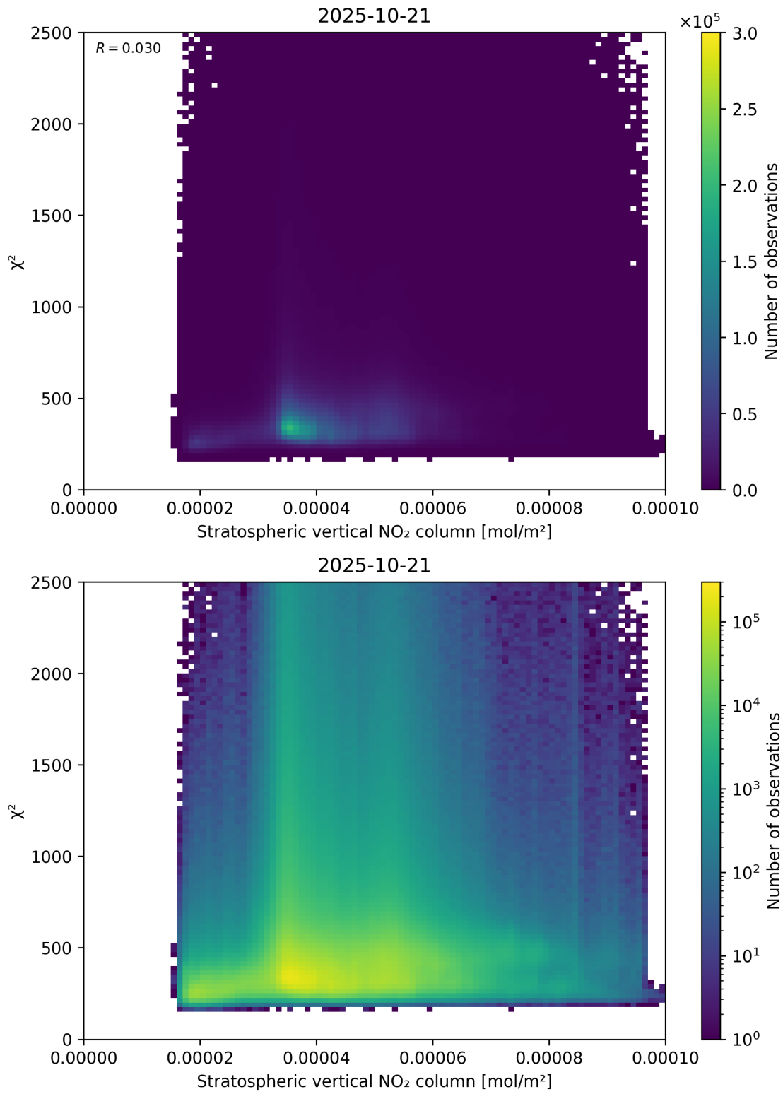
Figure 97: Scatter density plot of “Stratospheric vertical NO 2 column” against “ \chi^2 ” for 2025-10-20 to 2025-10-22.
