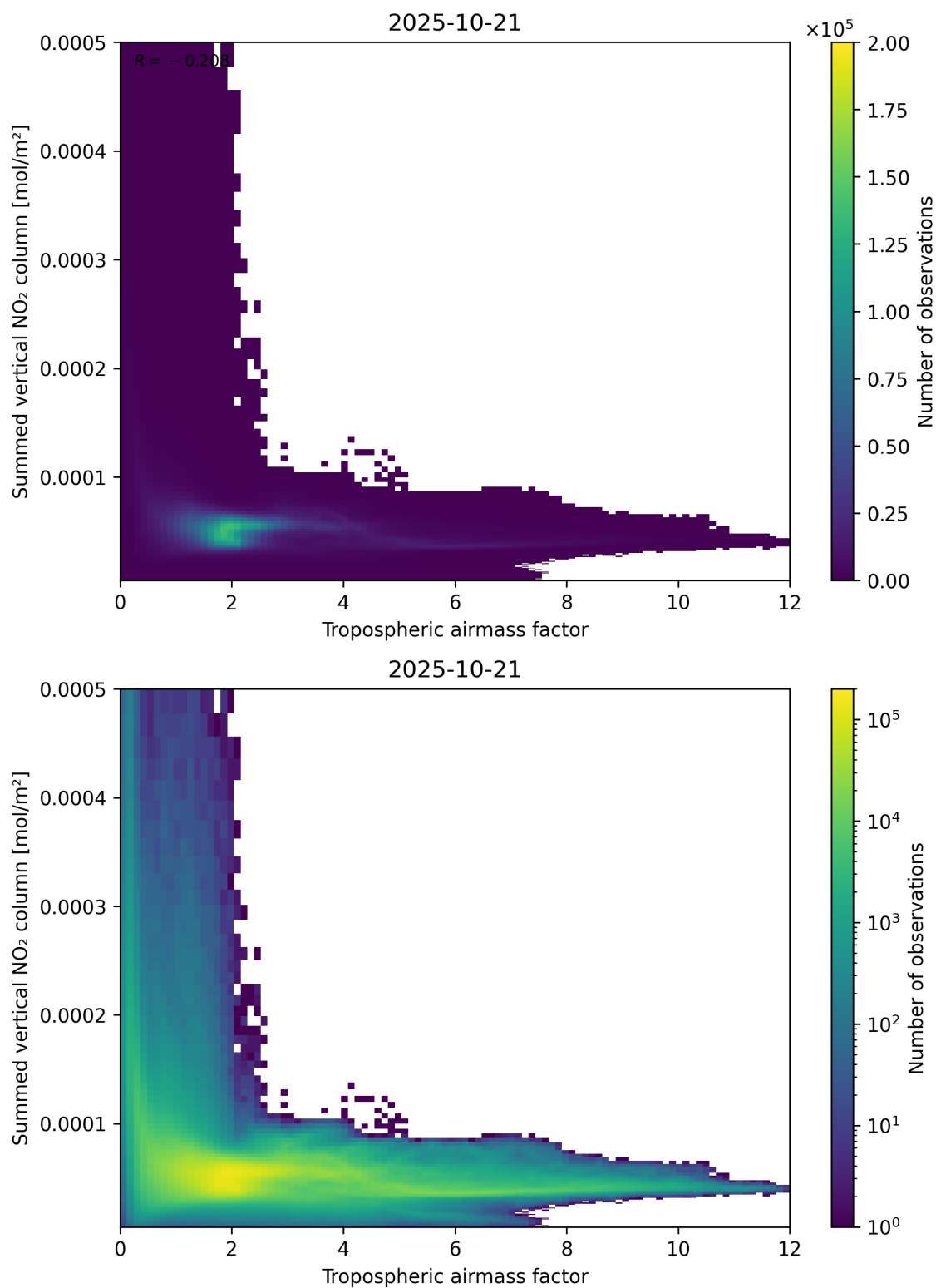
Figure 75: Scatter density plot of “Tropospheric airmass factor” against “Summed vertical NO 2 column” for 2025-10-20 to 2025-10-22.
