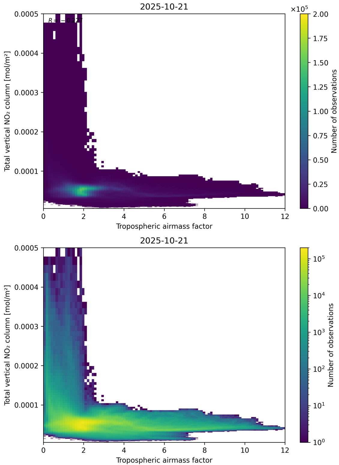
Figure 77: Scatter density plot of “Tropospheric airmass factor” against “Total vertical NO 2 column” for 2025-10-20 to 2025-10-22.
