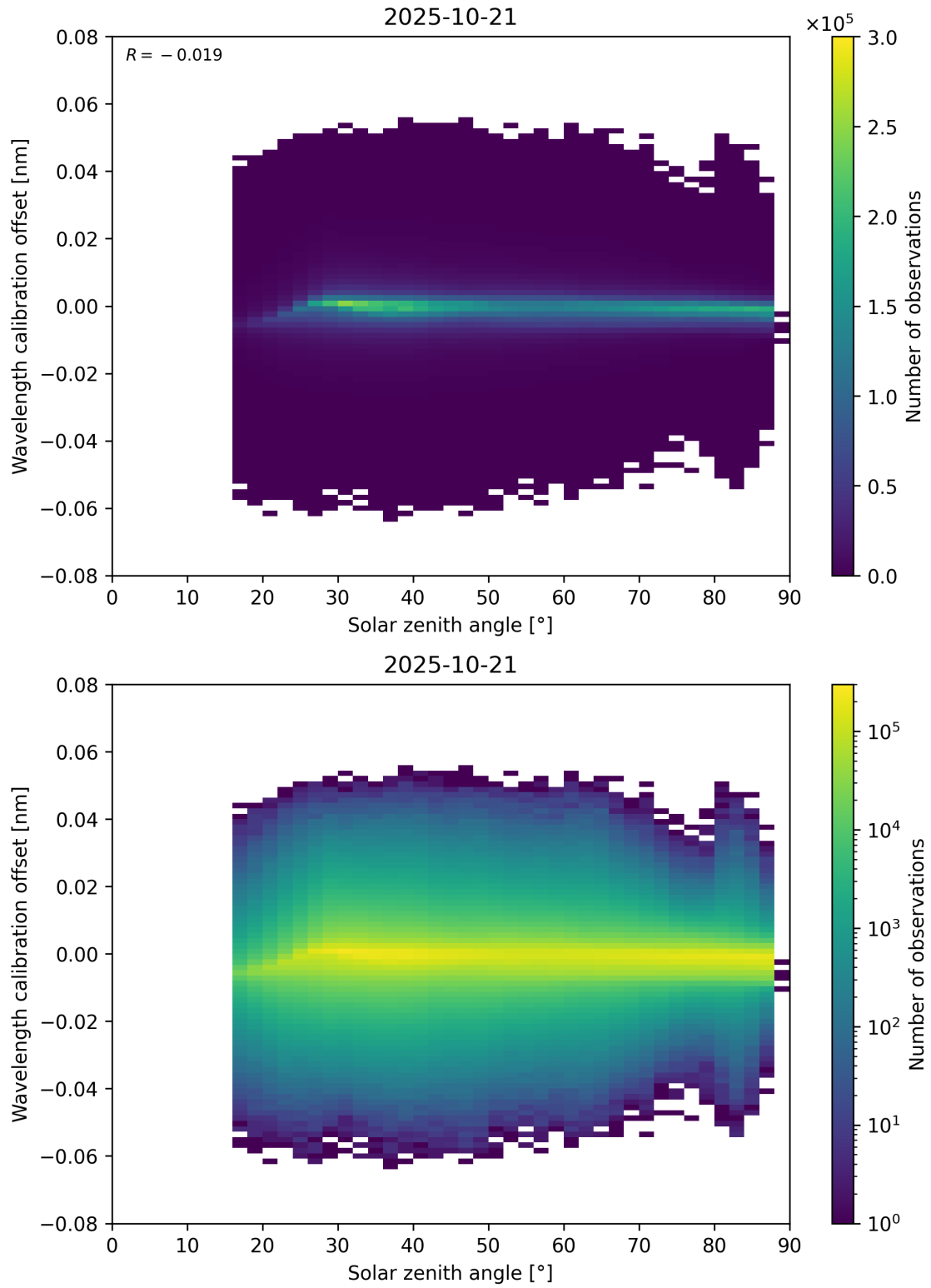
Figure 158: Scatter density plot of “Solar zenith angle” against “Wavelength calibration offset” for 2025-10-20 to 2025-10-22.
