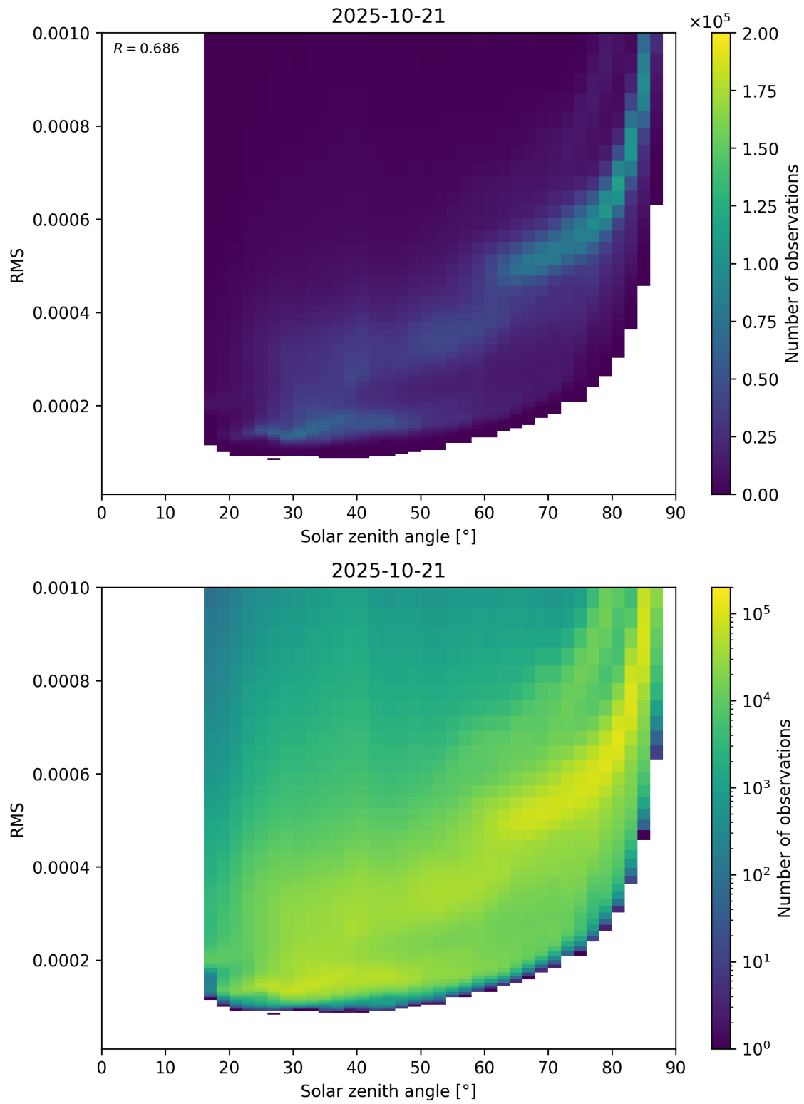
Figure 157: Scatter density plot of “Solar zenith angle” against “RMS” for 2025-10-20 to 2025-10-22.
