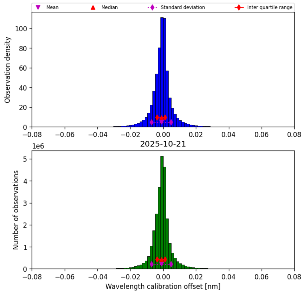
Figure 35: Histogram of “Wavelength calibration offset” for 2025-10-20 to 2025-10-22
