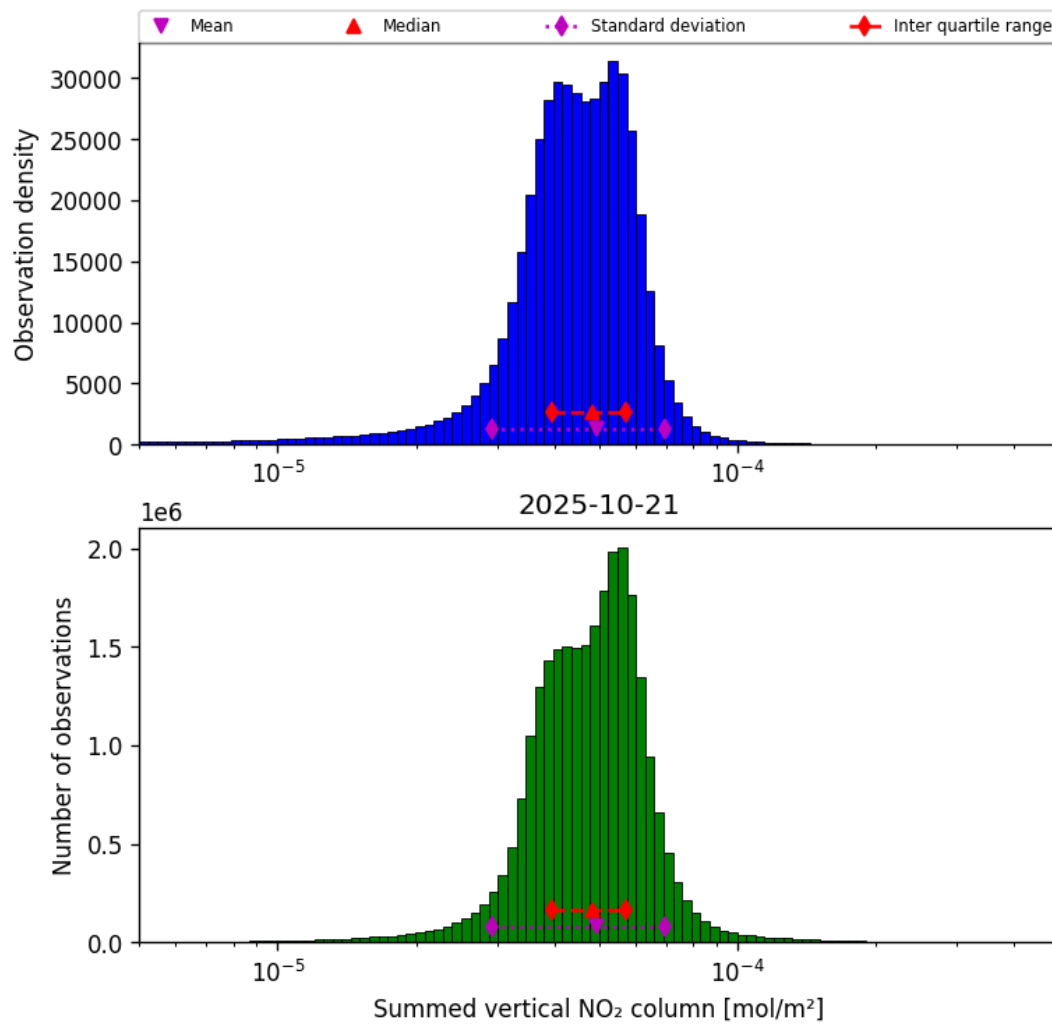
Figure 40: Histogram of “Summed vertical NO 2 column” for 2025-10-20 to 2025-10-22
