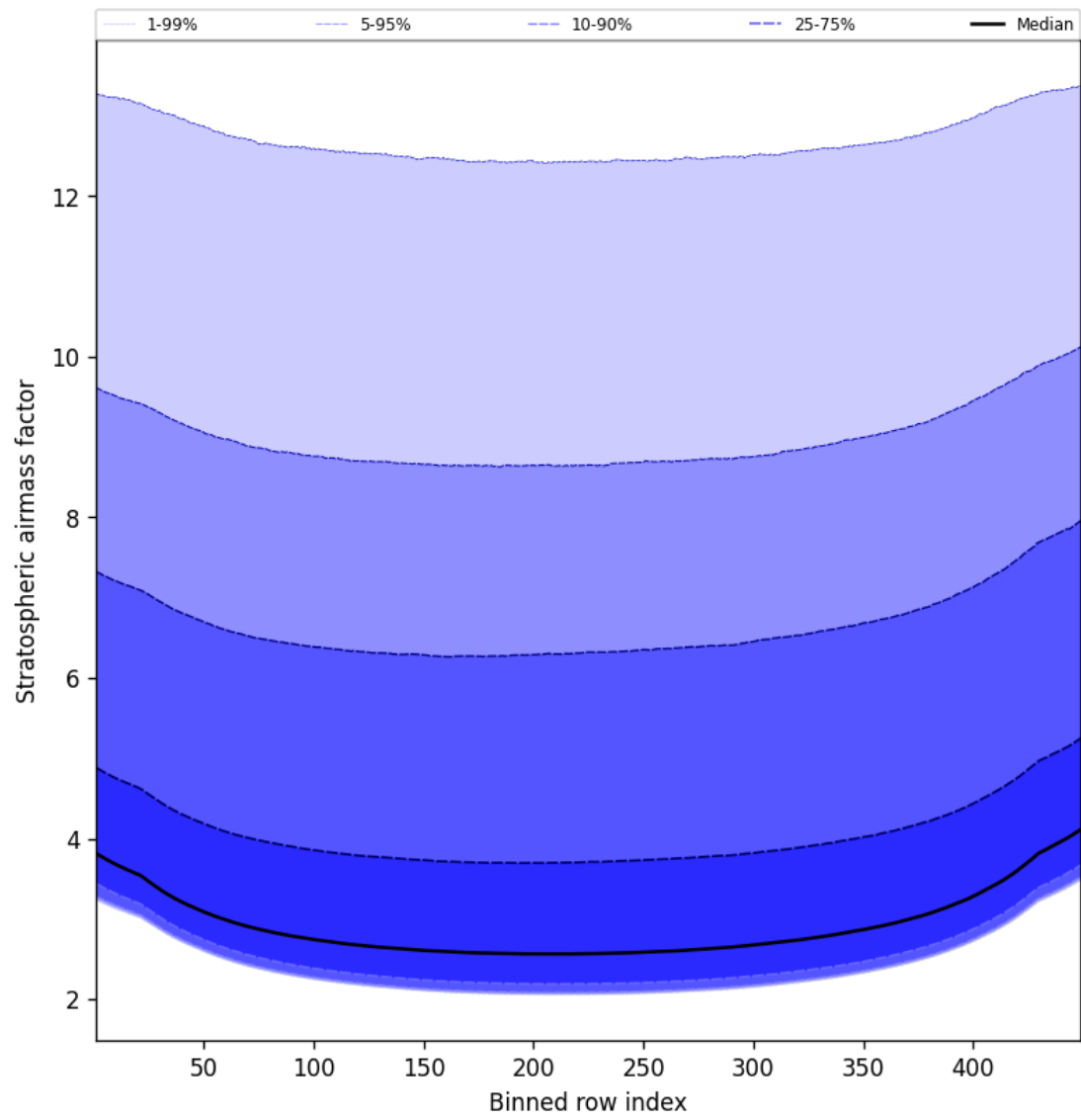
Figure 61: Along track statistics of “Stratospheric airmass factor” for 2025-10-20 to 2025-10-22
