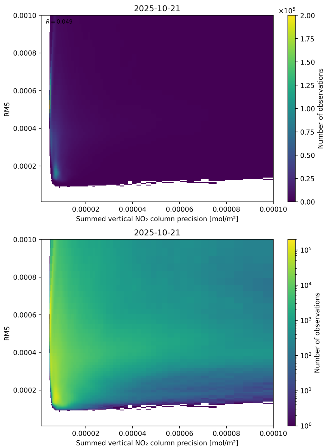
Figure 108: Scatter density plot of “Summed vertical NO 2 column precision” against “RMS” for 2025-10-20 to 2025-10-22.
