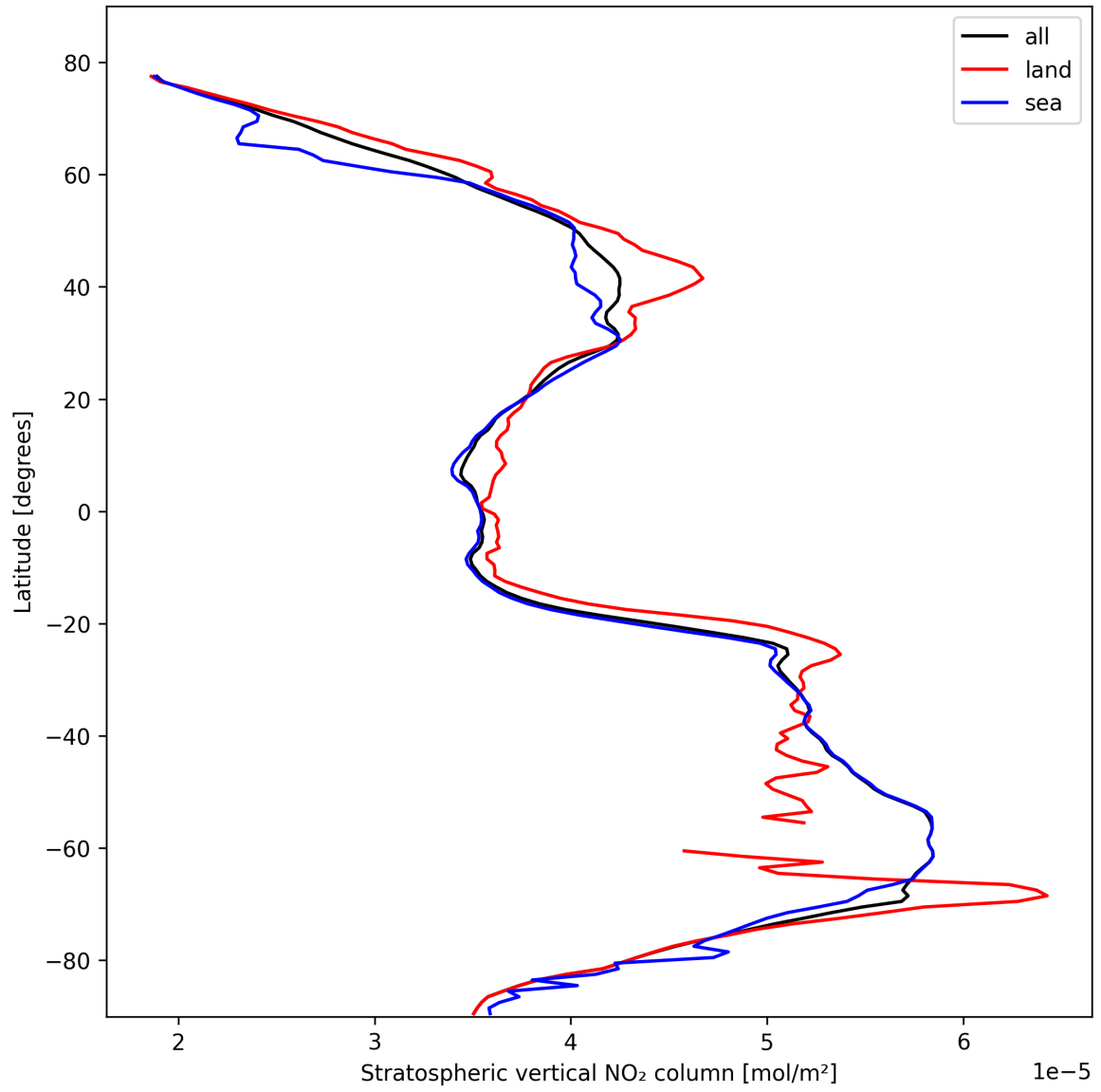
Figure 19: Zonal average of “Stratospheric vertical NO 2 column” for 2025-10-20 to 2025-10-22.
