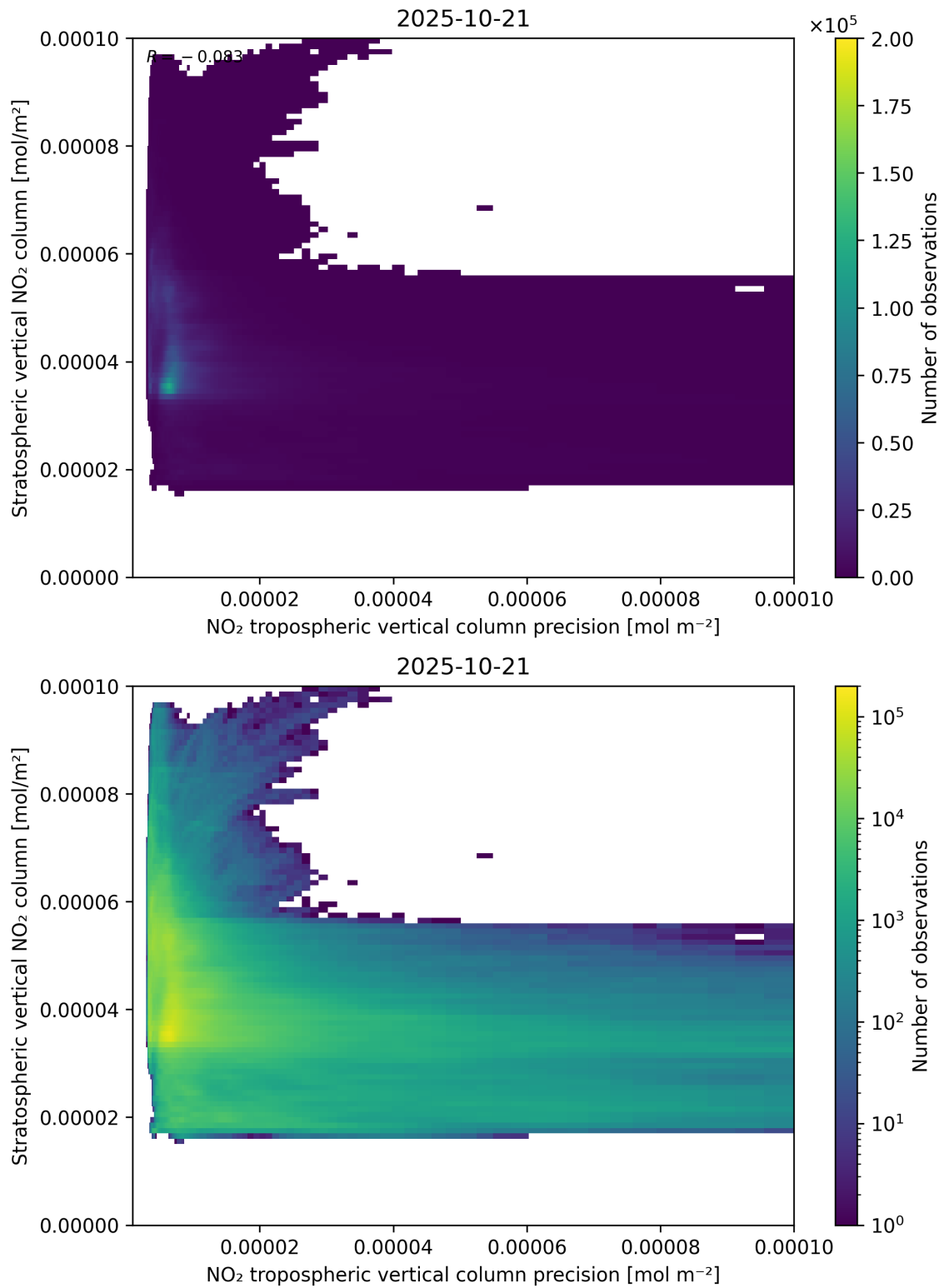
Figure 135: Scatter density plot of “NO 2 tropospheric vertical column precision” against “Stratospheric vertical NO 2 column” for 2025-10-20 to 2025-10-22.
