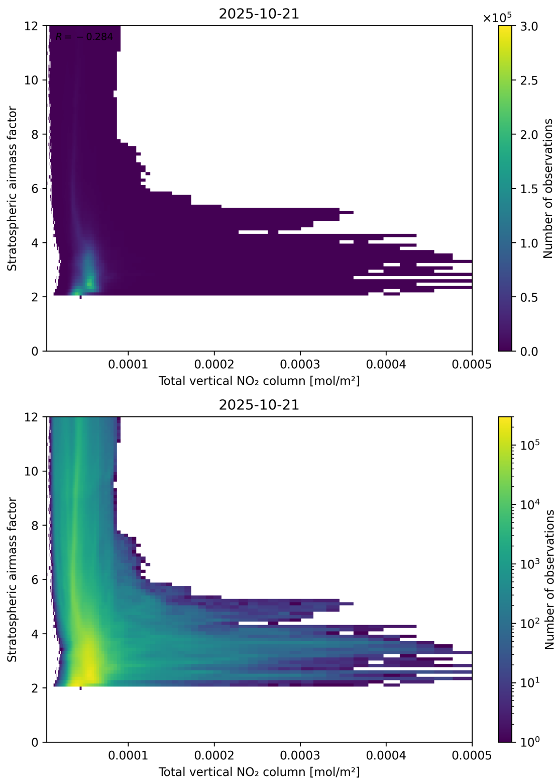
Figure 110: Scatter density plot of “Total vertical NO 2 column” against “Stratospheric airmass factor” for 2025-10-20 to 2025-10-22.
