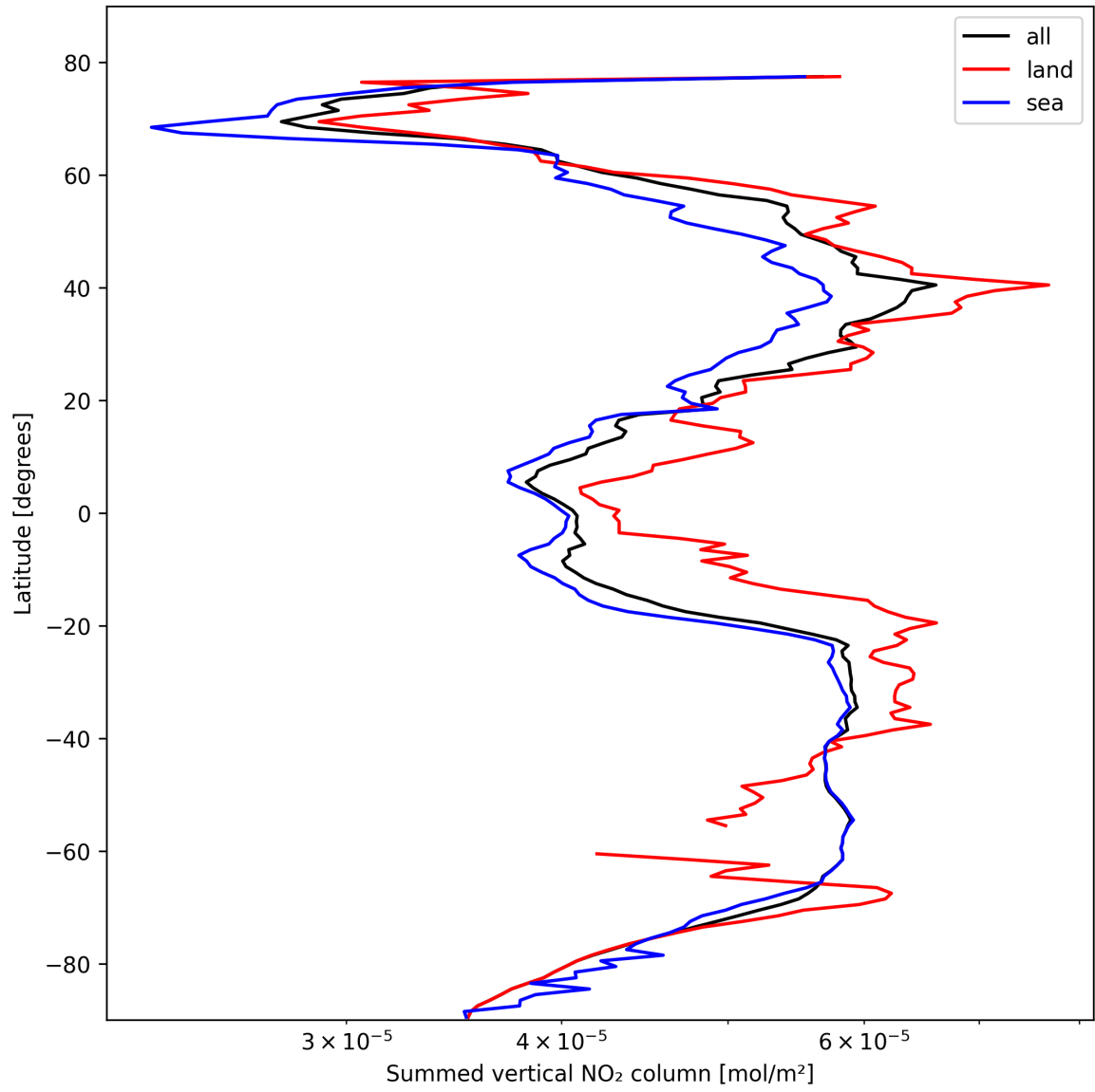
Figure 23: Zonal average of “Summed vertical NO 2 column” for 2025-10-20 to 2025-10-22.
