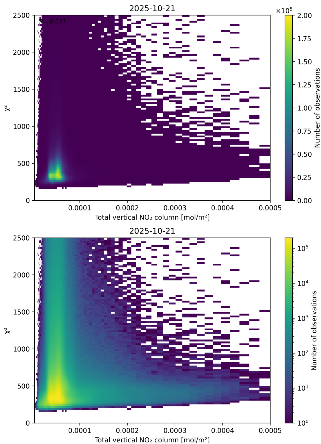
Figure 111: Scatter density plot of “Total vertical NO 2 column” against “ \chi^2 ” for 2025-10-20 to 2025-10-22.
