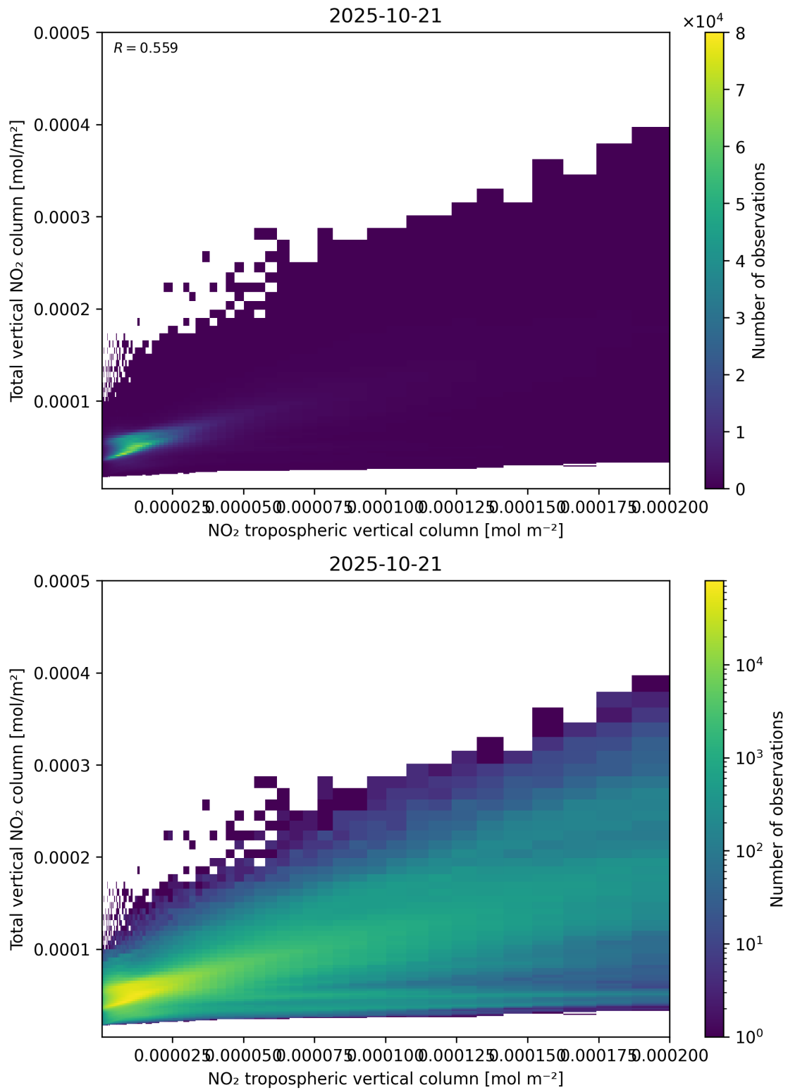
Figure 128: Scatter density plot of “NO 2 tropospheric vertical column” against “Total vertical NO 2 column” for 2025-10-20 to 2025-10-22.
