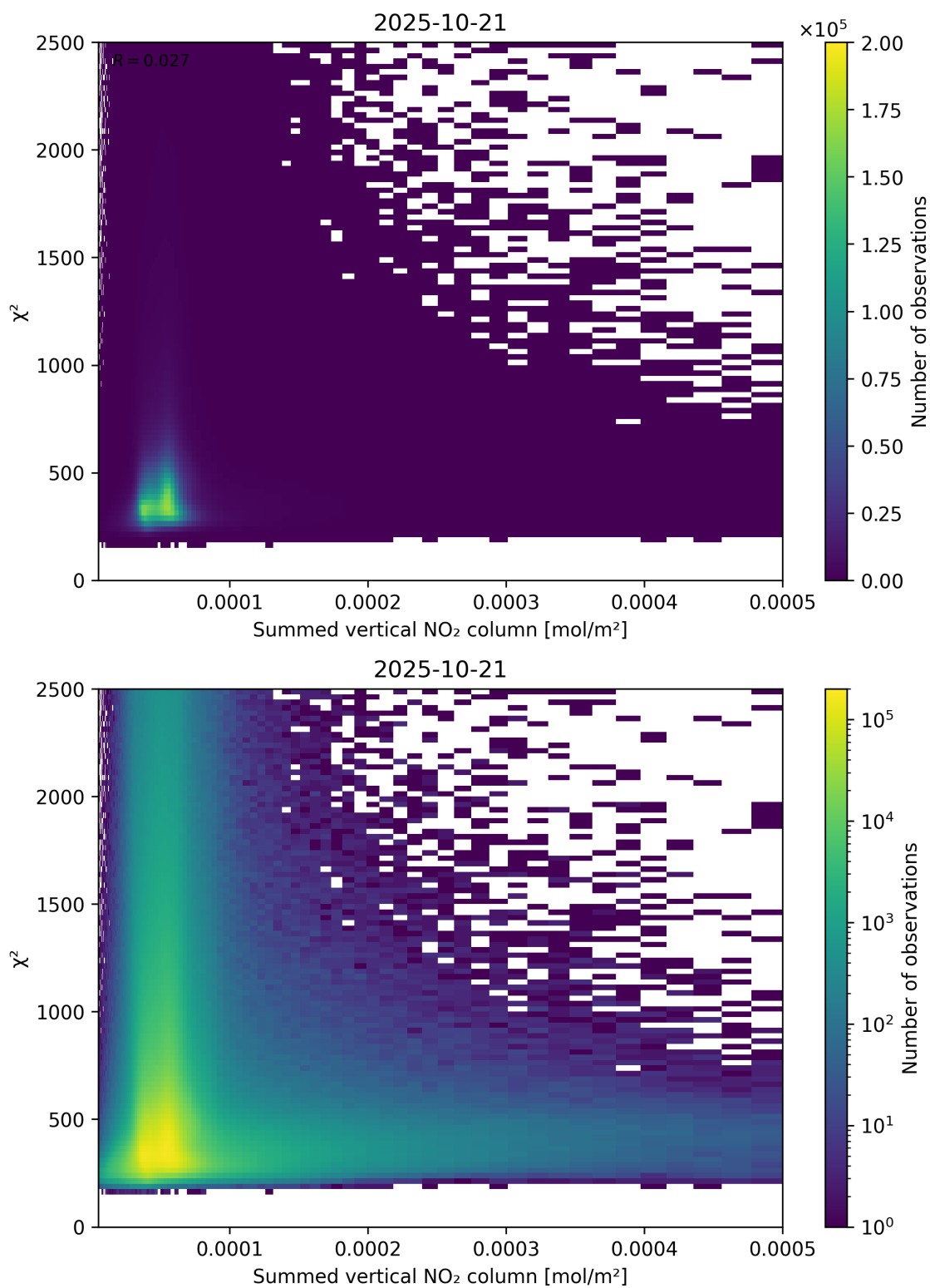
Figure 104: Scatter density plot of “Summed vertical NO 2 column” against “ \chi^2 ” for 2025-10-20 to 2025-10-22.
