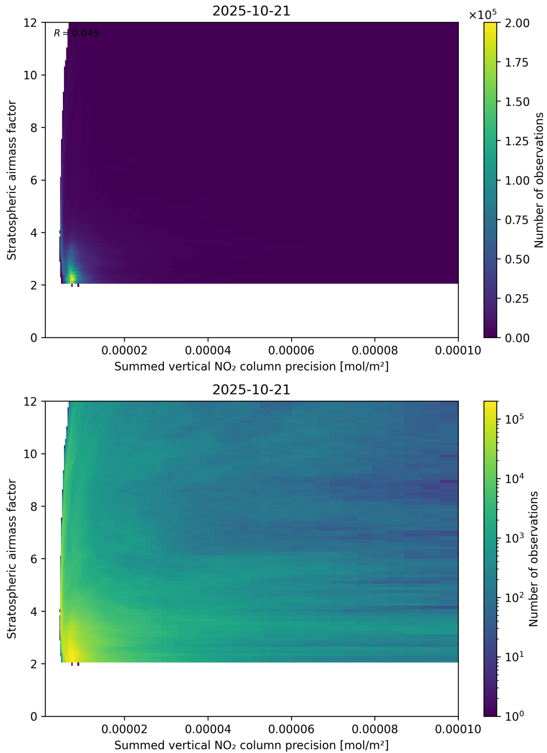
Figure 106: Scatter density plot of “Summed vertical NO 2 column precision” against “Stratospheric airmass factor” for 2025-10-20 to 2025-10-22.
