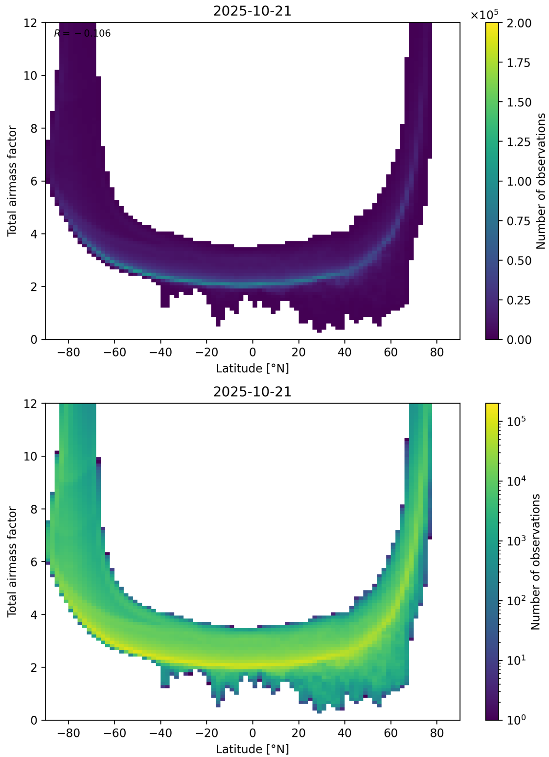
Figure 84: Scatter density plot of “Latitude” against “Total airmass factor” for 2025-10-20 to 2025-10-22.
