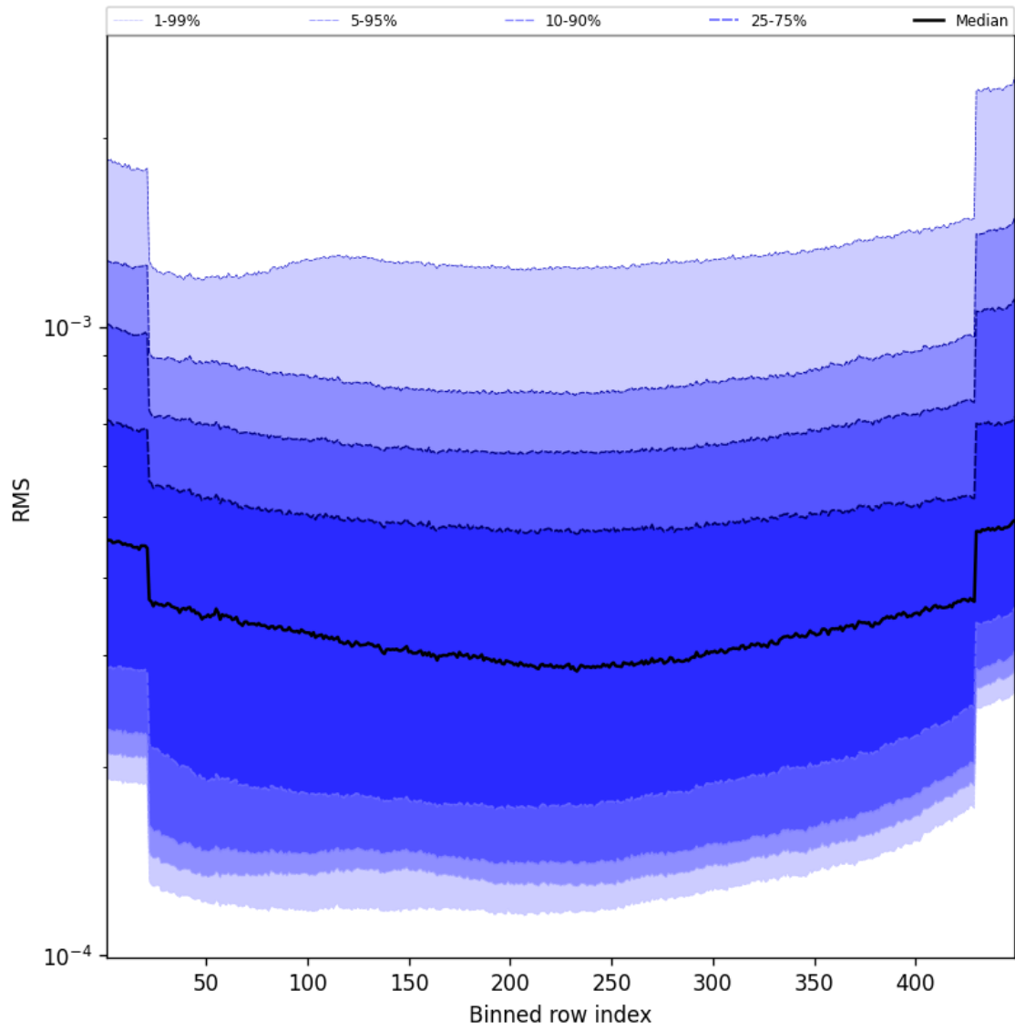
Figure 60: Along track statistics of “RMS” for 2025-10-20 to 2025-10-22
