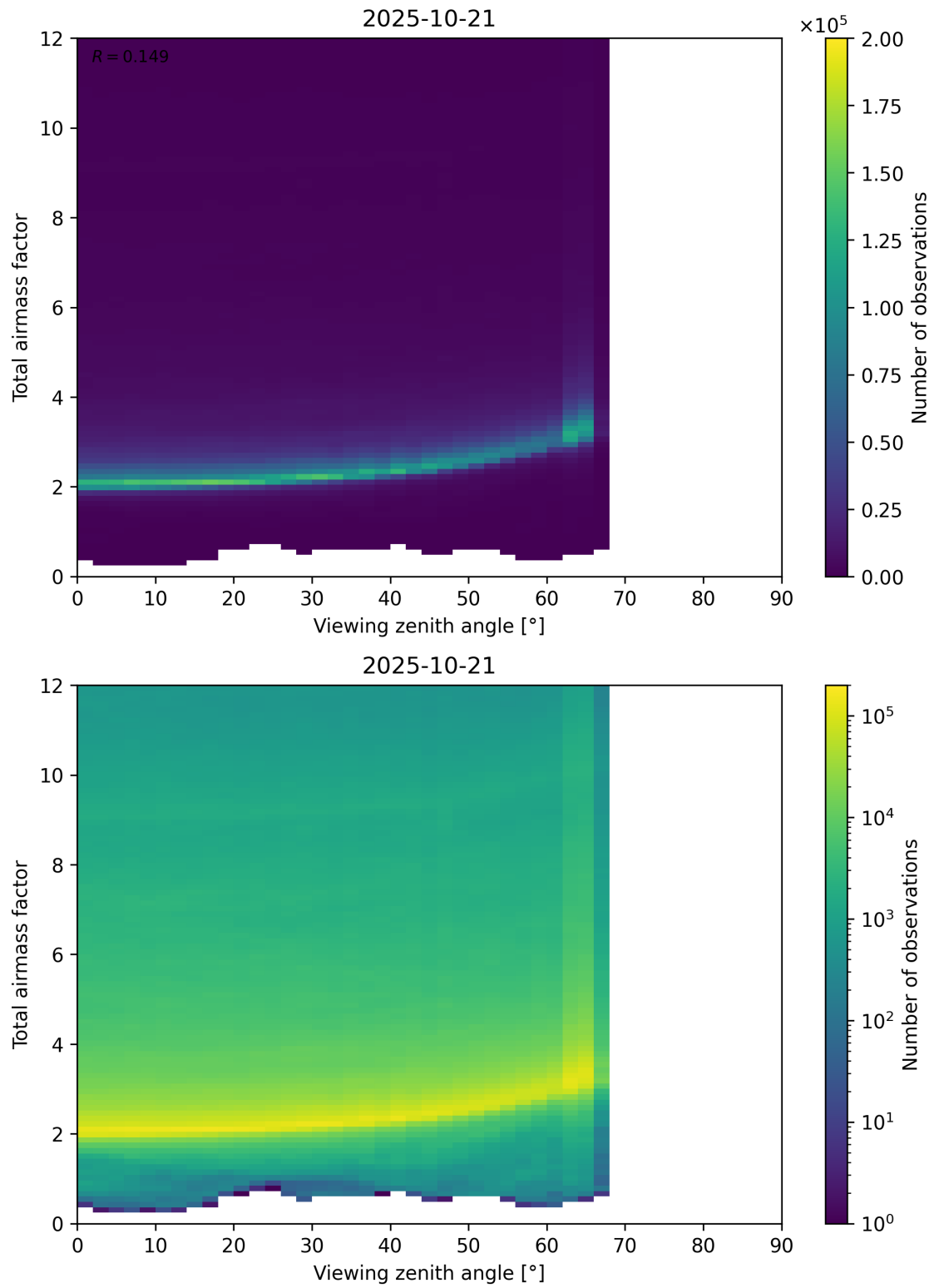
Figure 160: Scatter density plot of “Viewing zenith angle” against “Total airmass factor” for 2025-10-20 to 2025-10-22.
