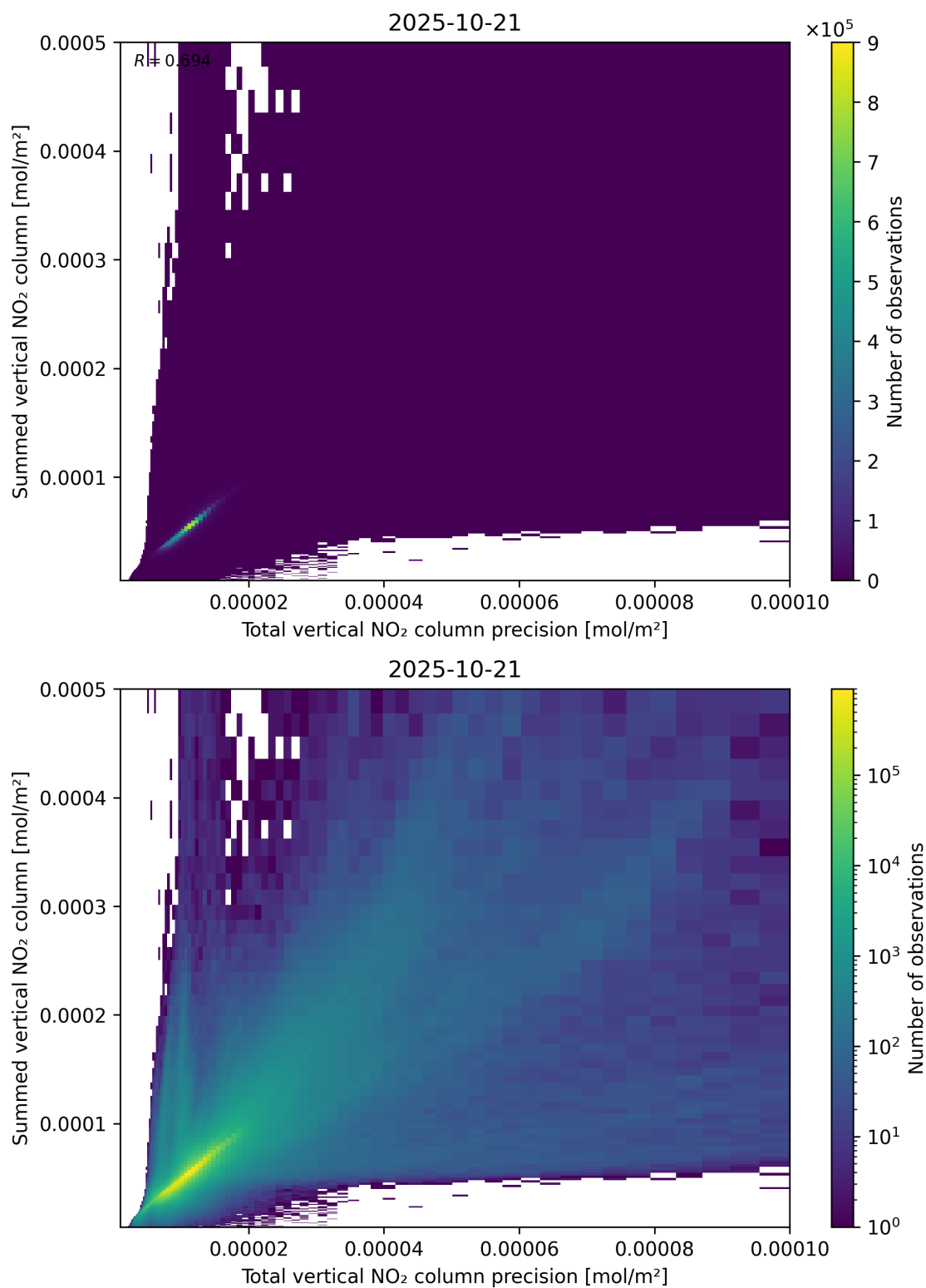
Figure 117: Scatter density plot of “Total vertical NO 2 column precision” against “Summed vertical NO 2 column” for 2025-10-20 to 2025-10-22.
