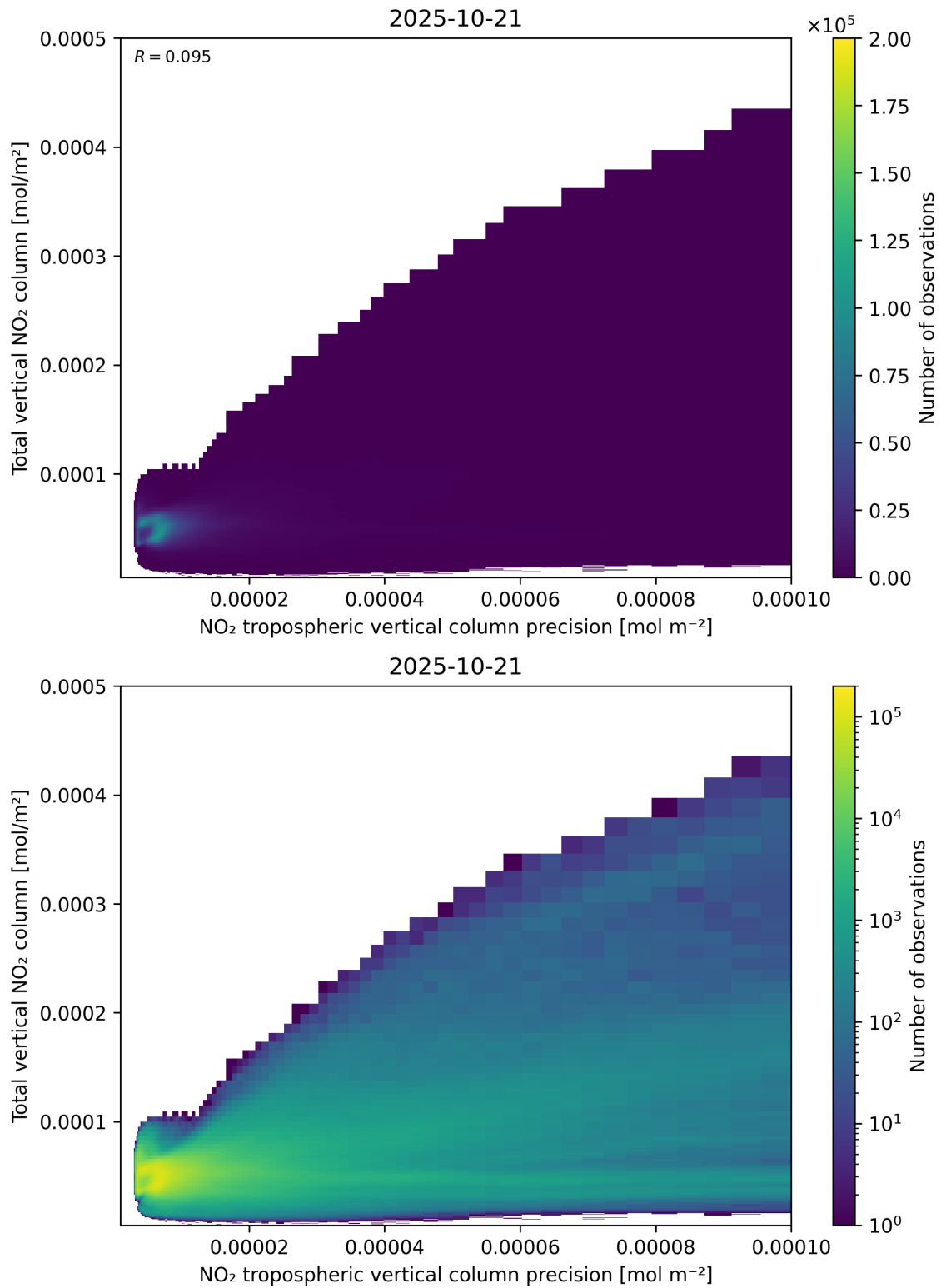
Figure 138: Scatter density plot of “NO 2 tropospheric vertical column precision” against “Total vertical NO 2 column” for 2025-10-20 to 2025-10-22.
