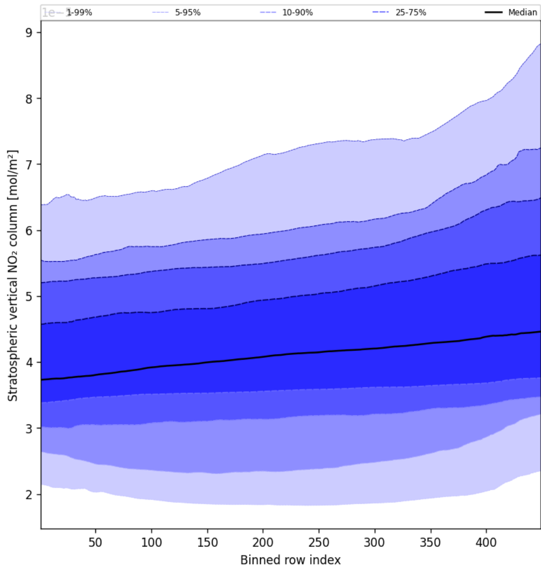
Figure 53: Along track statistics of “Stratospheric vertical NO 2 column” for 2025-10-20 to 2025-10-22
