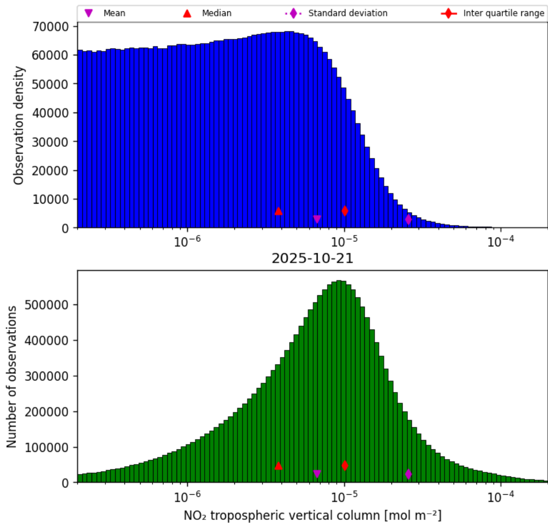
Figure 29: Histogram of “NO 2 tropospheric vertical column” for 2025-10-20 to 2025-10-22
