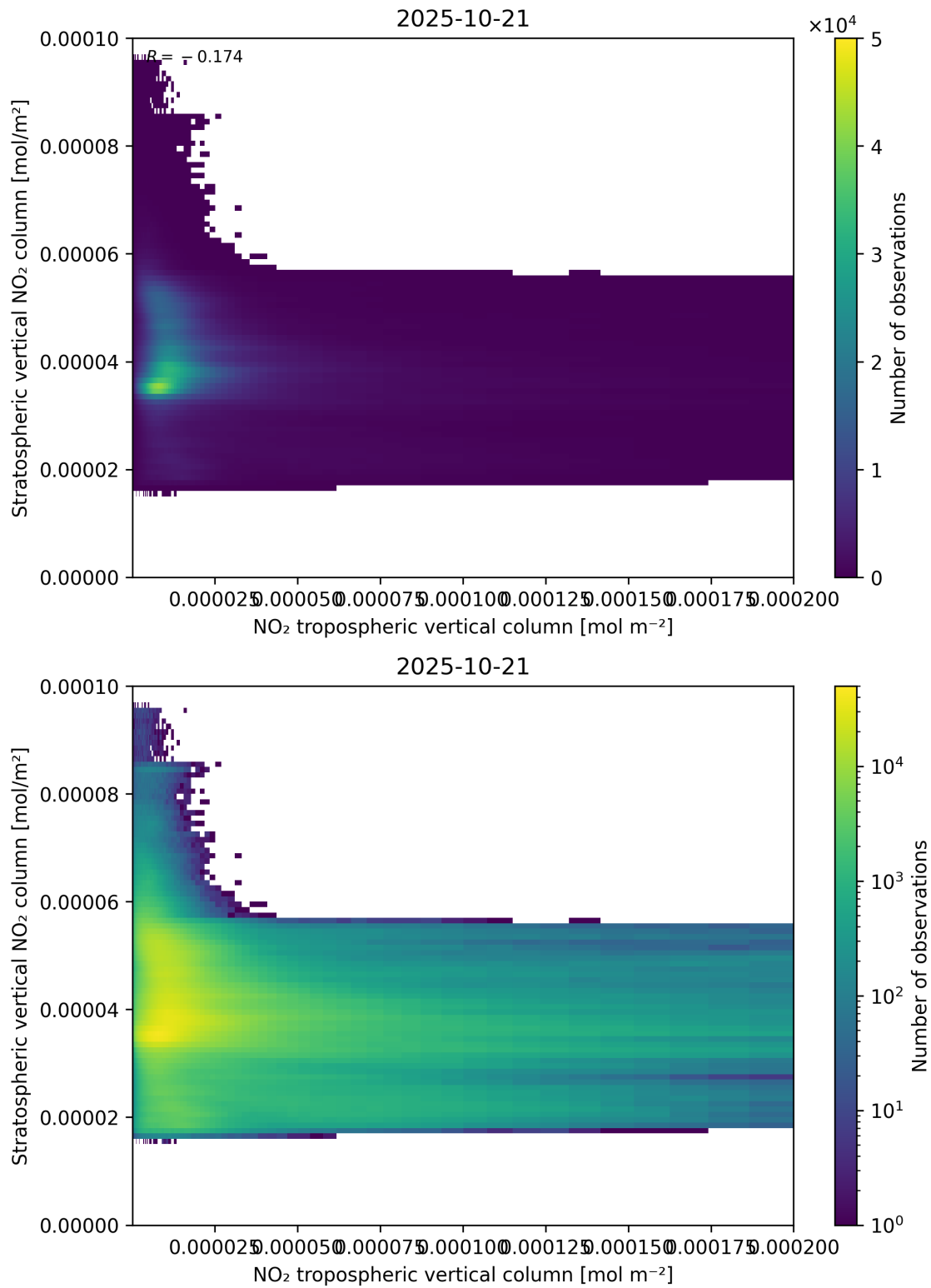
Figure 125: Scatter density plot of “NO 2 tropospheric vertical column” against “Stratospheric vertical NO 2 column” for 2025-10-20 to 2025-10-22.
