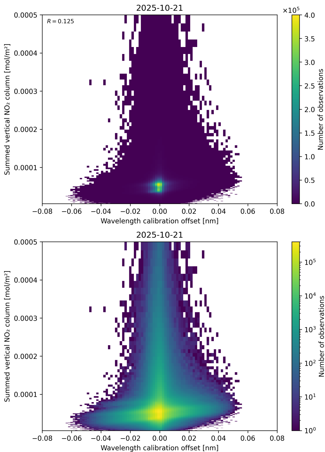
Figure 177: Scatter density plot of “Wavelength calibration offset” against “Summed vertical NO 2 column” for 2025-10-20 to 2025-10-22.
