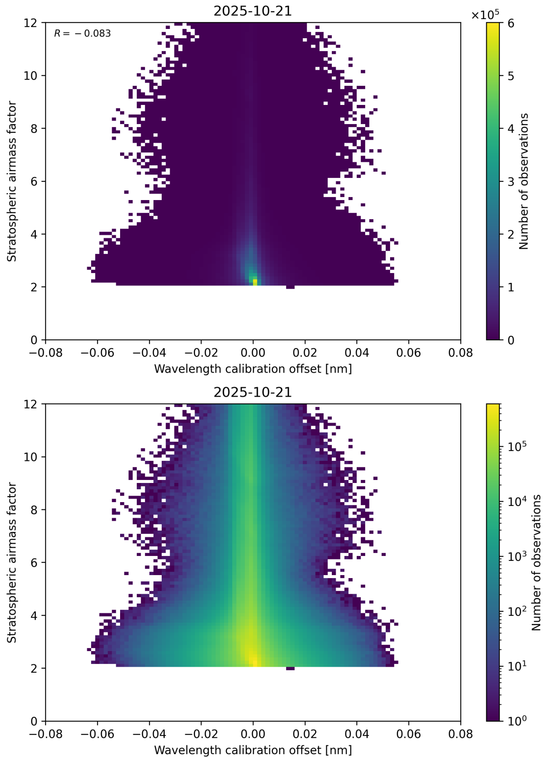
Figure 174: Scatter density plot of “Wavelength calibration offset” against “Stratospheric airmass factor” for 2025-10-20 to 2025-10-22.
