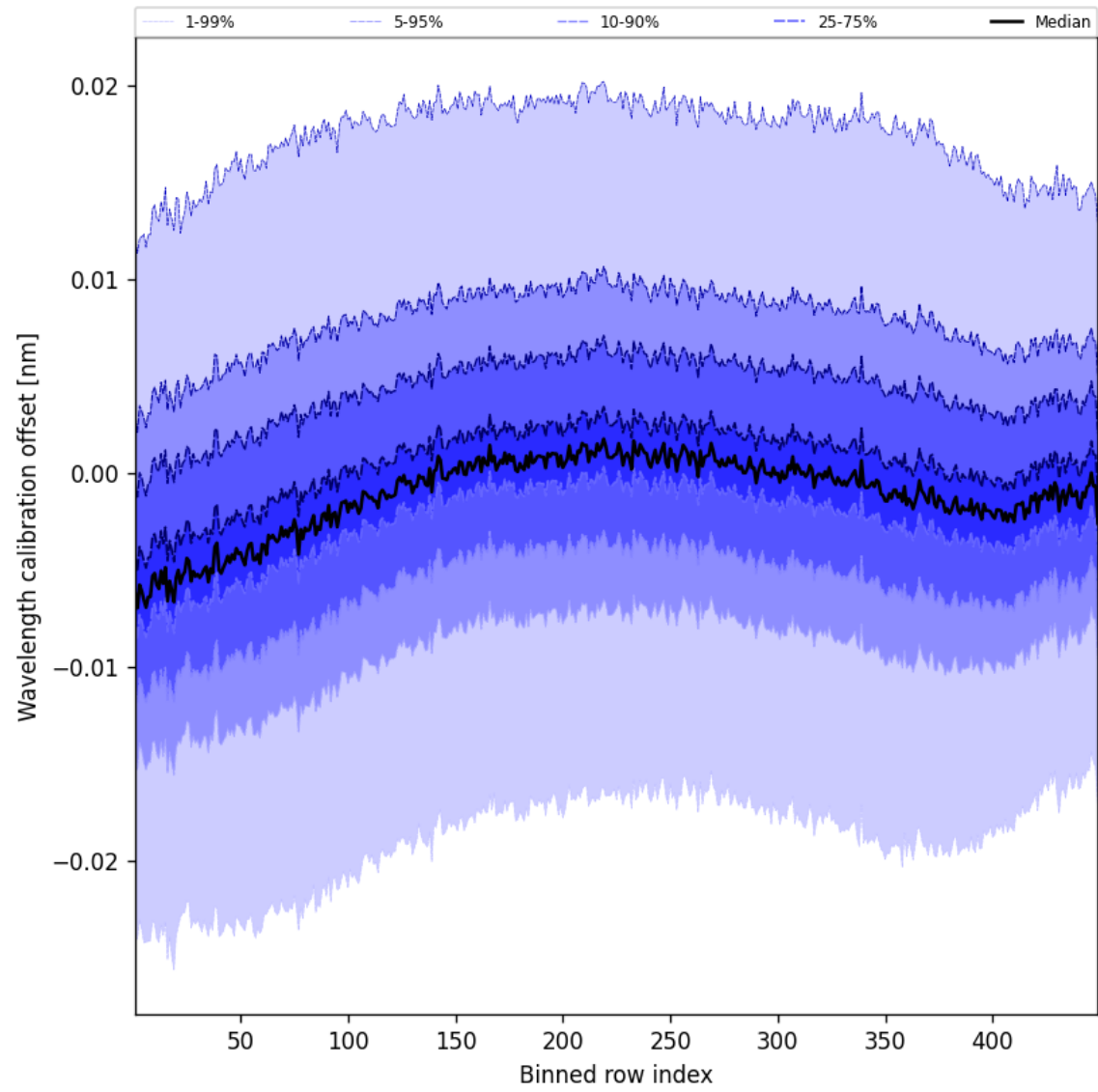
Figure 52: Along track statistics of “Wavelength calibration offset” for 2025-10-20 to 2025-10-22
