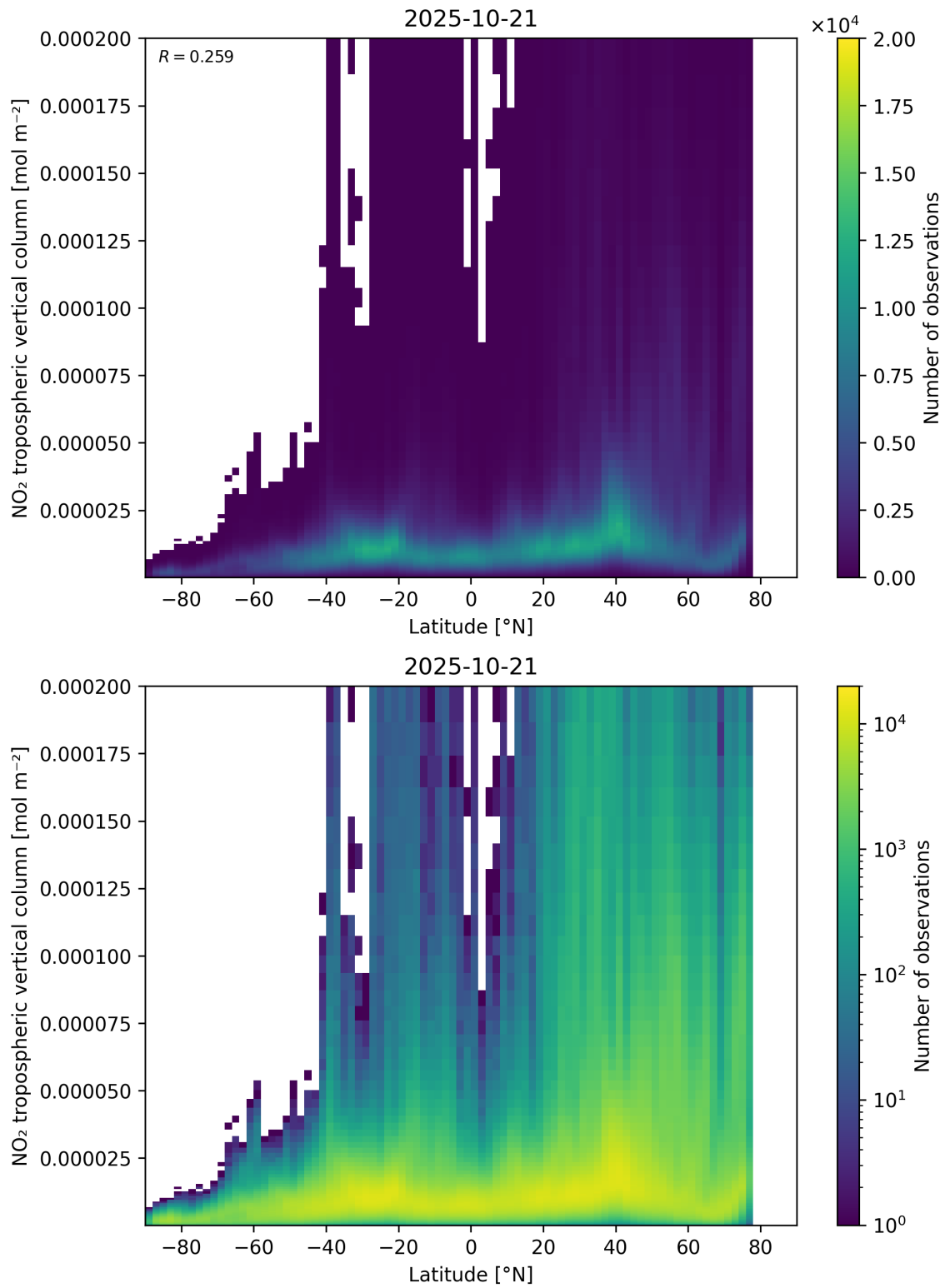
Figure 92: Scatter density plot of “Latitude” against “NO 2 tropospheric vertical column” for 2025-10-20 to 2025-10-22.
