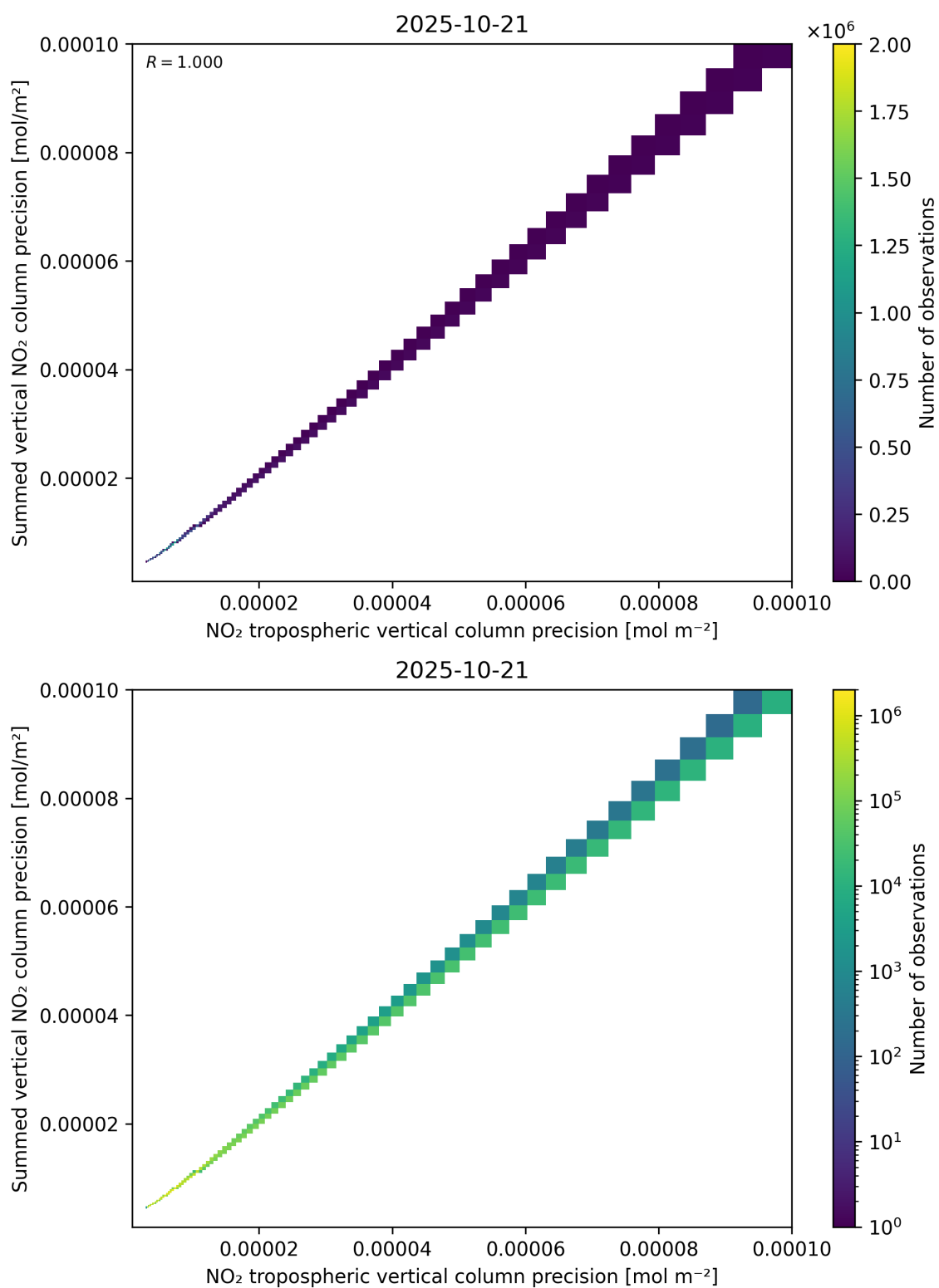
Figure 137: Scatter density plot of “NO 2 tropospheric vertical column precision” against “Summed vertical NO 2 column precision” for 2025-10-20 to 2025-10-22.
