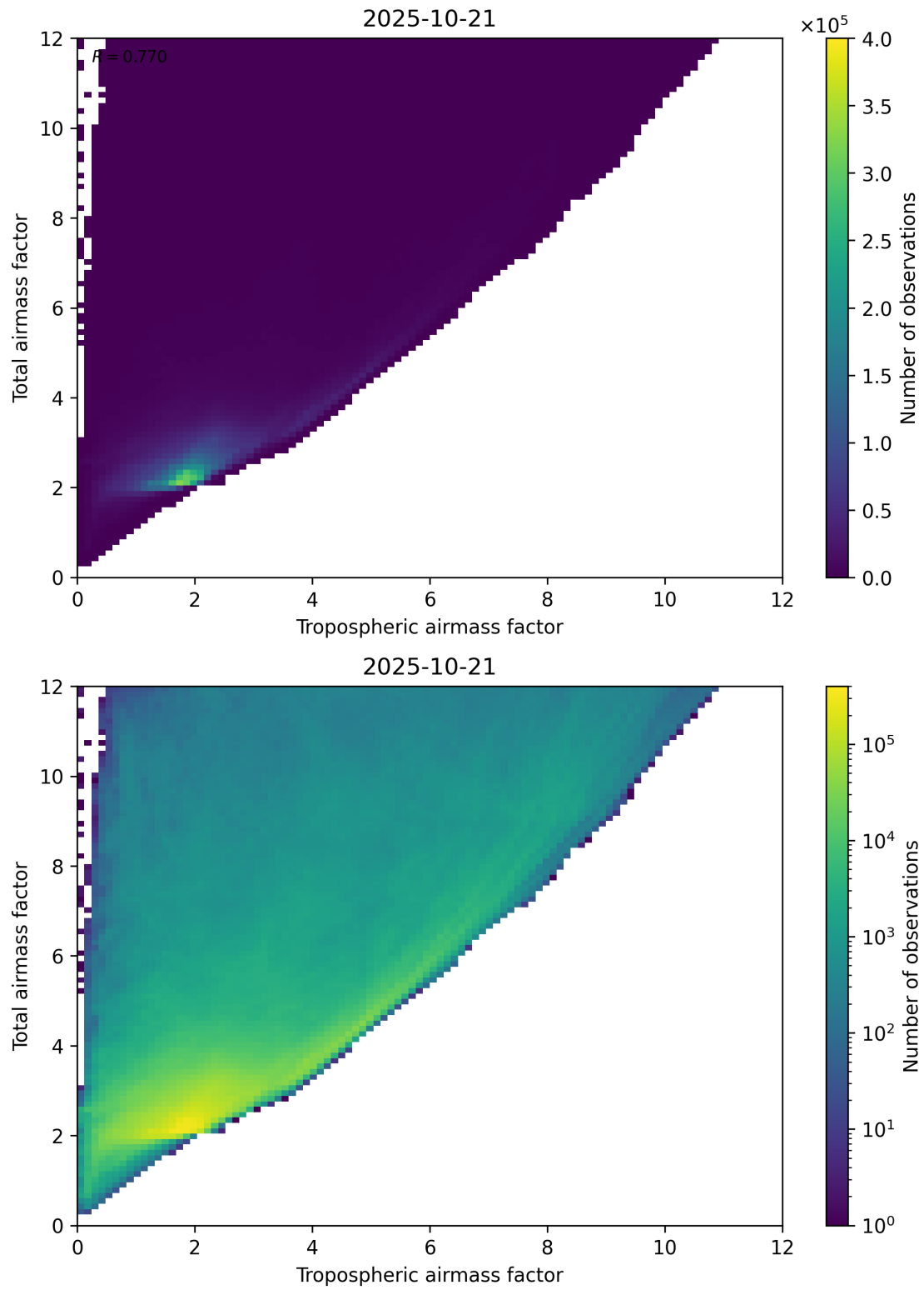
Figure 72: Scatter density plot of “Tropospheric airmass factor” against “Total airmass factor” for 2025-10-20 to 2025-10-22.
