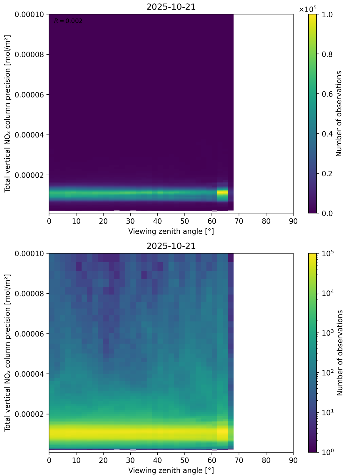
Figure 168: Scatter density plot of “Viewing zenith angle” against “Total vertical NO 2 column precision” for 2025-10-20 to 2025-10-22.
