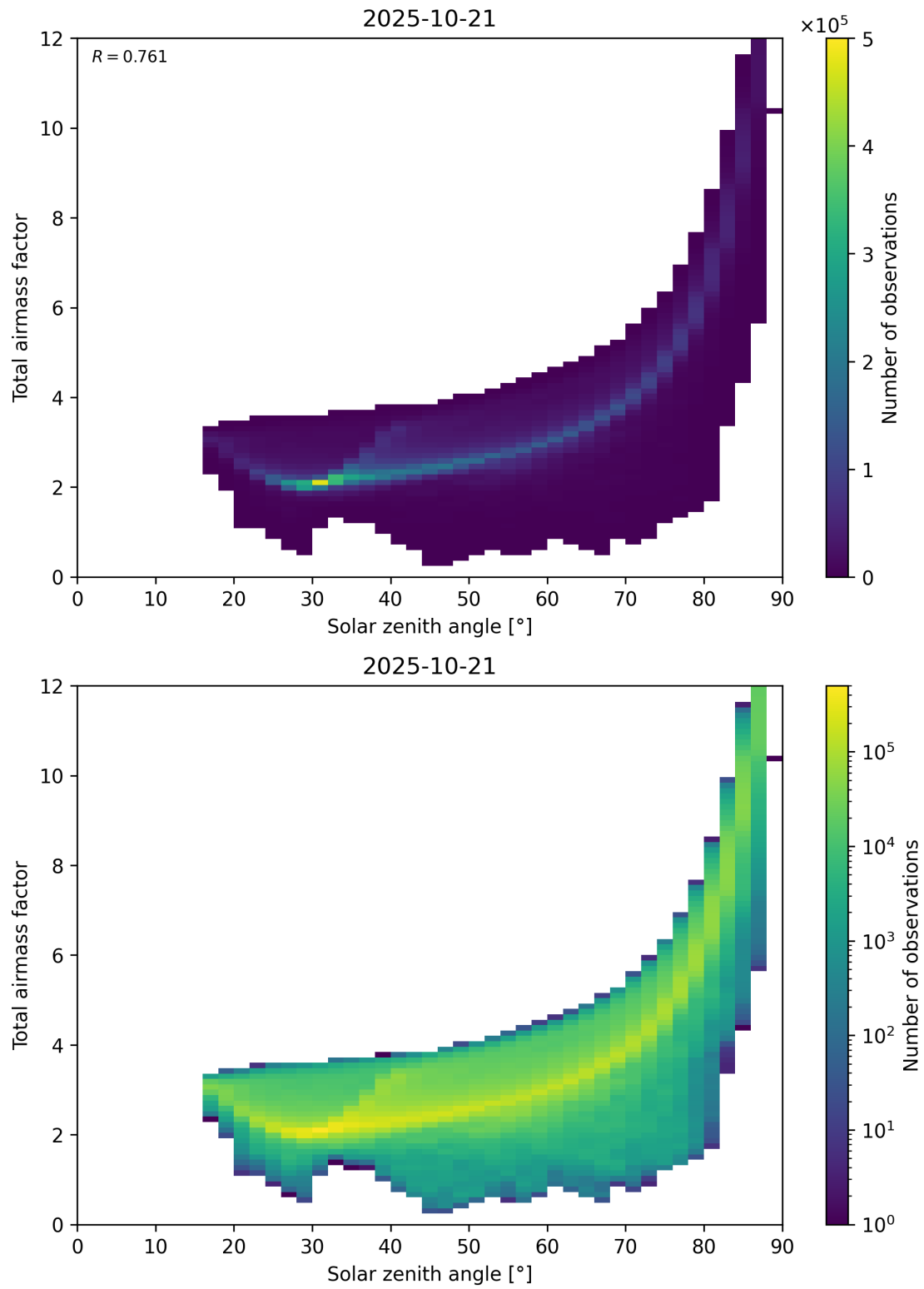
Figure 146: Scatter density plot of “Solar zenith angle” against “Total airmass factor” for 2025-10-20 to 2025-10-22.
