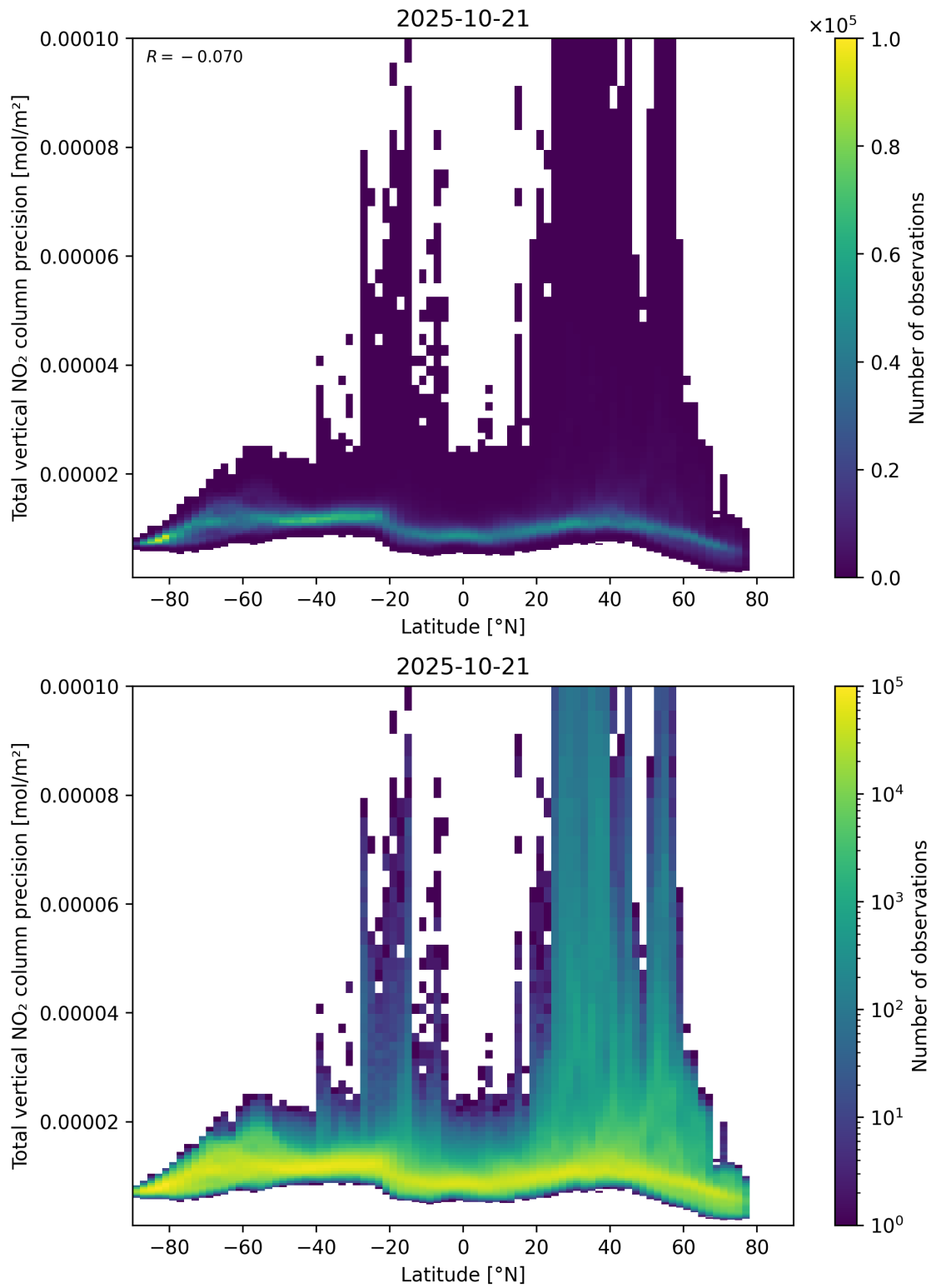
Figure 91: Scatter density plot of “Latitude” against “Total vertical NO 2 column precision” for 2025-10-20 to 2025-10-22.
