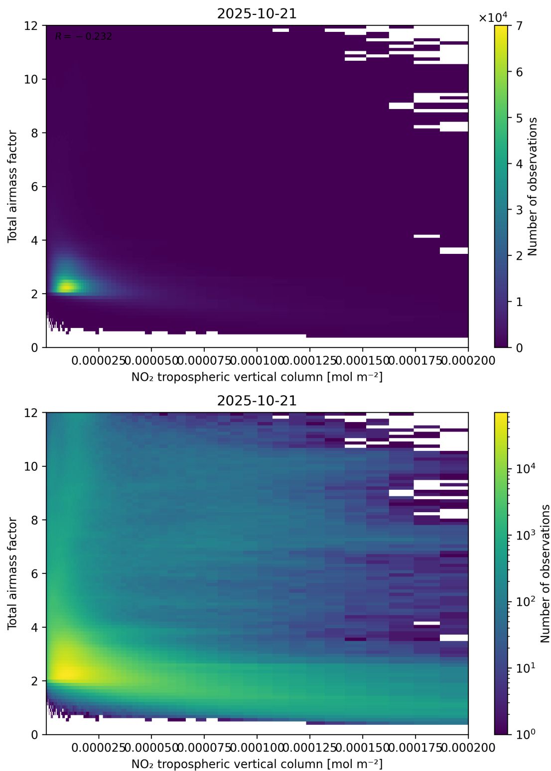
Figure 122: Scatter density plot of “NO 2 tropospheric vertical column” against “Total air mass factor” for 2025-10-20 to 2025-10-22.
