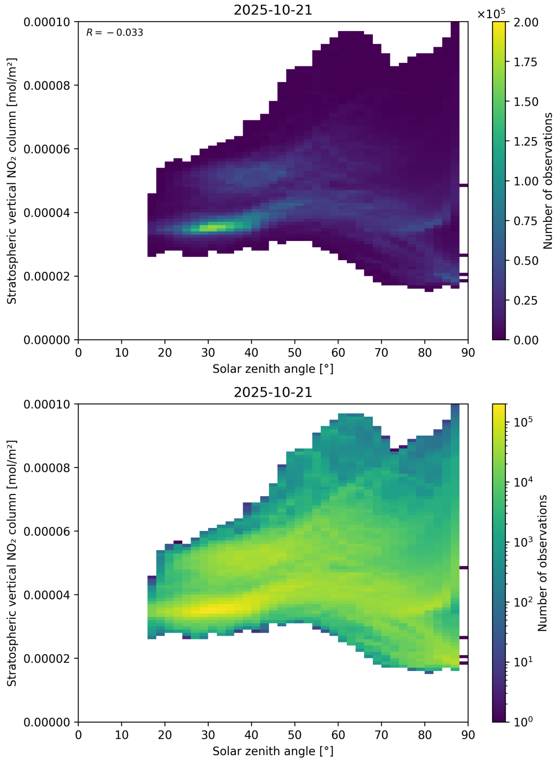
Figure 150: Scatter density plot of “Solar zenith angle” against “Stratospheric vertical NO 2 column” for 2025-10-20 to 2025-10-22.
