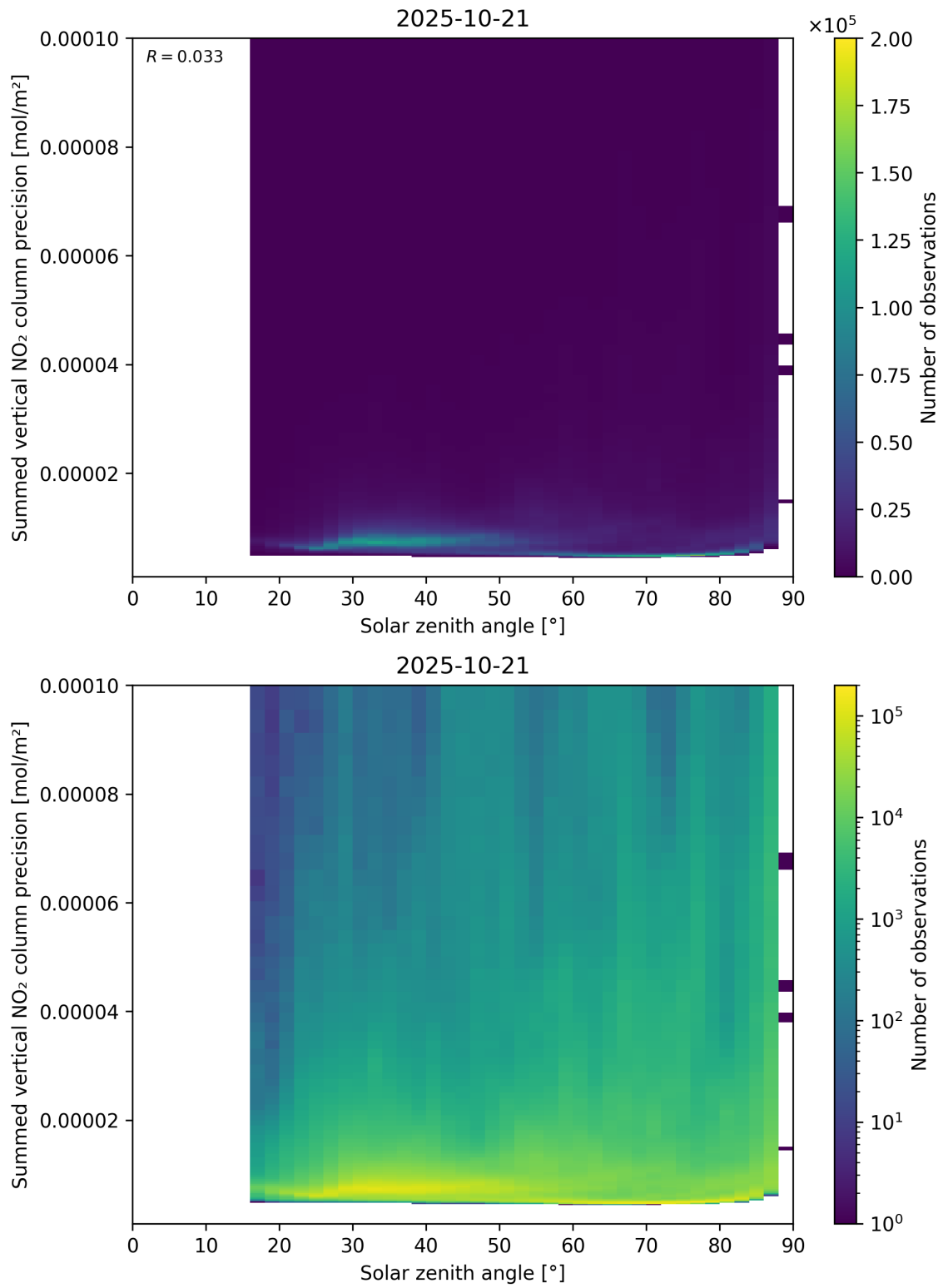
Figure 152: Scatter density plot of “Solar zenith angle” against “Summed vertical NO 2 column precision” for 2025-10-20 to 2025-10-22.
