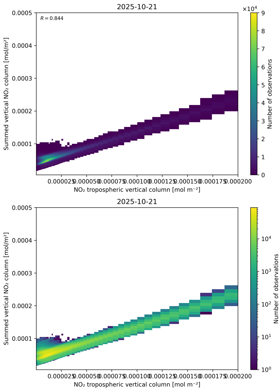
Figure 126: Scatter density plot of “NO 2 tropospheric vertical column” against “Summed vertical NO 2 column” for 2025-10-20 to 2025-10-22.
