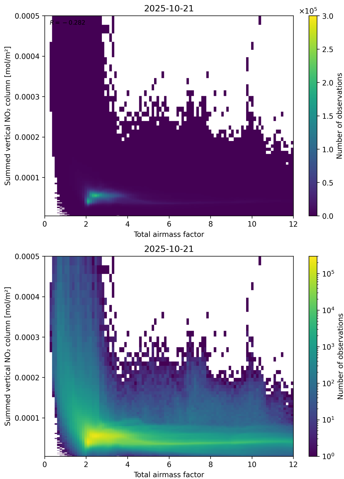
Figure 65: Scatter density plot of “Total airmass factor” against “Summed vertical NO 2 column” for 2025-10-20 to 2025-10-22.
