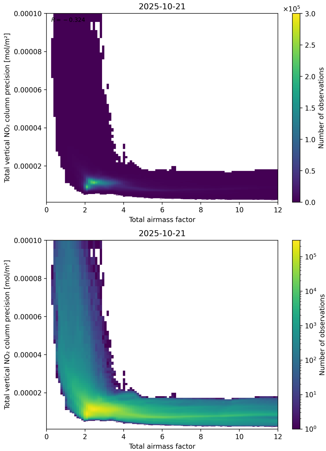
Figure 68: Scatter density plot of “Total airmass factor” against “Total vertical NO 2 column precision” for 2025-10-20 to 2025-10-22.
