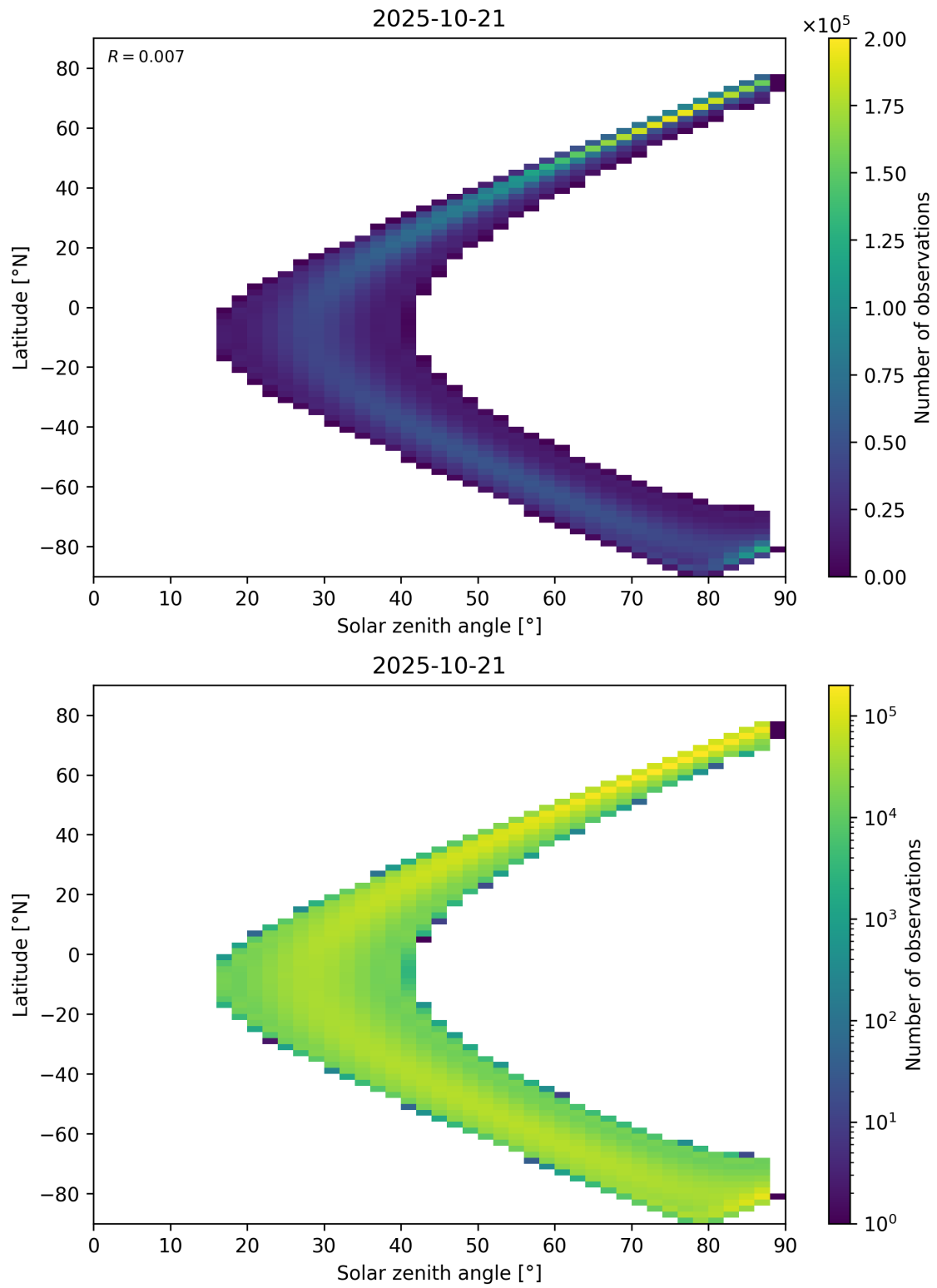
Figure 149: Scatter density plot of “Solar zenith angle” against “Latitude” for 2025-10-20 to 2025-10-22.
