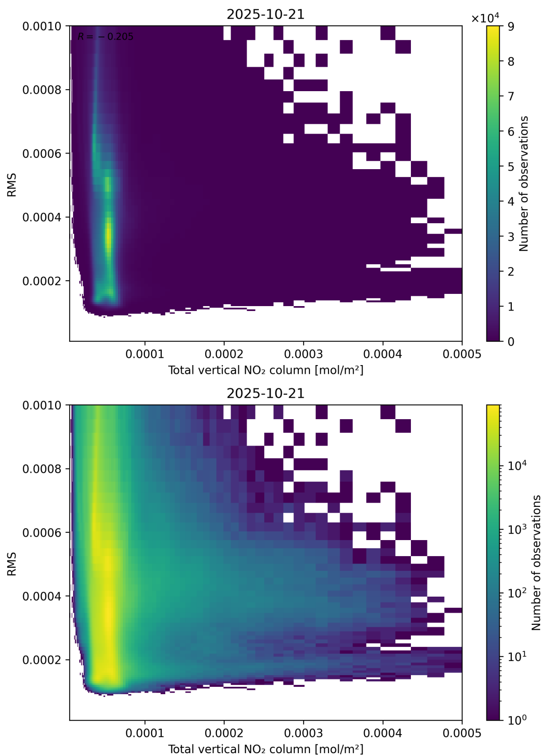
Figure 120: Scatter density plot of “Total vertical NO 2 column” against “RMS” for 2025-10-20 to 2025-10-22.
