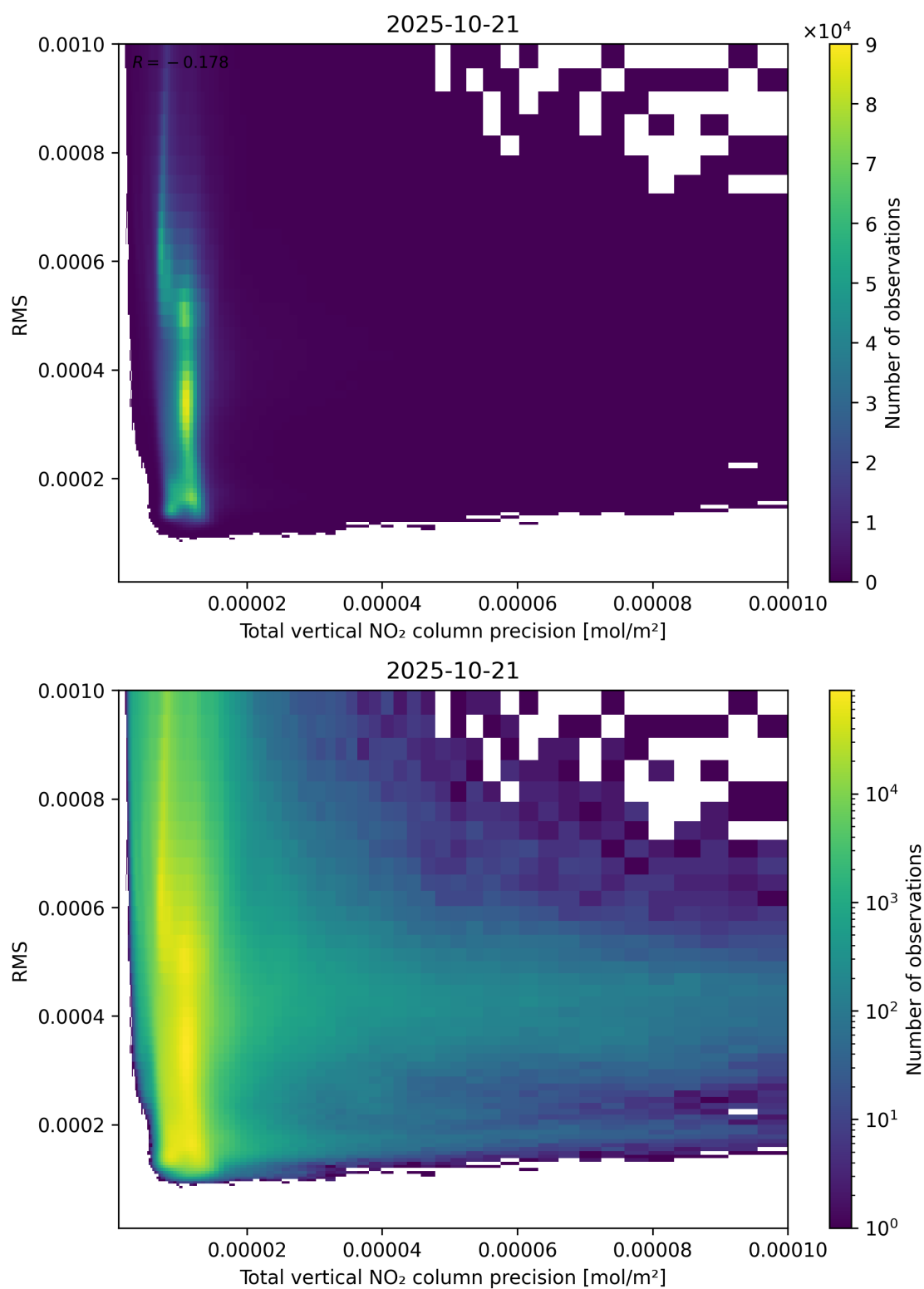
Figure 119: Scatter density plot of “Total vertical NO 2 column precision” against “RMS” for 2025-10-20 to 2025-10-22.
