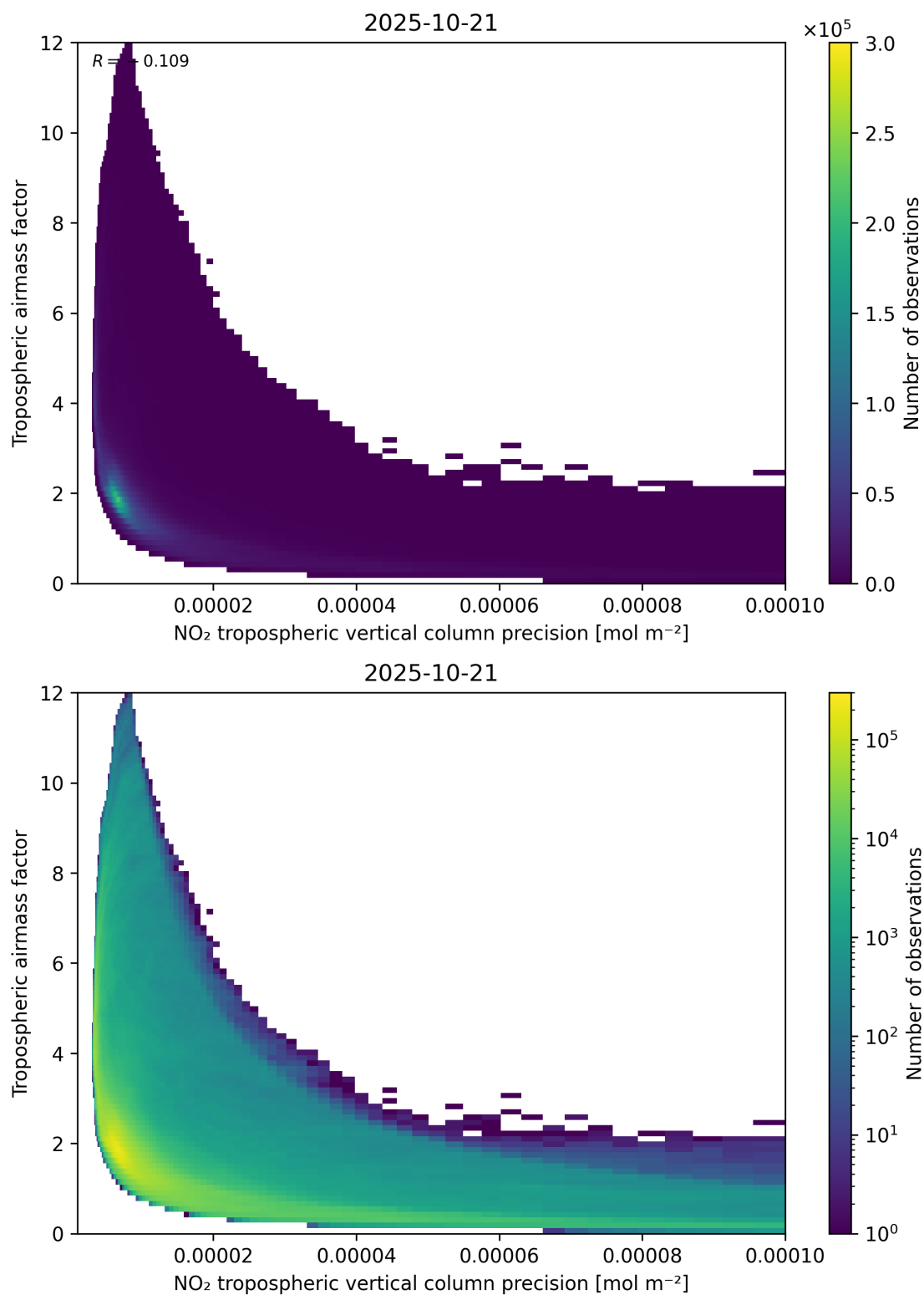
Figure 133: Scatter density plot of “NO 2 tropospheric vertical column precision” against “Tropospheric airmass factor” for 2025-10-20 to 2025-10-22.
