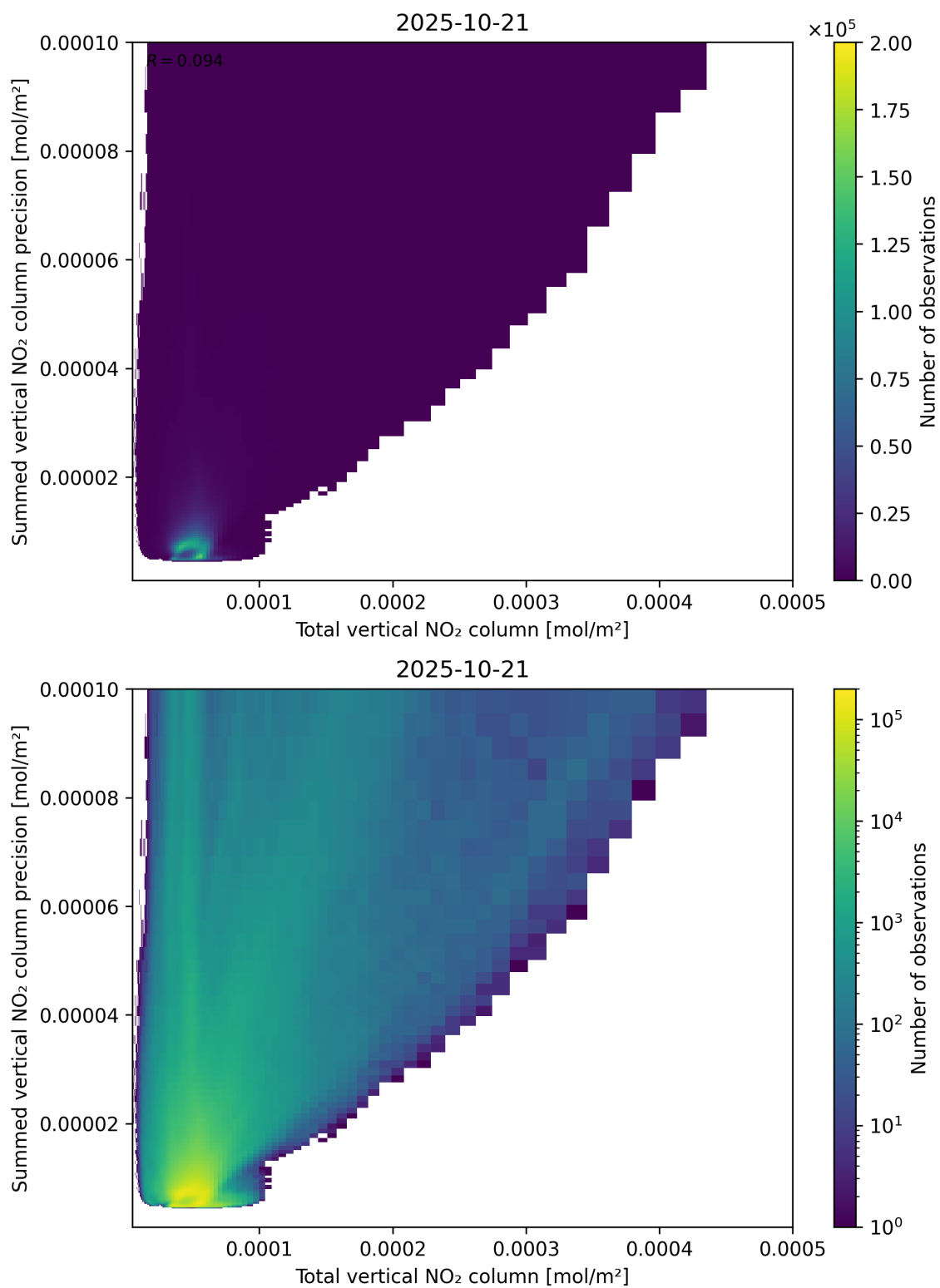
Figure 113: Scatter density plot of “Total vertical NO 2 column” against “Summed vertical NO 2 column precision” for 2025-10-20 to 2025-10-22.
