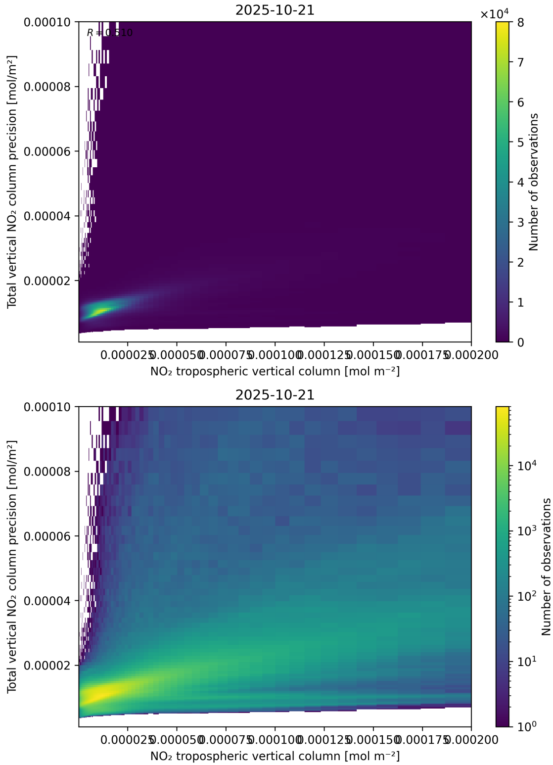
Figure 129: Scatter density plot of “NO 2 tropospheric vertical column” against “Total vertical NO 2 column precision” for 2025-10-20 to 2025-10-22.
