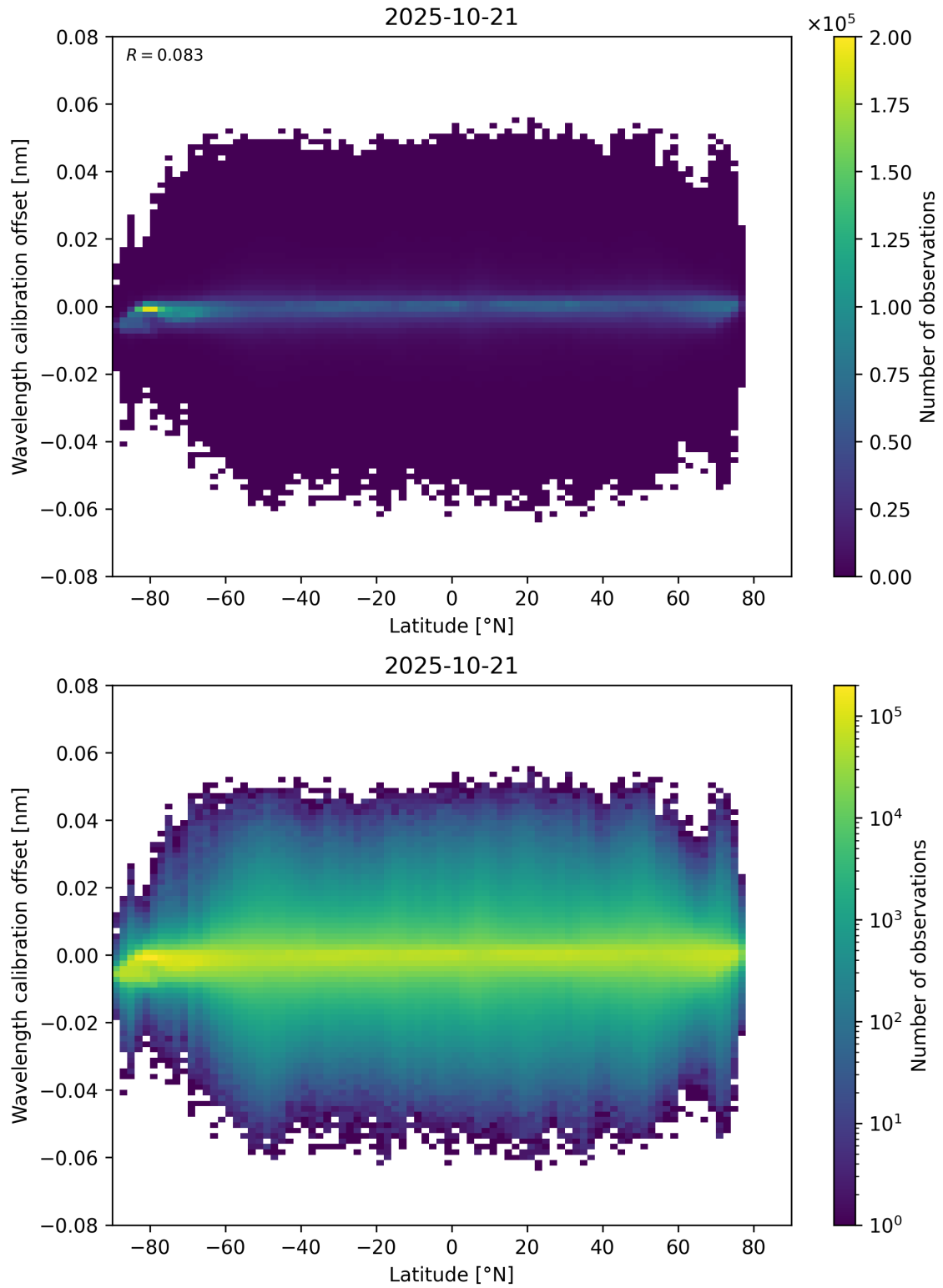
Figure 95: Scatter density plot of “Latitude” against “Wavelength calibration offset” for 2025-10-20 to 2025-10-22.
