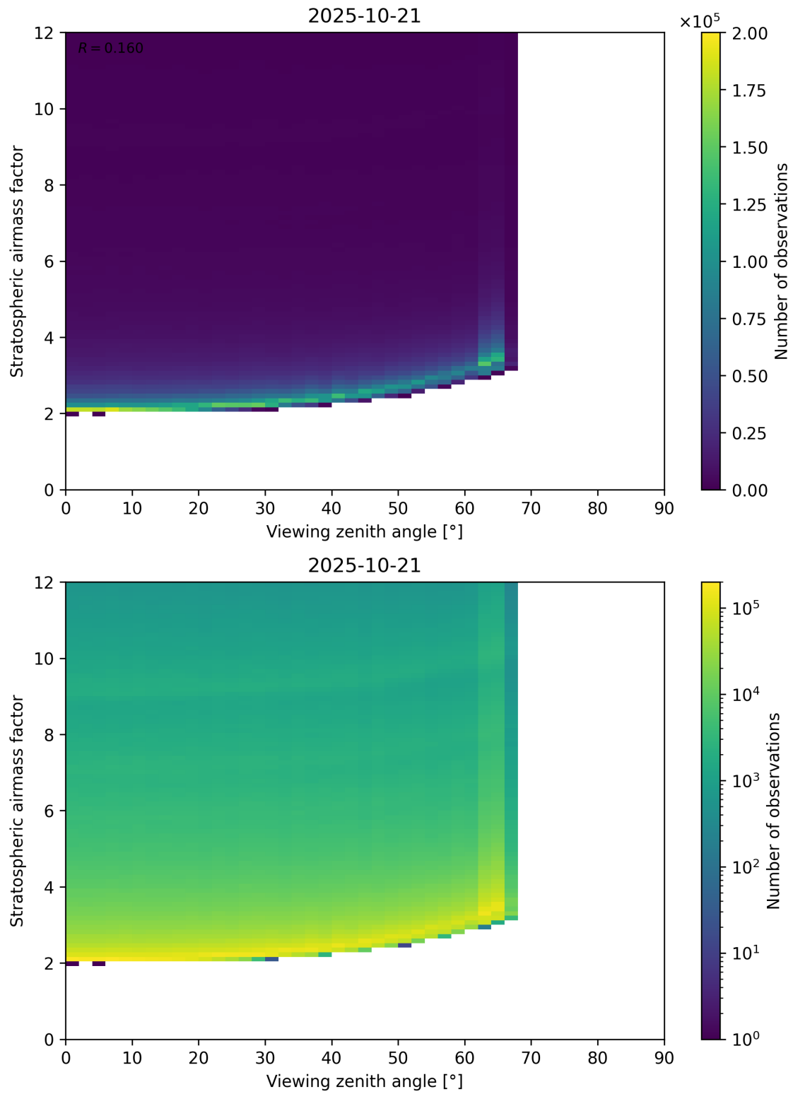
Figure 159: Scatter density plot of “Viewing zenith angle” against “Stratospheric airmass factor” for 2025-10-20 to 2025-10-22.
