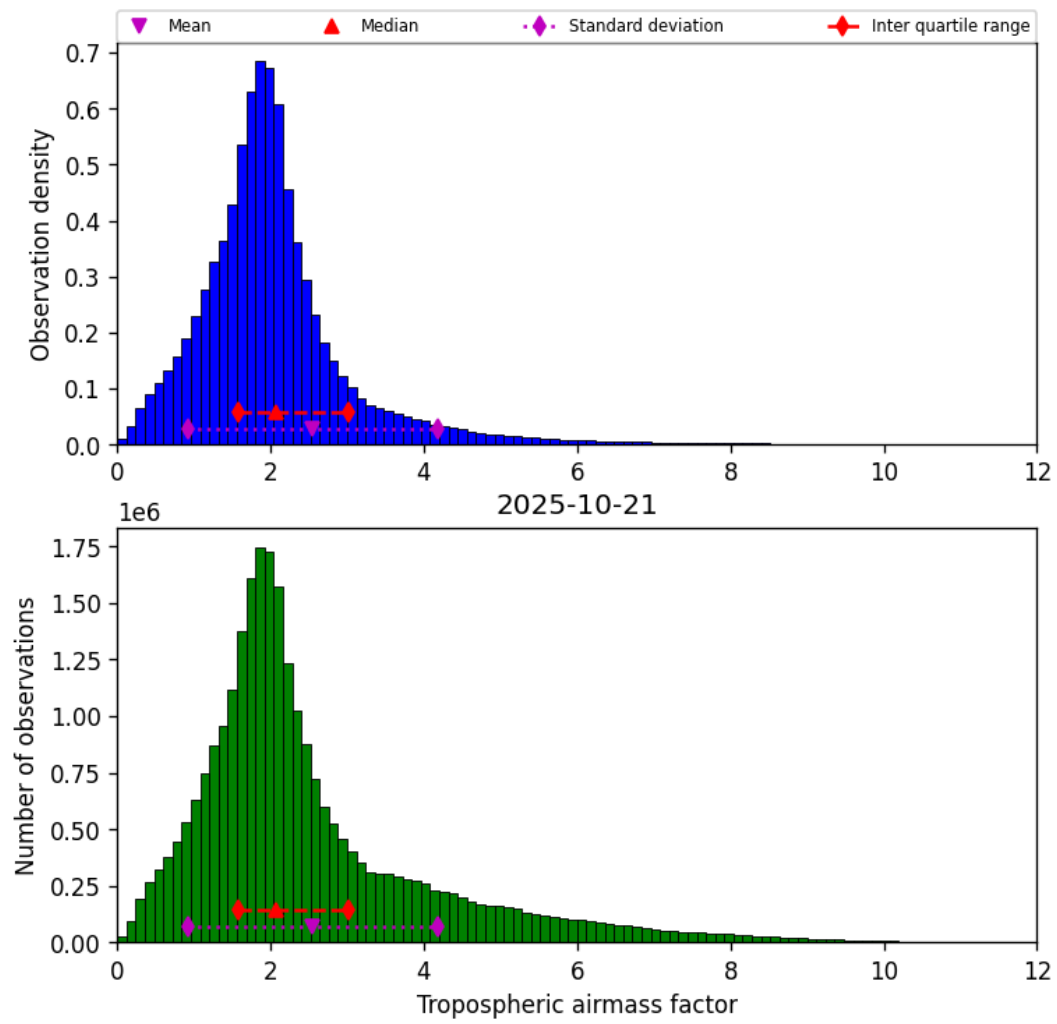
Figure 31: Histogram of “Tropospheric airmass factor” for 2025-10-20 to 2025-10-22
