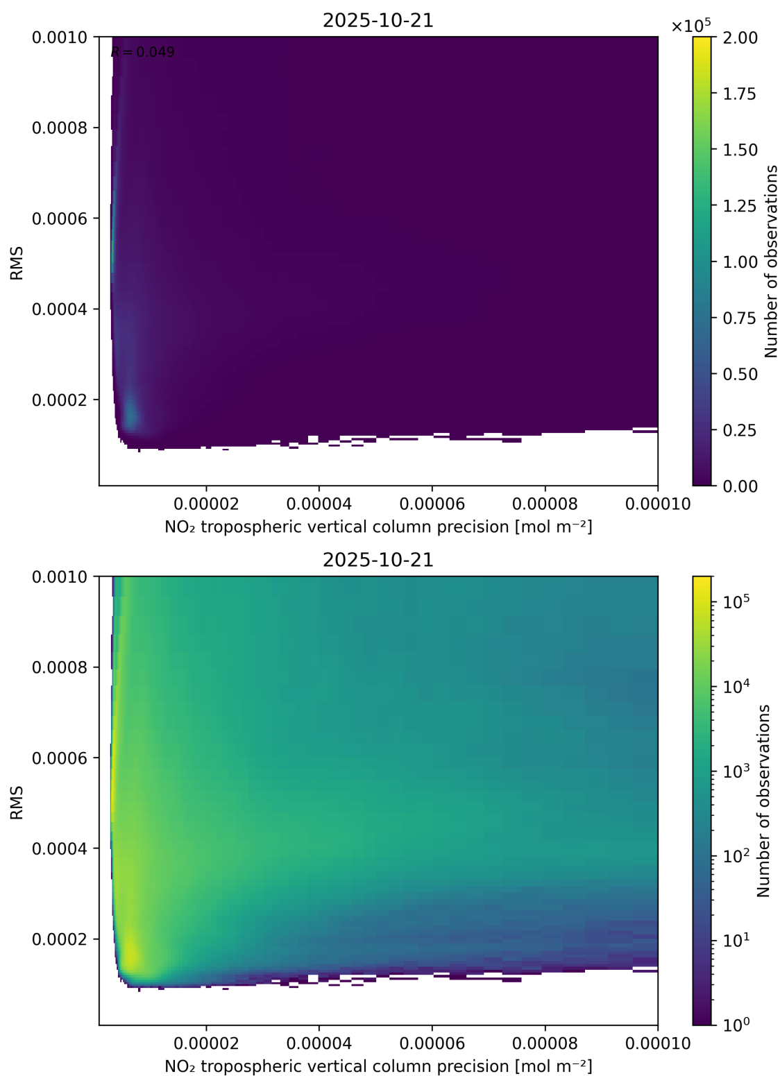
Figure 140: Scatter density plot of “NO 2 tropospheric vertical column precision” against “RMS” for 2025-10-20 to 2025-10-22.
