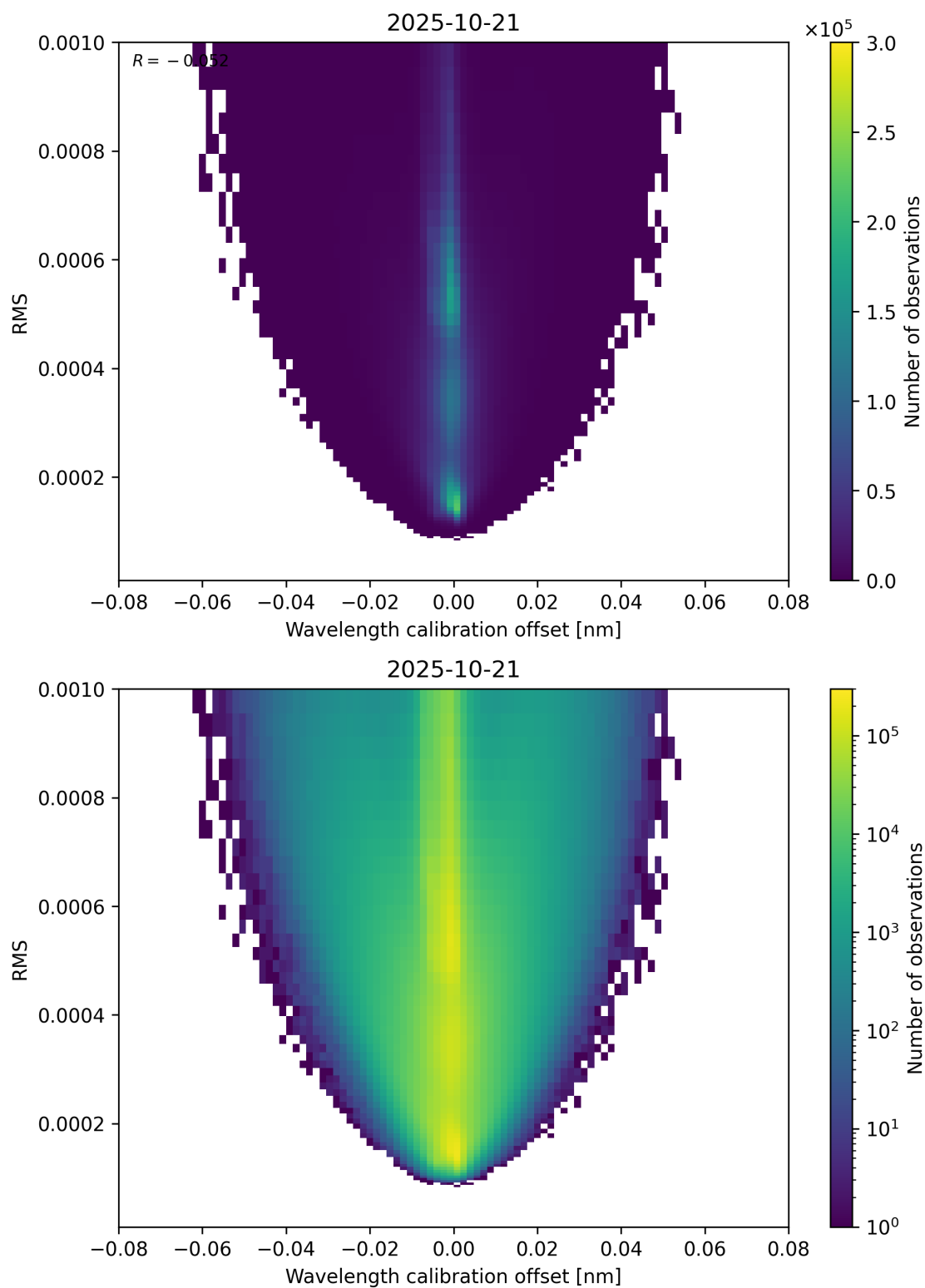
Figure 181: Scatter density plot of “Wavelength calibration offset” against “RMS” for 2025-10-20 to 2025-10-22.
