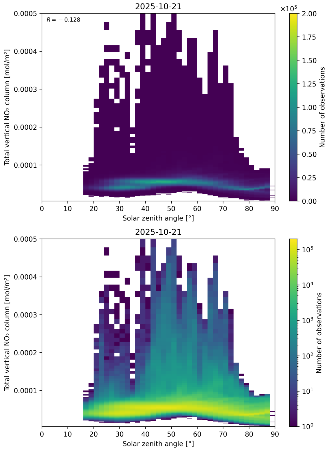
Figure 153: Scatter density plot of “Solar zenith angle” against “Total vertical NO 2 column” for 2025-10-20 to 2025-10-22.
