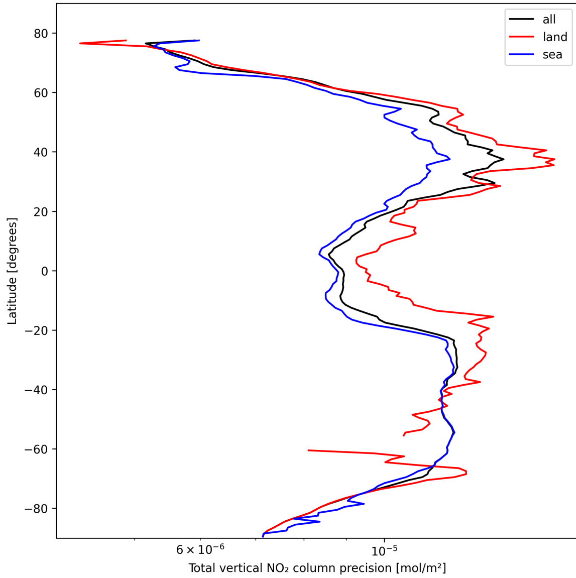
Figure 22: Zonal average of “Total vertical NO 2 column precision” for 2025-10-20 to 2025-10-22.
