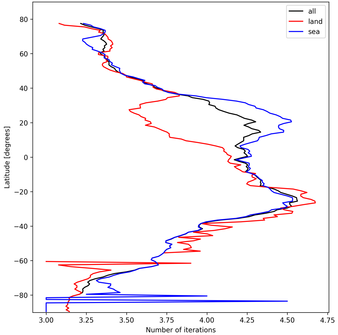
Figure 17: Zonal average of “Number of iterations” for 2025-10-20 to 2025-10-22.
