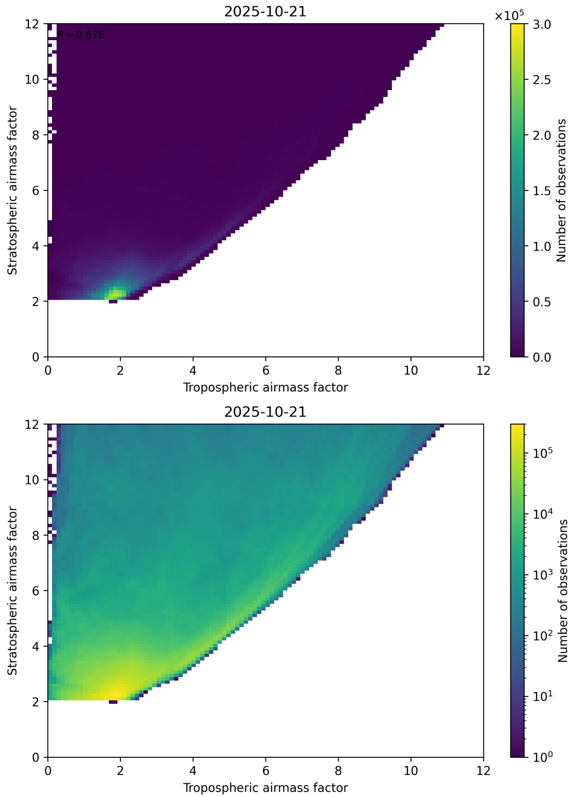
Figure 71: Scatter density plot of “Tropospheric airmass factor” against “Stratospheric airmass factor” for 2025-10-20 to 2025-10-22.
