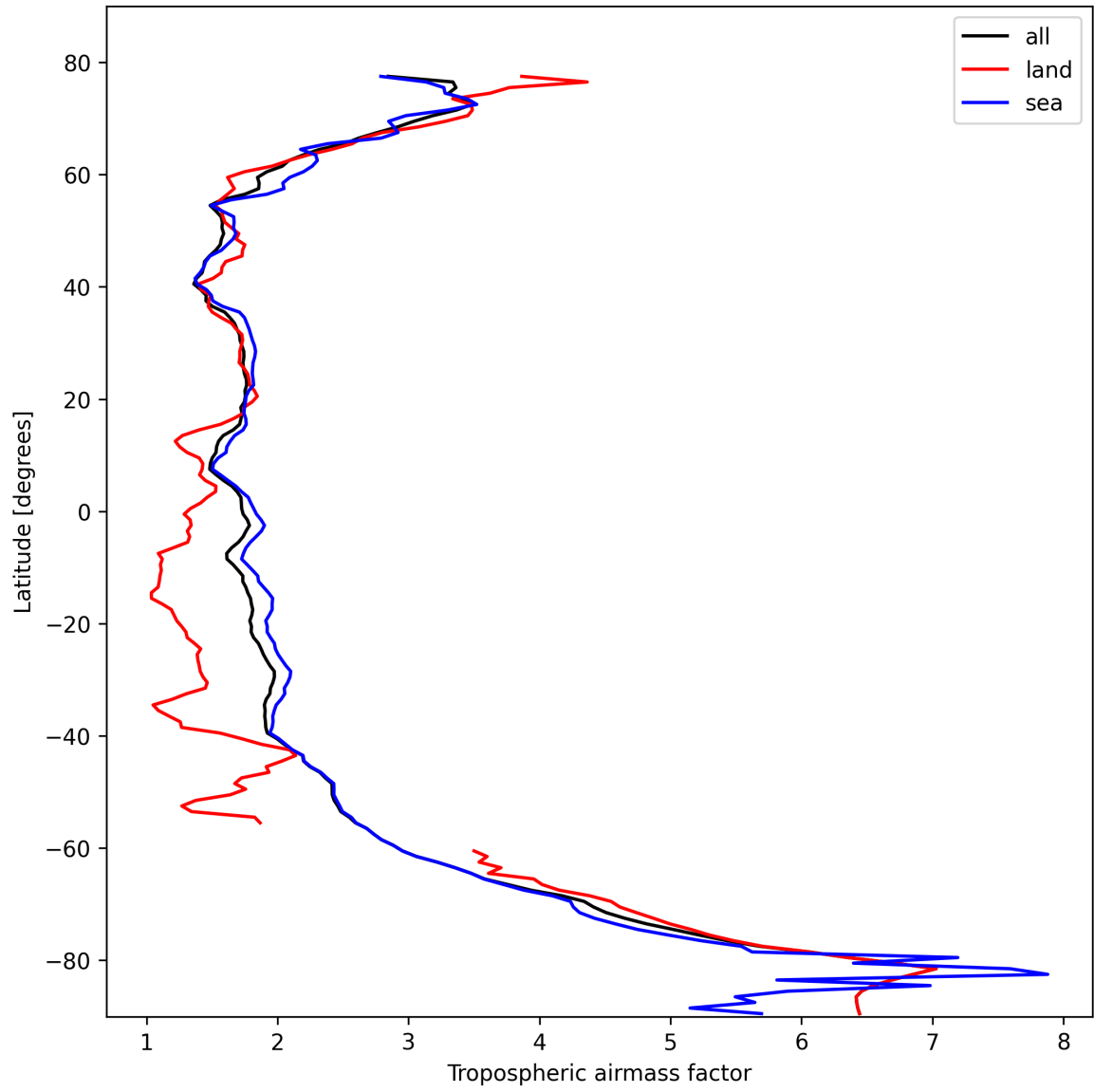
Figure 14: Zonal average of “Tropospheric airmass factor” for 2025-10-20 to 2025-10-22.
