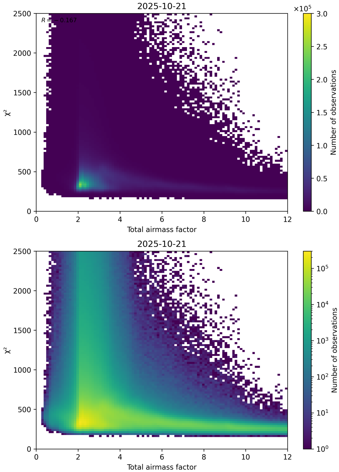
Figure 63: Scatter density plot of “Total airmass factor” against “ \chi^2 ” for 2025-10-20 to 2025-10-22.
