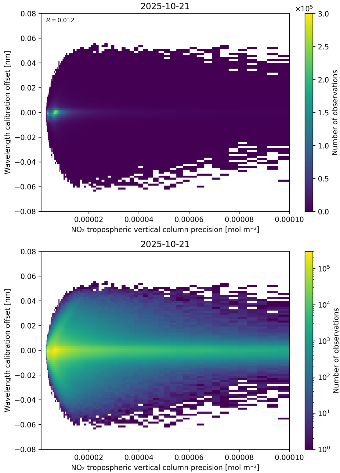
Figure 141: Scatter density plot of “NO 2 tropospheric vertical column precision” against “Wavelength calibration offset” for 2025-10-20 to 2025-10-22.
