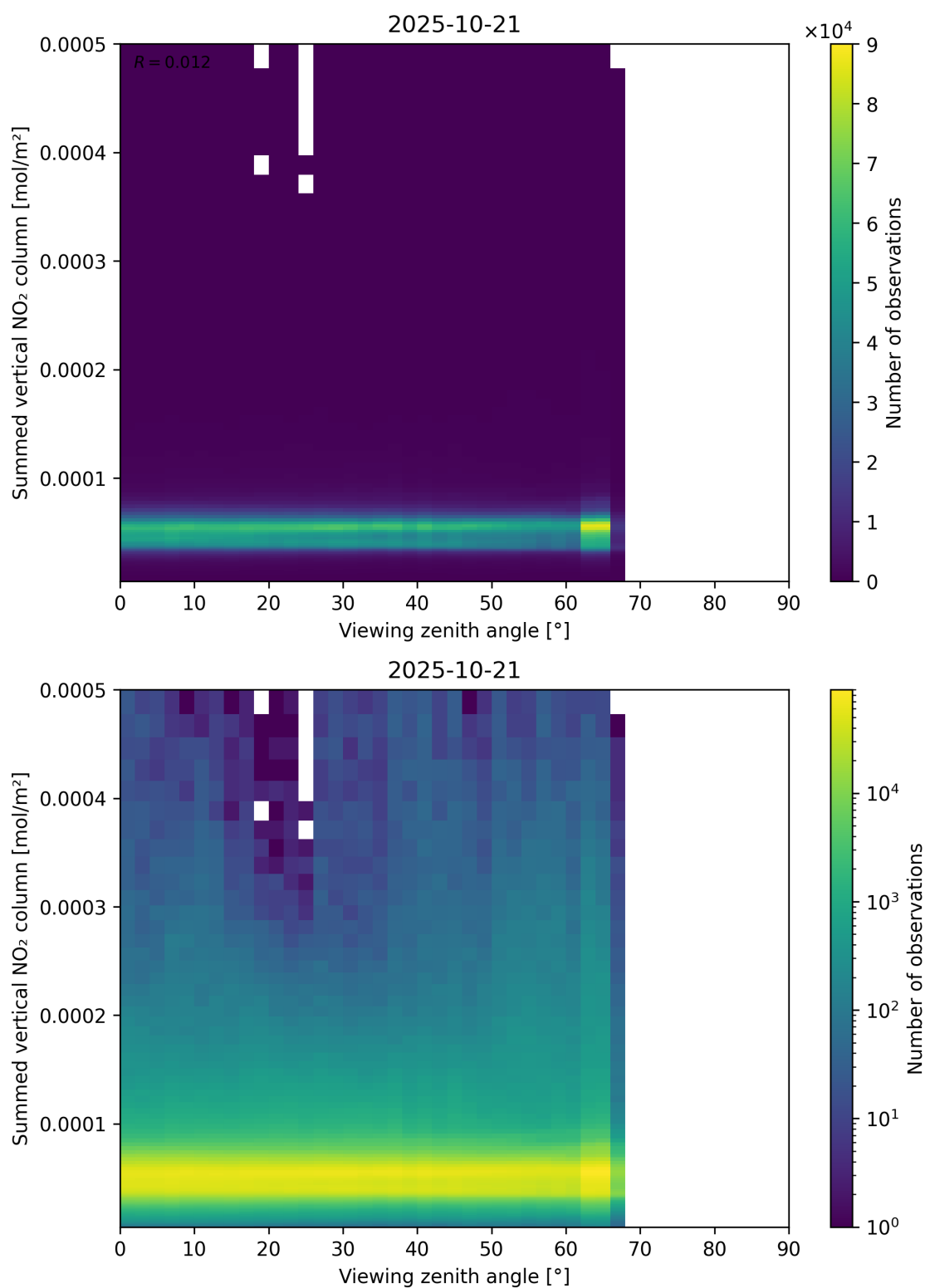
Figure 165: Scatter density plot of “Viewing zenith angle” against “Summed vertical NO 2 column” for 2025-10-20 to 2025-10-22.
