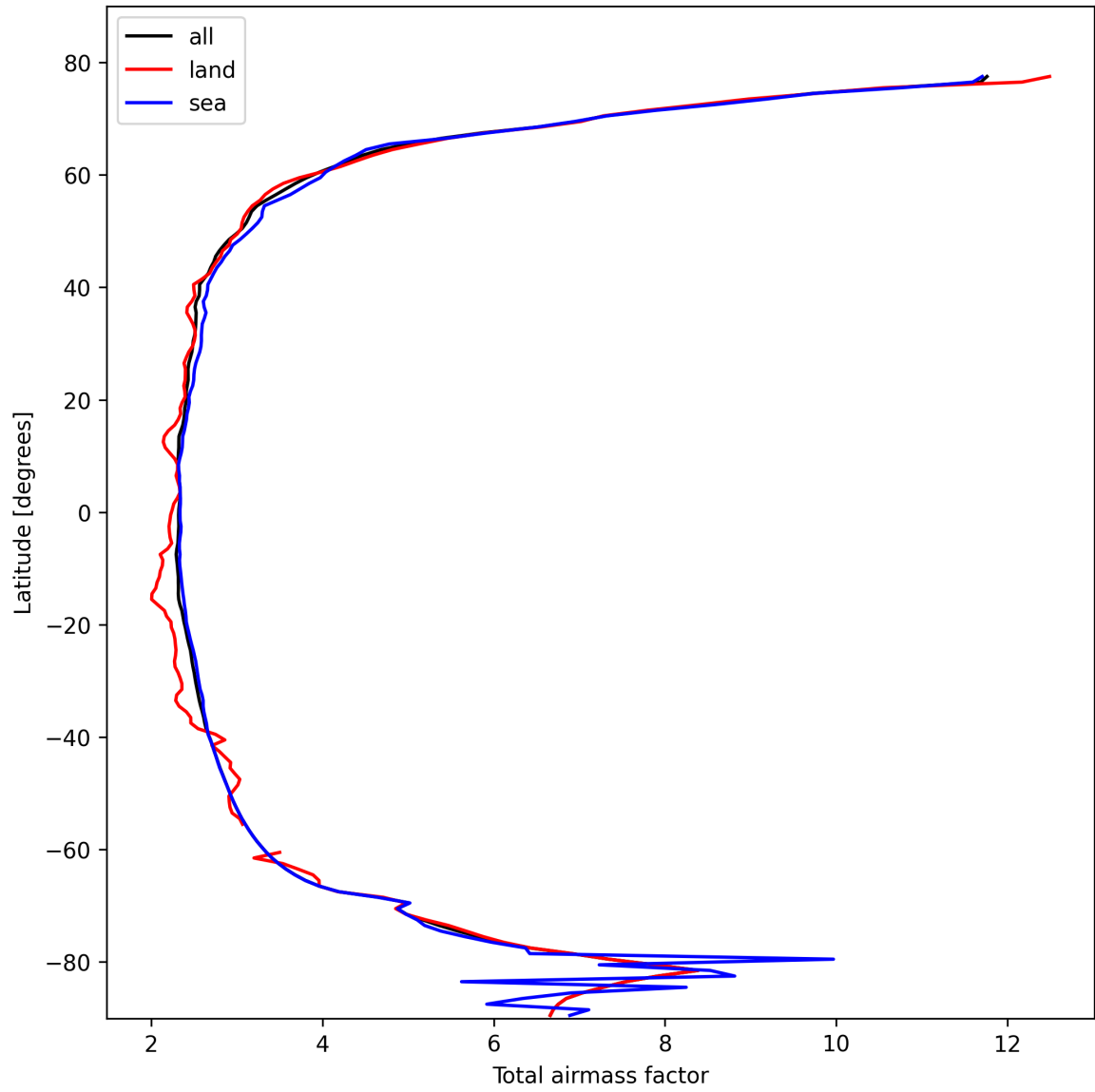
Figure 15: Zonal average of “Total airmass factor” for 2025-10-20 to 2025-10-22.
