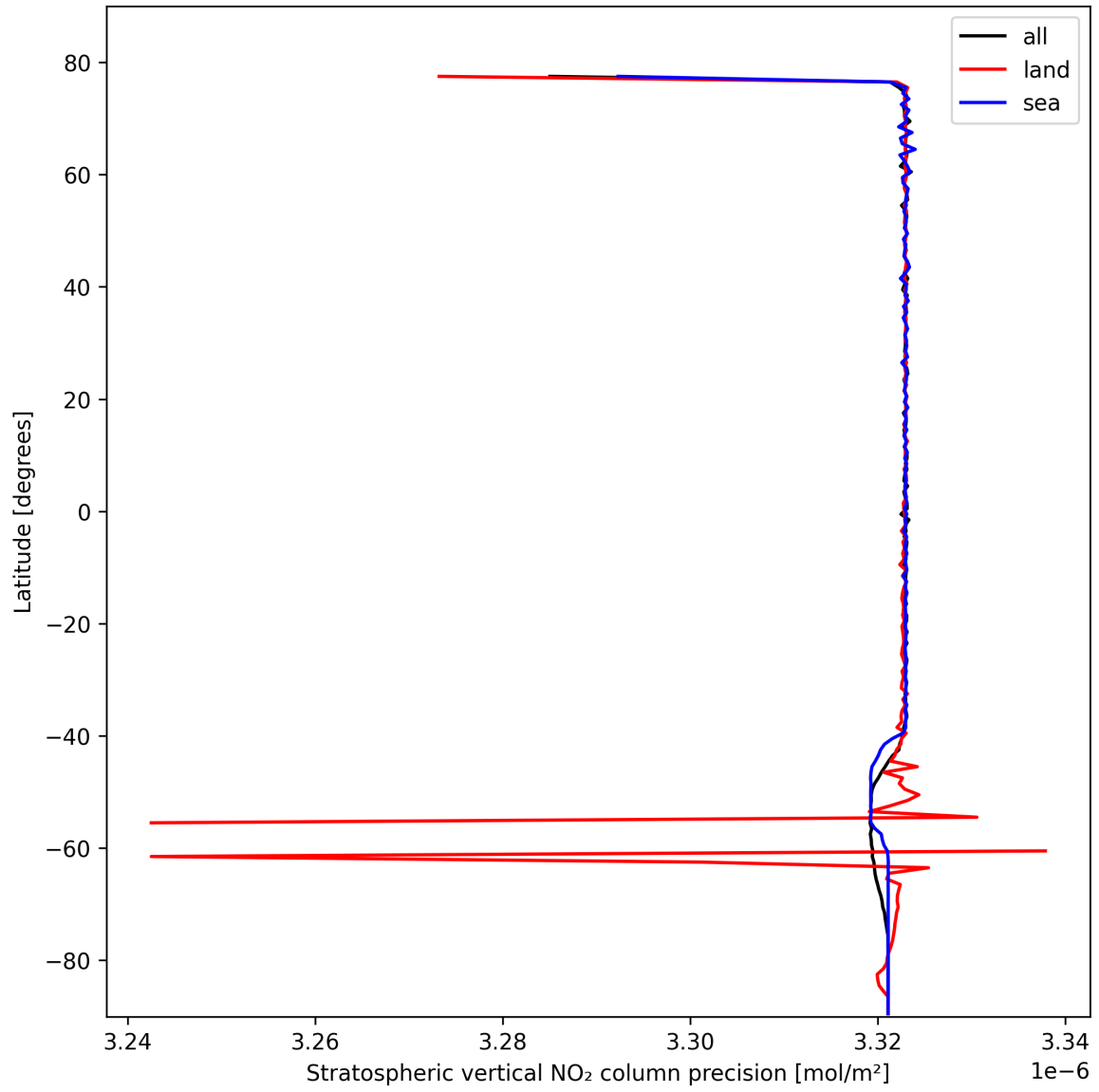
Figure 20: Zonal average of “Stratospheric vertical NO 2 column precision” for 2025-10-20 to 2025-10-22.
