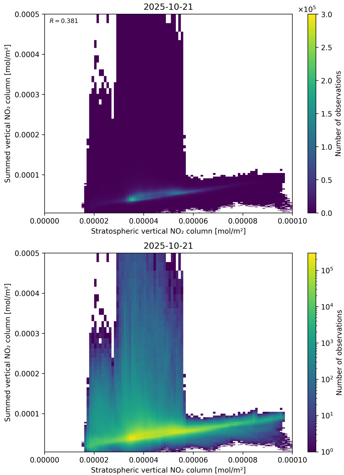
Figure 98: Scatter density plot of “Stratospheric vertical NO 2 column” against “Summed vertical NO 2 column” for 2025-10-20 to 2025-10-22.
