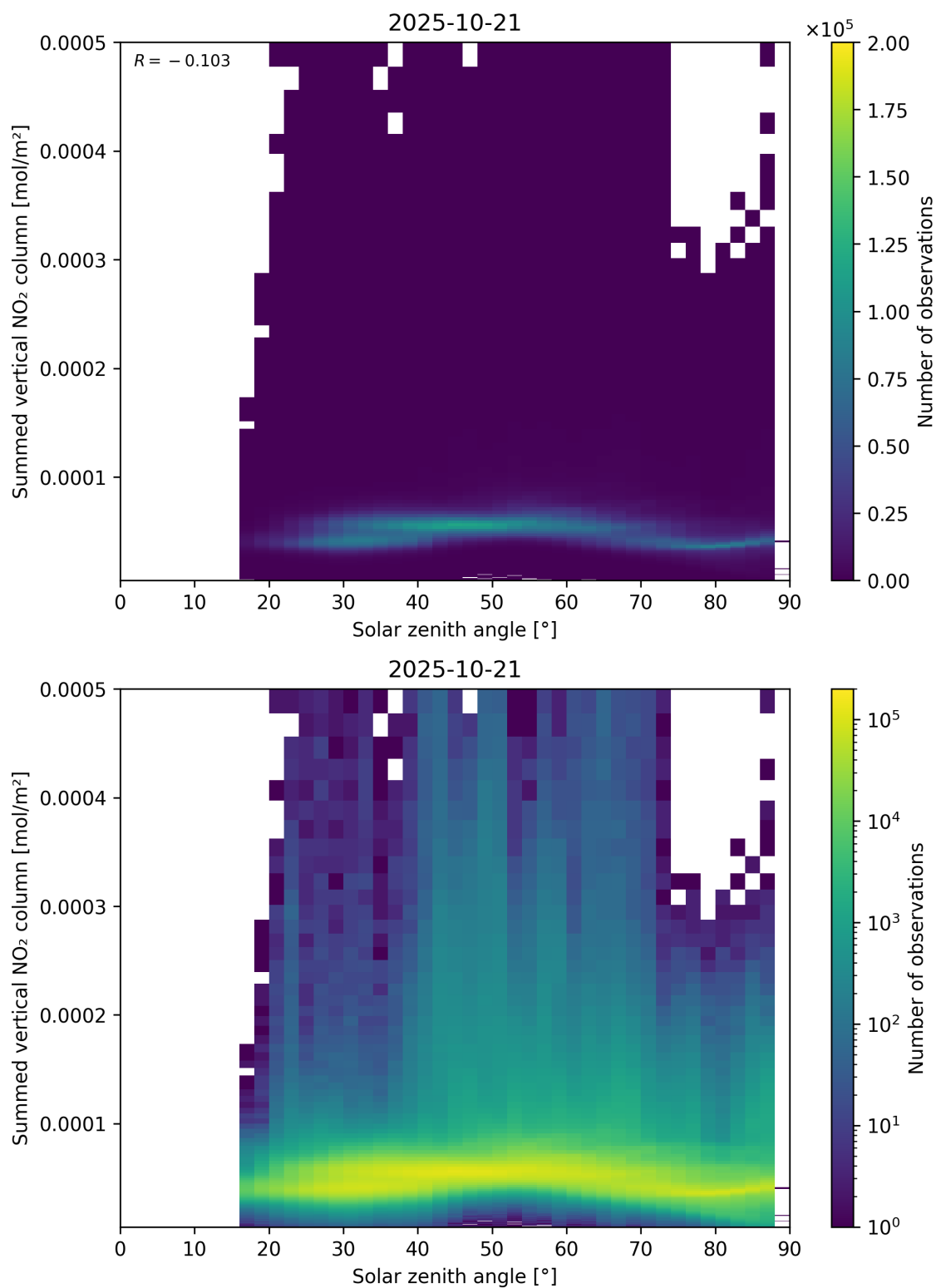
Figure 151: Scatter density plot of “Solar zenith angle” against “Summed vertical NO 2 column” for 2025-10-20 to 2025-10-22.
