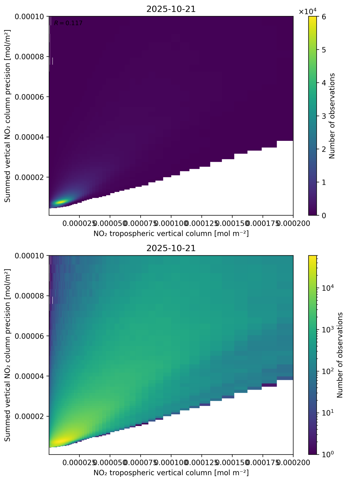
Figure 127: Scatter density plot of “NO 2 tropospheric vertical column” against “Summed vertical NO 2 column precision” for 2025-10-20 to 2025-10-22.
