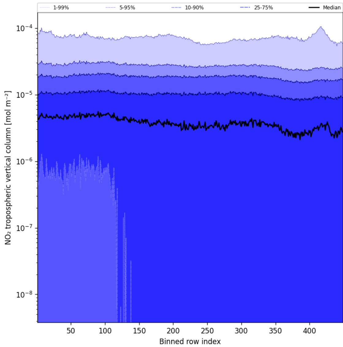
Figure 46: Along track statistics of “NO 2 tropospheric vertical column” for 2025-10-20 to 2025-10-22
