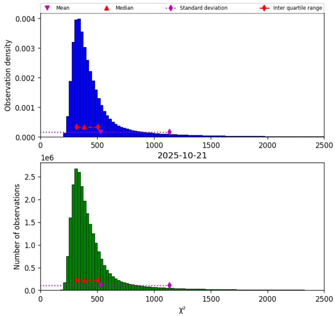
Figure 42: Histogram of " \chi^2 " for 2025-10-20 to 2025-10-22
