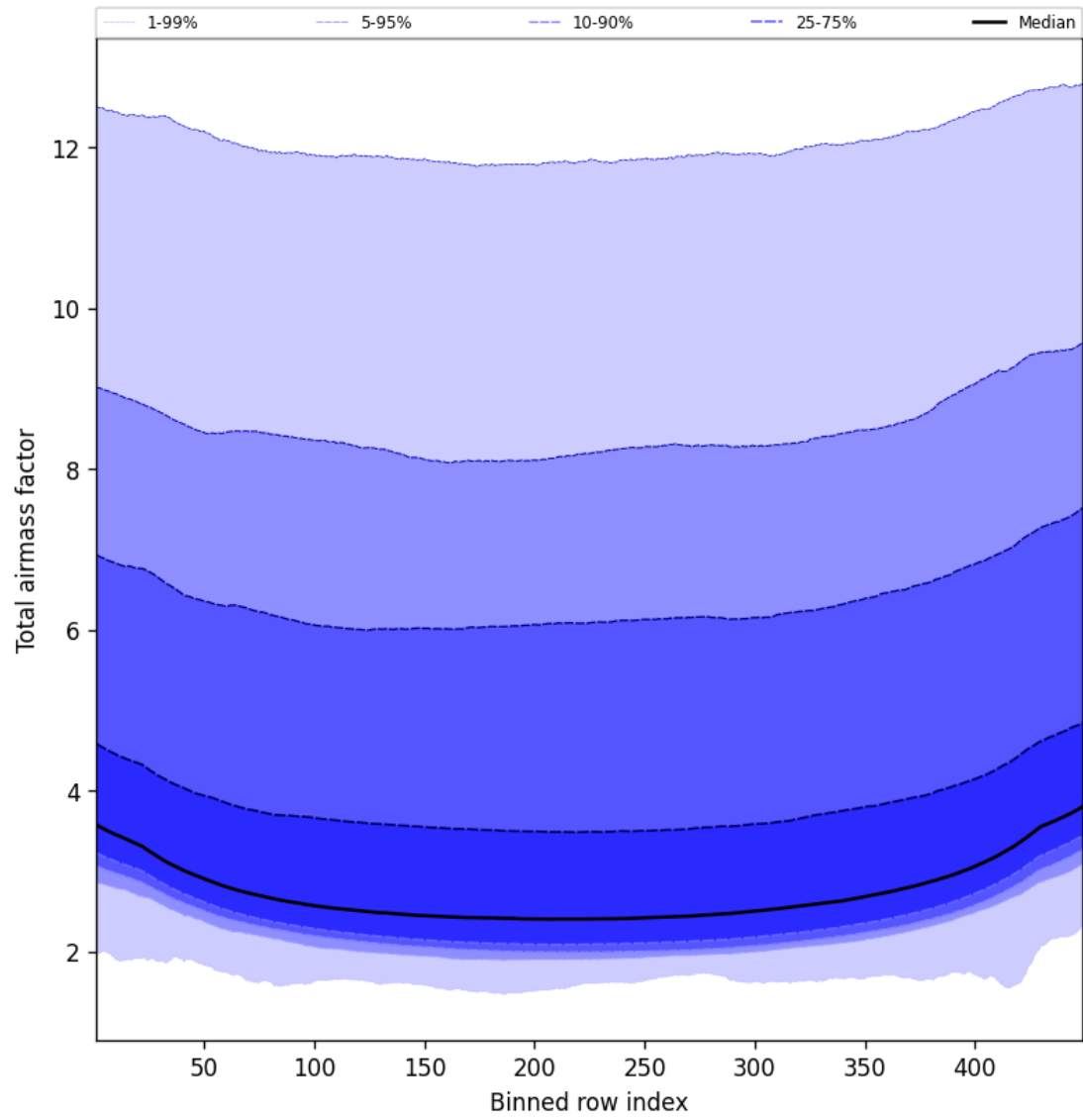
Figure 49: Along track statistics of “Total airmass factor” for 2025-10-20 to 2025-10-22
