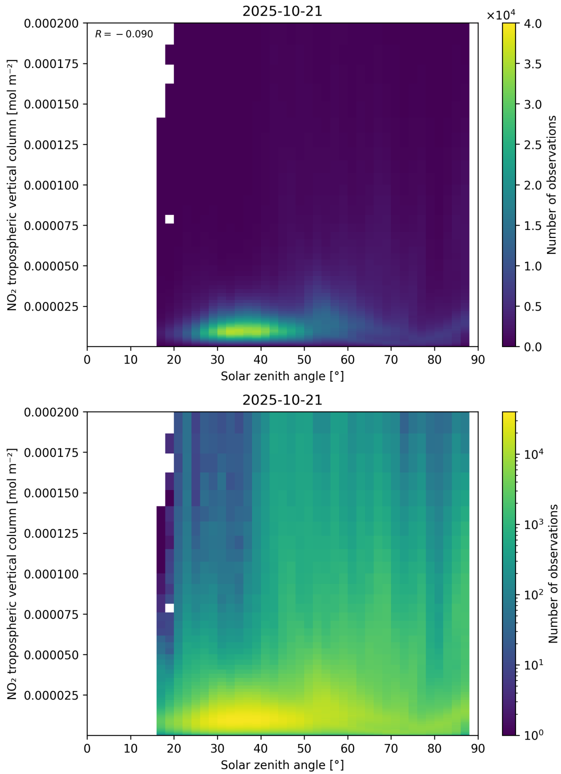
Figure 155: Scatter density plot of “Solar zenith angle” against “NO 2 tropospheric vertical column” for 2025-10-20 to 2025-10-22.
