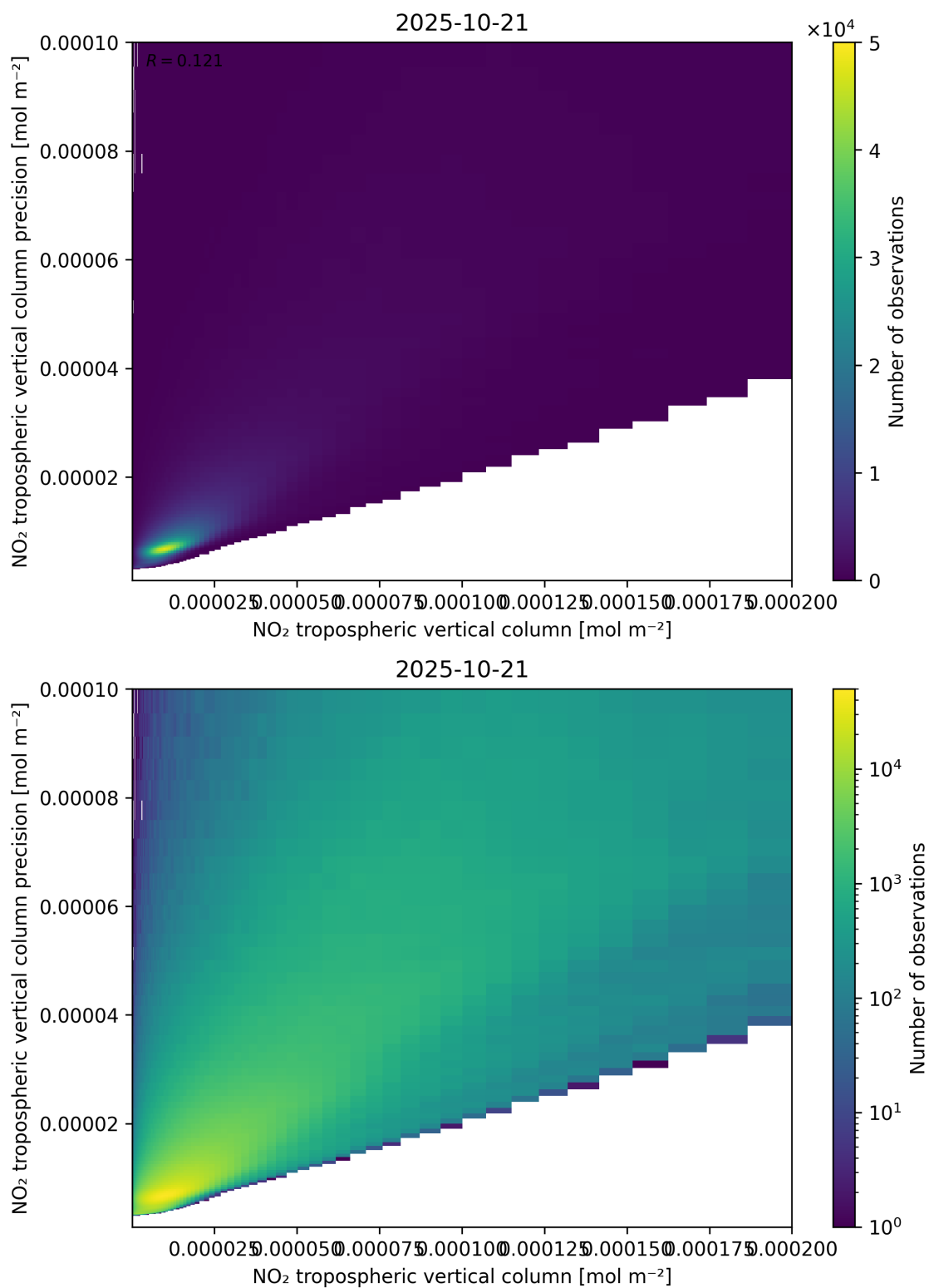
Figure 130: Scatter density plot of “NO 2 tropospheric vertical column” against “NO 2 tropospheric vertical column precision” for 2025-10-20 to 2025-10-22.
