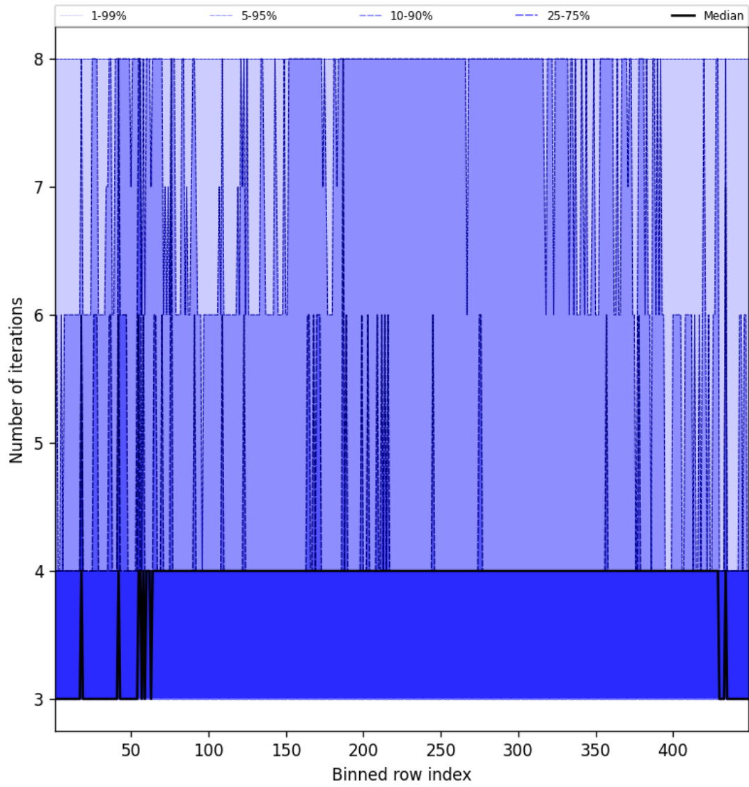
Figure 51: Along track statistics of “Number of iterations” for 2025-10-20 to 2025-10-22
