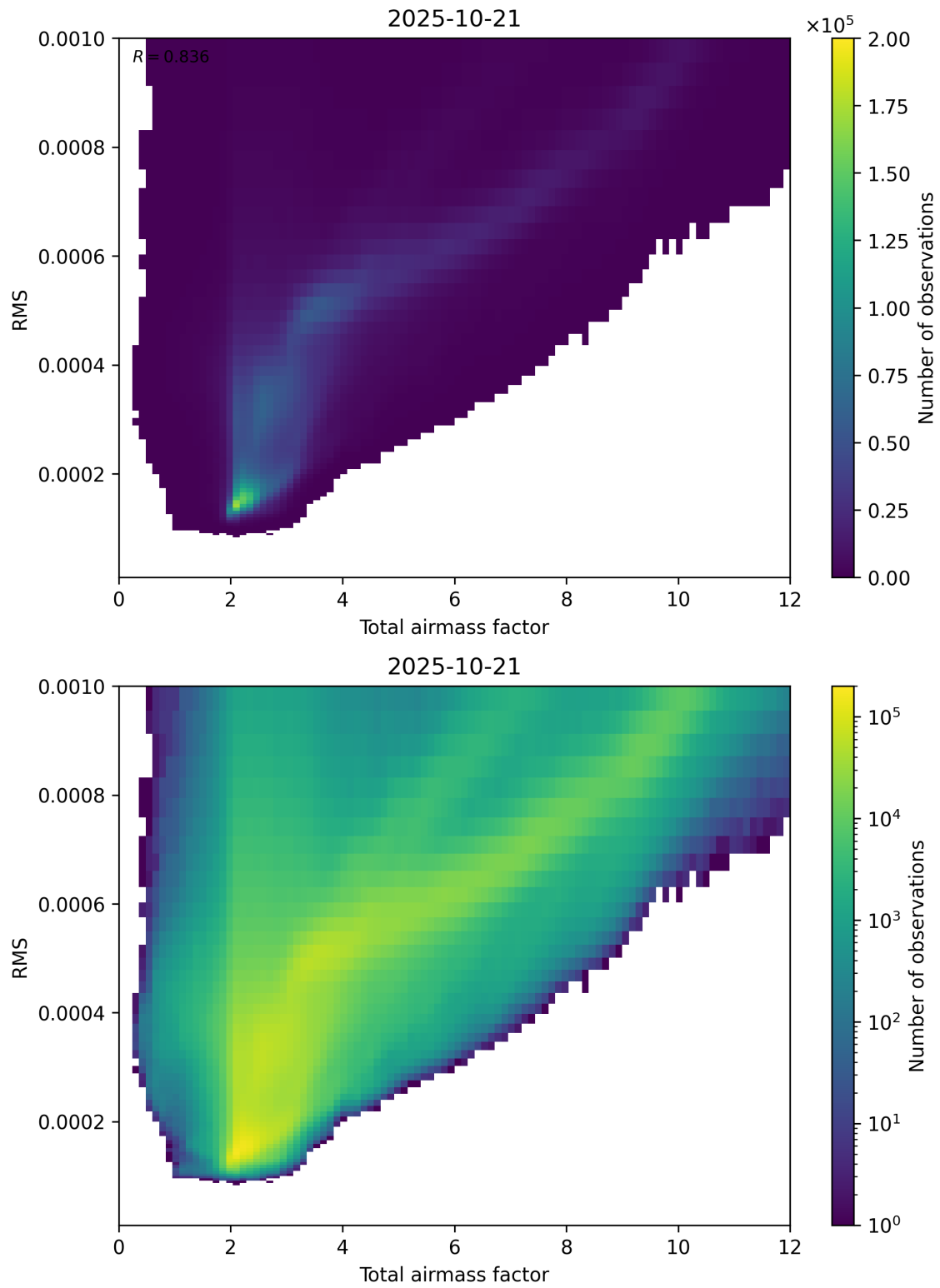
Figure 69: Scatter density plot of “Total airmass factor” against “RMS” for 2025-10-20 to 2025-10-22.
