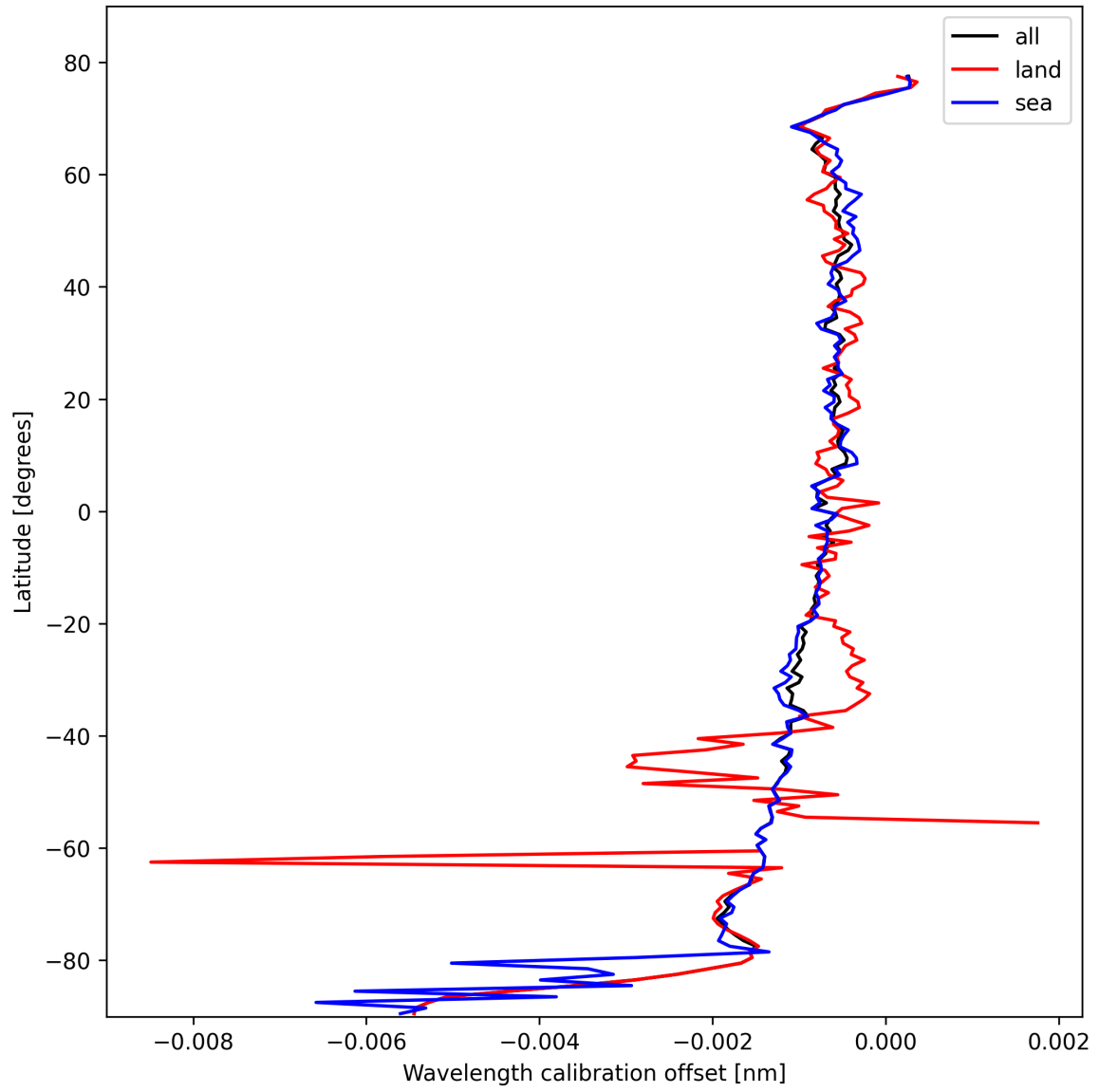
Figure 18: Zonal average of “Wavelength calibration offset” for 2025-10-20 to 2025-10-22.
