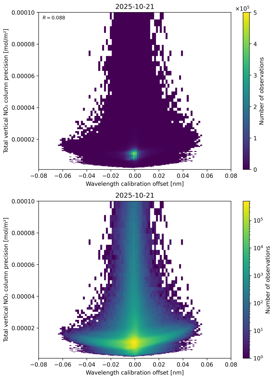
Figure 180: Scatter density plot of “Wavelength calibration offset” against “Total vertical NO 2 column precision” for 2025-10-20 to 2025-10-22.
