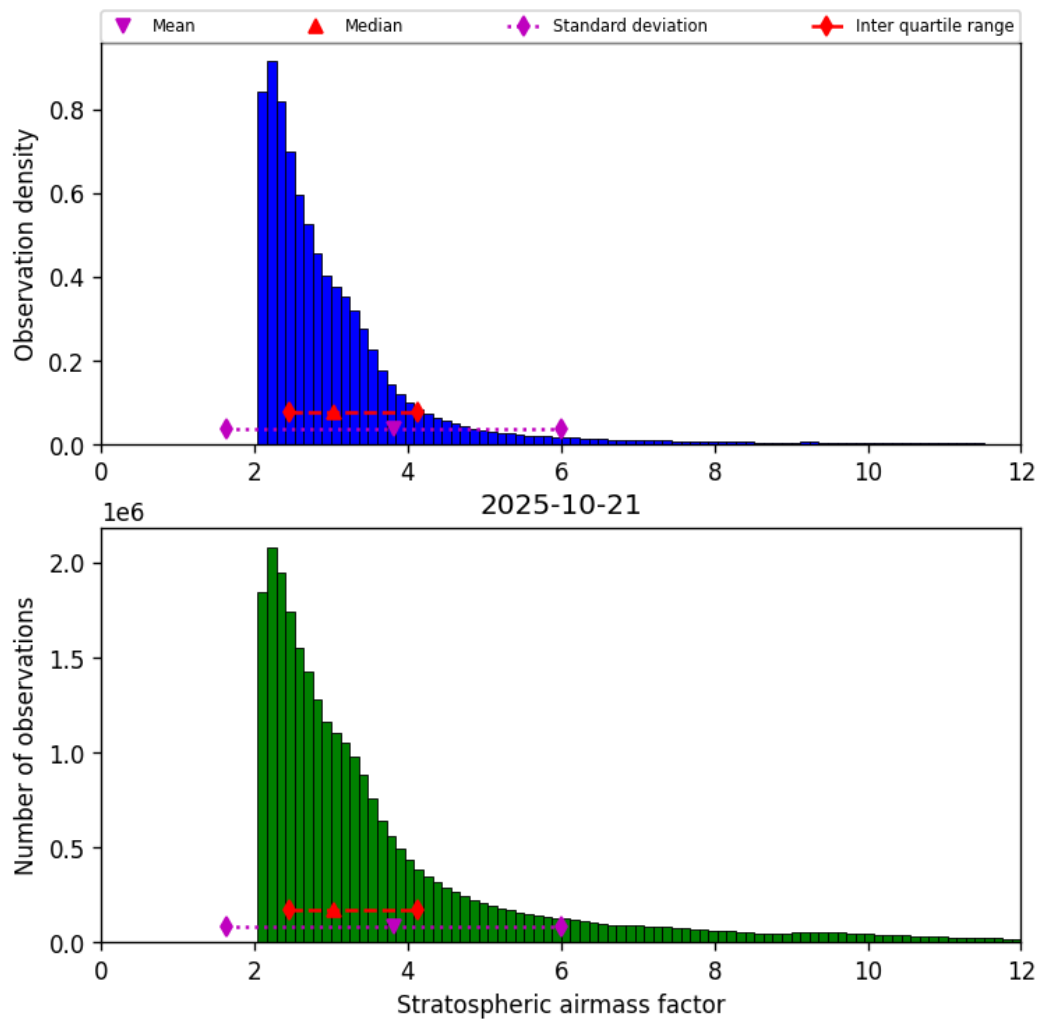
Figure 44: Histogram of “Stratospheric airmass factor” for 2025-10-20 to 2025-10-22
