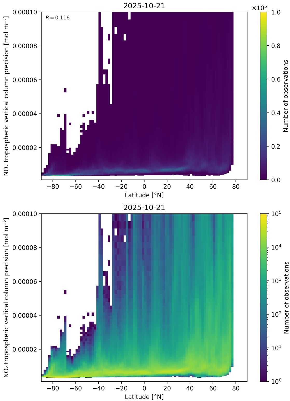
Figure 93: Scatter density plot of “Latitude” against “NO 2 tropospheric vertical column precision” for 2025-10-20 to 2025-10-22.
