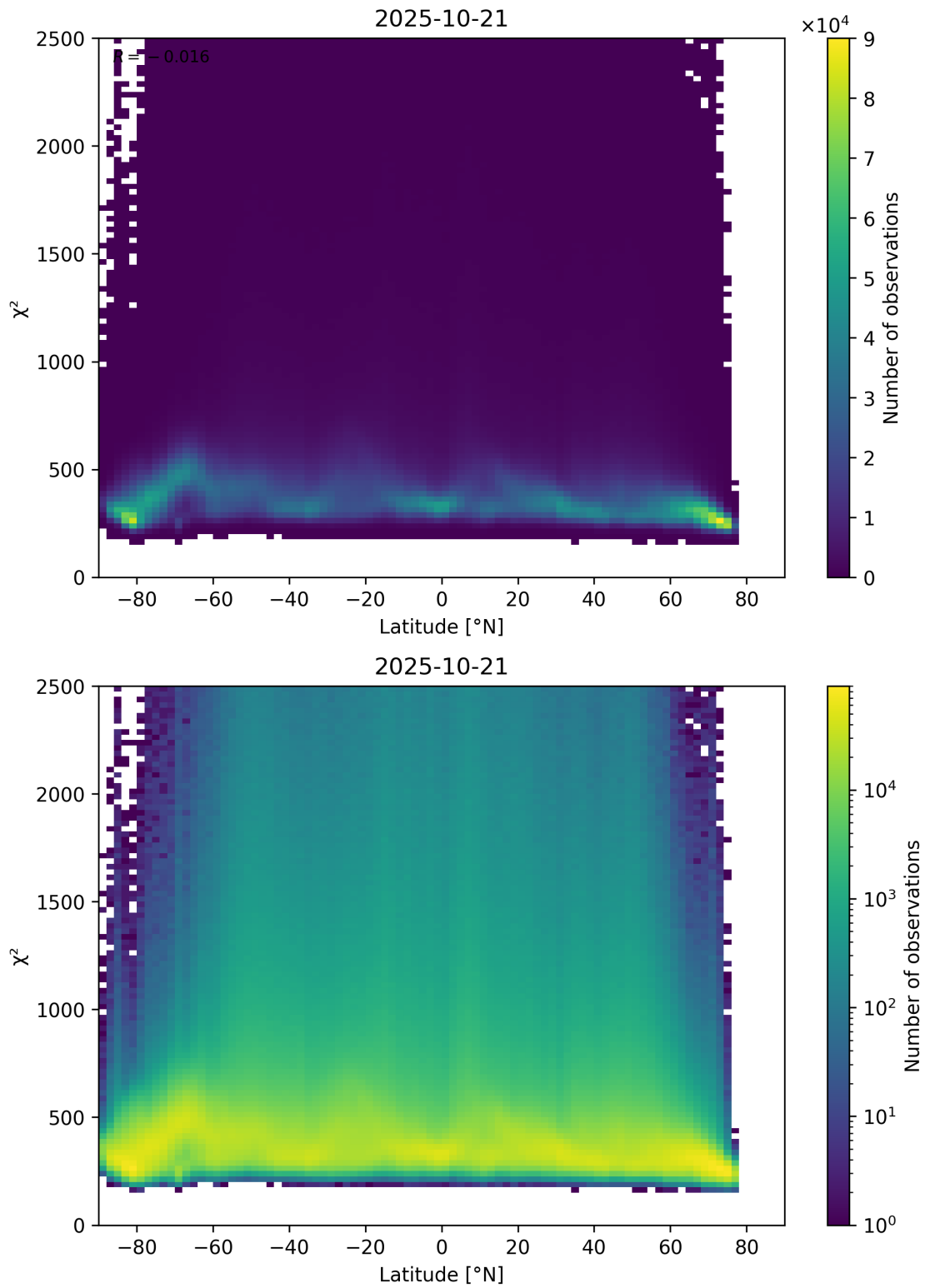
Figure 86: Scatter density plot of “Latitude” against “ \chi^2 ” for 2025-10-20 to 2025-10-22.
