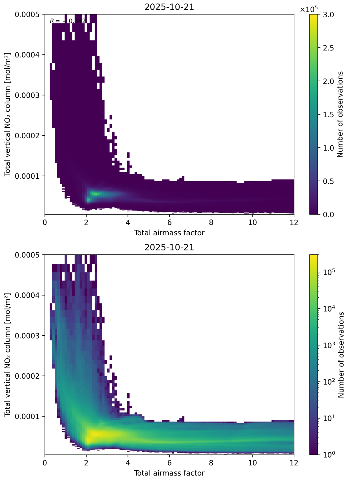
Figure 67: Scatter density plot of “Total airmass factor” against “Total vertical NO 2 column” for 2025-10-20 to 2025-10-22.
