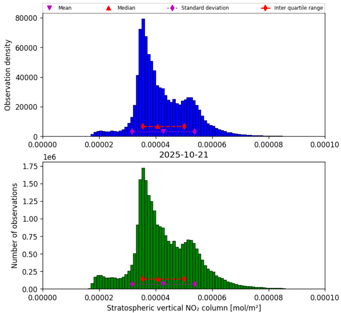
Figure 36: Histogram of “Stratospheric vertical NO 2 column” for 2025-10-20 to 2025-10-22
