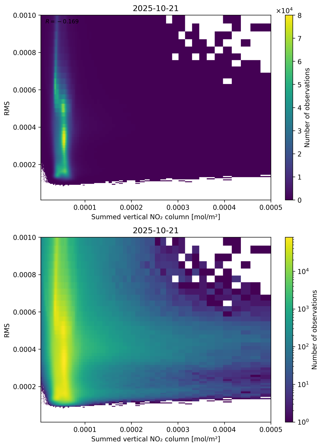
Figure 109: Scatter density plot of “Summed vertical NO 2 column” against “RMS” for 2025-10-20 to 2025-10-22.
