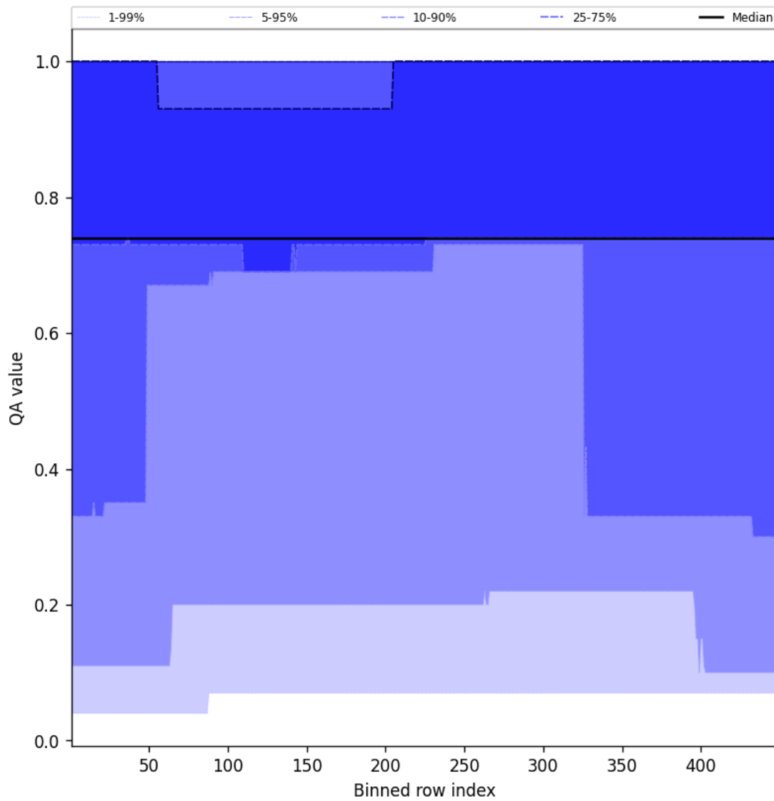
Figure 45: Along track statistics of “QA value” for 2025-10-20 to 2025-10-22
