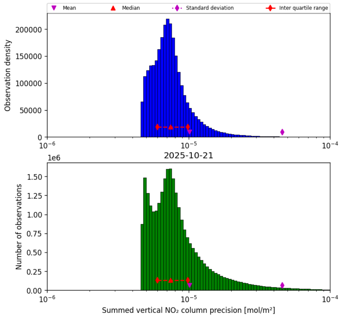
Figure 41: Histogram of “Summed vertical NO 2 column precision” for 2025-10-20 to 2025-10-22
