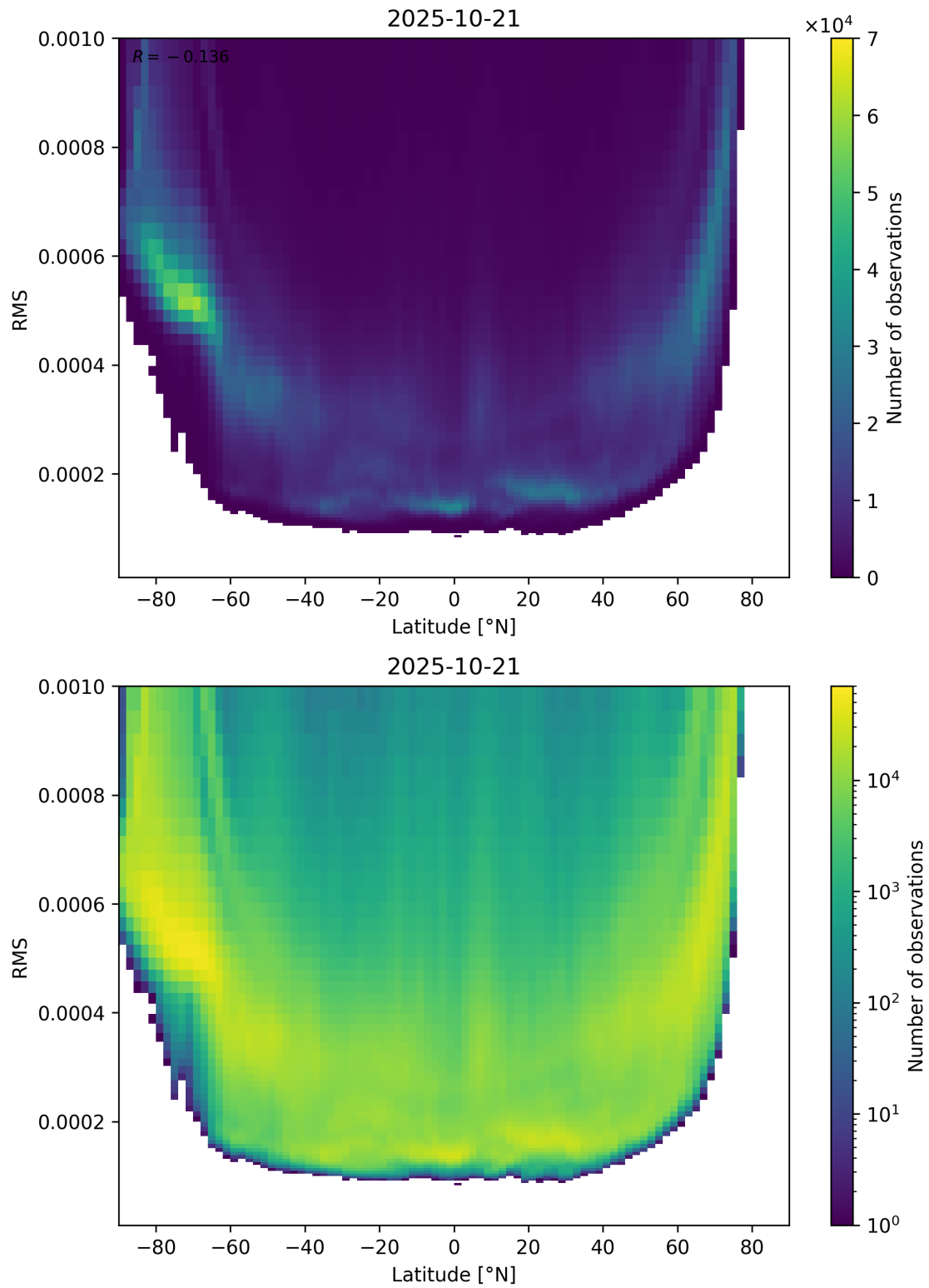
Figure 94: Scatter density plot of “Latitude” against “RMS” for 2025-10-20 to 2025-10-22.
