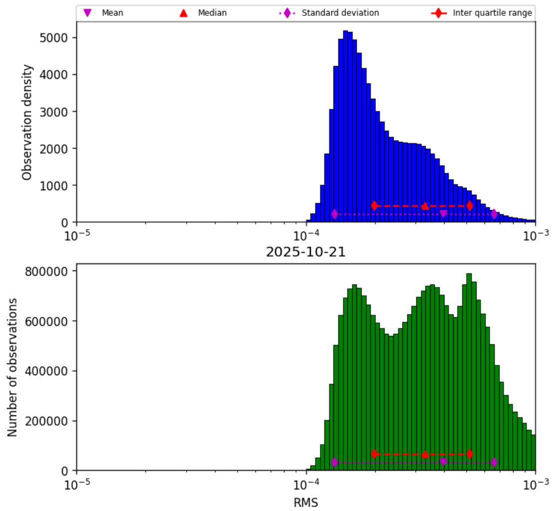
Figure 43: Histogram of “RMS” for 2025-10-20 to 2025-10-22
