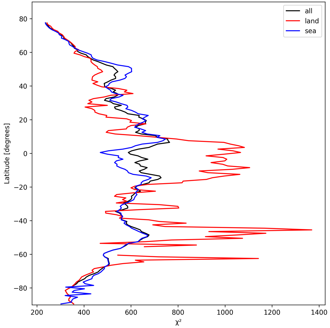
Figure 25: Zonal average of “ \chi^2 ” for 2025-10-20 to 2025-10-22.
