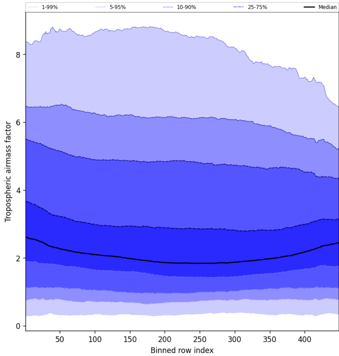
Figure 48: Along track statistics of “Tropospheric air mass factor” for 2025-10-20 to 2025-10-22
