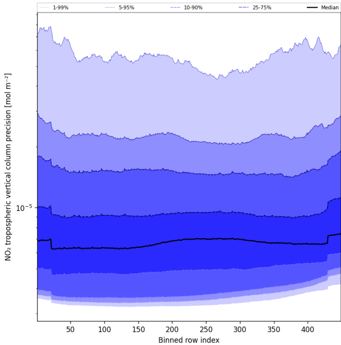
Figure 47: Along track statistics of “NO 2 tropospheric vertical column precision” for 2025-10-20 to 2025-10-22
