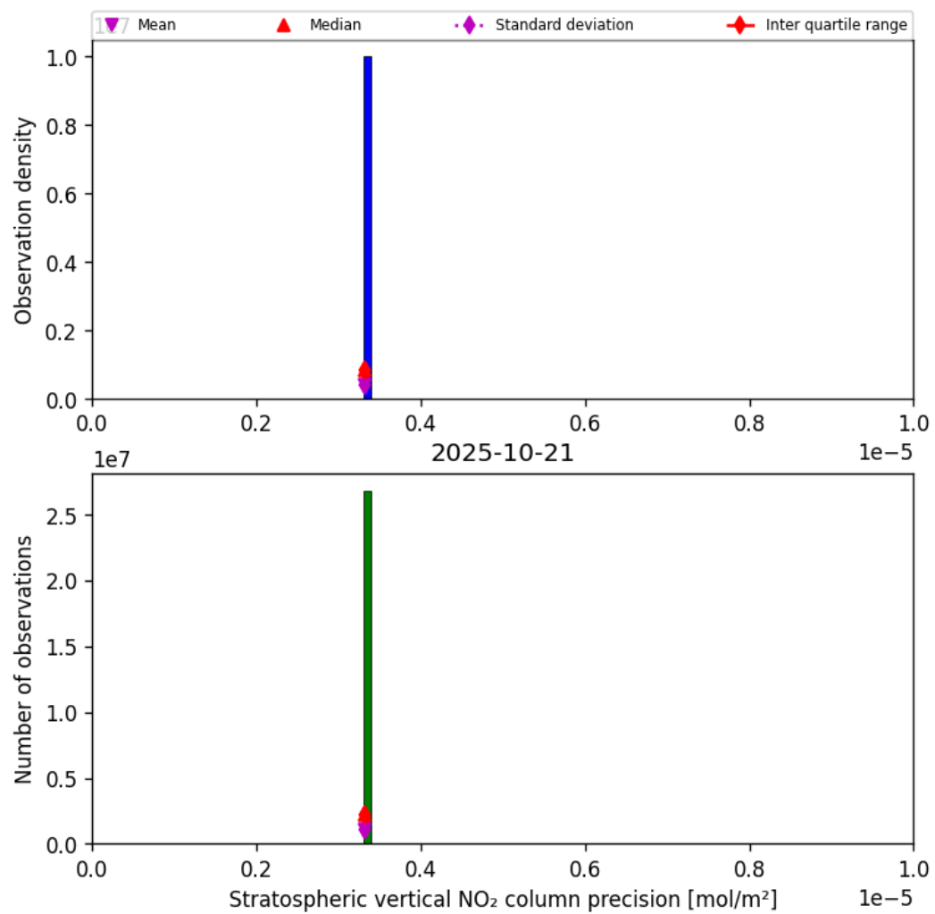
Figure 37: Histogram of “Stratospheric vertical NO 2 column precision” for 2025-10-20 to 2025-10-22
