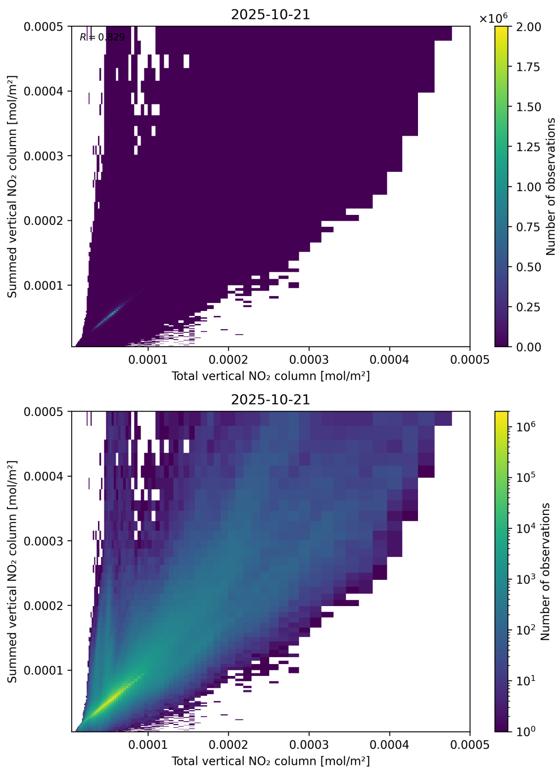
Figure 112: Scatter density plot of “Total vertical NO 2 column” against “Summed vertical NO 2 column” for 2025-10-20 to 2025-10-22.
