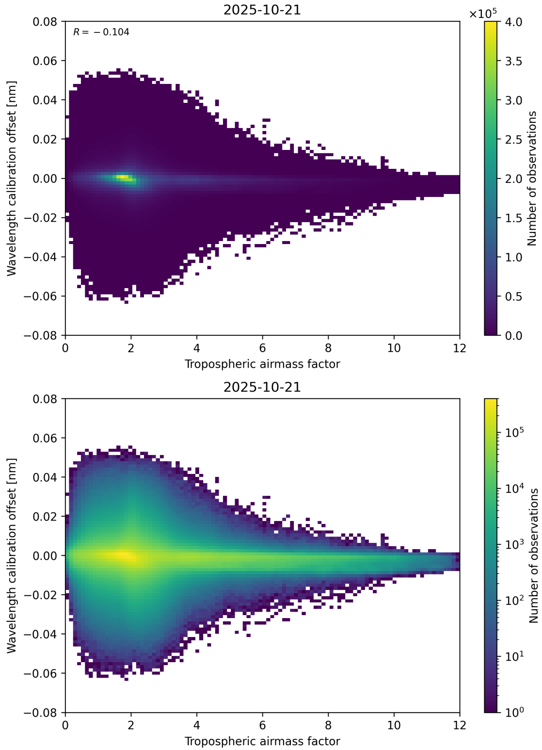
Figure 80: Scatter density plot of “Tropospheric airmass factor” against “Wavelength calibration offset” for 2025-10-20 to 2025-10-22.
