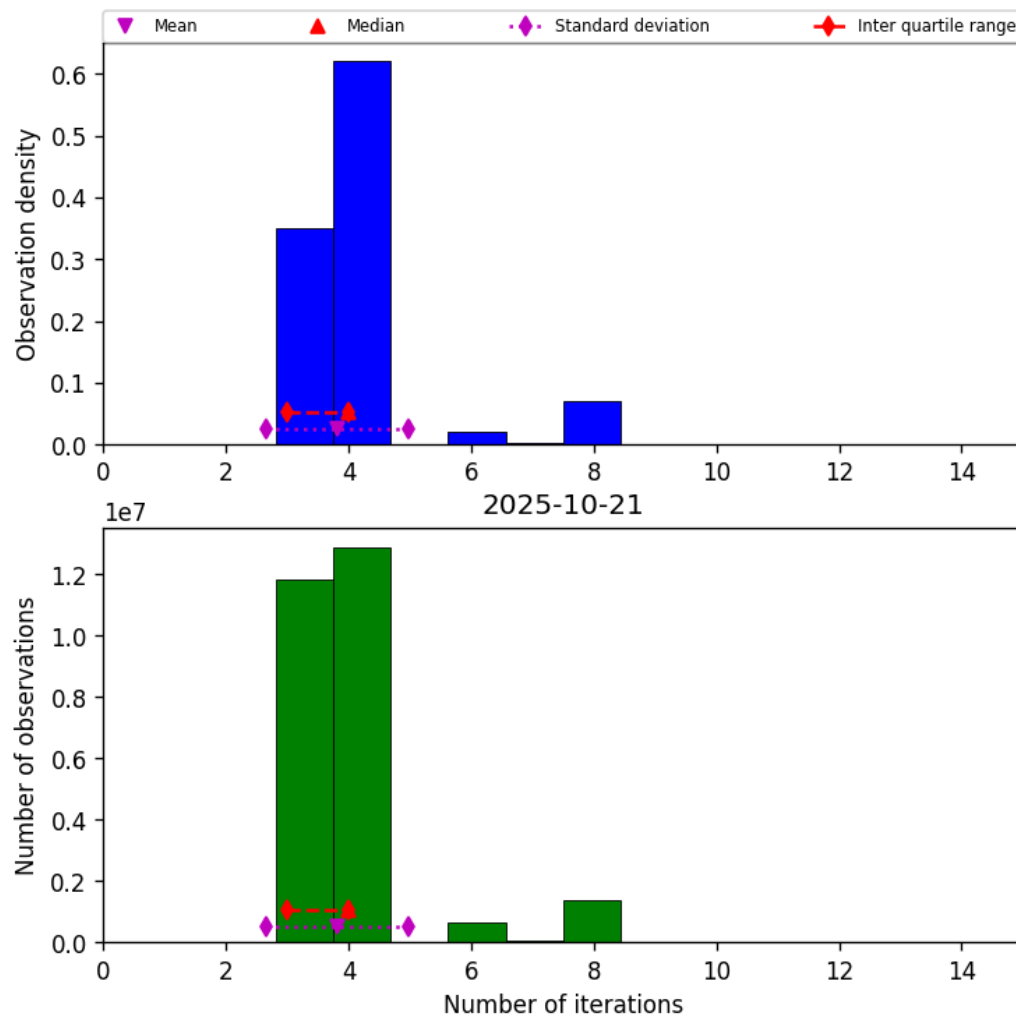
Figure 34: Histogram of “Number of iterations” for 2025-10-20 to 2025-10-22
