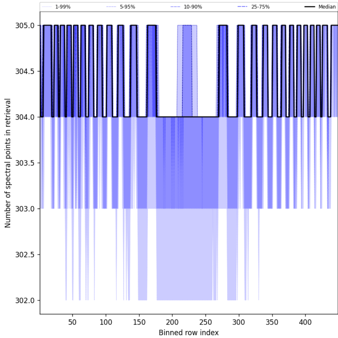
Figure 50: Along track statistics of “Number of spectral points in retrieval” for 2025-10-20 to 2025-10-22
