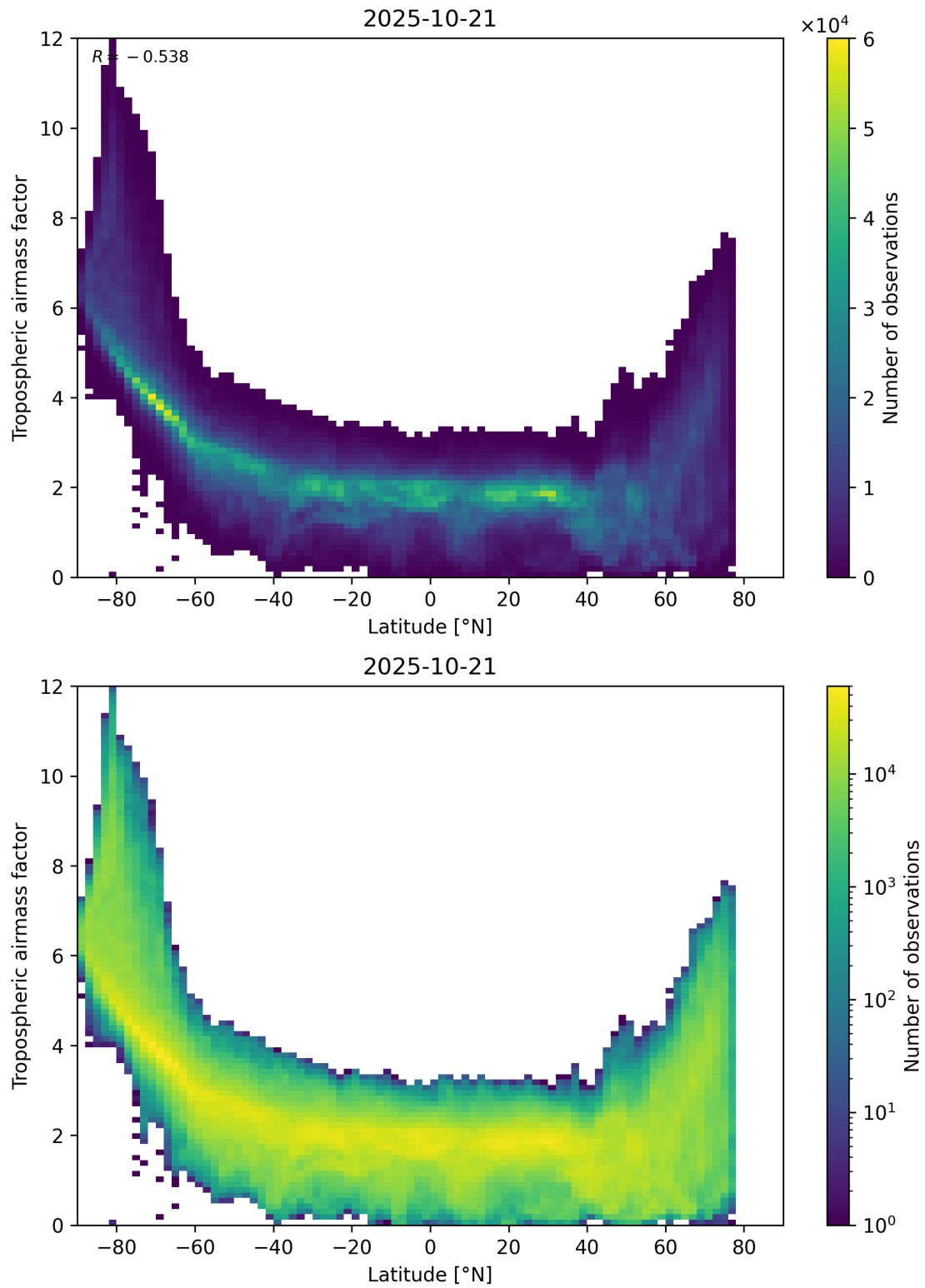
Figure 85: Scatter density plot of “Latitude” against “Tropospheric airmass factor” for 2025-10-20 to 2025-10-22.
