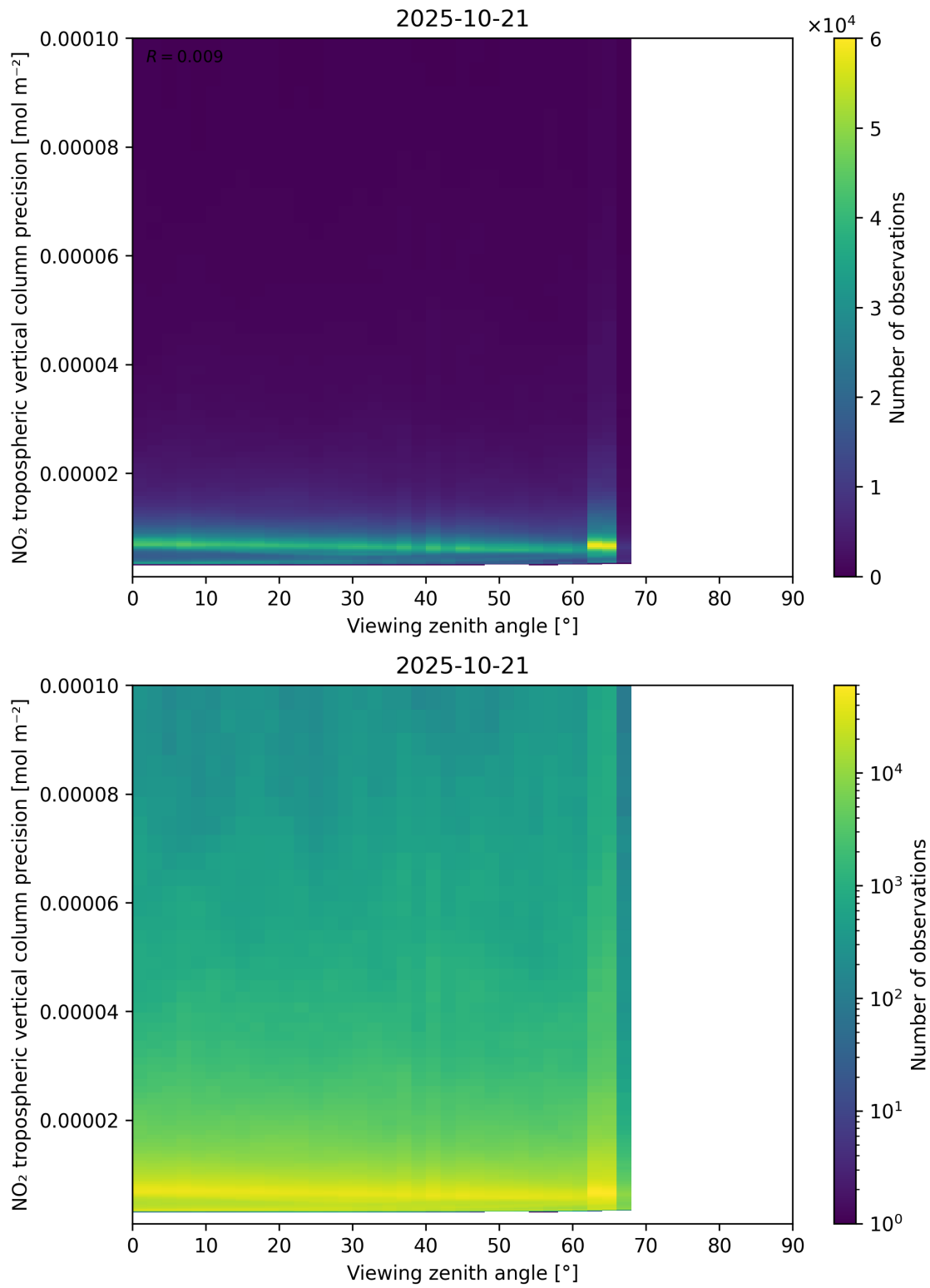
Figure 170: Scatter density plot of “Viewing zenith angle” against “NO 2 tropospheric vertical column precision” for 2025-10-20 to 2025-10-22.
