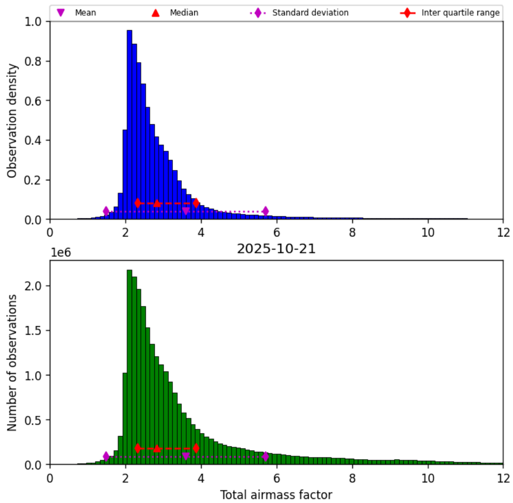
Figure 32: Histogram of “Total airmass factor” for 2025-10-20 to 2025-10-22
