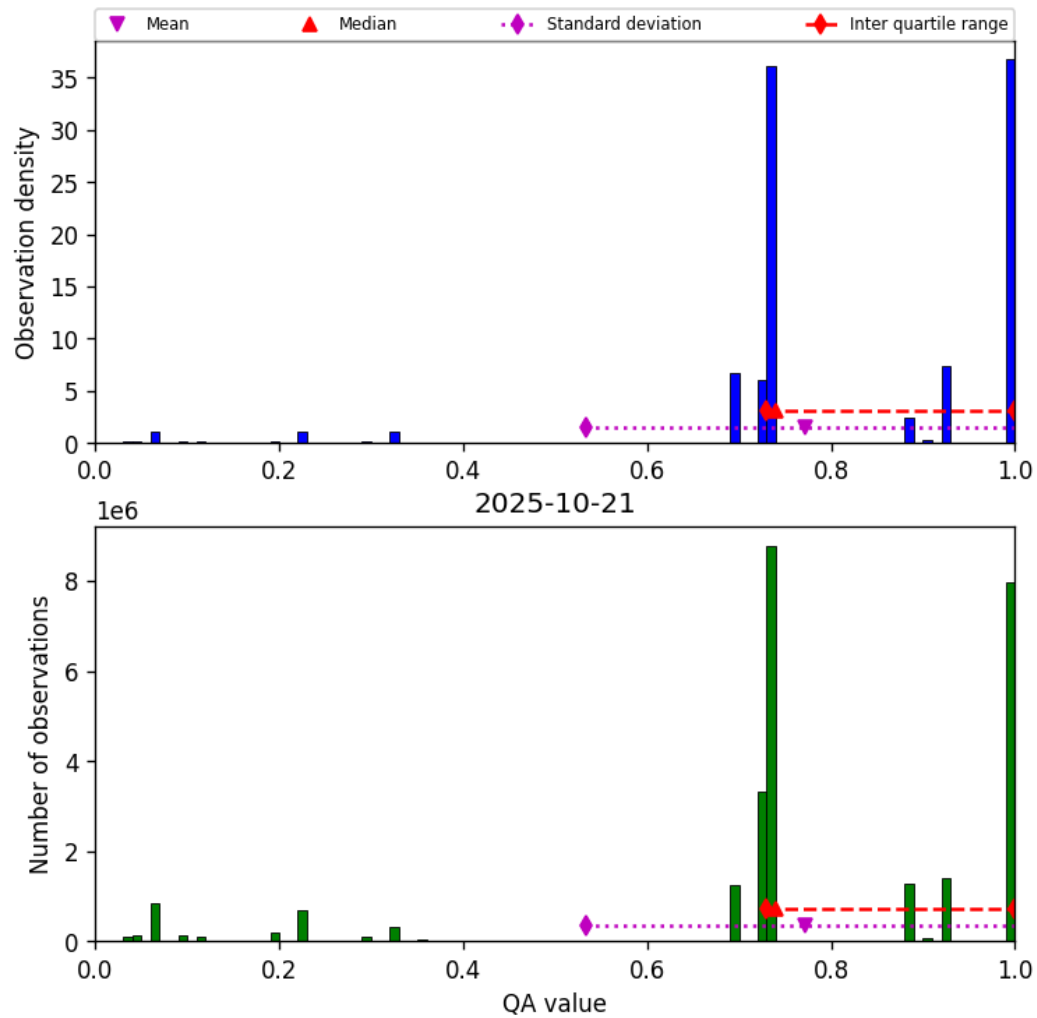
Figure 28: Histogram of “QA value” for 2025-10-20 to 2025-10-22
