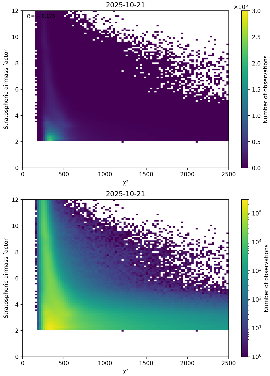
Figure 81: Scatter density plot of “ \chi^2 ” against “Stratospheric airmass factor” for 2025-10-20 to 2025-10-22.
