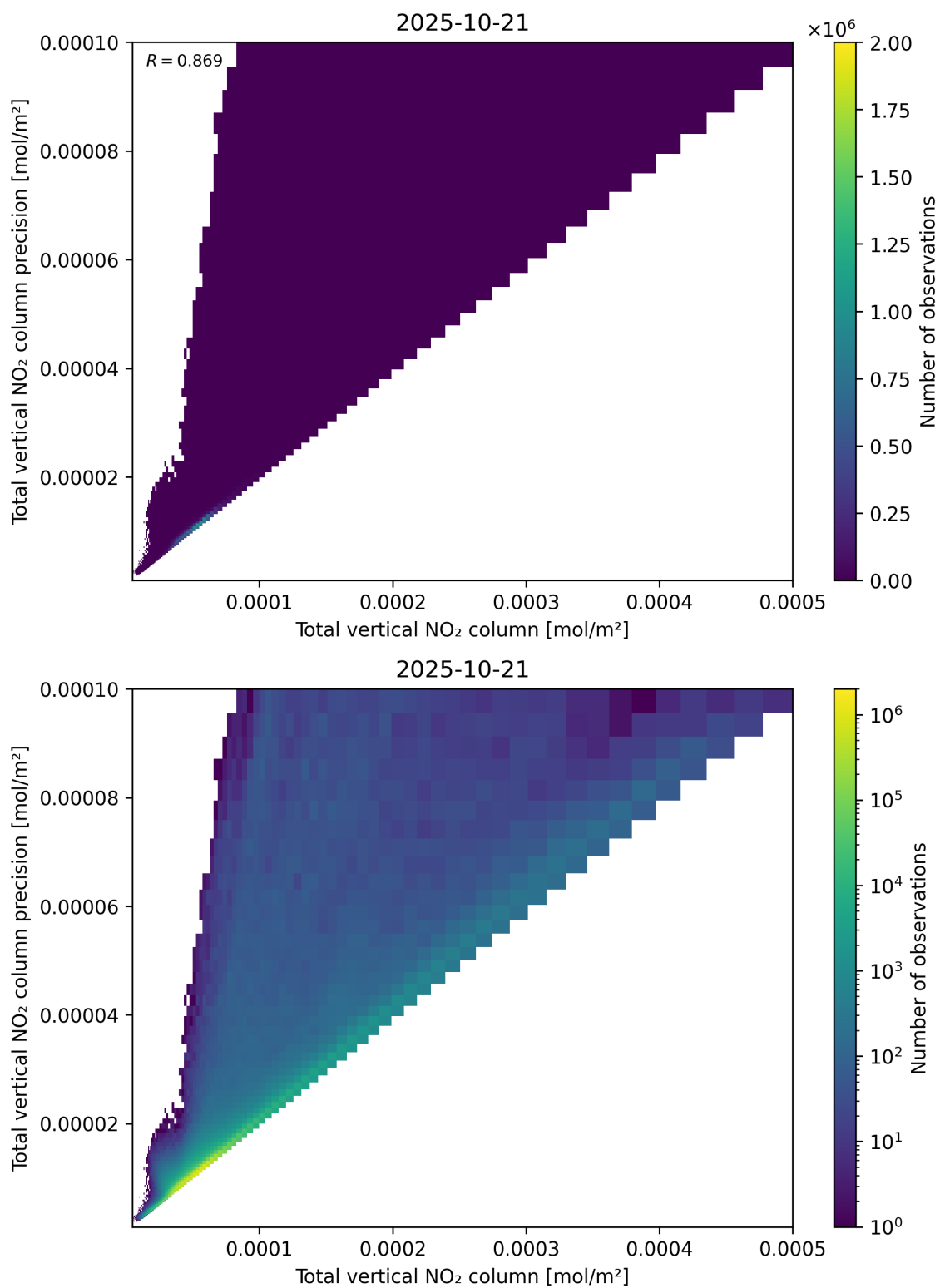
Figure 114: Scatter density plot of “Total vertical NO 2 column” against “Total vertical NO 2 column precision” for 2025-10-20 to 2025-10-22.
