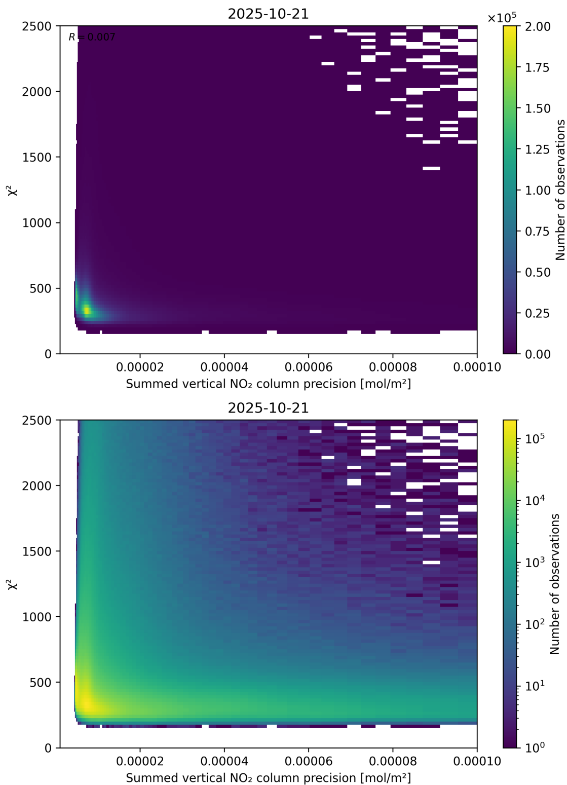
Figure 107: Scatter density plot of “Summed vertical NO 2 column precision” against “ \chi^2 ” for 2025-10-20 to 2025-10-22.
