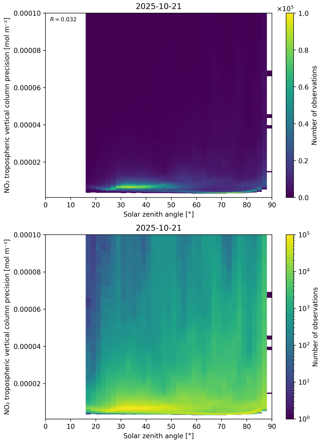
Figure 156: Scatter density plot of “Solar zenith angle” against “NO 2 tropospheric vertical column precision” for 2025-10-20 to 2025-10-22.
