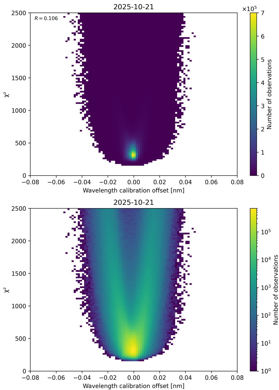
Figure 175: Scatter density plot of “Wavelength calibration offset” against “ \chi^2 ” for 2025-10-20 to 2025-10-22.
