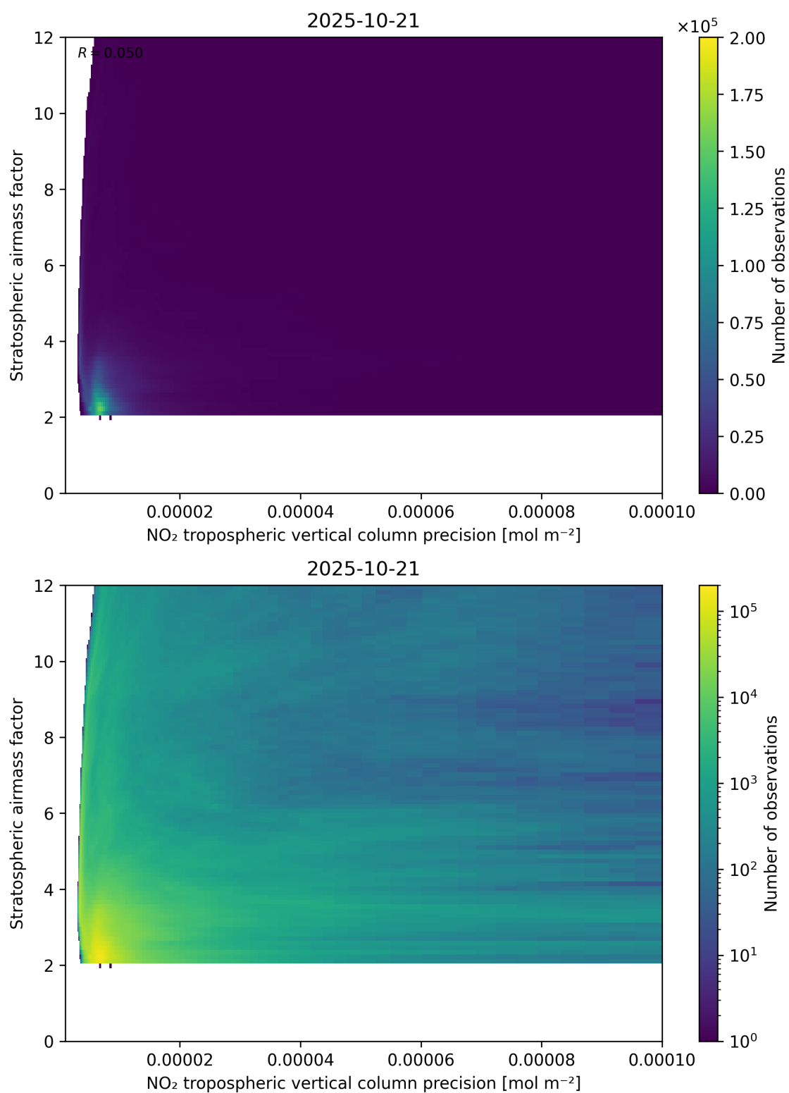
Figure 131: Scatter density plot of “NO 2 tropospheric vertical column precision” against “Stratospheric airmass factor” for 2025-10-20 to 2025-10-22.
