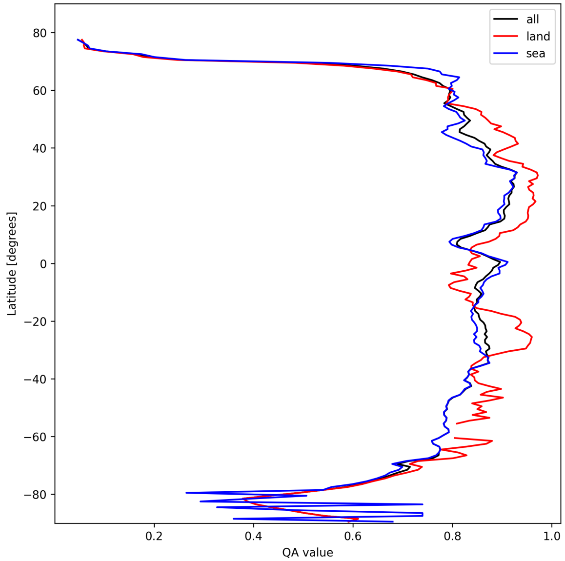
Figure 11: Zonal average of “QA value” for 2025-10-20 to 2025-10-22.
