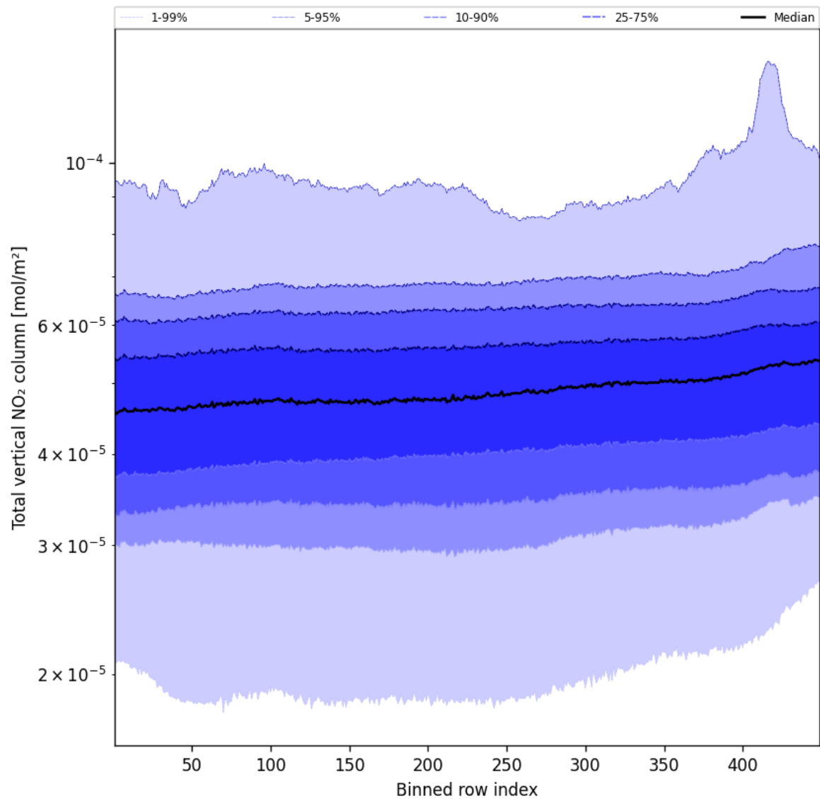
Figure 55: Along track statistics of “Total vertical NO 2 column” for 2025-10-20 to 2025-10-22
