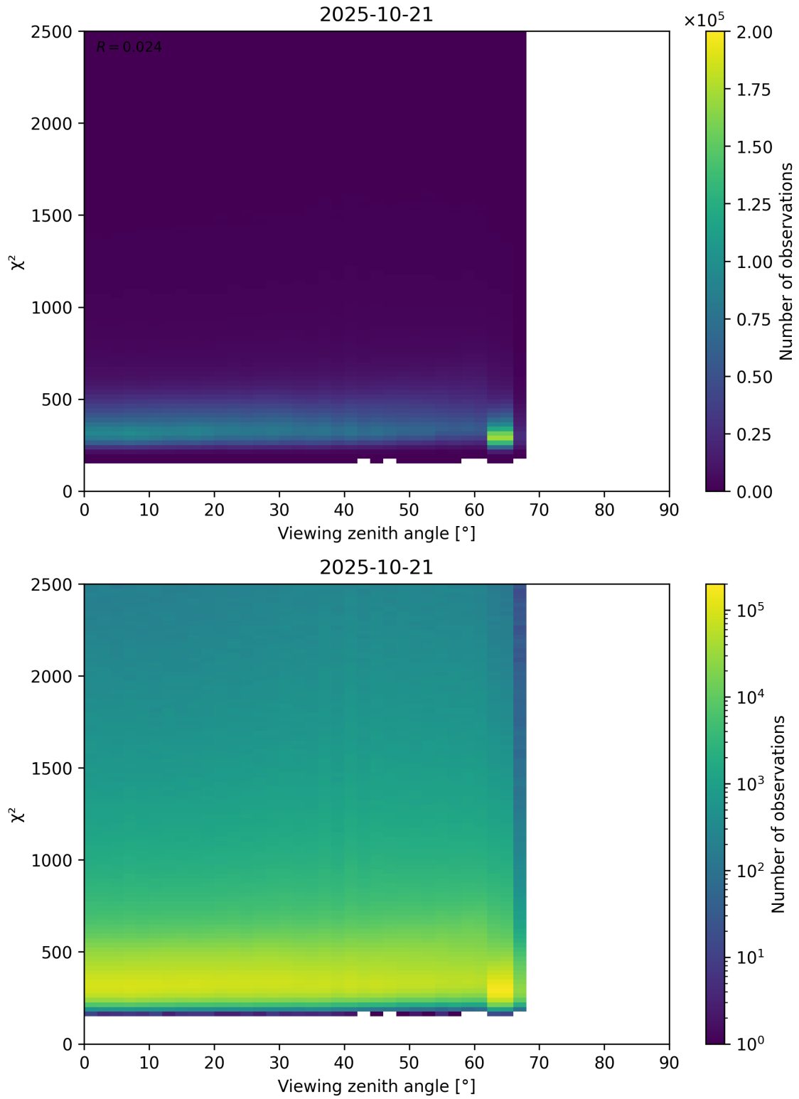
Figure 162: Scatter density plot of “Viewing zenith angle” against “ \chi^2 ” for 2025-10-20 to 2025-10-22.
