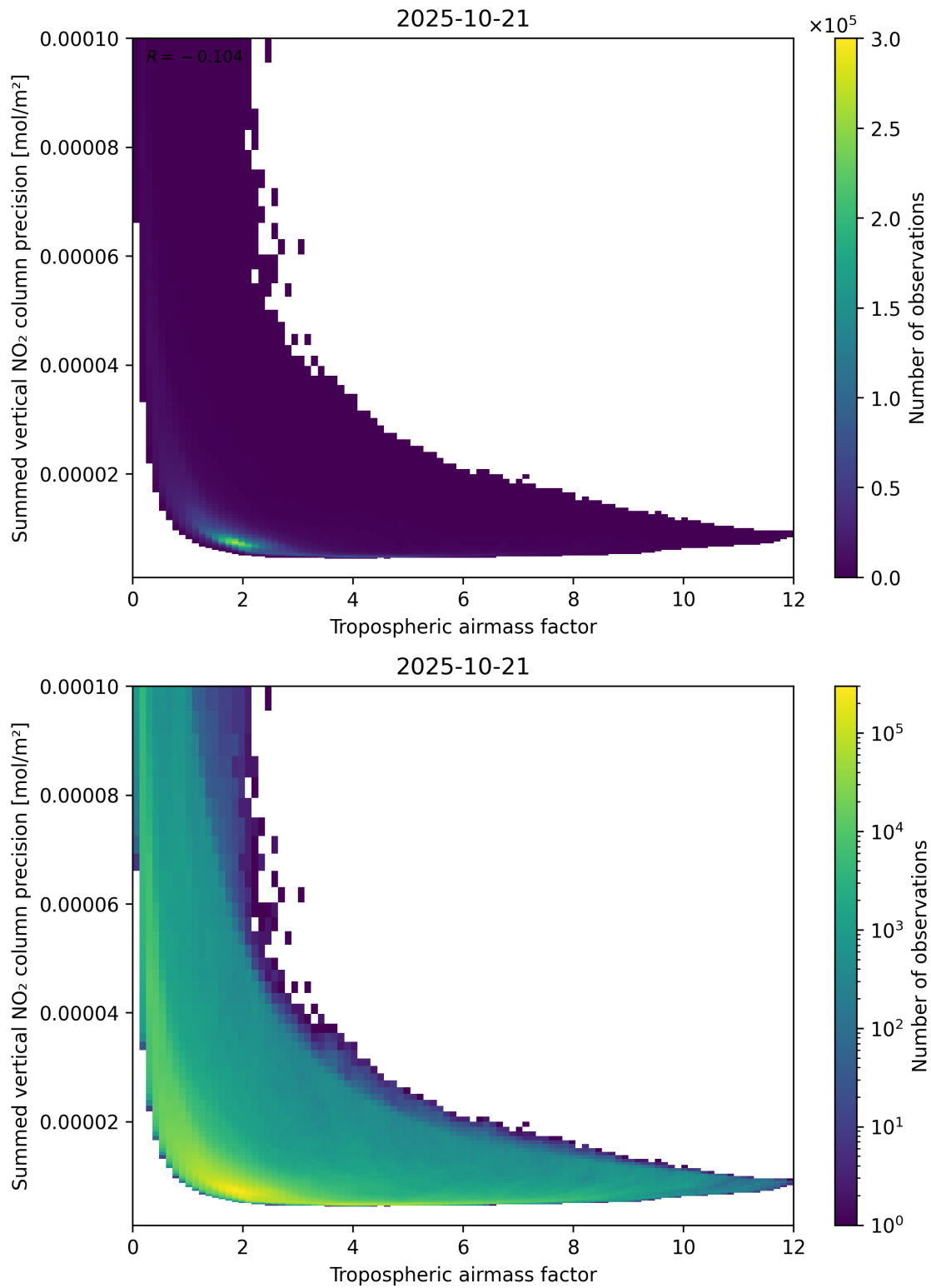
Figure 76: Scatter density plot of “Tropospheric air mass factor” against “Summed vertical NO 2 column precision” for 2025-10-20 to 2025-10-22.
