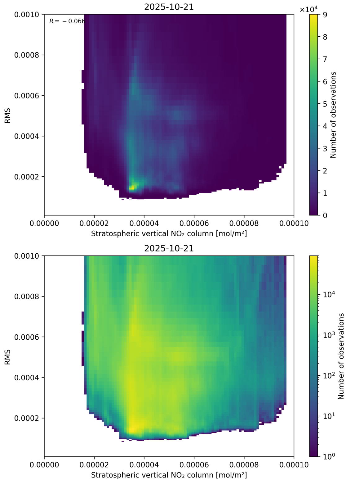
Figure 102: Scatter density plot of “Stratospheric vertical NO 2 column” against “RMS” for 2025-10-20 to 2025-10-22.
