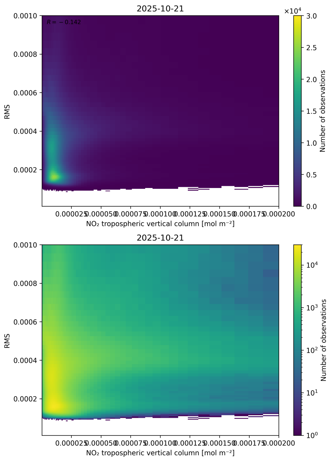
Figure 142: Scatter density plot of “NO 2 tropospheric vertical column” against “RMS” for 2025-10-20 to 2025-10-22.
