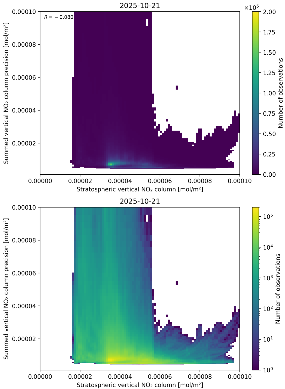
Figure 99: Scatter density plot of “Stratospheric vertical NO 2 column” against “Summed vertical NO 2 column precision” for 2025-10-20 to 2025-10-22.
