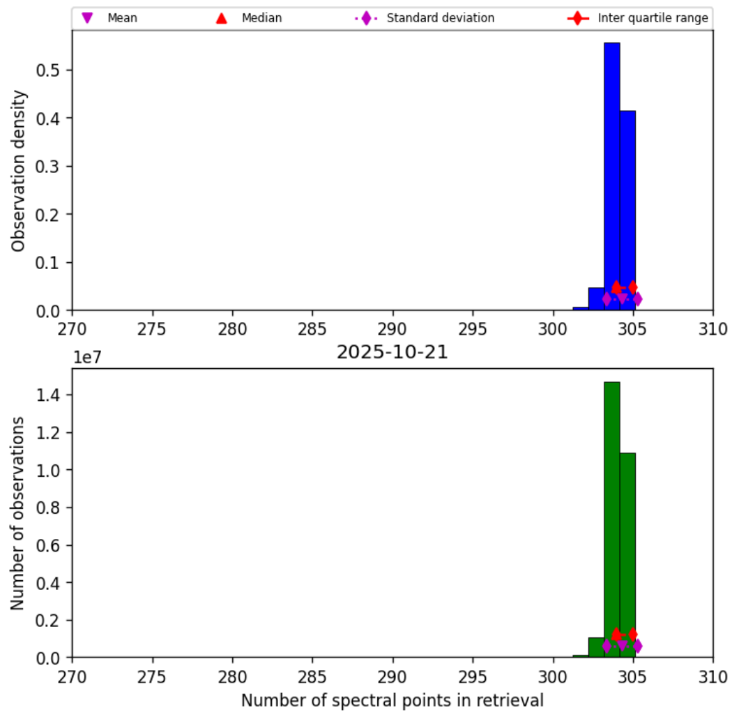
Figure 33: Histogram of “Number of spectral points in retrieval” for 2025-10-20 to 2025-10-22
