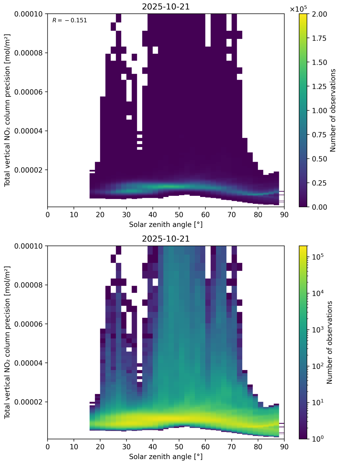
Figure 154: Scatter density plot of “Solar zenith angle” against “Total vertical NO 2 column precision” for 2025-10-20 to 2025-10-22.
