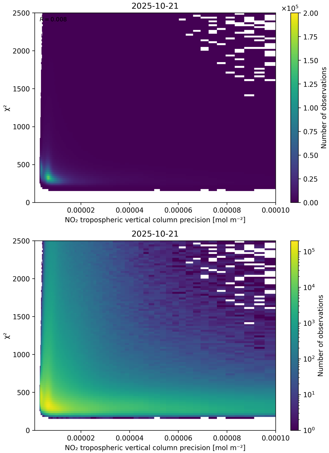
Figure 134: Scatter density plot of “NO 2 tropospheric vertical column precision” against “ \chi^2 ” for 2025-10-20 to 2025-10-22.
