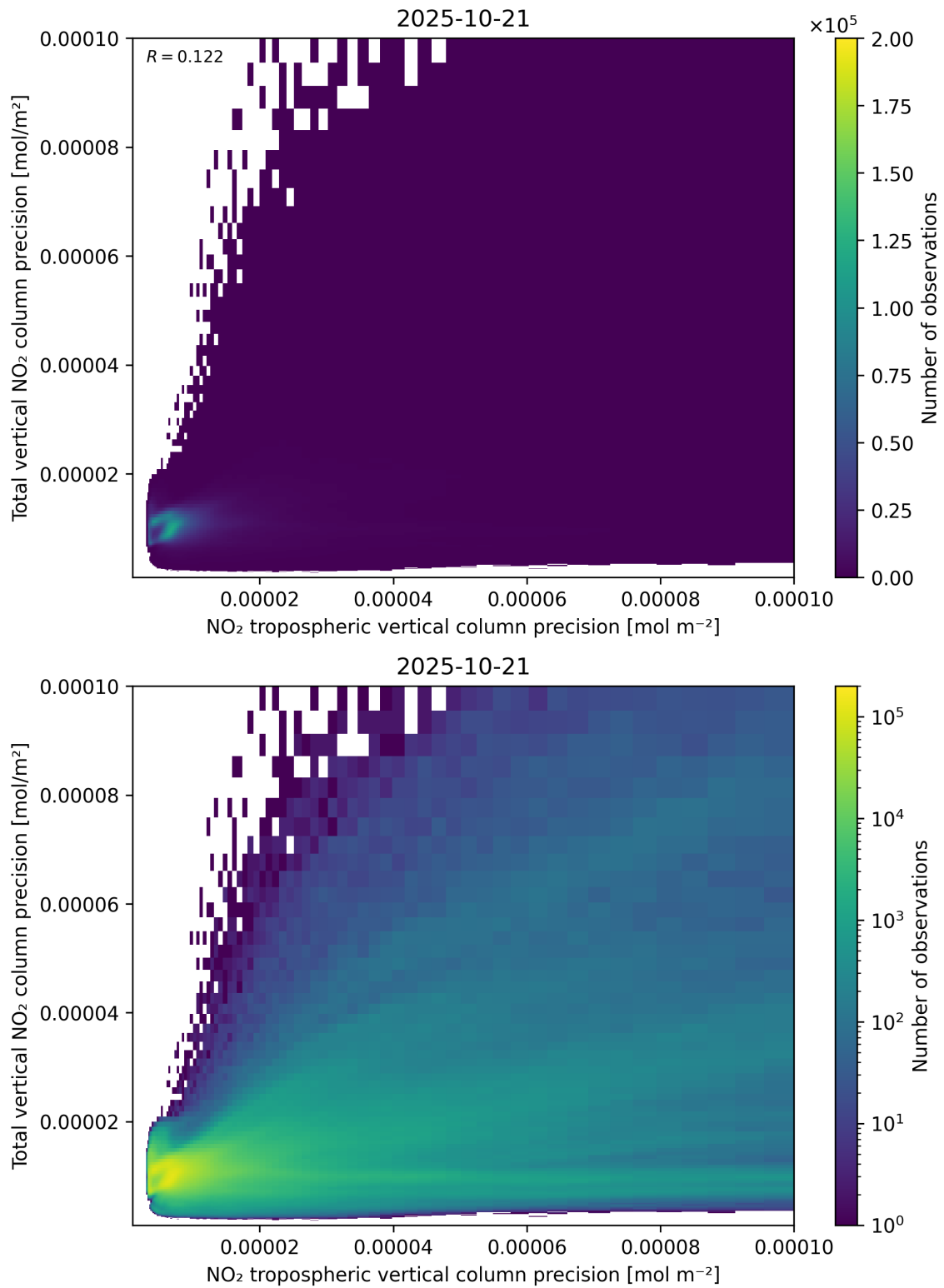
Figure 139: Scatter density plot of “NO 2 tropospheric vertical column precision” against “Total vertical NO 2 column precision” for 2025-10-20 to 2025-10-22.
