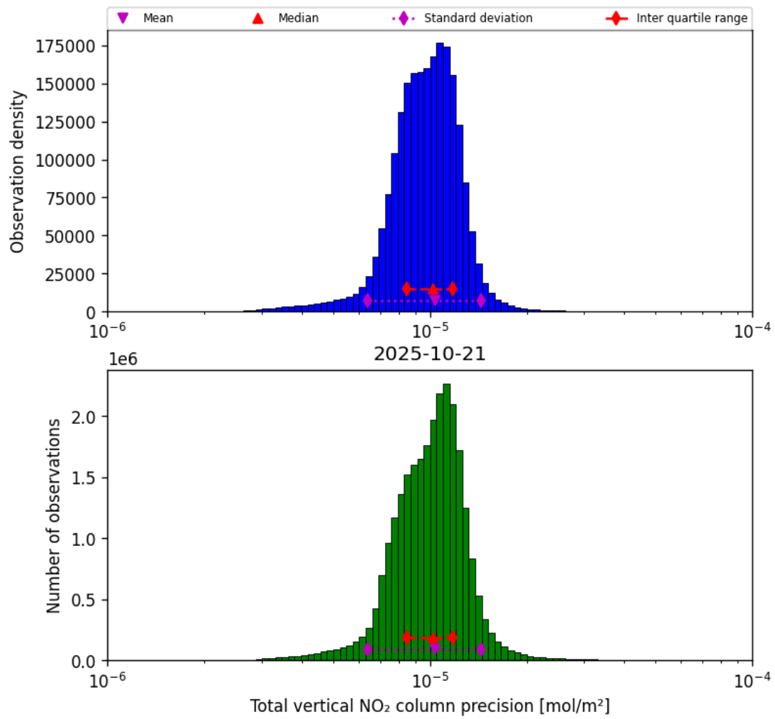
Figure 39: Histogram of “Total vertical NO 2 column precision” for 2025-10-20 to 2025-10-22
