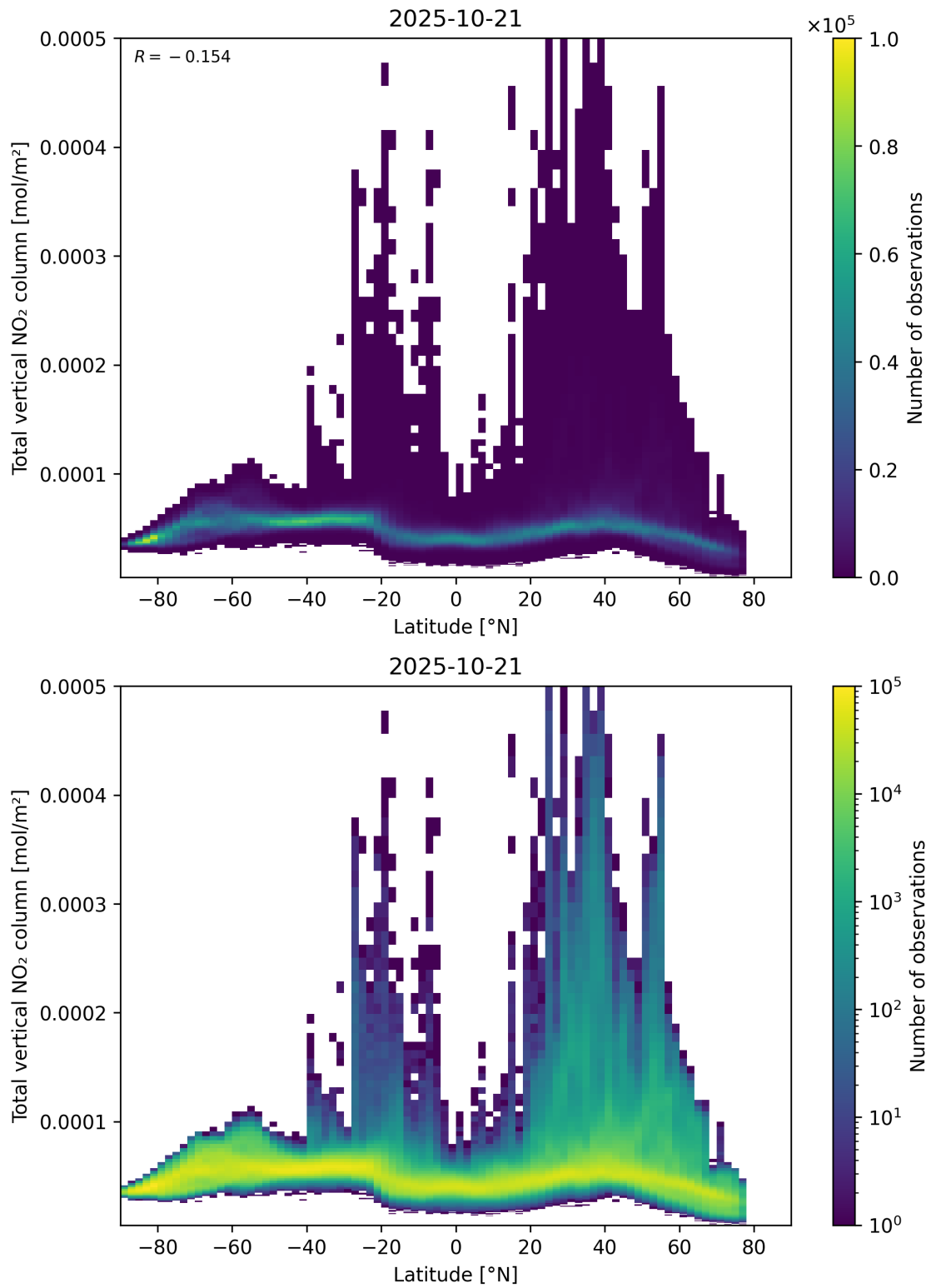
Figure 90: Scatter density plot of “Latitude” against “Total vertical NO 2 column” for 2025-10-20 to 2025-10-22.
