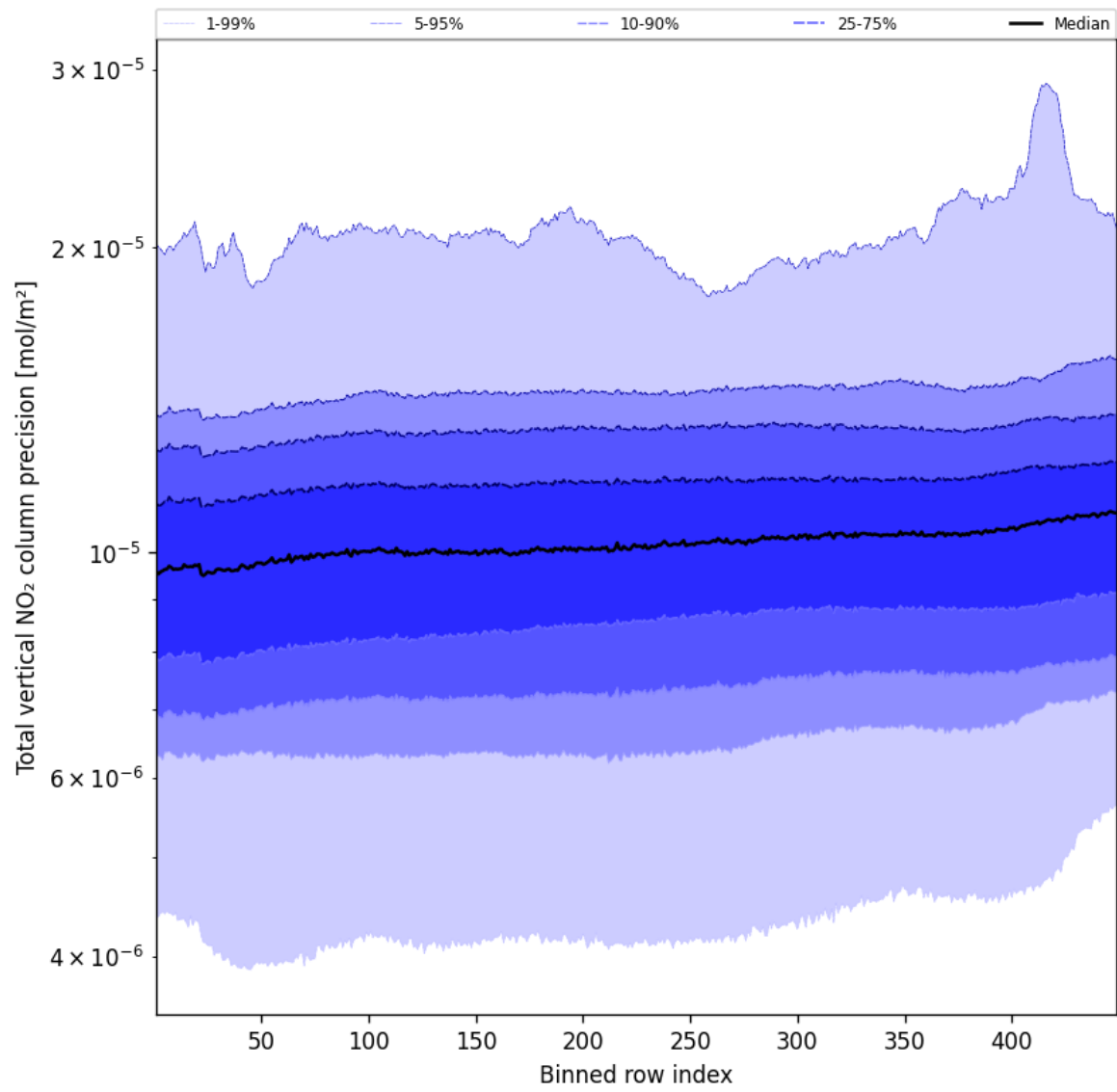
Figure 56: Along track statistics of “Total vertical NO 2 column precision” for 2025-10-20 to 2025-10-22
