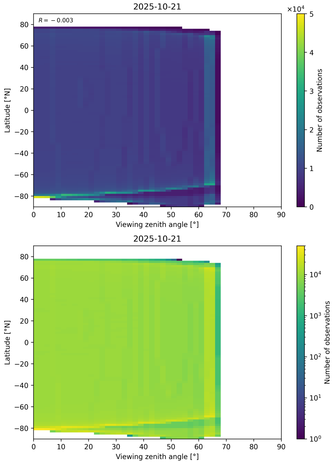
Figure 163: Scatter density plot of “Viewing zenith angle” against “Latitude” for 2025-10-20 to 2025-10-22.
