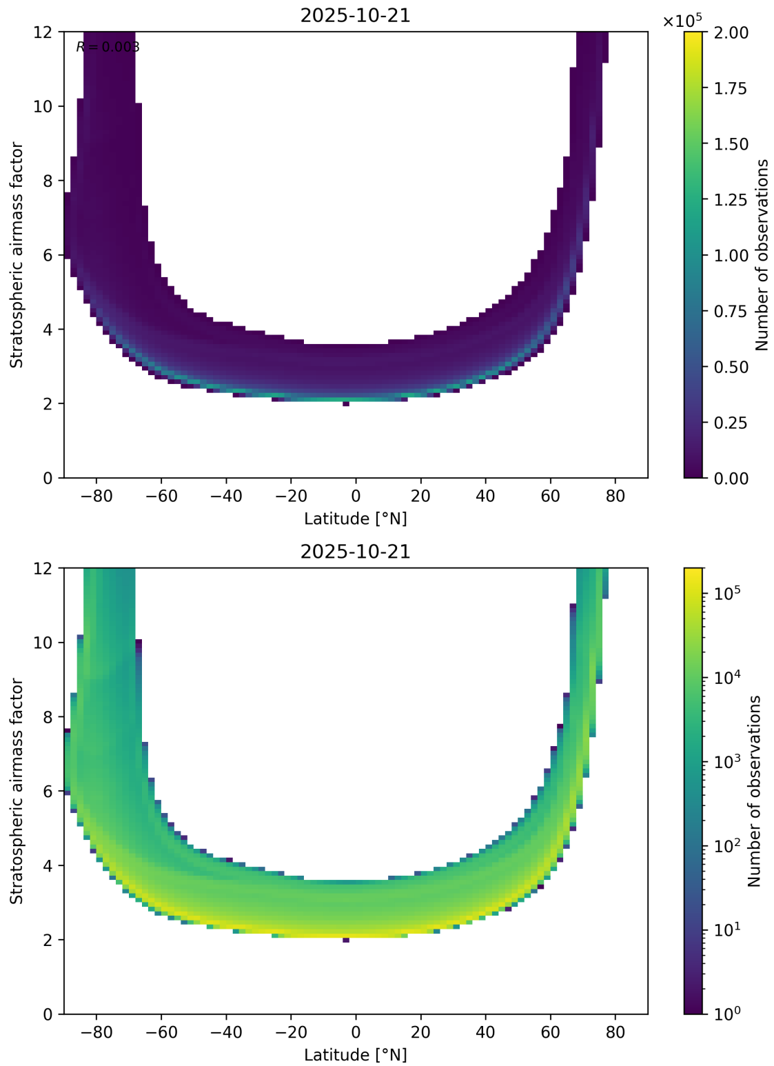
Figure 83: Scatter density plot of “Latitude” against “Stratospheric airmass factor” for 2025-10-20 to 2025-10-22.
