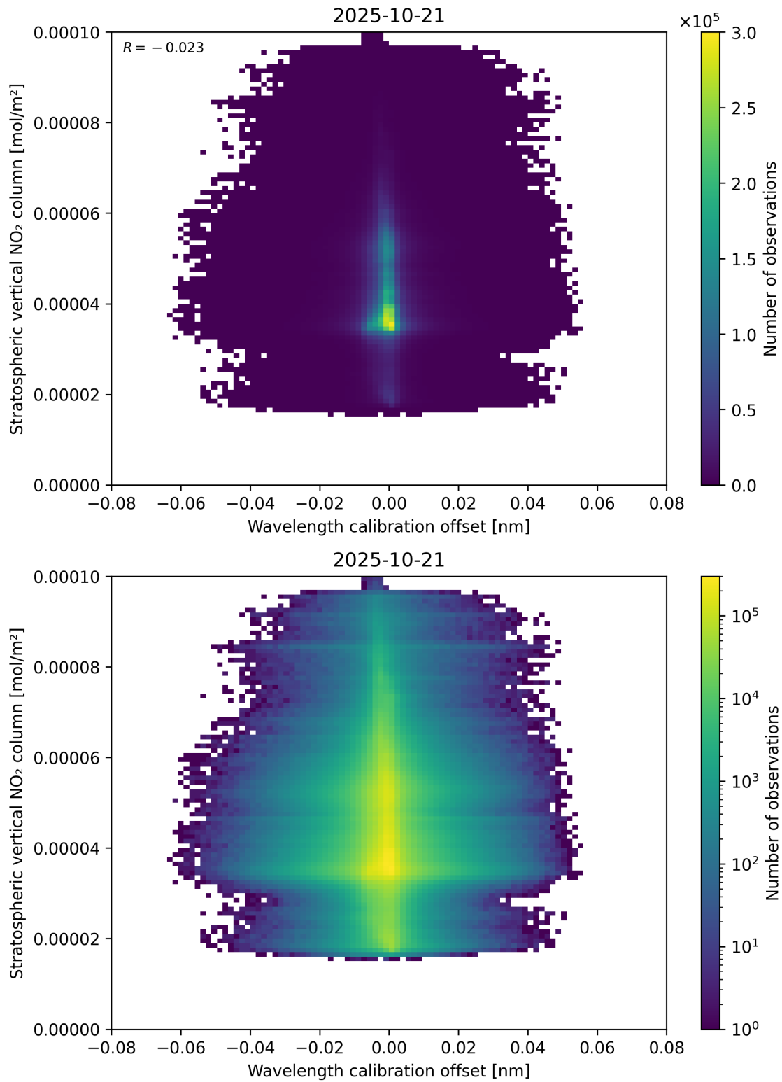
Figure 176: Scatter density plot of “Wavelength calibration offset” against “Stratospheric vertical NO 2 column” for 2025-10-20 to 2025-10-22.
