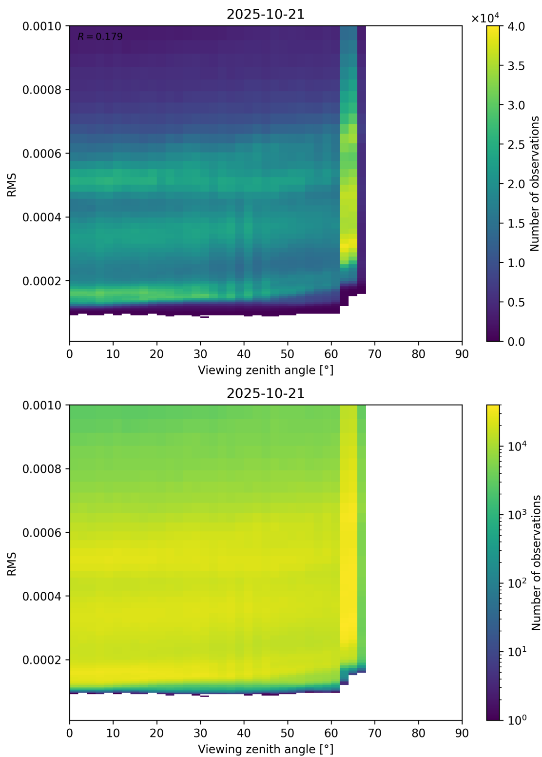
Figure 171: Scatter density plot of “Viewing zenith angle” against “RMS” for 2025-10-20 to 2025-10-22.
