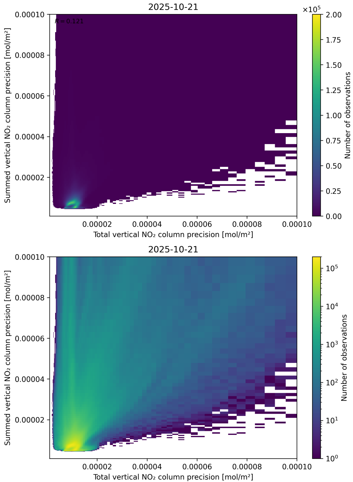
Figure 118: Scatter density plot of “Total vertical NO 2 column precision” against “Summed vertical NO 2 column precision” for 2025-10-20 to 2025-10-22.
