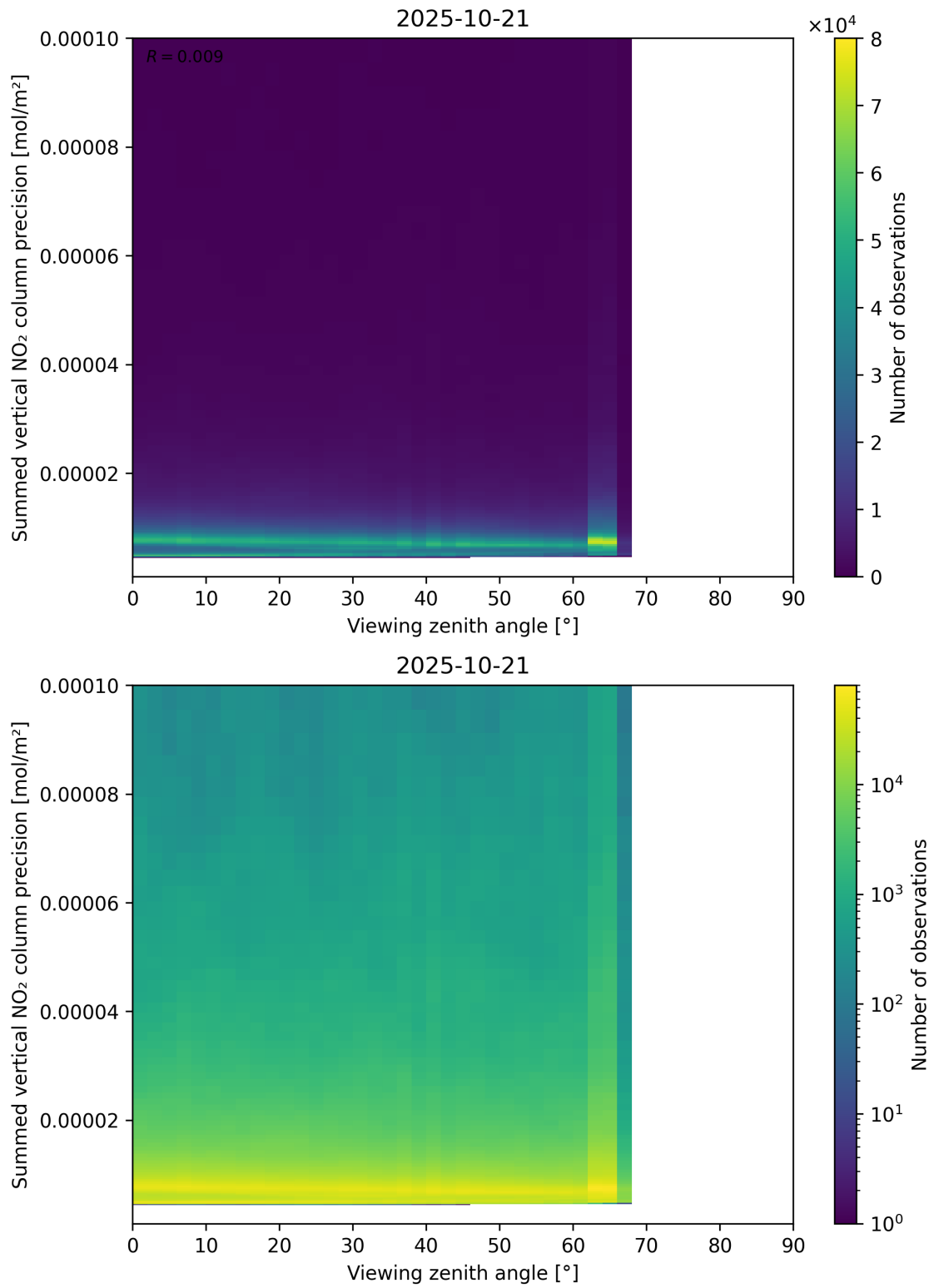
Figure 166: Scatter density plot of “Viewing zenith angle” against “Summed vertical NO 2 column precision” for 2025-10-20 to 2025-10-22.
