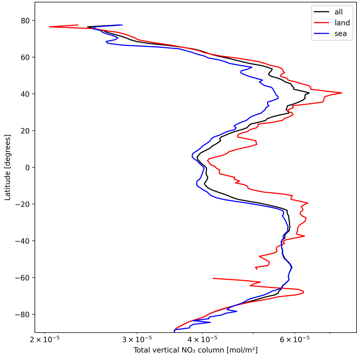
Figure 21: Zonal average of “Total vertical NO 2 column” for 2025-10-20 to 2025-10-22.
