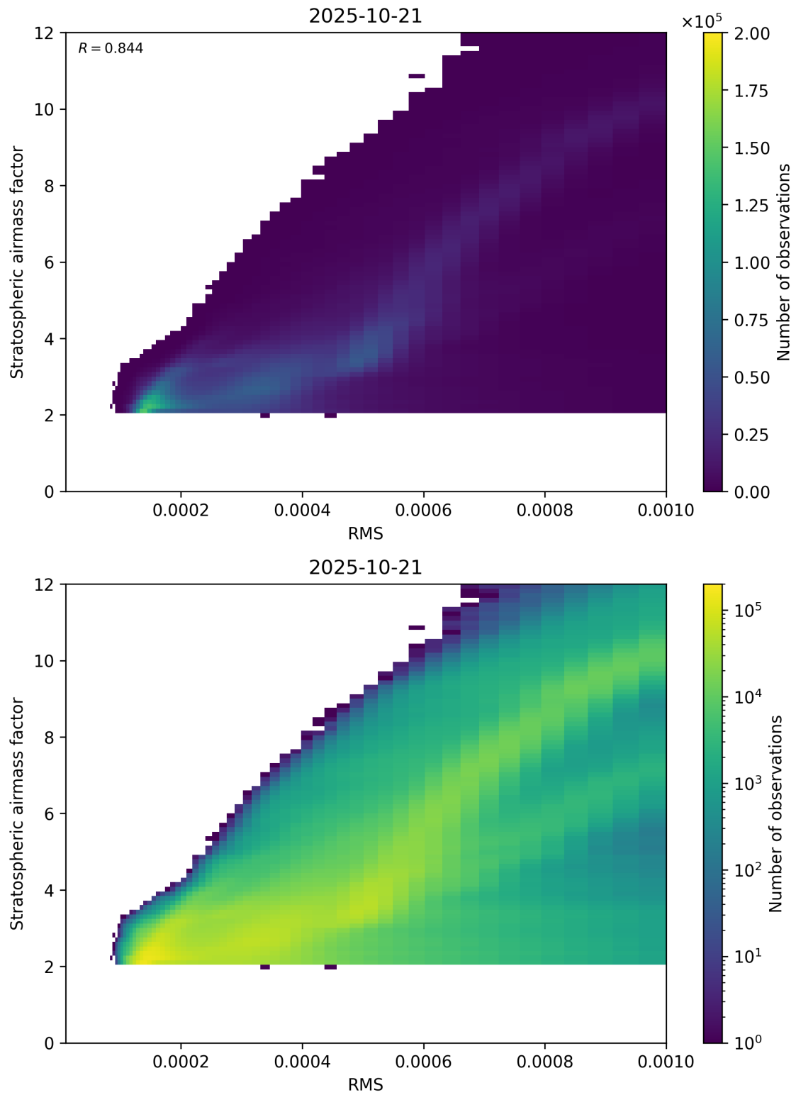
Figure 144: Scatter density plot of “RMS” against “Stratospheric airmass factor” for 2025-10-20 to 2025-10-22.
