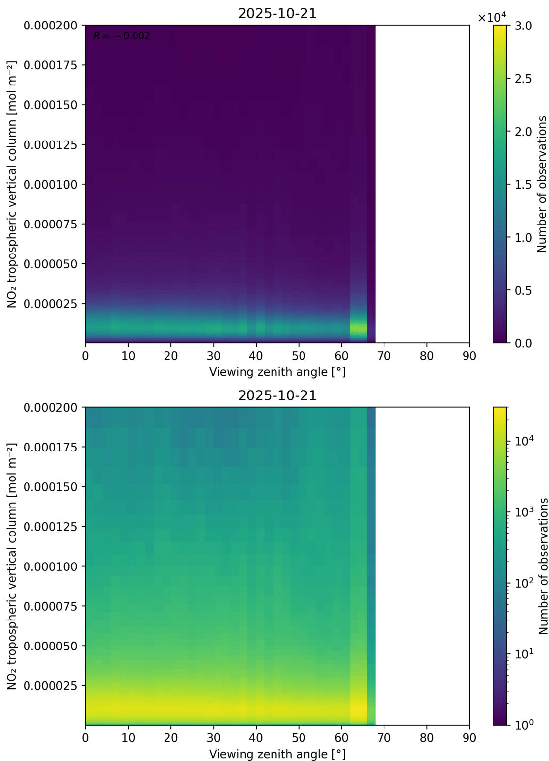
Figure 169: Scatter density plot of “Viewing zenith angle” against “NO 2 tropospheric vertical column” for 2025-10-20 to 2025-10-22.
