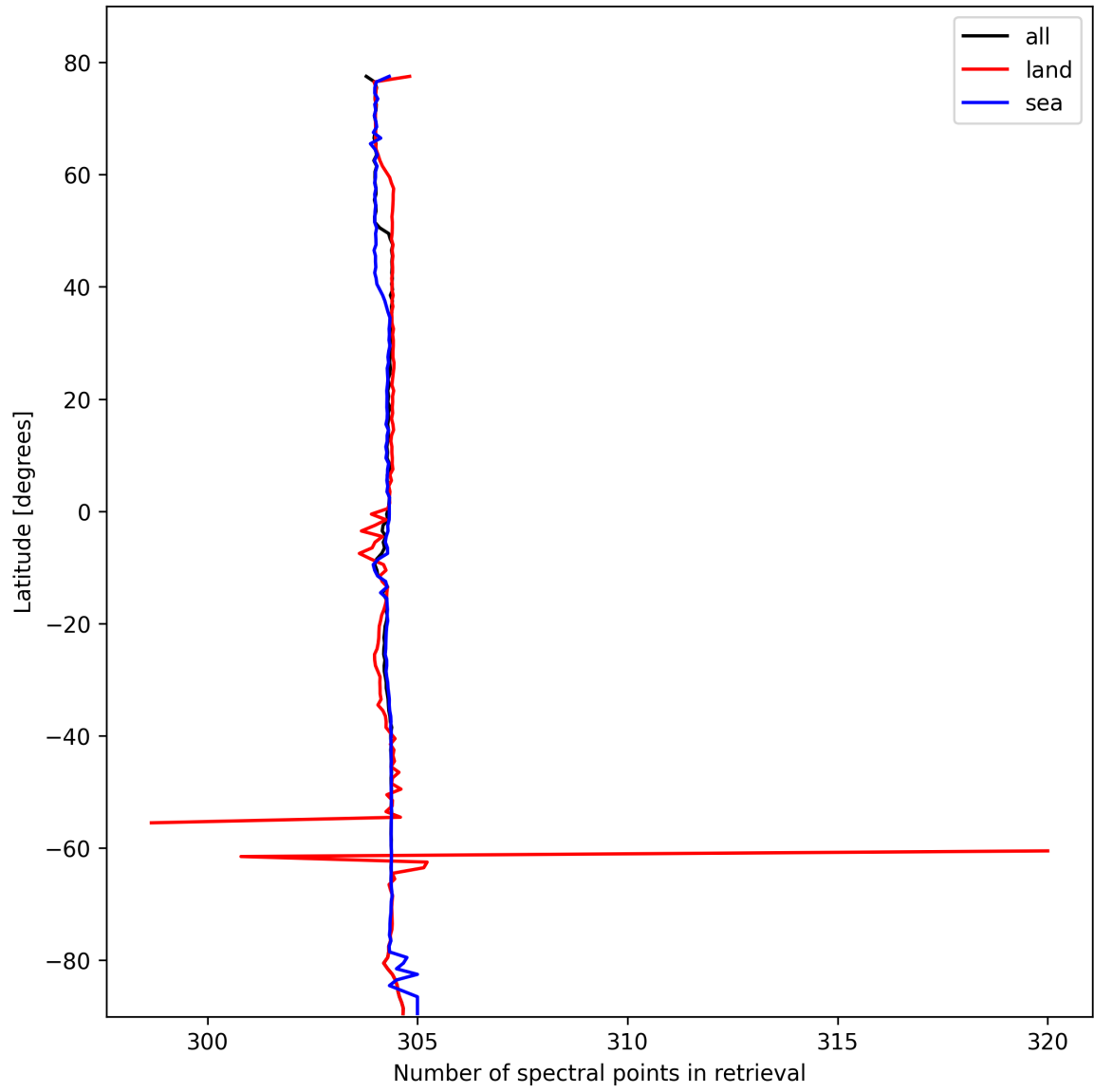
Figure 16: Zonal average of “Number of spectral points in retrieval” for 2025-10-20 to 2025-10-22.
