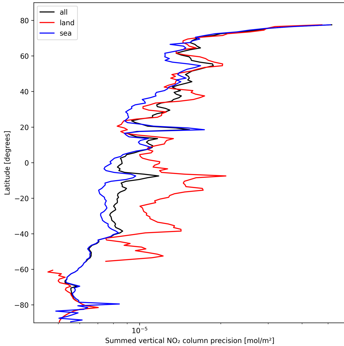
Figure 24: Zonal average of “Summed vertical NO 2 column precision” for 2025-10-20 to 2025-10-22.
