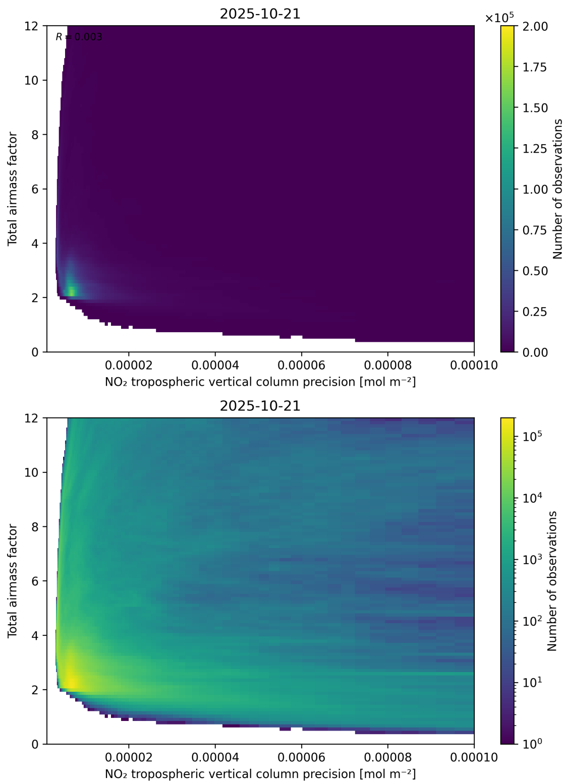
Figure 132: Scatter density plot of “NO 2 tropospheric vertical column precision” against “Total air mass factor” for 2025-10-20 to 2025-10-22.
