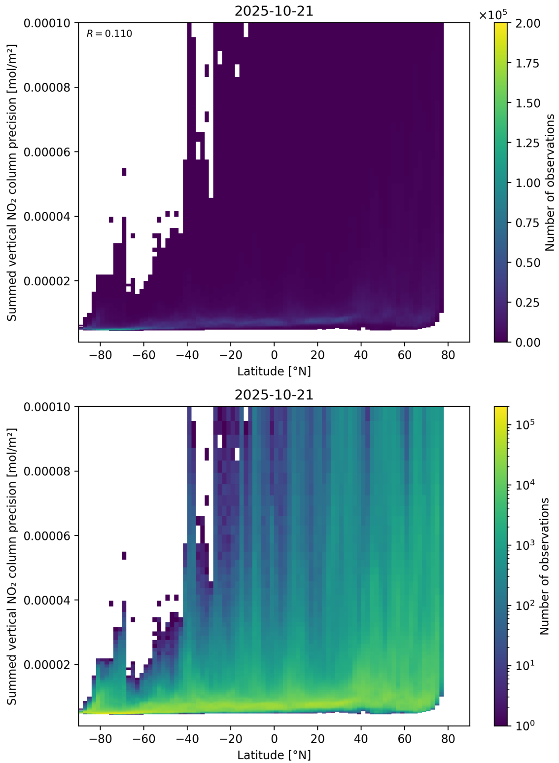
Figure 89: Scatter density plot of “Latitude” against “Summed vertical NO 2 column precision” for 2025-10-20 to 2025-10-22.
