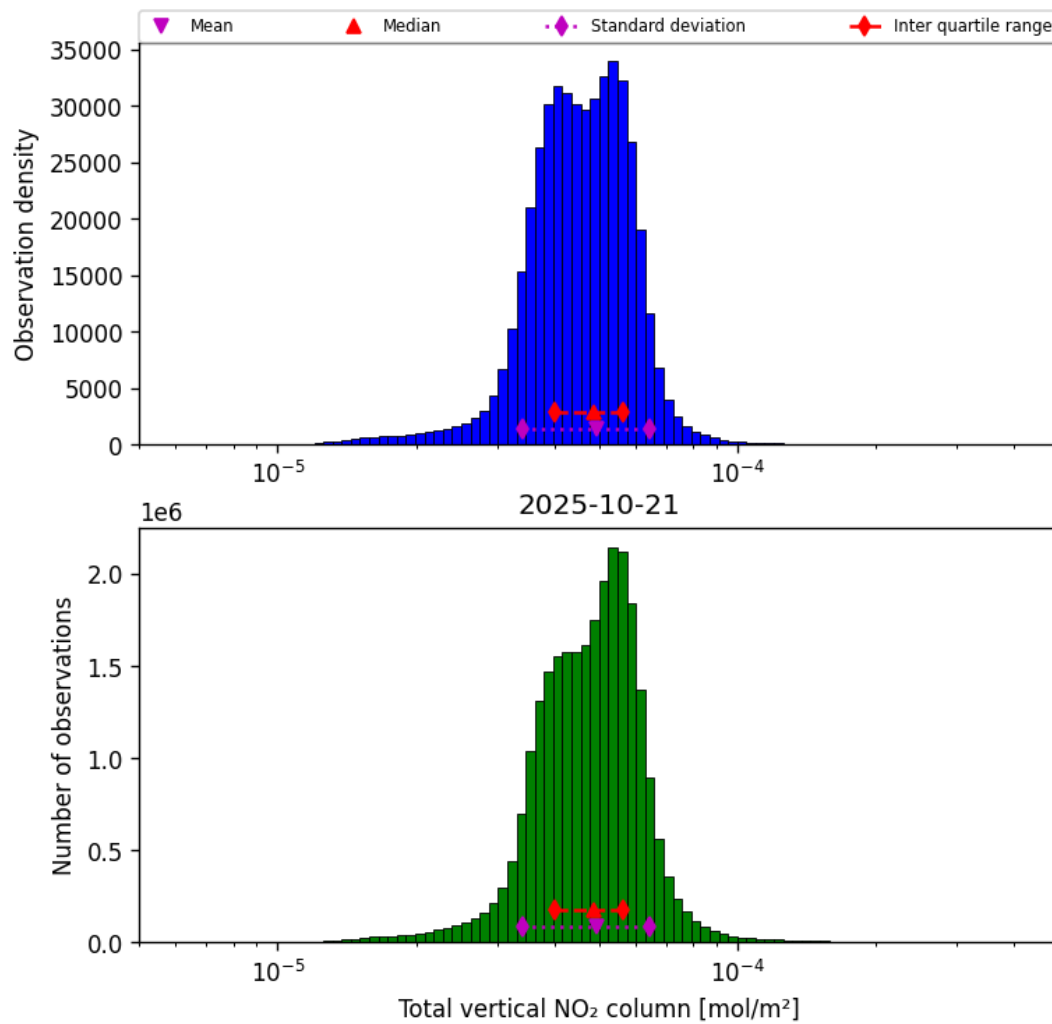
Figure 38: Histogram of “Total vertical NO 2 column” for 2025-10-20 to 2025-10-22
