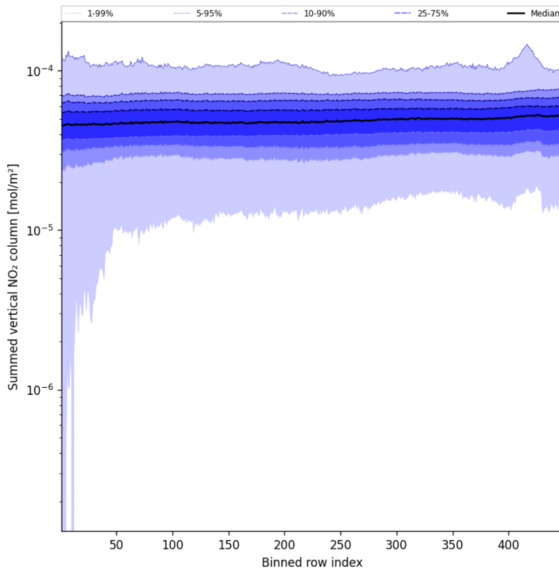
Figure 57: Along track statistics of “Summed vertical NO 2 column” for 2025-10-20 to 2025-10-22
