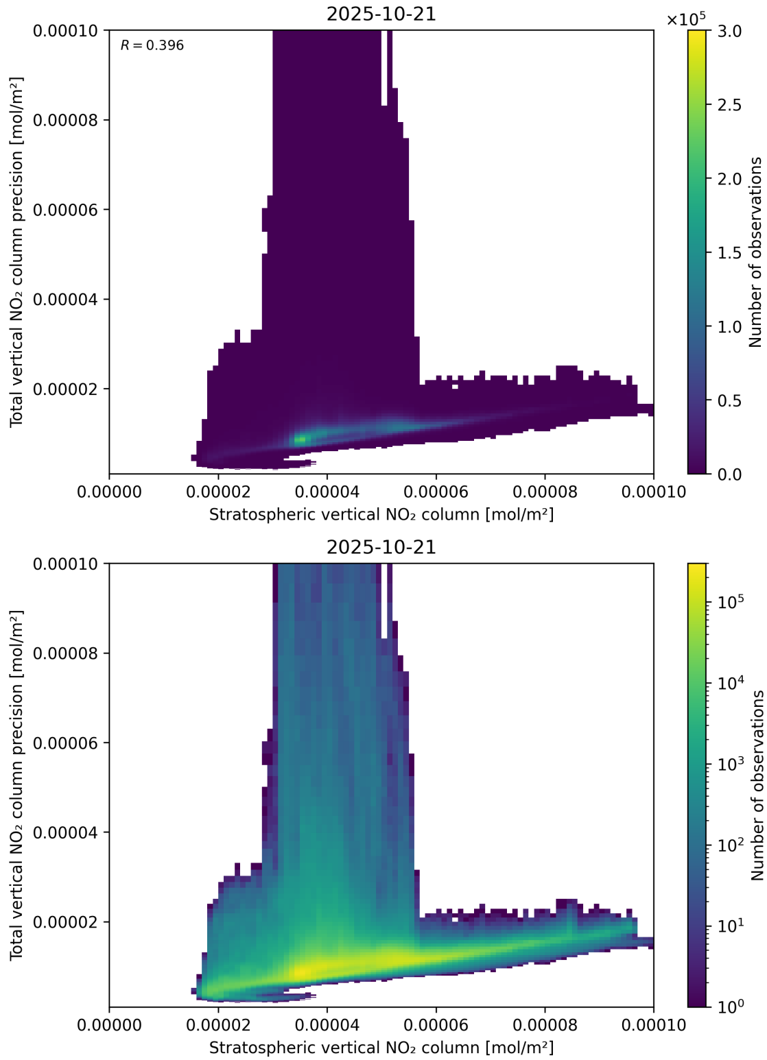
Figure 101: Scatter density plot of “Stratospheric vertical NO 2 column” against “Total vertical NO 2 column precision” for 2025-10-20 to 2025-10-22.
