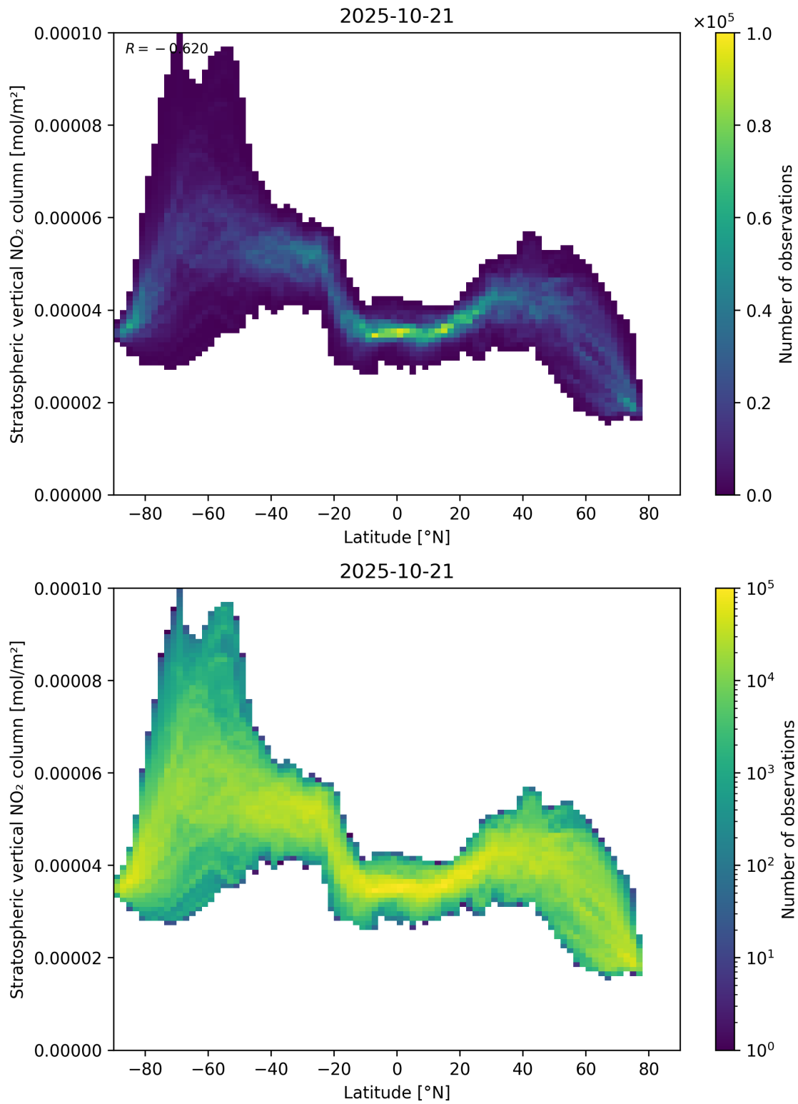
Figure 87: Scatter density plot of “Latitude” against “Stratospheric vertical NO 2 column” for 2025-10-20 to 2025-10-22.
