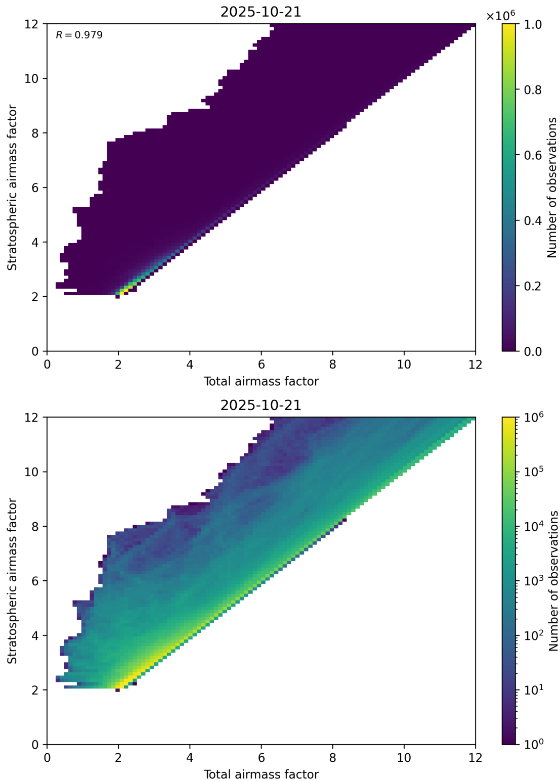
Figure 62: Scatter density plot of “Total airmass factor” against “Stratospheric airmass factor” for 2025-10-20 to 2025-10-22.
