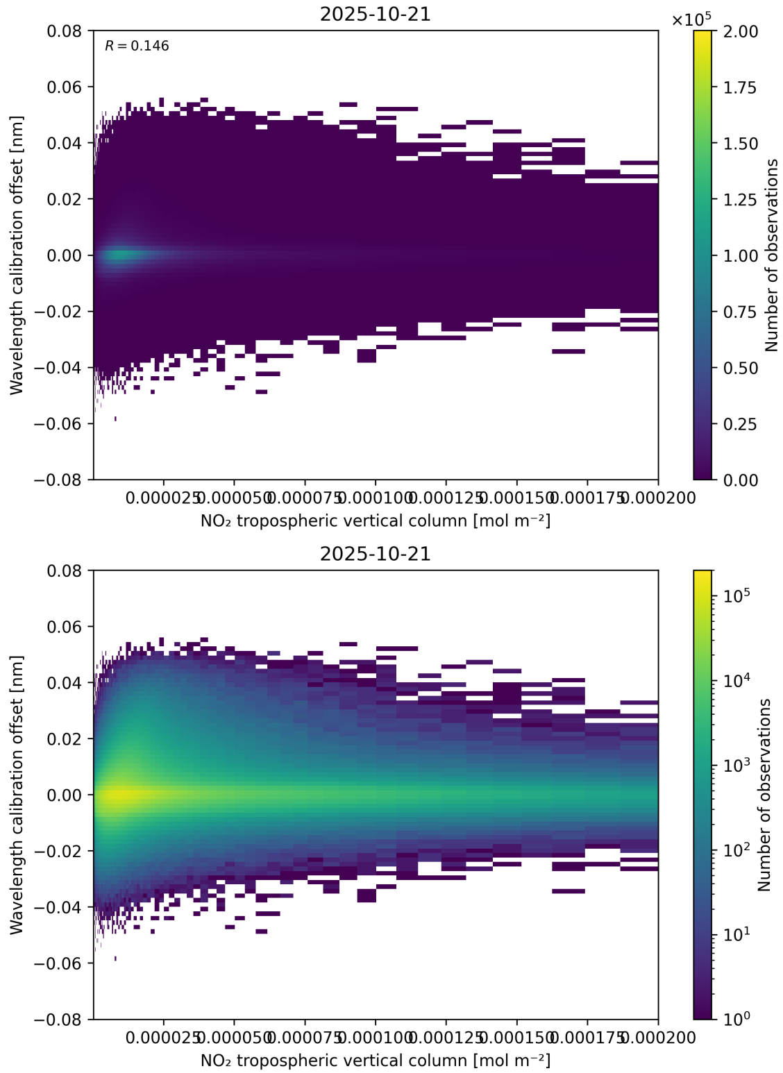
Figure 143: Scatter density plot of “NO 2 tropospheric vertical column” against “Wavelength calibration offset” for 2025-10-20 to 2025-10-22.
