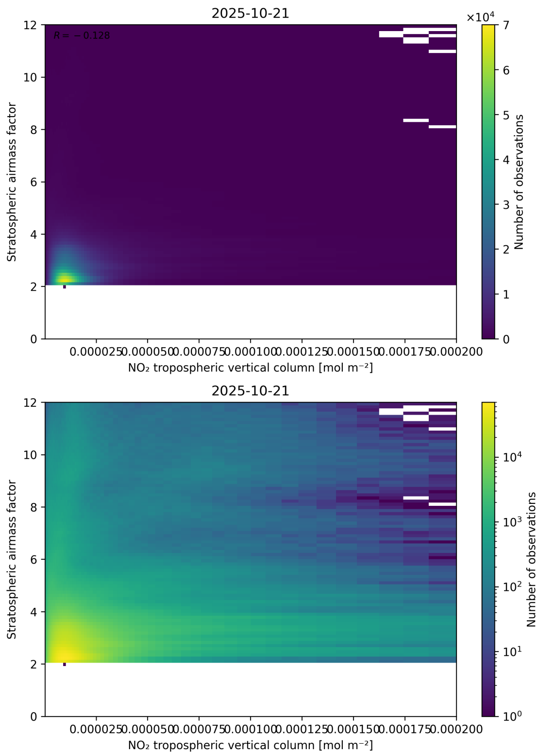
Figure 121: Scatter density plot of “NO 2 tropospheric vertical column” against “Stratospheric airmass factor” for 2025-10-20 to 2025-10-22.
