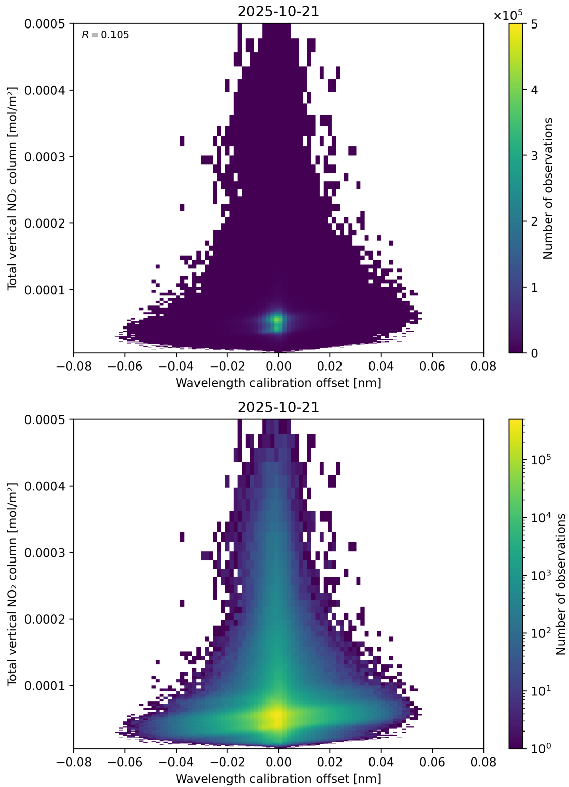
Figure 179: Scatter density plot of “Wavelength calibration offset” against “Total vertical NO 2 column” for 2025-10-20 to 2025-10-22.
