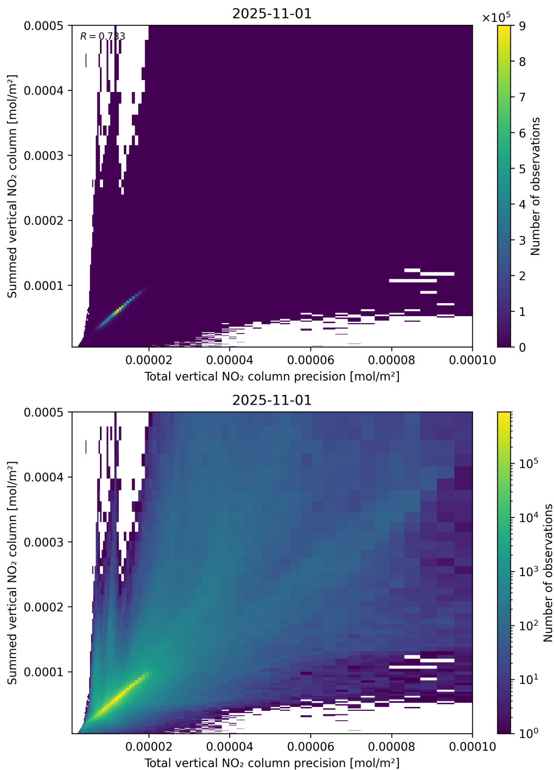
Figure 117: Scatter density plot of “Total vertical NO 2 column precision” against “Summed vertical NO 2 column” for 2025-10-31 to 2025-11-02.
