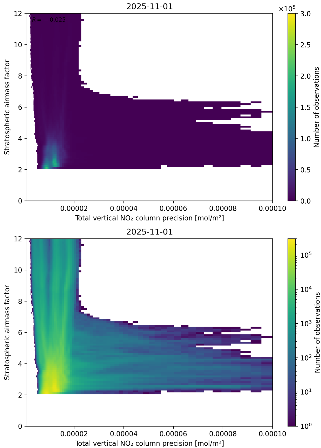
Figure 115: Scatter density plot of “Total vertical NO 2 column precision” against “Stratospheric air mass factor” for 2025-10-31 to 2025-11-02.
