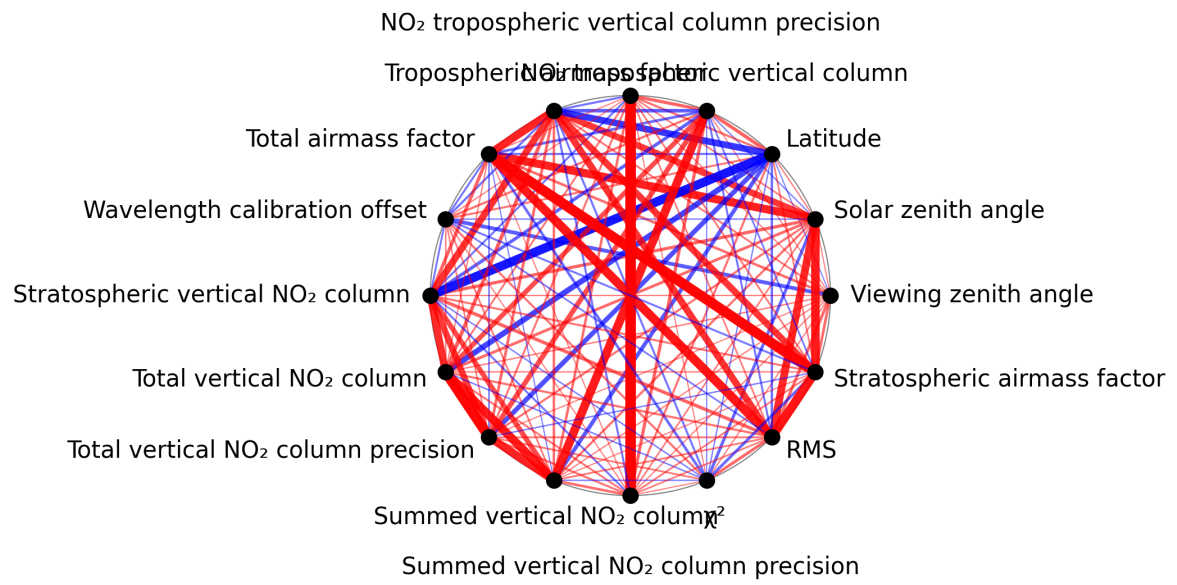
Figure 1: Map of correlation graph for 2025-10-31 to 2025-11-02.
