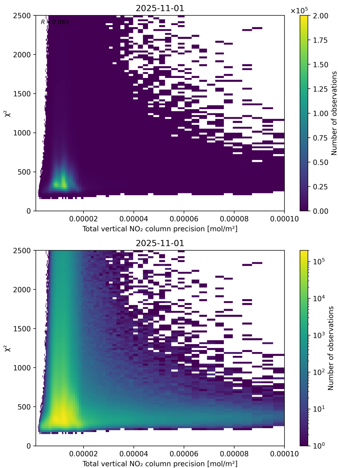
Figure 116: Scatter density plot of “Total vertical NO 2 column precision” against “ \chi^2 ” for 2025-10-31 to 2025-11-02.
