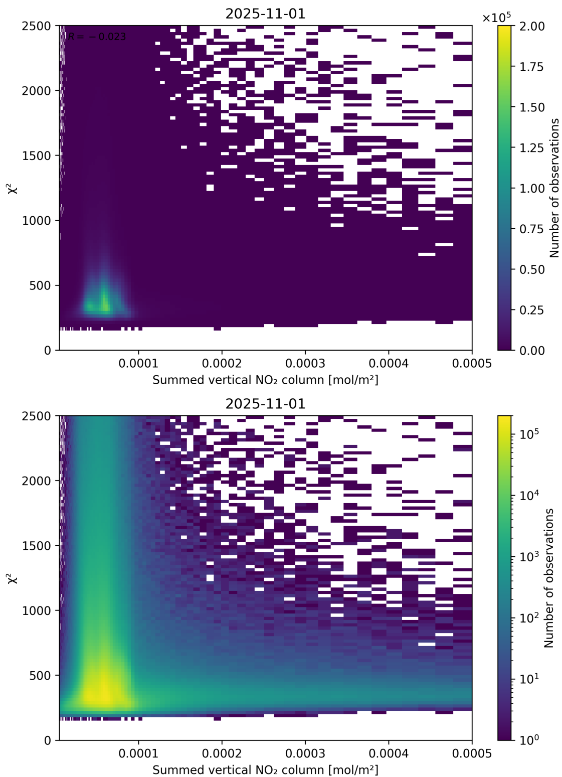
Figure 104: Scatter density plot of “Summed vertical NO 2 column” against “ \chi^2 ” for 2025-10-31 to 2025-11-02.
