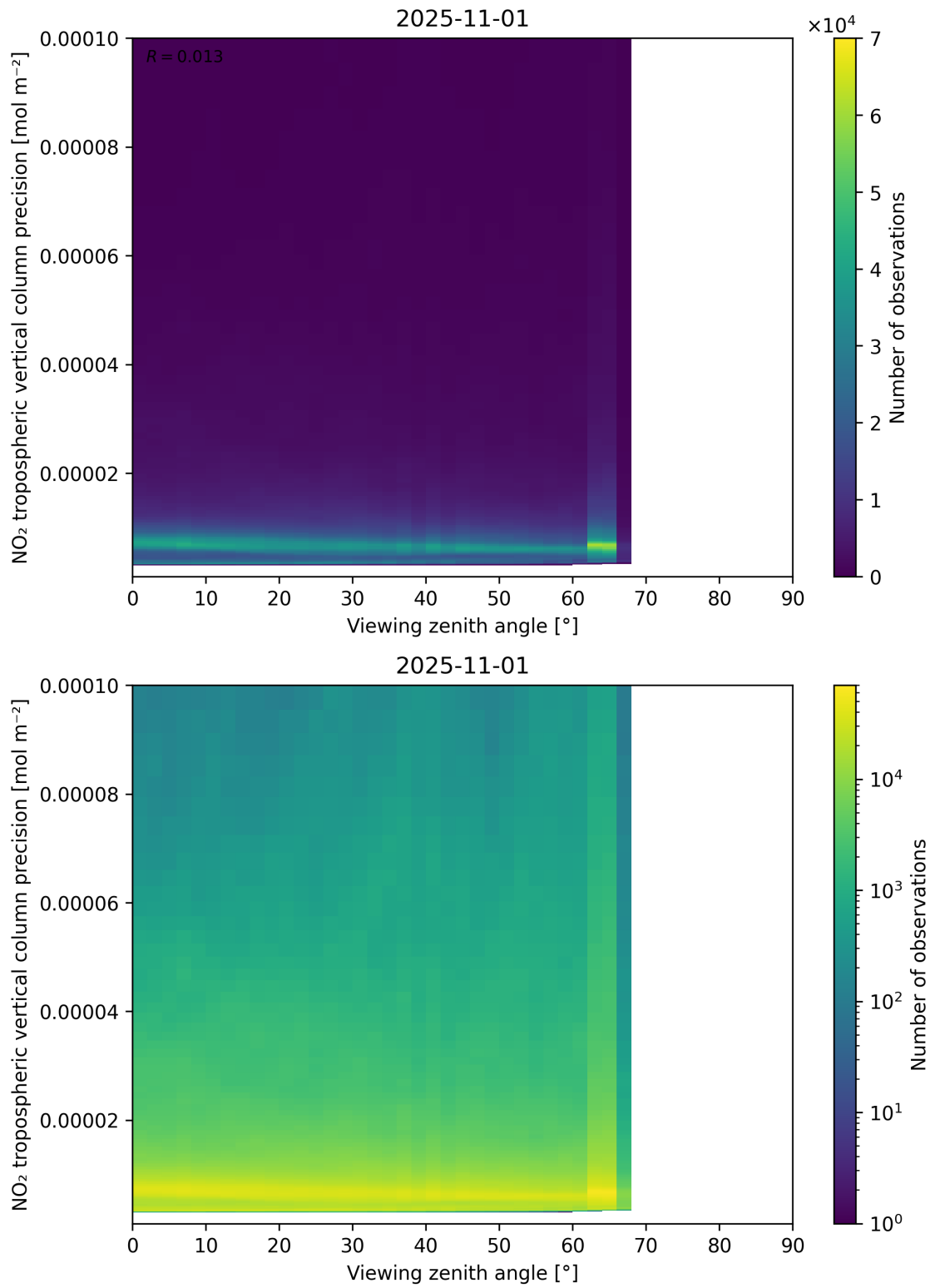
Figure 170: Scatter density plot of “Viewing zenith angle” against “NO 2 tropospheric vertical column precision” for 2025-10-31 to 2025-11-02.
