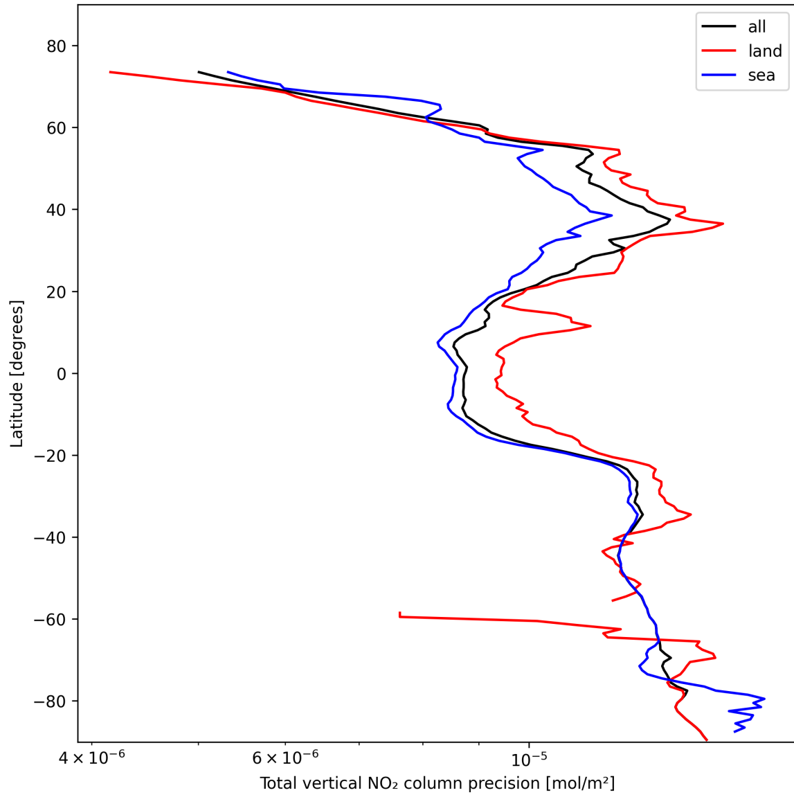
Figure 22: Zonal average of “Total vertical NO 2 column precision” for 2025-10-31 to 2025-11-02.
