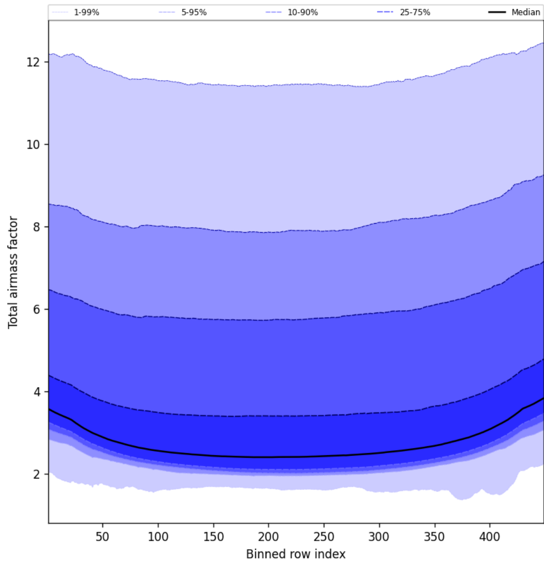
Figure 49: Along track statistics of “Total airmass factor” for 2025-10-31 to 2025-11-02
