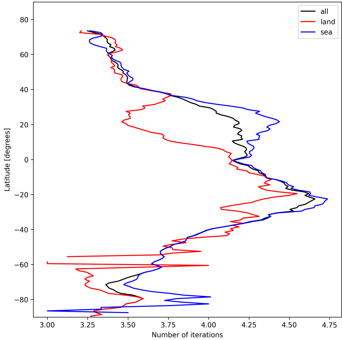
Figure 17: Zonal average of “Number of iterations” for 2025-10-31 to 2025-11-02.
