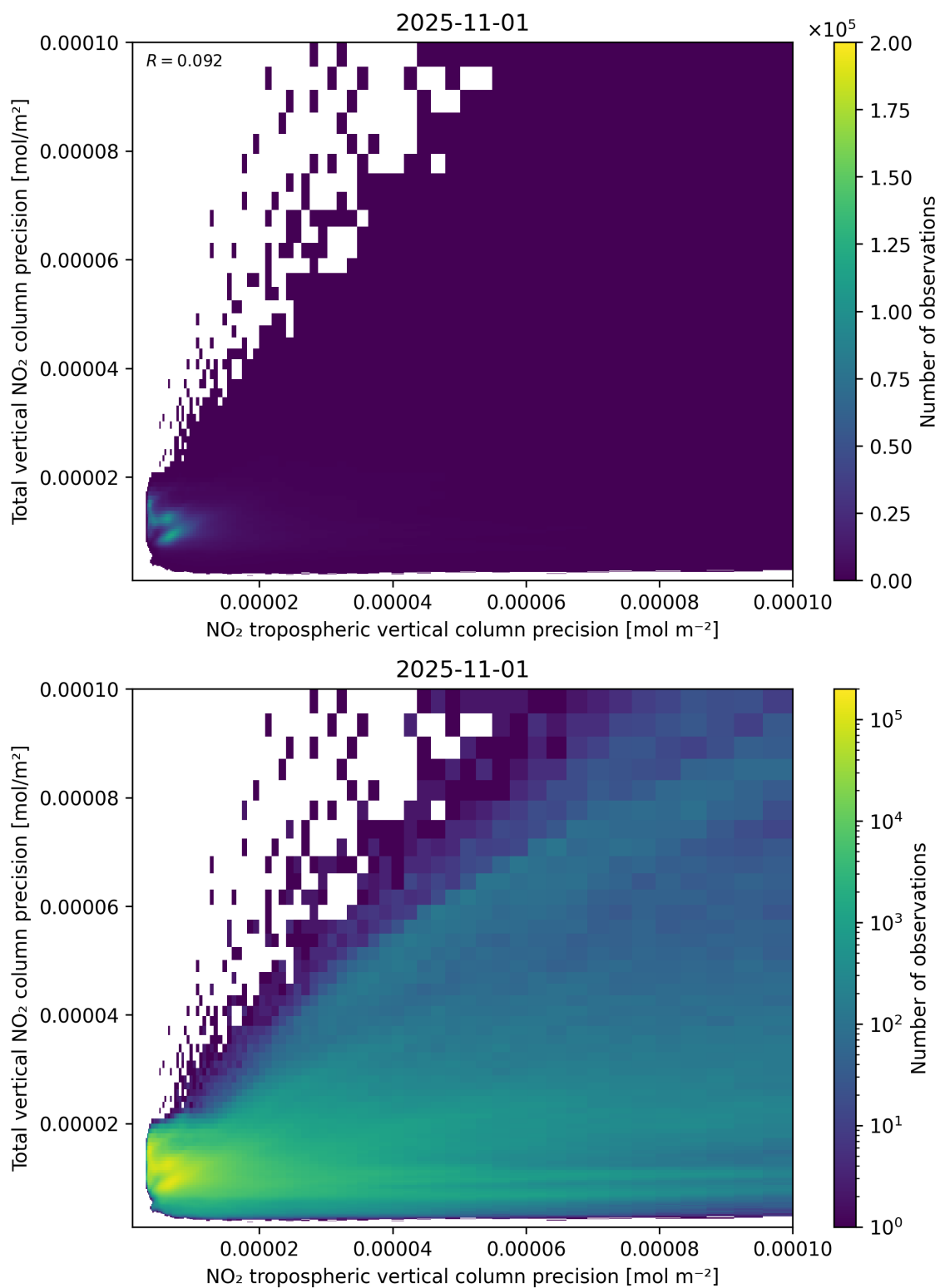
Figure 139: Scatter density plot of “NO 2 tropospheric vertical column precision” against “Total vertical NO 2 column precision” for 2025-10-31 to 2025-11-02.
