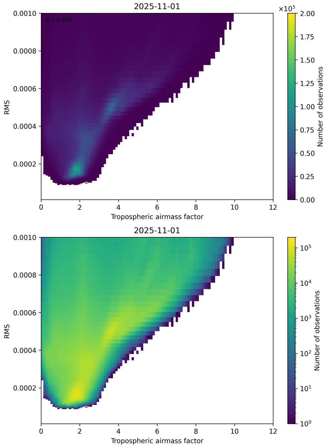
Figure 79: Scatter density plot of “Tropospheric airmass factor” against “RMS” for 2025-10-31 to 2025-11-02.
