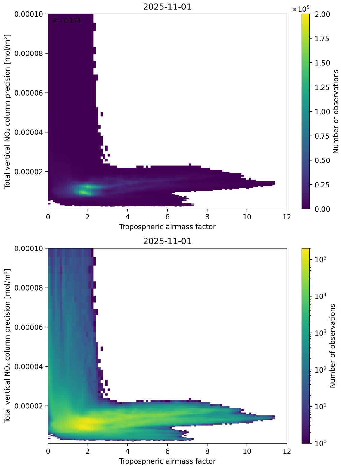
Figure 78: Scatter density plot of “Tropospheric airmass factor” against “Total vertical NO 2 column precision” for 2025-10-31 to 2025-11-02.
