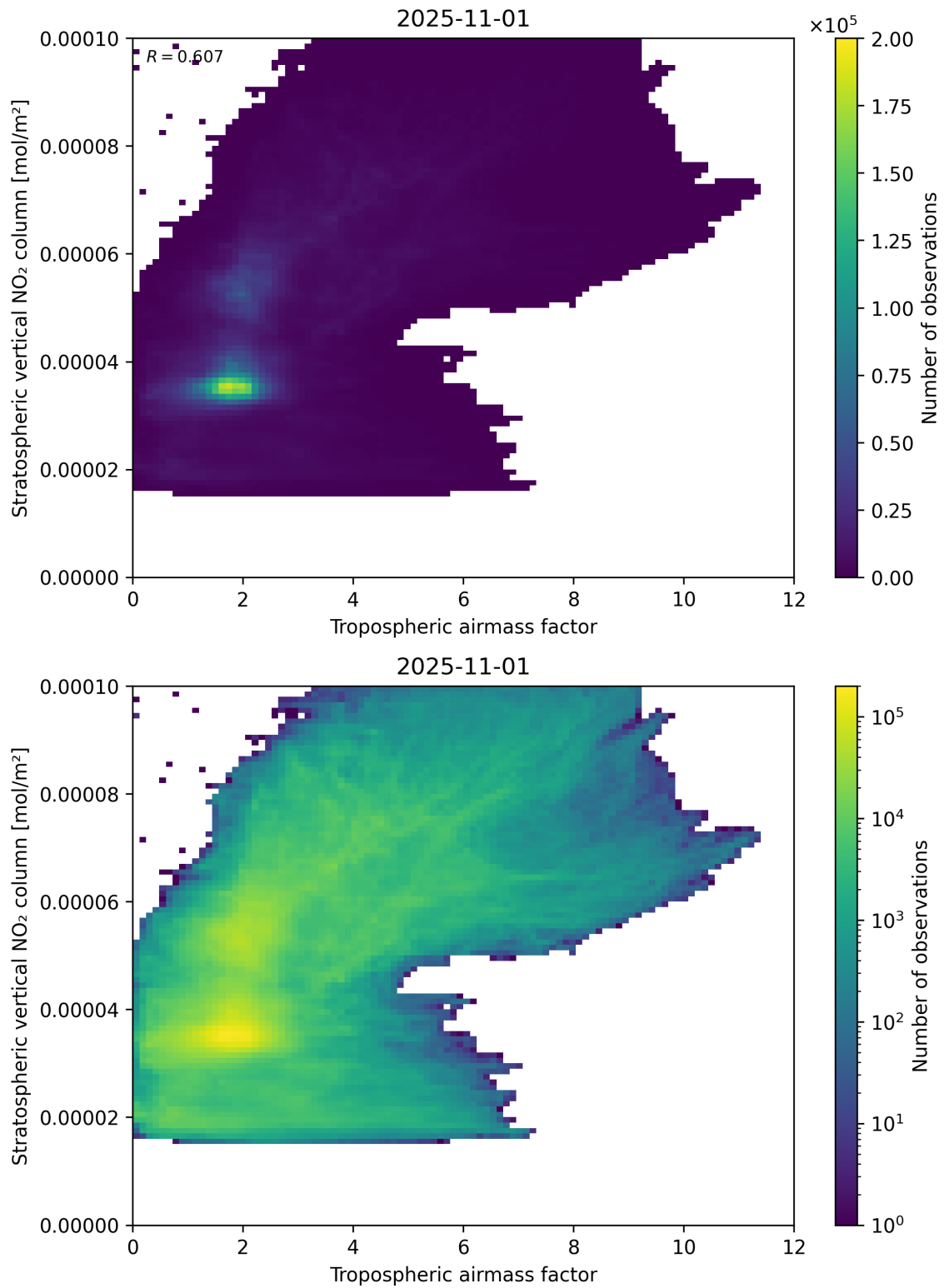
Figure 74: Scatter density plot of “Tropospheric air mass factor” against “Stratospheric vertical NO 2 column” for 2025-10-31 to 2025-11-02.
