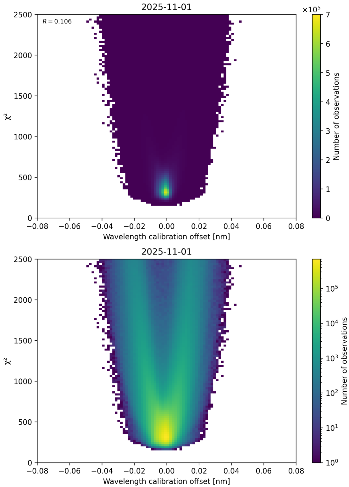
Figure 175: Scatter density plot of “Wavelength calibration offset” against “ \chi^2 ” for 2025-10-31 to 2025-11-02.
