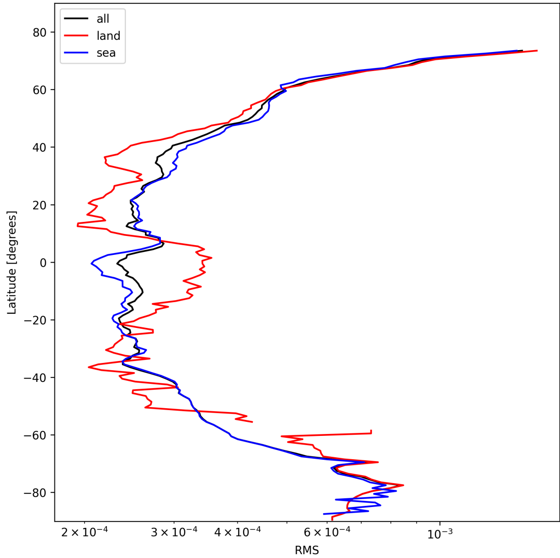
Figure 26: Zonal average of “RMS” for 2025-10-31 to 2025-11-02.
