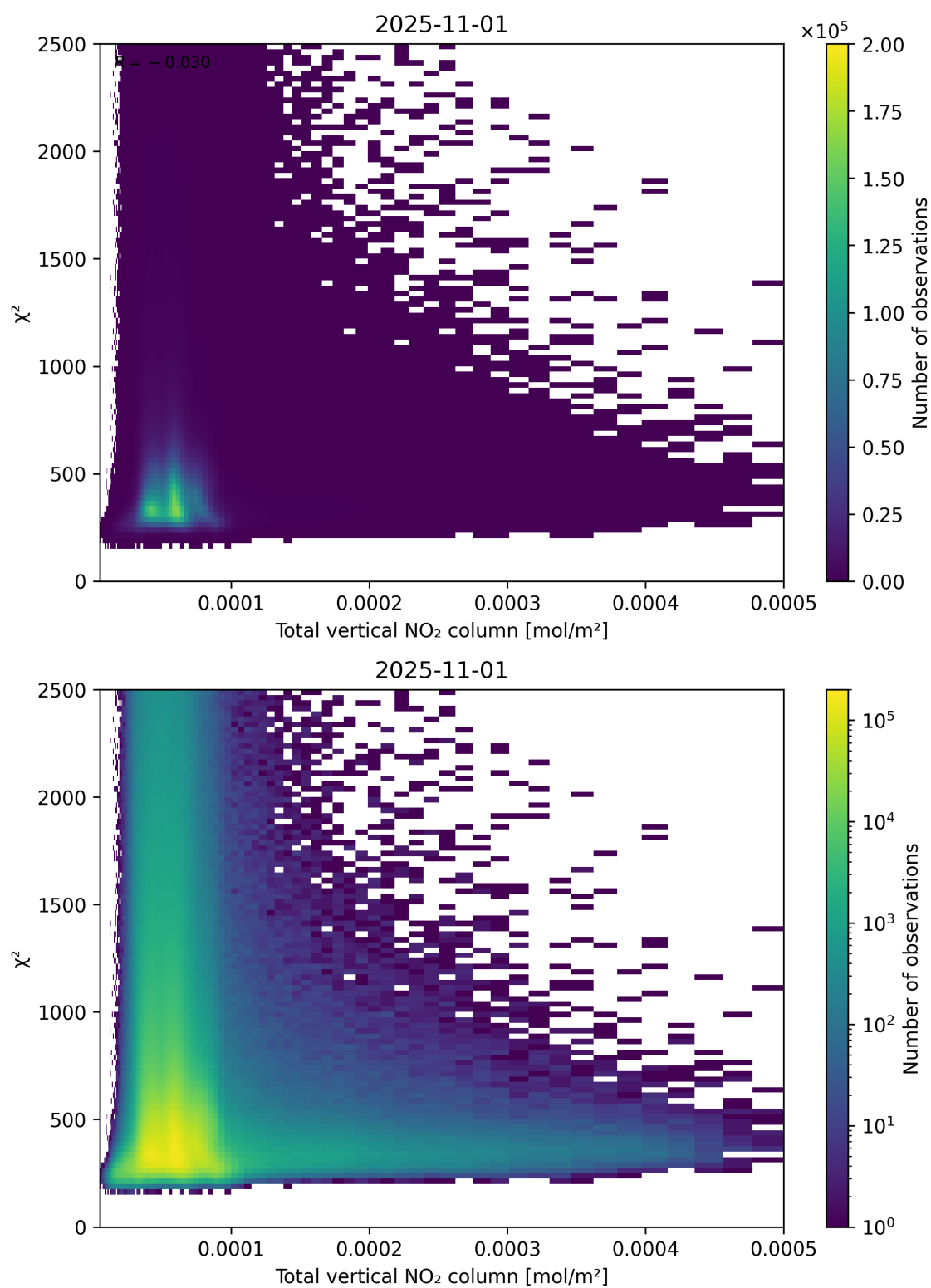
Figure 111: Scatter density plot of “Total vertical NO 2 column” against “ \chi^2 ” for 2025-10-31 to 2025-11-02.
