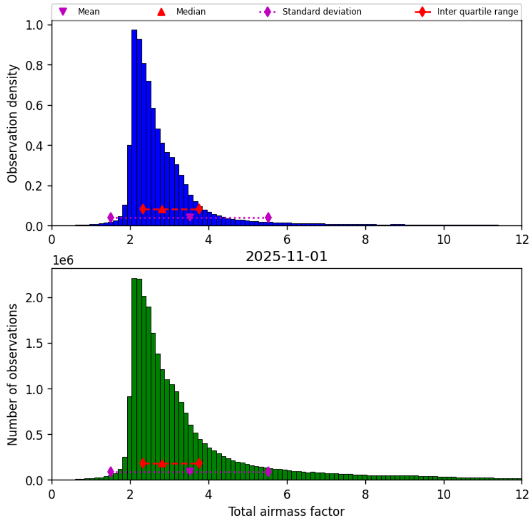
Figure 32: Histogram of “Total airmass factor” for 2025-10-31 to 2025-11-02
