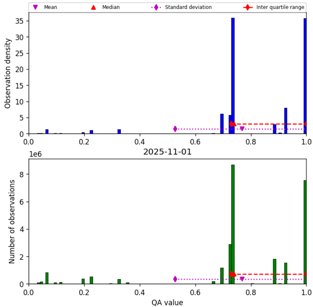
Figure 28: Histogram of “QA value” for 2025-10-31 to 2025-11-02
