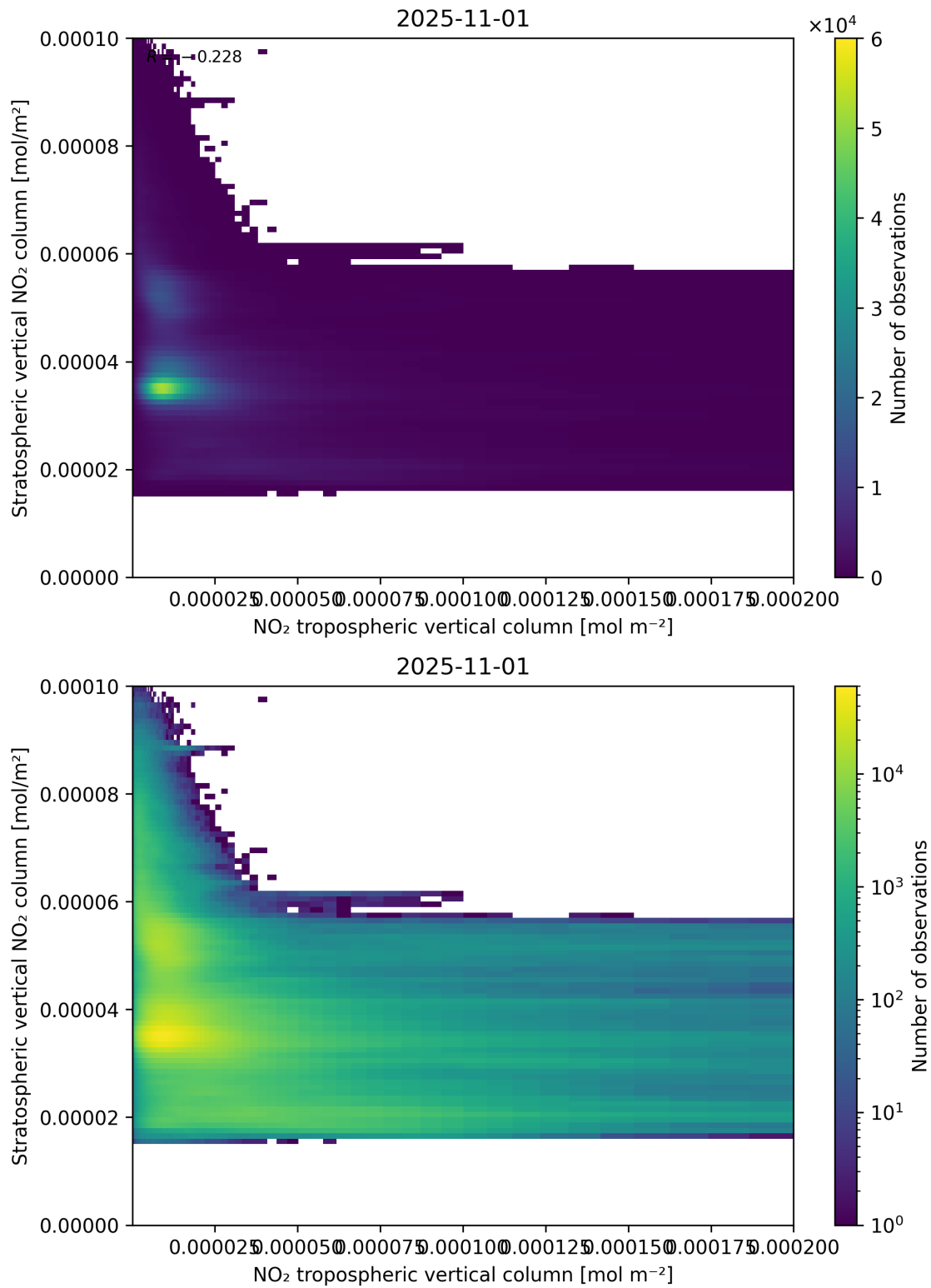
Figure 125: Scatter density plot of “NO 2 tropospheric vertical column” against “Stratospheric vertical NO 2 column” for 2025-10-31 to 2025-11-02.
