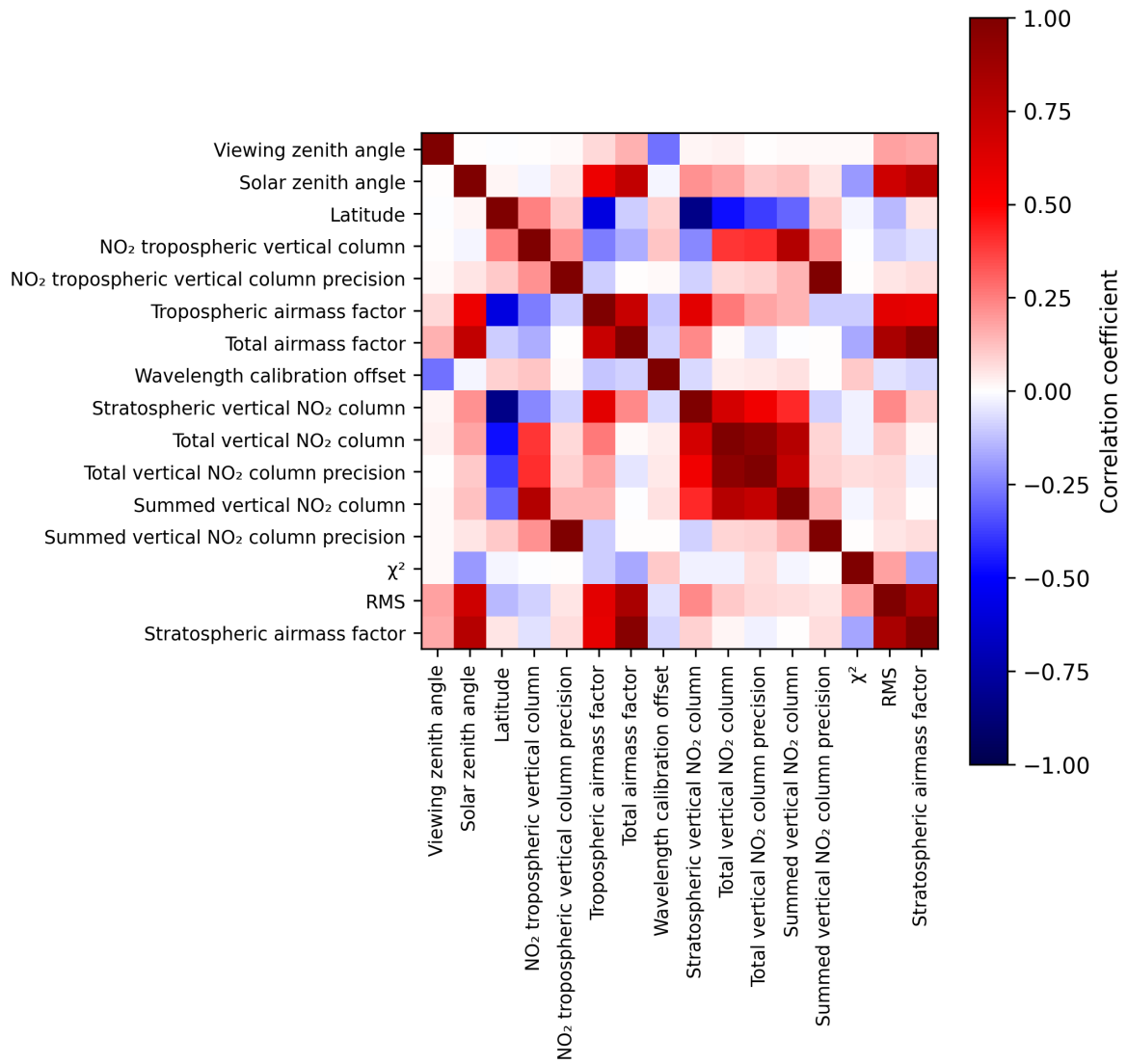
Figure 2: Map of correlation matrix for 2025-10-31 to 2025-11-02.
