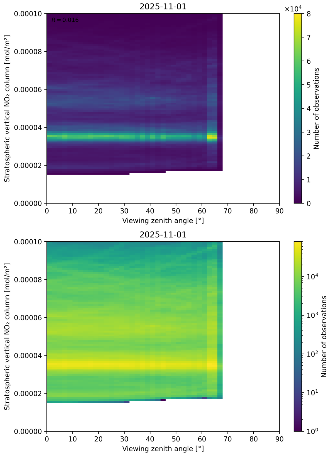
Figure 164: Scatter density plot of “Viewing zenith angle” against “Stratospheric vertical NO 2 column” for 2025-10-31 to 2025-11-02.
