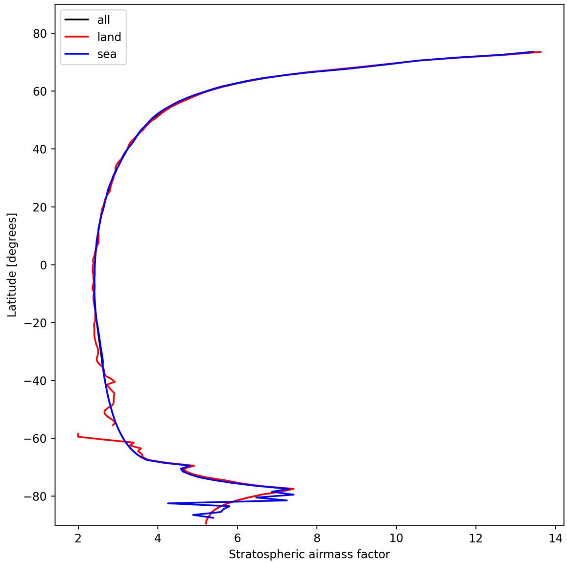
Figure 27: Zonal average of “Stratospheric airmass factor” for 2025-10-31 to 2025-11-02.
