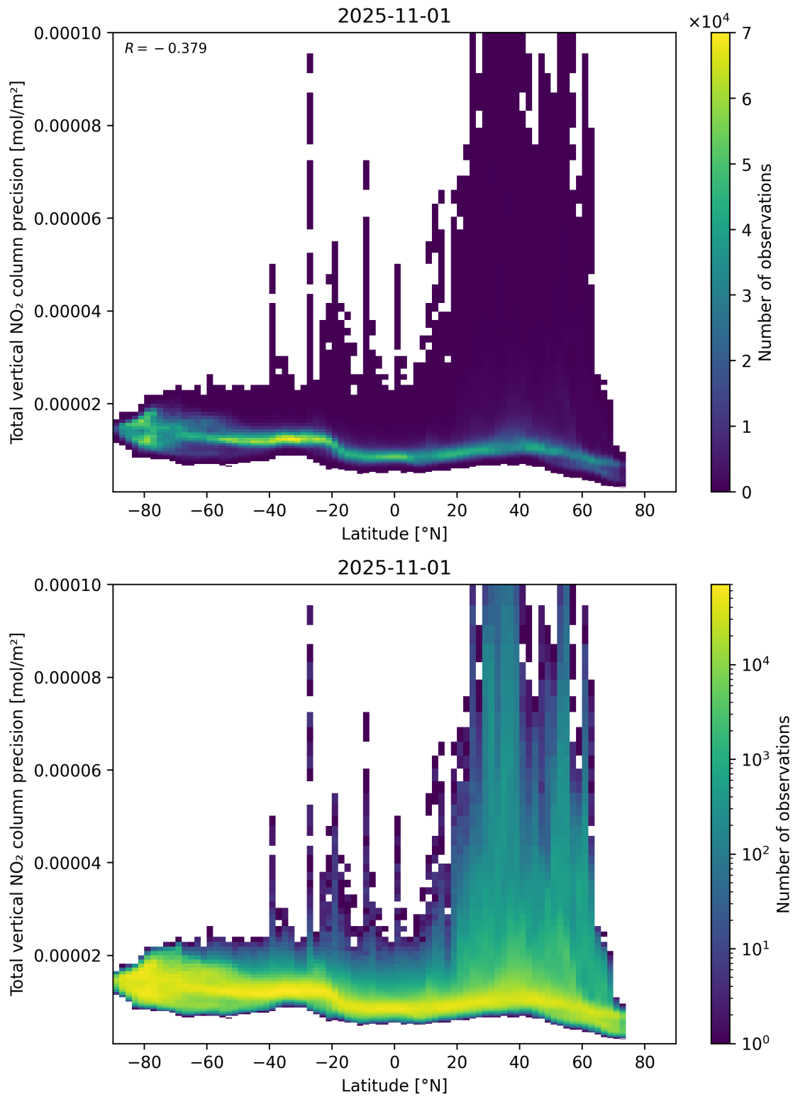
Figure 91: Scatter density plot of “Latitude” against “Total vertical NO 2 column precision” for 2025-10-31 to 2025-11-02.
