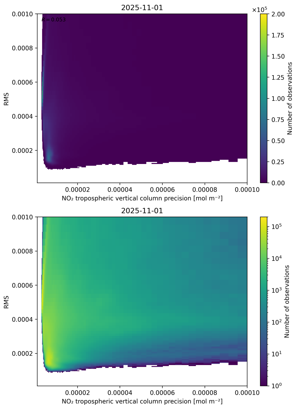
Figure 140: Scatter density plot of “NO 2 tropospheric vertical column precision” against “RMS” for 2025-10-31 to 2025-11-02.
