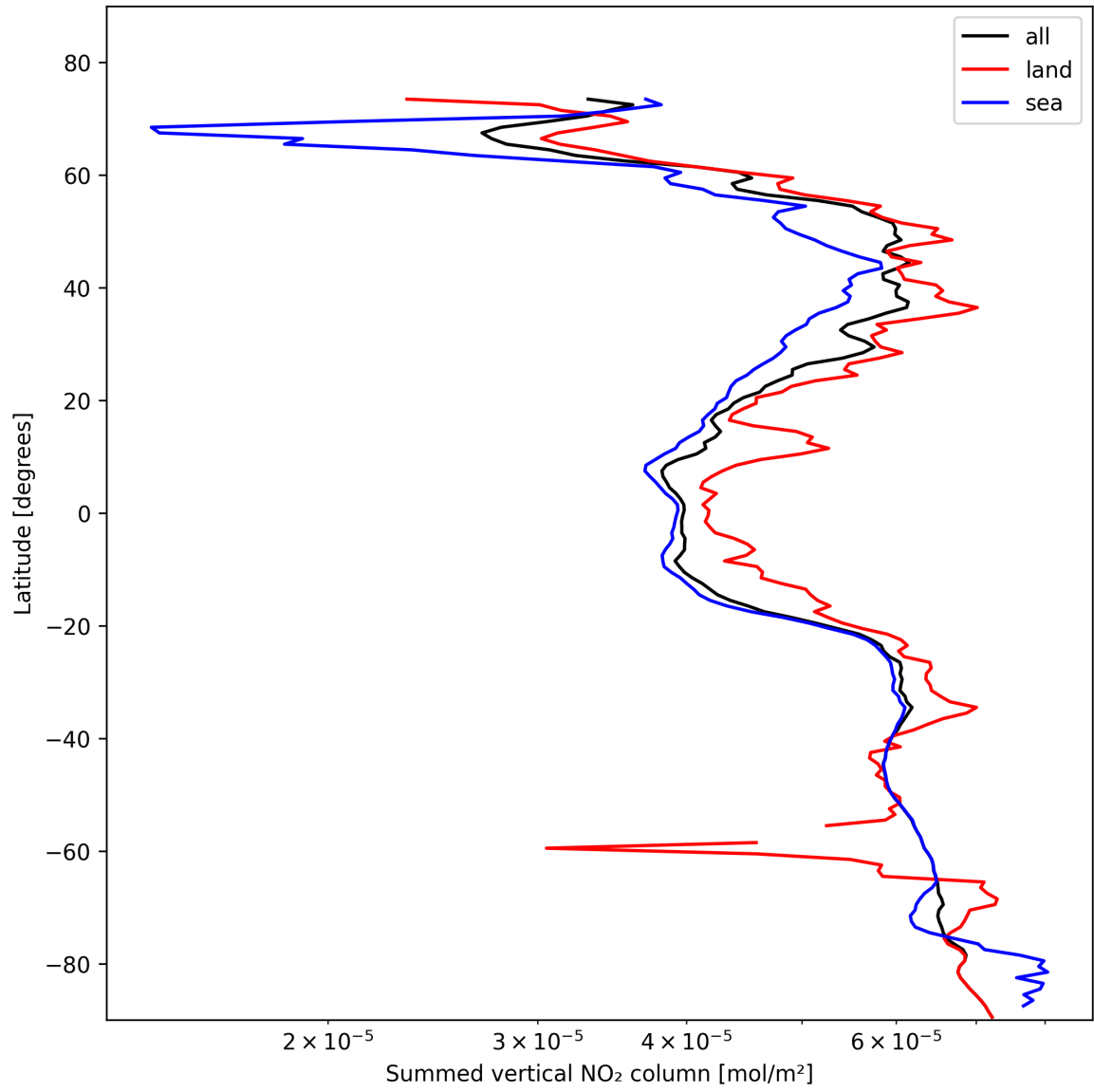
Figure 23: Zonal average of “Summed vertical NO 2 column” for 2025-10-31 to 2025-11-02.
