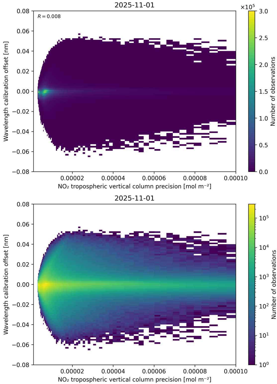
Figure 141: Scatter density plot of “NO 2 tropospheric vertical column precision” against “Wavelength calibration offset” for 2025-10-31 to 2025-11-02.
