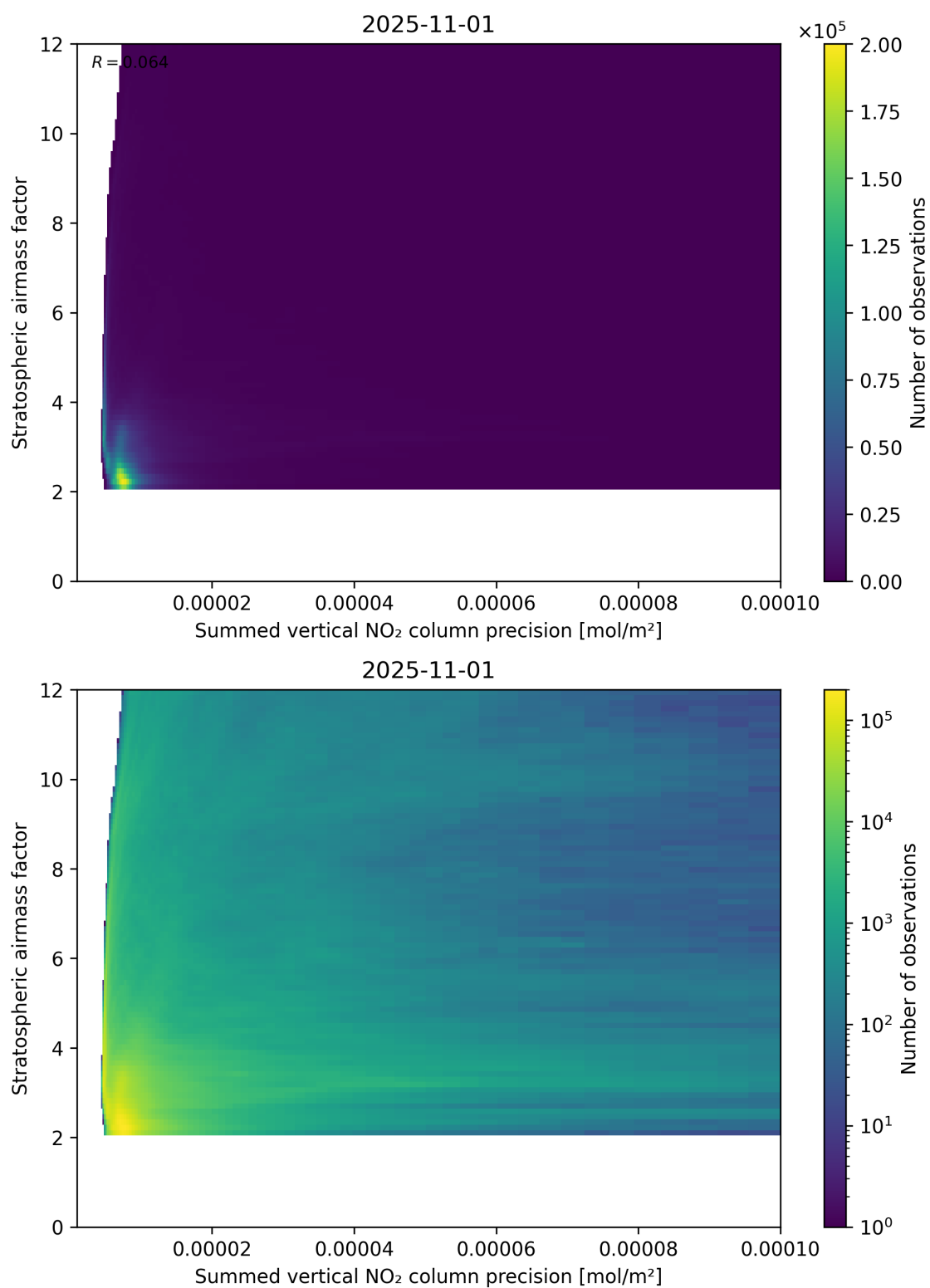
Figure 106: Scatter density plot of “Summed vertical NO 2 column precision” against “Stratospheric airmass factor” for 2025-10-31 to 2025-11-02.
