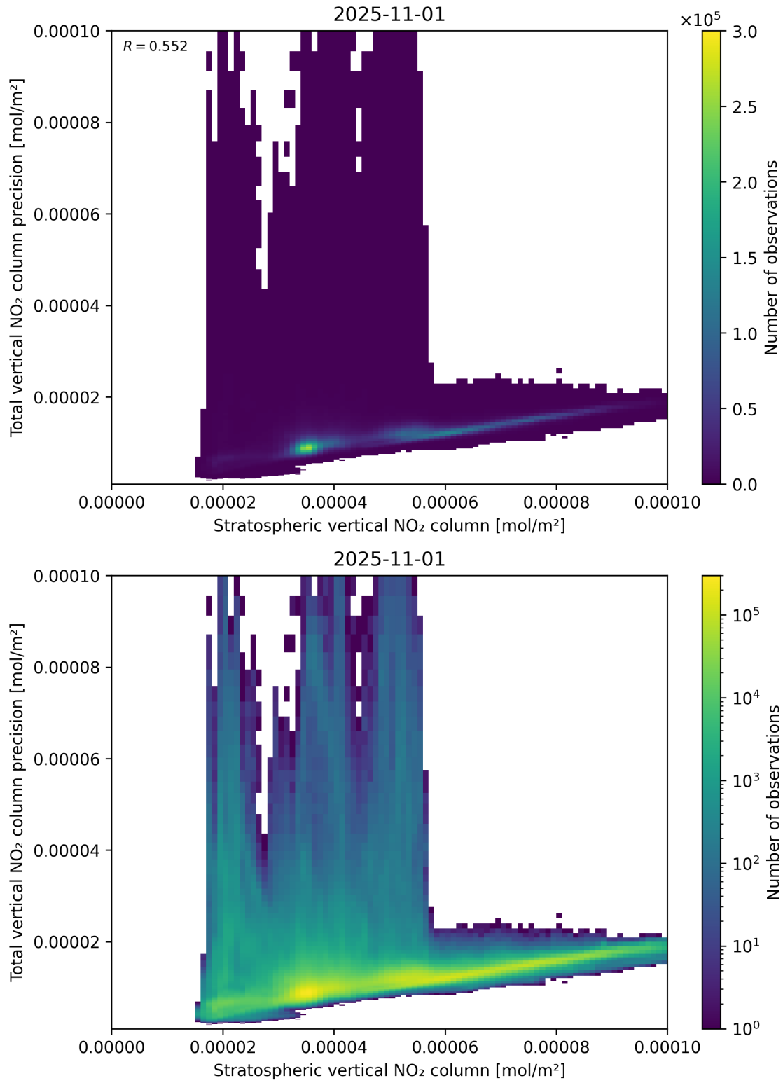
Figure 101: Scatter density plot of “Stratospheric vertical NO 2 column” against “Total vertical NO 2 column precision” for 2025-10-31 to 2025-11-02.
