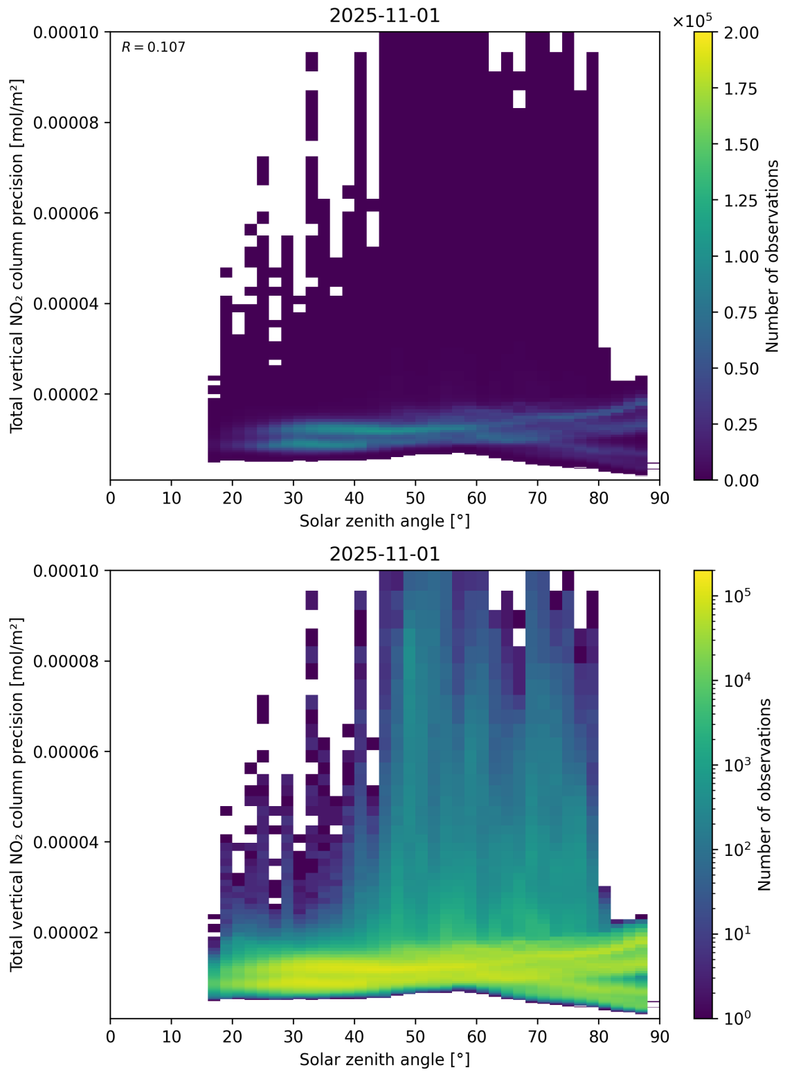
Figure 154: Scatter density plot of “Solar zenith angle” against “Total vertical NO 2 column precision” for 2025-10-31 to 2025-11-02.
