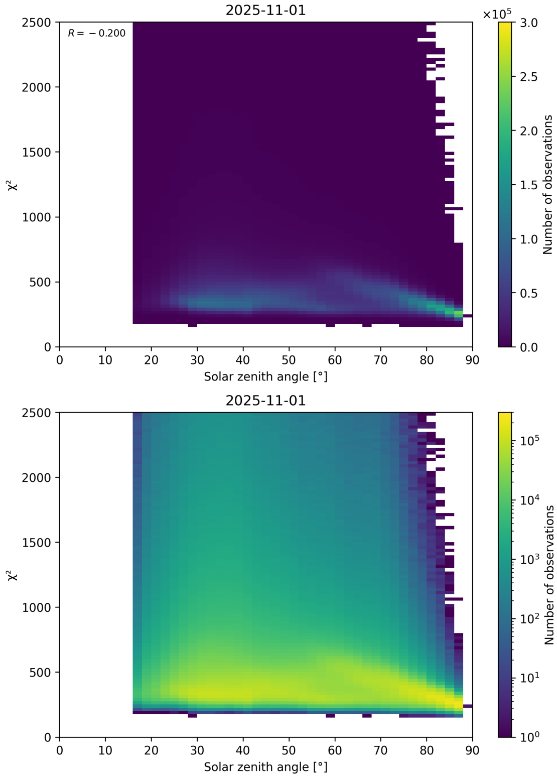
Figure 148: Scatter density plot of “Solar zenith angle” against “ \chi^2 ” for 2025-10-31 to 2025-11-02.
