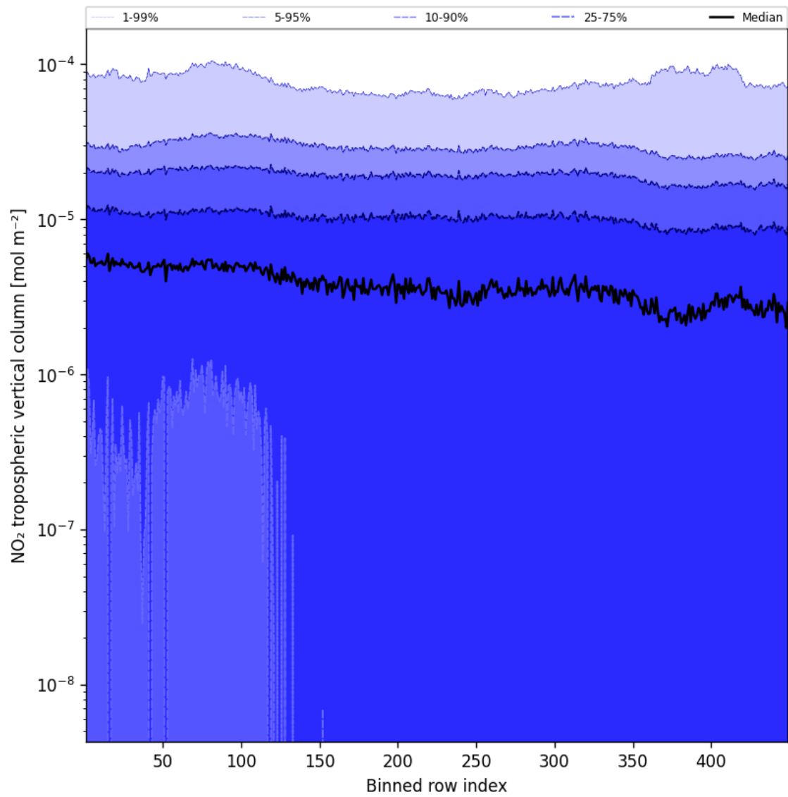
Figure 46: Along track statistics of “NO 2 tropospheric vertical column” for 2025-10-31 to 2025-11-02
