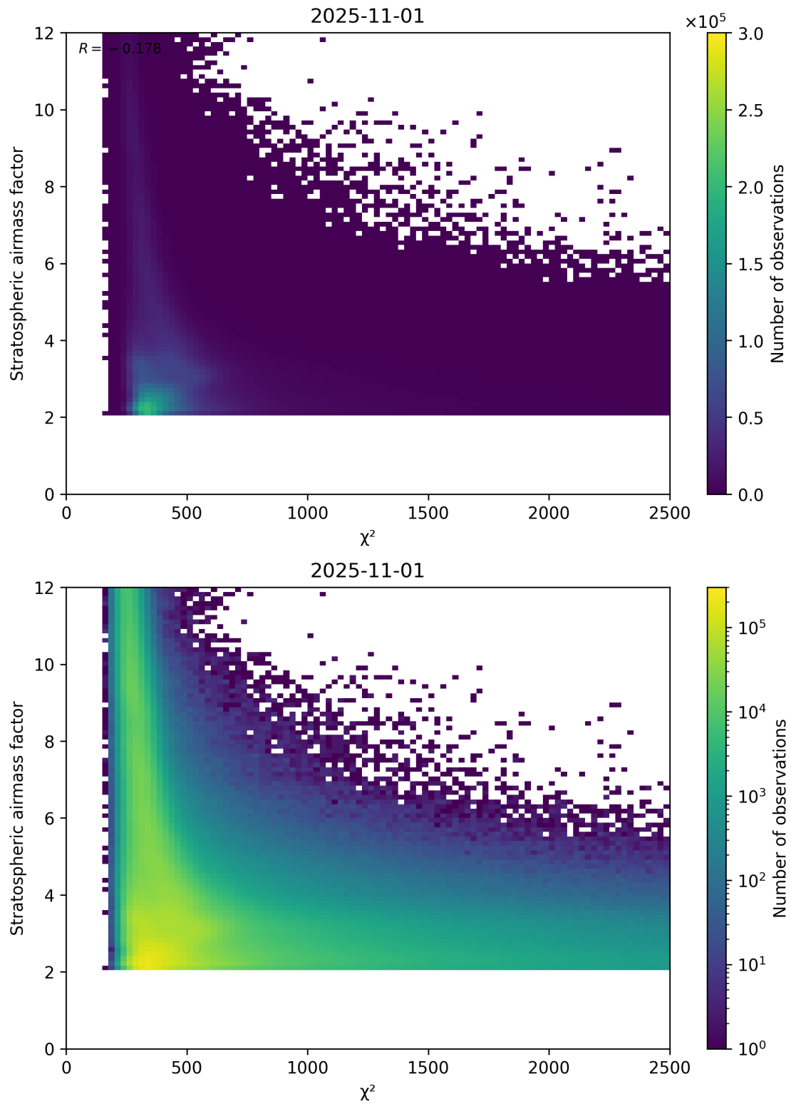
Figure 81: Scatter density plot of “ \chi^2 ” against “Stratospheric airmass factor” for 2025-10-31 to 2025-11-02.
