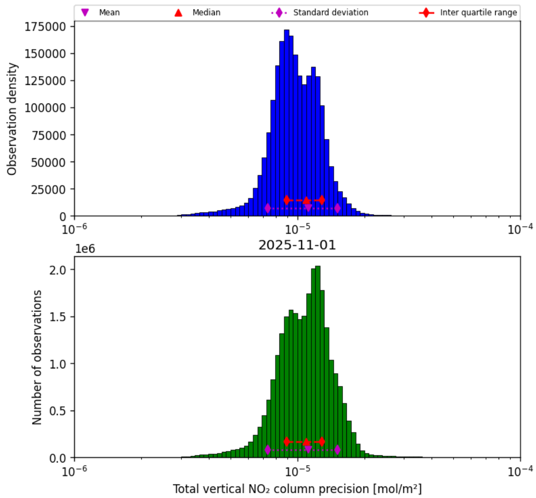
Figure 39: Histogram of “Total vertical NO 2 column precision” for 2025-10-31 to 2025-11-02
