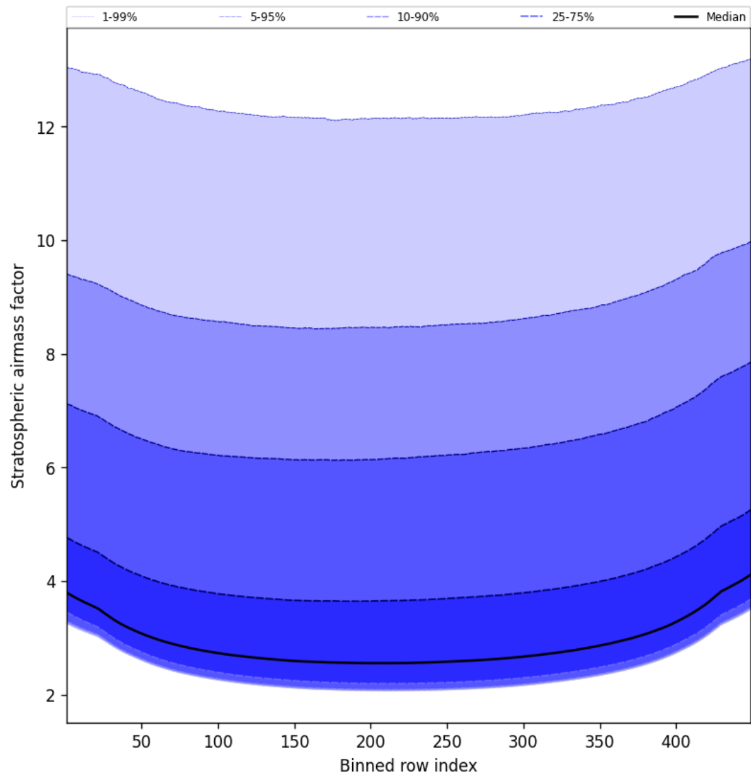
Figure 61: Along track statistics of “Stratospheric airmass factor” for 2025-10-31 to 2025-11-02
