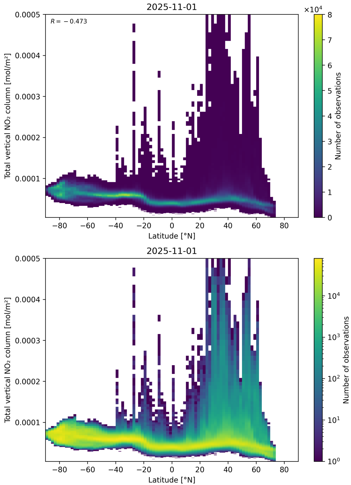
Figure 90: Scatter density plot of “Latitude” against “Total vertical NO 2 column” for 2025-10-31 to 2025-11-02.
