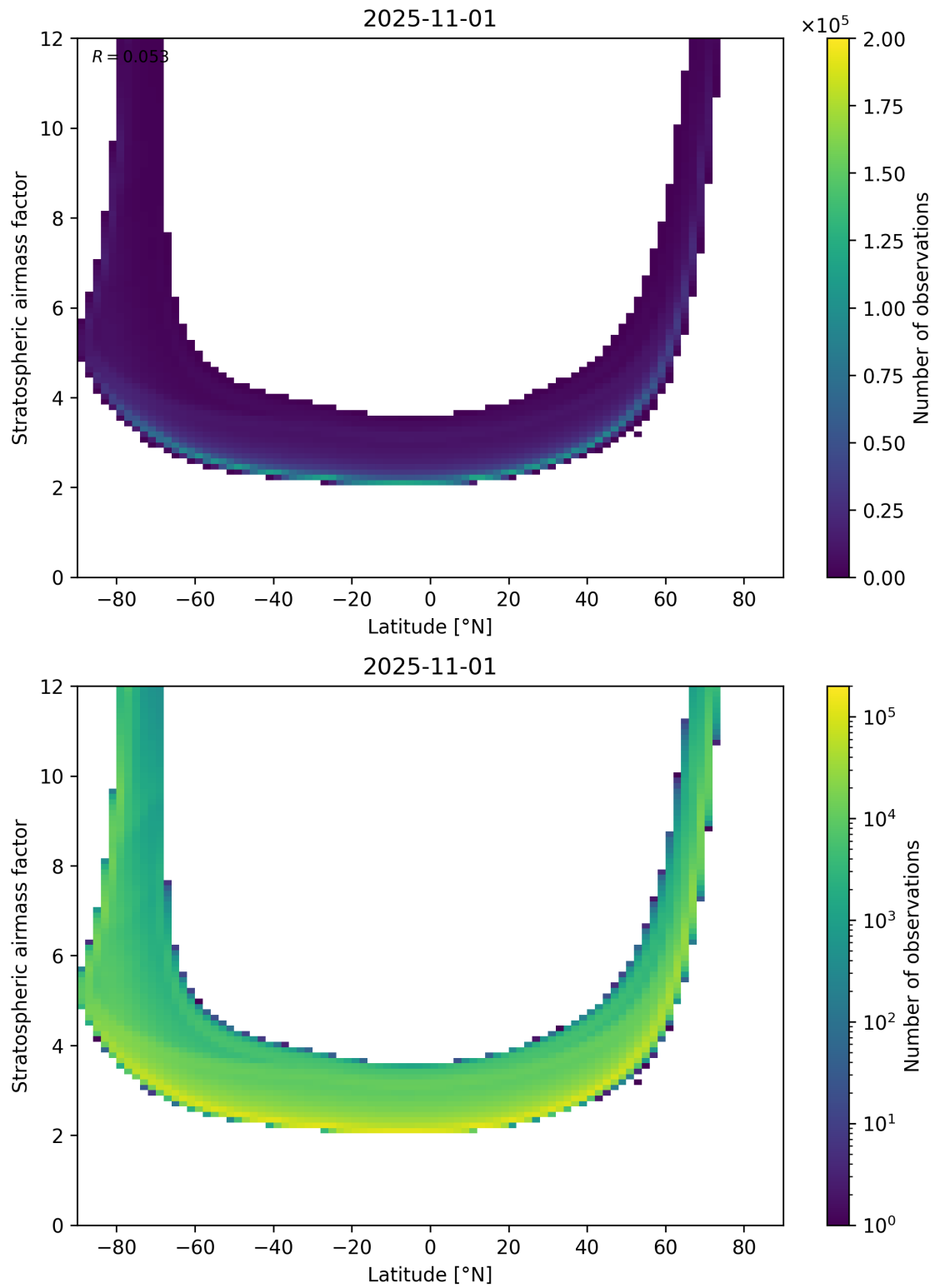
Figure 83: Scatter density plot of “Latitude” against “Stratospheric airmass factor” for 2025-10-31 to 2025-11-02.
