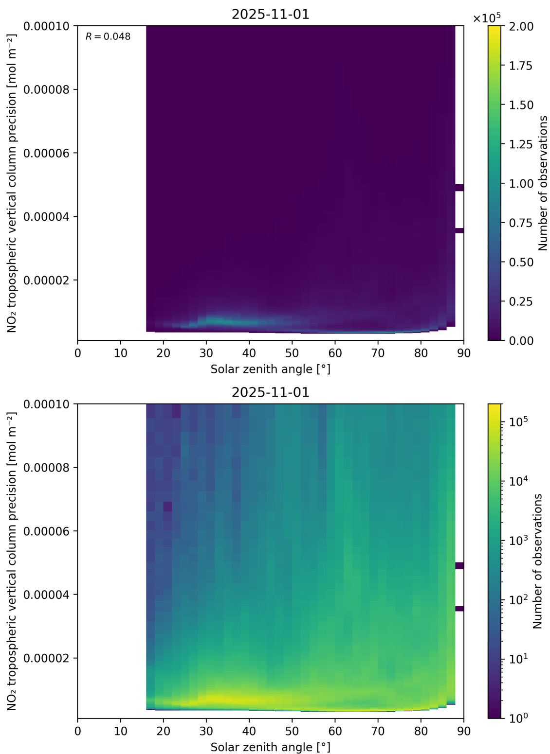
Figure 156: Scatter density plot of “Solar zenith angle” against “NO 2 tropospheric vertical column precision” for 2025-10-31 to 2025-11-02.
