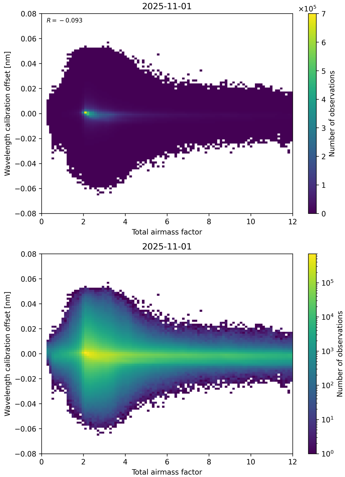
Figure 70: Scatter density plot of “Total airmass factor” against “Wavelength calibration offset” for 2025-10-31 to 2025-11-02.
