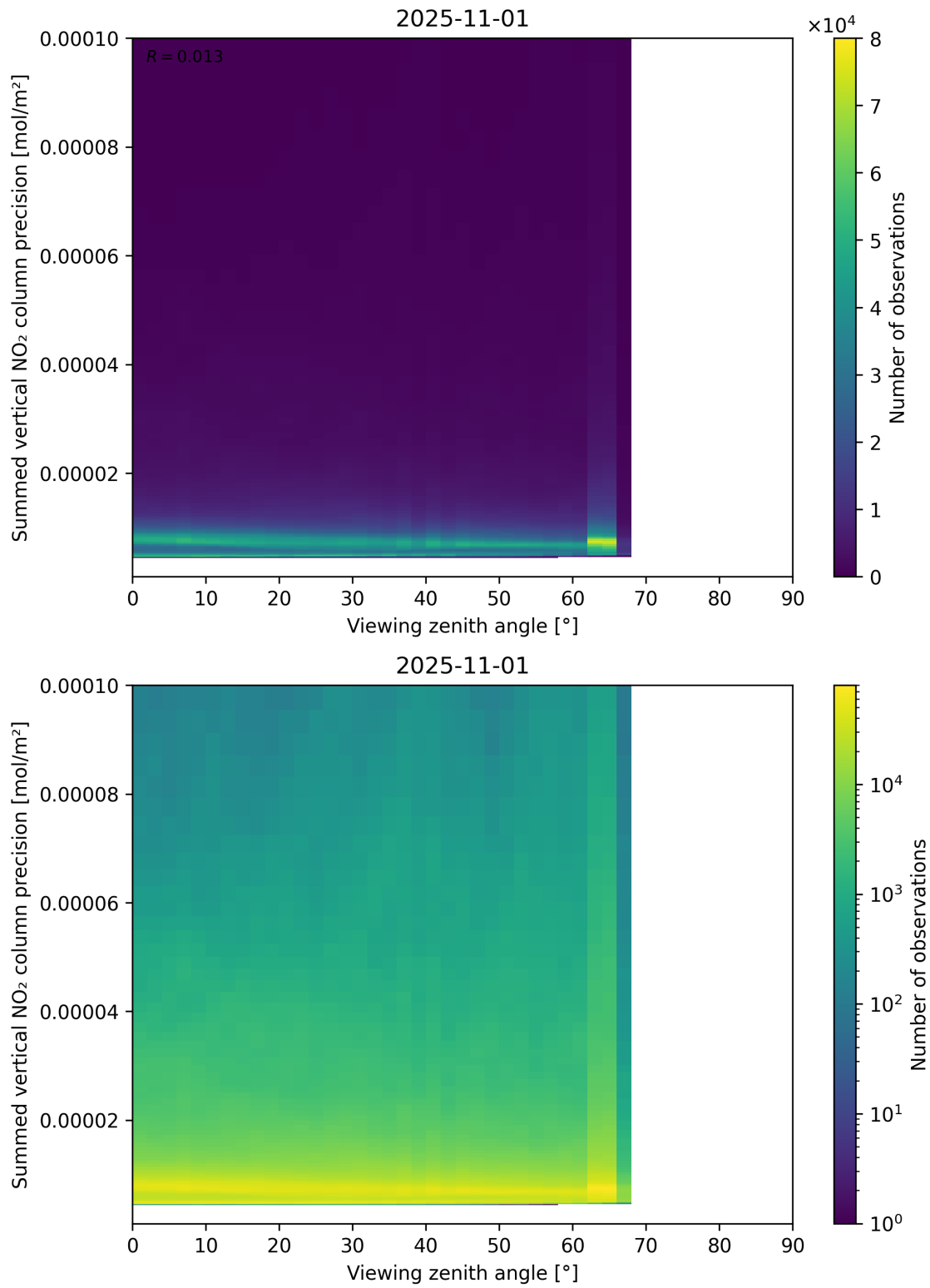
Figure 166: Scatter density plot of “Viewing zenith angle” against “Summed vertical NO 2 column precision” for 2025-10-31 to 2025-11-02.
