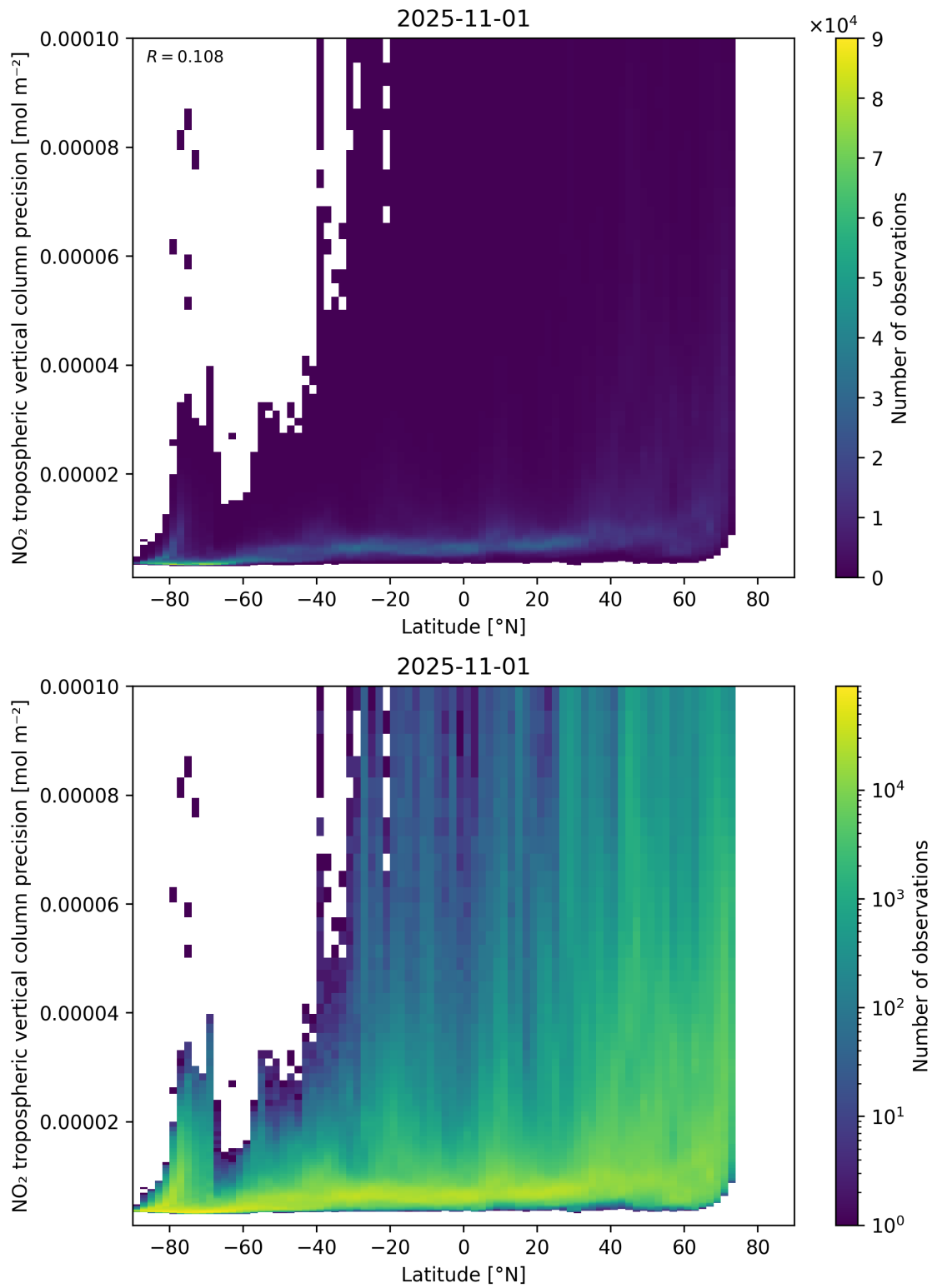
Figure 93: Scatter density plot of “Latitude” against “NO 2 tropospheric vertical column precision” for 2025-10-31 to 2025-11-02.
