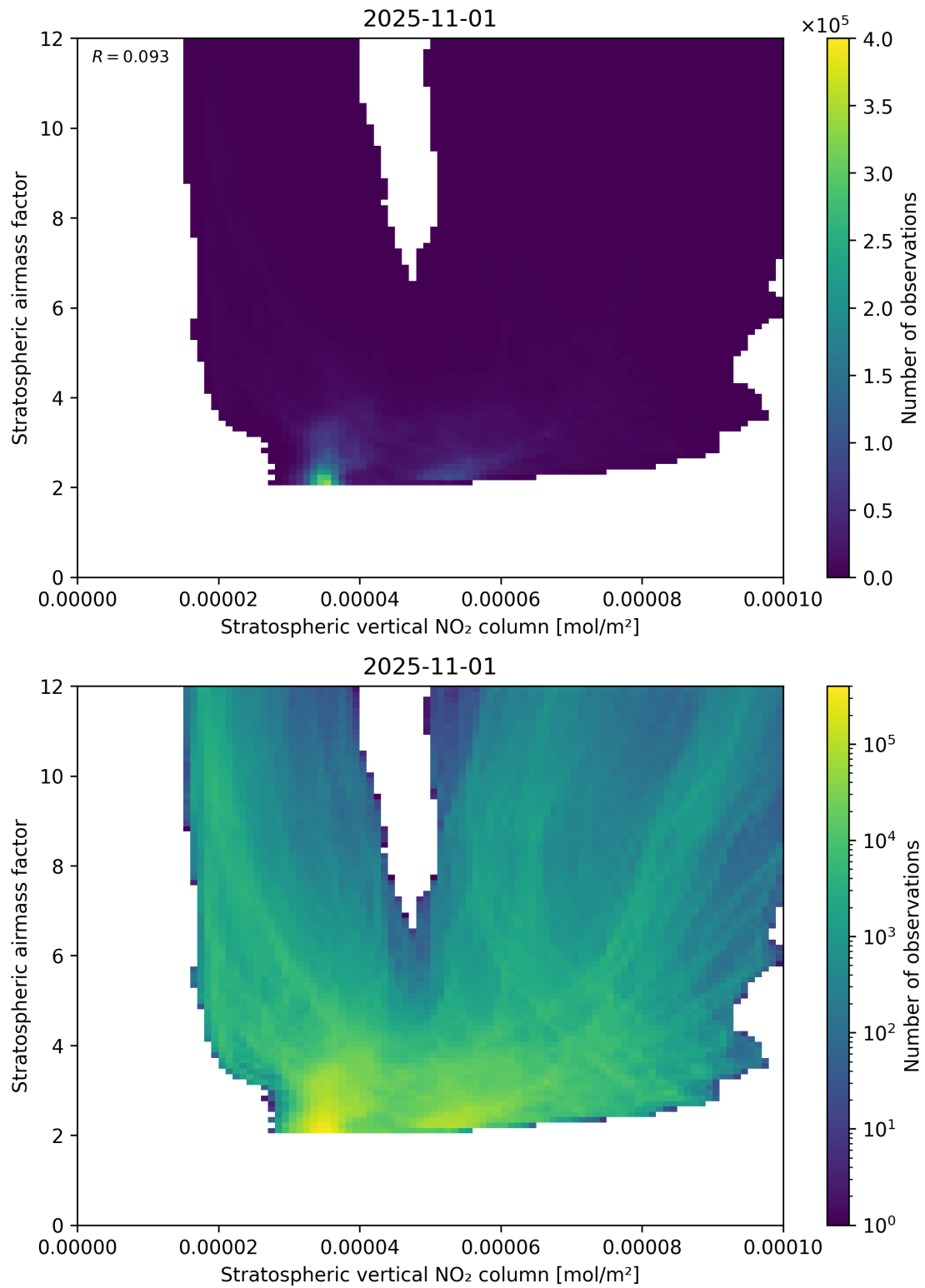
Figure 96: Scatter density plot of “Stratospheric vertical NO 2 column” against “Stratospheric airmass factor” for 2025-10-31 to 2025-11-02.
