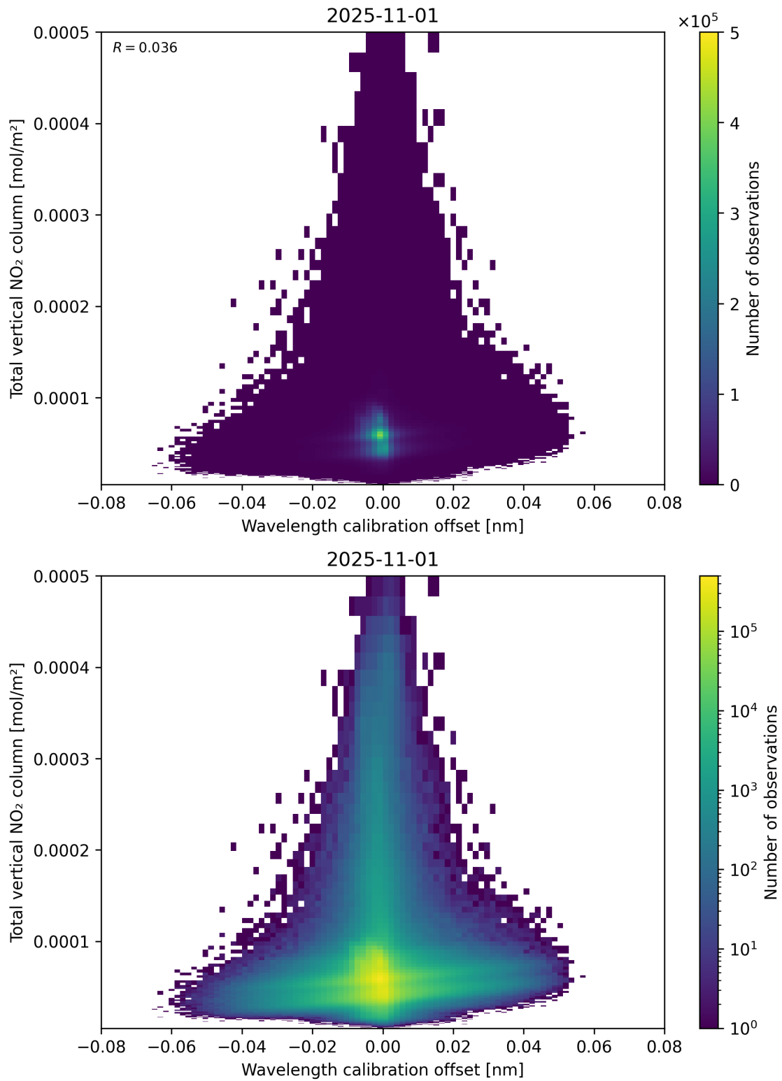
Figure 179: Scatter density plot of “Wavelength calibration offset” against “Total vertical NO 2 column” for 2025-10-31 to 2025-11-02.
