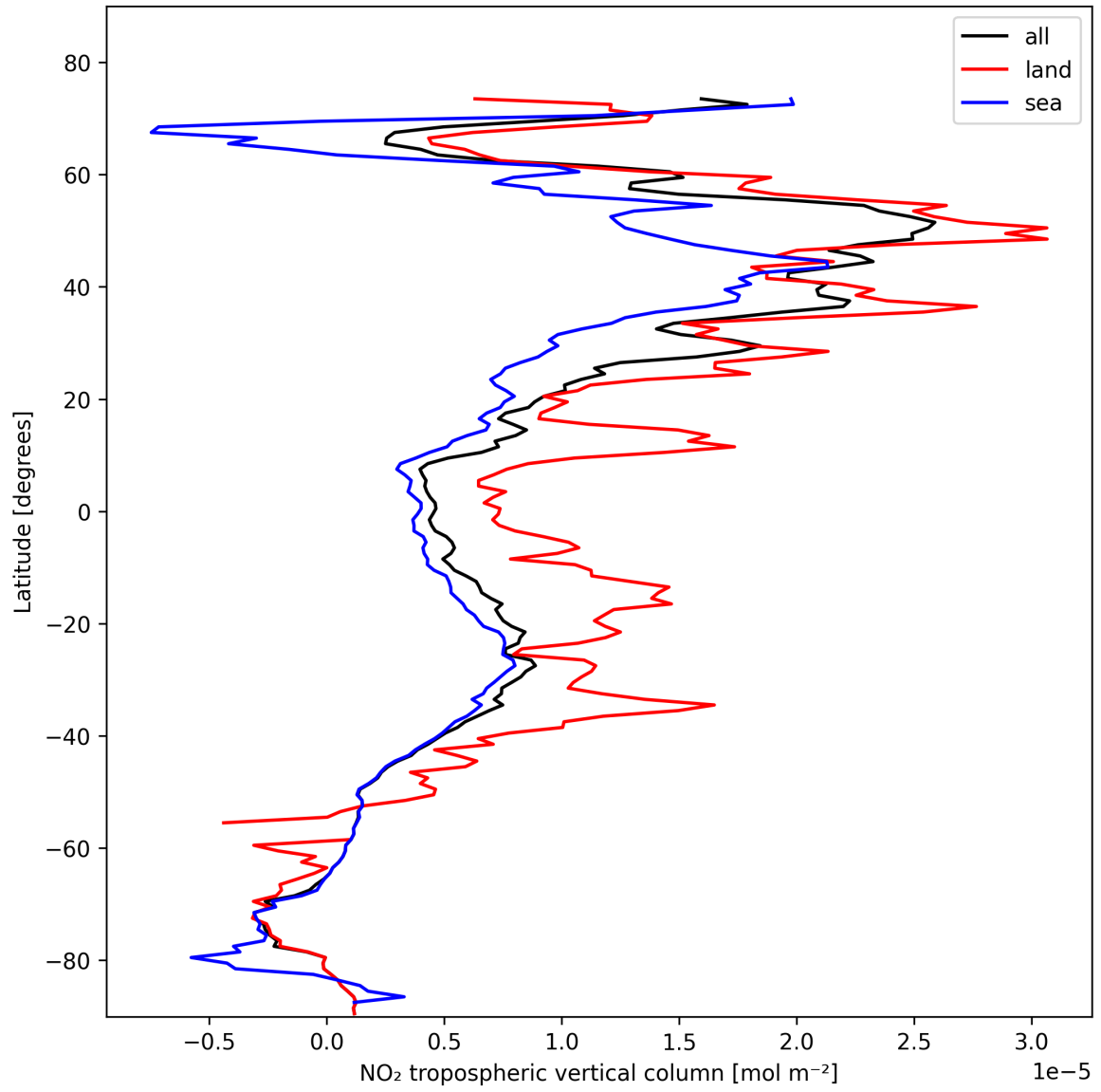
Figure 12: Zonal average of “NO 2 tropospheric vertical column” for 2025-10-31 to 2025-11-02.
