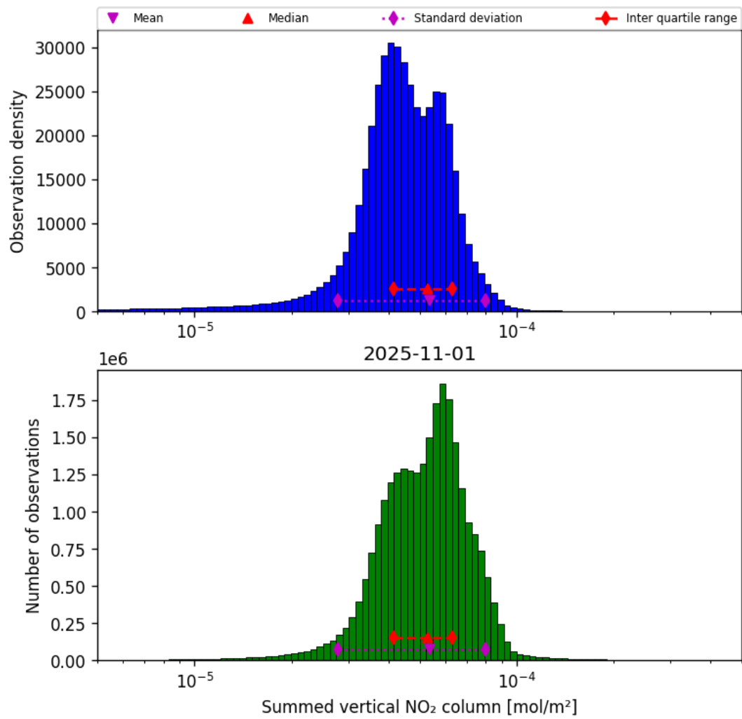
Figure 40: Histogram of “Summed vertical NO 2 column” for 2025-10-31 to 2025-11-02
