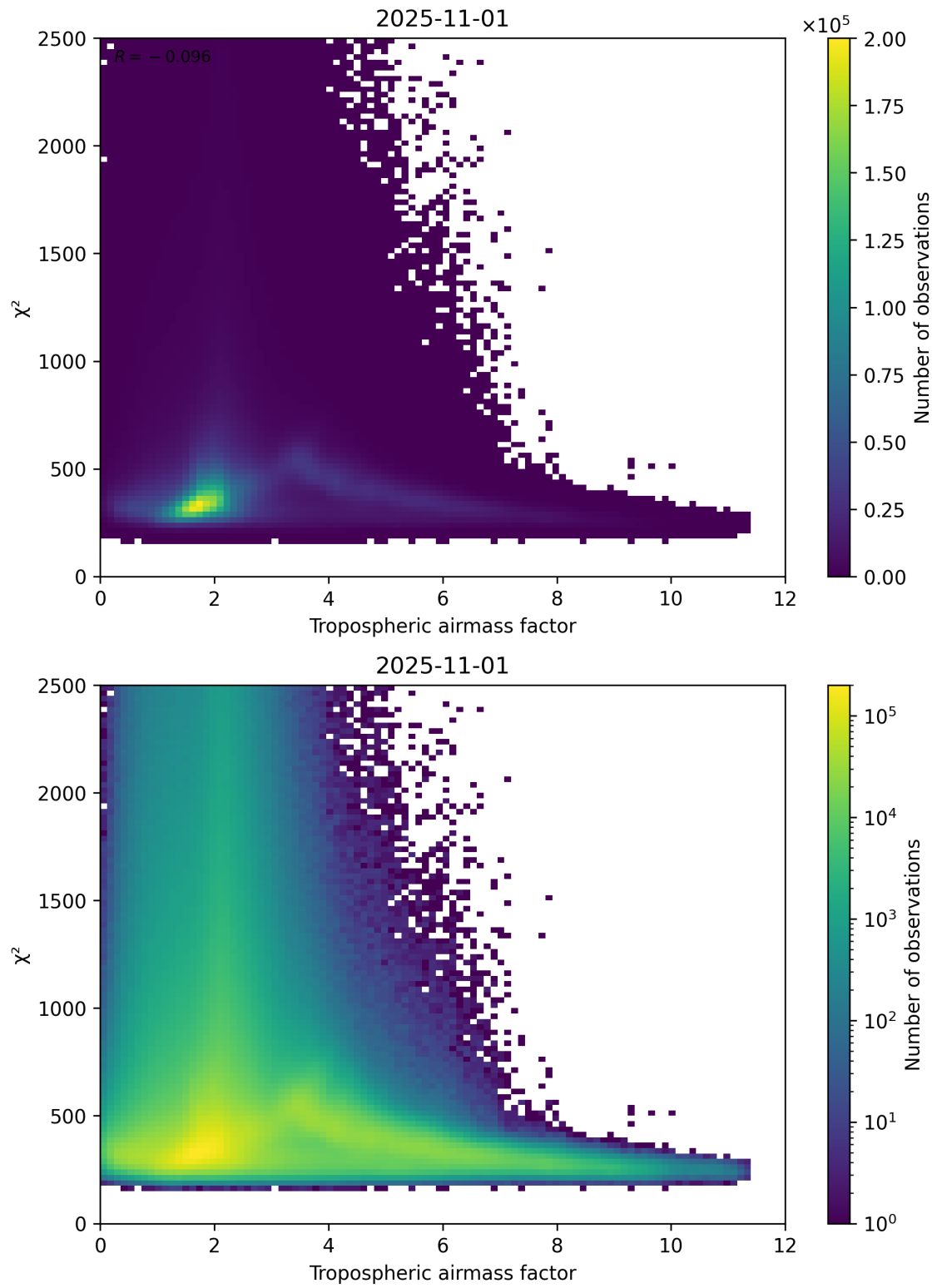
Figure 73: Scatter density plot of “Tropospheric airmass factor” against “ \chi^2 ” for 2025-10-31 to 2025-11-02.
