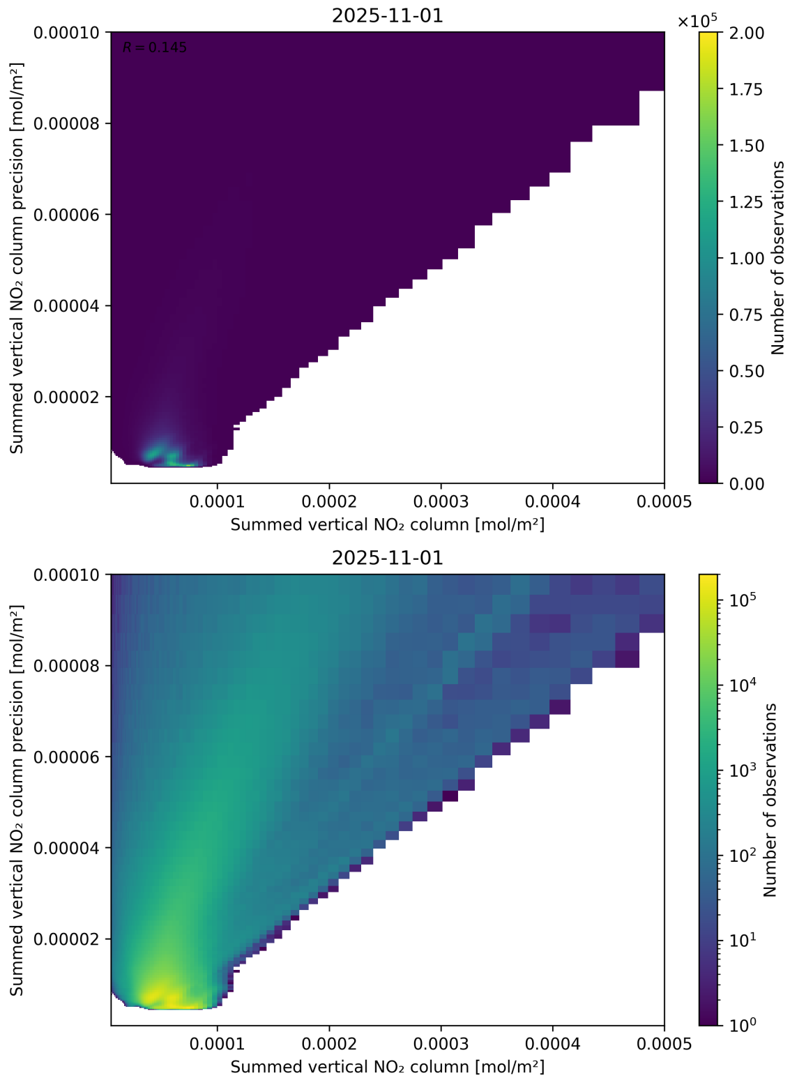
Figure 105: Scatter density plot of “Summed vertical NO 2 column” against “Summed vertical NO 2 column precision” for 2025-10-31 to 2025-11-02.
