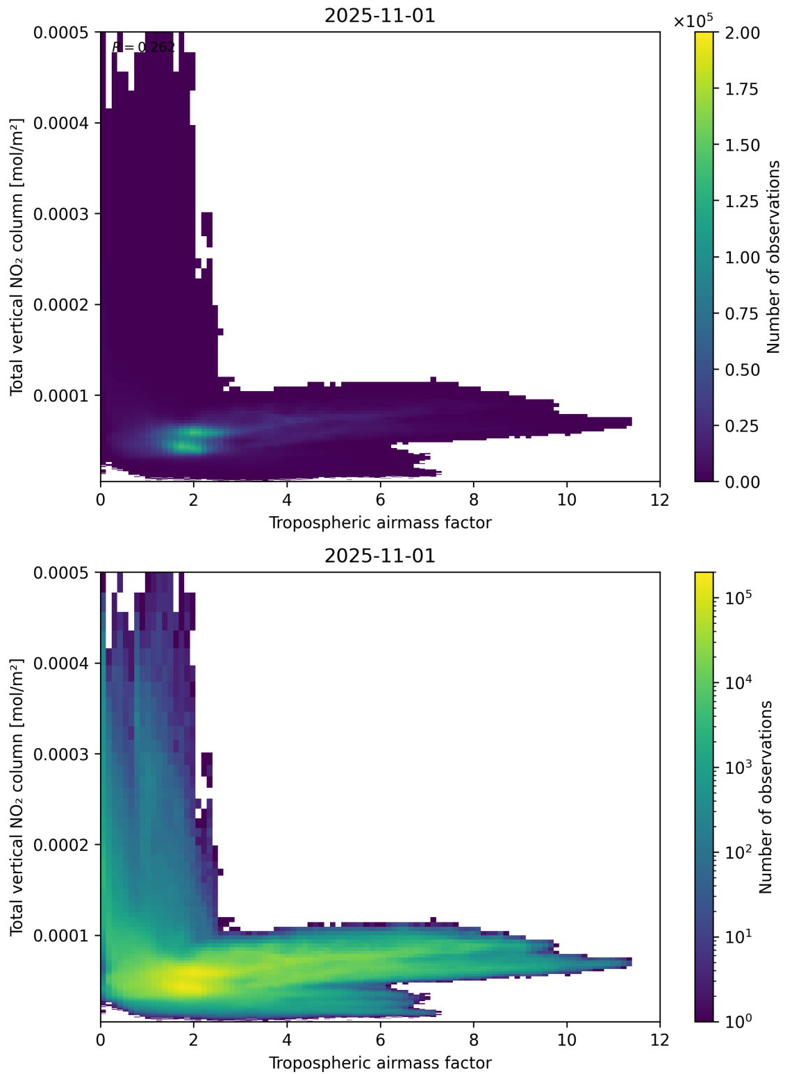
Figure 77: Scatter density plot of “Tropospheric airmass factor” against “Total vertical NO 2 column” for 2025-10-31 to 2025-11-02.
