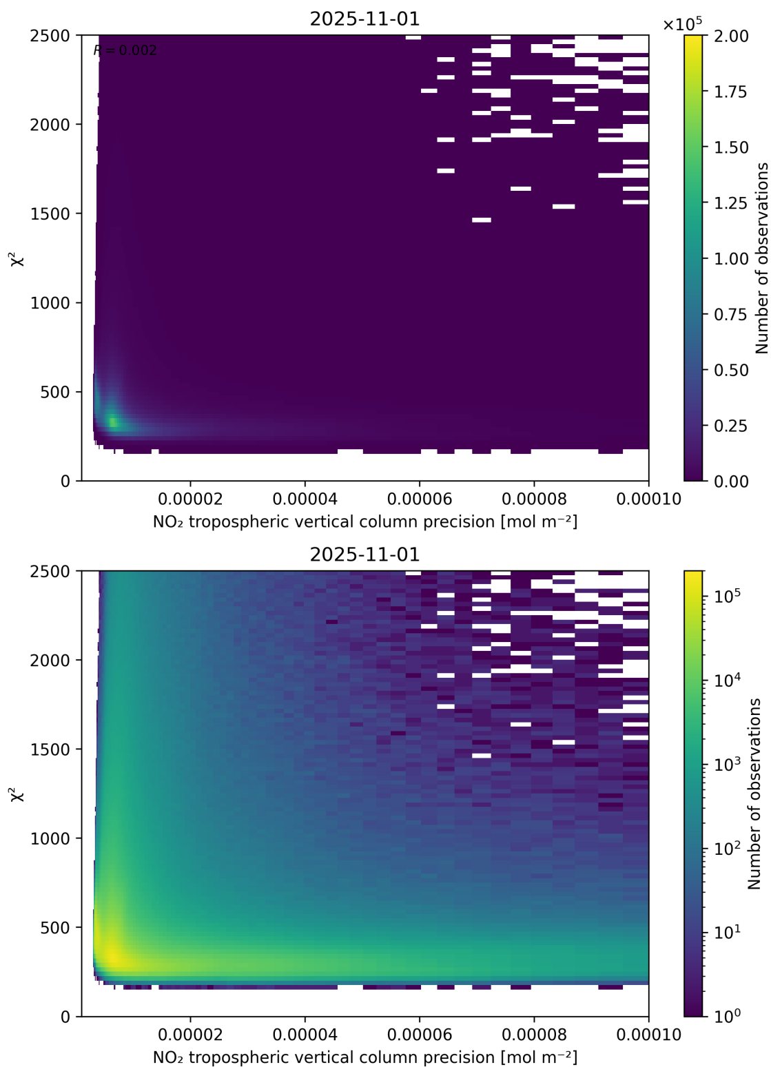
Figure 134: Scatter density plot of “NO 2 tropospheric vertical column precision” against “ \chi^2 ” for 2025-10-31 to 2025-11-02.
