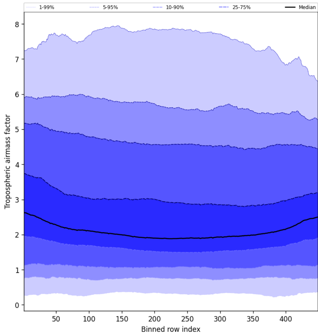
Figure 48: Along track statistics of “Tropospheric airmass factor” for 2025-10-31 to 2025-11-02
