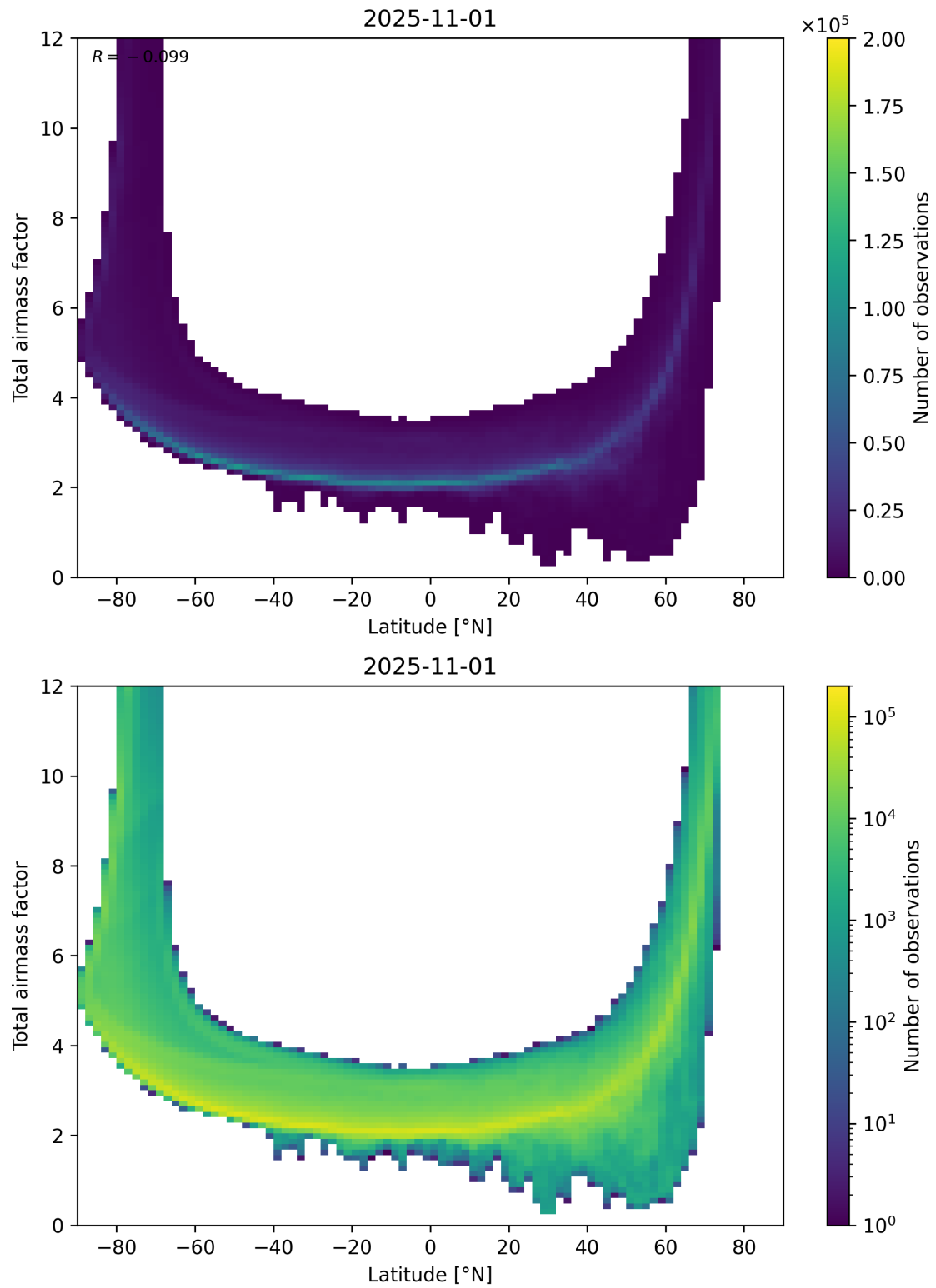
Figure 84: Scatter density plot of “Latitude” against “Total airmass factor” for 2025-10-31 to 2025-11-02.
