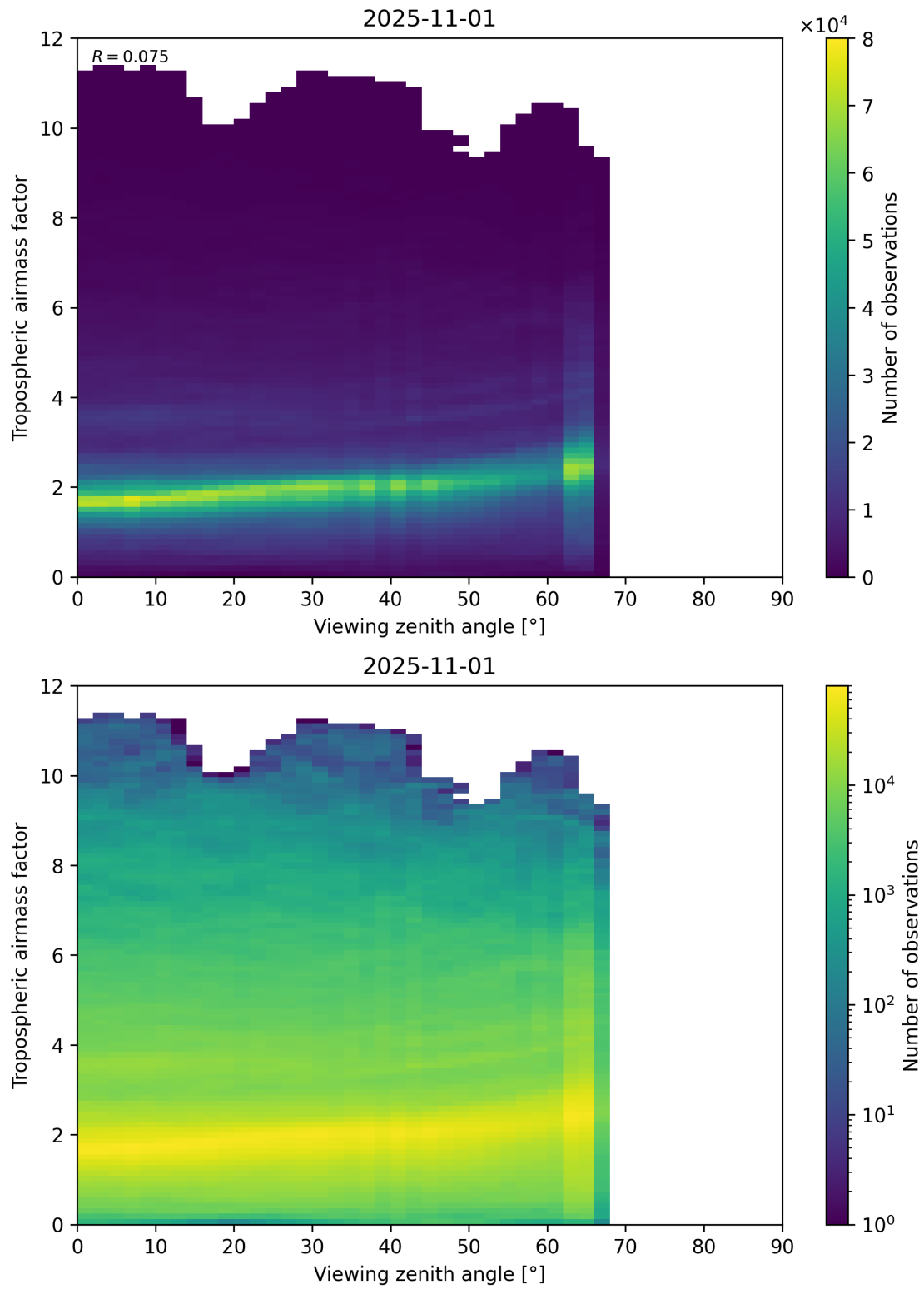
Figure 161: Scatter density plot of “Viewing zenith angle” against “Tropospheric airmass factor” for 2025-10-31 to 2025-11-02.
