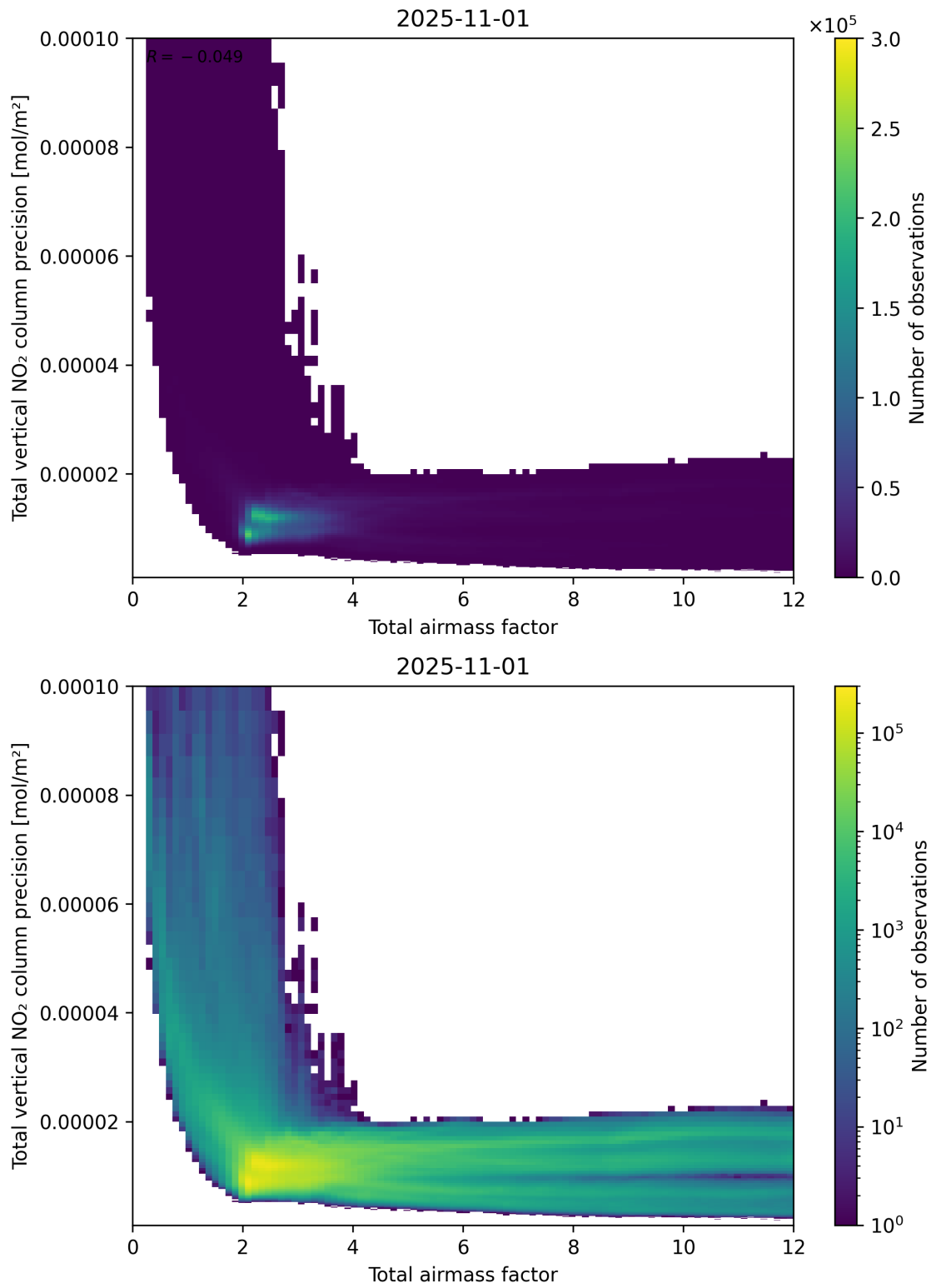
Figure 68: Scatter density plot of “Total airmass factor” against “Total vertical NO 2 column precision” for 2025-10-31 to 2025-11-02.
