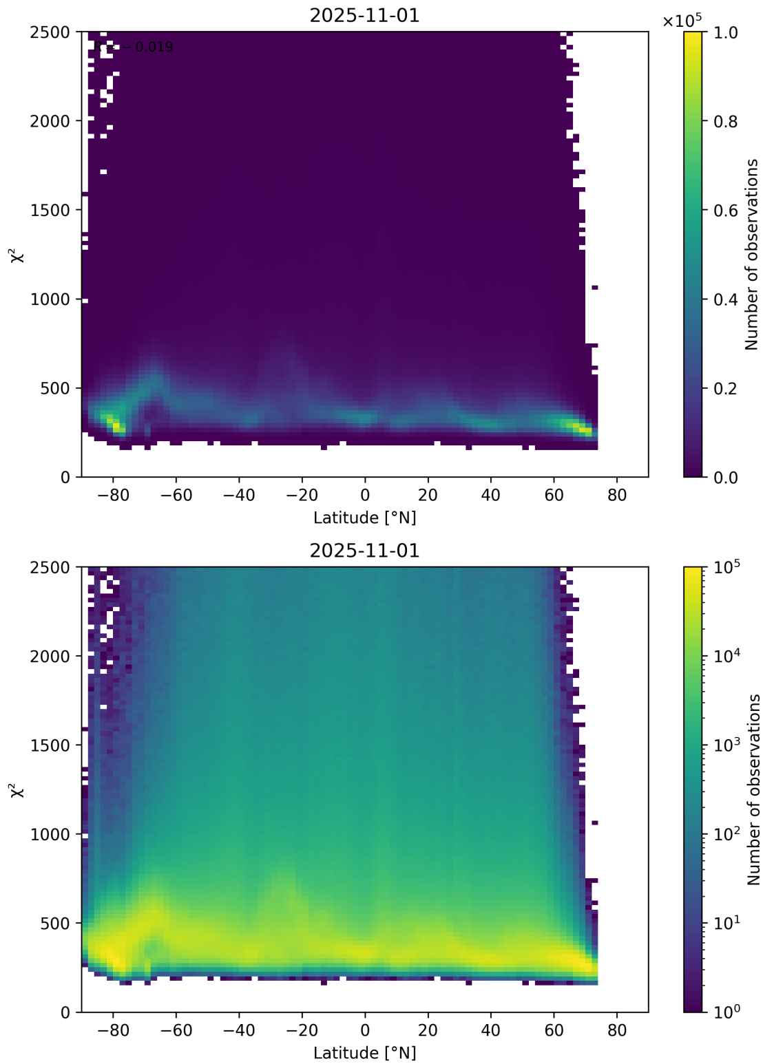
Figure 86: Scatter density plot of “Latitude” against “ \chi^2 ” for 2025-10-31 to 2025-11-02.
