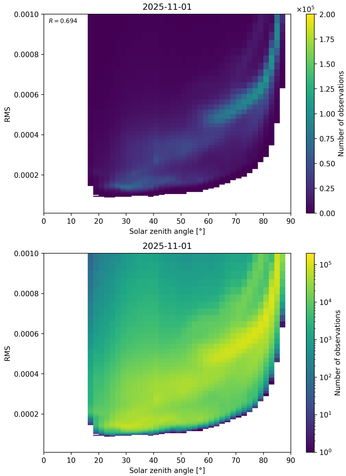
Figure 157: Scatter density plot of “Solar zenith angle” against “RMS” for 2025-10-31 to 2025-11-02.
