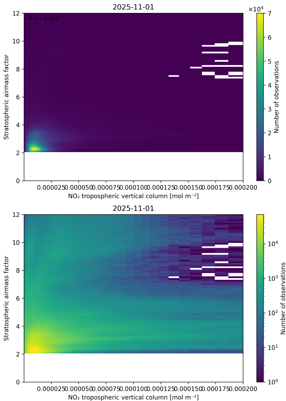
Figure 121: Scatter density plot of “NO 2 tropospheric vertical column” against “Stratospheric airmass factor” for 2025-10-31 to 2025-11-02.
