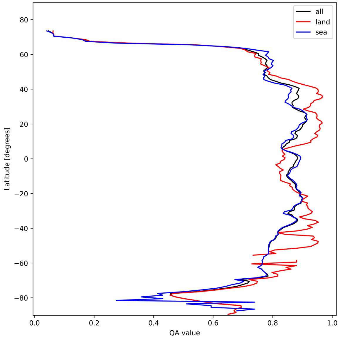
Figure 11: Zonal average of “QA value” for 2025-10-31 to 2025-11-02.
