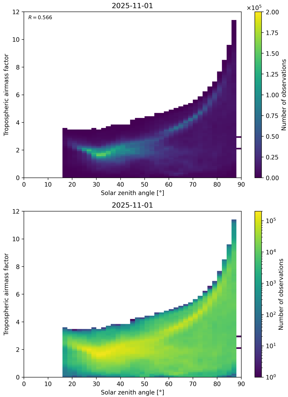
Figure 147: Scatter density plot of “Solar zenith angle” against “Tropospheric airmass factor” for 2025-10-31 to 2025-11-02.
