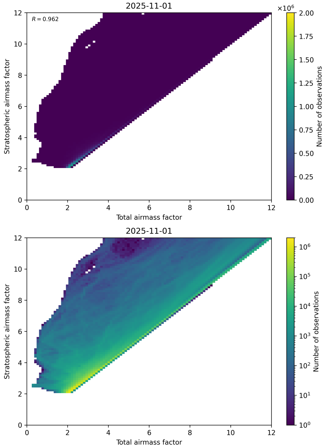
Figure 62: Scatter density plot of “Total airmass factor” against “Stratospheric airmass factor” for 2025-10-31 to 2025-11-02.
