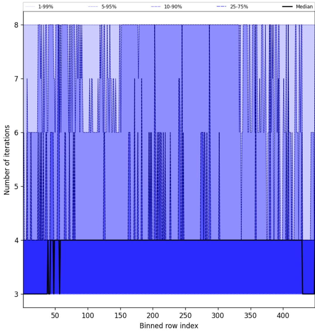
Figure 51: Along track statistics of “Number of iterations” for 2025-10-31 to 2025-11-02
