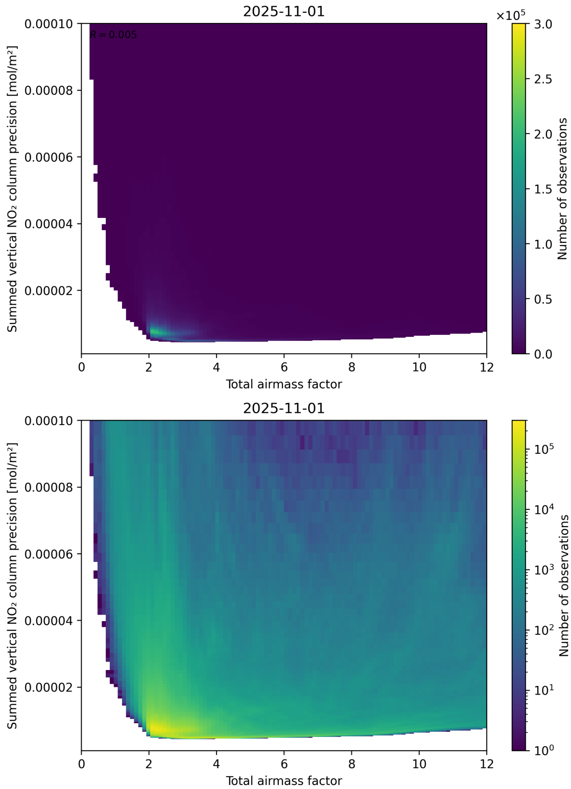
Figure 66: Scatter density plot of “Total airmass factor” against “Summed vertical NO 2 column precision” for 2025-10-31 to 2025-11-02.
