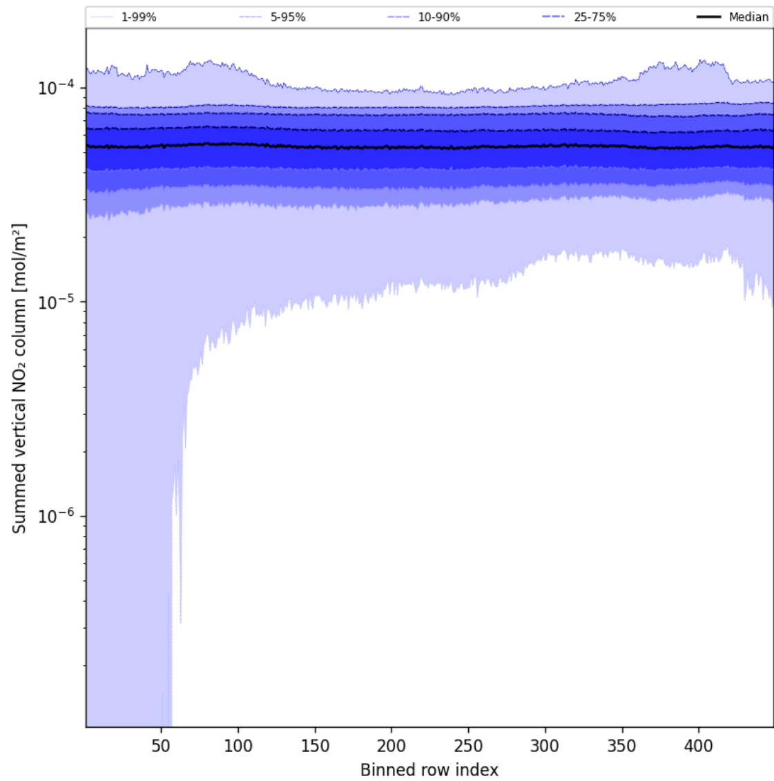
Figure 57: Along track statistics of “Summed vertical NO 2 column” for 2025-10-31 to 2025-11-02
