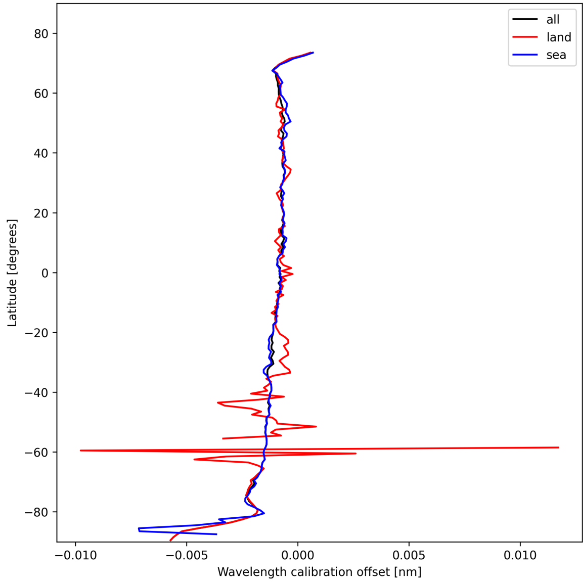
Figure 18: Zonal average of “Wavelength calibration offset” for 2025-10-31 to 2025-11-02.
