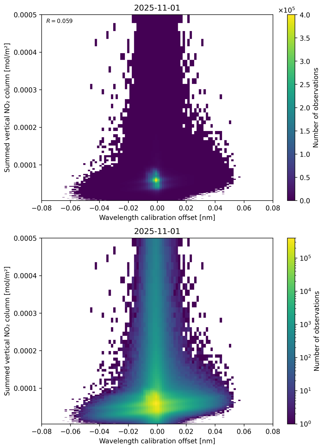
Figure 177: Scatter density plot of “Wavelength calibration offset” against “Summed vertical NO 2 column” for 2025-10-31 to 2025-11-02.
