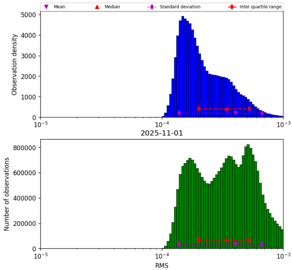
Figure 43: Histogram of “RMS” for 2025-10-31 to 2025-11-02
