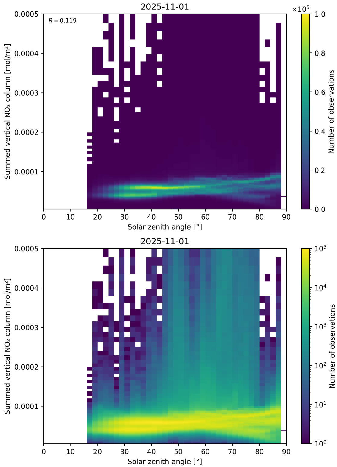
Figure 151: Scatter density plot of “Solar zenith angle” against “Summed vertical NO 2 column” for 2025-10-31 to 2025-11-02.
