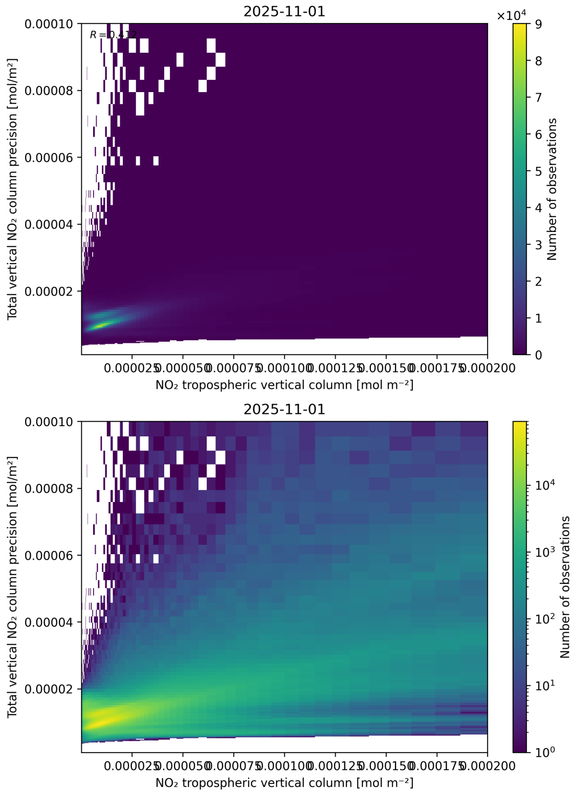
Figure 129: Scatter density plot of “NO 2 tropospheric vertical column” against “Total vertical NO 2 column precision” for 2025-10-31 to 2025-11-02.
