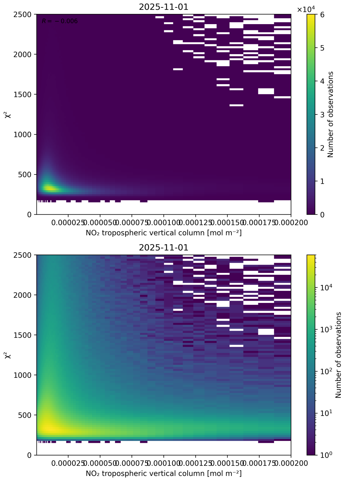
Figure 124: Scatter density plot of “NO 2 tropospheric vertical column” against “ \chi^2 ” for 2025-10-31 to 2025-11-02.
