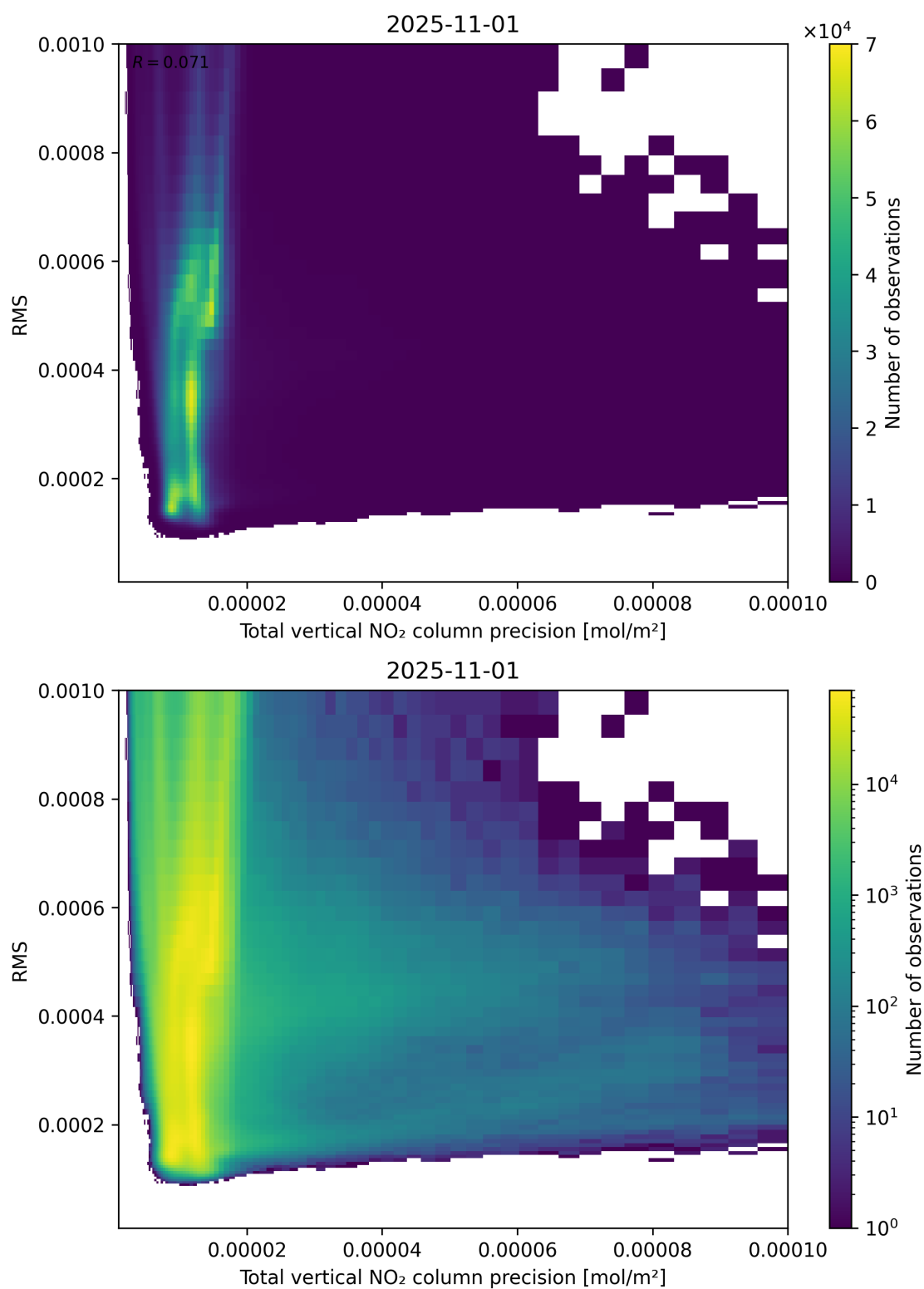
Figure 119: Scatter density plot of “Total vertical NO 2 column precision” against “RMS” for 2025-10-31 to 2025-11-02.
