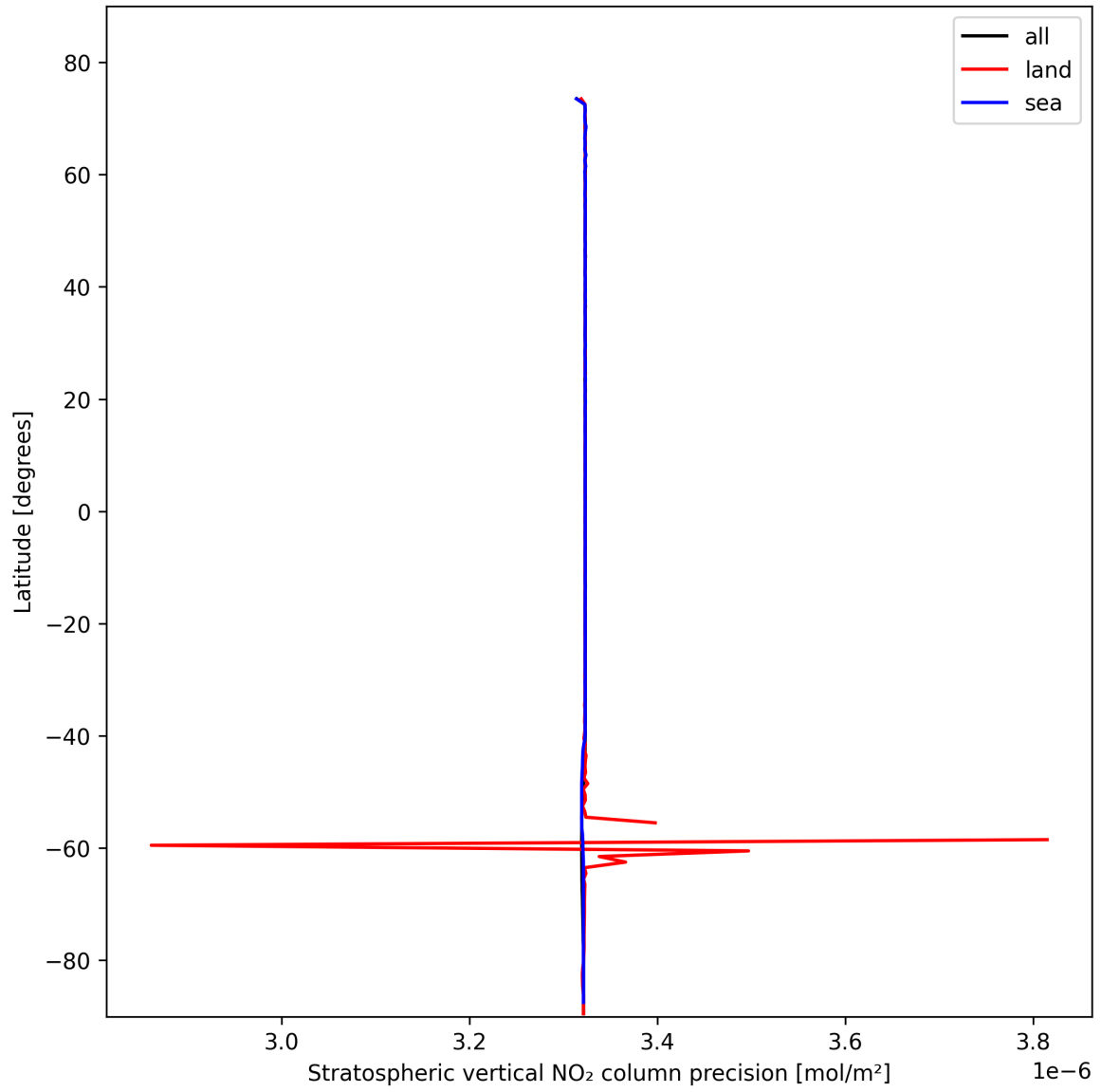
Figure 20: Zonal average of “Stratospheric vertical NO 2 column precision” for 2025-10-31 to 2025-11-02.
