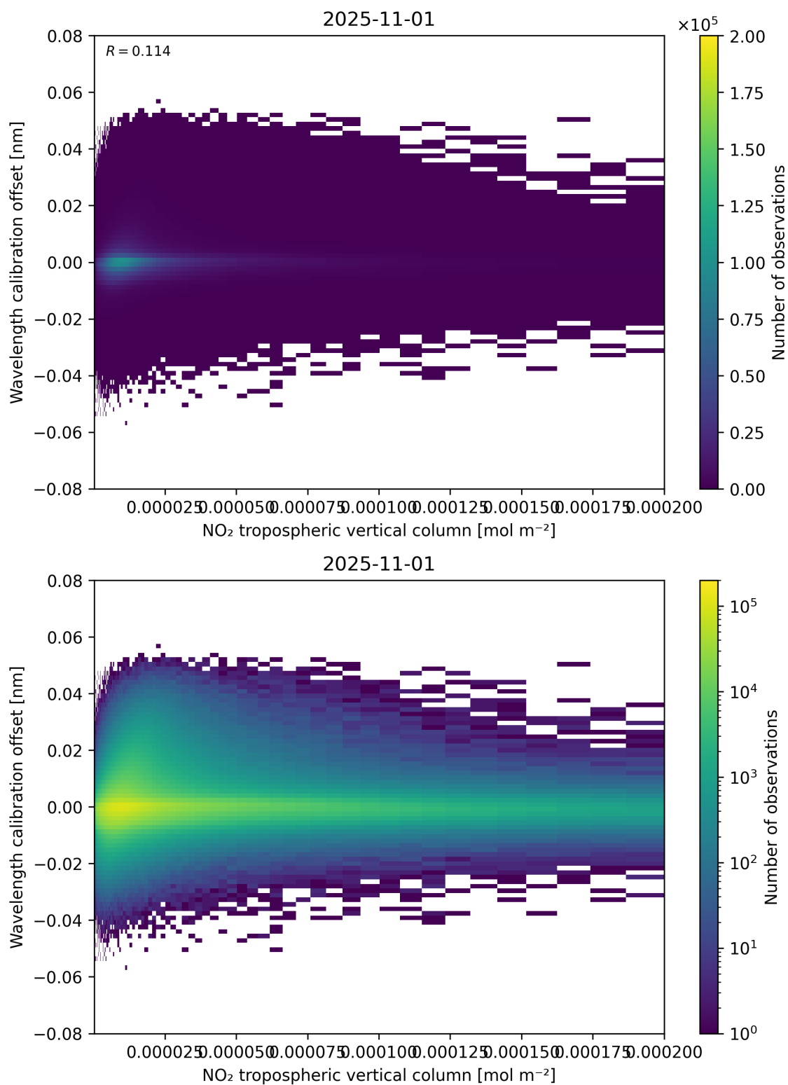
Figure 143: Scatter density plot of “NO 2 tropospheric vertical column” against “Wavelength calibration offset” for 2025-10-31 to 2025-11-02.
