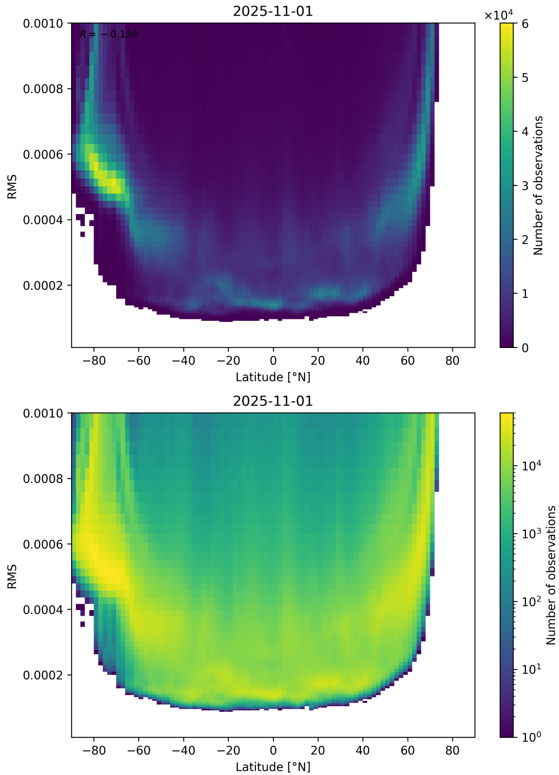
Figure 94: Scatter density plot of “Latitude” against “RMS” for 2025-10-31 to 2025-11-02.
