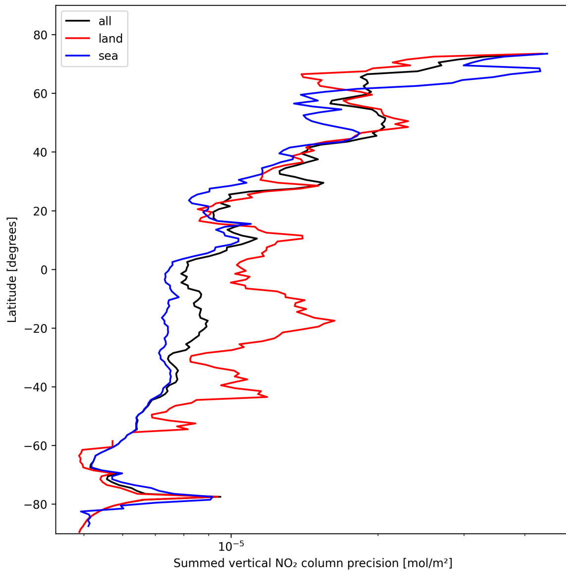
Figure 24: Zonal average of “Summed vertical NO 2 column precision” for 2025-10-31 to 2025-11-02.
