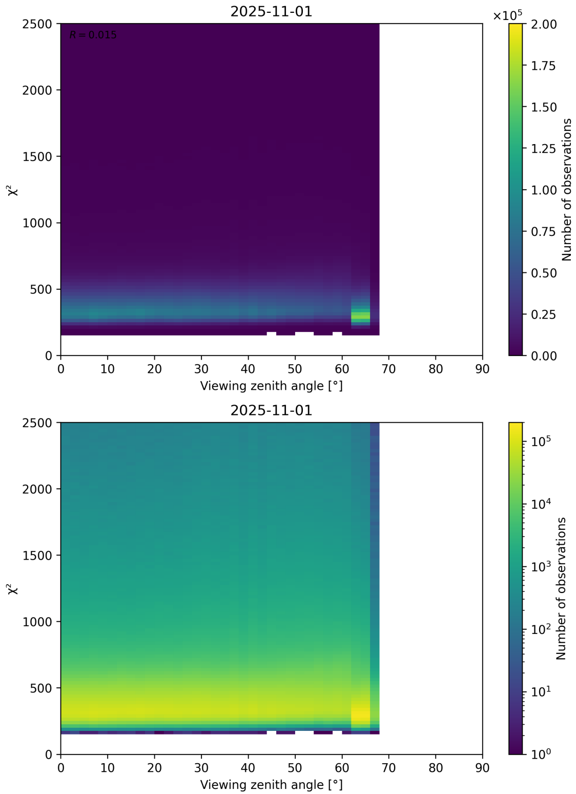
Figure 162: Scatter density plot of “Viewing zenith angle” against “ \chi^2 ” for 2025-10-31 to 2025-11-02.
