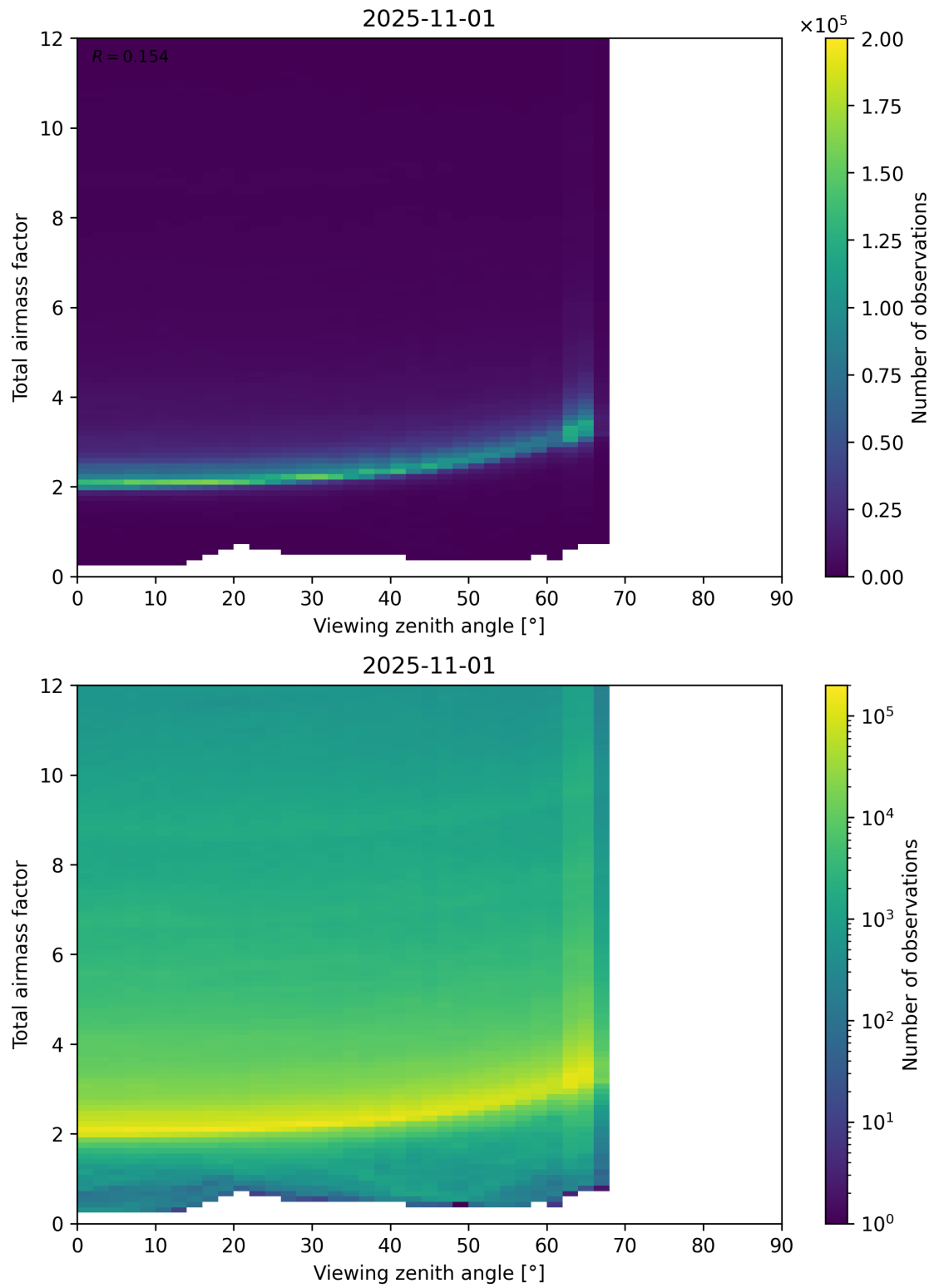
Figure 160: Scatter density plot of “Viewing zenith angle” against “Total airmass factor” for 2025-10-31 to 2025-11-02.
