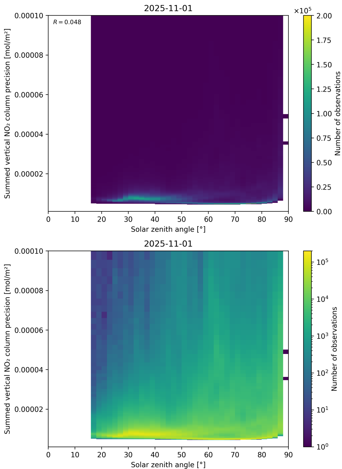
Figure 152: Scatter density plot of “Solar zenith angle” against “Summed vertical NO 2 column precision” for 2025-10-31 to 2025-11-02.
