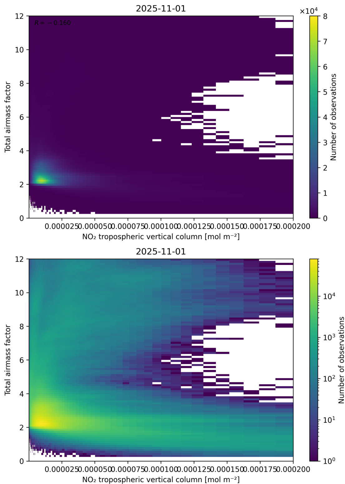
Figure 122: Scatter density plot of “NO 2 tropospheric vertical column” against “Total air mass factor” for 2025-10-31 to 2025-11-02.
