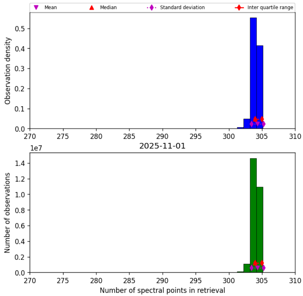
Figure 33: Histogram of “Number of spectral points in retrieval” for 2025-10-31 to 2025-11-02
