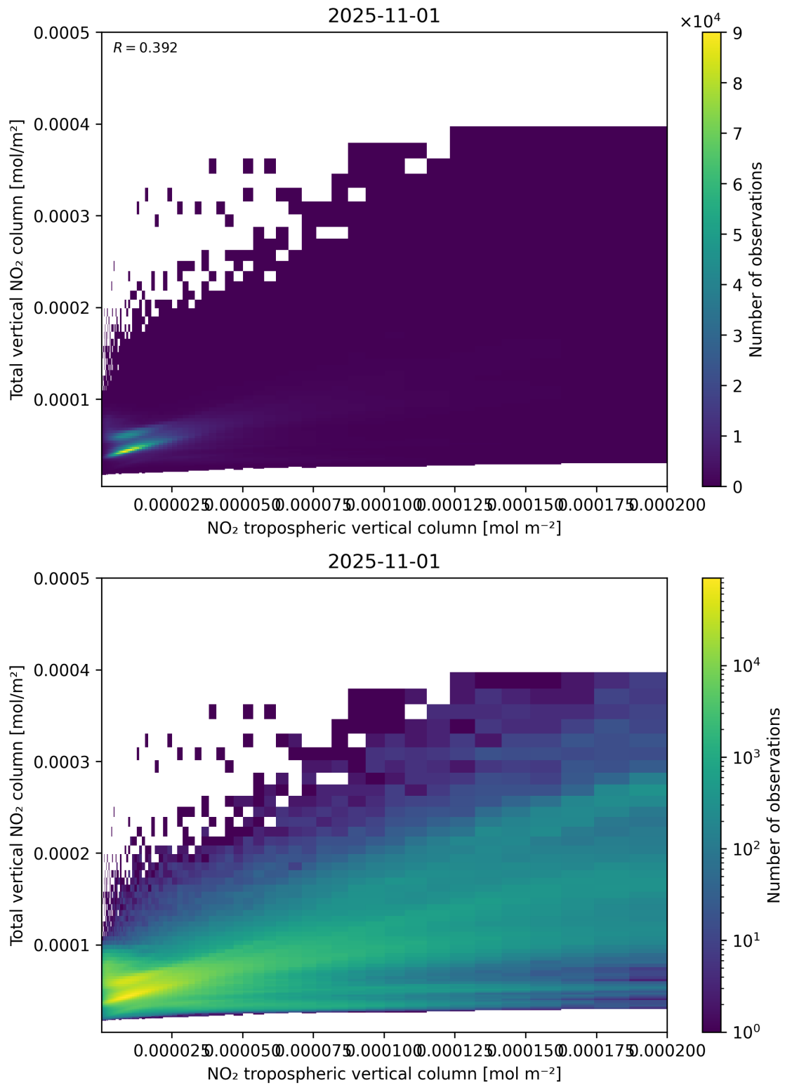
Figure 128: Scatter density plot of “NO 2 tropospheric vertical column” against “Total vertical NO 2 column” for 2025-10-31 to 2025-11-02.
