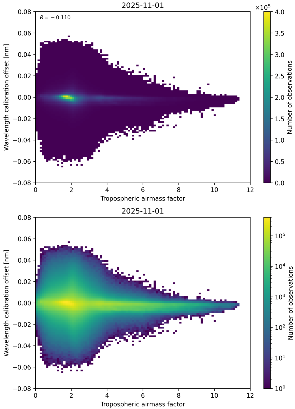
Figure 80: Scatter density plot of “Tropospheric airmass factor” against “Wavelength calibration offset” for 2025-10-31 to 2025-11-02.
