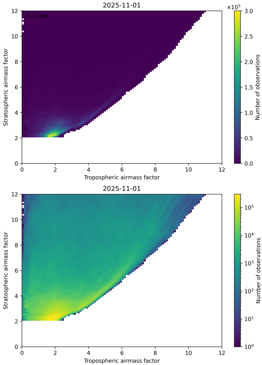
Figure 71: Scatter density plot of “Tropospheric airmass factor” against “Stratospheric airmass factor” for 2025-10-31 to 2025-11-02.
