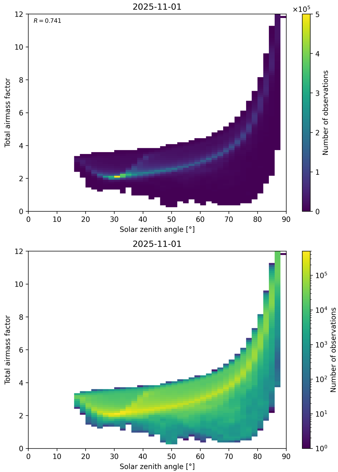
Figure 146: Scatter density plot of “Solar zenith angle” against “Total airmass factor” for 2025-10-31 to 2025-11-02.
