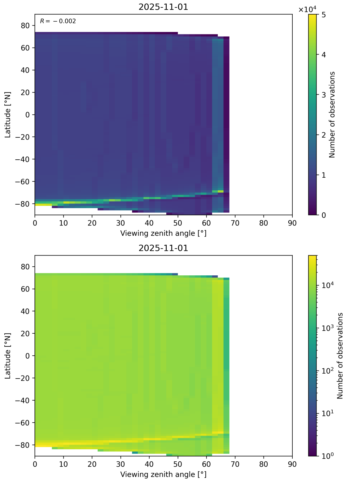
Figure 163: Scatter density plot of “Viewing zenith angle” against “Latitude” for 2025-10-31 to 2025-11-02.
