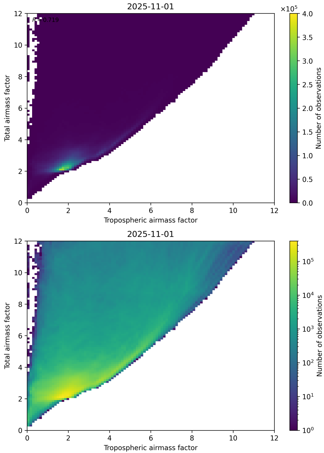
Figure 72: Scatter density plot of “Tropospheric airmass factor” against “Total airmass factor” for 2025-10-31 to 2025-11-02.
