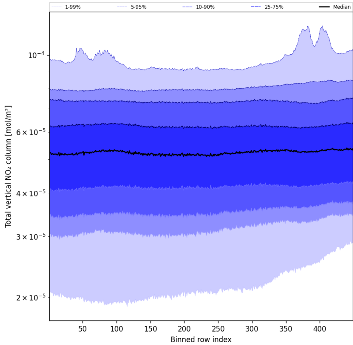
Figure 55: Along track statistics of “Total vertical NO 2 column” for 2025-10-31 to 2025-11-02
