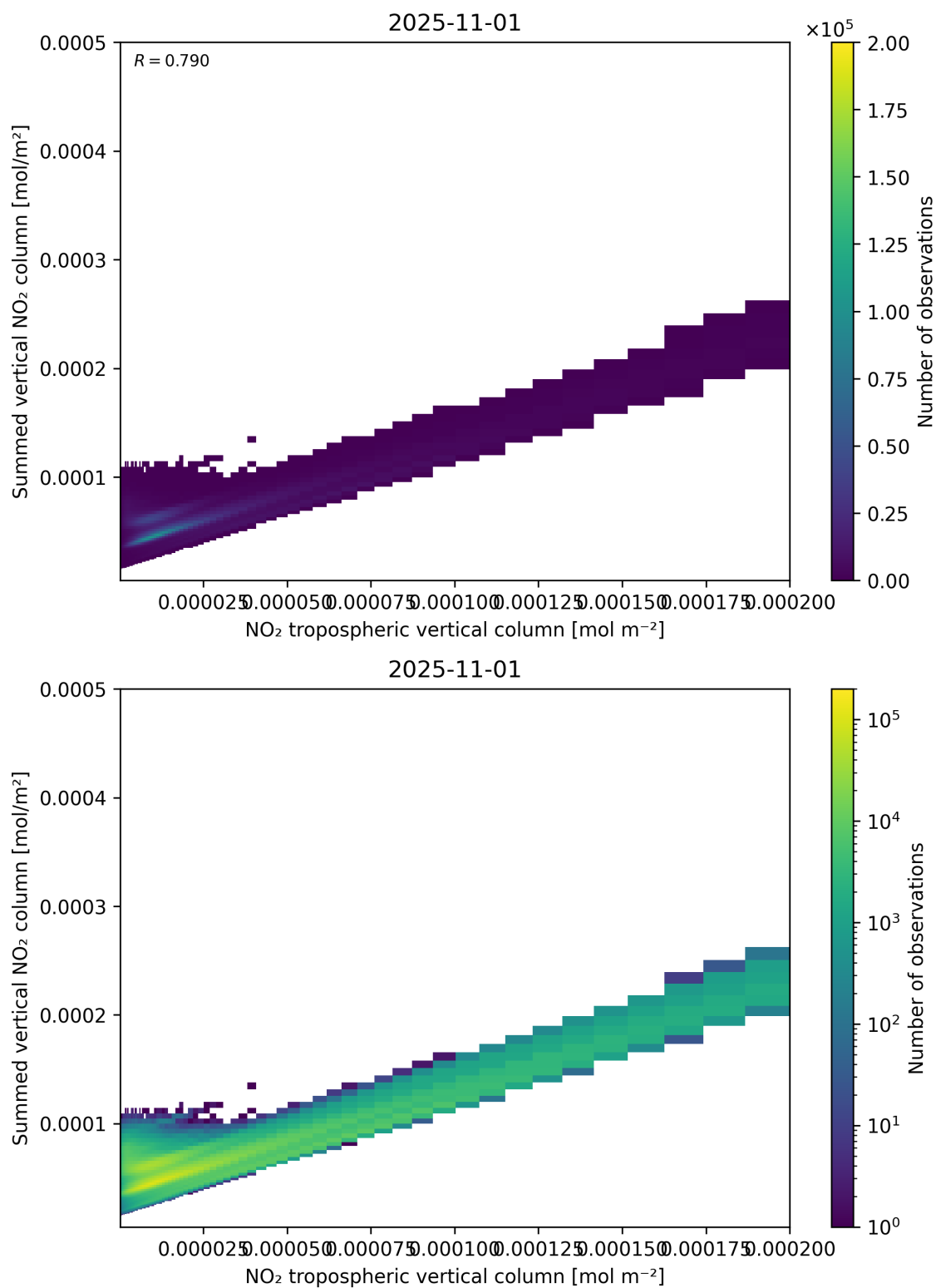
Figure 126: Scatter density plot of “NO 2 tropospheric vertical column” against “Summed vertical NO 2 column” for 2025-10-31 to 2025-11-02.
