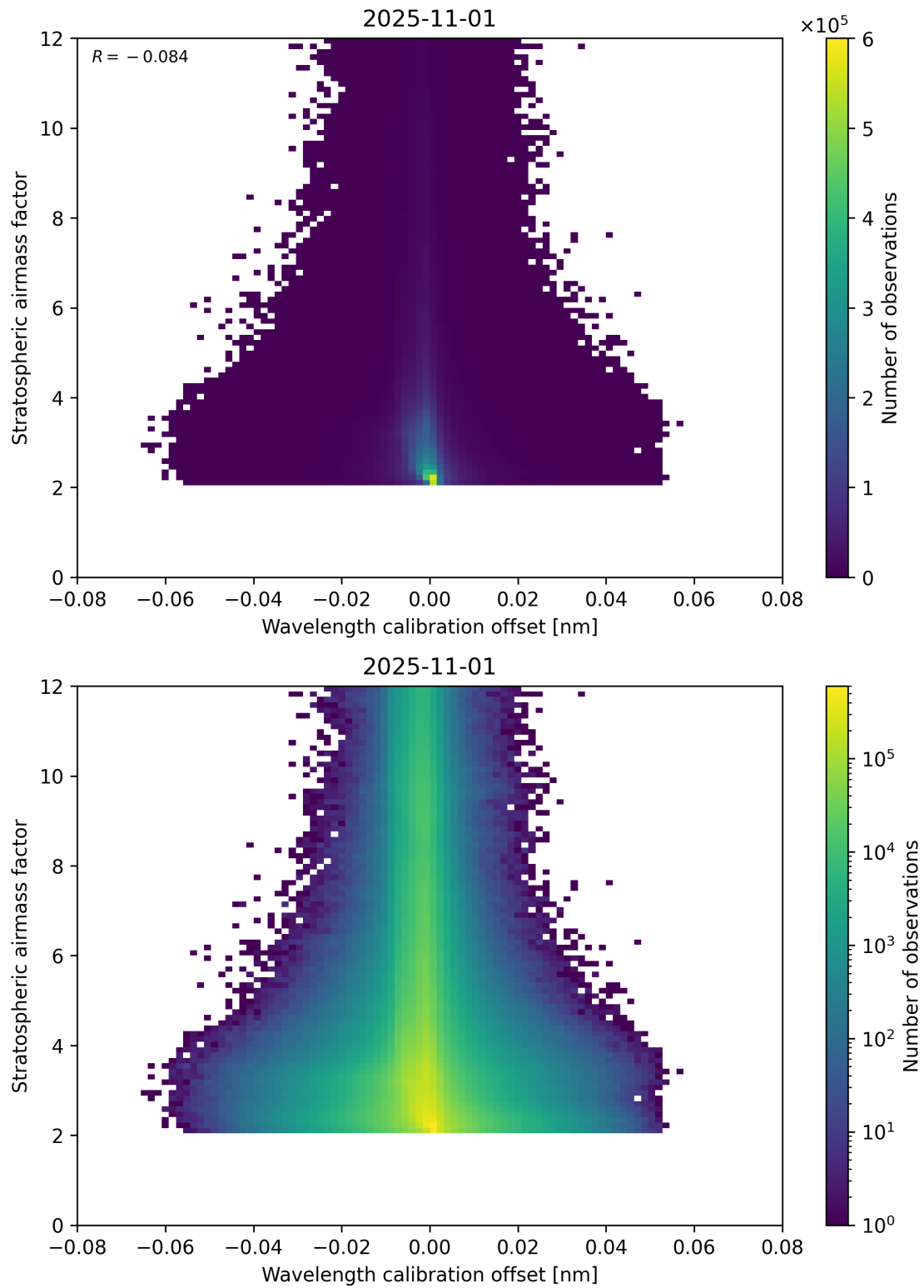
Figure 174: Scatter density plot of “Wavelength calibration offset” against “Stratospheric air mass factor” for 2025-10-31 to 2025-11-02.
