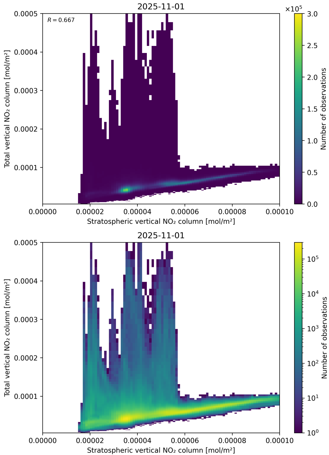
Figure 100: Scatter density plot of “Stratospheric vertical NO 2 column” against “Total vertical NO 2 column” for 2025-10-31 to 2025-11-02.
