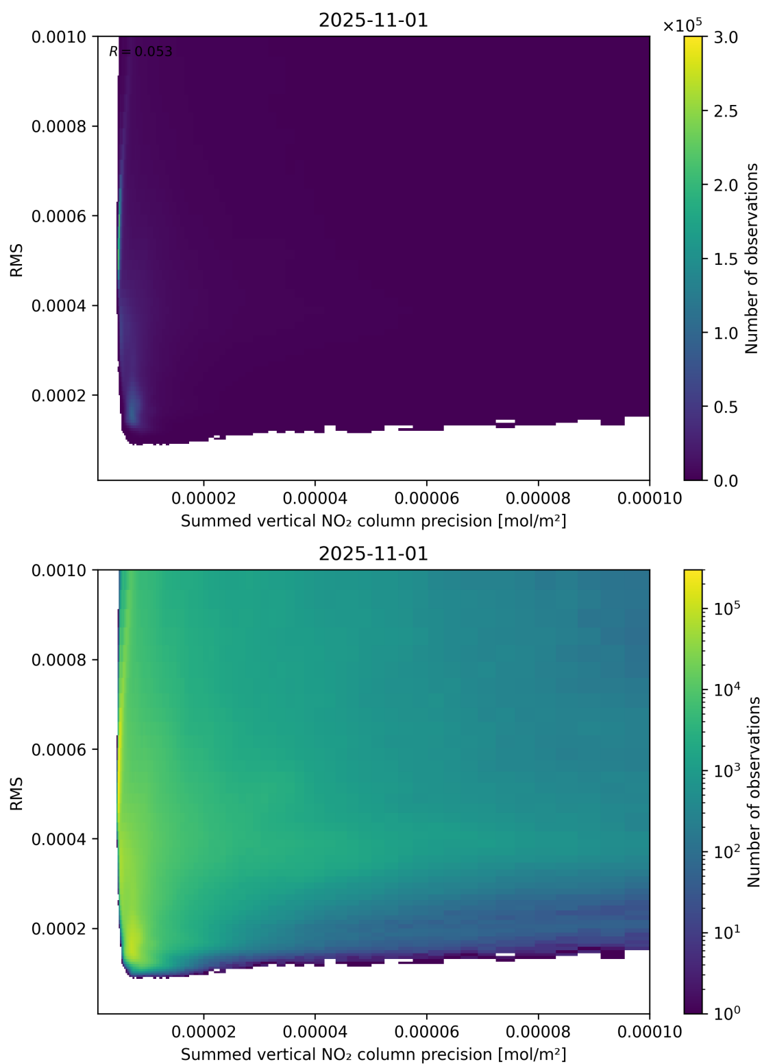
Figure 108: Scatter density plot of “Summed vertical NO 2 column precision” against “RMS” for 2025-10-31 to 2025-11-02.
