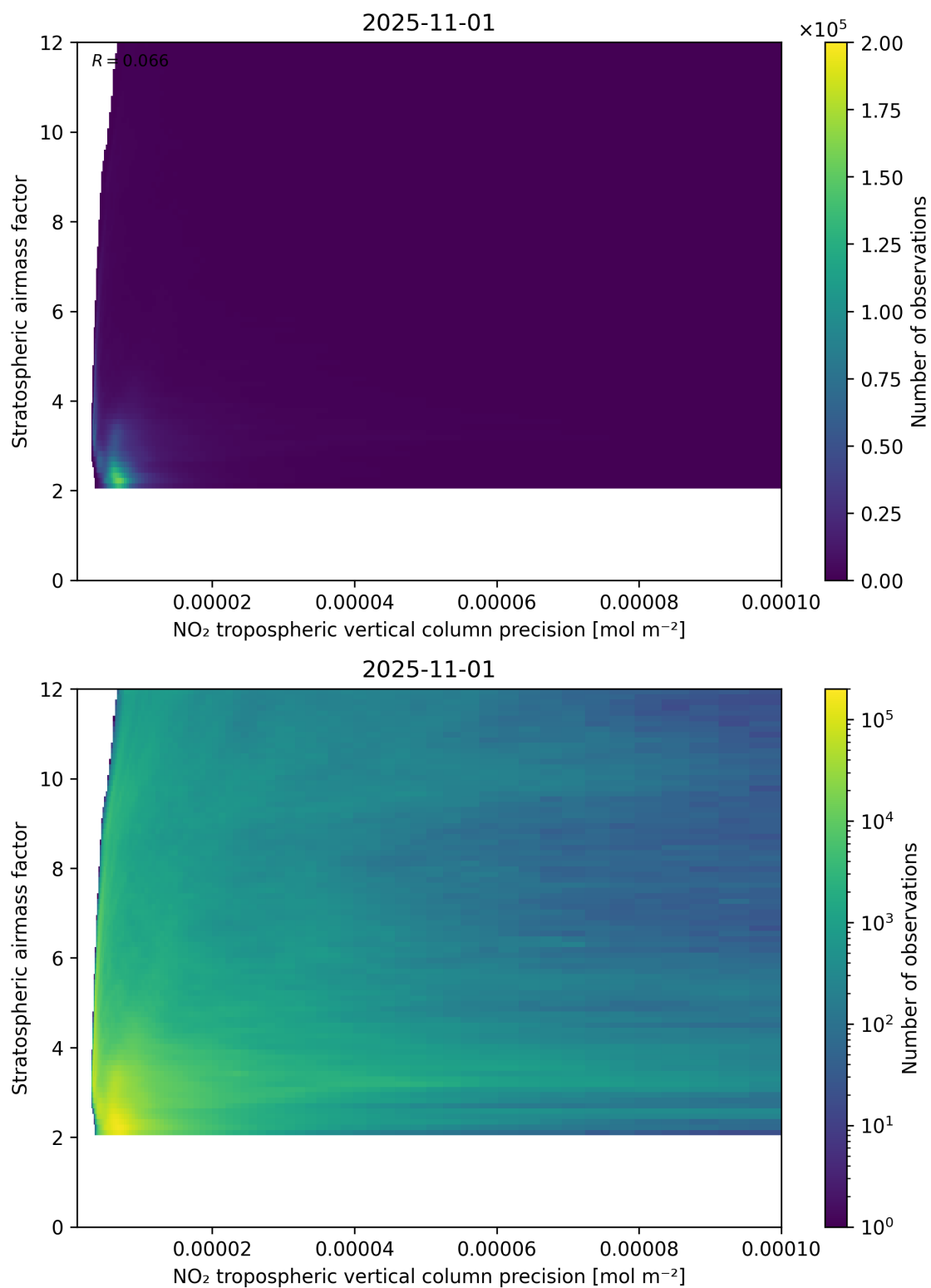
Figure 131: Scatter density plot of “NO 2 tropospheric vertical column precision” against “Stratospheric airmass factor” for 2025-10-31 to 2025-11-02.
