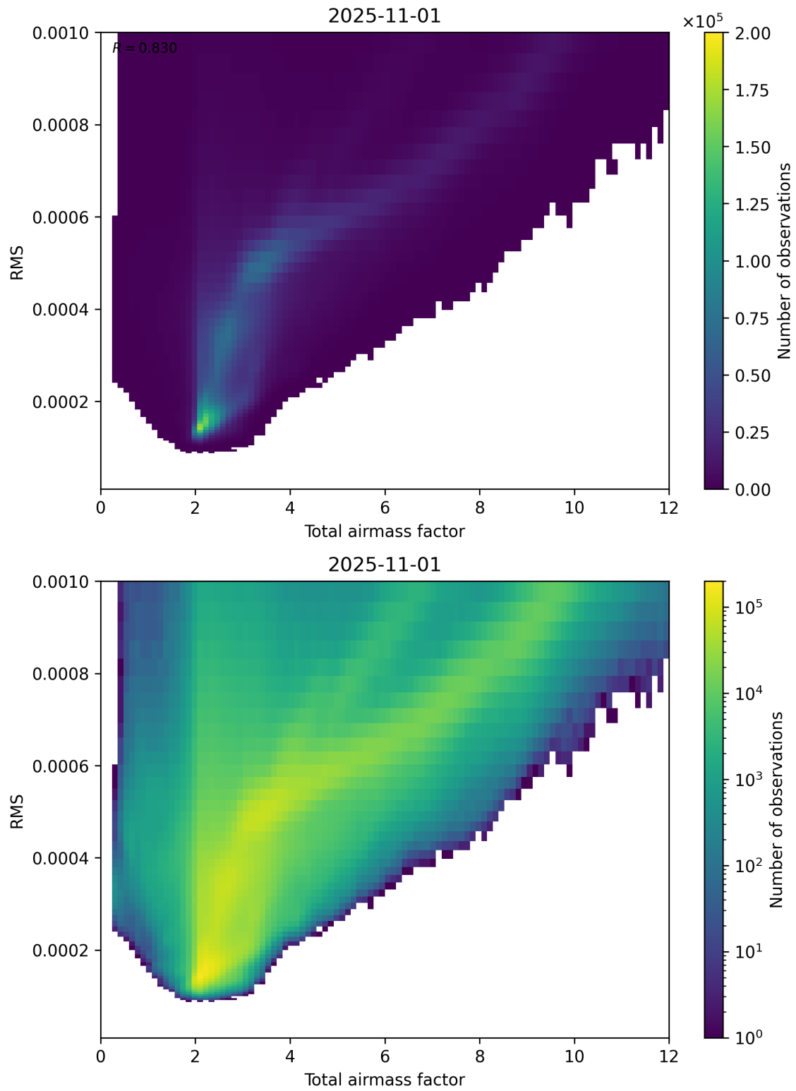
Figure 69: Scatter density plot of “Total airmass factor” against “RMS” for 2025-10-31 to 2025-11-02.
