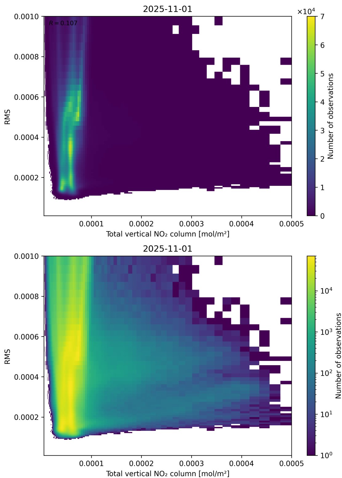
Figure 120: Scatter density plot of “Total vertical NO 2 column” against “RMS” for 2025-10-31 to 2025-11-02.
