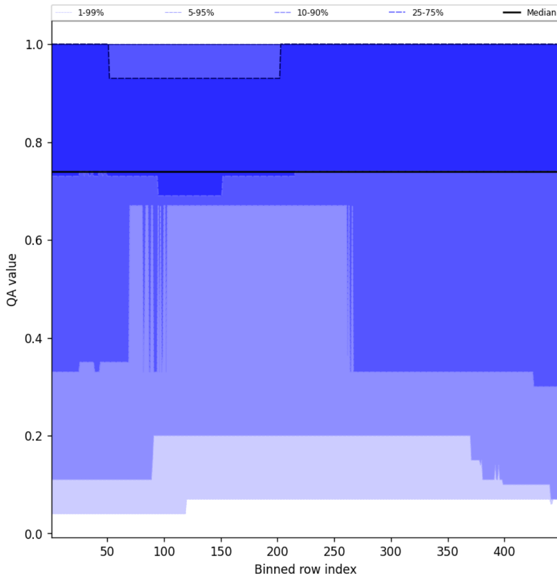
Figure 45: Along track statistics of “QA value” for 2025-10-31 to 2025-11-02
