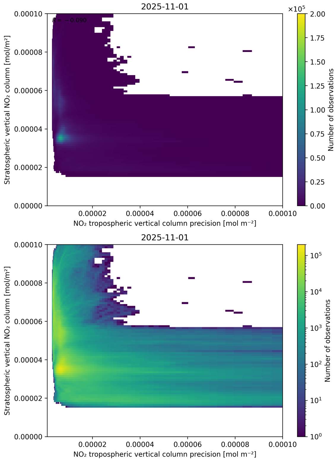
Figure 135: Scatter density plot of “NO 2 tropospheric vertical column precision” against “Stratospheric vertical NO 2 column” for 2025-10-31 to 2025-11-02.
