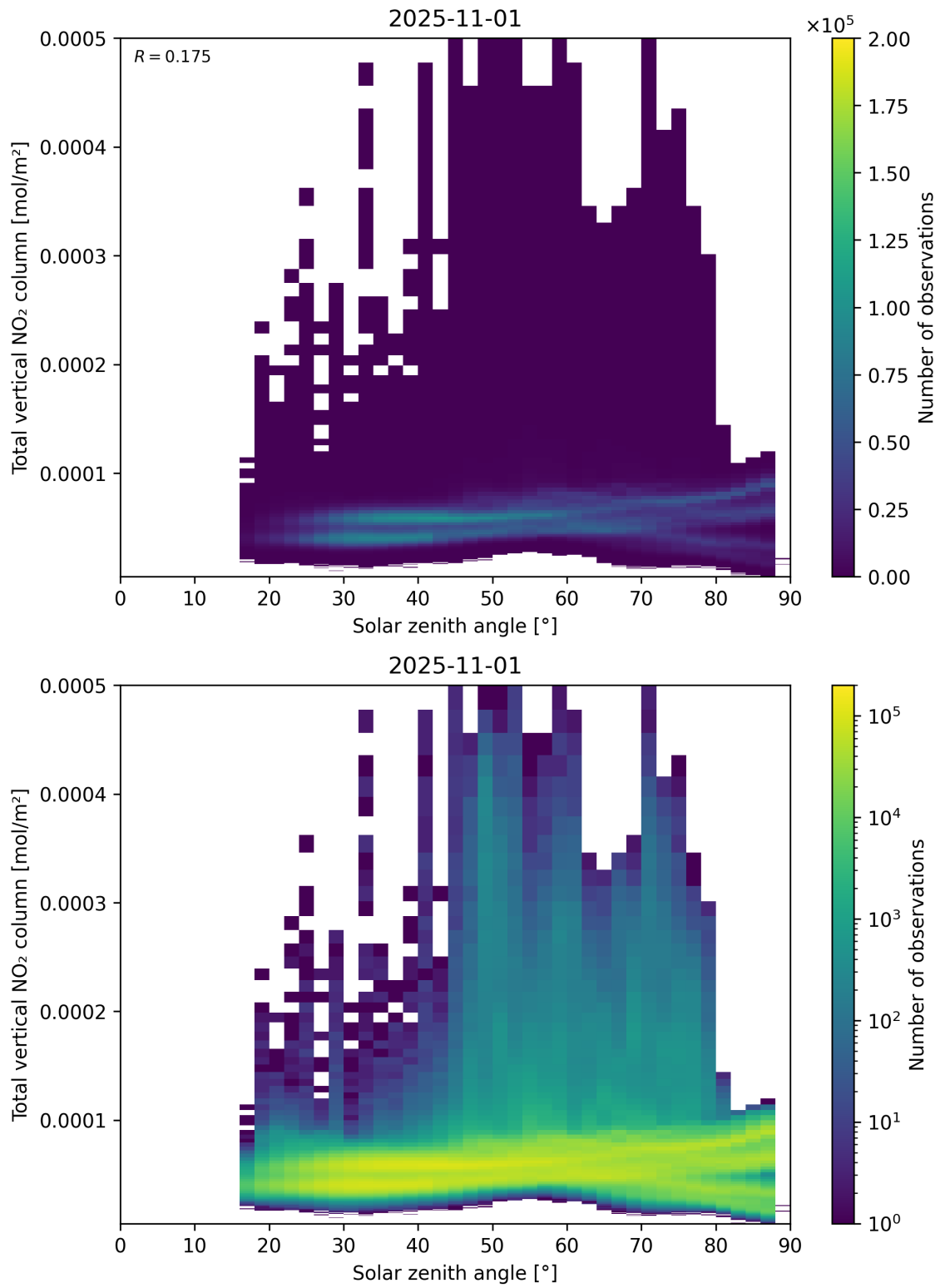
Figure 153: Scatter density plot of “Solar zenith angle” against “Total vertical NO 2 column” for 2025-10-31 to 2025-11-02.
