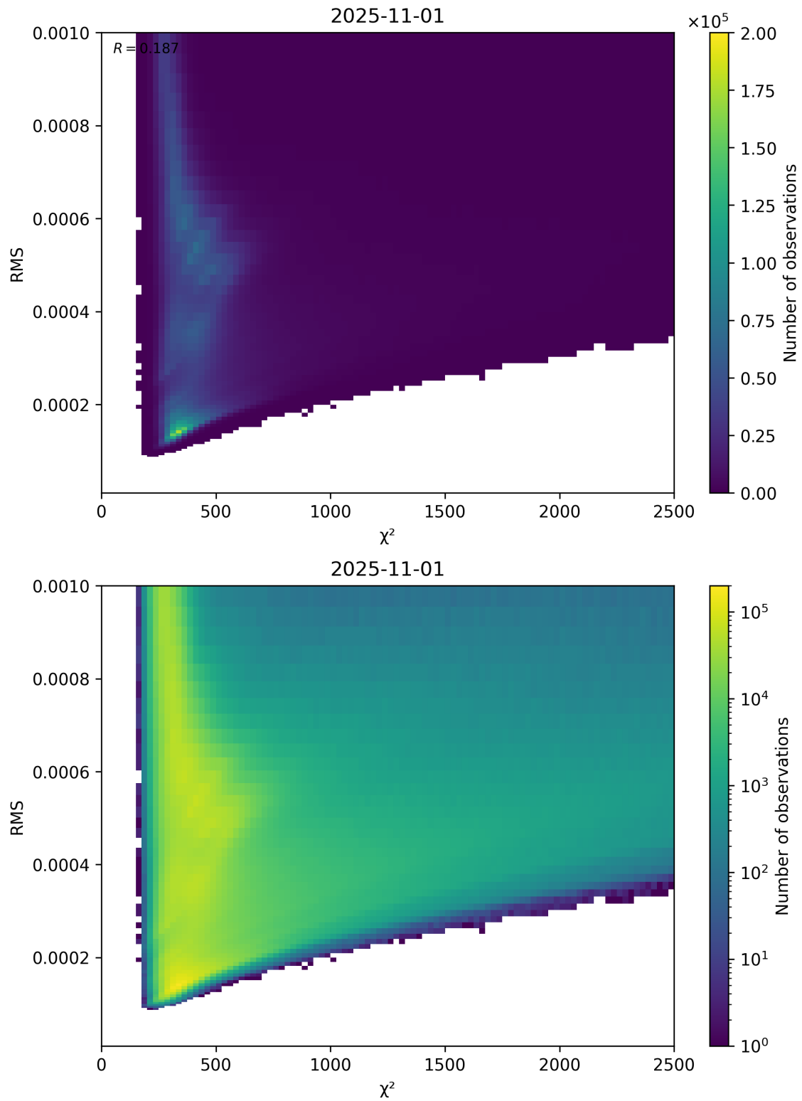
Figure 82: Scatter density plot of “ \chi^2 ” against “RMS” for 2025-10-31 to 2025-11-02.
