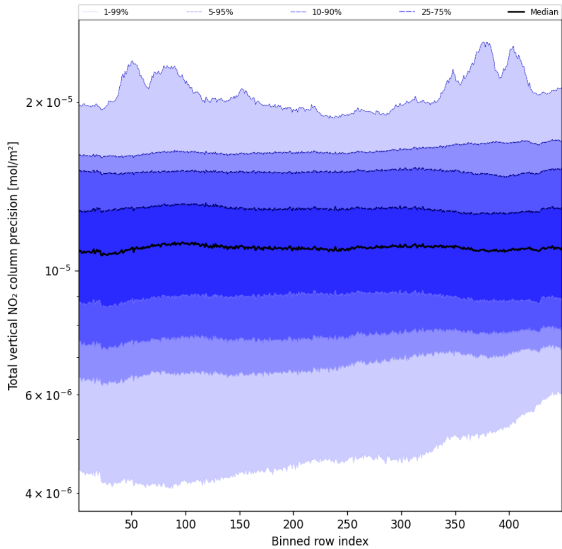
Figure 56: Along track statistics of “Total vertical NO 2 column precision” for 2025-10-31 to 2025-11-02
