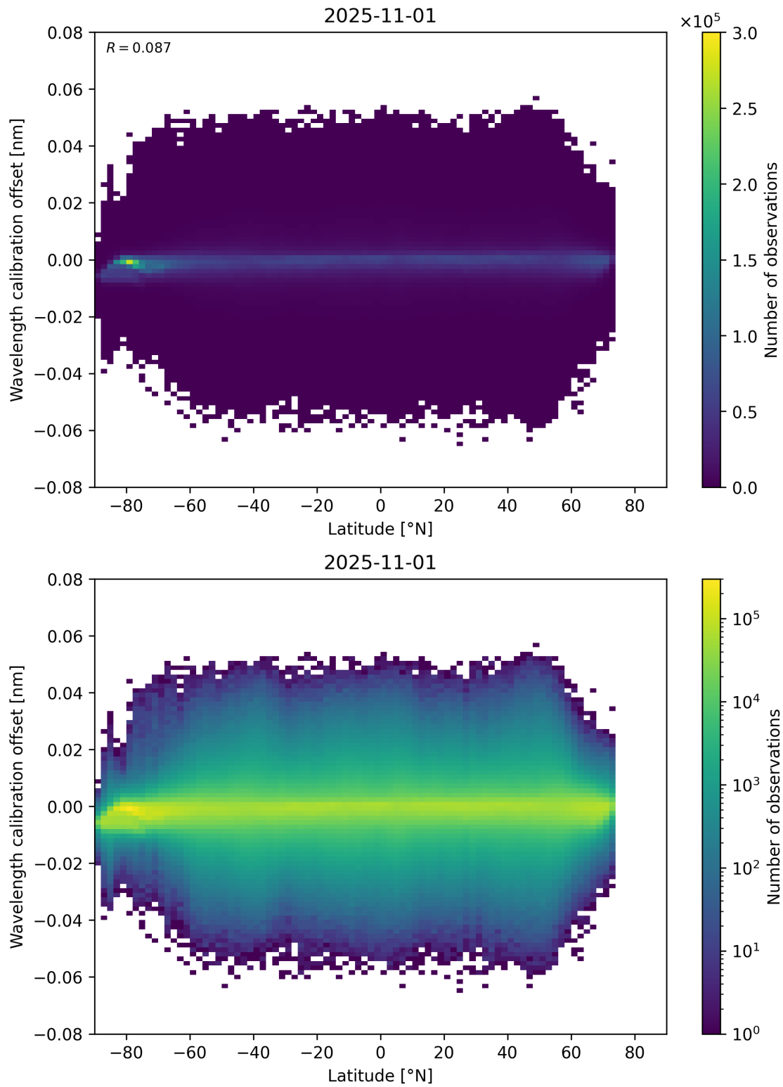
Figure 95: Scatter density plot of “Latitude” against “Wavelength calibration offset” for 2025-10-31 to 2025-11-02.
