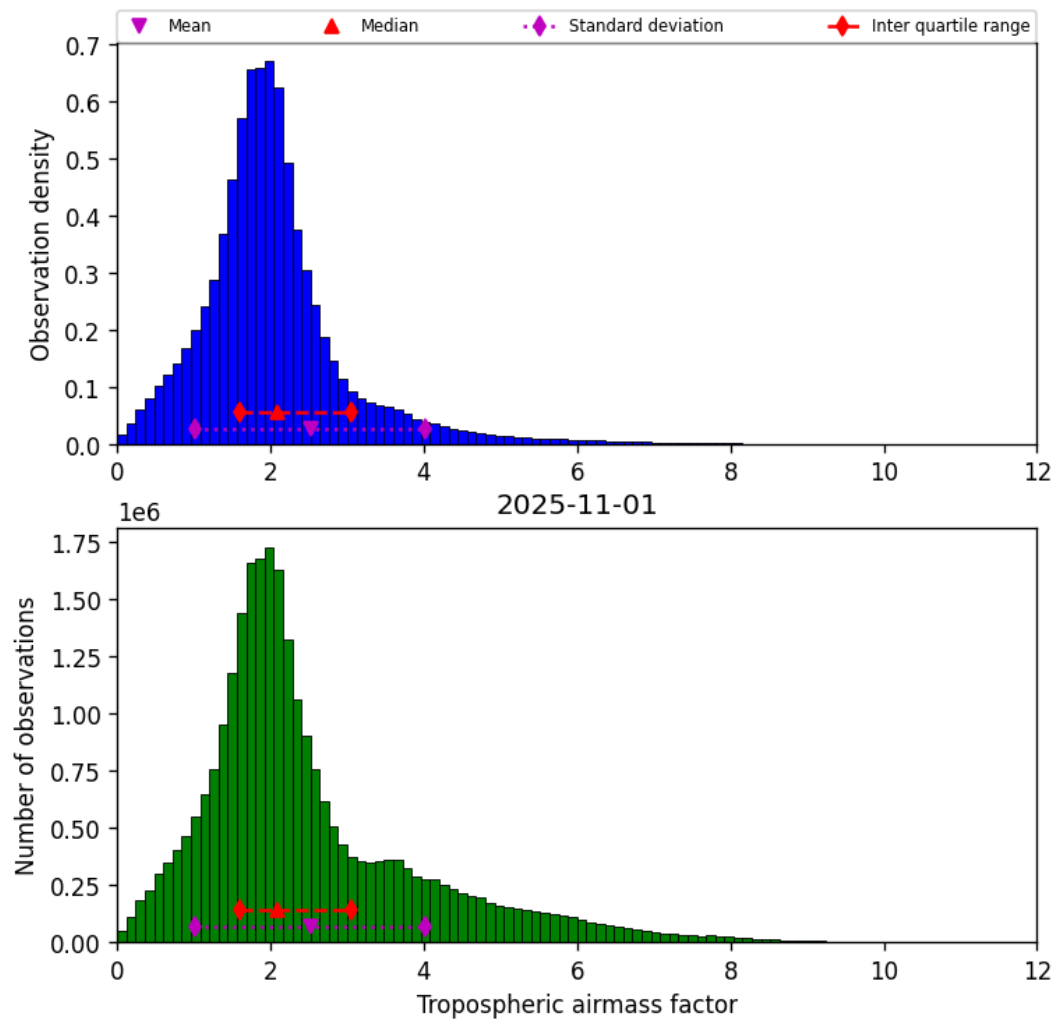
Figure 31: Histogram of “Tropospheric airmass factor” for 2025-10-31 to 2025-11-02
