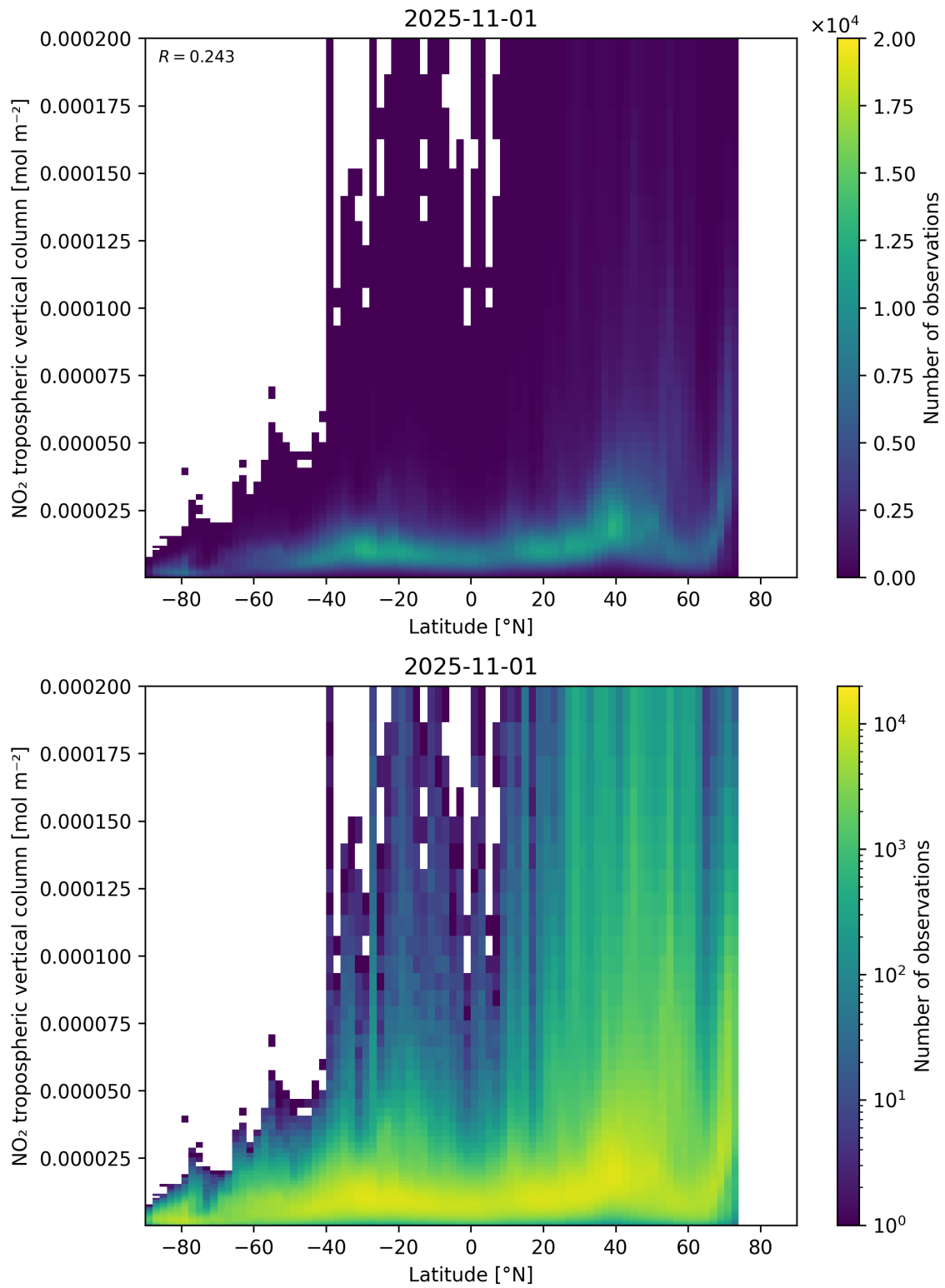
Figure 92: Scatter density plot of “Latitude” against “NO 2 tropospheric vertical column” for 2025-10-31 to 2025-11-02.
