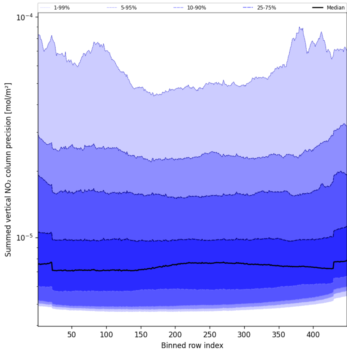
Figure 58: Along track statistics of “Summed vertical NO 2 column precision” for 2025-10-31 to 2025-11-02
