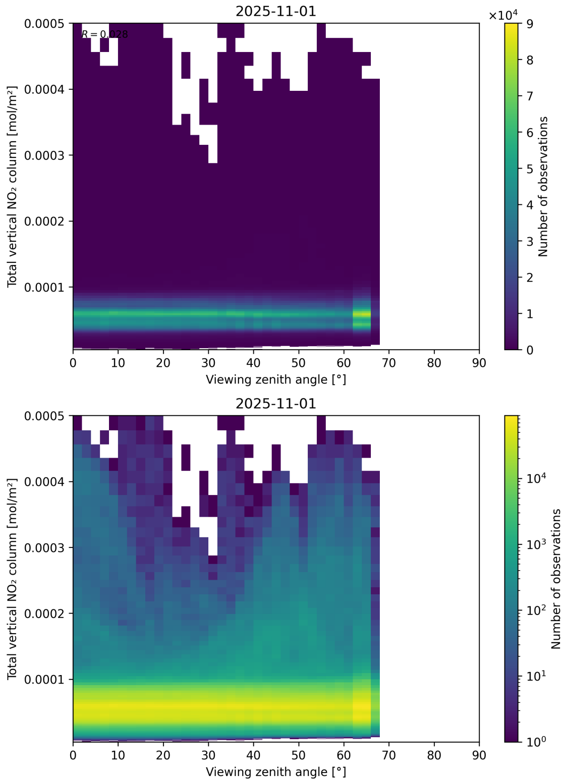
Figure 167: Scatter density plot of “Viewing zenith angle” against “Total vertical NO 2 column” for 2025-10-31 to 2025-11-02.
