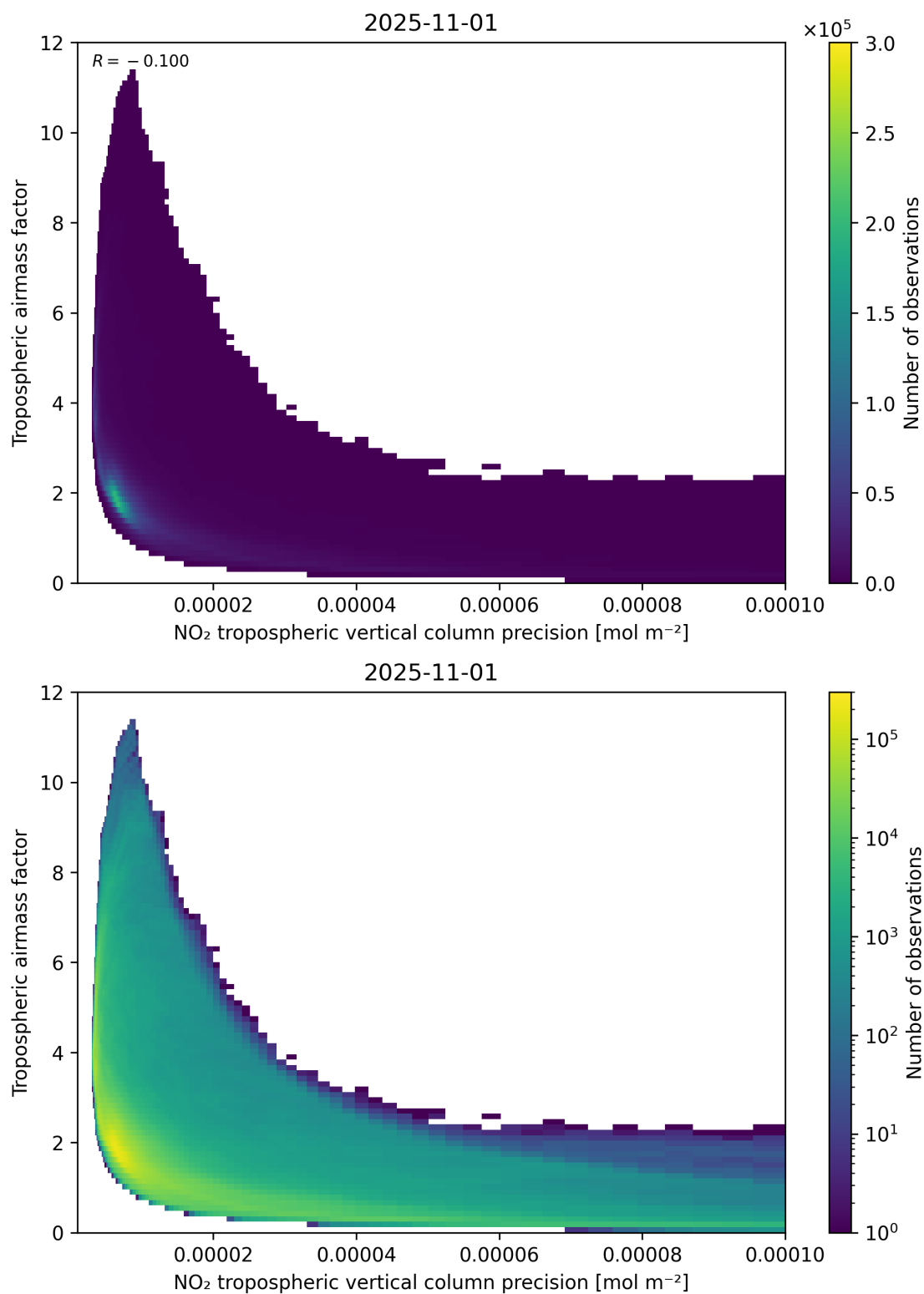
Figure 133: Scatter density plot of “NO 2 tropospheric vertical column precision” against “Tropospheric air mass factor” for 2025-10-31 to 2025-11-02.
