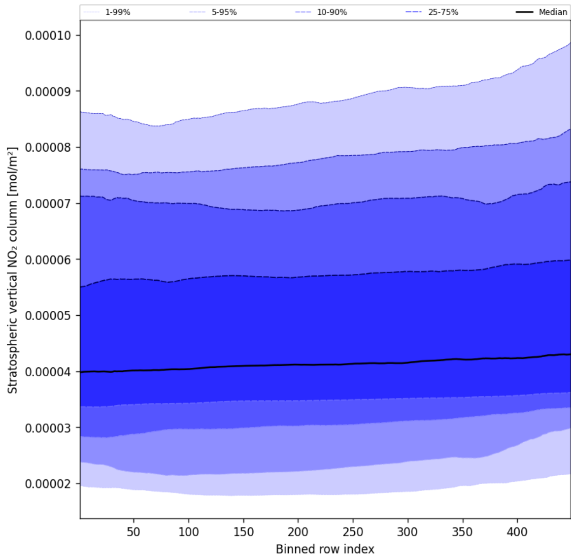
Figure 53: Along track statistics of “Stratospheric vertical NO 2 column” for 2025-10-31 to 2025-11-02
