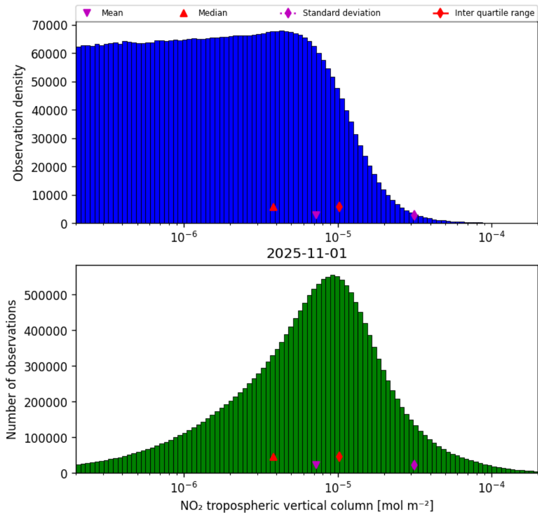
Figure 29: Histogram of “NO 2 tropospheric vertical column” for 2025-10-31 to 2025-11-02
