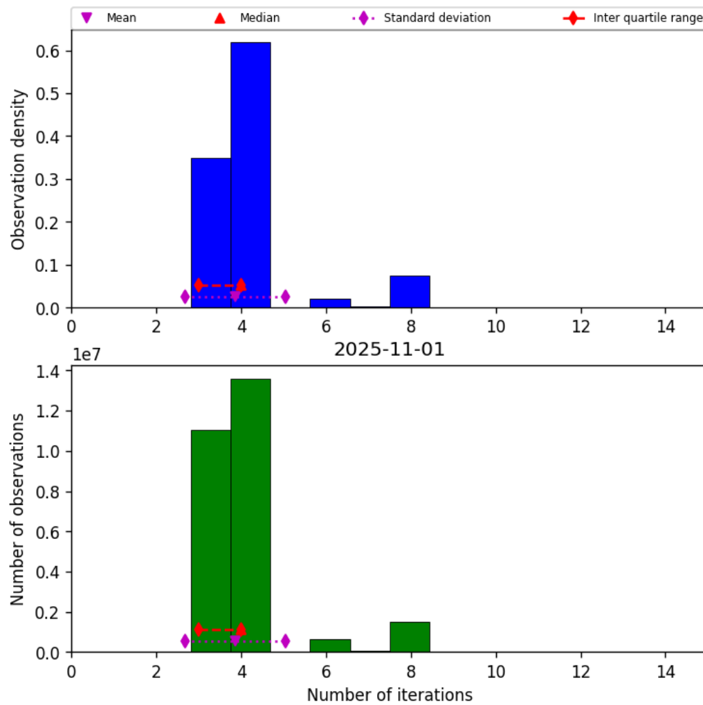
Figure 34: Histogram of “Number of iterations” for 2025-10-31 to 2025-11-02
