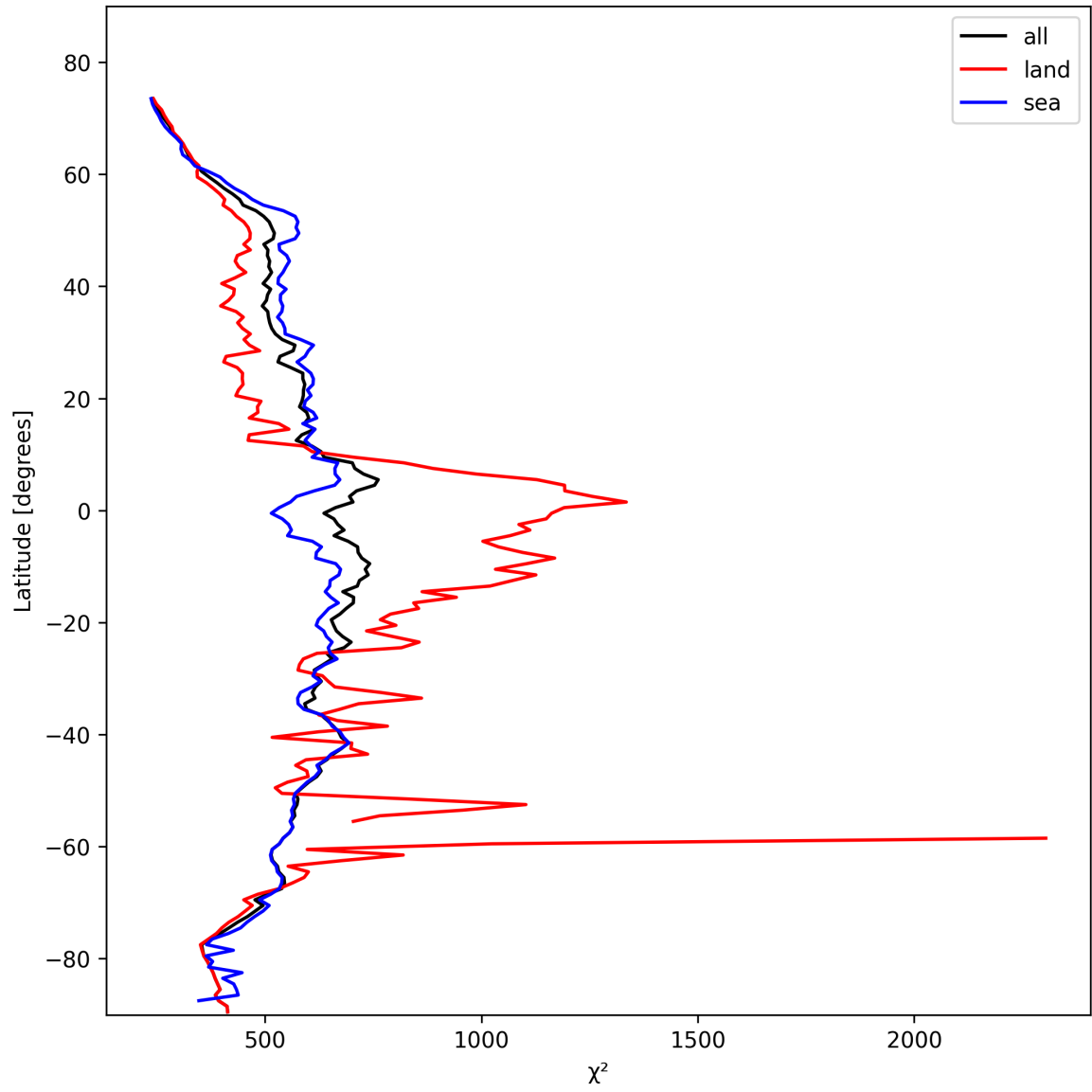
Figure 25: Zonal average of “ \chi^2 ” for 2025-10-31 to 2025-11-02.
