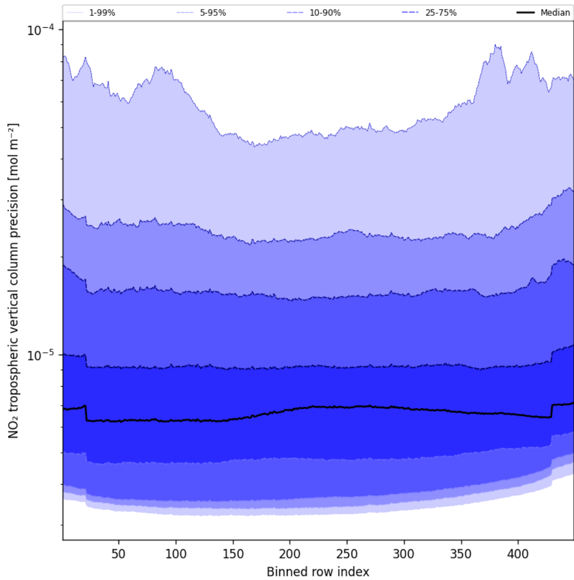
Figure 47: Along track statistics of “NO 2 tropospheric vertical column precision” for 2025-10-31 to 2025-11-02
