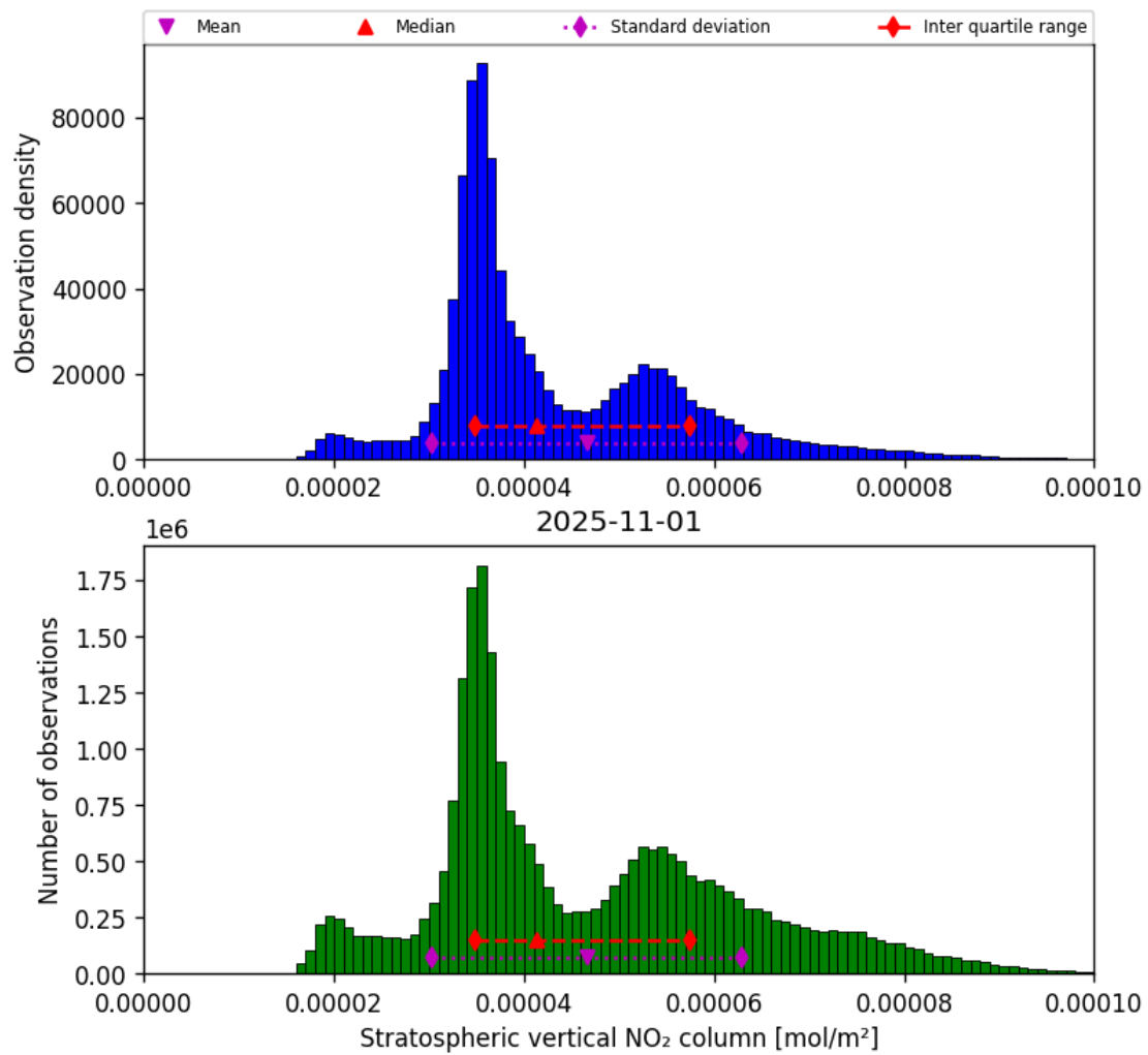
Figure 36: Histogram of “Stratospheric vertical NO 2 column” for 2025-10-31 to 2025-11-02
