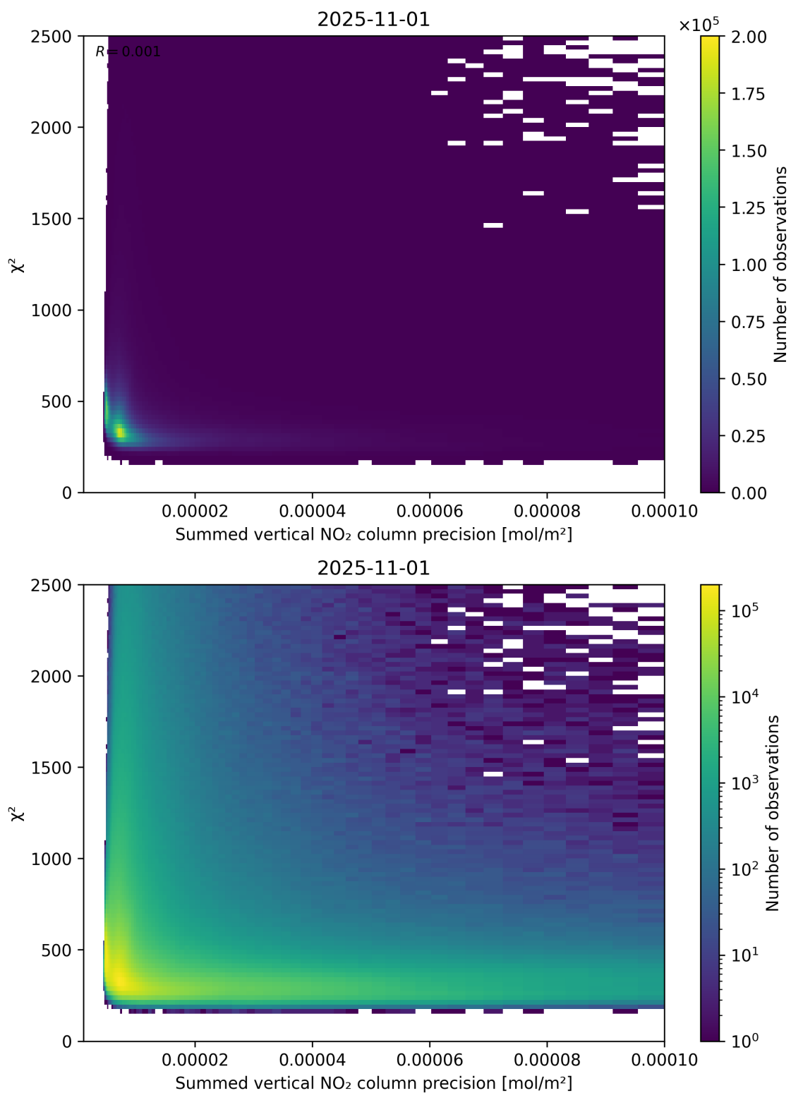
Figure 107: Scatter density plot of “Summed vertical NO 2 column precision” against “ \chi^2 ” for 2025-10-31 to 2025-11-02.
