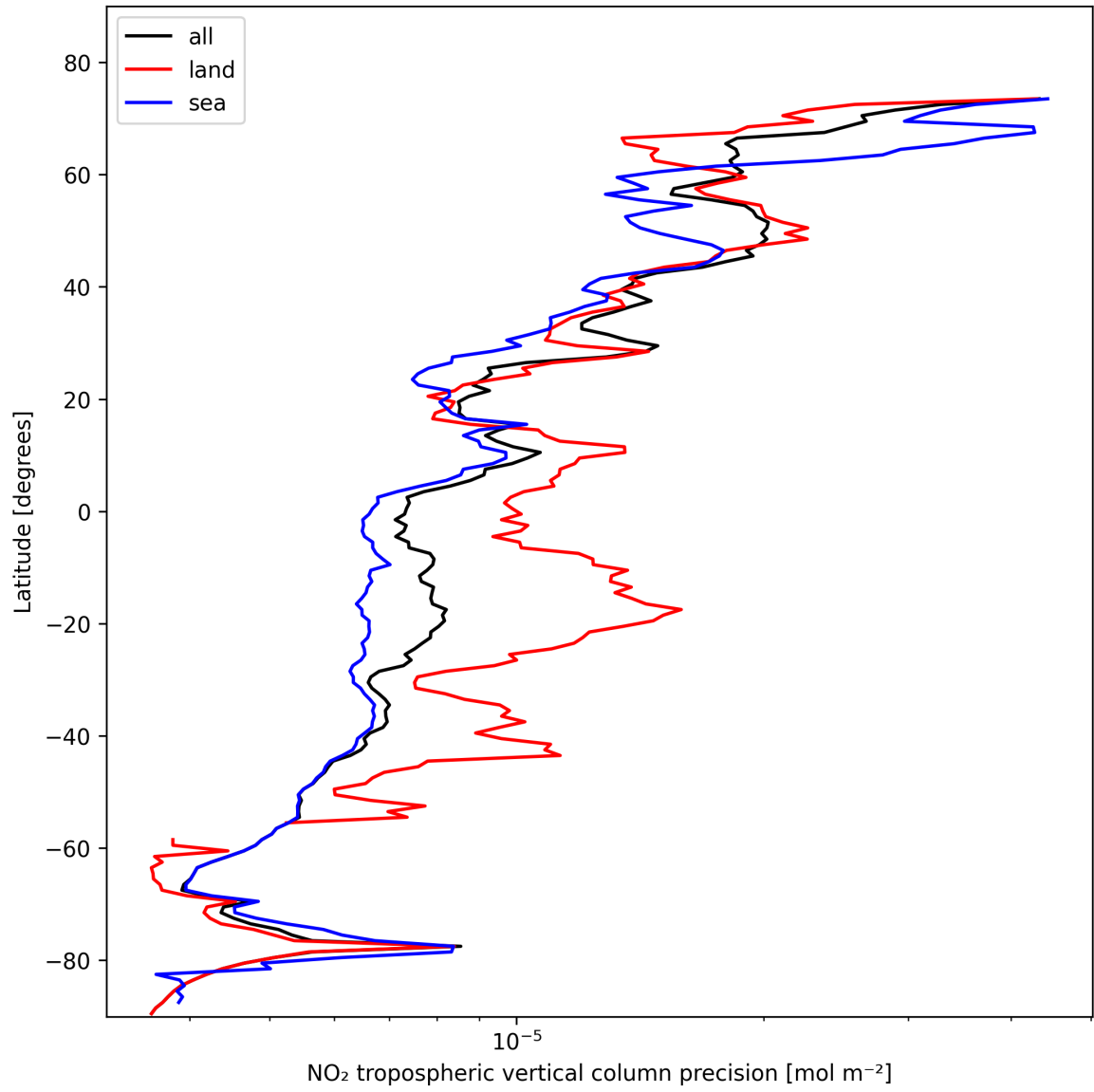
Figure 13: Zonal average of “NO 2 tropospheric vertical column precision” for 2025-10-31 to 2025-11-02.
