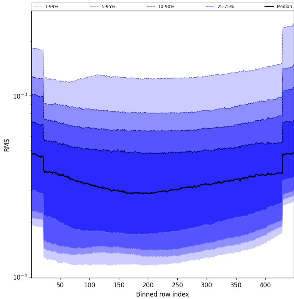
Figure 60: Along track statistics of “RMS” for 2025-10-31 to 2025-11-02
