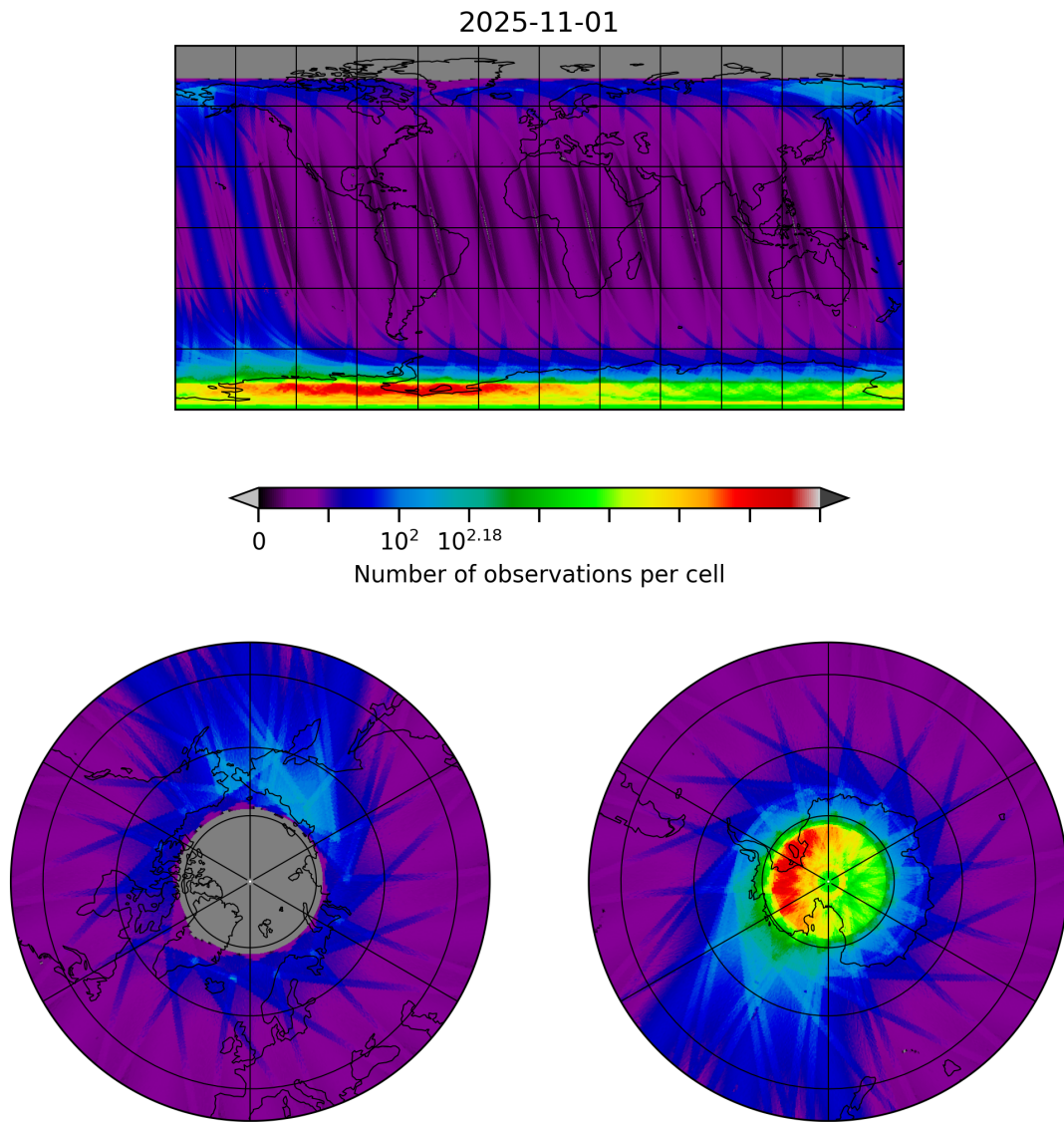
Figure 10: Map of the number of observations for 2025-10-31 to 2025-11-02
