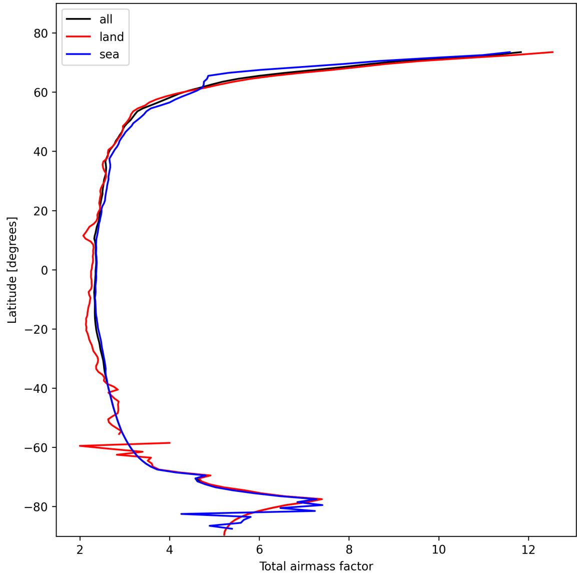
Figure 15: Zonal average of “Total airmass factor” for 2025-10-31 to 2025-11-02.
