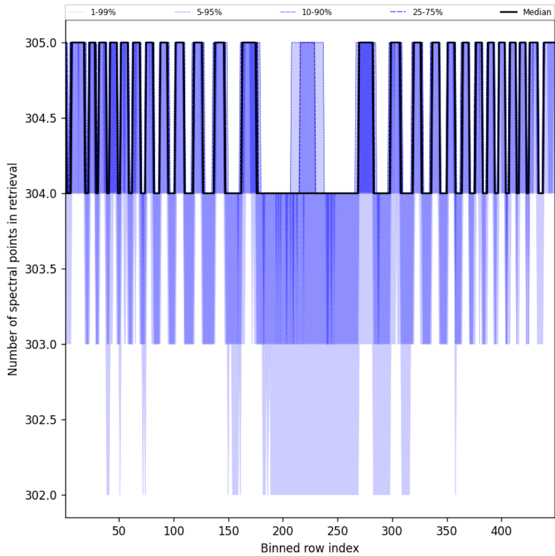
Figure 50: Along track statistics of “Number of spectral points in retrieval” for 2025-10-31 to 2025-11-02
