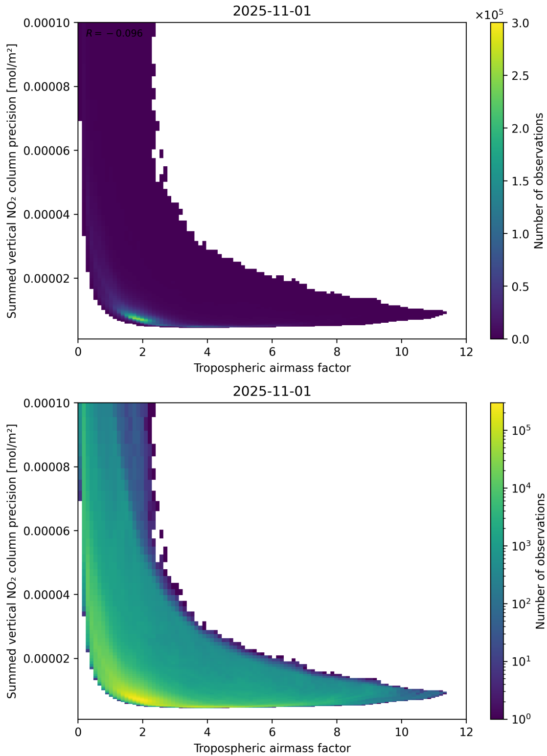
Figure 76: Scatter density plot of “Tropospheric airmass factor” against “Summed vertical NO 2 column precision” for 2025-10-31 to 2025-11-02.
