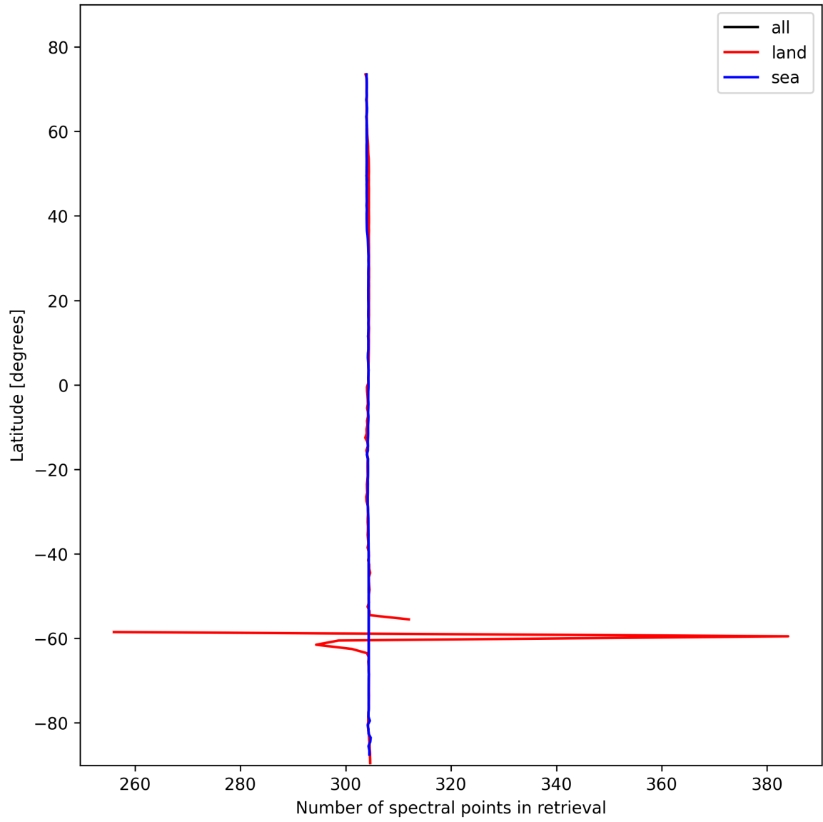
Figure 16: Zonal average of “Number of spectral points in retrieval” for 2025-10-31 to 2025-11-02.
