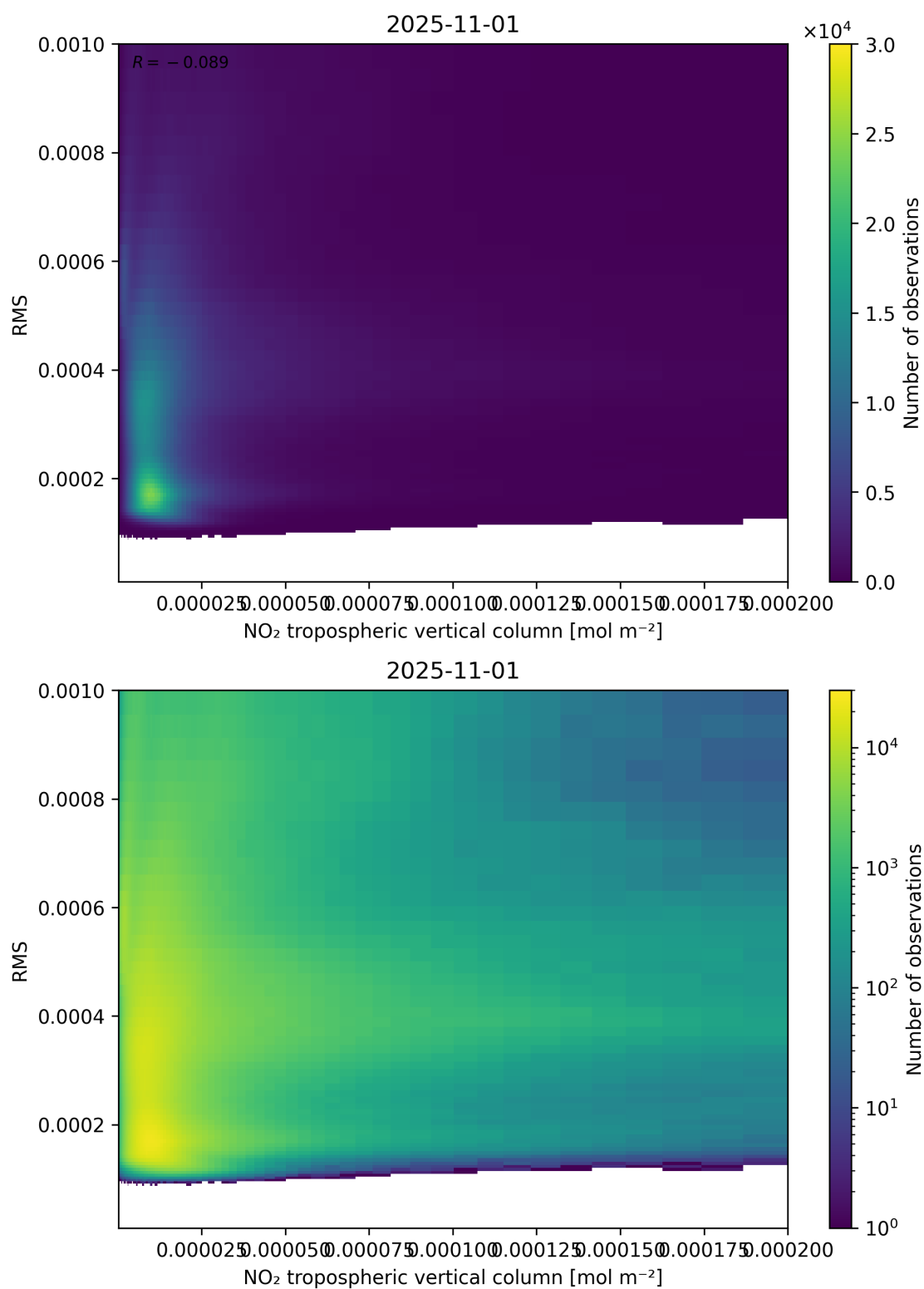
Figure 142: Scatter density plot of “NO 2 tropospheric vertical column” against “RMS” for 2025-10-31 to 2025-11-02.
