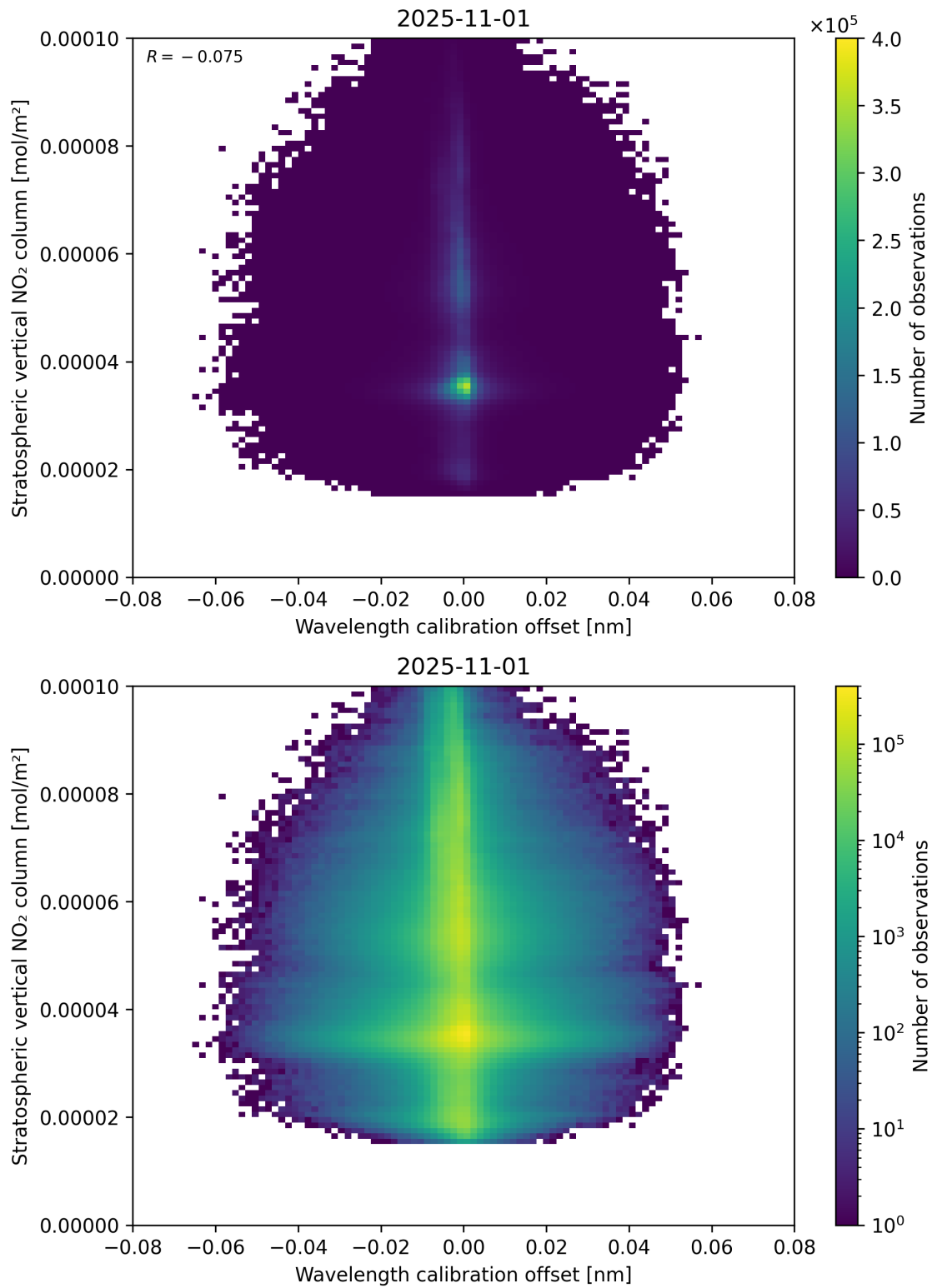
Figure 176: Scatter density plot of “Wavelength calibration offset” against “Stratospheric vertical NO 2 column” for 2025-10-31 to 2025-11-02.
