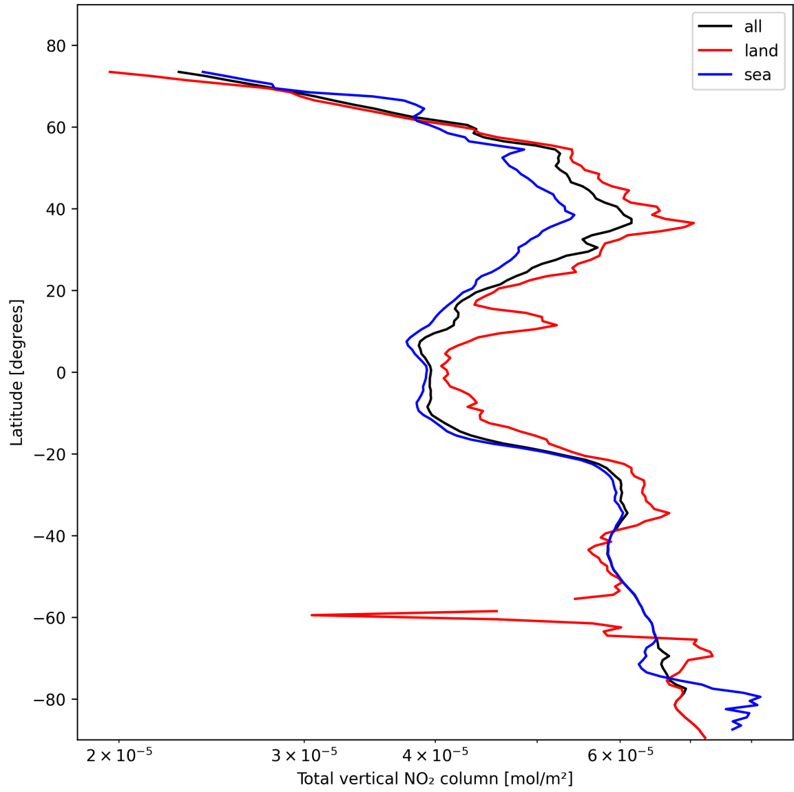
Figure 21: Zonal average of “Total vertical NO 2 column” for 2025-10-31 to 2025-11-02.
