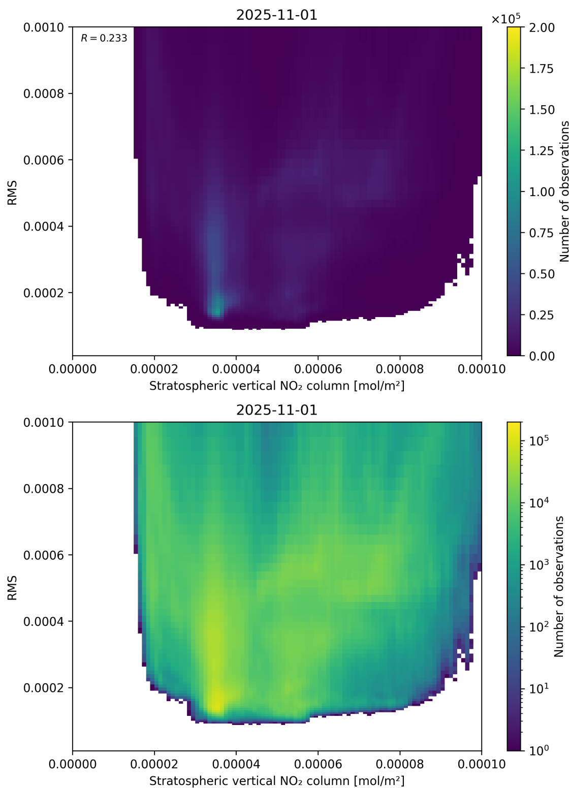
Figure 102: Scatter density plot of “Stratospheric vertical NO 2 column” against “RMS” for 2025-10-31 to 2025-11-02.
