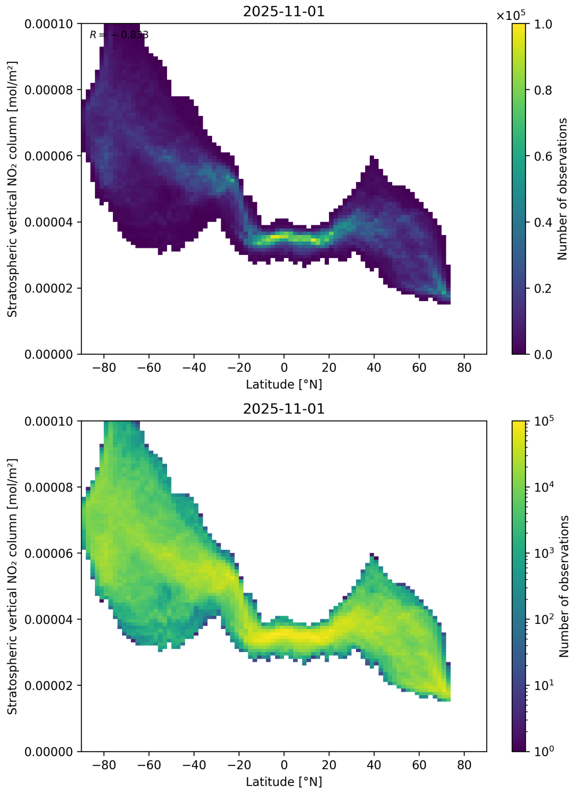
Figure 87: Scatter density plot of “Latitude” against “Stratospheric vertical NO 2 column” for 2025-10-31 to 2025-11-02.
