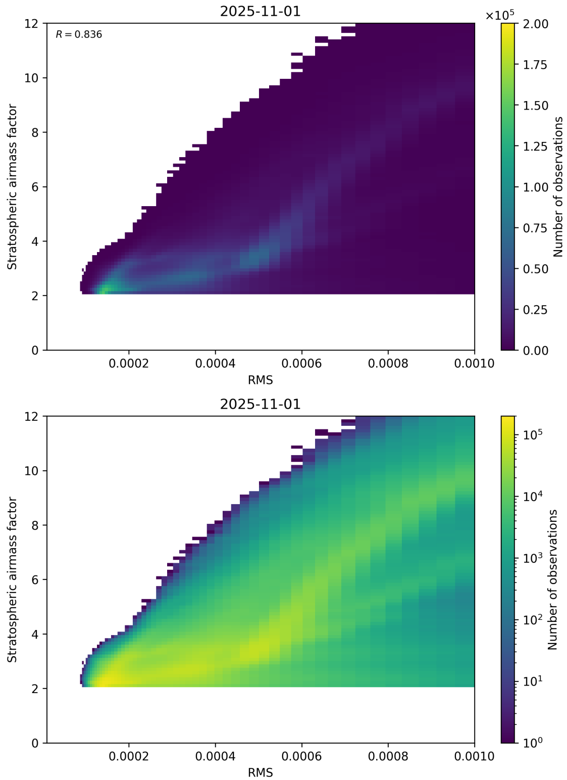
Figure 144: Scatter density plot of “RMS” against “Stratospheric airmass factor” for 2025-10-31 to 2025-11-02.
