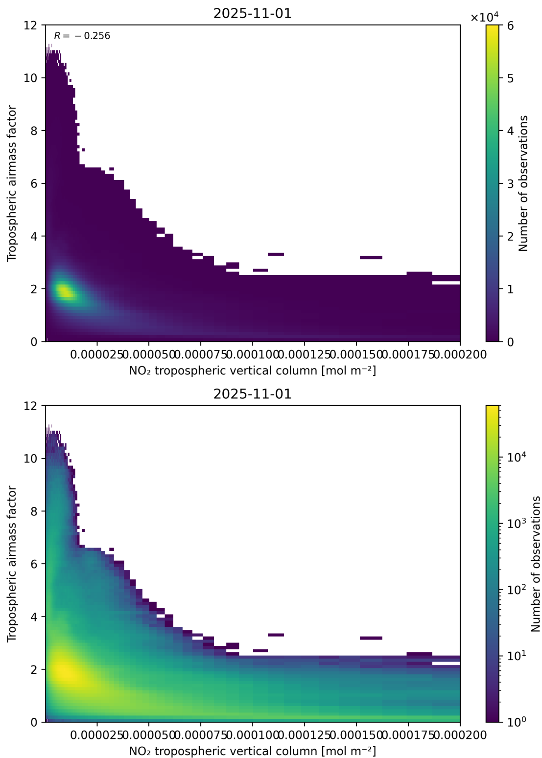
Figure 123: Scatter density plot of “NO 2 tropospheric vertical column” against “Tropospheric air mass factor” for 2025-10-31 to 2025-11-02.
