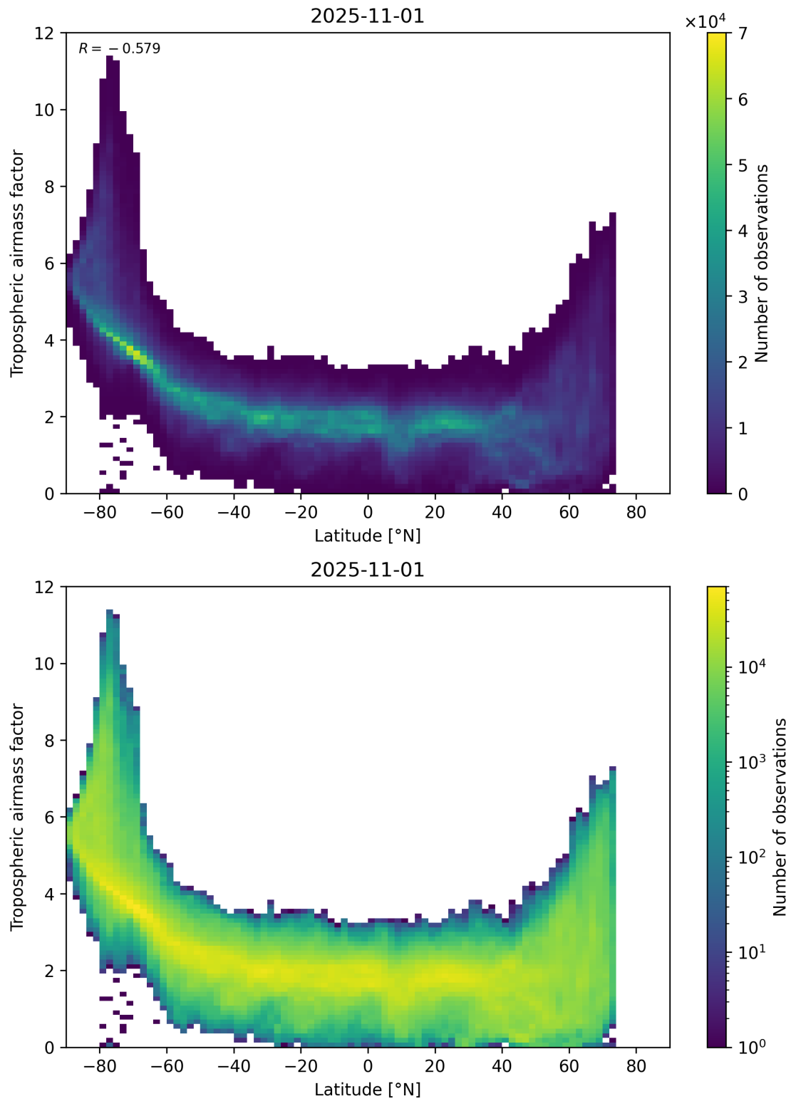
Figure 85: Scatter density plot of “Latitude” against “Tropospheric air mass factor” for 2025-10-31 to 2025-11-02.
