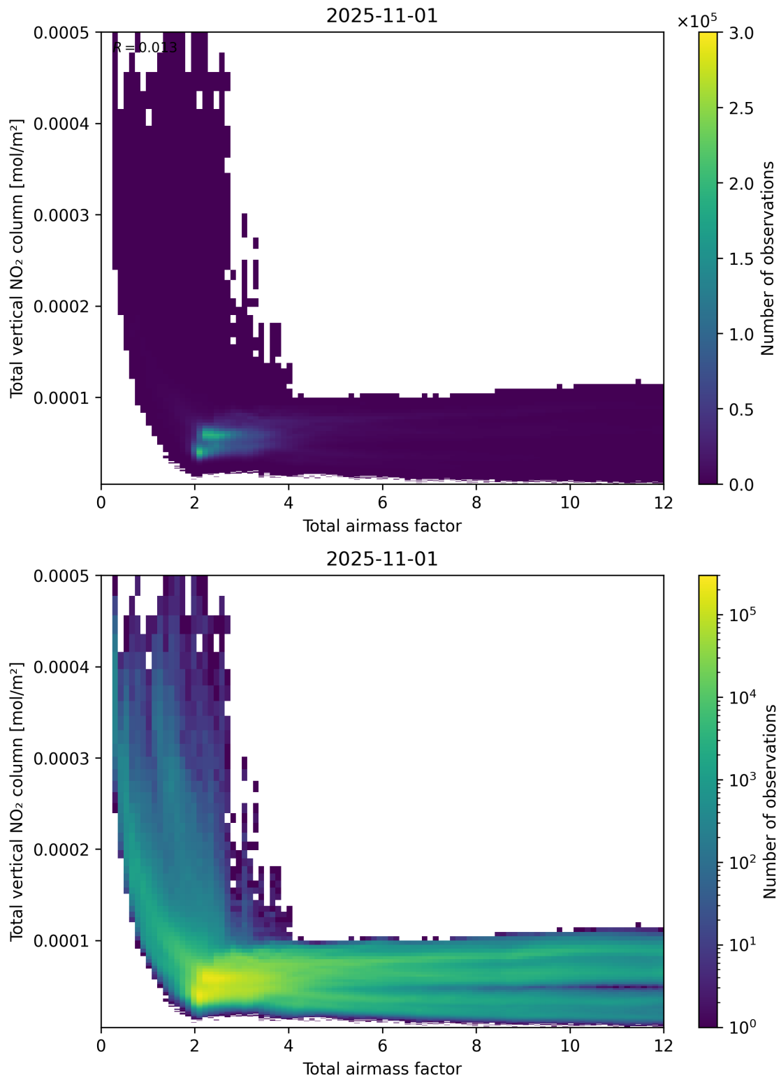
Figure 67: Scatter density plot of “Total airmass factor” against “Total vertical NO 2 column” for 2025-10-31 to 2025-11-02.
