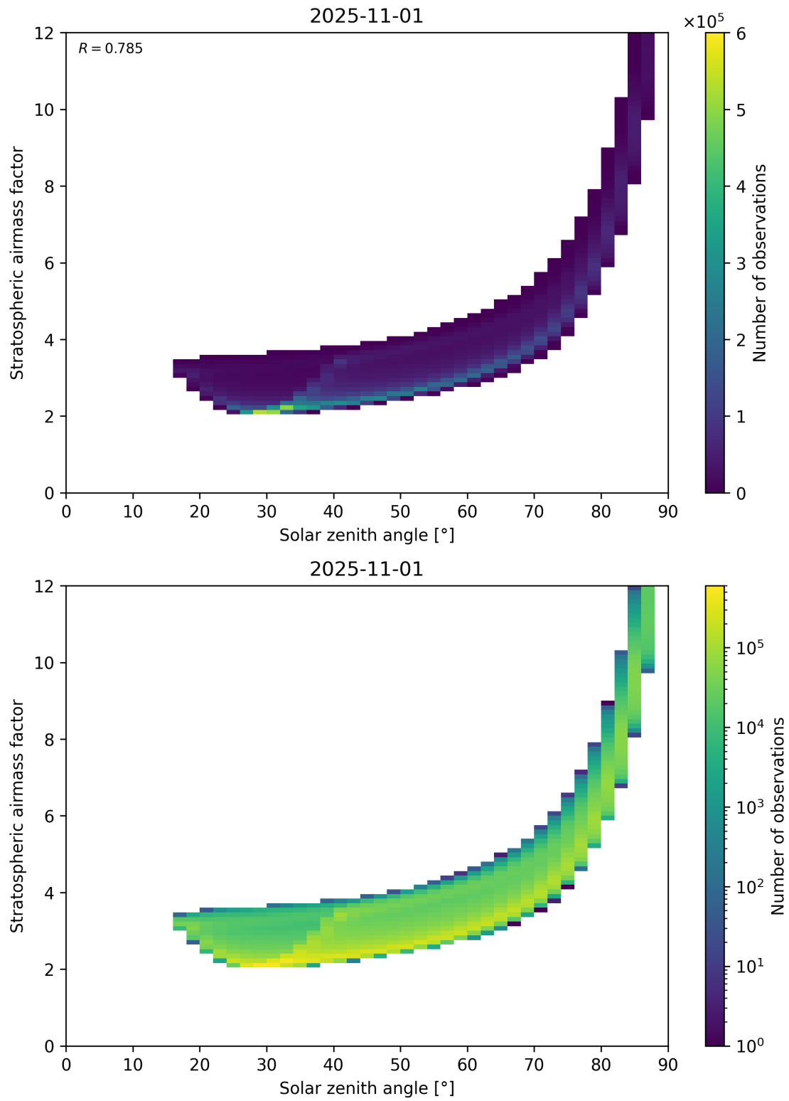
Figure 145: Scatter density plot of “Solar zenith angle” against “Stratospheric airmass factor” for 2025-10-31 to 2025-11-02.
