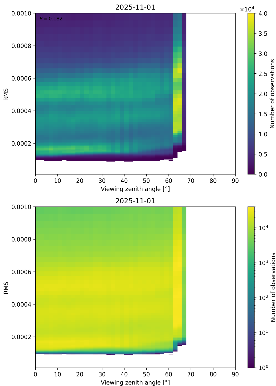
Figure 171: Scatter density plot of “Viewing zenith angle” against “RMS” for 2025-10-31 to 2025-11-02.
