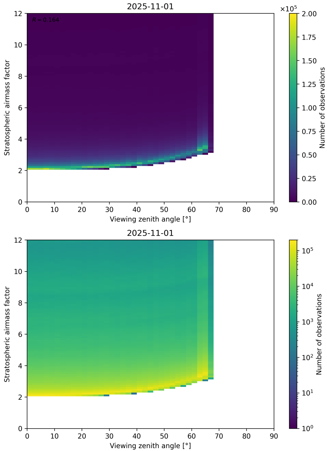
Figure 159: Scatter density plot of “Viewing zenith angle” against “Stratospheric airmass factor” for 2025-10-31 to 2025-11-02.
