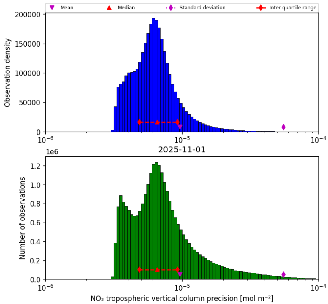
Figure 30: Histogram of "NO 2 tropospheric vertical column precision" for 2025-10-31 to 2025-11-02
