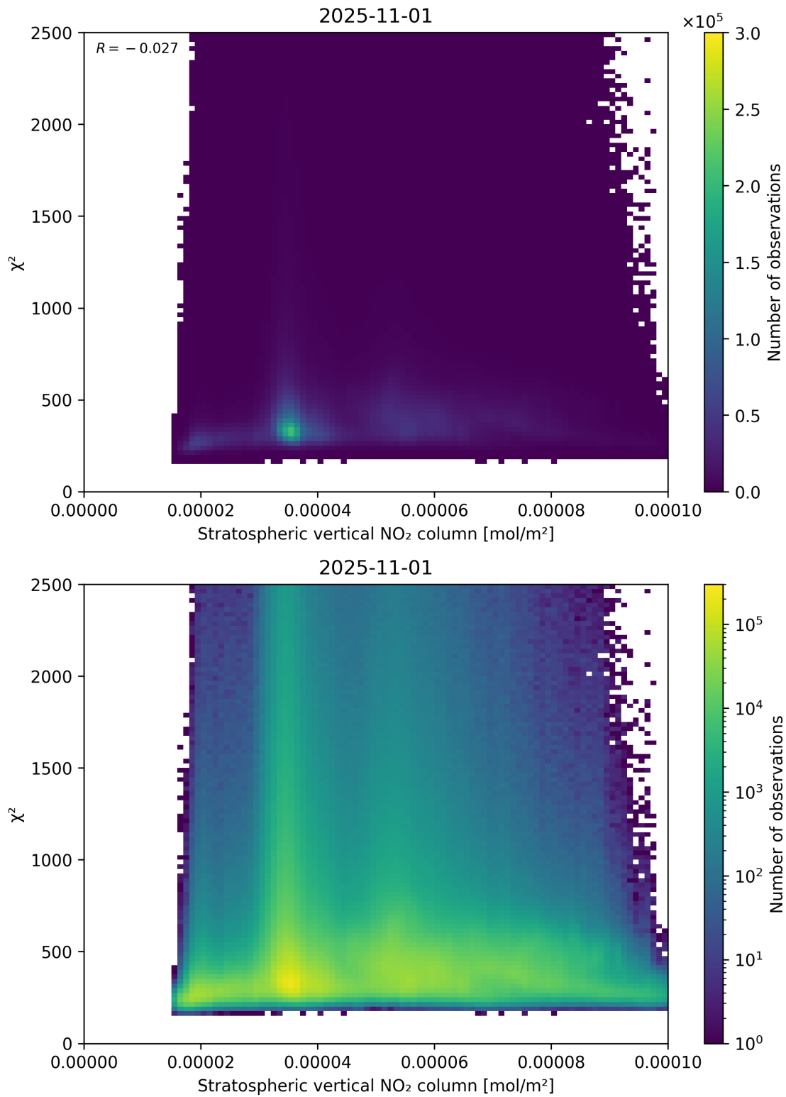
Figure 97: Scatter density plot of “Stratospheric vertical NO 2 column” against “ \chi^2 ” for 2025-10-31 to 2025-11-02.
