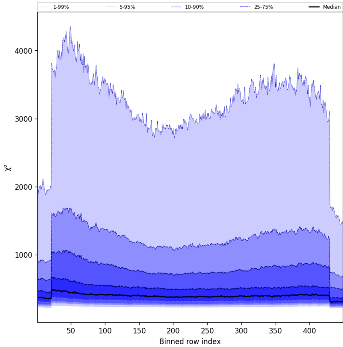
Figure 59: Along track statistics of “ \chi^2 ” for 2025-10-31 to 2025-11-02
