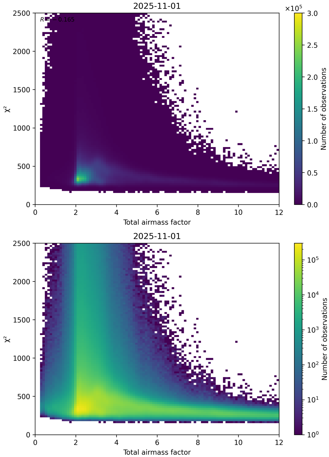
Figure 63: Scatter density plot of “Total airmass factor” against “ \chi^2 ” for 2025-10-31 to 2025-11-02.
