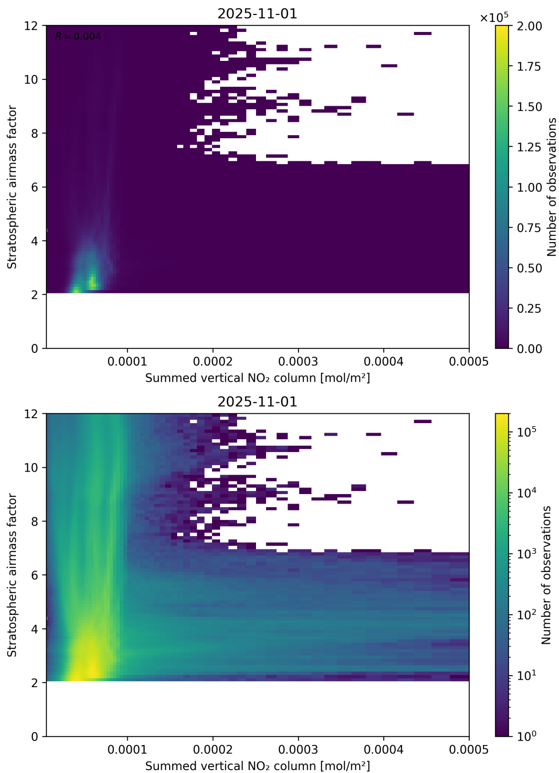
Figure 103: Scatter density plot of “Summed vertical NO 2 column” against “Stratospheric air mass factor” for 2025-10-31 to 2025-11-02.
