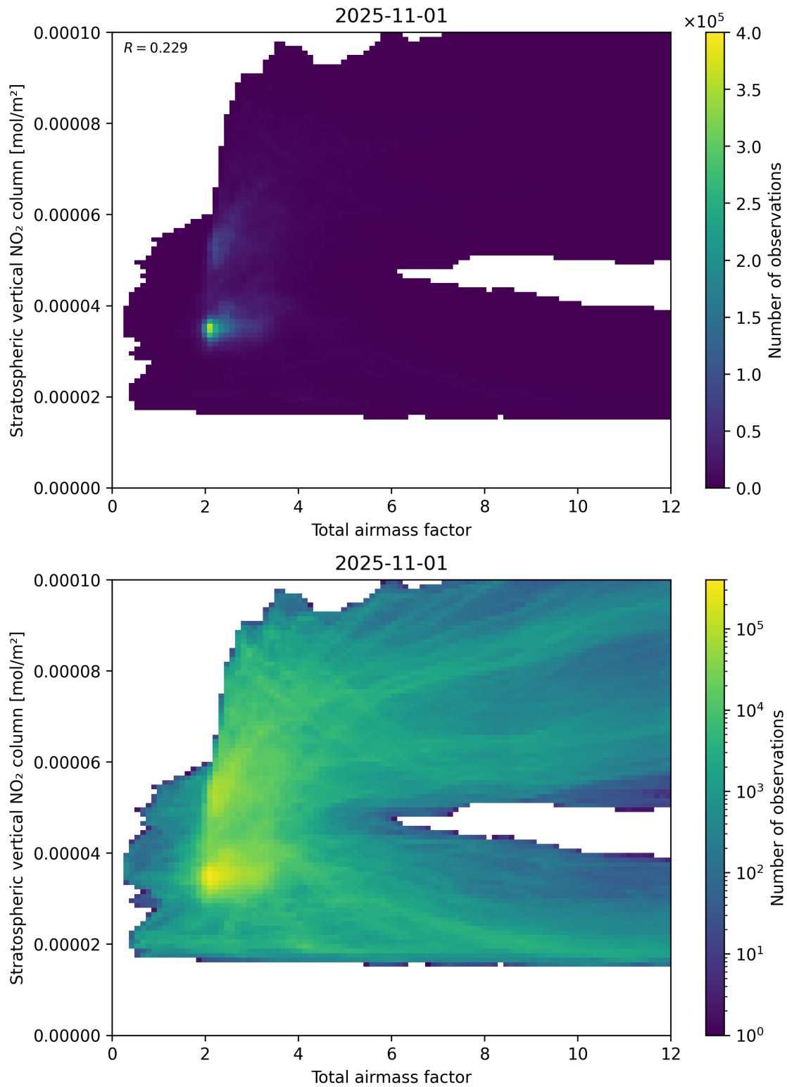
Figure 64: Scatter density plot of “Total airmass factor” against “Stratospheric vertical NO 2 column” for 2025-10-31 to 2025-11-02.
