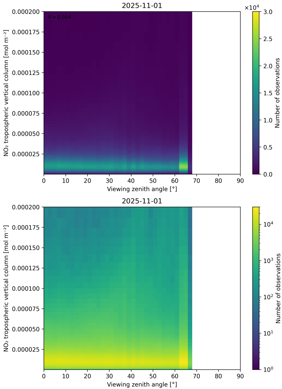
Figure 169: Scatter density plot of “Viewing zenith angle” against “NO 2 tropospheric vertical column” for 2025-10-31 to 2025-11-02.
