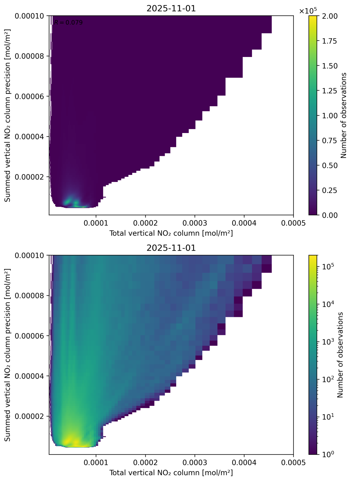
Figure 113: Scatter density plot of “Total vertical NO 2 column” against “Summed vertical NO 2 column precision” for 2025-10-31 to 2025-11-02.
