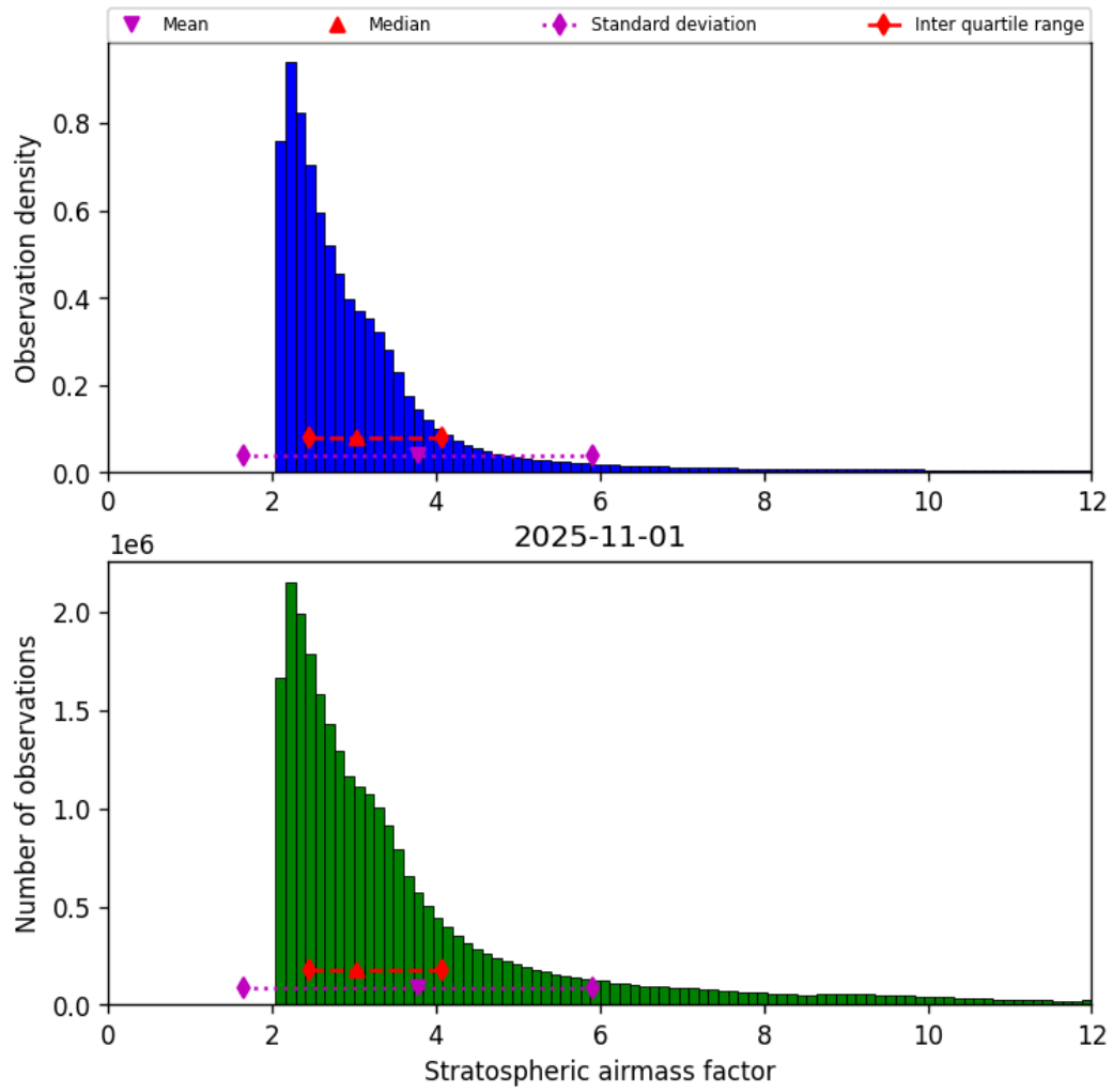
Figure 44: Histogram of “Stratospheric airmass factor” for 2025-10-31 to 2025-11-02
