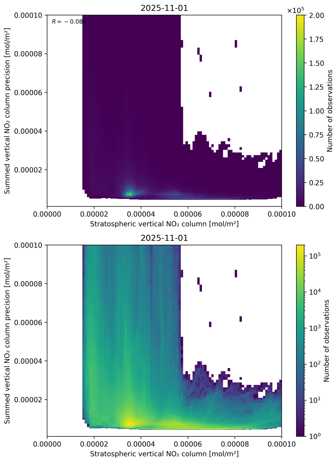
Figure 99: Scatter density plot of “Stratospheric vertical NO 2 column” against “Summed vertical NO 2 column precision” for 2025-10-31 to 2025-11-02.
