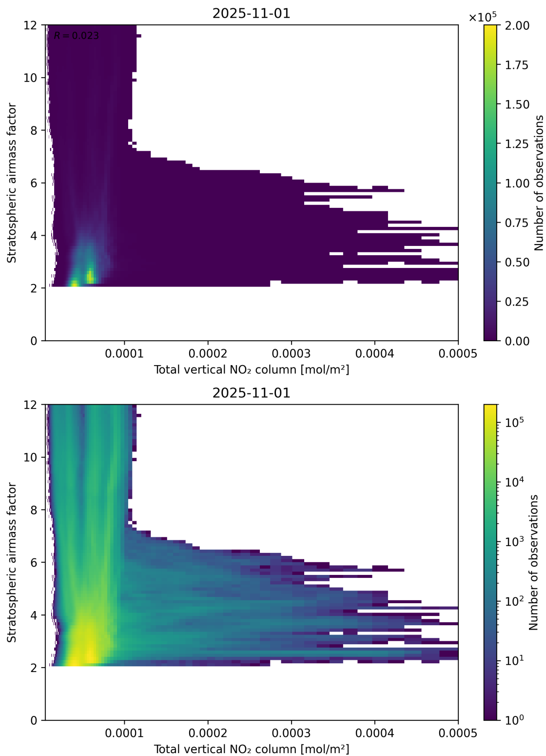
Figure 110: Scatter density plot of “Total vertical NO 2 column” against “Stratospheric airmass factor” for 2025-10-31 to 2025-11-02.
