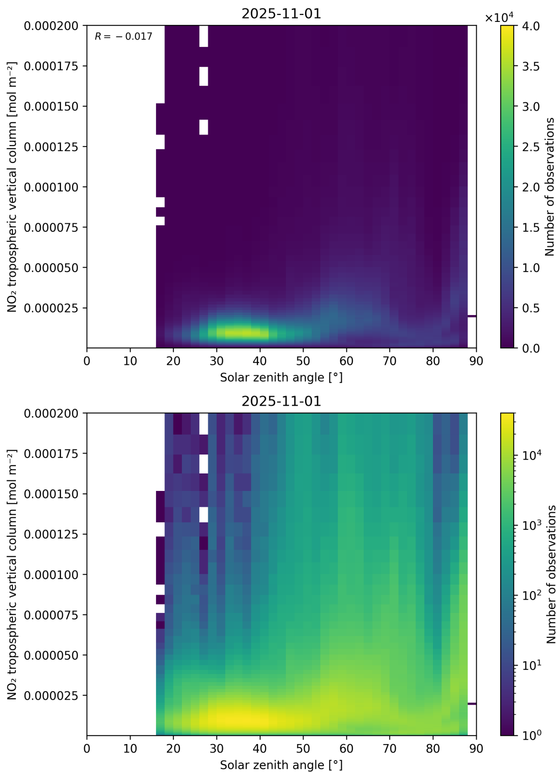
Figure 155: Scatter density plot of “Solar zenith angle” against “NO 2 tropospheric vertical column” for 2025-10-31 to 2025-11-02.
