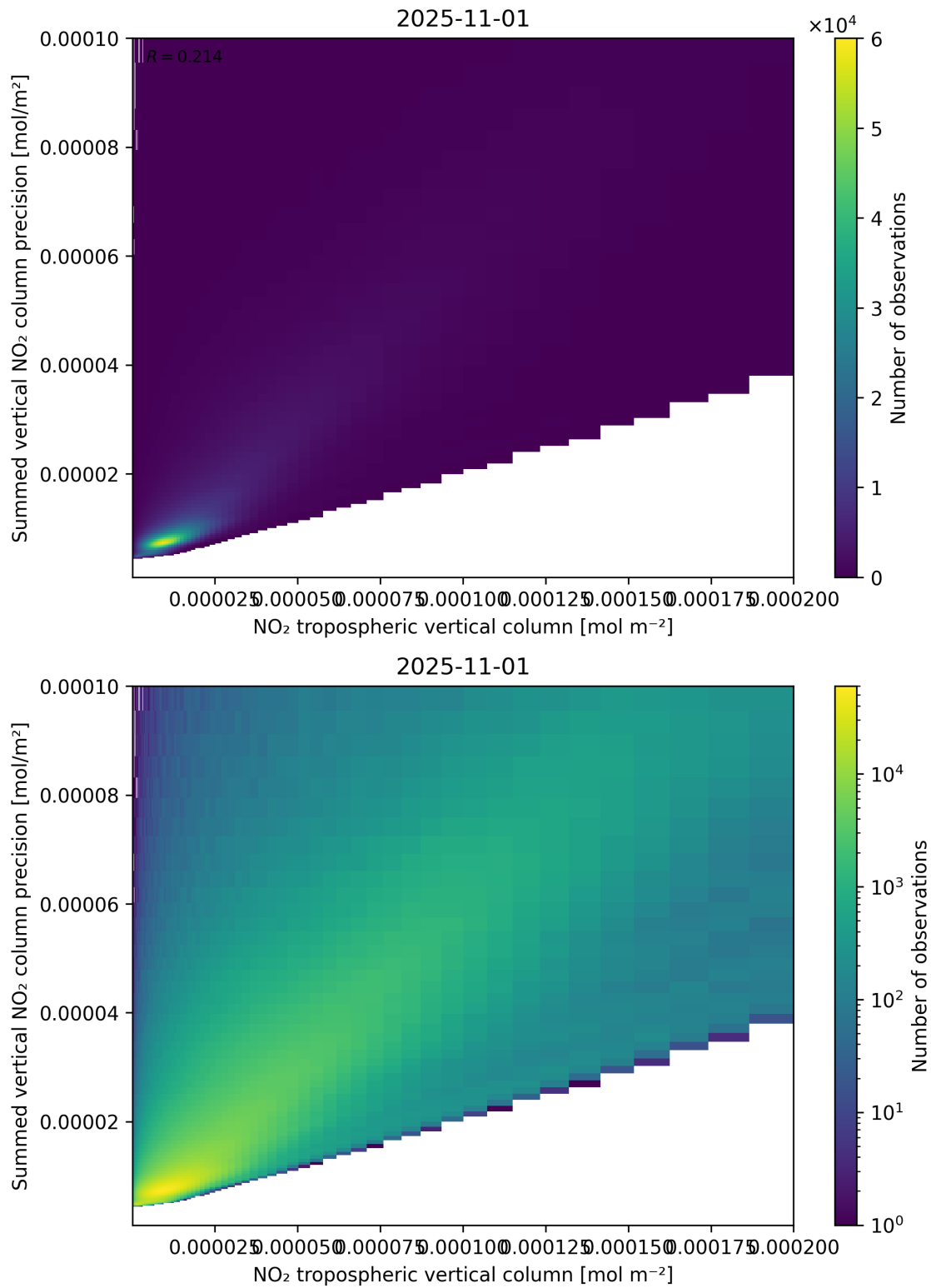
Figure 127: Scatter density plot of “NO 2 tropospheric vertical column” against “Summed vertical NO 2 column precision” for 2025-10-31 to 2025-11-02.
