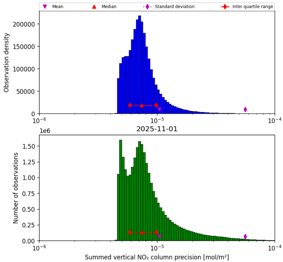
Figure 41: Histogram of “Summed vertical NO 2 column precision” for 2025-10-31 to 2025-11-02
