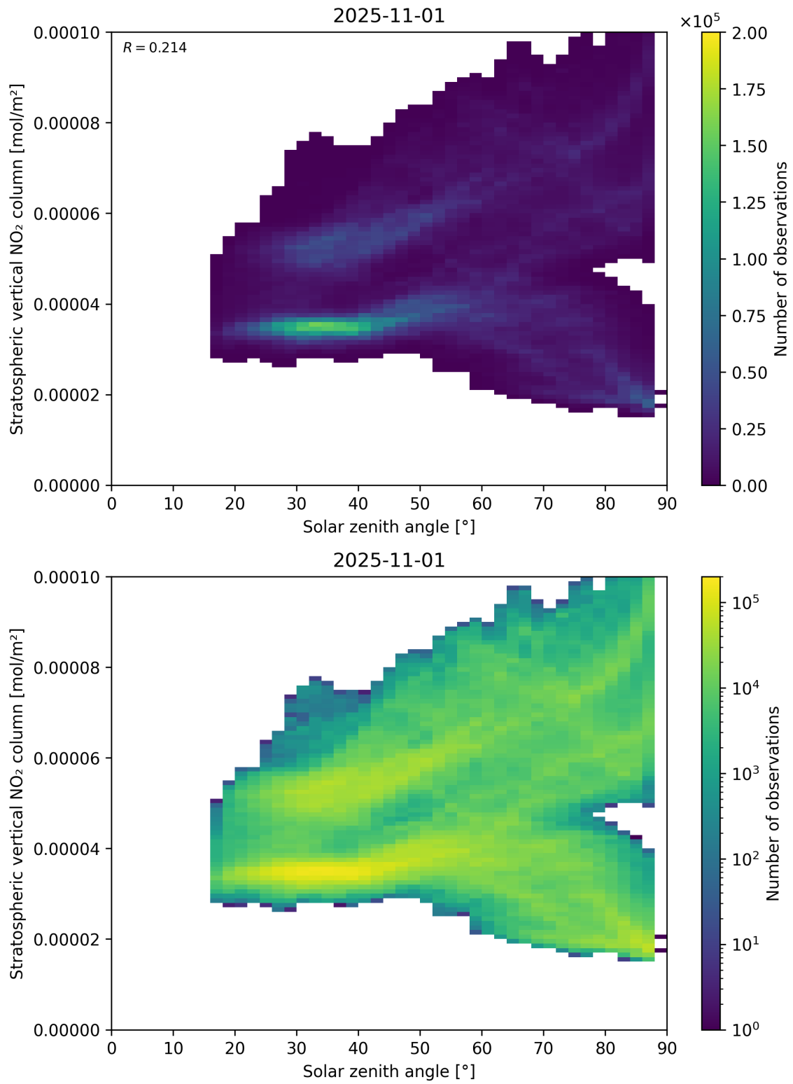
Figure 150: Scatter density plot of “Solar zenith angle” against “Stratospheric vertical NO 2 column” for 2025-10-31 to 2025-11-02.
