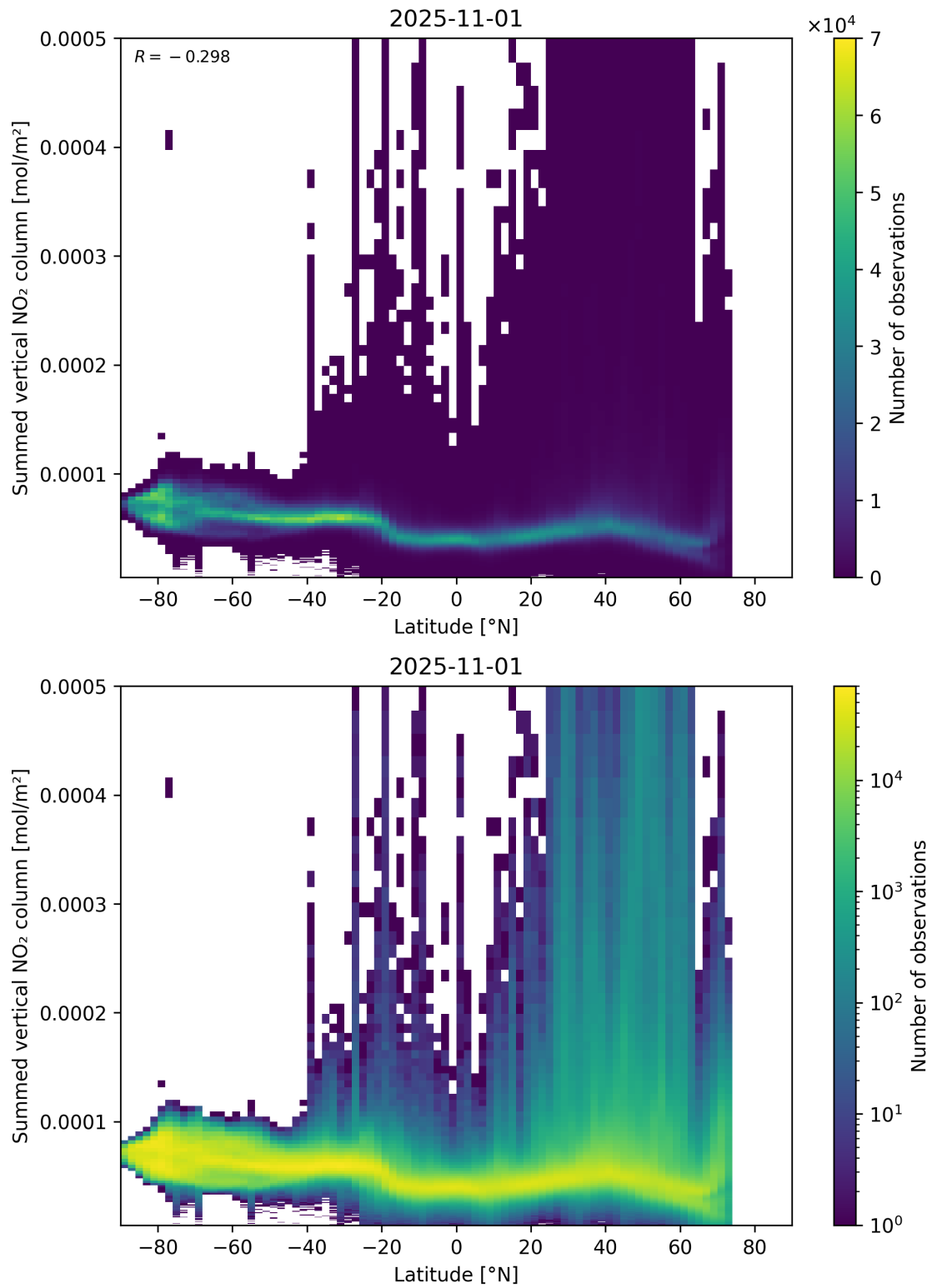
Figure 88: Scatter density plot of “Latitude” against “Summed vertical NO 2 column” for 2025-10-31 to 2025-11-02.
