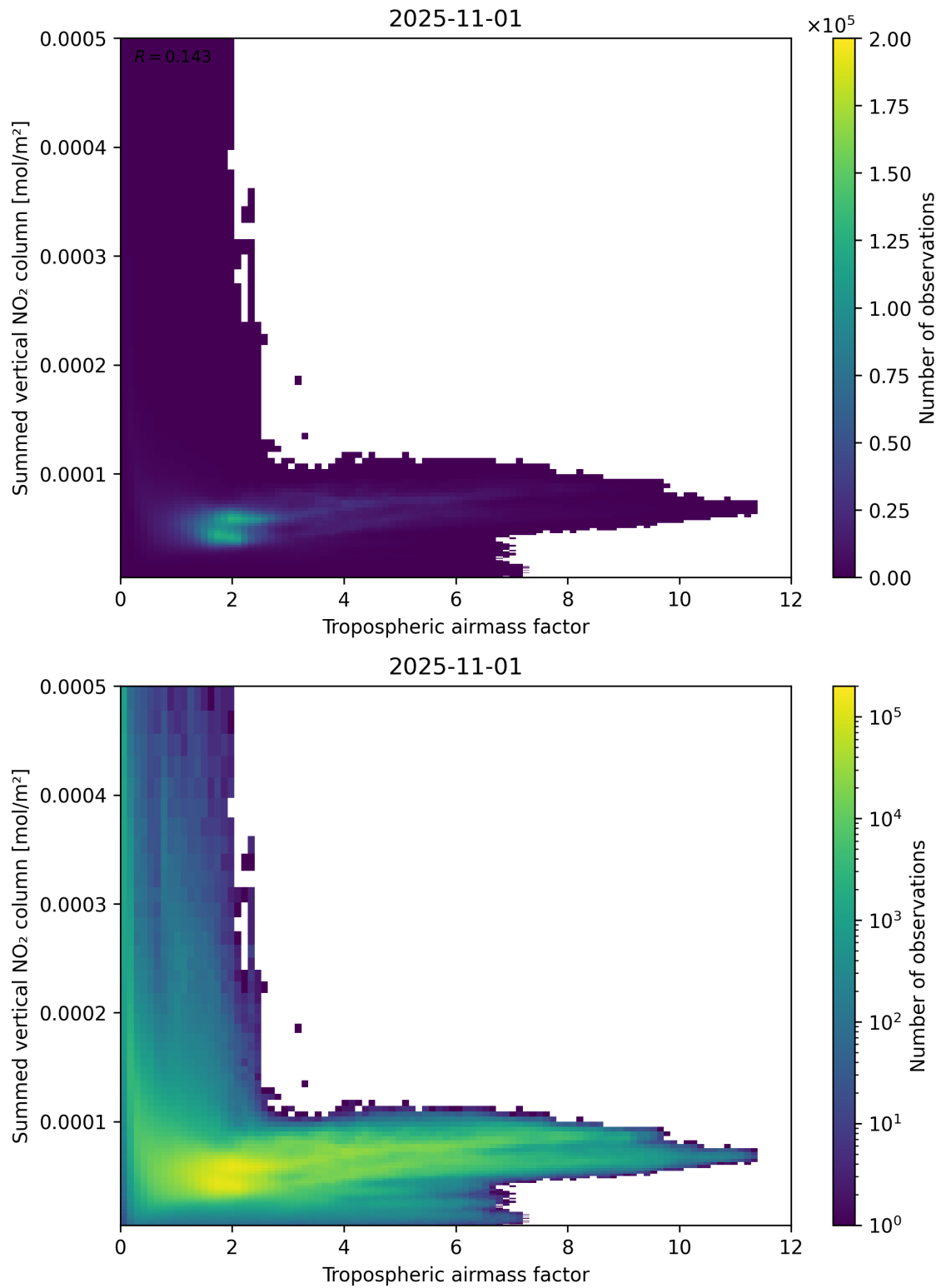
Figure 75: Scatter density plot of “Tropospheric airmass factor” against “Summed vertical NO 2 column” for 2025-10-31 to 2025-11-02.
