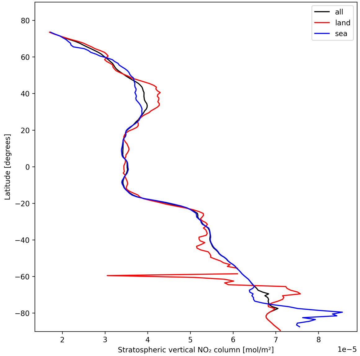
Figure 19: Zonal average of “Stratospheric vertical NO 2 column” for 2025-10-31 to 2025-11-02.
