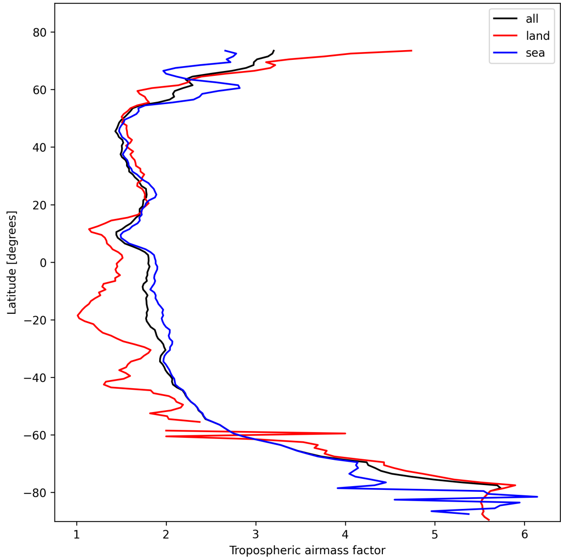
Figure 14: Zonal average of “Tropospheric airmass factor” for 2025-10-31 to 2025-11-02.
