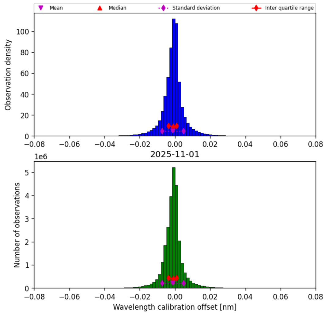
Figure 35: Histogram of “Wavelength calibration offset” for 2025-10-31 to 2025-11-02
