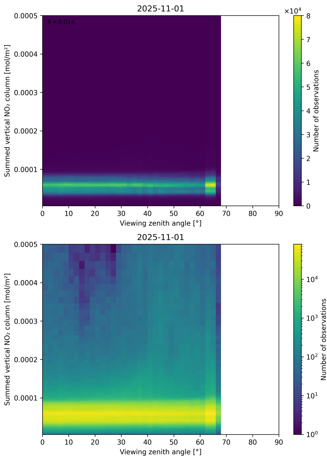
Figure 165: Scatter density plot of “Viewing zenith angle” against “Summed vertical NO 2 column” for 2025-10-31 to 2025-11-02.
