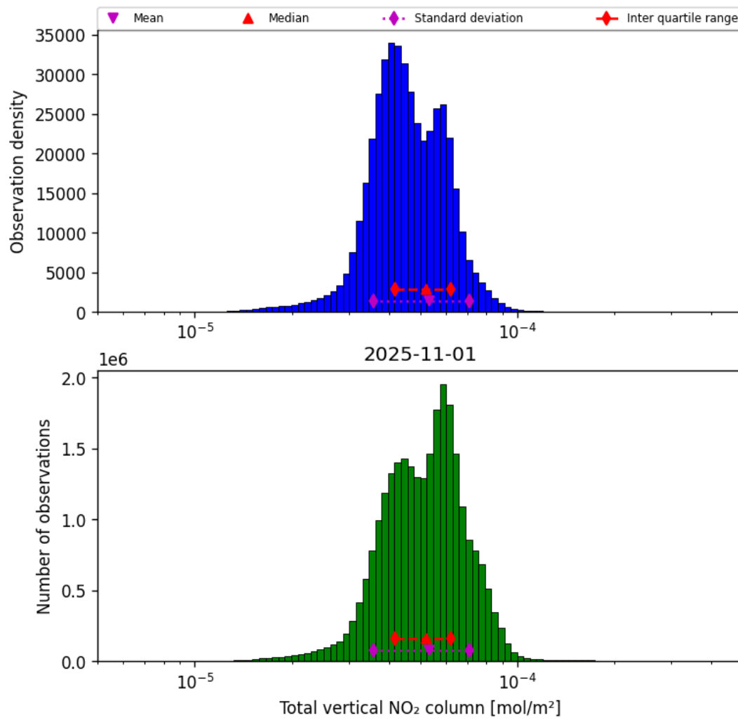
Figure 38: Histogram of “Total vertical NO 2 column” for 2025-10-31 to 2025-11-02
