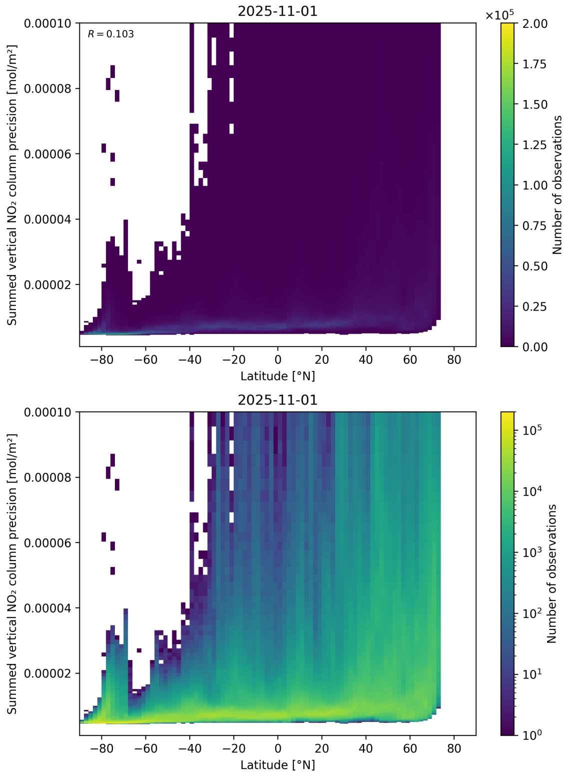
Figure 89: Scatter density plot of “Latitude” against “Summed vertical NO 2 column precision” for 2025-10-31 to 2025-11-02.
