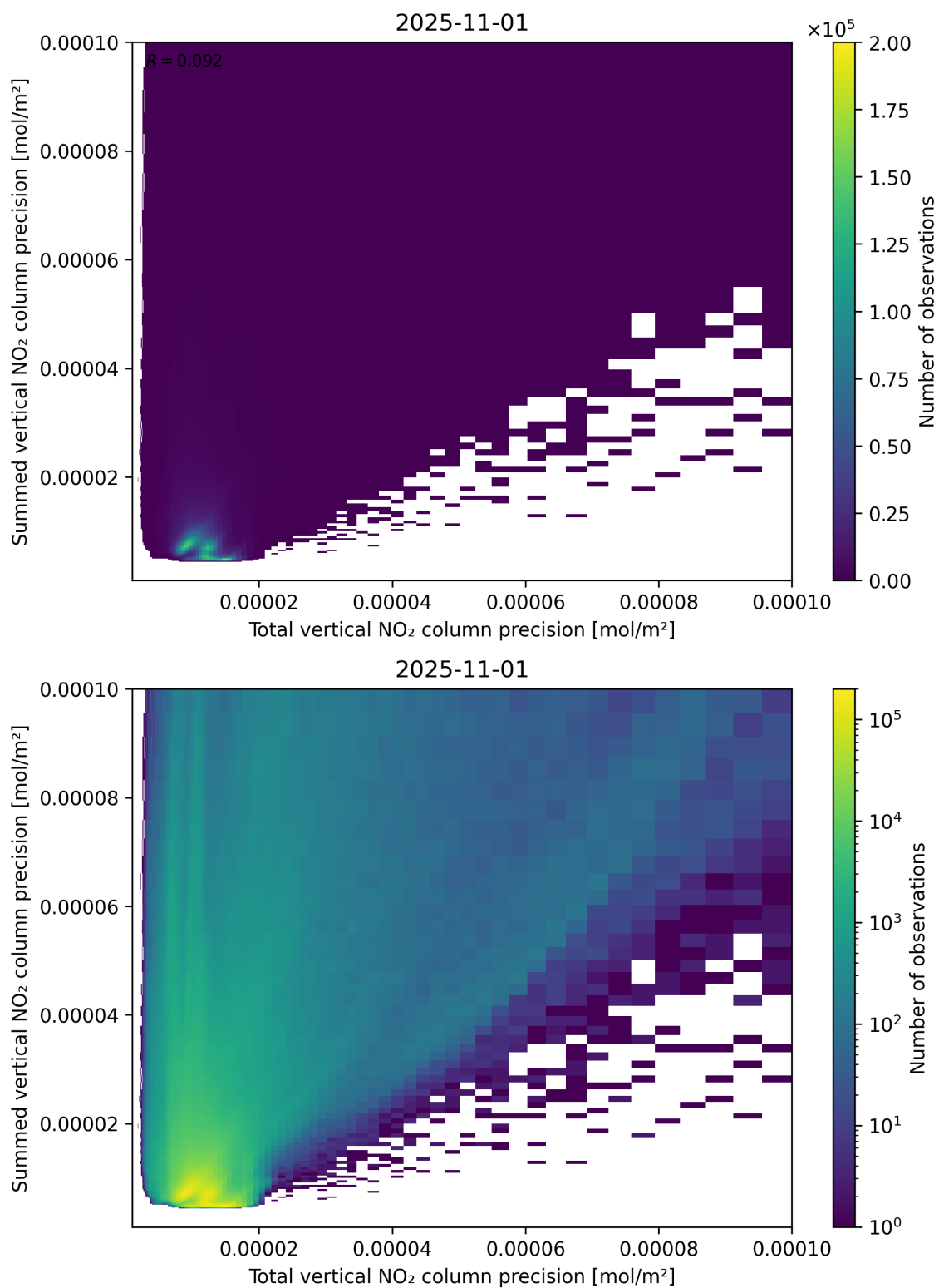
Figure 118: Scatter density plot of “Total vertical NO 2 column precision” against “Summed vertical NO 2 column precision” for 2025-10-31 to 2025-11-02.
