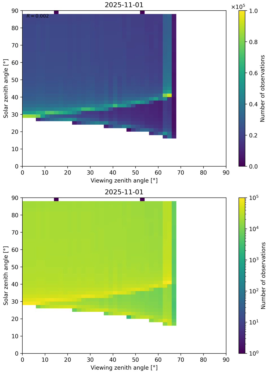
Figure 172: Scatter density plot of “Viewing zenith angle” against “Solar zenith angle” for 2025-10-31 to 2025-11-02.
