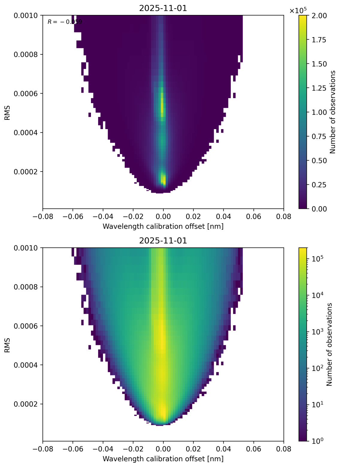
Figure 181: Scatter density plot of “Wavelength calibration offset” against “RMS” for 2025-10-31 to 2025-11-02.
