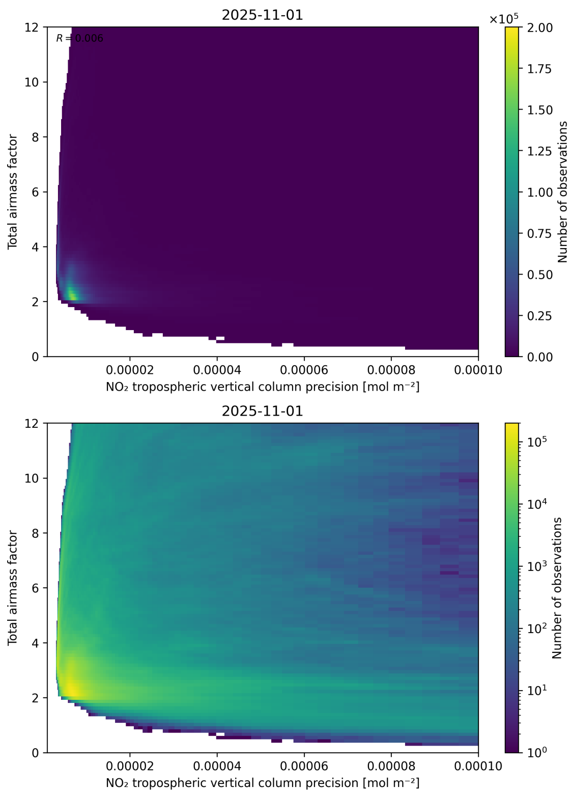
Figure 132: Scatter density plot of “NO 2 tropospheric vertical column precision” against “Total air mass factor” for 2025-10-31 to 2025-11-02.
