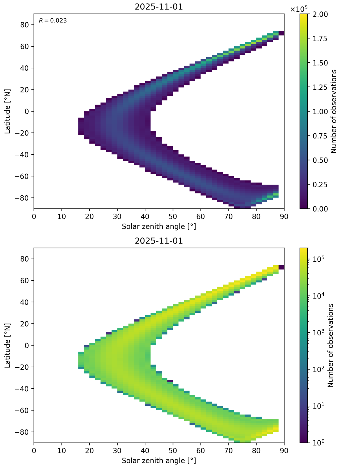
Figure 149: Scatter density plot of “Solar zenith angle” against “Latitude” for 2025-10-31 to 2025-11-02.
