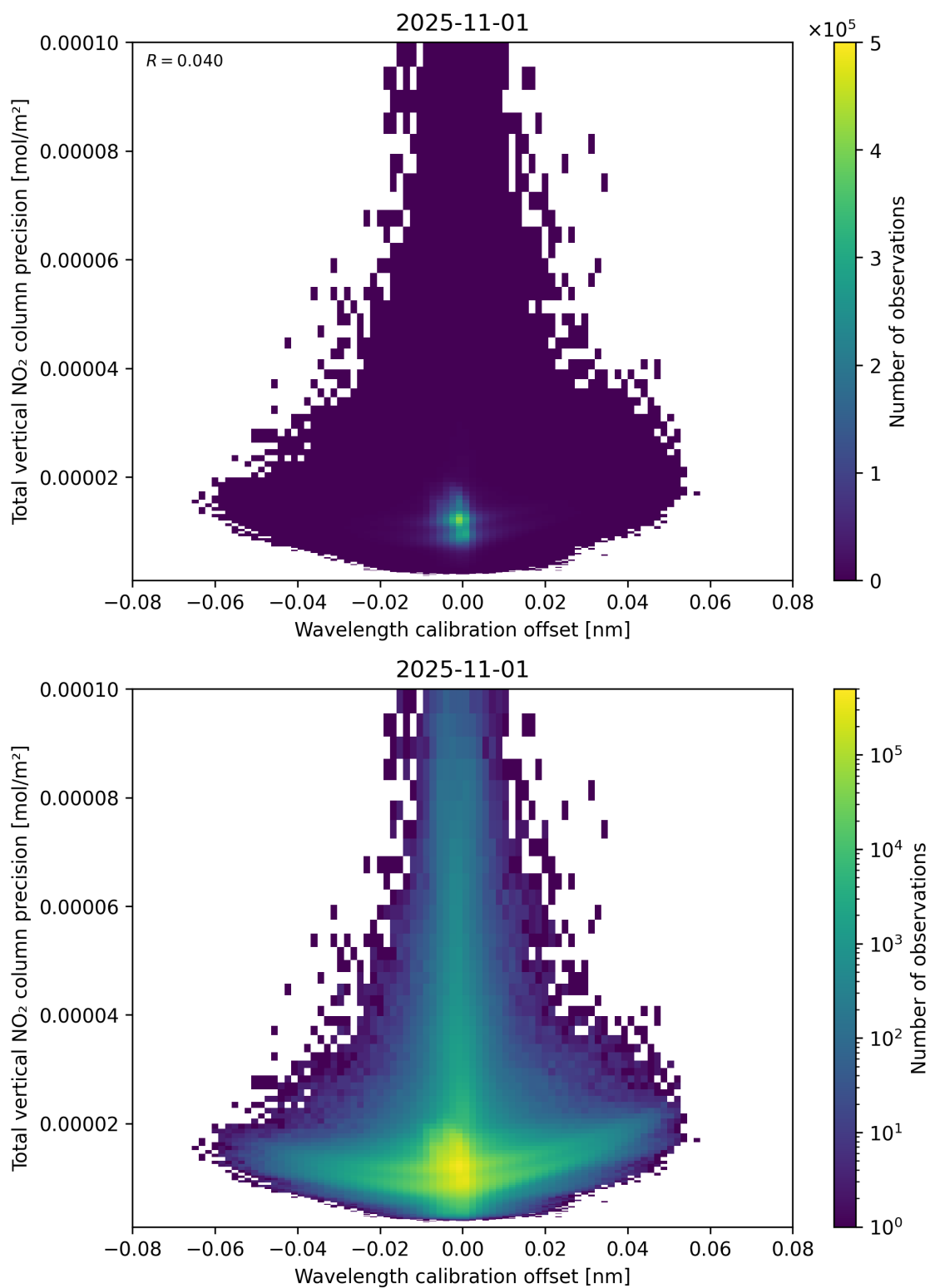
Figure 180: Scatter density plot of “Wavelength calibration offset” against “Total vertical NO 2 column precision” for 2025-10-31 to 2025-11-02.
