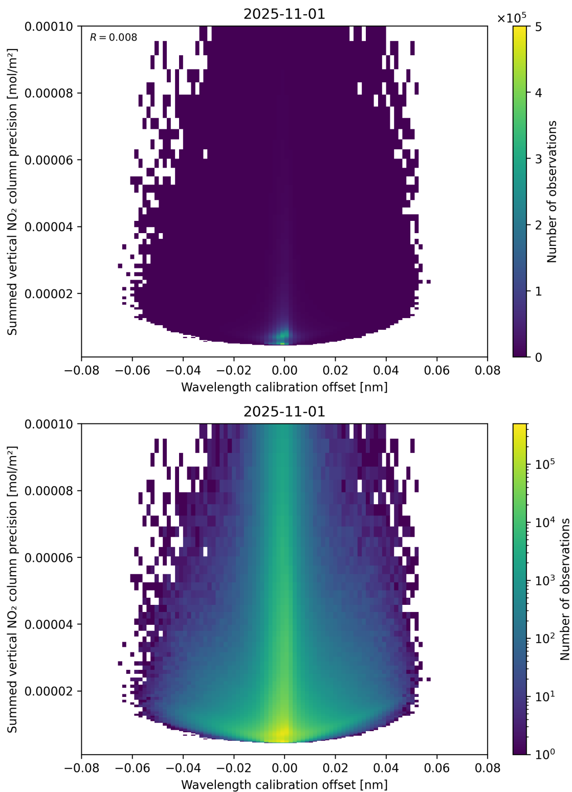
Figure 178: Scatter density plot of “Wavelength calibration offset” against “Summed vertical NO 2 column precision” for 2025-10-31 to 2025-11-02.
