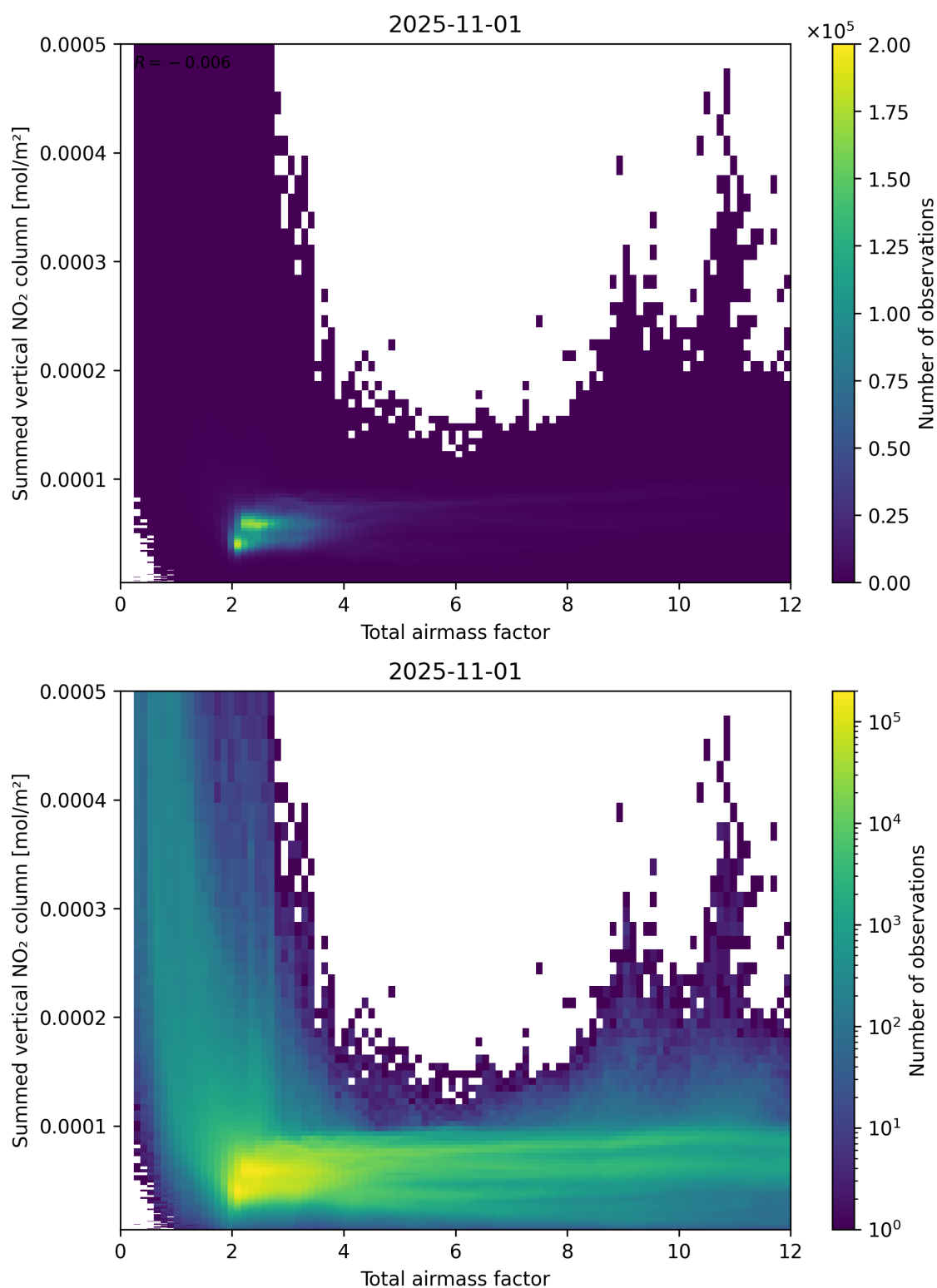
Figure 65: Scatter density plot of “Total airmass factor” against “Summed vertical NO 2 column” for 2025-10-31 to 2025-11-02.
