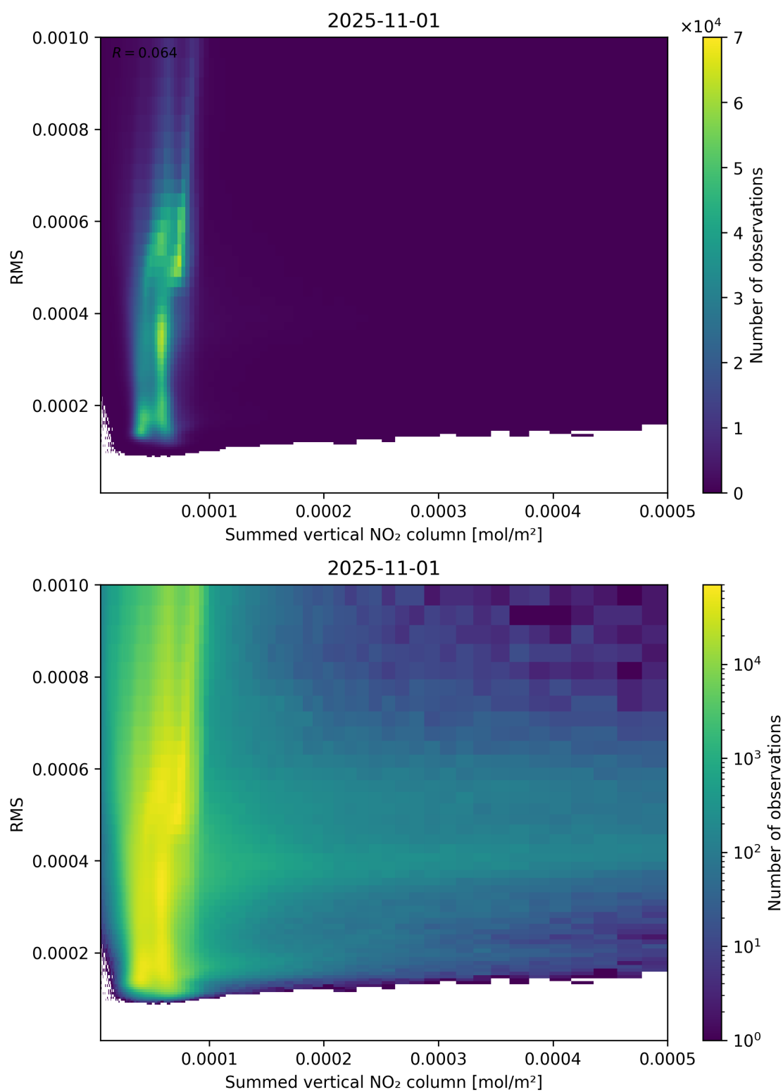
Figure 109: Scatter density plot of “Summed vertical NO 2 column” against “RMS” for 2025-10-31 to 2025-11-02.
