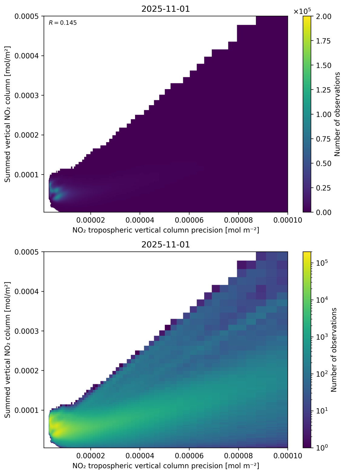
Figure 136: Scatter density plot of “NO 2 tropospheric vertical column precision” against “Summed vertical NO 2 column” for 2025-10-31 to 2025-11-02.
