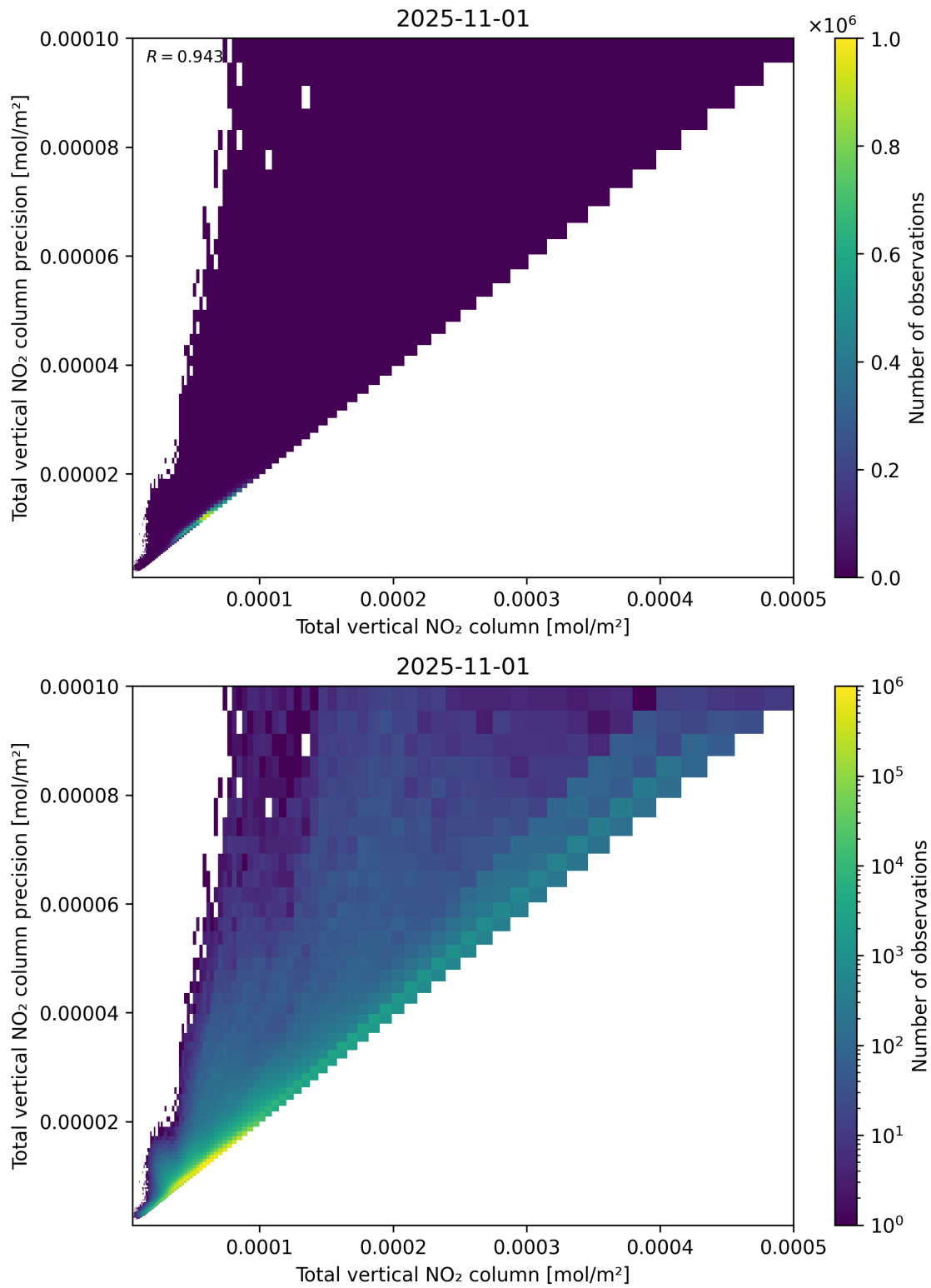
Figure 114: Scatter density plot of “Total vertical NO 2 column” against “Total vertical NO 2 column precision” for 2025-10-31 to 2025-11-02.
