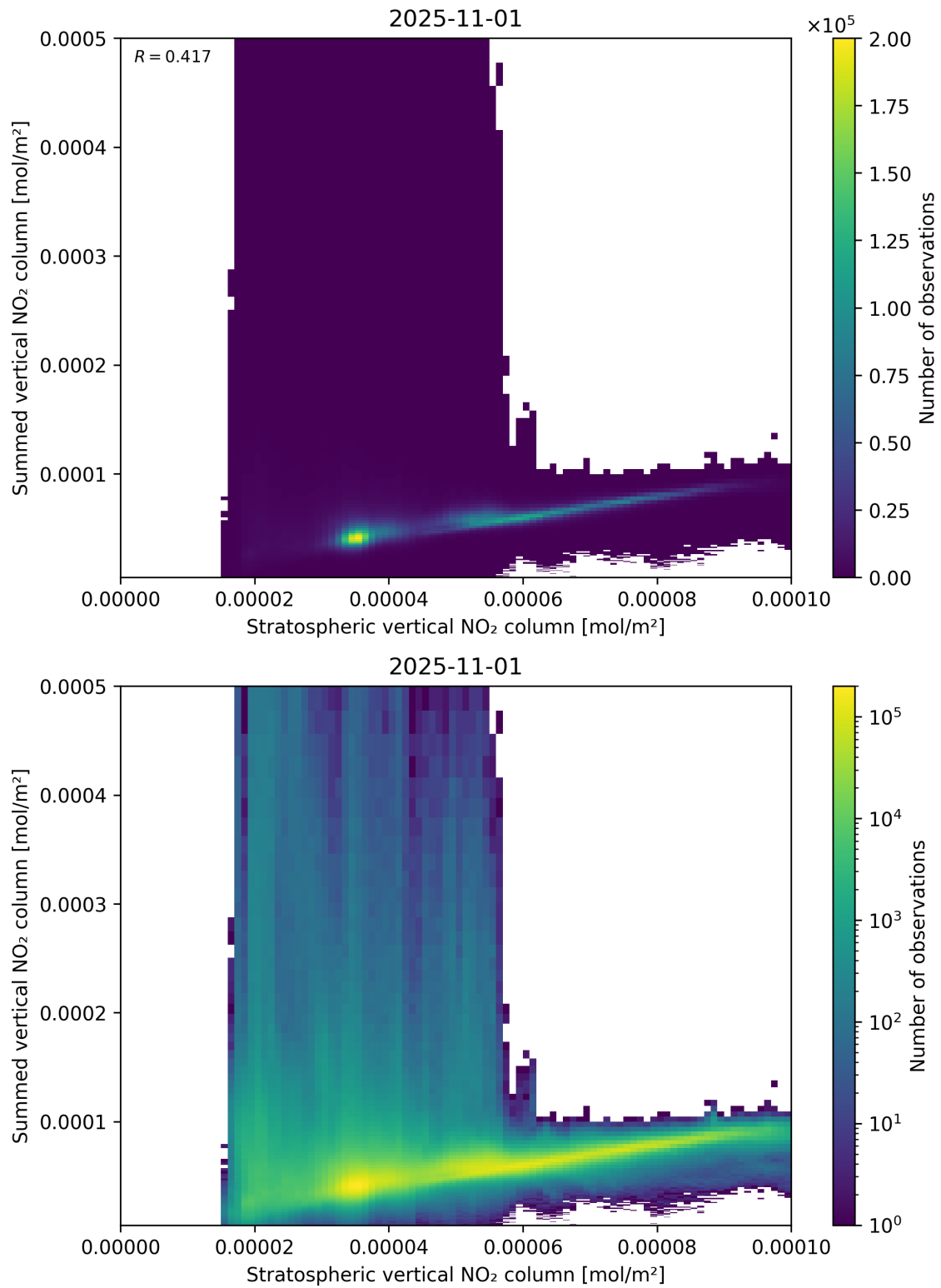
Figure 98: Scatter density plot of “Stratospheric vertical NO 2 column” against “Summed vertical NO 2 column” for 2025-10-31 to 2025-11-02.
