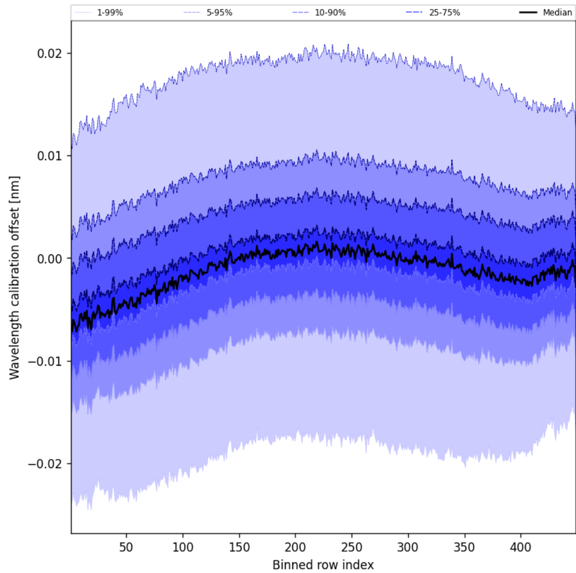
Figure 52: Along track statistics of “Wavelength calibration offset” for 2025-10-31 to 2025-11-02
