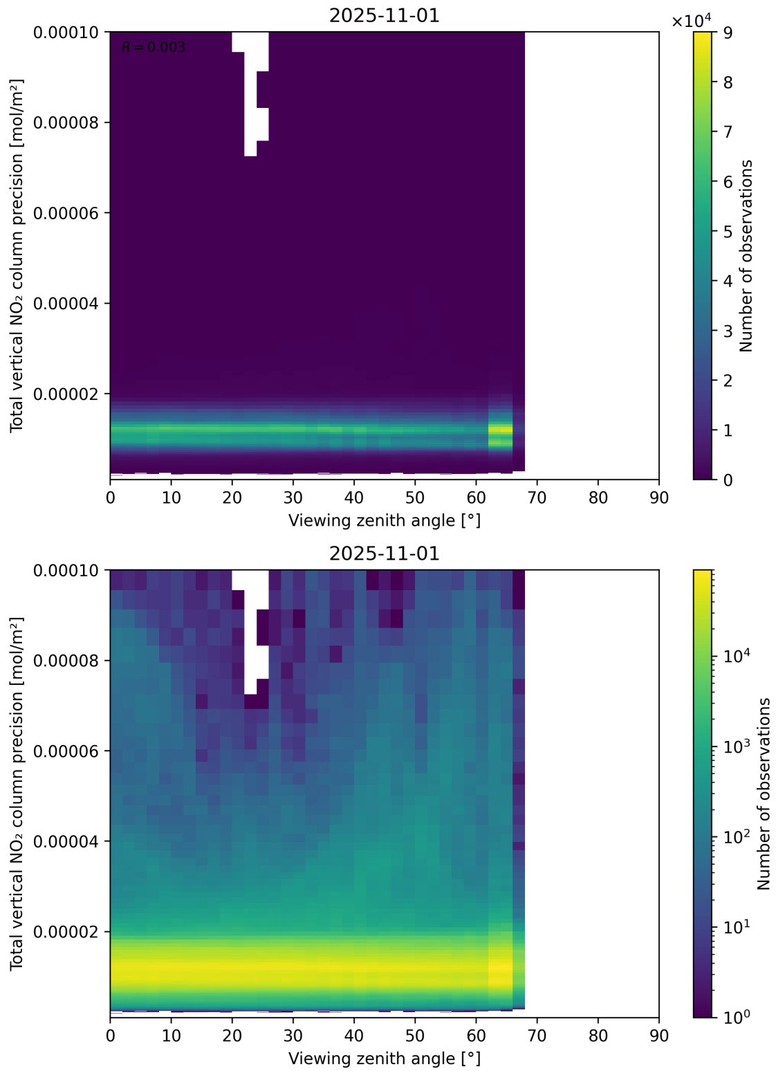
Figure 168: Scatter density plot of “Viewing zenith angle” against “Total vertical NO 2 column precision” for 2025-10-31 to 2025-11-02.
