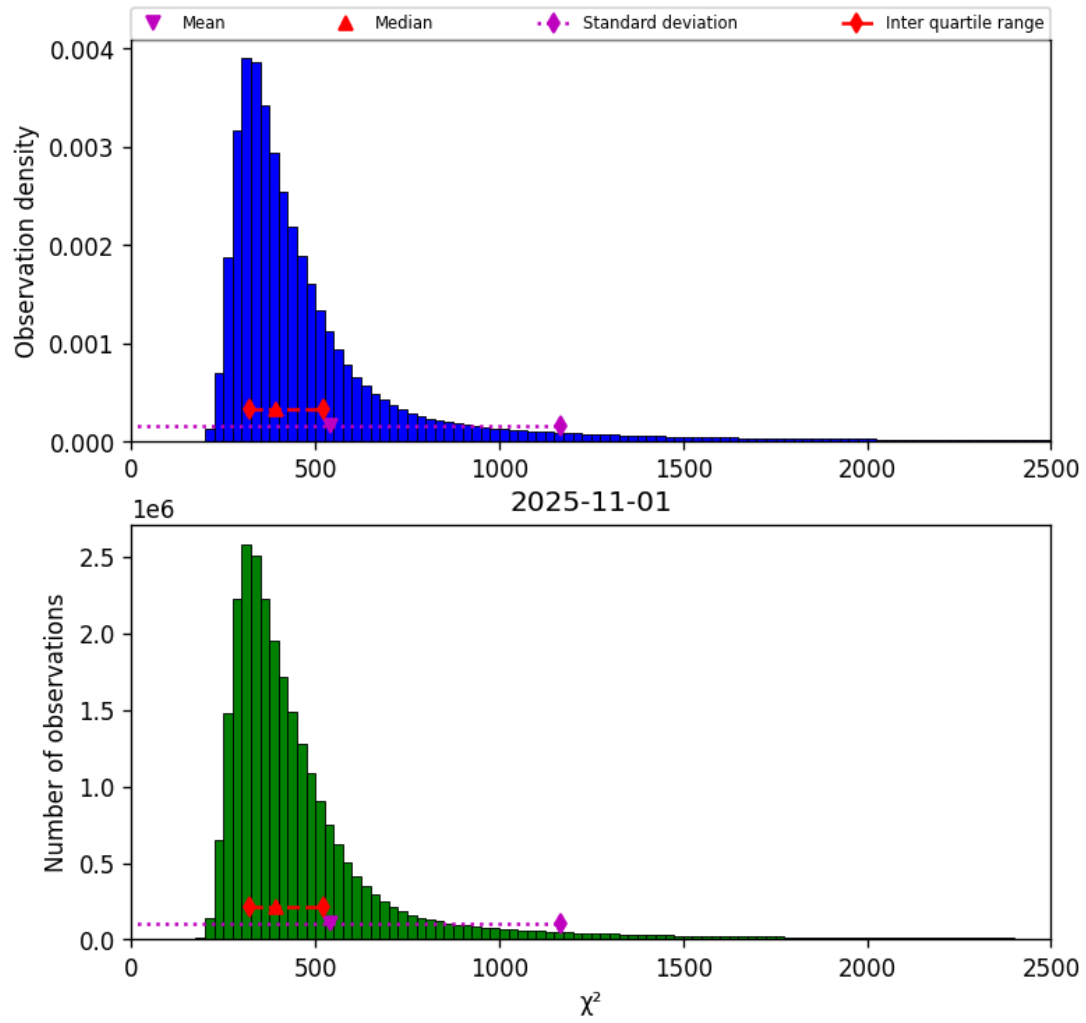
Figure 42: Histogram of “ \chi^2 ” for 2025-10-31 to 2025-11-02
