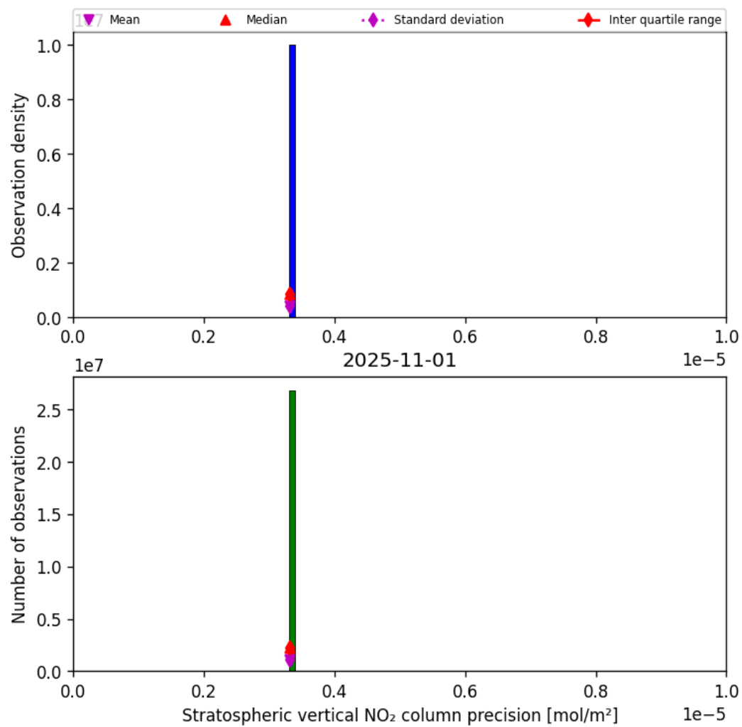
Figure 37: Histogram of “Stratospheric vertical NO 2 column precision” for 2025-10-31 to 2025-11-02
