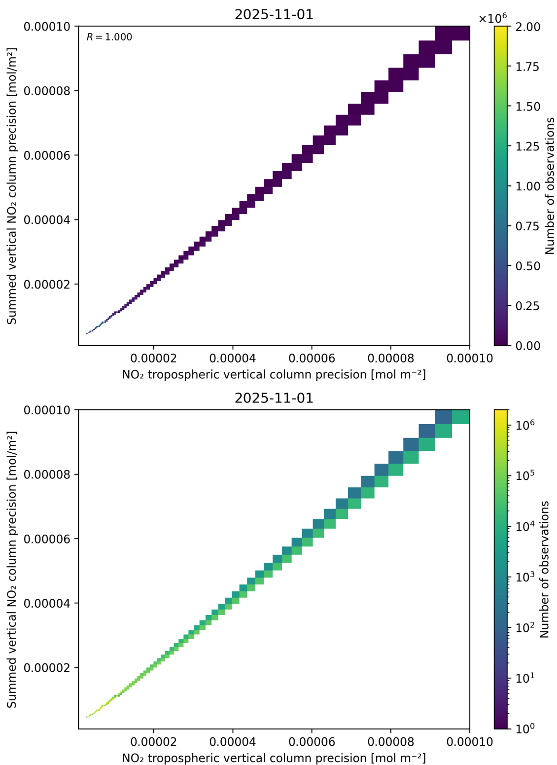
Figure 137: Scatter density plot of “NO 2 tropospheric vertical column precision” against “Summed vertical NO 2 column precision” for 2025-10-31 to 2025-11-02.
