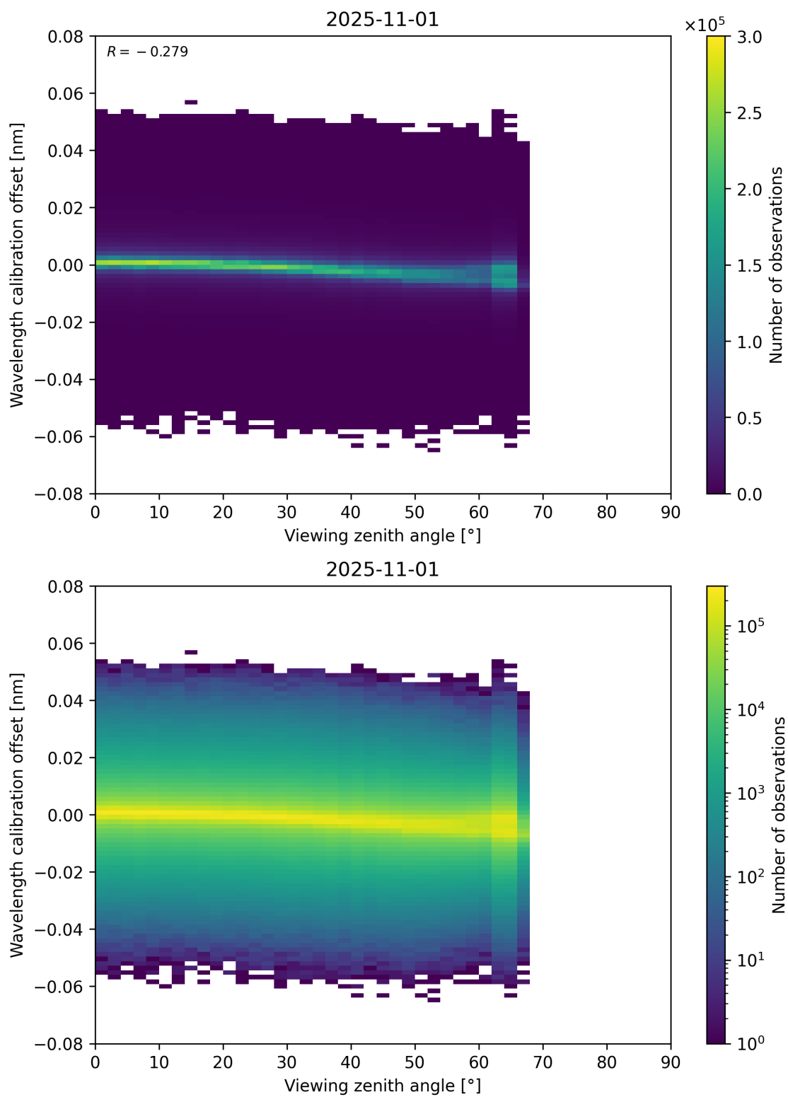
Figure 173: Scatter density plot of “Viewing zenith angle” against “Wavelength calibration offset” for 2025-10-31 to 2025-11-02.
