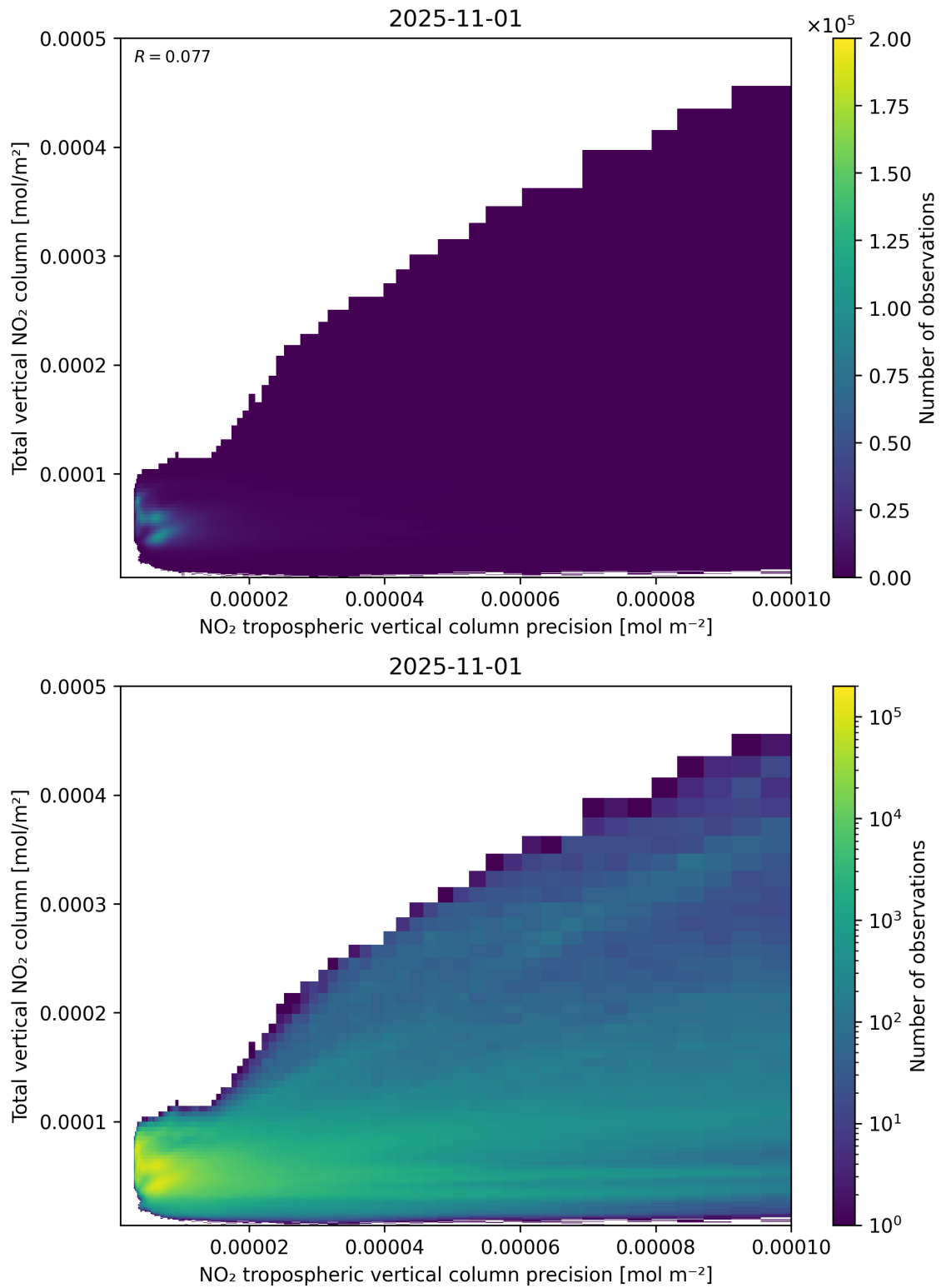
Figure 138: Scatter density plot of “NO 2 tropospheric vertical column precision” against “Total vertical NO 2 column” for 2025-10-31 to 2025-11-02.
