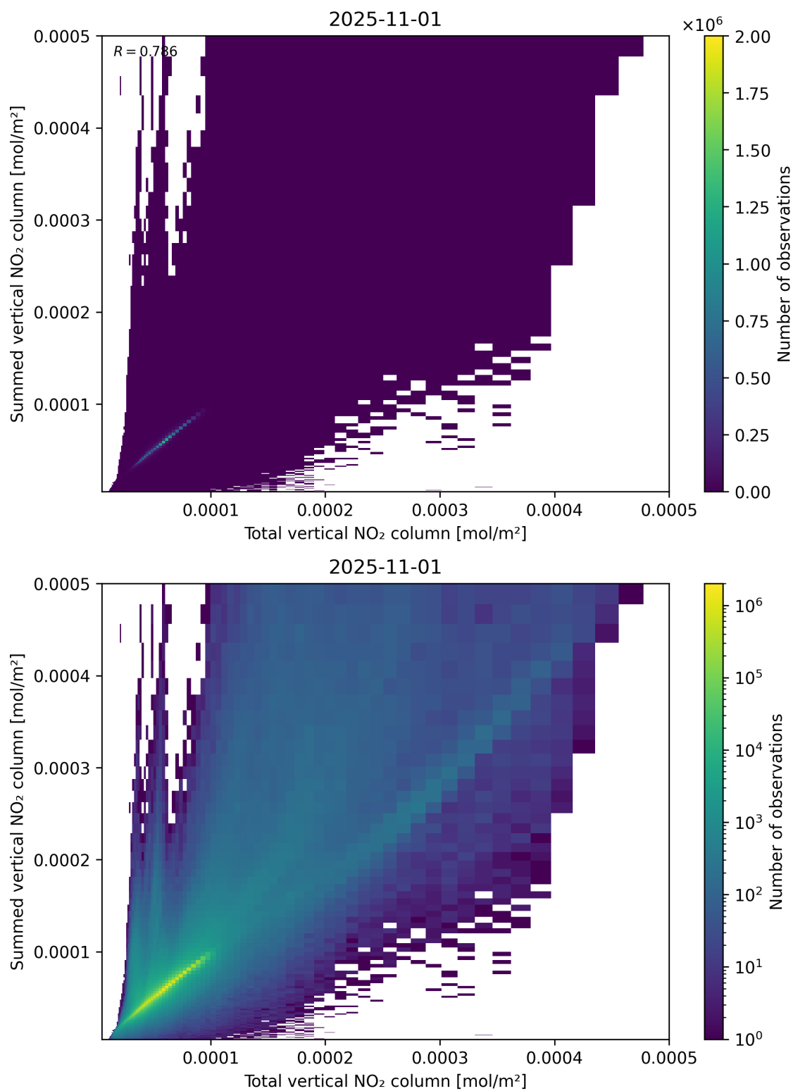
Figure 112: Scatter density plot of “Total vertical NO 2 column” against “Summed vertical NO 2 column” for 2025-10-31 to 2025-11-02.
