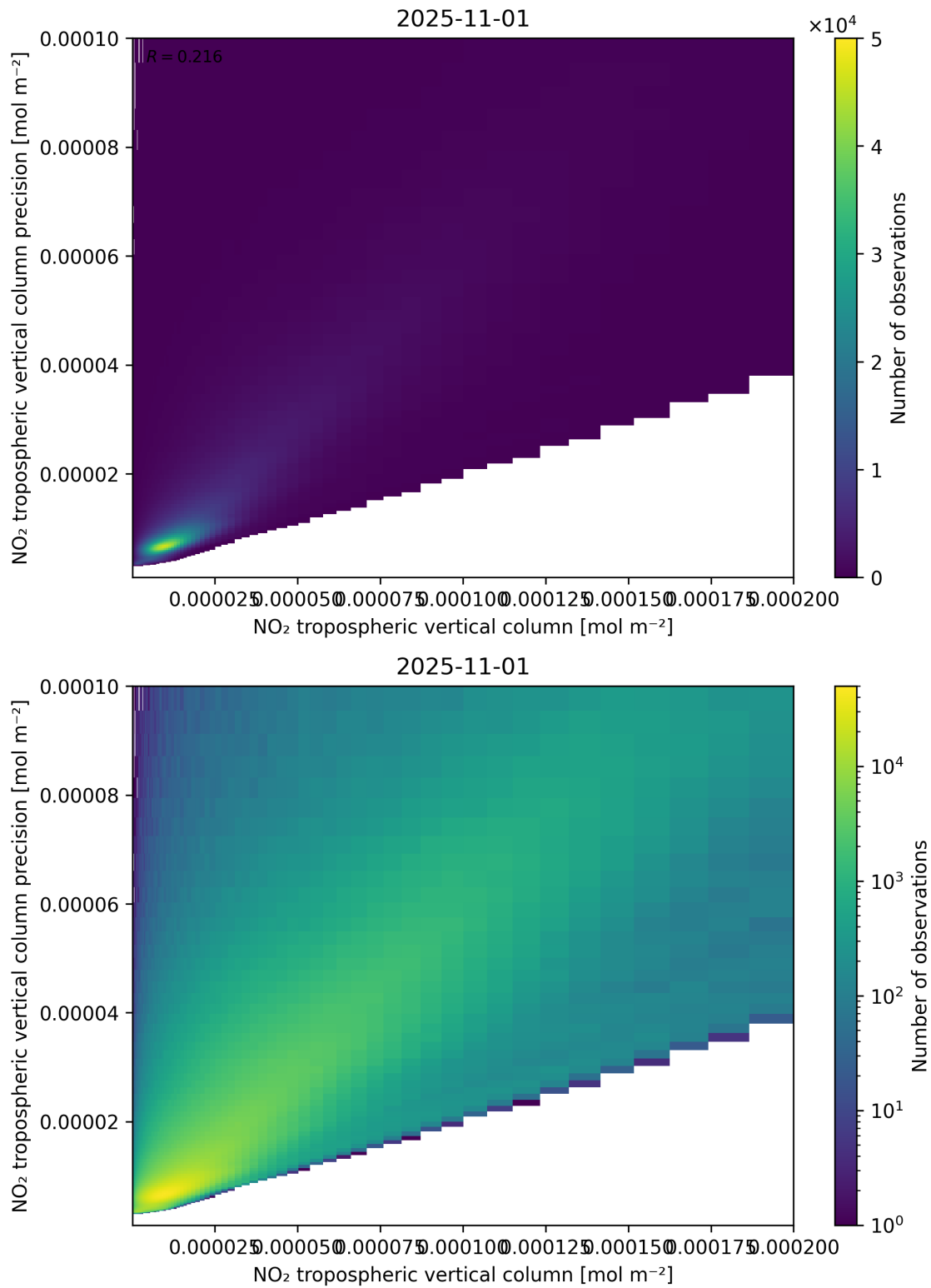
Figure 130: Scatter density plot of “NO 2 tropospheric vertical column” against “NO 2 tropospheric vertical column precision” for 2025-10-31 to 2025-11-02.
