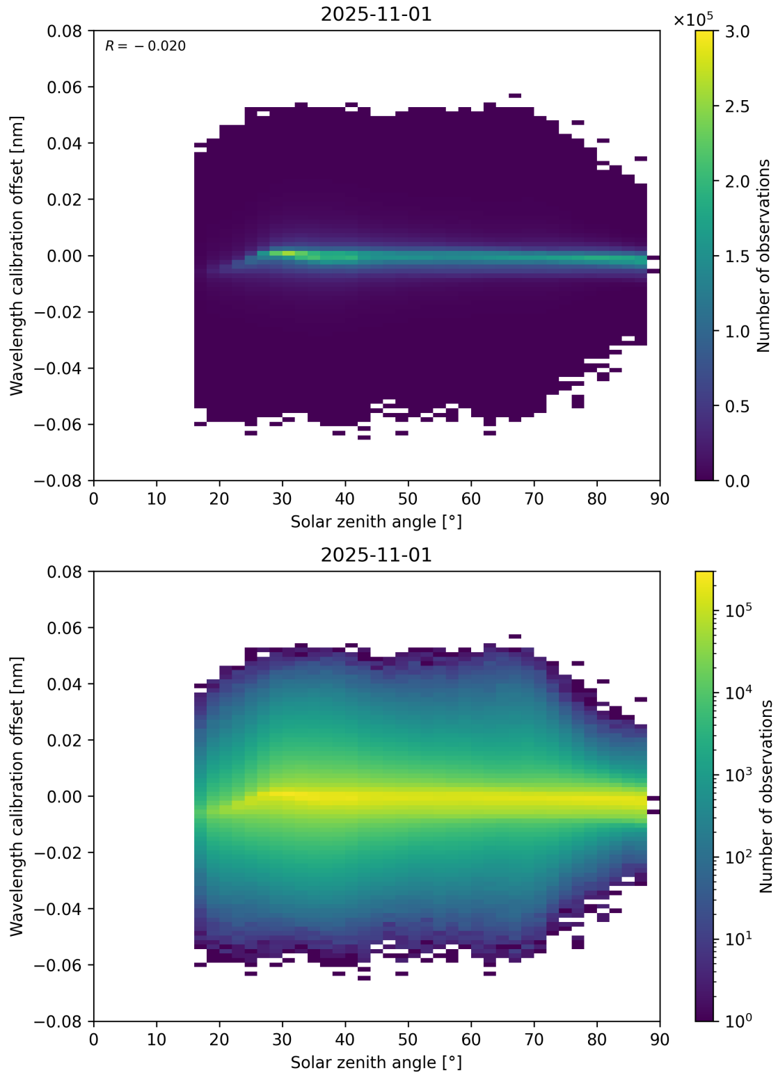
Figure 158: Scatter density plot of “Solar zenith angle” against “Wavelength calibration offset” for 2025-10-31 to 2025-11-02.
