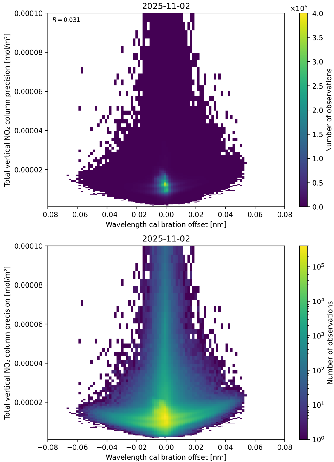
Figure 180: Scatter density plot of “Wavelength calibration offset” against “Total vertical NO 2 column precision” for 2025-11-02 to 2025-11-03.
