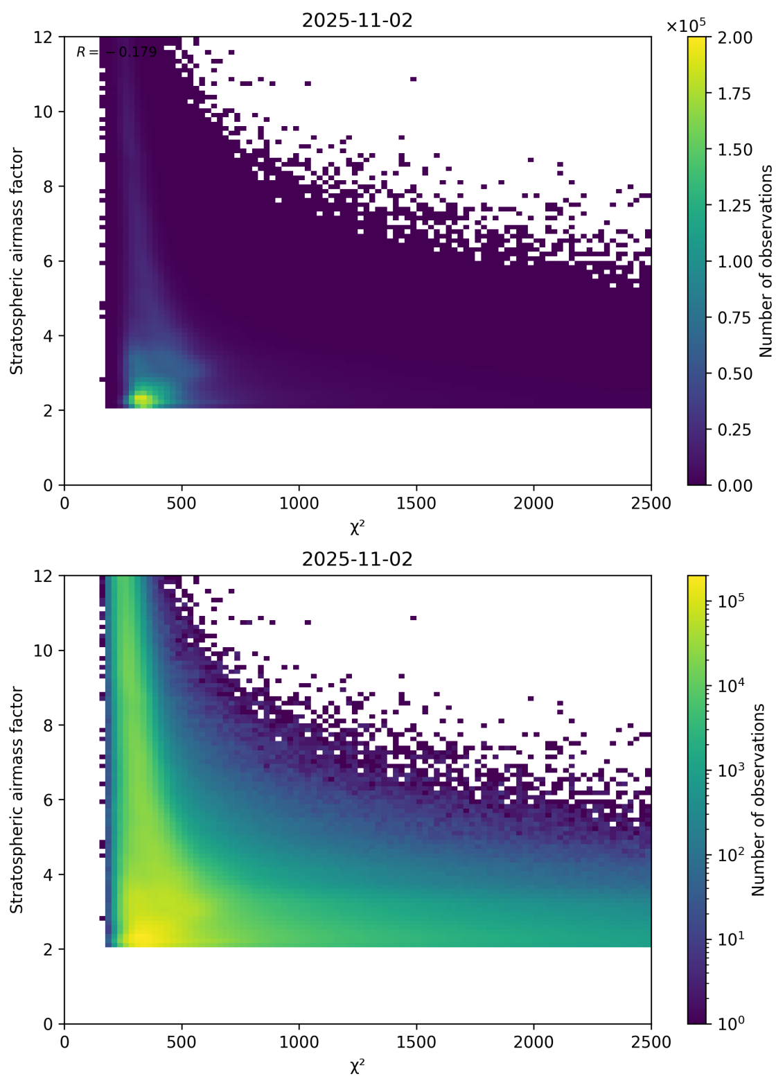
Figure 81: Scatter density plot of “ \chi^2 ” against “Stratospheric airmass factor” for 2025-11-02 to 2025-11-03.
