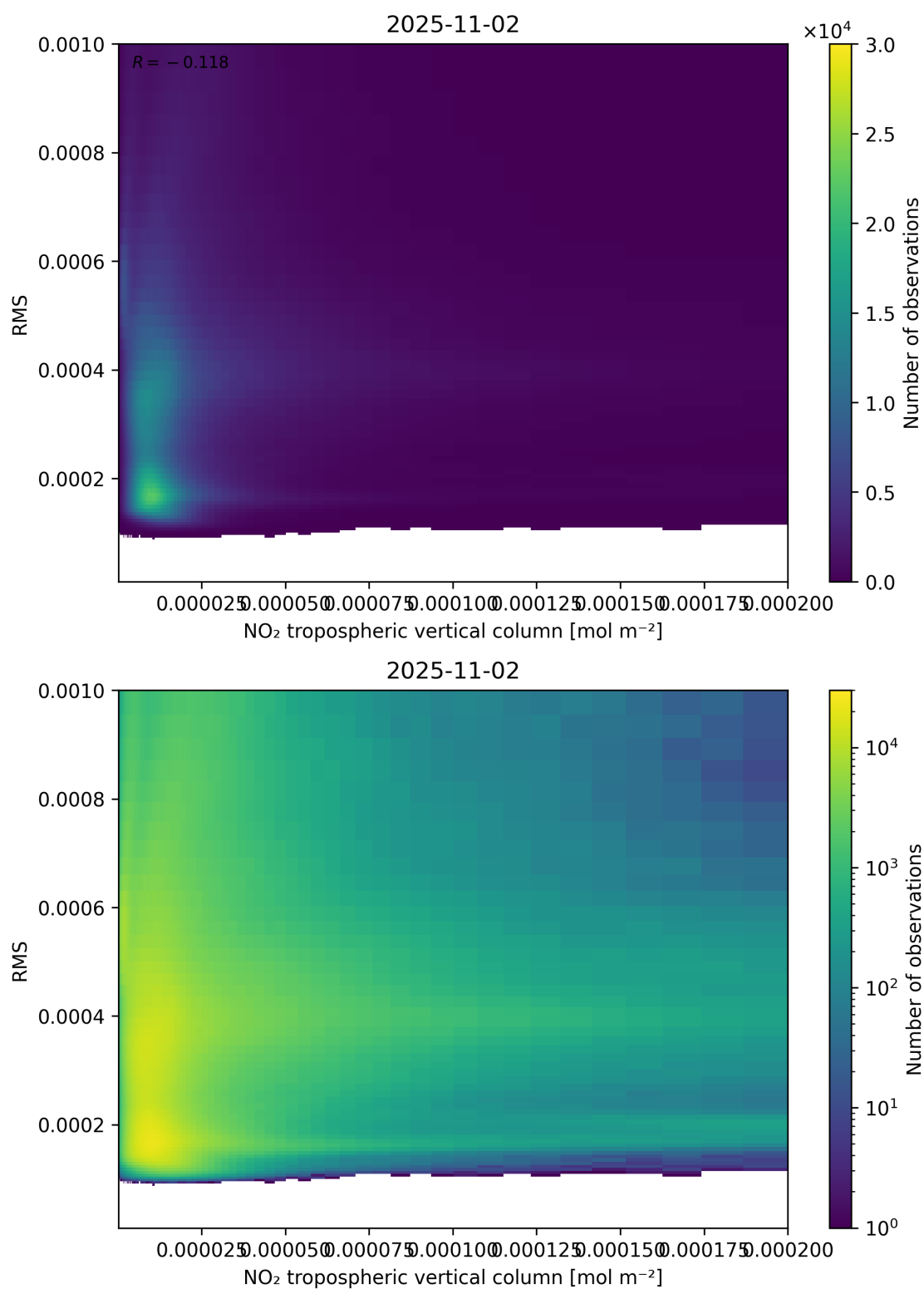
Figure 142: Scatter density plot of “NO 2 tropospheric vertical column” against “RMS” for 2025-11-02 to 2025-11-03.
