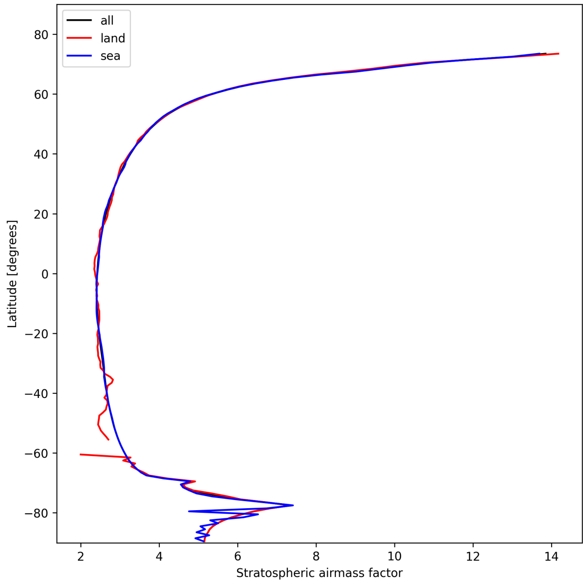
Figure 27: Zonal average of “Stratospheric air mass factor” for 2025-11-02 to 2025-11-03.
