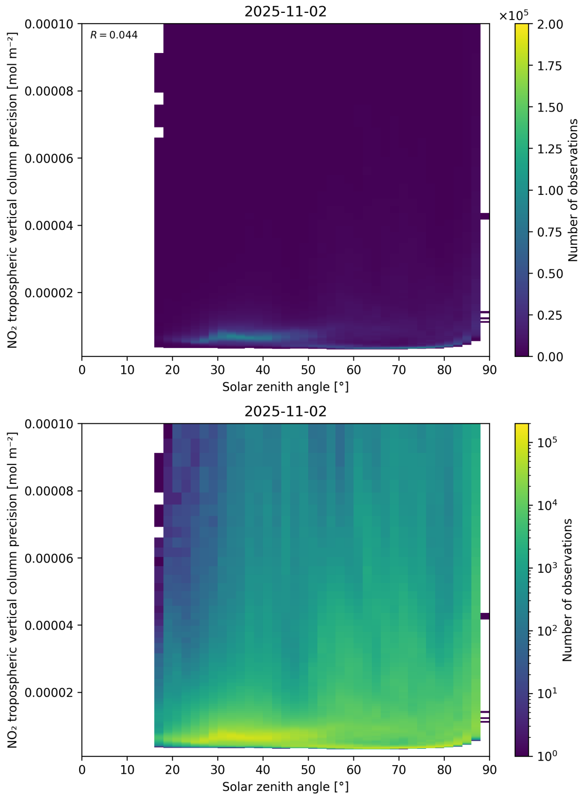
Figure 156: Scatter density plot of “Solar zenith angle” against “NO 2 tropospheric vertical column precision” for 2025-11-02 to 2025-11-03.
