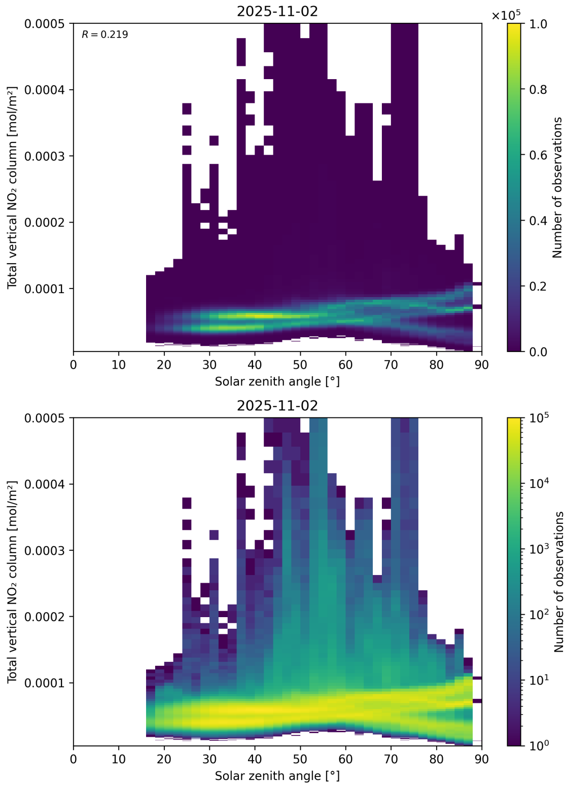
Figure 153: Scatter density plot of “Solar zenith angle” against “Total vertical NO 2 column” for 2025-11-02 to 2025-11-03.
