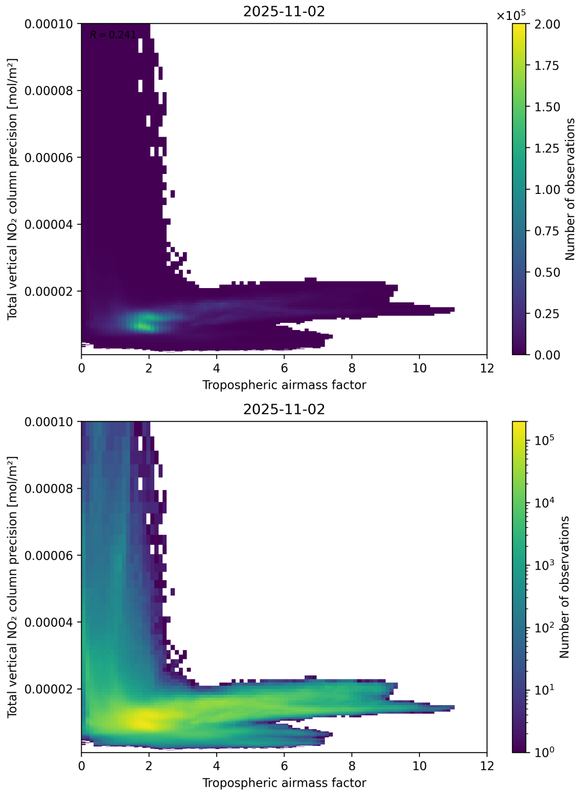
Figure 78: Scatter density plot of “Tropospheric air mass factor” against “Total vertical NO 2 column precision” for 2025-11-02 to 2025-11-03.
