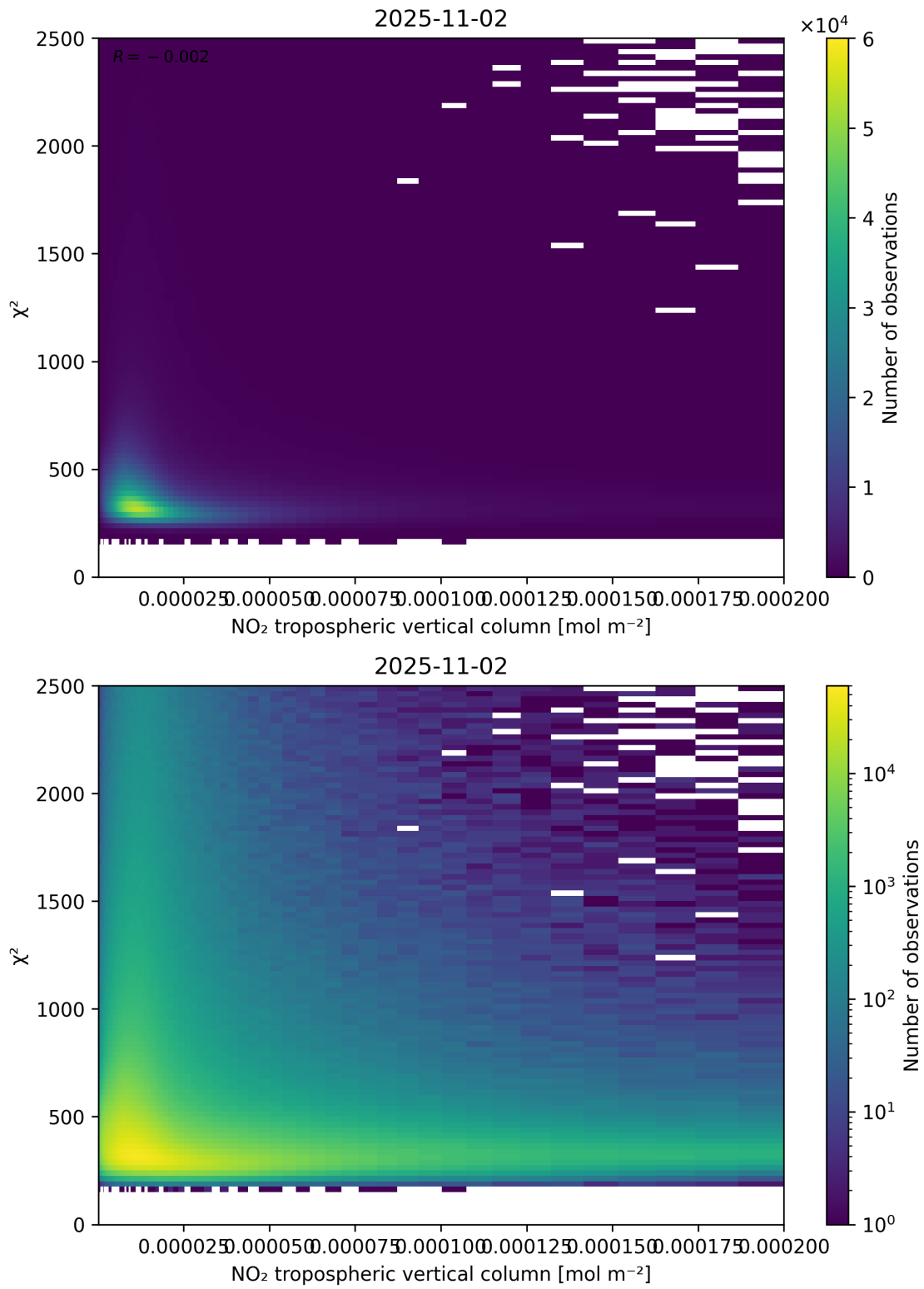
Figure 124: Scatter density plot of “NO 2 tropospheric vertical column” against “ \chi^2 ” for 2025-11-02 to 2025-11-03.
