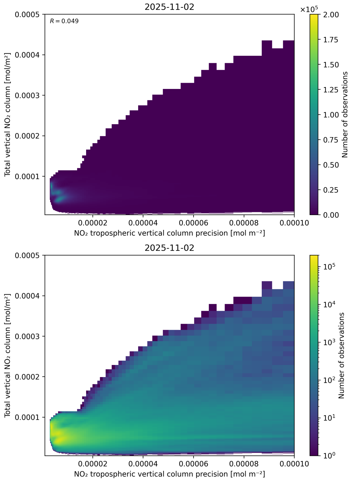
Figure 138: Scatter density plot of “NO 2 tropospheric vertical column precision” against “Total vertical NO 2 column” for 2025-11-02 to 2025-11-03.
