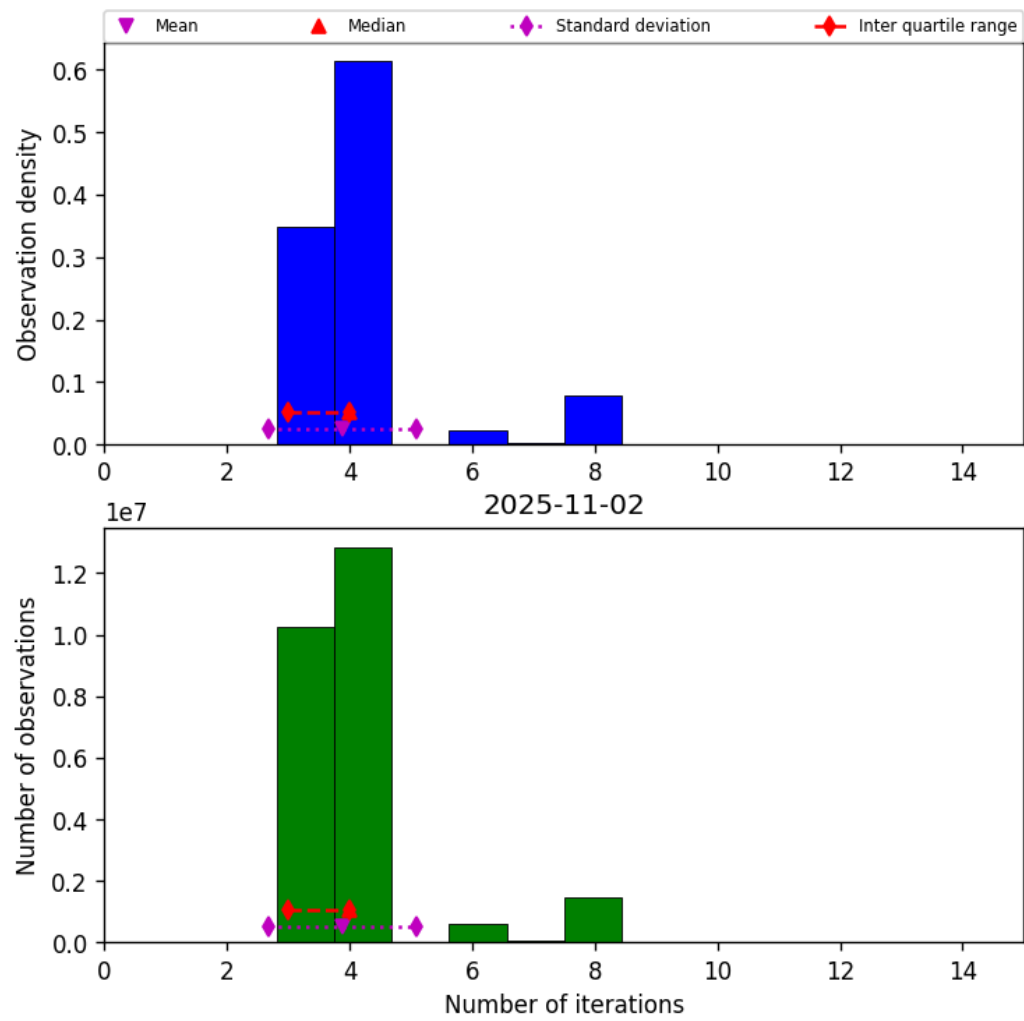
Figure 34: Histogram of “Number of iterations” for 2025-11-02 to 2025-11-03
