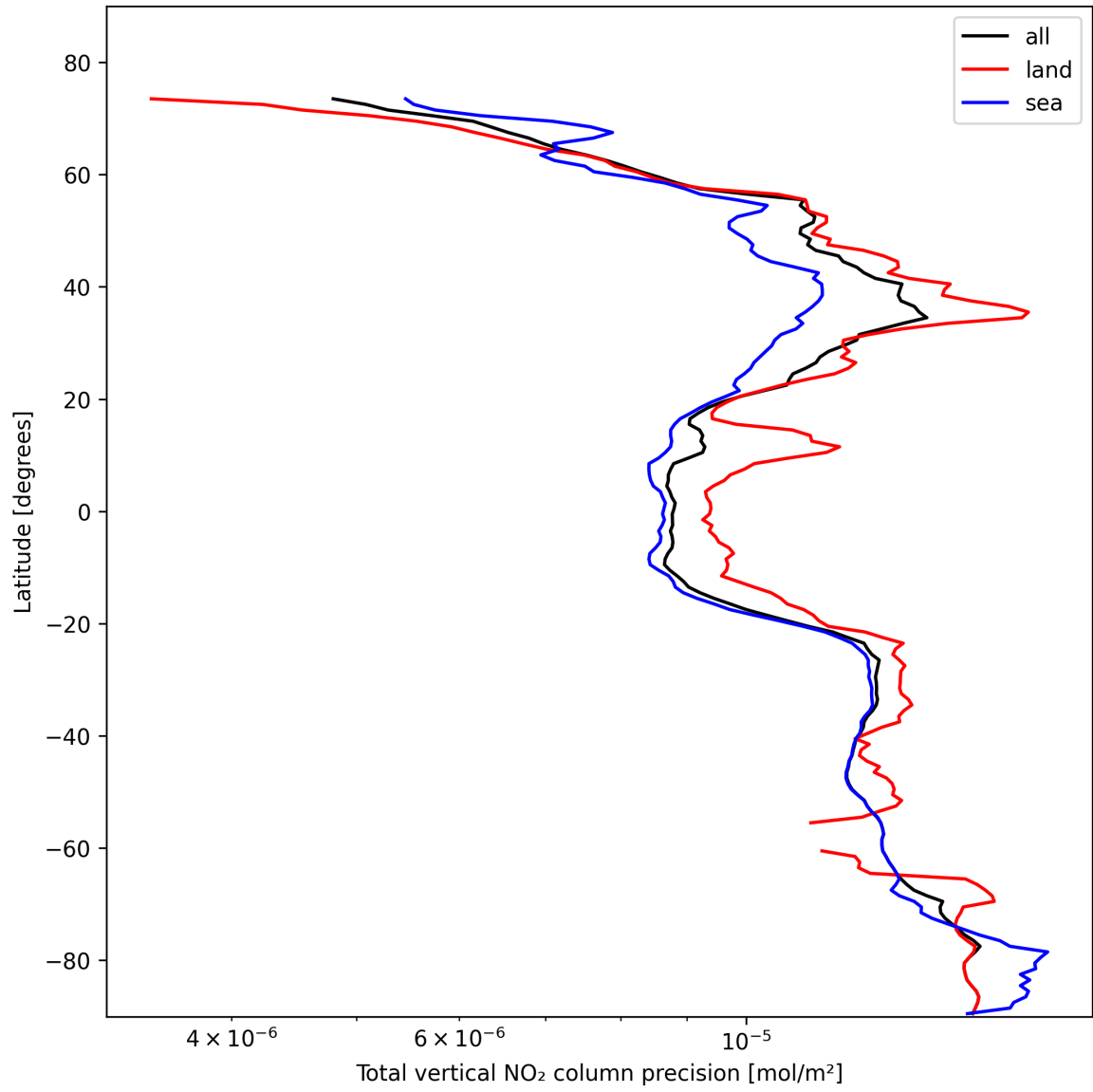
Figure 22: Zonal average of “Total vertical NO 2 column precision” for 2025-11-02 to 2025-11-03.
