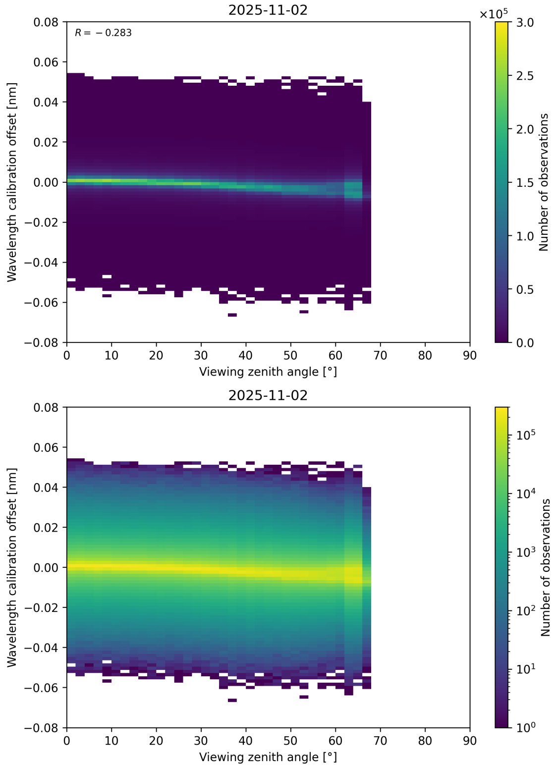
Figure 173: Scatter density plot of “Viewing zenith angle” against “Wavelength calibration offset” for 2025-11-02 to 2025-11-03.
