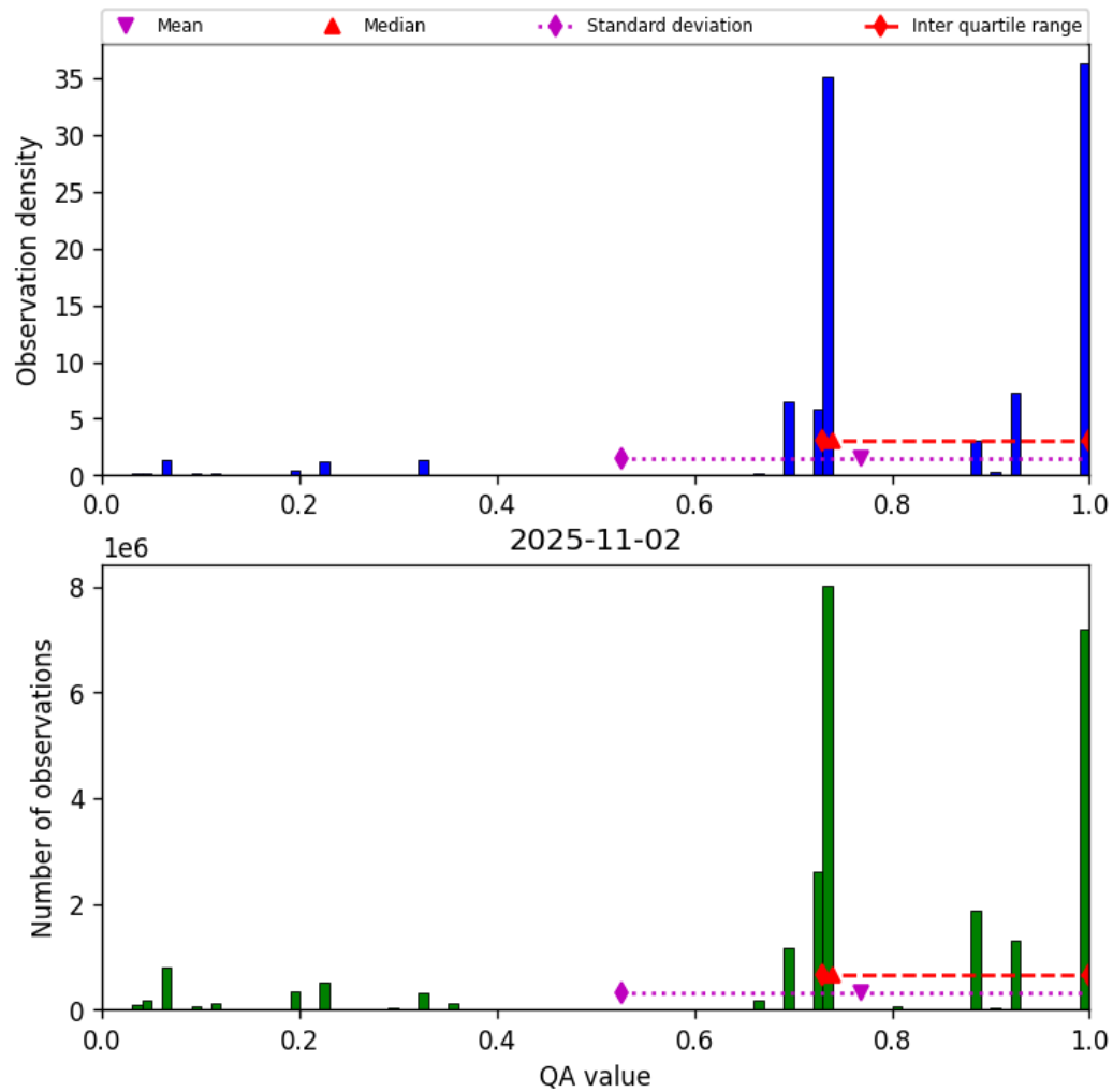
Figure 28: Histogram of “QA value” for 2025-11-02 to 2025-11-03
