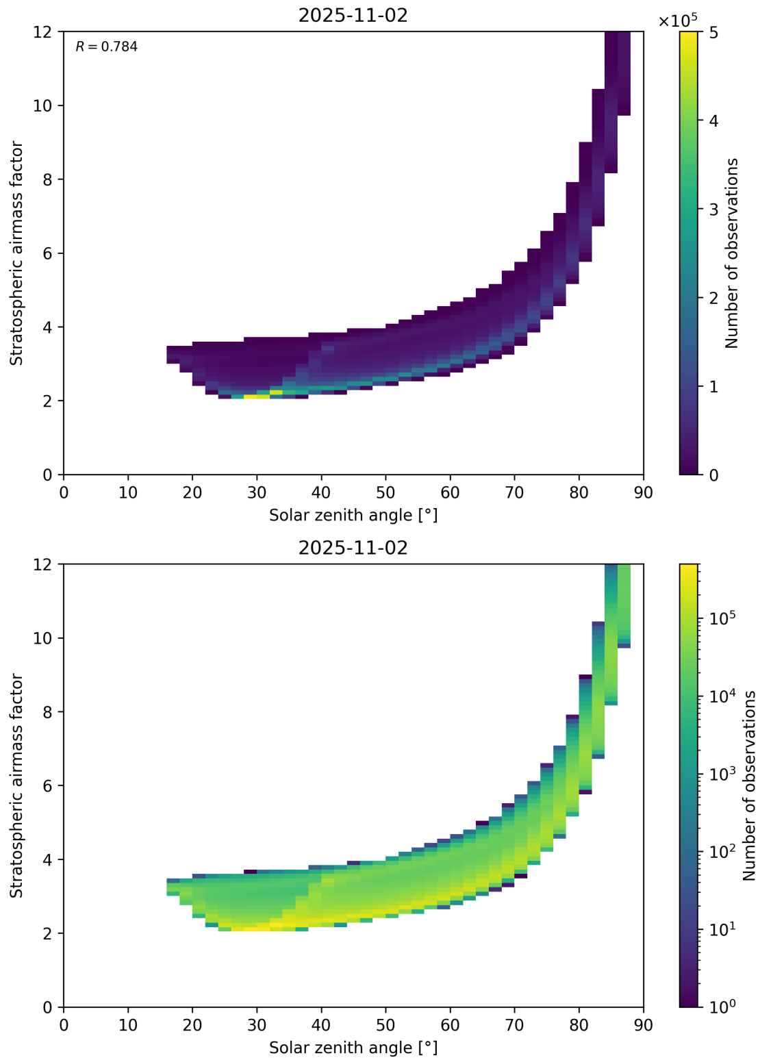
Figure 145: Scatter density plot of “Solar zenith angle” against “Stratospheric airmass factor” for 2025-11-02 to 2025-11-03.
