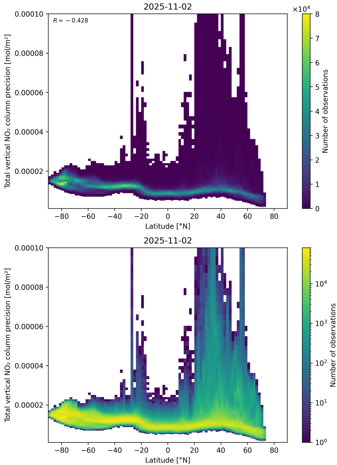
Figure 91: Scatter density plot of “Latitude” against “Total vertical NO 2 column precision” for 2025-11-02 to 2025-11-03.
