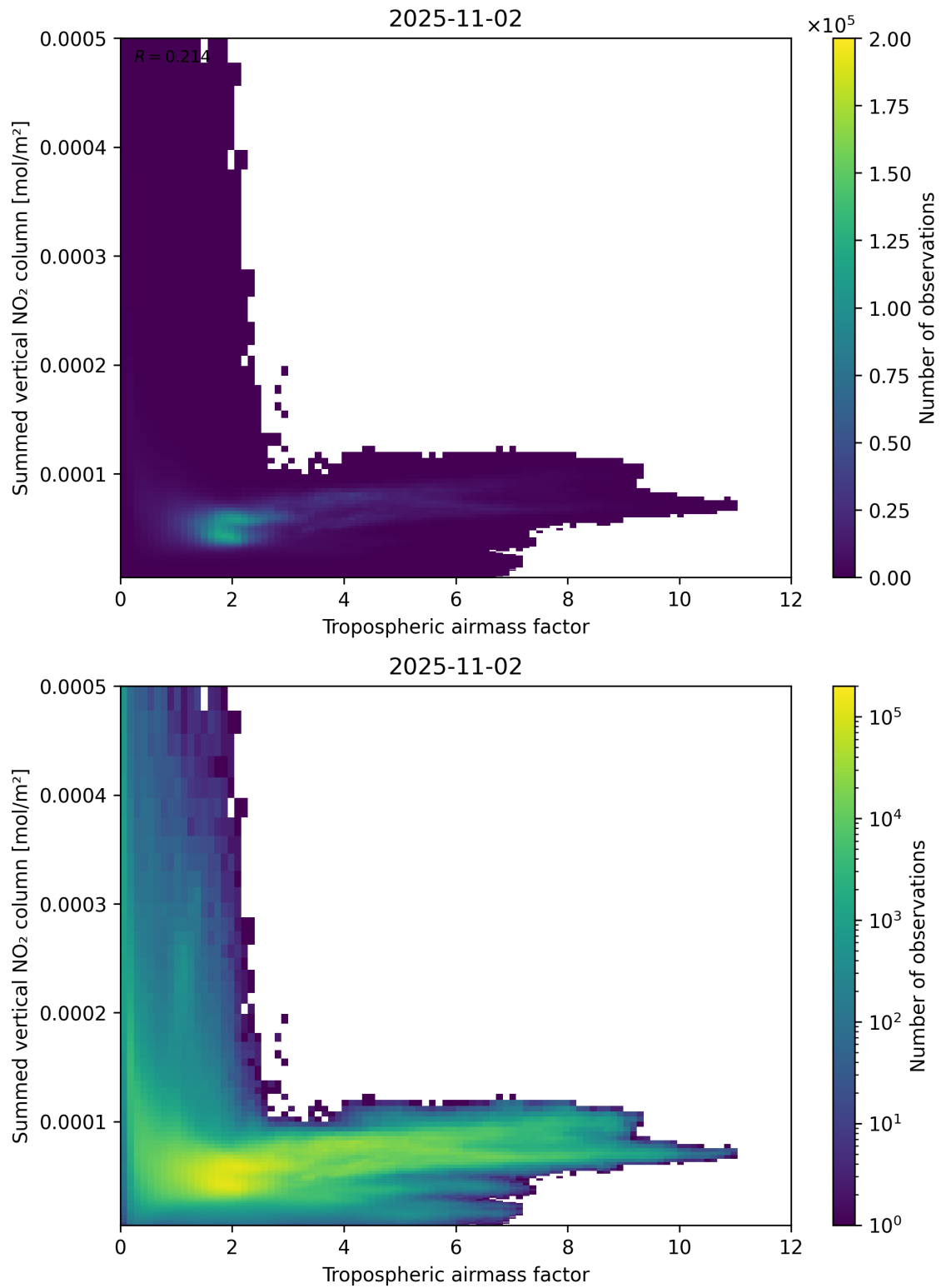
Figure 75: Scatter density plot of “Tropospheric airmass factor” against “Summed vertical NO 2 column” for 2025-11-02 to 2025-11-03.
