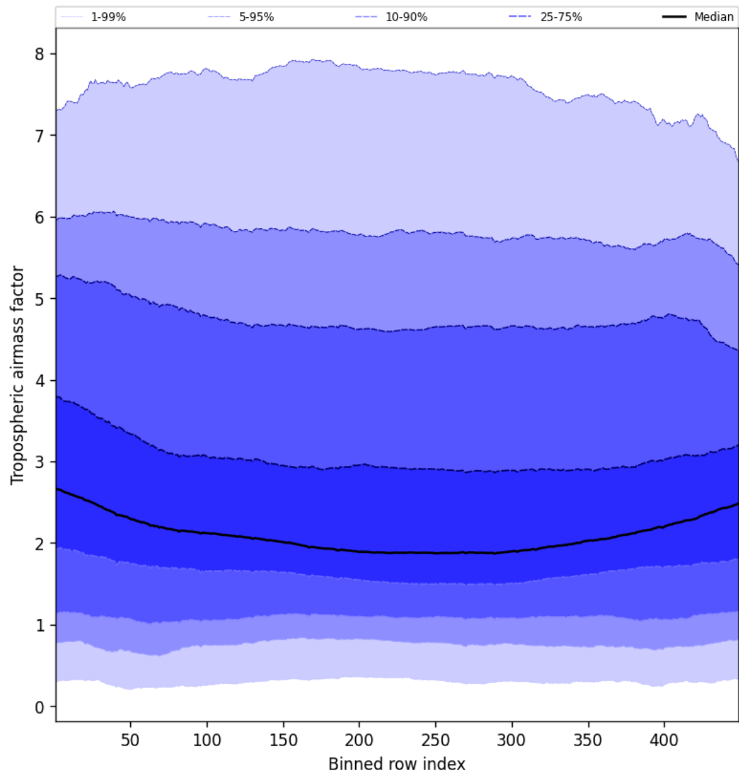
Figure 48: Along track statistics of “Tropospheric airmass factor” for 2025-11-02 to 2025-11-03
