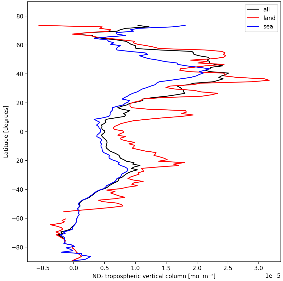
Figure 12: Zonal average of “NO 2 tropospheric vertical column” for 2025-11-02 to 2025-11-03.
