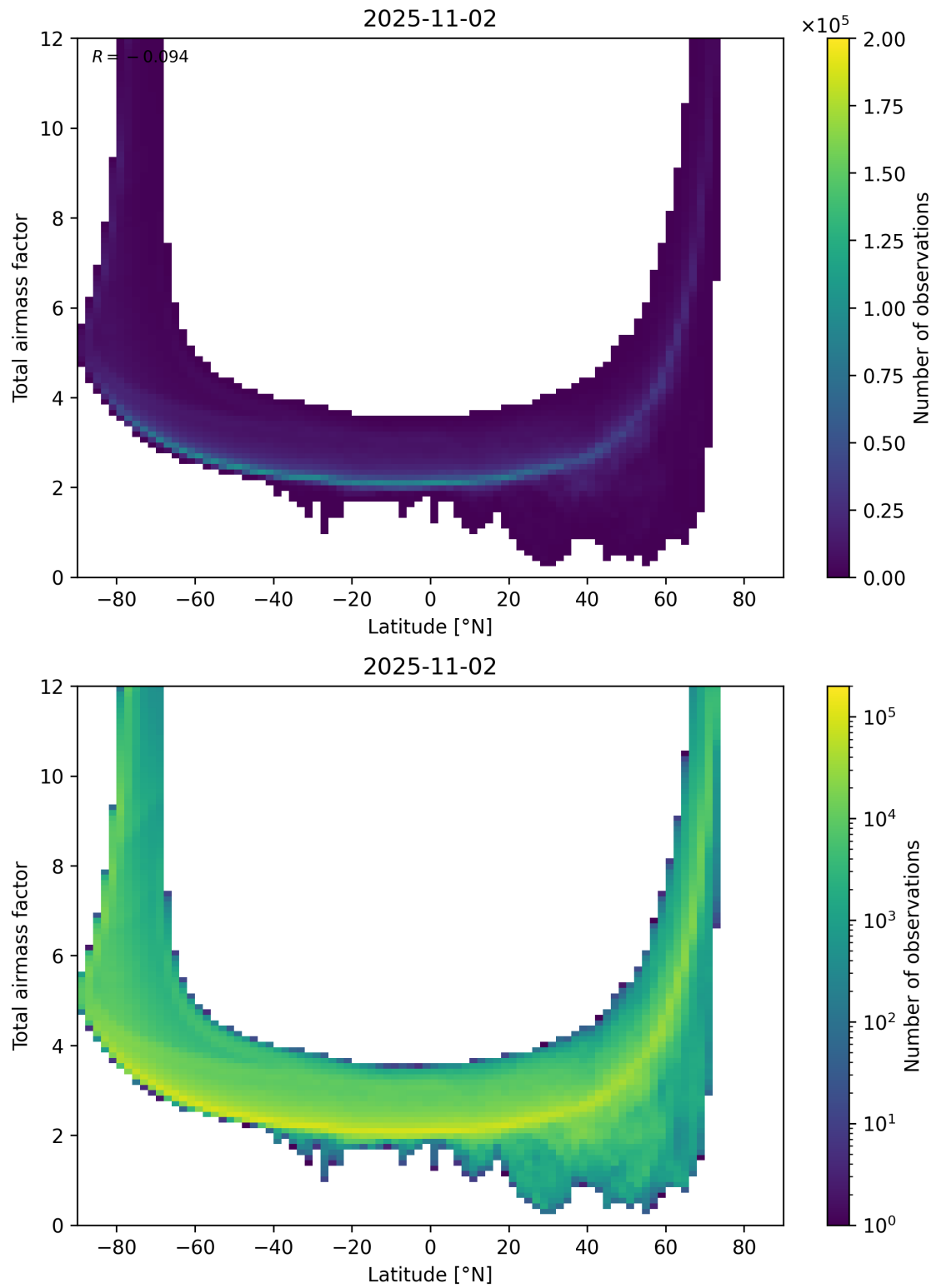
Figure 84: Scatter density plot of “Latitude” against “Total airmass factor” for 2025-11-02 to 2025-11-03.
