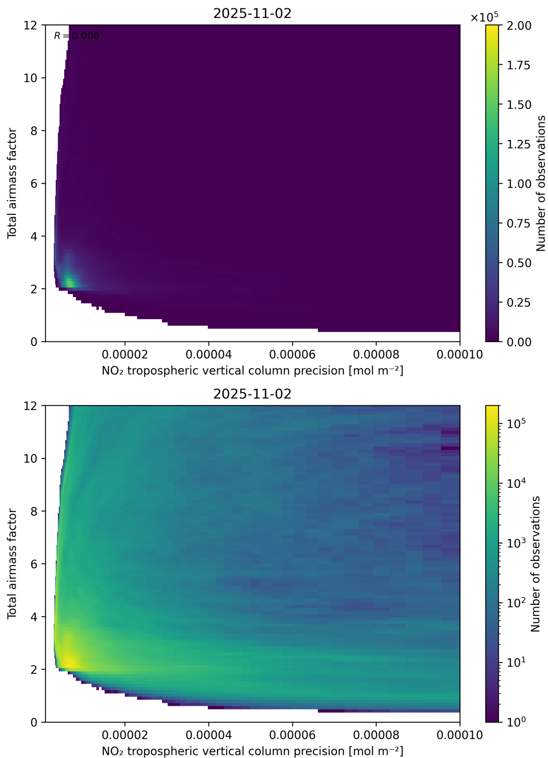
Figure 132: Scatter density plot of “NO 2 tropospheric vertical column precision” against “Total air mass factor” for 2025-11-02 to 2025-11-03.
