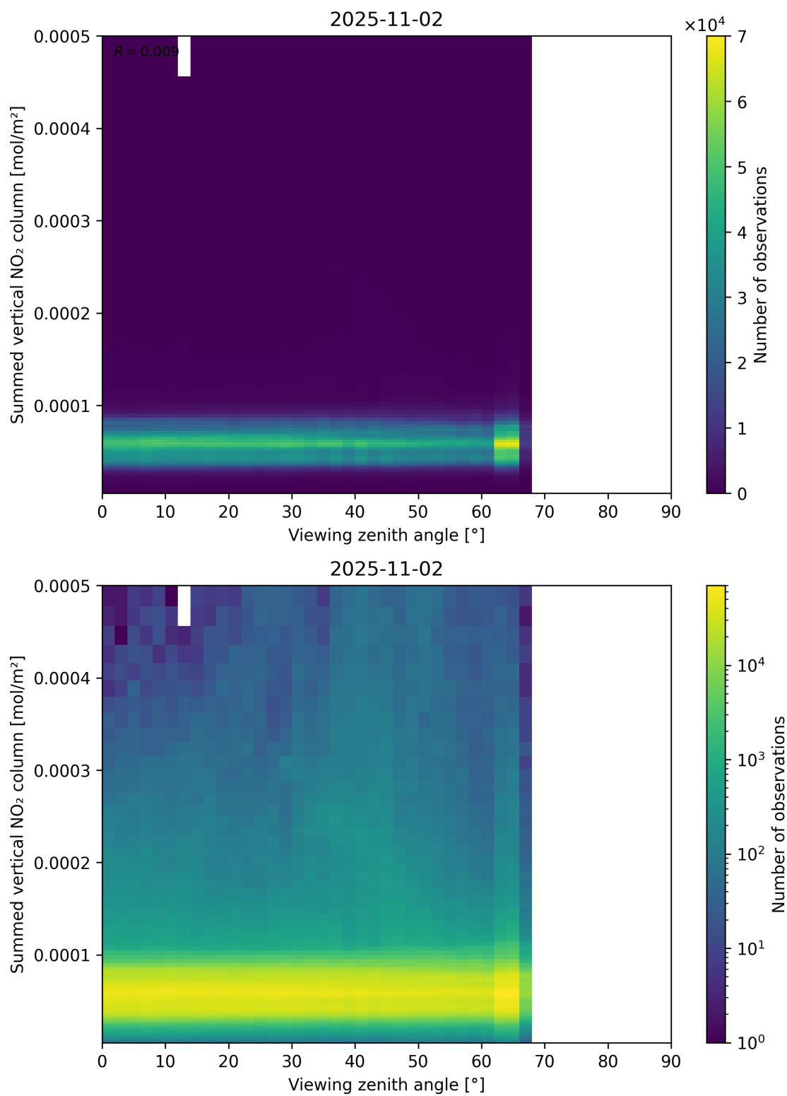
Figure 165: Scatter density plot of “Viewing zenith angle” against “Summed vertical NO 2 column” for 2025-11-02 to 2025-11-03.
