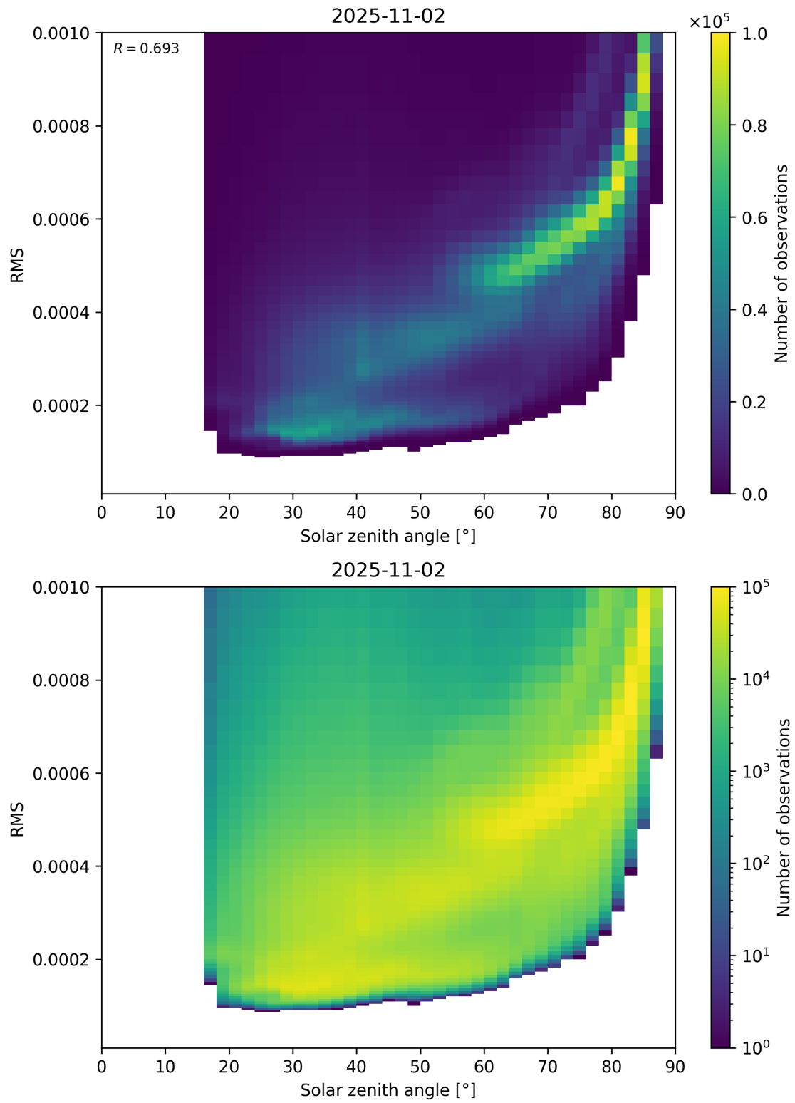
Figure 157: Scatter density plot of “Solar zenith angle” against “RMS” for 2025-11-02 to 2025-11-03.
