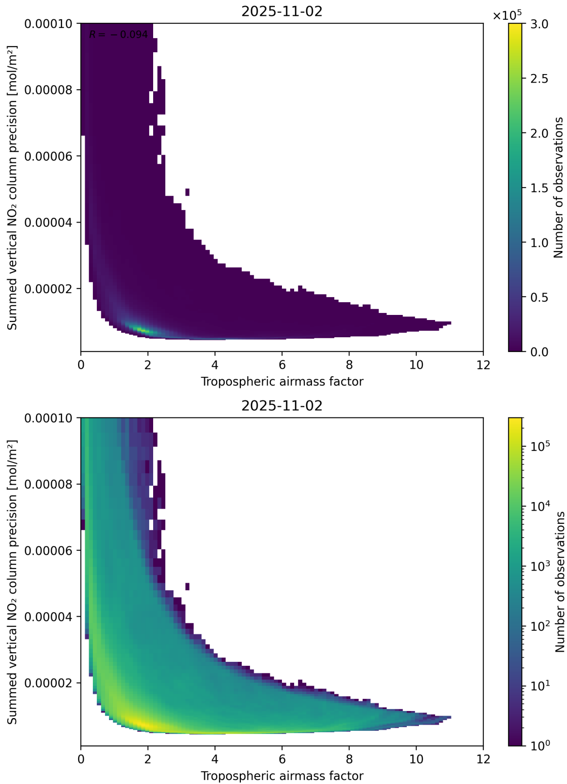
Figure 76: Scatter density plot of “Tropospheric air mass factor” against “Summed vertical NO 2 column precision” for 2025-11-02 to 2025-11-03.
