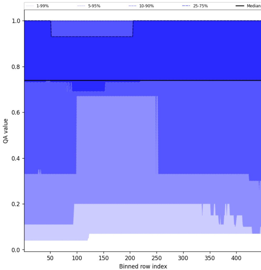
Figure 45: Along track statistics of “QA value” for 2025-11-02 to 2025-11-03
