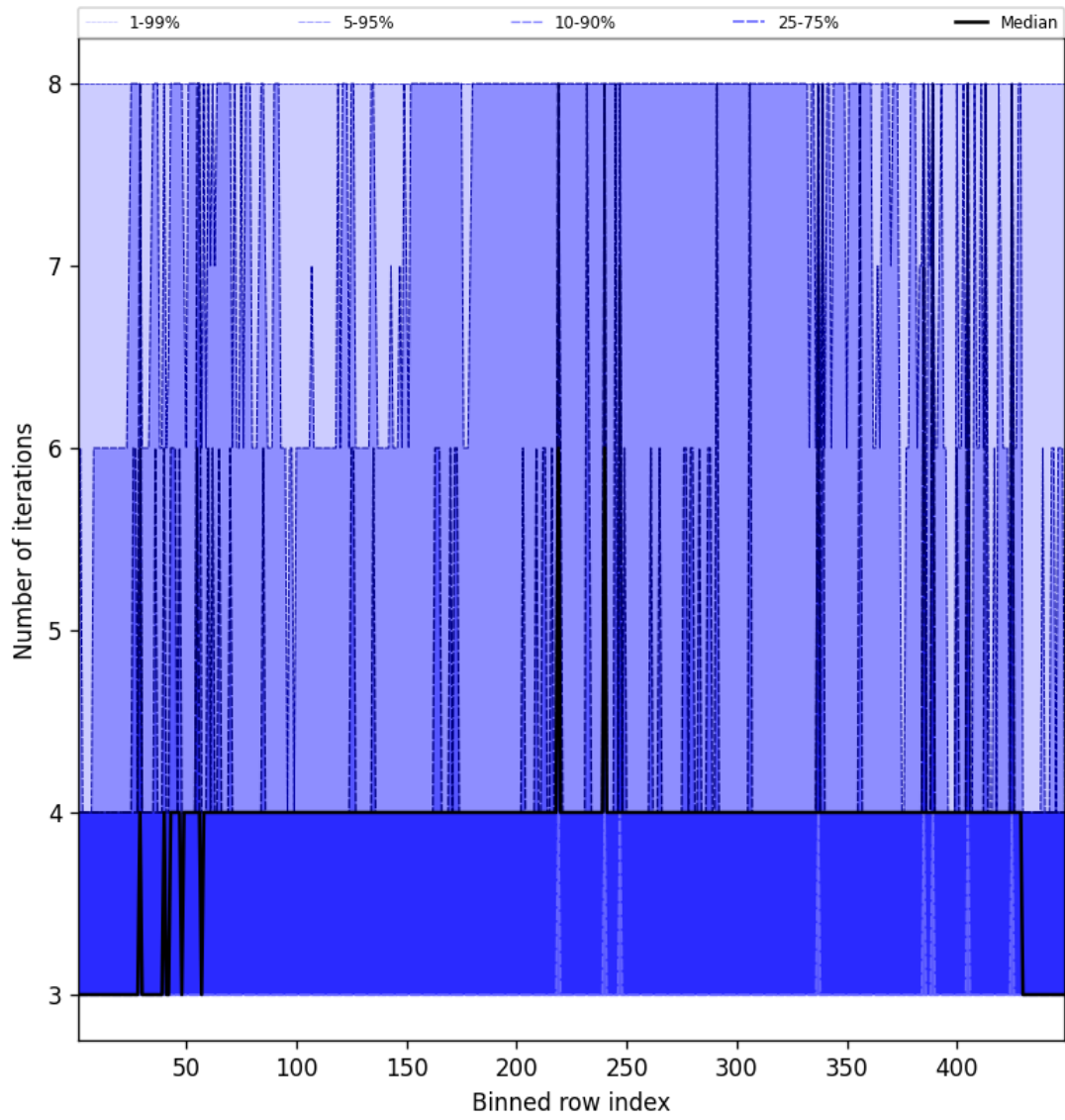
Figure 51: Along track statistics of “Number of iterations” for 2025-11-02 to 2025-11-03
