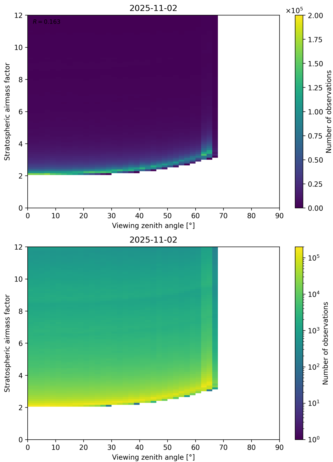
Figure 159: Scatter density plot of “Viewing zenith angle” against “Stratospheric airmass factor” for 2025-11-02 to 2025-11-03.
