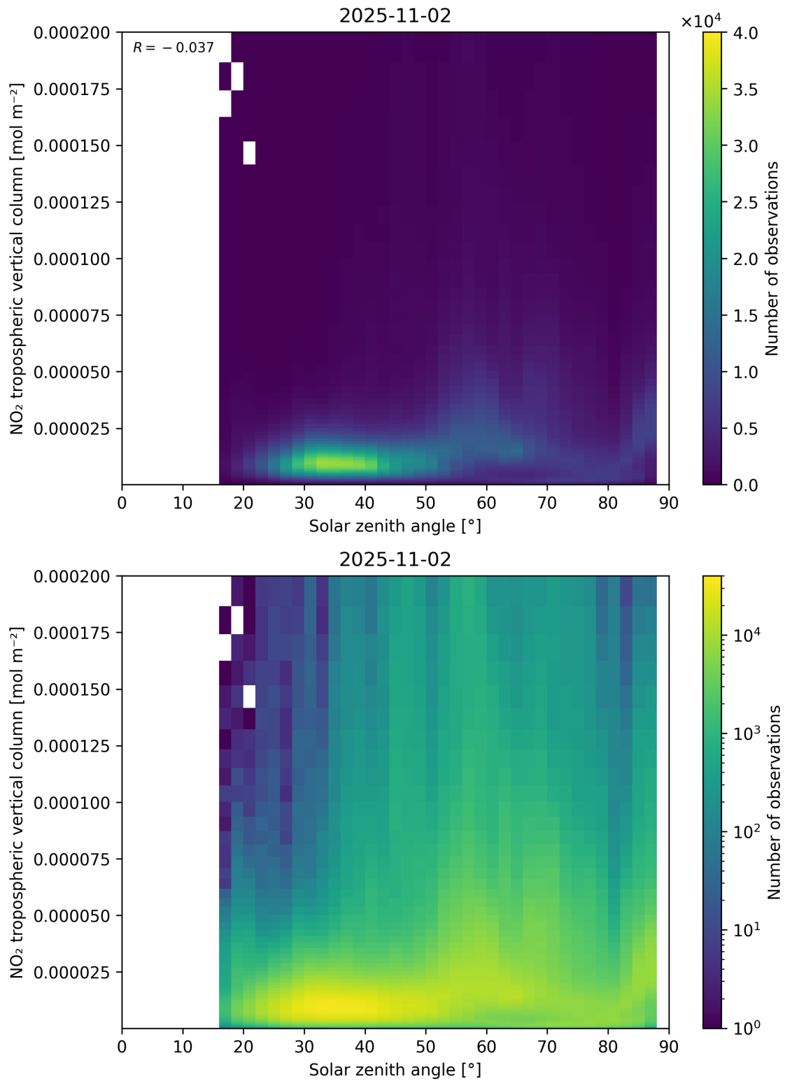
Figure 155: Scatter density plot of “Solar zenith angle” against “NO 2 tropospheric vertical column” for 2025-11-02 to 2025-11-03.
