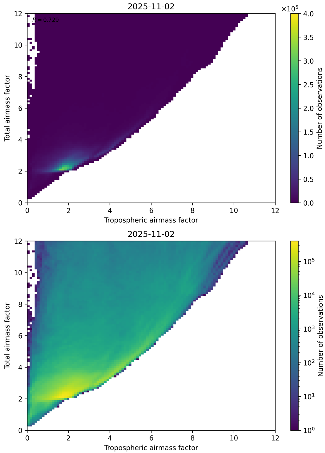
Figure 72: Scatter density plot of “Tropospheric airmass factor” against “Total airmass factor” for 2025-11-02 to 2025-11-03.
