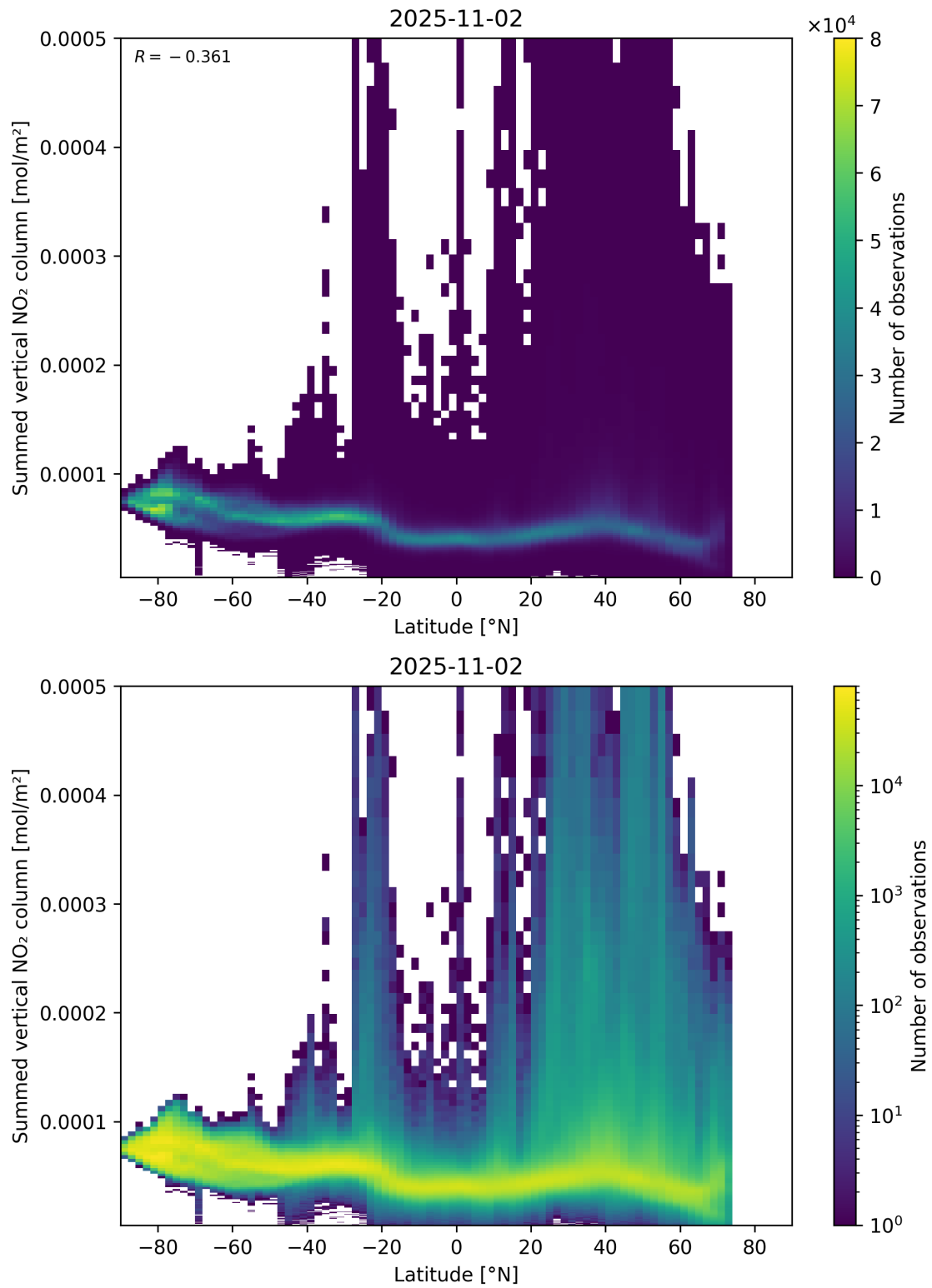
Figure 88: Scatter density plot of “Latitude” against “Summed vertical NO 2 column” for 2025-11-02 to 2025-11-03.
