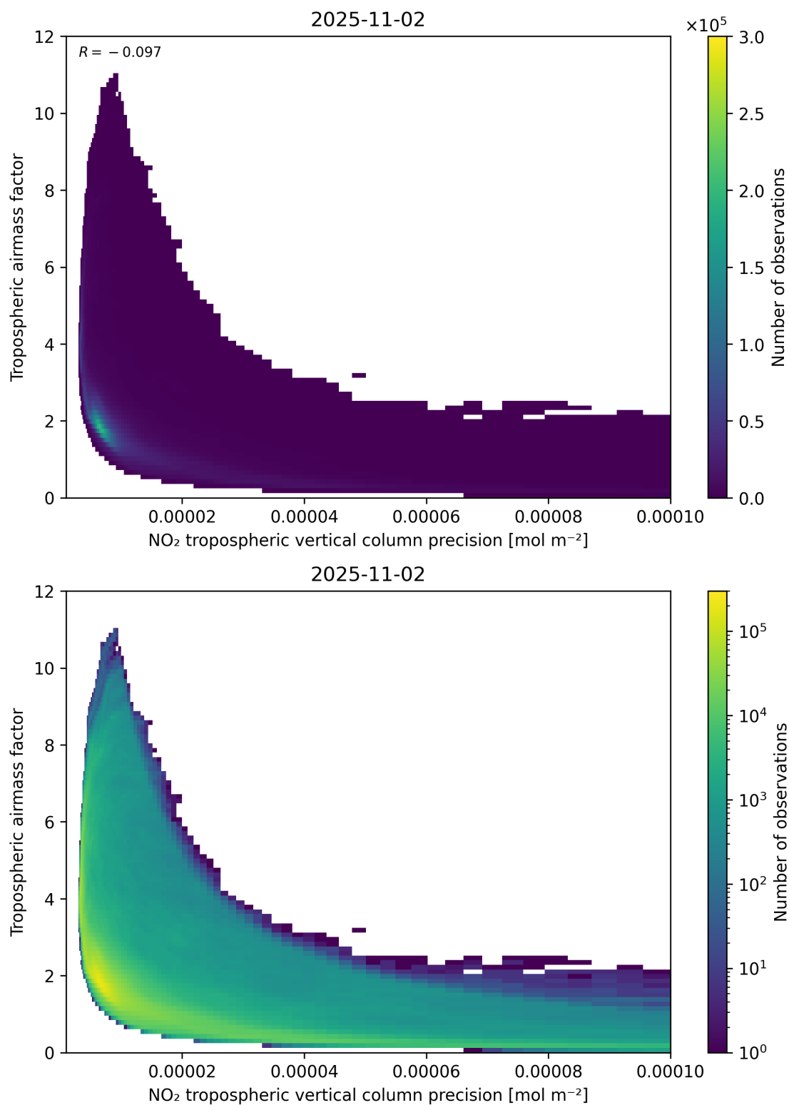
Figure 133: Scatter density plot of “NO 2 tropospheric vertical column precision” against “Tropospheric airmass factor” for 2025-11-02 to 2025-11-03.
