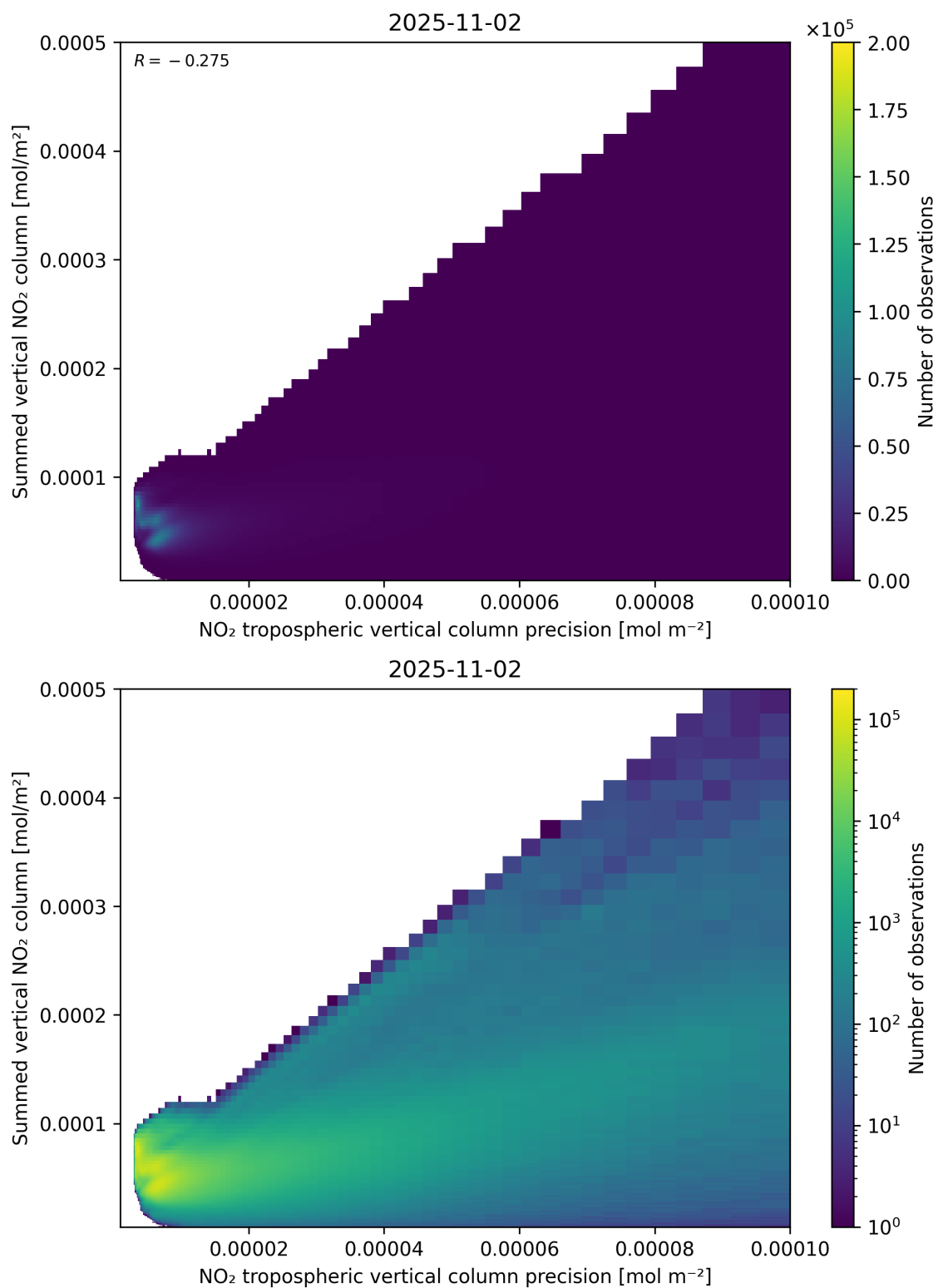
Figure 136: Scatter density plot of “NO 2 tropospheric vertical column precision” against “Summed vertical NO 2 column” for 2025-11-02 to 2025-11-03.
