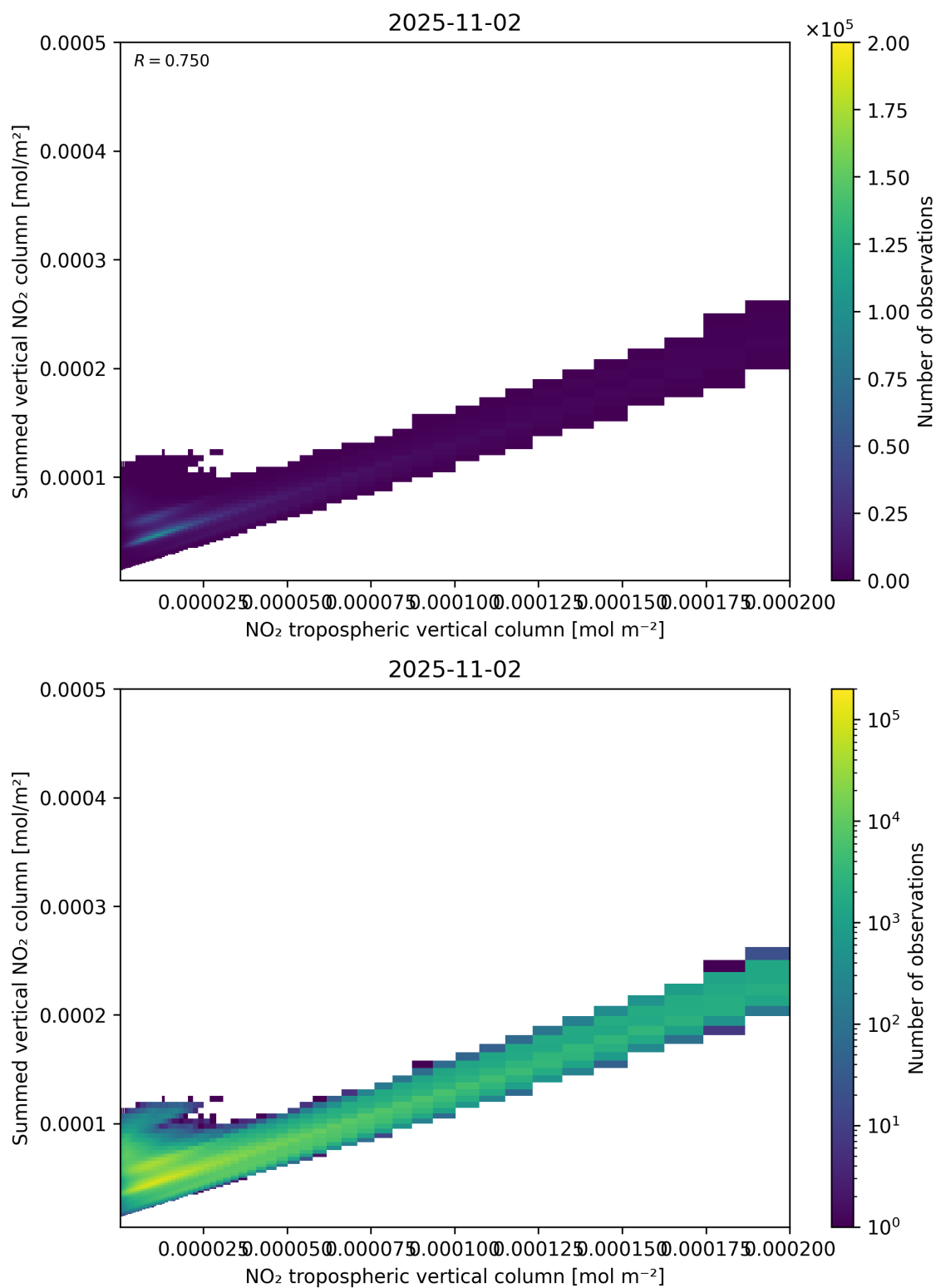
Figure 126: Scatter density plot of “NO 2 tropospheric vertical column” against “Summed vertical NO 2 column” for 2025-11-02 to 2025-11-03.
