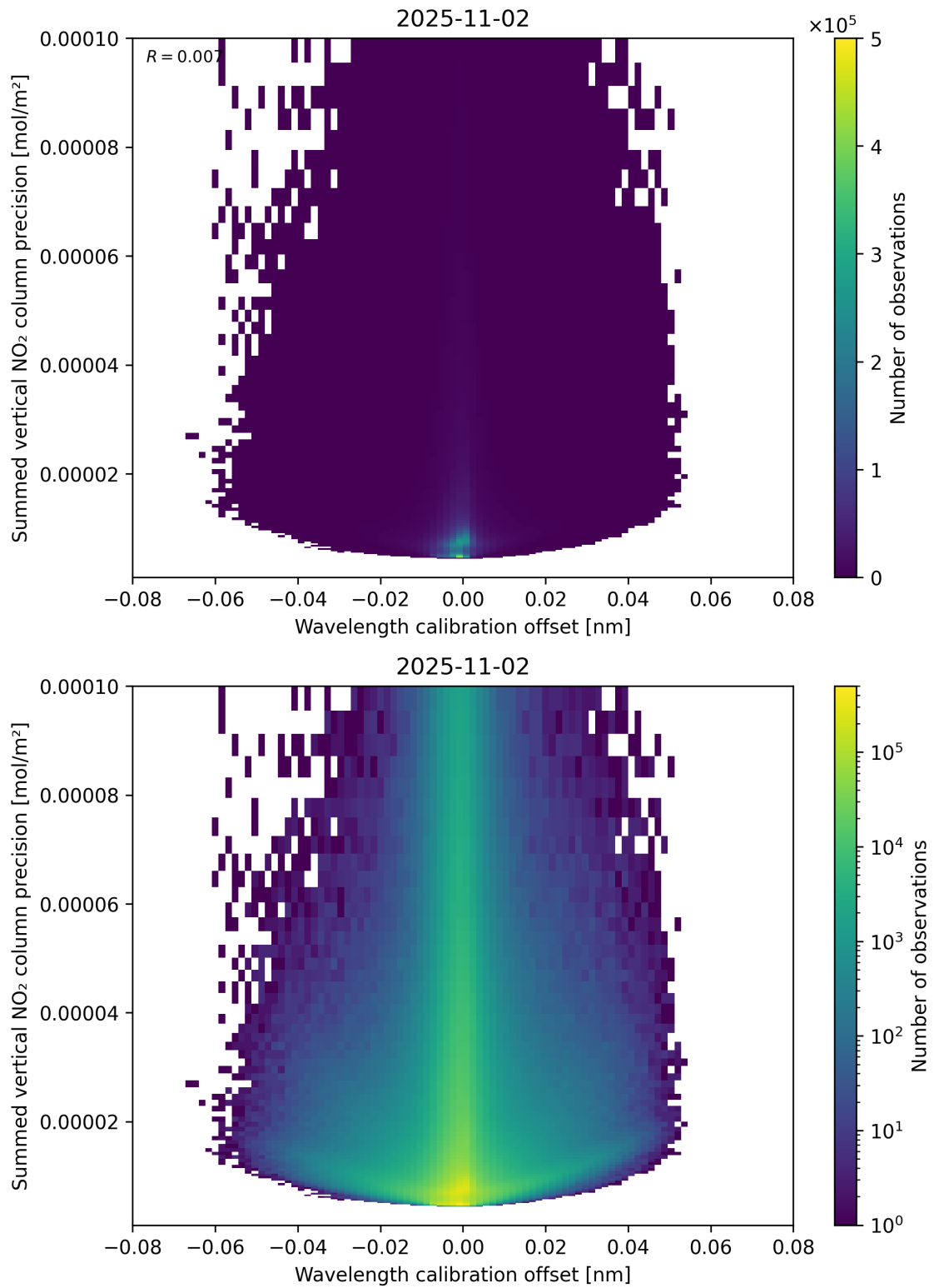
Figure 178: Scatter density plot of “Wavelength calibration offset” against “Summed vertical NO 2 column precision” for 2025-11-02 to 2025-11-03.
