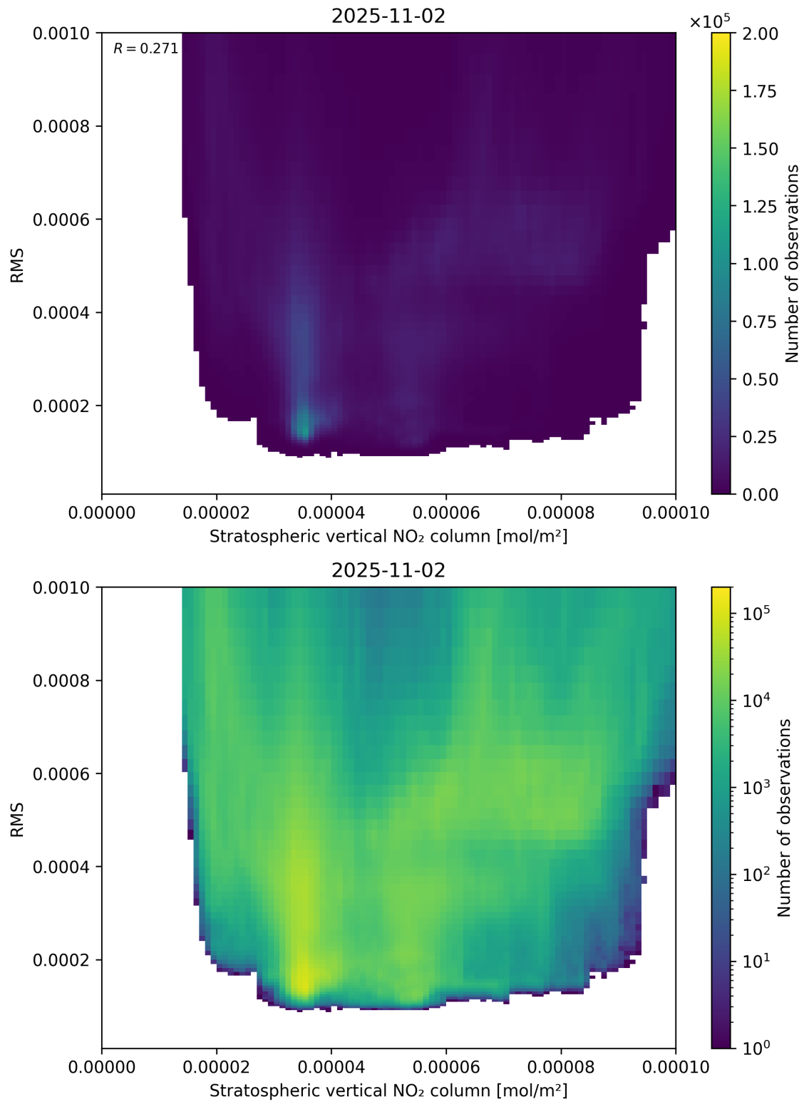
Figure 102: Scatter density plot of “Stratospheric vertical NO 2 column” against “RMS” for 2025-11-02 to 2025-11-03.
