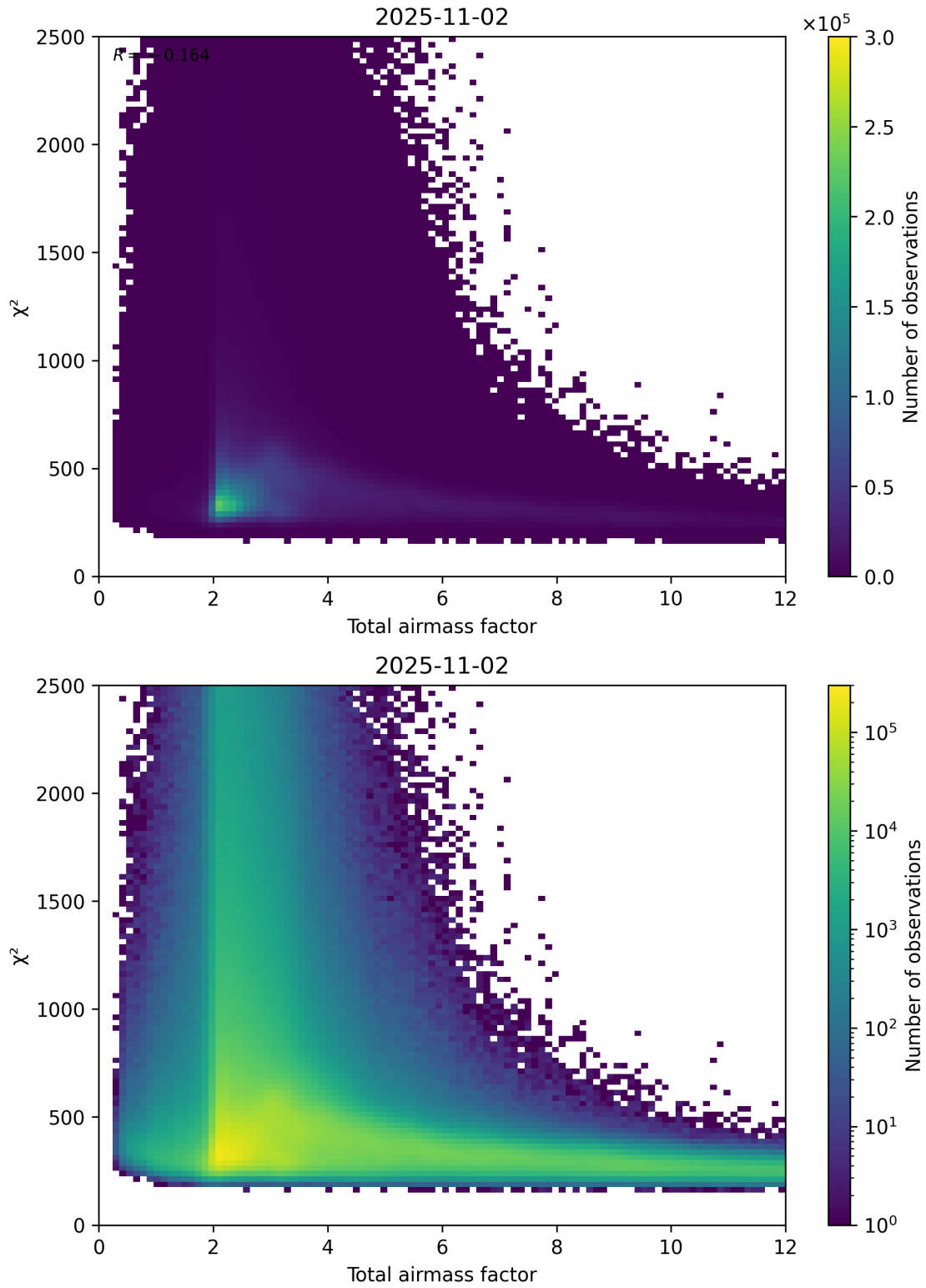
Figure 63: Scatter density plot of “Total airmass factor” against “ \chi^2 ” for 2025-11-02 to 2025-11-03.
