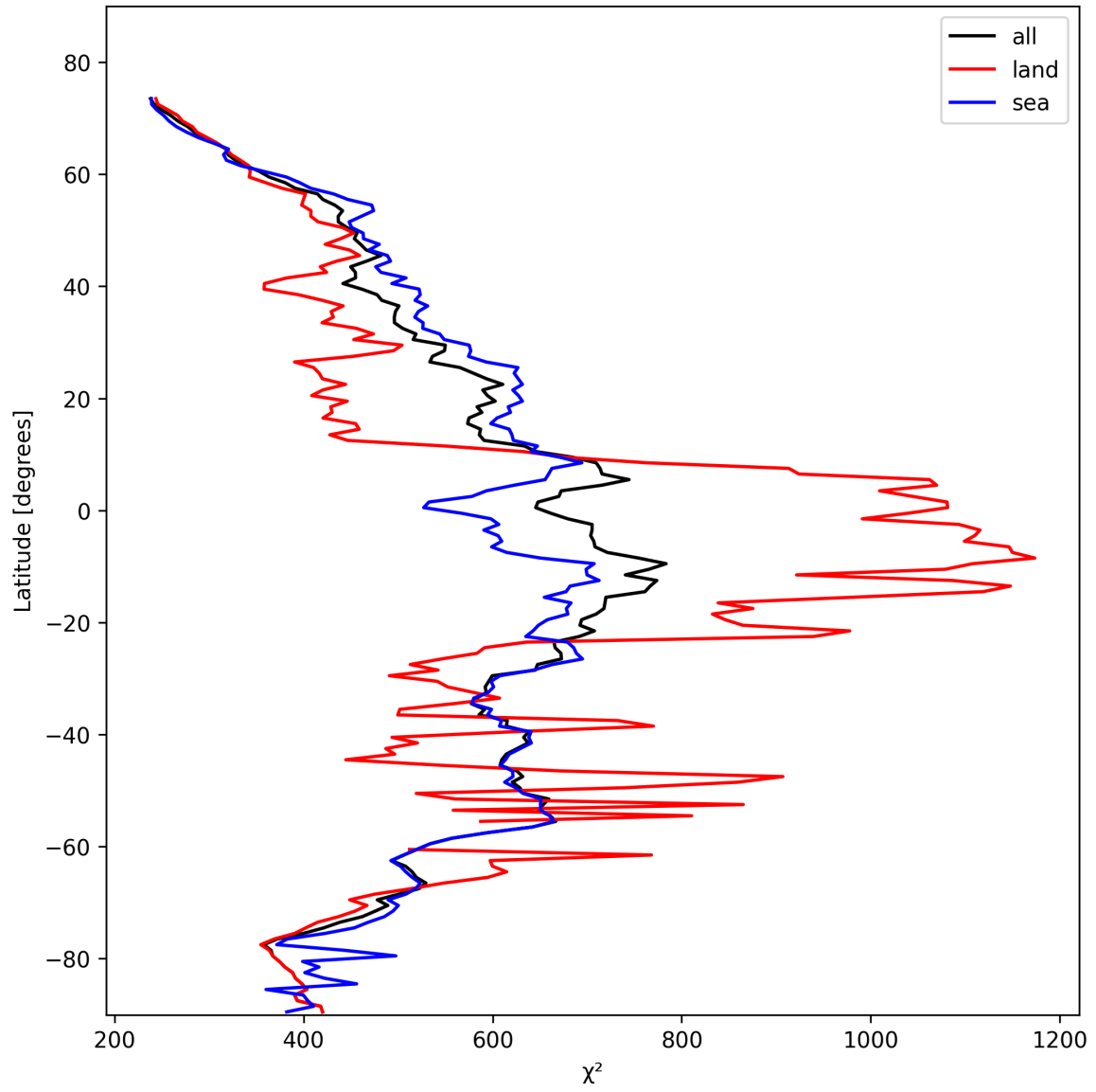
Figure 25: Zonal average of “ \chi^2 ” for 2025-11-02 to 2025-11-03.
