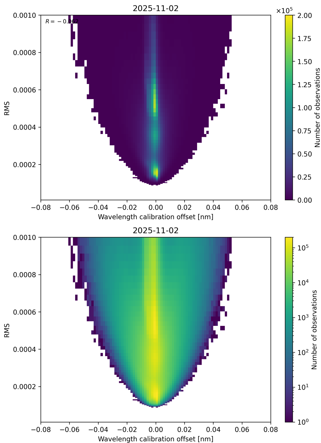
Figure 181: Scatter density plot of “Wavelength calibration offset” against “RMS” for 2025-11-02 to 2025-11-03.
