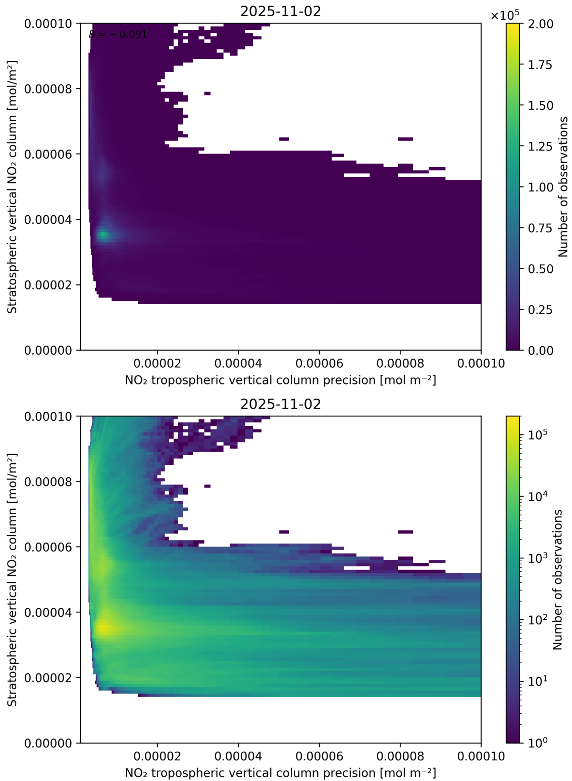
Figure 135: Scatter density plot of “NO 2 tropospheric vertical column precision” against “Stratospheric vertical NO 2 column” for 2025-11-02 to 2025-11-03.
