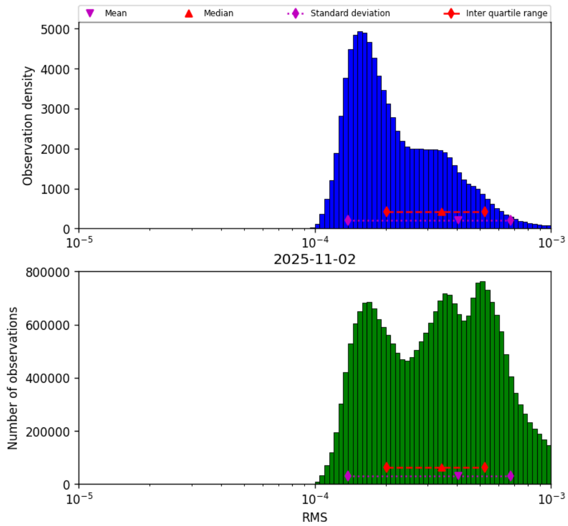
Figure 43: Histogram of “RMS” for 2025-11-02 to 2025-11-03
