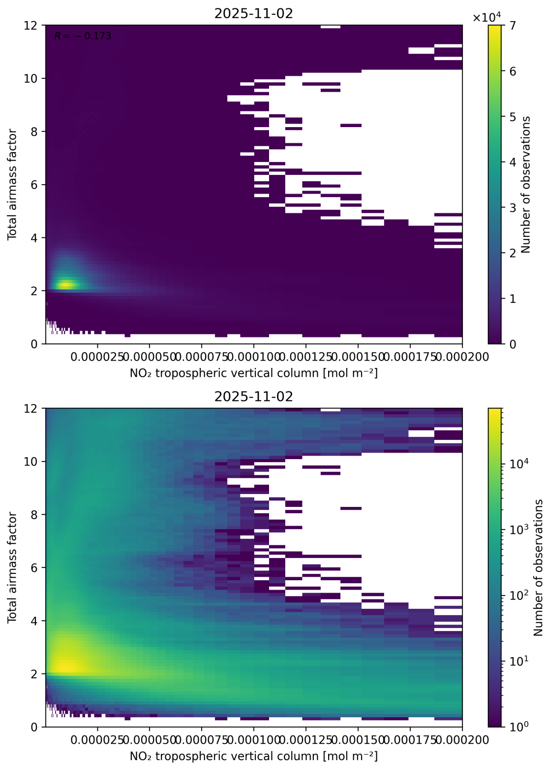
Figure 122: Scatter density plot of “NO 2 tropospheric vertical column” against “Total air mass factor” for 2025-11-02 to 2025-11-03.
