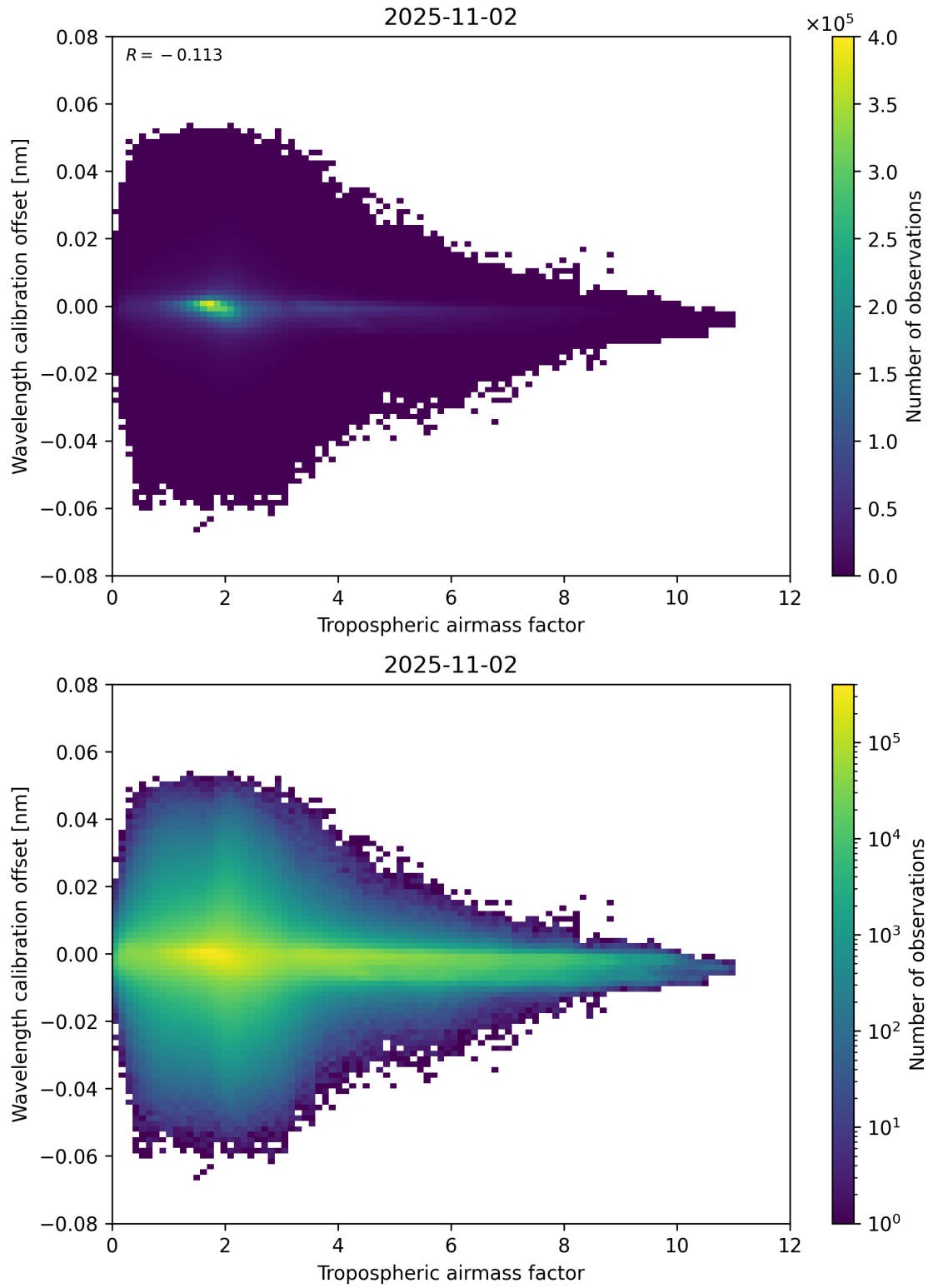
Figure 80: Scatter density plot of “Tropospheric airmass factor” against “Wavelength calibration offset” for 2025-11-02 to 2025-11-03.
