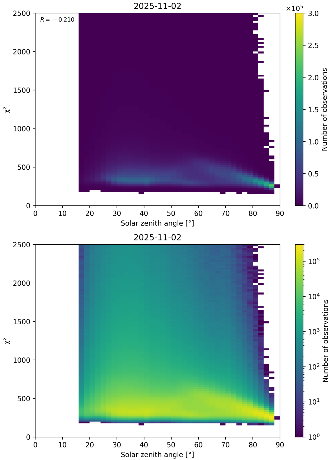
Figure 148: Scatter density plot of “Solar zenith angle” against “ \chi^2 ” for 2025-11-02 to 2025-11-03.
