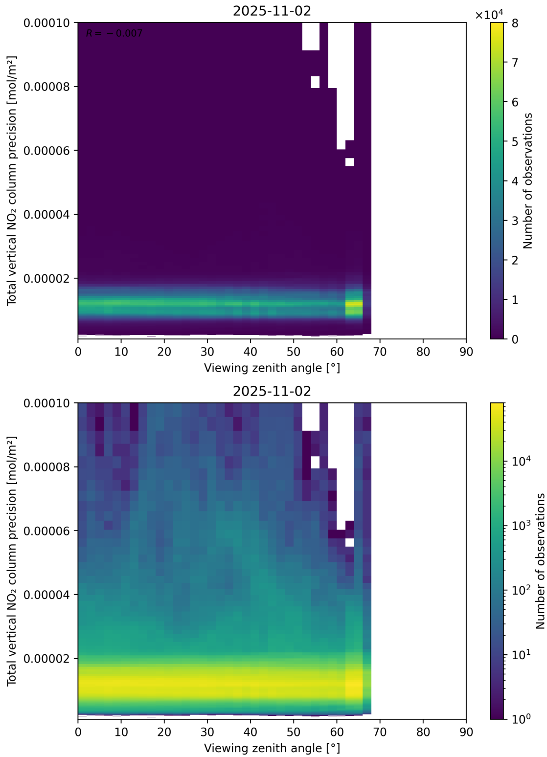
Figure 168: Scatter density plot of “Viewing zenith angle” against “Total vertical NO 2 column precision” for 2025-11-02 to 2025-11-03.
