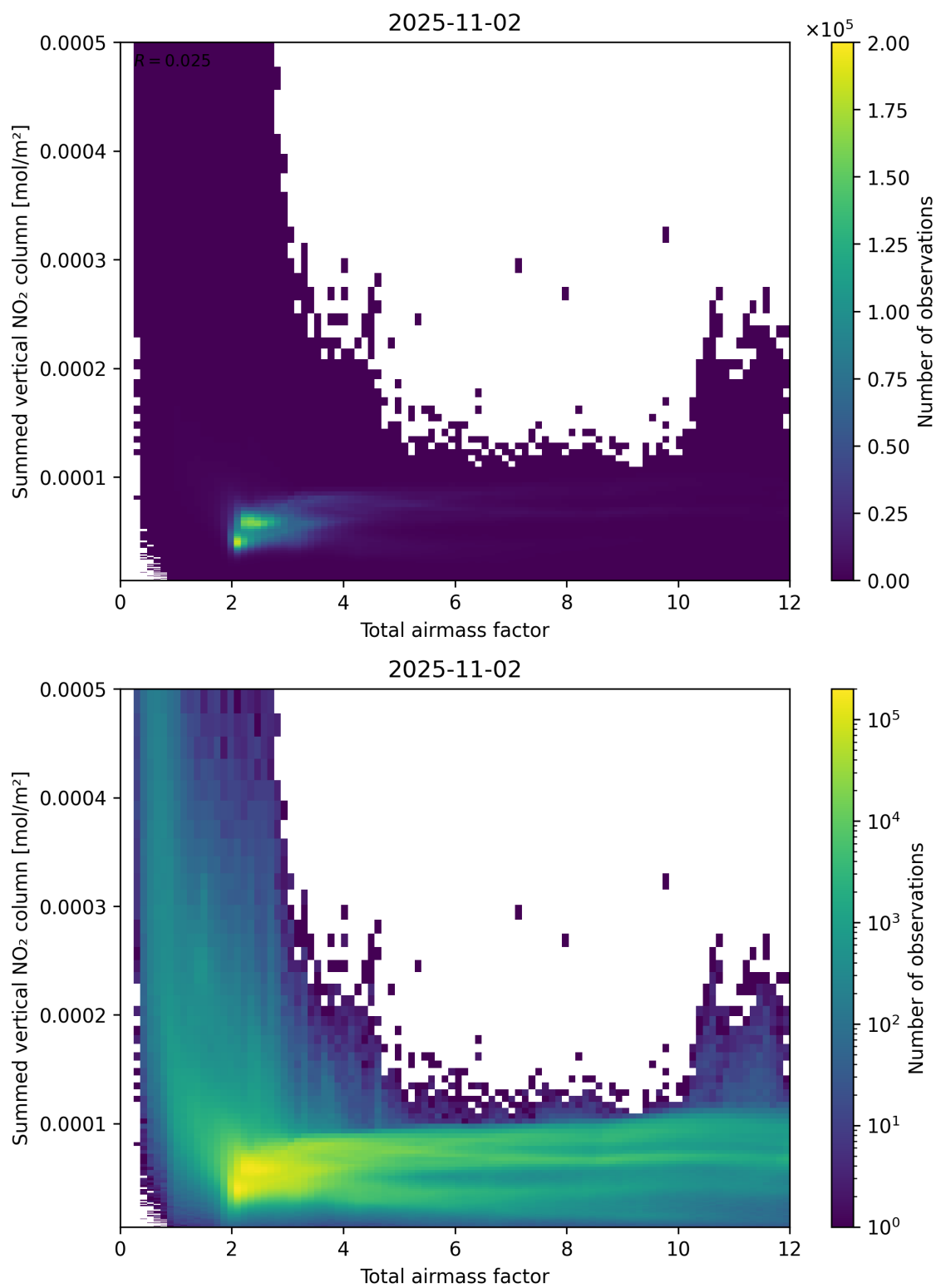
Figure 65: Scatter density plot of “Total airmass factor” against “Summed vertical NO 2 column” for 2025-11-02 to 2025-11-03.
