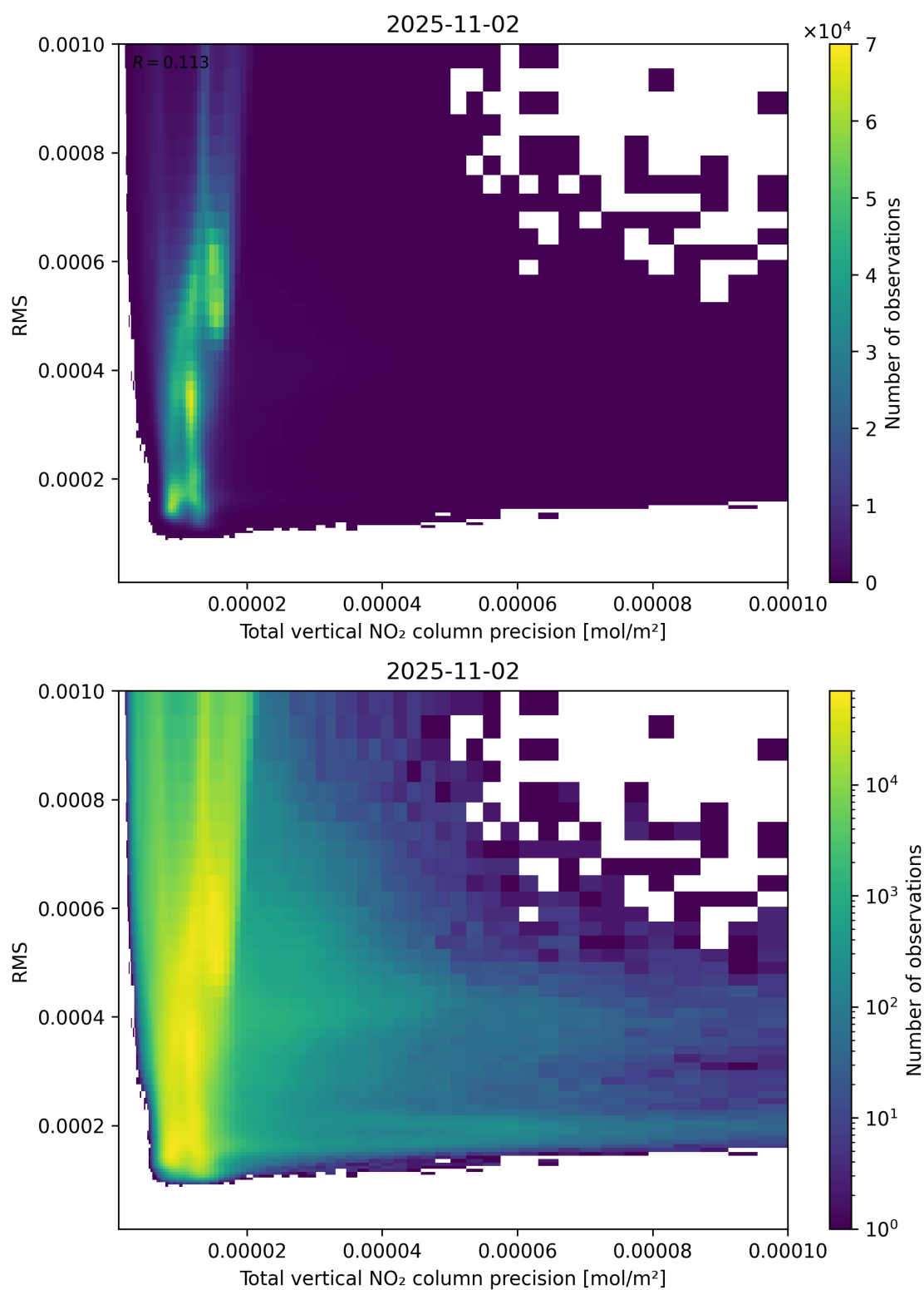
Figure 119: Scatter density plot of “Total vertical NO 2 column precision” against “RMS” for 2025-11-02 to 2025-11-03.
