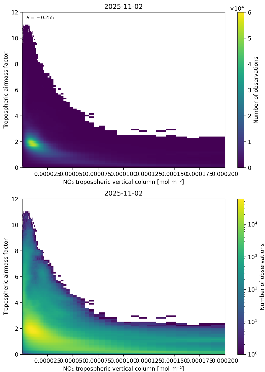
Figure 123: Scatter density plot of “NO 2 tropospheric vertical column” against “Tropospheric air mass factor” for 2025-11-02 to 2025-11-03.
