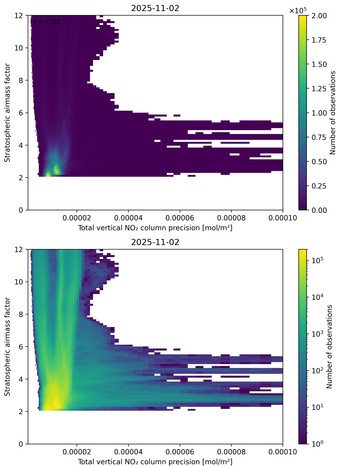
Figure 115: Scatter density plot of “Total vertical NO 2 column precision” against “Stratospheric air mass factor” for 2025-11-02 to 2025-11-03.
