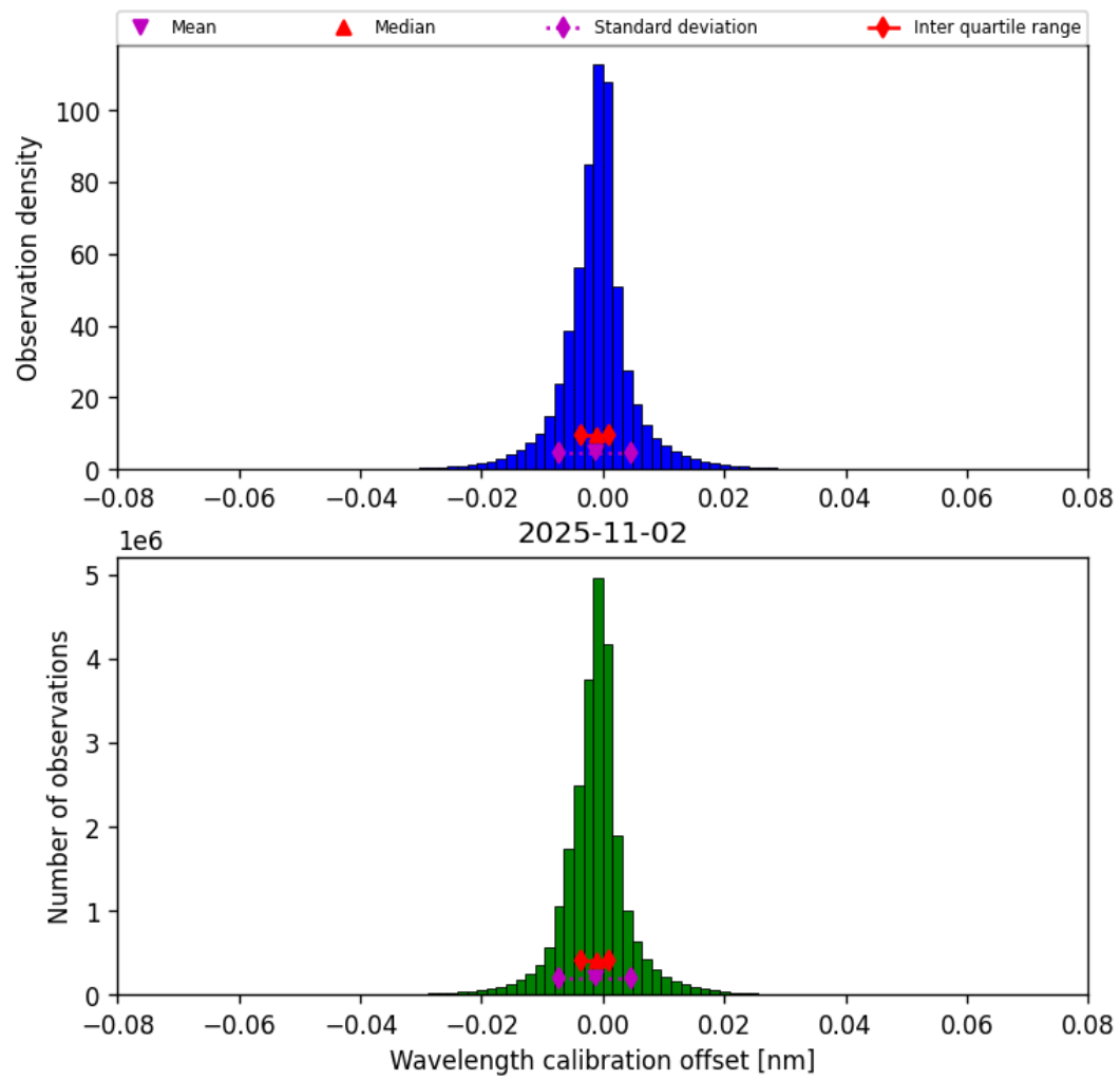
Figure 35: Histogram of “Wavelength calibration offset” for 2025-11-02 to 2025-11-03
