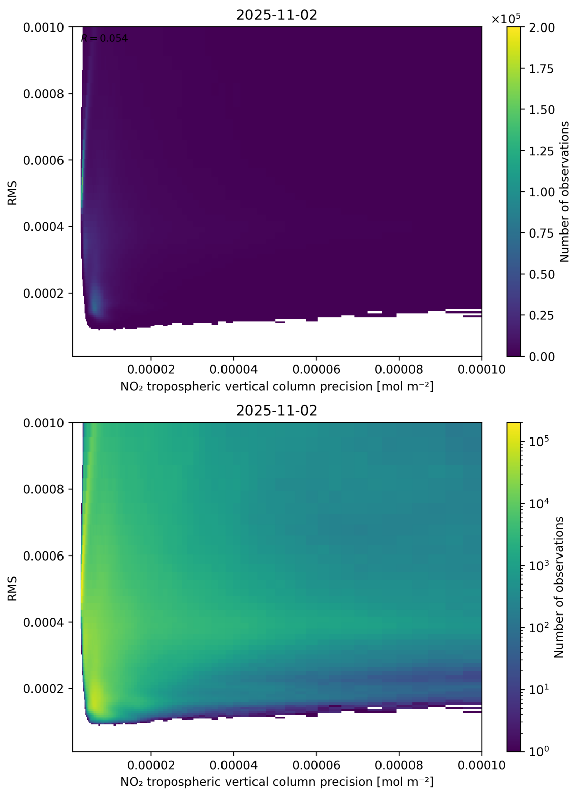
Figure 140: Scatter density plot of “NO 2 tropospheric vertical column precision” against “RMS” for 2025-11-02 to 2025-11-03.
