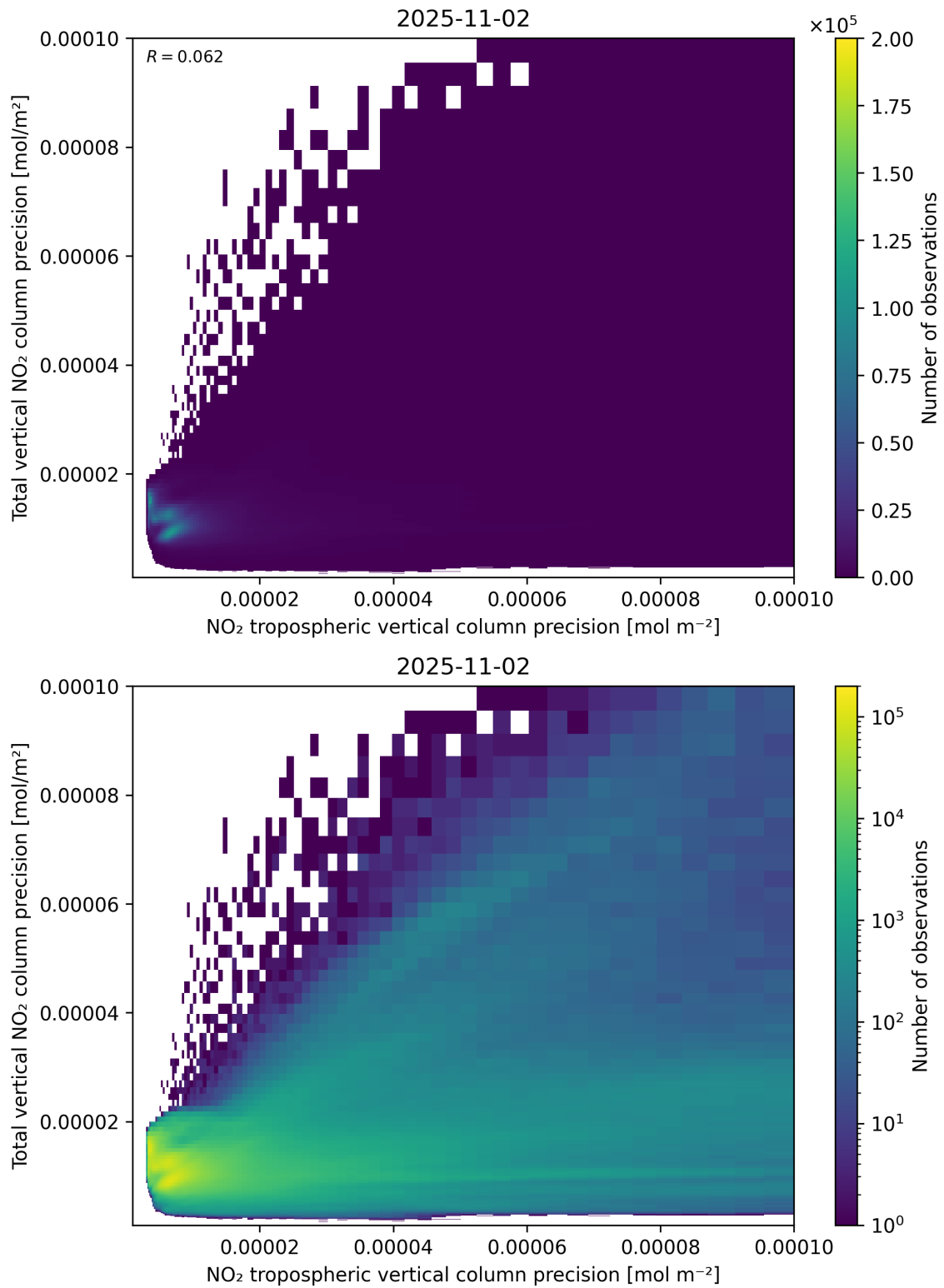
Figure 139: Scatter density plot of “NO 2 tropospheric vertical column precision” against “Total vertical NO 2 column precision” for 2025-11-02 to 2025-11-03.
