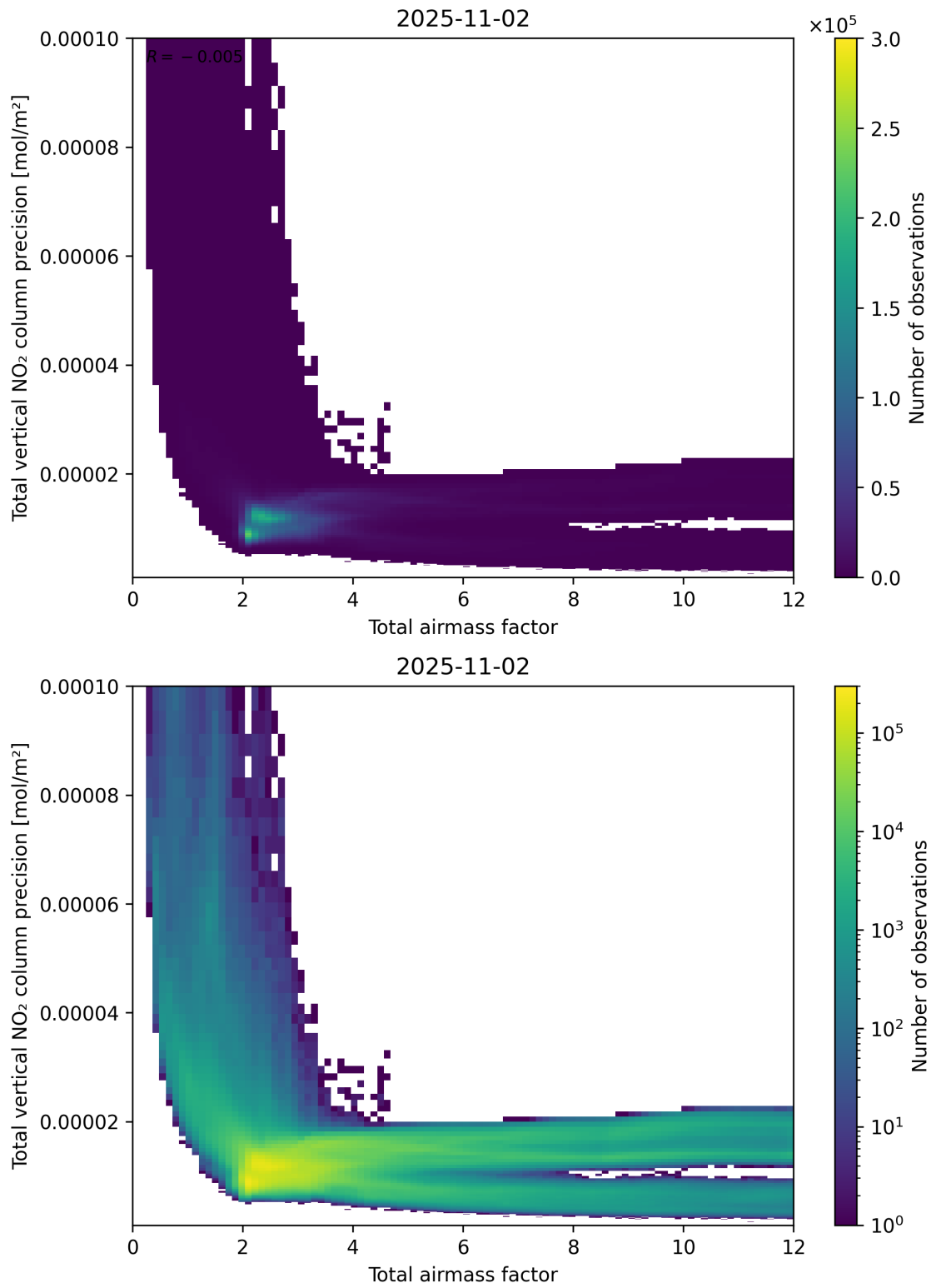
Figure 68: Scatter density plot of “Total airmass factor” against “Total vertical NO 2 column precision” for 2025-11-02 to 2025-11-03.
