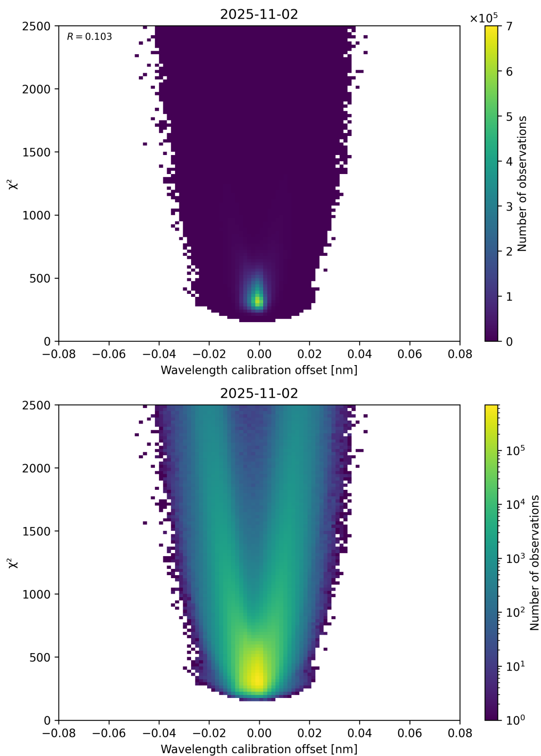
Figure 175: Scatter density plot of “Wavelength calibration offset” against “ \chi^2 ” for 2025-11-02 to 2025-11-03.
