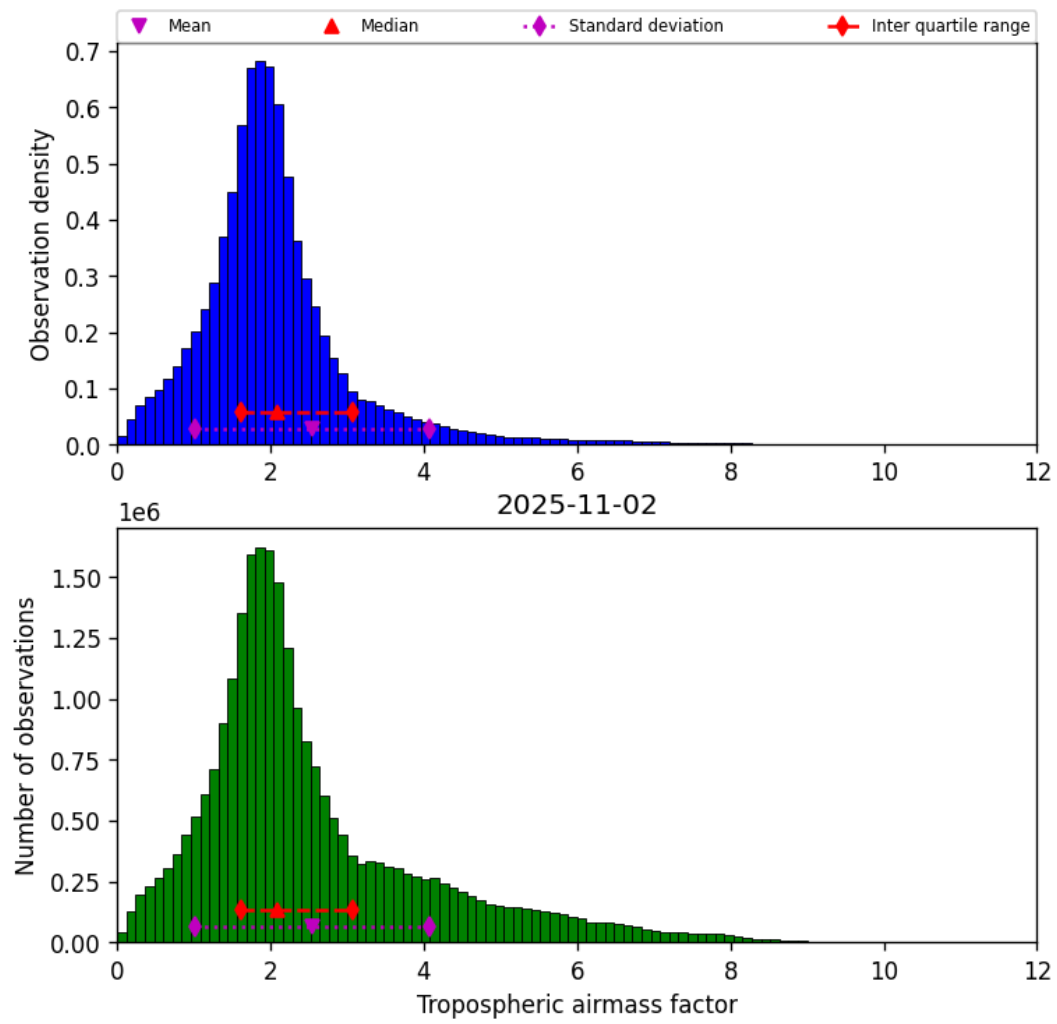
Figure 31: Histogram of “Tropospheric airmass factor” for 2025-11-02 to 2025-11-03
