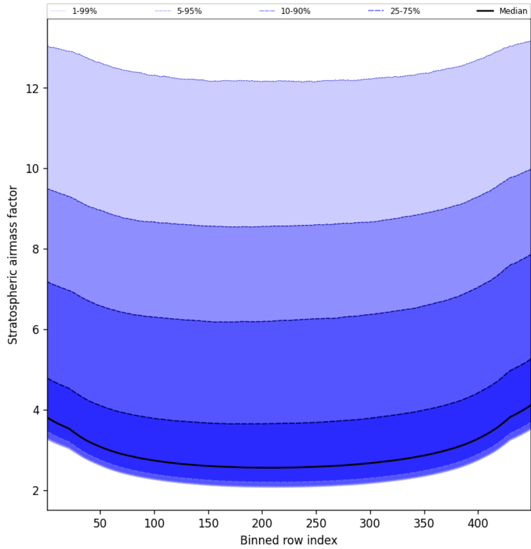
Figure 61: Along track statistics of “Stratospheric air mass factor” for 2025-11-02 to 2025-11-03
