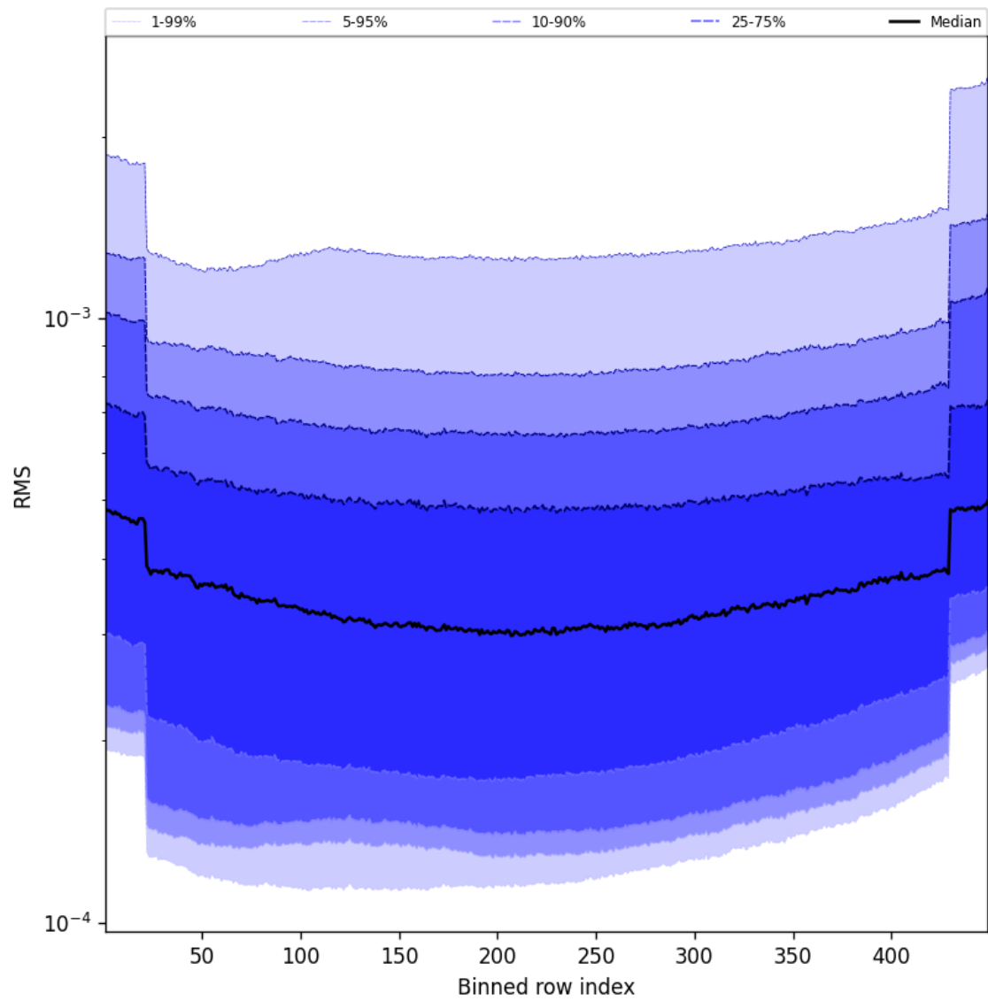
Figure 60: Along track statistics of “RMS” for 2025-11-02 to 2025-11-03
