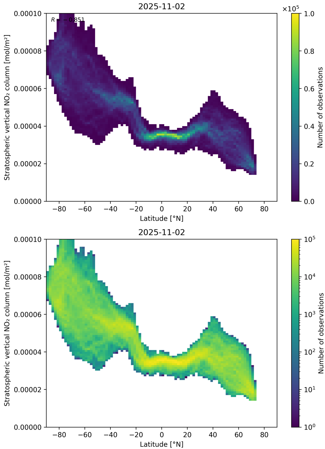
Figure 87: Scatter density plot of “Latitude” against “Stratospheric vertical NO 2 column” for 2025-11-02 to 2025-11-03.
