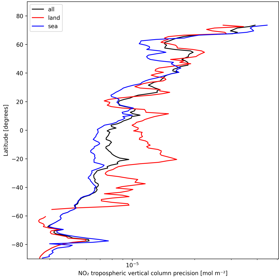
Figure 13: Zonal average of “NO 2 tropospheric vertical column precision” for 2025-11-02 to 2025-11-03.
