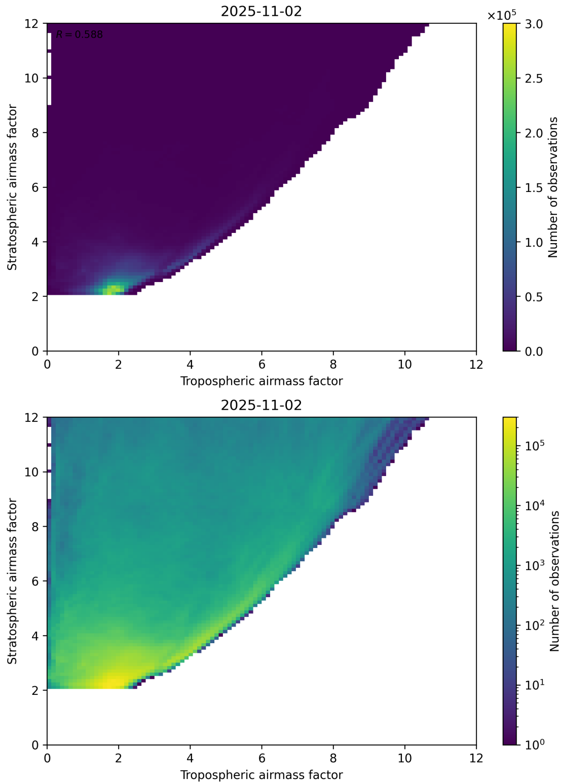
Figure 71: Scatter density plot of “Tropospheric airmass factor” against “Stratospheric airmass factor” for 2025-11-02 to 2025-11-03.
