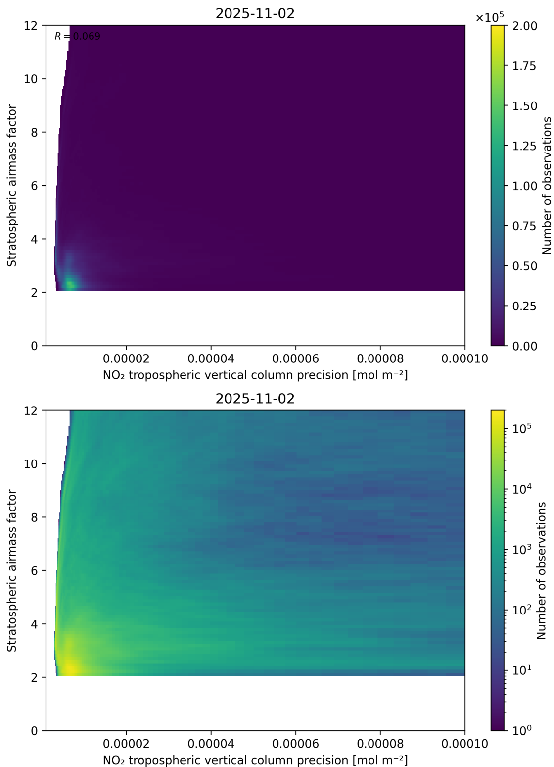
Figure 131: Scatter density plot of “NO 2 tropospheric vertical column precision” against “Stratospheric airmass factor” for 2025-11-02 to 2025-11-03.
