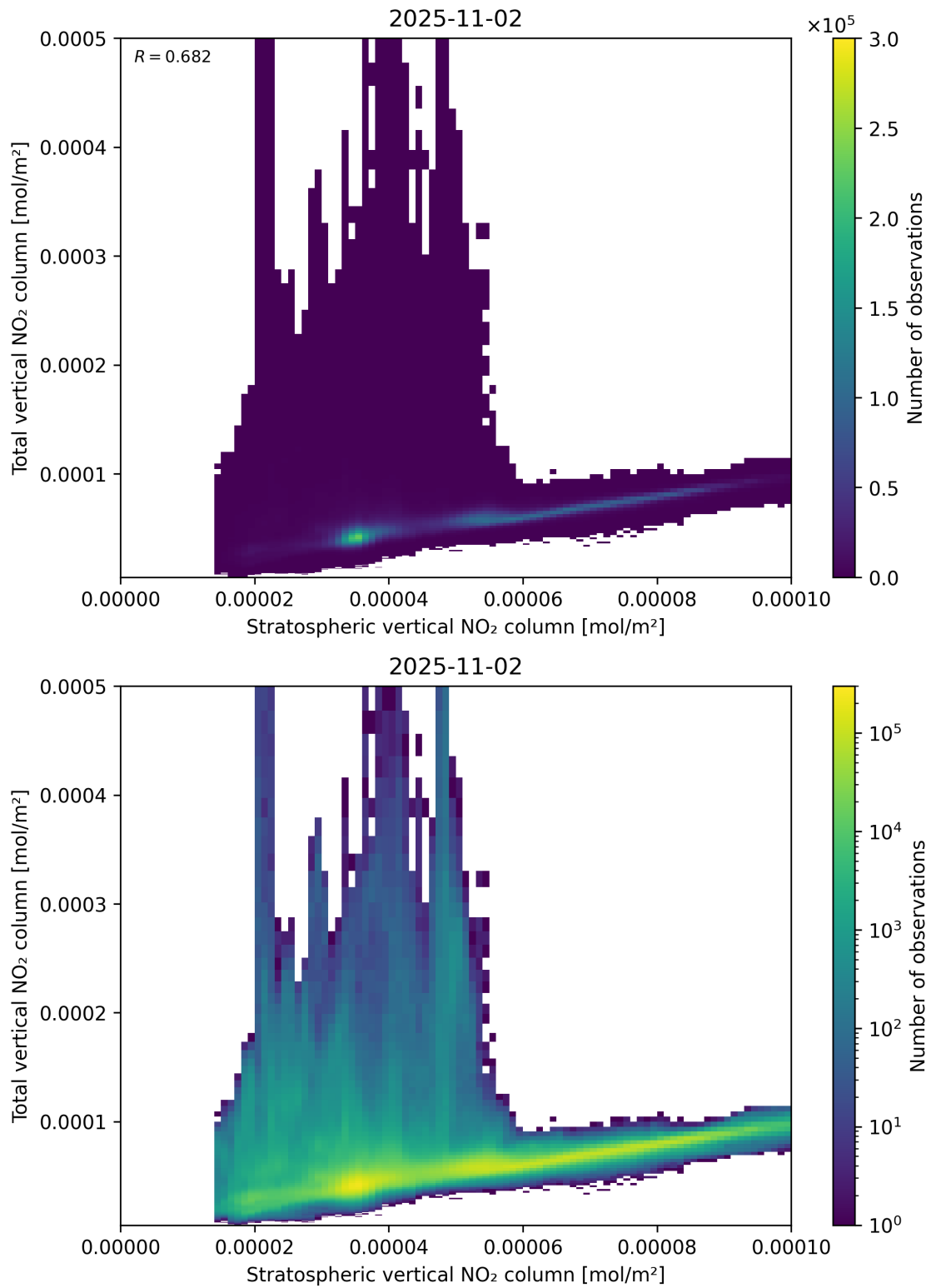
Figure 100: Scatter density plot of “Stratospheric vertical NO 2 column” against “Total vertical NO 2 column” for 2025-11-02 to 2025-11-03.
