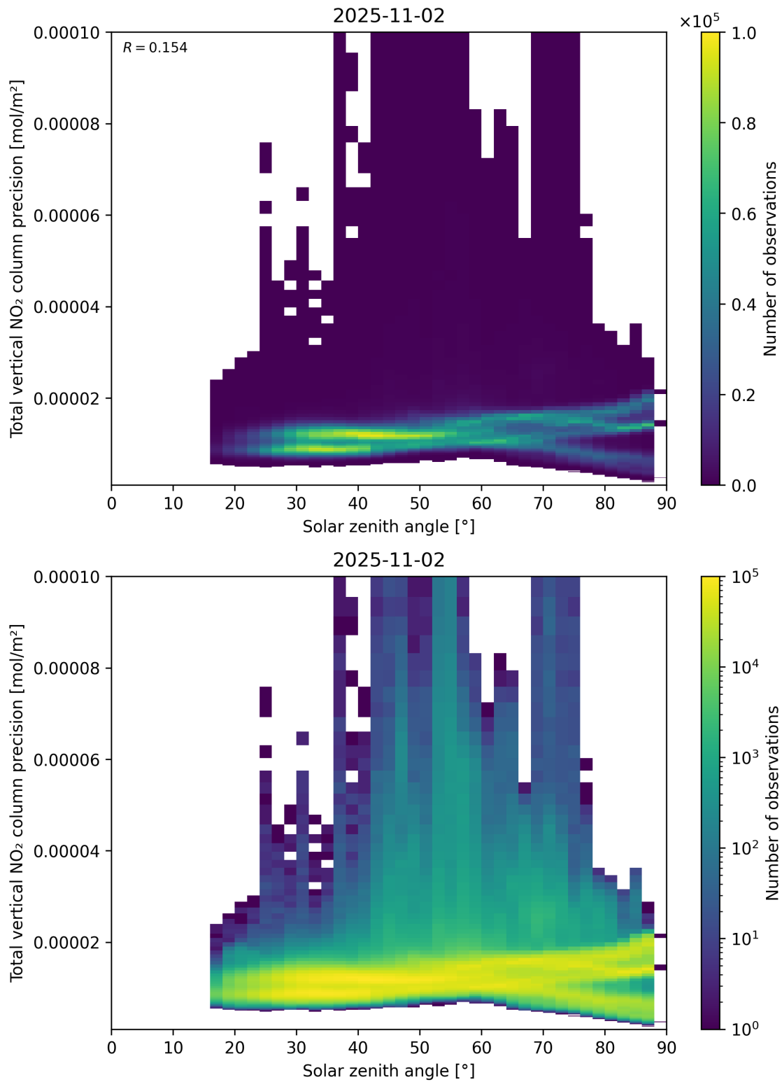
Figure 154: Scatter density plot of “Solar zenith angle” against “Total vertical NO 2 column precision” for 2025-11-02 to 2025-11-03.
