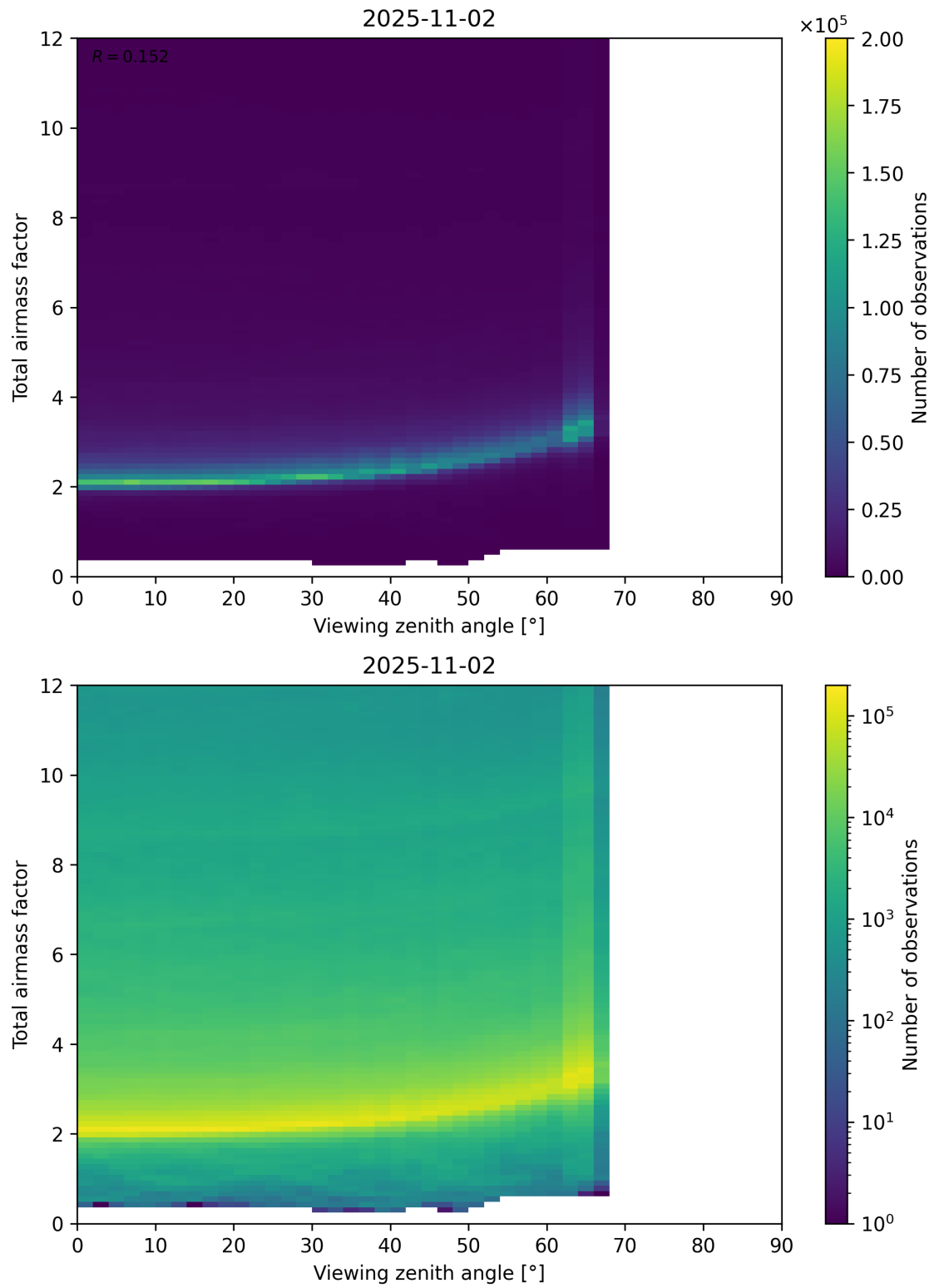
Figure 160: Scatter density plot of “Viewing zenith angle” against “Total airmass factor” for 2025-11-02 to 2025-11-03.
