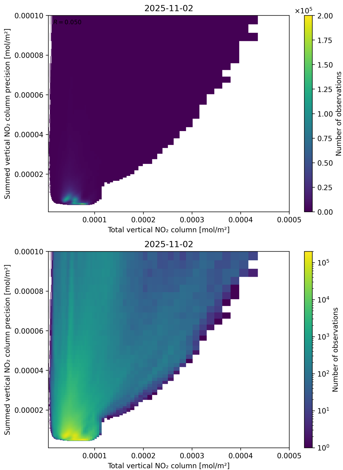
Figure 113: Scatter density plot of “Total vertical NO 2 column” against “Summed vertical NO 2 column precision” for 2025-11-02 to 2025-11-03.
