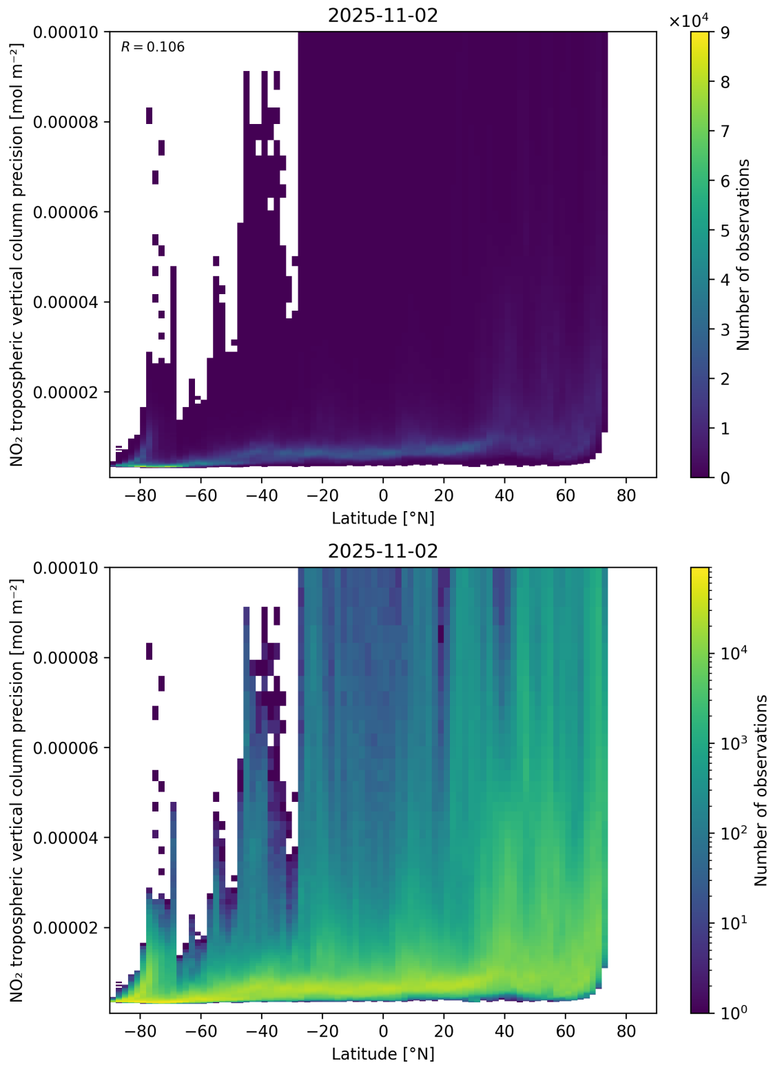
Figure 93: Scatter density plot of “Latitude” against “NO 2 tropospheric vertical column precision” for 2025-11-02 to 2025-11-03.
