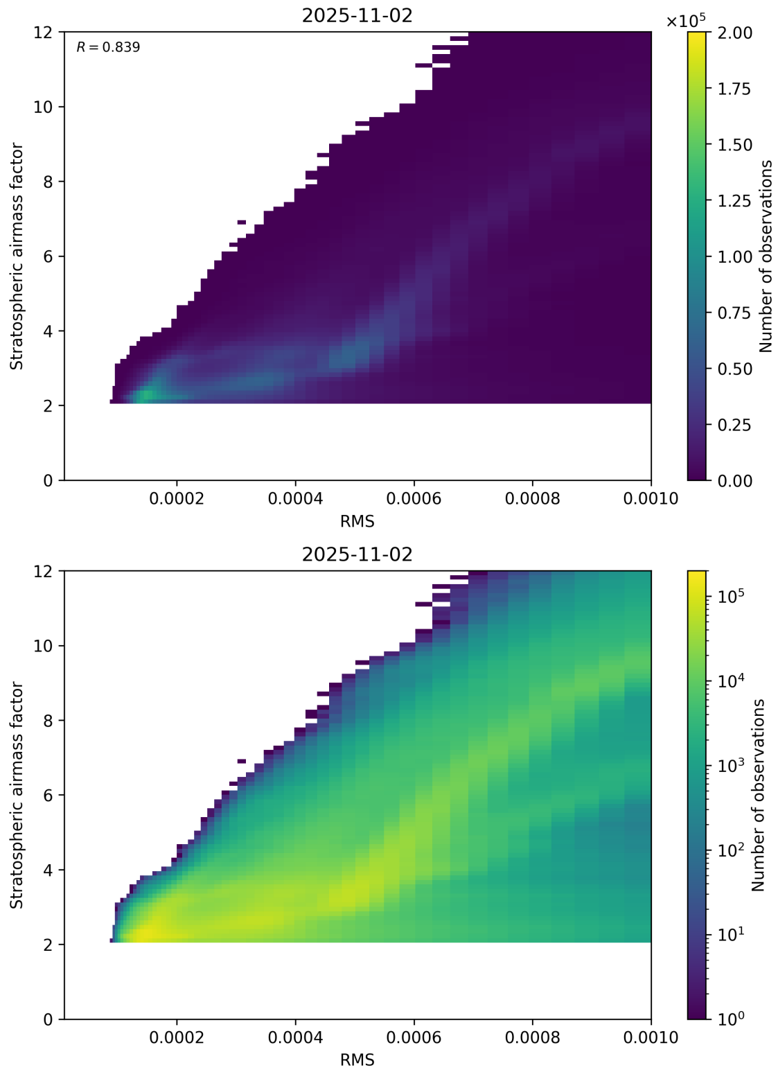
Figure 144: Scatter density plot of “RMS” against “Stratospheric airmass factor” for 2025-11-02 to 2025-11-03.
