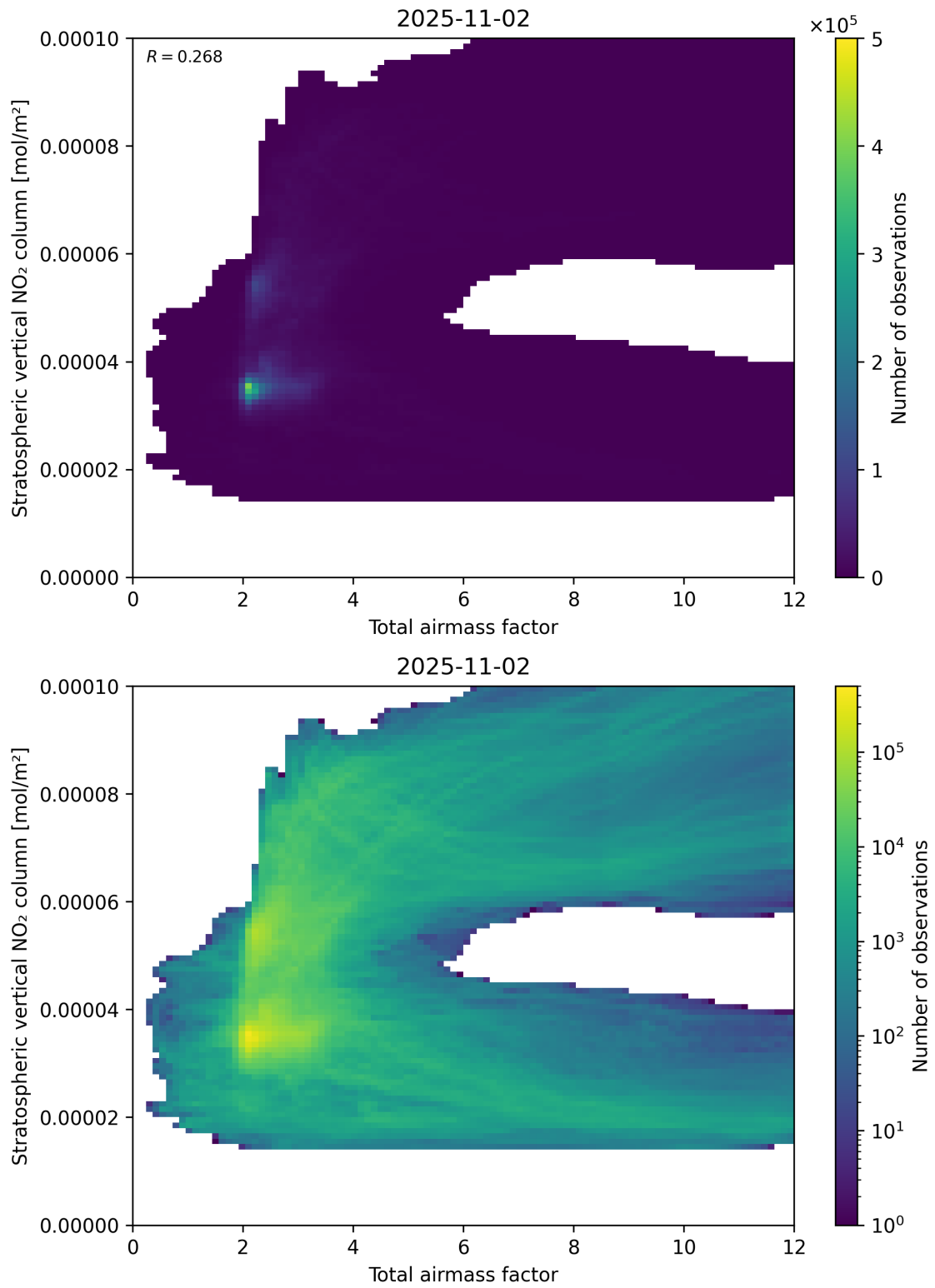
Figure 64: Scatter density plot of “Total airmass factor” against “Stratospheric vertical \text{NO}_2 column” for 2025-11-02 to 2025-11-03.
