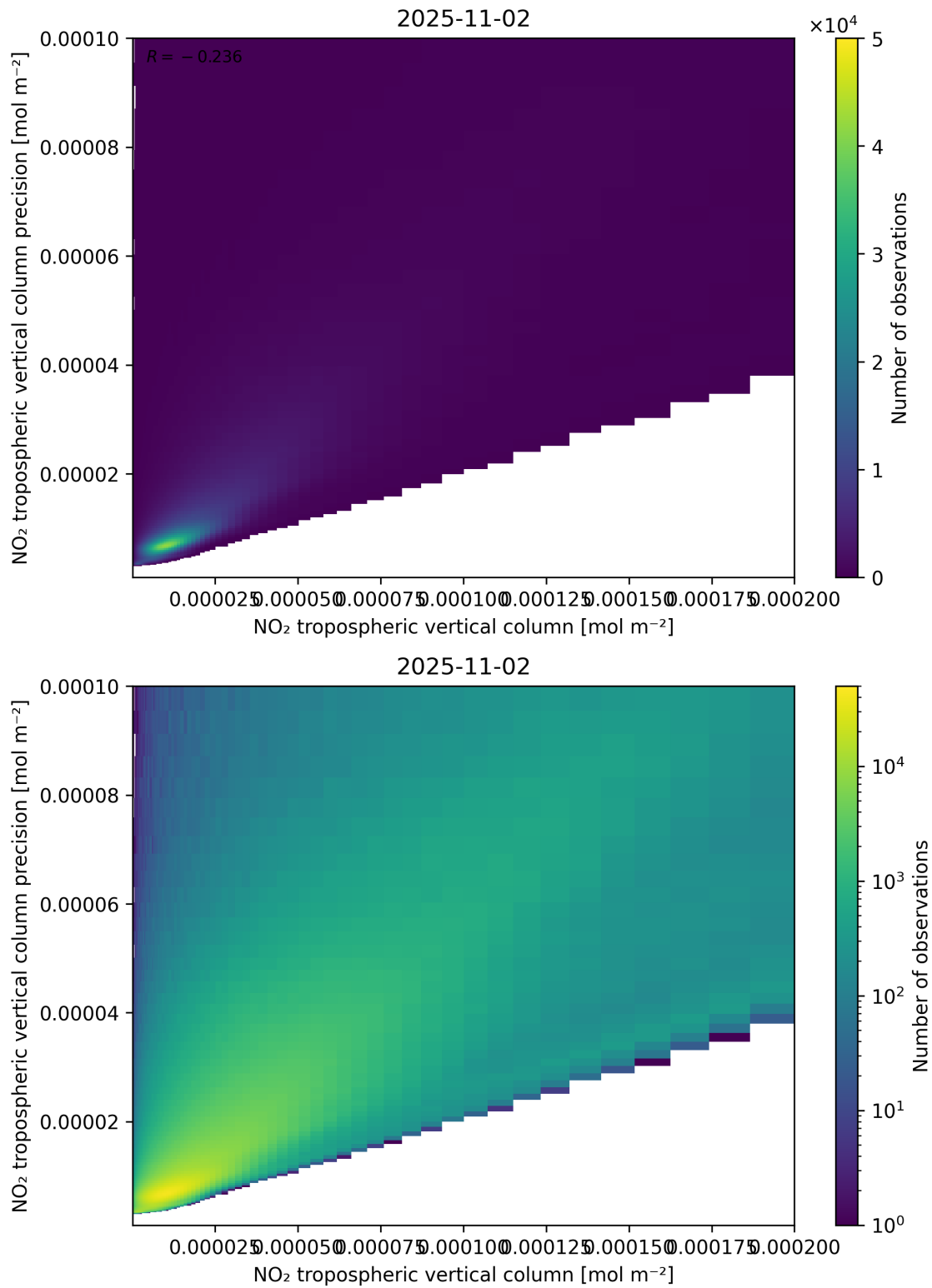
Figure 130: Scatter density plot of “NO 2 tropospheric vertical column” against “NO 2 tropospheric vertical column precision” for 2025-11-02 to 2025-11-03.
