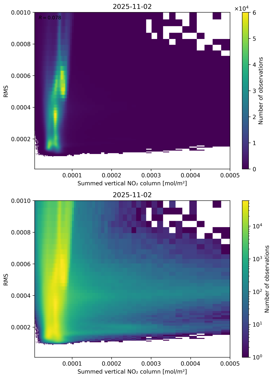
Figure 109: Scatter density plot of “Summed vertical NO 2 column” against “RMS” for 2025-11-02 to 2025-11-03.
