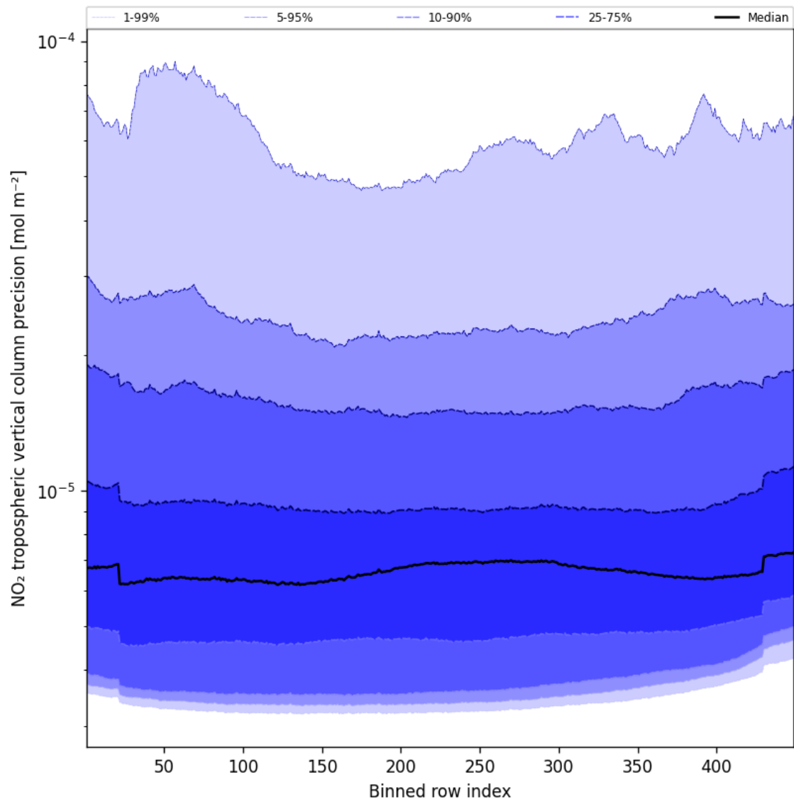
Figure 47: Along track statistics of “NO 2 tropospheric vertical column precision” for 2025-11-02 to 2025-11-03
