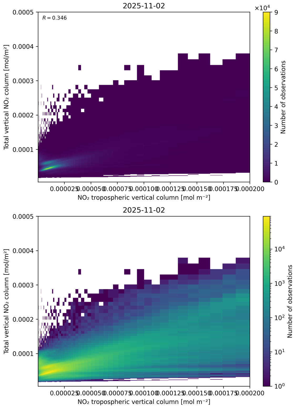
Figure 128: Scatter density plot of “NO 2 tropospheric vertical column” against “Total vertical NO 2 column” for 2025-11-02 to 2025-11-03.
