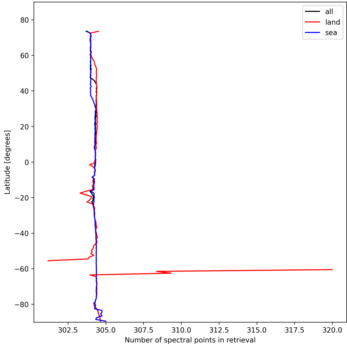
Figure 16: Zonal average of “Number of spectral points in retrieval” for 2025-11-02 to 2025-11-03.
