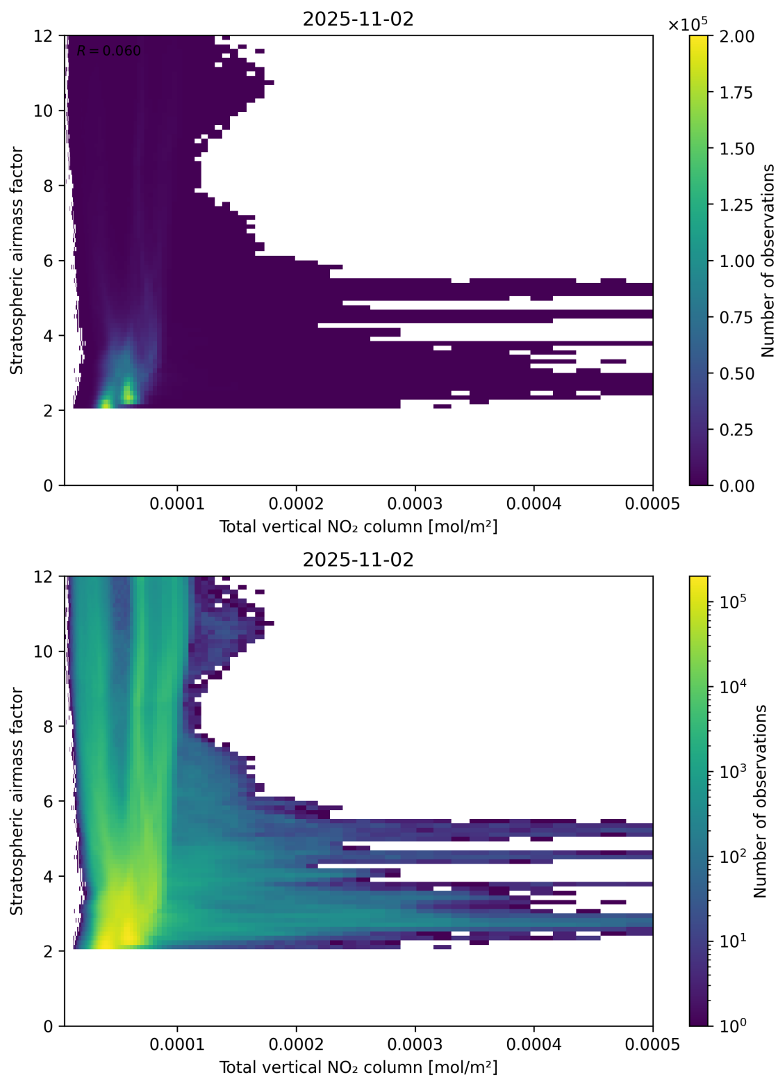
Figure 110: Scatter density plot of “Total vertical NO 2 column” against “Stratospheric airmass factor” for 2025-11-02 to 2025-11-03.
