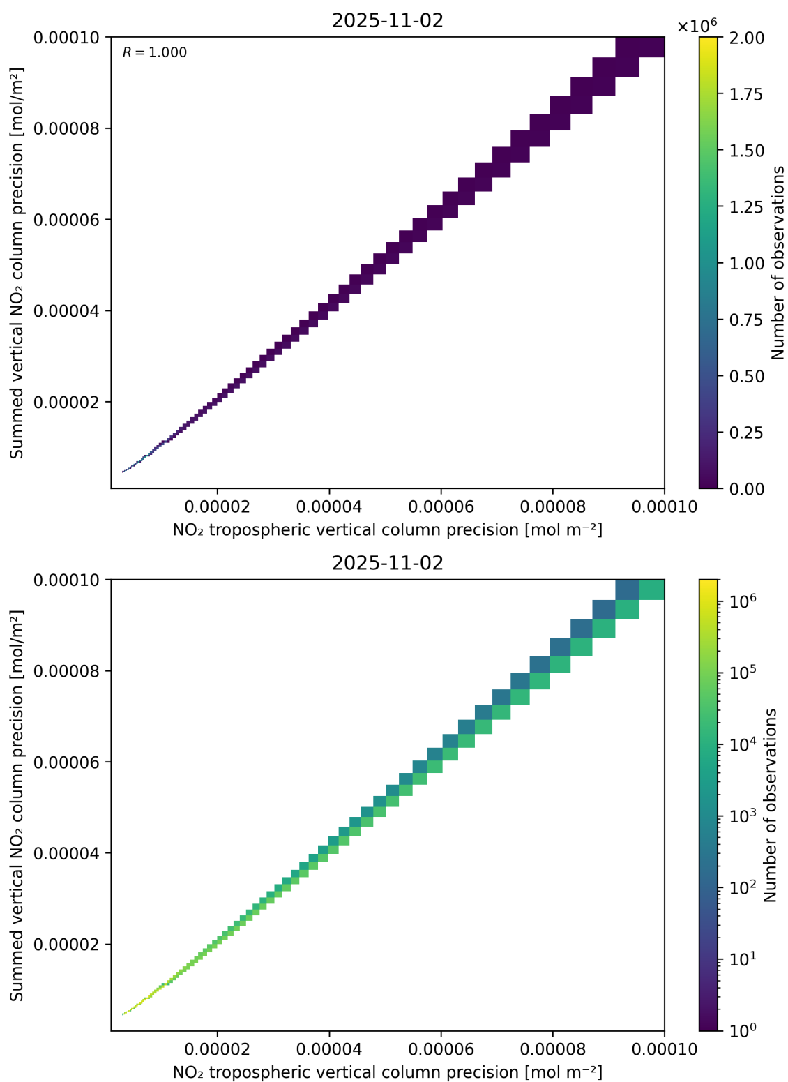
Figure 137: Scatter density plot of “NO 2 tropospheric vertical column precision” against “Summed vertical NO 2 column precision” for 2025-11-02 to 2025-11-03.
