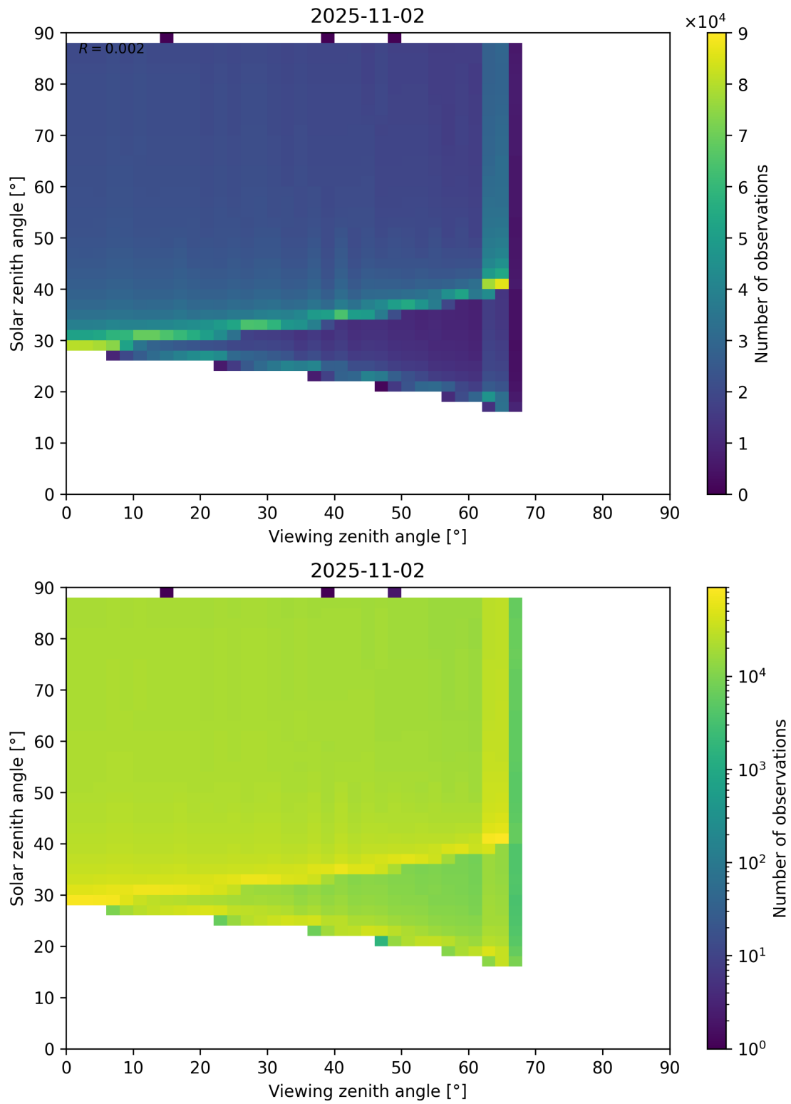
Figure 172: Scatter density plot of “Viewing zenith angle” against “Solar zenith angle” for 2025-11-02 to 2025-11-03.
