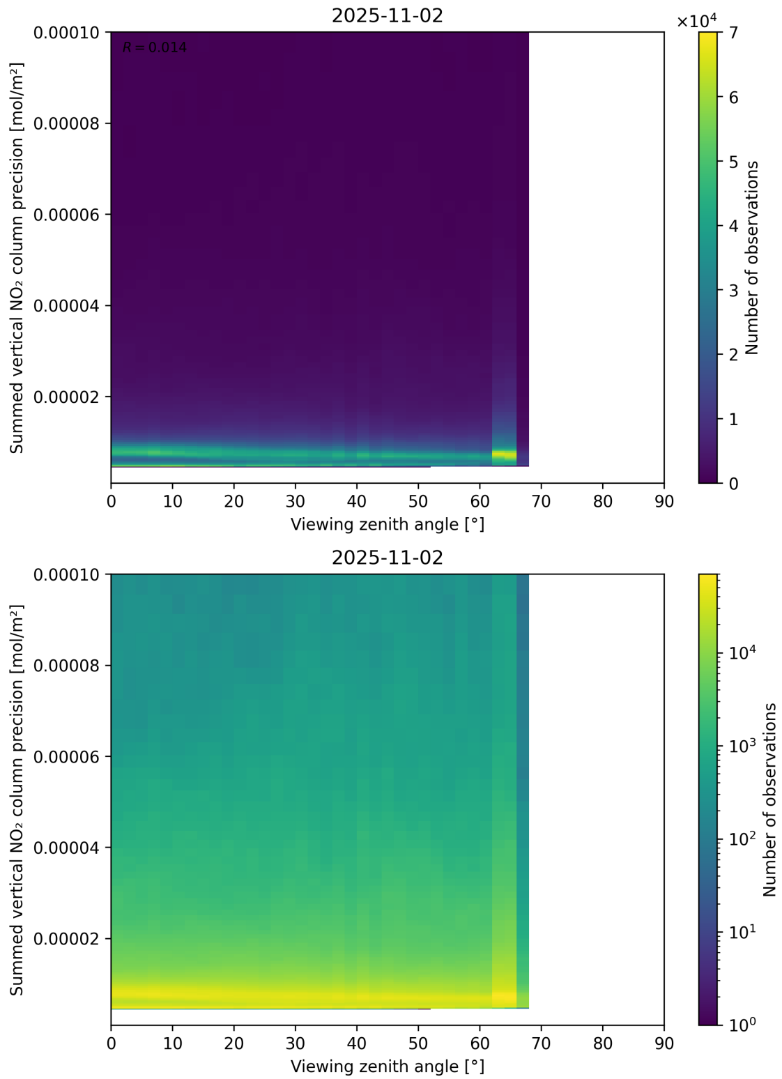
Figure 166: Scatter density plot of “Viewing zenith angle” against “Summed vertical NO 2 column precision” for 2025-11-02 to 2025-11-03.
