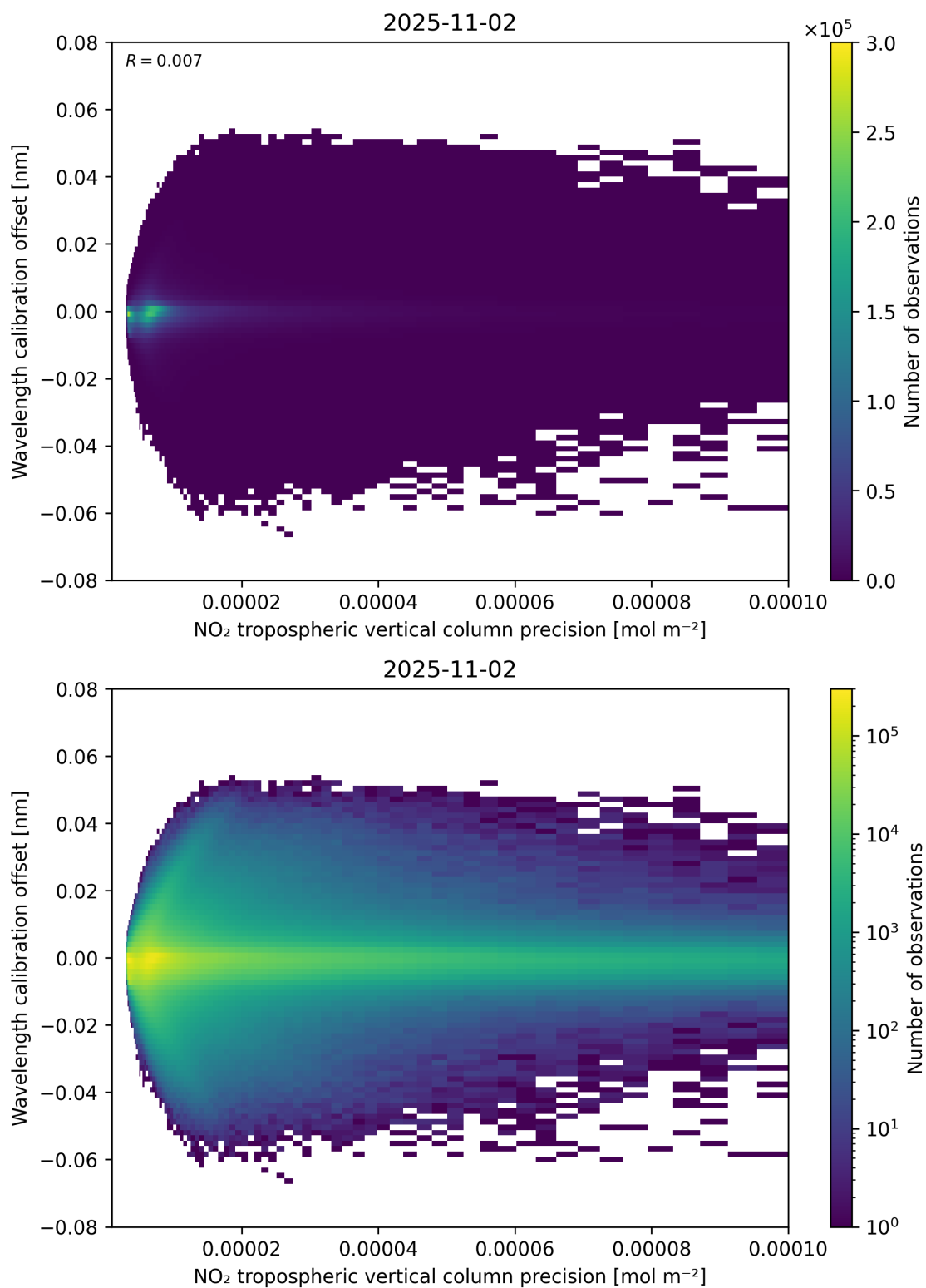
Figure 141: Scatter density plot of “NO 2 tropospheric vertical column precision” against “Wavelength calibration offset” for 2025-11-02 to 2025-11-03.
