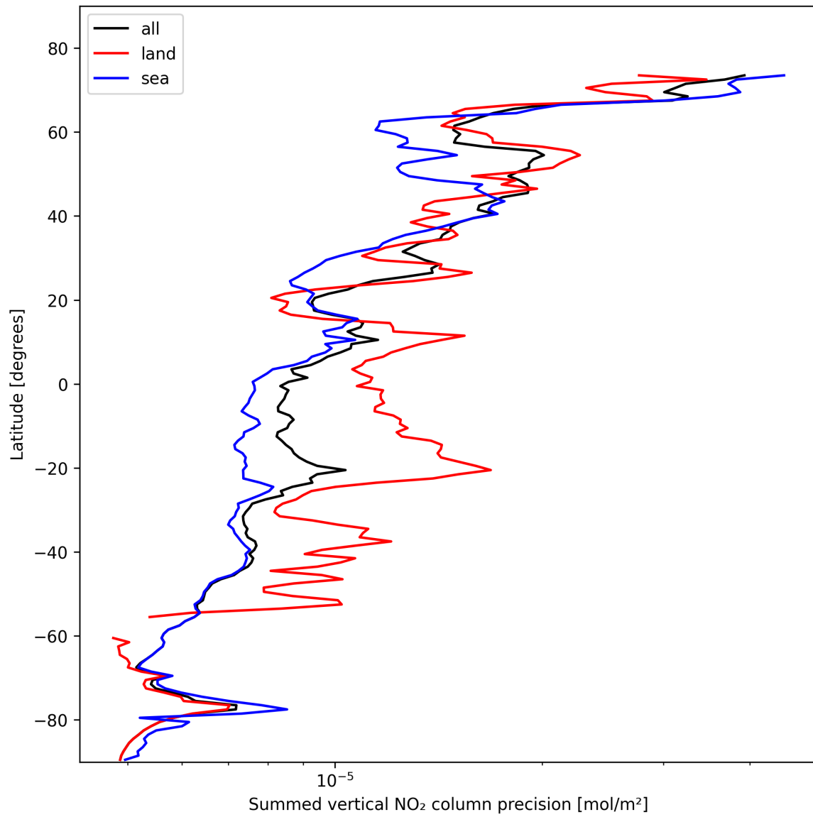
Figure 24: Zonal average of “Summed vertical NO 2 column precision” for 2025-11-02 to 2025-11-03.
