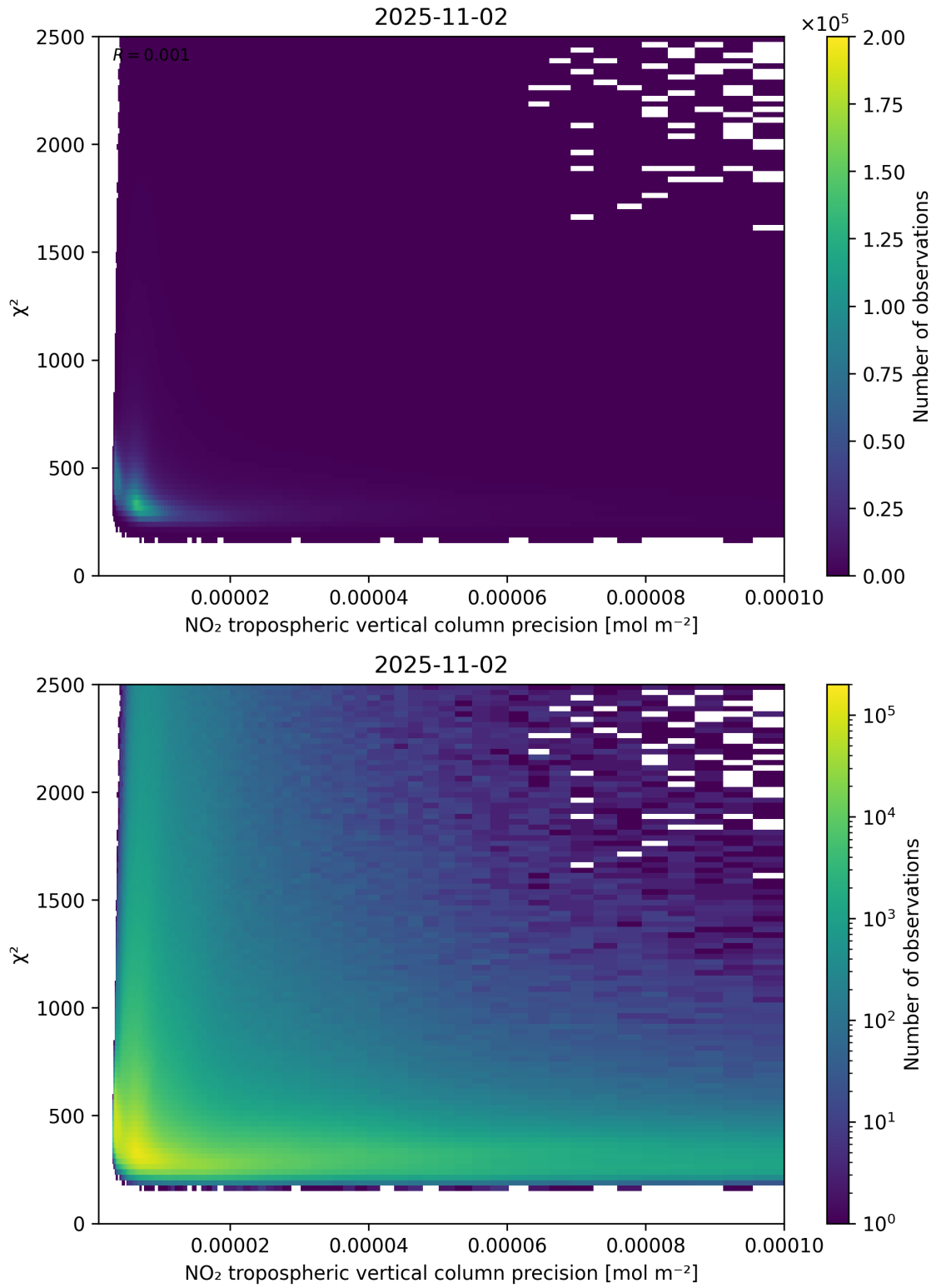
Figure 134: Scatter density plot of “NO 2 tropospheric vertical column precision” against “ \chi^2 ” for 2025-11-02 to 2025-11-03.
