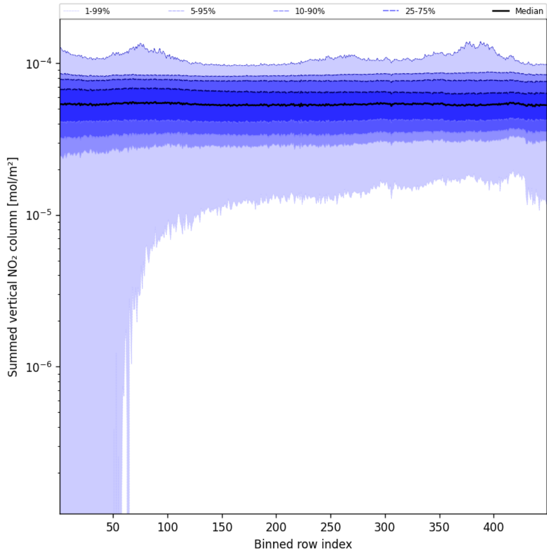
Figure 57: Along track statistics of “Summed vertical NO 2 column” for 2025-11-02 to 2025-11-03
