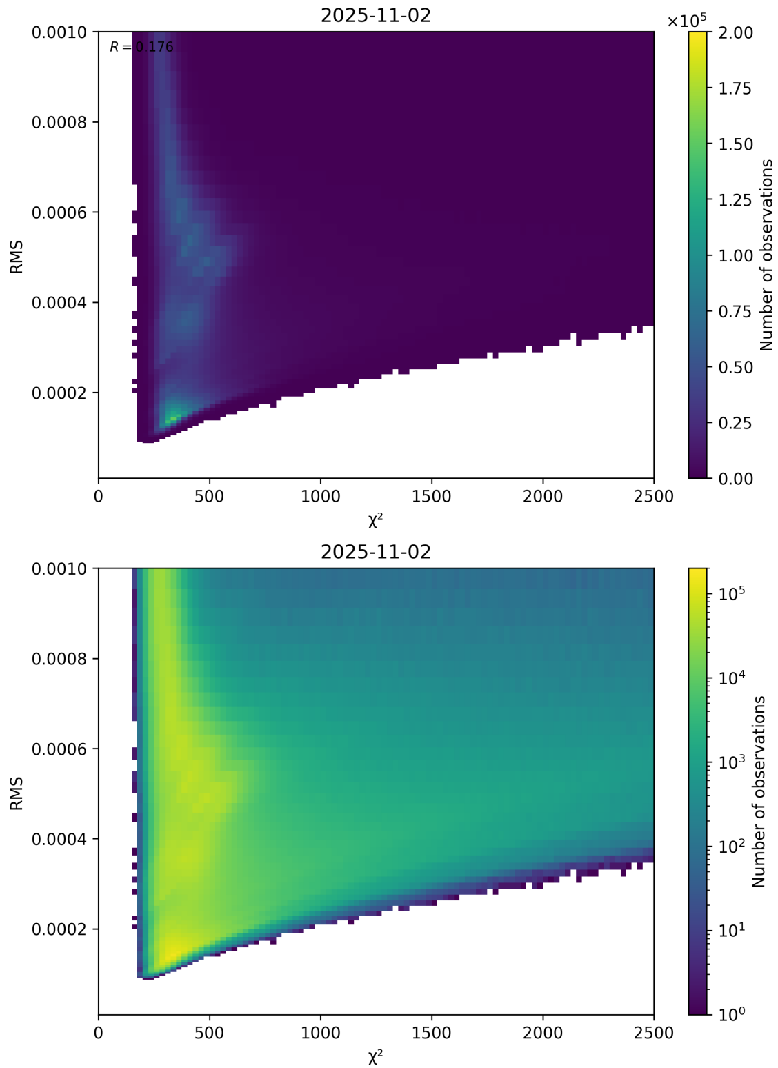
Figure 82: Scatter density plot of “ \chi^2 ” against “RMS” for 2025-11-02 to 2025-11-03.
