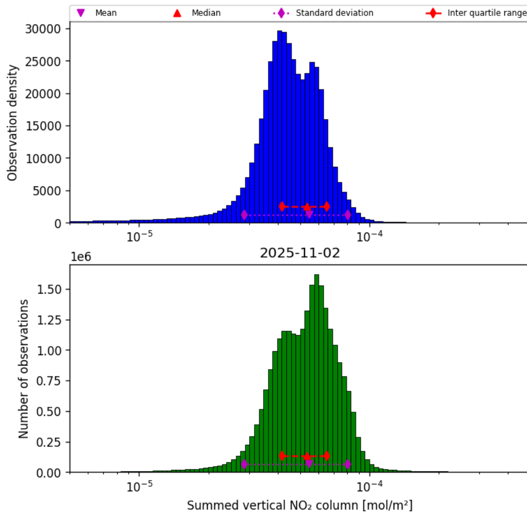
Figure 40: Histogram of “Summed vertical NO 2 column” for 2025-11-02 to 2025-11-03
