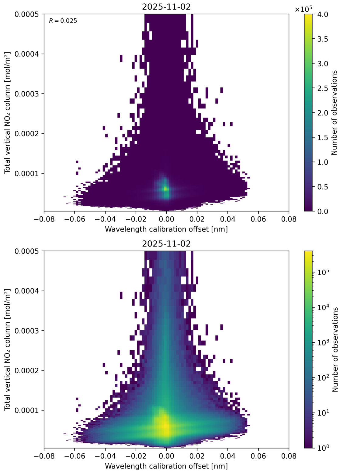
Figure 179: Scatter density plot of “Wavelength calibration offset” against “Total vertical NO 2 column” for 2025-11-02 to 2025-11-03.
