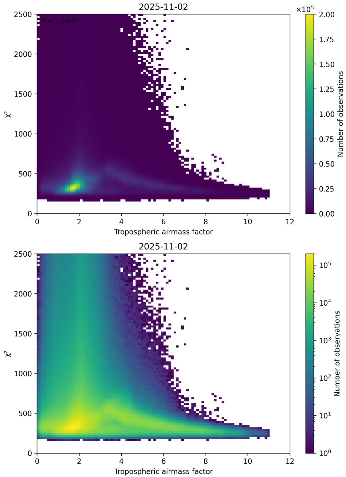
Figure 73: Scatter density plot of “Tropospheric airmass factor” against “ \chi^2 ” for 2025-11-02 to 2025-11-03.
