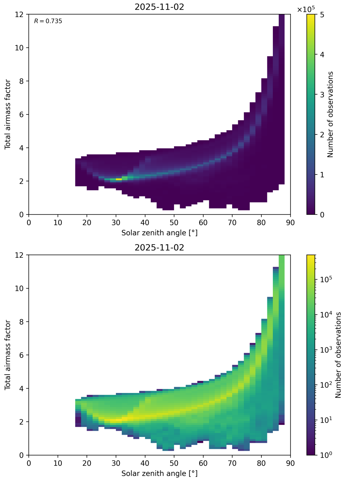
Figure 146: Scatter density plot of “Solar zenith angle” against “Total airmass factor” for 2025-11-02 to 2025-11-03.
