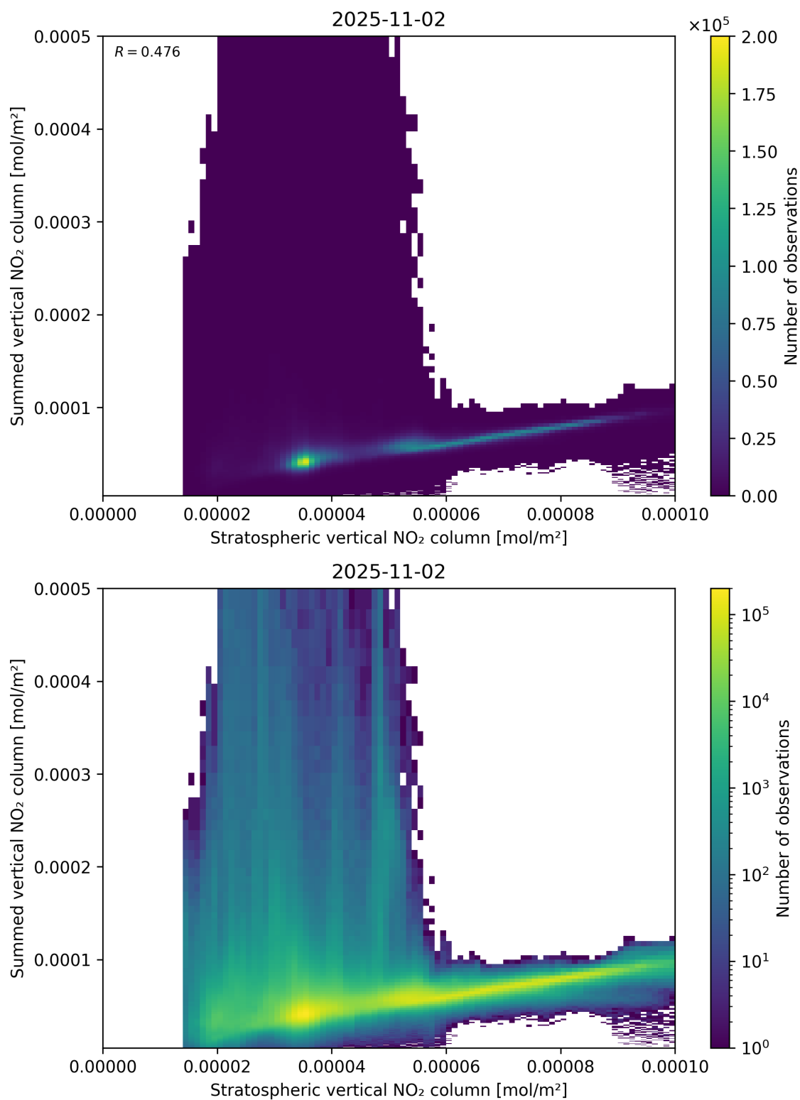
Figure 98: Scatter density plot of “Stratospheric vertical NO 2 column” against “Summed vertical NO 2 column” for 2025-11-02 to 2025-11-03.
