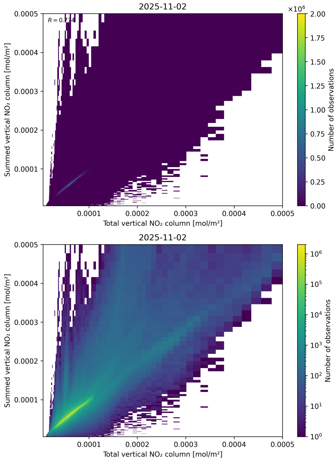
Figure 112: Scatter density plot of “Total vertical NO 2 column” against “Summed vertical NO 2 column” for 2025-11-02 to 2025-11-03.
