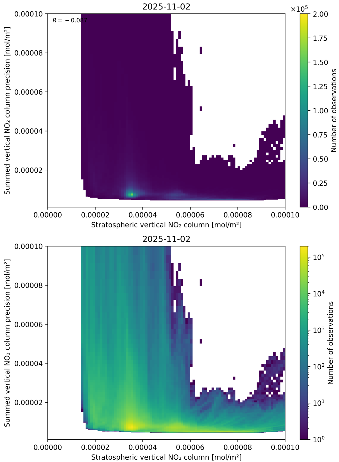
Figure 99: Scatter density plot of “Stratospheric vertical NO 2 column” against “Summed vertical NO 2 column precision” for 2025-11-02 to 2025-11-03.
