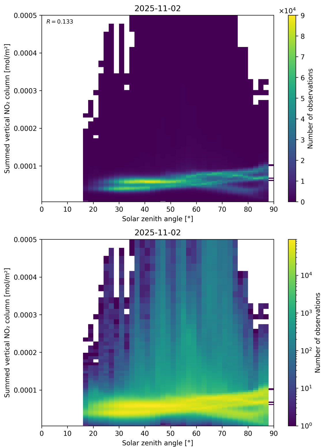
Figure 151: Scatter density plot of “Solar zenith angle” against “Summed vertical NO 2 column” for 2025-11-02 to 2025-11-03.
