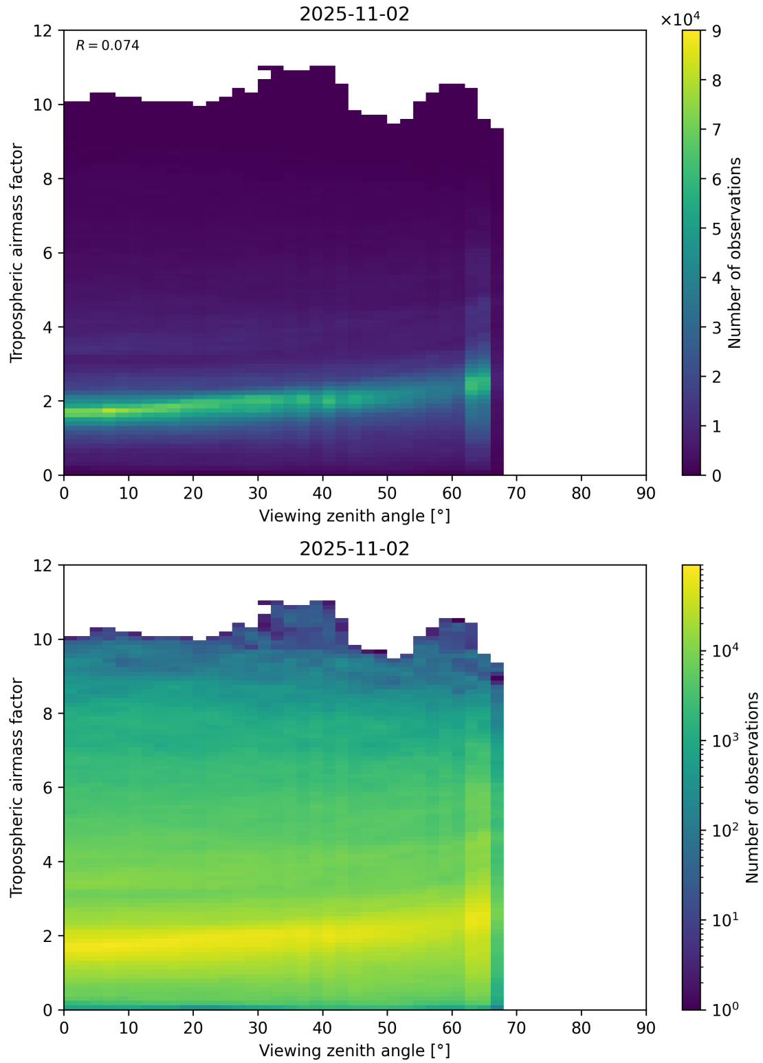
Figure 161: Scatter density plot of “Viewing zenith angle” against “Tropospheric airmass factor” for 2025-11-02 to 2025-11-03.
