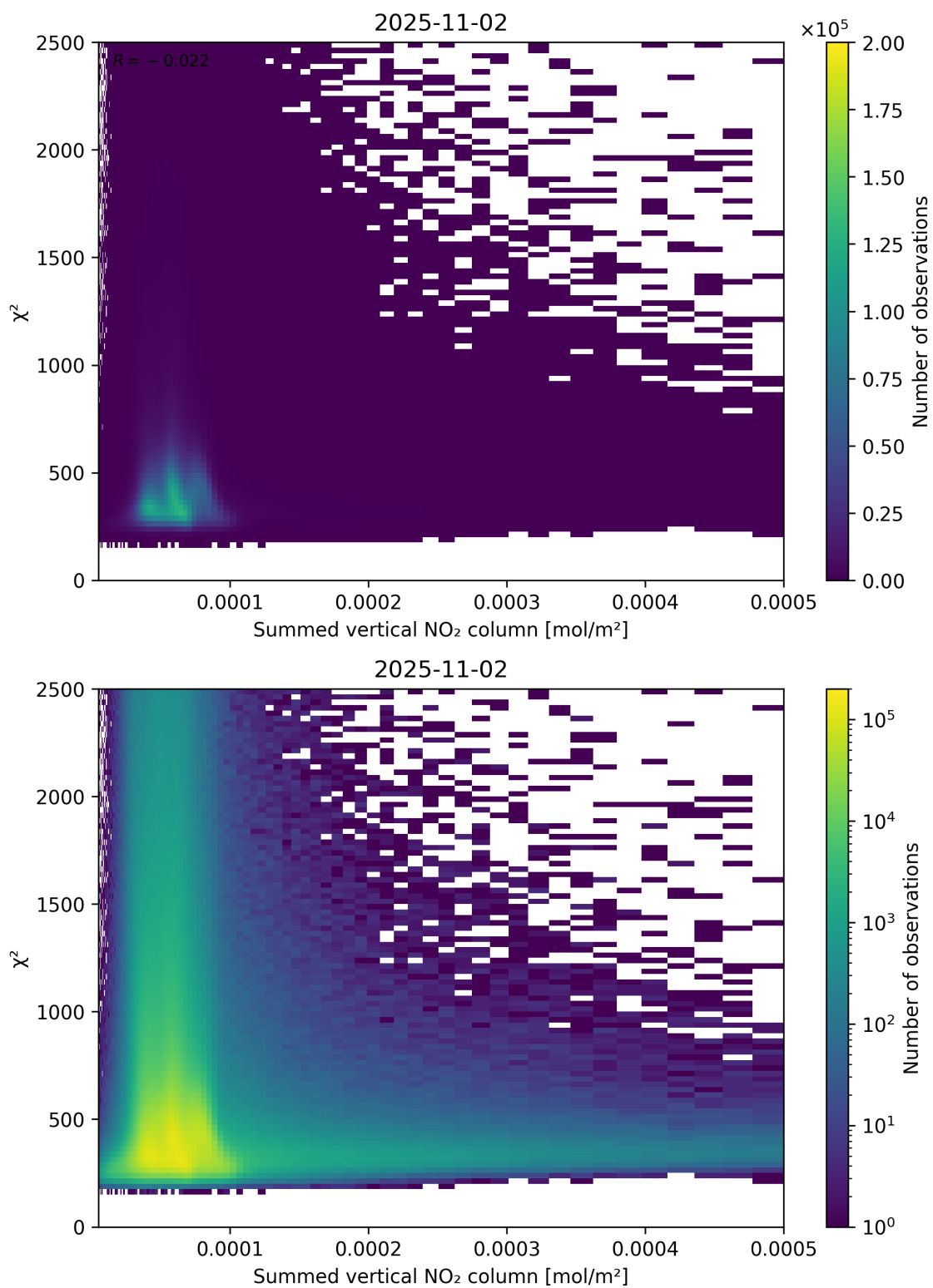
Figure 104: Scatter density plot of “Summed vertical NO 2 column” against “ \chi^2 ” for 2025-11-02 to 2025-11-03.
