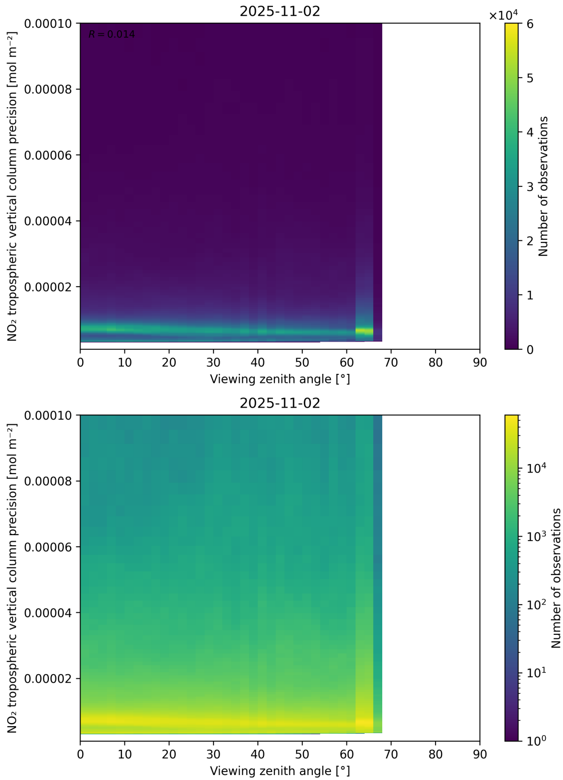
Figure 170: Scatter density plot of “Viewing zenith angle” against “NO 2 tropospheric vertical column precision” for 2025-11-02 to 2025-11-03.
