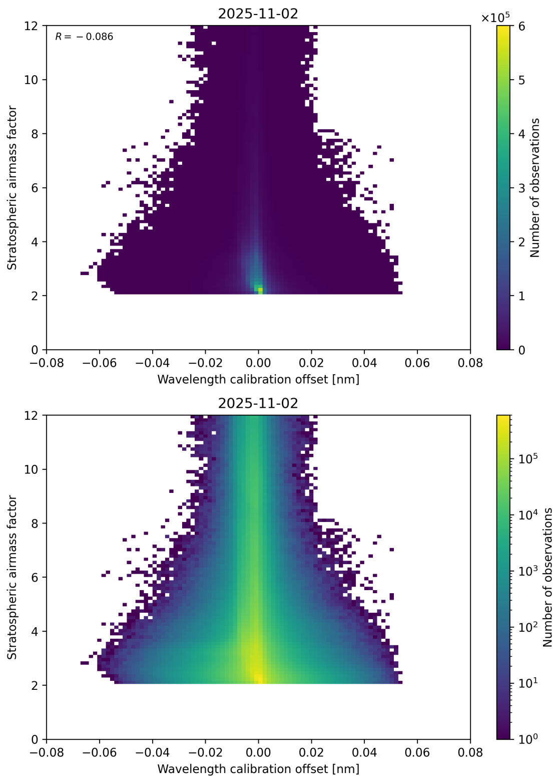
Figure 174: Scatter density plot of “Wavelength calibration offset” against “Stratospheric airmass factor” for 2025-11-02 to 2025-11-03.
