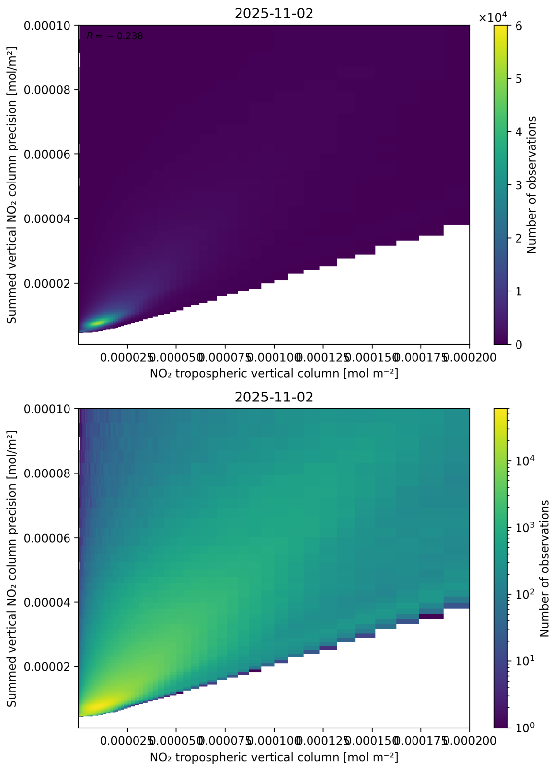
Figure 127: Scatter density plot of “NO 2 tropospheric vertical column” against “Summed vertical NO 2 column precision” for 2025-11-02 to 2025-11-03.
