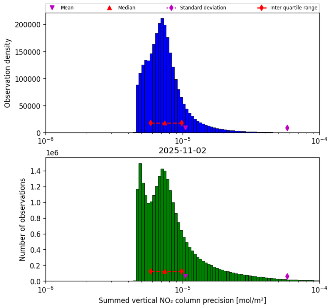
Figure 41: Histogram of “Summed vertical NO 2 column precision” for 2025-11-02 to 2025-11-03
