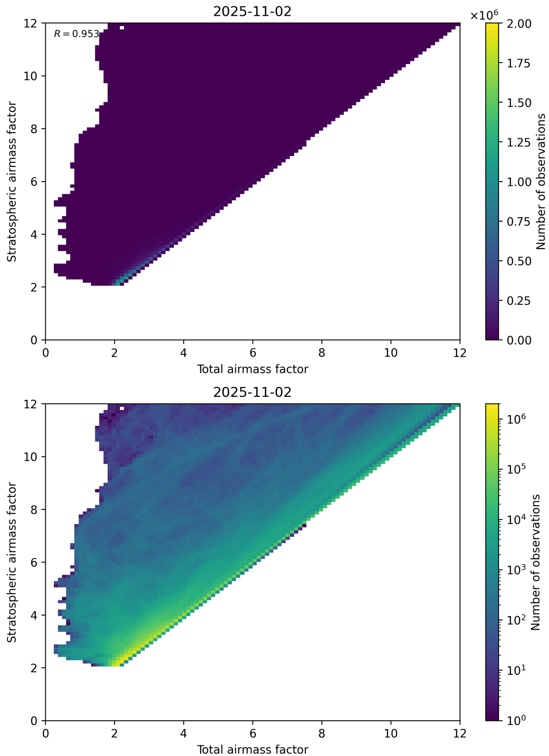
Figure 62: Scatter density plot of “Total air mass factor” against “Stratospheric air mass factor” for 2025-11-02 to 2025-11-03.
