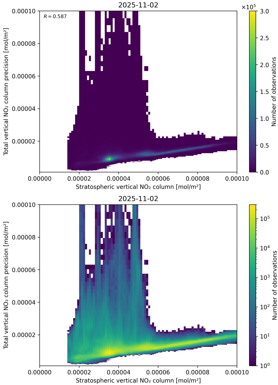
Figure 101: Scatter density plot of “Stratospheric vertical NO 2 column” against “Total vertical NO 2 column precision” for 2025-11-02 to 2025-11-03.
