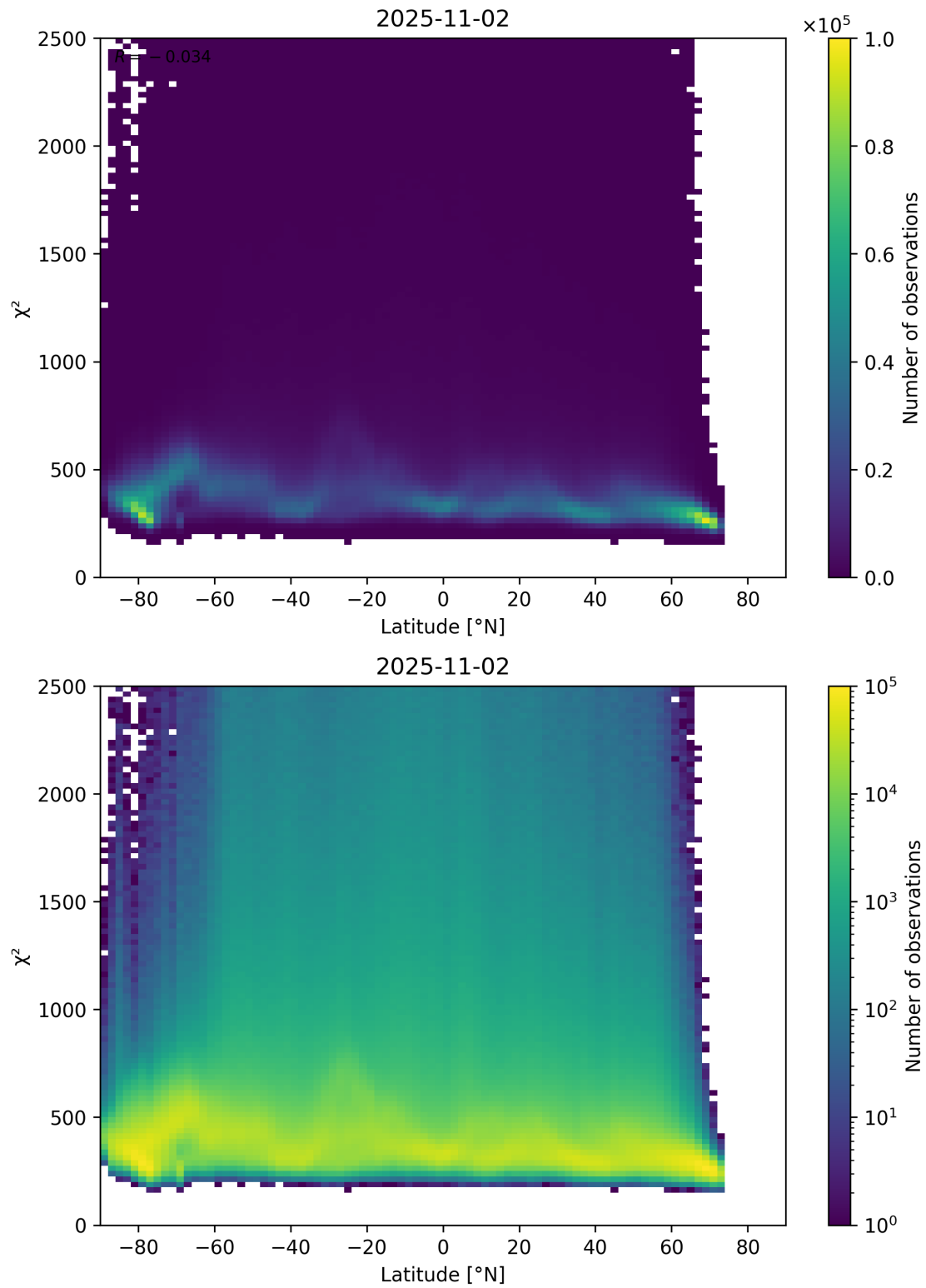
Figure 86: Scatter density plot of “Latitude” against “ \chi^2 ” for 2025-11-02 to 2025-11-03.
