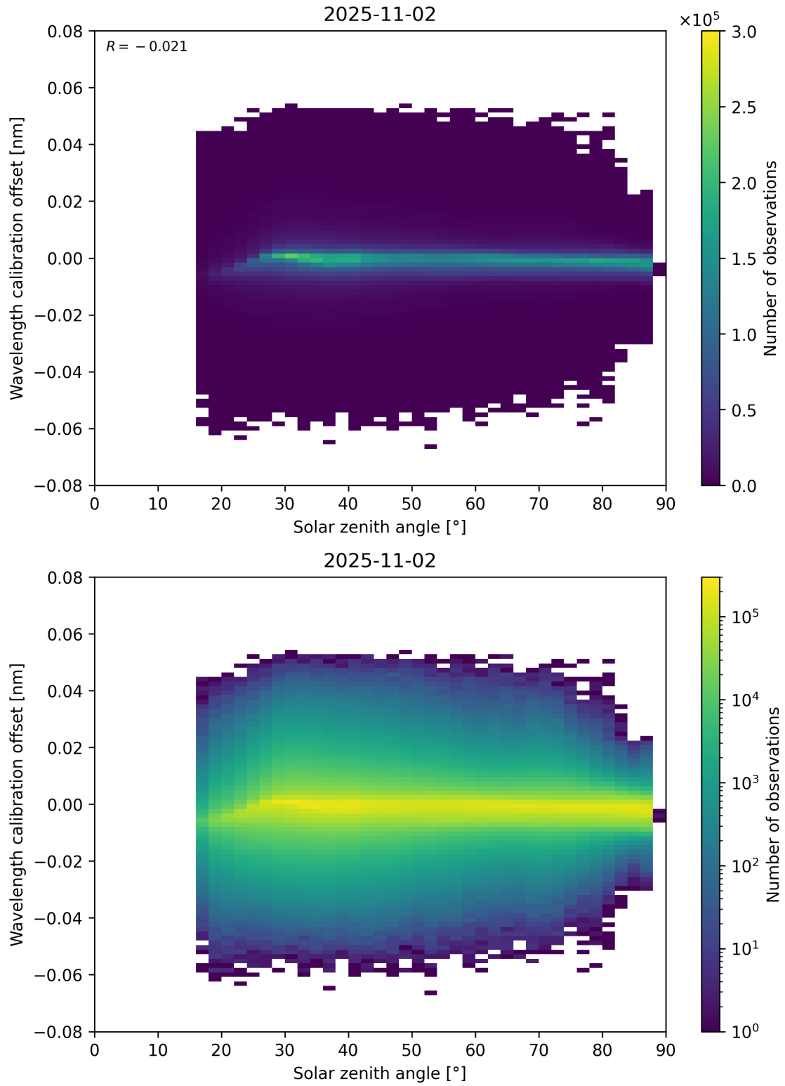
Figure 158: Scatter density plot of “Solar zenith angle” against “Wavelength calibration offset” for 2025-11-02 to 2025-11-03.
