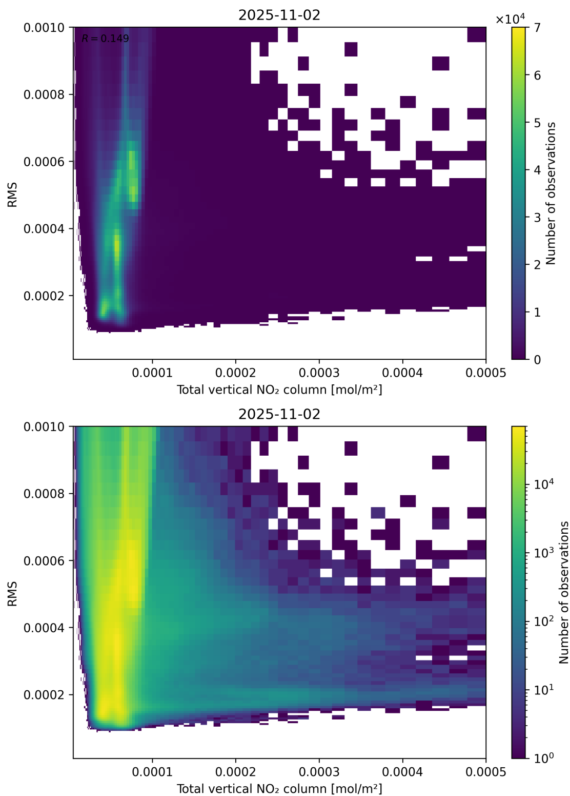
Figure 120: Scatter density plot of “Total vertical NO 2 column” against “RMS” for 2025-11-02 to 2025-11-03.
