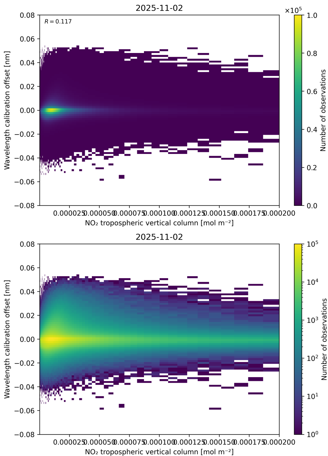
Figure 143: Scatter density plot of “NO 2 tropospheric vertical column” against “Wavelength calibration offset” for 2025-11-02 to 2025-11-03.
