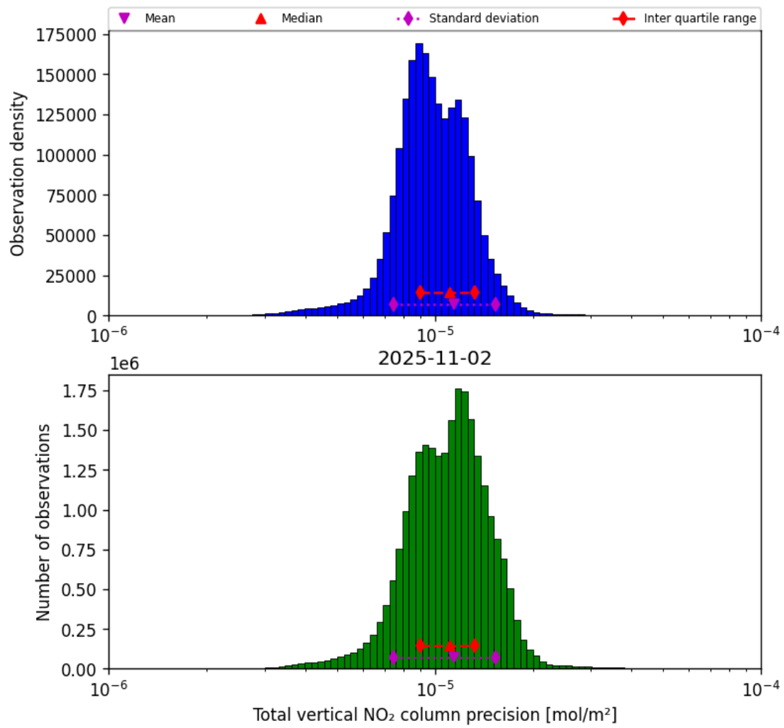
Figure 39: Histogram of “Total vertical NO 2 column precision” for 2025-11-02 to 2025-11-03
