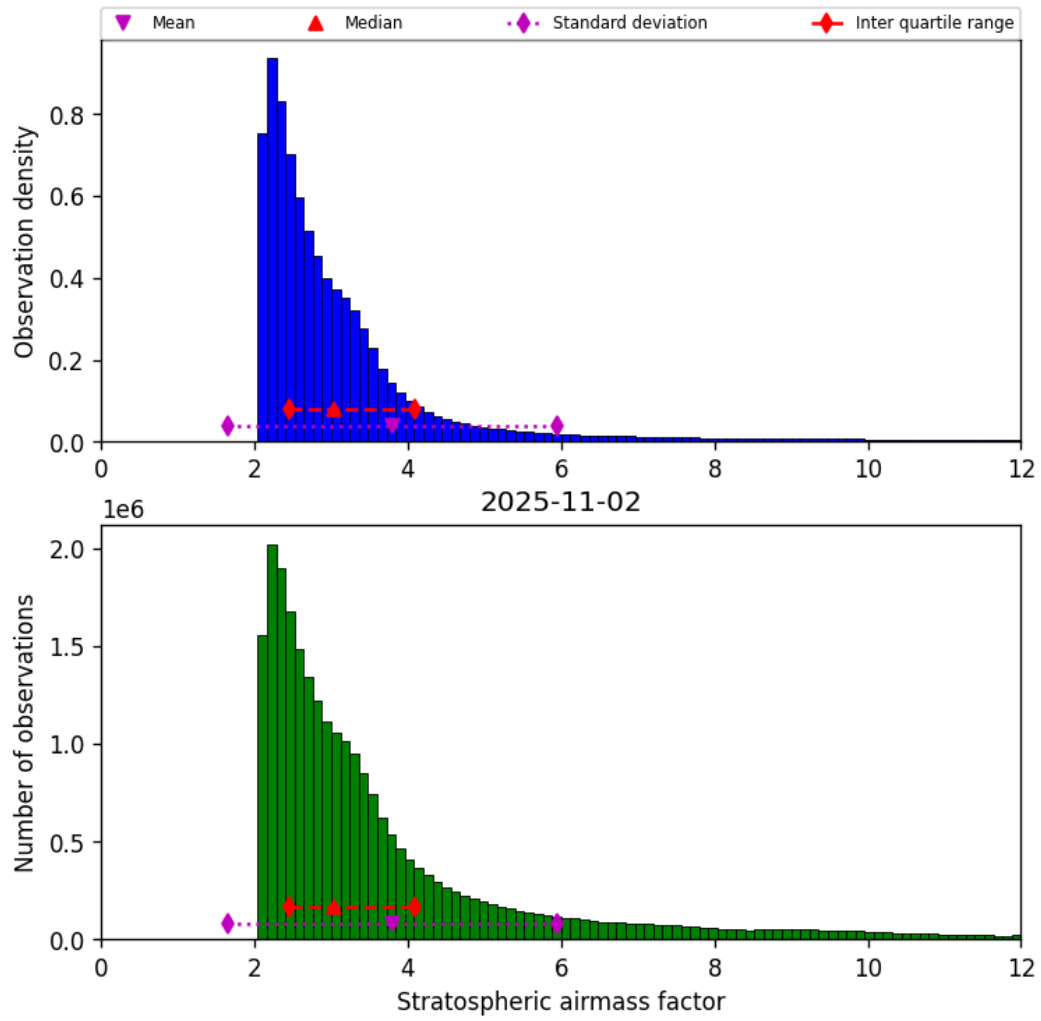
Figure 44: Histogram of “Stratospheric airmass factor” for 2025-11-02 to 2025-11-03
