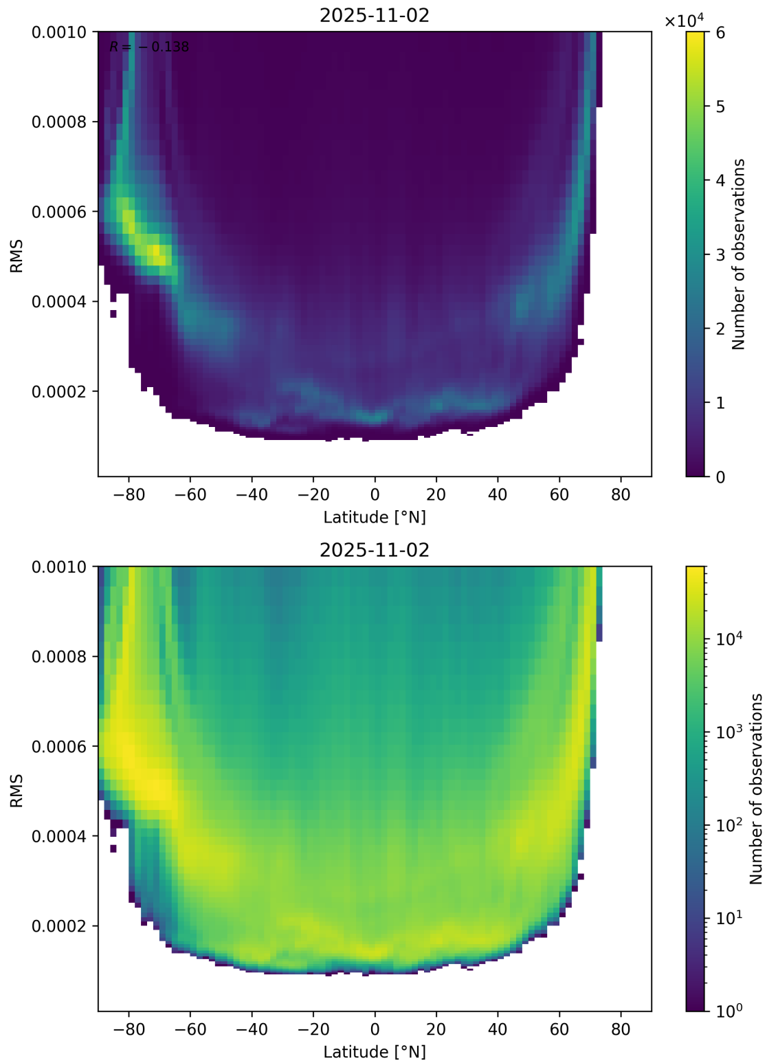
Figure 94: Scatter density plot of “Latitude” against “RMS” for 2025-11-02 to 2025-11-03.
