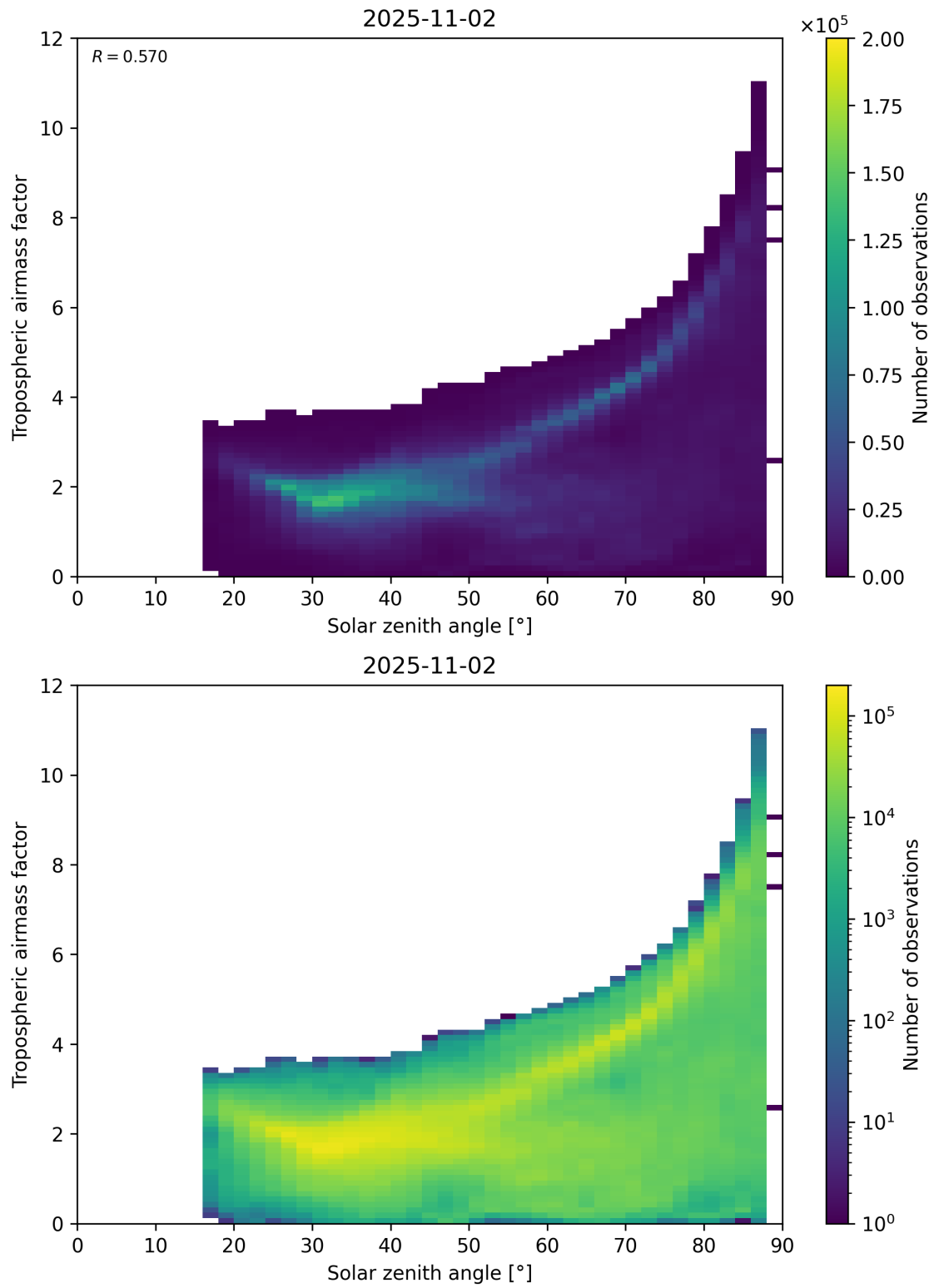
Figure 147: Scatter density plot of “Solar zenith angle” against “Tropospheric airmass factor” for 2025-11-02 to 2025-11-03.
