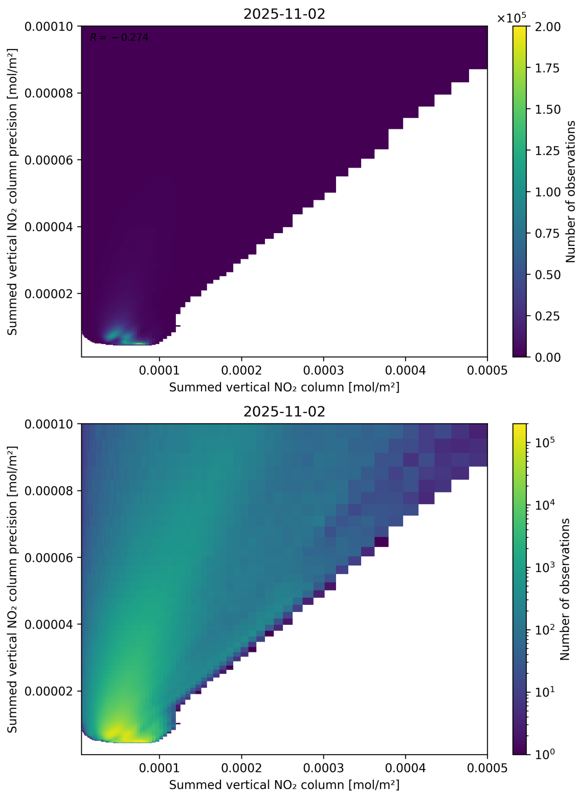
Figure 105: Scatter density plot of “Summed vertical NO 2 column” against “Summed vertical NO 2 column precision” for 2025-11-02 to 2025-11-03.
