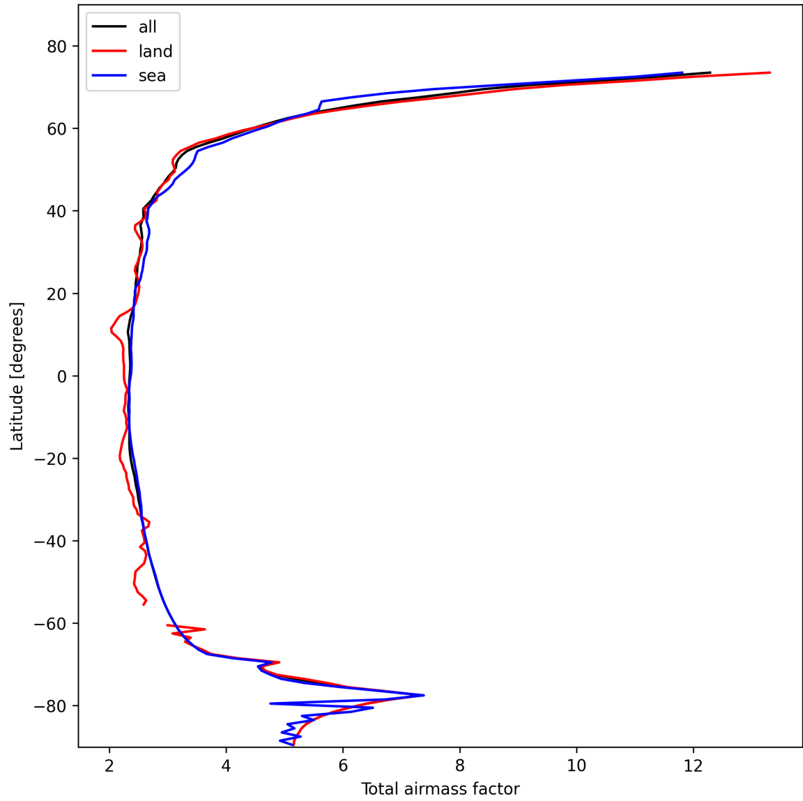
Figure 15: Zonal average of “Total airmass factor” for 2025-11-02 to 2025-11-03.
