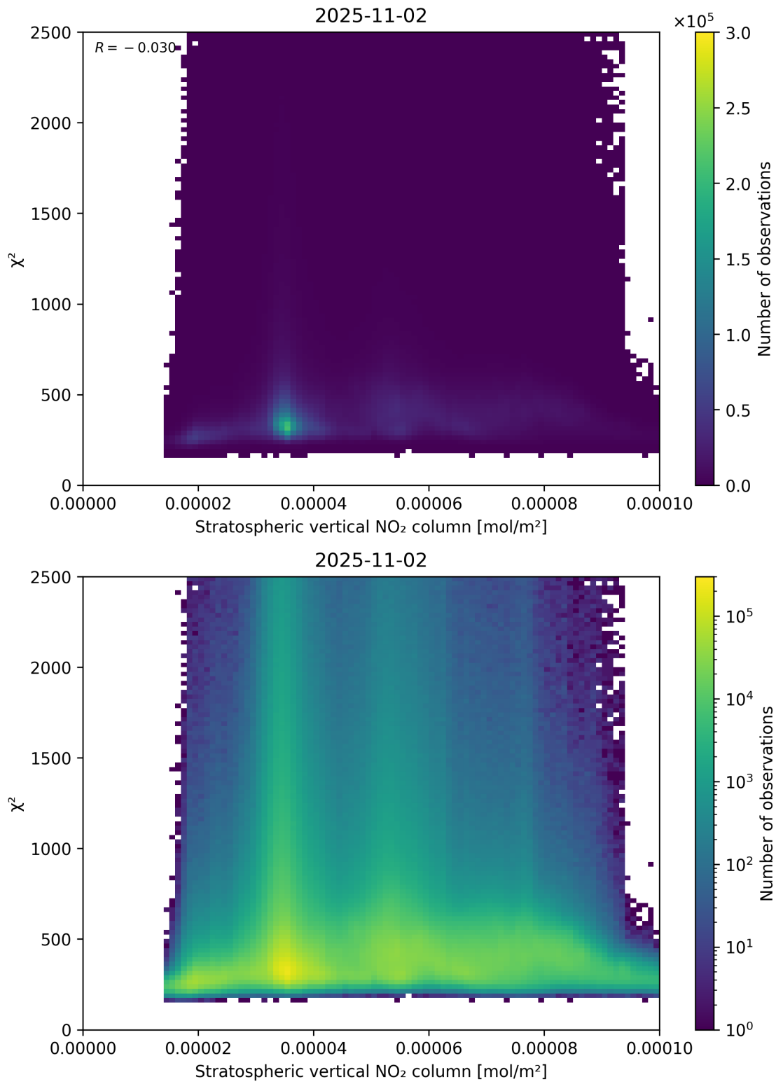
Figure 97: Scatter density plot of “Stratospheric vertical NO 2 column” against “ \chi^2 ” for 2025-11-02 to 2025-11-03.
