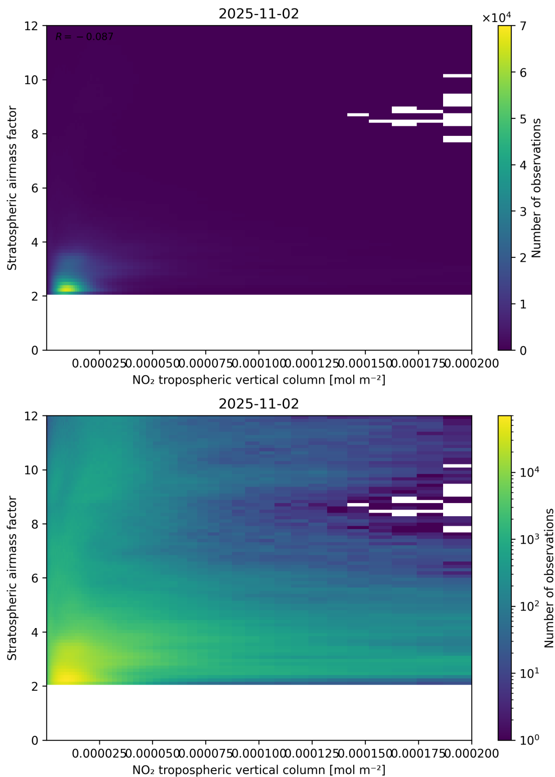
Figure 121: Scatter density plot of “NO 2 tropospheric vertical column” against “Stratospheric airmass factor” for 2025-11-02 to 2025-11-03.
