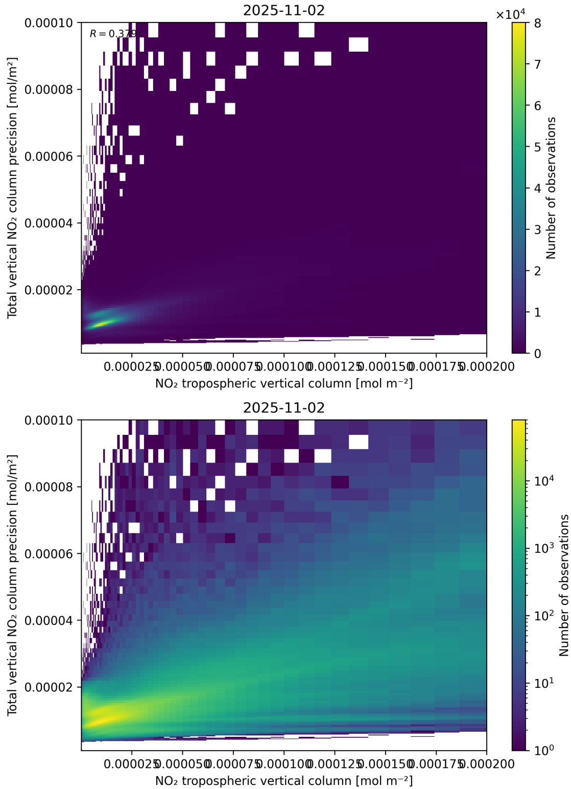
Figure 129: Scatter density plot of “NO 2 tropospheric vertical column” against “Total vertical NO 2 column precision” for 2025-11-02 to 2025-11-03.
