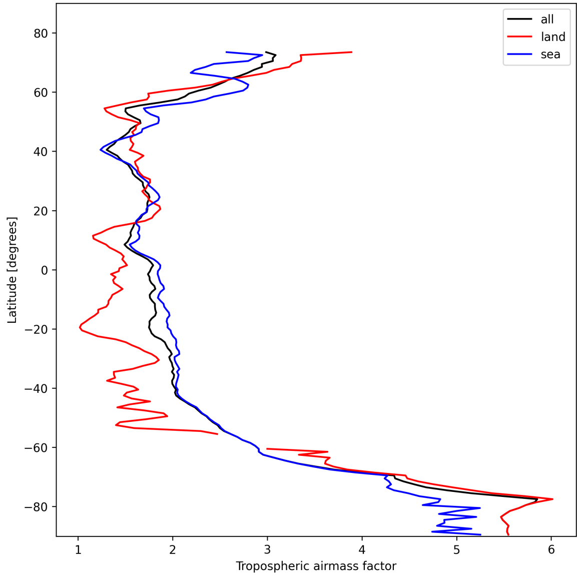
Figure 14: Zonal average of “Tropospheric airmass factor” for 2025-11-02 to 2025-11-03.
