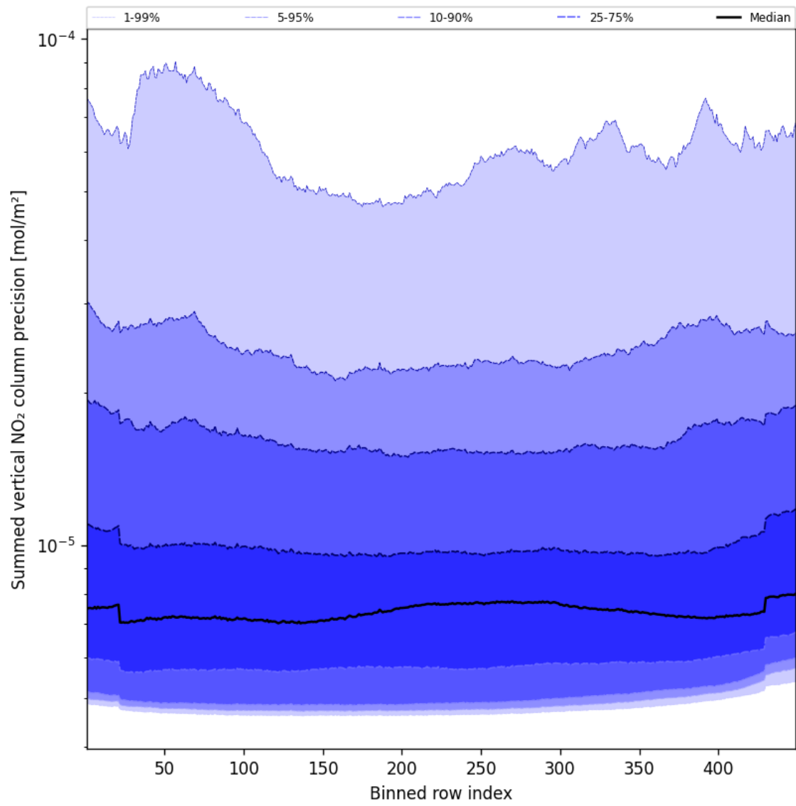
Figure 58: Along track statistics of “Summed vertical NO 2 column precision” for 2025-11-02 to 2025-11-03
