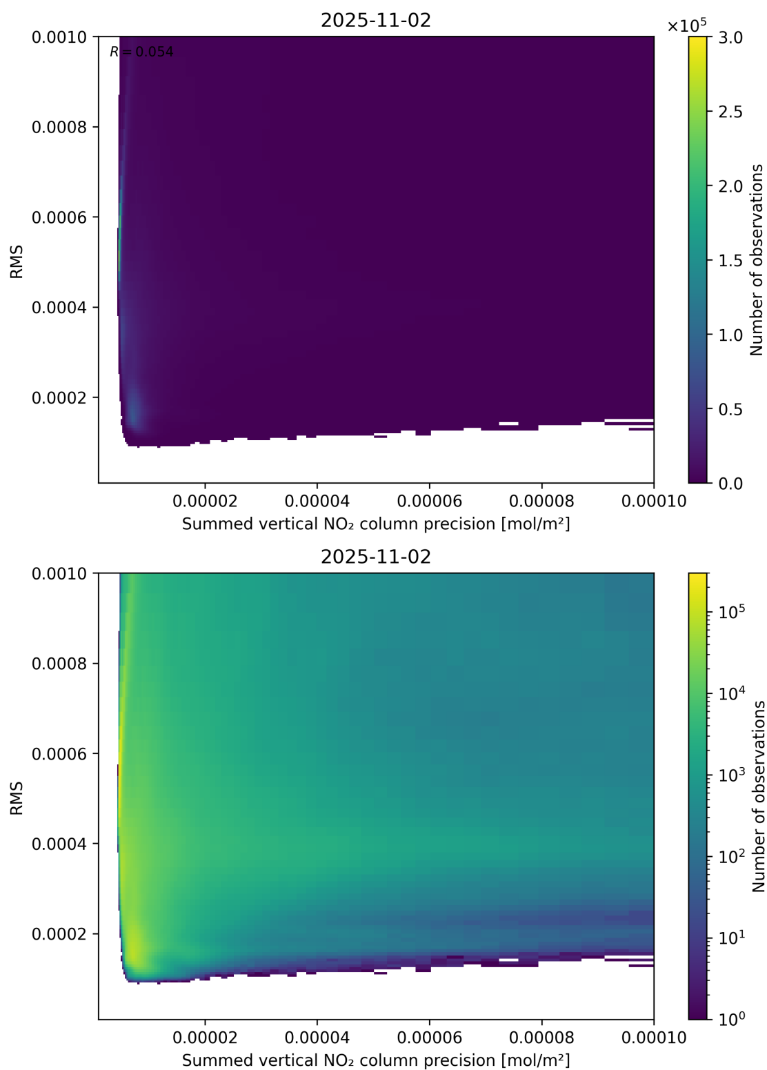
Figure 108: Scatter density plot of “Summed vertical NO 2 column precision” against “RMS” for 2025-11-02 to 2025-11-03.
