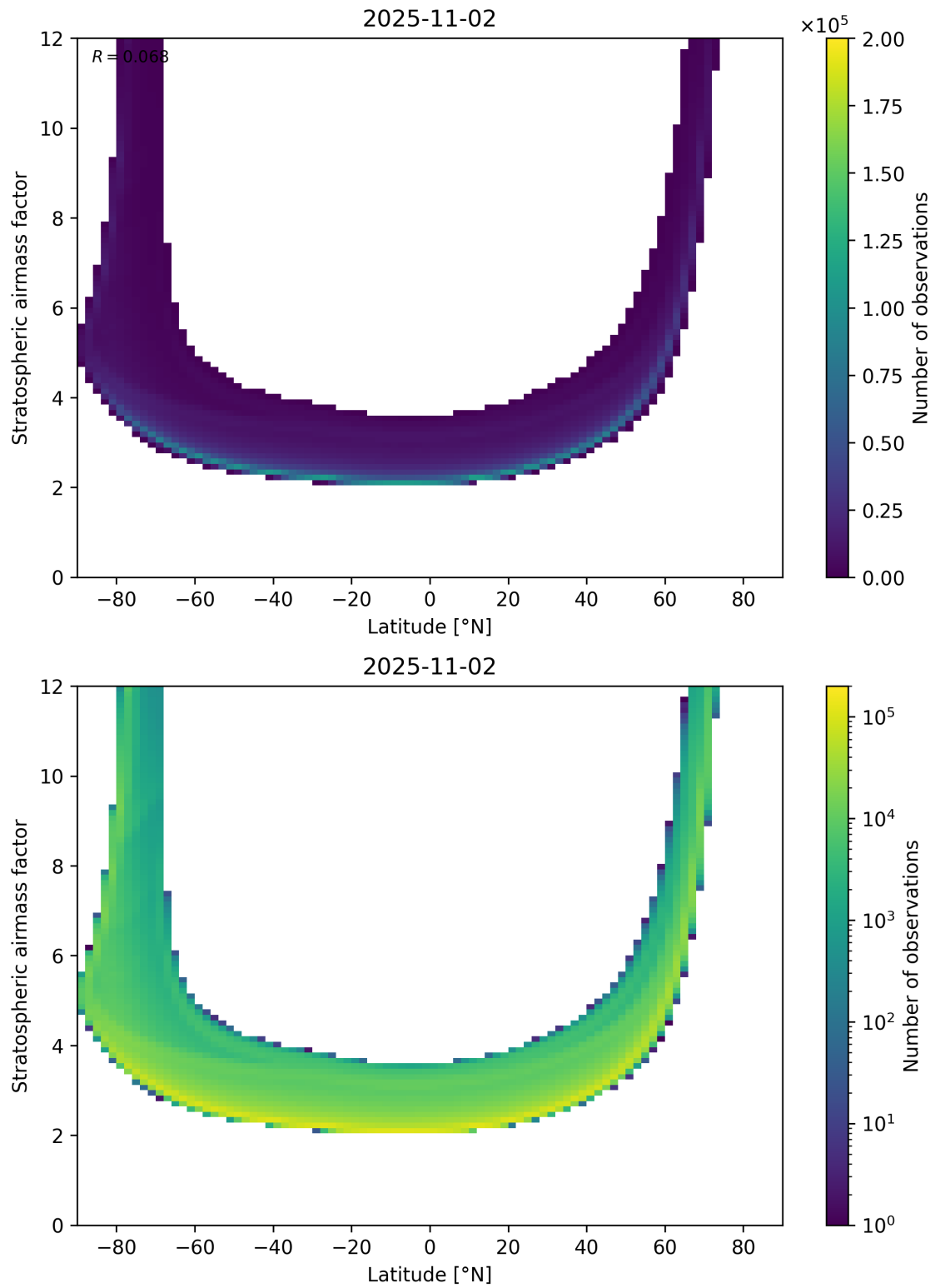
Figure 83: Scatter density plot of “Latitude” against “Stratospheric air mass factor” for 2025-11-02 to 2025-11-03.
