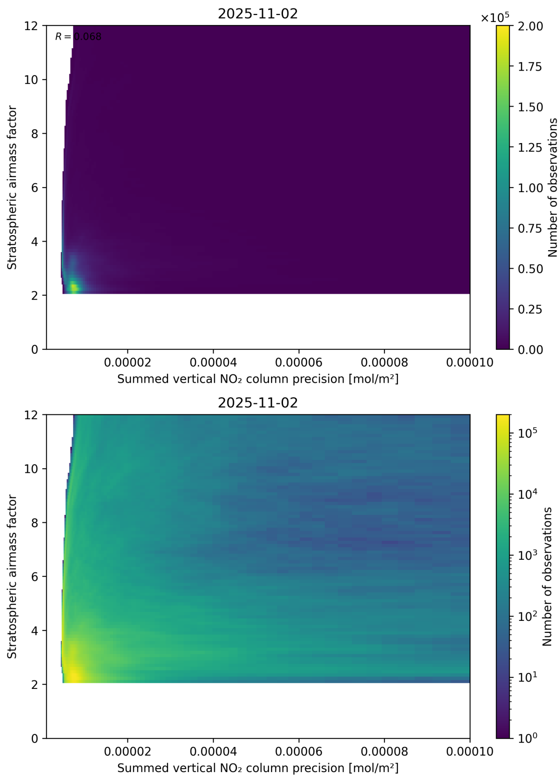
Figure 106: Scatter density plot of “Summed vertical NO 2 column precision” against “Stratospheric airmass factor” for 2025-11-02 to 2025-11-03.
