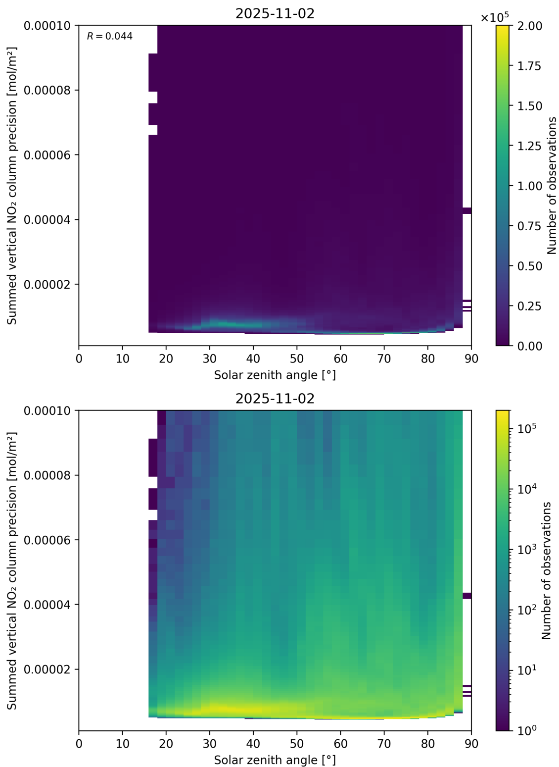
Figure 152: Scatter density plot of “Solar zenith angle” against “Summed vertical NO 2 column precision” for 2025-11-02 to 2025-11-03.
