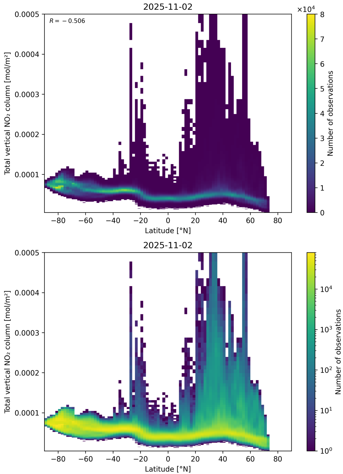
Figure 90: Scatter density plot of “Latitude” against “Total vertical NO 2 column” for 2025-11-02 to 2025-11-03.
