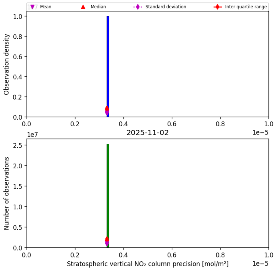
Figure 37: Histogram of “Stratospheric vertical NO 2 column precision” for 2025-11-02 to 2025-11-03
