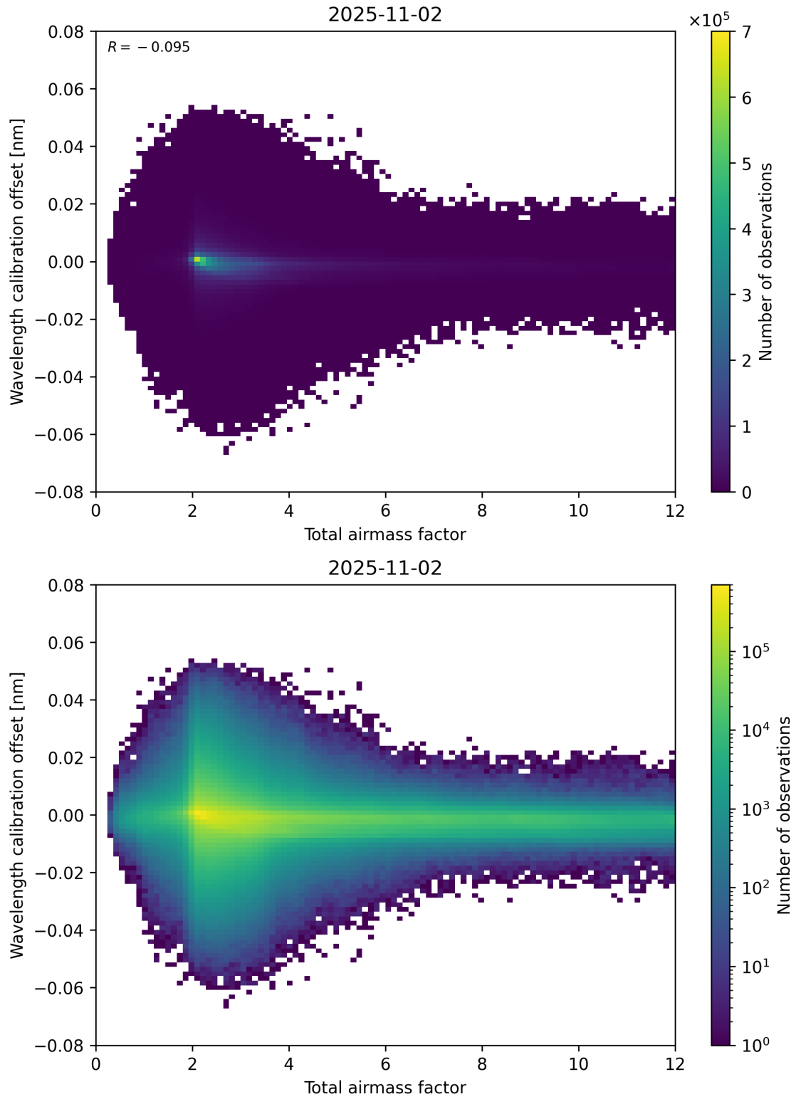
Figure 70: Scatter density plot of “Total airmass factor” against “Wavelength calibration offset” for 2025-11-02 to 2025-11-03.
