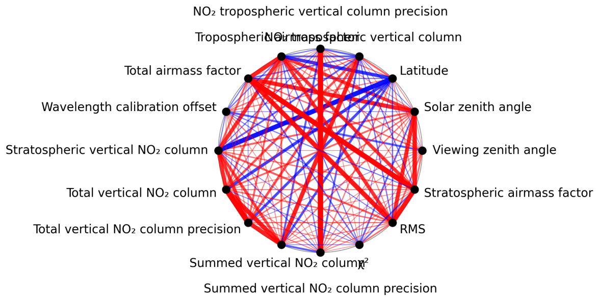
Figure 1: Map of correlation graph for 2025-11-02 to 2025-11-03.
