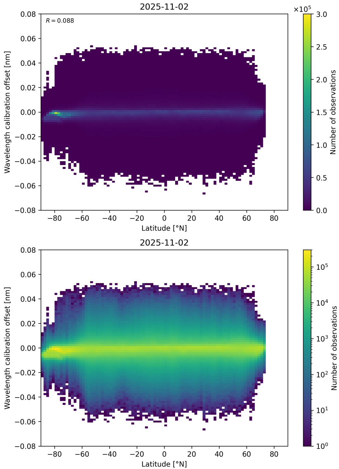
Figure 95: Scatter density plot of “Latitude” against “Wavelength calibration offset” for 2025-11-02 to 2025-11-03.
