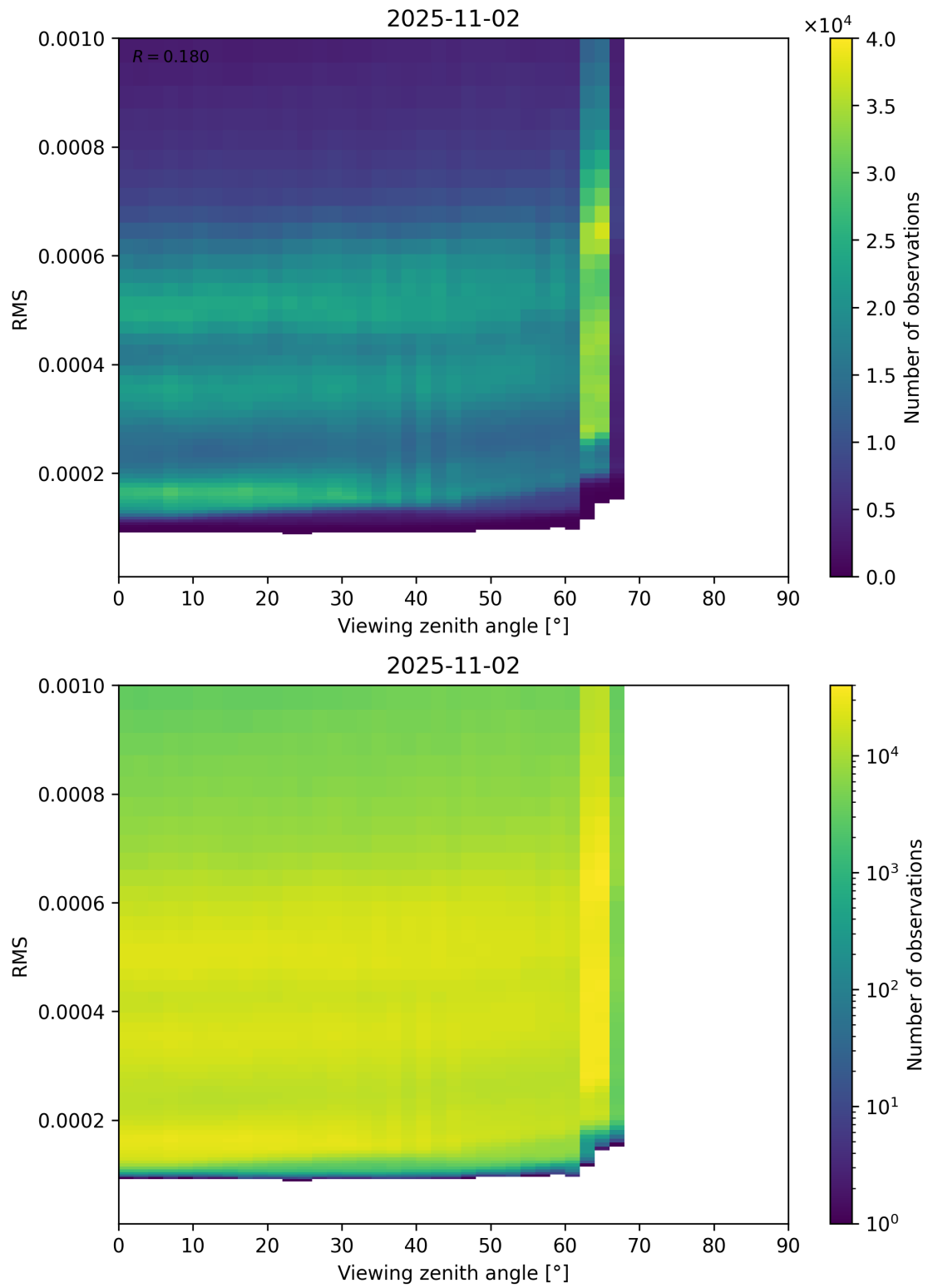
Figure 171: Scatter density plot of “Viewing zenith angle” against “RMS” for 2025-11-02 to 2025-11-03.
