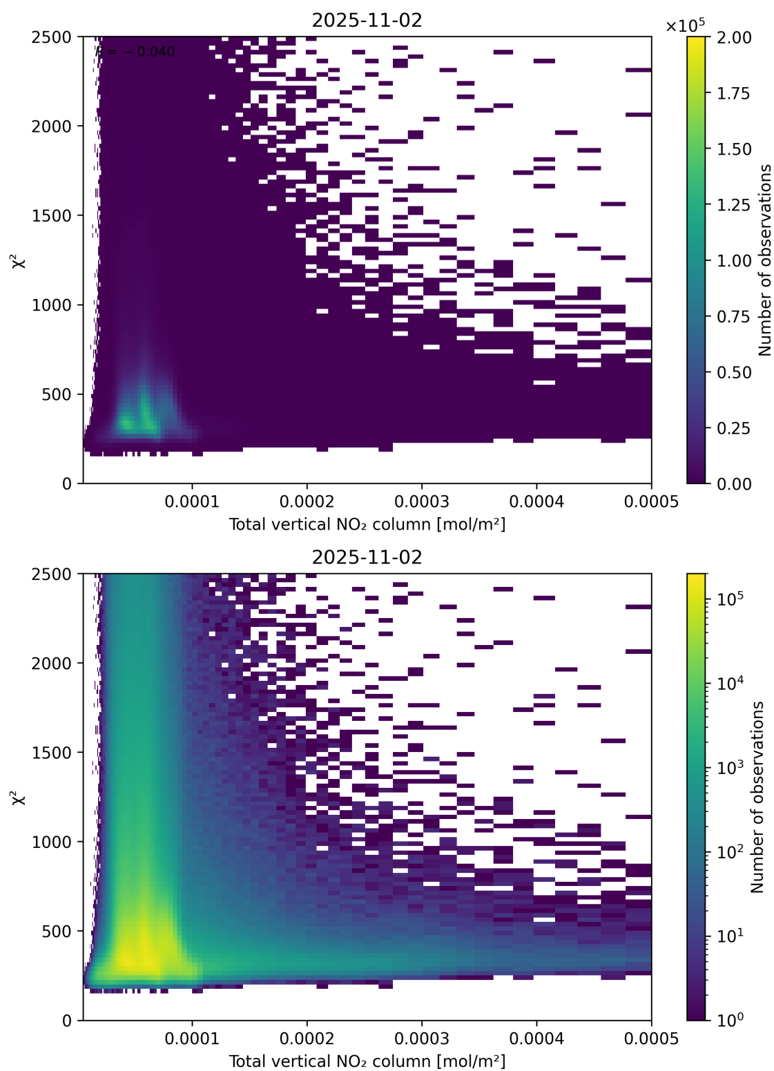
Figure 111: Scatter density plot of “Total vertical NO 2 column” against “ \chi^2 ” for 2025-11-02 to 2025-11-03.
