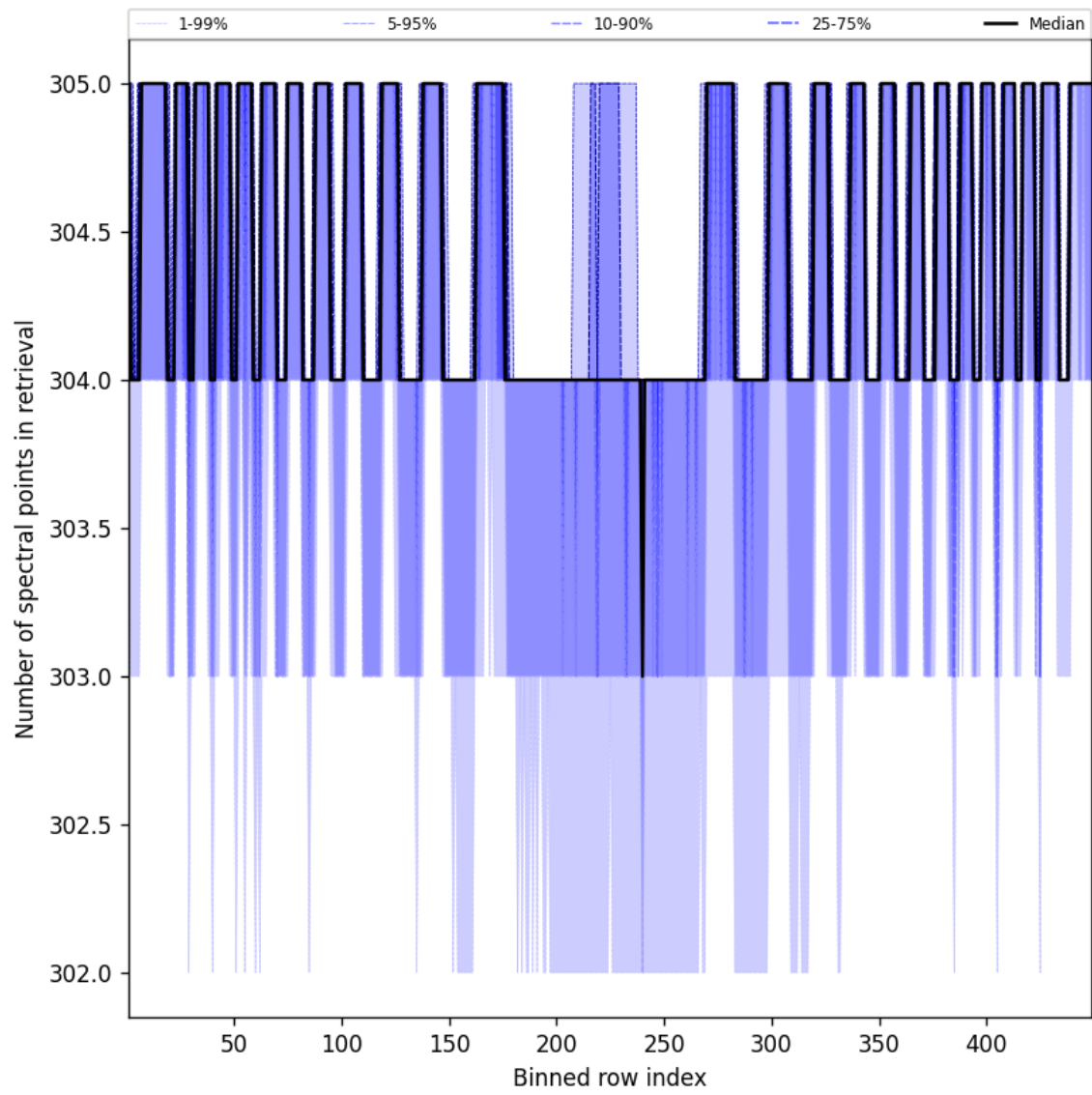
Figure 50: Along track statistics of “Number of spectral points in retrieval” for 2025-11-02 to 2025-11-03
