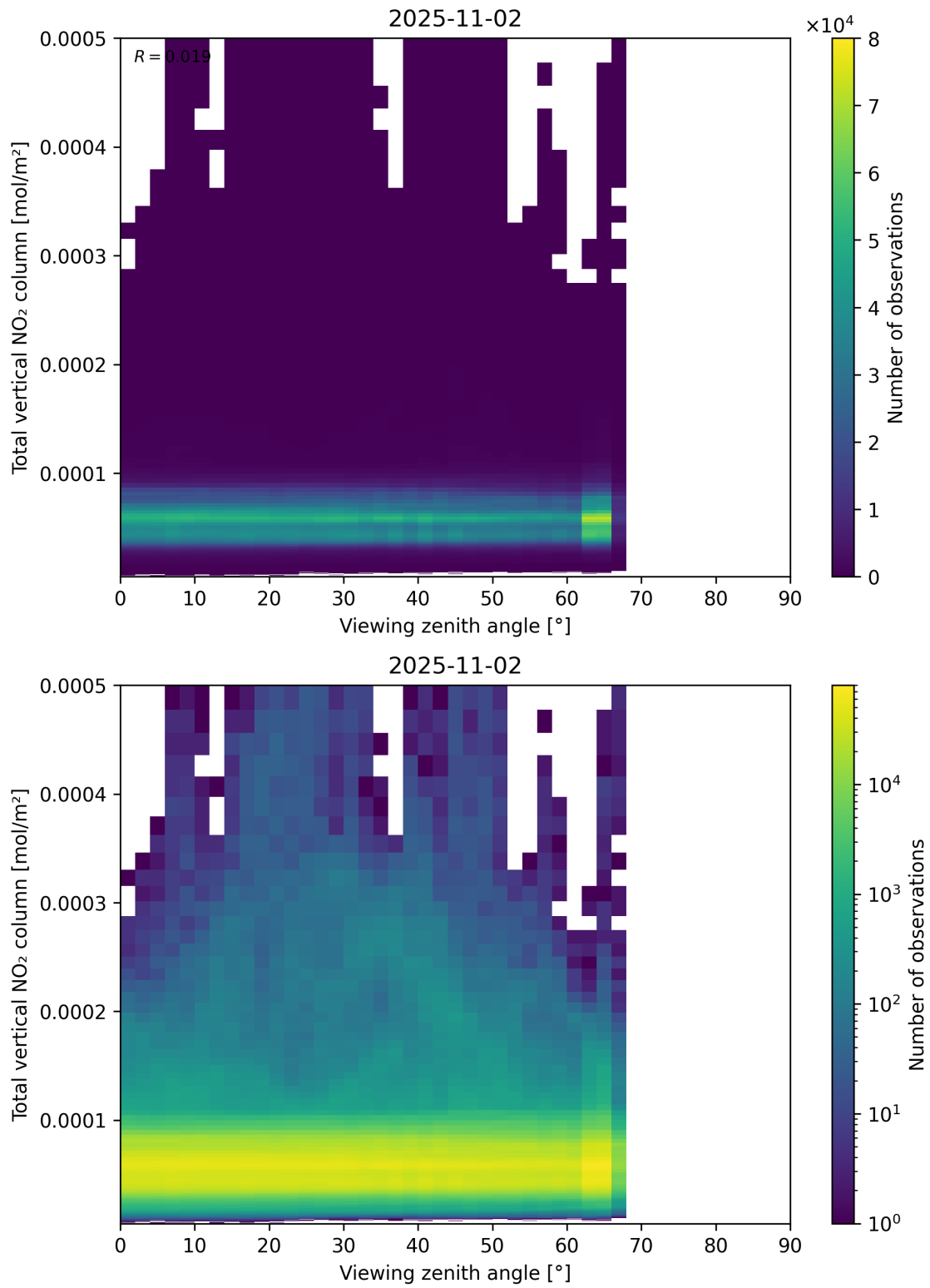
Figure 167: Scatter density plot of “Viewing zenith angle” against “Total vertical NO 2 column” for 2025-11-02 to 2025-11-03.
