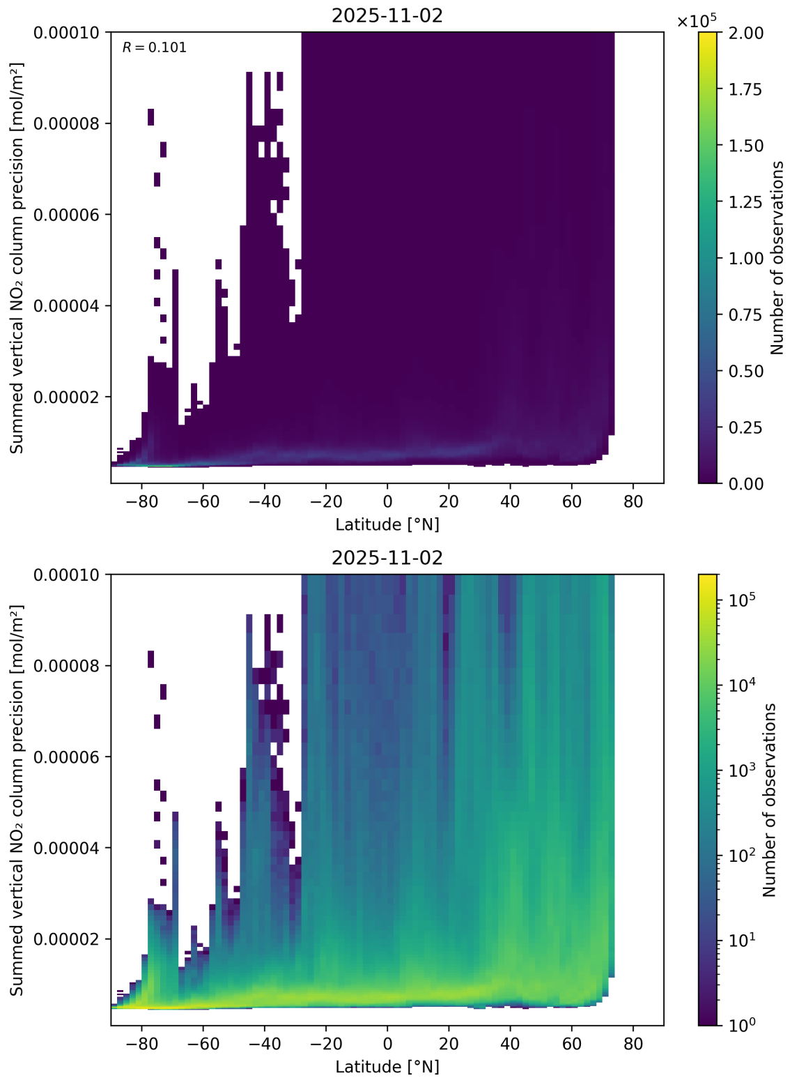
Figure 89: Scatter density plot of “Latitude” against “Summed vertical NO 2 column precision” for 2025-11-02 to 2025-11-03.
