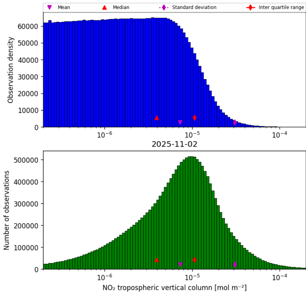
Figure 29: Histogram of “NO 2 tropospheric vertical column” for 2025-11-02 to 2025-11-03
