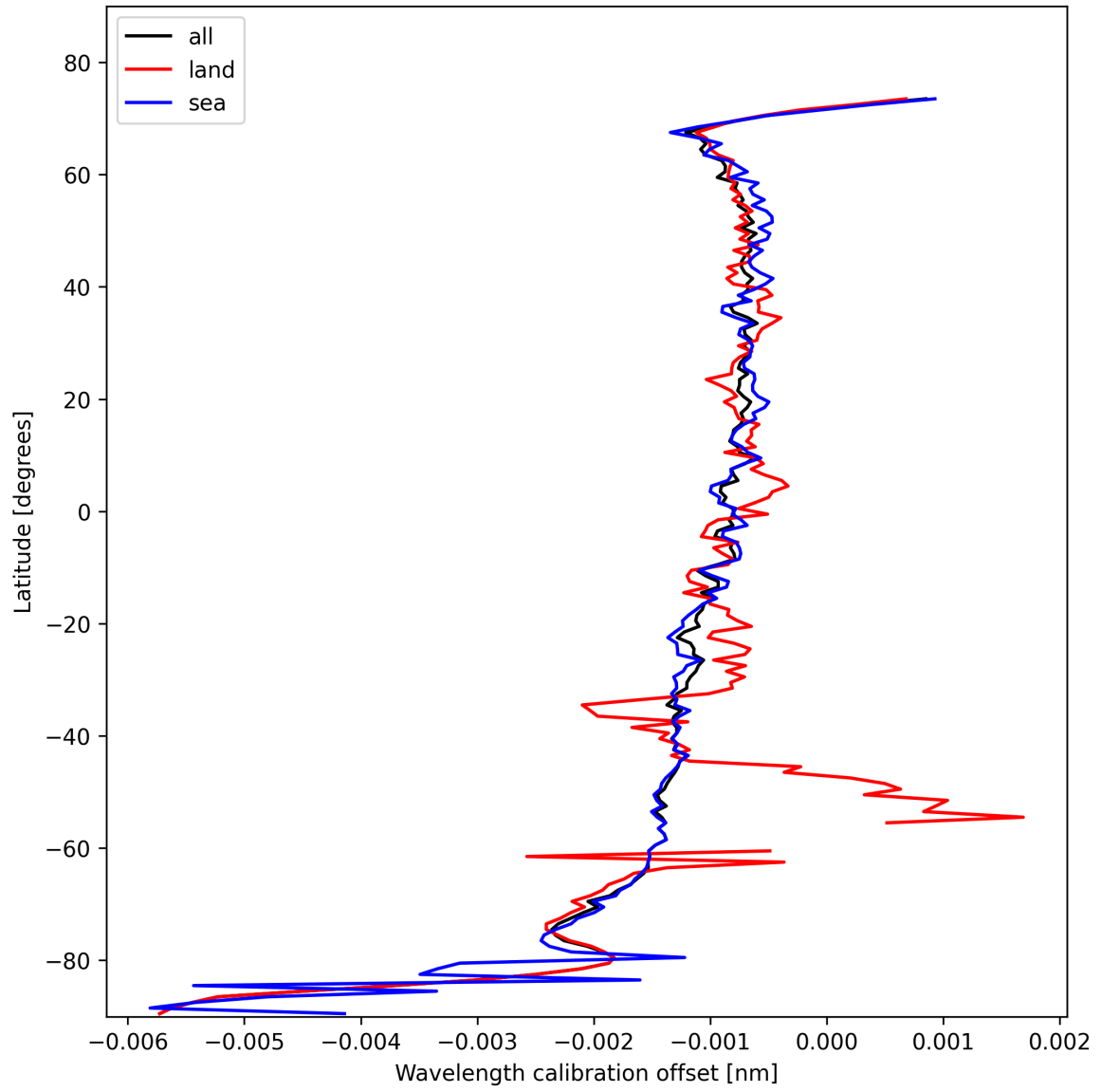
Figure 18: Zonal average of “Wavelength calibration offset” for 2025-11-02 to 2025-11-03.
