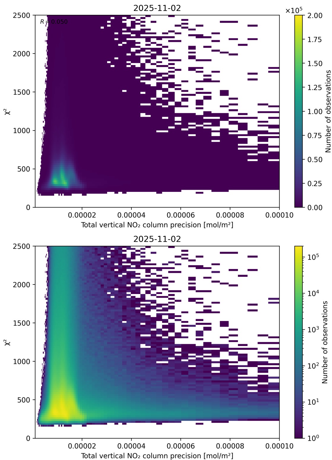
Figure 116: Scatter density plot of “Total vertical NO 2 column precision” against “ \chi^2 ” for 2025-11-02 to 2025-11-03.
