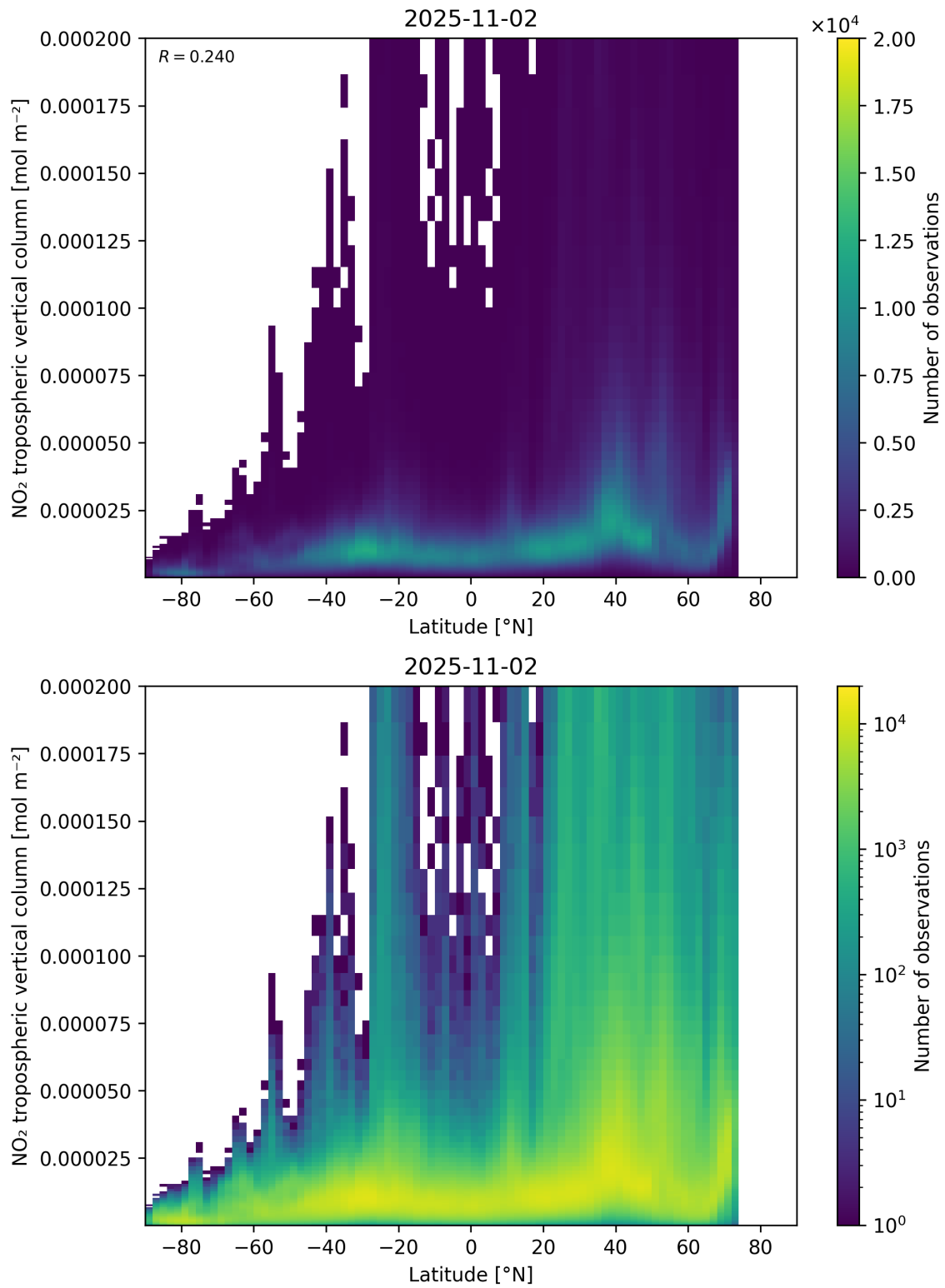
Figure 92: Scatter density plot of “Latitude” against “NO 2 tropospheric vertical column” for 2025-11-02 to 2025-11-03.
