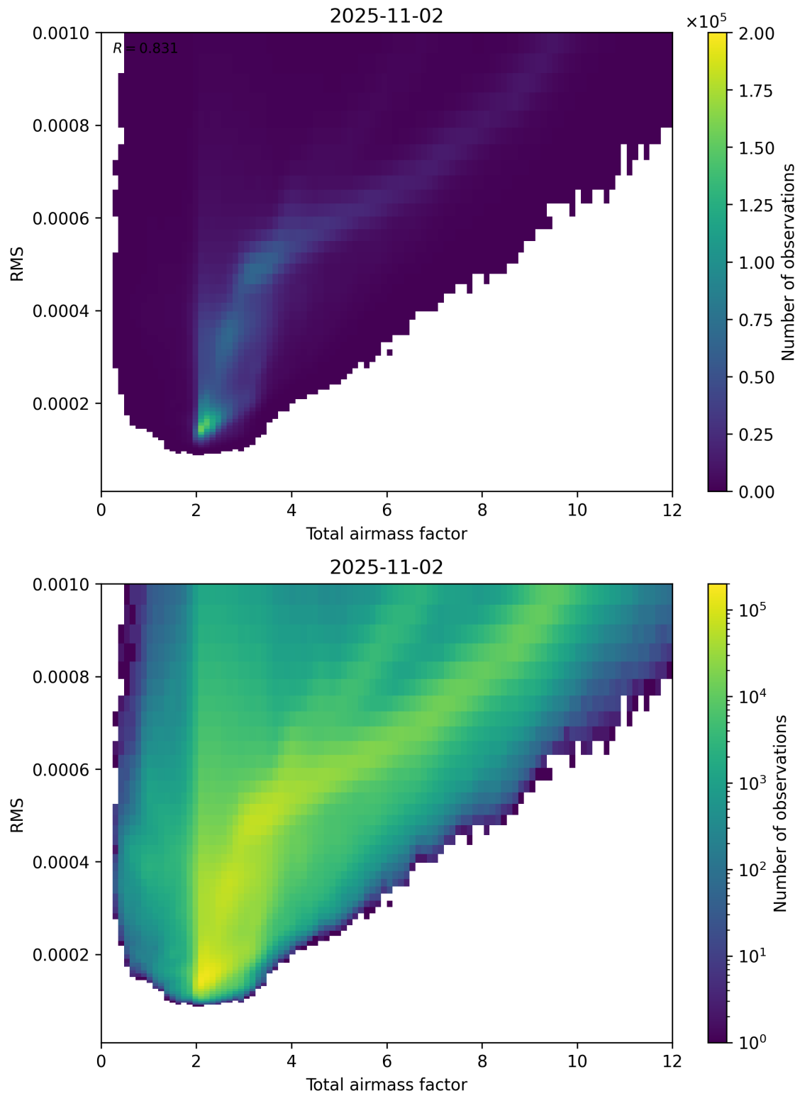
Figure 69: Scatter density plot of “Total airmass factor” against “RMS” for 2025-11-02 to 2025-11-03.
