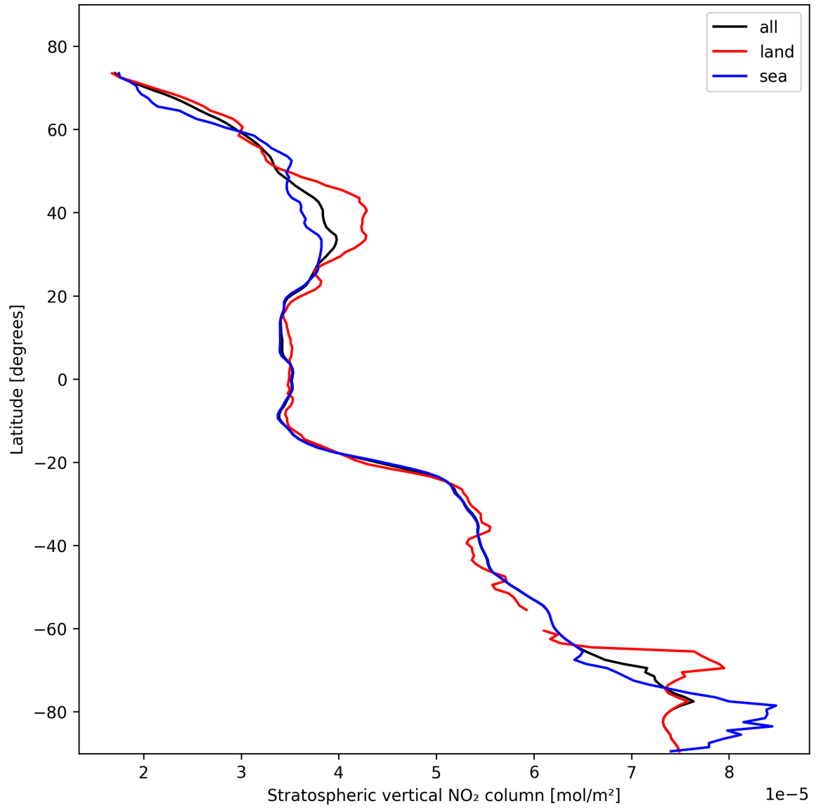
Figure 19: Zonal average of “Stratospheric vertical NO 2 column” for 2025-11-02 to 2025-11-03.
