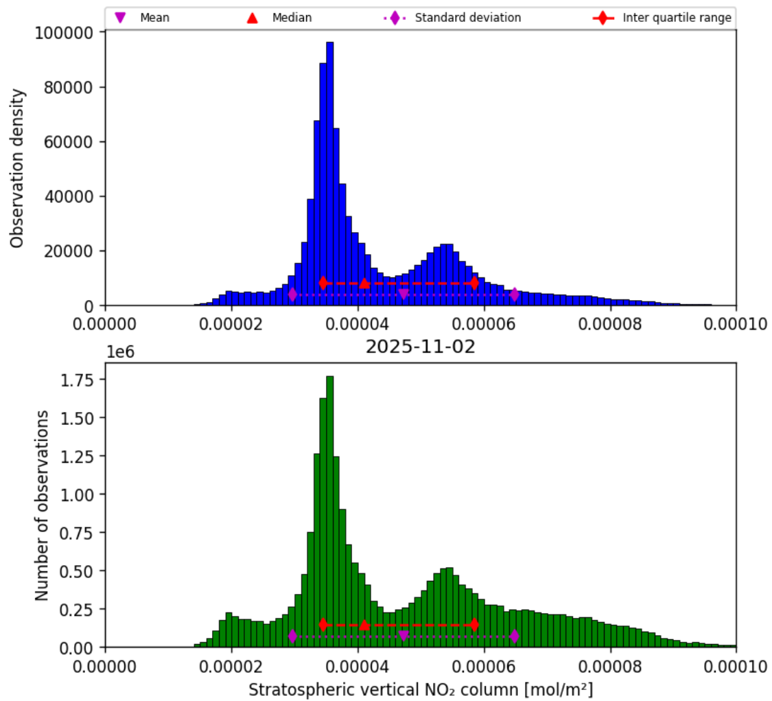
Figure 36: Histogram of “Stratospheric vertical NO 2 column” for 2025-11-02 to 2025-11-03
