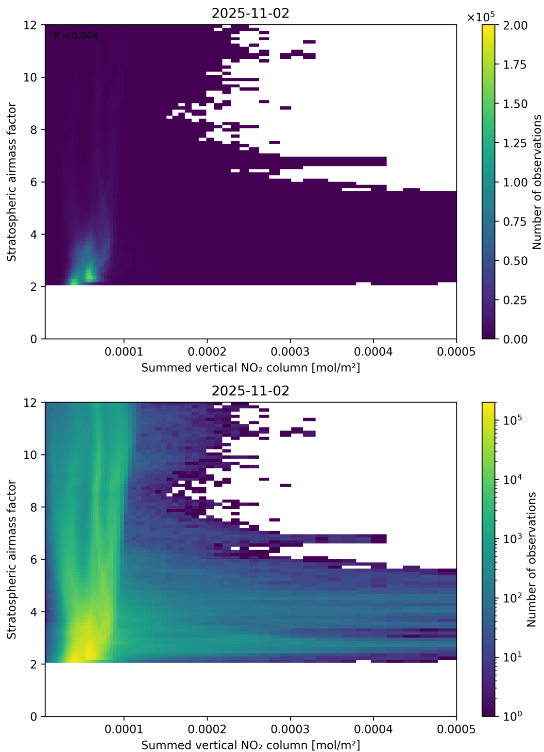
Figure 103: Scatter density plot of “Summed vertical NO 2 column” against “Stratospheric airmass factor” for 2025-11-02 to 2025-11-03.
