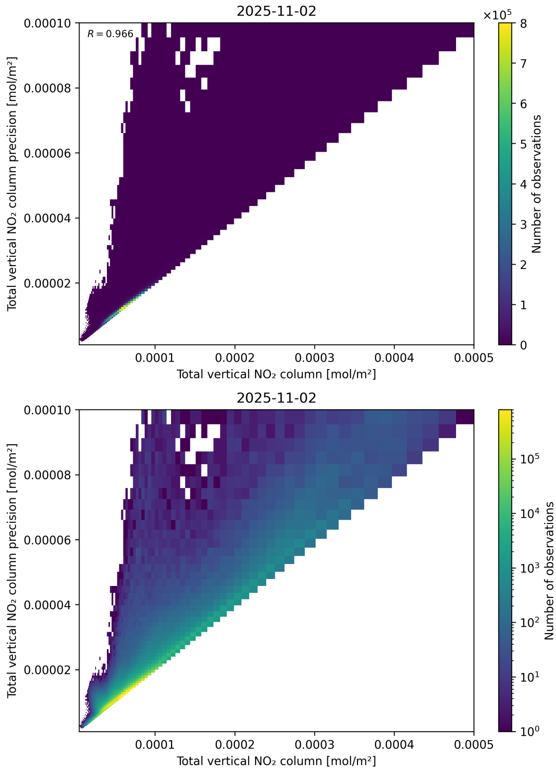
Figure 114: Scatter density plot of “Total vertical NO 2 column” against “Total vertical NO 2 column precision” for 2025-11-02 to 2025-11-03.
