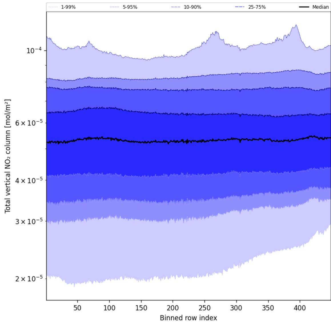
Figure 55: Along track statistics of “Total vertical NO 2 column” for 2025-11-02 to 2025-11-03
