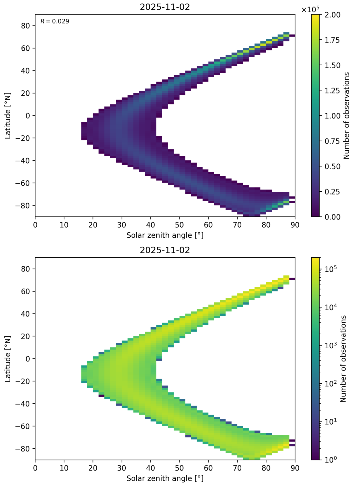
Figure 149: Scatter density plot of “Solar zenith angle” against “Latitude” for 2025-11-02 to 2025-11-03.
