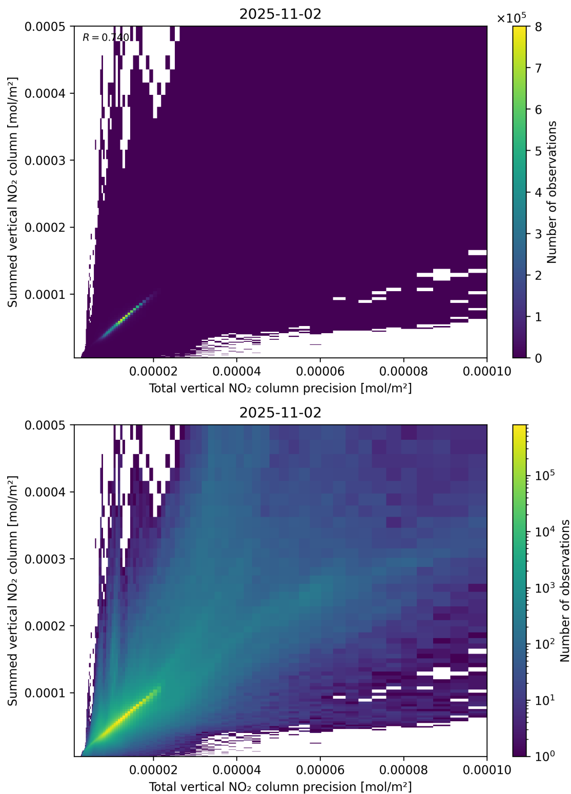
Figure 117: Scatter density plot of “Total vertical NO 2 column precision” against “Summed vertical NO 2 column” for 2025-11-02 to 2025-11-03.
