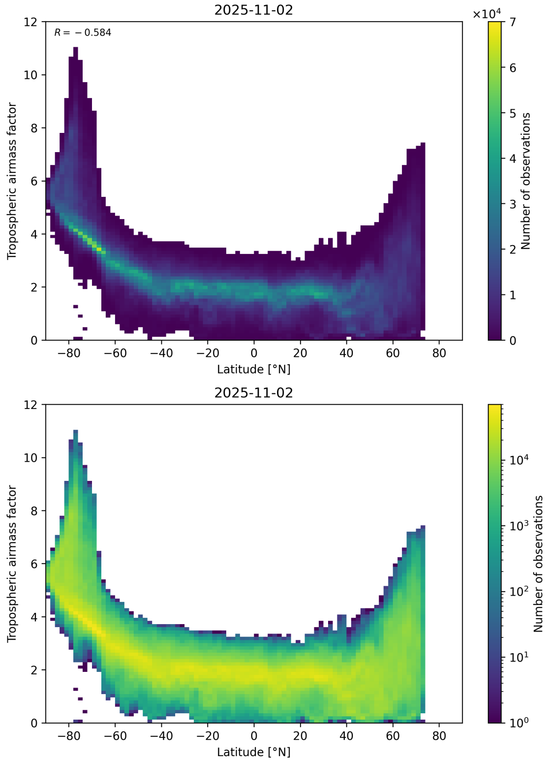
Figure 85: Scatter density plot of “Latitude” against “Tropospheric airmass factor” for 2025-11-02 to 2025-11-03.
