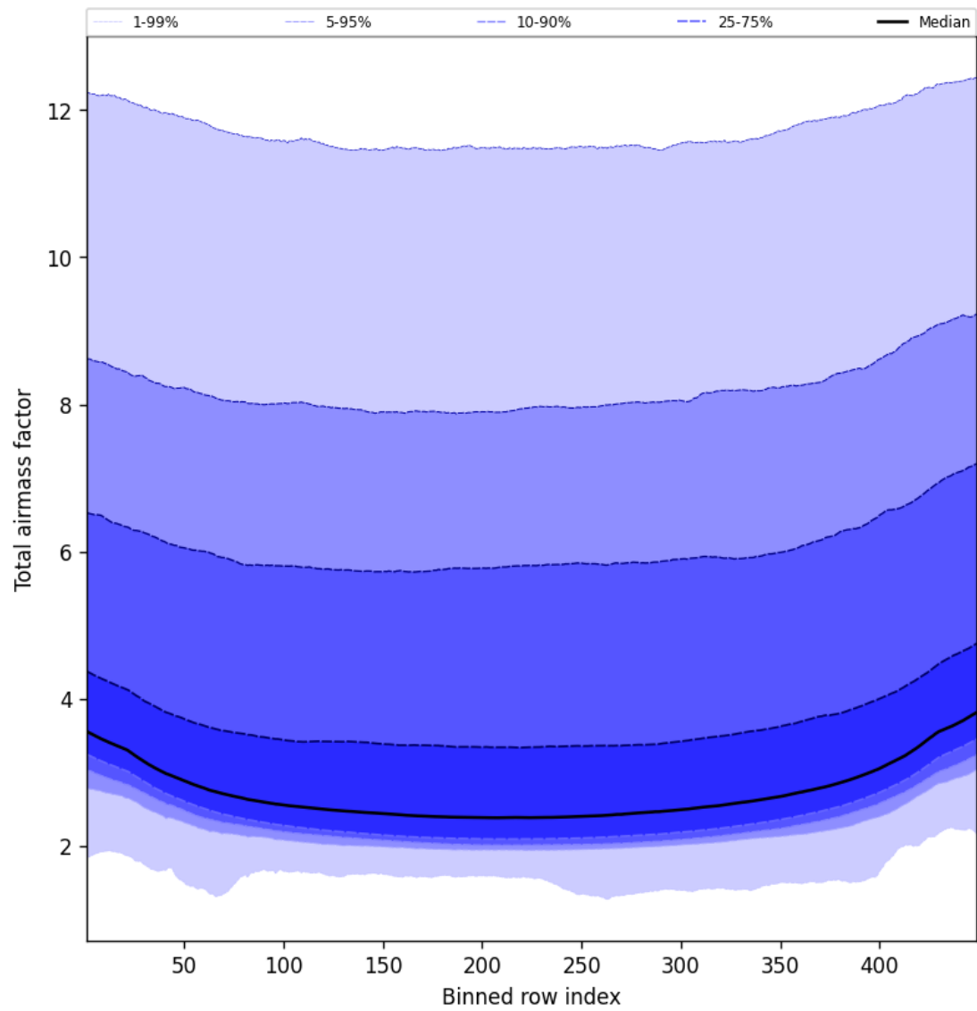
Figure 49: Along track statistics of “Total airmass factor” for 2025-11-02 to 2025-11-03
