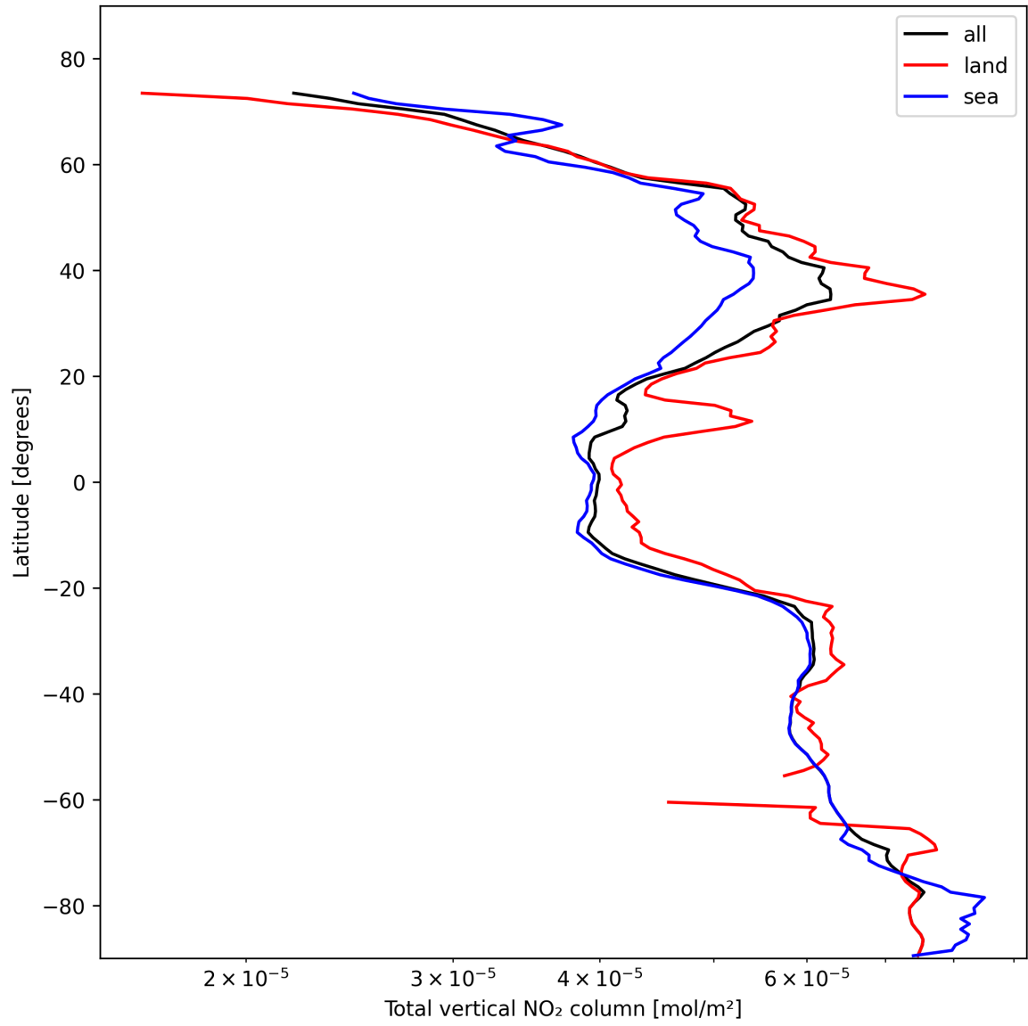
Figure 21: Zonal average of “Total vertical NO 2 column” for 2025-11-02 to 2025-11-03.
