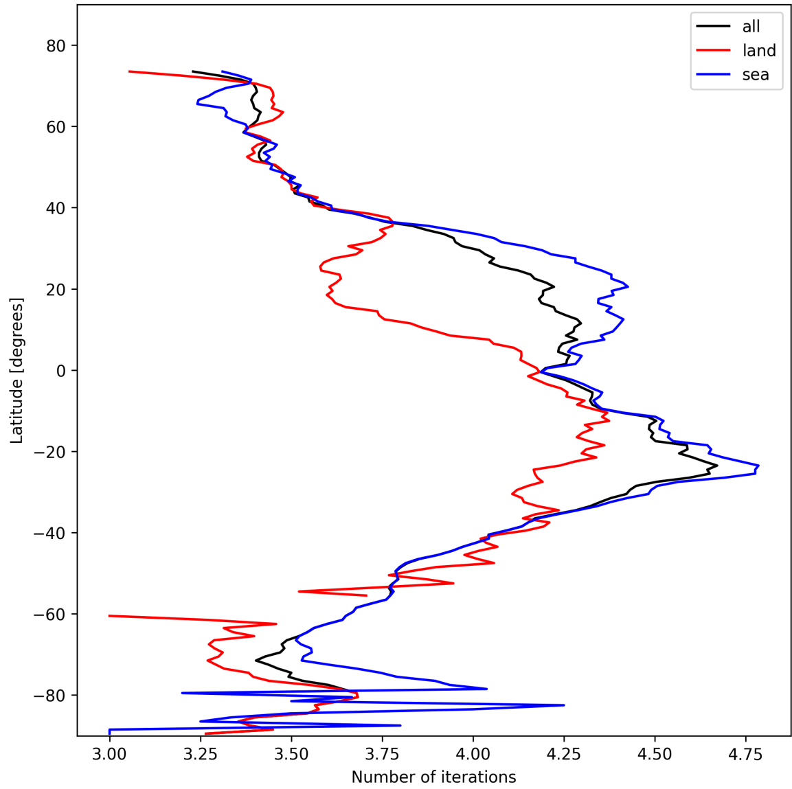
Figure 17: Zonal average of “Number of iterations” for 2025-11-02 to 2025-11-03.
