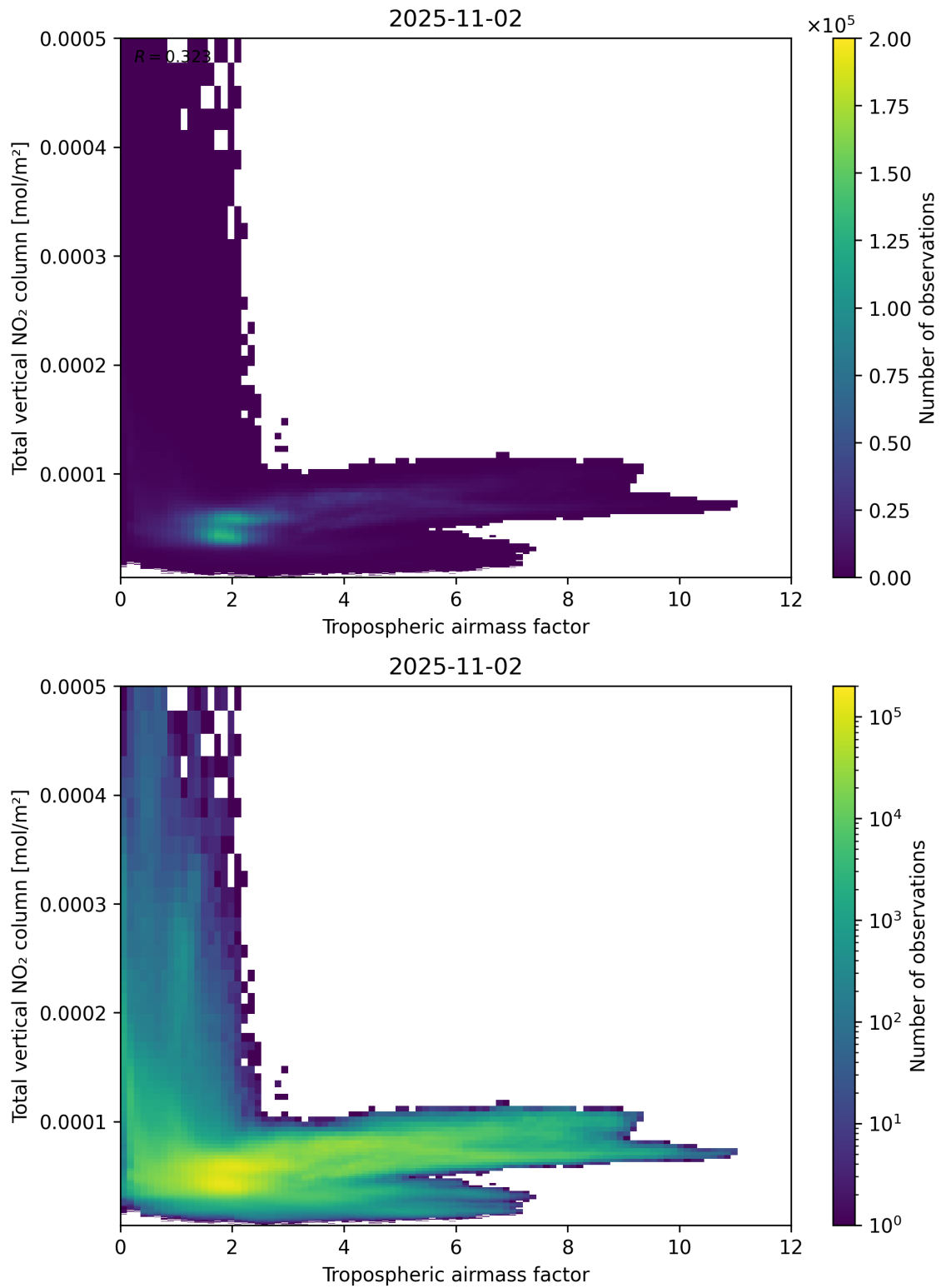
Figure 77: Scatter density plot of “Tropospheric airmass factor” against “Total vertical NO 2 column” for 2025-11-02 to 2025-11-03.
