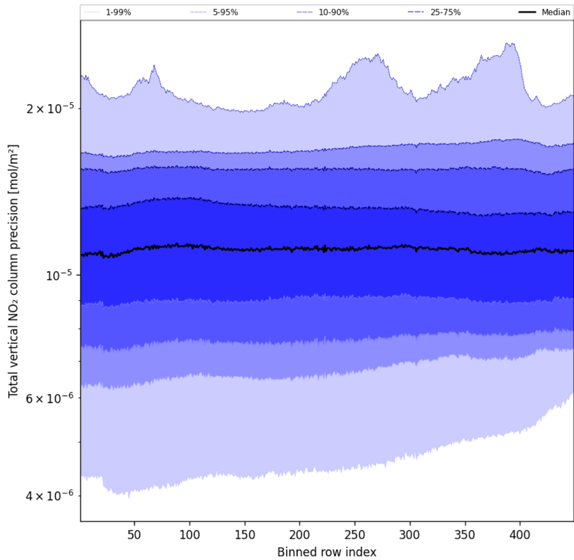
Figure 56: Along track statistics of "Total vertical NO 2 column precision" for 2025-11-02 to 2025-11-03
