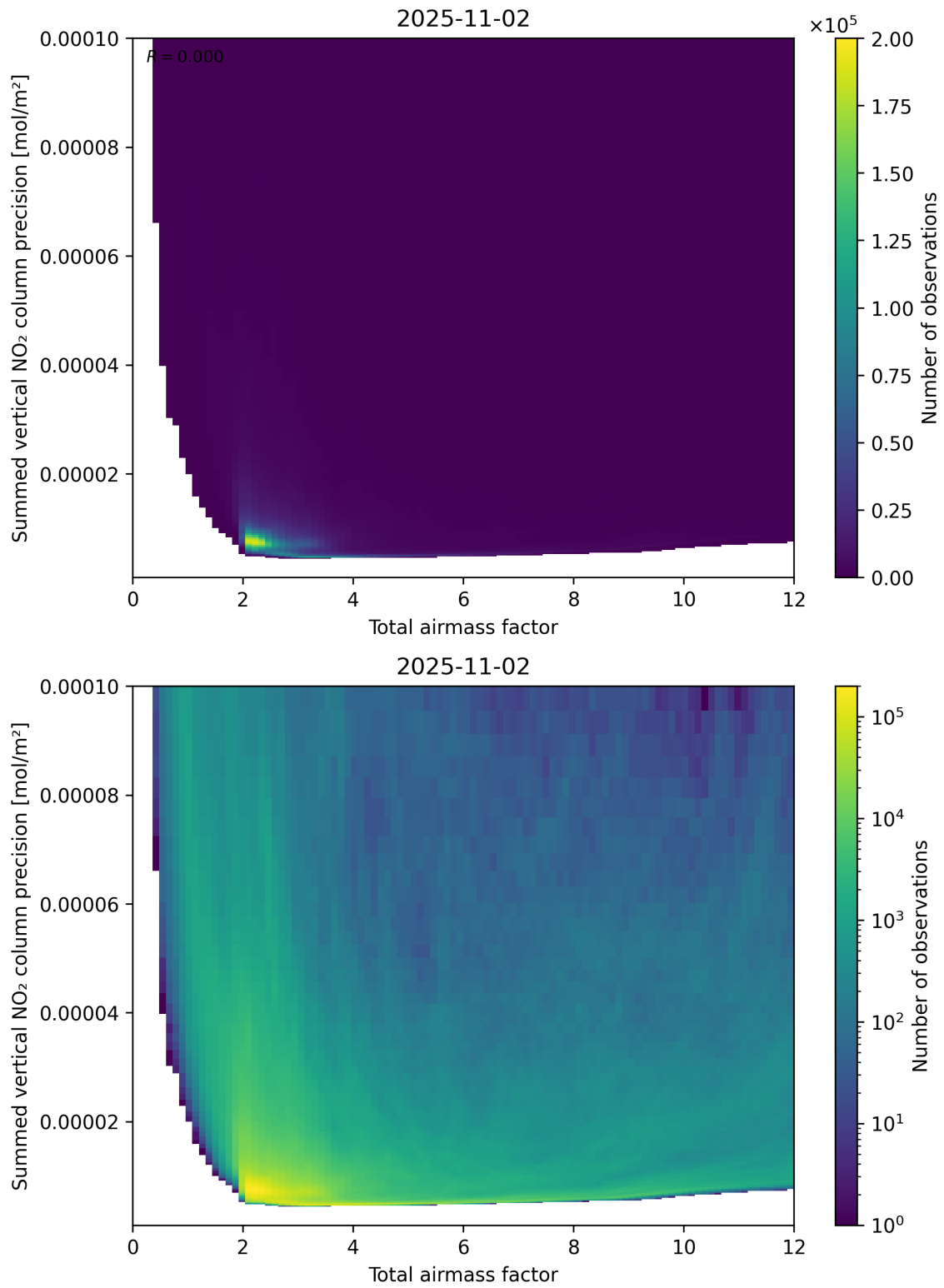
Figure 66: Scatter density plot of “Total airmass factor” against “Summed vertical NO 2 column precision” for 2025-11-02 to 2025-11-03.
