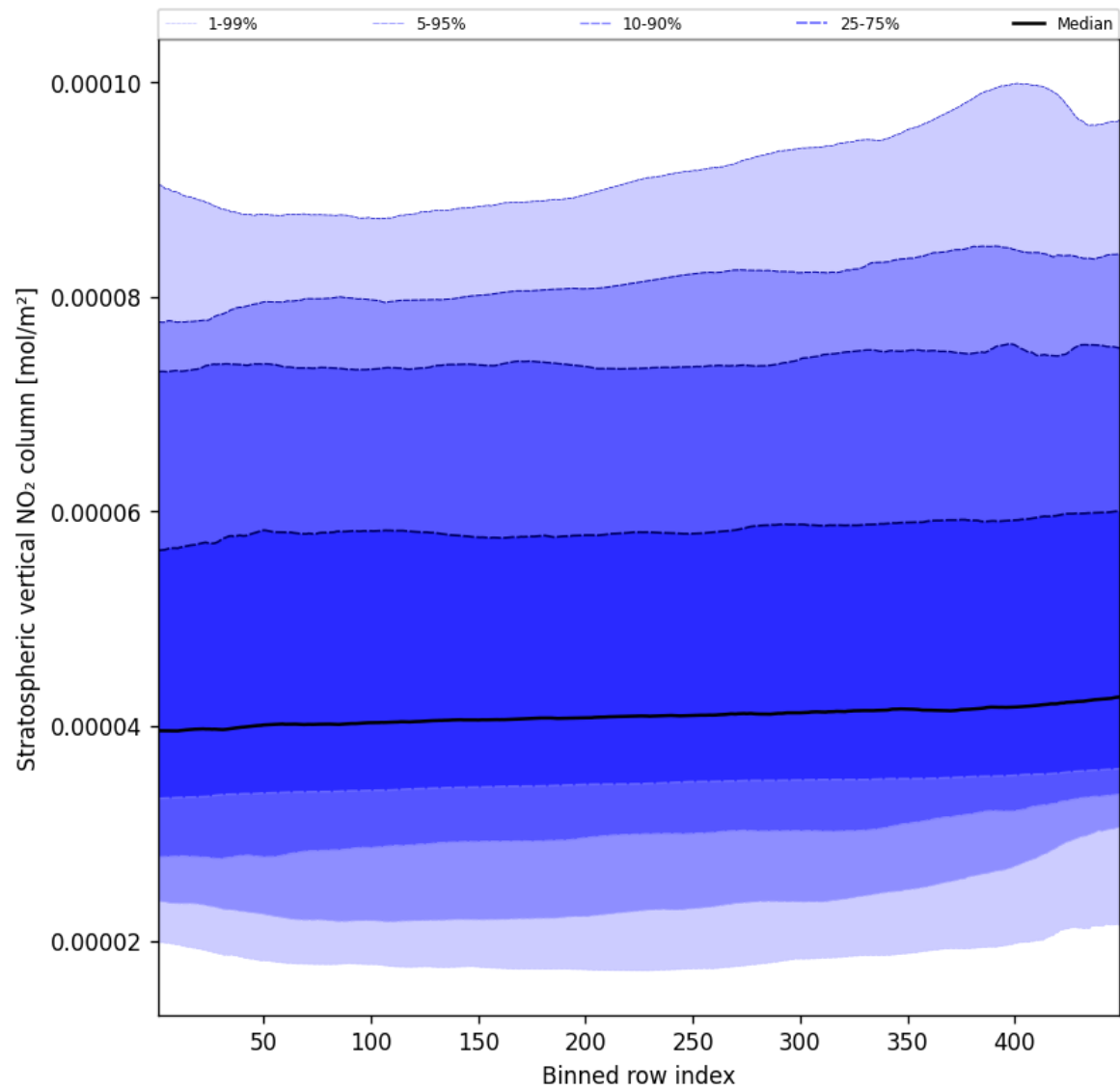
Figure 53: Along track statistics of “Stratospheric vertical NO 2 column” for 2025-11-02 to 2025-11-03
