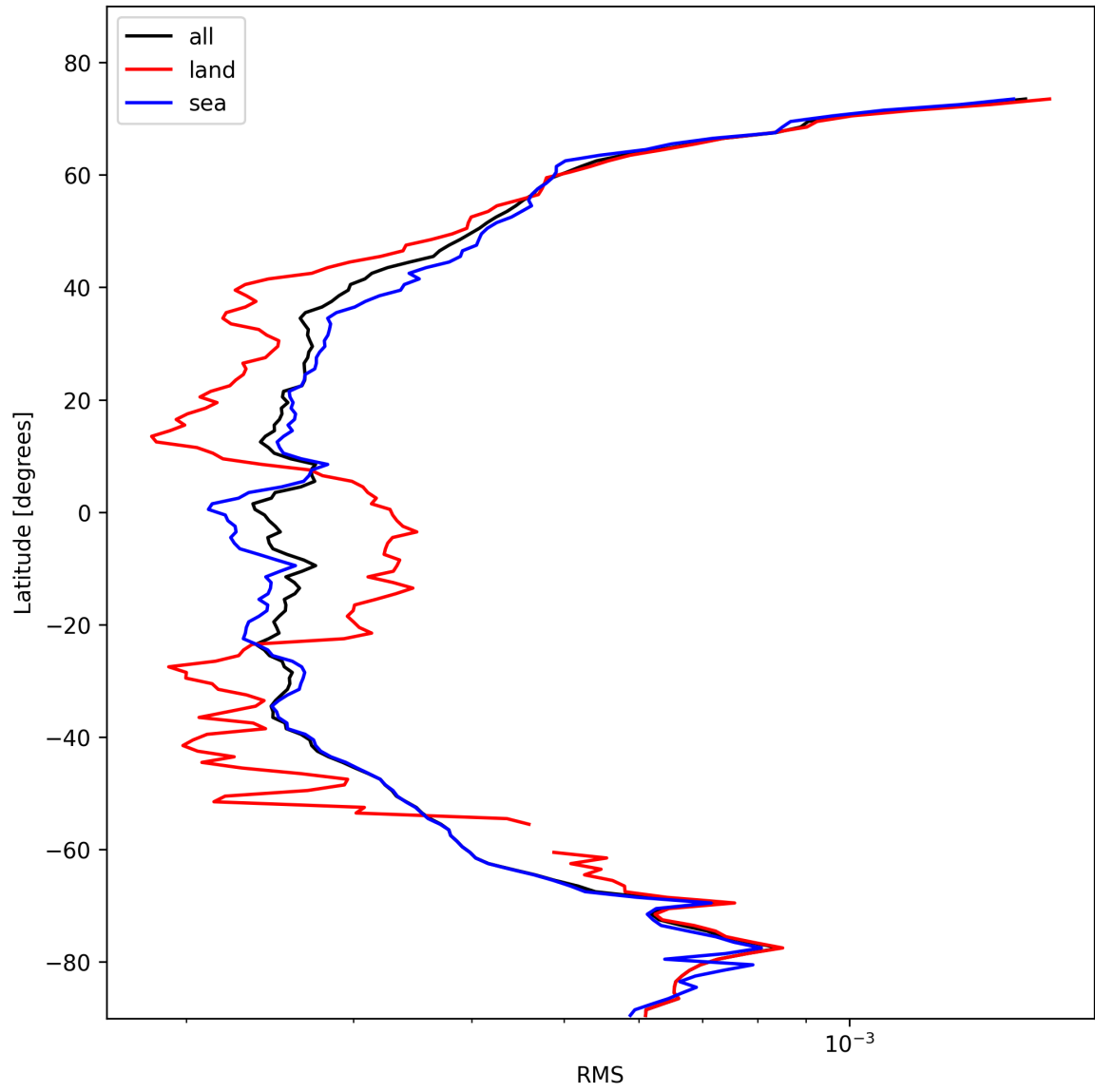
Figure 26: Zonal average of “RMS” for 2025-11-02 to 2025-11-03.
