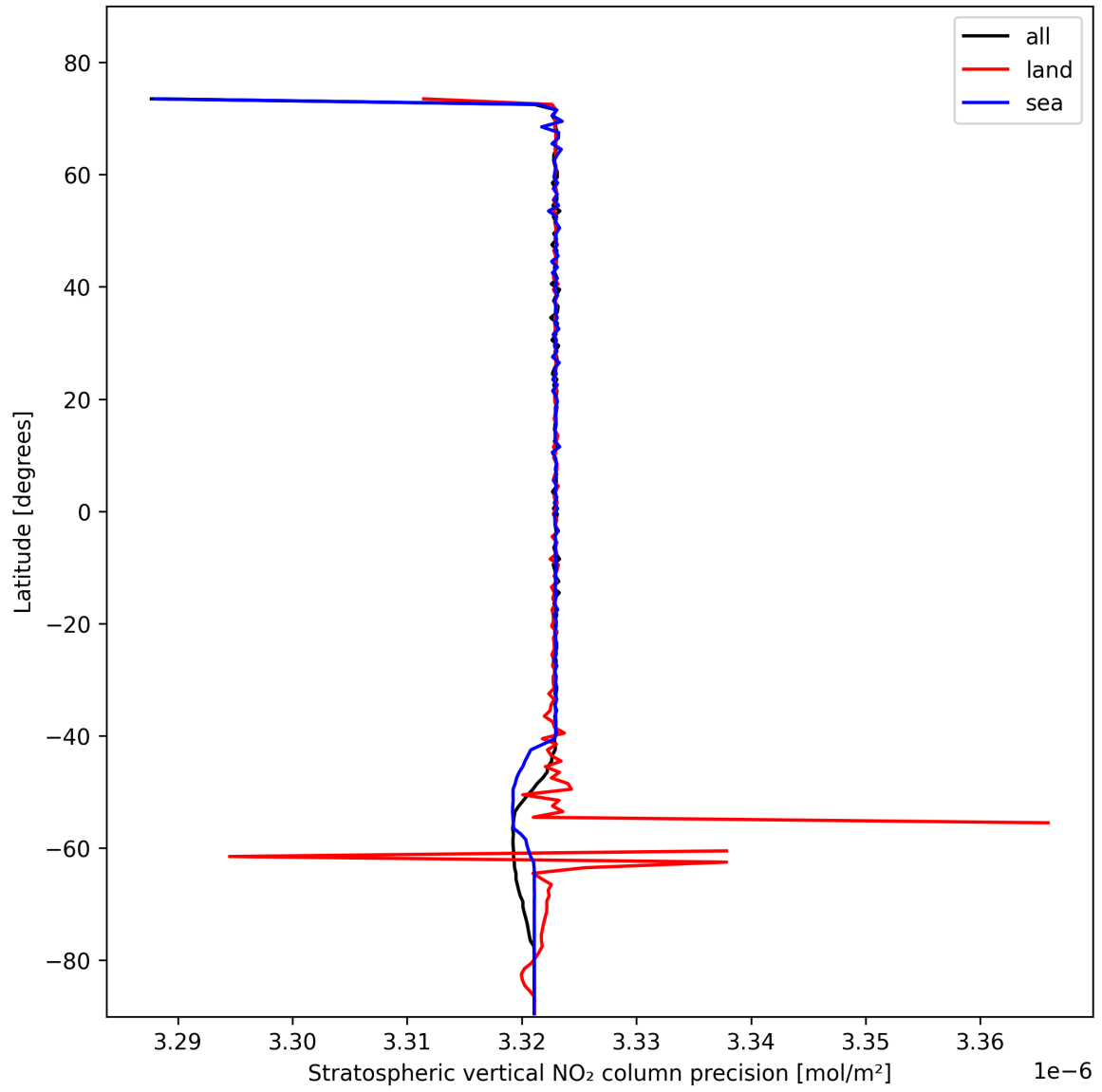
Figure 20: Zonal average of “Stratospheric vertical NO 2 column precision” for 2025-11-02 to 2025-11-03.
