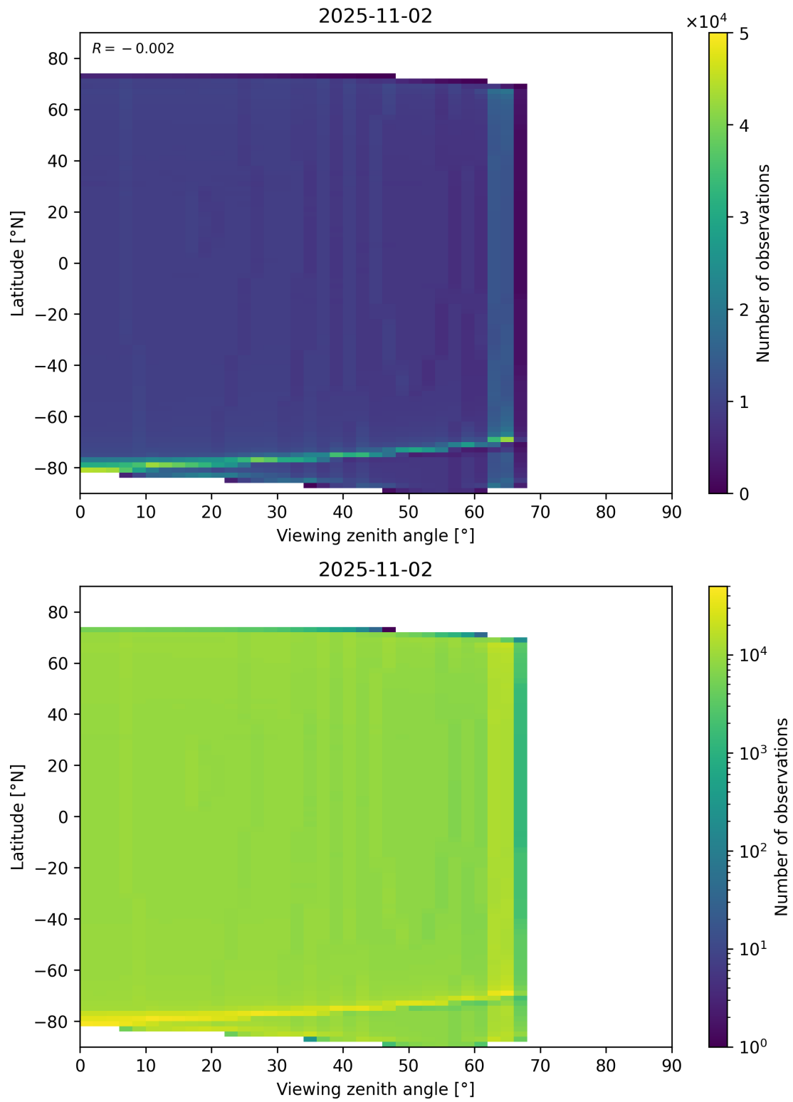
Figure 163: Scatter density plot of “Viewing zenith angle” against “Latitude” for 2025-11-02 to 2025-11-03.
