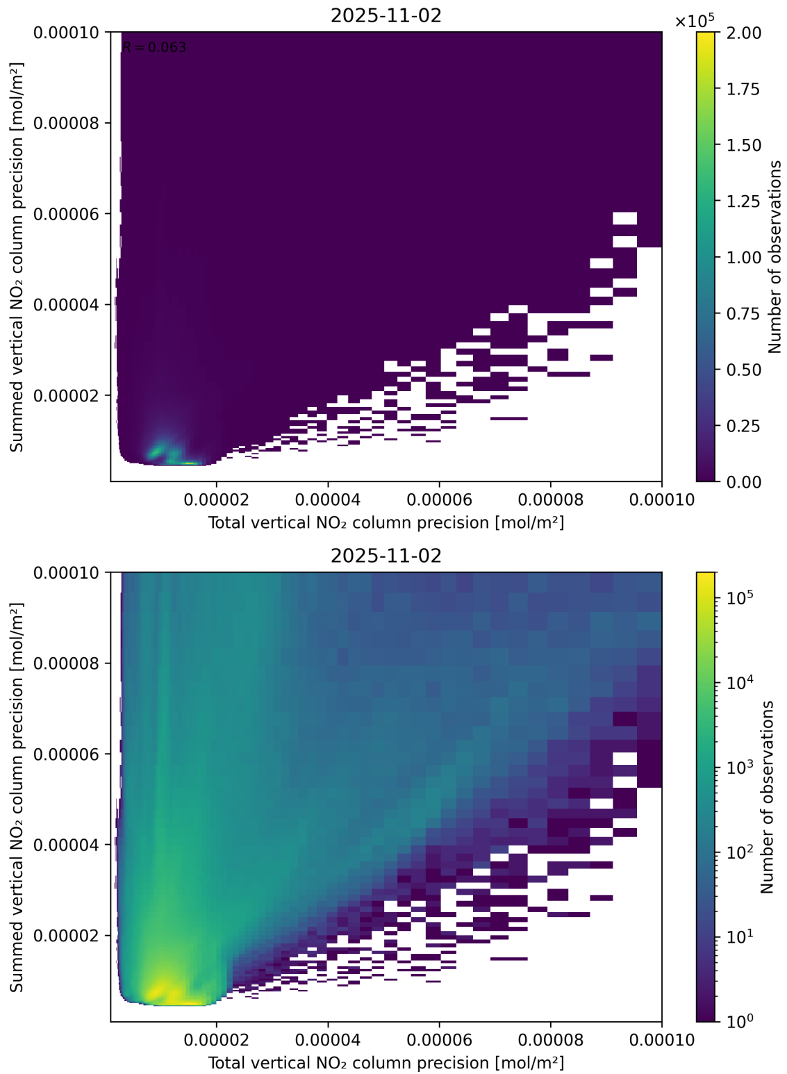
Figure 118: Scatter density plot of “Total vertical NO 2 column precision” against “Summed vertical NO 2 column precision” for 2025-11-02 to 2025-11-03.
