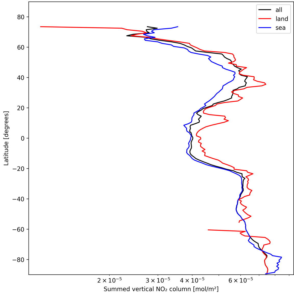
Figure 23: Zonal average of “Summed vertical NO 2 column” for 2025-11-02 to 2025-11-03.
