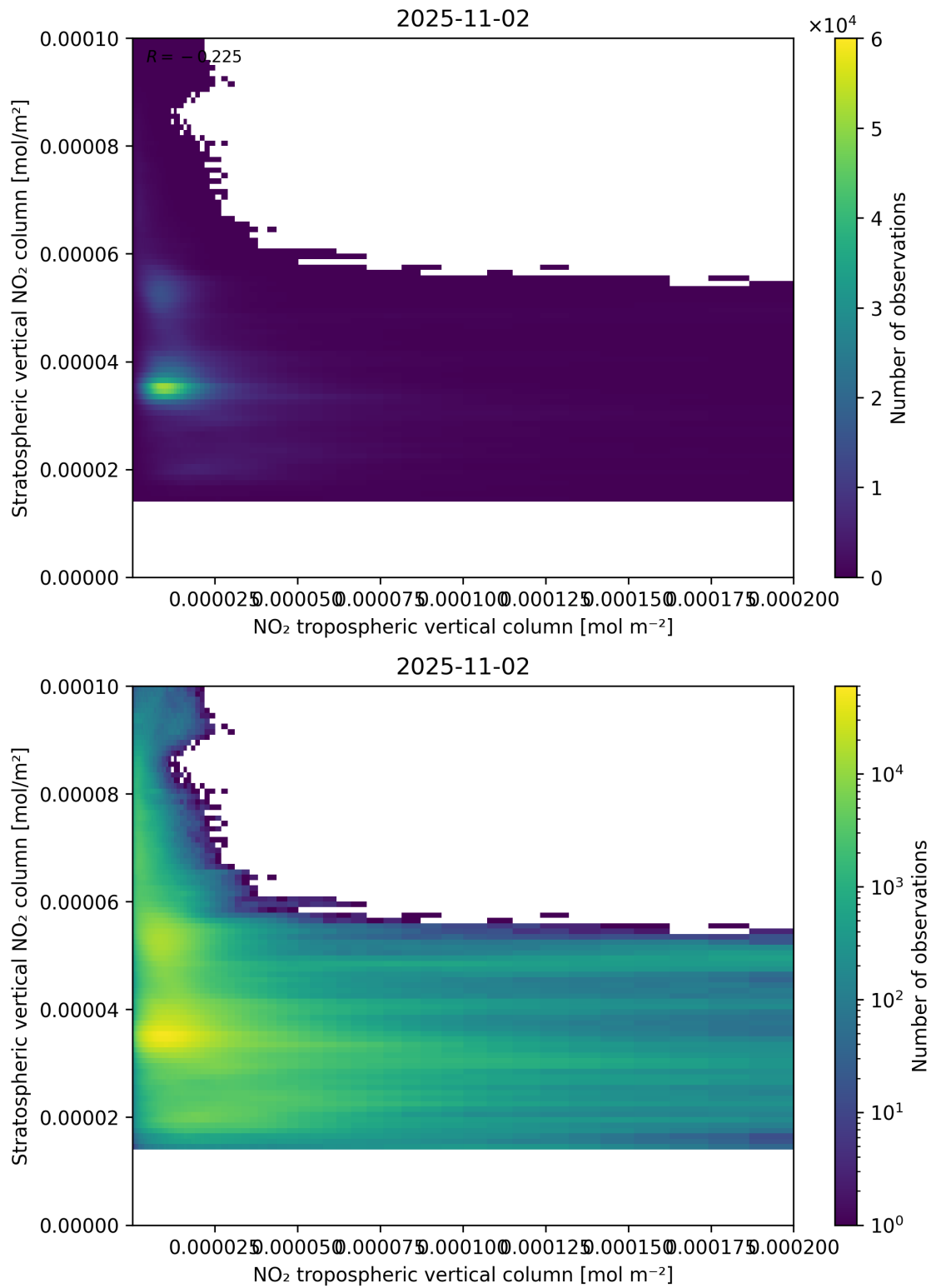
Figure 125: Scatter density plot of “NO 2 tropospheric vertical column” against “Stratospheric vertical NO 2 column” for 2025-11-02 to 2025-11-03.
