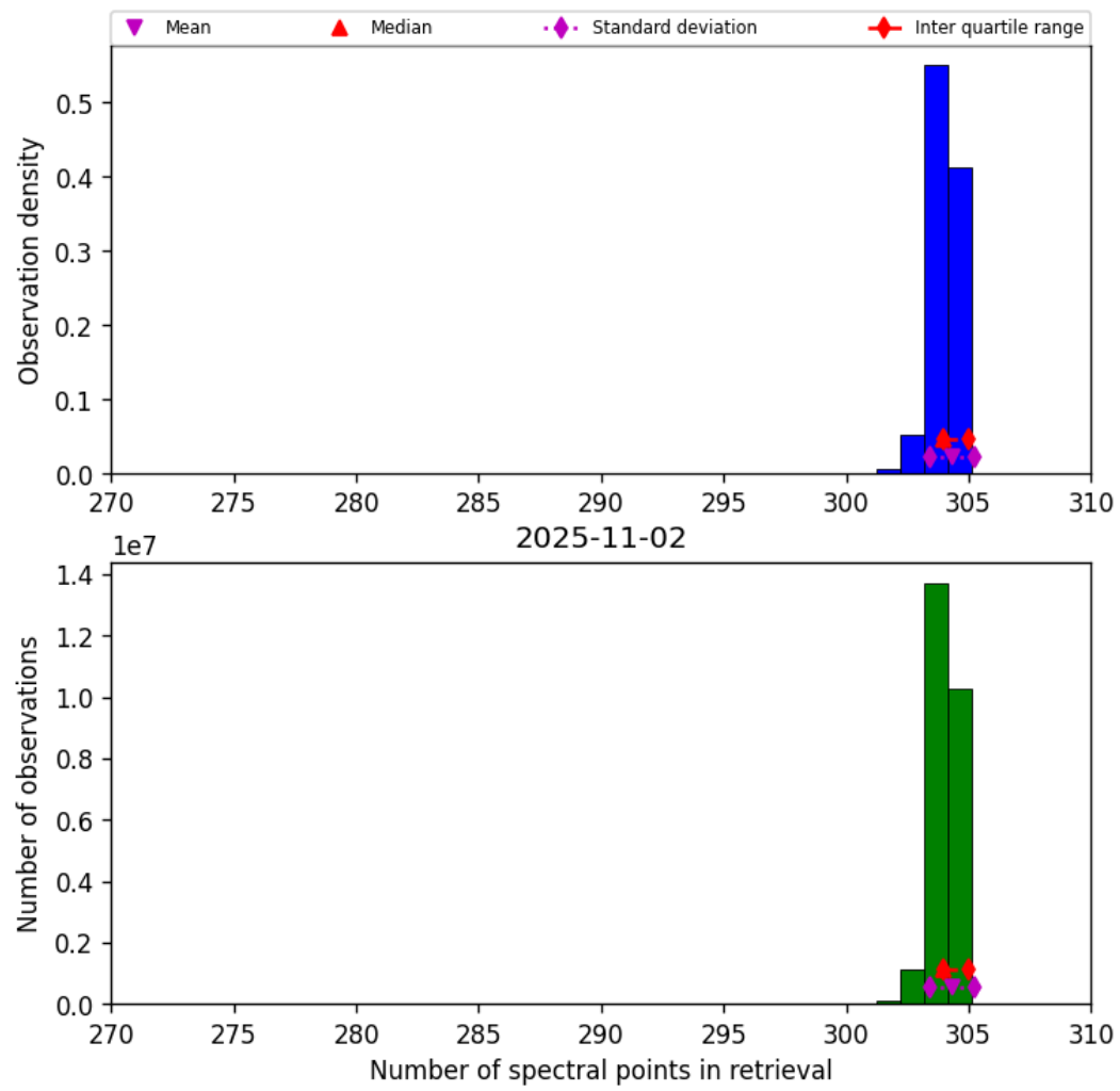
Figure 33: Histogram of “Number of spectral points in retrieval” for 2025-11-02 to 2025-11-03
