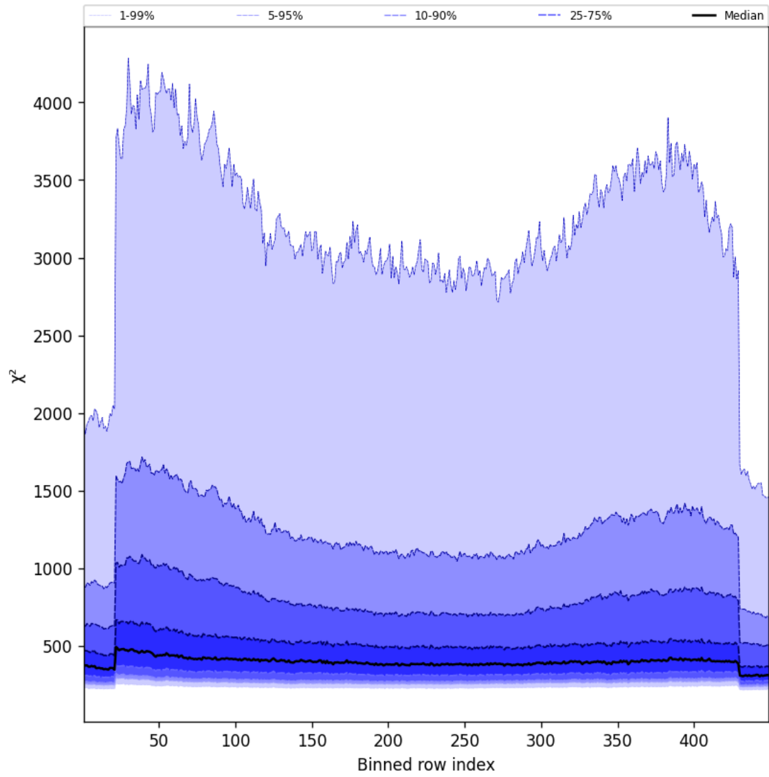
Figure 59: Along track statistics of “ \chi^2 ” for 2025-11-02 to 2025-11-03
