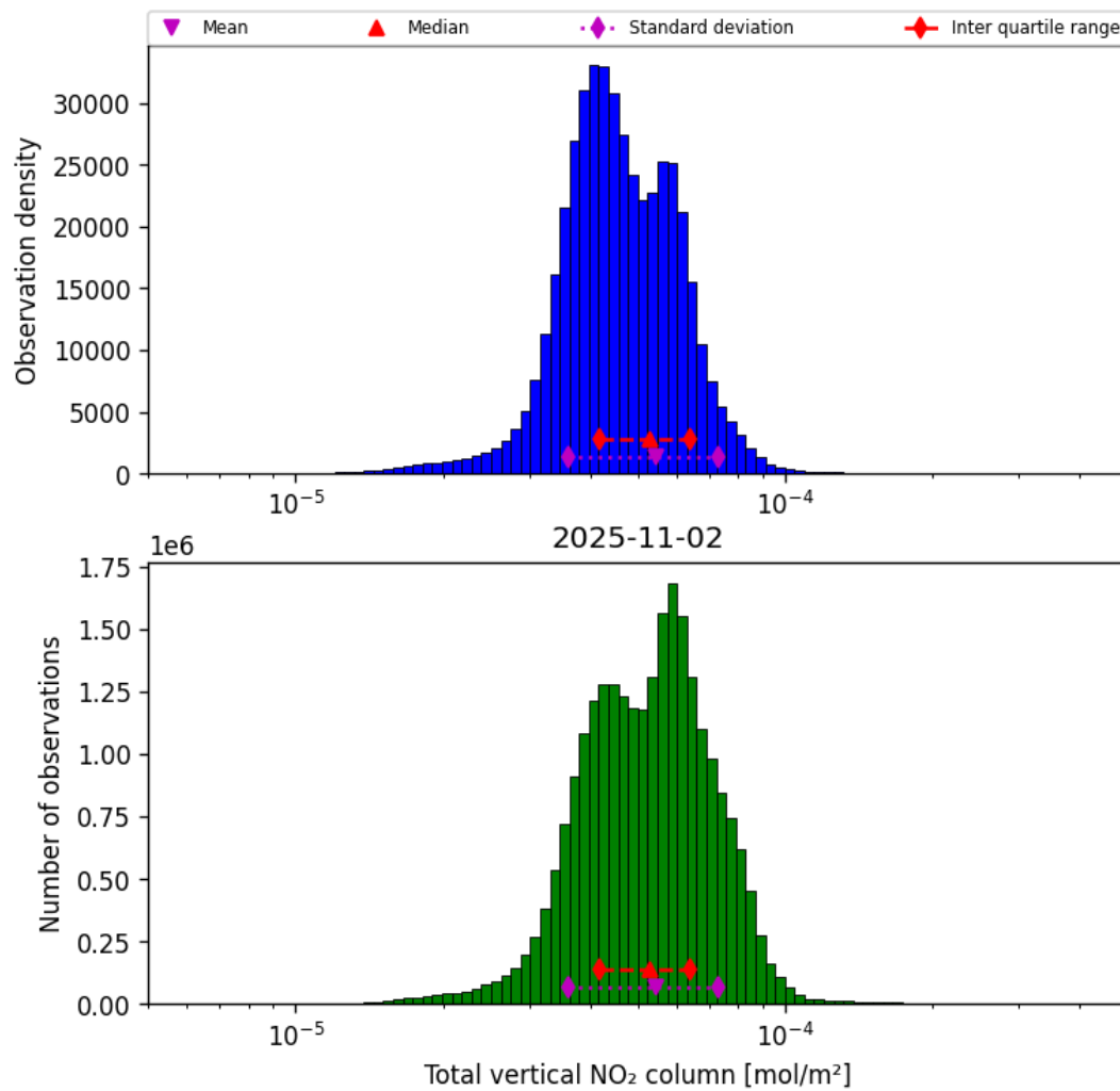
Figure 38: Histogram of “Total vertical NO 2 column” for 2025-11-02 to 2025-11-03
