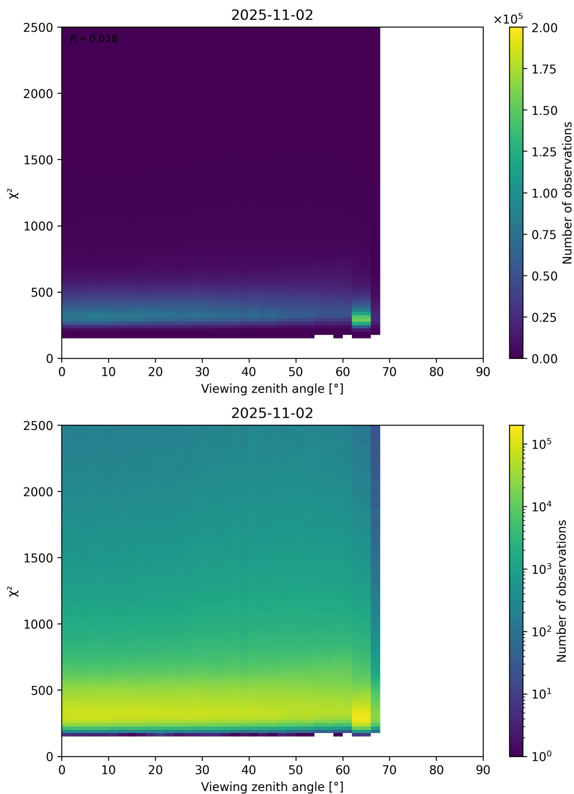
Figure 162: Scatter density plot of “Viewing zenith angle” against “ \chi^2 ” for 2025-11-02 to 2025-11-03.
