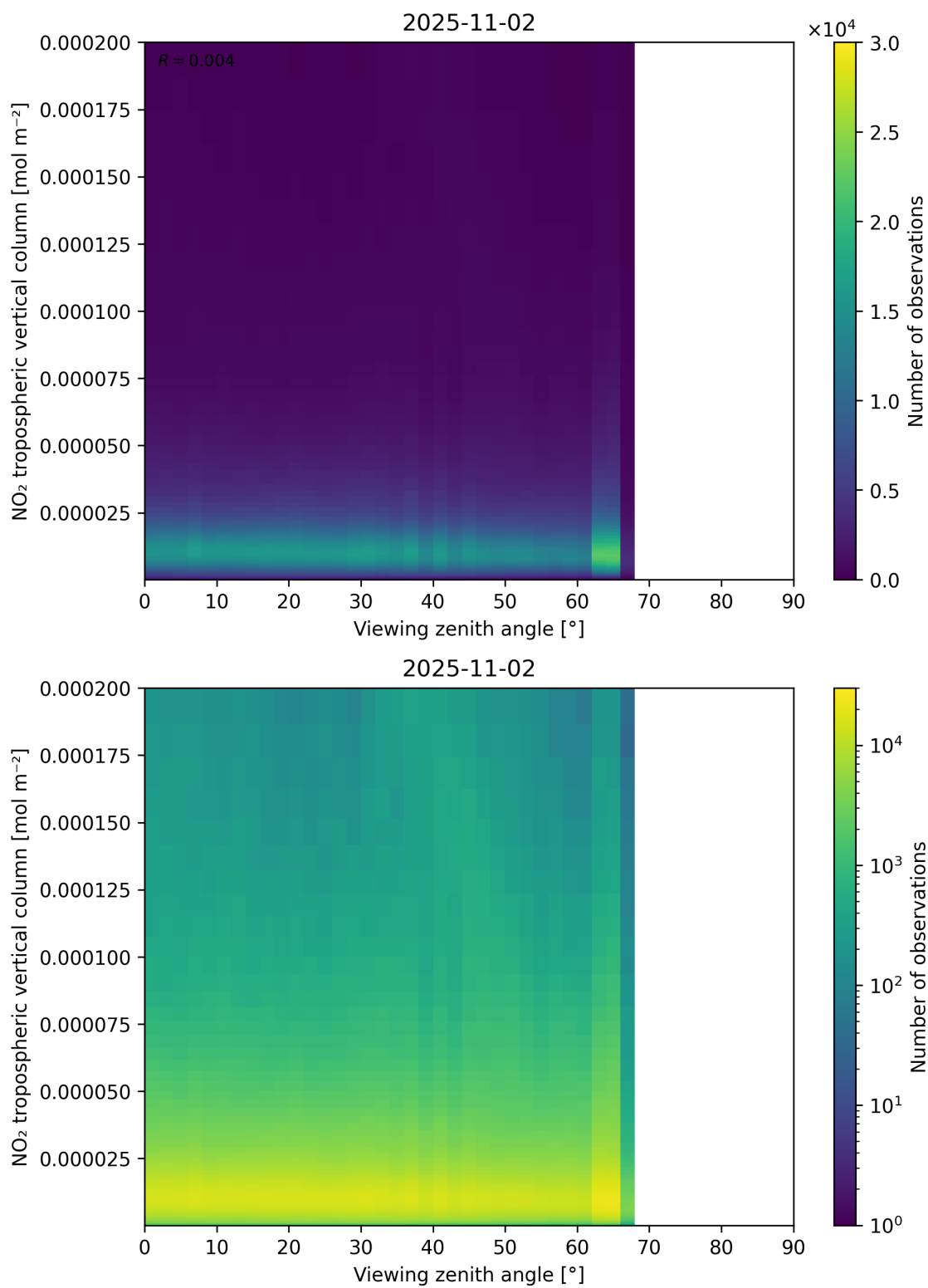
Figure 169: Scatter density plot of “Viewing zenith angle” against “NO 2 tropospheric vertical column” for 2025-11-02 to 2025-11-03.
