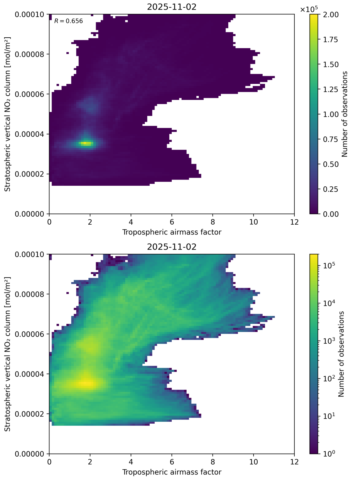
Figure 74: Scatter density plot of “Tropospheric airmass factor” against “Stratospheric vertical NO 2 column” for 2025-11-02 to 2025-11-03.
