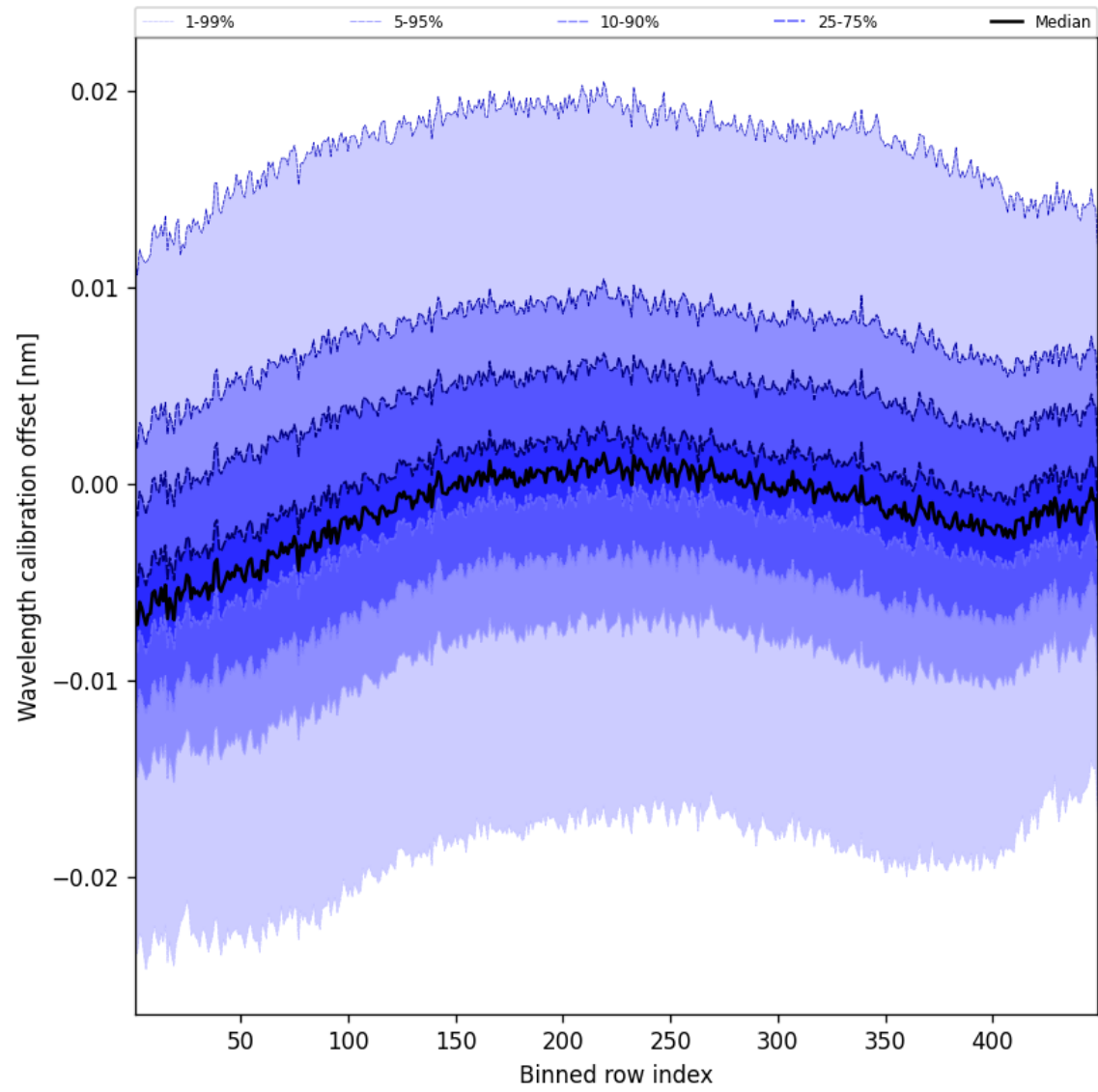
Figure 52: Along track statistics of “Wavelength calibration offset” for 2025-11-02 to 2025-11-03
