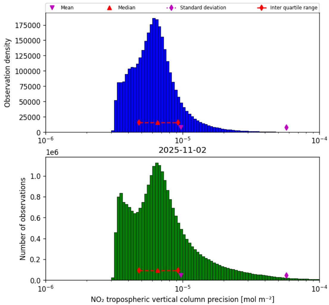
Figure 30: Histogram of “NO 2 tropospheric vertical column precision” for 2025-11-02 to 2025-11-03
