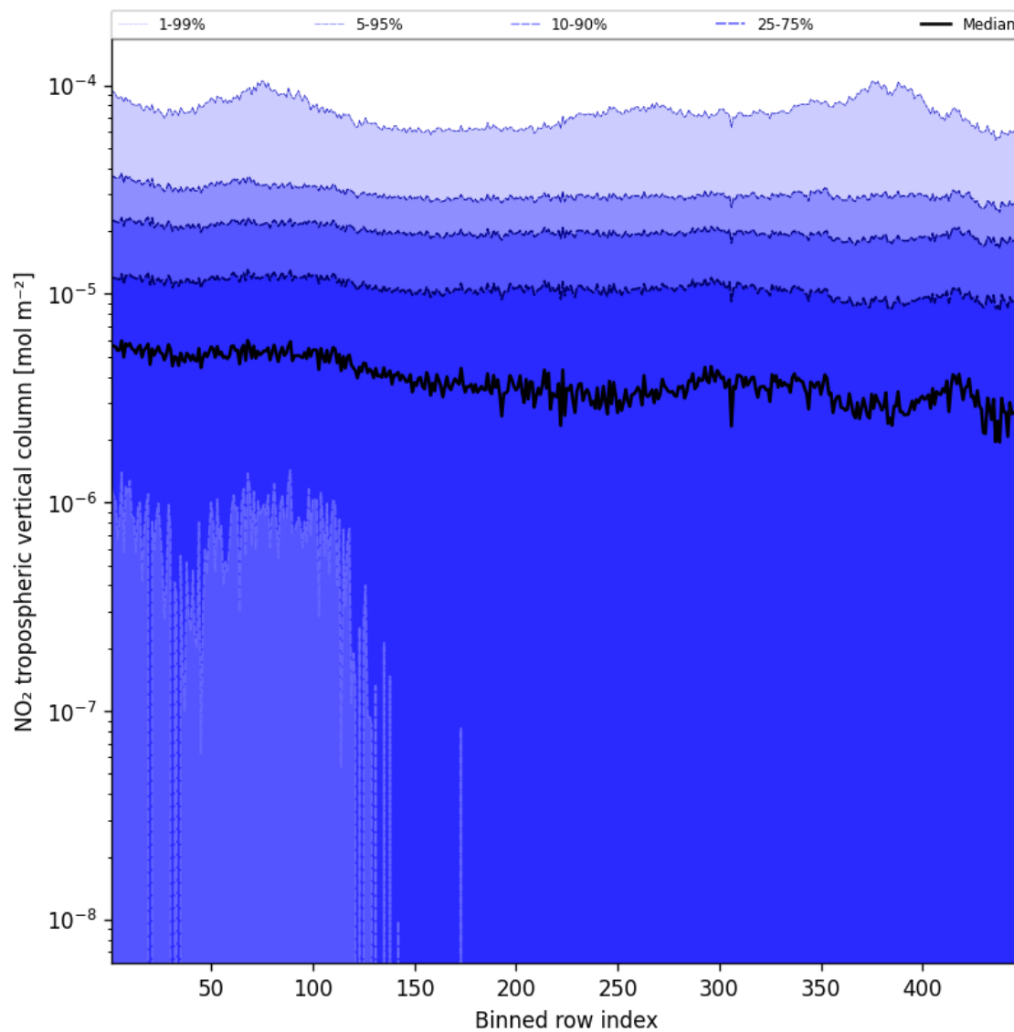
Figure 46: Along track statistics of “NO 2 tropospheric vertical column” for 2025-11-02 to 2025-11-03
