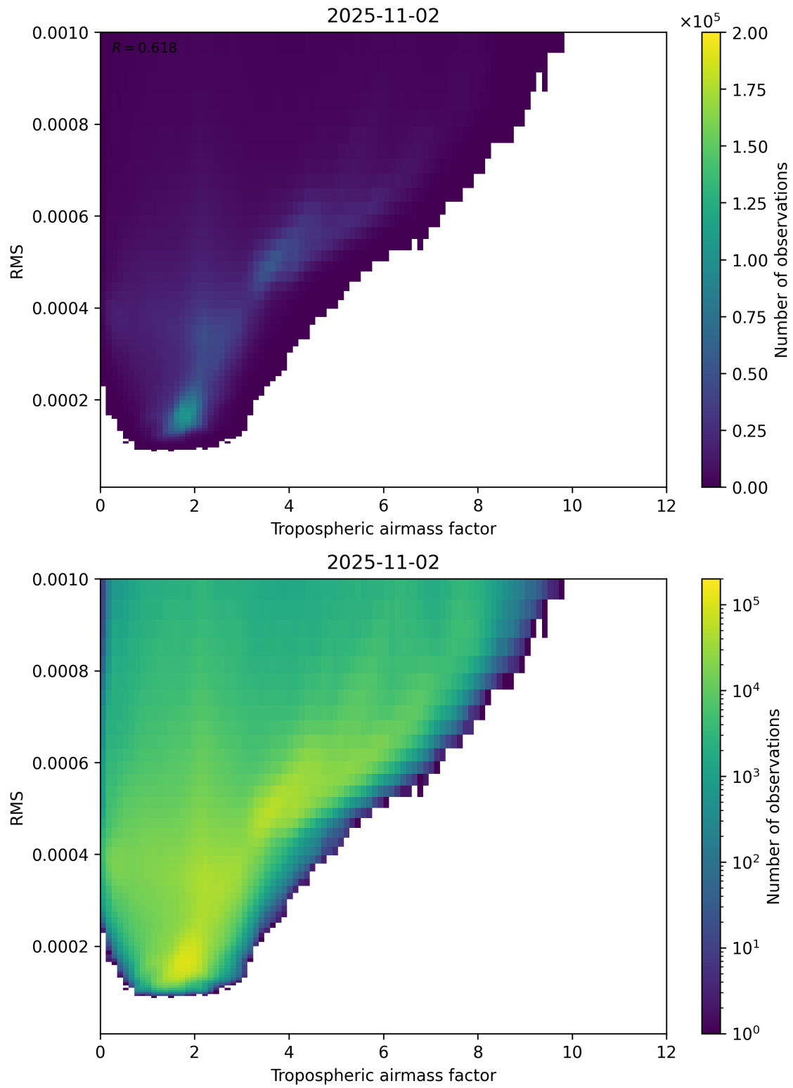
Figure 79: Scatter density plot of “Tropospheric airmass factor” against “RMS” for 2025-11-02 to 2025-11-03.
