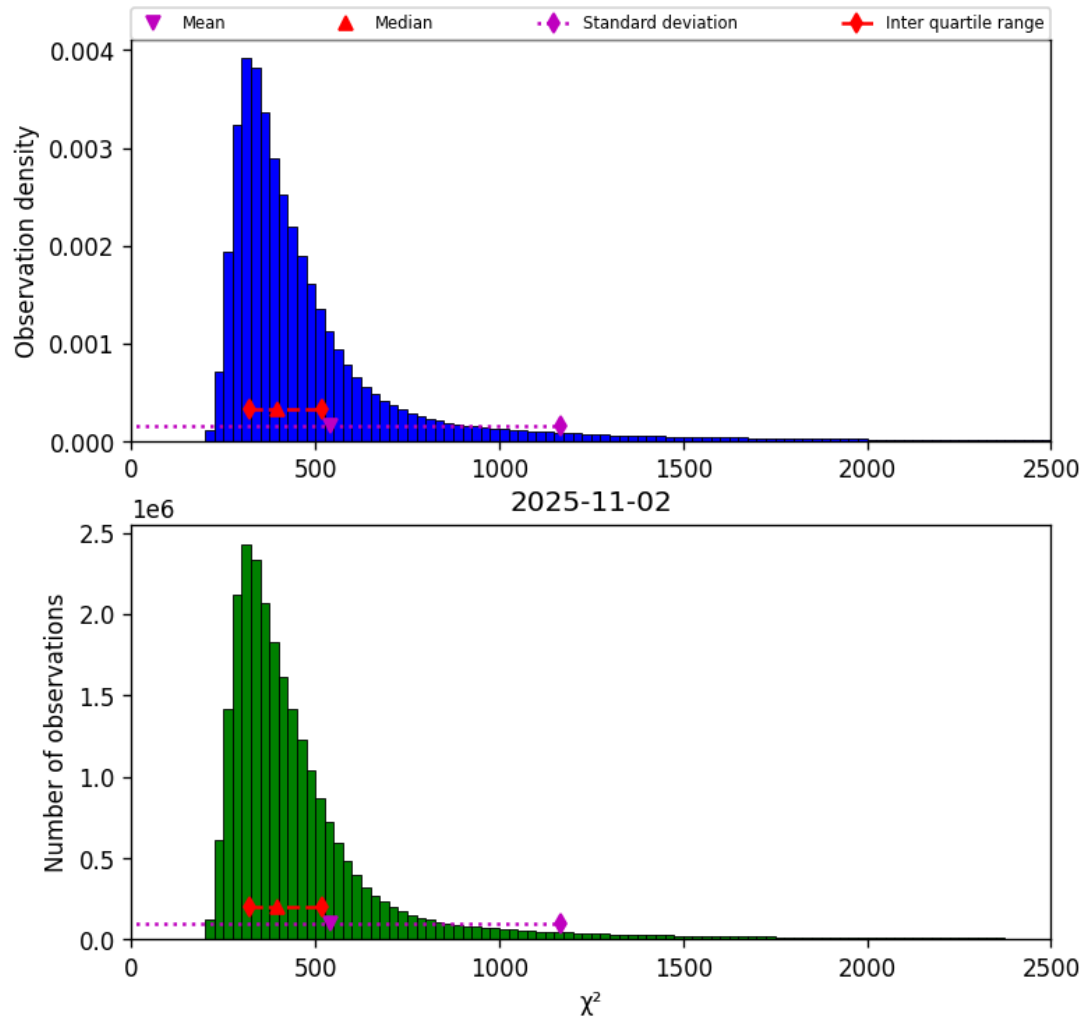
Figure 42: Histogram of “ \chi^2 ” for 2025-11-02 to 2025-11-03
