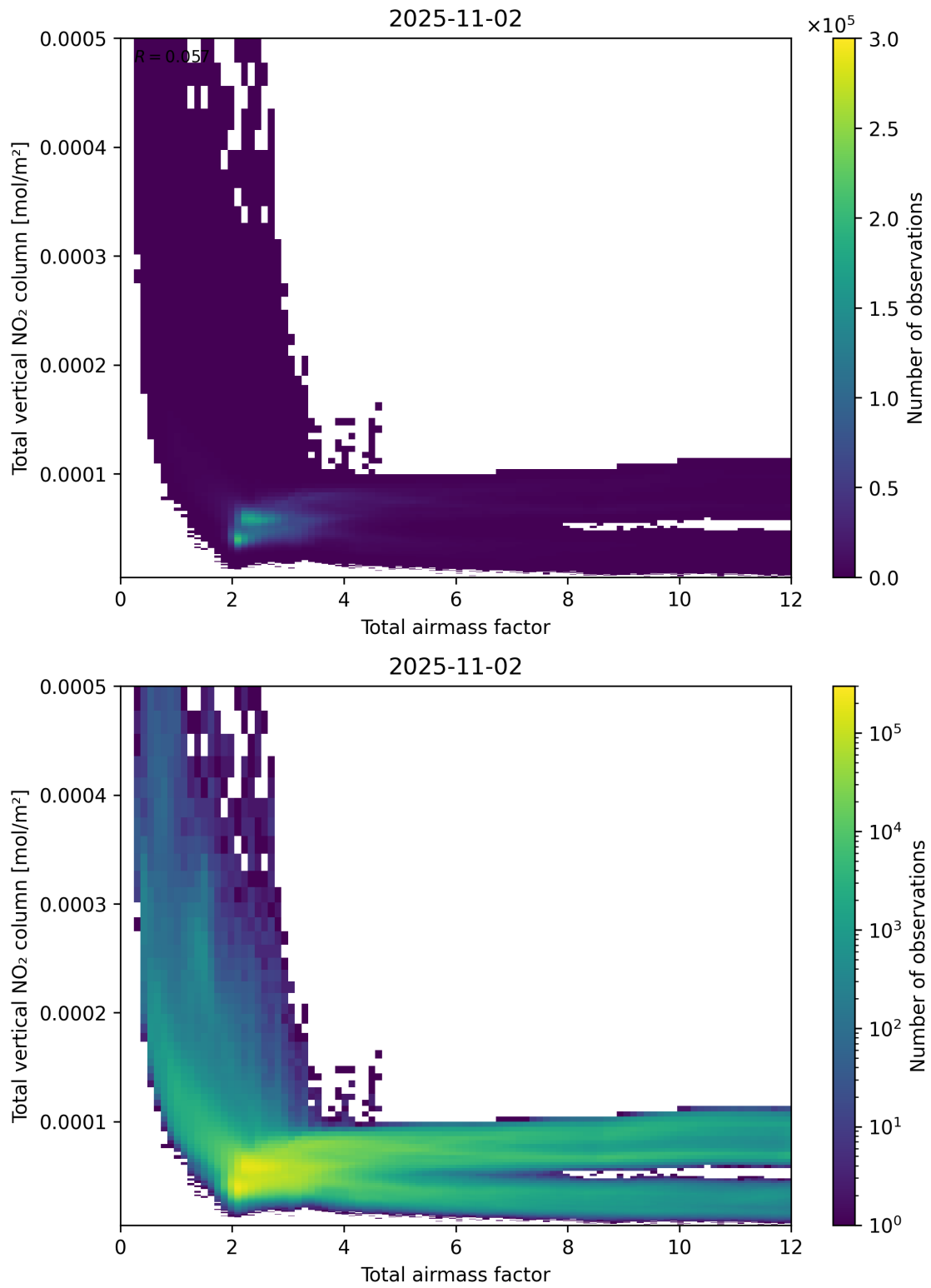
Figure 67: Scatter density plot of “Total air mass factor” against “Total vertical NO 2 column” for 2025-11-02 to 2025-11-03.
