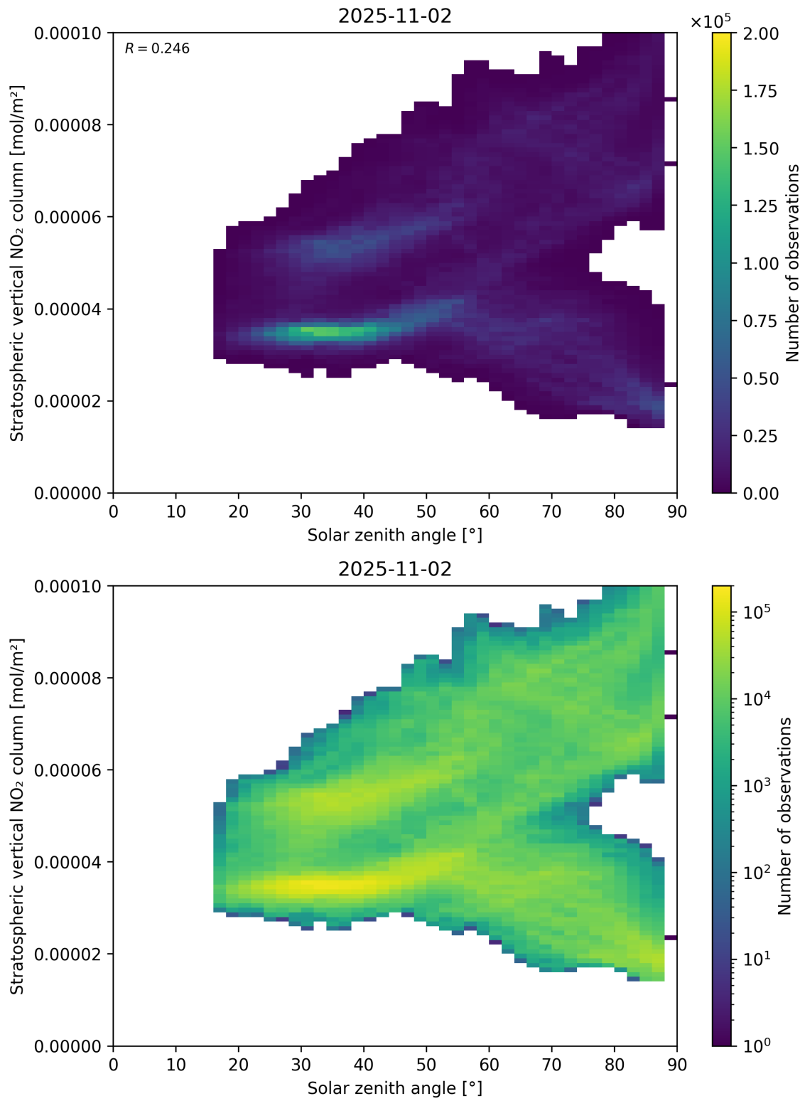
Figure 150: Scatter density plot of “Solar zenith angle” against “Stratospheric vertical NO 2 column” for 2025-11-02 to 2025-11-03.
