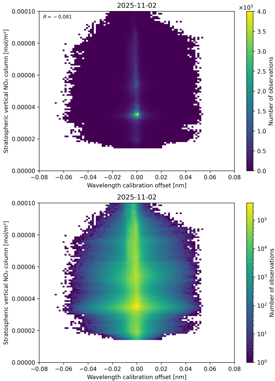
Figure 176: Scatter density plot of “Wavelength calibration offset” against “Stratospheric vertical NO 2 column” for 2025-11-02 to 2025-11-03.
