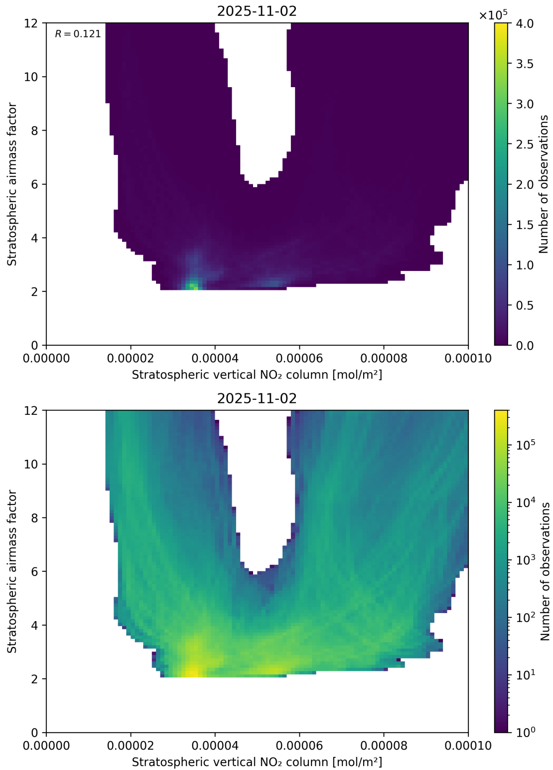
Figure 96: Scatter density plot of “Stratospheric vertical NO 2 column” against “Stratospheric airmass factor” for 2025-11-02 to 2025-11-03.
