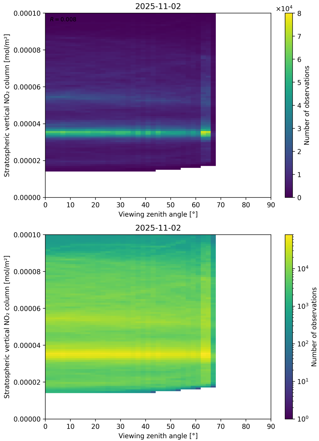
Figure 164: Scatter density plot of “Viewing zenith angle” against “Stratospheric vertical NO 2 column” for 2025-11-02 to 2025-11-03.
