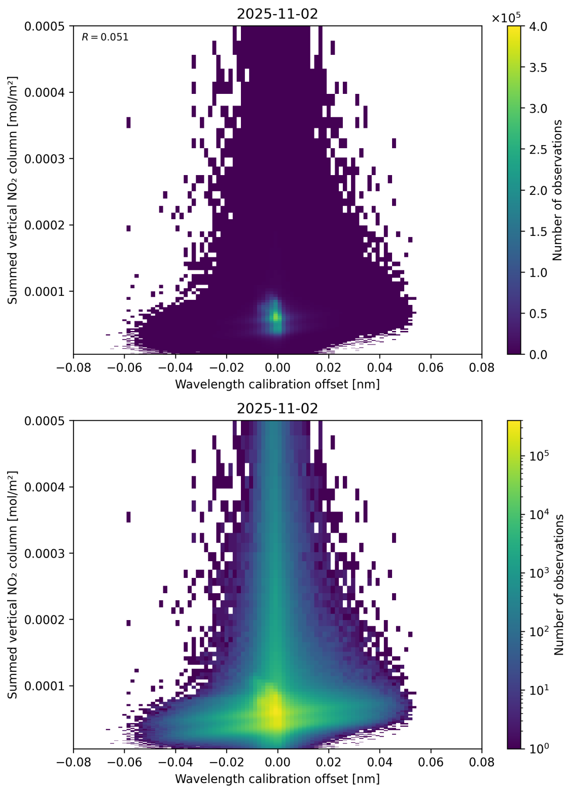
Figure 177: Scatter density plot of “Wavelength calibration offset” against “Summed vertical NO 2 column” for 2025-11-02 to 2025-11-03.
