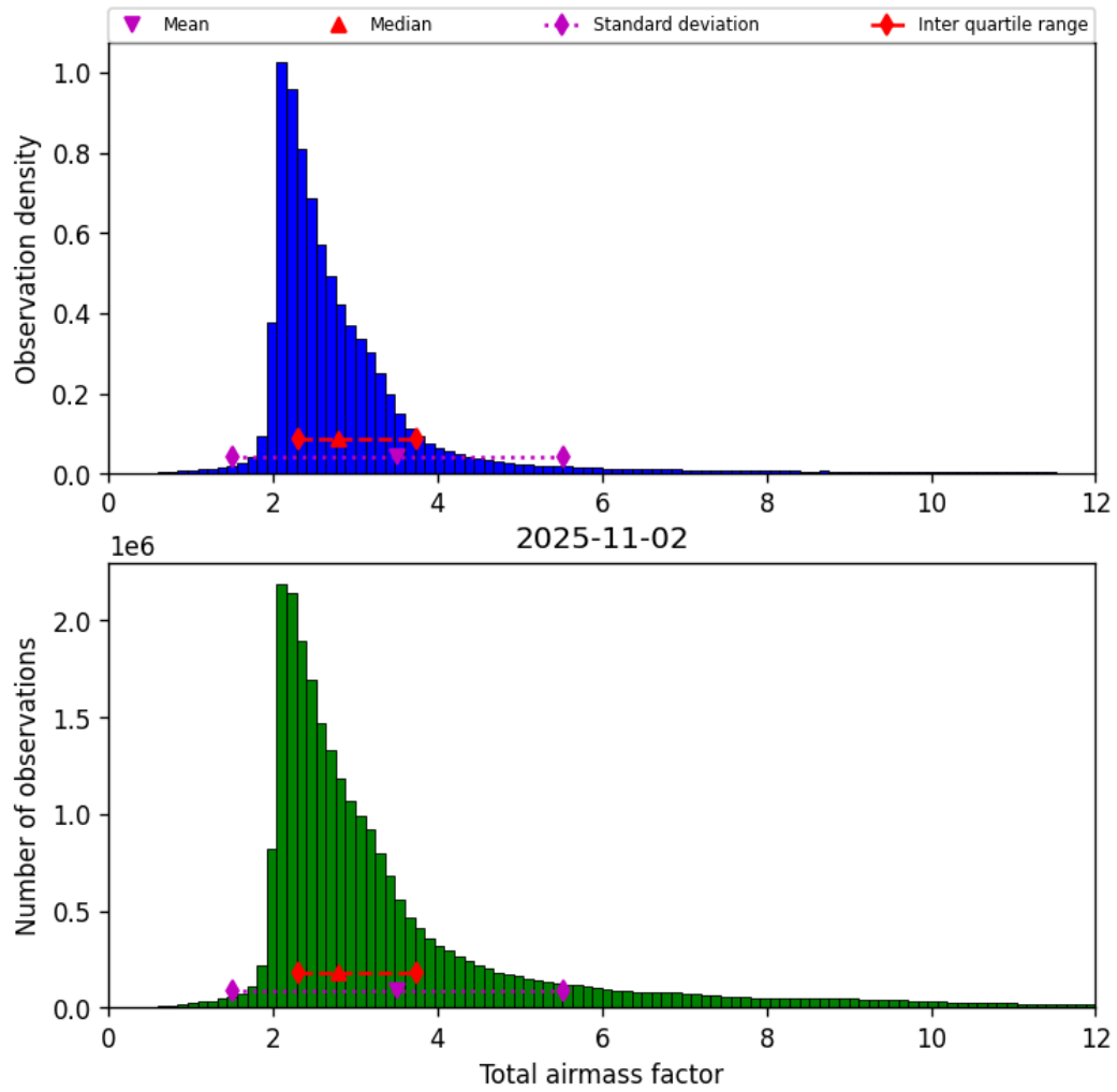
Figure 32: Histogram of “Total airmass factor” for 2025-11-02 to 2025-11-03
