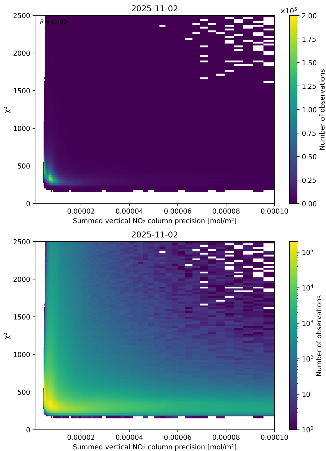
Figure 107: Scatter density plot of “Summed vertical NO 2 column precision” against “ \chi^2 ” for 2025-11-02 to 2025-11-03.
