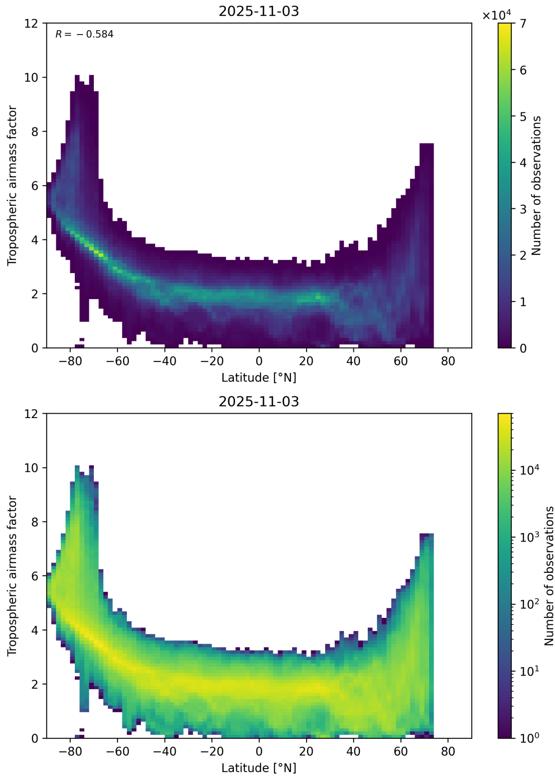
Figure 85: Scatter density plot of “Latitude” against “Tropospheric air mass factor” for 2025-11-02 to 2025-11-04.
