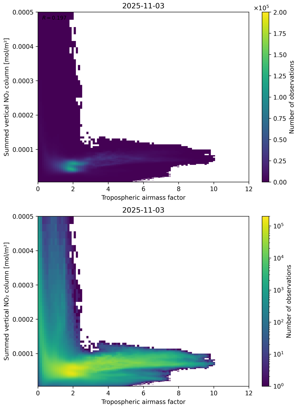
Figure 75: Scatter density plot of “Tropospheric airmass factor” against “Summed vertical NO 2 column” for 2025-11-02 to 2025-11-04.
