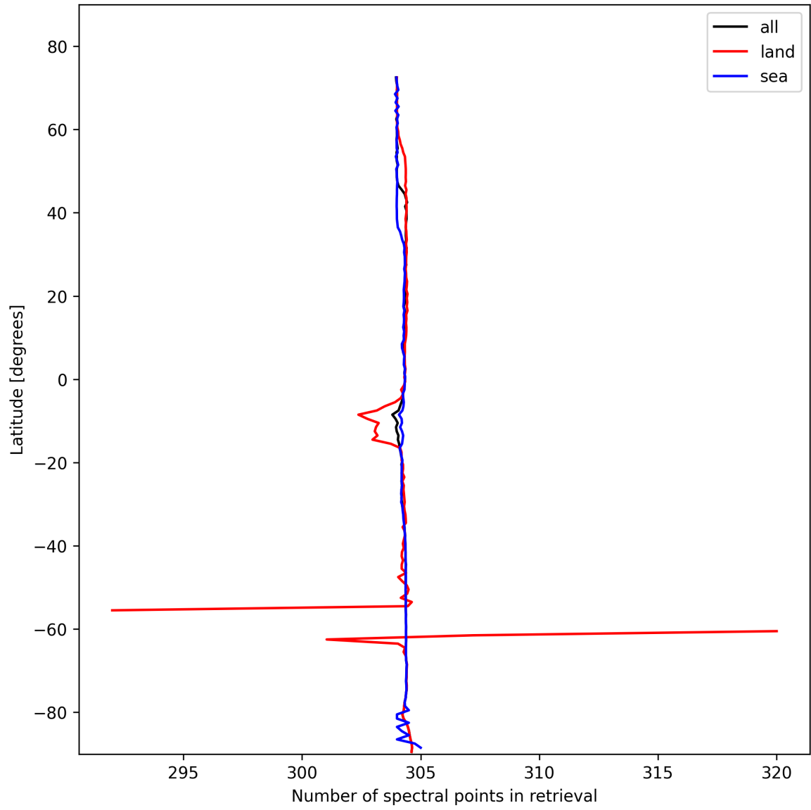
Figure 16: Zonal average of “Number of spectral points in retrieval” for 2025-11-02 to 2025-11-04.
