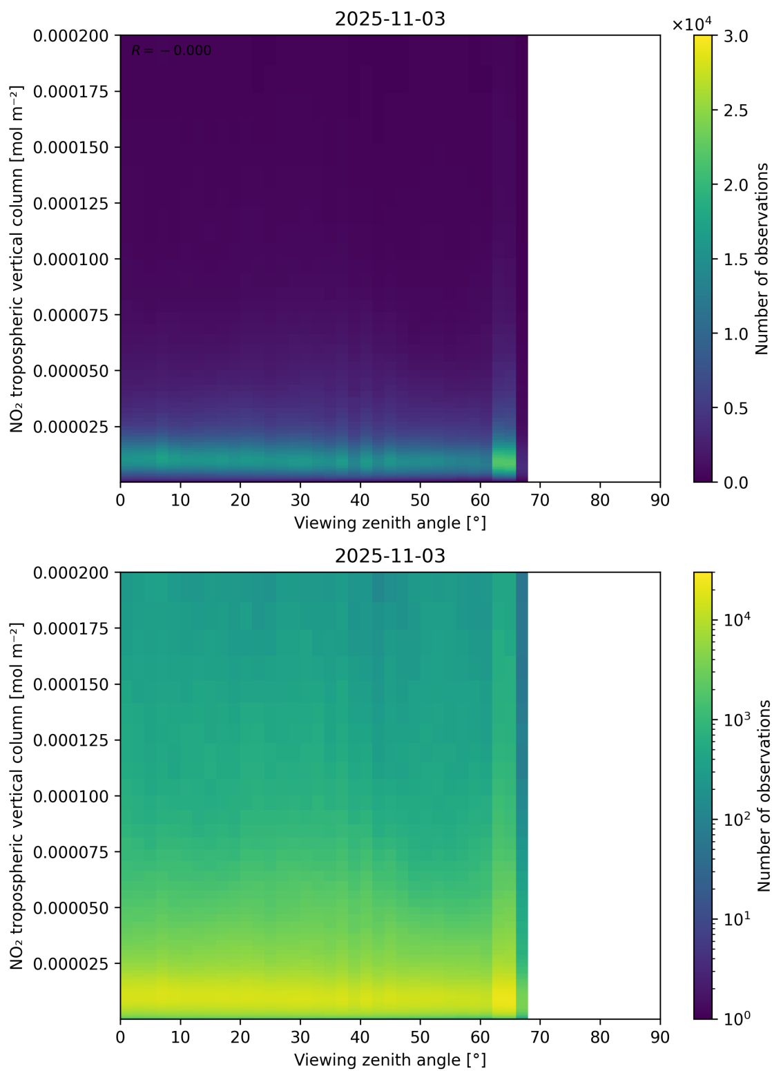
Figure 169: Scatter density plot of “Viewing zenith angle” against “NO 2 tropospheric vertical column” for 2025-11-02 to 2025-11-04.
