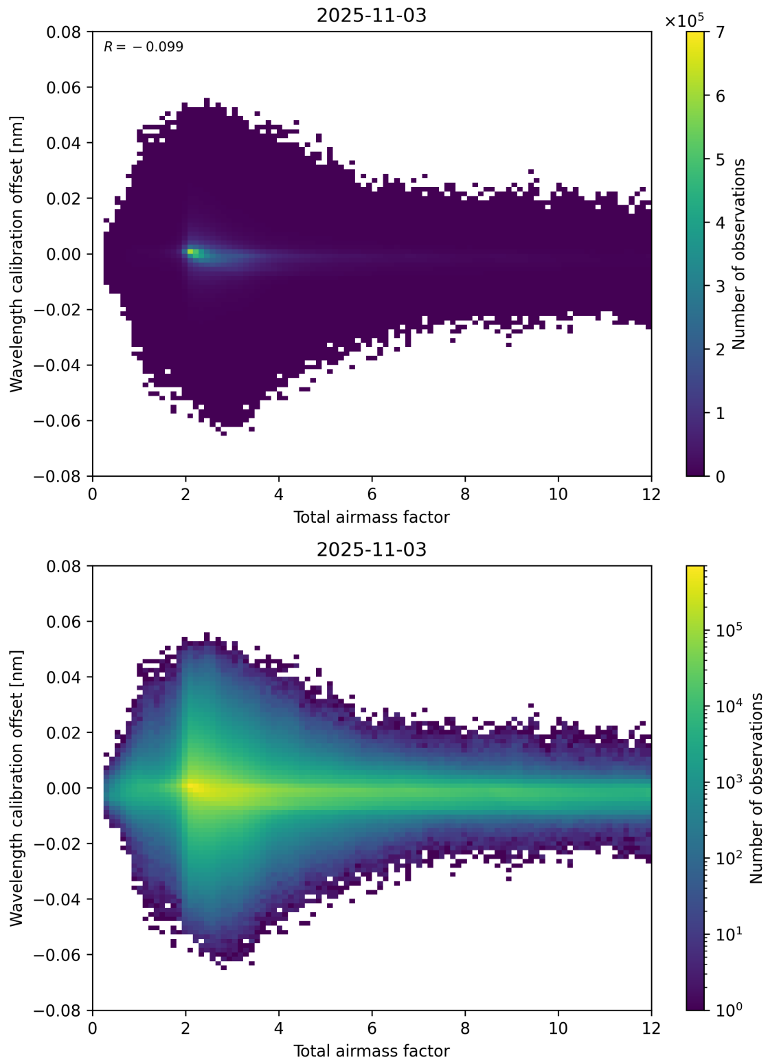
Figure 70: Scatter density plot of “Total airmass factor” against “Wavelength calibration offset” for 2025-11-02 to 2025-11-04.
