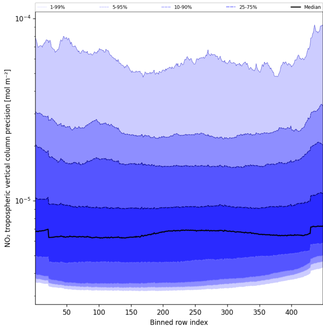
Figure 47: Along track statistics of “NO 2 tropospheric vertical column precision” for 2025-11-02 to 2025-11-04
