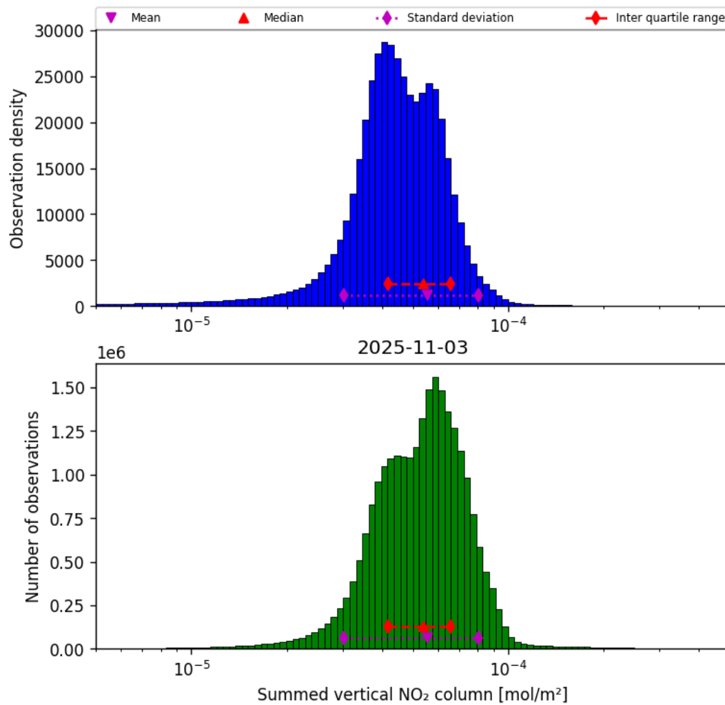
Figure 40: Histogram of "Summed vertical NO 2 column" for 2025-11-02 to 2025-11-04
