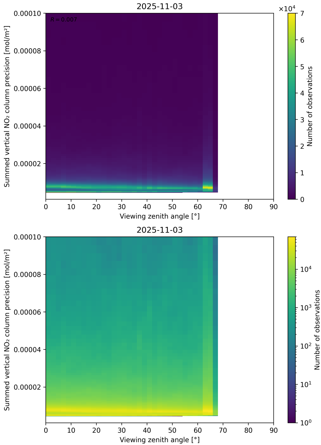
Figure 166: Scatter density plot of “Viewing zenith angle” against “Summed vertical NO 2 column precision” for 2025-11-02 to 2025-11-04.
