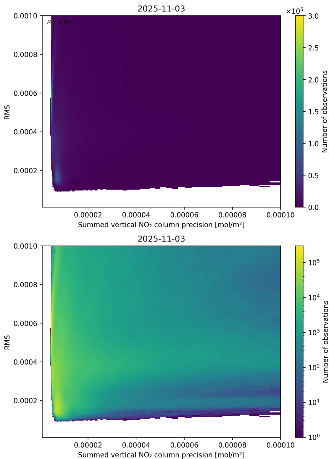
Figure 108: Scatter density plot of “Summed vertical NO 2 column precision” against “RMS” for 2025-11-02 to 2025-11-04.
