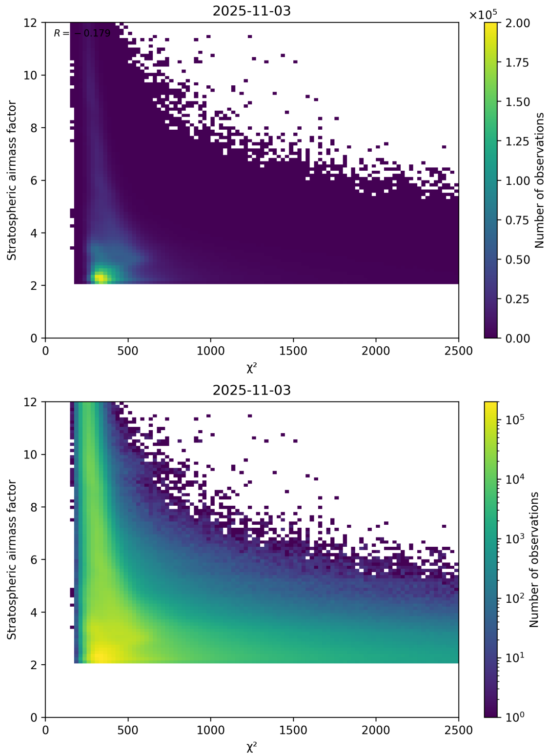
Figure 81: Scatter density plot of “ \chi^2 ” against “Stratospheric airmass factor” for 2025-11-02 to 2025-11-04.
