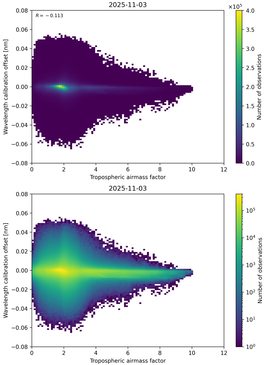
Figure 80: Scatter density plot of “Tropospheric airmass factor” against “Wavelength calibration offset” for 2025-11-02 to 2025-11-04.
