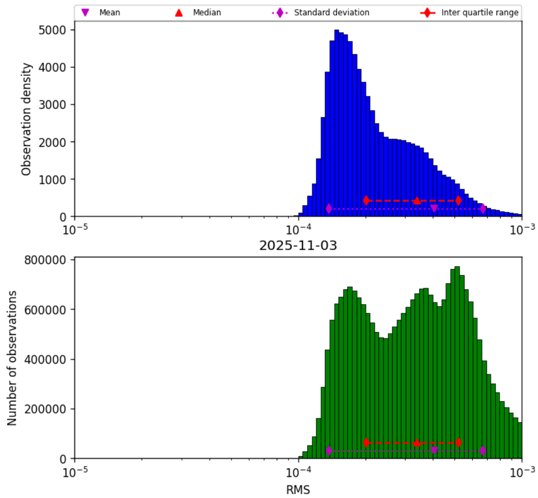
Figure 43: Histogram of “RMS” for 2025-11-02 to 2025-11-04
