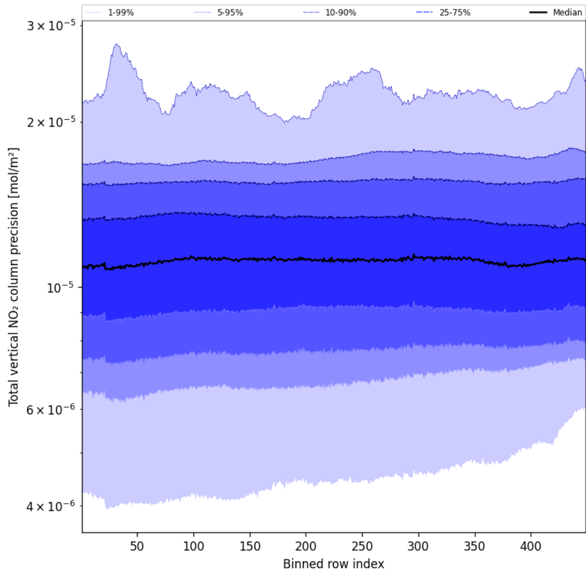
Figure 56: Along track statistics of “Total vertical NO 2 column precision” for 2025-11-02 to 2025-11-04
