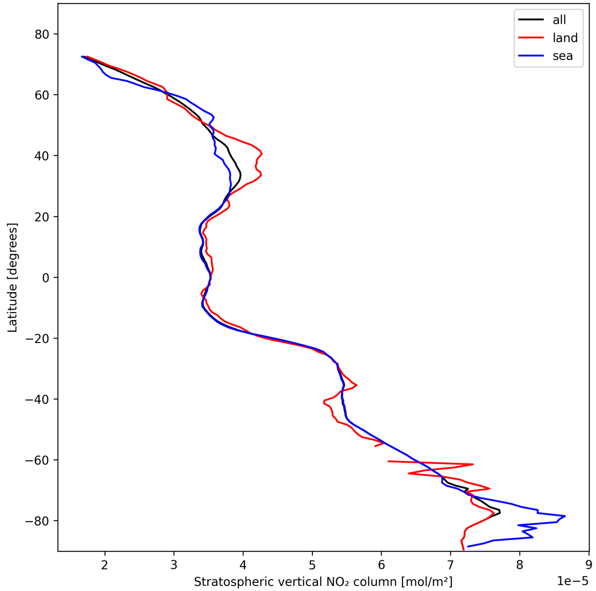
Figure 19: Zonal average of “Stratospheric vertical NO 2 column” for 2025-11-02 to 2025-11-04.
