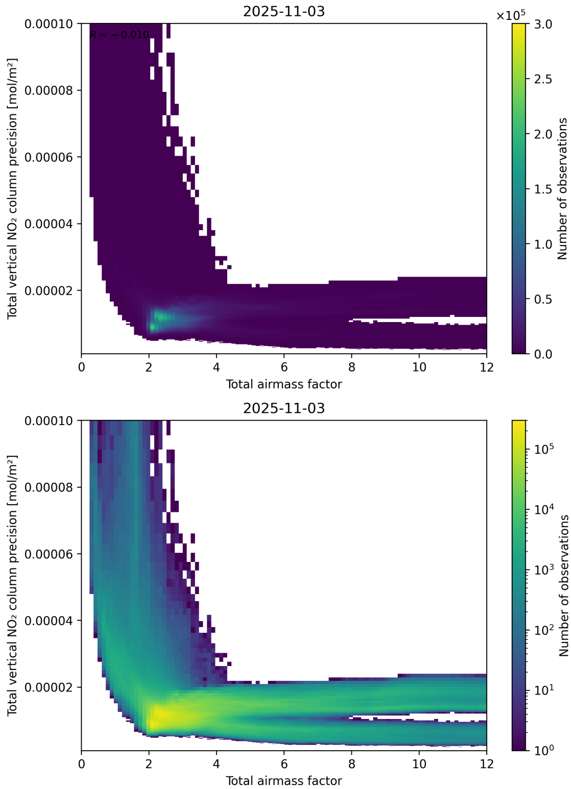
Figure 68: Scatter density plot of “Total airmass factor” against “Total vertical NO 2 column precision” for 2025-11-02 to 2025-11-04.
