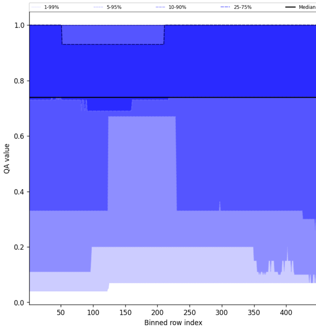
Figure 45: Along track statistics of “QA value” for 2025-11-02 to 2025-11-04
