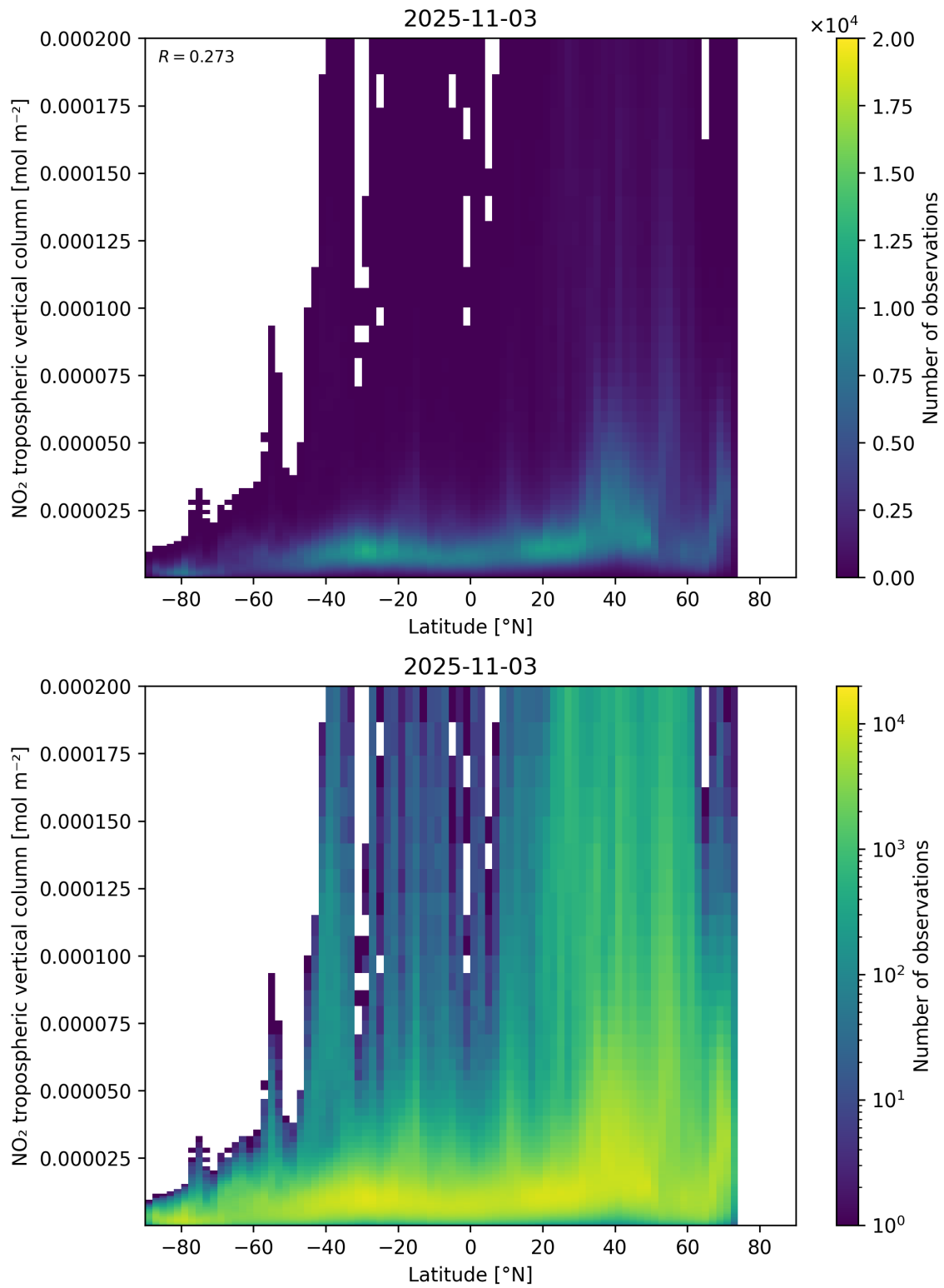
Figure 92: Scatter density plot of “Latitude” against “NO 2 tropospheric vertical column” for 2025-11-02 to 2025-11-04.
