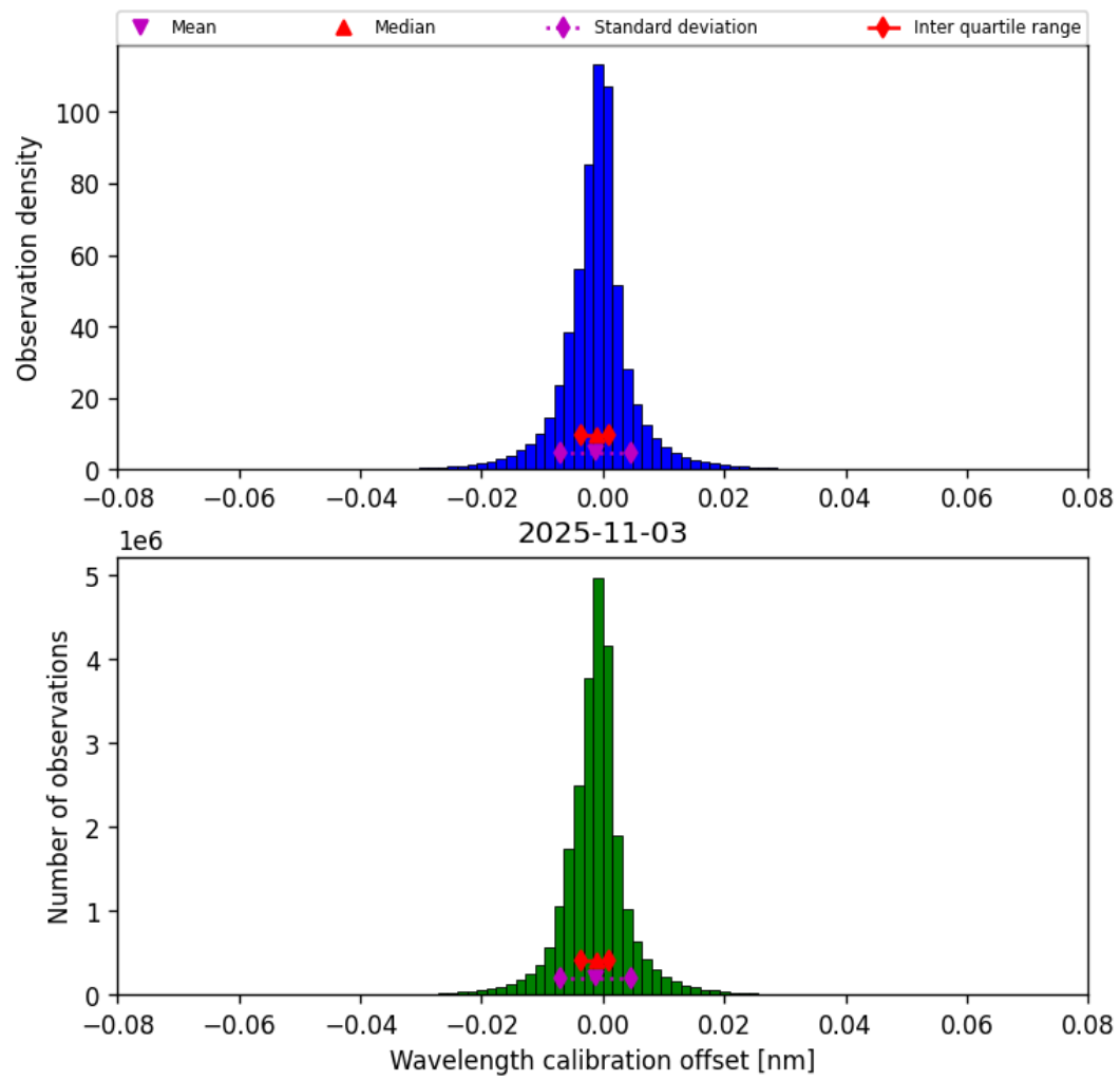
Figure 35: Histogram of “Wavelength calibration offset” for 2025-11-02 to 2025-11-04
