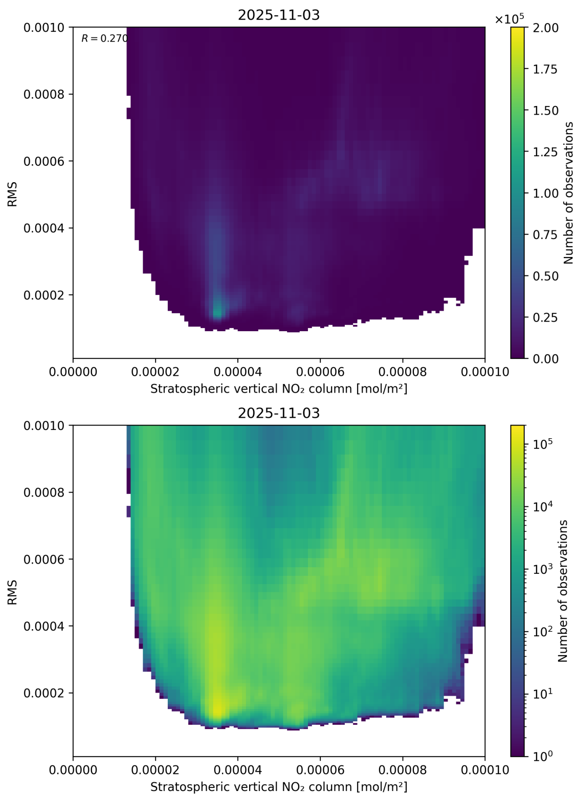
Figure 102: Scatter density plot of “Stratospheric vertical NO 2 column” against “RMS” for 2025-11-02 to 2025-11-04.
