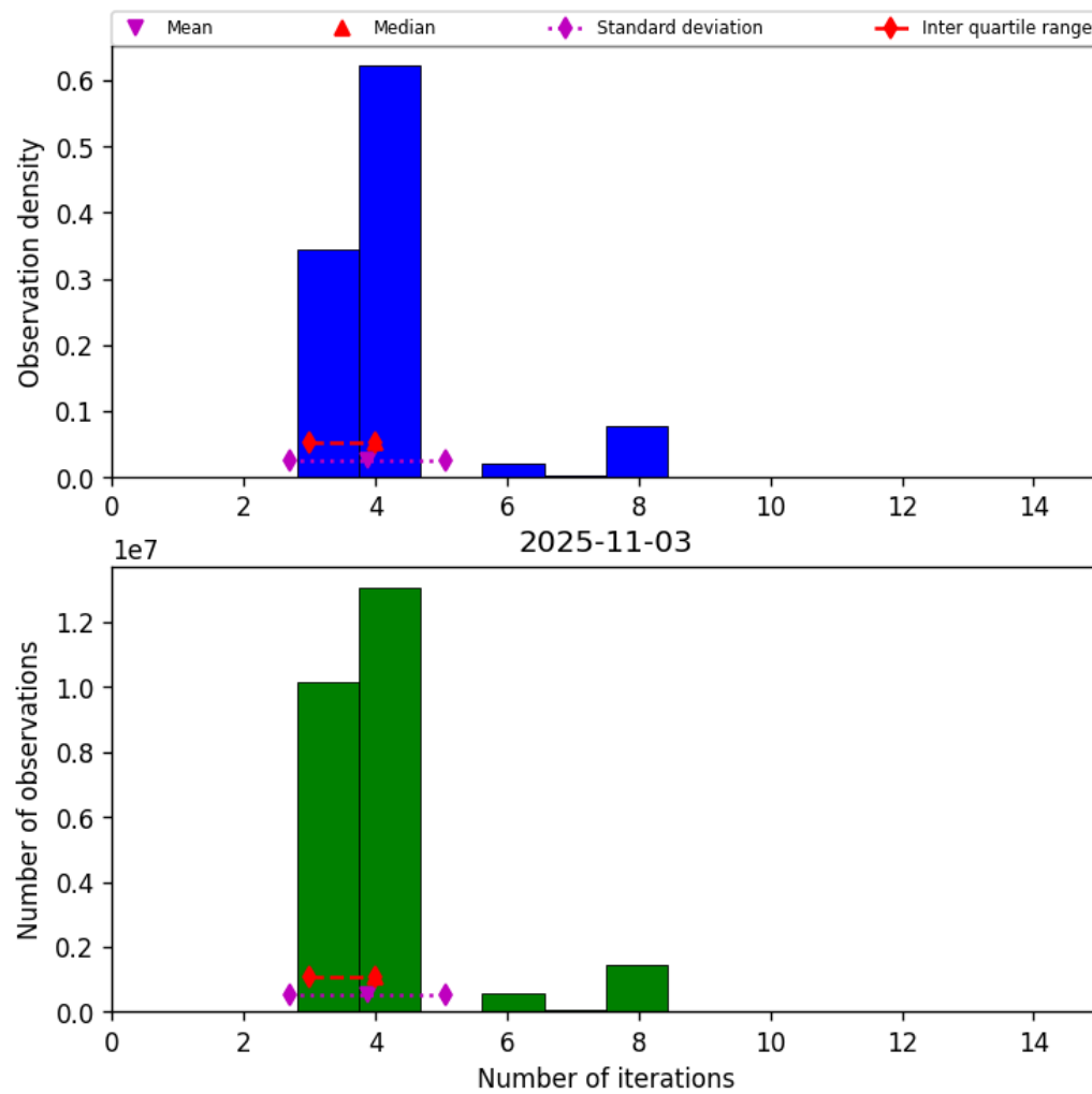
Figure 34: Histogram of “Number of iterations” for 2025-11-02 to 2025-11-04
