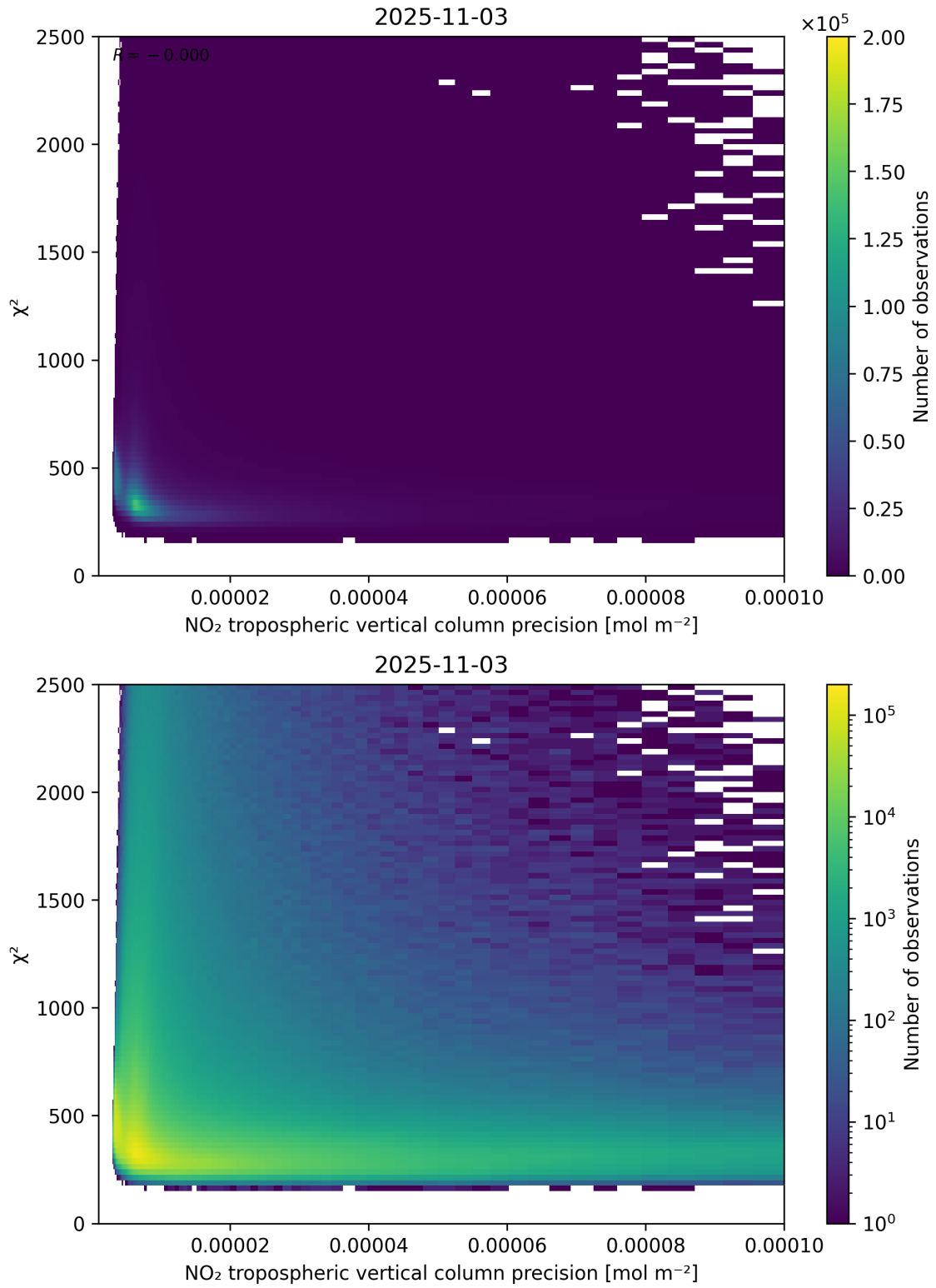
Figure 134: Scatter density plot of “NO 2 tropospheric vertical column precision” against “ \chi^2 ” for 2025-11-02 to 2025-11-04.
