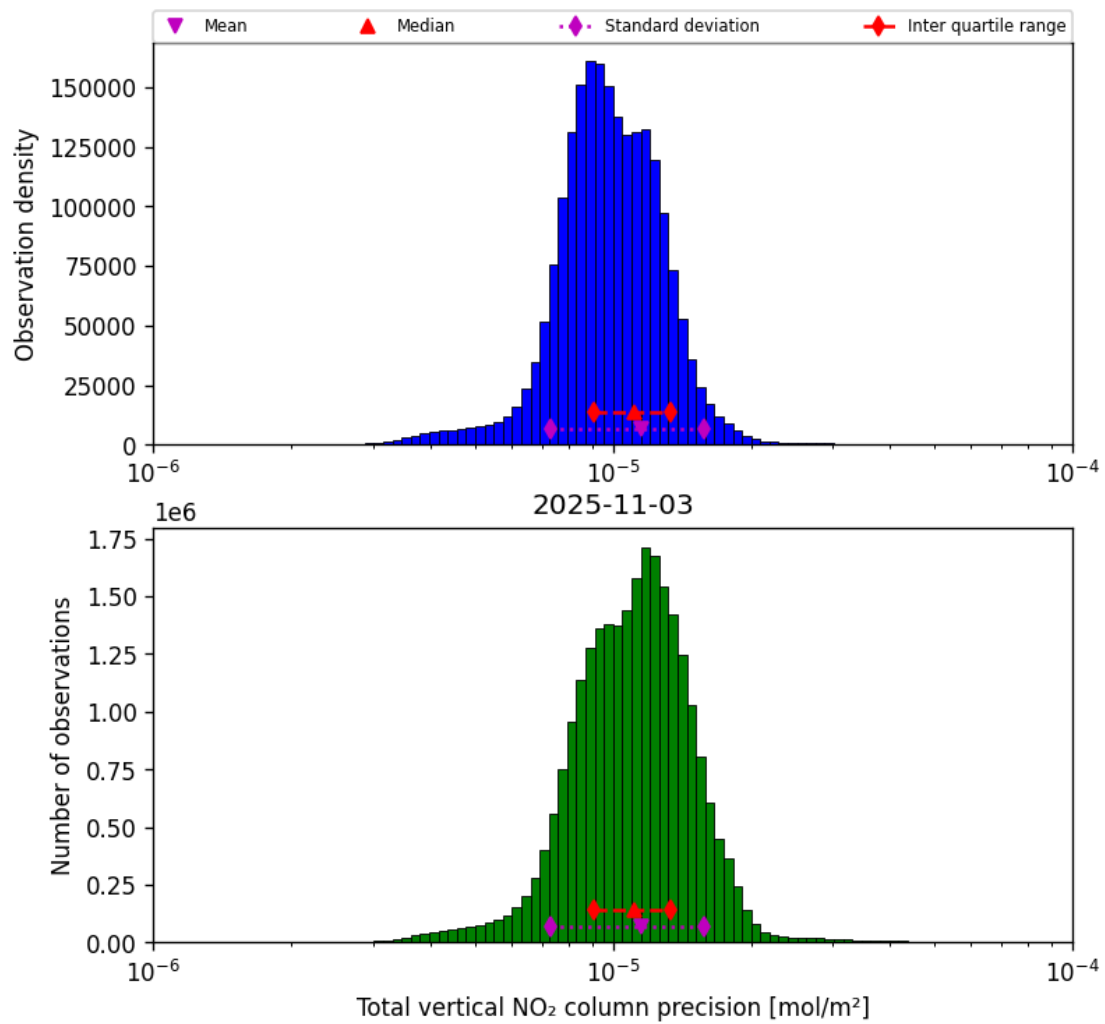
Figure 39: Histogram of “Total vertical NO 2 column precision” for 2025-11-02 to 2025-11-04
