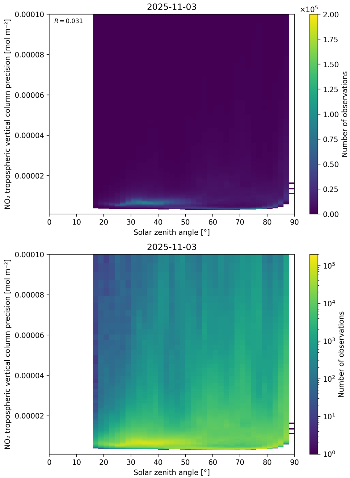
Figure 156: Scatter density plot of “Solar zenith angle” against “NO 2 tropospheric vertical column precision” for 2025-11-02 to 2025-11-04.
