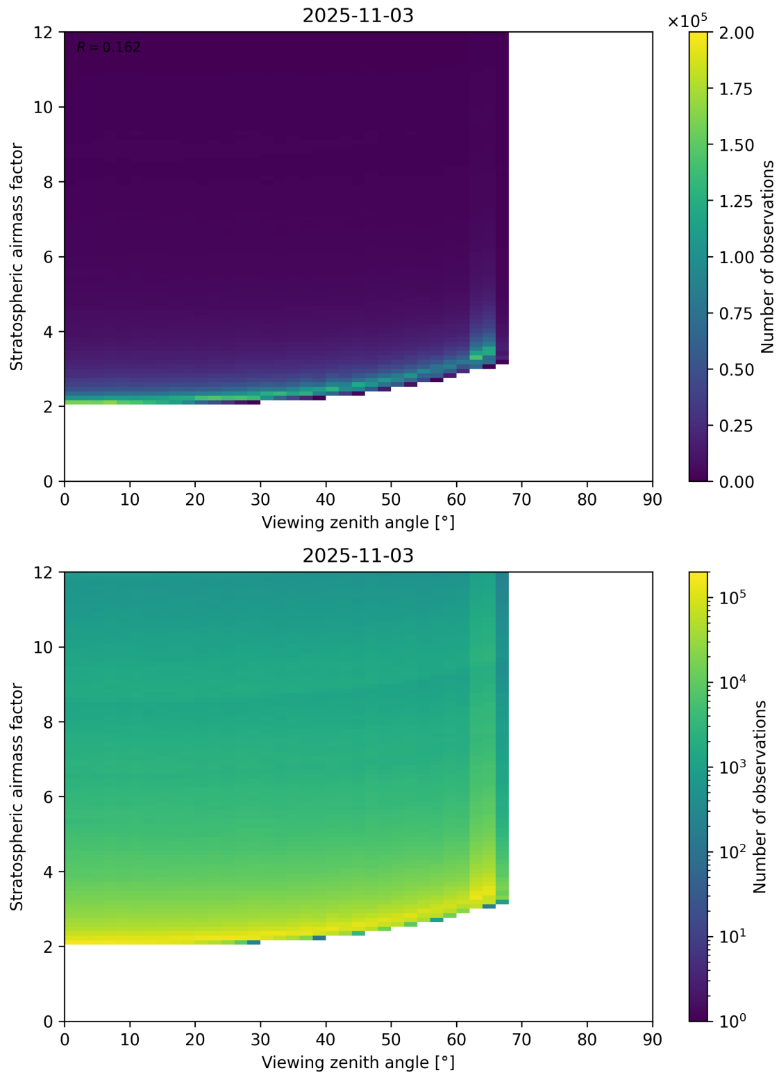
Figure 159: Scatter density plot of “Viewing zenith angle” against “Stratospheric airmass factor” for 2025-11-02 to 2025-11-04.
