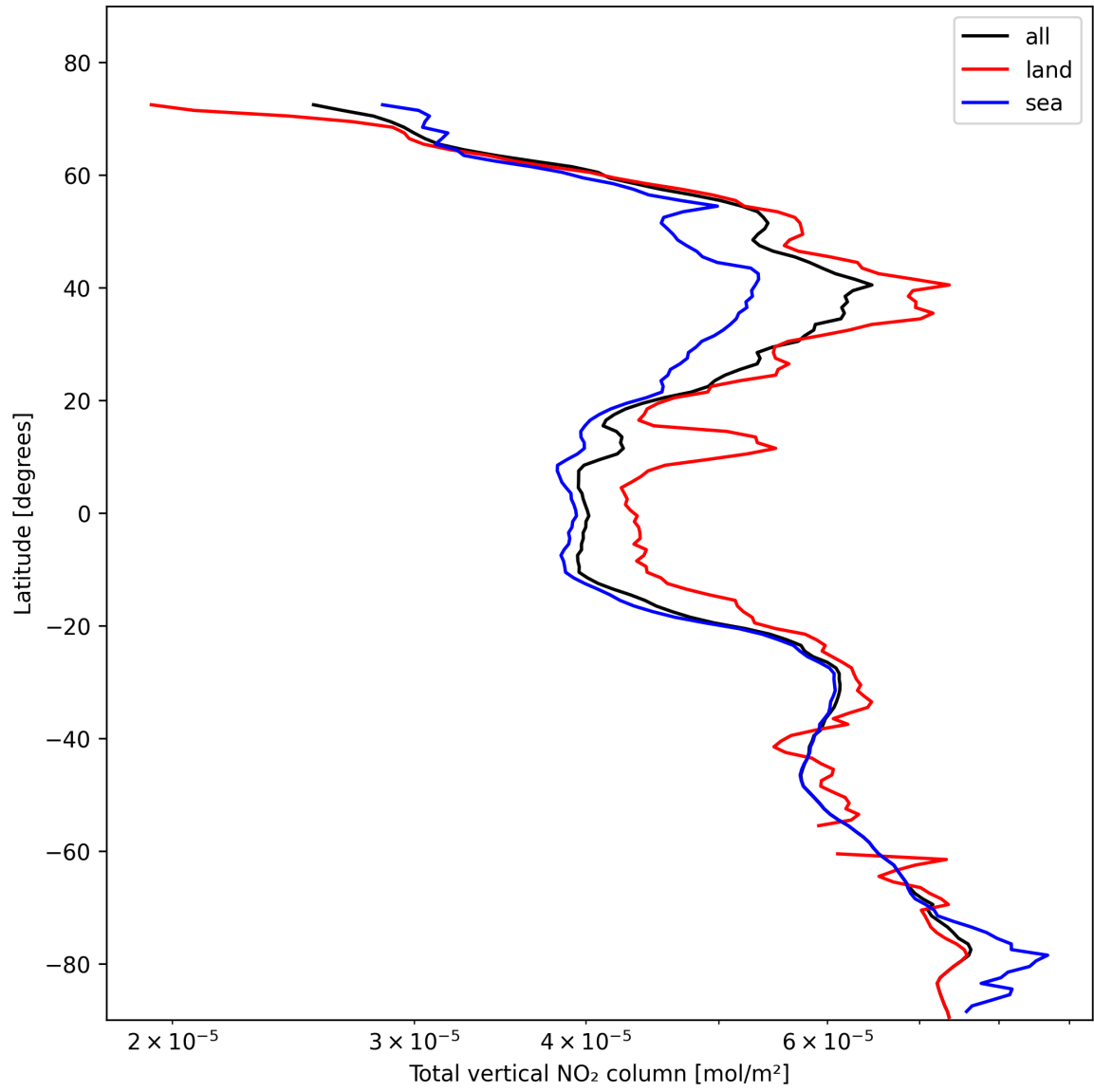
Figure 21: Zonal average of “Total vertical NO 2 column” for 2025-11-02 to 2025-11-04.
