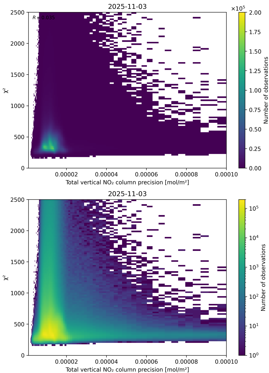
Figure 116: Scatter density plot of “Total vertical NO 2 column precision” against “ \chi^2 ” for 2025-11-02 to 2025-11-04.
