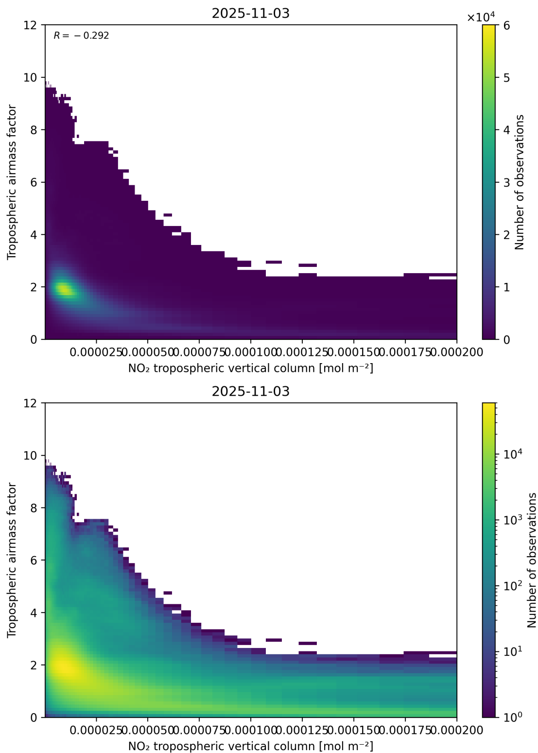
Figure 123: Scatter density plot of “NO 2 tropospheric vertical column” against “Tropospheric air mass factor” for 2025-11-02 to 2025-11-04.
