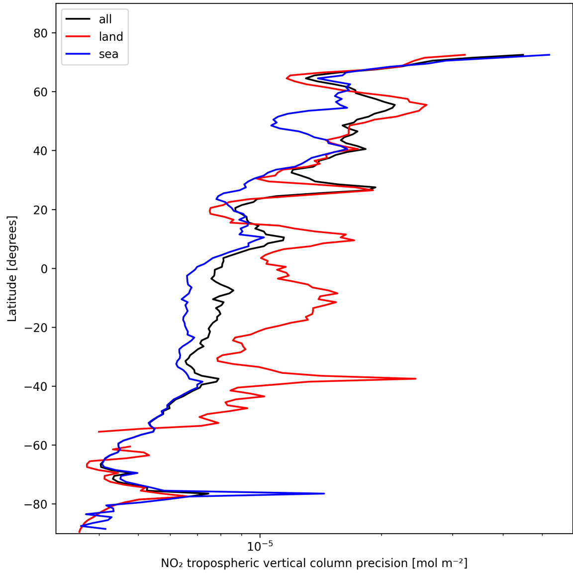
Figure 13: Zonal average of "NO 2 tropospheric vertical column precision" for 2025-11-02 to 2025-11-04.
