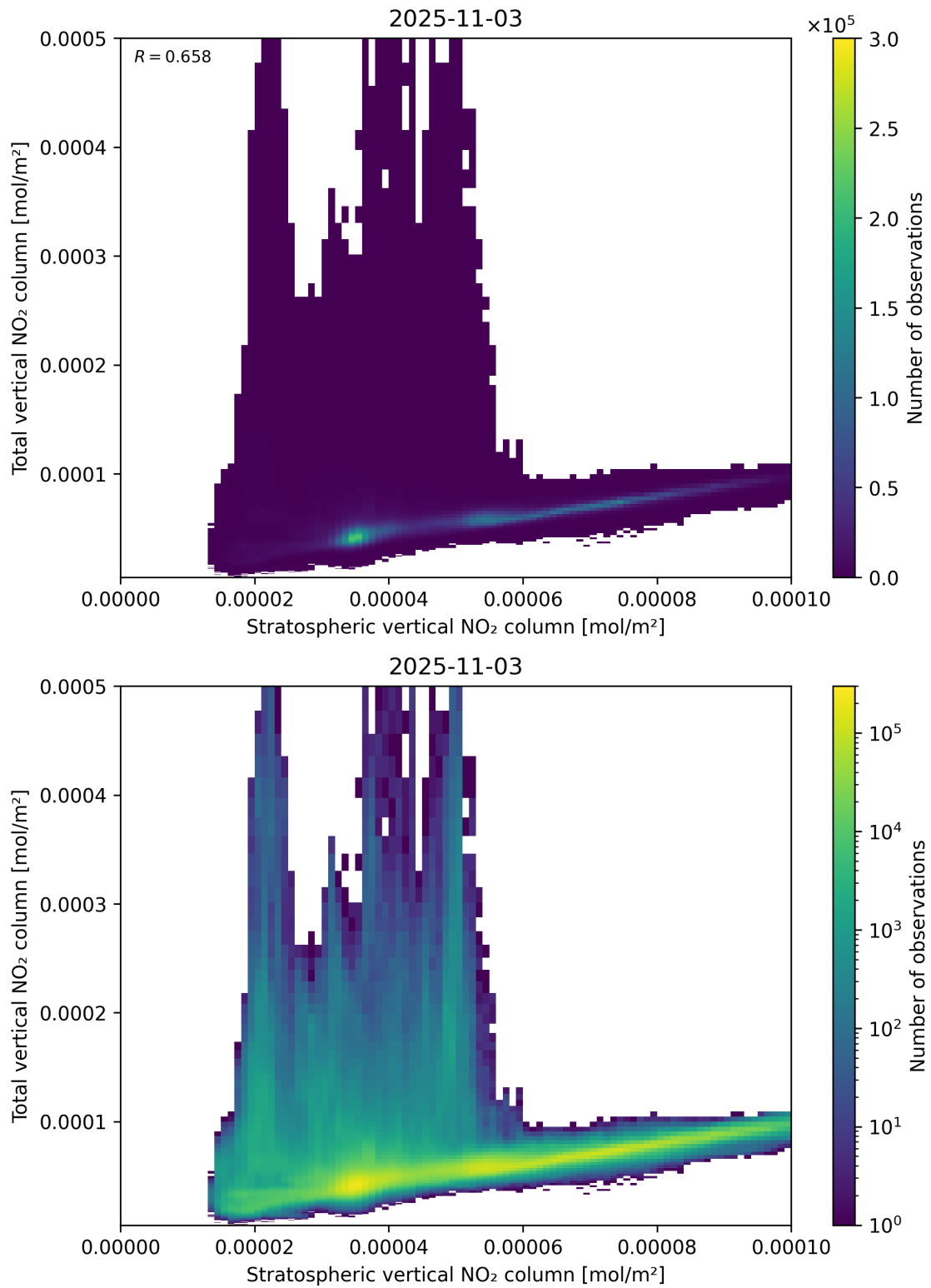
Figure 100: Scatter density plot of “Stratospheric vertical NO 2 column” against “Total vertical NO 2 column” for 2025-11-02 to 2025-11-04.
