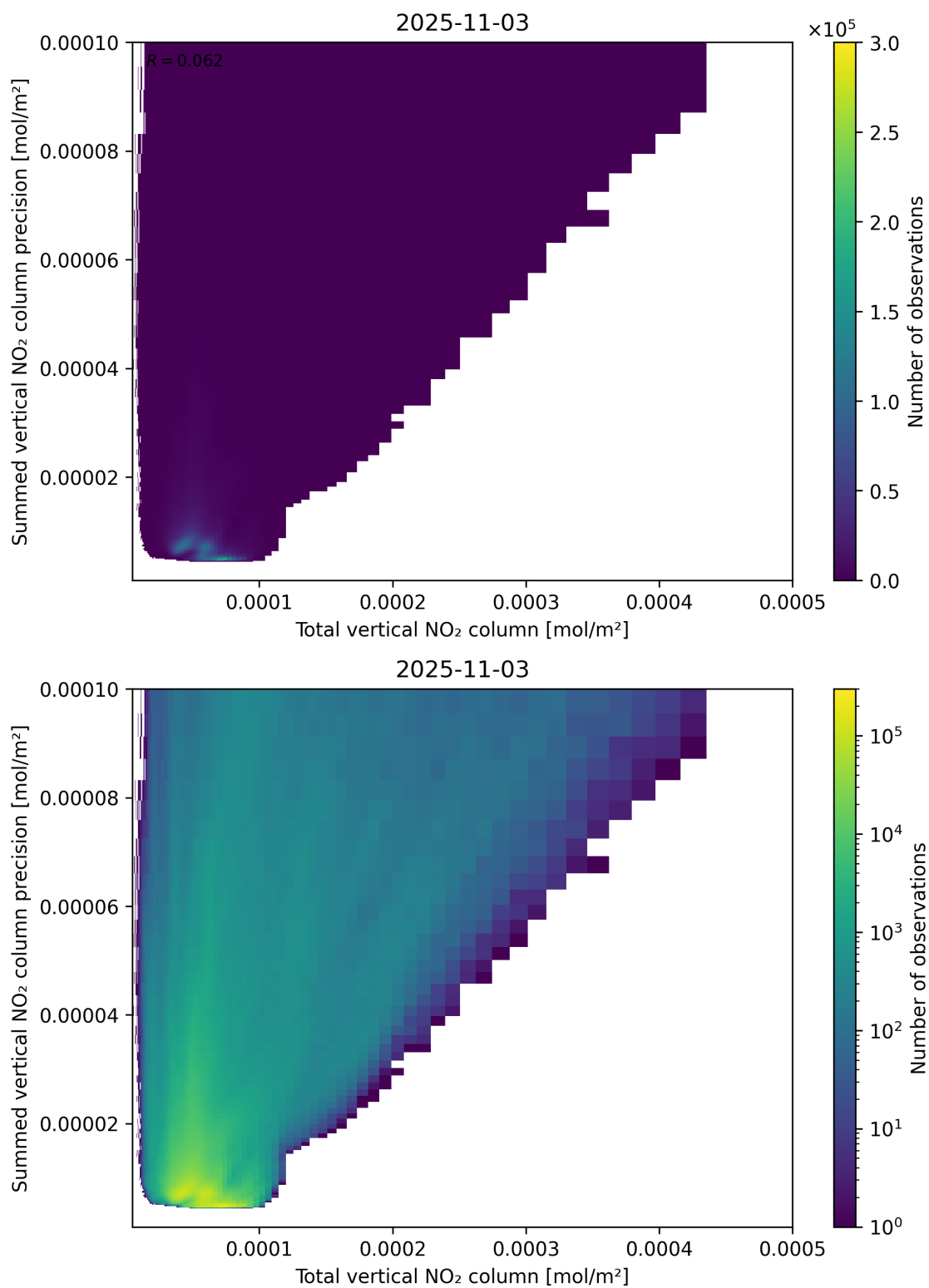
Figure 113: Scatter density plot of “Total vertical NO 2 column” against “Summed vertical NO 2 column precision” for 2025-11-02 to 2025-11-04.
