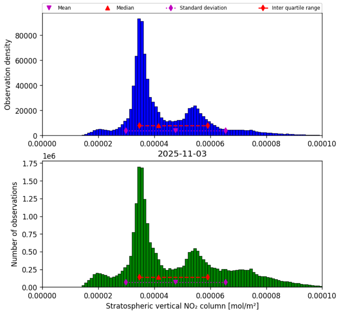
Figure 36: Histogram of “Stratospheric vertical NO 2 column” for 2025-11-02 to 2025-11-04
