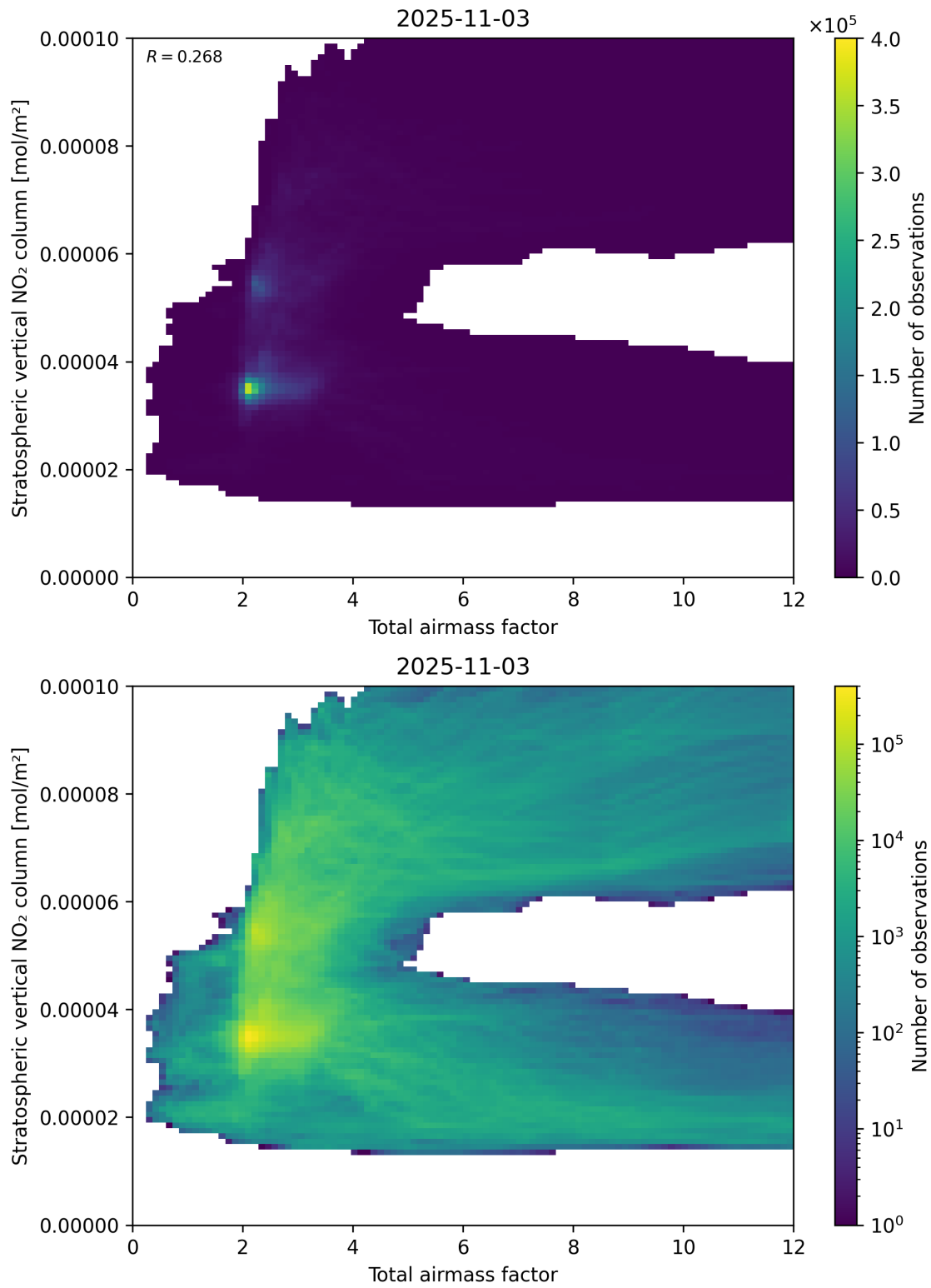
Figure 64: Scatter density plot of “Total airmass factor” against “Stratospheric vertical NO 2 column” for 2025-11-02 to 2025-11-04.
