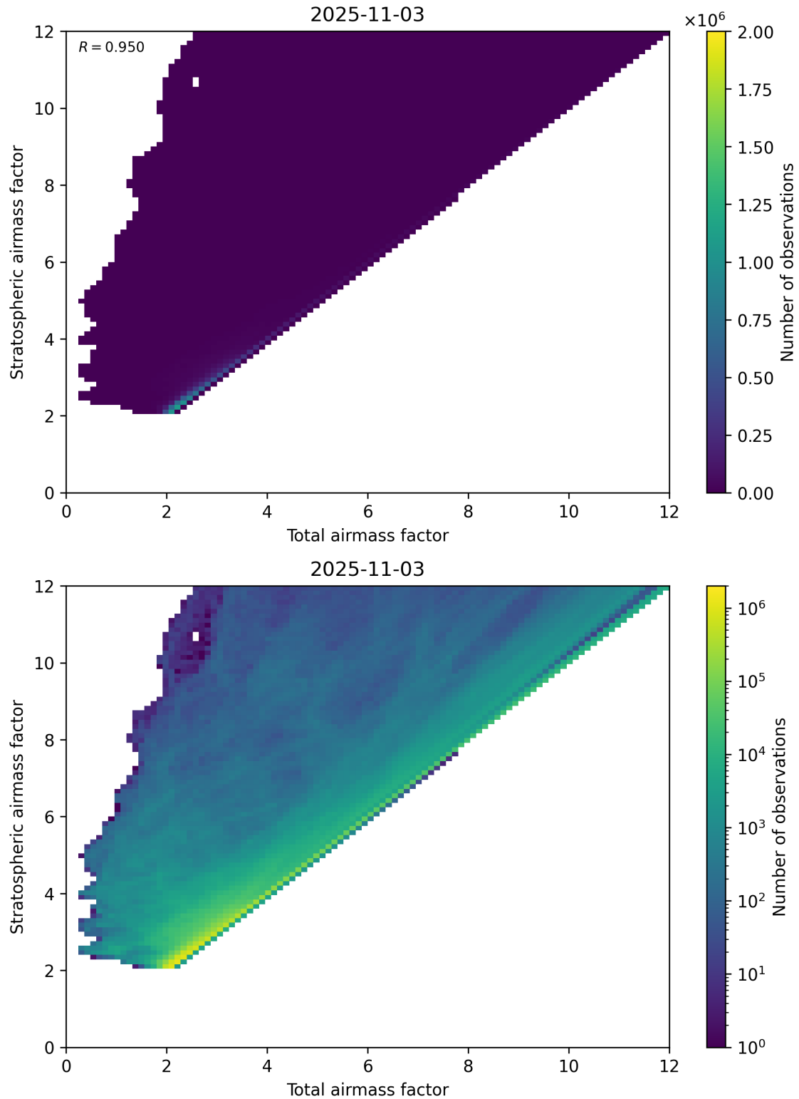
Figure 62: Scatter density plot of “Total airmass factor” against “Stratospheric airmass factor” for 2025-11-02 to 2025-11-04.
