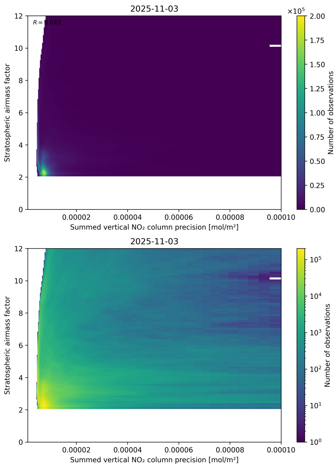
Figure 106: Scatter density plot of “Summed vertical NO 2 column precision” against “Stratospheric airmass factor” for 2025-11-02 to 2025-11-04.
