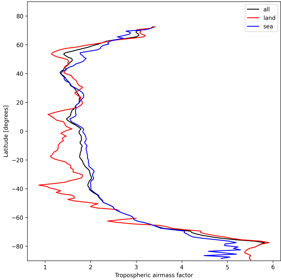
Figure 14: Zonal average of “Tropospheric airmass factor” for 2025-11-02 to 2025-11-04.
