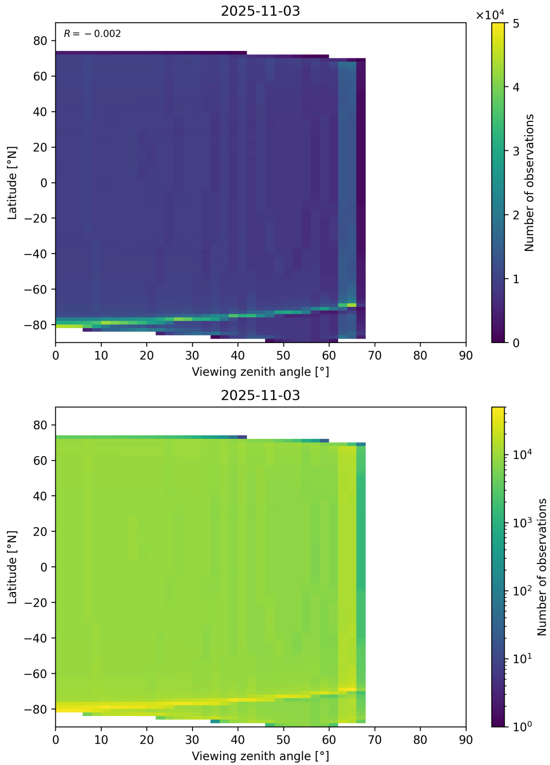
Figure 163: Scatter density plot of “Viewing zenith angle” against “Latitude” for 2025-11-02 to 2025-11-04.
