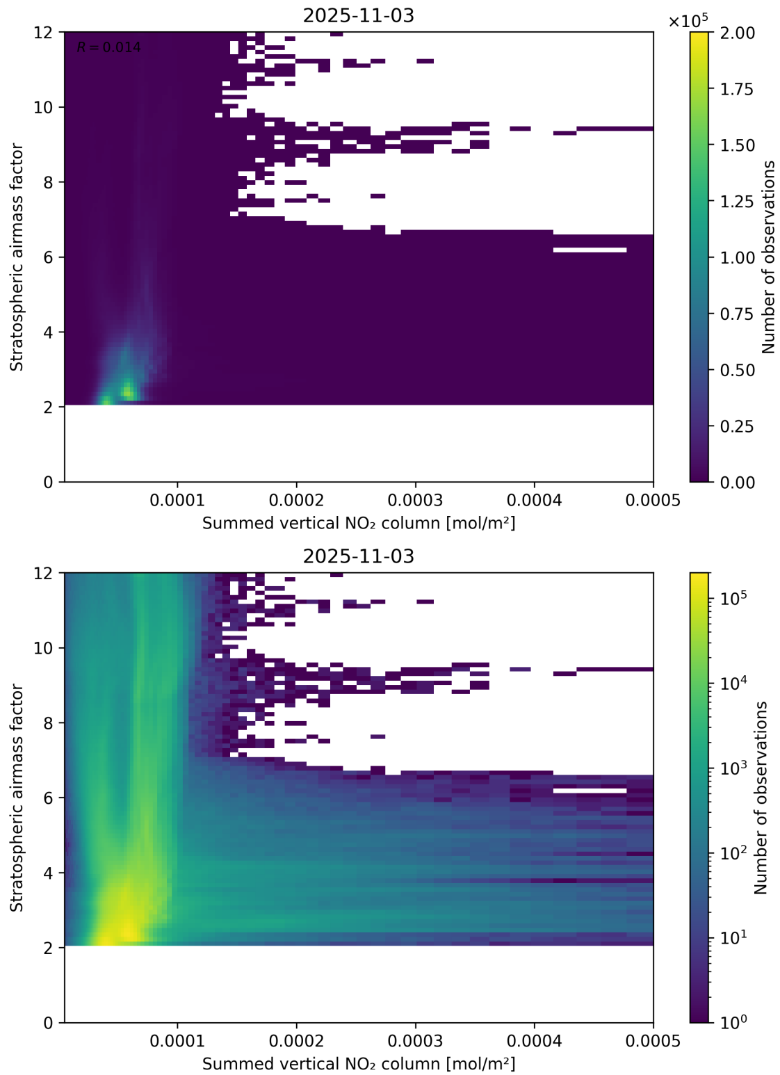
Figure 103: Scatter density plot of “Summed vertical NO 2 column” against “Stratospheric air mass factor” for 2025-11-02 to 2025-11-04.
