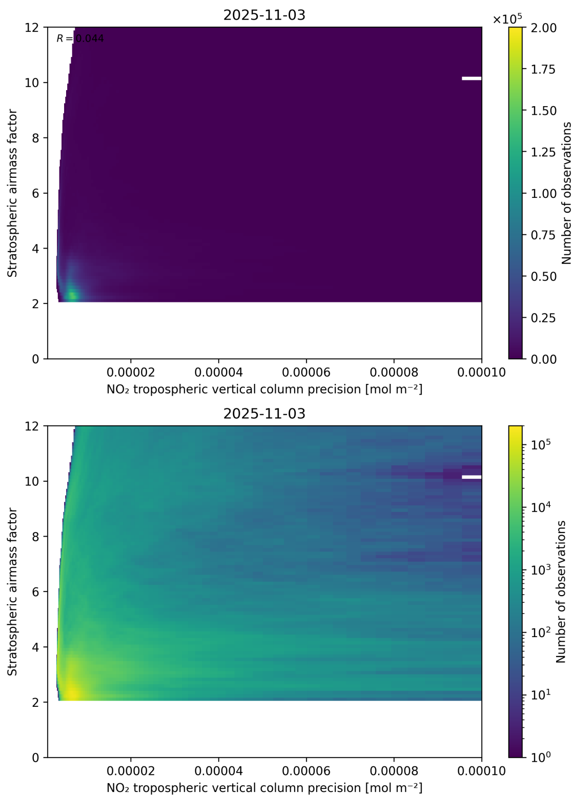
Figure 131: Scatter density plot of “NO 2 tropospheric vertical column precision” against “Stratospheric airmass factor” for 2025-11-02 to 2025-11-04.
