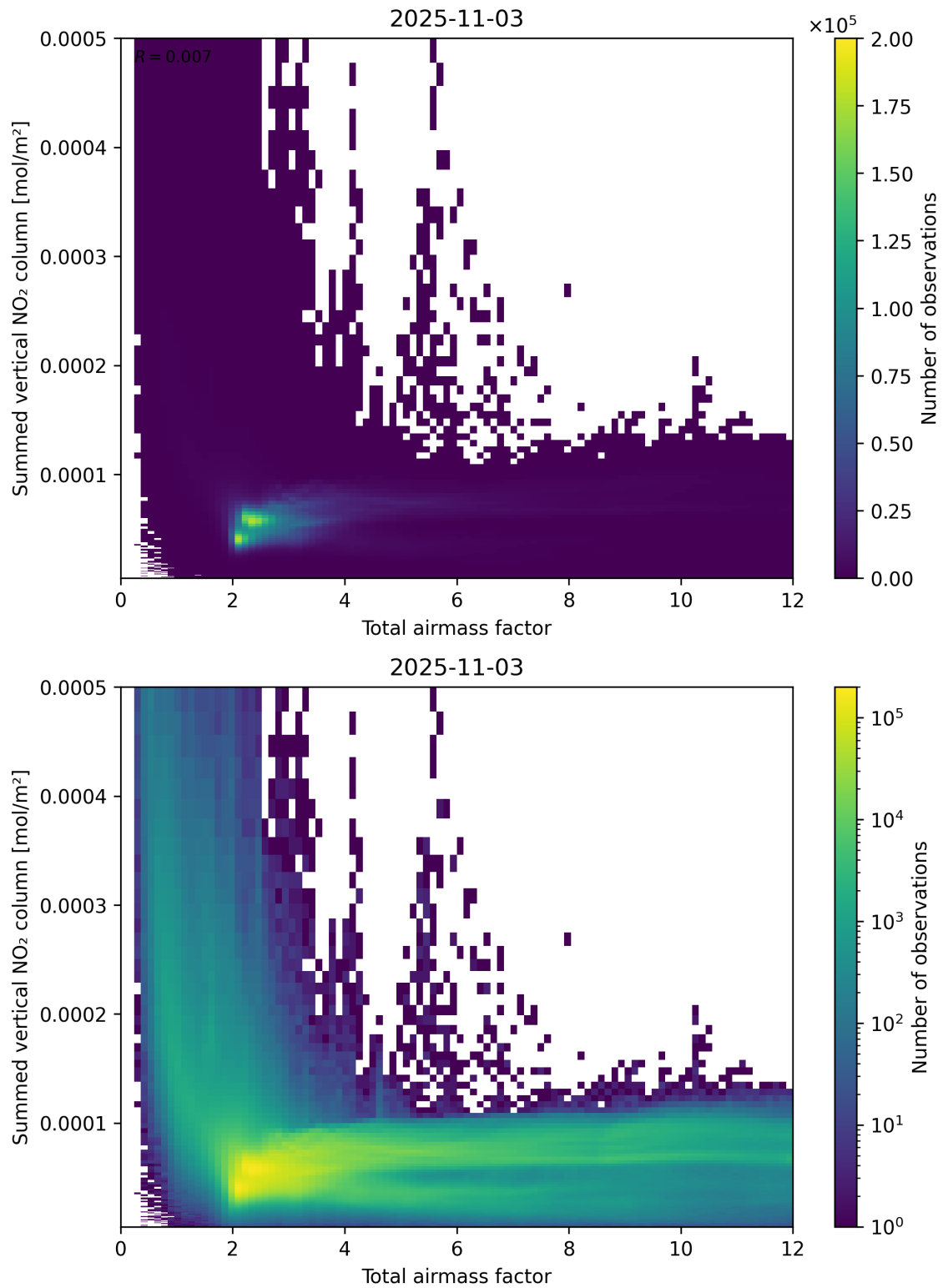
Figure 65: Scatter density plot of “Total airmass factor” against “Summed vertical NO 2 column” for 2025-11-02 to 2025-11-04.
