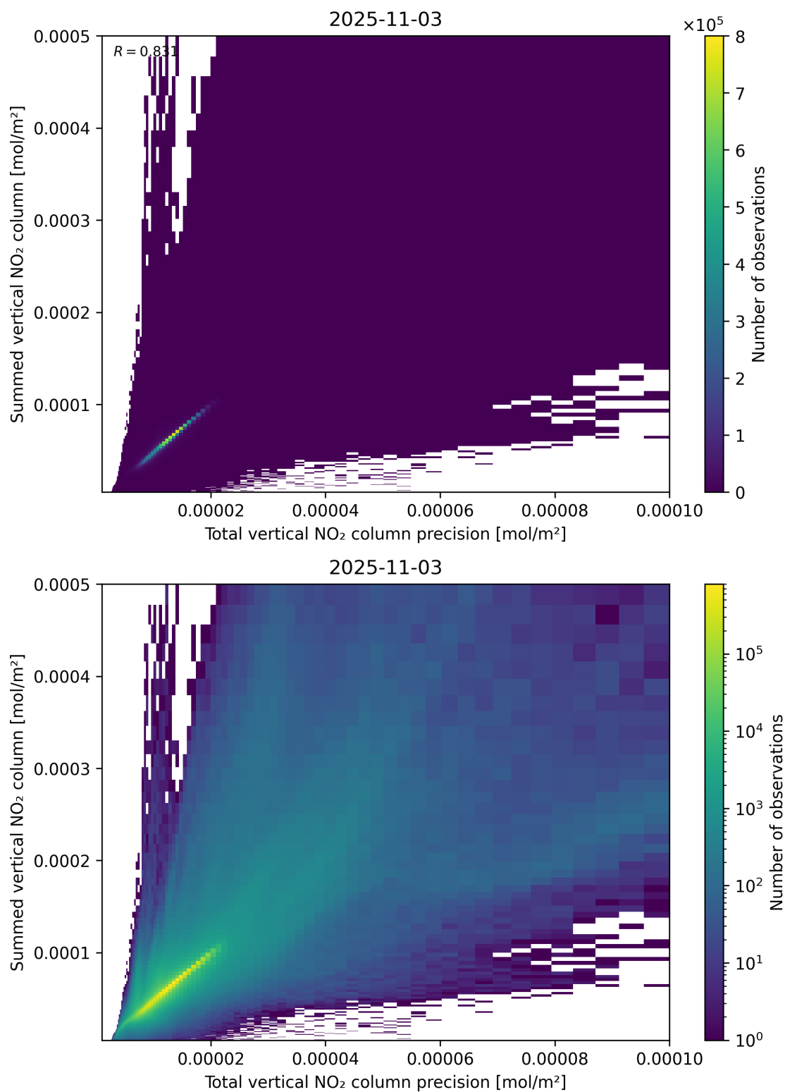
Figure 117: Scatter density plot of “Total vertical NO 2 column precision” against “Summed vertical NO 2 column” for 2025-11-02 to 2025-11-04.
