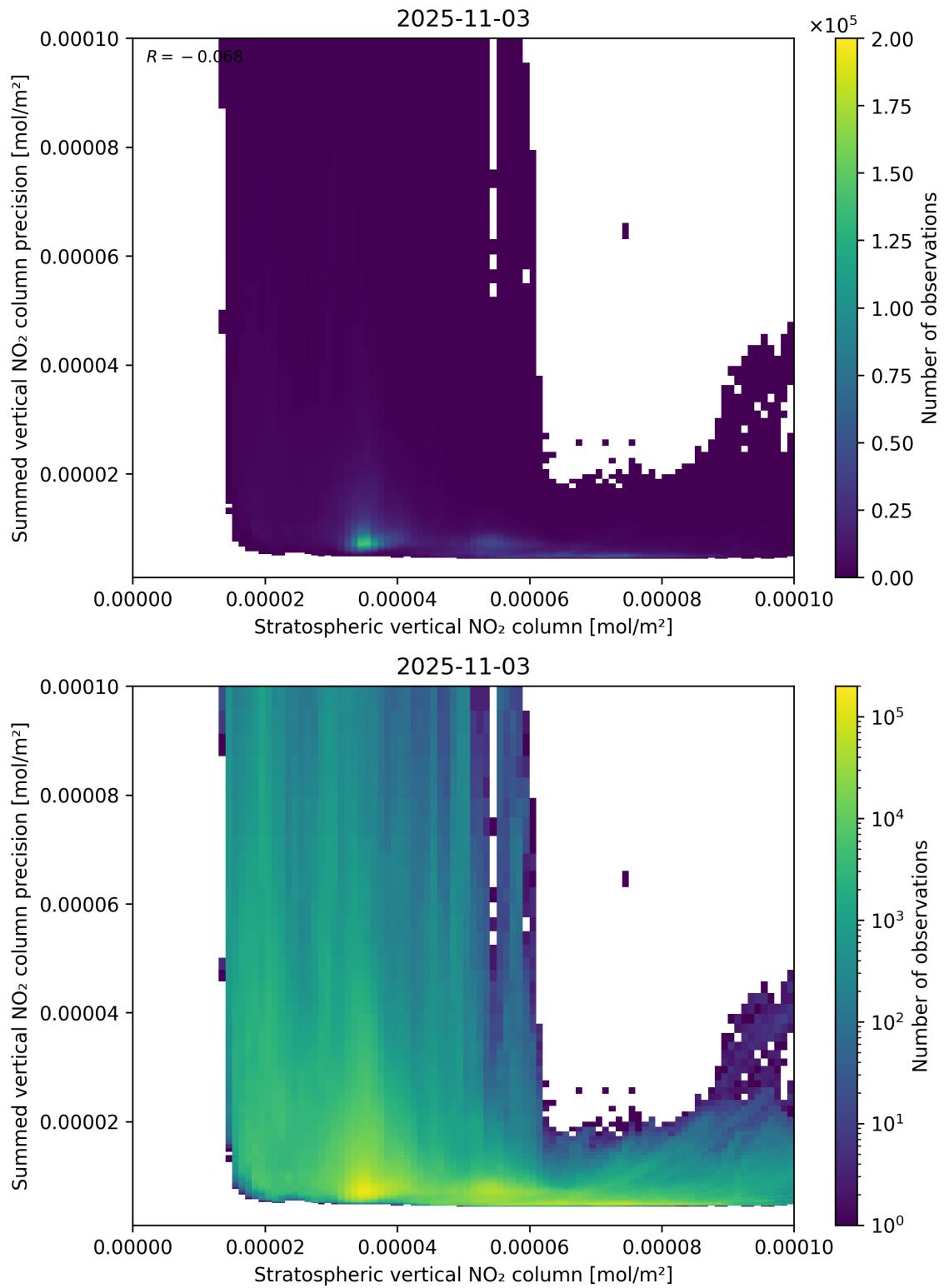
Figure 99: Scatter density plot of “Stratospheric vertical NO 2 column” against “Summed vertical NO 2 column precision” for 2025-11-02 to 2025-11-04.
