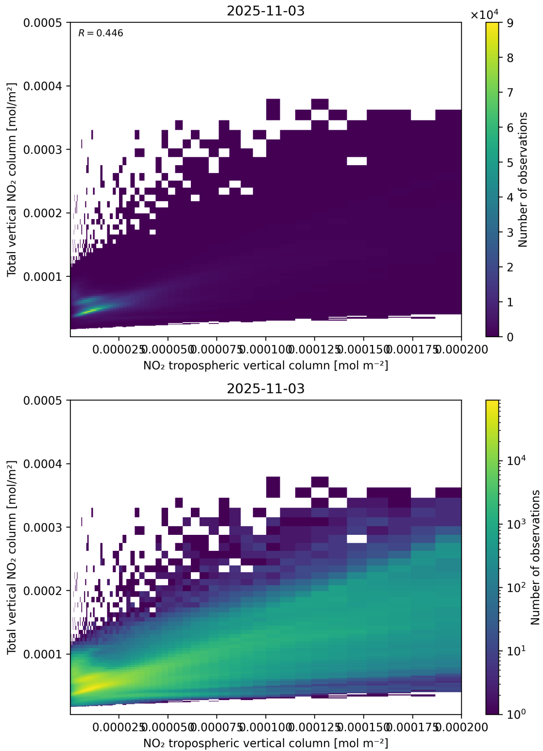
Figure 128: Scatter density plot of “NO 2 tropospheric vertical column” against “Total vertical NO 2 column” for 2025-11-02 to 2025-11-04.
