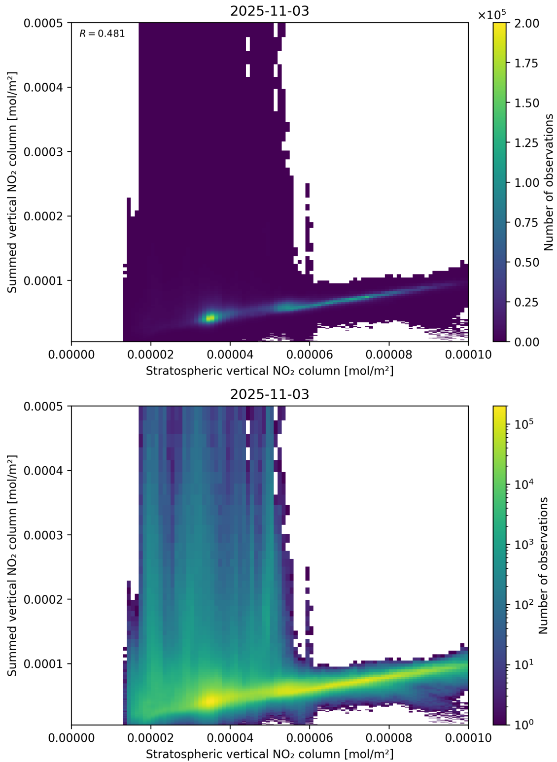
Figure 98: Scatter density plot of “Stratospheric vertical NO 2 column” against “Summed vertical NO 2 column” for 2025-11-02 to 2025-11-04.
