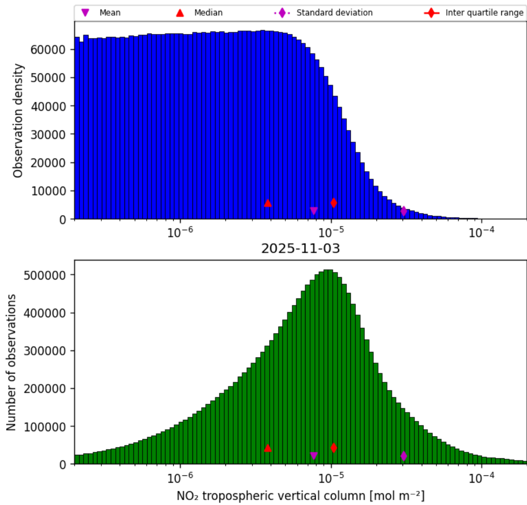
Figure 29: Histogram of “NO 2 tropospheric vertical column” for 2025-11-02 to 2025-11-04
