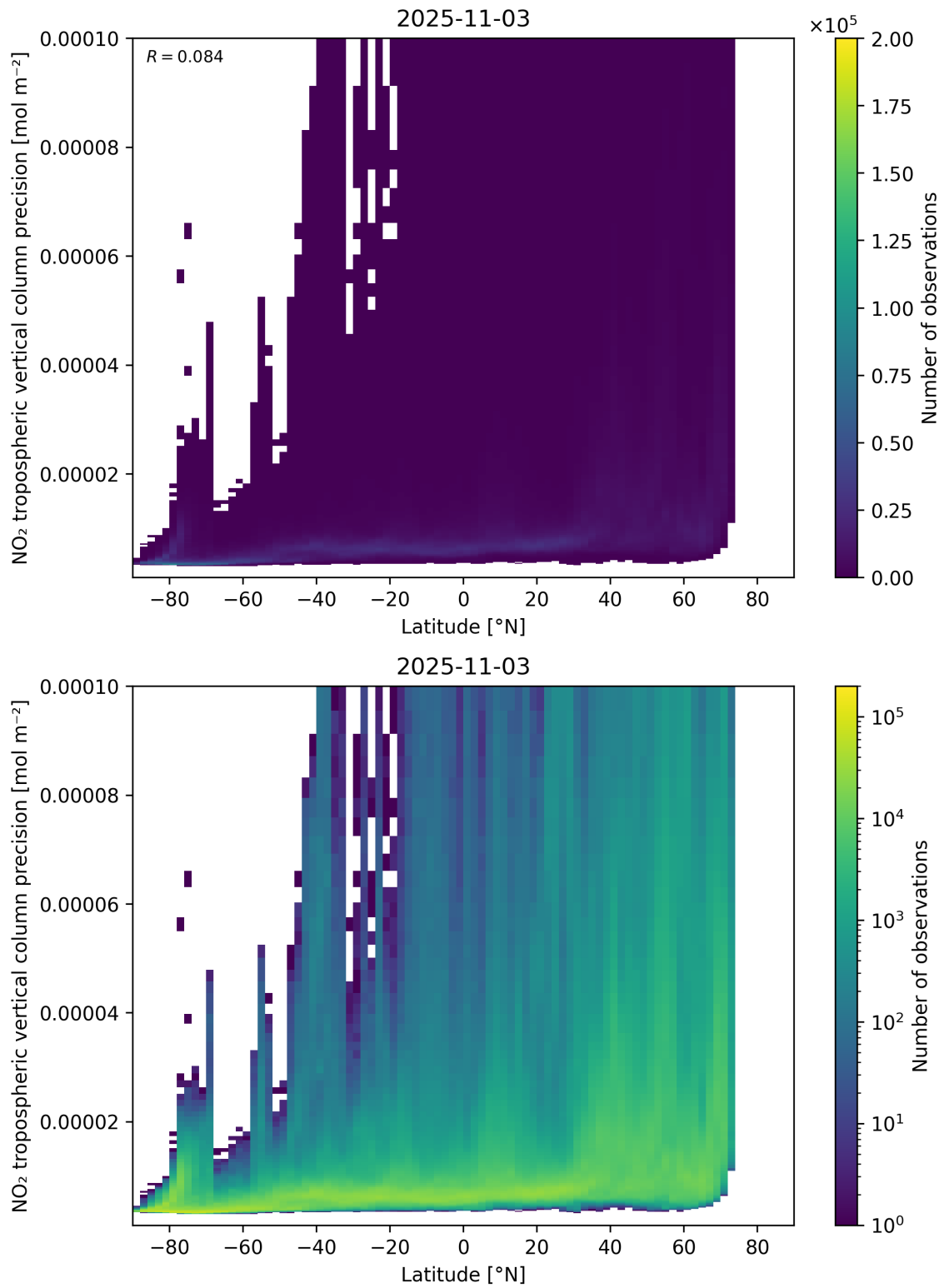
Figure 93: Scatter density plot of “Latitude” against “NO 2 tropospheric vertical column precision” for 2025-11-02 to 2025-11-04.
