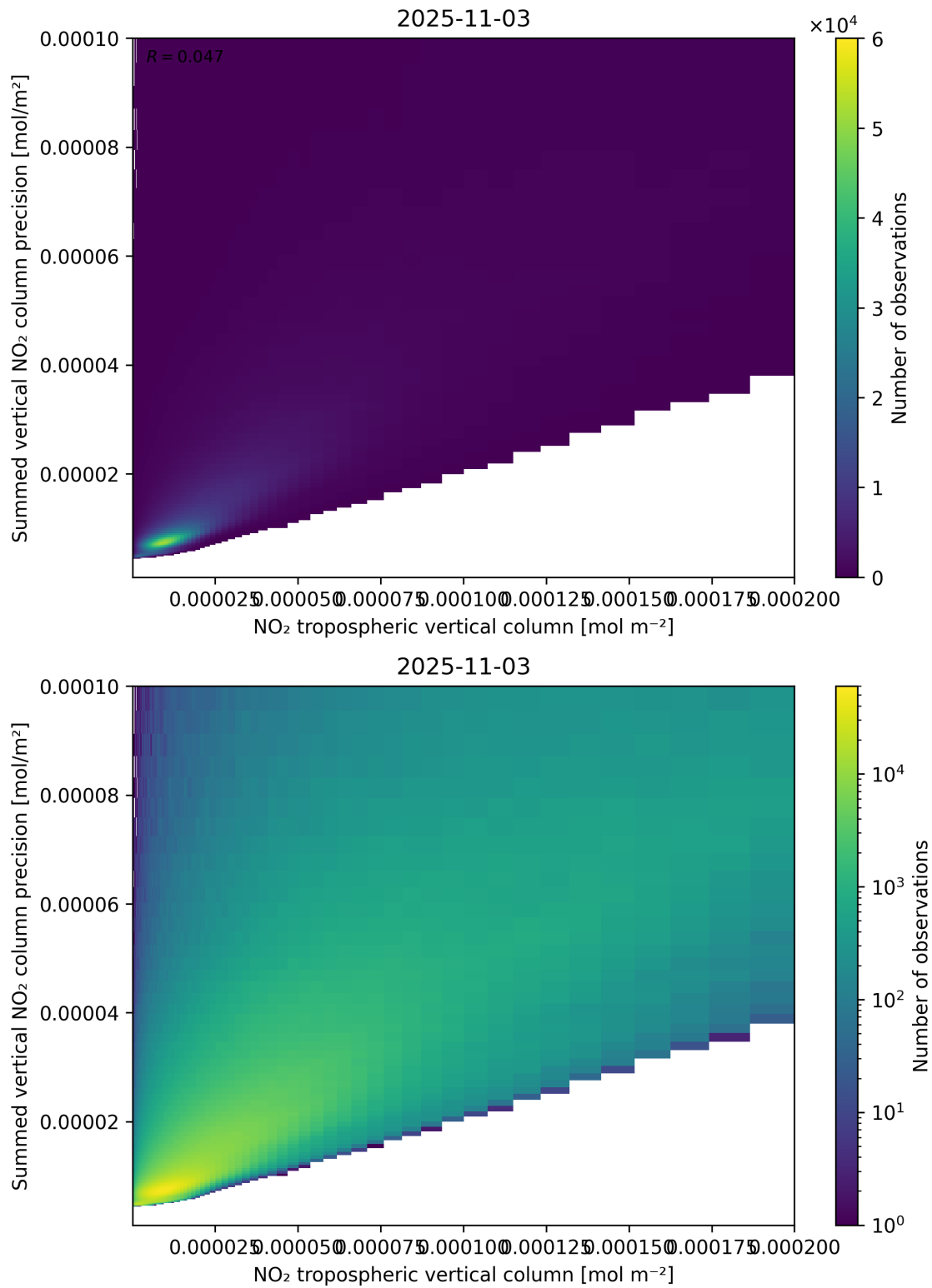
Figure 127: Scatter density plot of “NO 2 tropospheric vertical column” against “Summed vertical NO 2 column precision” for 2025-11-02 to 2025-11-04.
