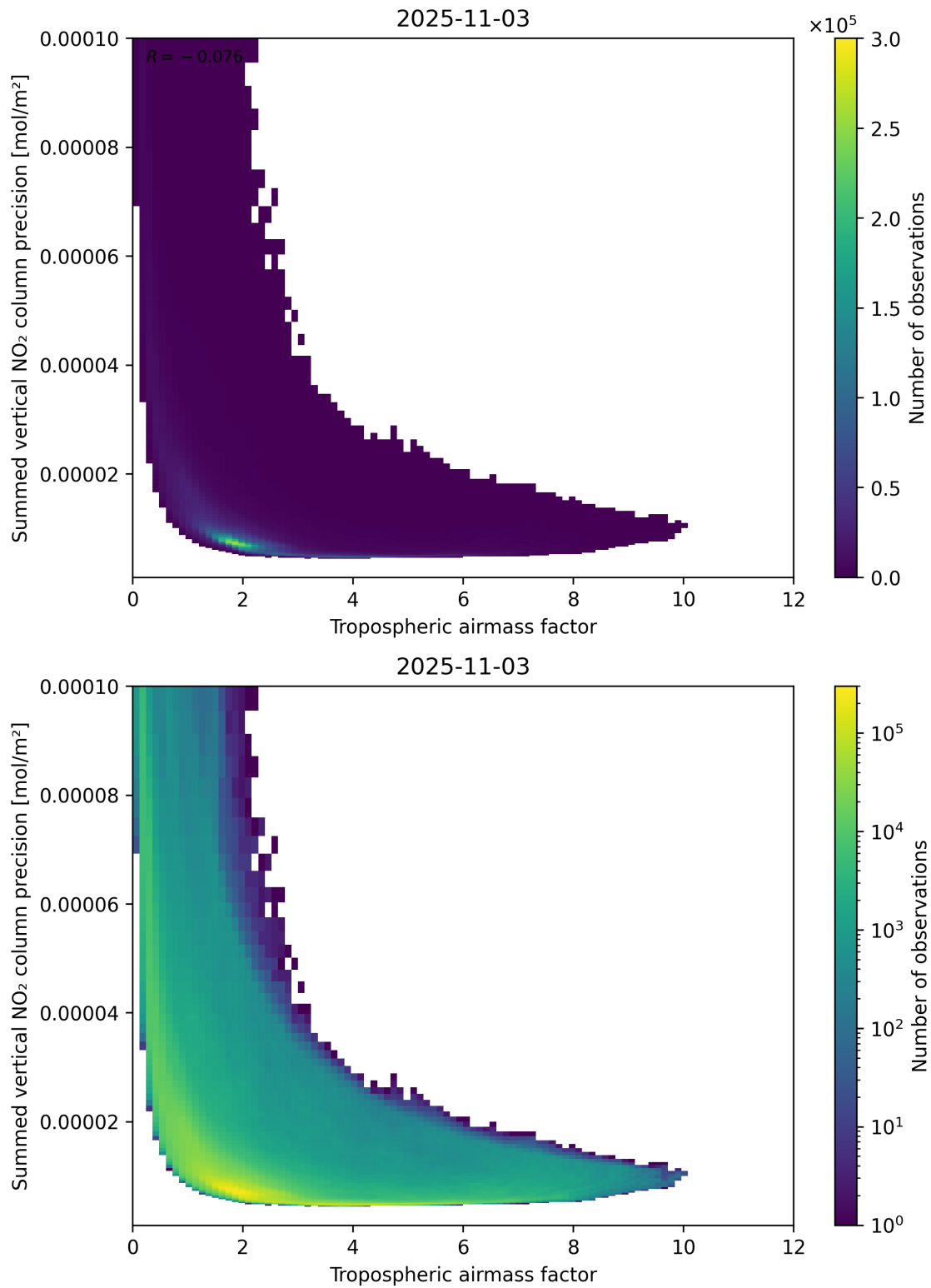
Figure 76: Scatter density plot of “Tropospheric air mass factor” against “Summed vertical NO 2 column precision” for 2025-11-02 to 2025-11-04.
