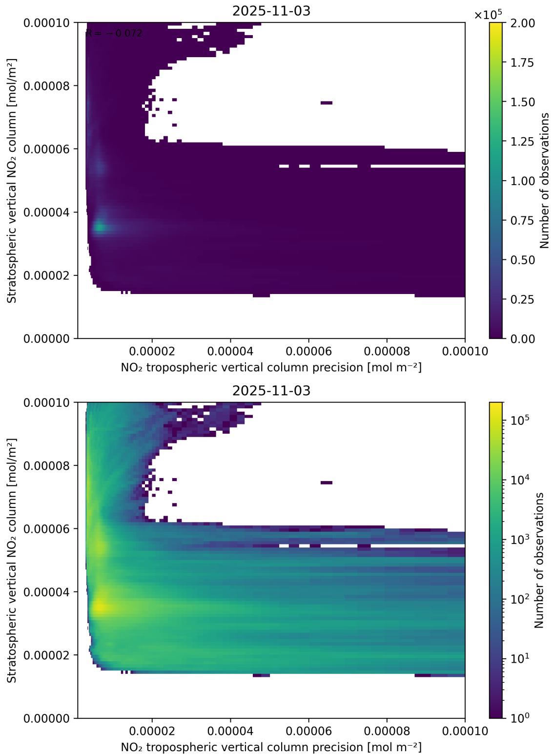
Figure 135: Scatter density plot of “NO 2 tropospheric vertical column precision” against “Stratospheric vertical NO 2 column” for 2025-11-02 to 2025-11-04.
