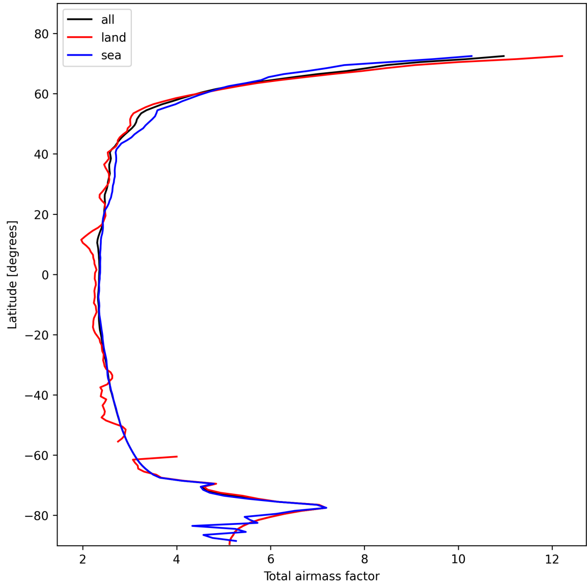
Figure 15: Zonal average of “Total airmass factor” for 2025-11-02 to 2025-11-04.
