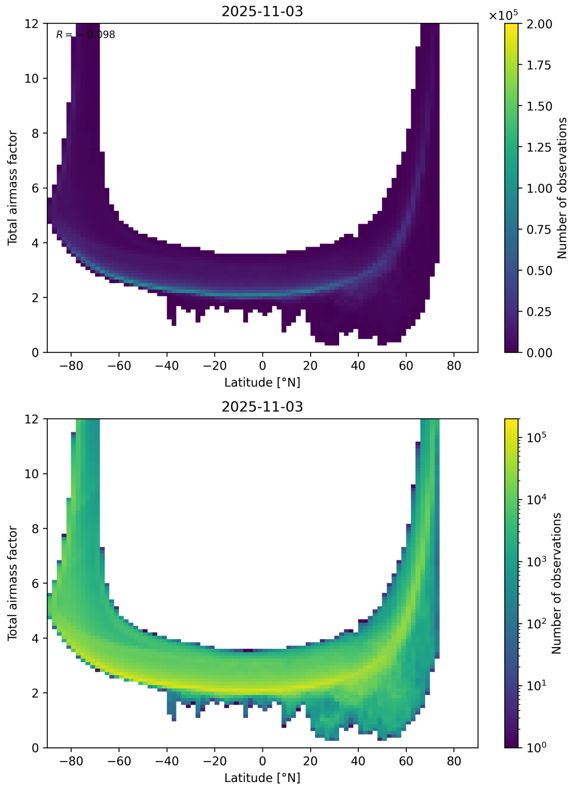
Figure 84: Scatter density plot of “Latitude” against “Total airmass factor” for 2025-11-02 to 2025-11-04.
