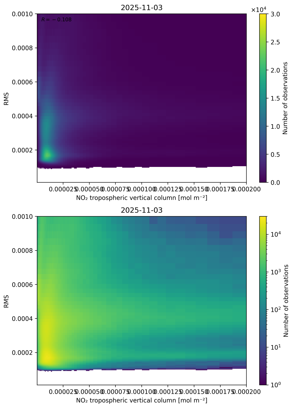
Figure 142: Scatter density plot of “NO 2 tropospheric vertical column” against “RMS” for 2025-11-02 to 2025-11-04.
