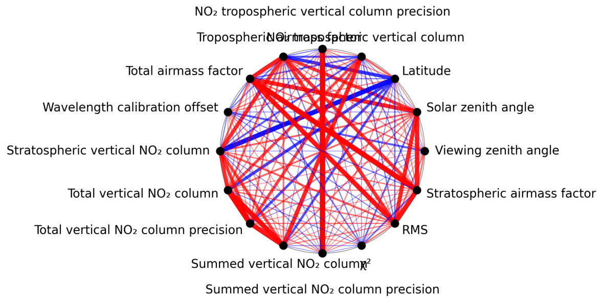
Figure 1: Map of correlation graph for 2025-11-02 to 2025-11-04.
