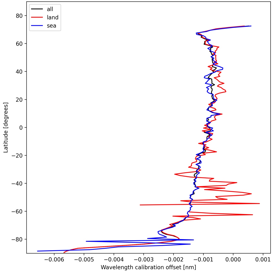
Figure 18: Zonal average of “Wavelength calibration offset” for 2025-11-02 to 2025-11-04.
