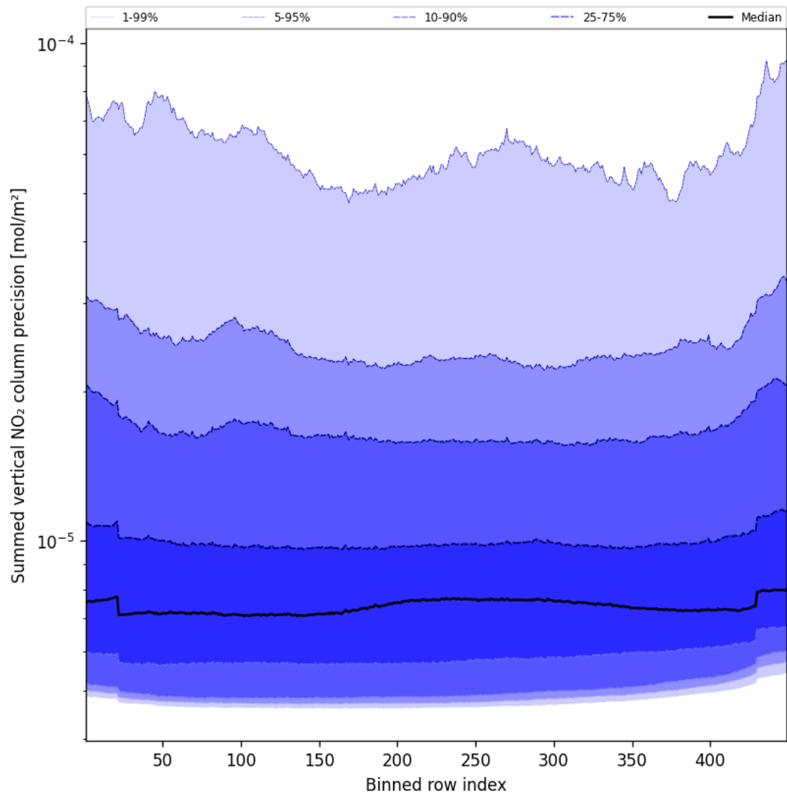
Figure 58: Along track statistics of “Summed vertical NO 2 column precision” for 2025-11-02 to 2025-11-04
