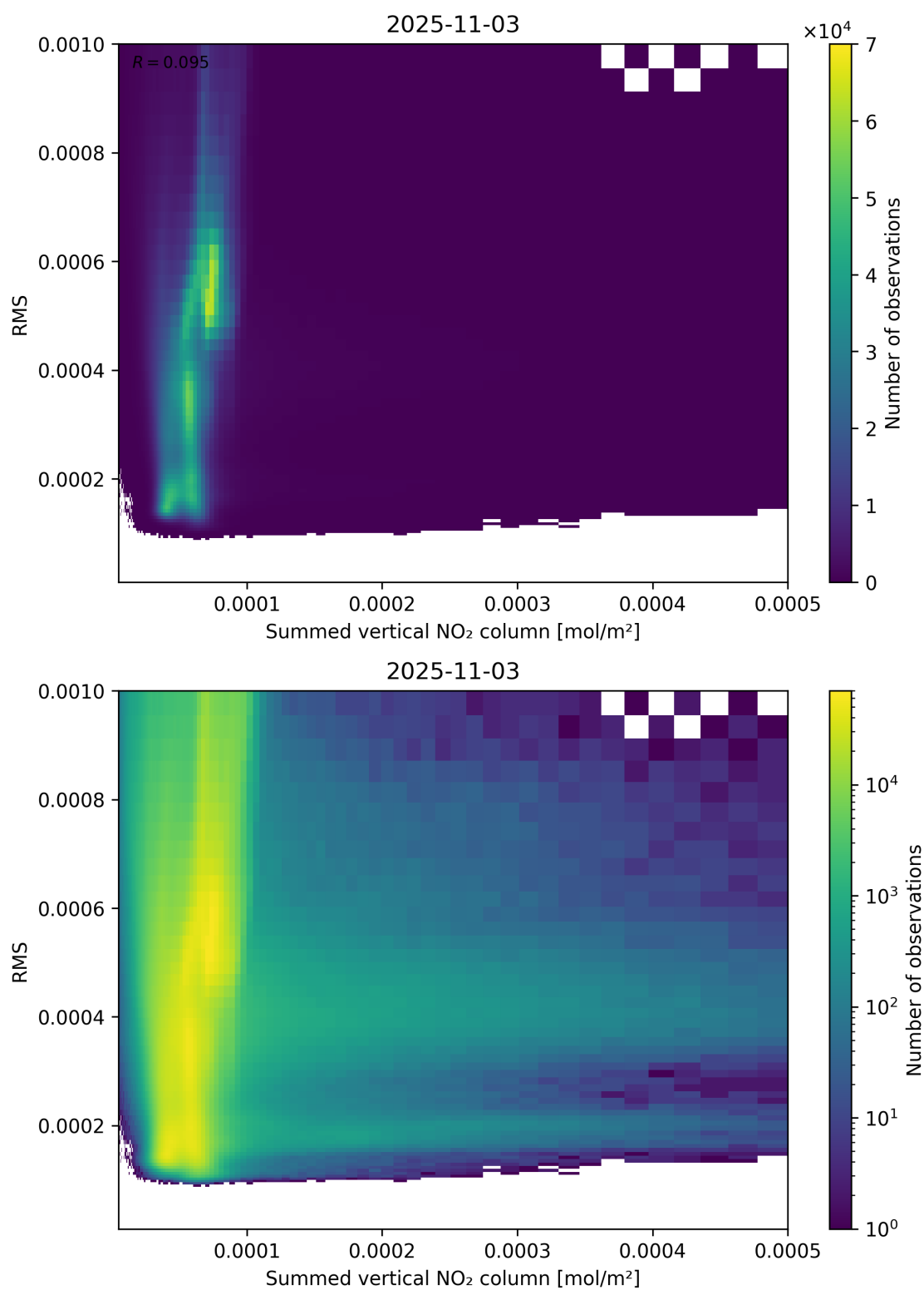
Figure 109: Scatter density plot of “Summed vertical NO 2 column” against “RMS” for 2025-11-02 to 2025-11-04.
