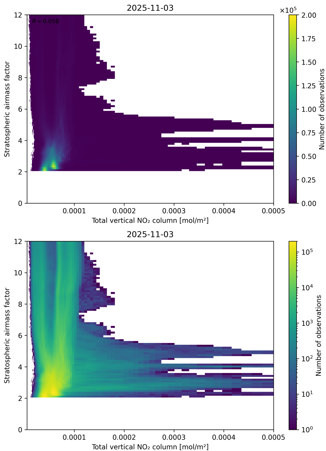
Figure 110: Scatter density plot of “Total vertical NO 2 column” against “Stratospheric airmass factor” for 2025-11-02 to 2025-11-04.
