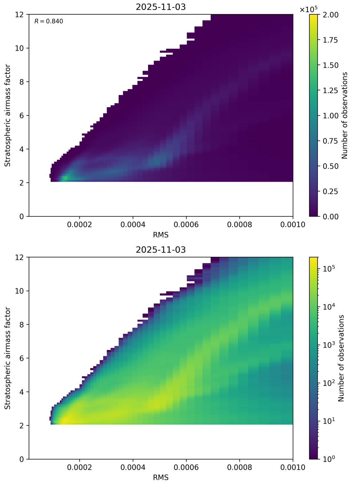
Figure 144: Scatter density plot of “RMS” against “Stratospheric airmass factor” for 2025-11-02 to 2025-11-04.
