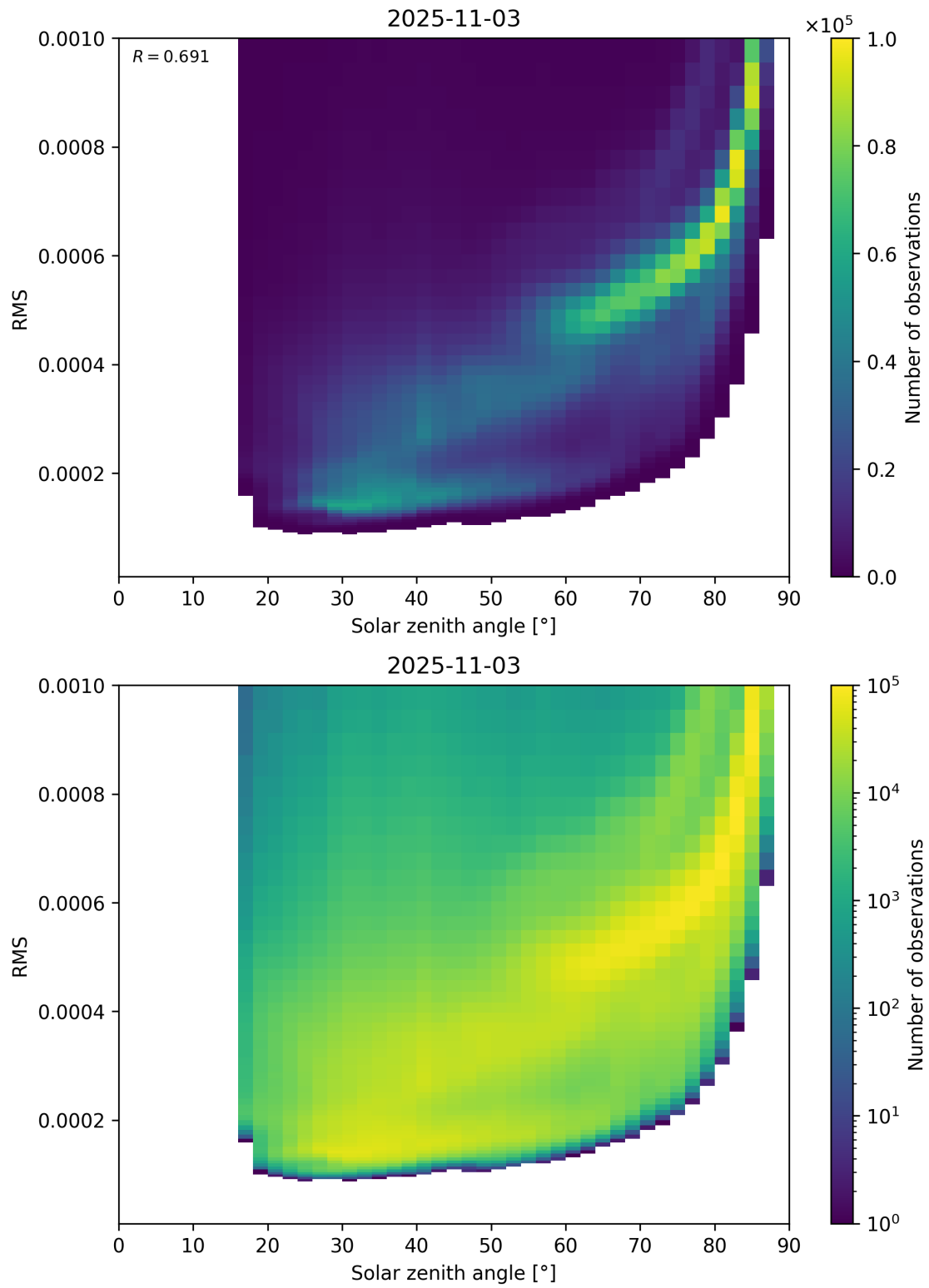
Figure 157: Scatter density plot of “Solar zenith angle” against “RMS” for 2025-11-02 to 2025-11-04.
