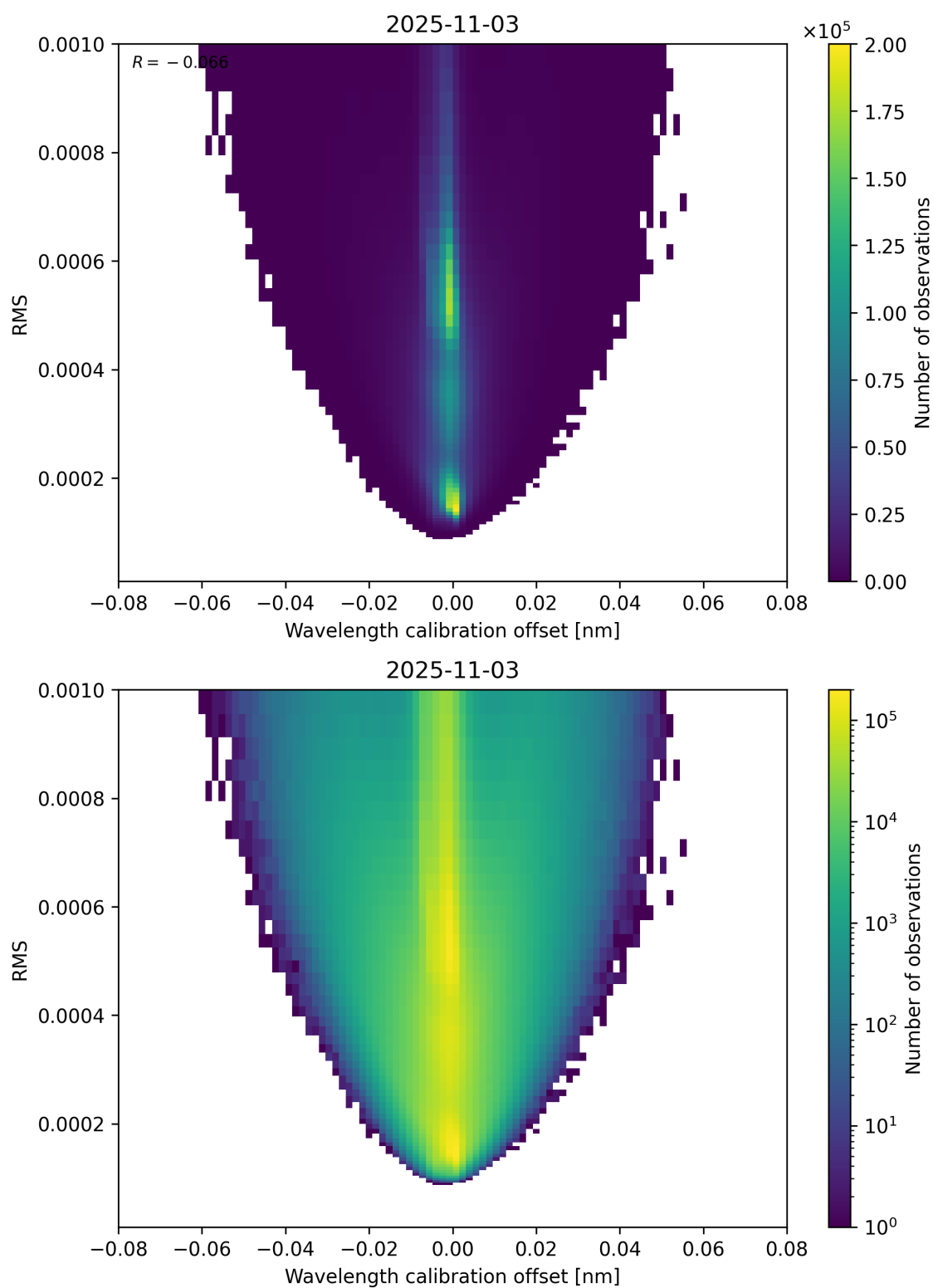
Figure 181: Scatter density plot of “Wavelength calibration offset” against “RMS” for 2025-11-02 to 2025-11-04.
