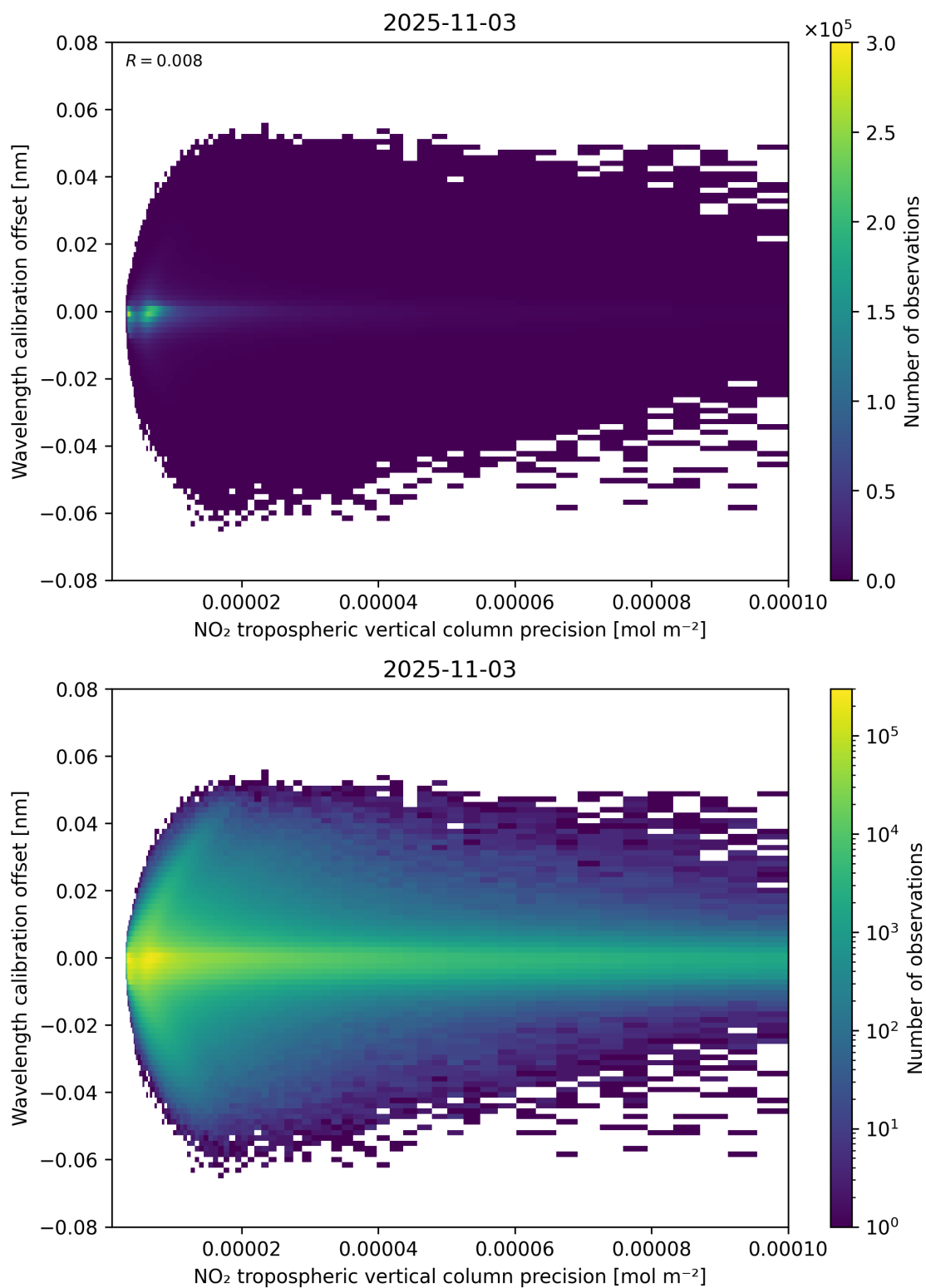
Figure 141: Scatter density plot of “NO 2 tropospheric vertical column precision” against “Wavelength calibration offset” for 2025-11-02 to 2025-11-04.
