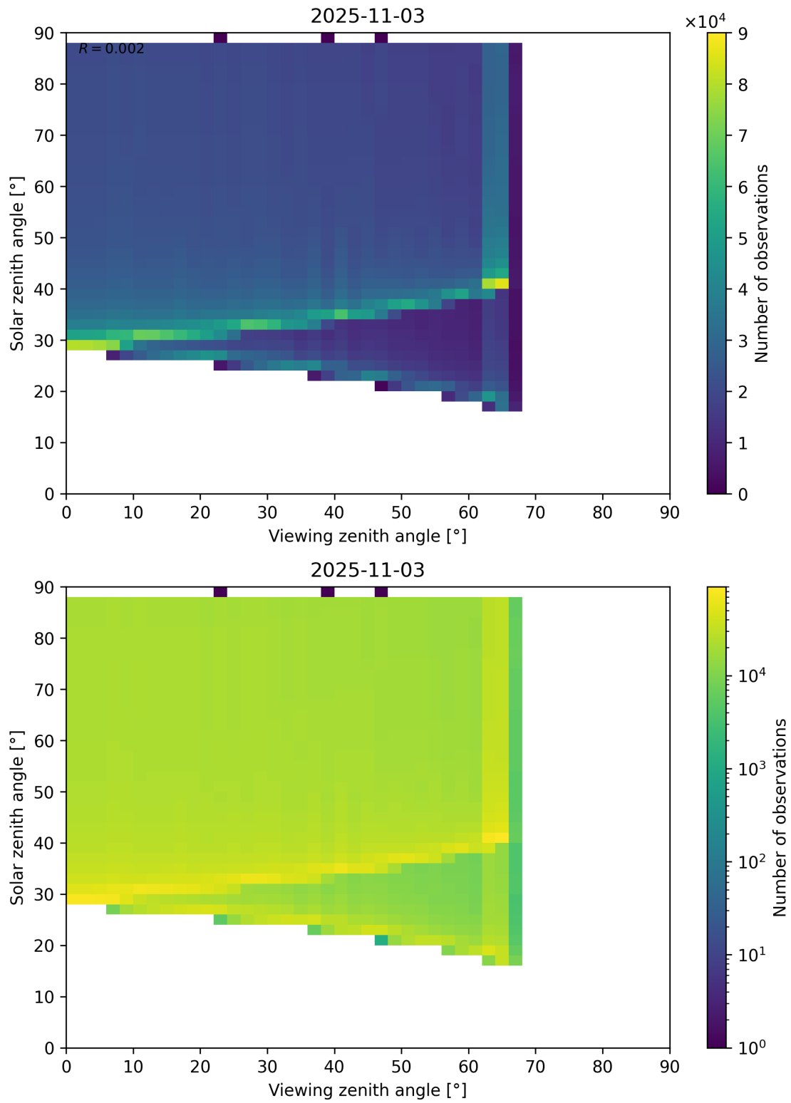
Figure 172: Scatter density plot of “Viewing zenith angle” against “Solar zenith angle” for 2025-11-02 to 2025-11-04.
