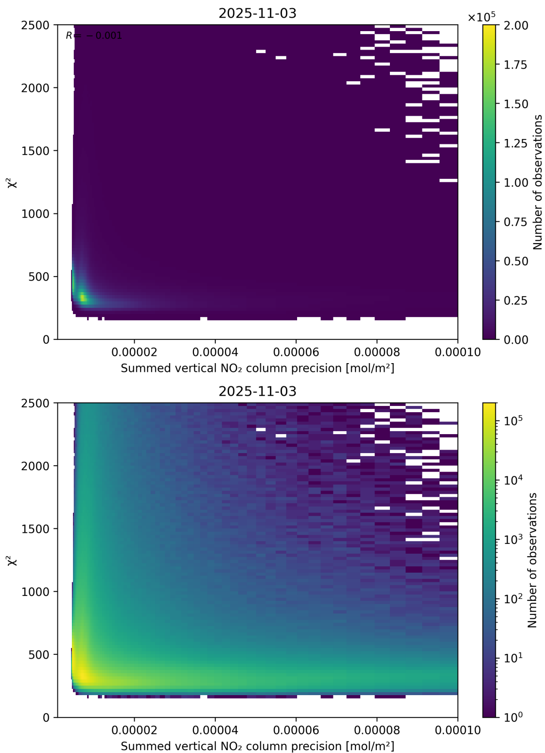
Figure 107: Scatter density plot of “Summed vertical NO 2 column precision” against “ \chi^2 ” for 2025-11-02 to 2025-11-04.
