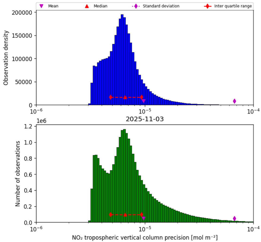
Figure 30: Histogram of “NO 2 tropospheric vertical column precision” for 2025-11-02 to 2025-11-04
