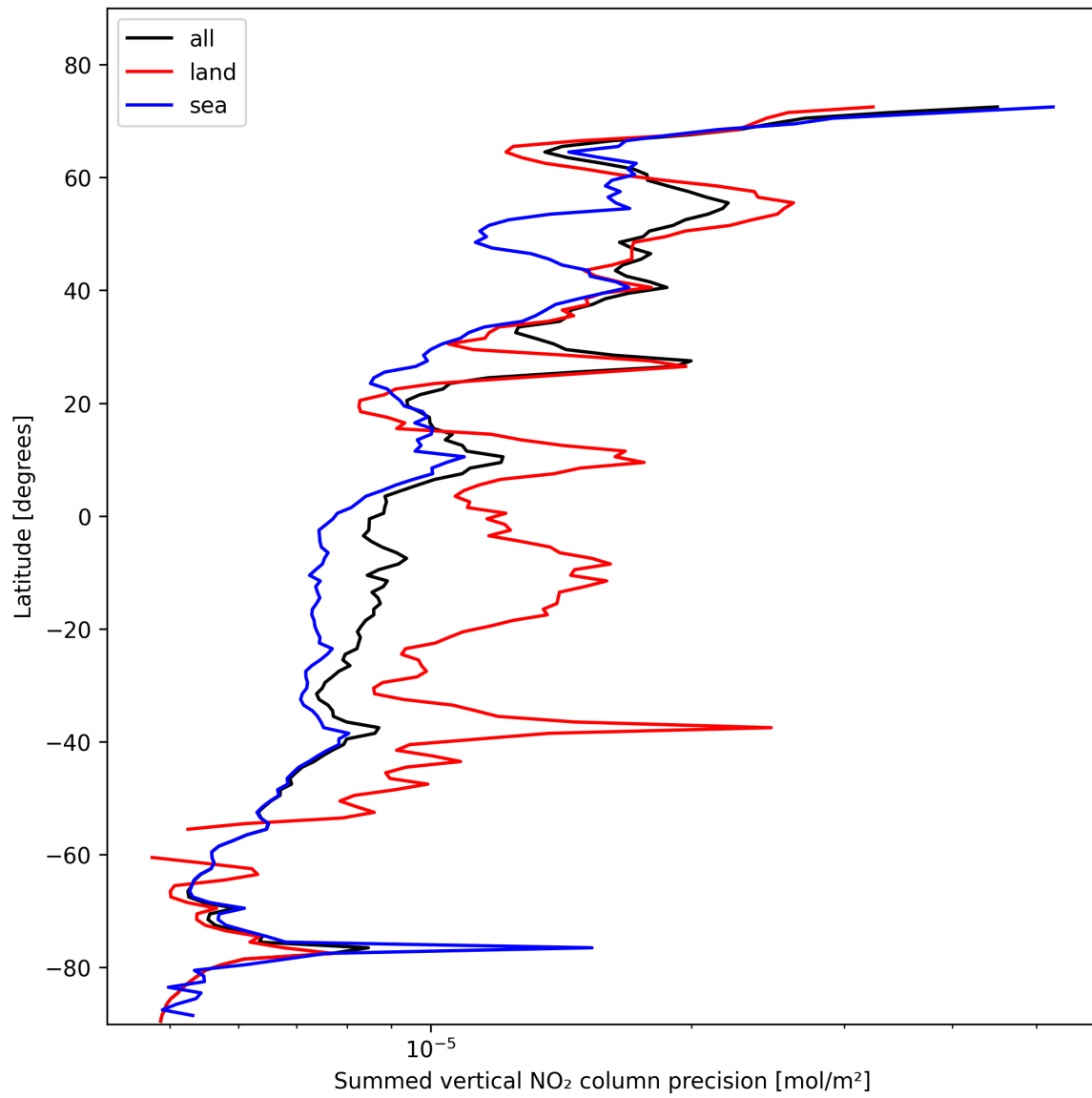
Figure 24: Zonal average of “Summed vertical NO 2 column precision” for 2025-11-02 to 2025-11-04.
