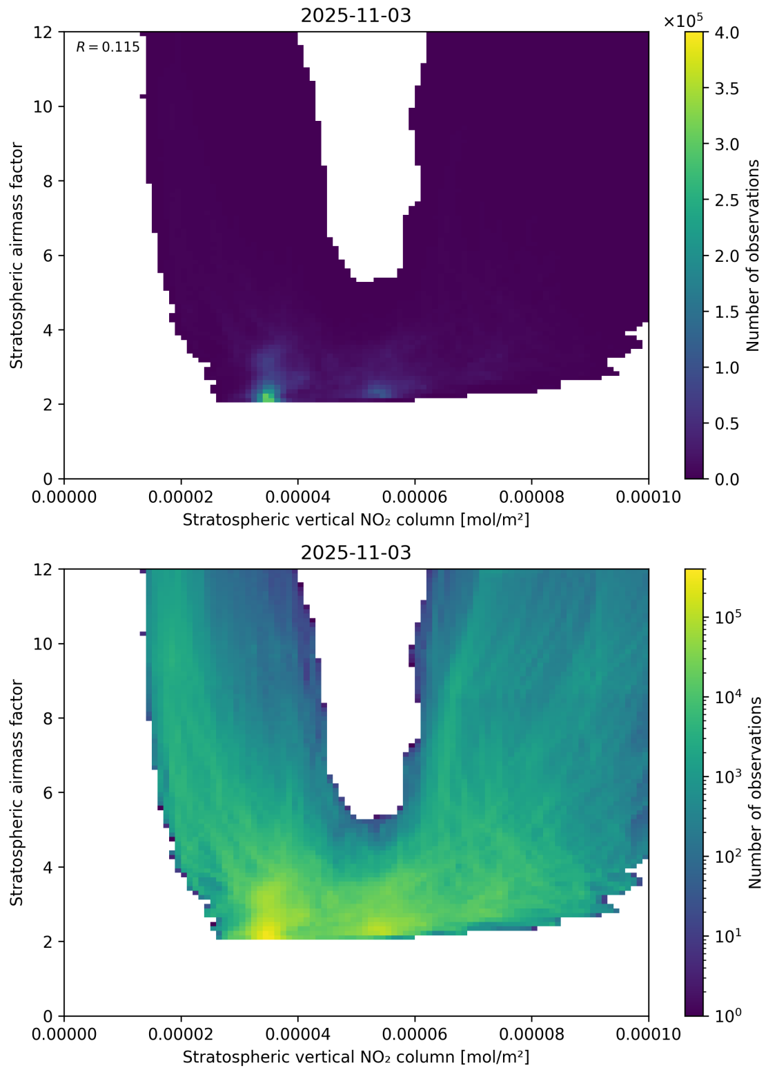
Figure 96: Scatter density plot of “Stratospheric vertical NO 2 column” against “Stratospheric airmass factor” for 2025-11-02 to 2025-11-04.
