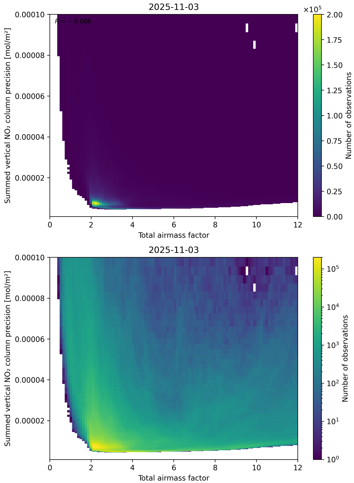
Figure 66: Scatter density plot of “Total airmass factor” against “Summed vertical NO 2 column precision” for 2025-11-02 to 2025-11-04.
