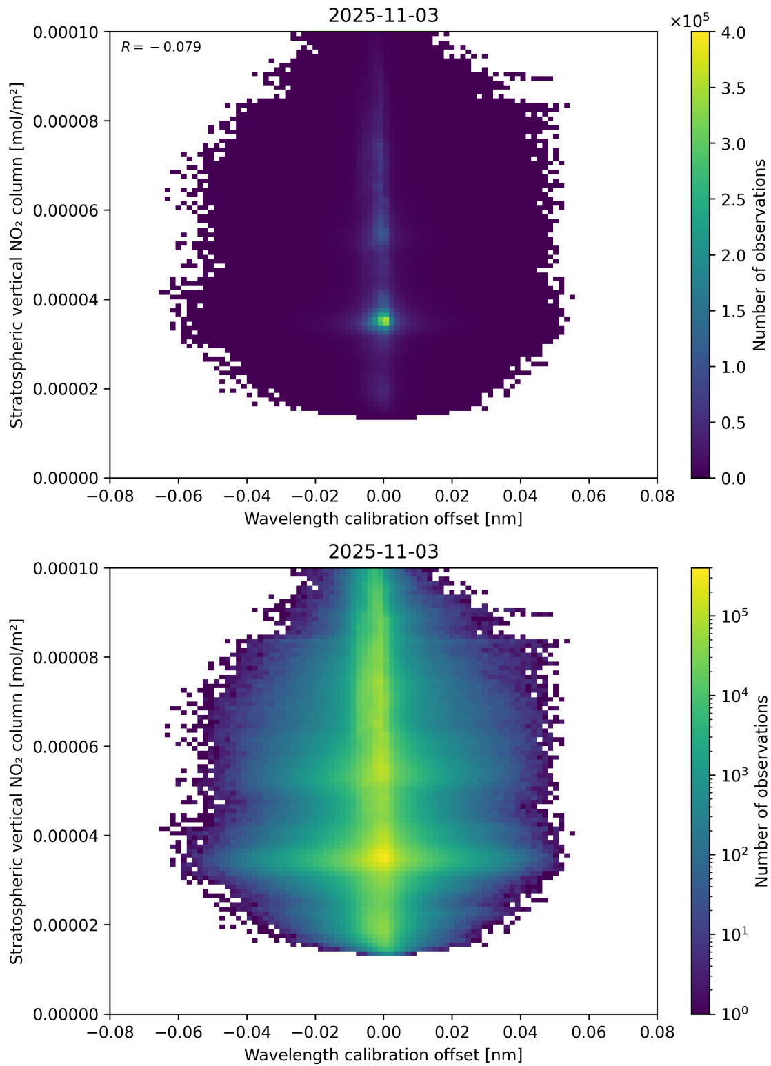
Figure 176: Scatter density plot of “Wavelength calibration offset” against “Stratospheric vertical NO 2 column” for 2025-11-02 to 2025-11-04.
