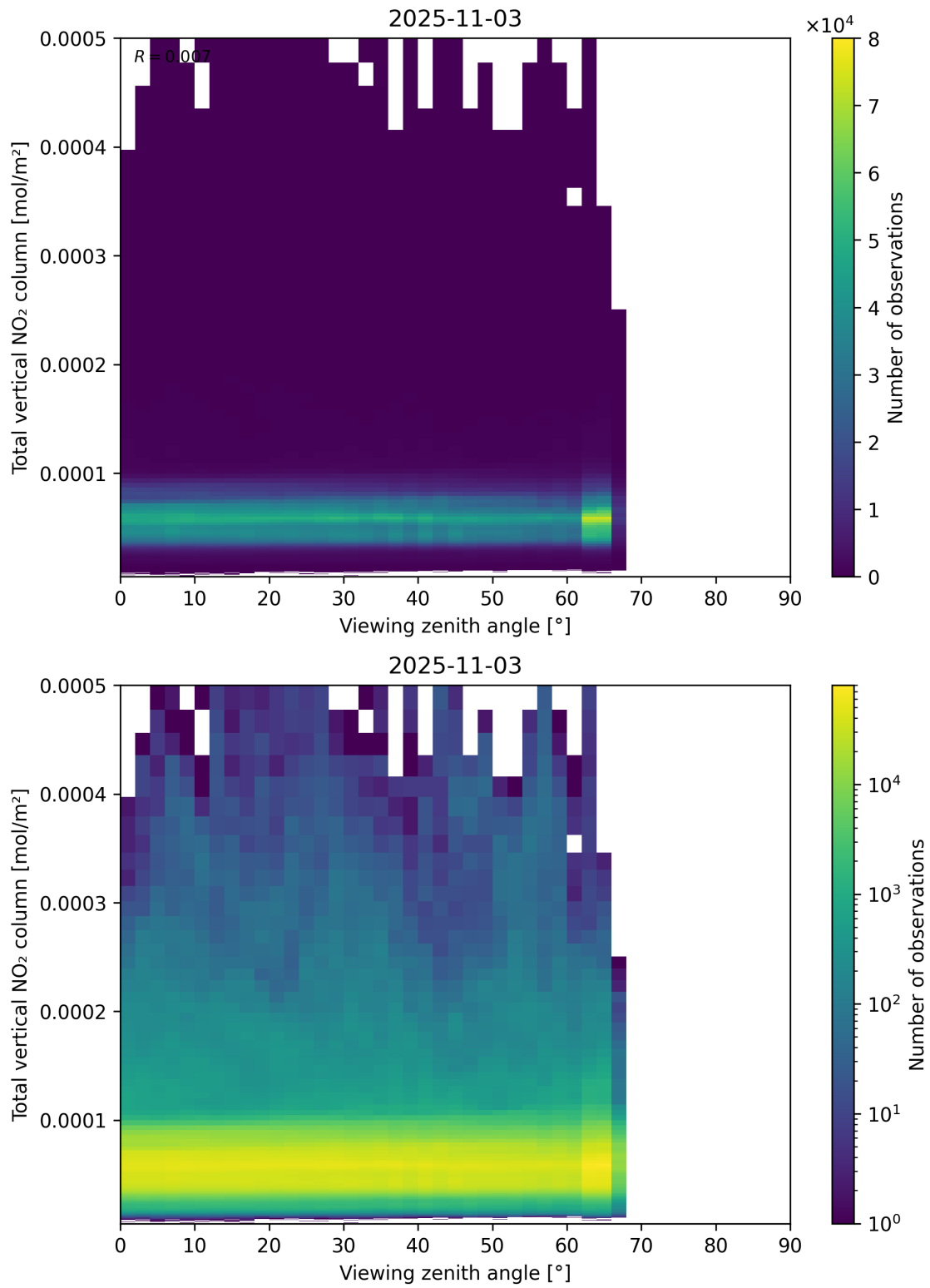
Figure 167: Scatter density plot of “Viewing zenith angle” against “Total vertical NO 2 column” for 2025-11-02 to 2025-11-04.
