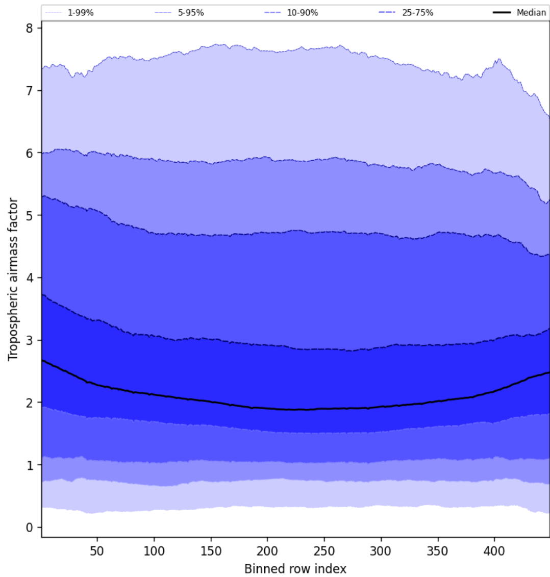
Figure 48: Along track statistics of “Tropospheric air mass factor” for 2025-11-02 to 2025-11-04
