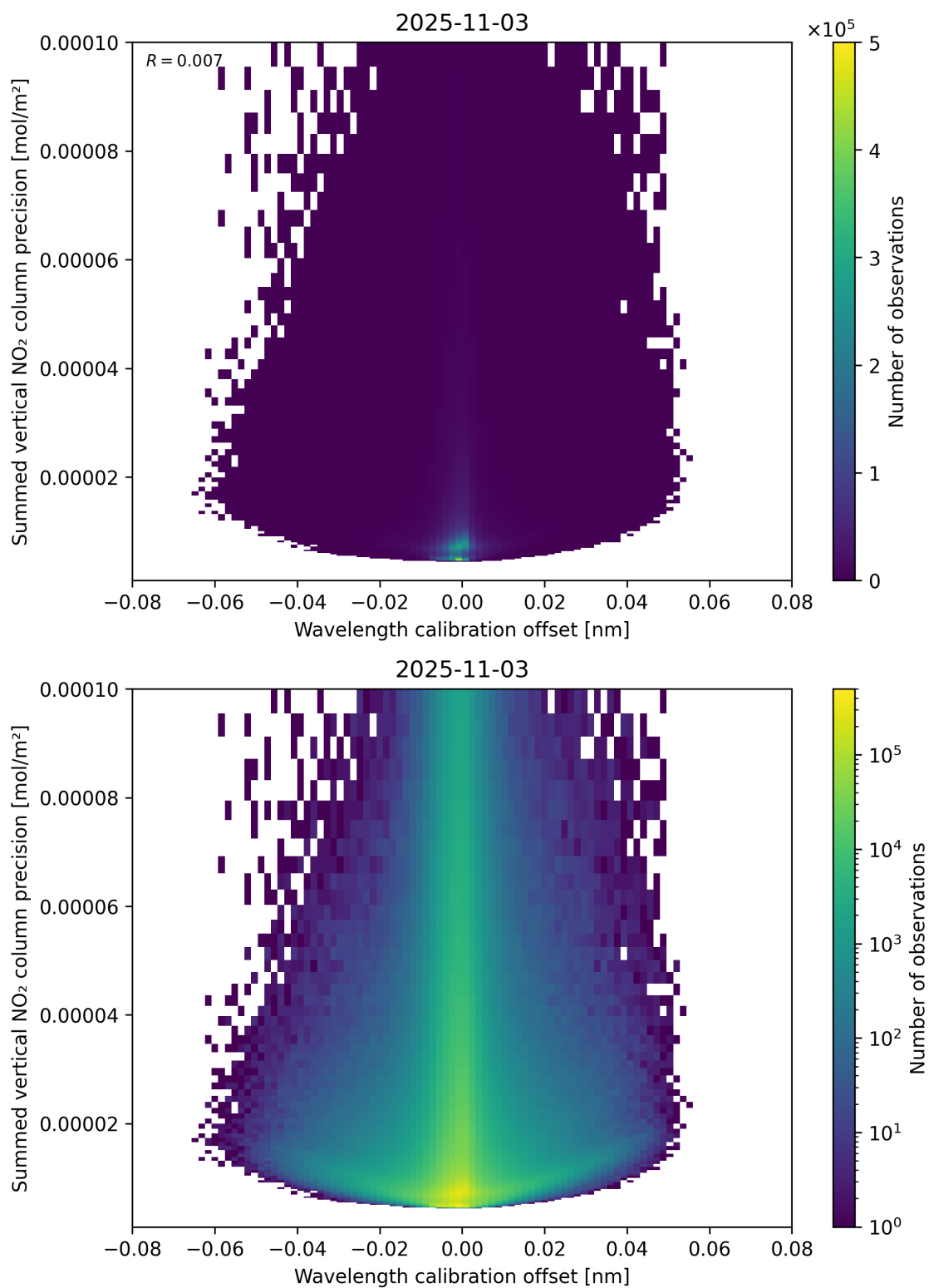
Figure 178: Scatter density plot of “Wavelength calibration offset” against “Summed vertical NO 2 column precision” for 2025-11-02 to 2025-11-04.
