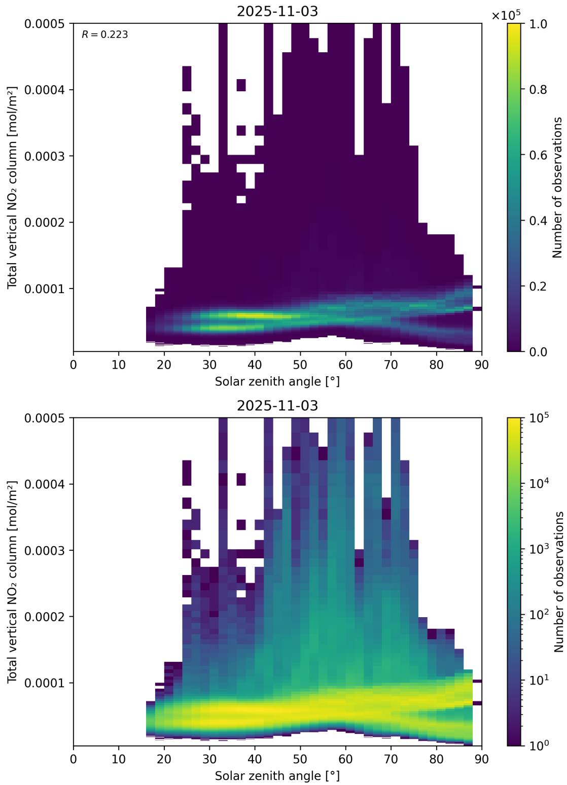
Figure 153: Scatter density plot of “Solar zenith angle” against “Total vertical NO 2 column” for 2025-11-02 to 2025-11-04.
