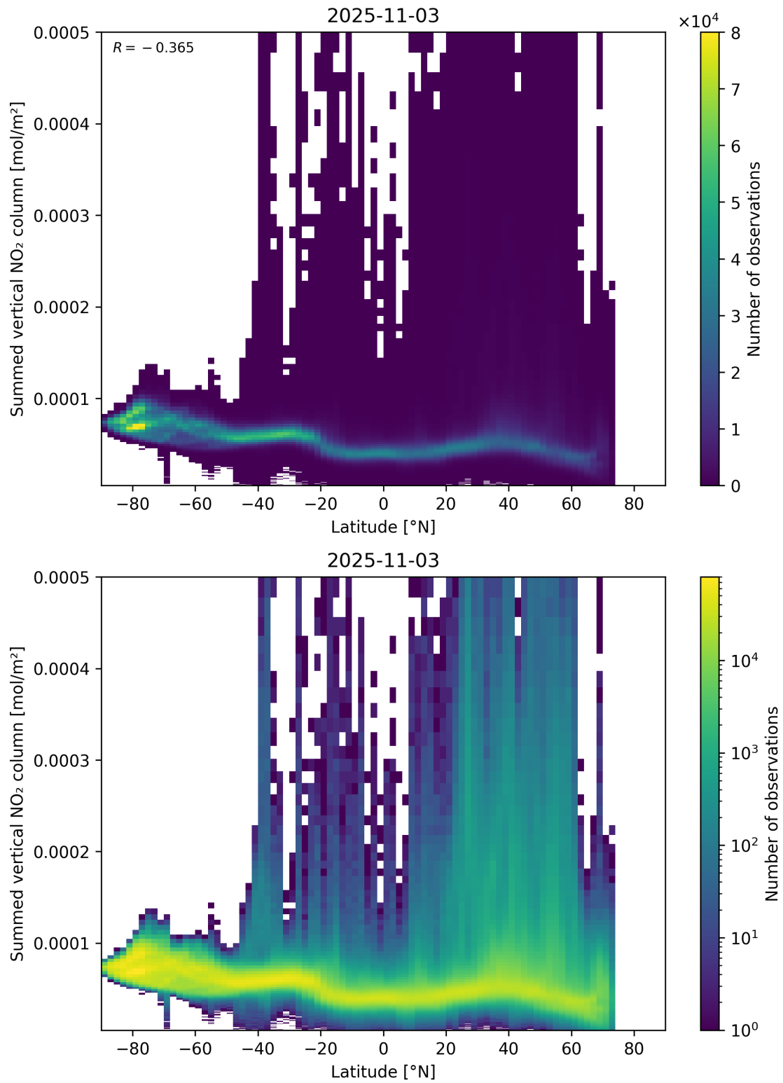
Figure 88: Scatter density plot of “Latitude” against “Summed vertical NO 2 column” for 2025-11-02 to 2025-11-04.
