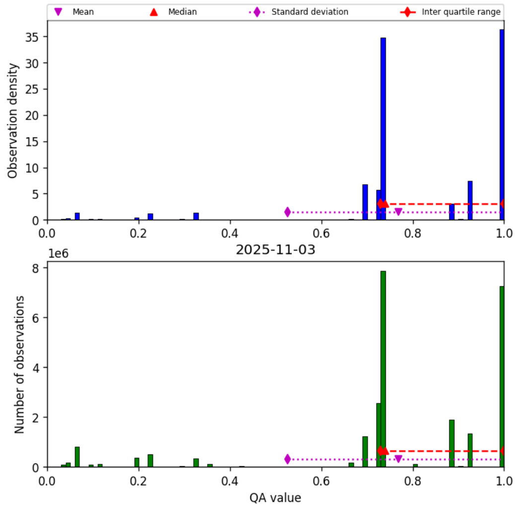
Figure 28: Histogram of “QA value” for 2025-11-02 to 2025-11-04
