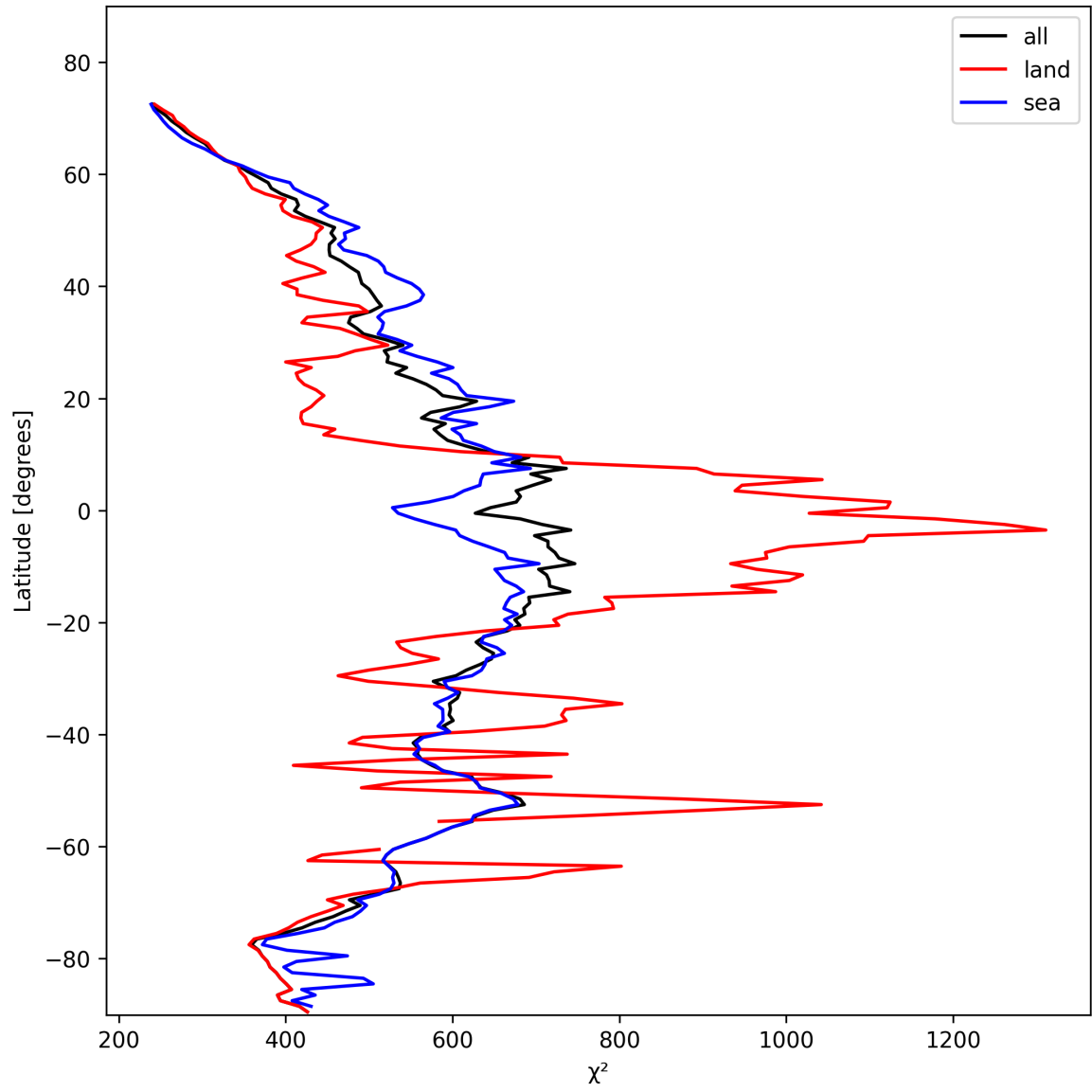
Figure 25: Zonal average of “ \chi^2 ” for 2025-11-02 to 2025-11-04.
