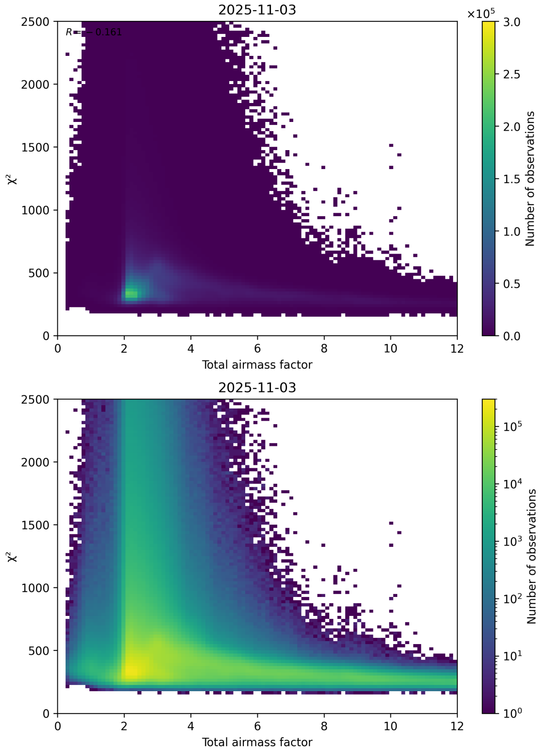
Figure 63: Scatter density plot of “Total airmass factor” against “ \chi^2 ” for 2025-11-02 to 2025-11-04.
