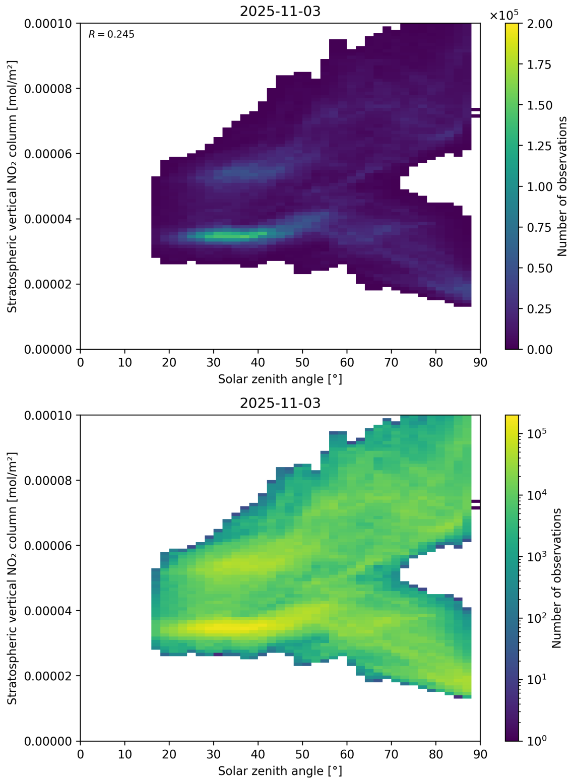
Figure 150: Scatter density plot of “Solar zenith angle” against “Stratospheric vertical NO 2 column” for 2025-11-02 to 2025-11-04.
