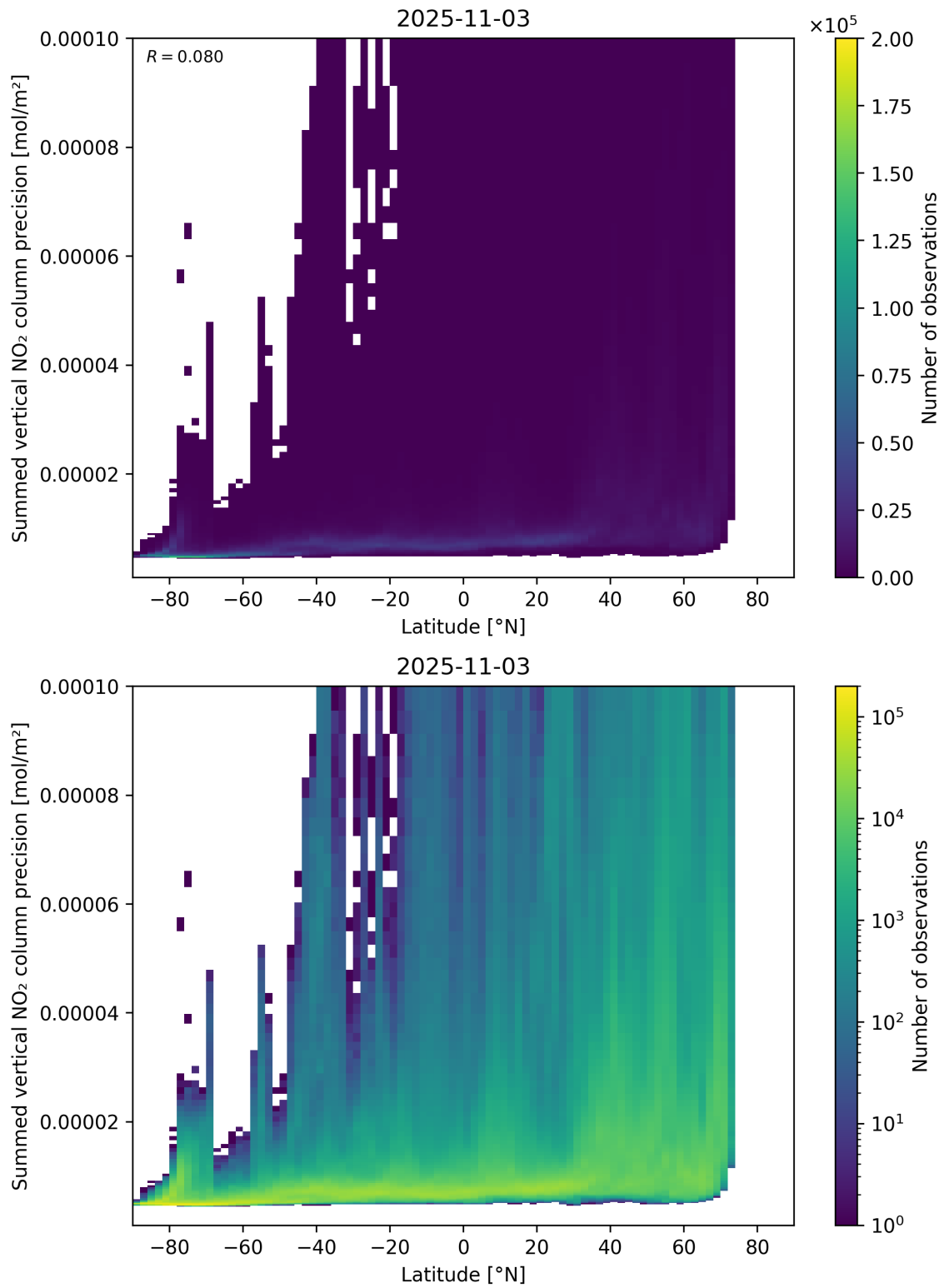
Figure 89: Scatter density plot of “Latitude” against “Summed vertical NO 2 column precision” for 2025-11-02 to 2025-11-04.
