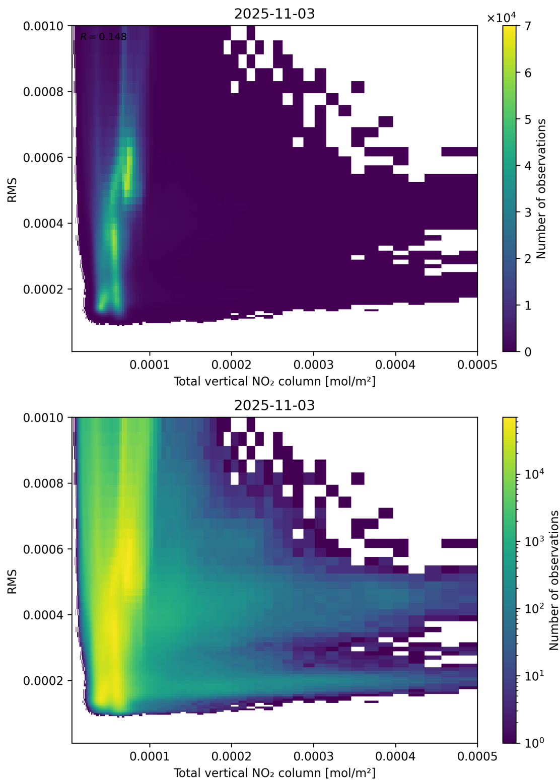
Figure 120: Scatter density plot of “Total vertical NO 2 column” against “RMS” for 2025-11-02 to 2025-11-04.
