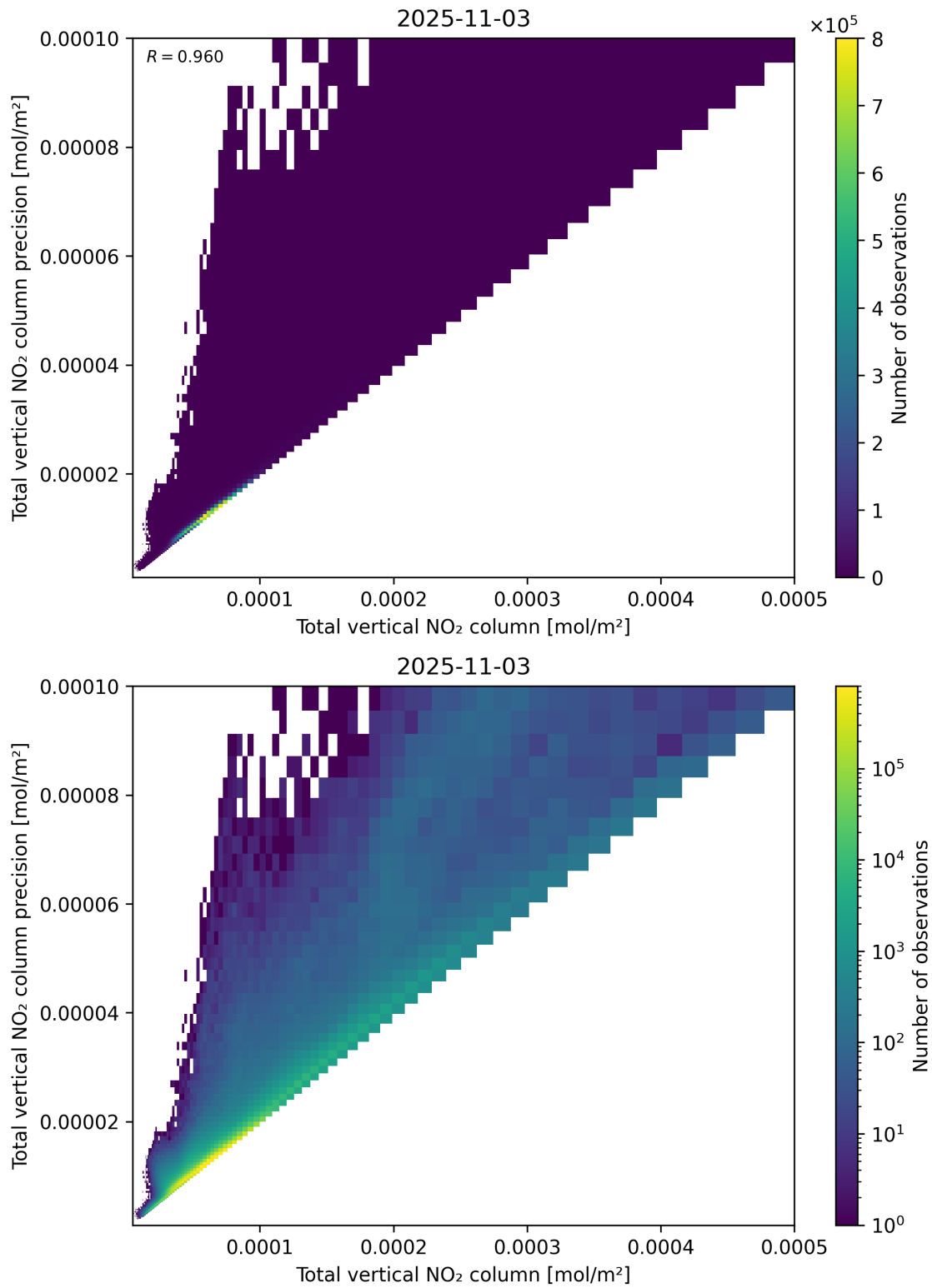
Figure 114: Scatter density plot of “Total vertical NO 2 column” against “Total vertical NO 2 column precision” for 2025-11-02 to 2025-11-04.
