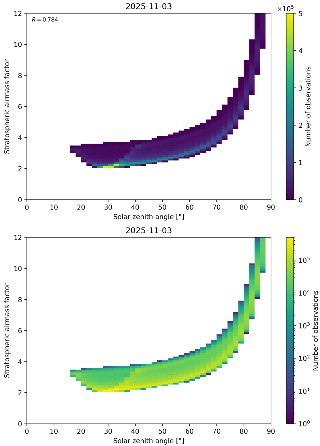
Figure 145: Scatter density plot of “Solar zenith angle” against “Stratospheric airmass factor” for 2025-11-02 to 2025-11-04.
