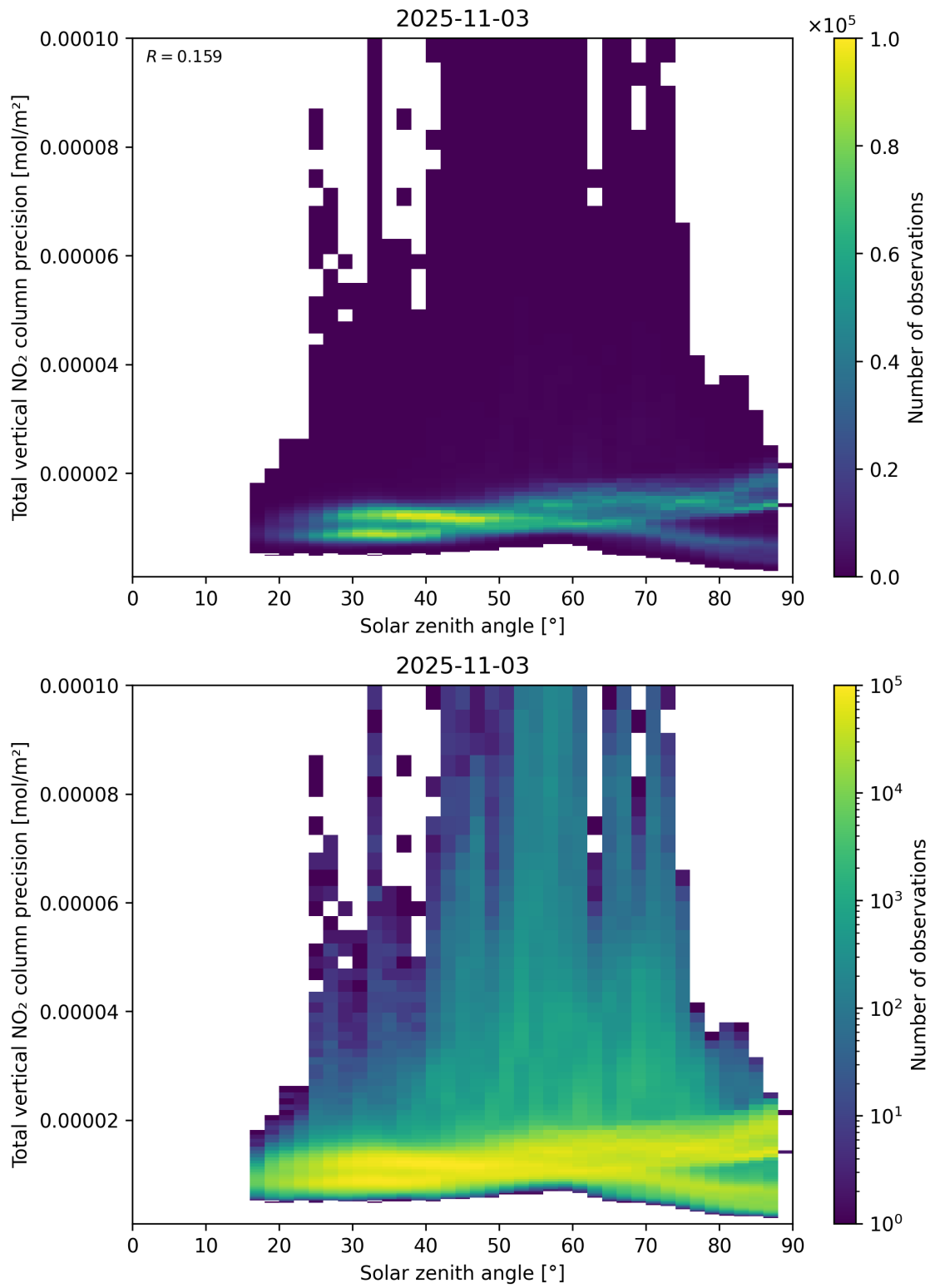
Figure 154: Scatter density plot of “Solar zenith angle” against “Total vertical NO 2 column precision” for 2025-11-02 to 2025-11-04.
