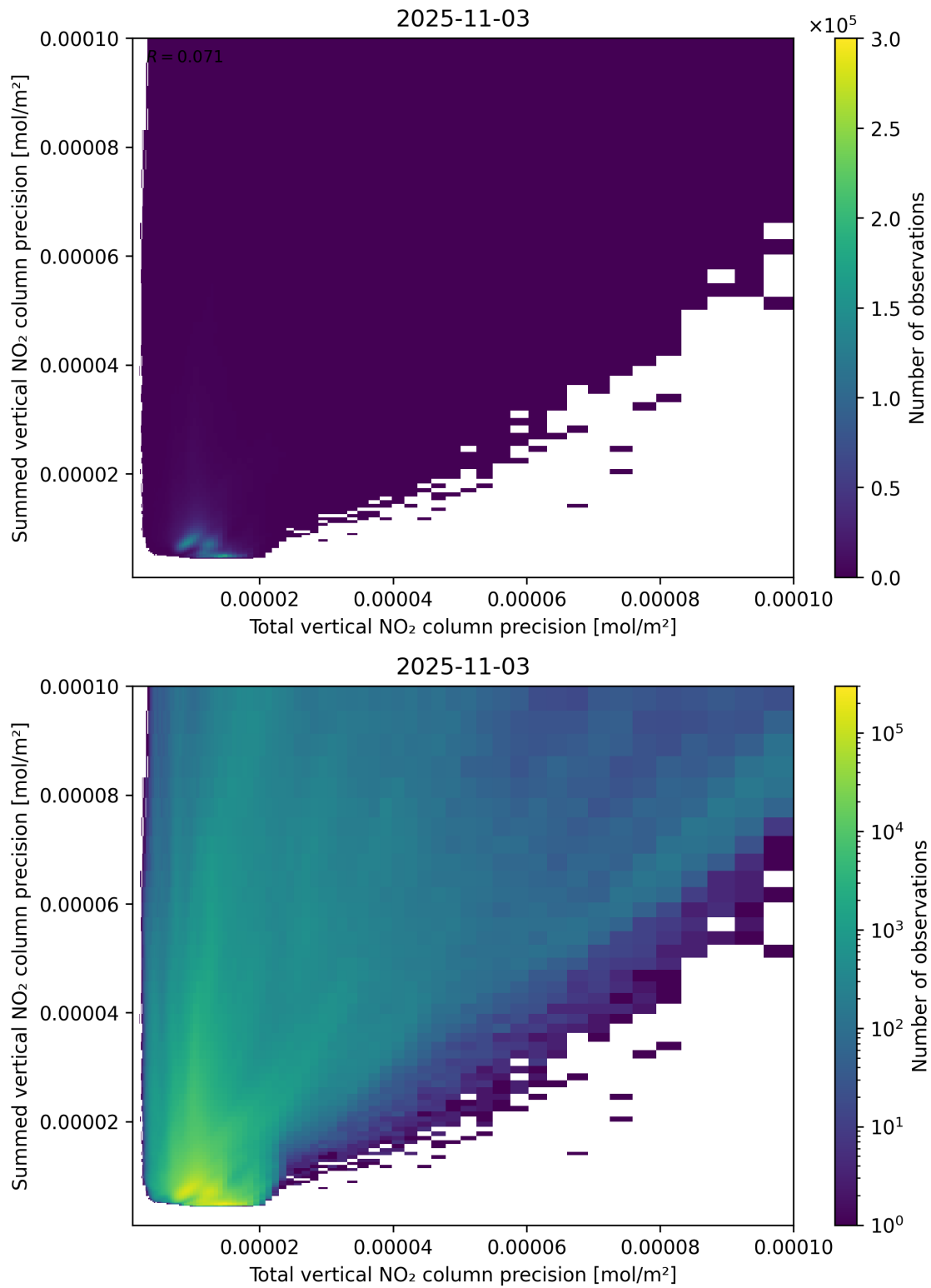
Figure 118: Scatter density plot of “Total vertical NO 2 column precision” against “Summed vertical NO 2 column precision” for 2025-11-02 to 2025-11-04.
