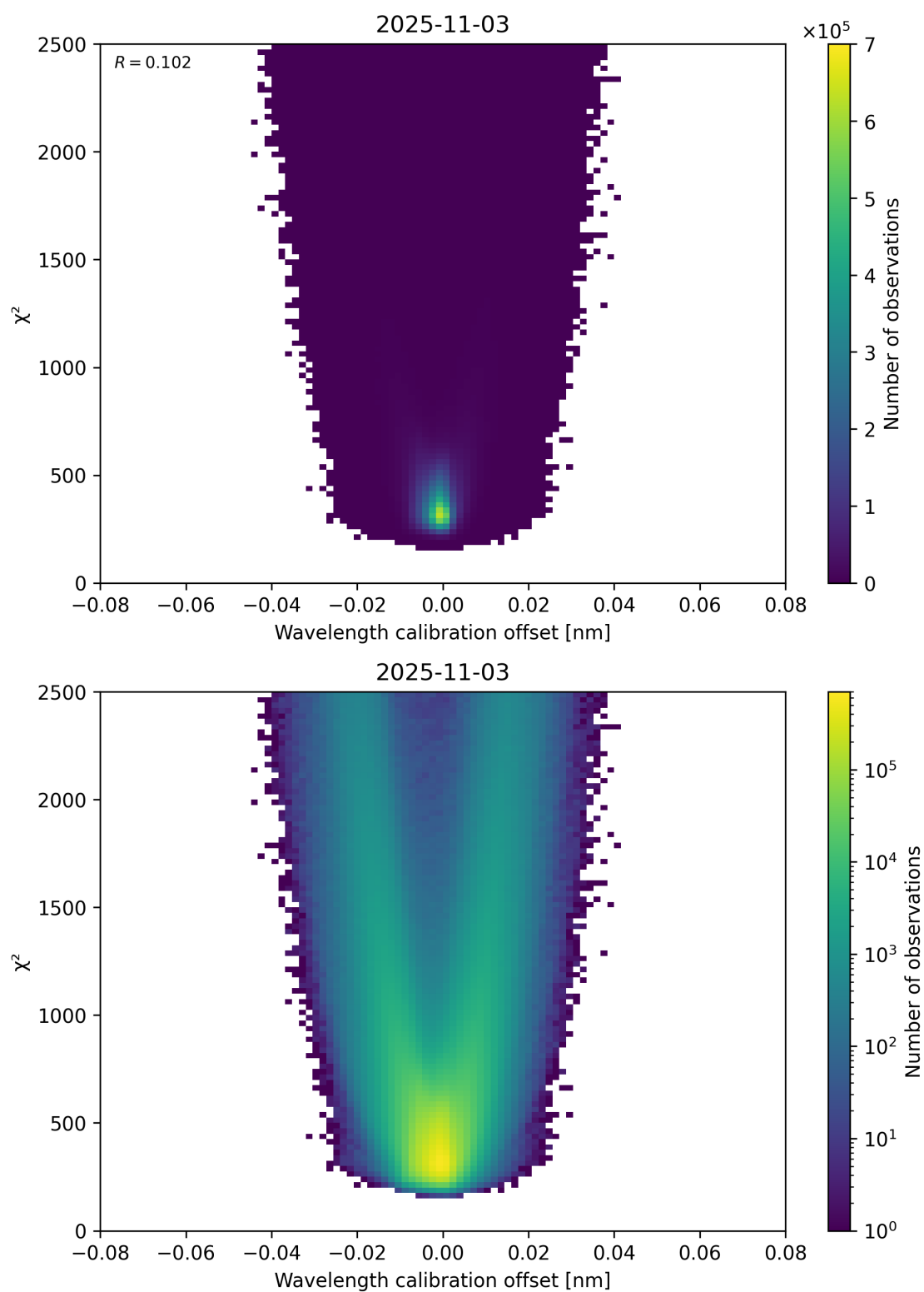
Figure 175: Scatter density plot of “Wavelength calibration offset” against “ \chi^2 ” for 2025-11-02 to 2025-11-04.
