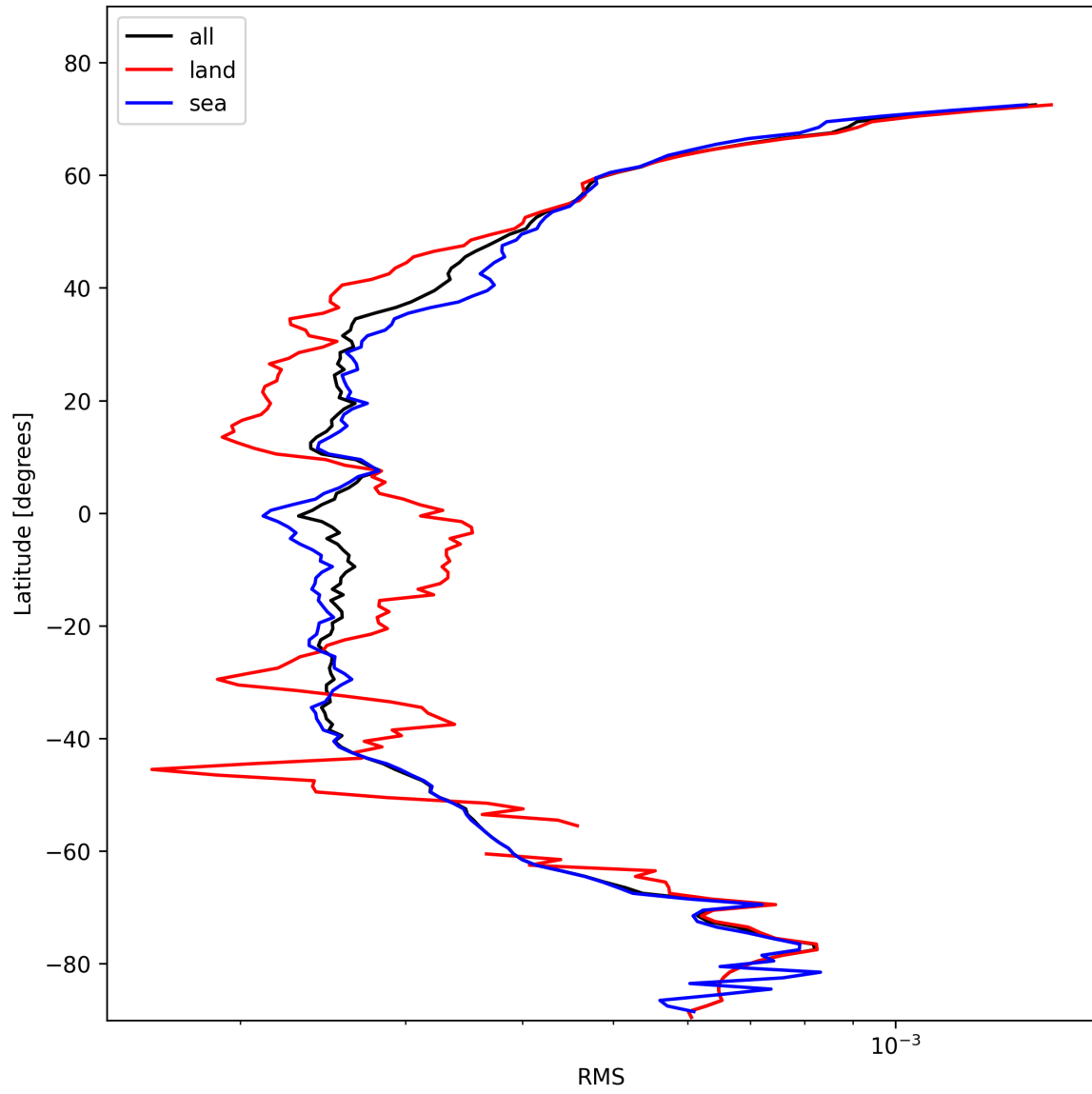
Figure 26: Zonal average of “RMS” for 2025-11-02 to 2025-11-04.
