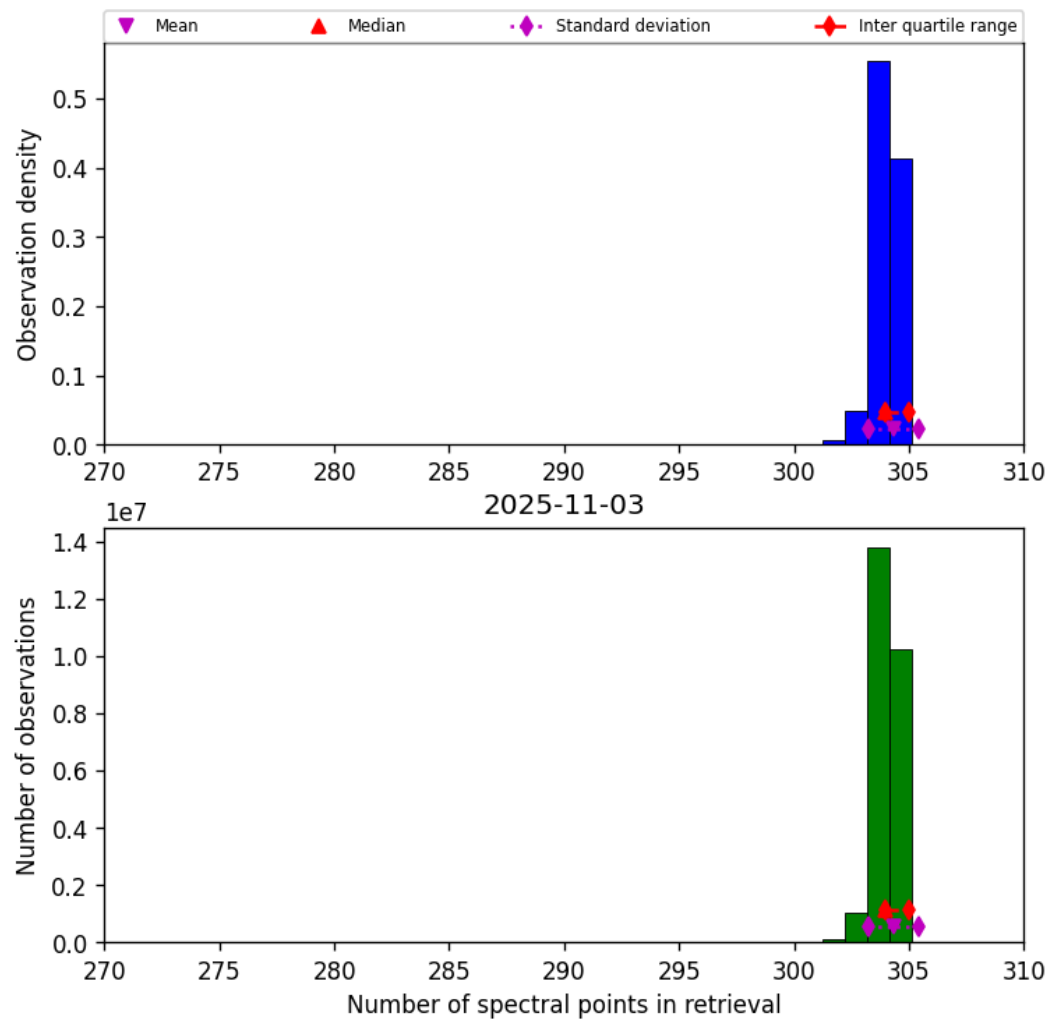
Figure 33: Histogram of “Number of spectral points in retrieval” for 2025-11-02 to 2025-11-04
