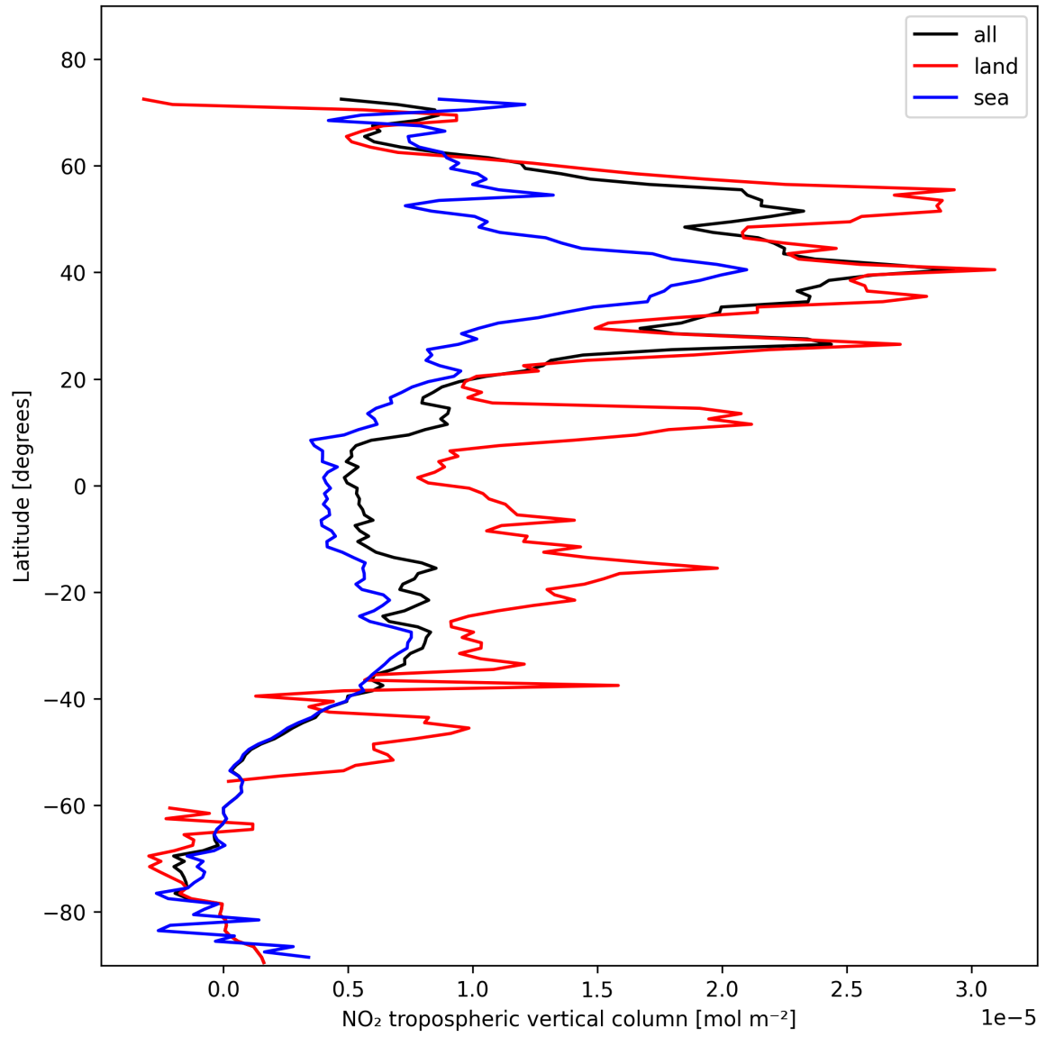
Figure 12: Zonal average of “NO 2 tropospheric vertical column” for 2025-11-02 to 2025-11-04.
