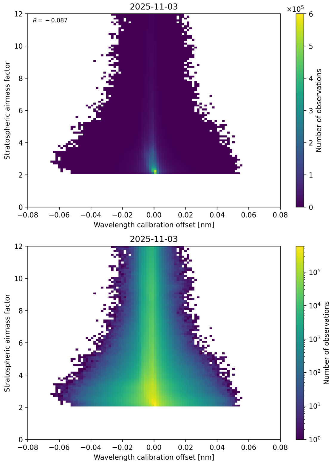
Figure 174: Scatter density plot of “Wavelength calibration offset” against “Stratospheric air mass factor” for 2025-11-02 to 2025-11-04.
