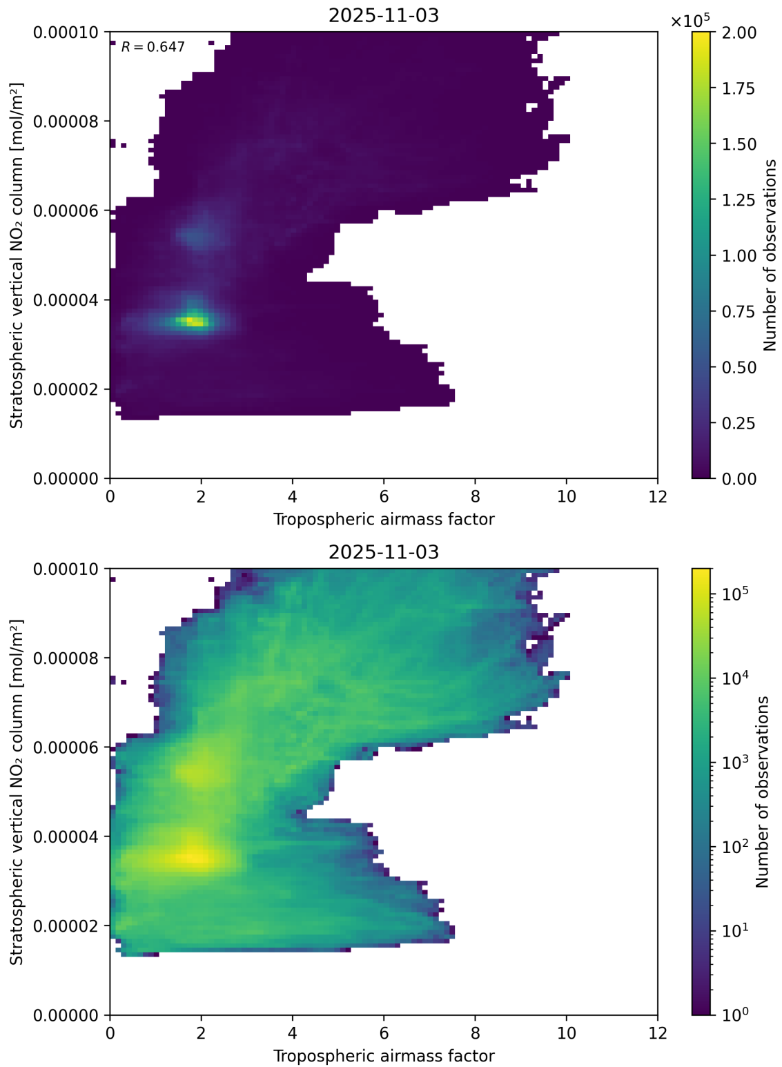
Figure 74: Scatter density plot of “Tropospheric air mass factor” against “Stratospheric vertical NO 2 column” for 2025-11-02 to 2025-11-04.
