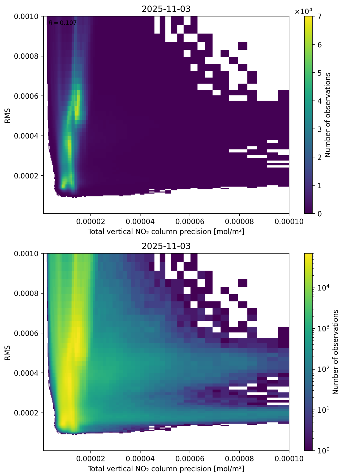
Figure 119: Scatter density plot of “Total vertical NO 2 column precision” against “RMS” for 2025-11-02 to 2025-11-04.
