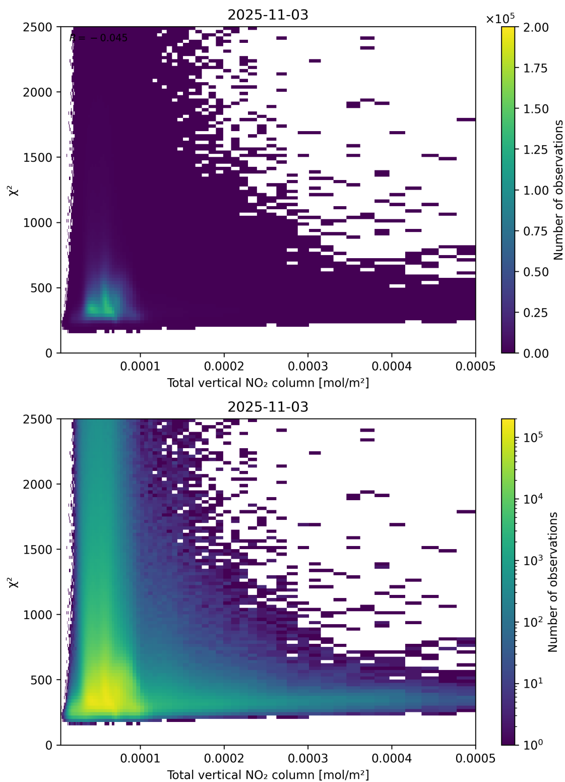
Figure 111: Scatter density plot of “Total vertical NO 2 column” against “ \chi^2 ” for 2025-11-02 to 2025-11-04.
