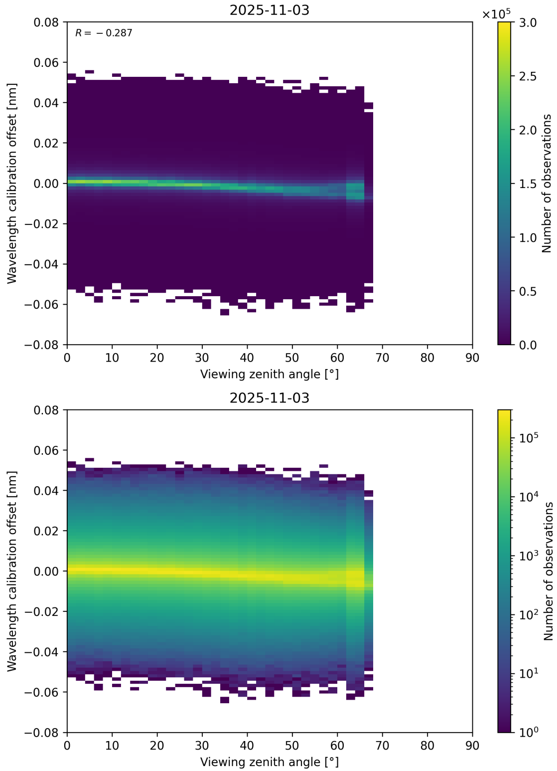
Figure 173: Scatter density plot of “Viewing zenith angle” against “Wavelength calibration offset” for 2025-11-02 to 2025-11-04.
