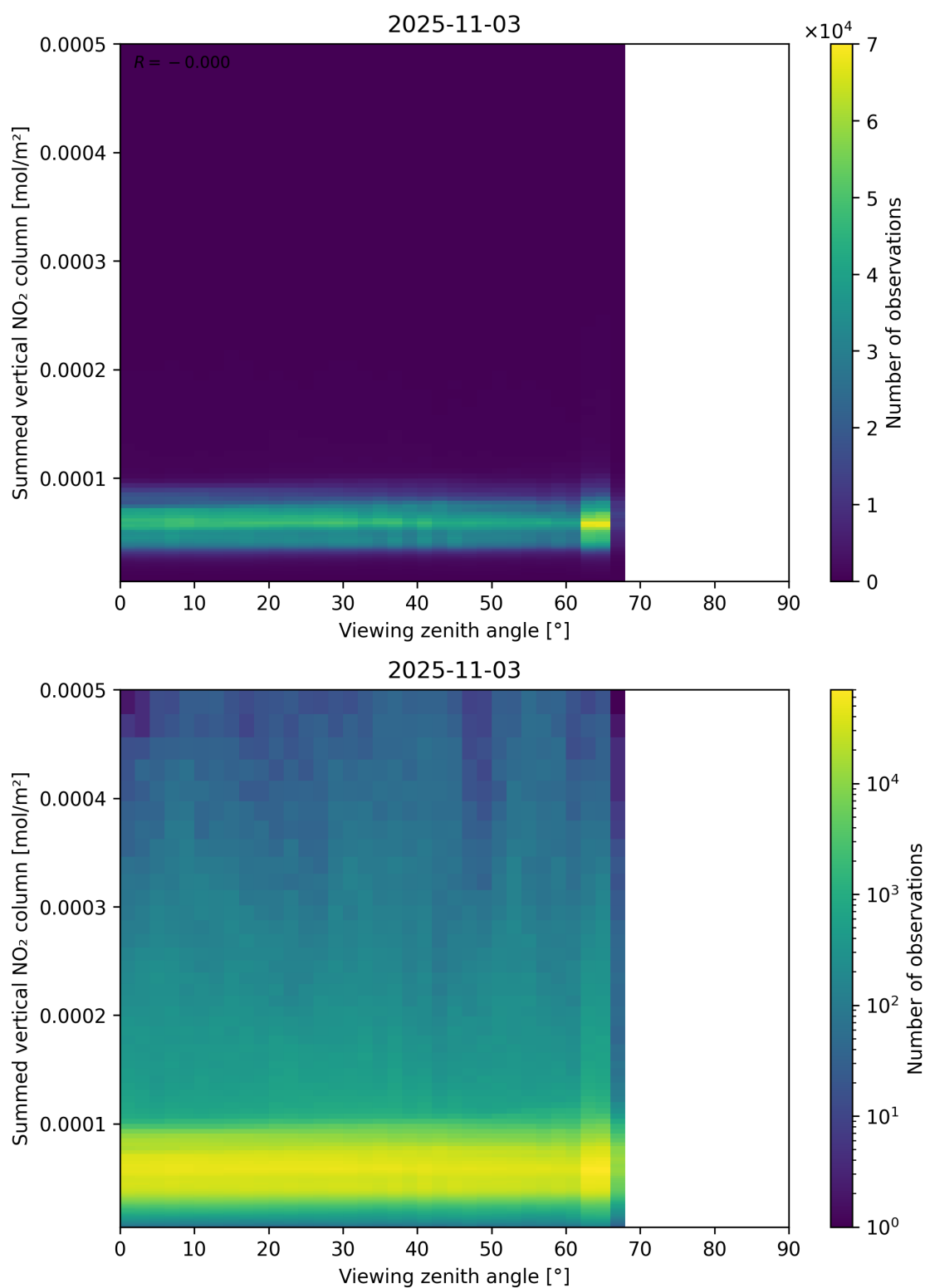
Figure 165: Scatter density plot of “Viewing zenith angle” against “Summed vertical NO 2 column” for 2025-11-02 to 2025-11-04.
