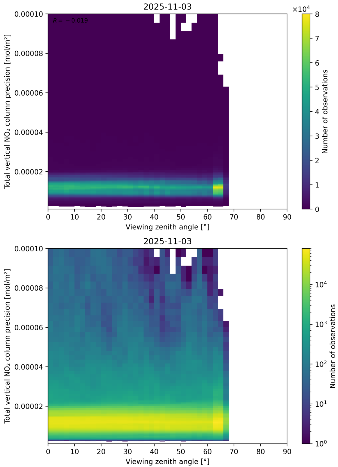
Figure 168: Scatter density plot of “Viewing zenith angle” against “Total vertical NO 2 column precision” for 2025-11-02 to 2025-11-04.
