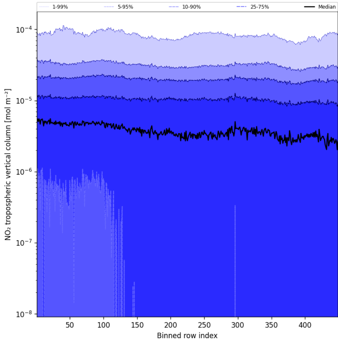
Figure 46: Along track statistics of “NO 2 tropospheric vertical column” for 2025-11-02 to 2025-11-04
