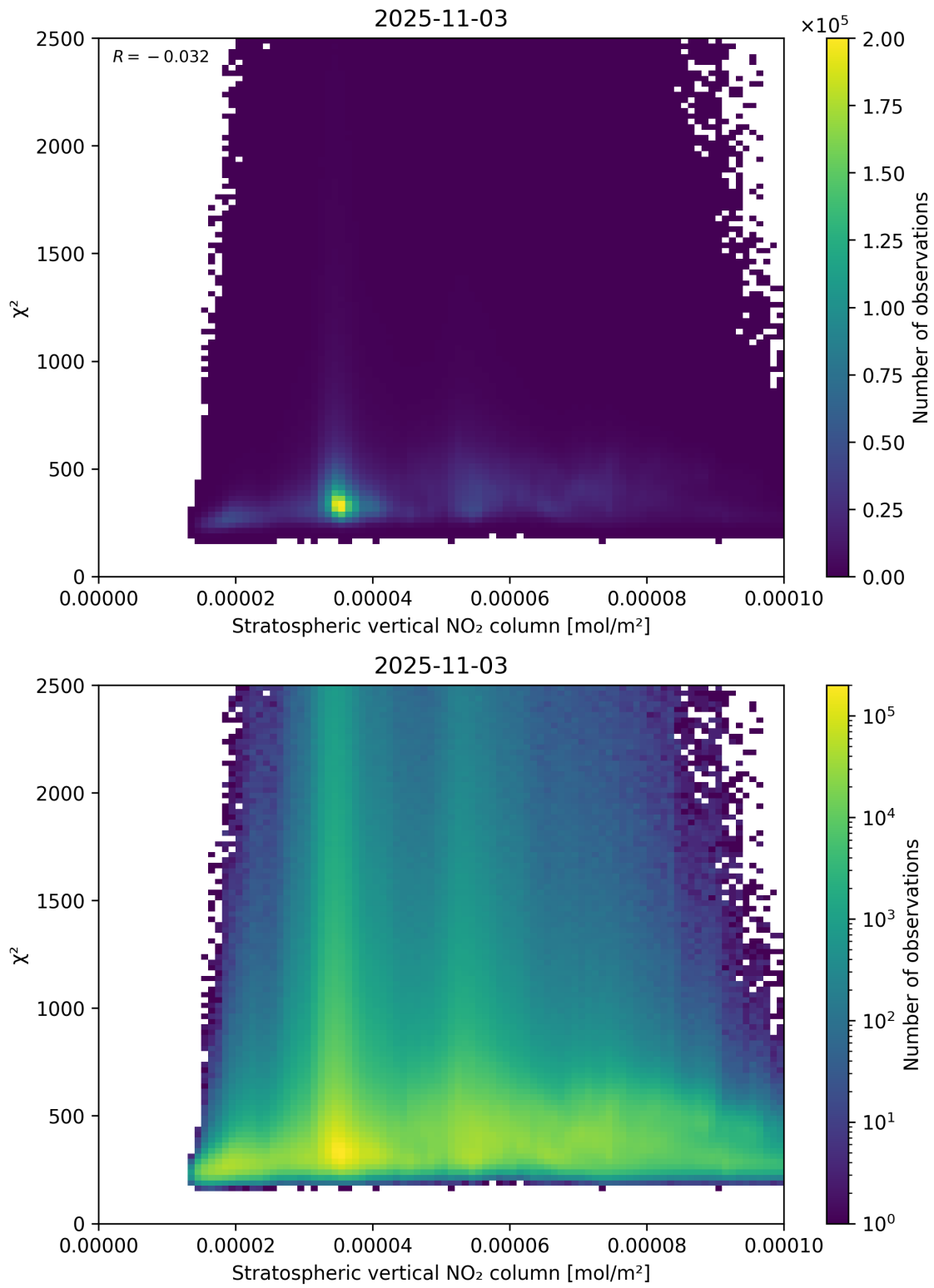
Figure 97: Scatter density plot of “Stratospheric vertical NO 2 column” against “ \chi^2 ” for 2025-11-02 to 2025-11-04.
