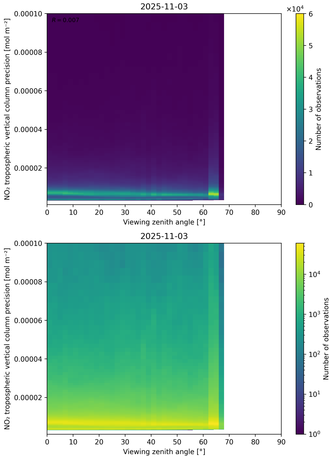
Figure 170: Scatter density plot of “Viewing zenith angle” against “NO 2 tropospheric vertical column precision” for 2025-11-02 to 2025-11-04.
