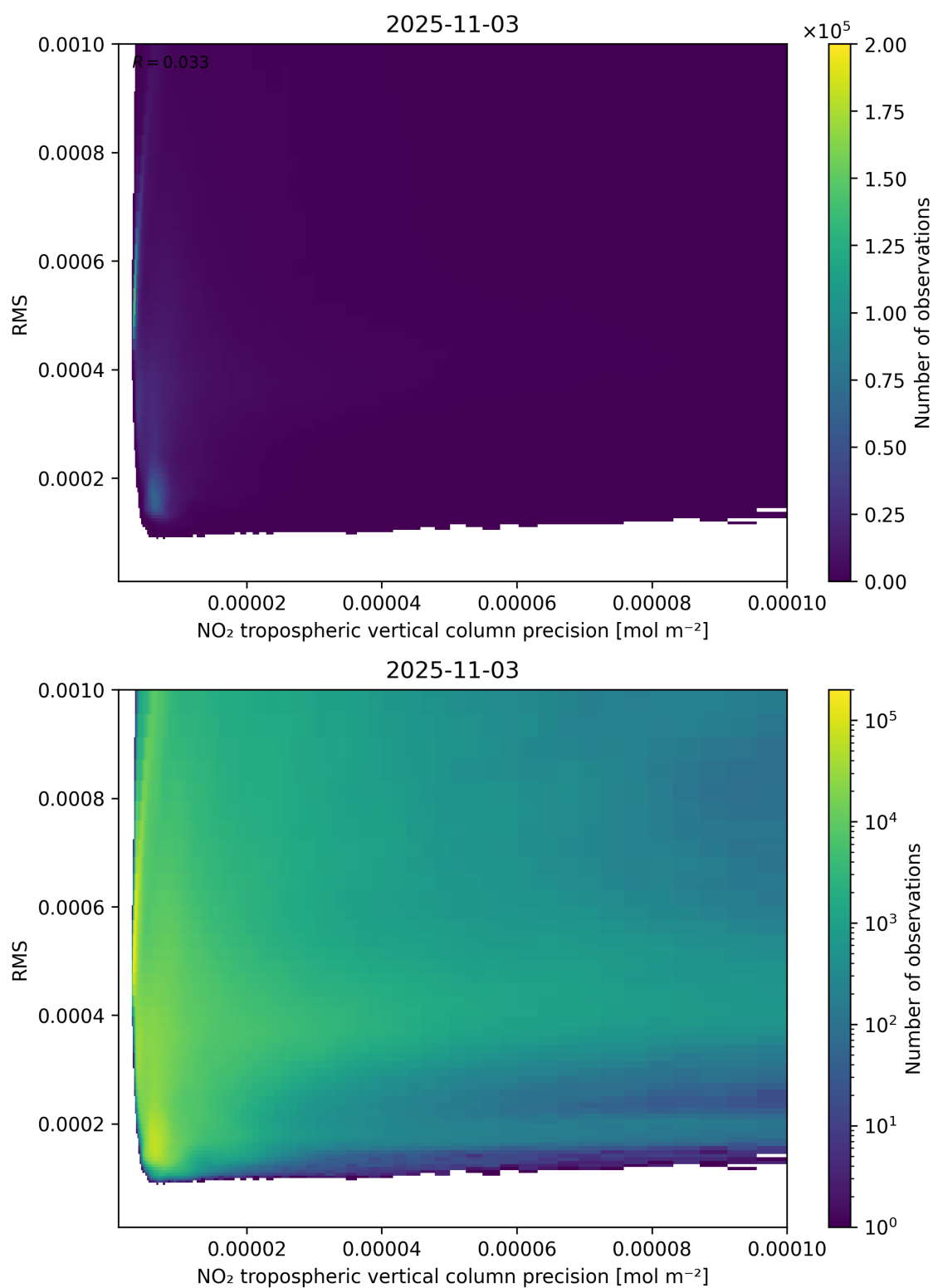
Figure 140: Scatter density plot of “NO 2 tropospheric vertical column precision” against “RMS” for 2025-11-02 to 2025-11-04.
