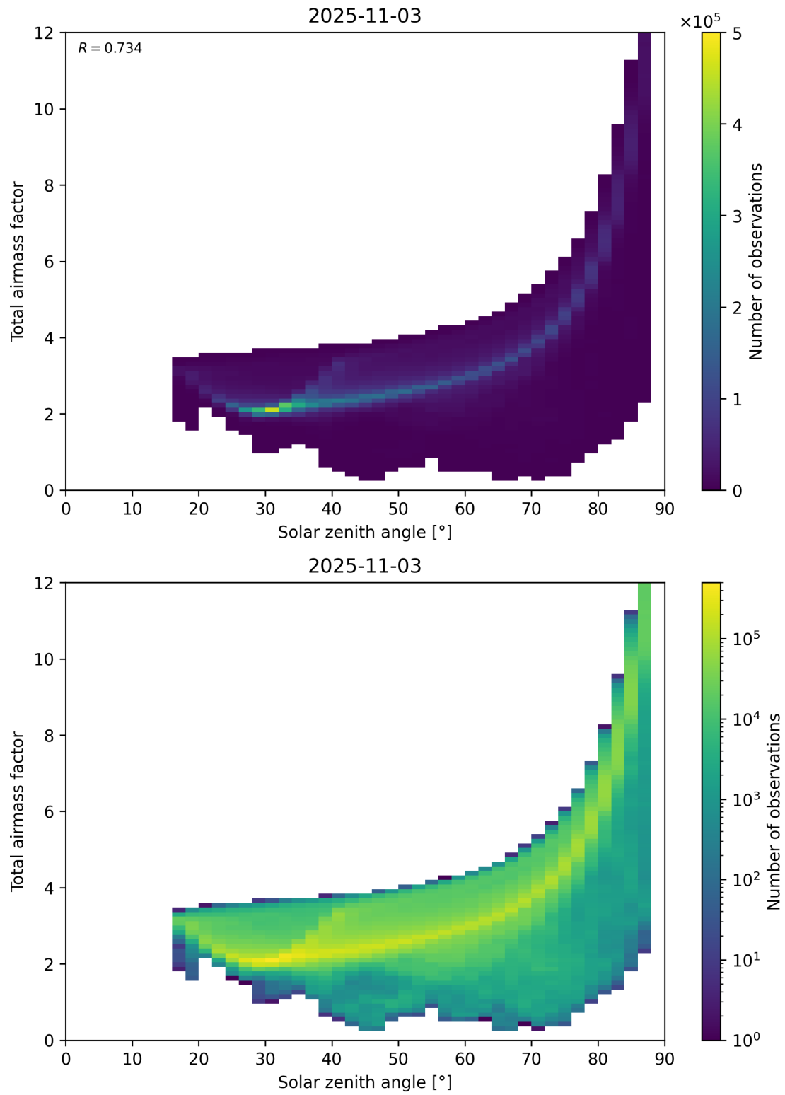
Figure 146: Scatter density plot of “Solar zenith angle” against “Total airmass factor” for 2025-11-02 to 2025-11-04.
