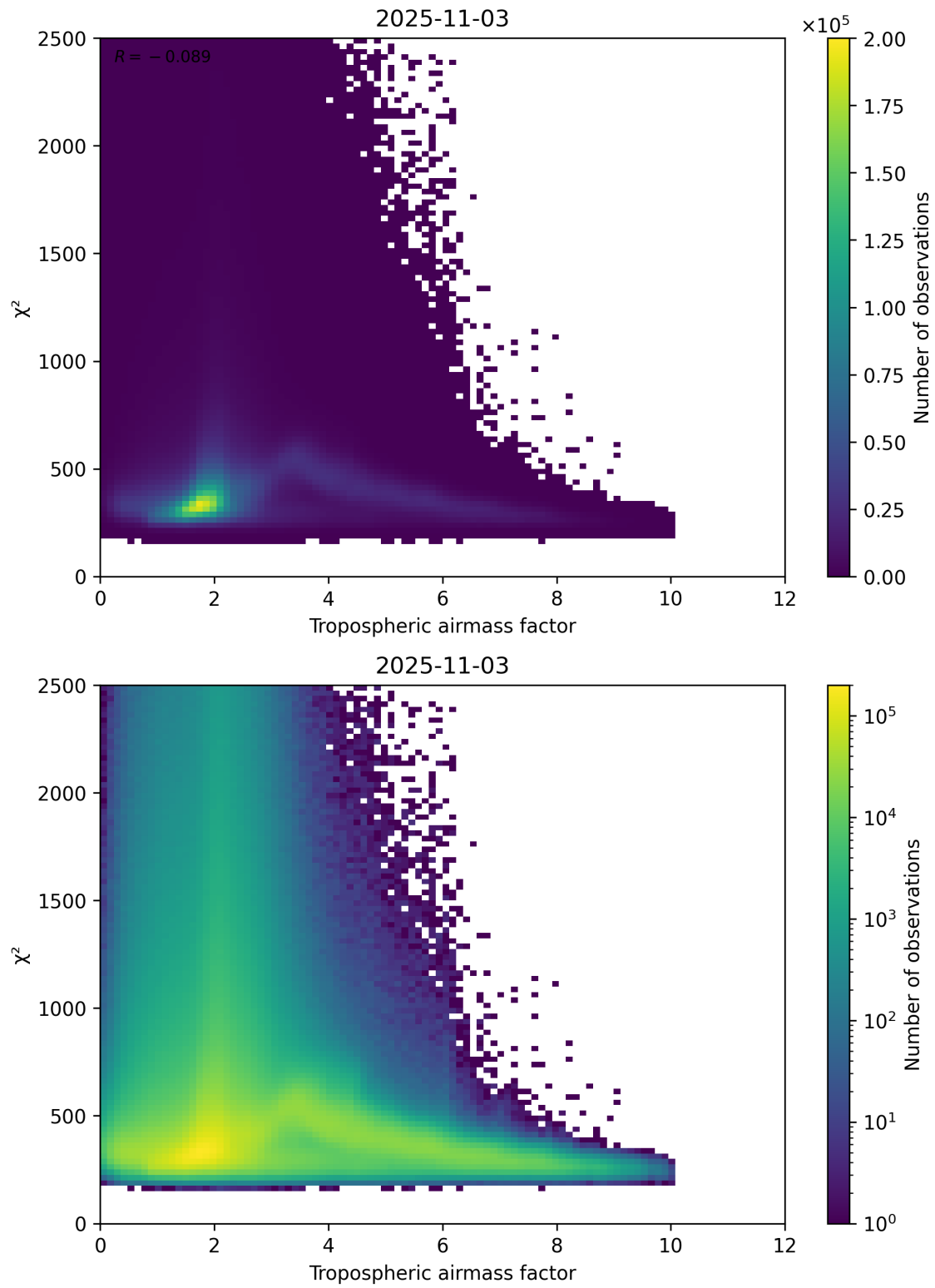
Figure 73: Scatter density plot of “Tropospheric airmass factor” against “ \chi^2 ” for 2025-11-02 to 2025-11-04.
