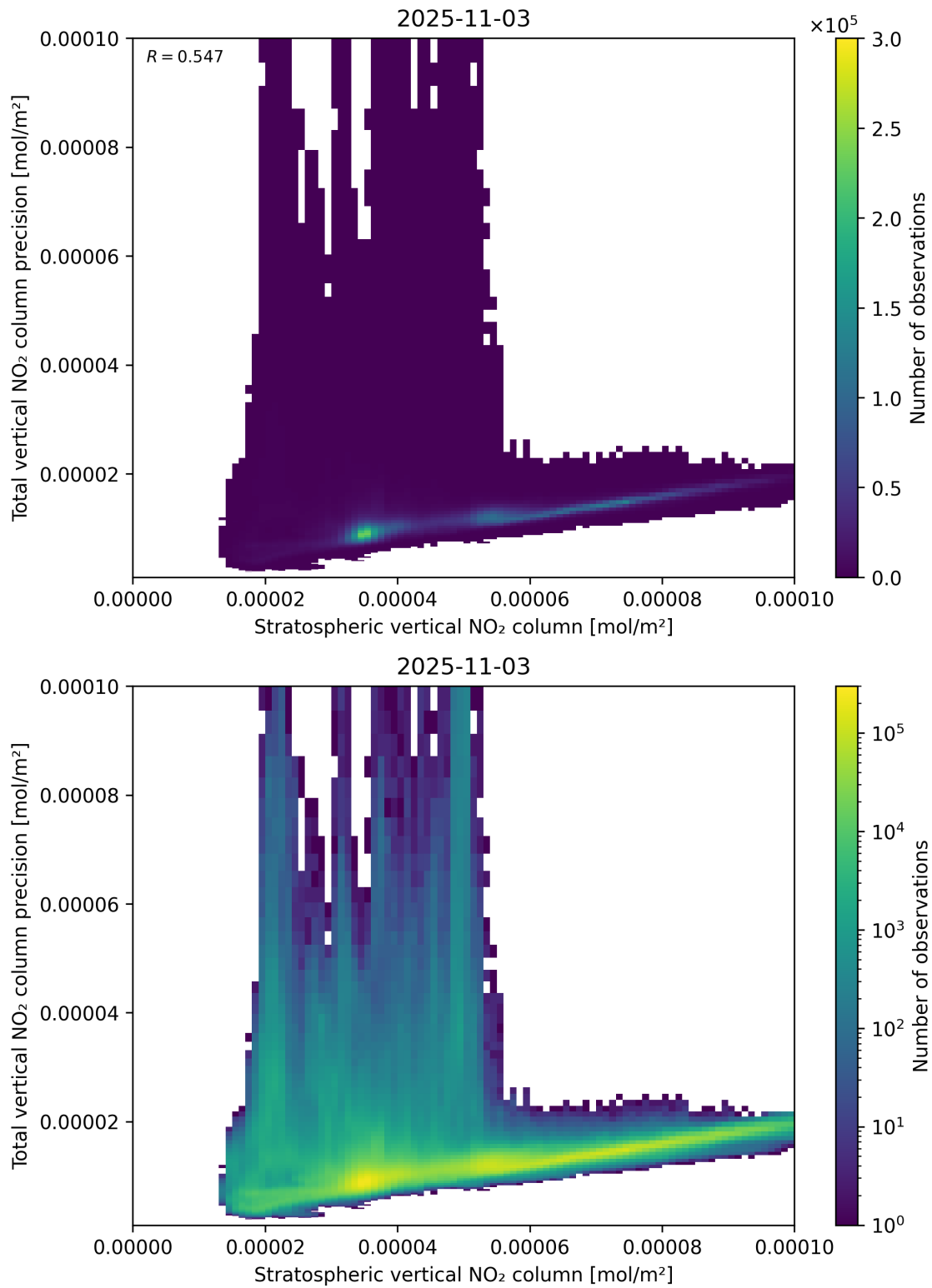
Figure 101: Scatter density plot of “Stratospheric vertical NO 2 column” against “Total vertical NO 2 column precision” for 2025-11-02 to 2025-11-04.
