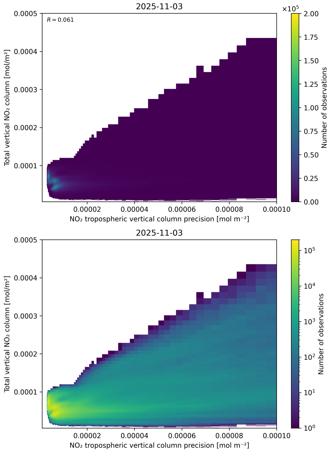
Figure 138: Scatter density plot of “NO 2 tropospheric vertical column precision” against “Total vertical NO 2 column” for 2025-11-02 to 2025-11-04.
