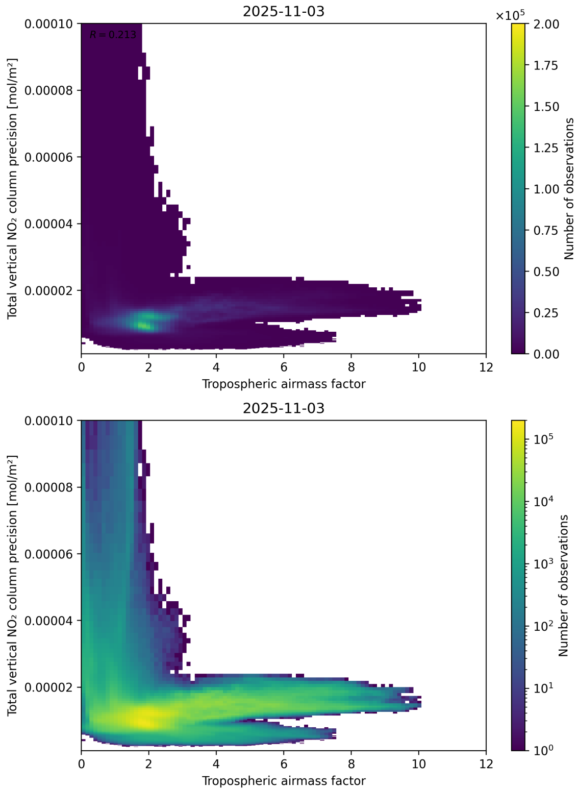
Figure 78: Scatter density plot of “Tropospheric airmass factor” against “Total vertical NO 2 column precision” for 2025-11-02 to 2025-11-04.
