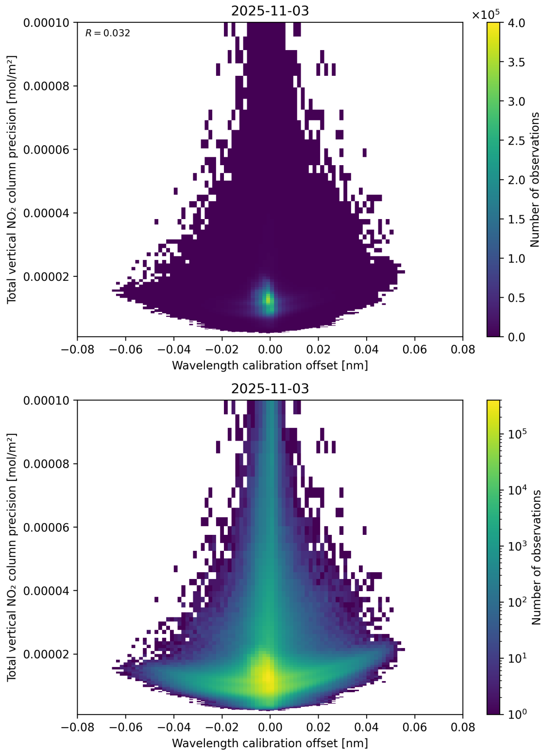
Figure 180: Scatter density plot of “Wavelength calibration offset” against “Total vertical NO 2 column precision” for 2025-11-02 to 2025-11-04.
