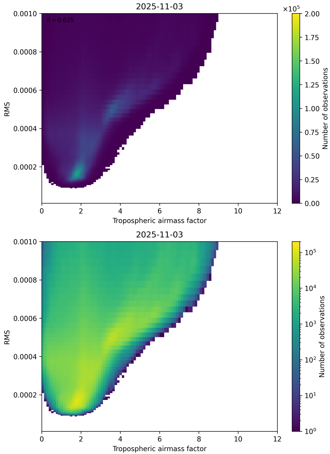
Figure 79: Scatter density plot of “Tropospheric airmass factor” against “RMS” for 2025-11-02 to 2025-11-04.
