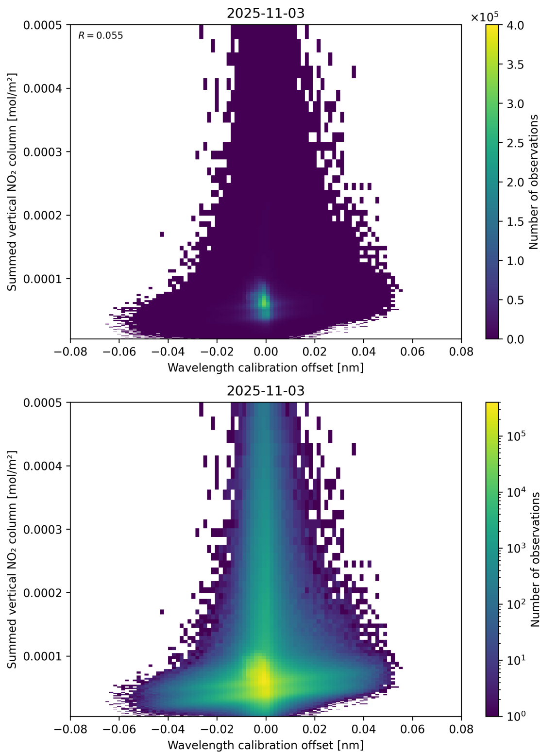
Figure 177: Scatter density plot of “Wavelength calibration offset” against “Summed vertical NO 2 column” for 2025-11-02 to 2025-11-04.
