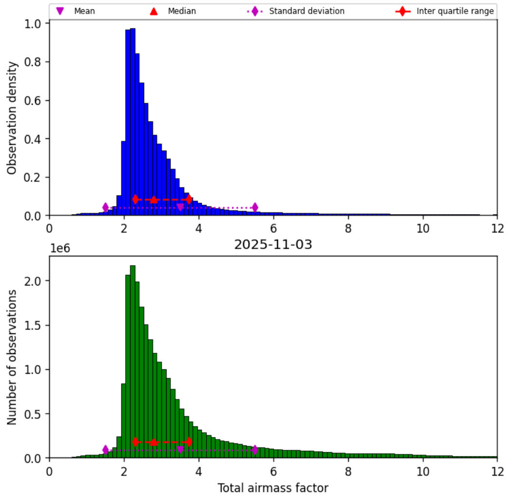
Figure 32: Histogram of “Total airmass factor” for 2025-11-02 to 2025-11-04
