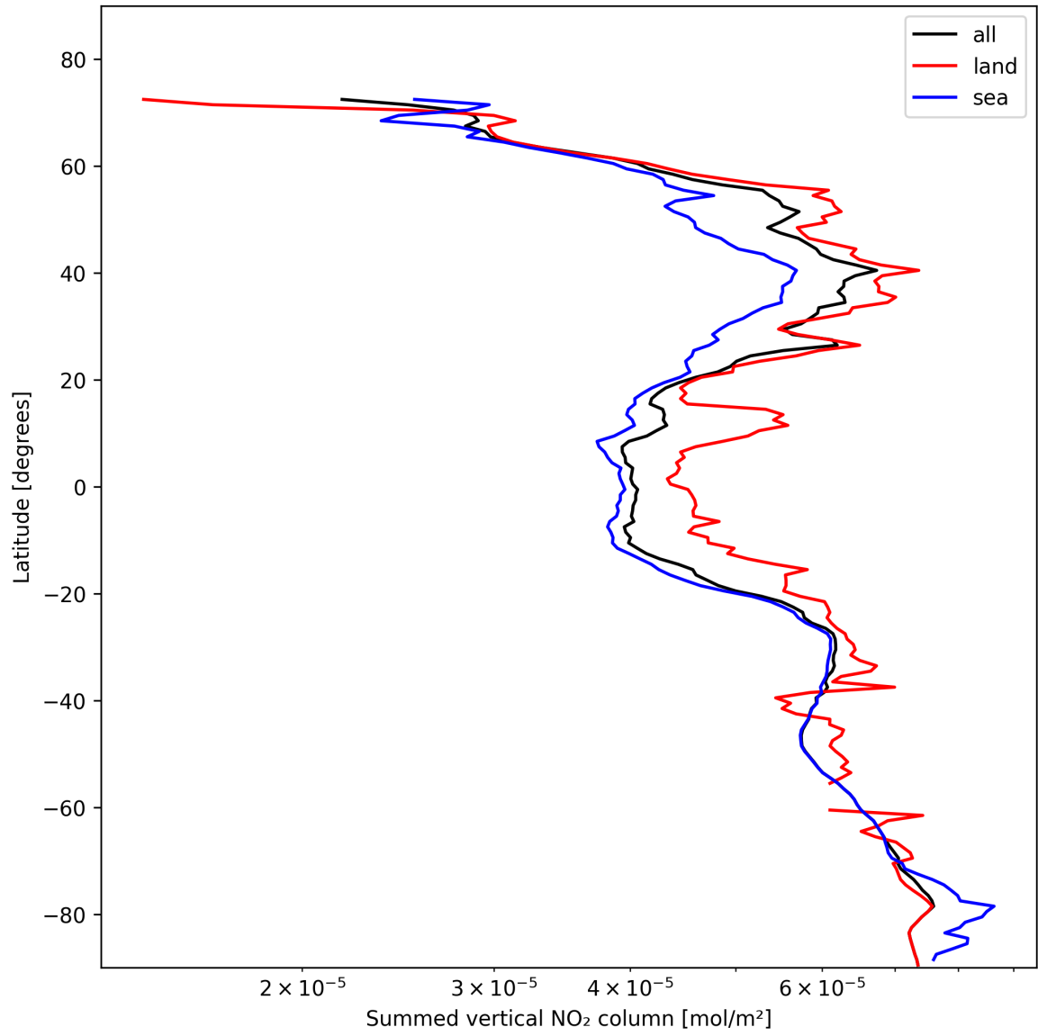
Figure 23: Zonal average of “Summed vertical NO 2 column” for 2025-11-02 to 2025-11-04.
