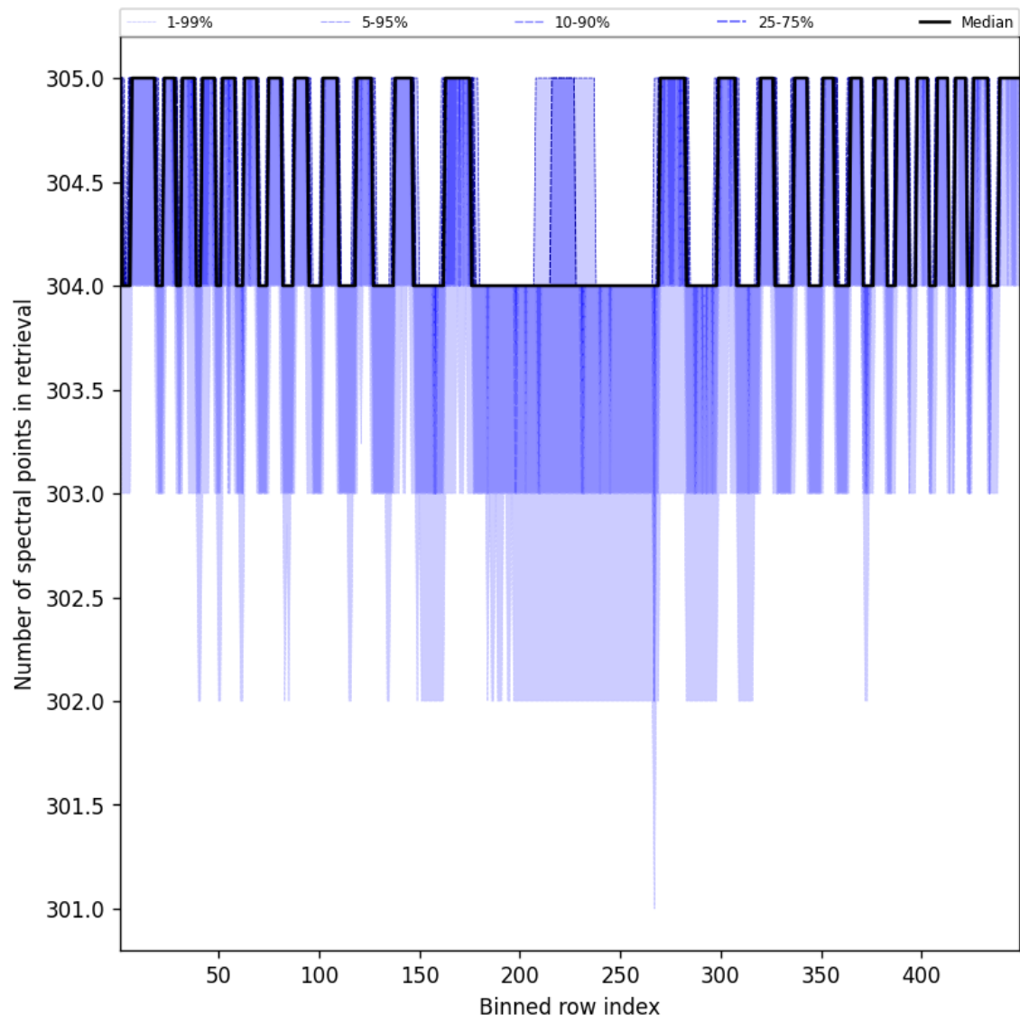
Figure 50: Along track statistics of “Number of spectral points in retrieval” for 2025-11-02 to 2025-11-04
