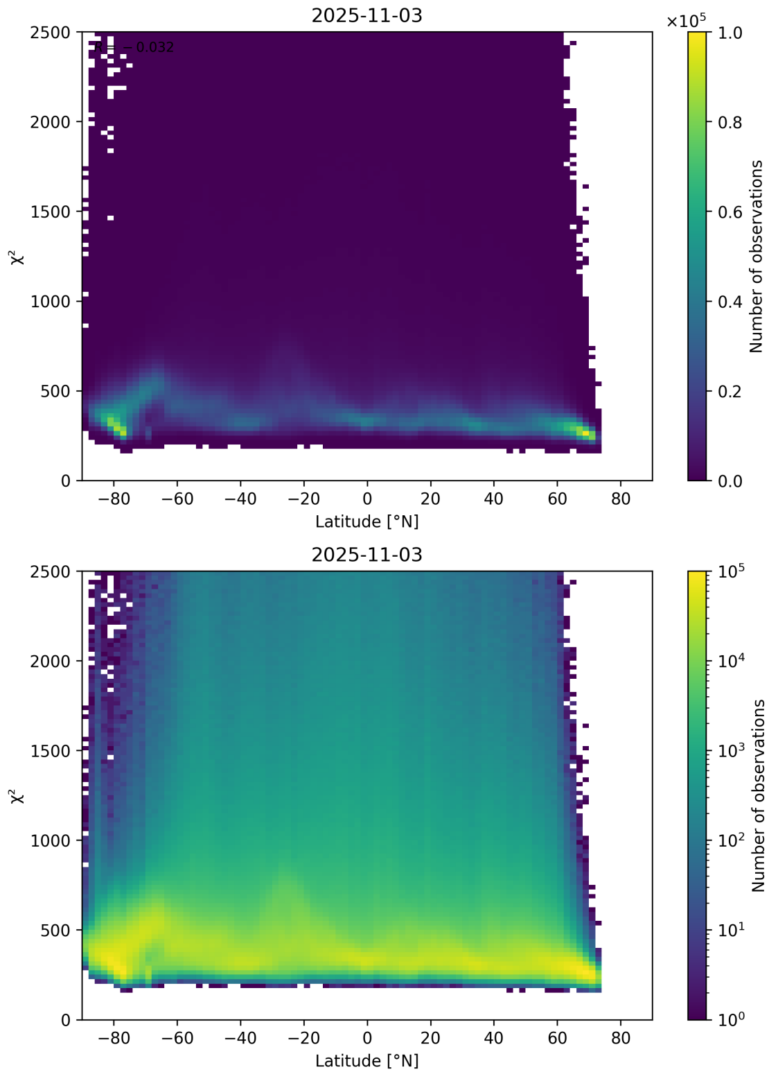
Figure 86: Scatter density plot of “Latitude” against “ \chi^2 ” for 2025-11-02 to 2025-11-04.
