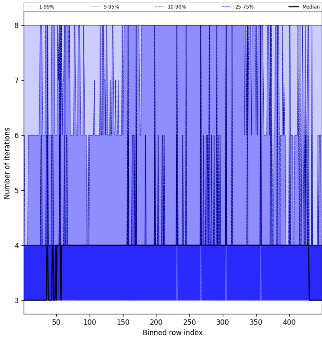
Figure 51: Along track statistics of “Number of iterations” for 2025-11-02 to 2025-11-04
