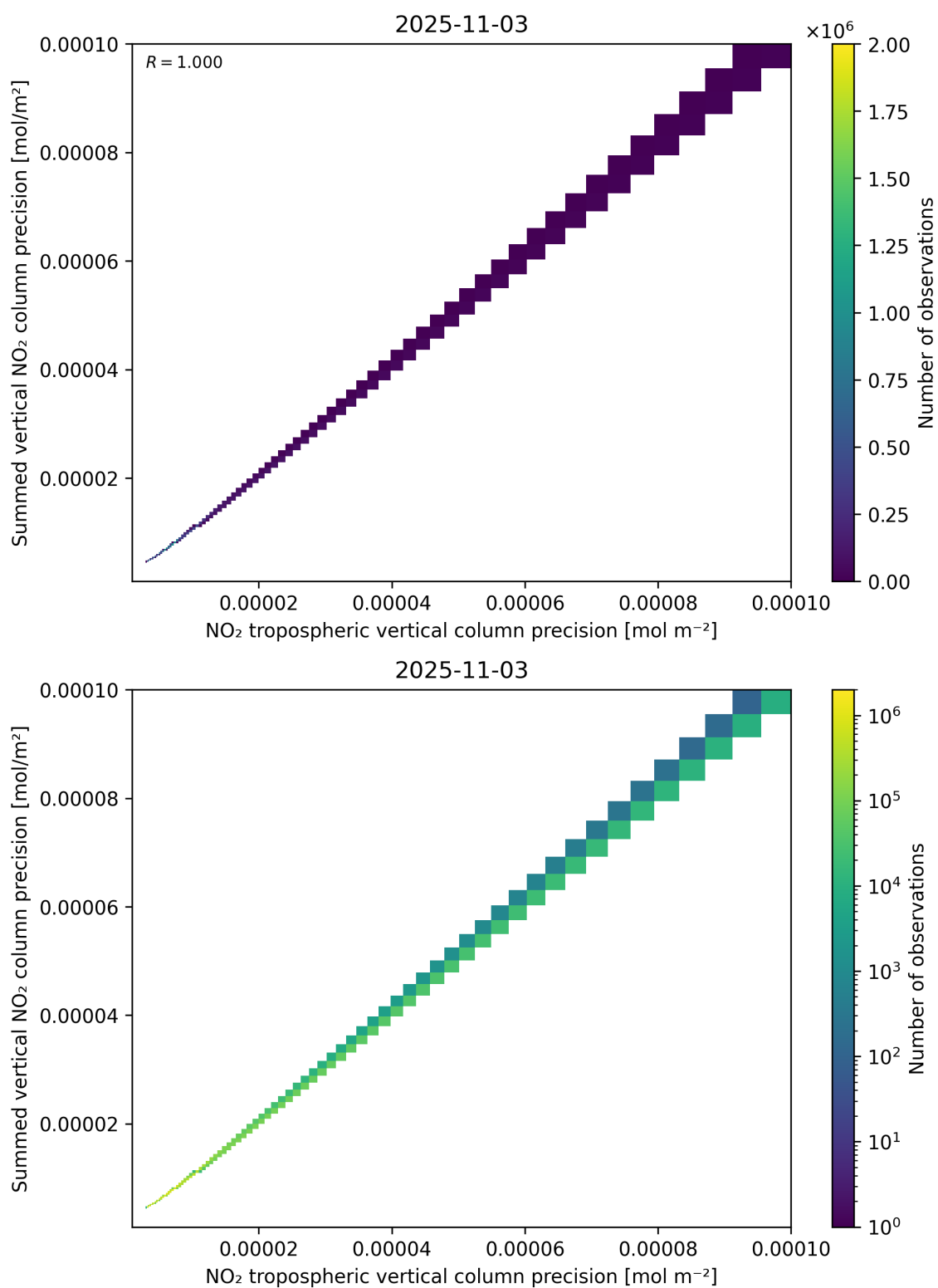
Figure 137: Scatter density plot of “NO 2 tropospheric vertical column precision” against “Summed vertical NO 2 column precision” for 2025-11-02 to 2025-11-04.
