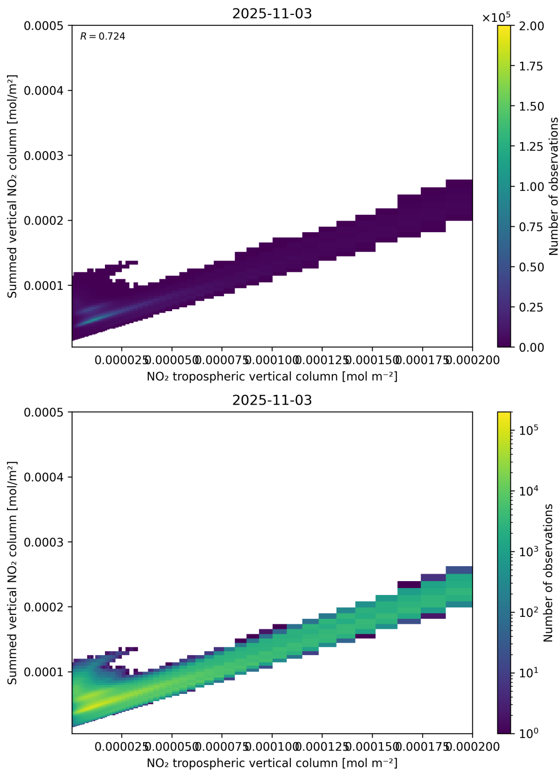
Figure 126: Scatter density plot of “NO 2 tropospheric vertical column” against “Summed vertical NO 2 column” for 2025-11-02 to 2025-11-04.
