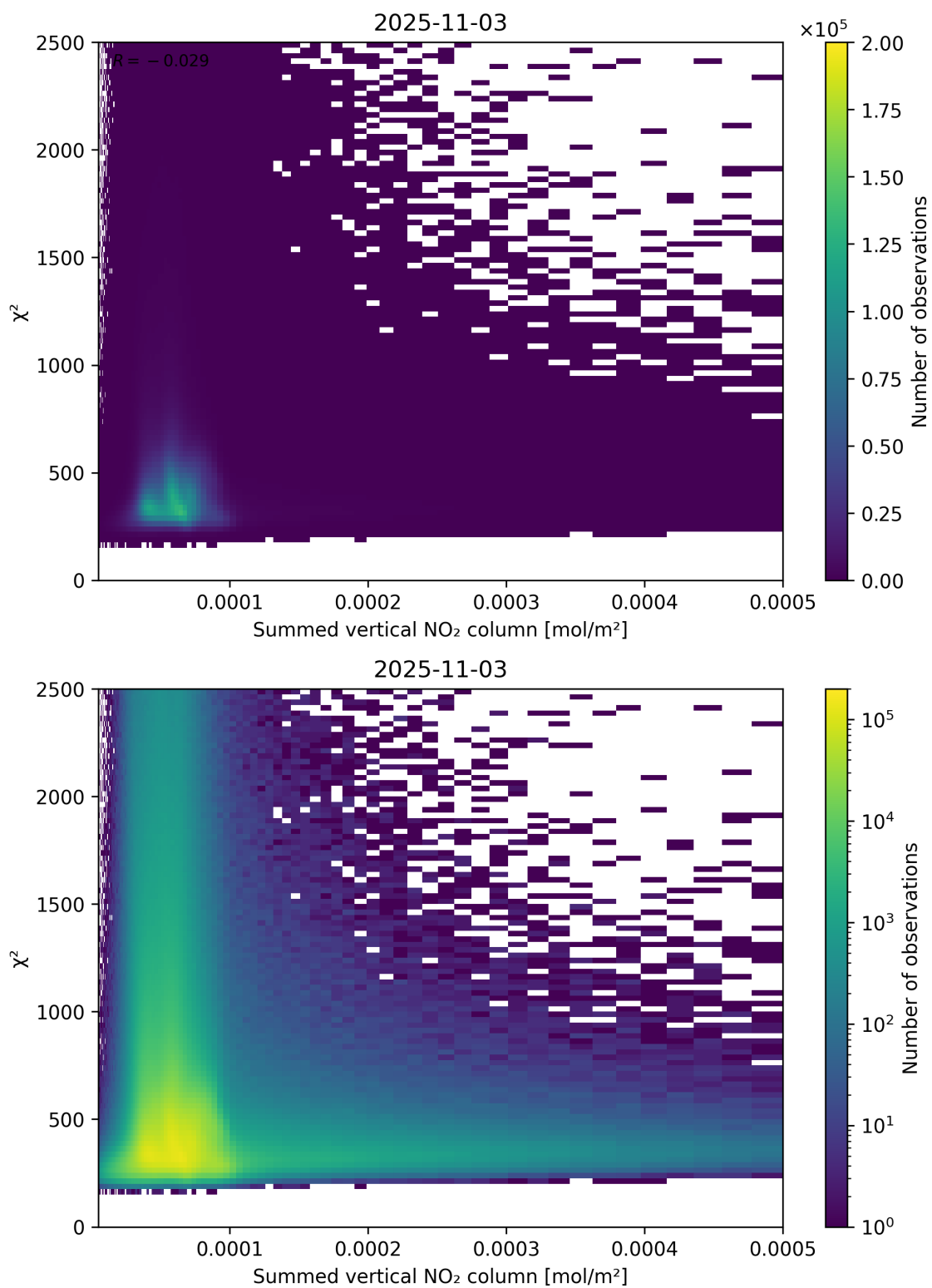
Figure 104: Scatter density plot of “Summed vertical NO 2 column” against “ \chi^2 ” for 2025-11-02 to 2025-11-04.
