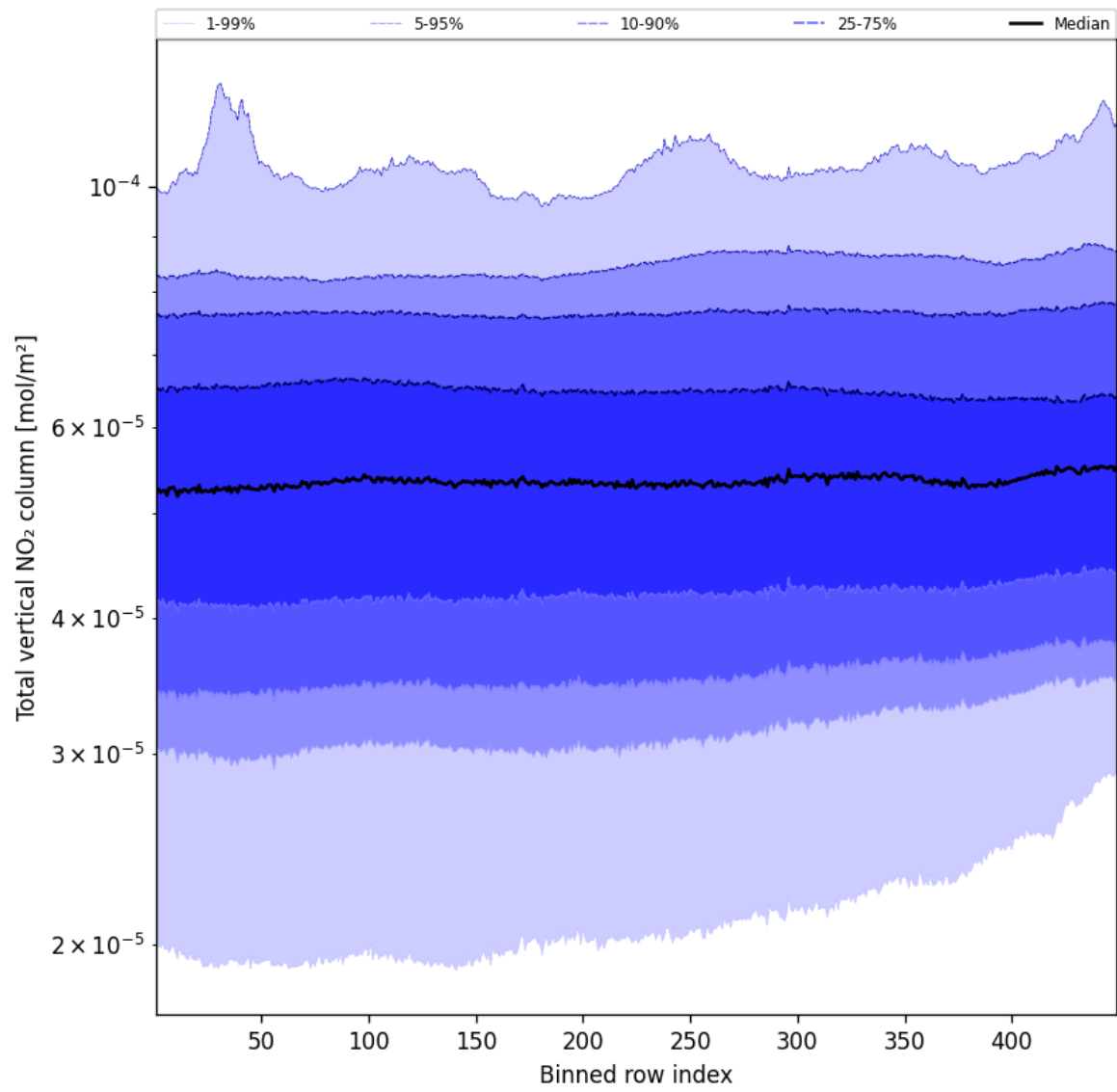
Figure 55: Along track statistics of "Total vertical NO 2 column" for 2025-11-02 to 2025-11-04
