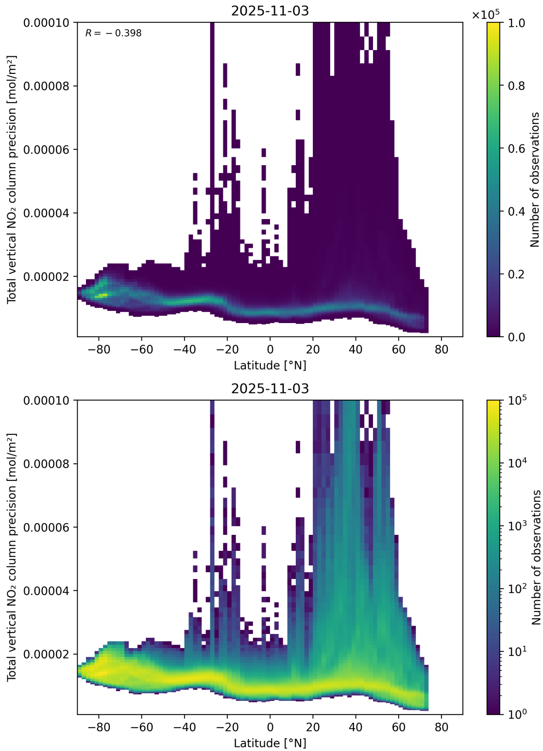
Figure 91: Scatter density plot of “Latitude” against “Total vertical NO 2 column precision” for 2025-11-02 to 2025-11-04.
