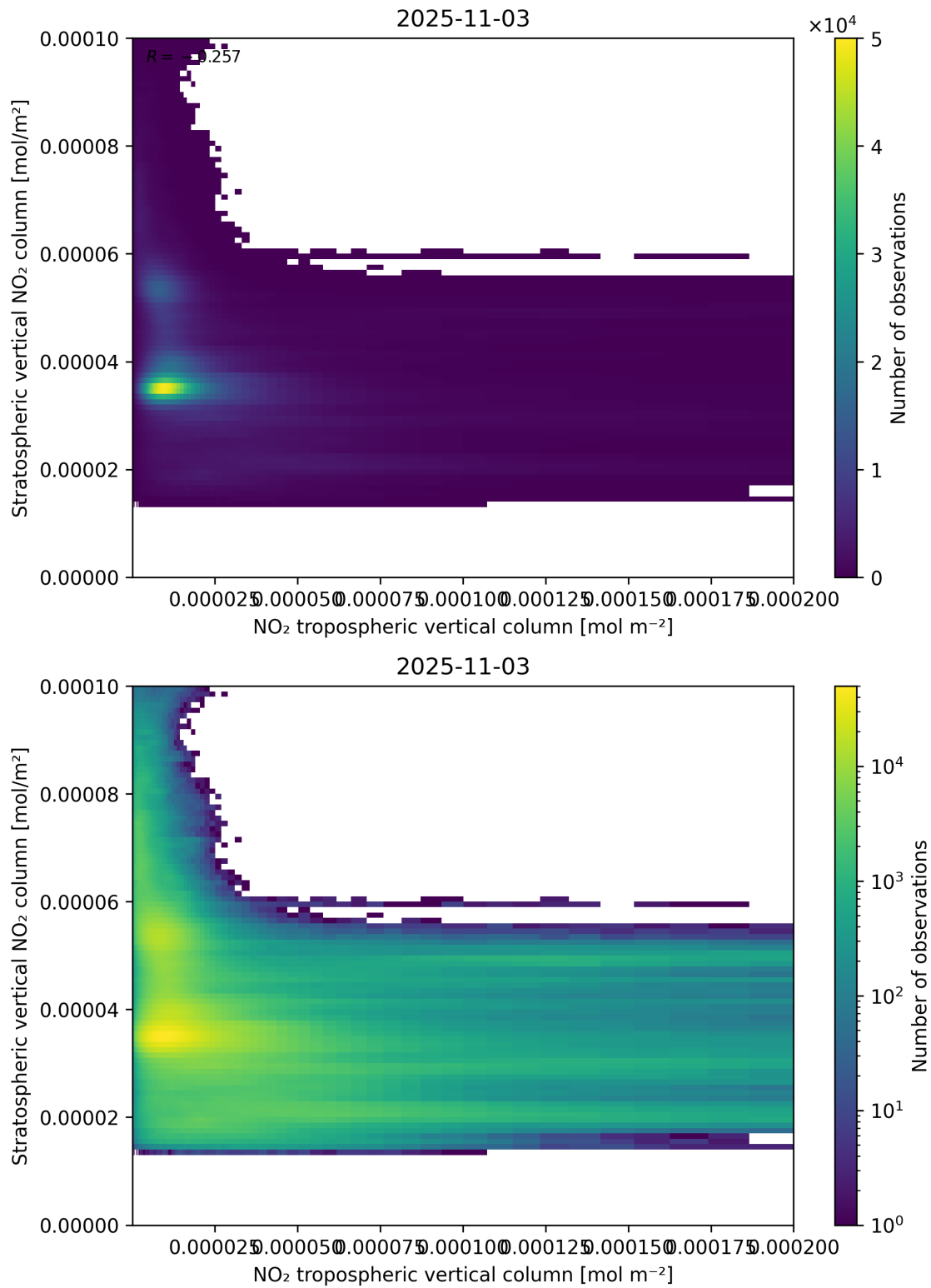
Figure 125: Scatter density plot of “NO 2 tropospheric vertical column” against “Stratospheric vertical NO 2 column” for 2025-11-02 to 2025-11-04.
