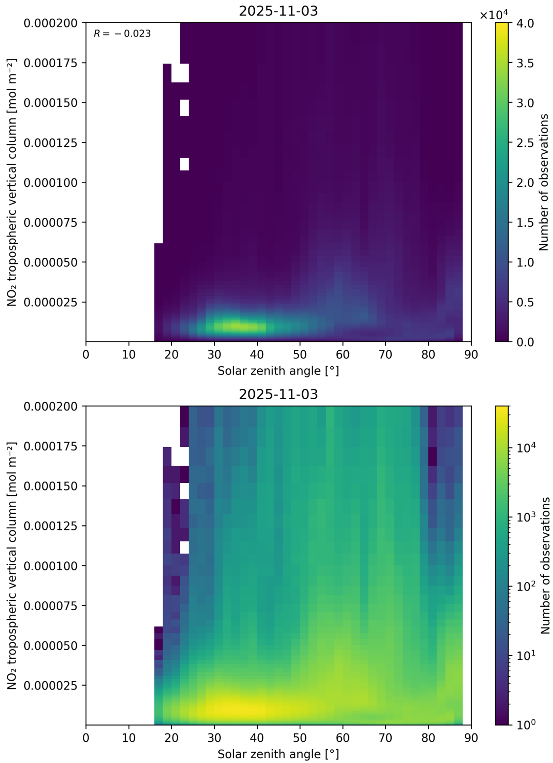
Figure 155: Scatter density plot of “Solar zenith angle” against “NO 2 tropospheric vertical column” for 2025-11-02 to 2025-11-04.
