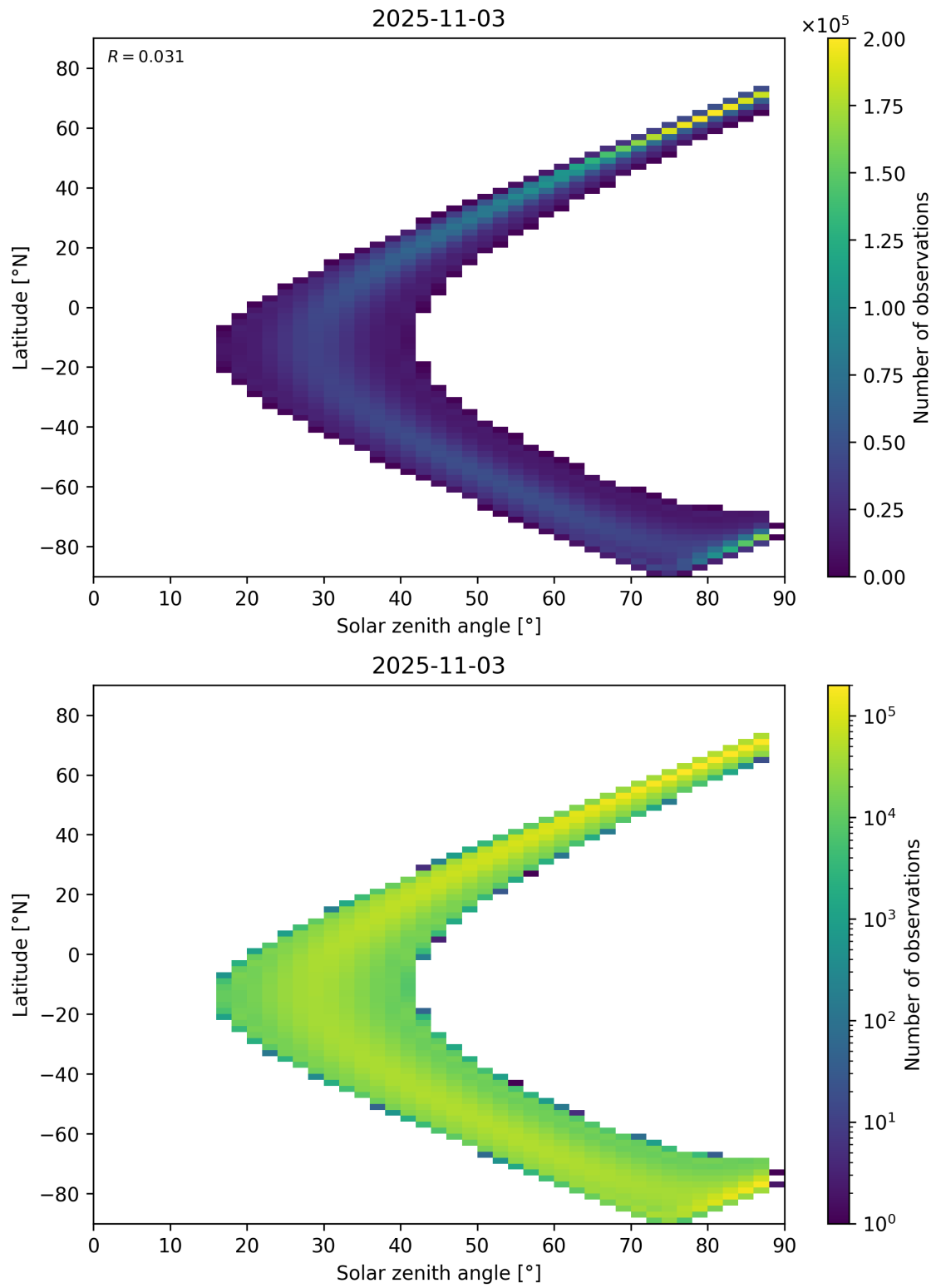
Figure 149: Scatter density plot of “Solar zenith angle” against “Latitude” for 2025-11-02 to 2025-11-04.
