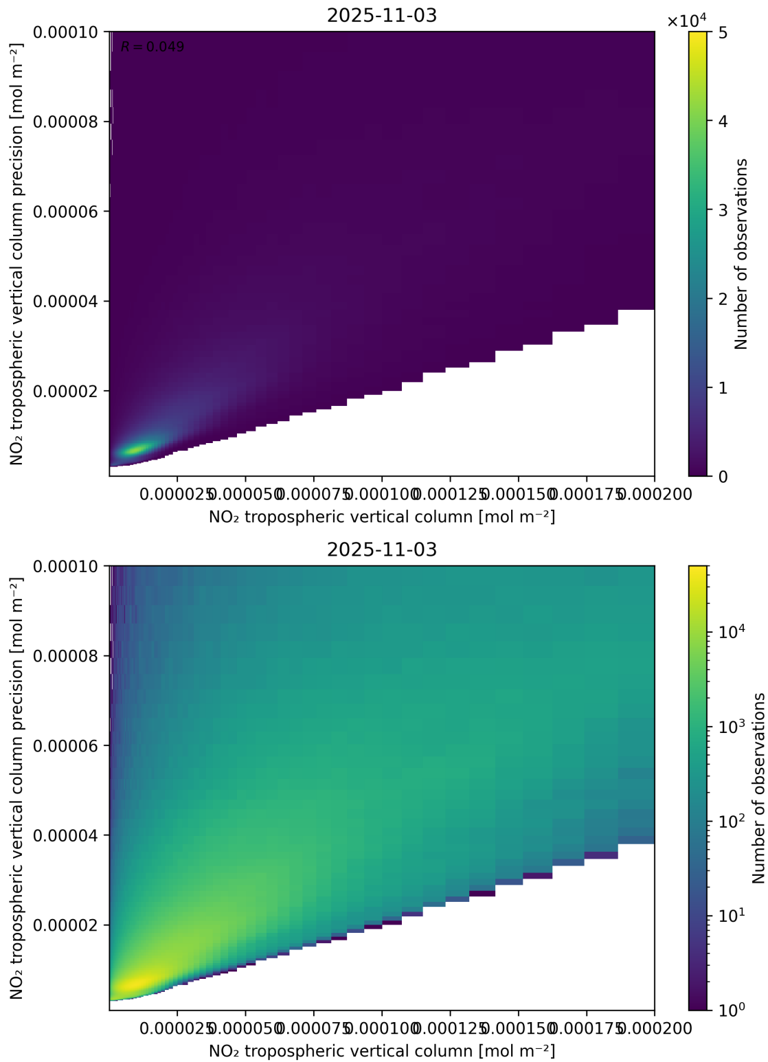
Figure 130: Scatter density plot of “NO 2 tropospheric vertical column” against “NO 2 tropospheric vertical column precision” for 2025-11-02 to 2025-11-04.
