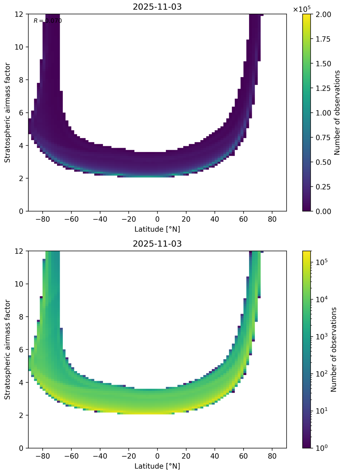
Figure 83: Scatter density plot of “Latitude” against “Stratospheric air mass factor” for 2025-11-02 to 2025-11-04.
