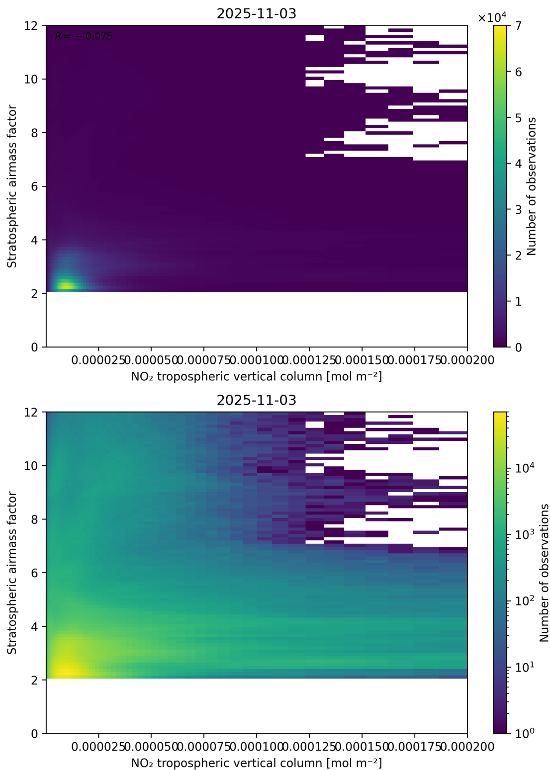
Figure 121: Scatter density plot of “NO 2 tropospheric vertical column” against “Stratospheric airmass factor” for 2025-11-02 to 2025-11-04.
