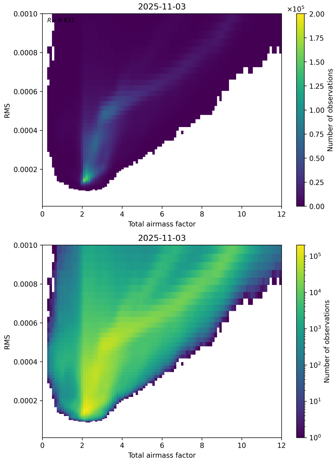
Figure 69: Scatter density plot of “Total airmass factor” against “RMS” for 2025-11-02 to 2025-11-04.
