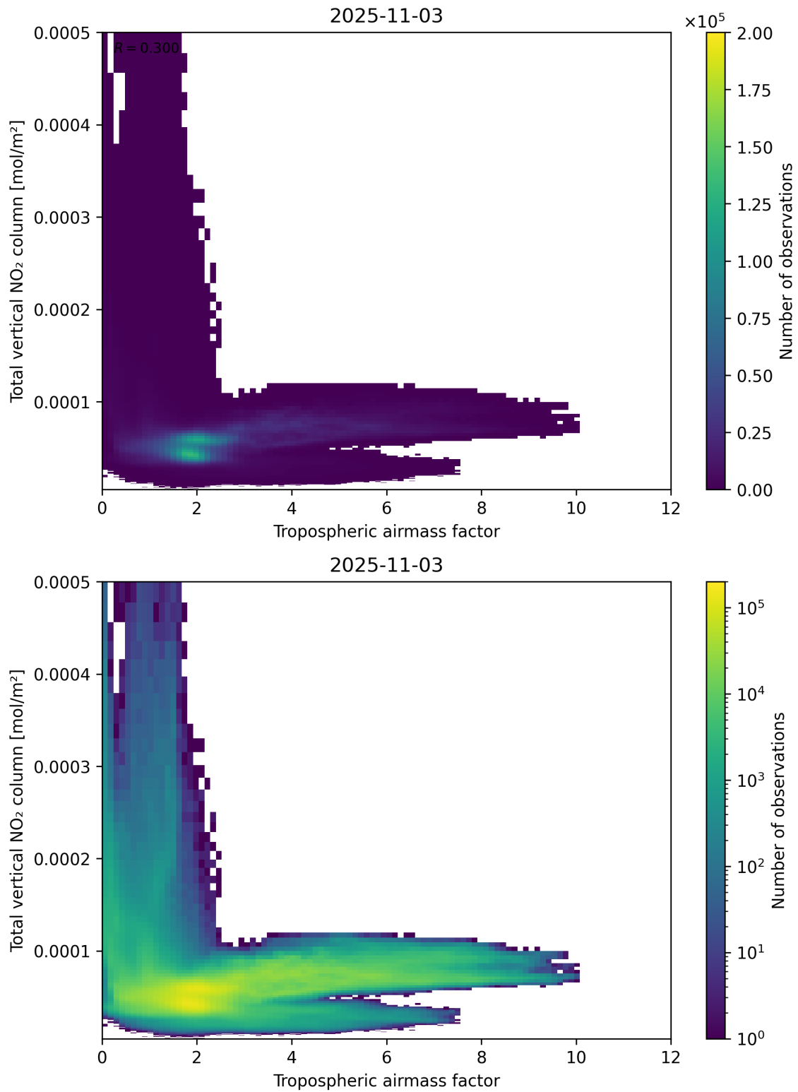
Figure 77: Scatter density plot of “Tropospheric airmass factor” against “Total vertical \text{NO}_2 column” for 2025-11-02 to 2025-11-04.
