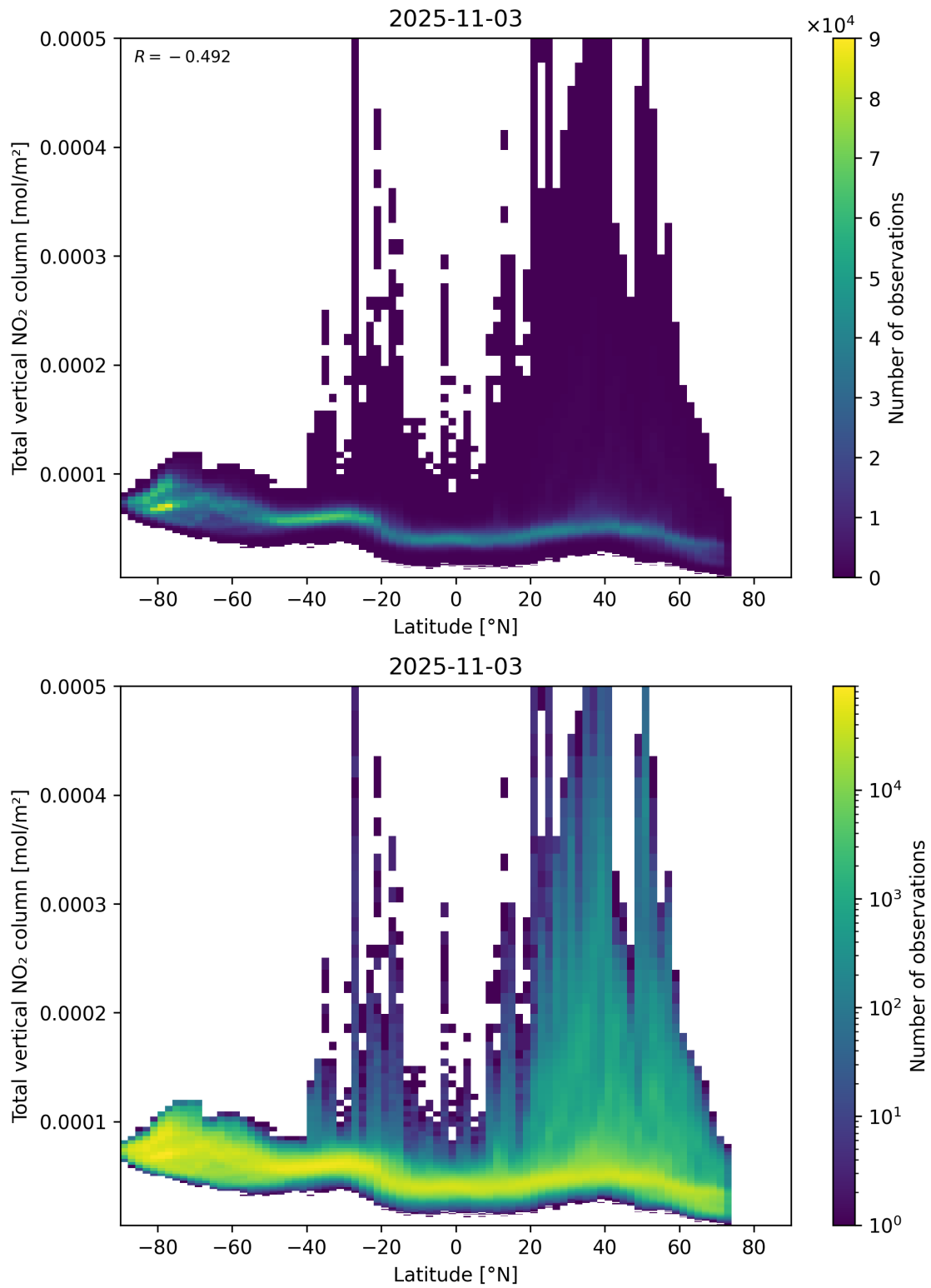
Figure 90: Scatter density plot of “Latitude” against “Total vertical NO 2 column” for 2025-11-02 to 2025-11-04.
