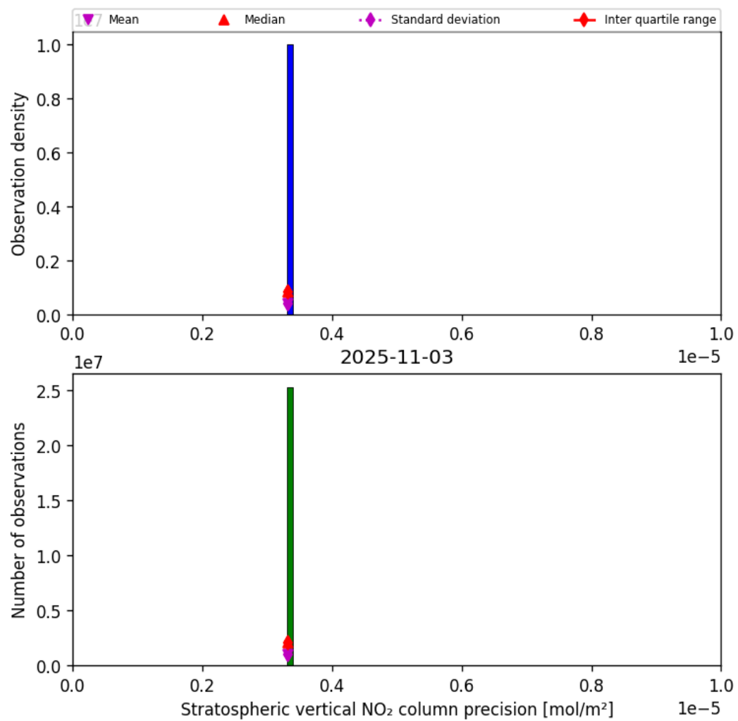
Figure 37: Histogram of “Stratospheric vertical NO 2 column precision” for 2025-11-02 to 2025-11-04
