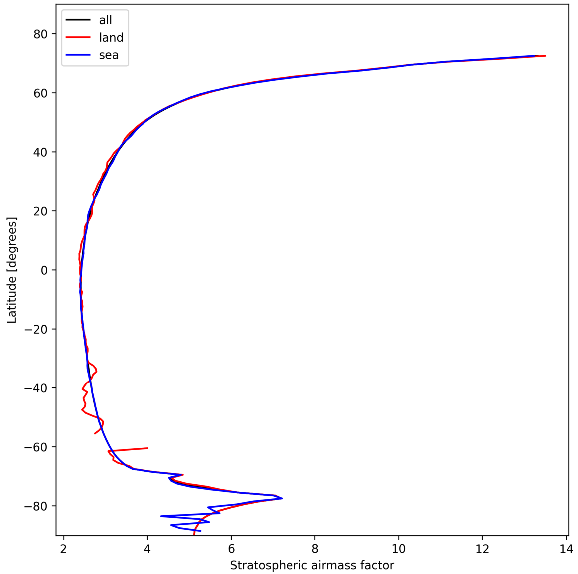
Figure 27: Zonal average of “Stratospheric air mass factor” for 2025-11-02 to 2025-11-04.
