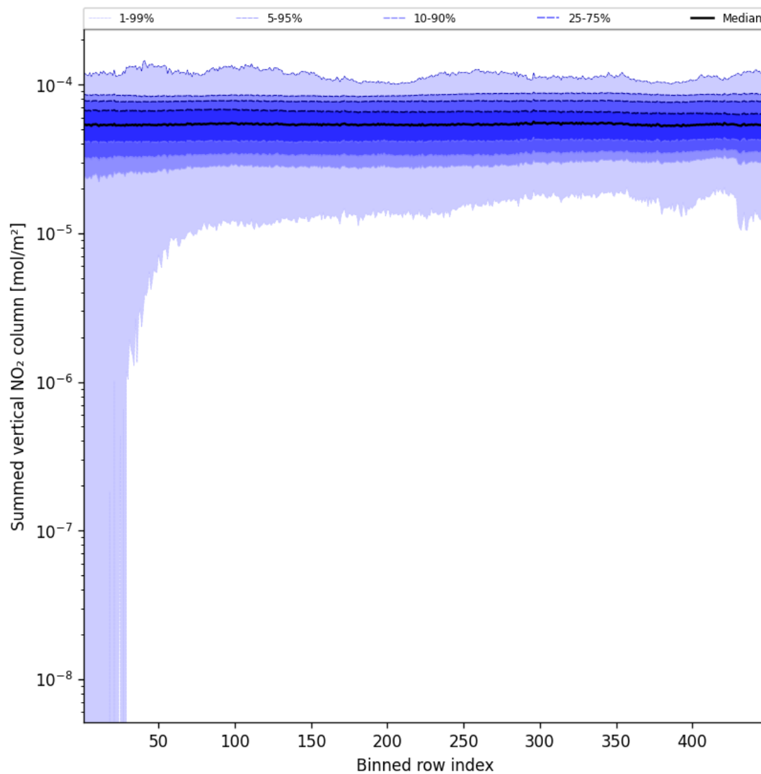
Figure 57: Along track statistics of “Summed vertical NO 2 column” for 2025-11-02 to 2025-11-04
