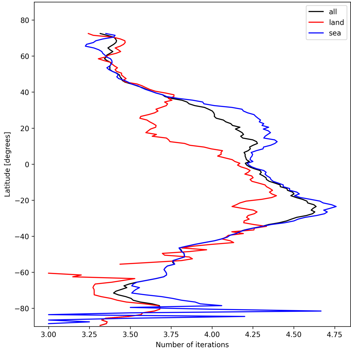
Figure 17: Zonal average of “Number of iterations” for 2025-11-02 to 2025-11-04.
