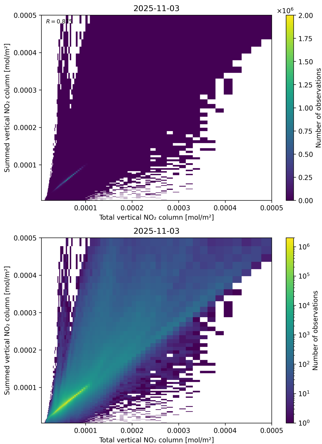
Figure 112: Scatter density plot of “Total vertical NO 2 column” against “Summed vertical NO 2 column” for 2025-11-02 to 2025-11-04.
