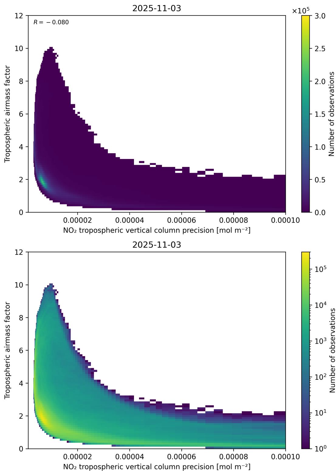
Figure 133: Scatter density plot of “NO 2 tropospheric vertical column precision” against “Tropospheric airmass factor” for 2025-11-02 to 2025-11-04.
