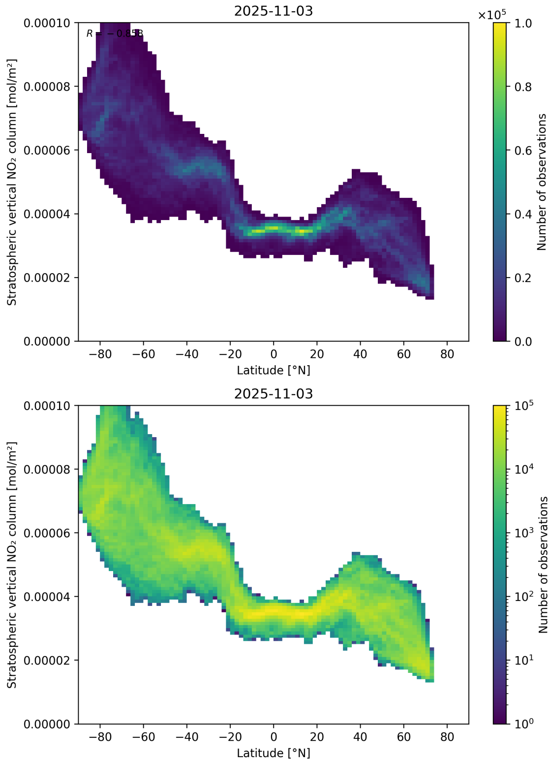
Figure 87: Scatter density plot of “Latitude” against “Stratospheric vertical NO 2 column” for 2025-11-02 to 2025-11-04.
