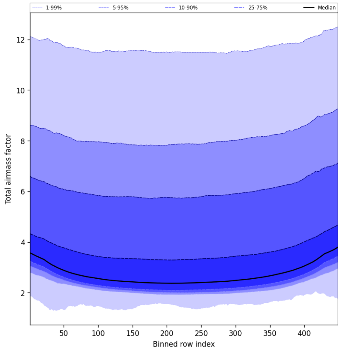
Figure 49: Along track statistics of “Total airmass factor” for 2025-11-02 to 2025-11-04
