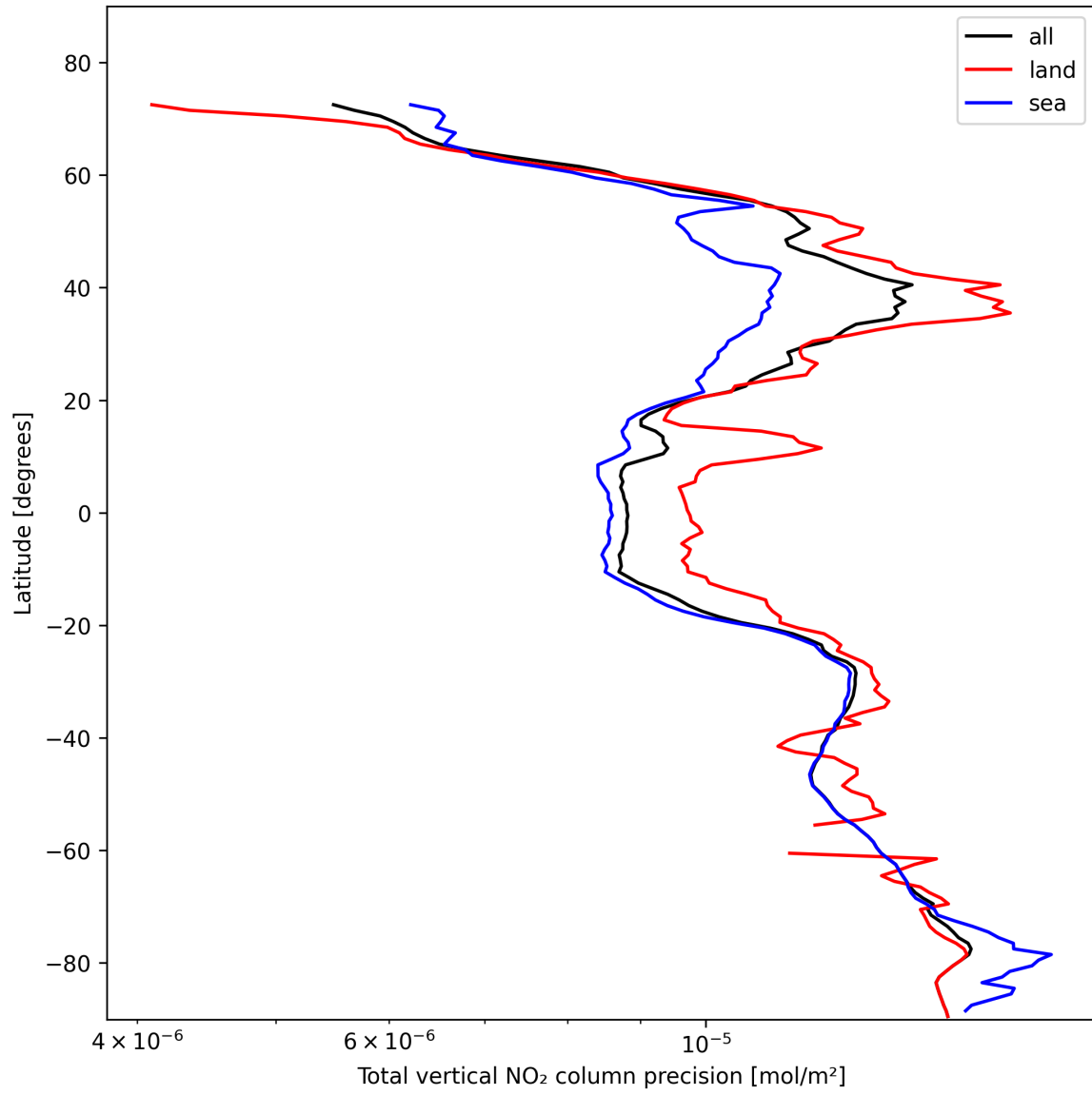
Figure 22: Zonal average of “Total vertical NO 2 column precision” for 2025-11-02 to 2025-11-04.
