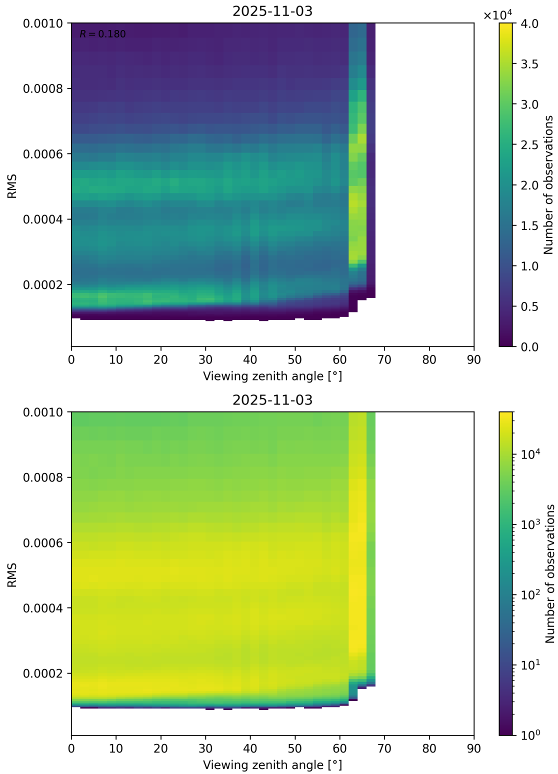
Figure 171: Scatter density plot of “Viewing zenith angle” against “RMS” for 2025-11-02 to 2025-11-04.
