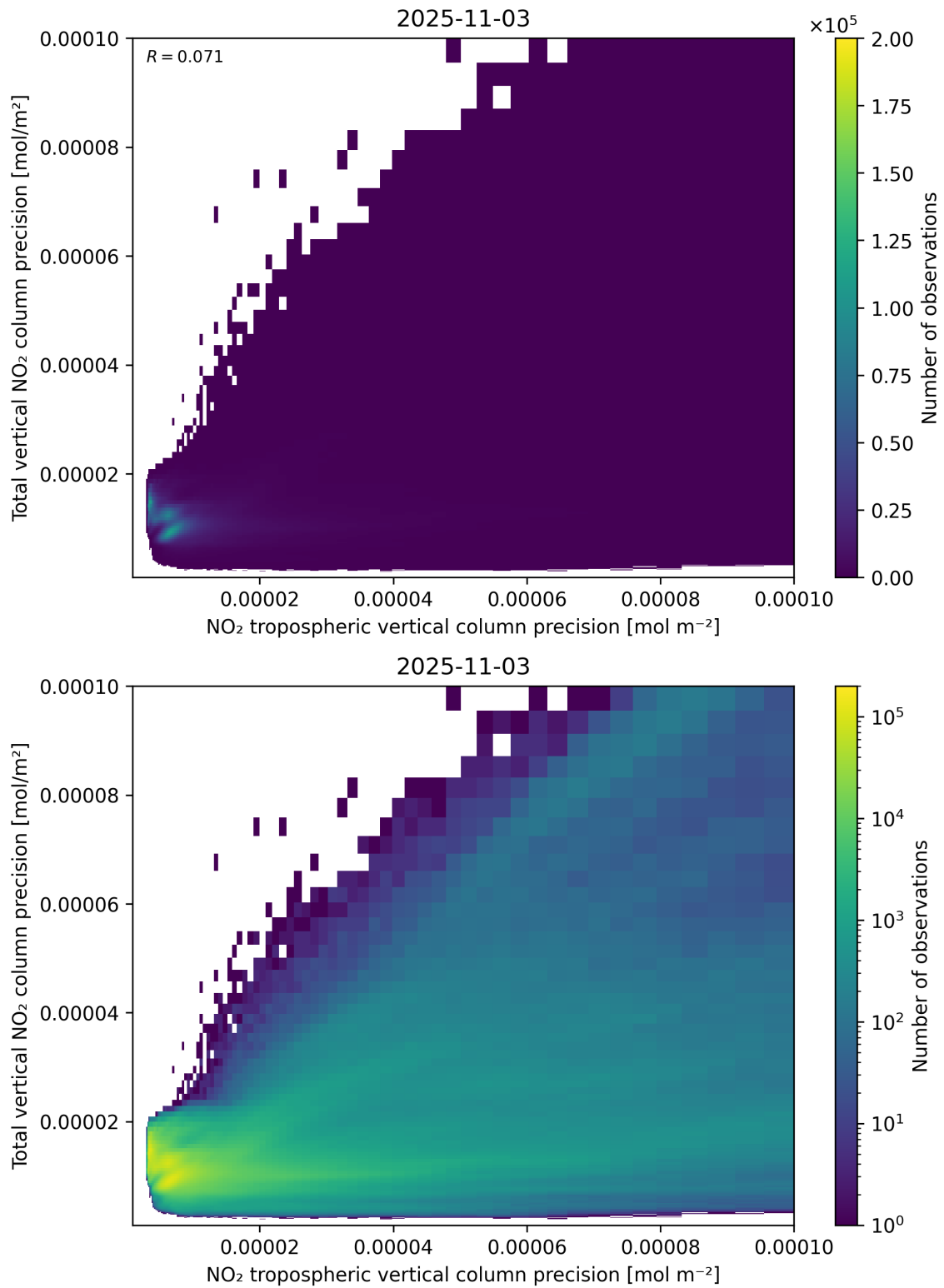
Figure 139: Scatter density plot of “NO 2 tropospheric vertical column precision” against “Total vertical NO 2 column precision” for 2025-11-02 to 2025-11-04.
