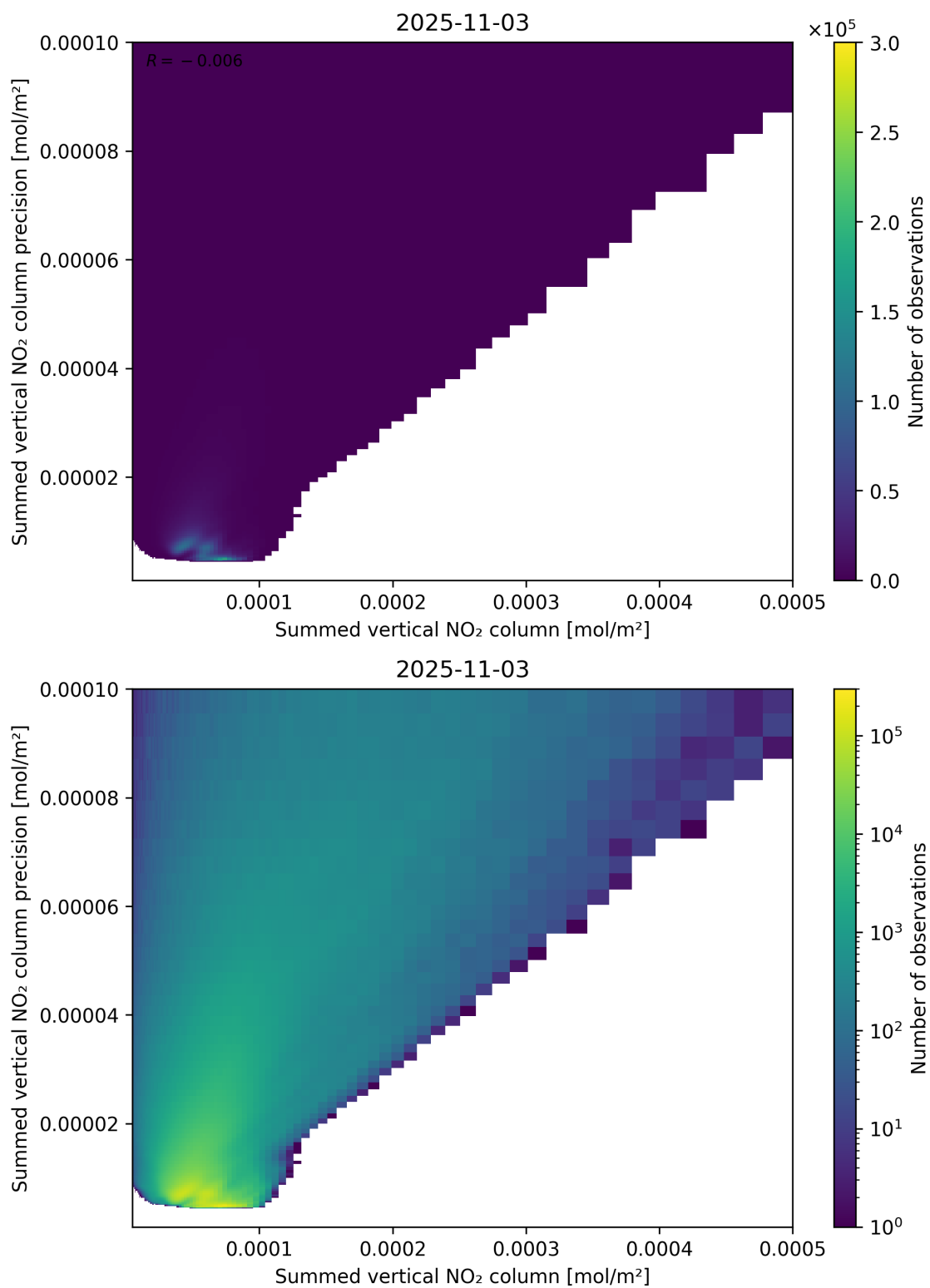
Figure 105: Scatter density plot of “Summed vertical NO 2 column” against “Summed vertical NO 2 column precision” for 2025-11-02 to 2025-11-04.
