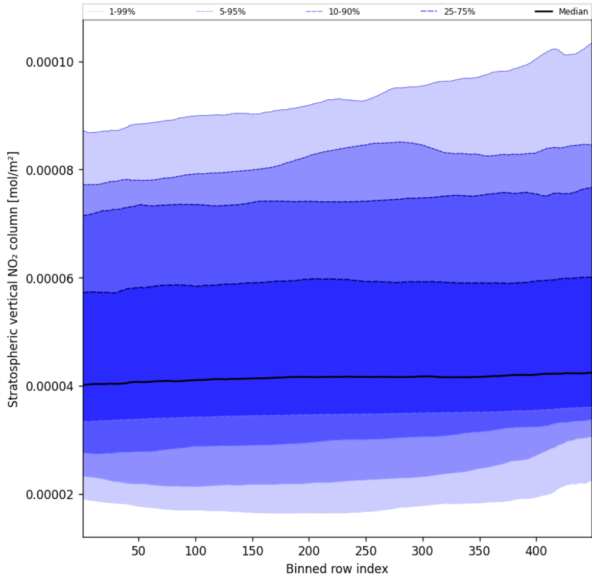
Figure 53: Along track statistics of “Stratospheric vertical NO 2 column” for 2025-11-02 to 2025-11-04
