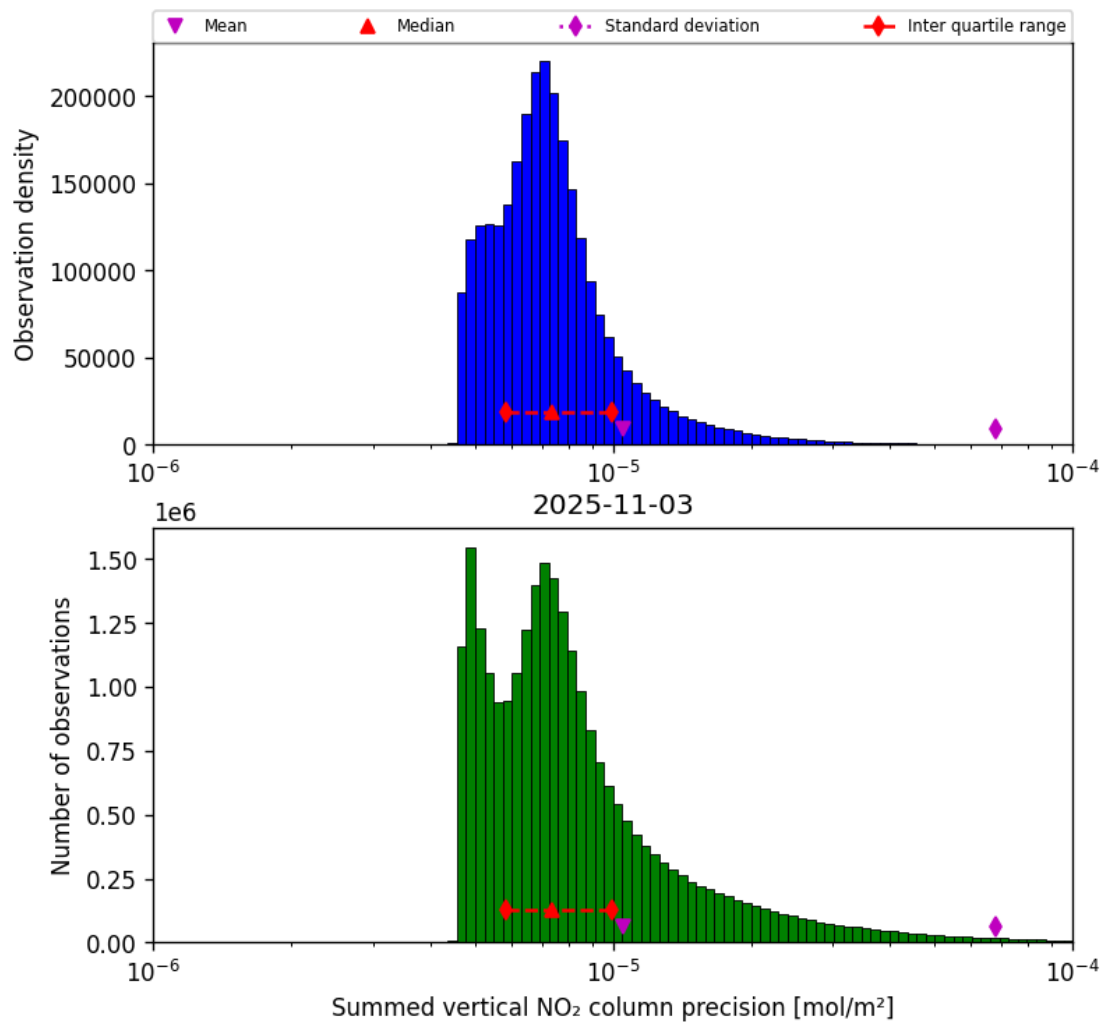
Figure 41: Histogram of “Summed vertical NO 2 column precision” for 2025-11-02 to 2025-11-04
