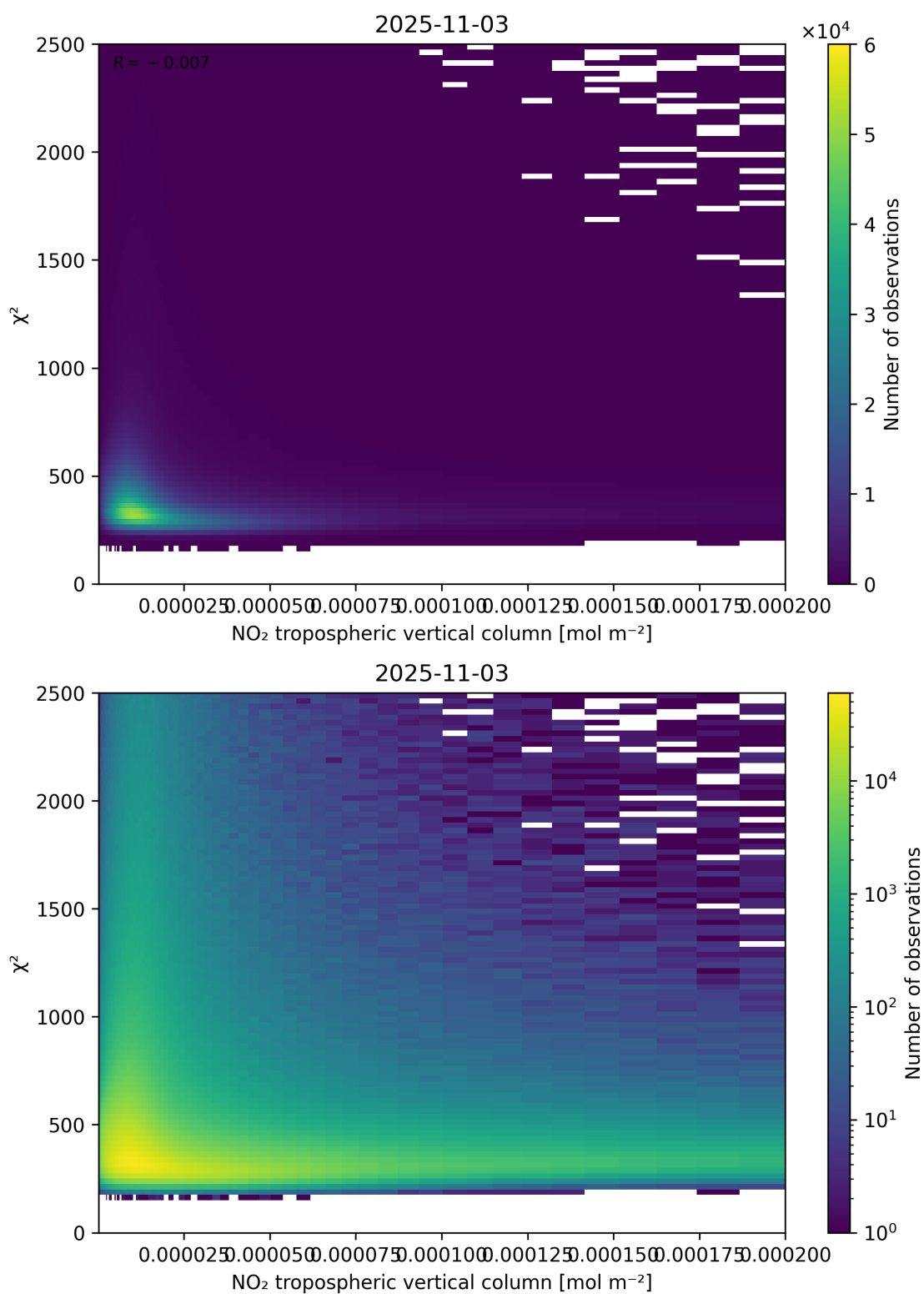
Figure 124: Scatter density plot of “NO 2 tropospheric vertical column” against “ \chi^2 ” for 2025-11-02 to 2025-11-04.
