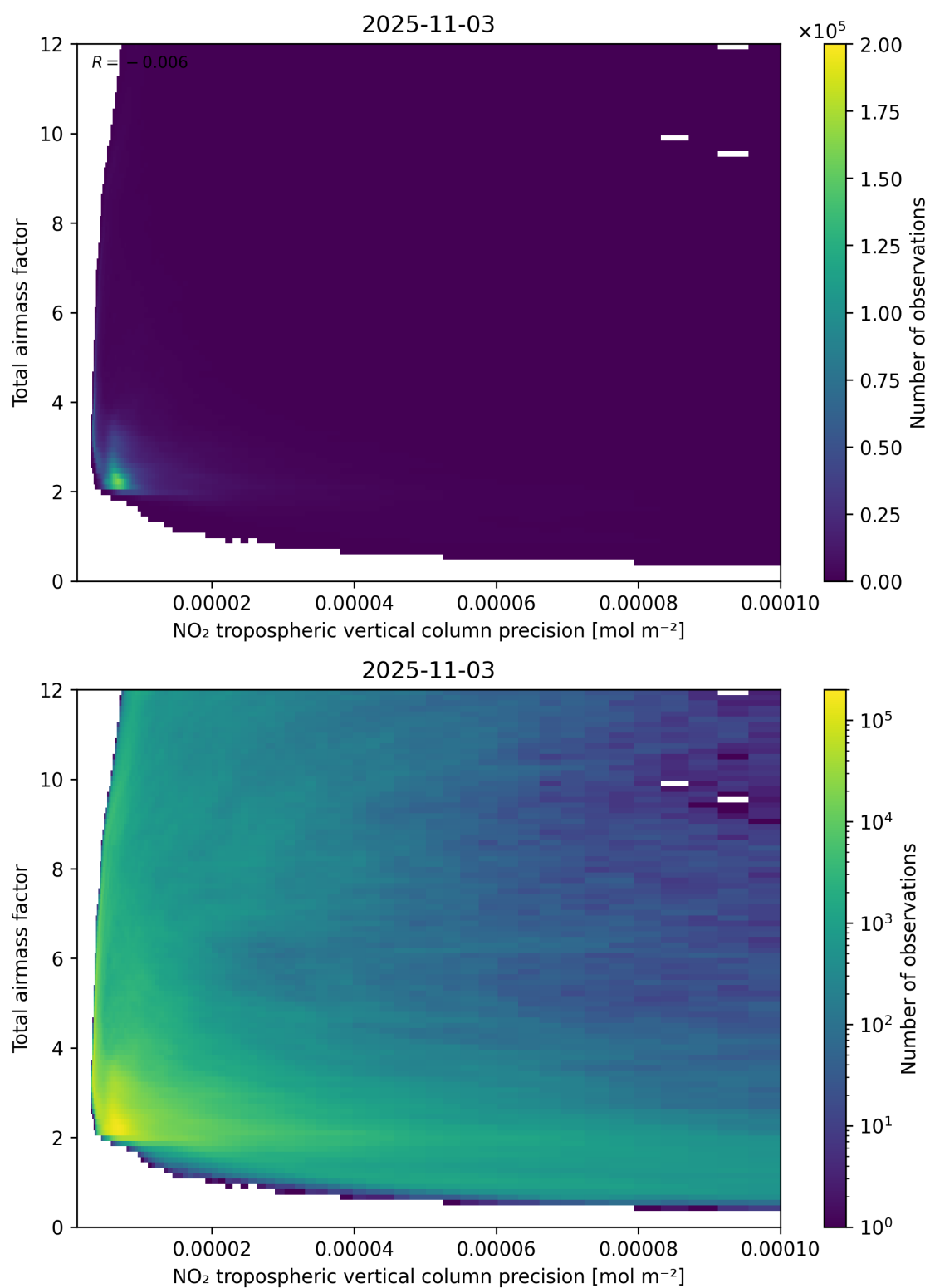
Figure 132: Scatter density plot of “NO 2 tropospheric vertical column precision” against “Total air mass factor” for 2025-11-02 to 2025-11-04.
