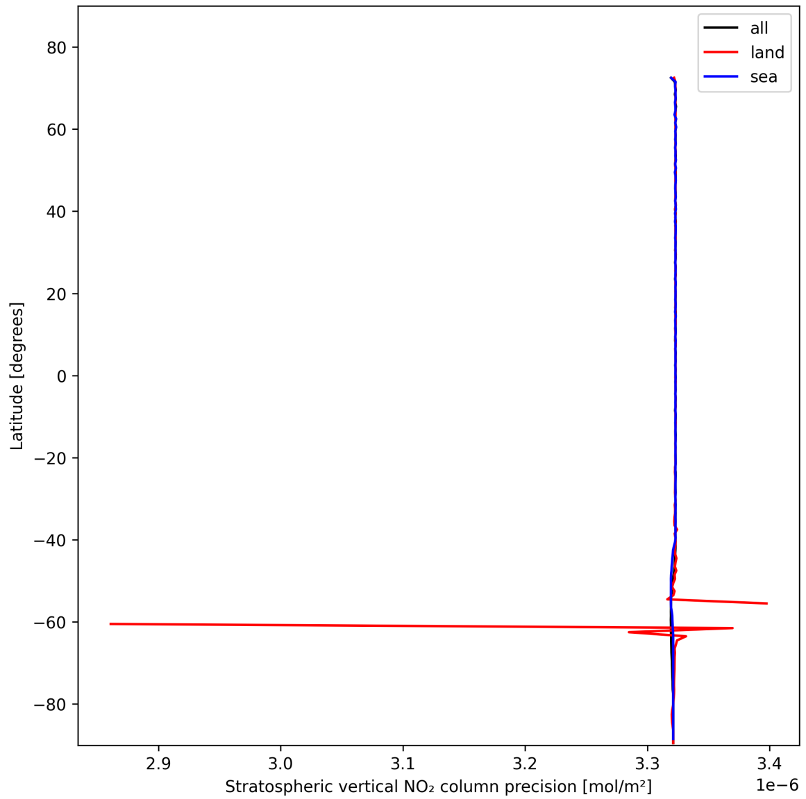
Figure 20: Zonal average of “Stratospheric vertical NO 2 column precision” for 2025-11-02 to 2025-11-04.
