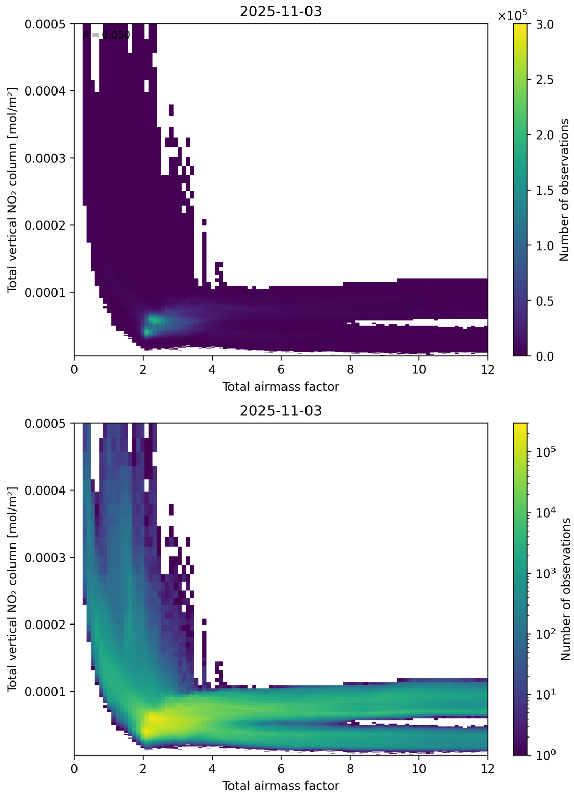
Figure 67: Scatter density plot of “Total airmass factor” against “Total vertical NO 2 column” for 2025-11-02 to 2025-11-04.
