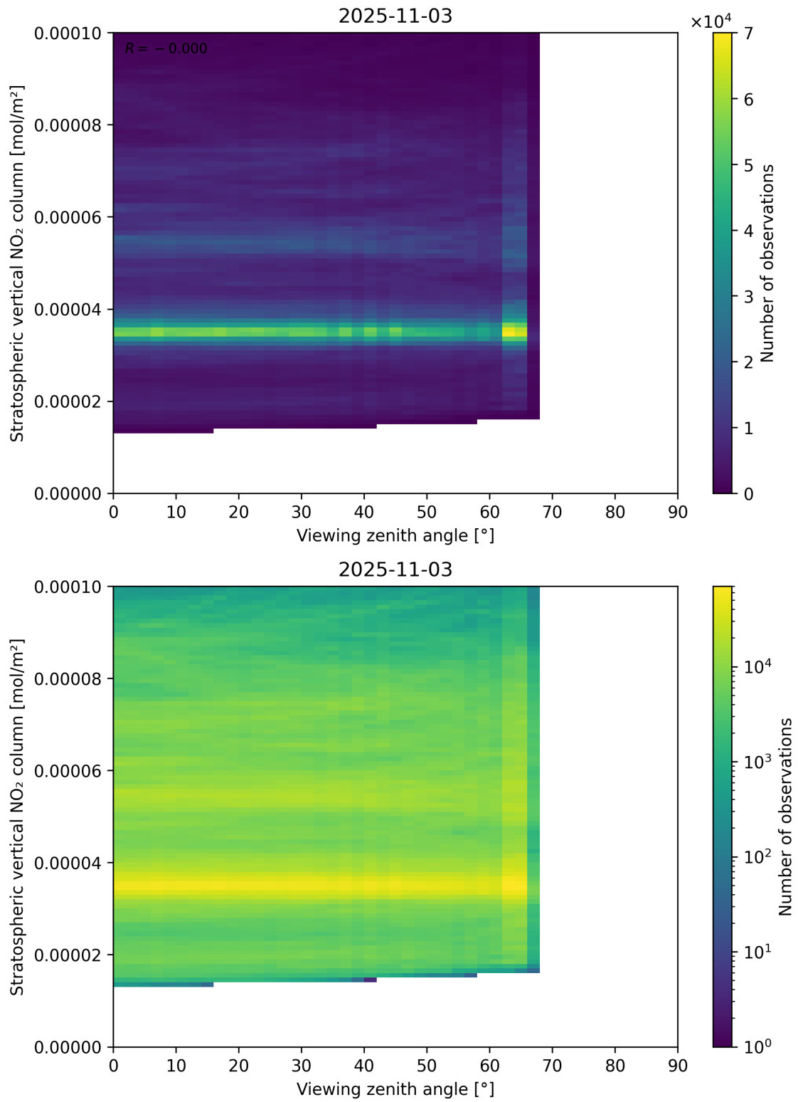
Figure 164: Scatter density plot of “Viewing zenith angle” against “Stratospheric vertical NO 2 column” for 2025-11-02 to 2025-11-04.
