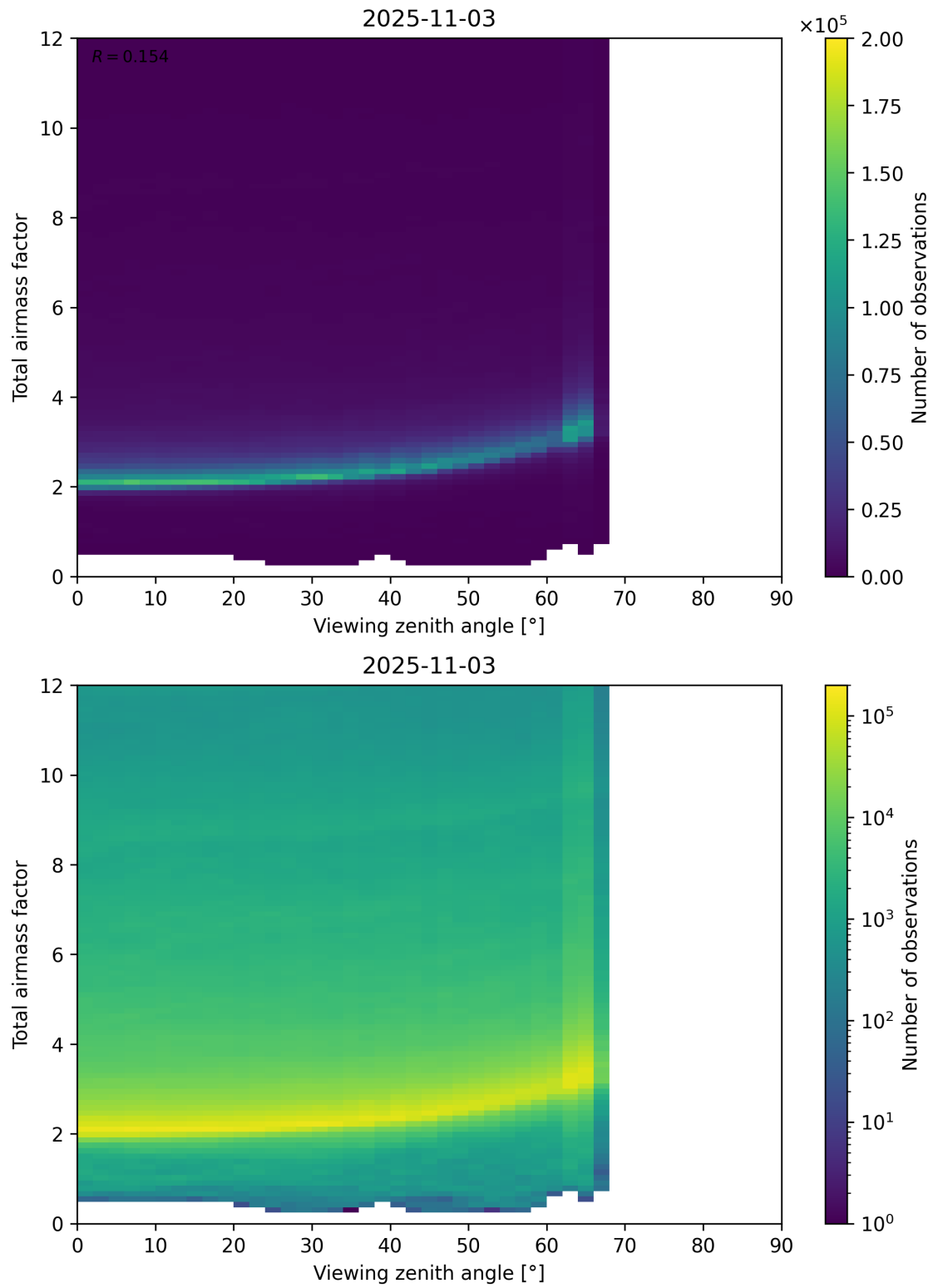
Figure 160: Scatter density plot of “Viewing zenith angle” against “Total airmass factor” for 2025-11-02 to 2025-11-04.
