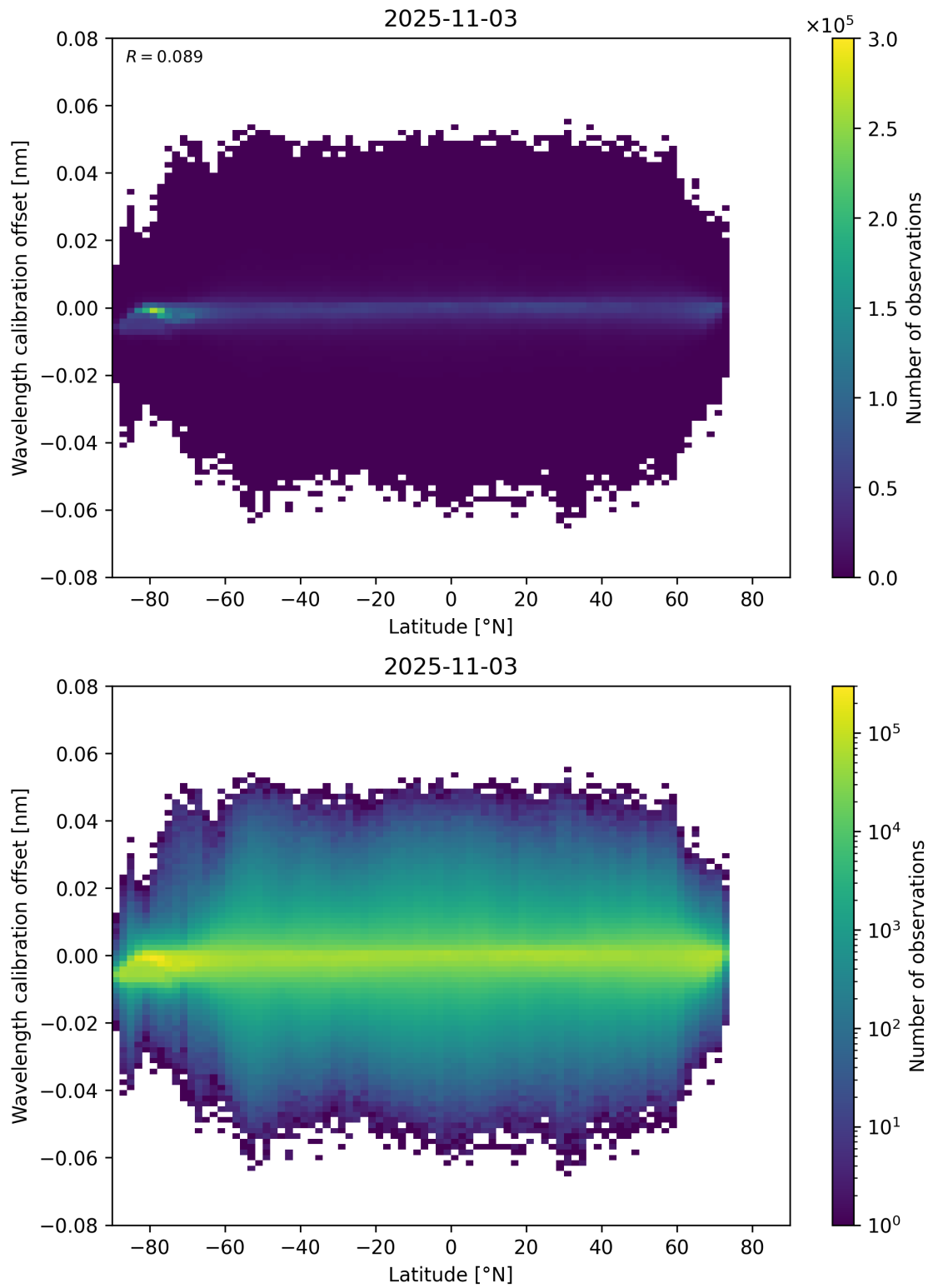
Figure 95: Scatter density plot of “Latitude” against “Wavelength calibration offset” for 2025-11-02 to 2025-11-04.
