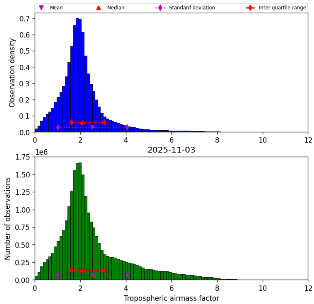
Figure 31: Histogram of “Tropospheric airmass factor” for 2025-11-02 to 2025-11-04
