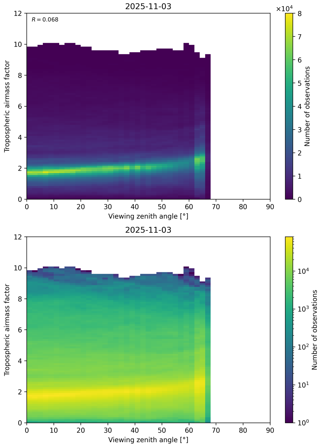
Figure 161: Scatter density plot of “Viewing zenith angle” against “Tropospheric airmass factor” for 2025-11-02 to 2025-11-04.
