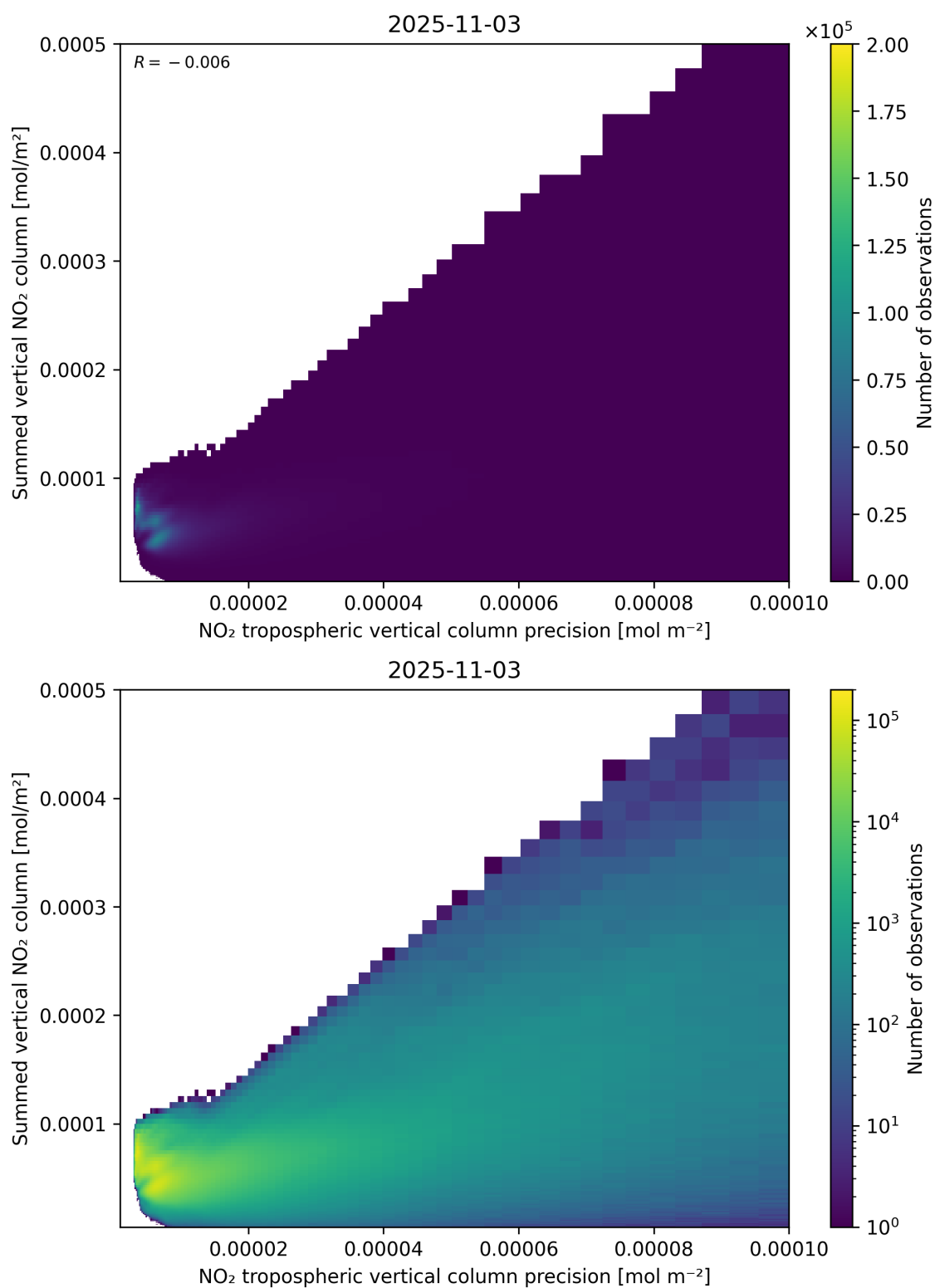
Figure 136: Scatter density plot of “NO 2 tropospheric vertical column precision” against “Summed vertical NO 2 column” for 2025-11-02 to 2025-11-04.
