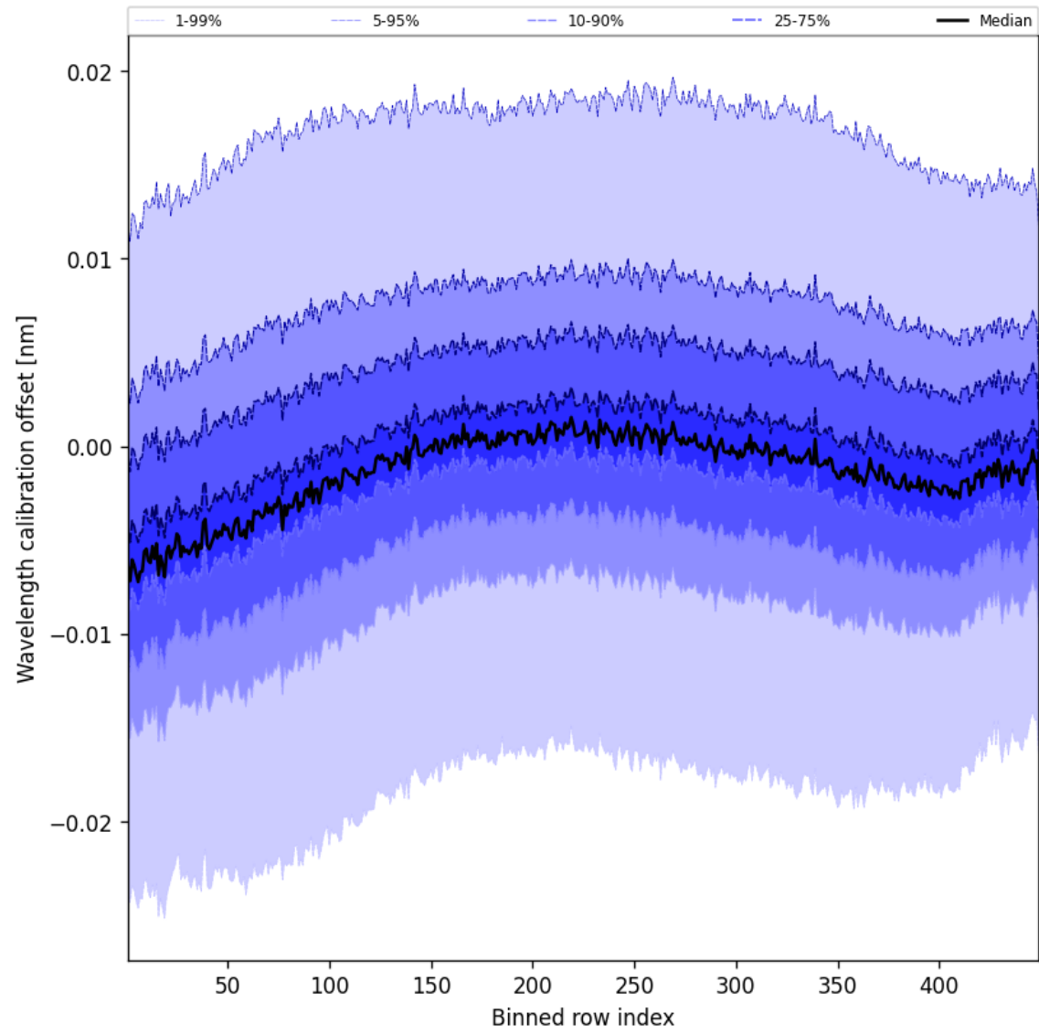
Figure 52: Along track statistics of “Wavelength calibration offset” for 2025-11-02 to 2025-11-04
