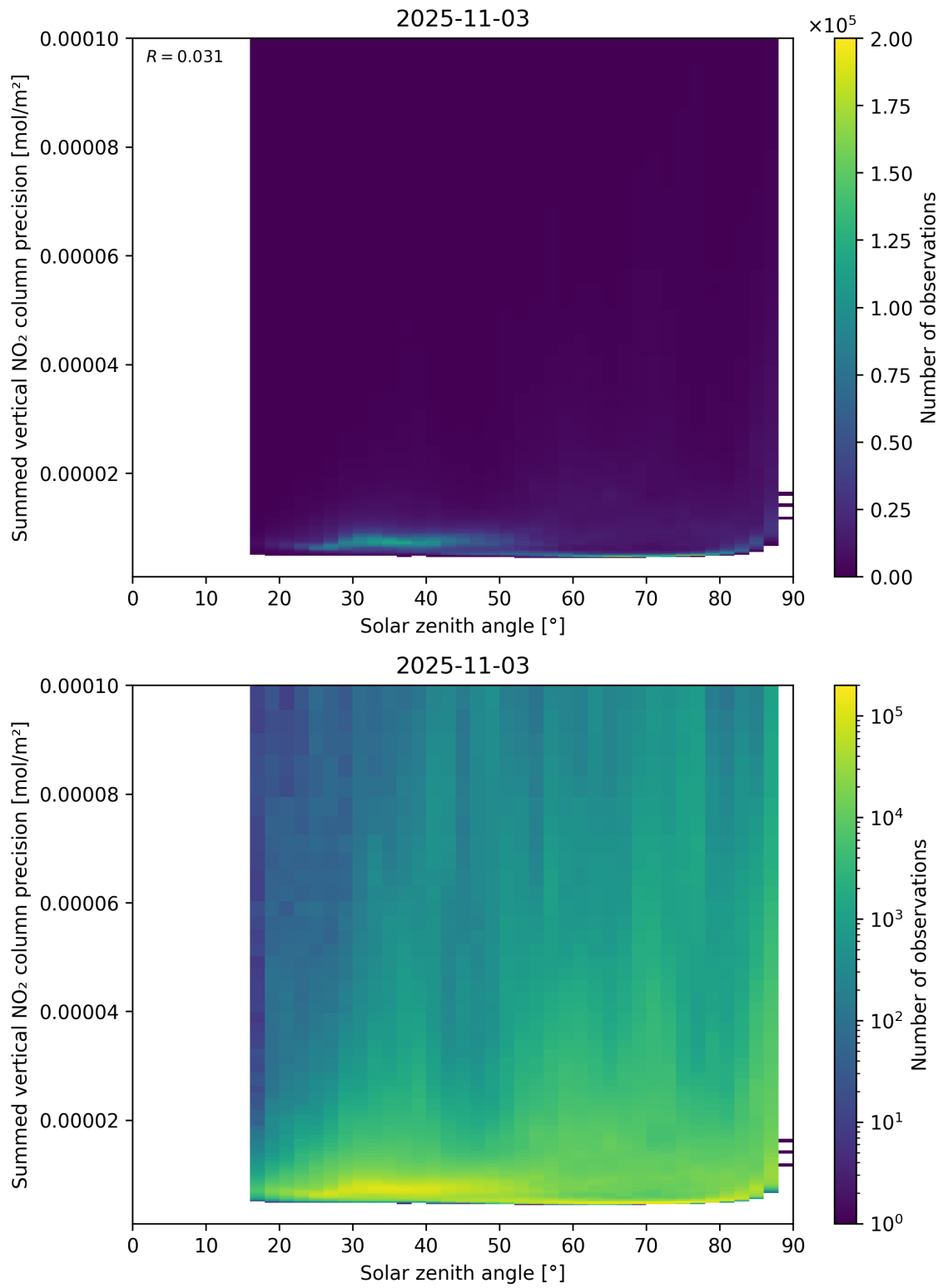
Figure 152: Scatter density plot of “Solar zenith angle” against “Summed vertical NO 2 column precision” for 2025-11-02 to 2025-11-04.
