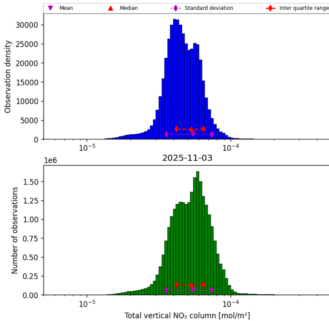
Figure 38: Histogram of “Total vertical NO 2 column” for 2025-11-02 to 2025-11-04
