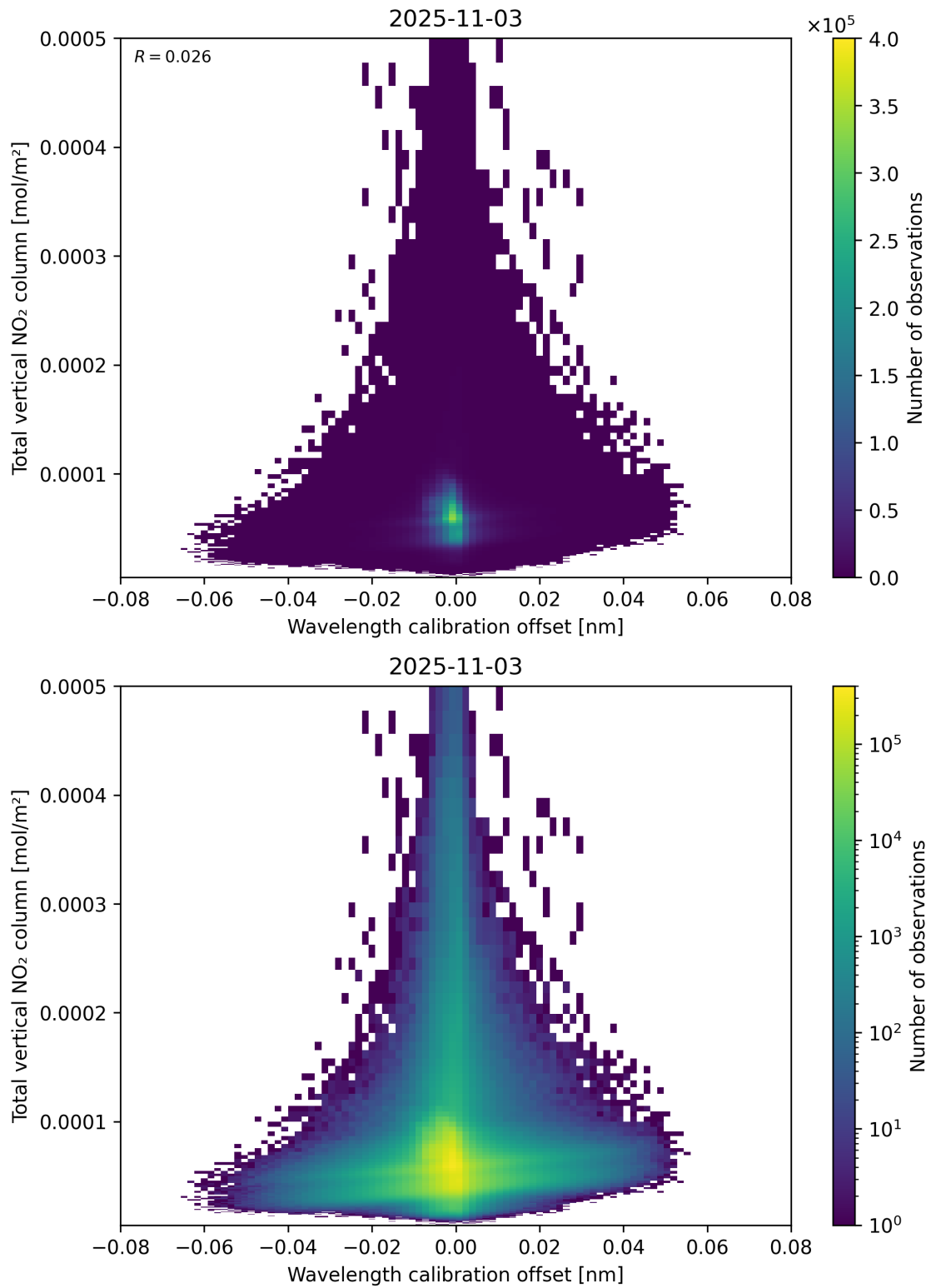
Figure 179: Scatter density plot of “Wavelength calibration offset” against “Total vertical NO 2 column” for 2025-11-02 to 2025-11-04.
