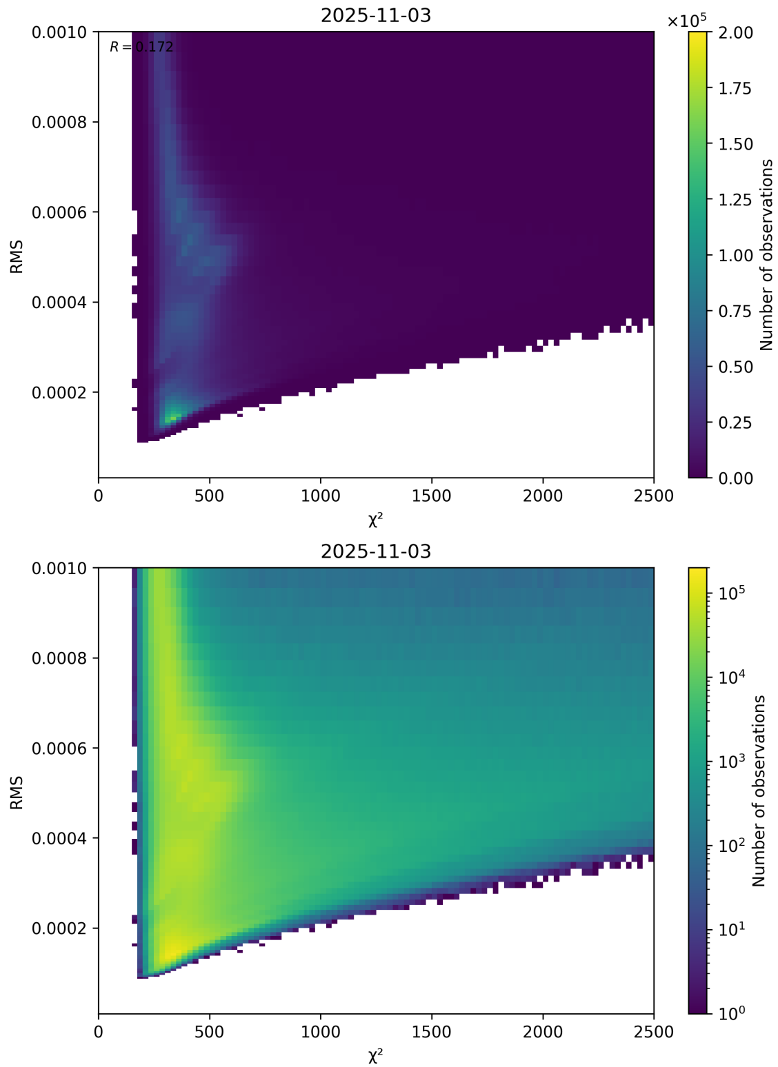
Figure 82: Scatter density plot of “ \chi^2 ” against “RMS” for 2025-11-02 to 2025-11-04.
