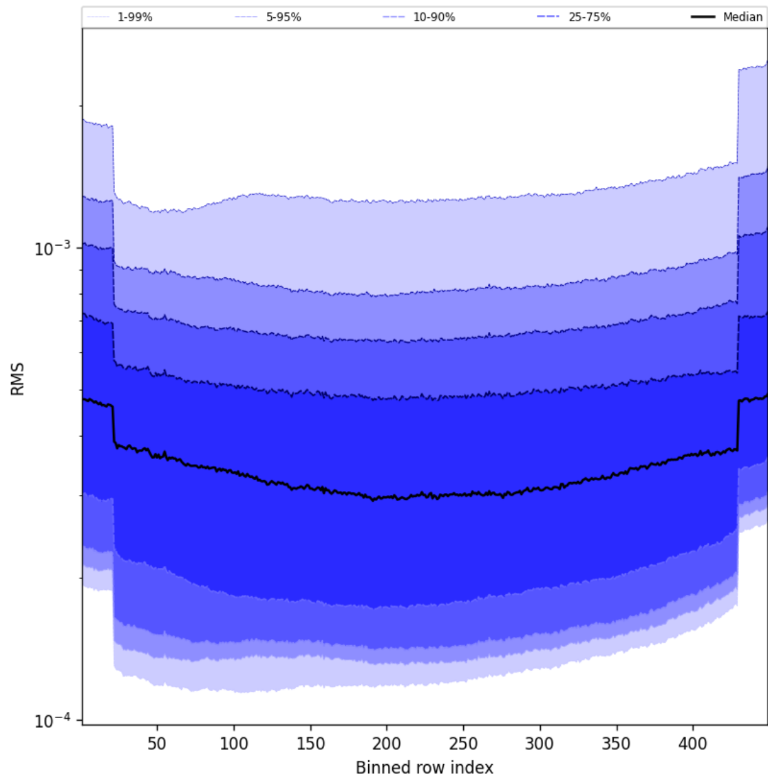
Figure 60: Along track statistics of “RMS” for 2025-11-02 to 2025-11-04
