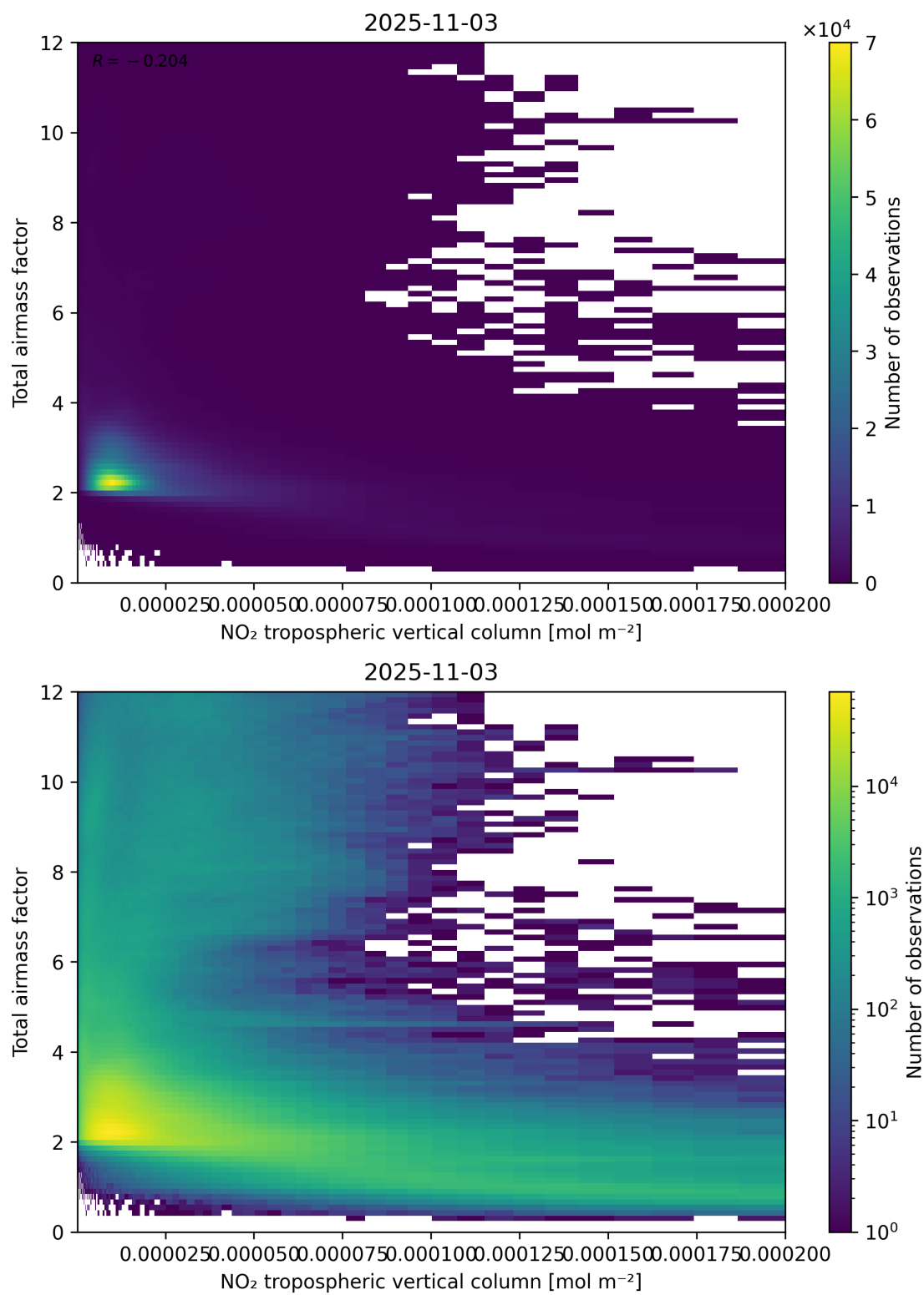
Figure 122: Scatter density plot of “NO 2 tropospheric vertical column” against “Total air mass factor” for 2025-11-02 to 2025-11-04.
