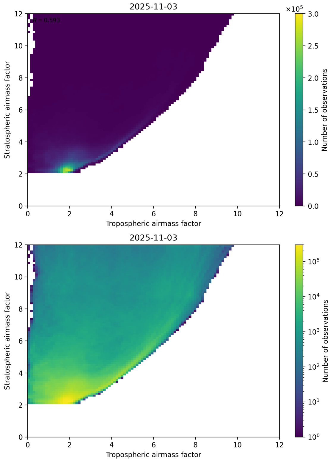
Figure 71: Scatter density plot of “Tropospheric airmass factor” against “Stratospheric airmass factor” for 2025-11-02 to 2025-11-04.
