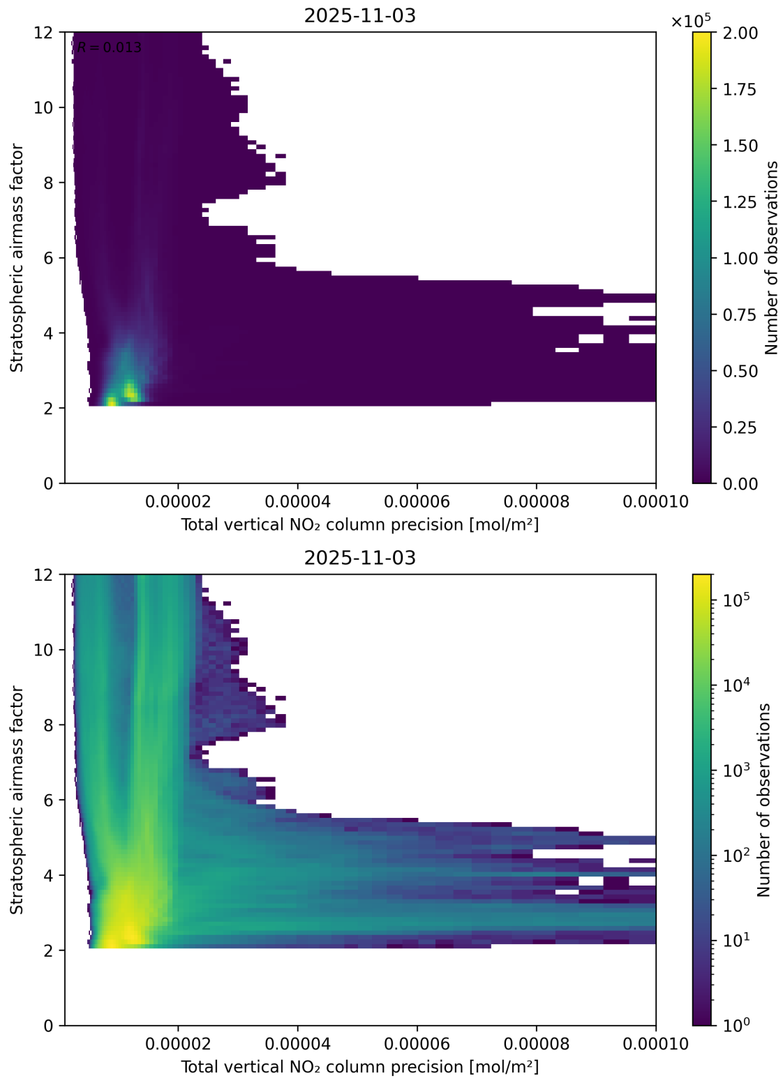
Figure 115: Scatter density plot of “Total vertical NO 2 column precision” against “Stratospheric air mass factor” for 2025-11-02 to 2025-11-04.
