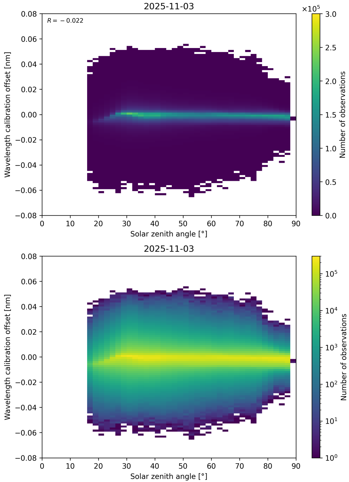
Figure 158: Scatter density plot of “Solar zenith angle” against “Wavelength calibration offset” for 2025-11-02 to 2025-11-04.
