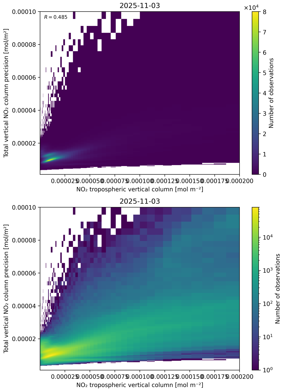
Figure 129: Scatter density plot of “NO 2 tropospheric vertical column” against “Total vertical NO 2 column precision” for 2025-11-02 to 2025-11-04.
