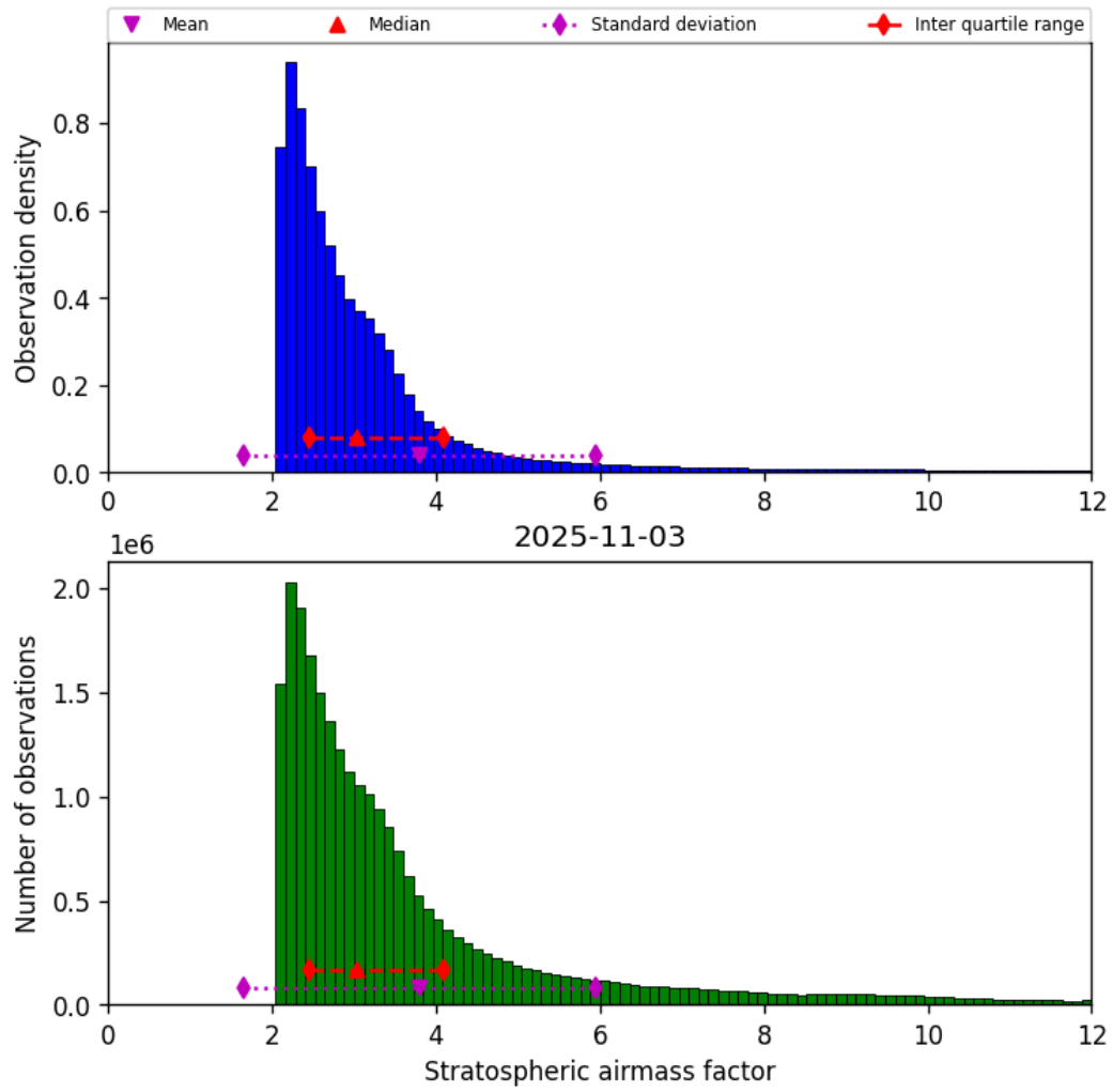
Figure 44: Histogram of “Stratospheric airmass factor” for 2025-11-02 to 2025-11-04
