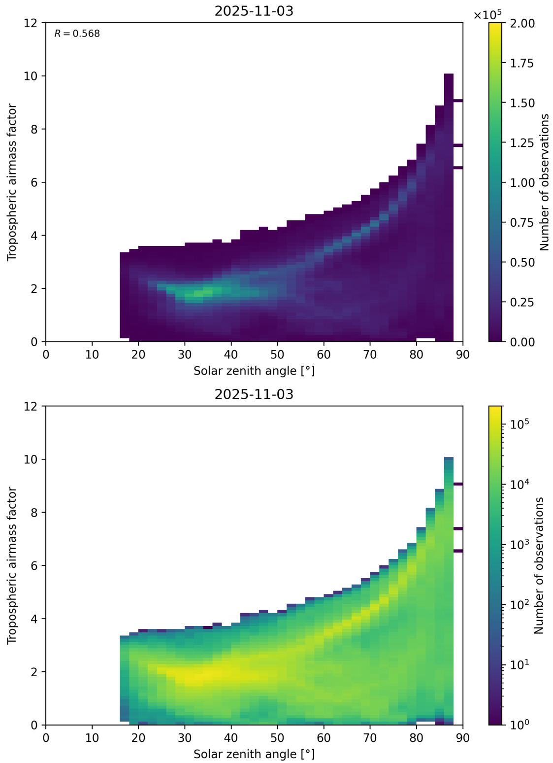
Figure 147: Scatter density plot of “Solar zenith angle” against “Tropospheric airmass factor” for 2025-11-02 to 2025-11-04.
