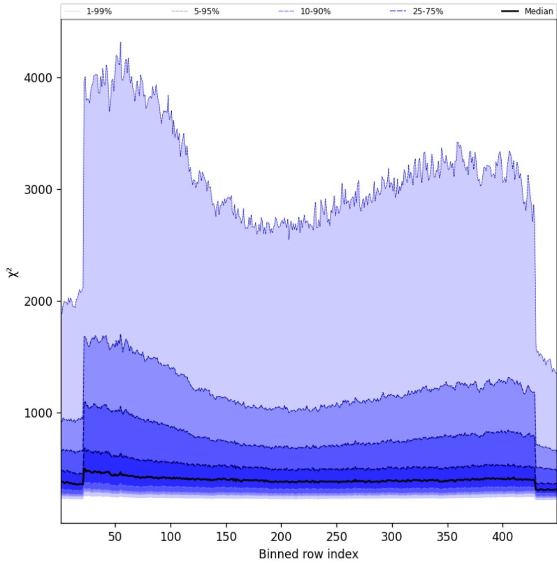
Figure 59: Along track statistics of “ \chi^2 ” for 2025-11-02 to 2025-11-04
