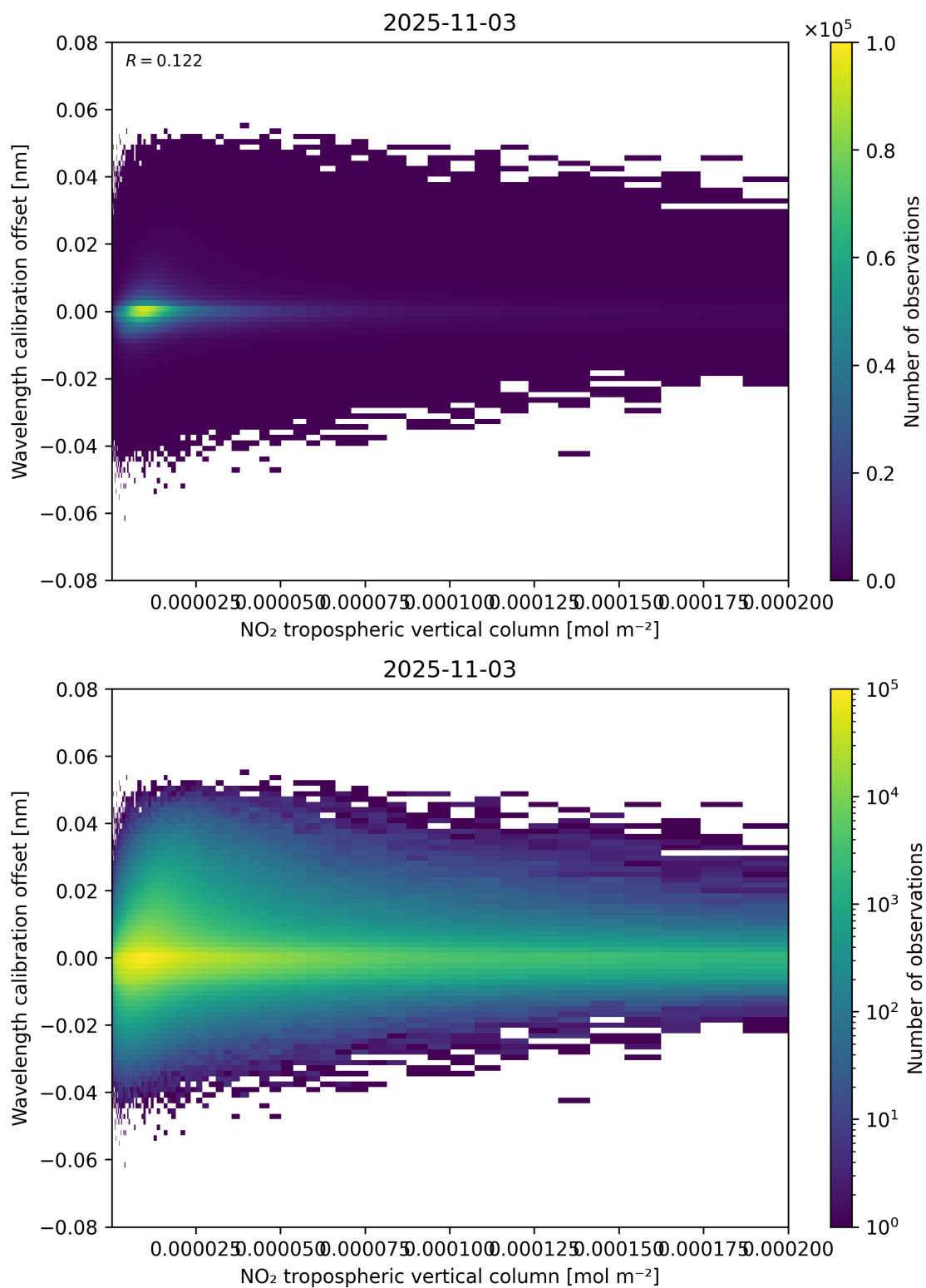
Figure 143: Scatter density plot of “NO 2 tropospheric vertical column” against “Wavelength calibration offset” for 2025-11-02 to 2025-11-04.
