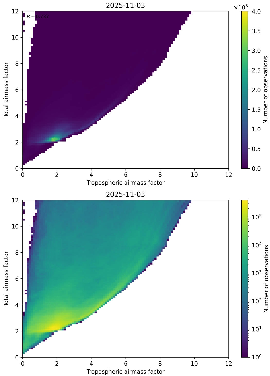
Figure 72: Scatter density plot of “Tropospheric airmass factor” against “Total airmass factor” for 2025-11-02 to 2025-11-04.
