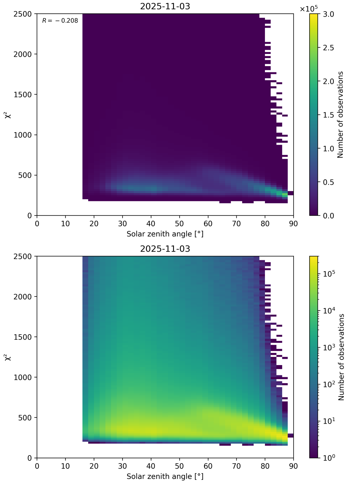
Figure 148: Scatter density plot of “Solar zenith angle” against “ \chi^2 ” for 2025-11-02 to 2025-11-04.
