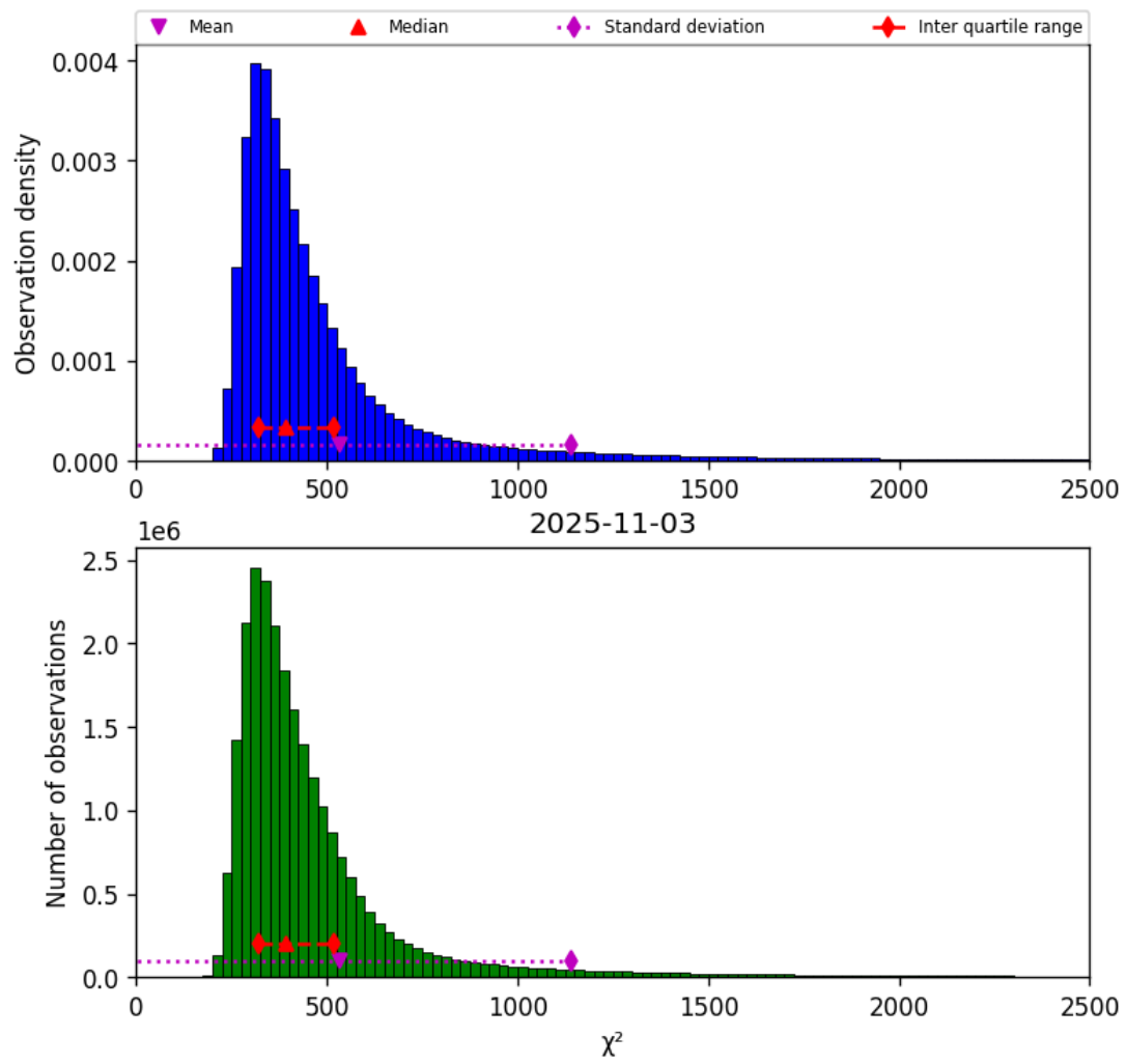
Figure 42: Histogram of “ \chi^2 ” for 2025-11-02 to 2025-11-04
