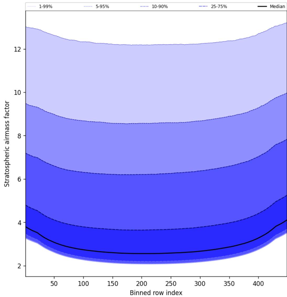
Figure 61: Along track statistics of “Stratospheric airmass factor” for 2025-11-02 to 2025-11-04
