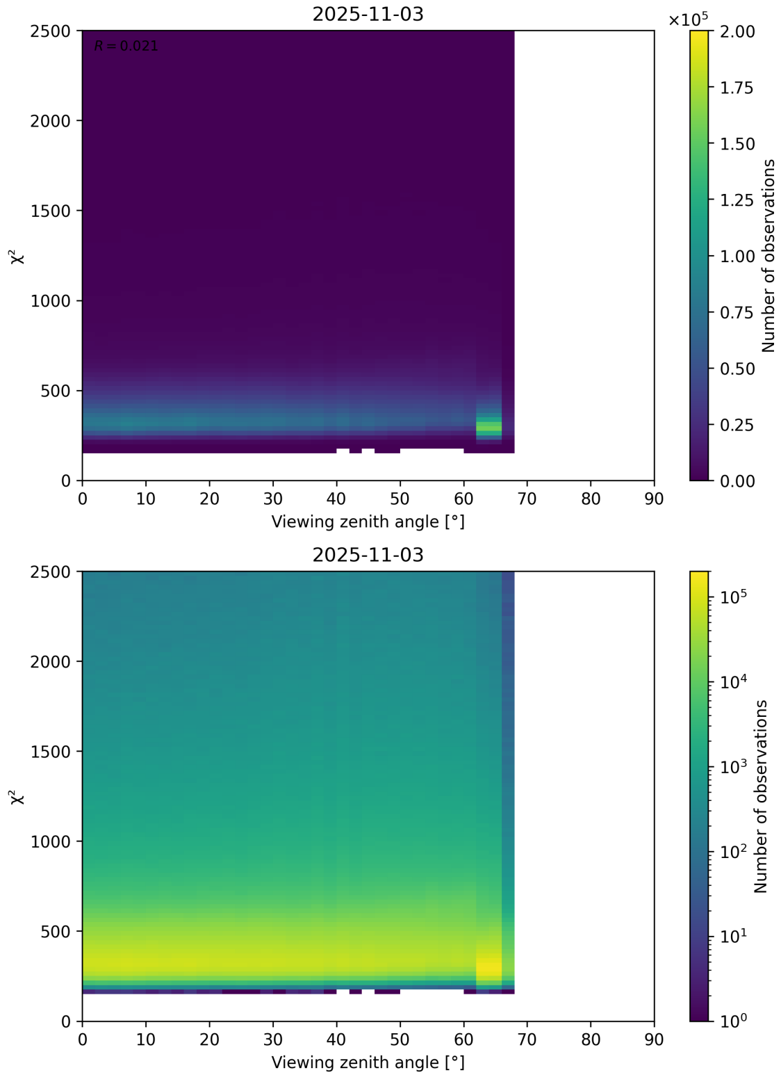
Figure 162: Scatter density plot of “Viewing zenith angle” against “ \chi^2 ” for 2025-11-02 to 2025-11-04.
