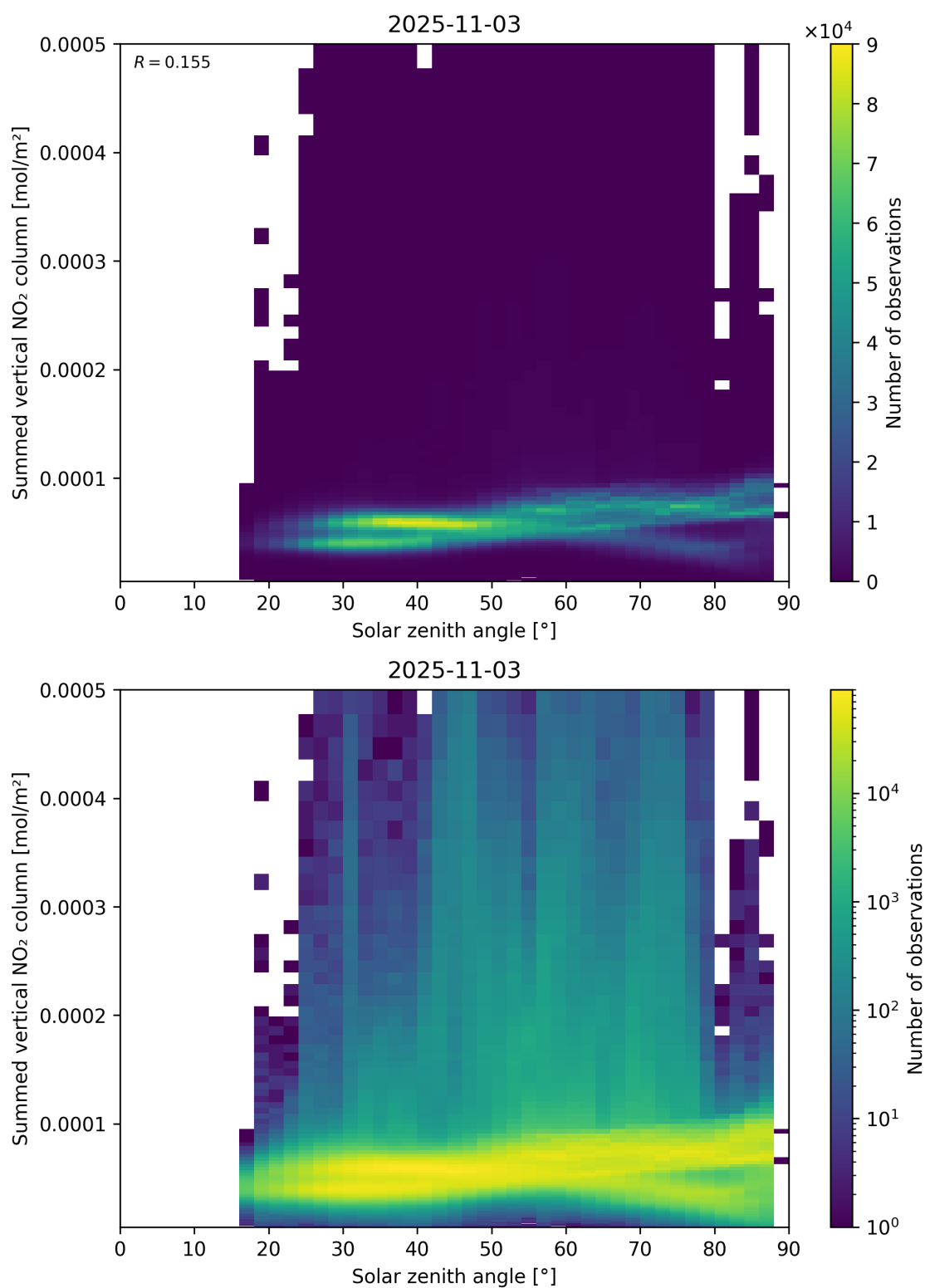
Figure 151: Scatter density plot of “Solar zenith angle” against “Summed vertical NO 2 column” for 2025-11-02 to 2025-11-04.
