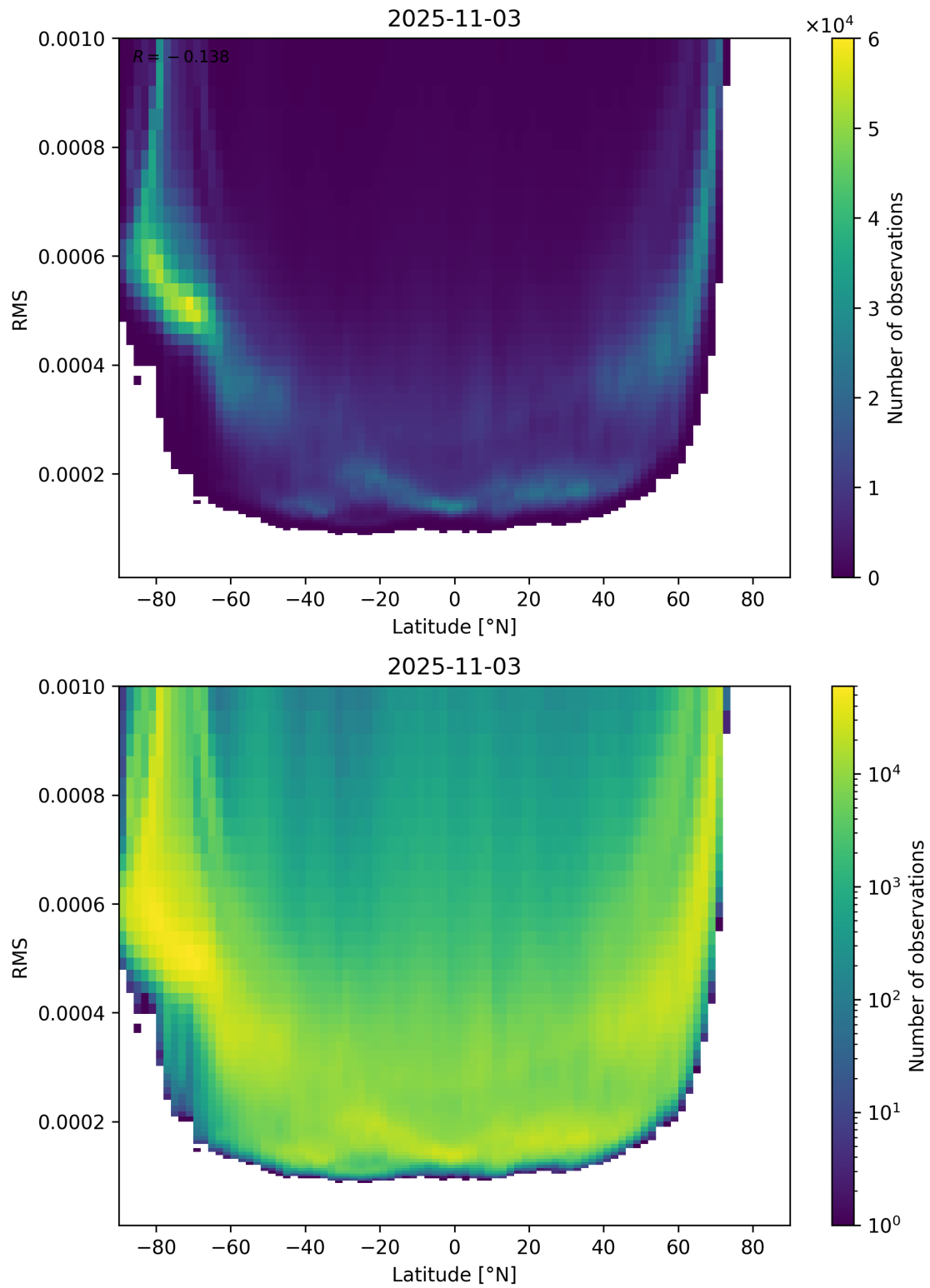
Figure 94: Scatter density plot of “Latitude” against “RMS” for 2025-11-02 to 2025-11-04.
