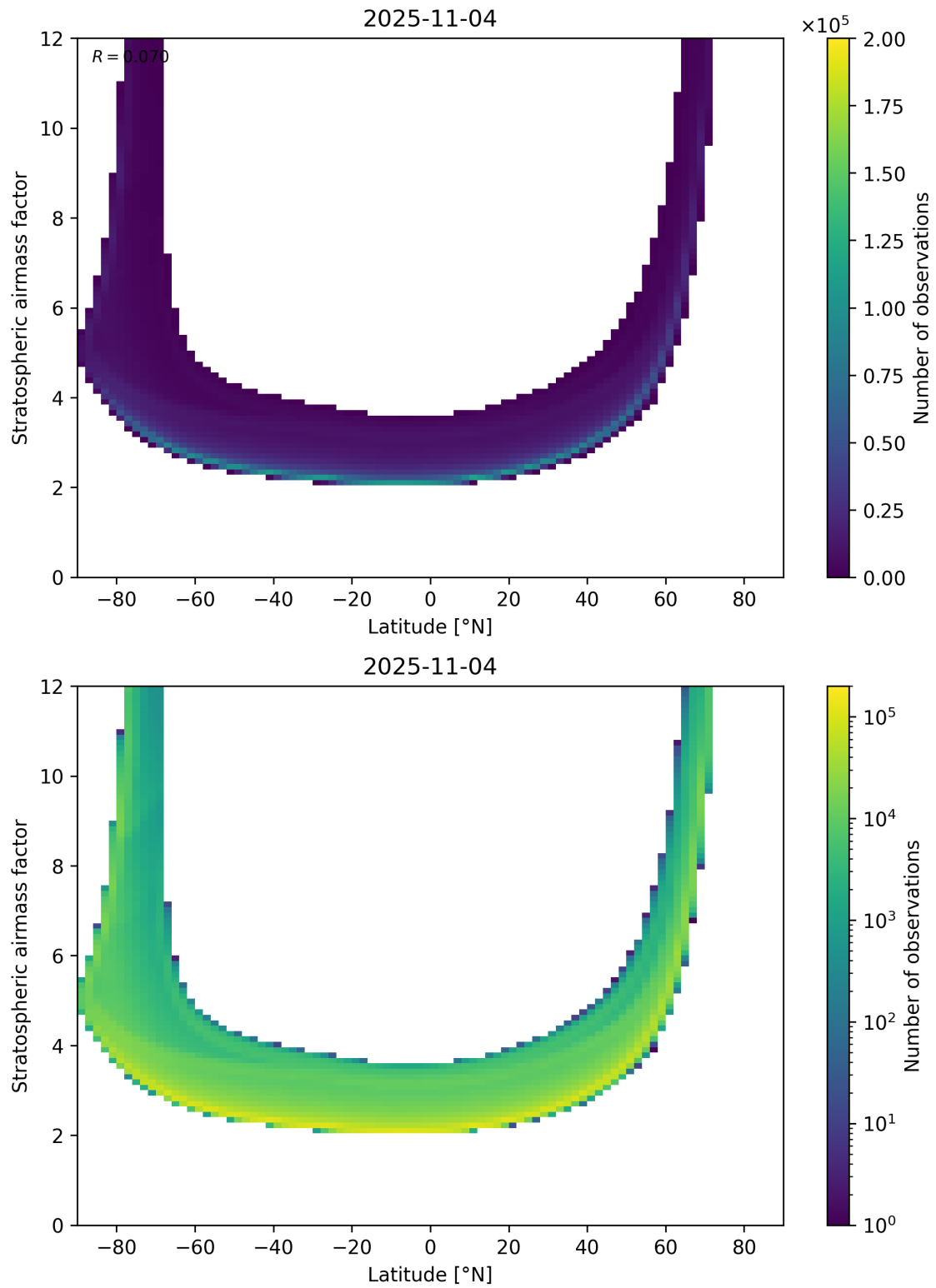
Figure 83: Scatter density plot of “Latitude” against “Stratospheric airmass factor” for 2025-11-03 to 2025-11-05.
