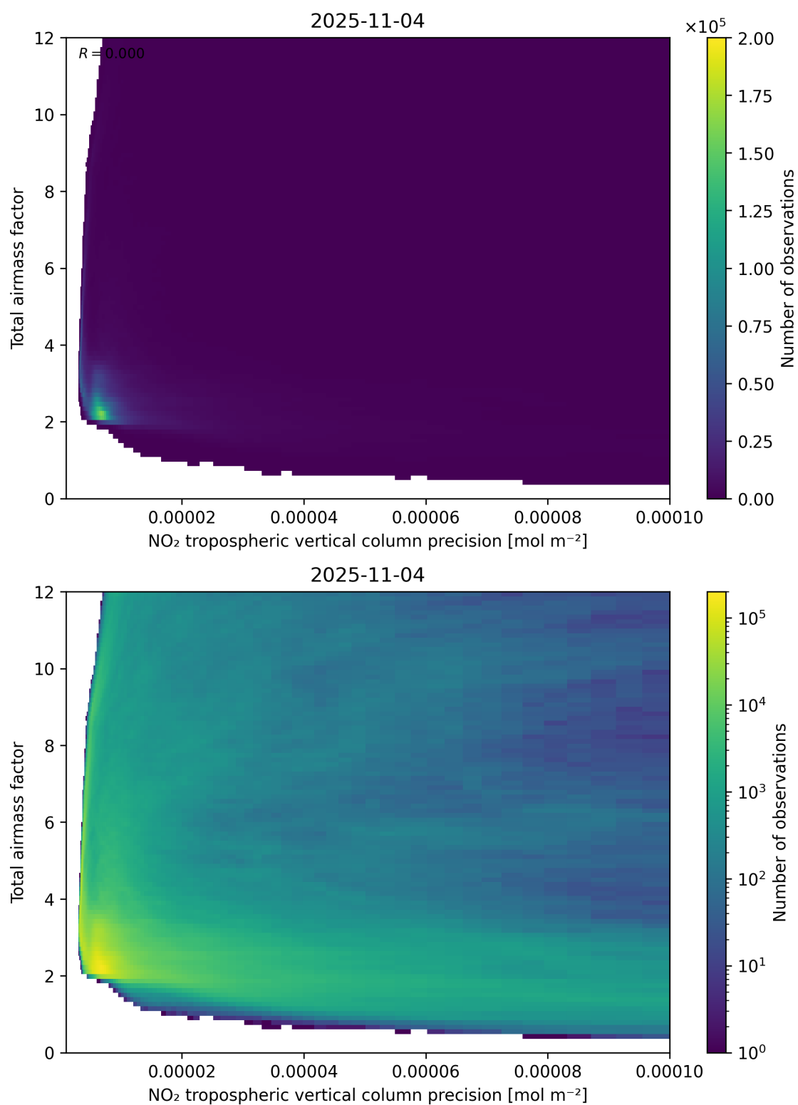
Figure 132: Scatter density plot of “NO 2 tropospheric vertical column precision” against “Total air mass factor” for 2025-11-03 to 2025-11-05.
