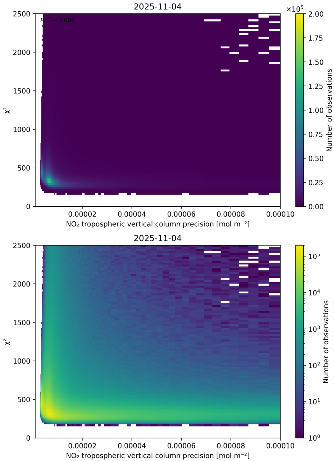
Figure 134: Scatter density plot of “NO 2 tropospheric vertical column precision” against “ \chi^2 ” for 2025-11-03 to 2025-11-05.
