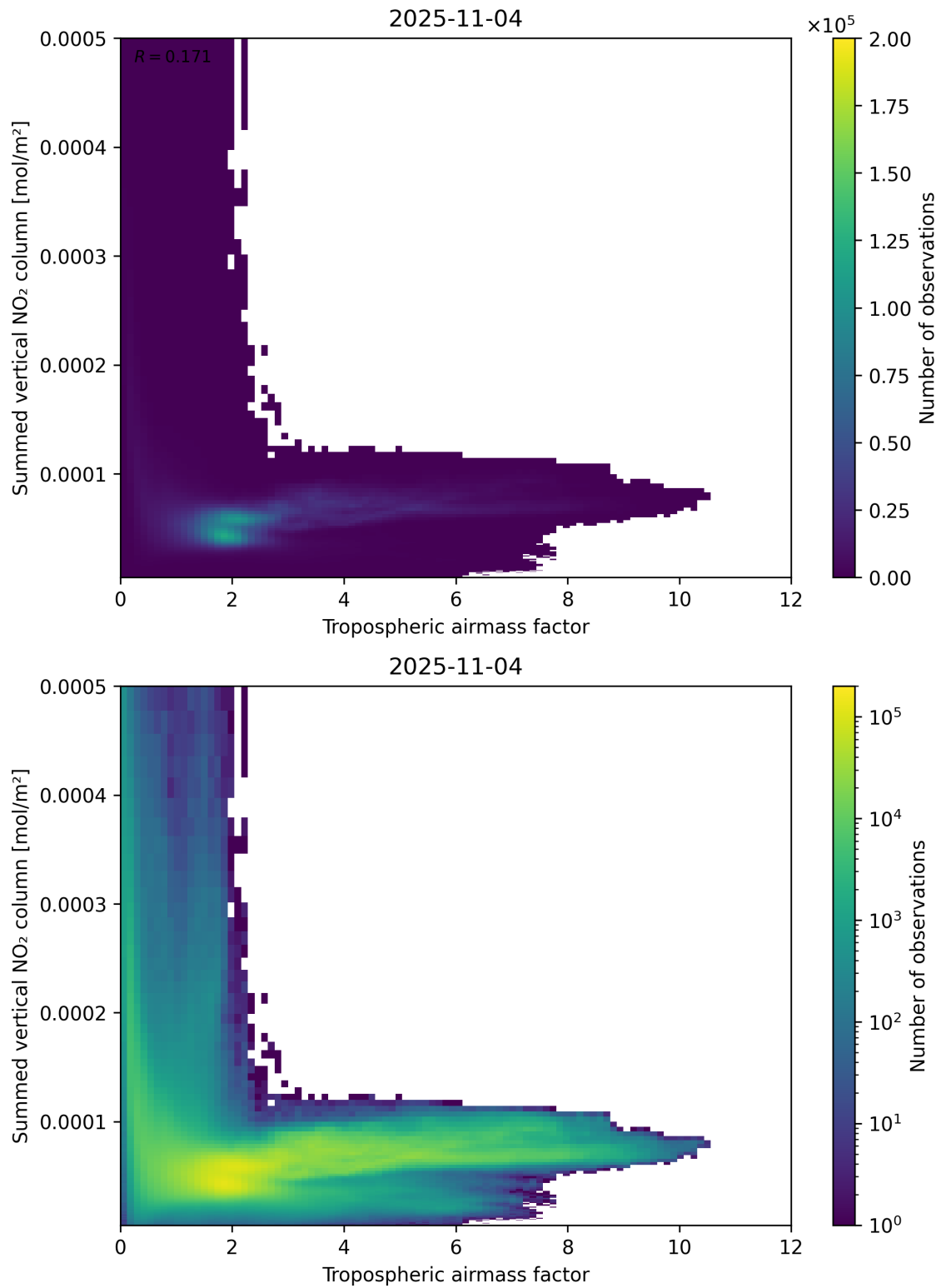
Figure 75: Scatter density plot of “Tropospheric air mass factor” against “Summed vertical NO 2 column” for 2025-11-03 to 2025-11-05.
