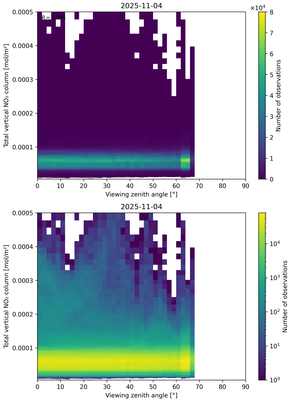
Figure 167: Scatter density plot of “Viewing zenith angle” against “Total vertical NO 2 column” for 2025-11-03 to 2025-11-05.
