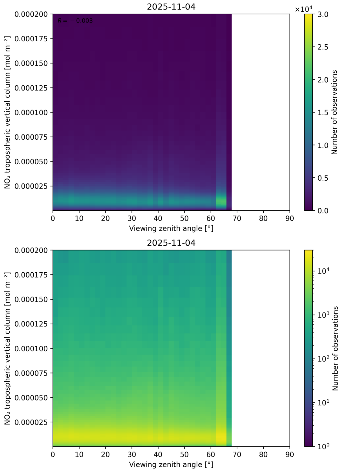
Figure 169: Scatter density plot of “Viewing zenith angle” against “NO 2 tropospheric vertical column” for 2025-11-03 to 2025-11-05.
