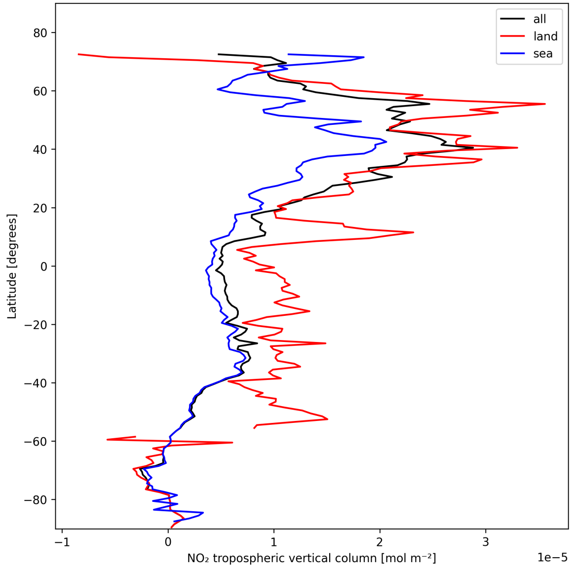
Figure 12: Zonal average of “NO 2 tropospheric vertical column” for 2025-11-03 to 2025-11-05.
