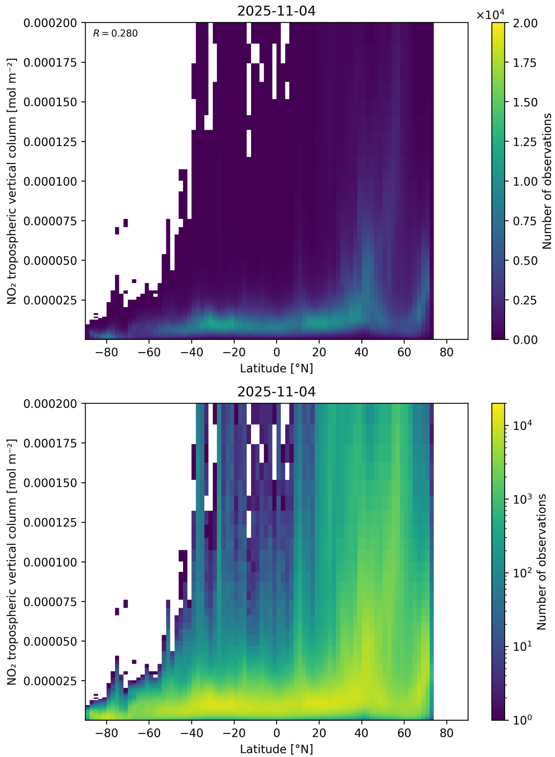
Figure 92: Scatter density plot of “Latitude” against “NO 2 tropospheric vertical column” for 2025-11-03 to 2025-11-05.
