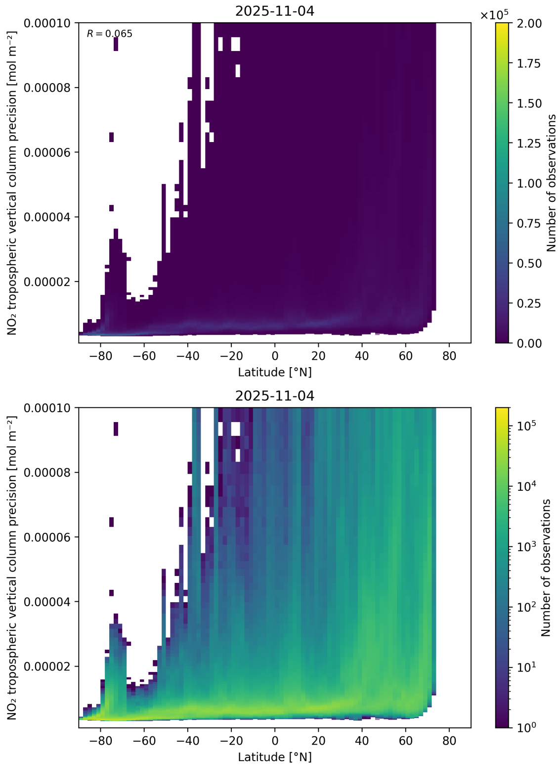
Figure 93: Scatter density plot of “Latitude” against “NO 2 tropospheric vertical column precision” for 2025-11-03 to 2025-11-05.
