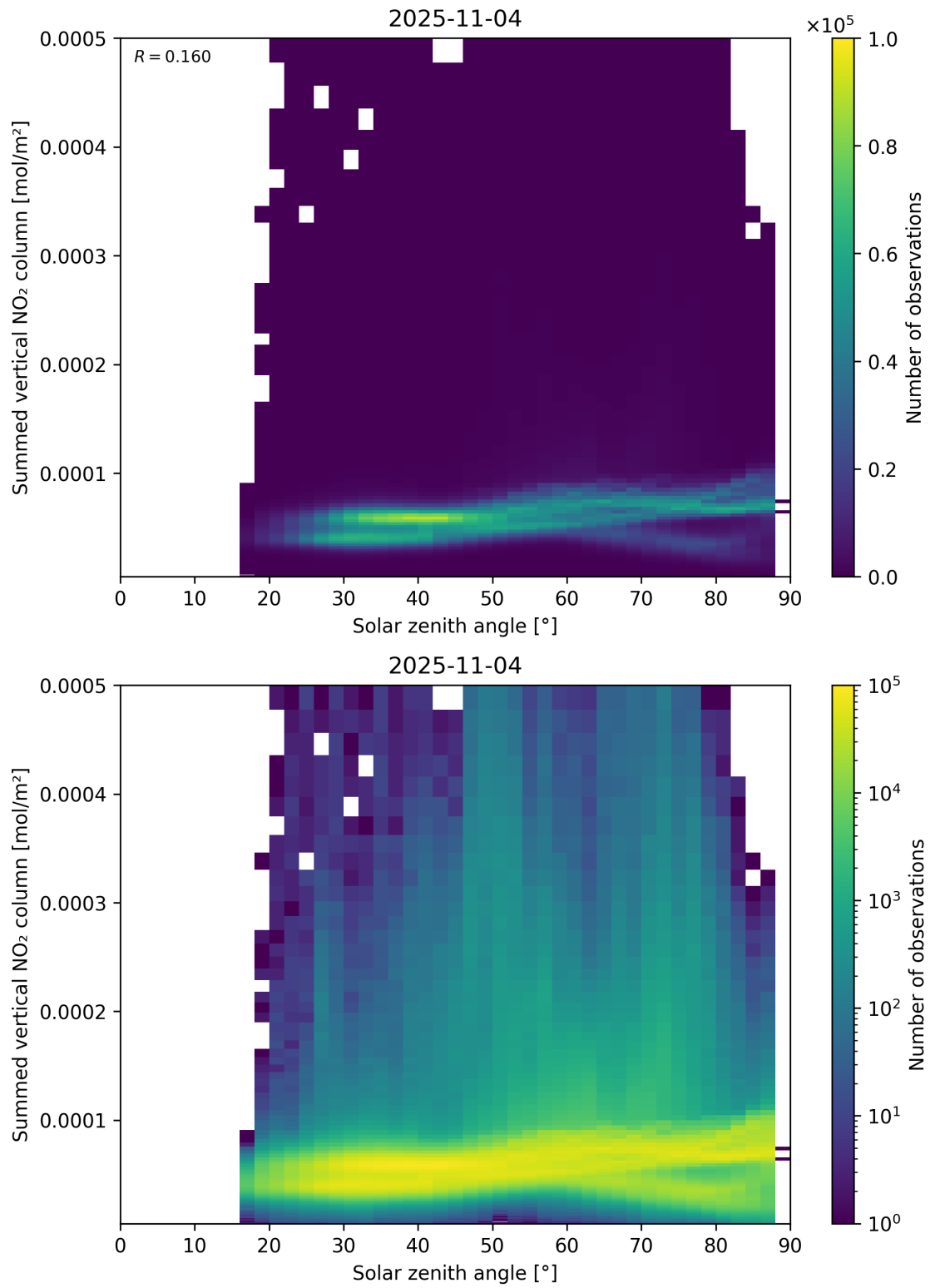
Figure 151: Scatter density plot of “Solar zenith angle” against “Summed vertical NO 2 column” for 2025-11-03 to 2025-11-05.
