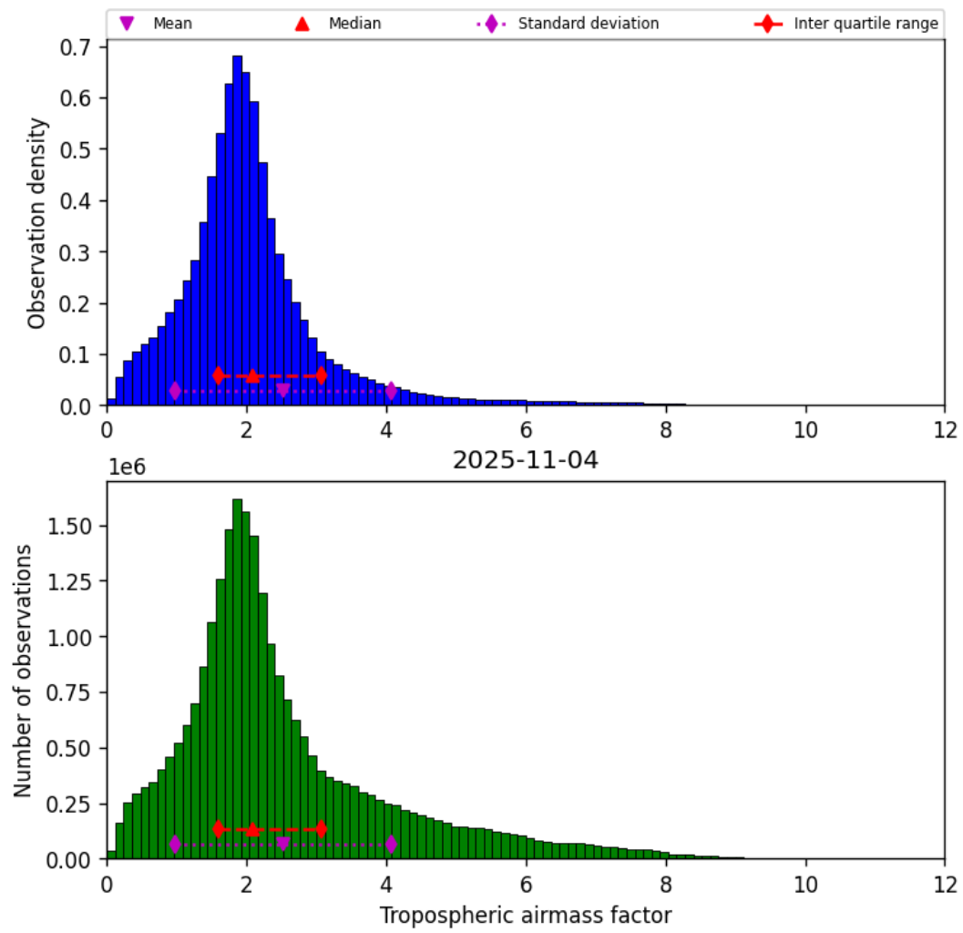
Figure 31: Histogram of “Tropospheric airmass factor” for 2025-11-03 to 2025-11-05
