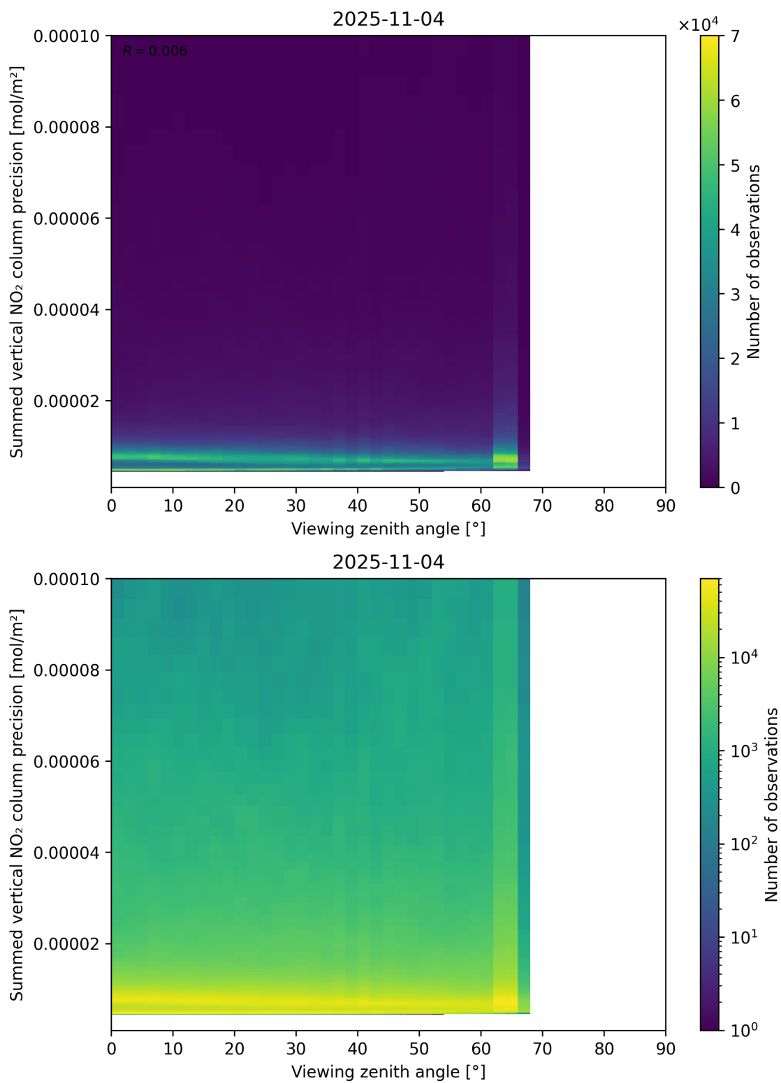
Figure 166: Scatter density plot of “Viewing zenith angle” against “Summed vertical NO 2 column precision” for 2025-11-03 to 2025-11-05.
