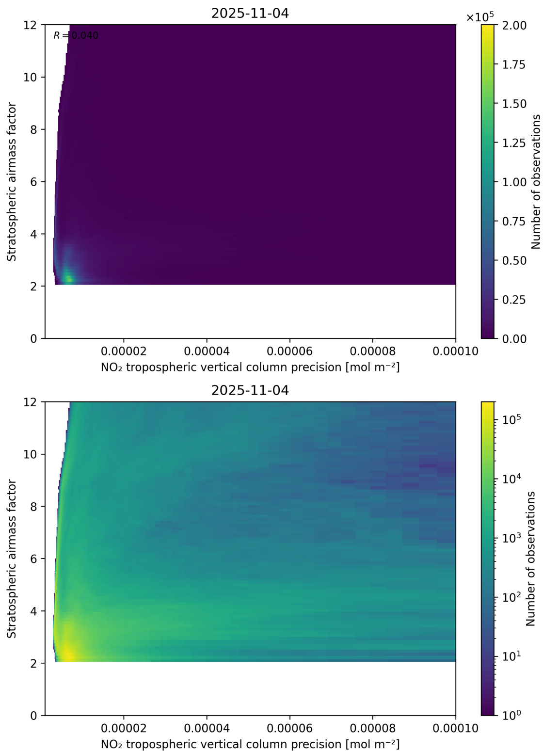
Figure 131: Scatter density plot of “NO 2 tropospheric vertical column precision” against “Stratospheric airmass factor” for 2025-11-03 to 2025-11-05.
