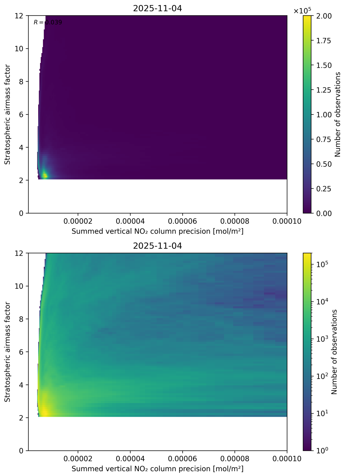
Figure 106: Scatter density plot of “Summed vertical NO 2 column precision” against “Stratospheric airmass factor” for 2025-11-03 to 2025-11-05.
