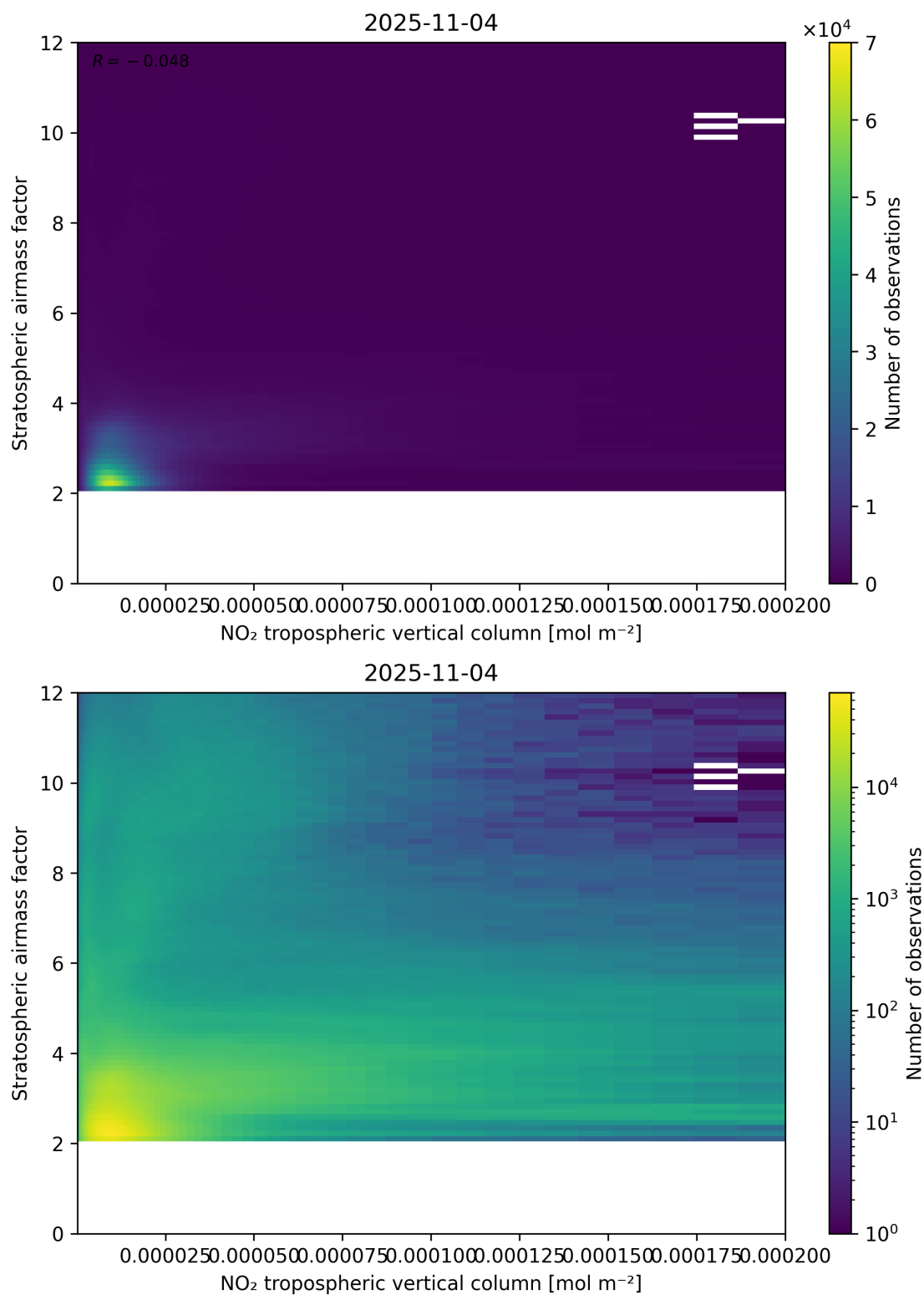
Figure 121: Scatter density plot of “NO 2 tropospheric vertical column” against “Stratospheric air mass factor” for 2025-11-03 to 2025-11-05.
