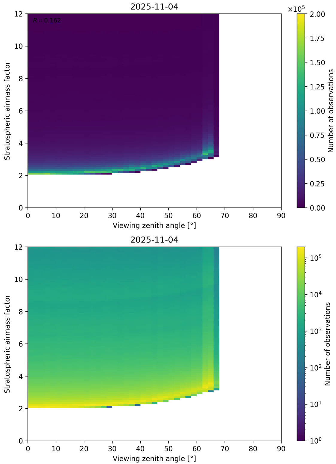
Figure 159: Scatter density plot of “Viewing zenith angle” against “Stratospheric airmass factor” for 2025-11-03 to 2025-11-05.
