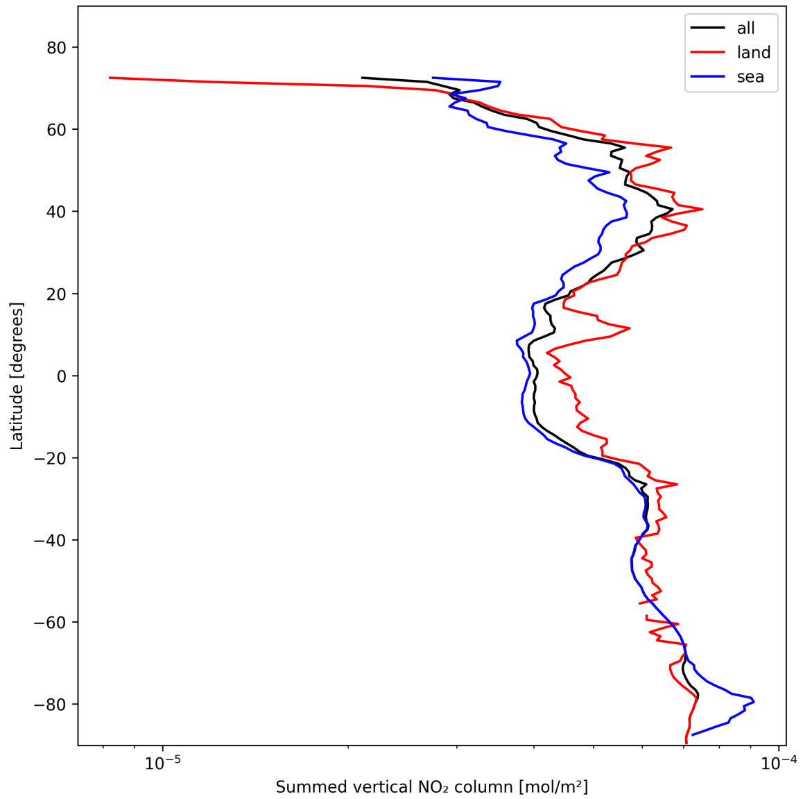
Figure 23: Zonal average of “Summed vertical NO 2 column” for 2025-11-03 to 2025-11-05.
