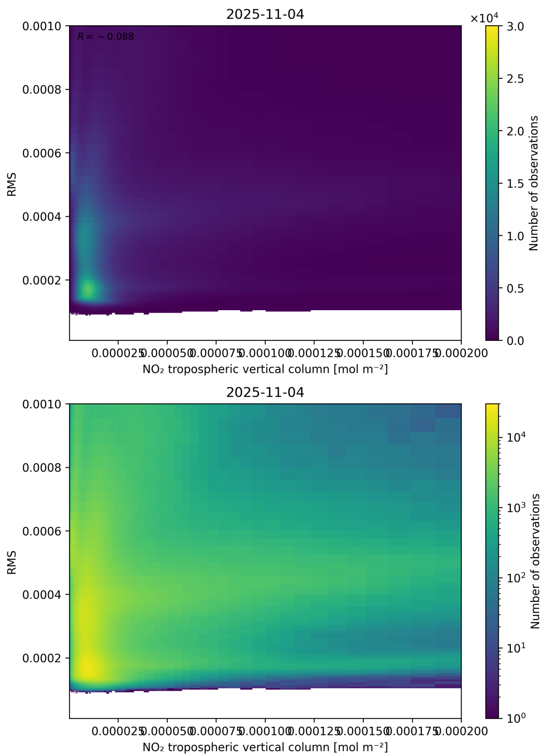
Figure 142: Scatter density plot of “NO 2 tropospheric vertical column” against “RMS” for 2025-11-03 to 2025-11-05.
