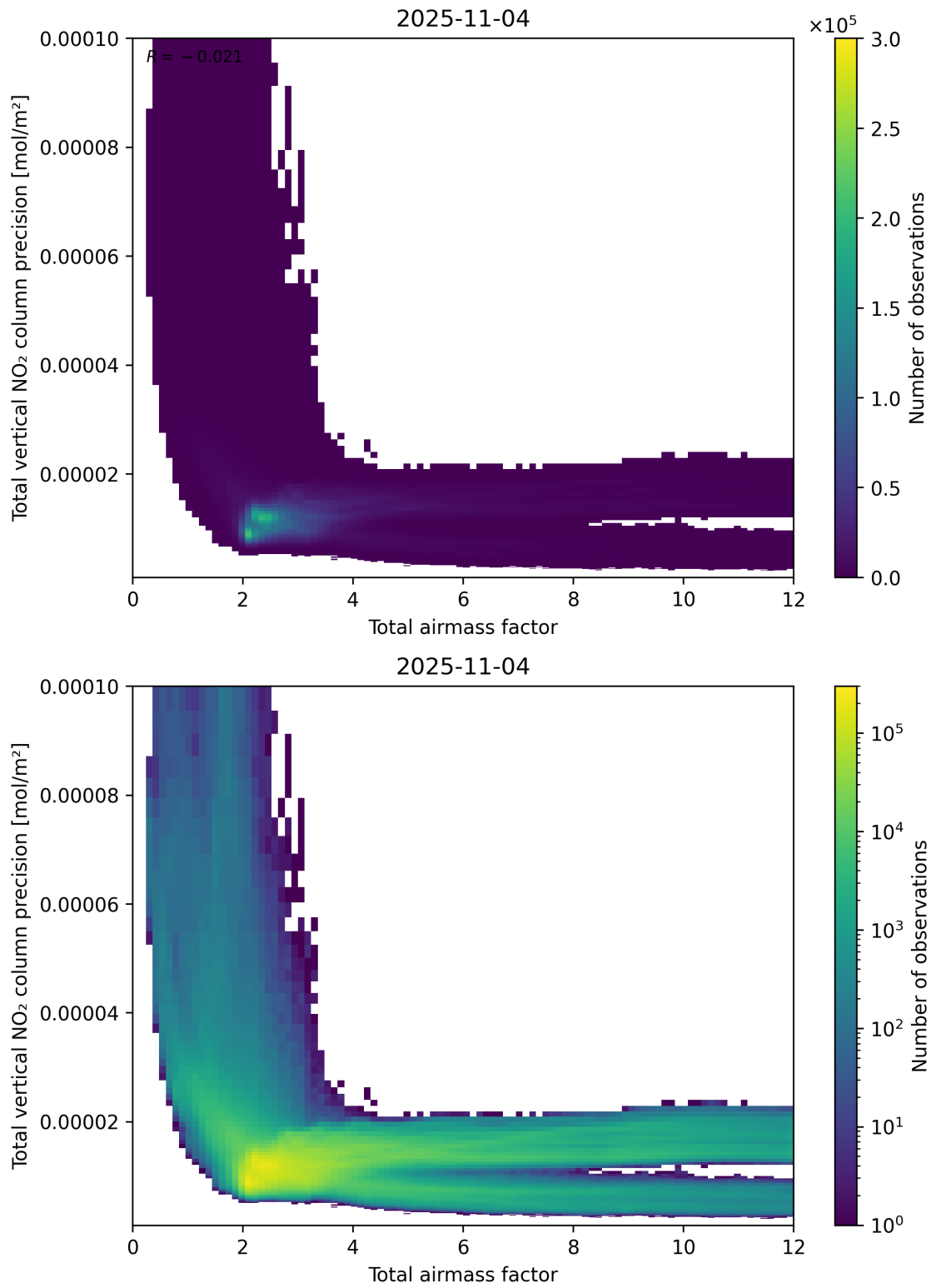
Figure 68: Scatter density plot of “Total airmass factor” against “Total vertical NO 2 column precision” for 2025-11-03 to 2025-11-05.
