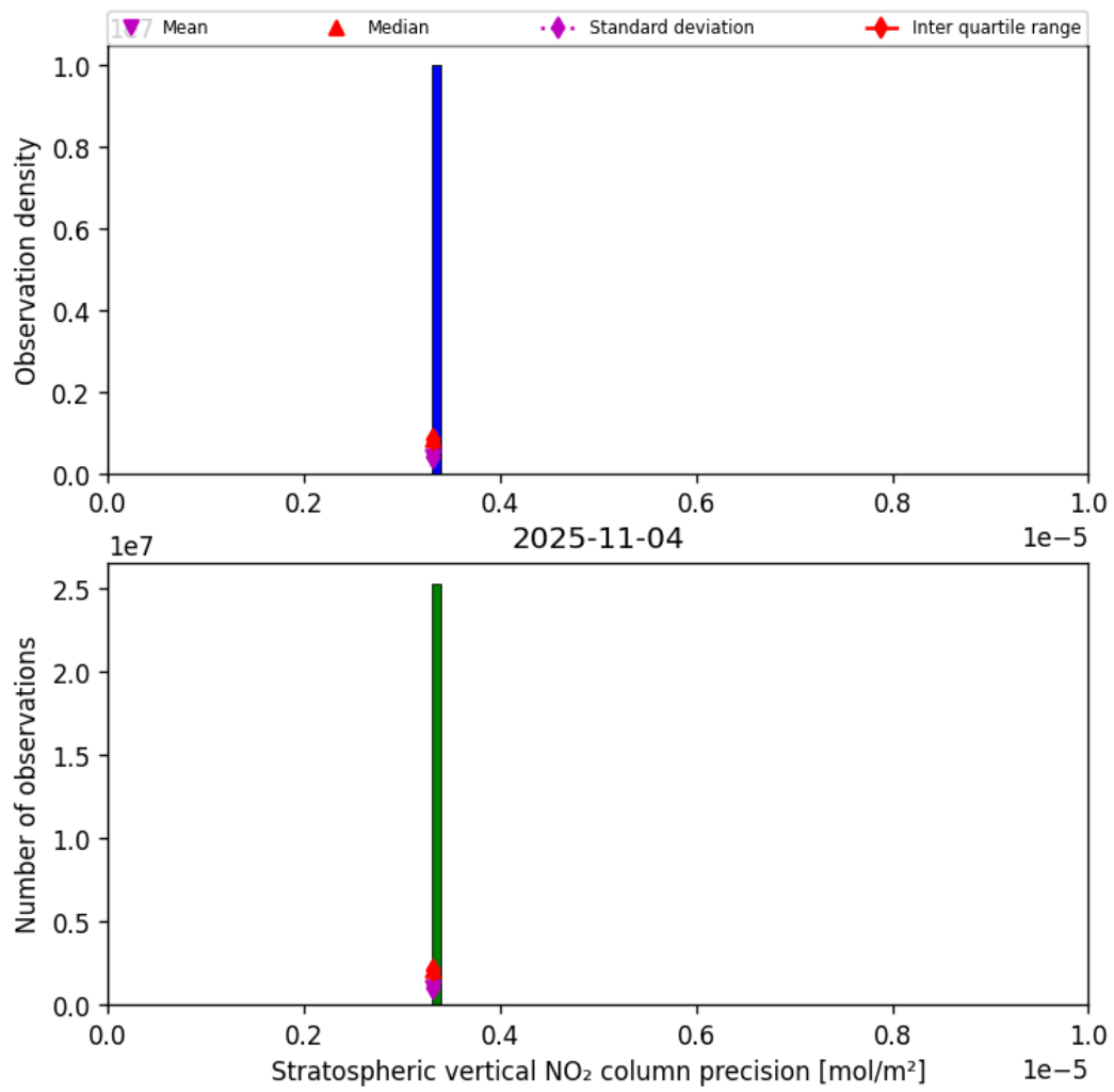
Figure 37: Histogram of “Stratospheric vertical NO 2 column precision” for 2025-11-03 to 2025-11-05
