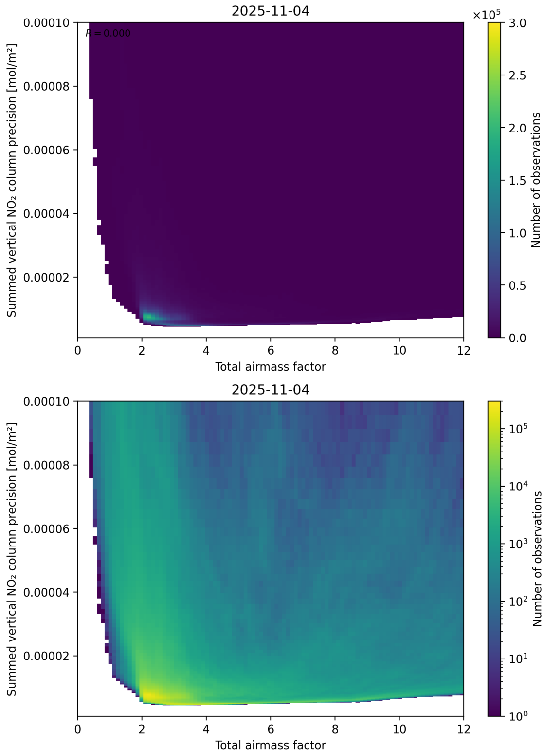
Figure 66: Scatter density plot of “Total airmass factor” against “Summed vertical NO 2 column precision” for 2025-11-03 to 2025-11-05.
