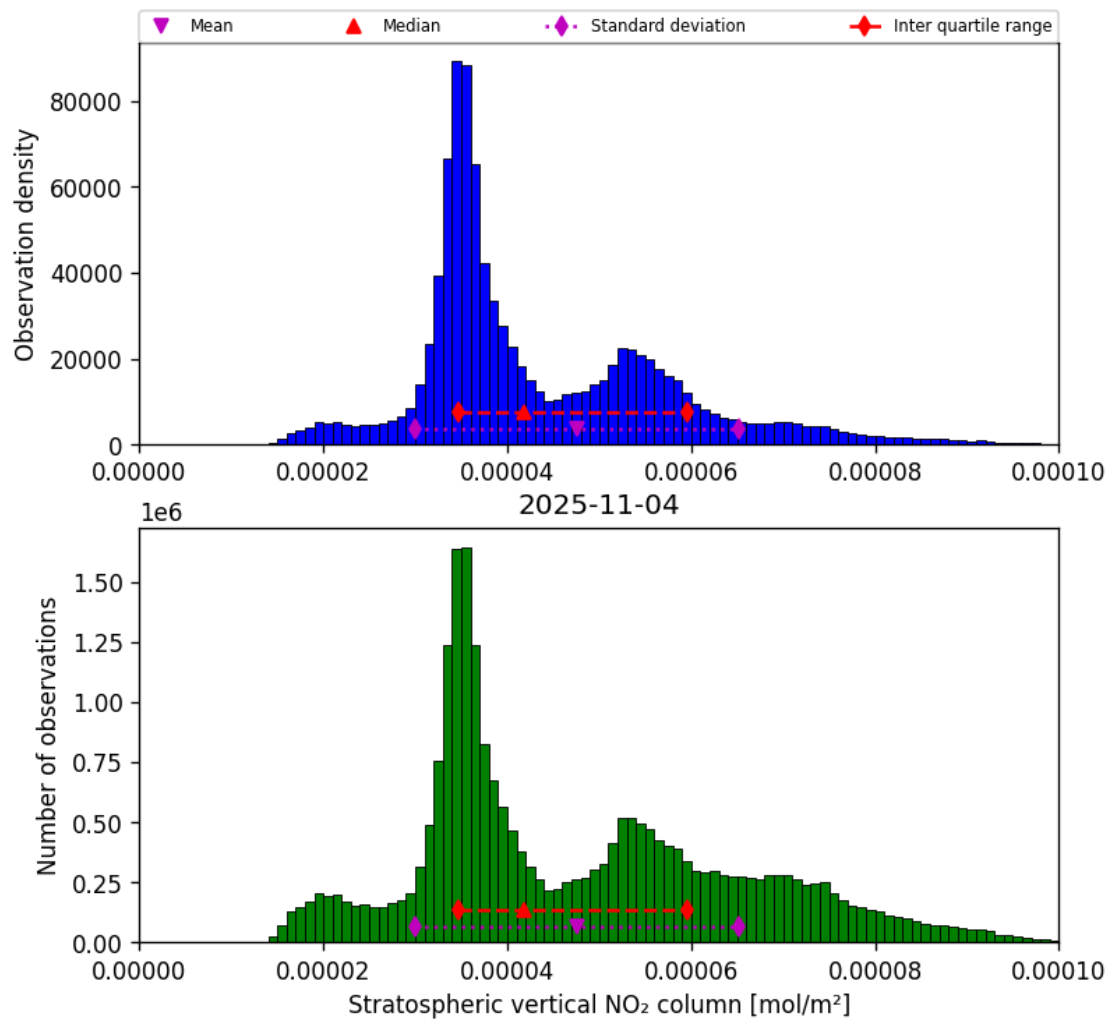
Figure 36: Histogram of “Stratospheric vertical NO 2 column” for 2025-11-03 to 2025-11-05
