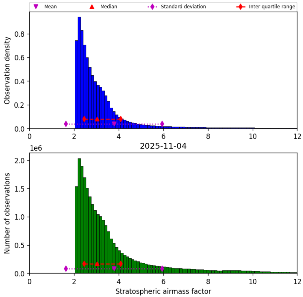
Figure 44: Histogram of “Stratospheric airmass factor” for 2025-11-03 to 2025-11-05
