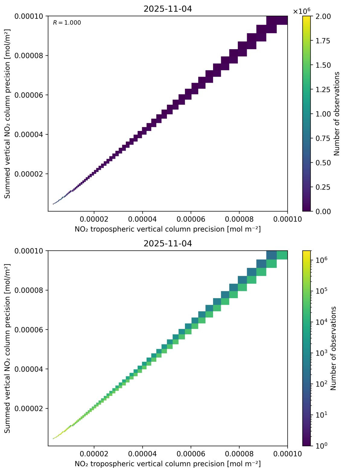
Figure 137: Scatter density plot of “NO 2 tropospheric vertical column precision” against “Summed vertical NO 2 column precision” for 2025-11-03 to 2025-11-05.
