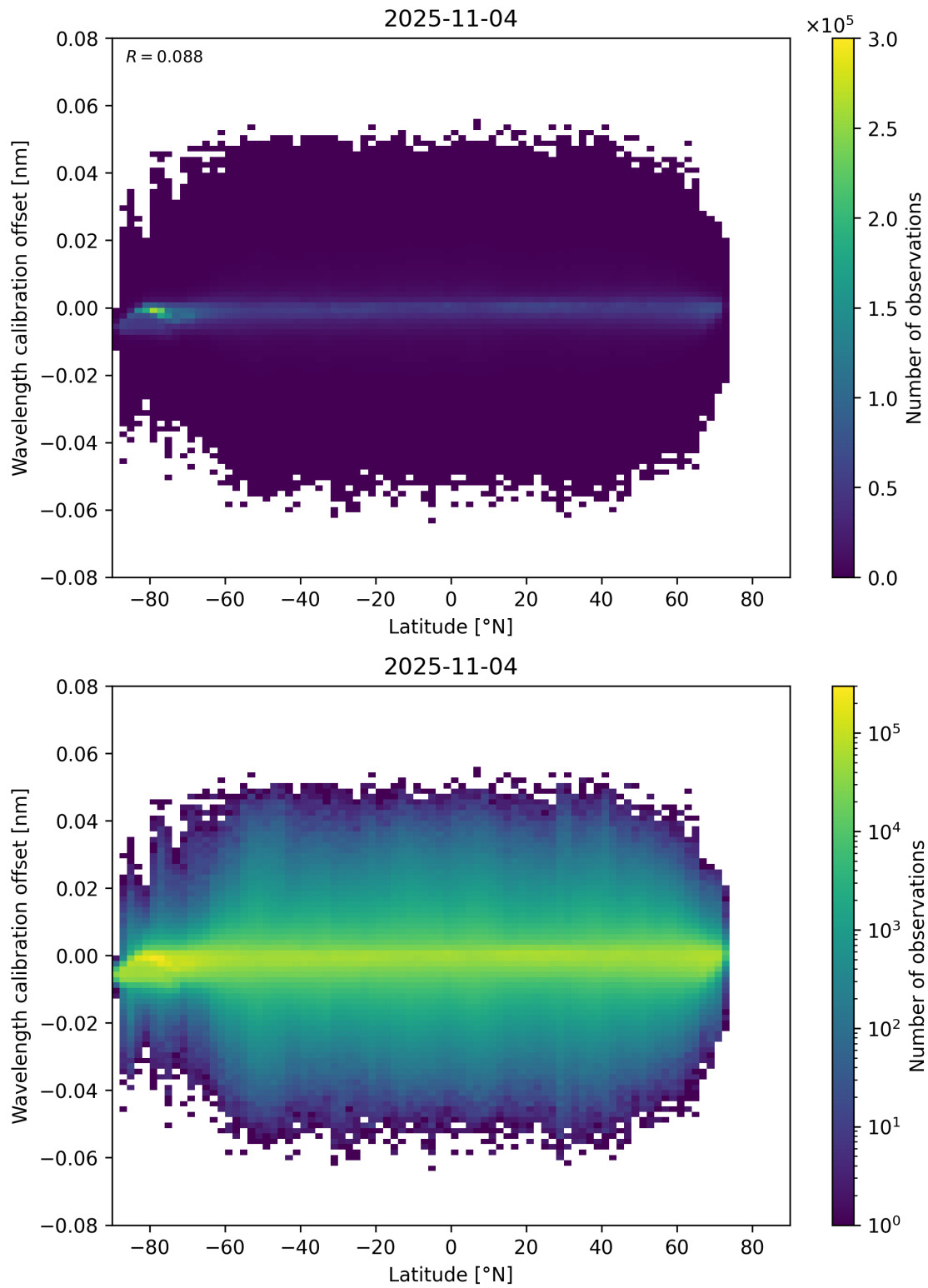
Figure 95: Scatter density plot of “Latitude” against “Wavelength calibration offset” for 2025-11-03 to 2025-11-05.
