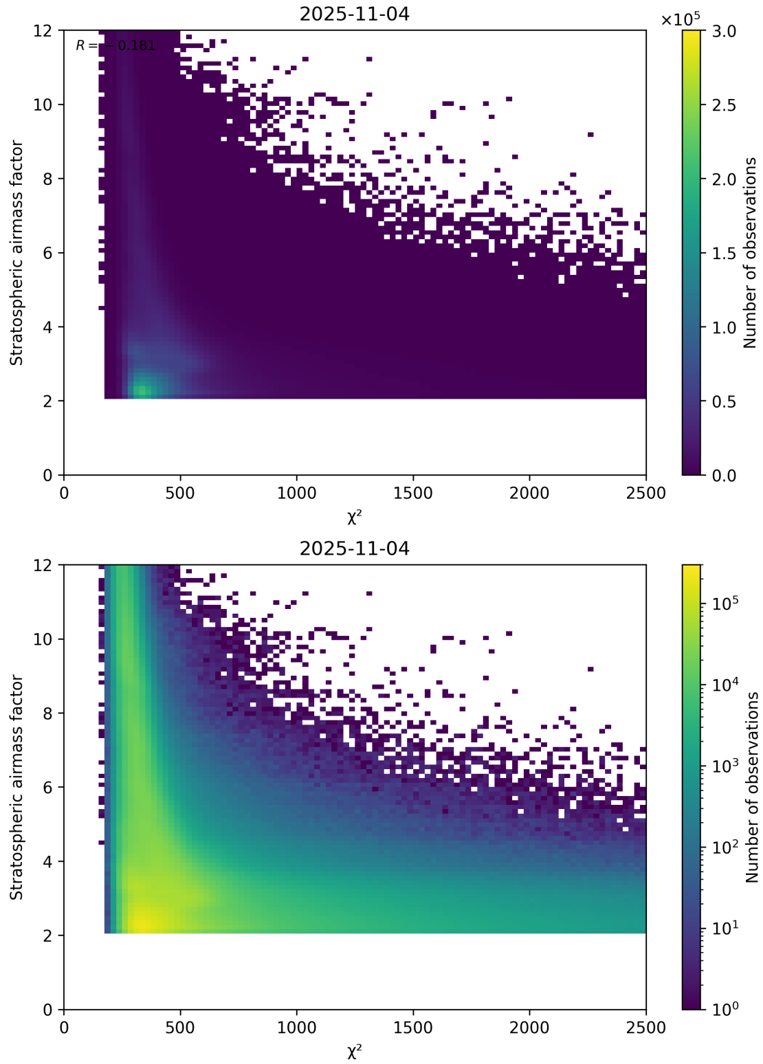
Figure 81: Scatter density plot of “ \chi^2 ” against “Stratospheric airmass factor” for 2025-11-03 to 2025-11-05.
