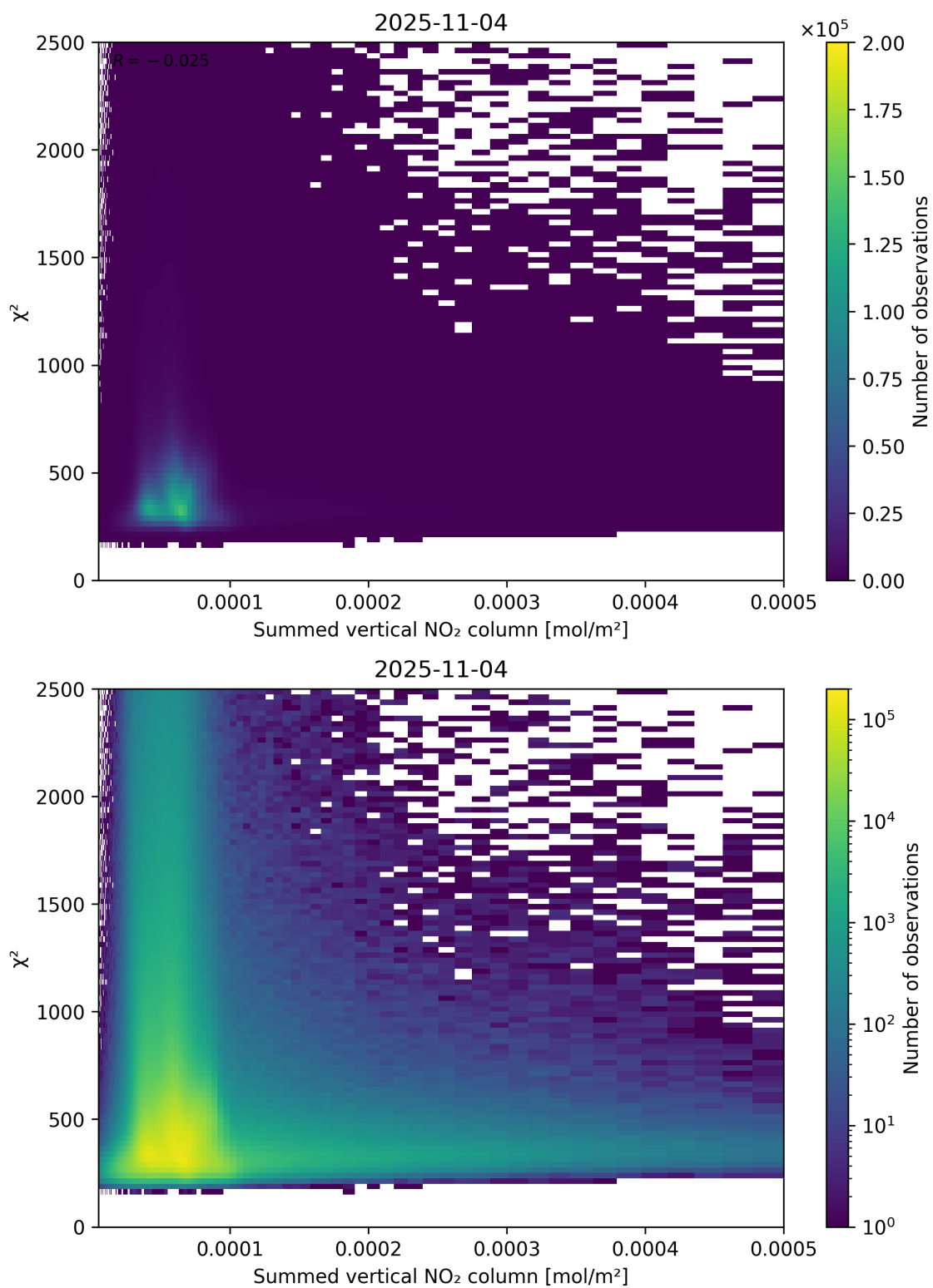
Figure 104: Scatter density plot of “Summed vertical NO 2 column” against “ \chi^2 ” for 2025-11-03 to 2025-11-05.
