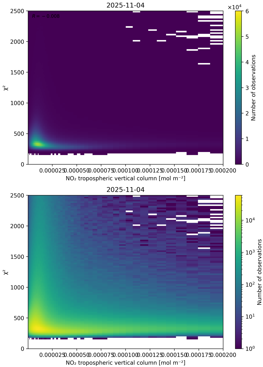
Figure 124: Scatter density plot of “NO 2 tropospheric vertical column” against “ \chi^2 ” for 2025-11-03 to 2025-11-05.
