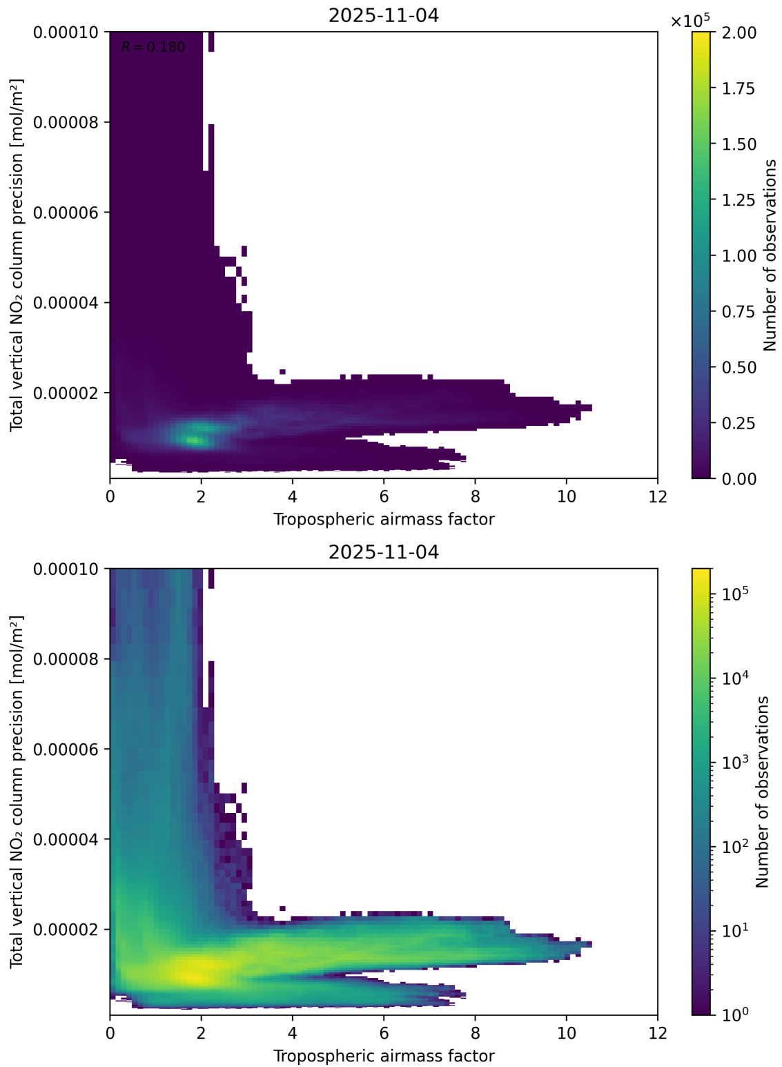
Figure 78: Scatter density plot of “Tropospheric airmass factor” against “Total vertical NO 2 column precision” for 2025-11-03 to 2025-11-05.
