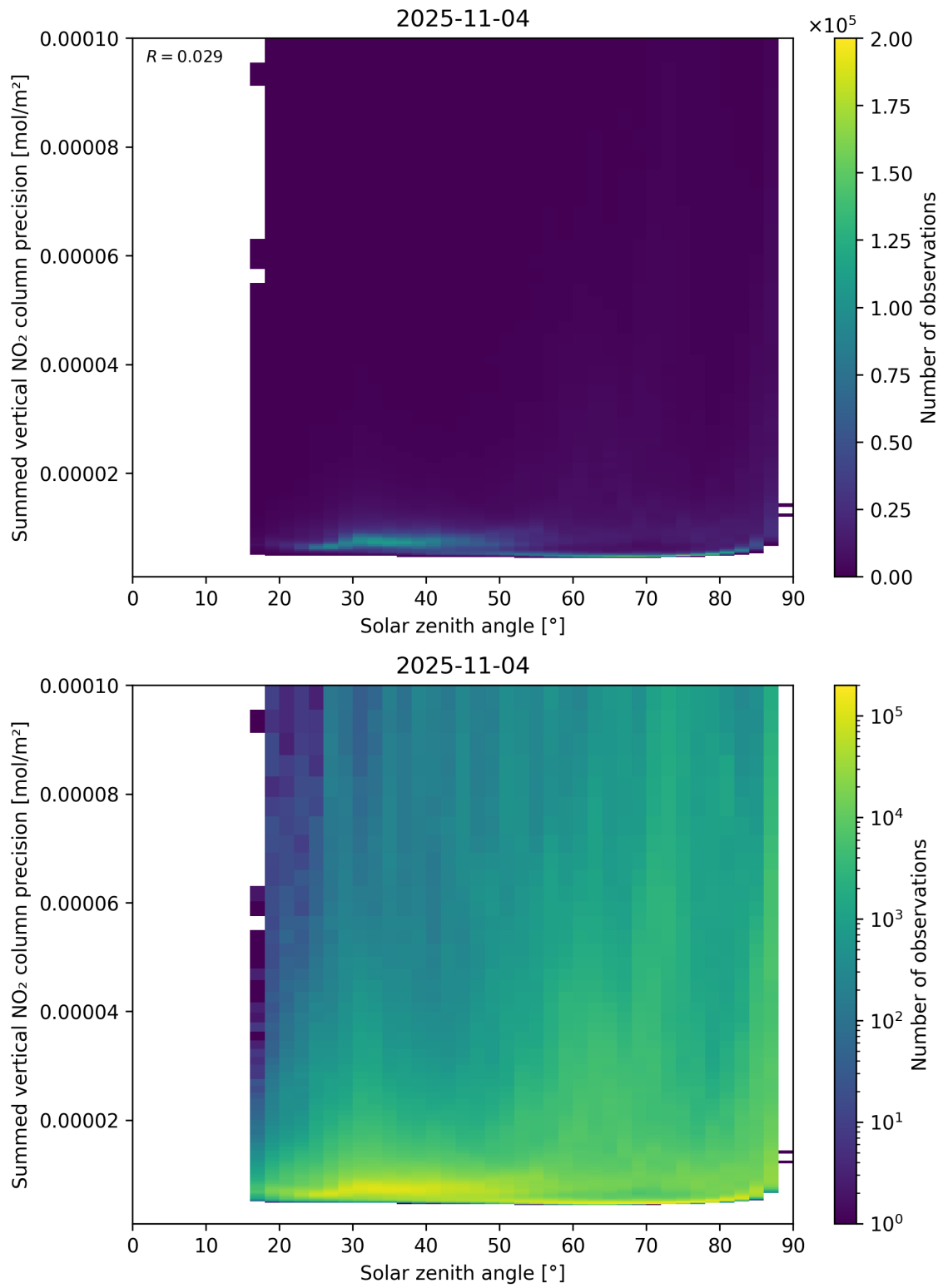
Figure 152: Scatter density plot of “Solar zenith angle” against “Summed vertical NO 2 column precision” for 2025-11-03 to 2025-11-05.
