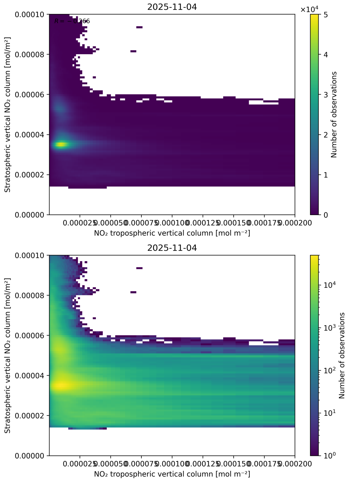
Figure 125: Scatter density plot of “NO 2 tropospheric vertical column” against “Stratospheric vertical NO 2 column” for 2025-11-03 to 2025-11-05.
