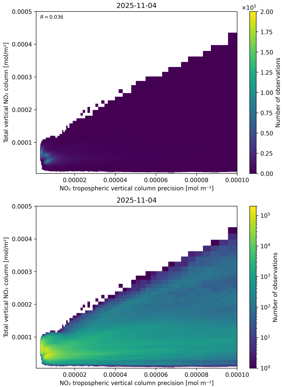
Figure 138: Scatter density plot of “NO 2 tropospheric vertical column precision” against “Total vertical NO 2 column” for 2025-11-03 to 2025-11-05.
