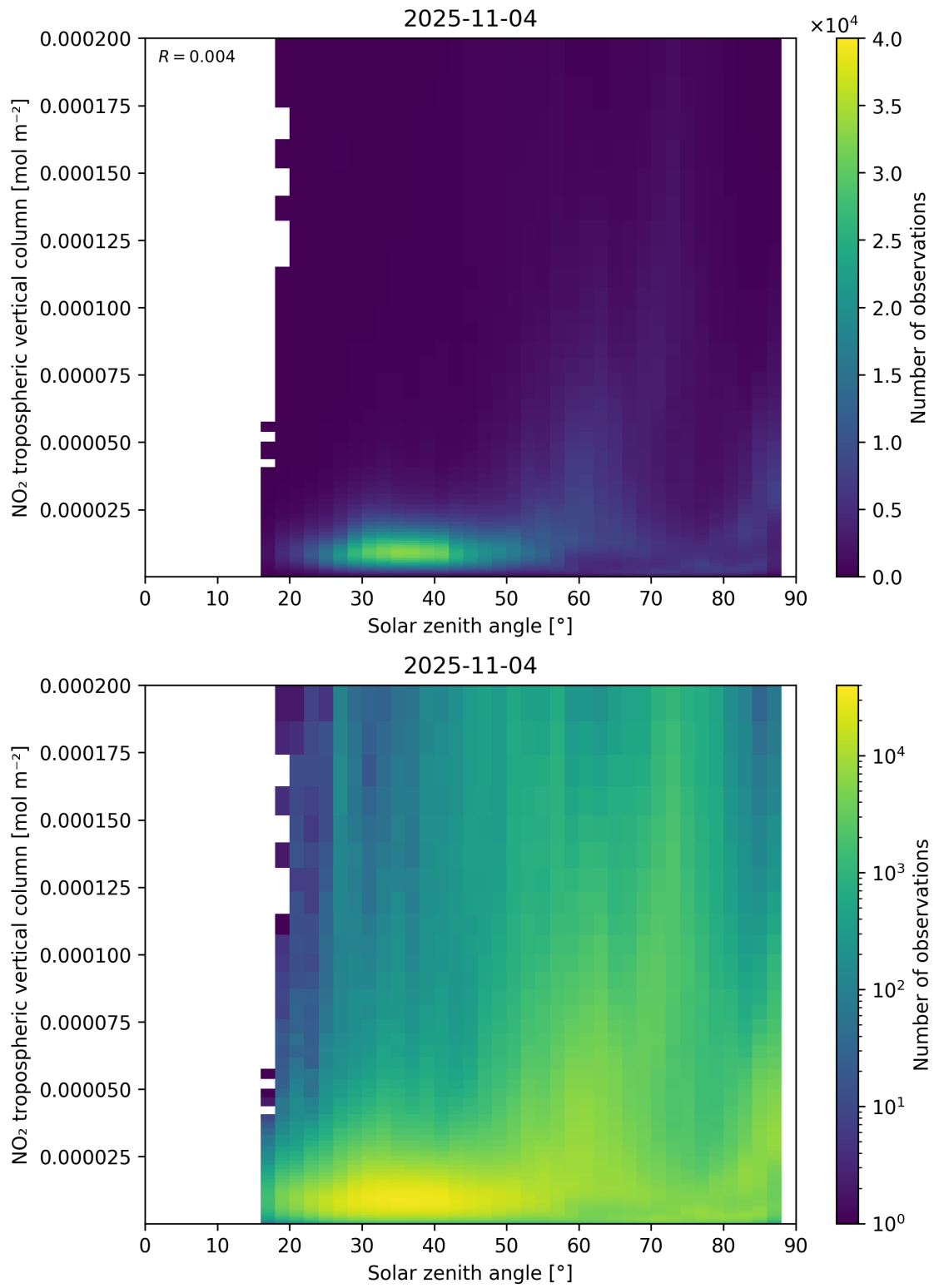
Figure 155: Scatter density plot of “Solar zenith angle” against “NO 2 tropospheric vertical column” for 2025-11-03 to 2025-11-05.
