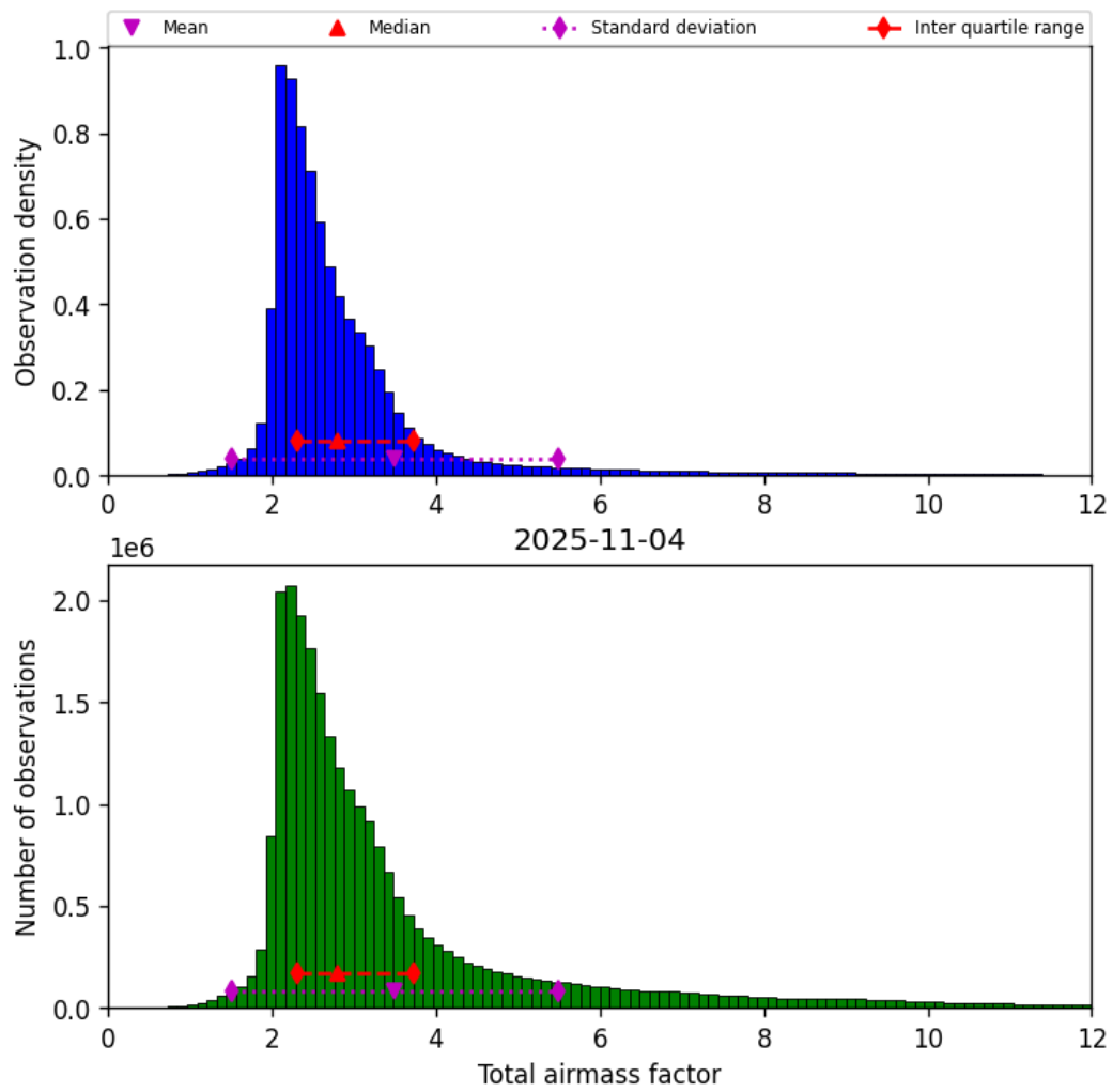
Figure 32: Histogram of “Total airmass factor” for 2025-11-03 to 2025-11-05
