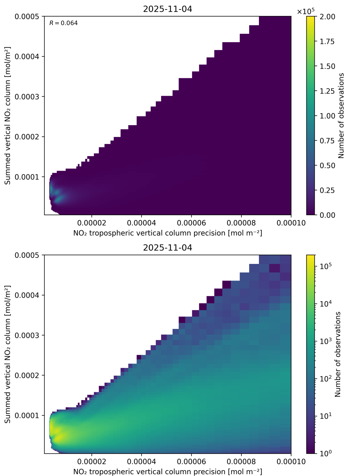
Figure 136: Scatter density plot of “NO 2 tropospheric vertical column precision” against “Summed vertical NO 2 column” for 2025-11-03 to 2025-11-05.
