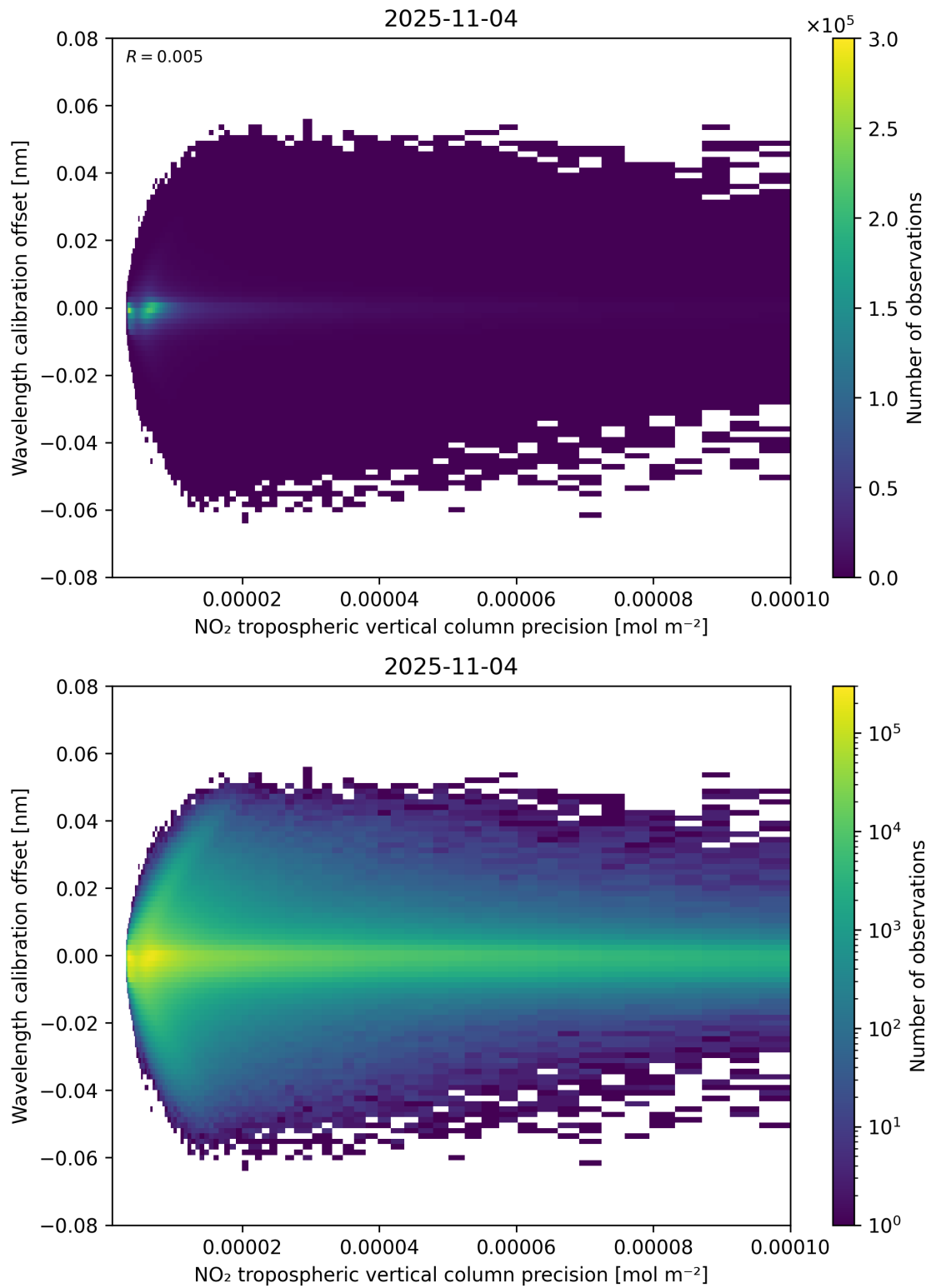
Figure 141: Scatter density plot of “NO 2 tropospheric vertical column precision” against “Wavelength calibration offset” for 2025-11-03 to 2025-11-05.
