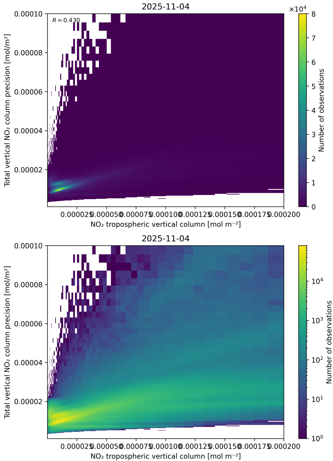
Figure 129: Scatter density plot of “NO 2 tropospheric vertical column” against “Total vertical NO 2 column precision” for 2025-11-03 to 2025-11-05.
