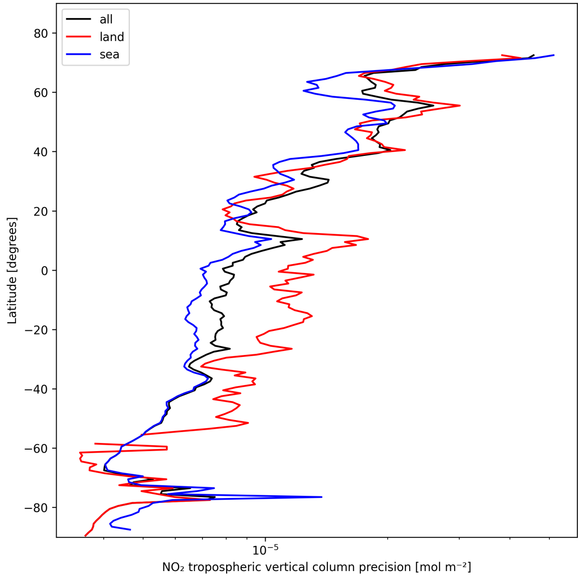
Figure 13: Zonal average of “NO 2 tropospheric vertical column precision” for 2025-11-03 to 2025-11-05.
