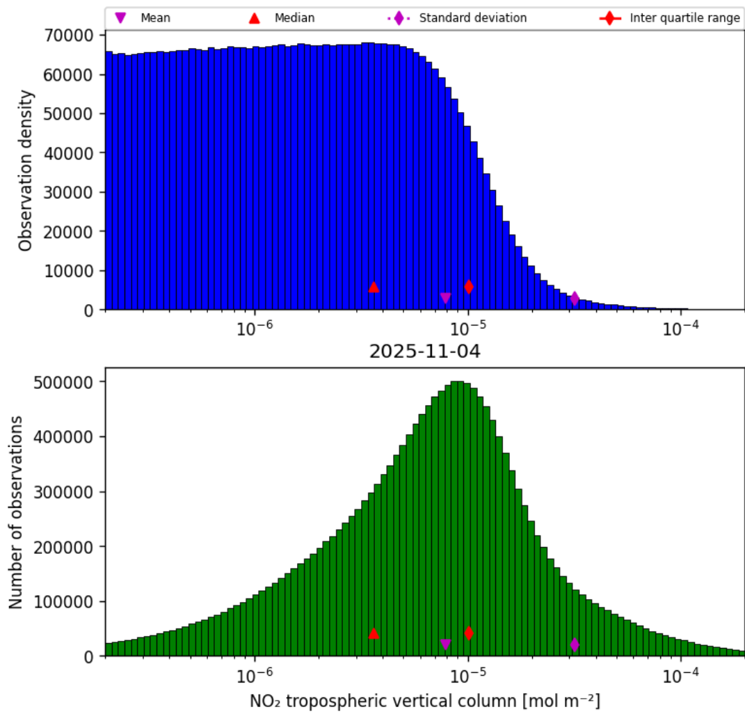
Figure 29: Histogram of “NO 2 tropospheric vertical column” for 2025-11-03 to 2025-11-05
