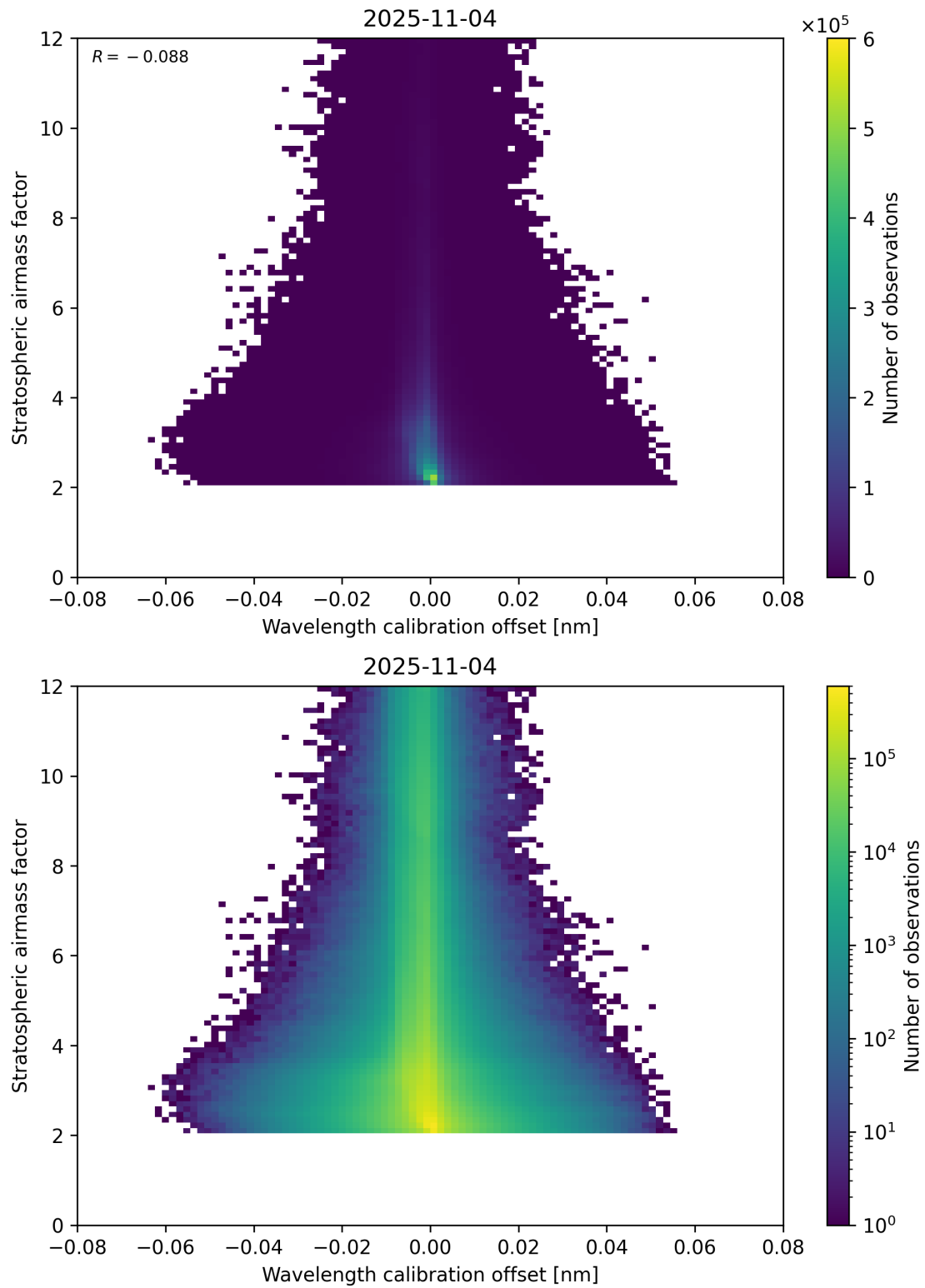
Figure 174: Scatter density plot of “Wavelength calibration offset” against “Stratospheric airmass factor” for 2025-11-03 to 2025-11-05.
