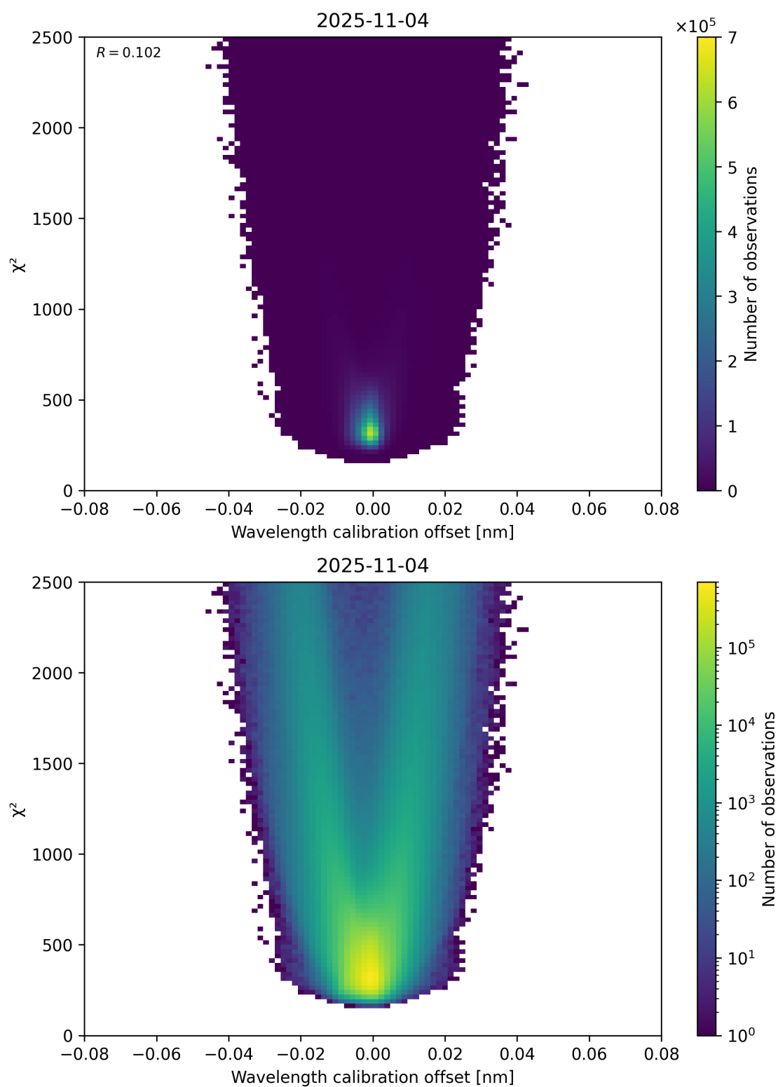
Figure 175: Scatter density plot of “Wavelength calibration offset” against “ \chi^2 ” for 2025-11-03 to 2025-11-05.
