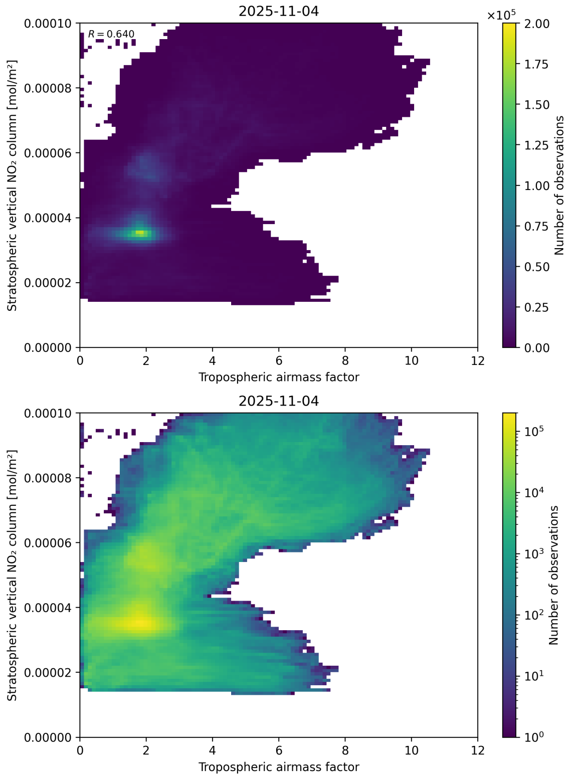
Figure 74: Scatter density plot of “Tropospheric air mass factor” against “Stratospheric vertical NO 2 column” for 2025-11-03 to 2025-11-05.
