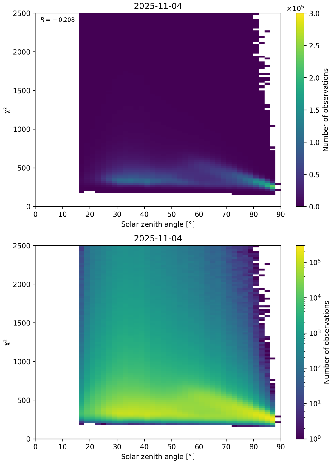
Figure 148: Scatter density plot of “Solar zenith angle” against “ \chi^2 ” for 2025-11-03 to 2025-11-05.
