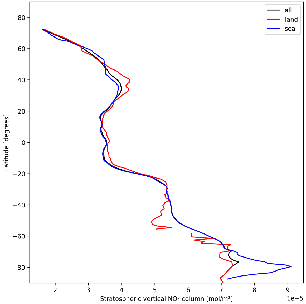
Figure 19: Zonal average of “Stratospheric vertical NO 2 column” for 2025-11-03 to 2025-11-05.
