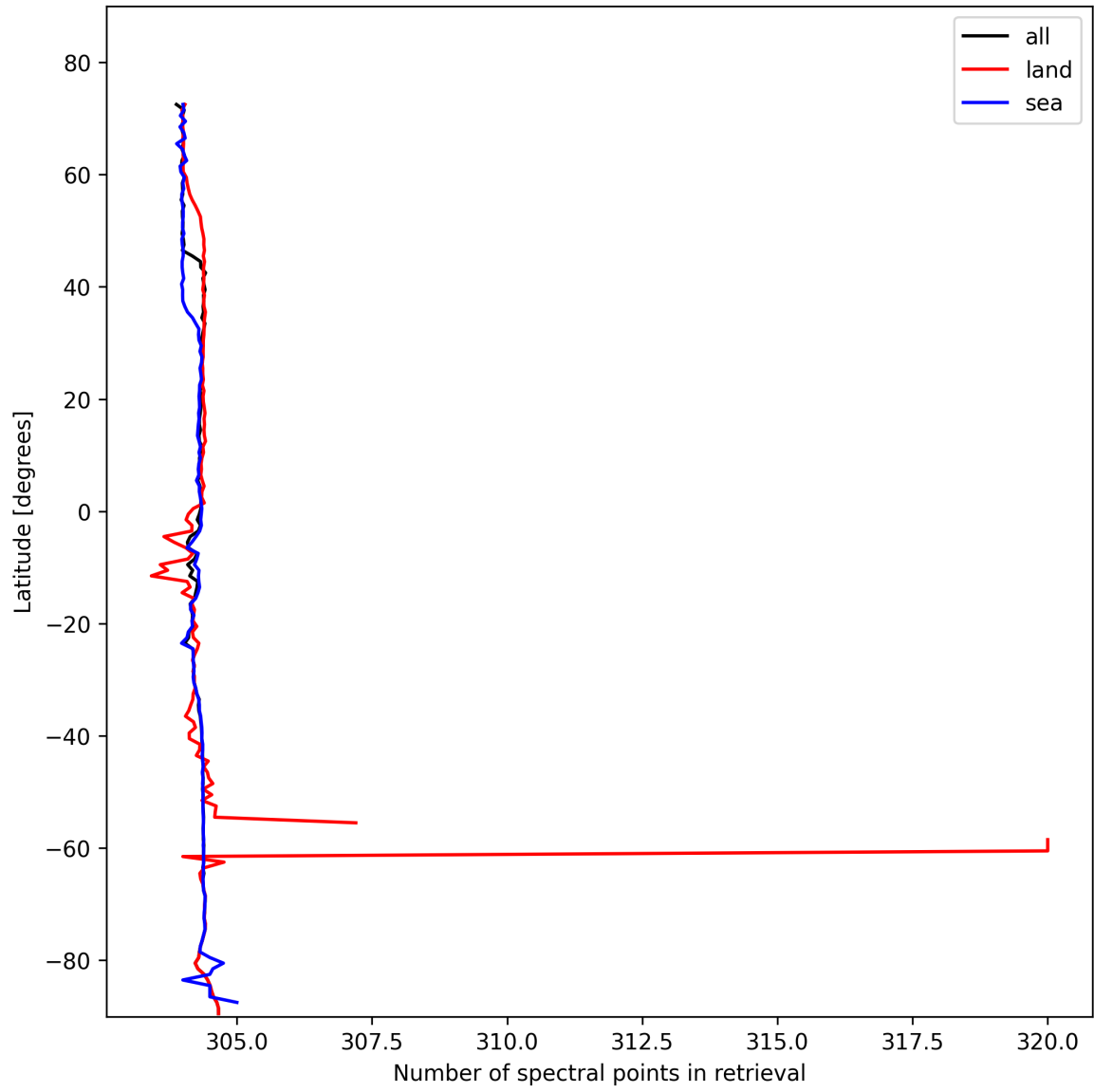
Figure 16: Zonal average of “Number of spectral points in retrieval” for 2025-11-03 to 2025-11-05.
