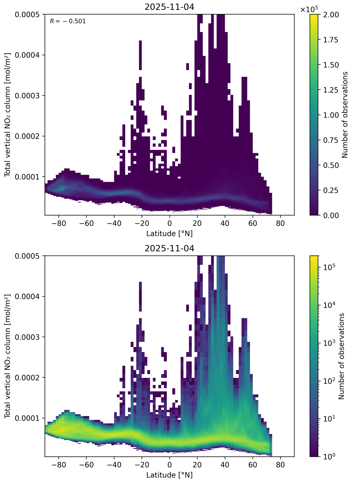
Figure 90: Scatter density plot of “Latitude” against “Total vertical NO 2 column” for 2025-11-03 to 2025-11-05.
