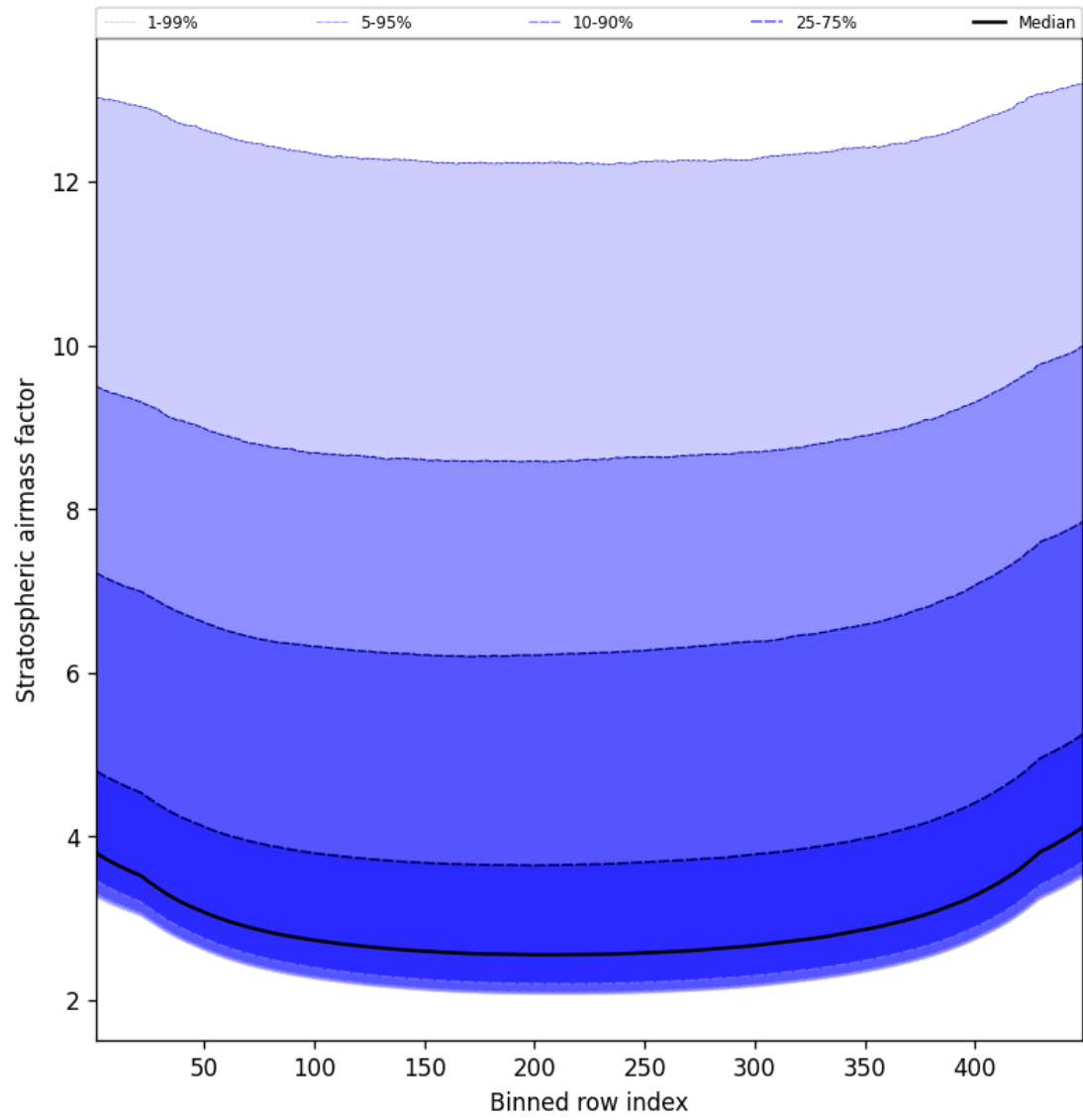
Figure 61: Along track statistics of “Stratospheric airmass factor” for 2025-11-03 to 2025-11-05
