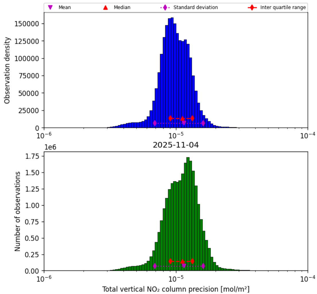
Figure 39: Histogram of “Total vertical NO 2 column precision” for 2025-11-03 to 2025-11-05
