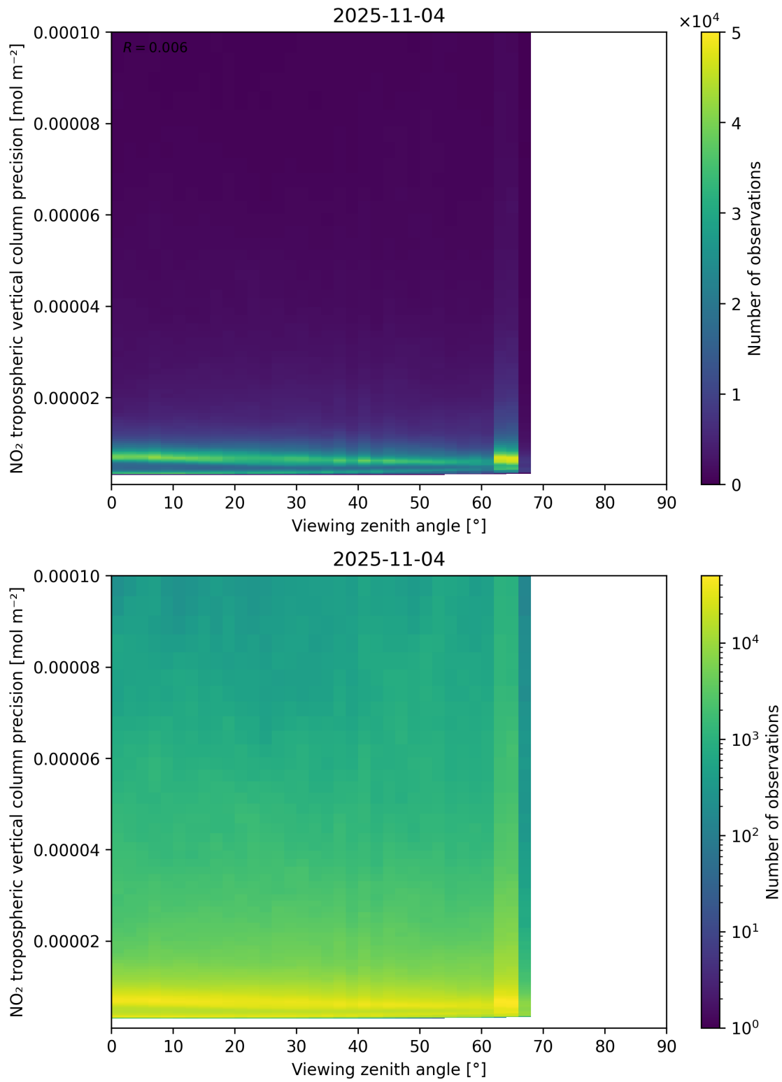
Figure 170: Scatter density plot of “Viewing zenith angle” against “NO 2 tropospheric vertical column precision” for 2025-11-03 to 2025-11-05.
