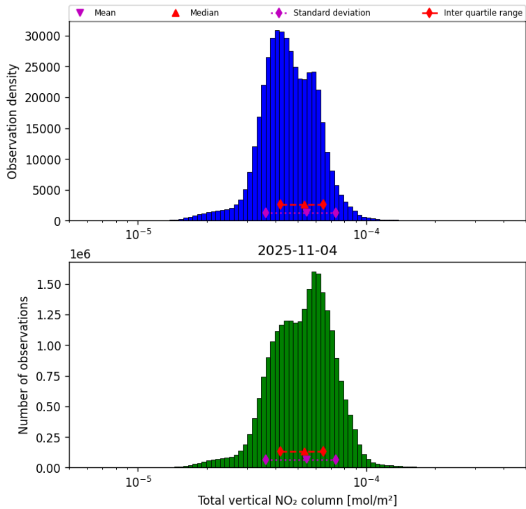
Figure 38: Histogram of “Total vertical NO 2 column” for 2025-11-03 to 2025-11-05
