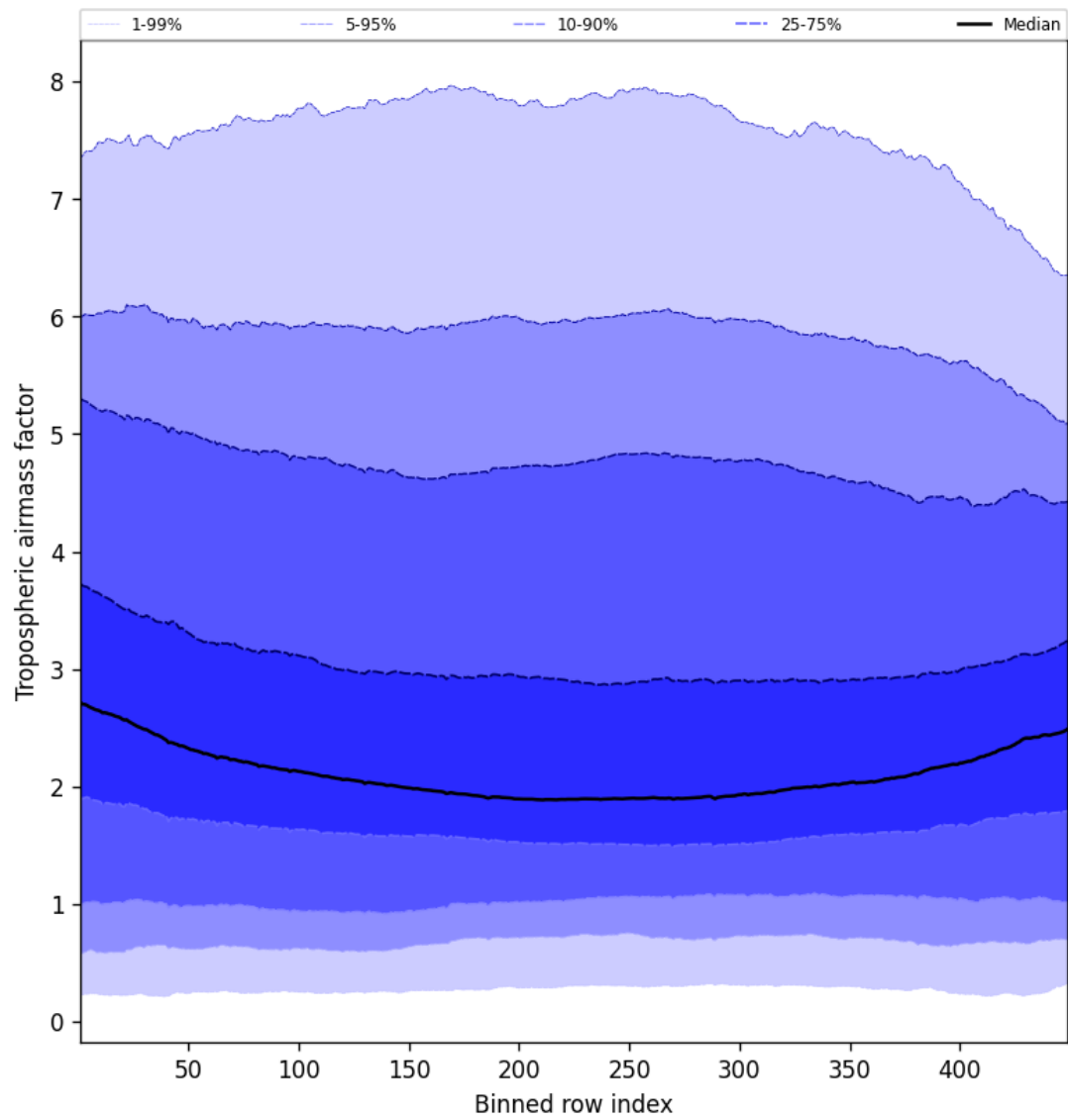
Figure 48: Along track statistics of “Tropospheric air mass factor” for 2025-11-03 to 2025-11-05
