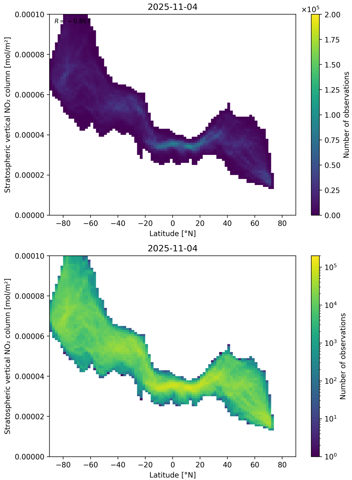
Figure 87: Scatter density plot of “Latitude” against “Stratospheric vertical NO 2 column” for 2025-11-03 to 2025-11-05.
