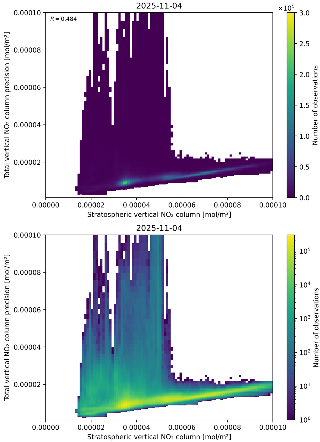
Figure 101: Scatter density plot of “Stratospheric vertical NO 2 column” against “Total vertical NO 2 column precision” for 2025-11-03 to 2025-11-05.
