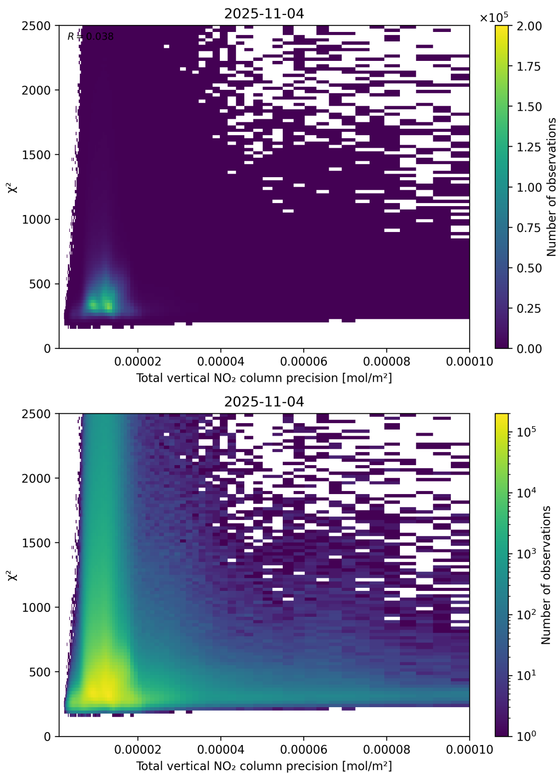
Figure 116: Scatter density plot of “Total vertical NO 2 column precision” against “ \chi^2 ” for 2025-11-03 to 2025-11-05.
