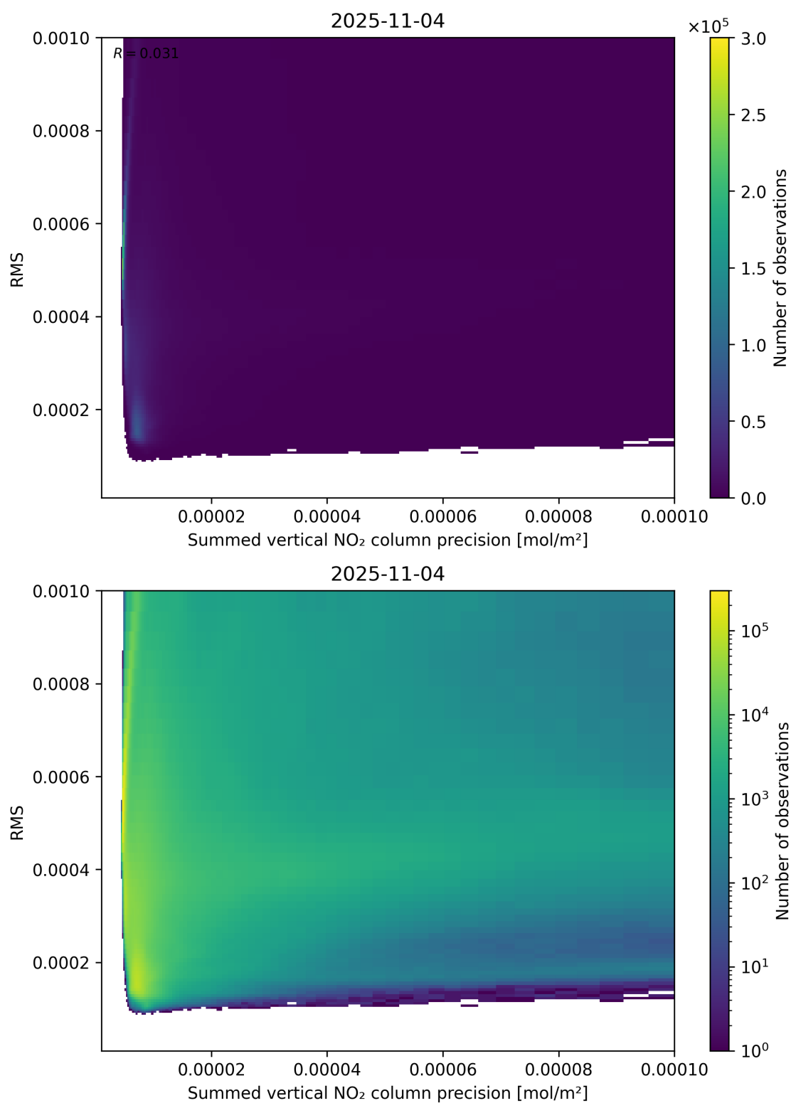
Figure 108: Scatter density plot of “Summed vertical NO 2 column precision” against “RMS” for 2025-11-03 to 2025-11-05.
