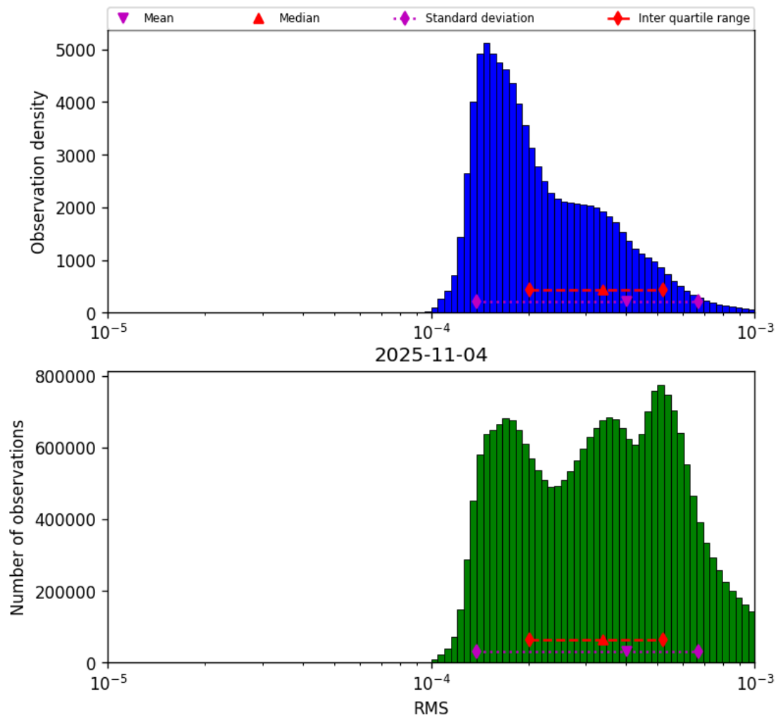
Figure 43: Histogram of “RMS” for 2025-11-03 to 2025-11-05
