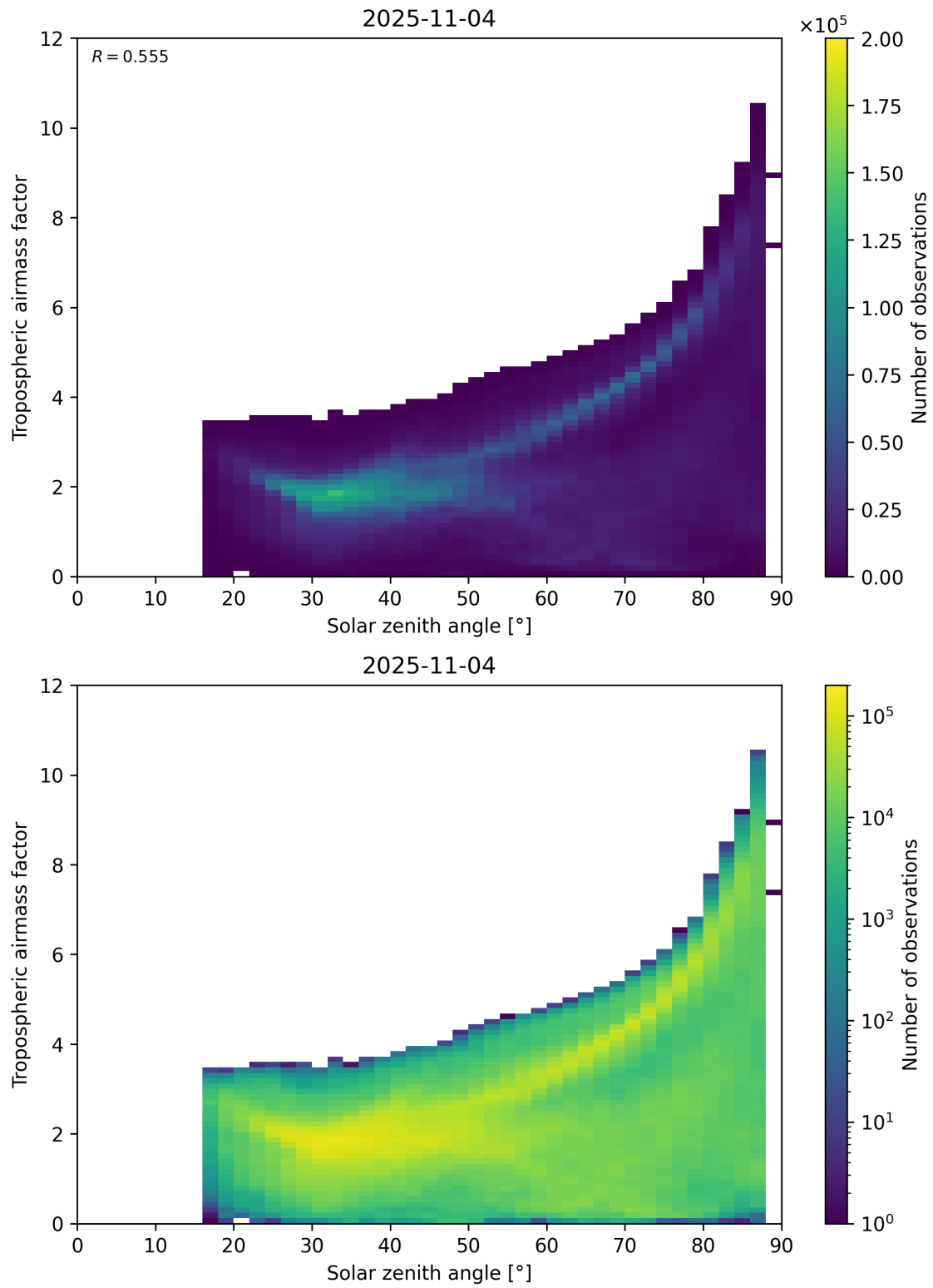
Figure 147: Scatter density plot of “Solar zenith angle” against “Tropospheric airmass factor” for 2025-11-03 to 2025-11-05.
