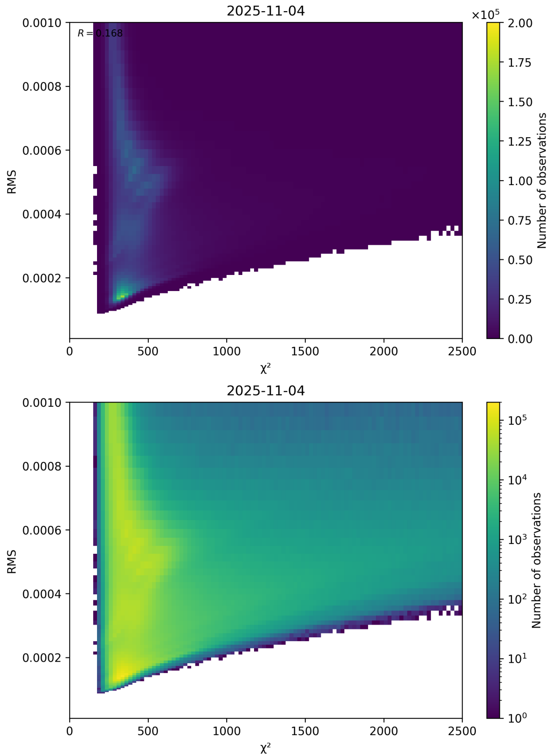
Figure 82: Scatter density plot of “ \chi^2 ” against “RMS” for 2025-11-03 to 2025-11-05.
