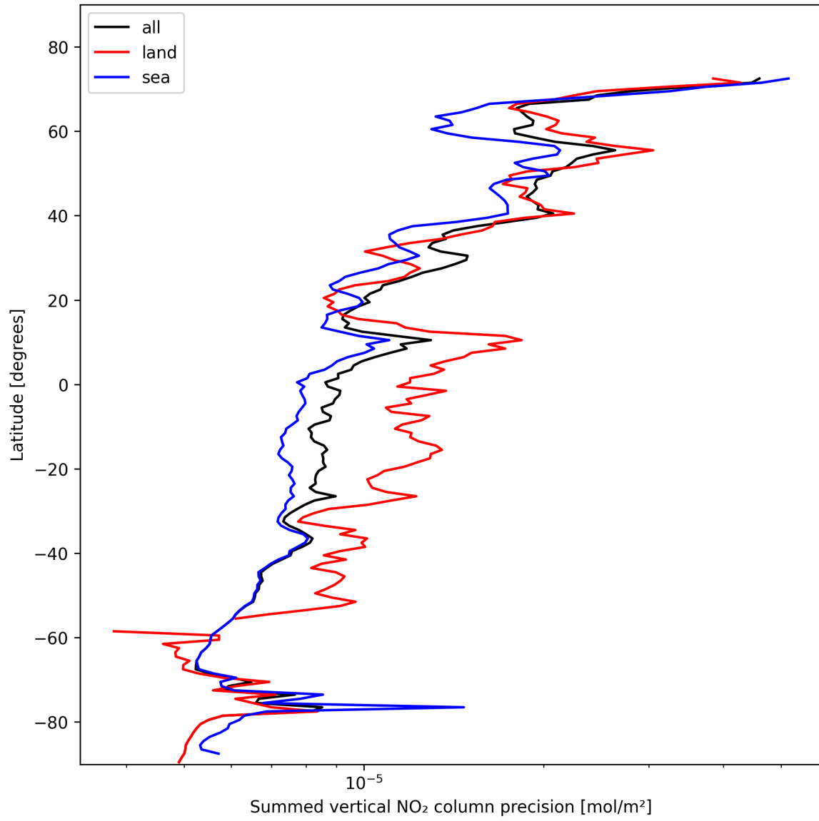
Figure 24: Zonal average of “Summed vertical NO 2 column precision” for 2025-11-03 to 2025-11-05.
