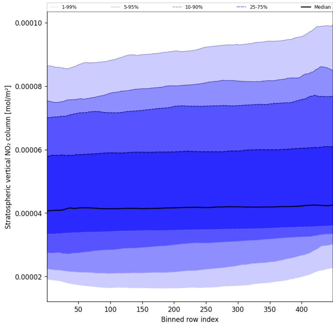
Figure 53: Along track statistics of “Stratospheric vertical NO 2 column” for 2025-11-03 to 2025-11-05
