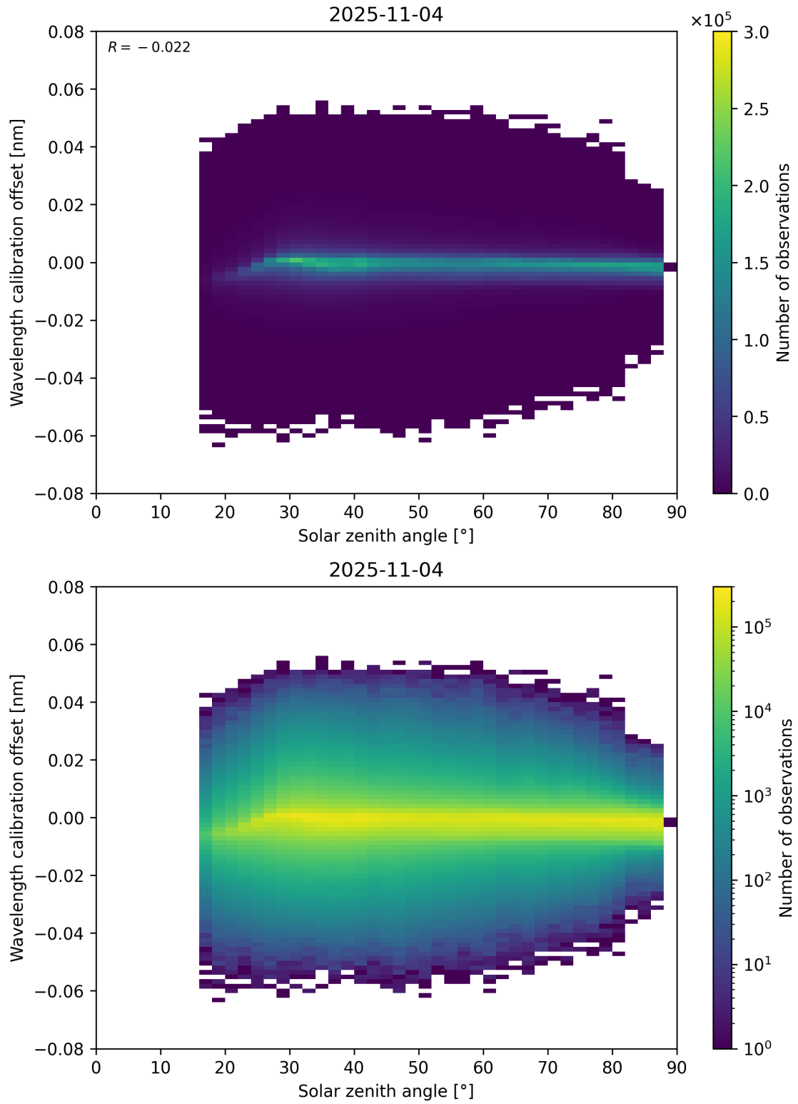
Figure 158: Scatter density plot of “Solar zenith angle” against “Wavelength calibration offset” for 2025-11-03 to 2025-11-05.
