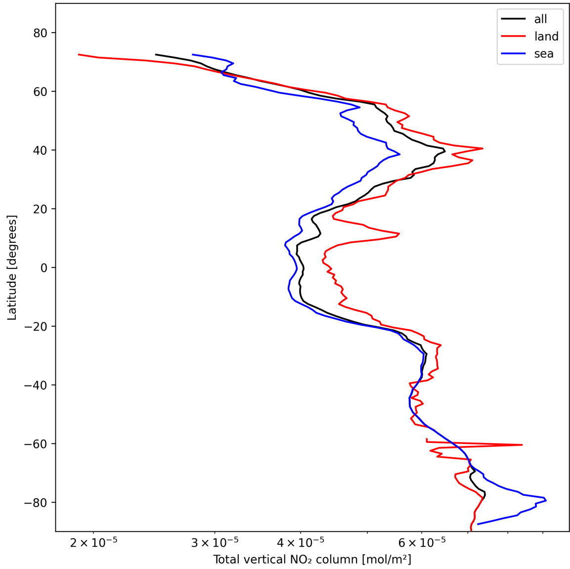
Figure 21: Zonal average of “Total vertical NO 2 column” for 2025-11-03 to 2025-11-05.
