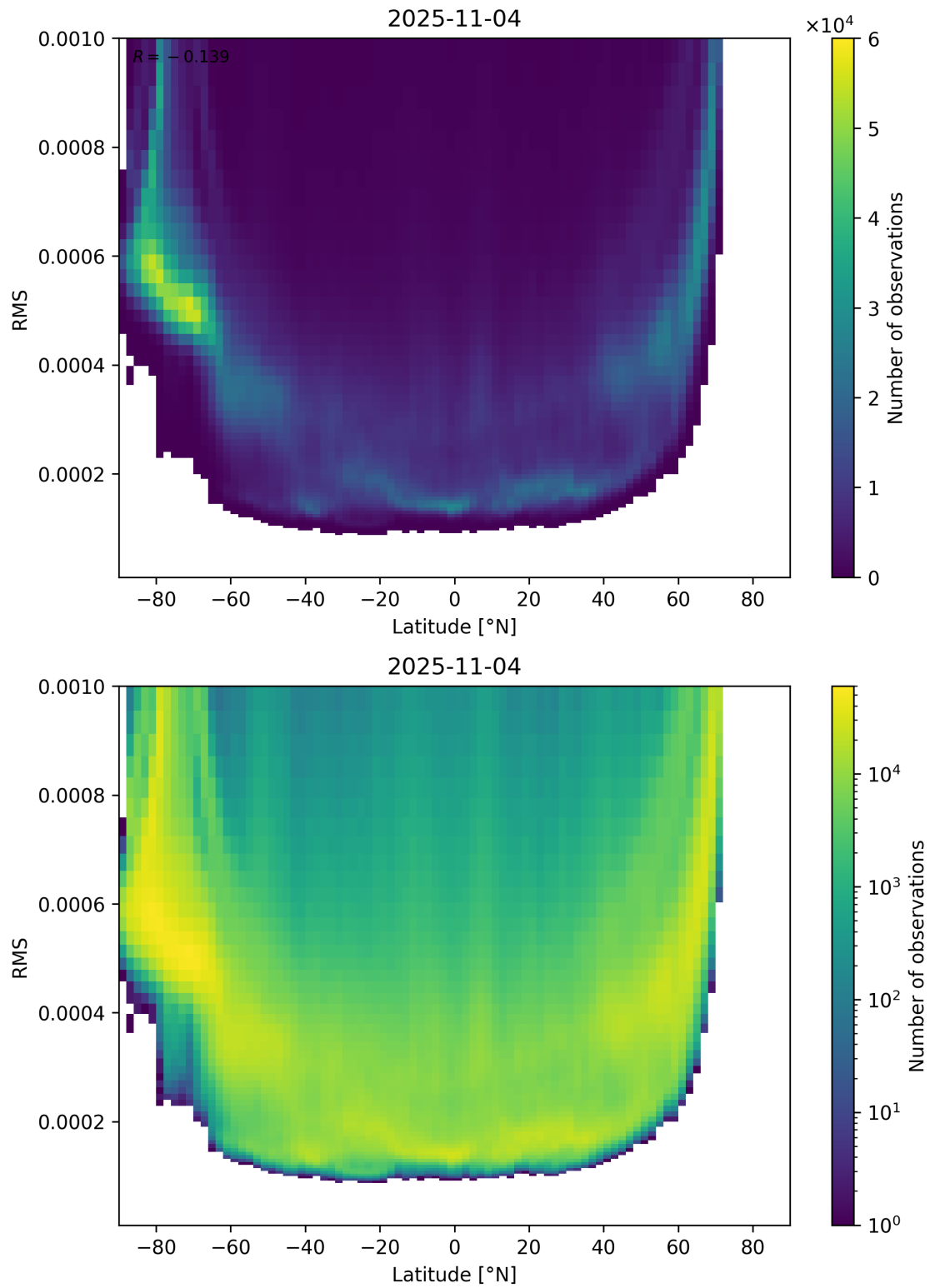
Figure 94: Scatter density plot of “Latitude” against “RMS” for 2025-11-03 to 2025-11-05.
