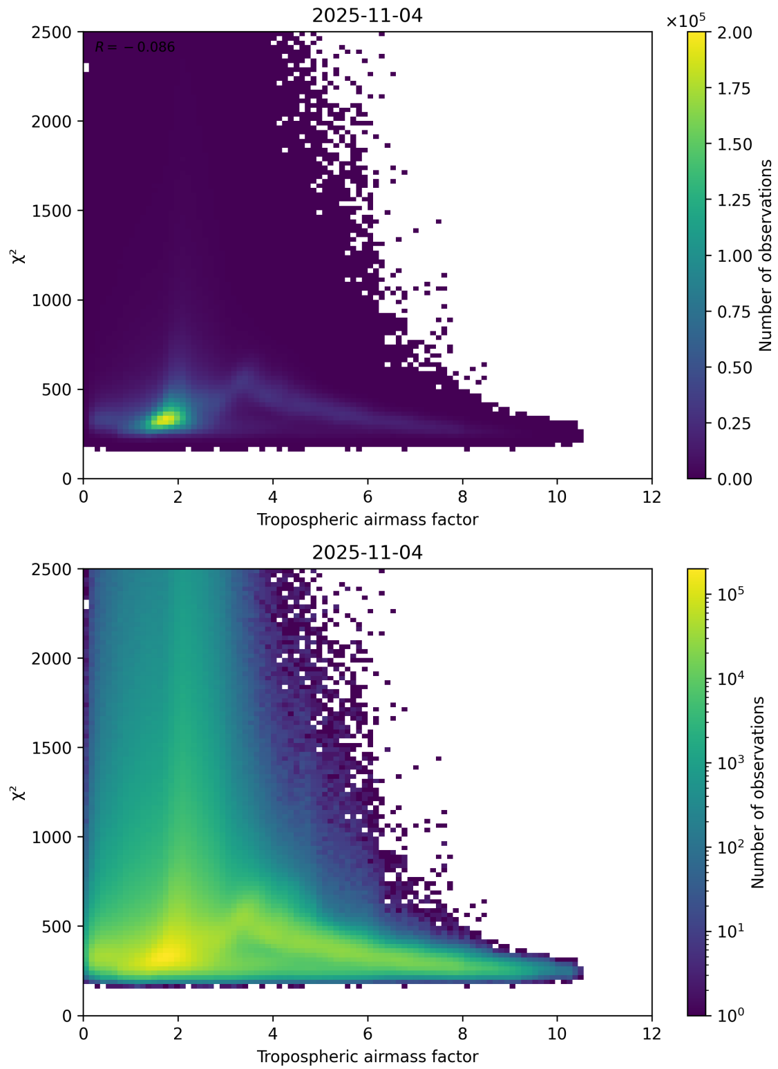
Figure 73: Scatter density plot of “Tropospheric airmass factor” against “ \chi^2 ” for 2025-11-03 to 2025-11-05.
