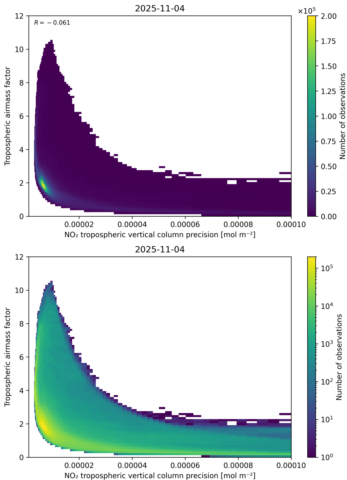
Figure 133: Scatter density plot of “NO 2 tropospheric vertical column precision” against “Tropospheric air mass factor” for 2025-11-03 to 2025-11-05.
