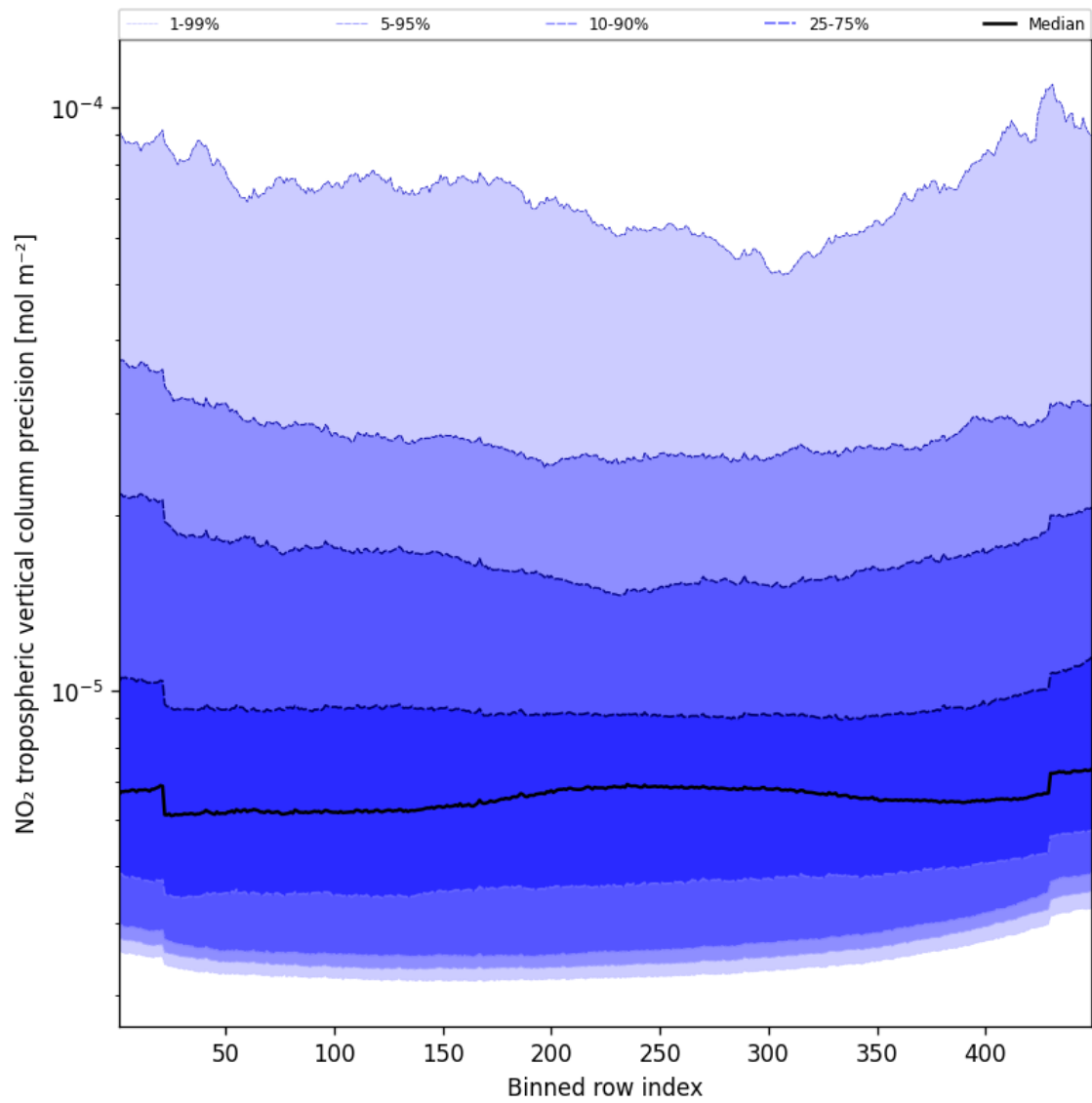
Figure 47: Along track statistics of “NO 2 tropospheric vertical column precision” for 2025-11-03 to 2025-11-05
