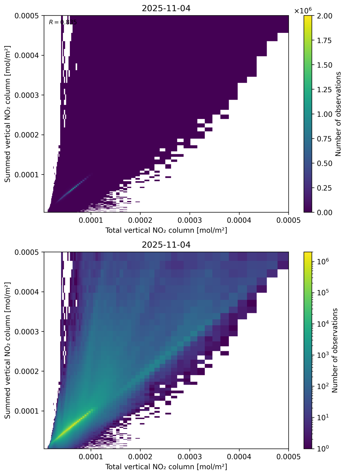
Figure 112: Scatter density plot of “Total vertical NO 2 column” against “Summed vertical NO 2 column” for 2025-11-03 to 2025-11-05.
