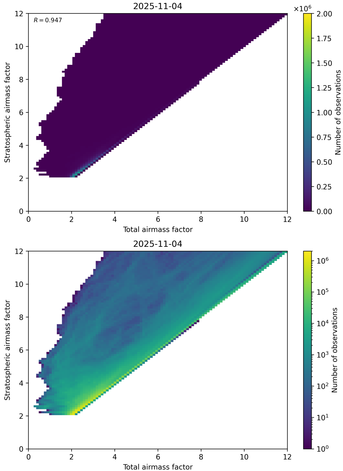
Figure 62: Scatter density plot of “Total airmass factor” against “Stratospheric airmass factor” for 2025-11-03 to 2025-11-05.
