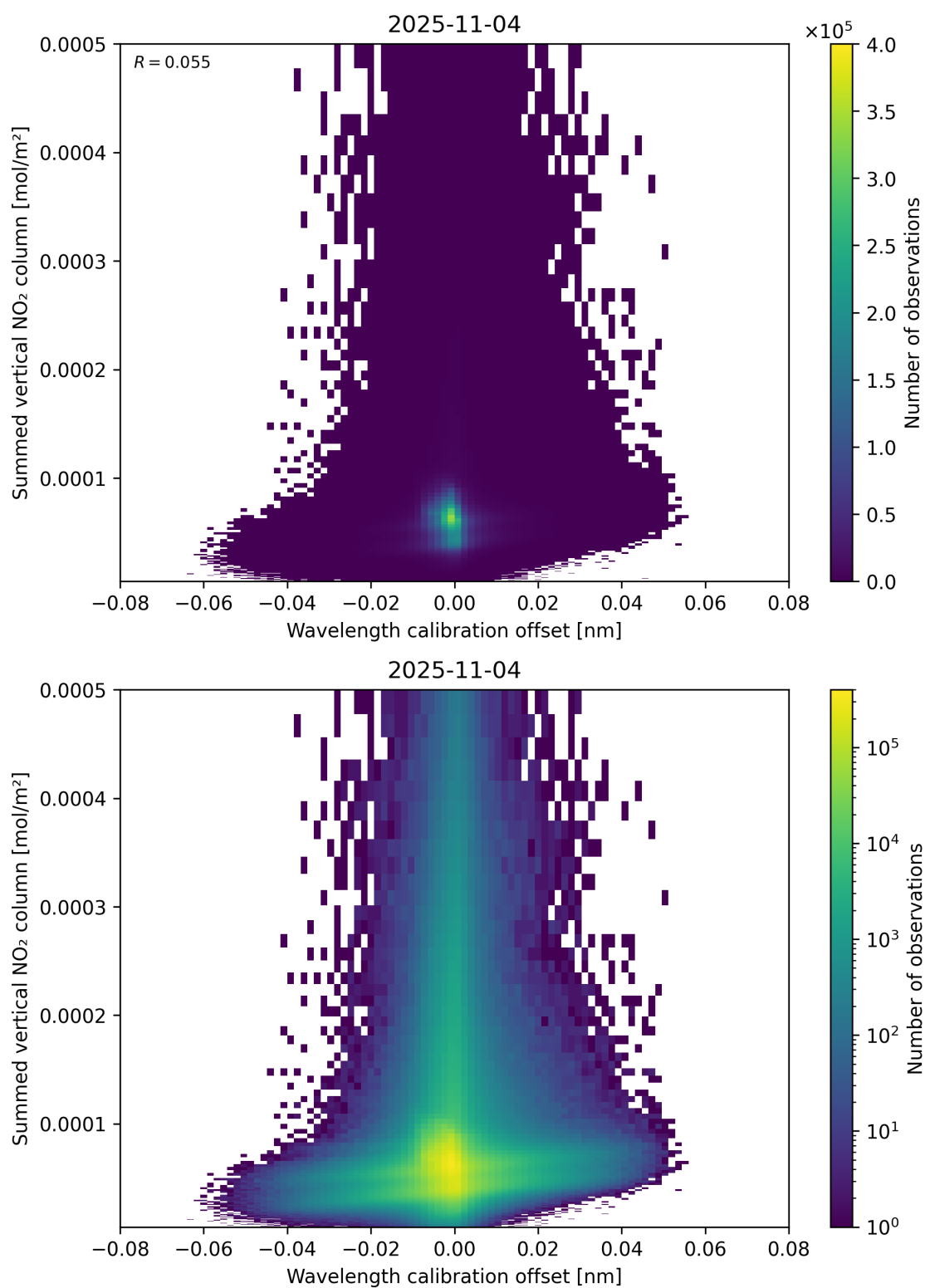
Figure 177: Scatter density plot of “Wavelength calibration offset” against “Summed vertical NO 2 column” for 2025-11-03 to 2025-11-05.
