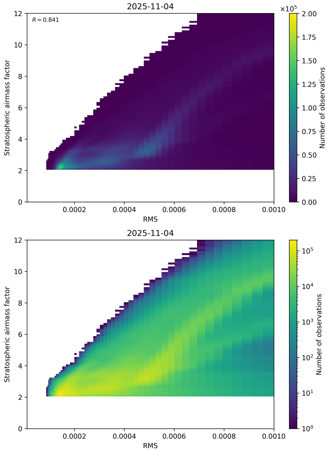
Figure 144: Scatter density plot of “RMS” against “Stratospheric airmass factor” for 2025-11-03 to 2025-11-05.
