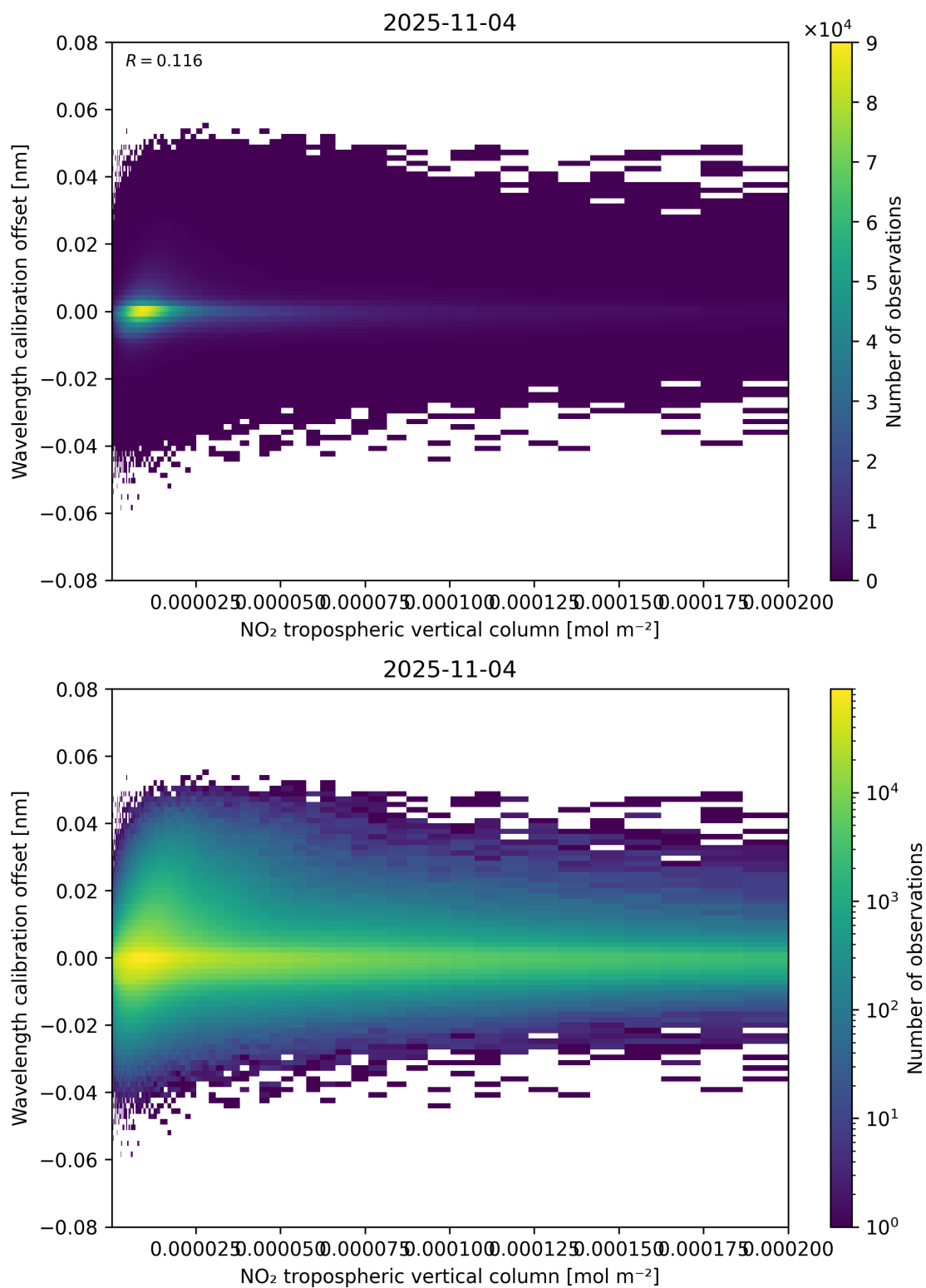
Figure 143: Scatter density plot of “NO 2 tropospheric vertical column” against “Wavelength calibration offset” for 2025-11-03 to 2025-11-05.
