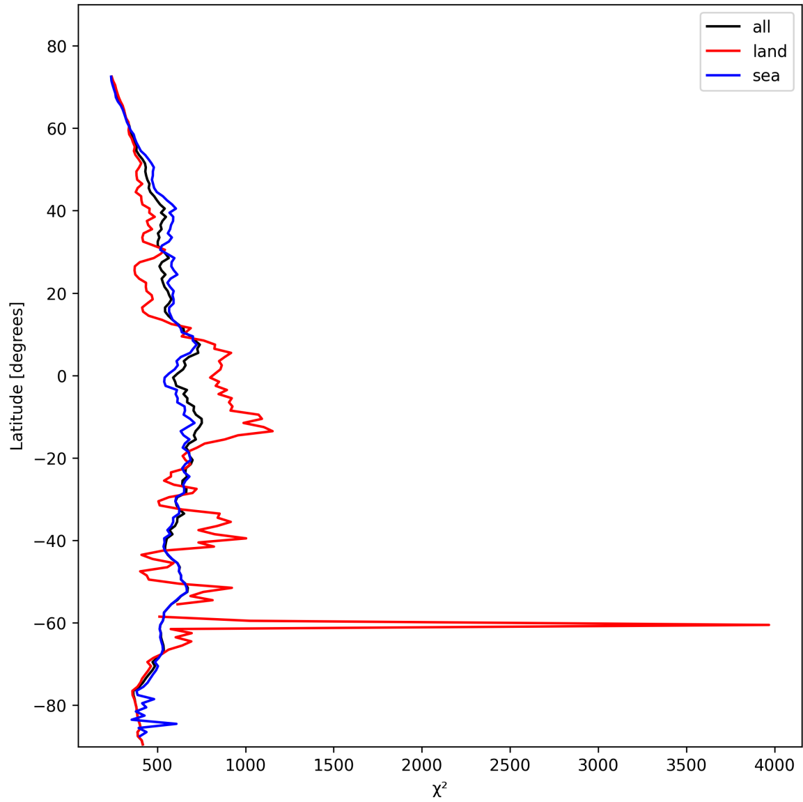
Figure 25: Zonal average of “ \chi^2 ” for 2025-11-03 to 2025-11-05.
