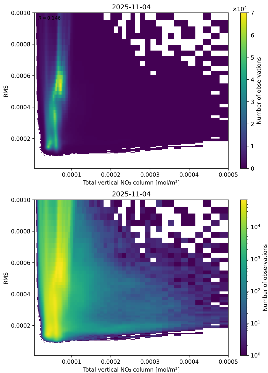
Figure 120: Scatter density plot of “Total vertical NO 2 column” against “RMS” for 2025-11-03 to 2025-11-05.
