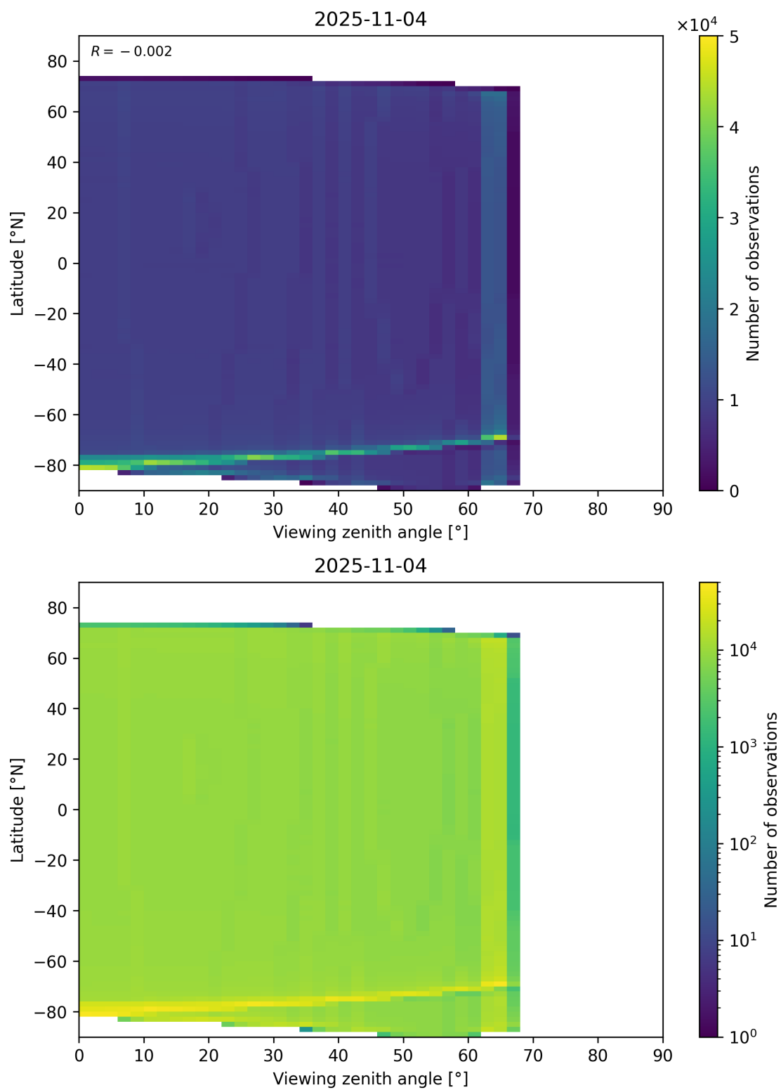
Figure 163: Scatter density plot of “Viewing zenith angle” against “Latitude” for 2025-11-03 to 2025-11-05.
