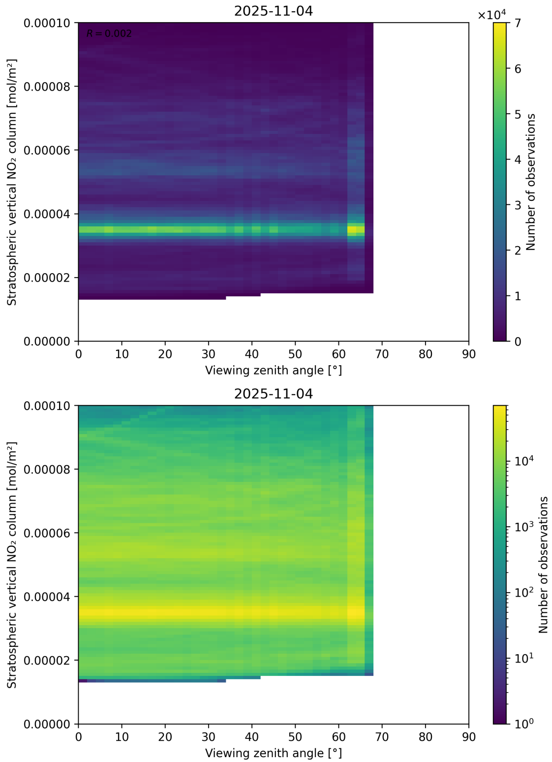
Figure 164: Scatter density plot of “Viewing zenith angle” against “Stratospheric vertical NO 2 column” for 2025-11-03 to 2025-11-05.
