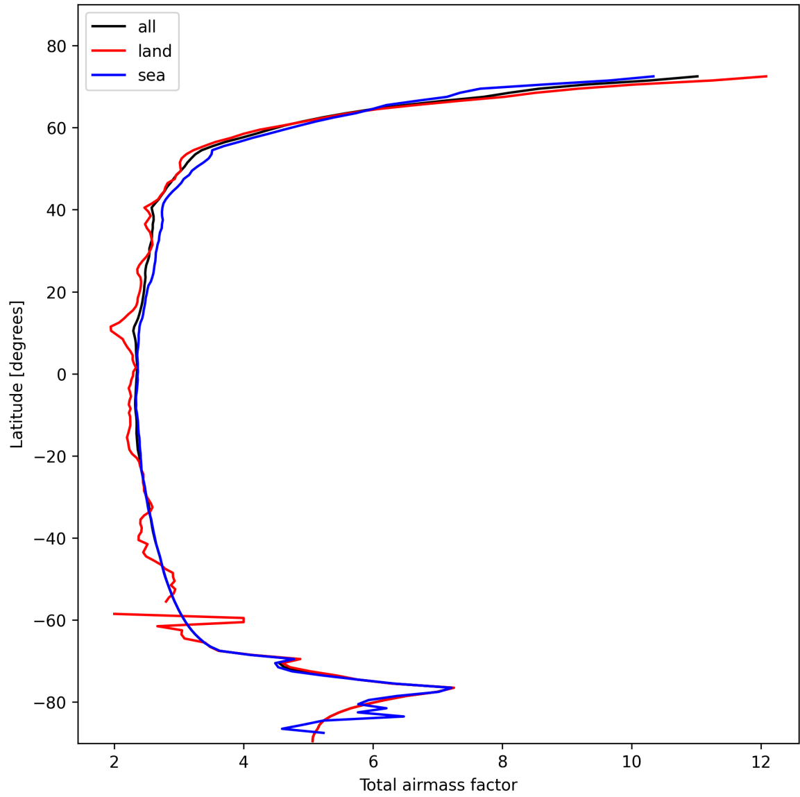
Figure 15: Zonal average of “Total airmass factor” for 2025-11-03 to 2025-11-05.
