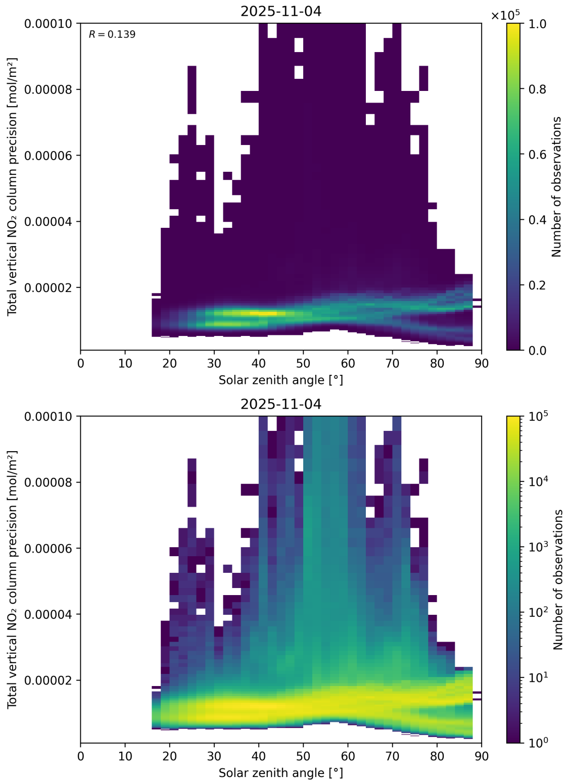
Figure 154: Scatter density plot of “Solar zenith angle” against “Total vertical NO 2 column precision” for 2025-11-03 to 2025-11-05.
