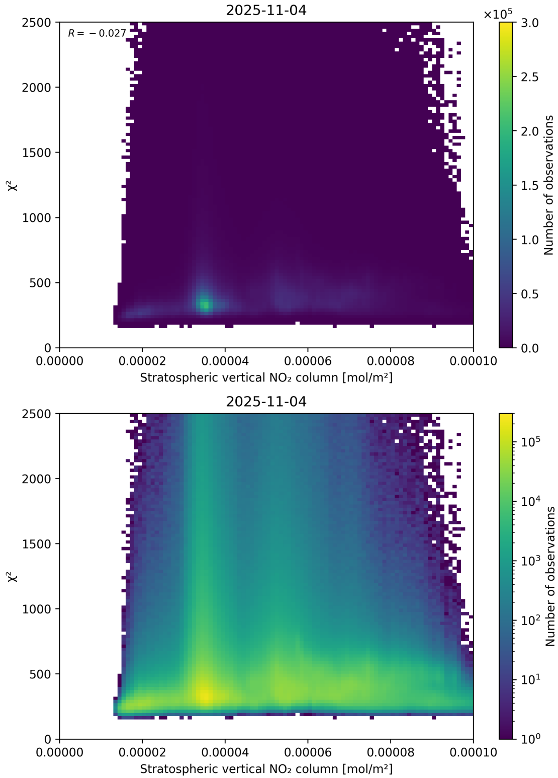
Figure 97: Scatter density plot of “Stratospheric vertical NO 2 column” against “ \chi^2 ” for 2025-11-03 to 2025-11-05.
