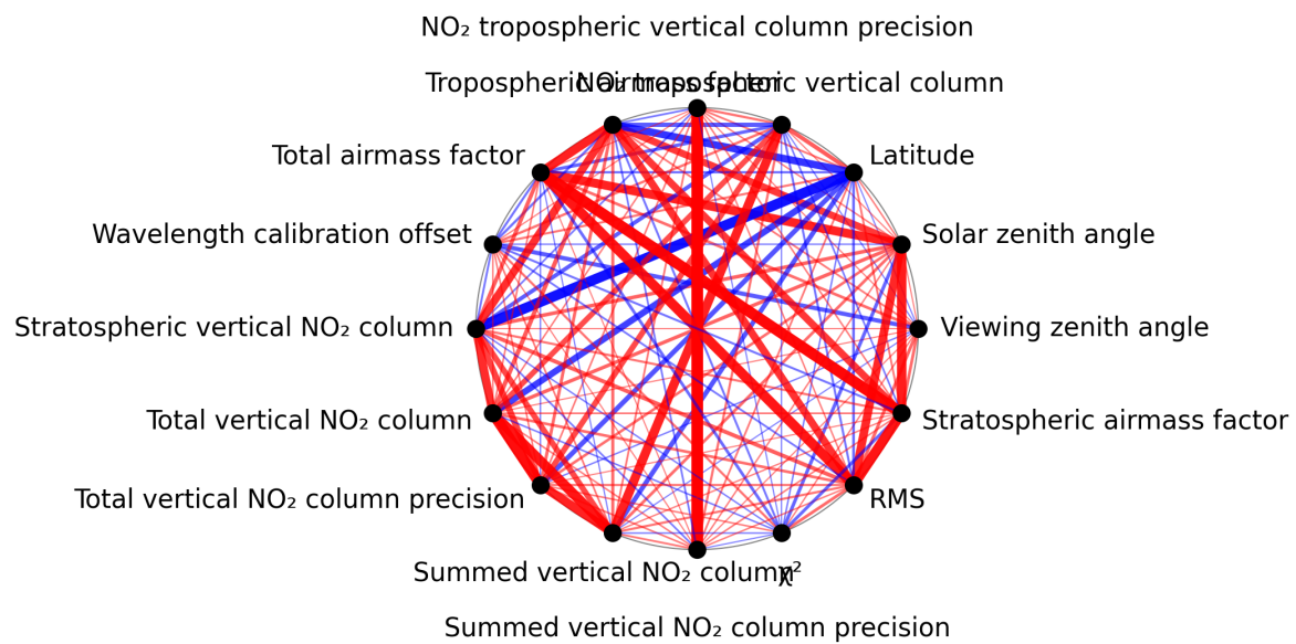
Figure 1: Map of correlation graph for 2025-11-03 to 2025-11-05.
