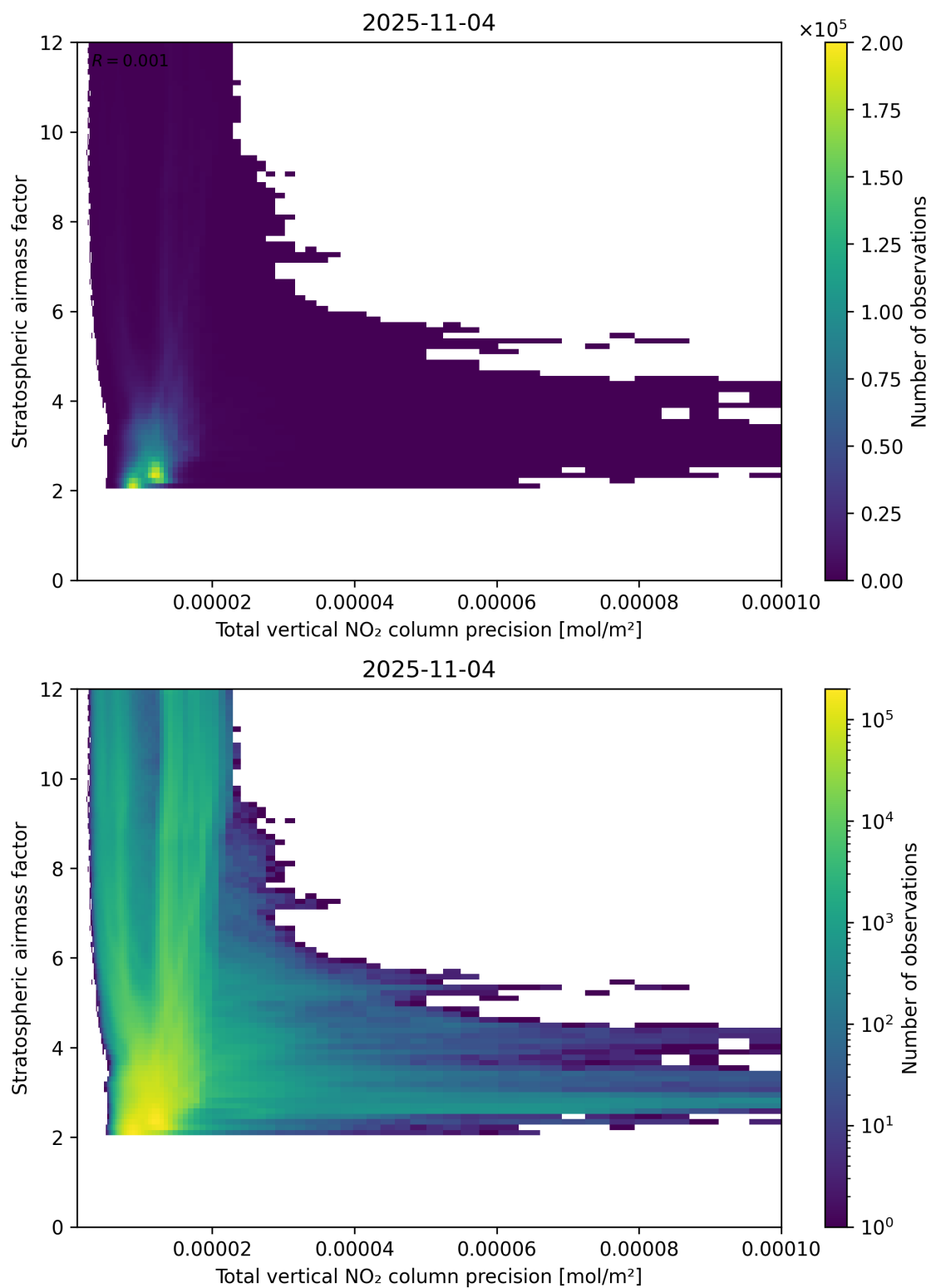
Figure 115: Scatter density plot of “Total vertical NO 2 column precision” against “Stratospheric air mass factor” for 2025-11-03 to 2025-11-05.
