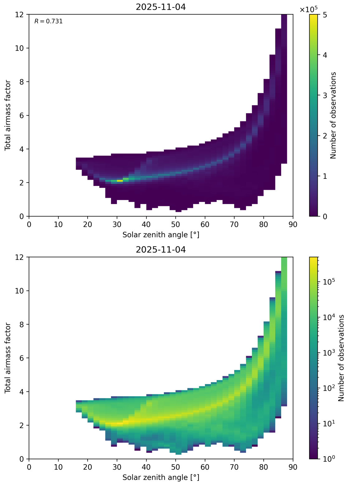
Figure 146: Scatter density plot of “Solar zenith angle” against “Total airmass factor” for 2025-11-03 to 2025-11-05.
