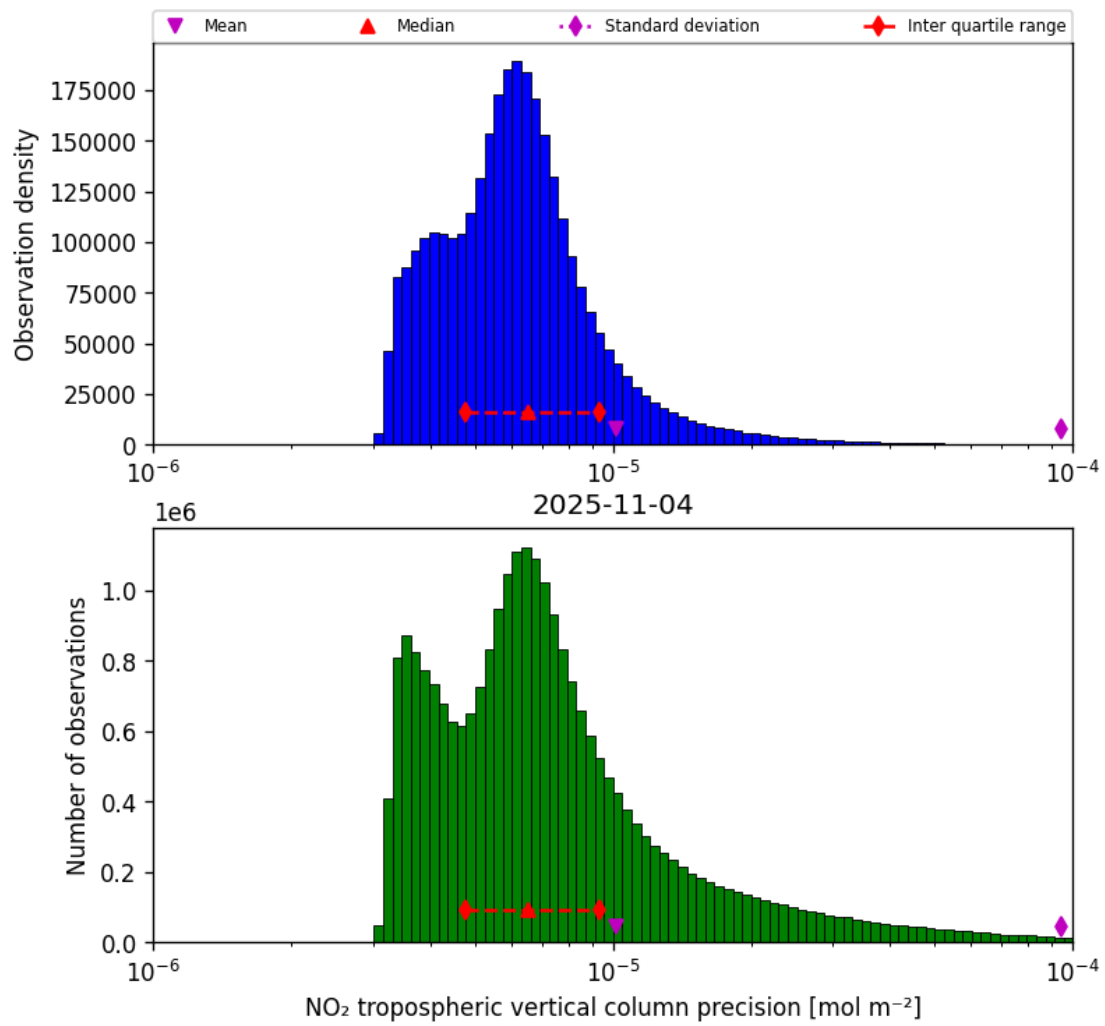
Figure 30: Histogram of “NO 2 tropospheric vertical column precision” for 2025-11-03 to 2025-11-05
