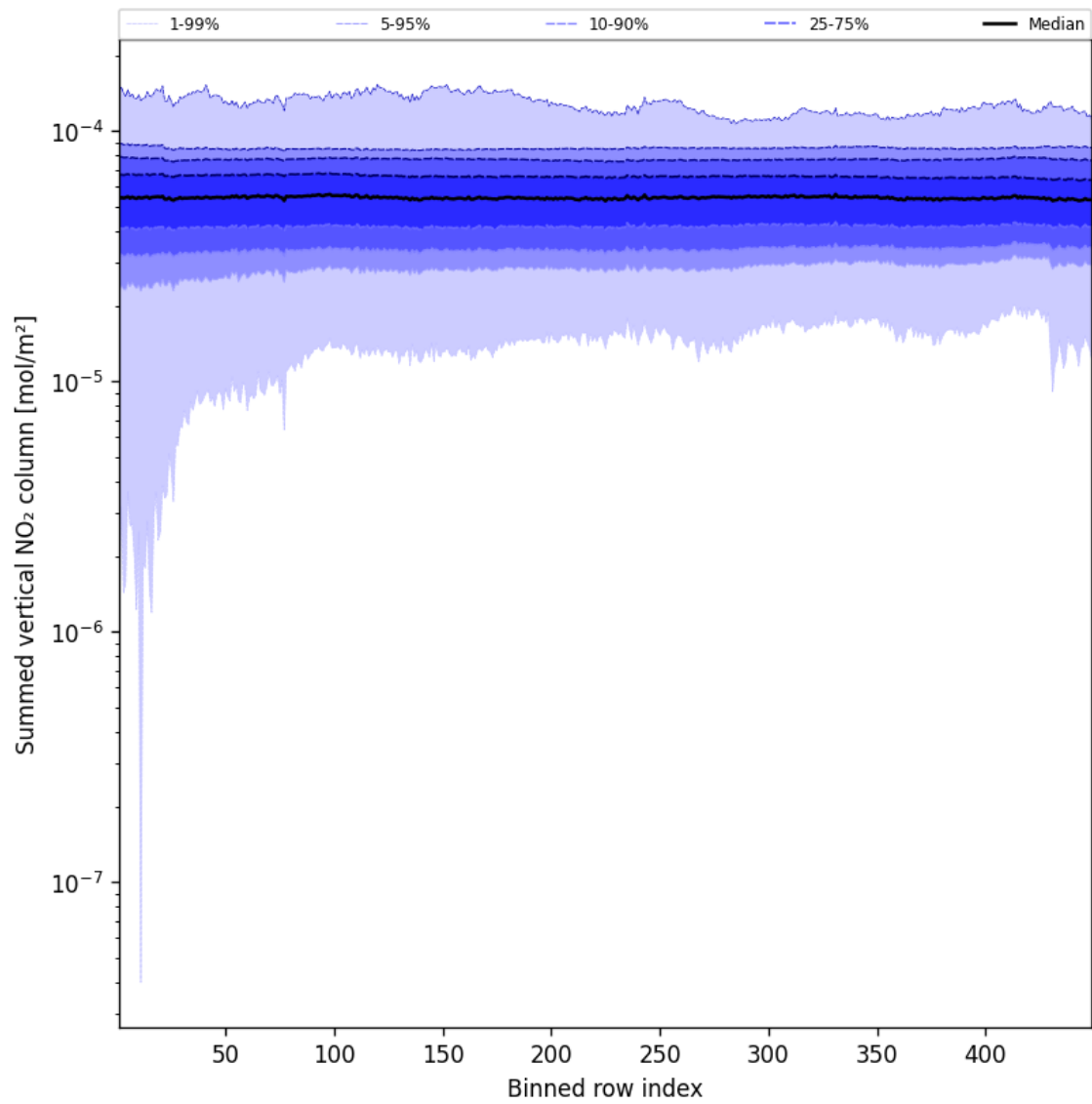
Figure 57: Along track statistics of “Summed vertical NO 2 column” for 2025-11-03 to 2025-11-05
