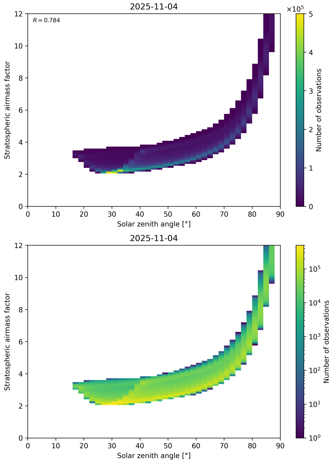
Figure 145: Scatter density plot of “Solar zenith angle” against “Stratospheric airmass factor” for 2025-11-03 to 2025-11-05.
