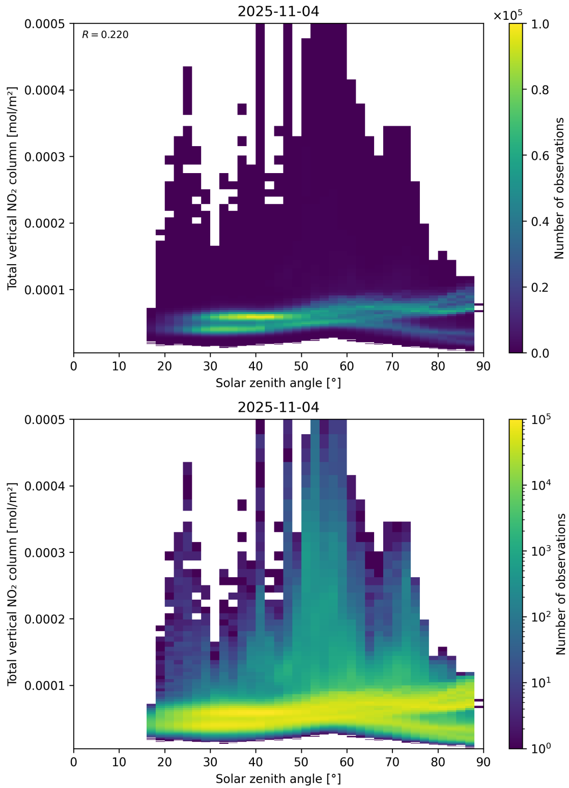
Figure 153: Scatter density plot of “Solar zenith angle” against “Total vertical NO 2 column” for 2025-11-03 to 2025-11-05.
