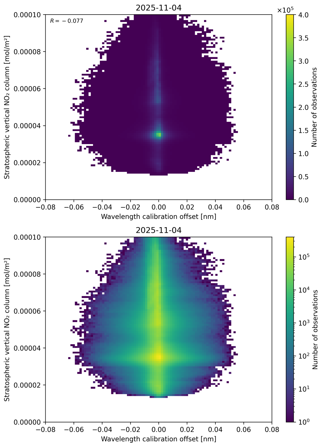
Figure 176: Scatter density plot of “Wavelength calibration offset” against “Stratospheric vertical NO 2 column” for 2025-11-03 to 2025-11-05.
