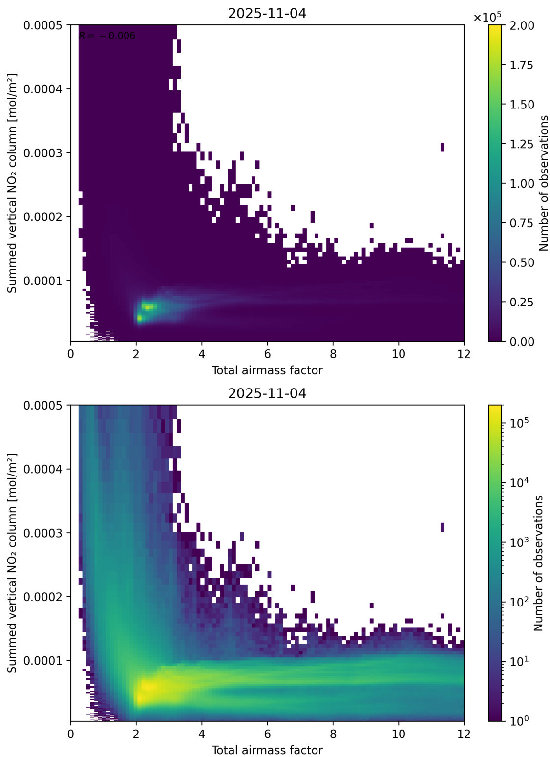
Figure 65: Scatter density plot of “Total airmass factor” against “Summed vertical NO 2 column” for 2025-11-03 to 2025-11-05.
