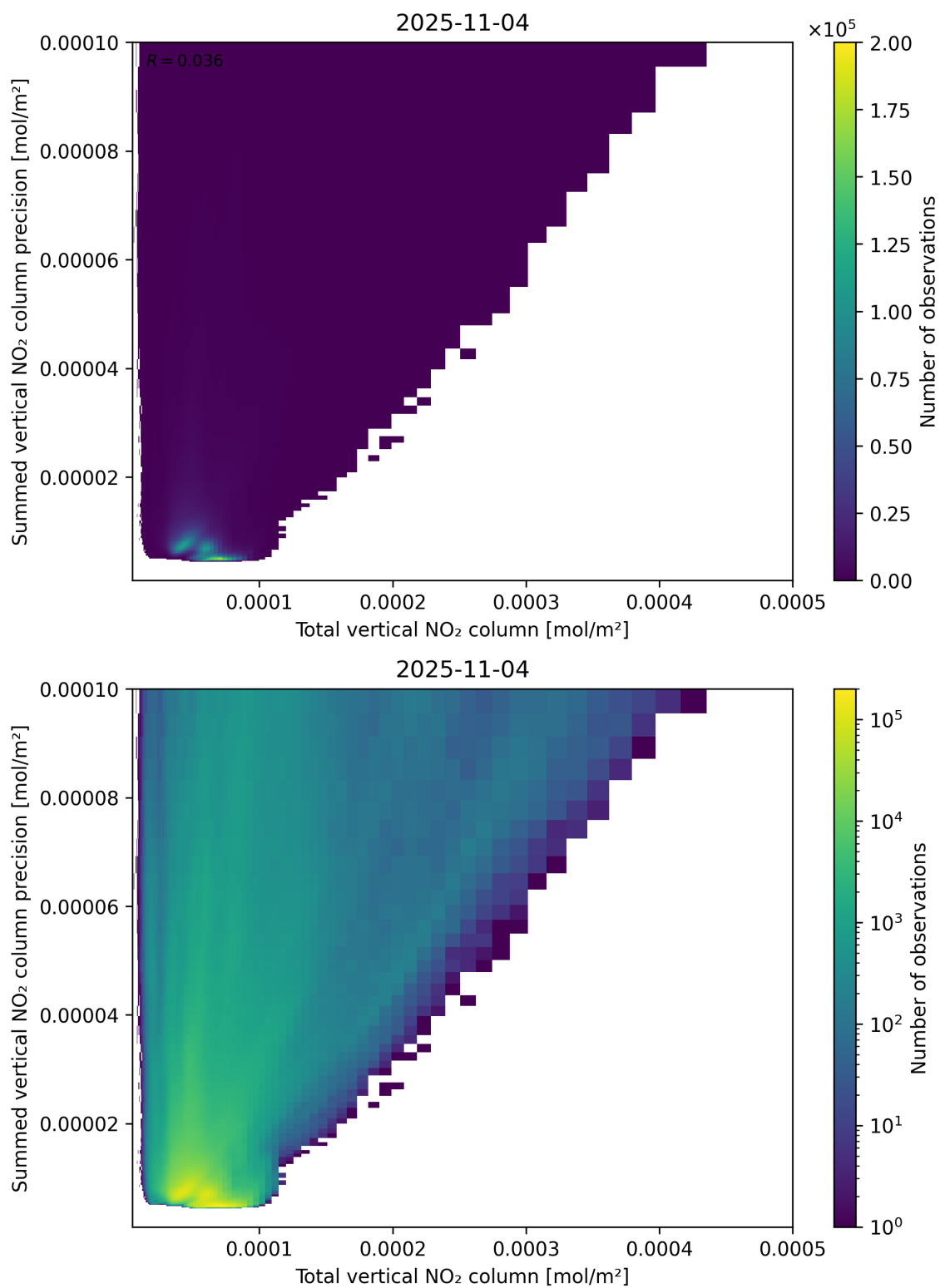
Figure 113: Scatter density plot of “Total vertical NO 2 column” against “Summed vertical NO 2 column precision” for 2025-11-03 to 2025-11-05.
