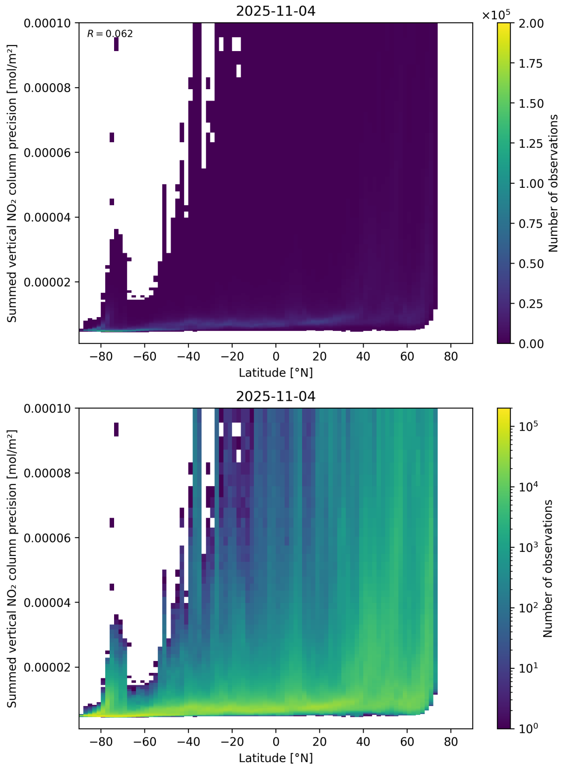
Figure 89: Scatter density plot of “Latitude” against “Summed vertical NO 2 column precision” for 2025-11-03 to 2025-11-05.
