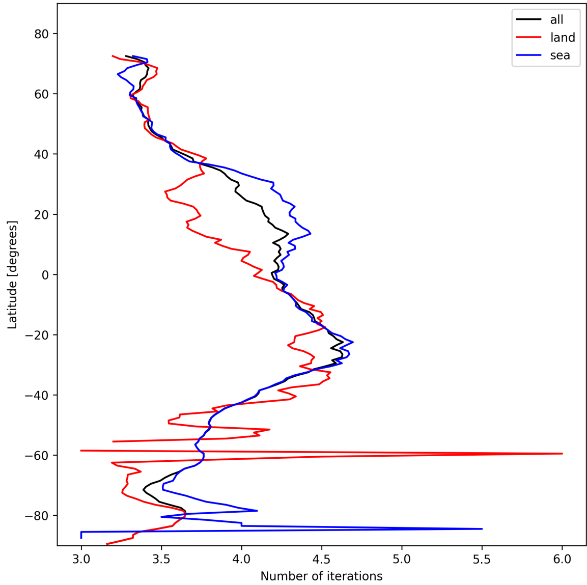
Figure 17: Zonal average of “Number of iterations” for 2025-11-03 to 2025-11-05.
