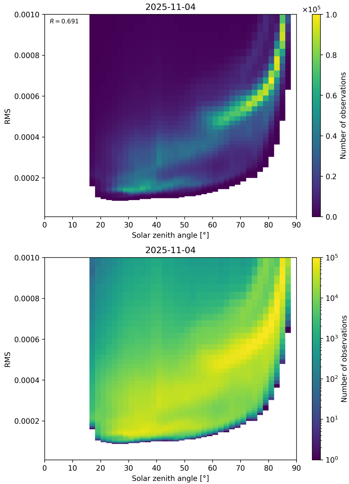
Figure 157: Scatter density plot of “Solar zenith angle” against “RMS” for 2025-11-03 to 2025-11-05.
