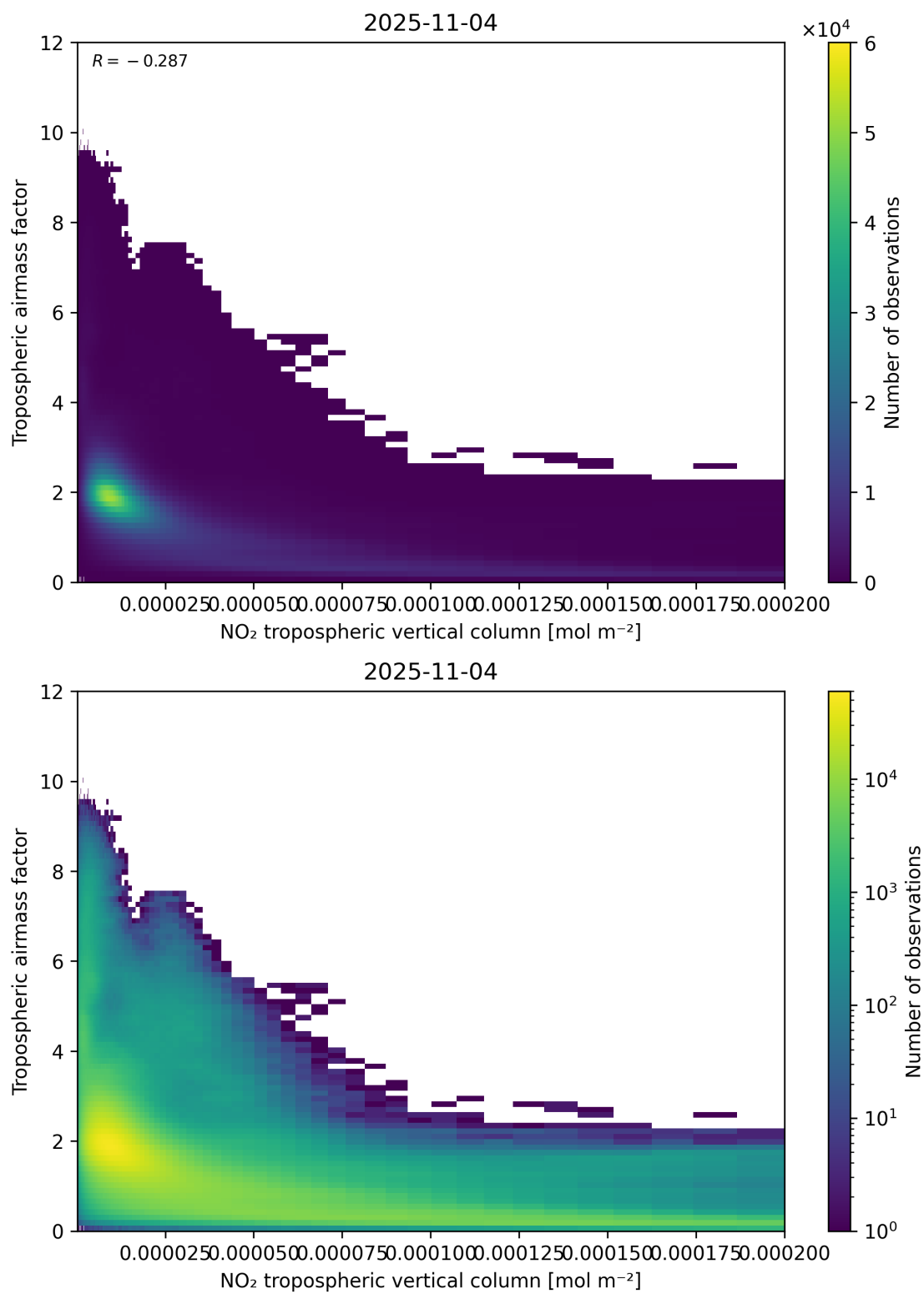
Figure 123: Scatter density plot of “NO 2 tropospheric vertical column” against “Tropospheric air mass factor” for 2025-11-03 to 2025-11-05.
