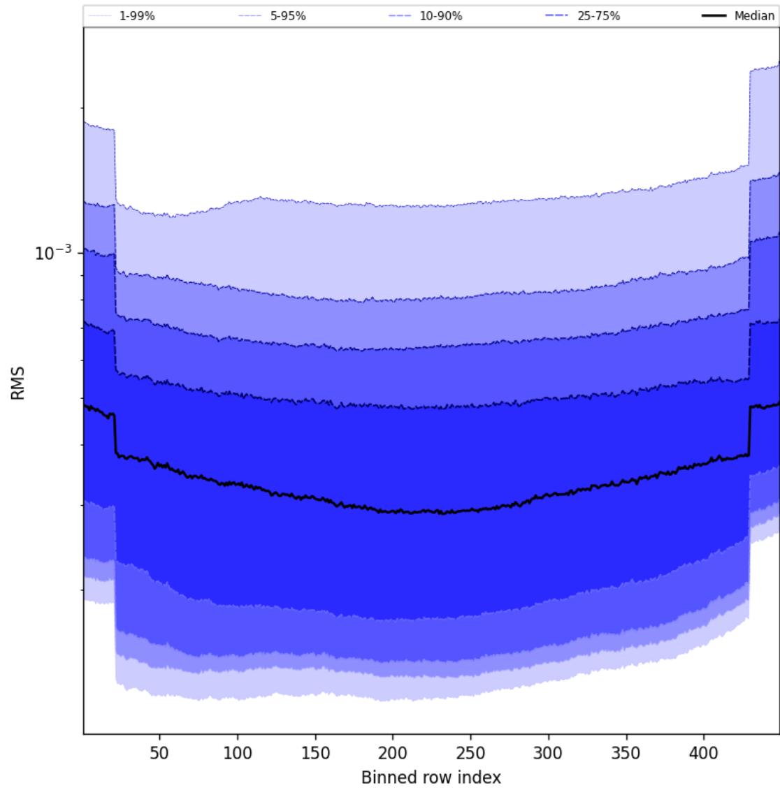
Figure 60: Along track statistics of “RMS” for 2025-11-03 to 2025-11-05
