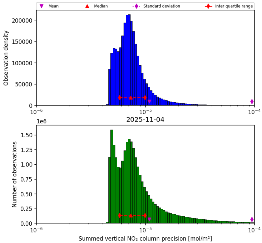
Figure 41: Histogram of "Summed vertical NO 2 column precision" for 2025-11-03 to 2025-11-05
