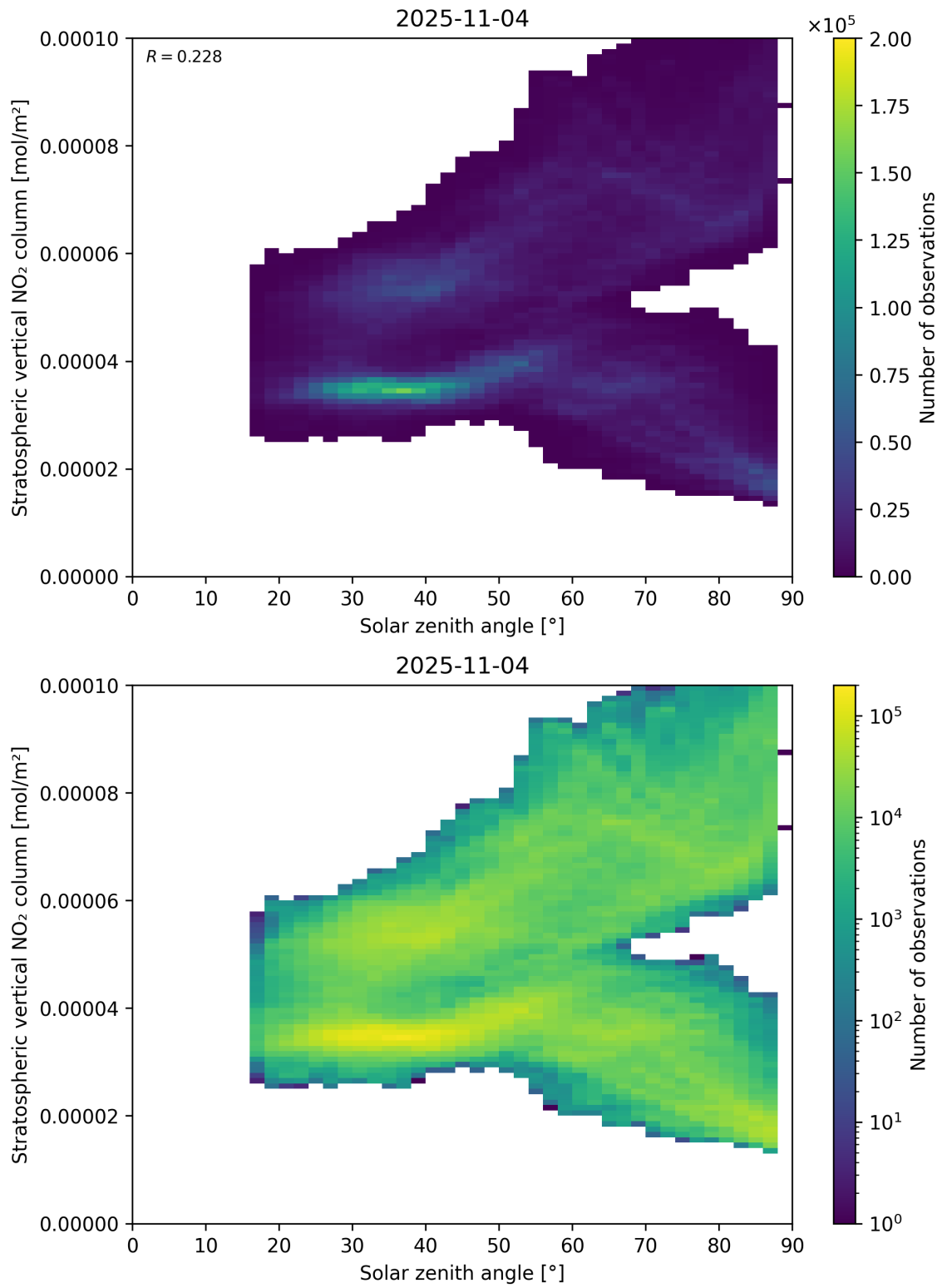
Figure 150: Scatter density plot of “Solar zenith angle” against “Stratospheric vertical NO 2 column” for 2025-11-03 to 2025-11-05.
