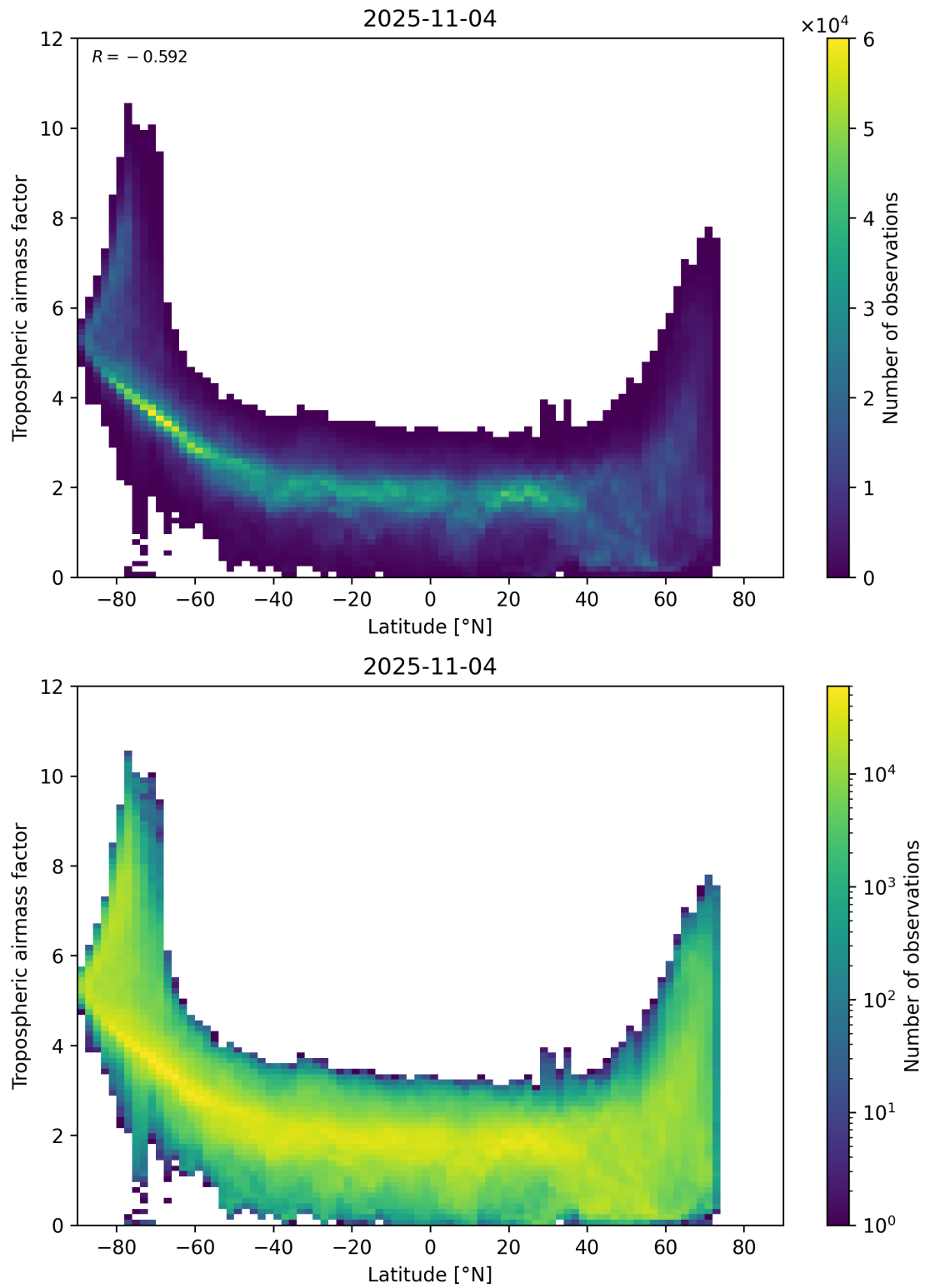
Figure 85: Scatter density plot of “Latitude” against “Tropospheric airmass factor” for 2025-11-03 to 2025-11-05.
