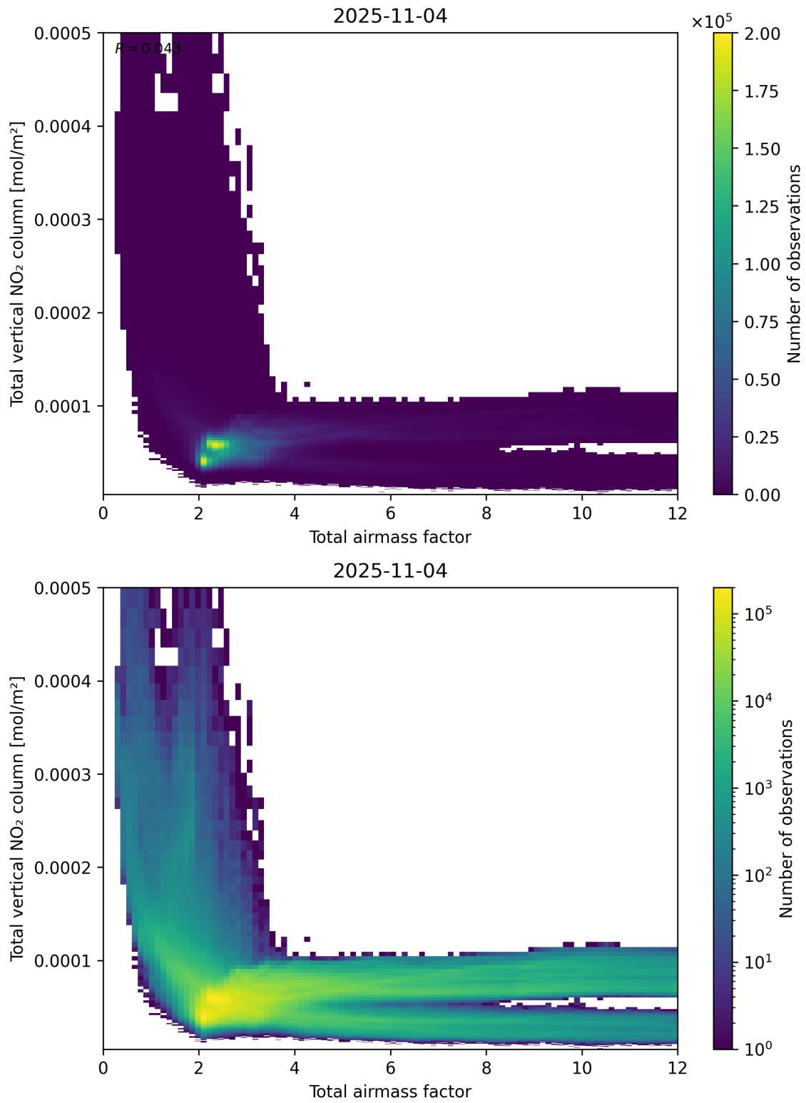
Figure 67: Scatter density plot of “Total airmass factor” against “Total vertical NO 2 column” for 2025-11-03 to 2025-11-05.
