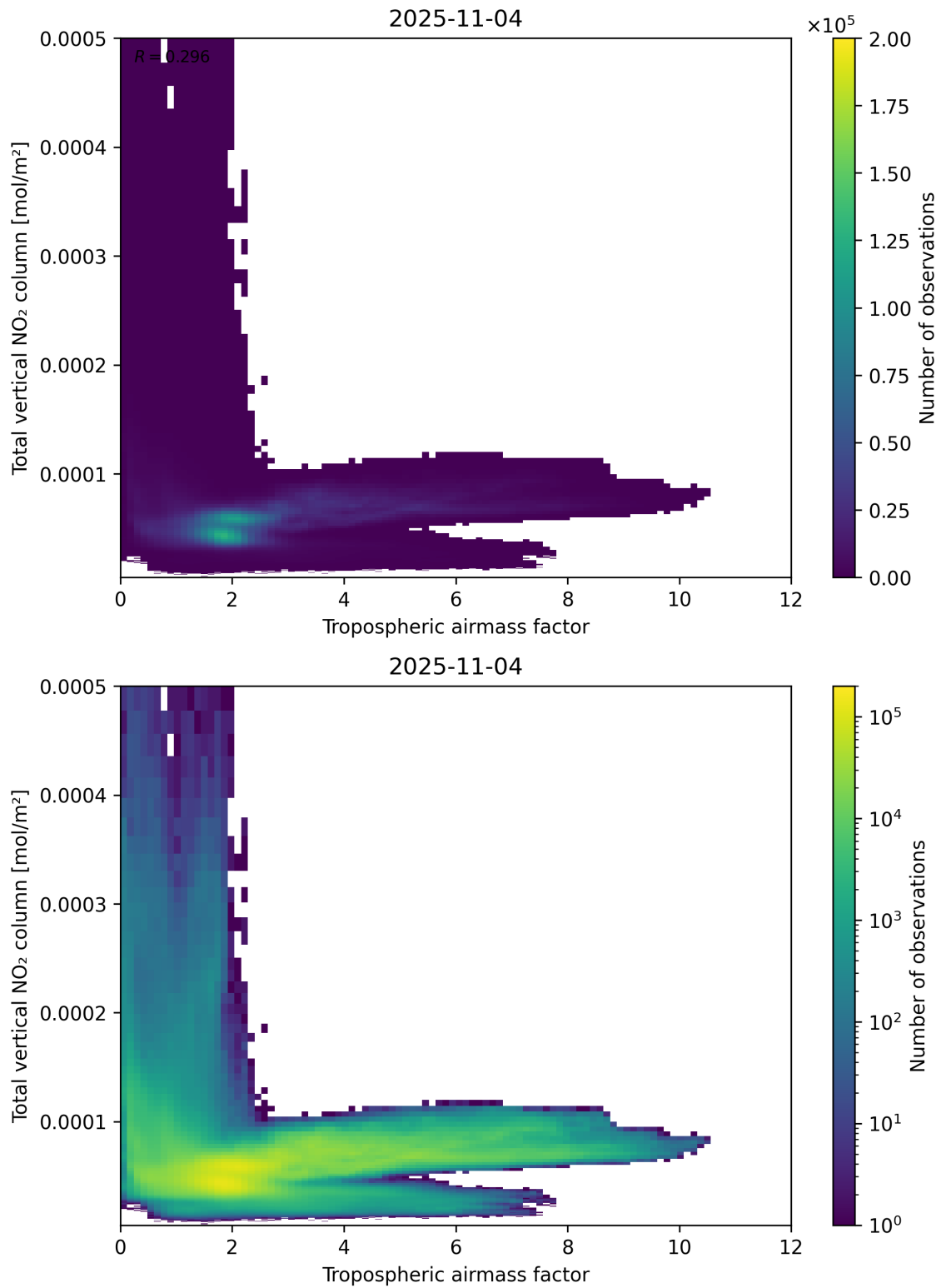
Figure 77: Scatter density plot of “Tropospheric airmass factor” against “Total vertical NO 2 column” for 2025-11-03 to 2025-11-05.
