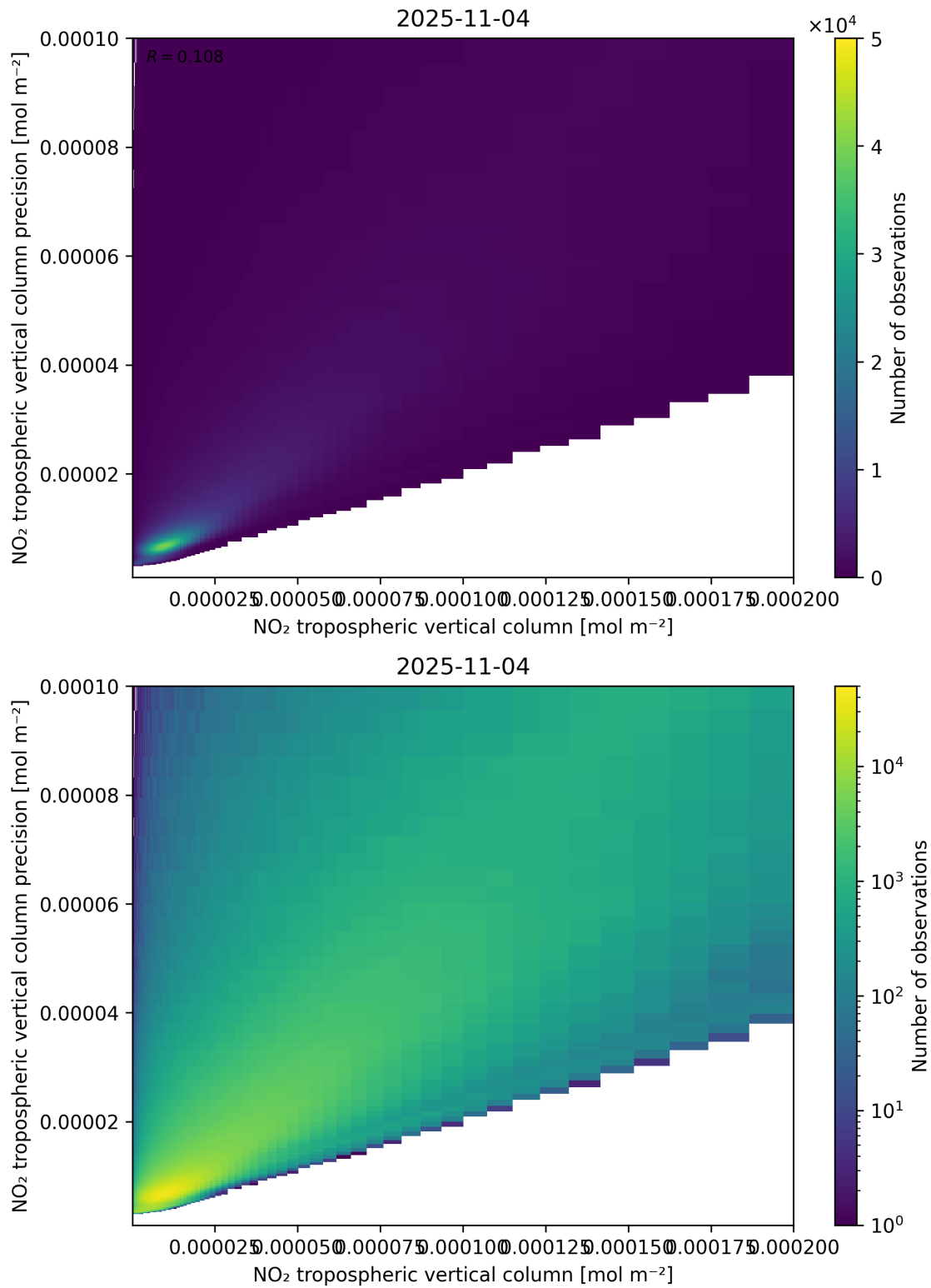
Figure 130: Scatter density plot of “NO 2 tropospheric vertical column” against “NO 2 tropospheric vertical column precision” for 2025-11-03 to 2025-11-05.
