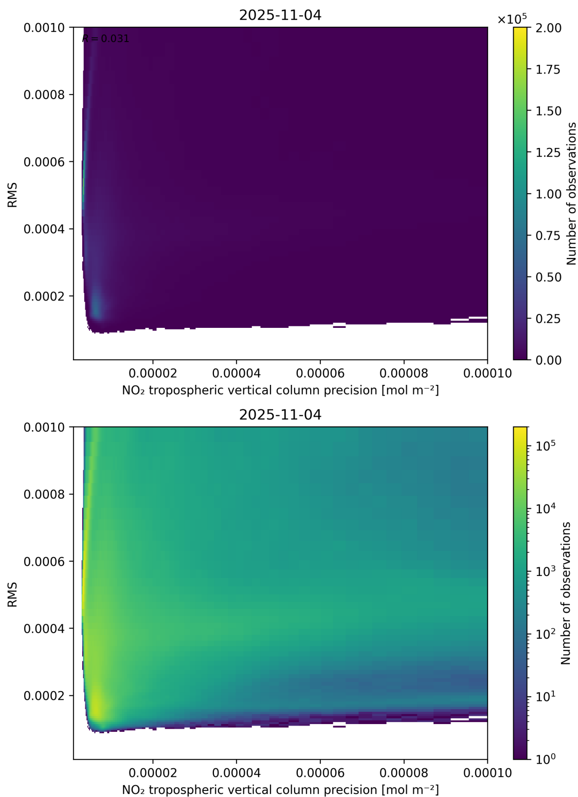
Figure 140: Scatter density plot of “NO 2 tropospheric vertical column precision” against “RMS” for 2025-11-03 to 2025-11-05.
