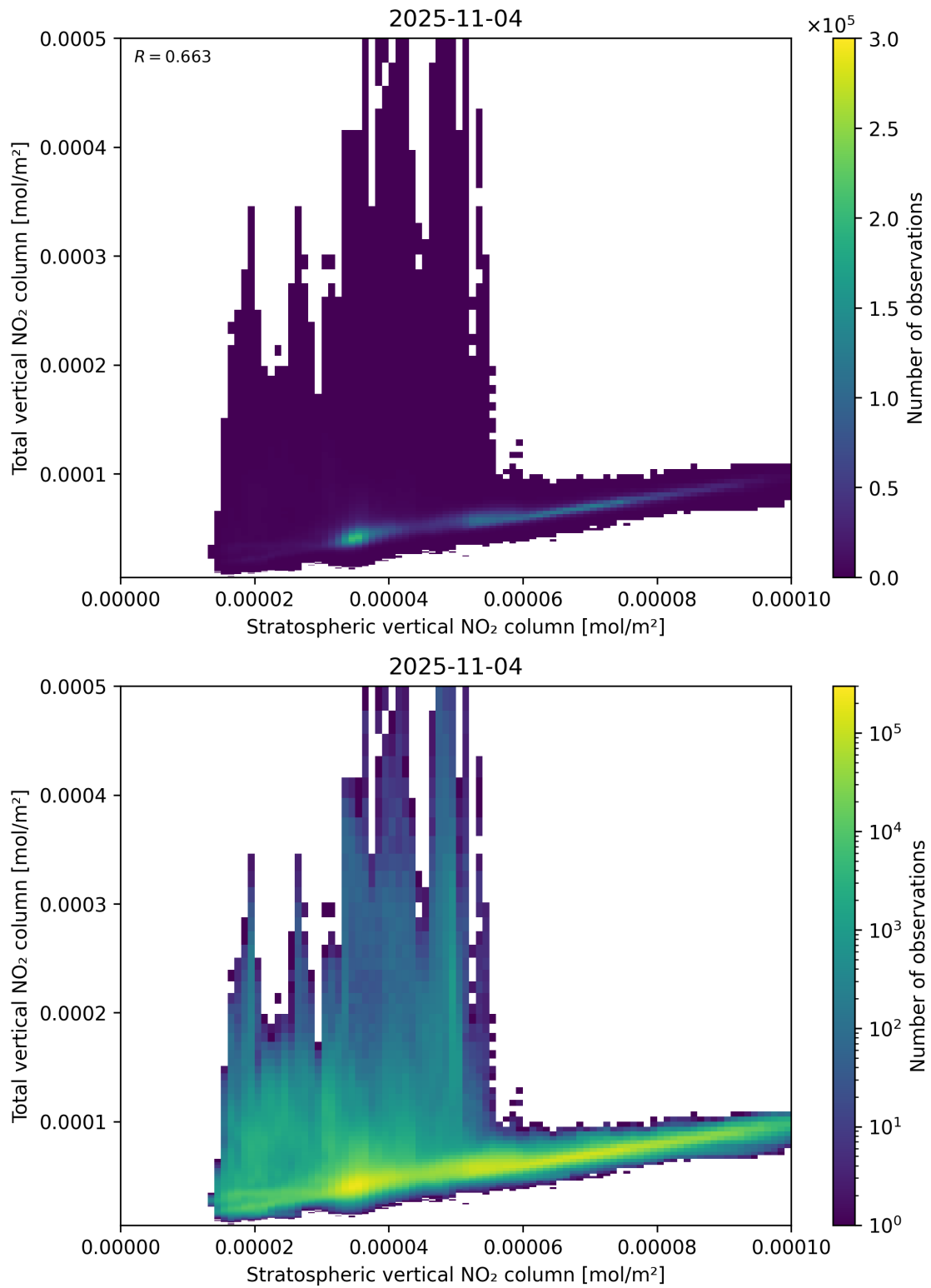
Figure 100: Scatter density plot of “Stratospheric vertical NO 2 column” against “Total vertical NO 2 column” for 2025-11-03 to 2025-11-05.
