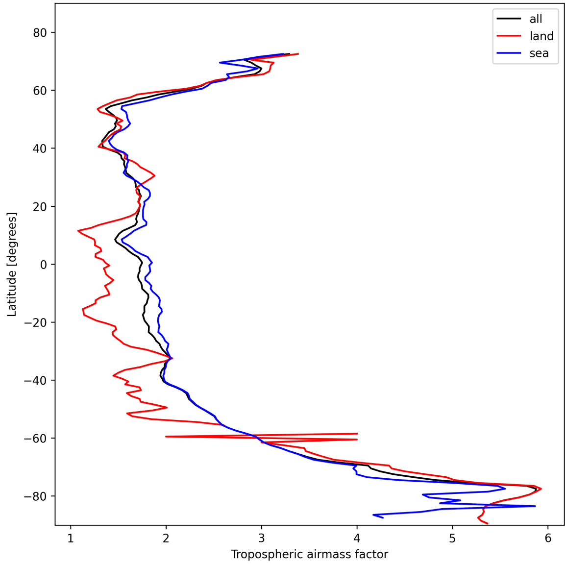
Figure 14: Zonal average of “Tropospheric airmass factor” for 2025-11-03 to 2025-11-05.
