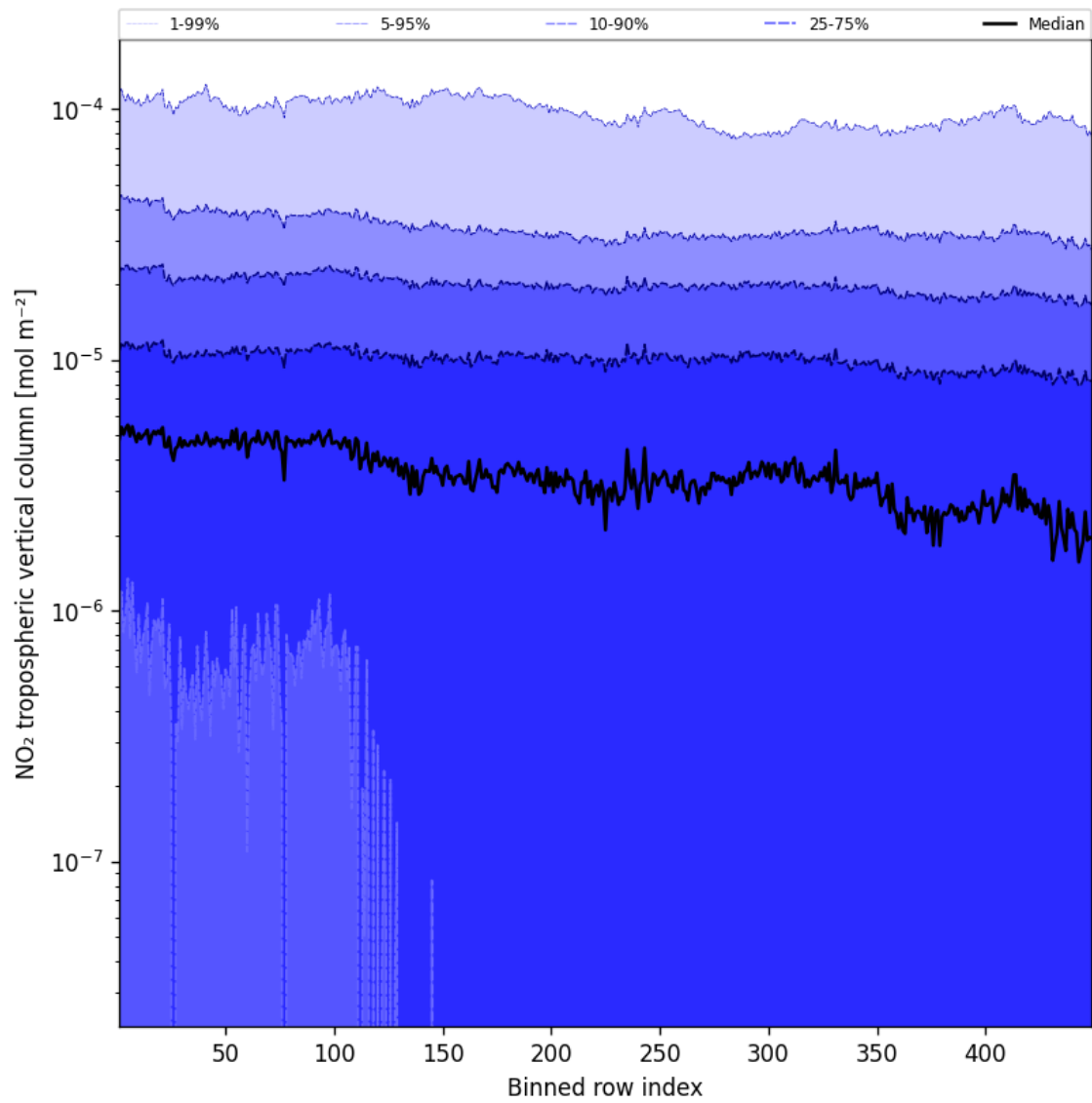
Figure 46: Along track statistics of "NO 2 tropospheric vertical column" for 2025-11-03 to 2025-11-05
