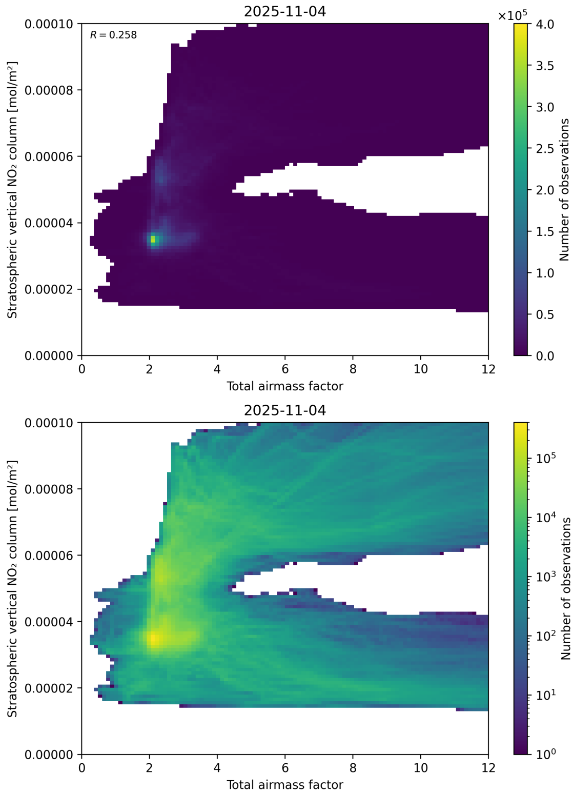
Figure 64: Scatter density plot of “Total airmass factor” against “Stratospheric vertical NO 2 column” for 2025-11-03 to 2025-11-05.
