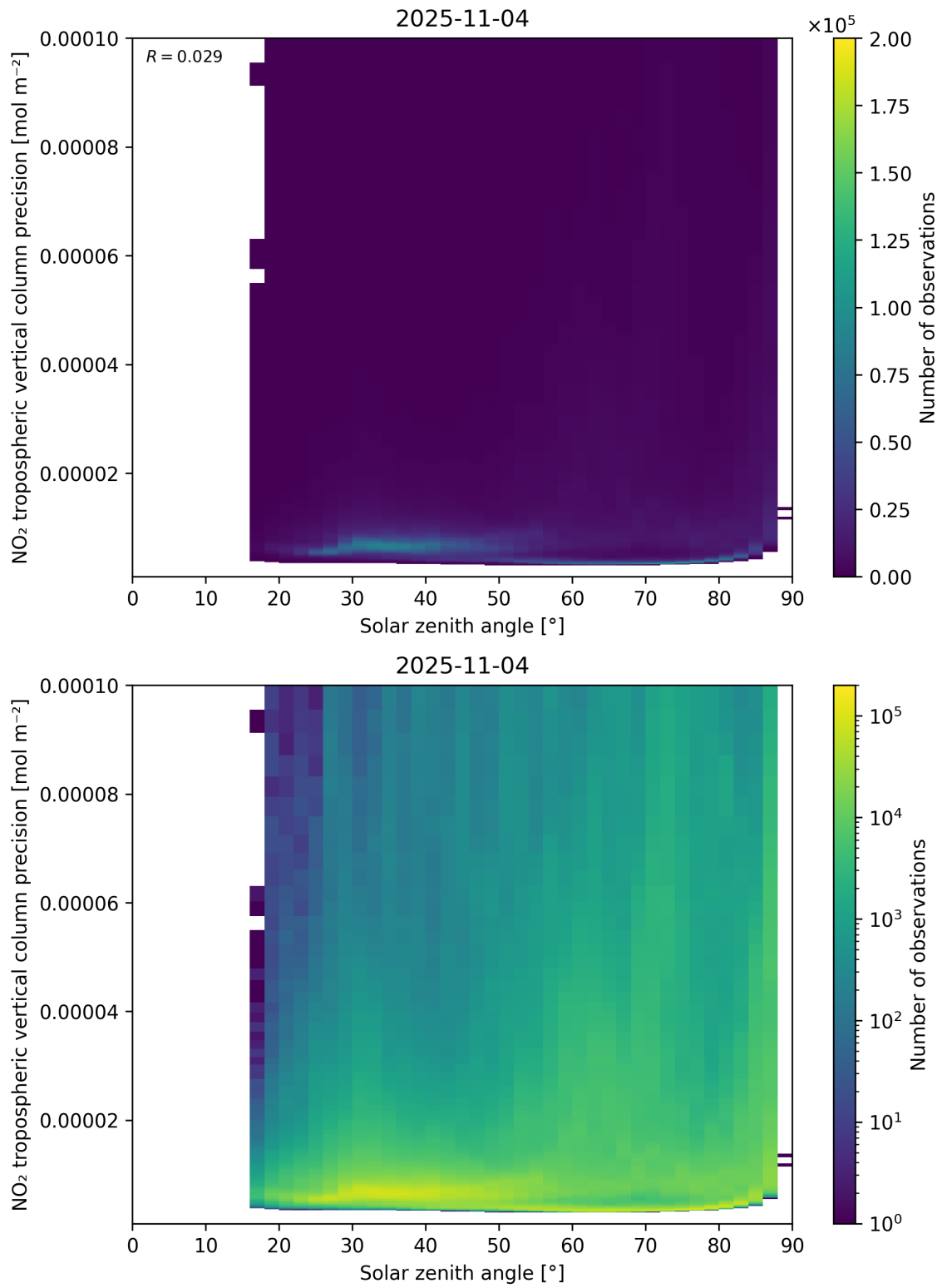
Figure 156: Scatter density plot of “Solar zenith angle” against “NO 2 tropospheric vertical column precision” for 2025-11-03 to 2025-11-05.
