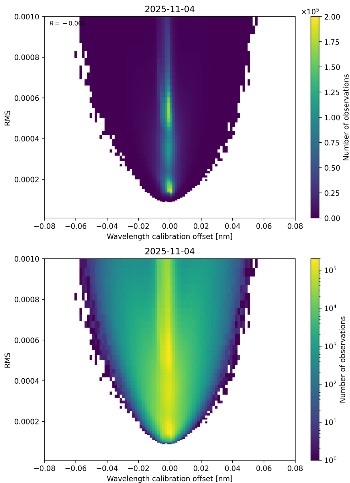
Figure 181: Scatter density plot of “Wavelength calibration offset” against “RMS” for 2025-11-03 to 2025-11-05.
