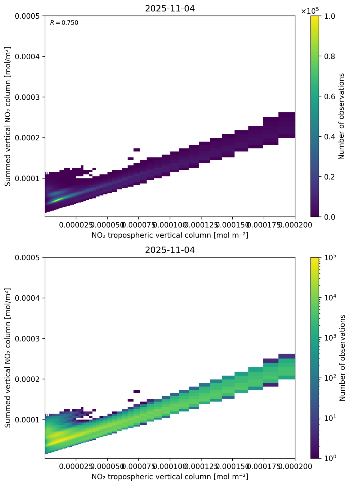
Figure 126: Scatter density plot of “NO 2 tropospheric vertical column” against “Summed vertical NO 2 column” for 2025-11-03 to 2025-11-05.
