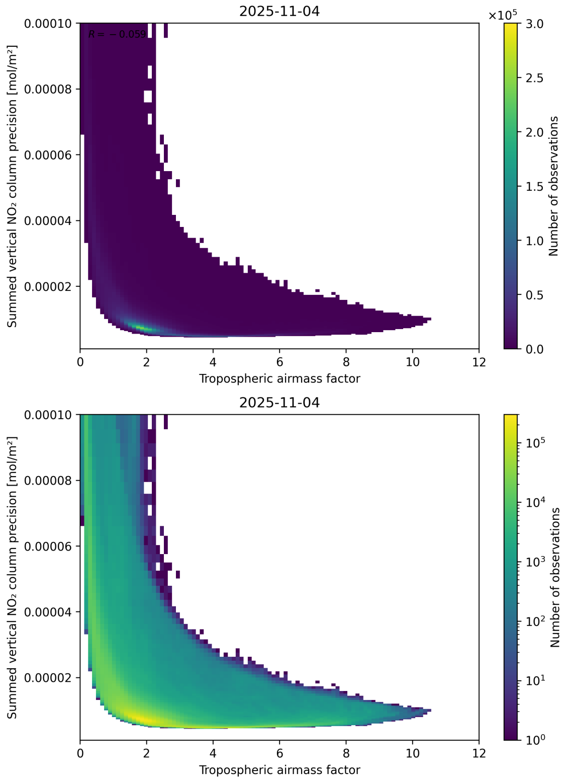
Figure 76: Scatter density plot of “Tropospheric air mass factor” against “Summed vertical NO 2 column precision” for 2025-11-03 to 2025-11-05.
