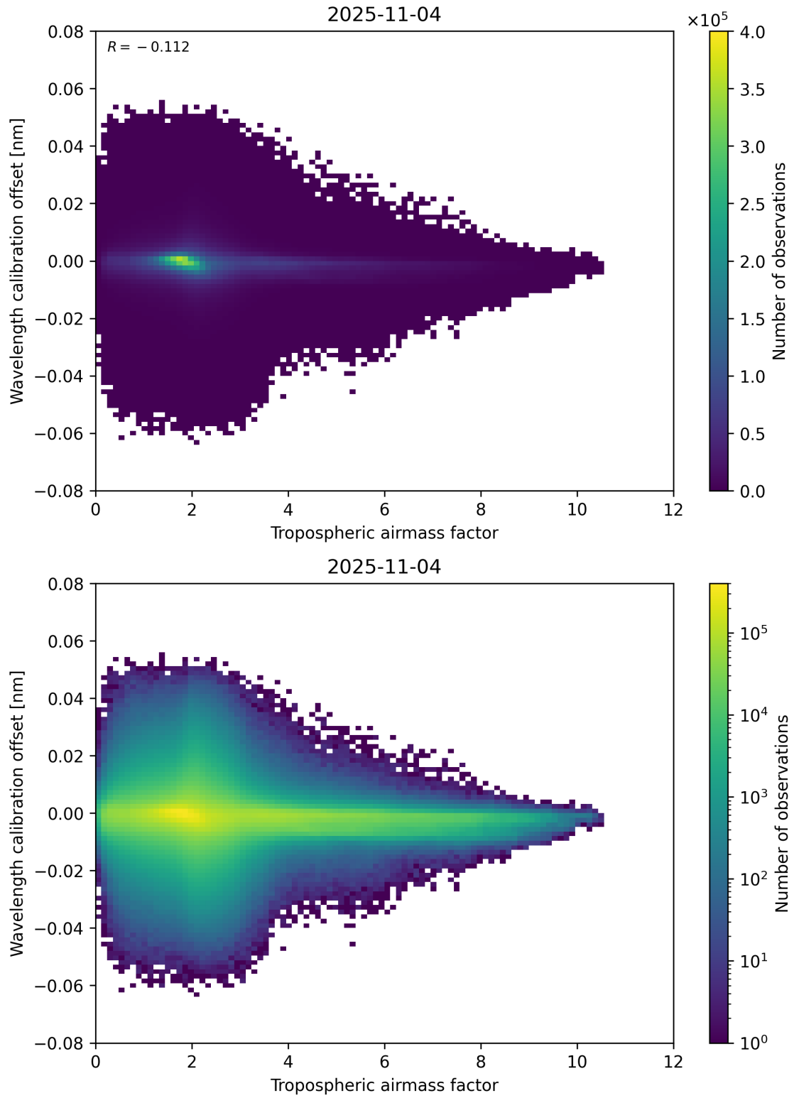
Figure 80: Scatter density plot of “Tropospheric airmass factor” against “Wavelength calibration offset” for 2025-11-03 to 2025-11-05.
