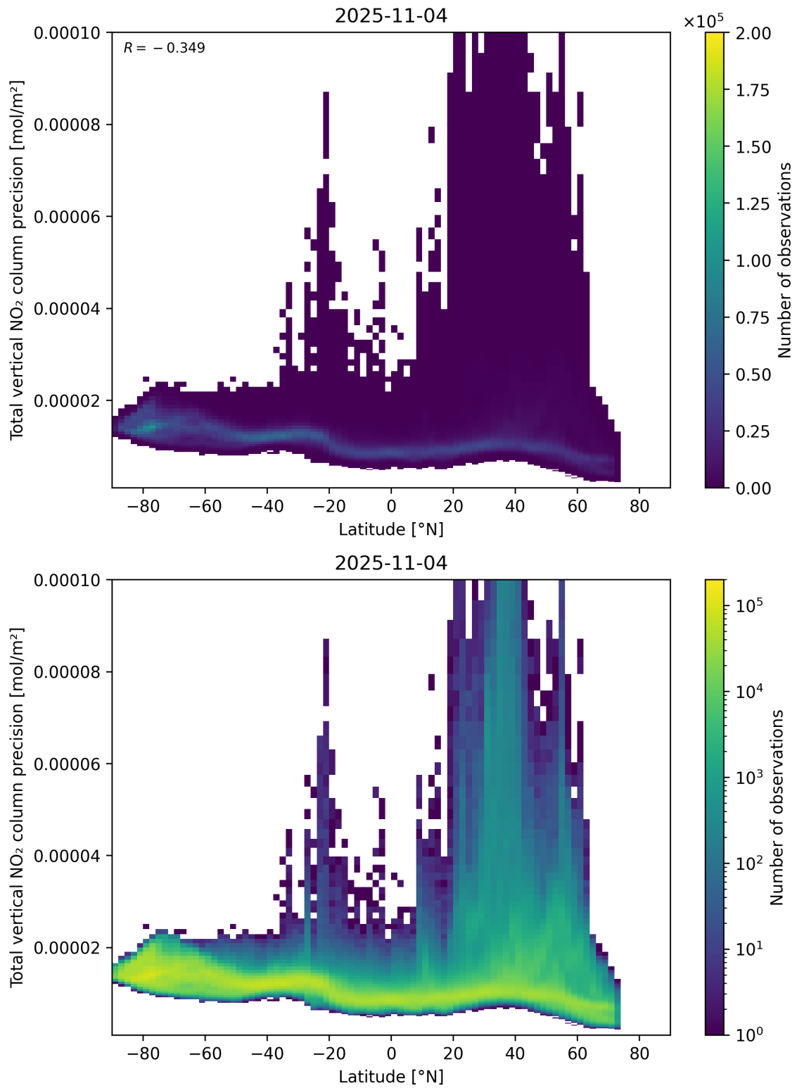
Figure 91: Scatter density plot of “Latitude” against “Total vertical NO 2 column precision” for 2025-11-03 to 2025-11-05.
