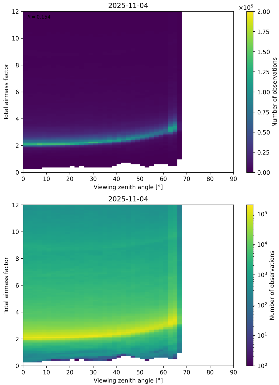
Figure 160: Scatter density plot of “Viewing zenith angle” against “Total airmass factor” for 2025-11-03 to 2025-11-05.
