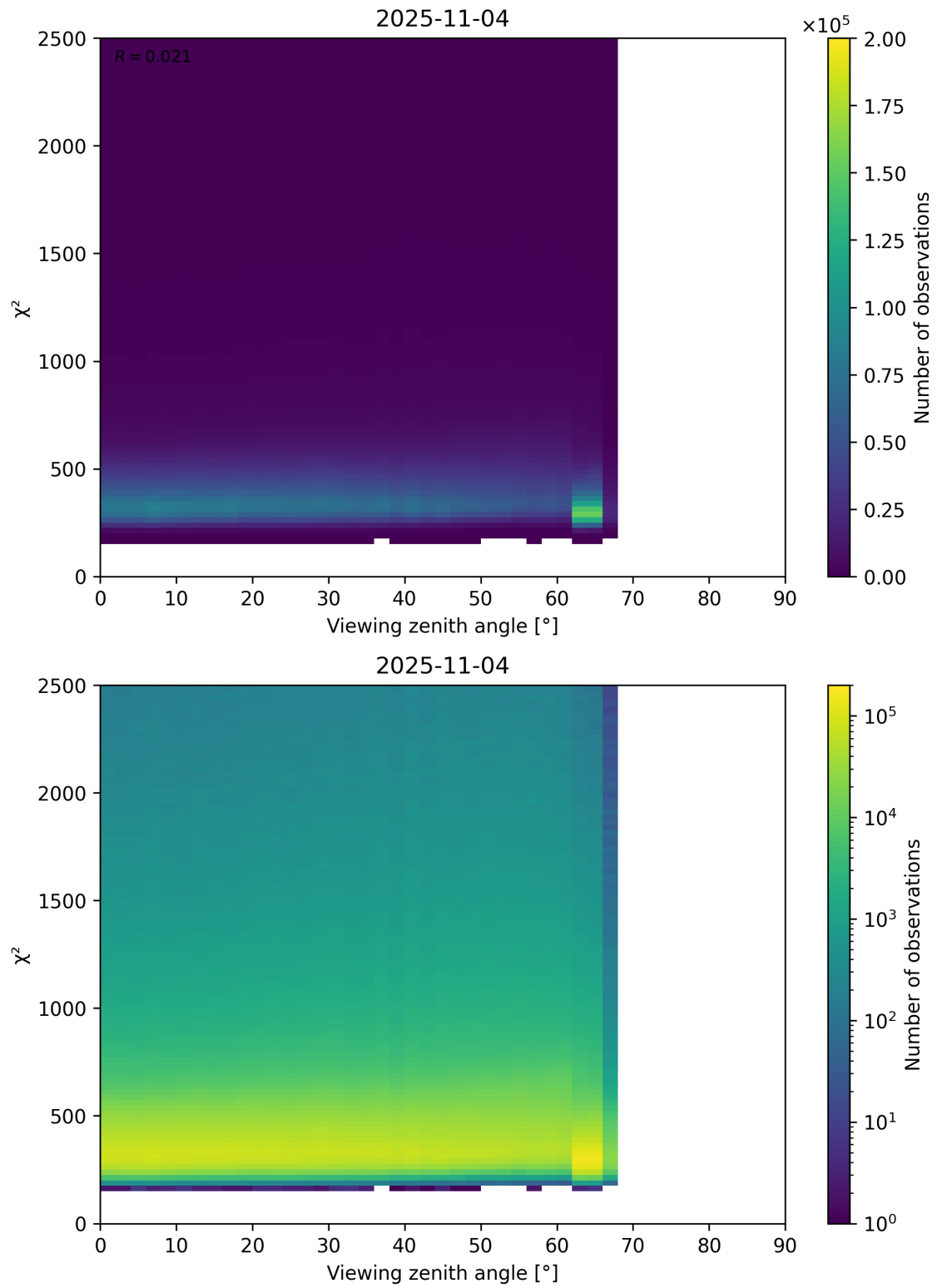
Figure 162: Scatter density plot of “Viewing zenith angle” against “ \chi^2 ” for 2025-11-03 to 2025-11-05.
