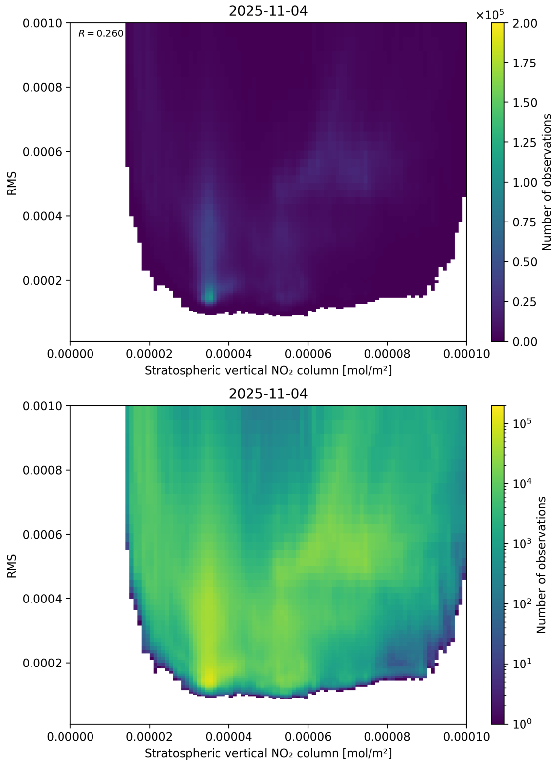
Figure 102: Scatter density plot of “Stratospheric vertical NO 2 column” against “RMS” for 2025-11-03 to 2025-11-05.
