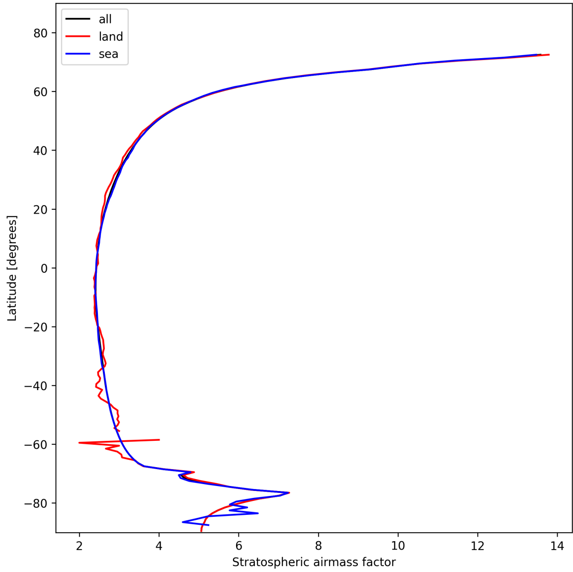
Figure 27: Zonal average of “Stratospheric air mass factor” for 2025-11-03 to 2025-11-05.
