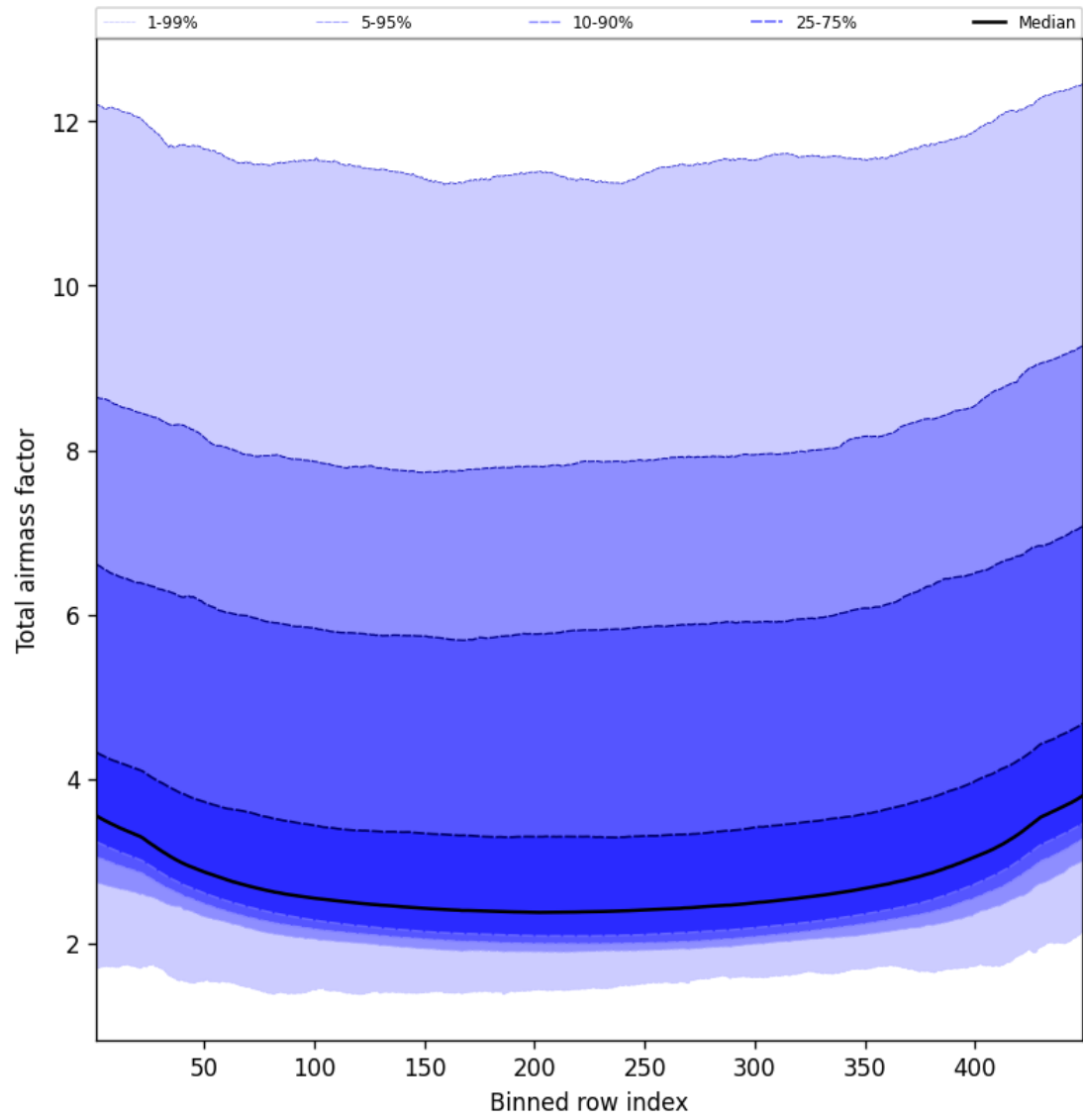
Figure 49: Along track statistics of “Total airmass factor” for 2025-11-03 to 2025-11-05
