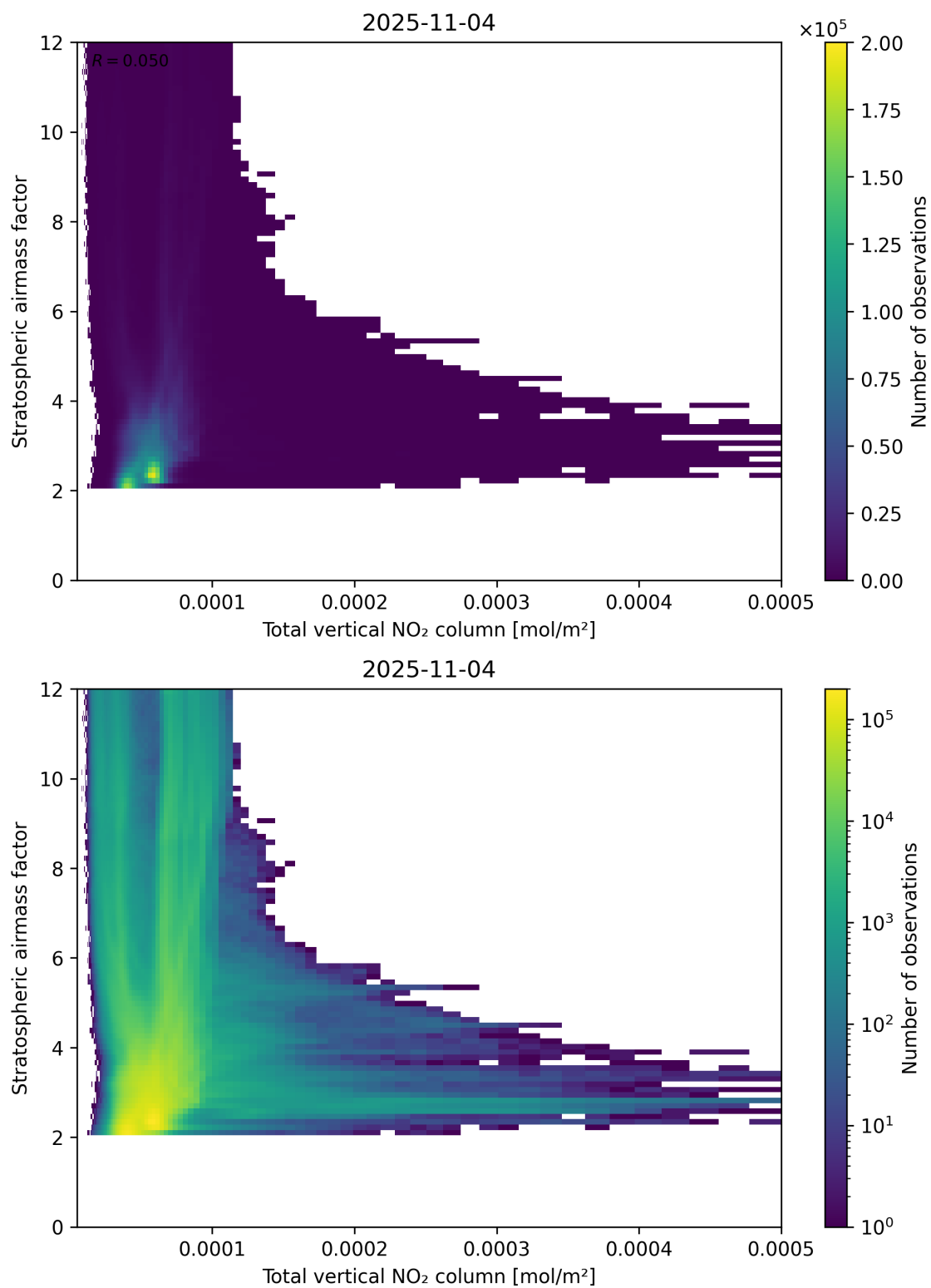
Figure 110: Scatter density plot of “Total vertical NO 2 column” against “Stratospheric air mass factor” for 2025-11-03 to 2025-11-05.
