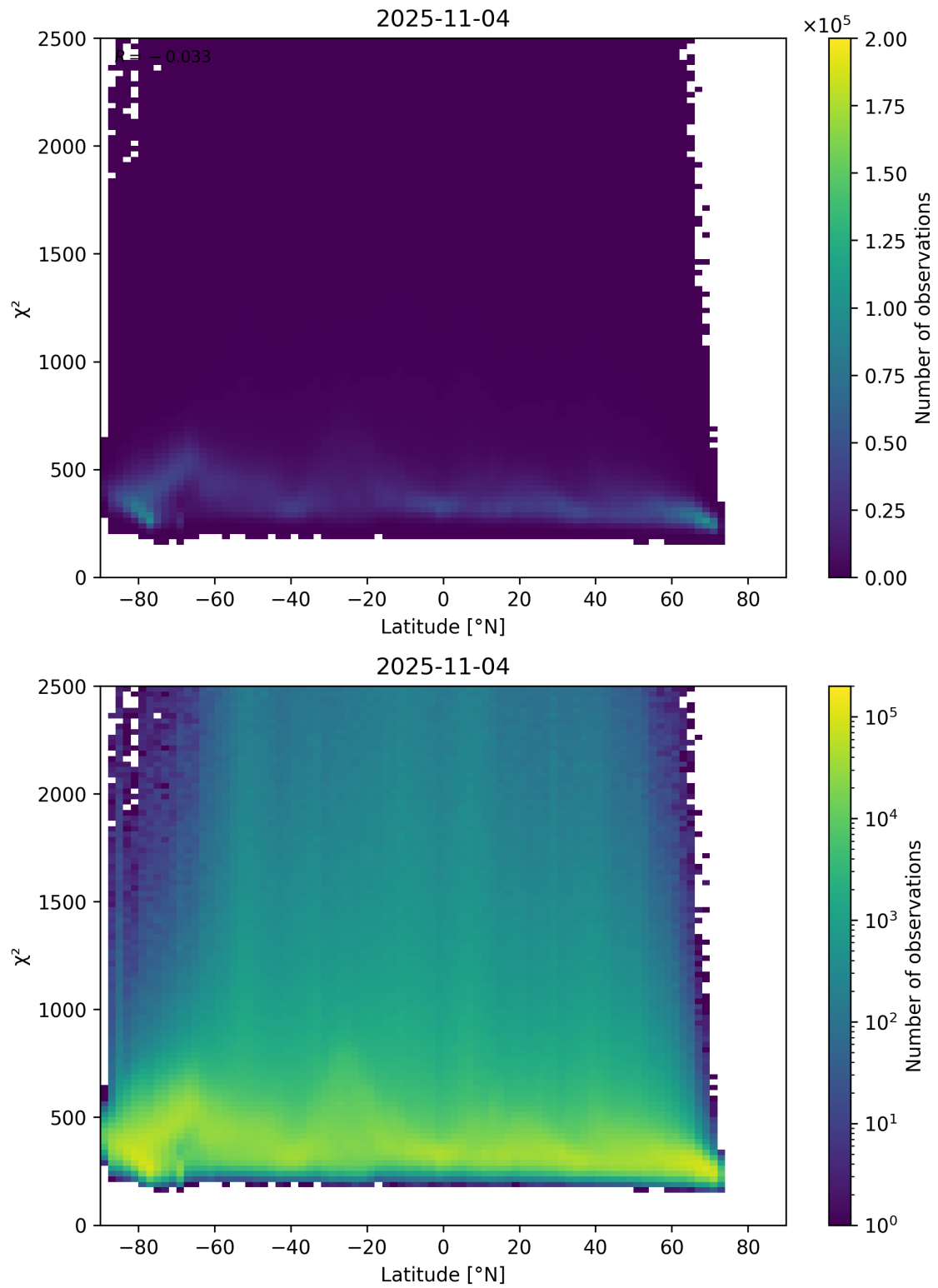
Figure 86: Scatter density plot of “Latitude” against “ \chi^2 ” for 2025-11-03 to 2025-11-05.
