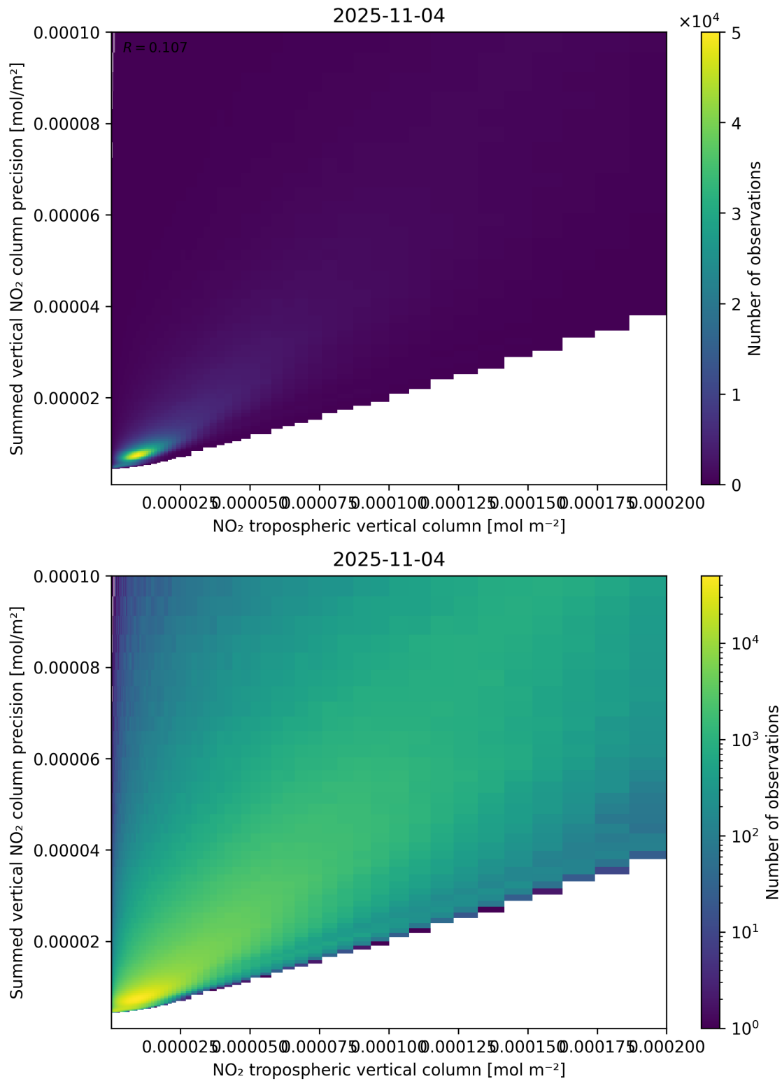
Figure 127: Scatter density plot of “NO 2 tropospheric vertical column” against “Summed vertical NO 2 column precision” for 2025-11-03 to 2025-11-05.
