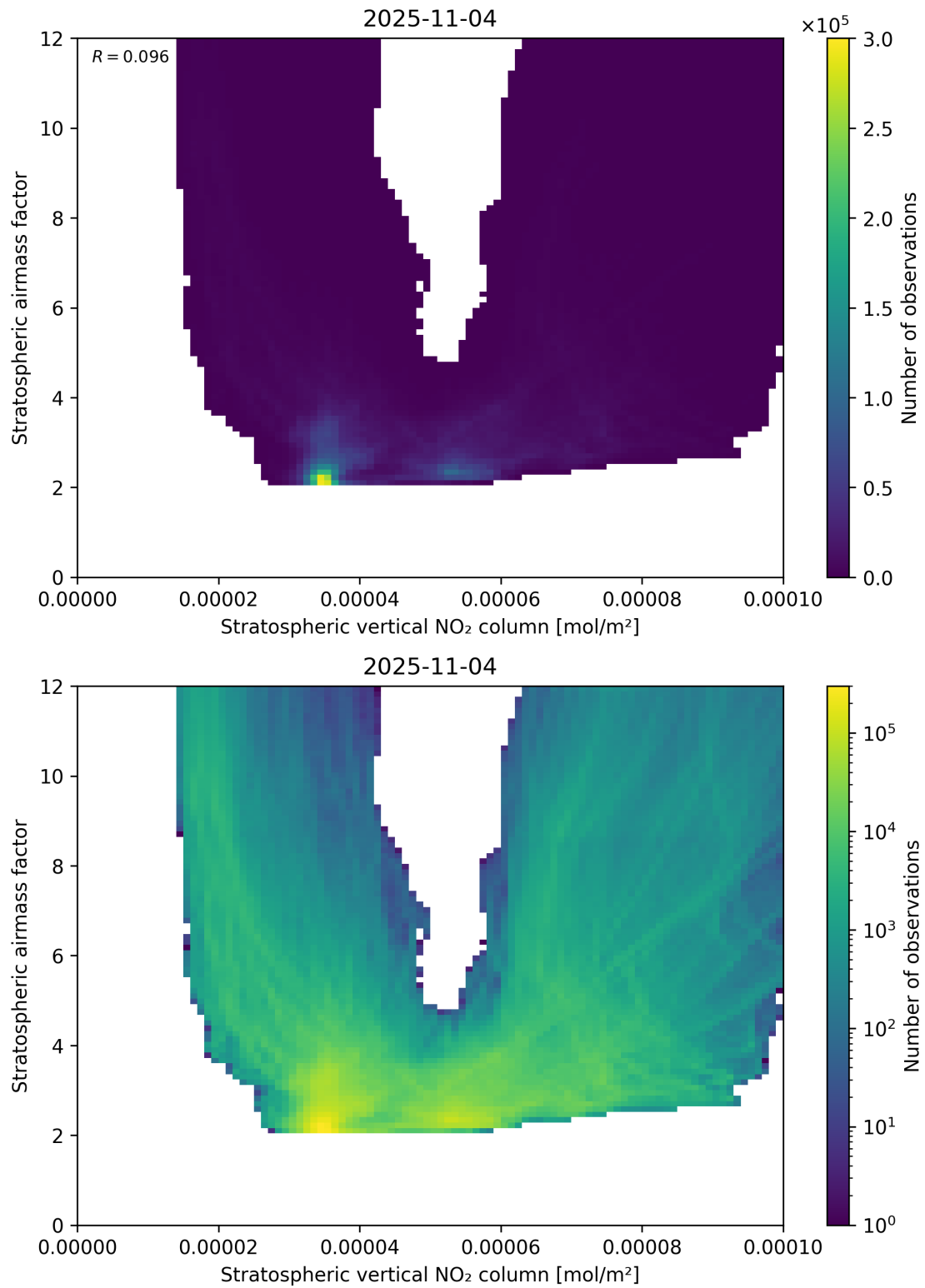
Figure 96: Scatter density plot of “Stratospheric vertical NO 2 column” against “Stratospheric airmass factor” for 2025-11-03 to 2025-11-05.
