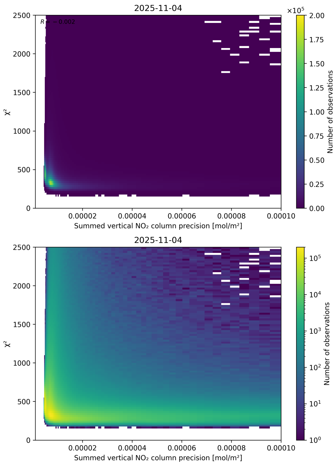
Figure 107: Scatter density plot of “Summed vertical NO 2 column precision” against “ \chi^2 ” for 2025-11-03 to 2025-11-05.
