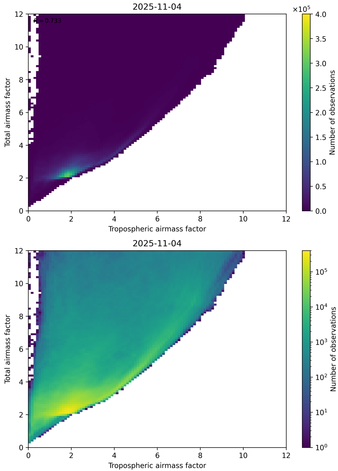
Figure 72: Scatter density plot of “Tropospheric airmass factor” against “Total airmass factor” for 2025-11-03 to 2025-11-05.
