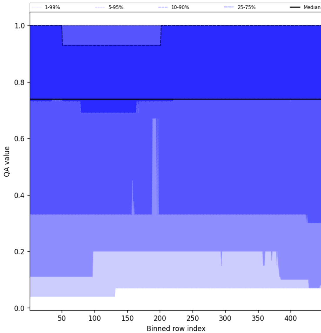
Figure 45: Along track statistics of “QA value” for 2025-11-03 to 2025-11-05
