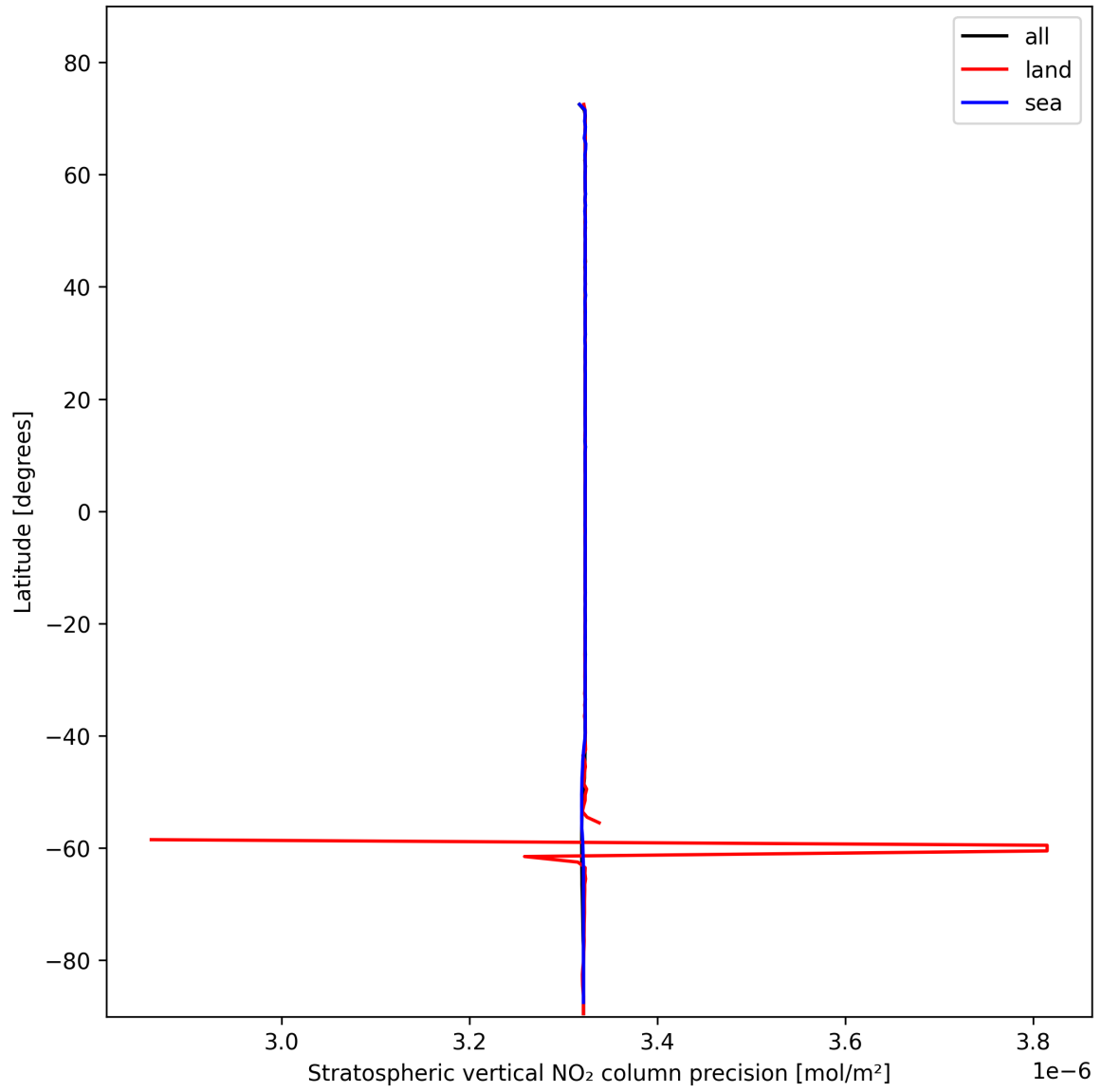
Figure 20: Zonal average of “Stratospheric vertical NO 2 column precision” for 2025-11-03 to 2025-11-05.
