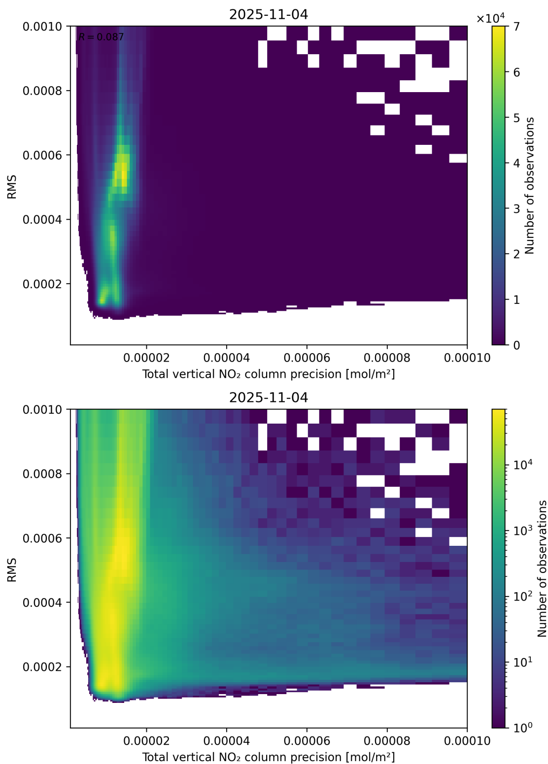
Figure 119: Scatter density plot of “Total vertical NO 2 column precision” against “RMS” for 2025-11-03 to 2025-11-05.
