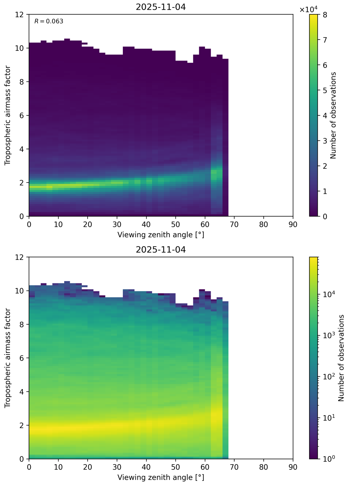
Figure 161: Scatter density plot of “Viewing zenith angle” against “Tropospheric airmass factor” for 2025-11-03 to 2025-11-05.
