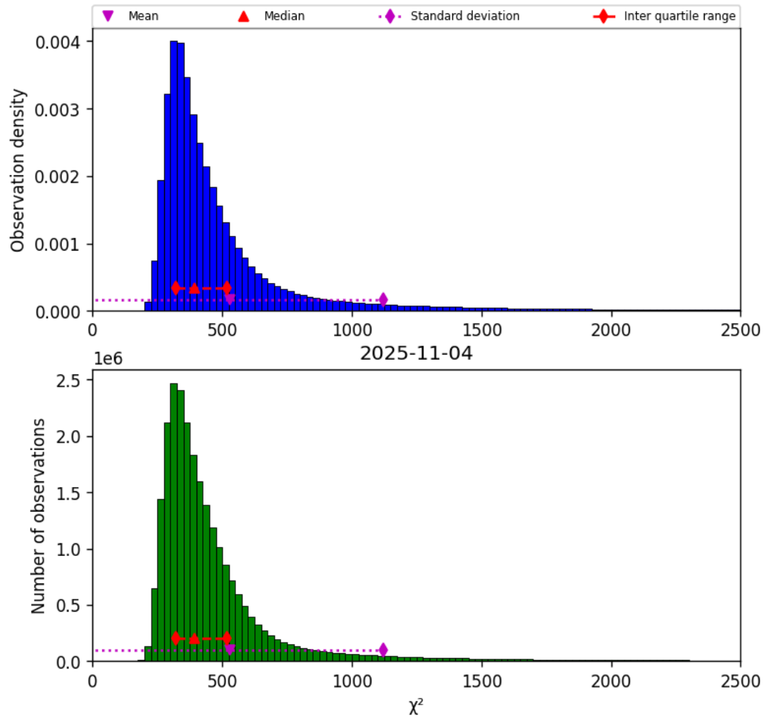
Figure 42: Histogram of " \chi^2 " for 2025-11-03 to 2025-11-05
