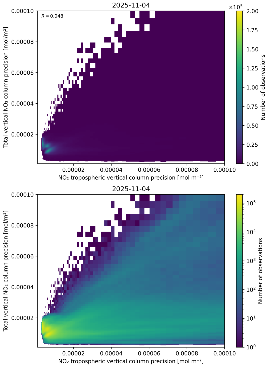
Figure 139: Scatter density plot of “NO 2 tropospheric vertical column precision” against “Total vertical NO 2 column precision” for 2025-11-03 to 2025-11-05.
