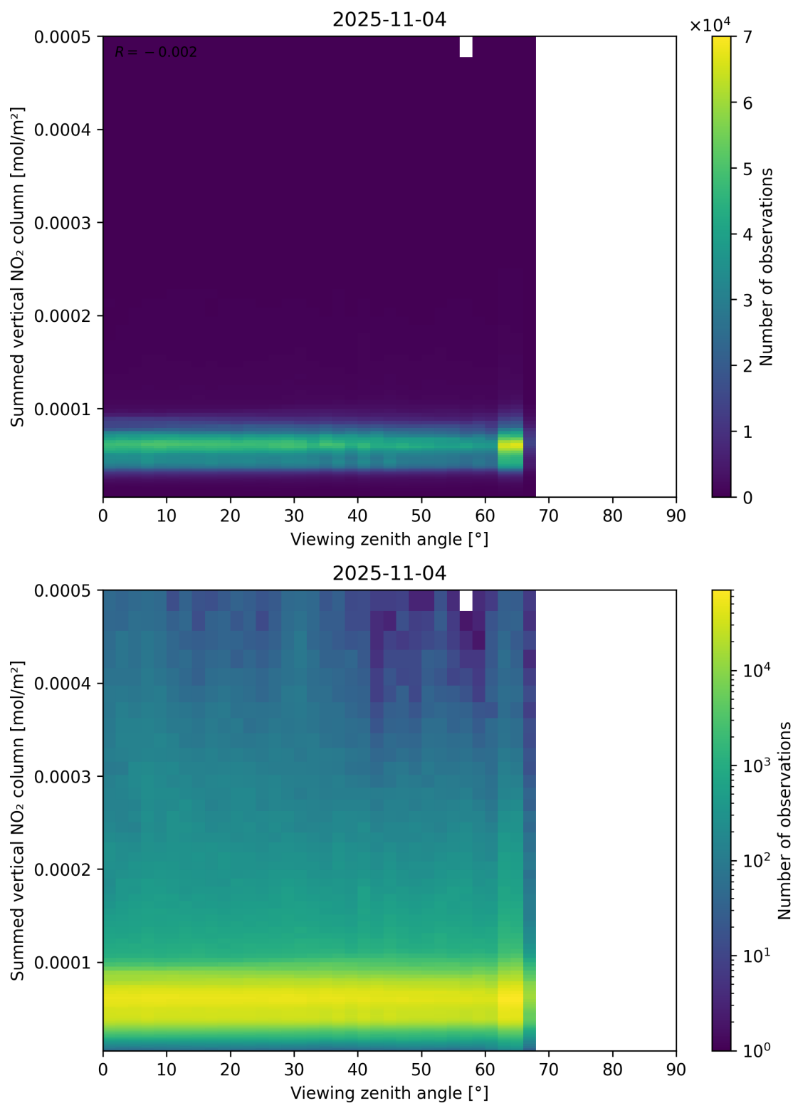
Figure 165: Scatter density plot of “Viewing zenith angle” against “Summed vertical NO 2 column” for 2025-11-03 to 2025-11-05.
