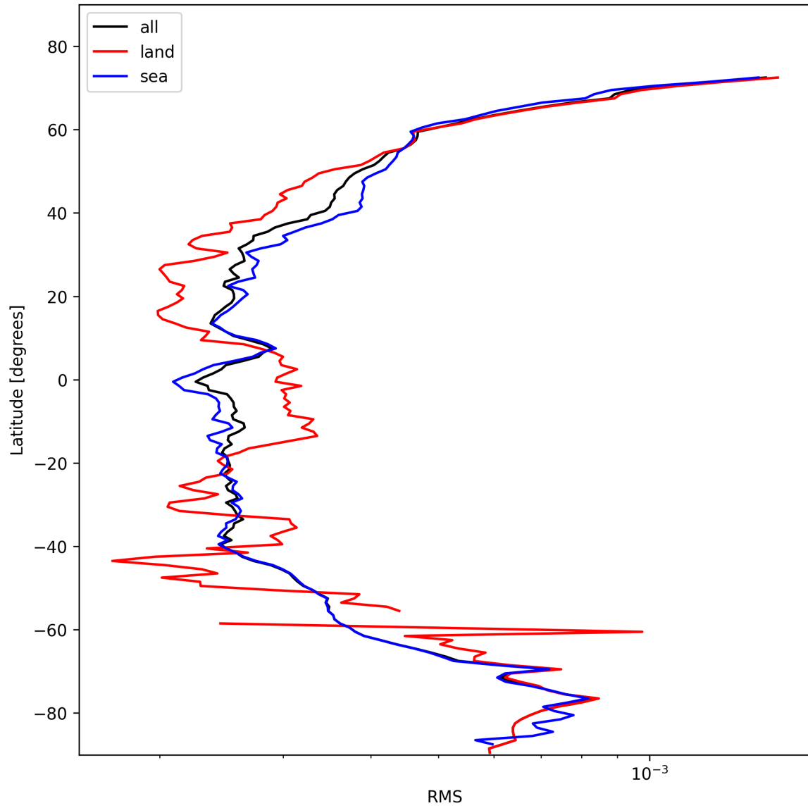
Figure 26: Zonal average of “RMS” for 2025-11-03 to 2025-11-05.
