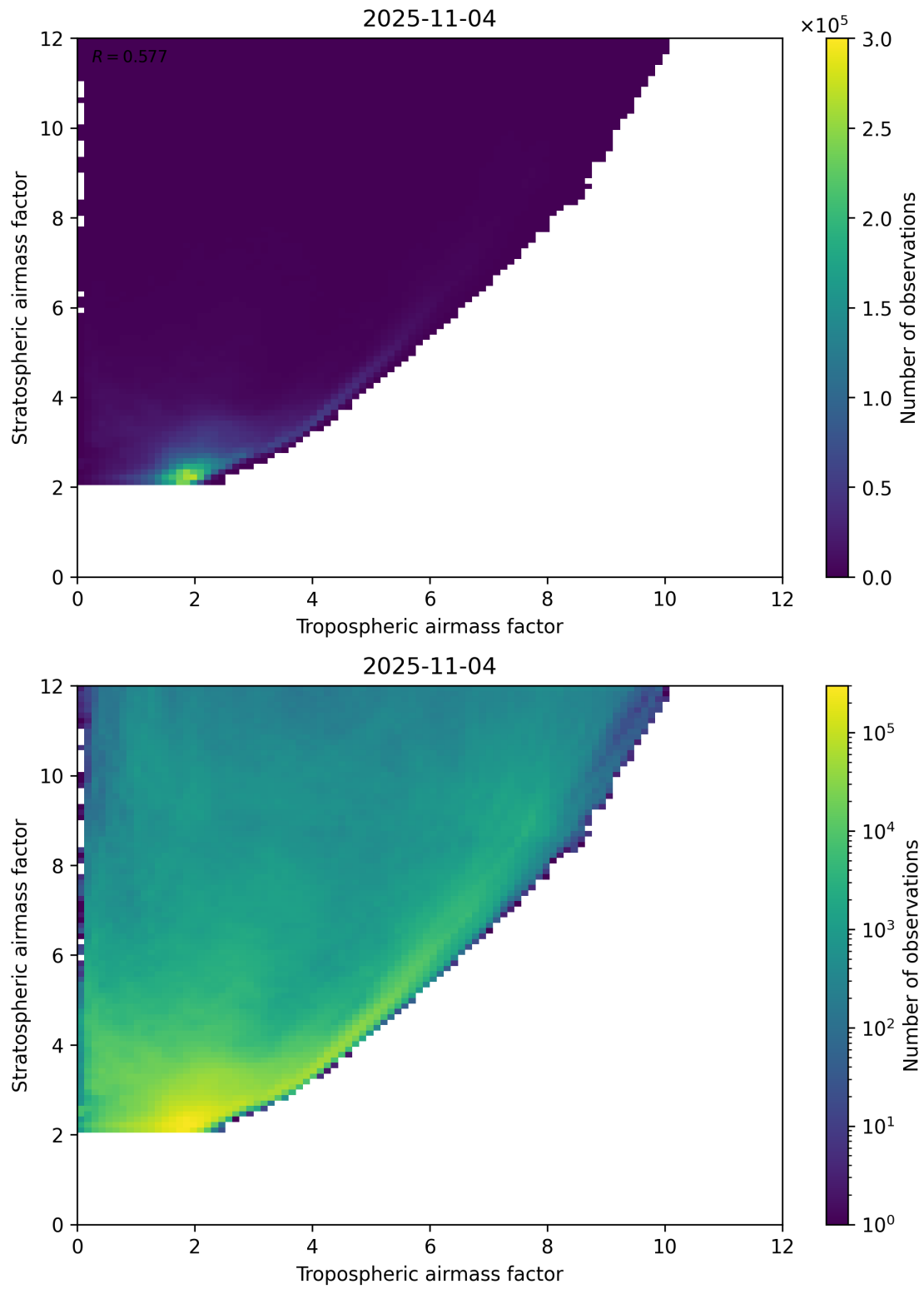
Figure 71: Scatter density plot of “Tropospheric airmass factor” against “Stratospheric airmass factor” for 2025-11-03 to 2025-11-05.
