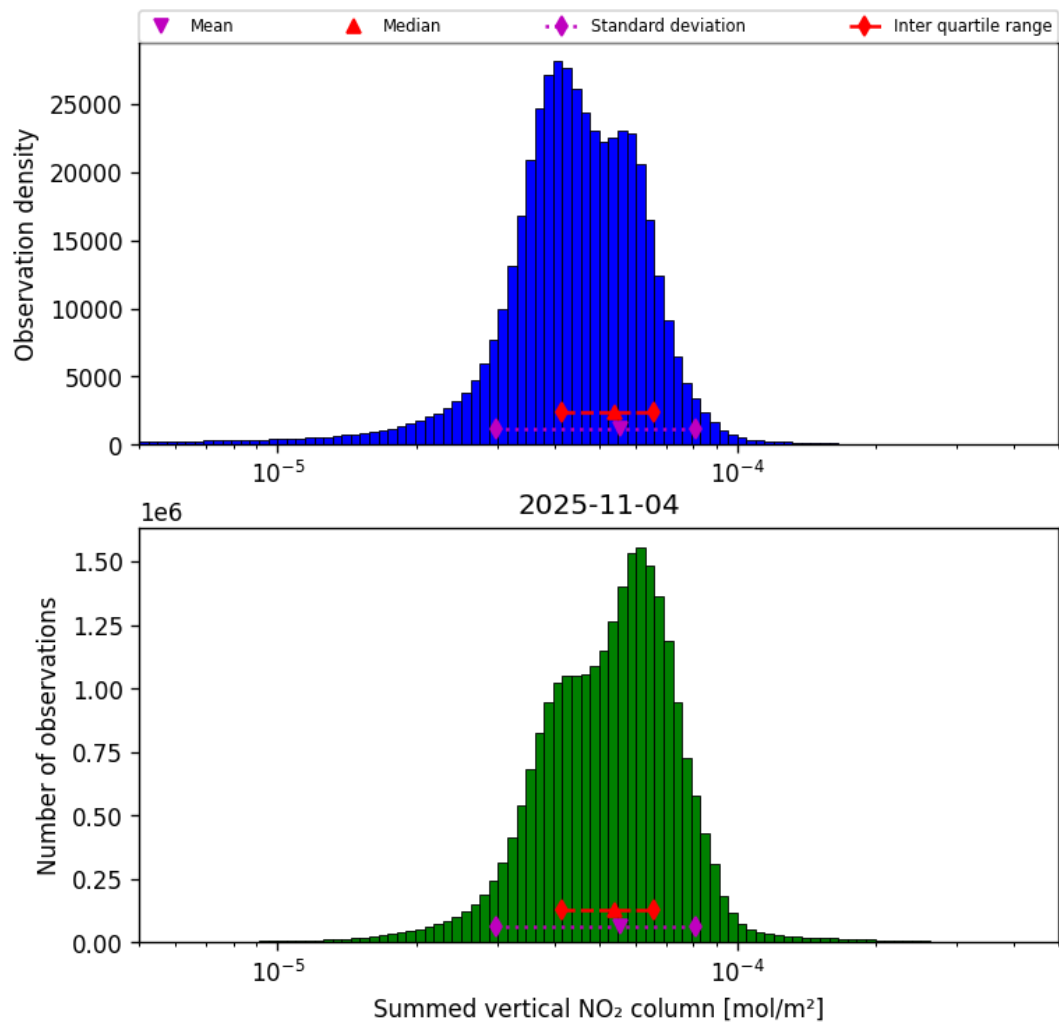
Figure 40: Histogram of “Summed vertical NO 2 column” for 2025-11-03 to 2025-11-05
