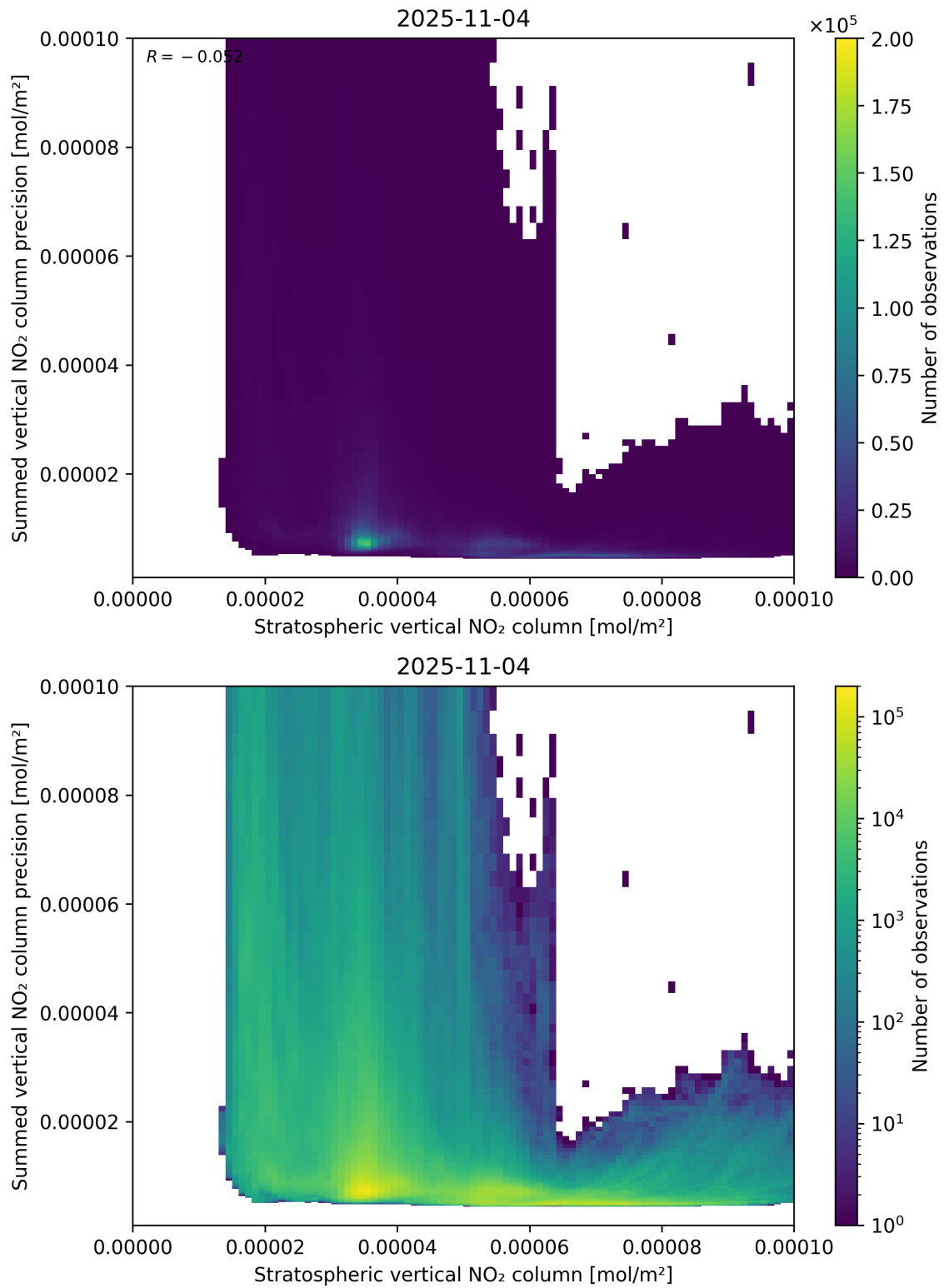
Figure 99: Scatter density plot of “Stratospheric vertical NO 2 column” against “Summed vertical NO 2 column precision” for 2025-11-03 to 2025-11-05.
