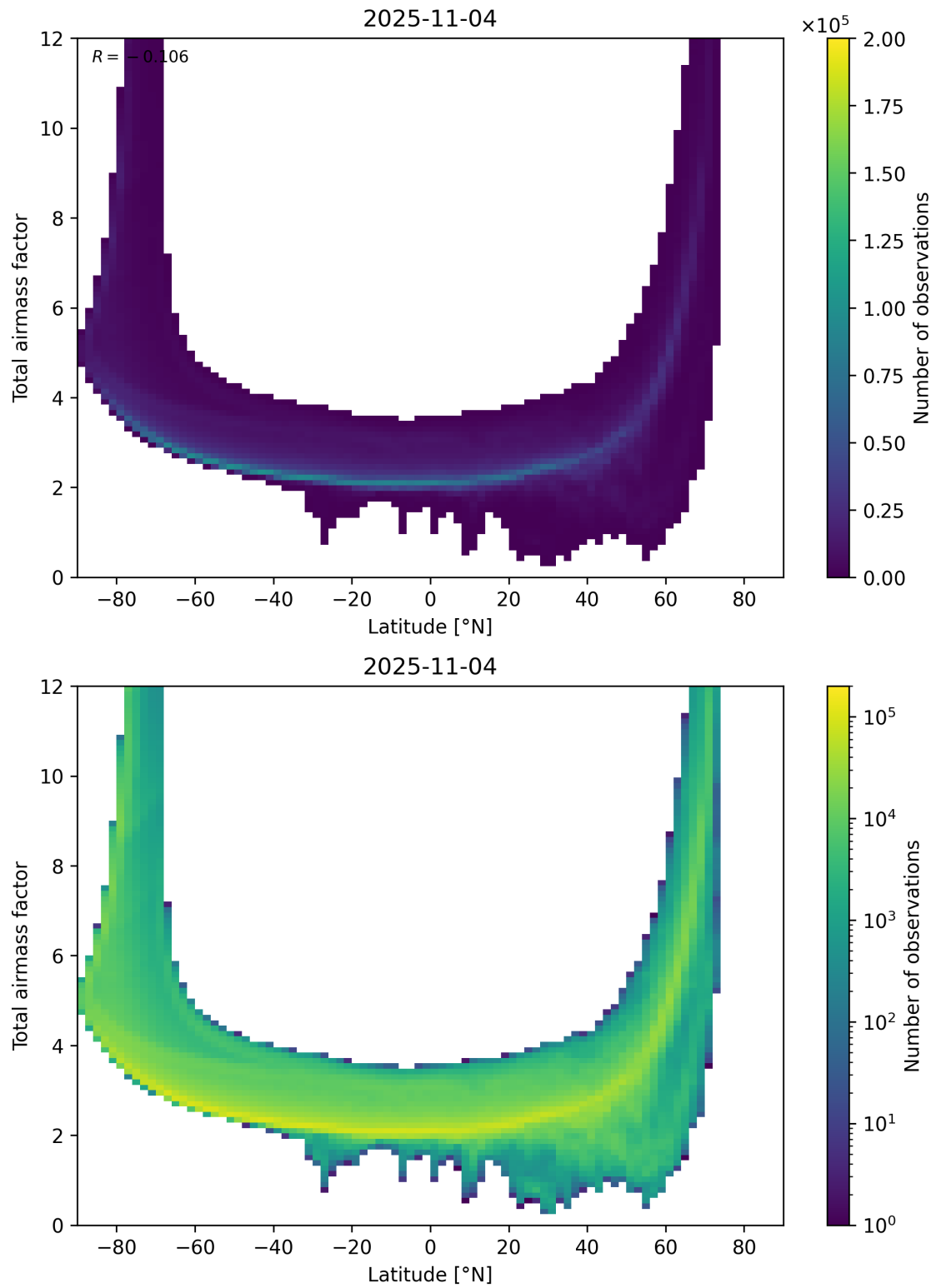
Figure 84: Scatter density plot of “Latitude” against “Total airmass factor” for 2025-11-03 to 2025-11-05.
