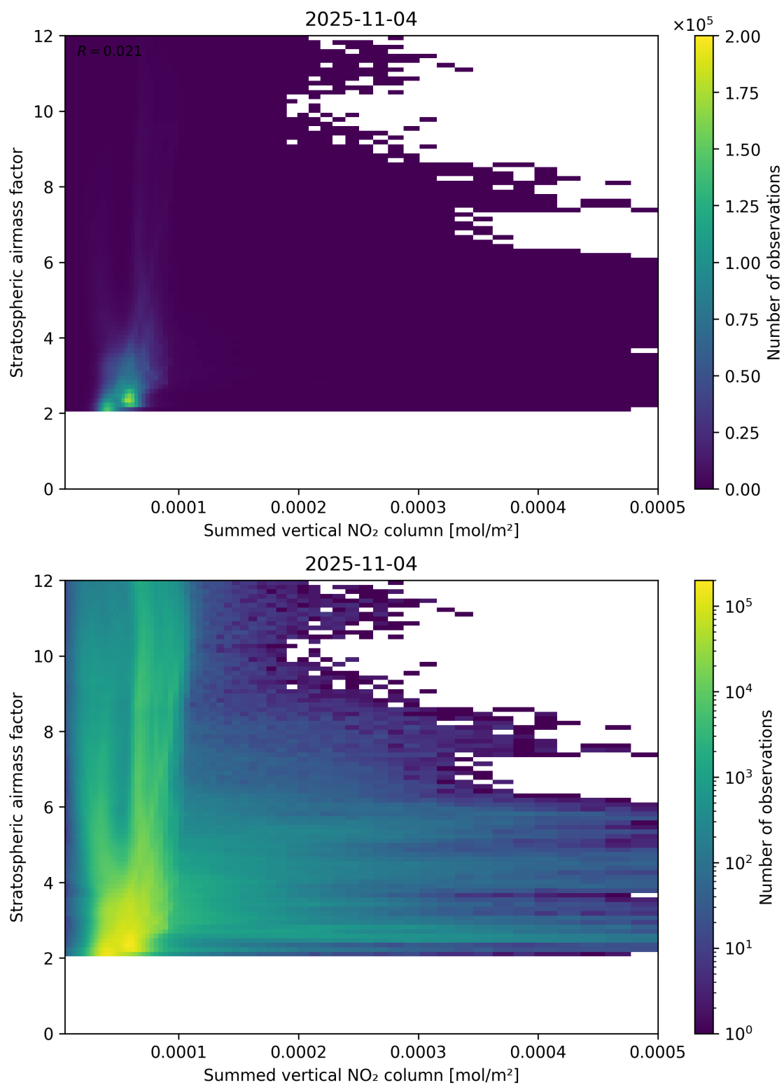
Figure 103: Scatter density plot of “Summed vertical NO 2 column” against “Stratospheric airmass factor” for 2025-11-03 to 2025-11-05.
