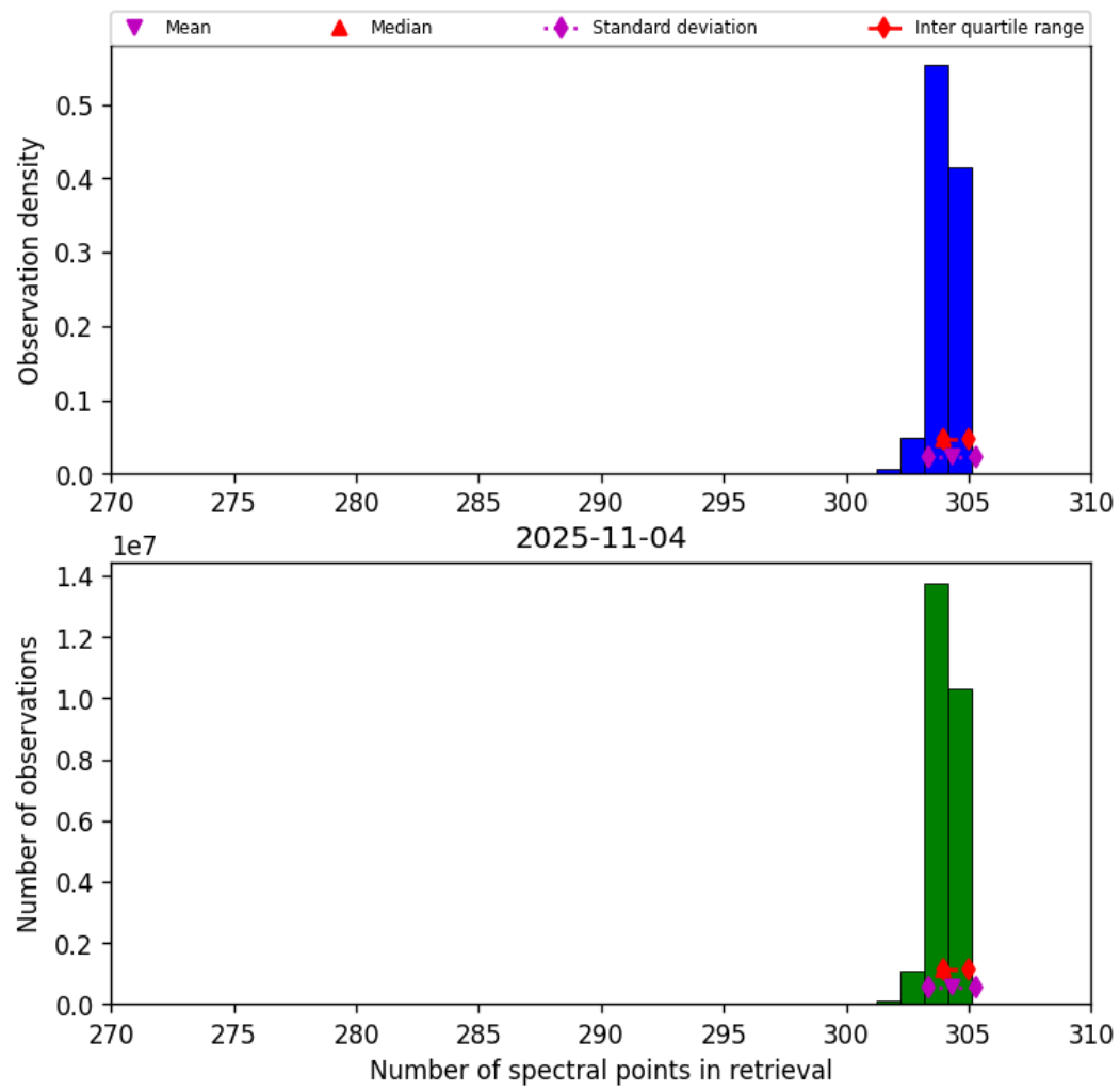
Figure 33: Histogram of “Number of spectral points in retrieval” for 2025-11-03 to 2025-11-05
