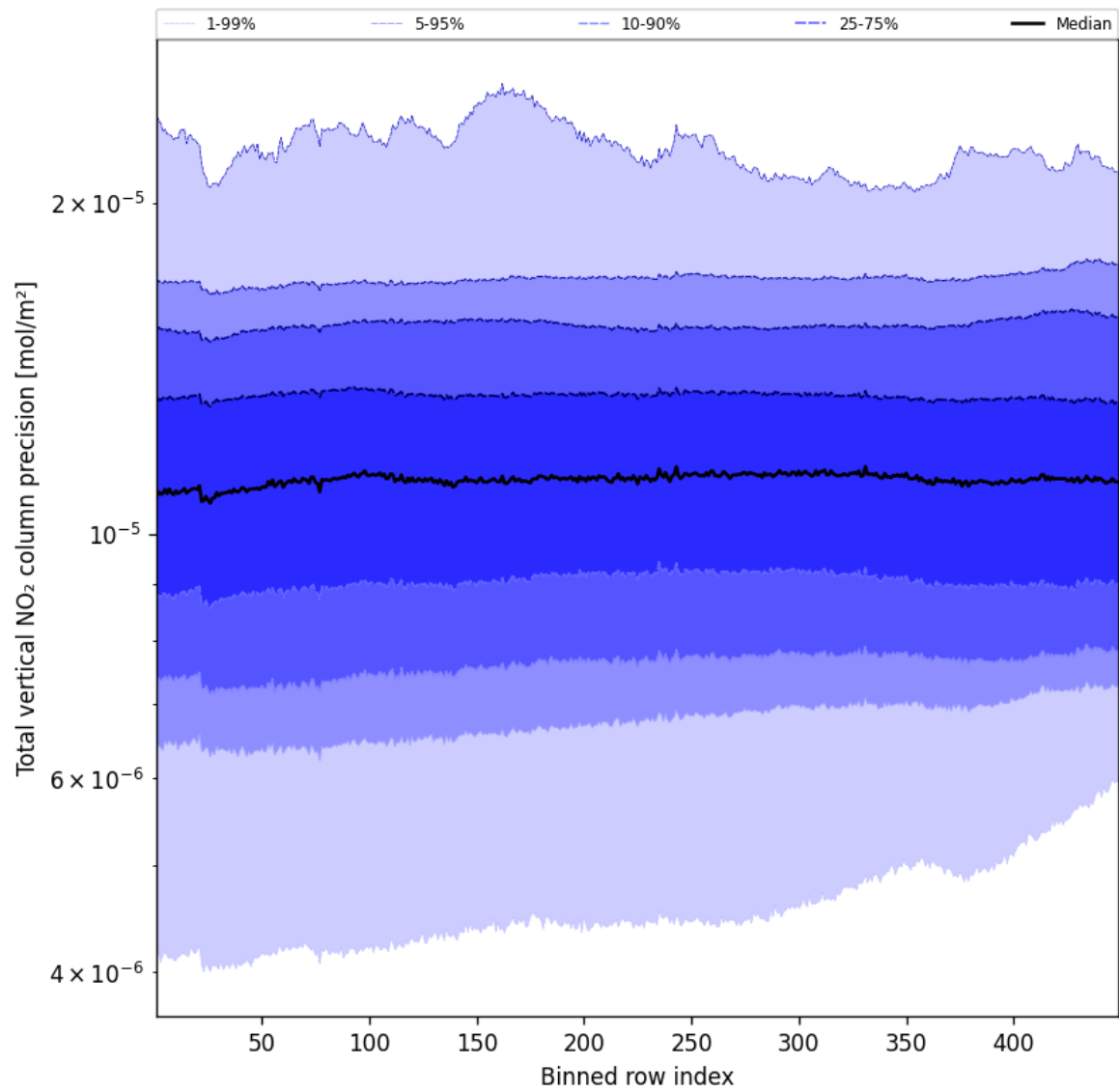
Figure 56: Along track statistics of “Total vertical NO 2 column precision” for 2025-11-03 to 2025-11-05
