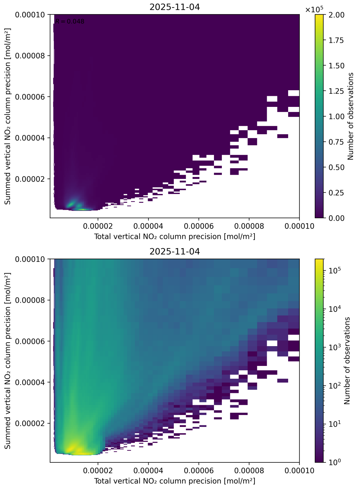
Figure 118: Scatter density plot of “Total vertical NO 2 column precision” against “Summed vertical NO 2 column precision” for 2025-11-03 to 2025-11-05.
