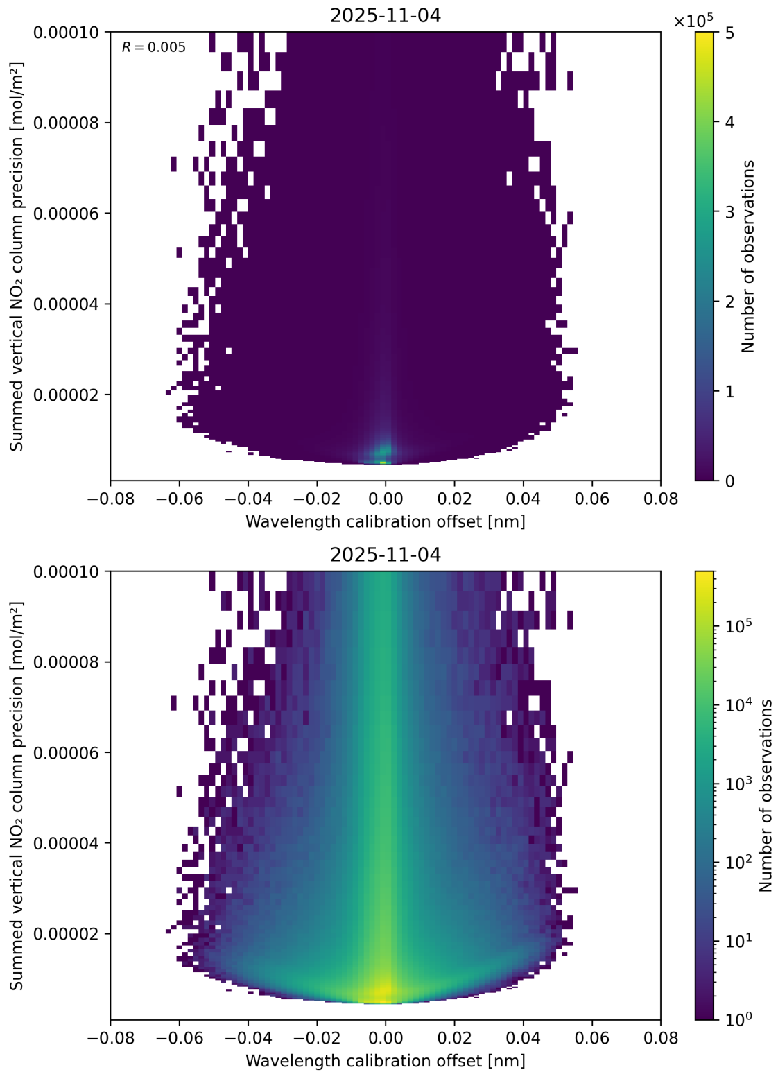
Figure 178: Scatter density plot of “Wavelength calibration offset” against “Summed vertical NO 2 column precision” for 2025-11-03 to 2025-11-05.
