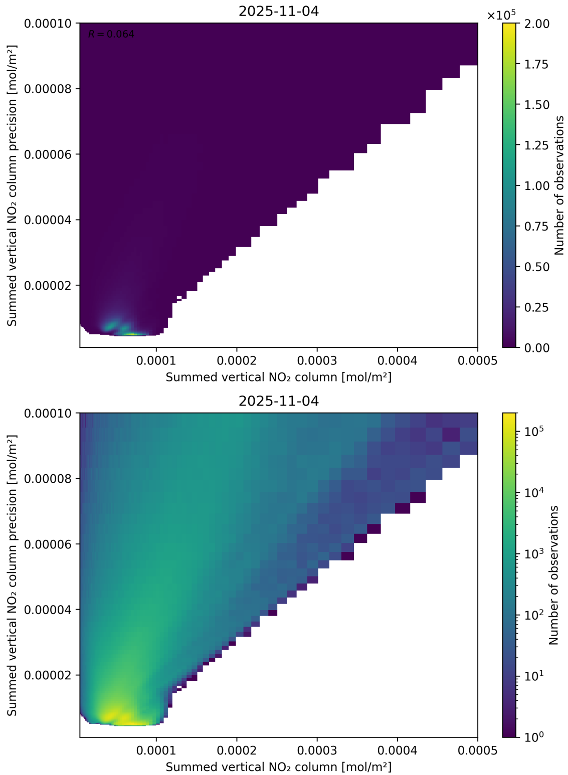
Figure 105: Scatter density plot of “Summed vertical NO 2 column” against “Summed vertical NO 2 column precision” for 2025-11-03 to 2025-11-05.
