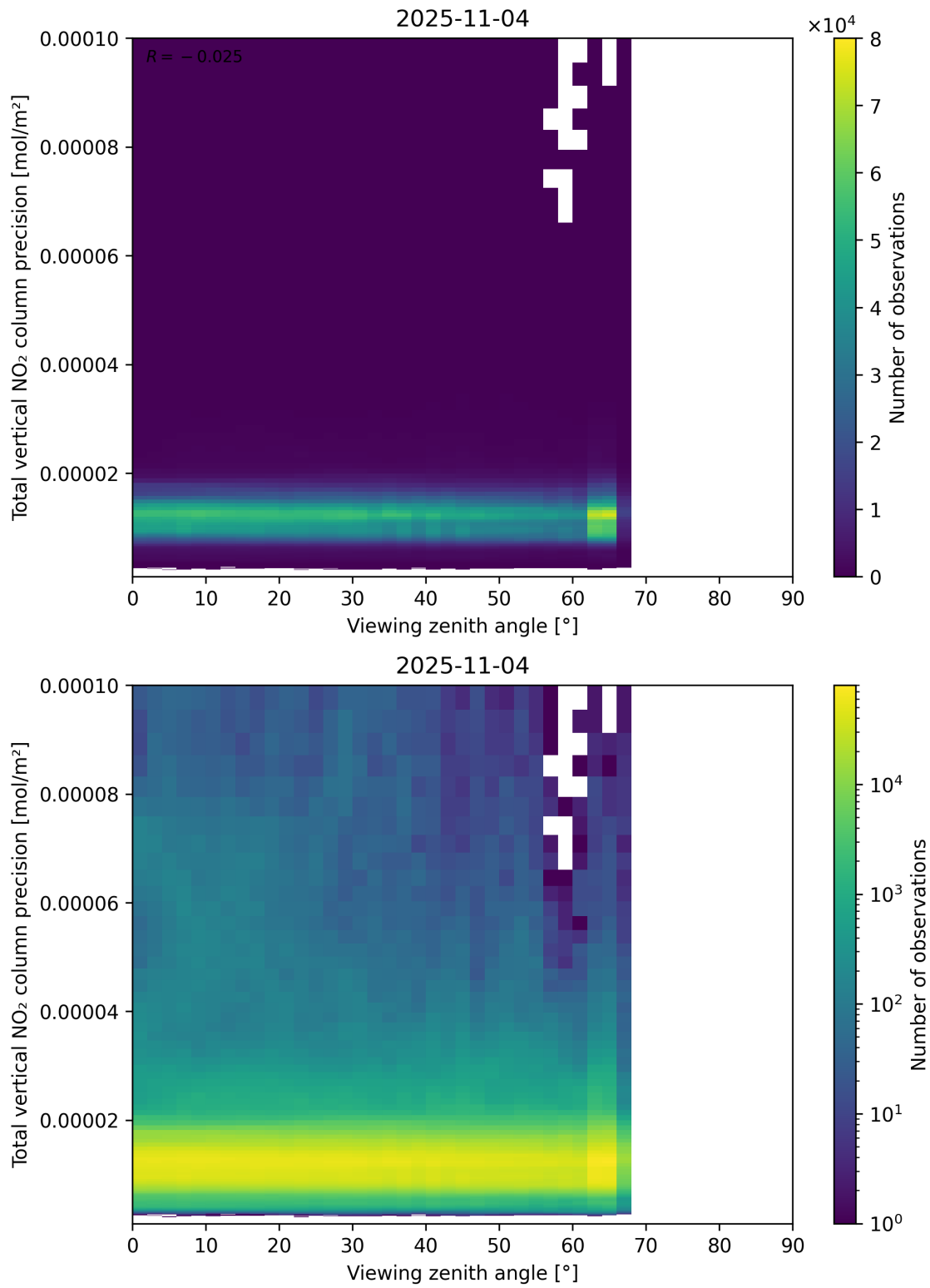
Figure 168: Scatter density plot of “Viewing zenith angle” against “Total vertical NO 2 column precision” for 2025-11-03 to 2025-11-05.
