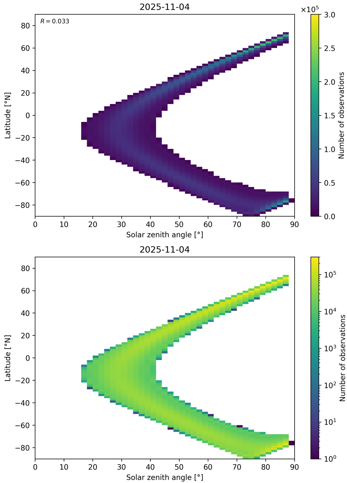
Figure 149: Scatter density plot of “Solar zenith angle” against “Latitude” for 2025-11-03 to 2025-11-05.
