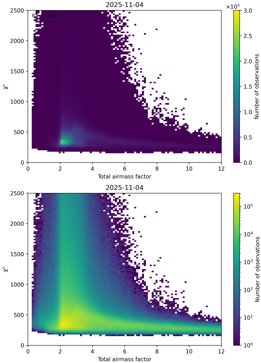
Figure 63: Scatter density plot of “Total airmass factor” against “ \chi^2 ” for 2025-11-03 to 2025-11-05.
