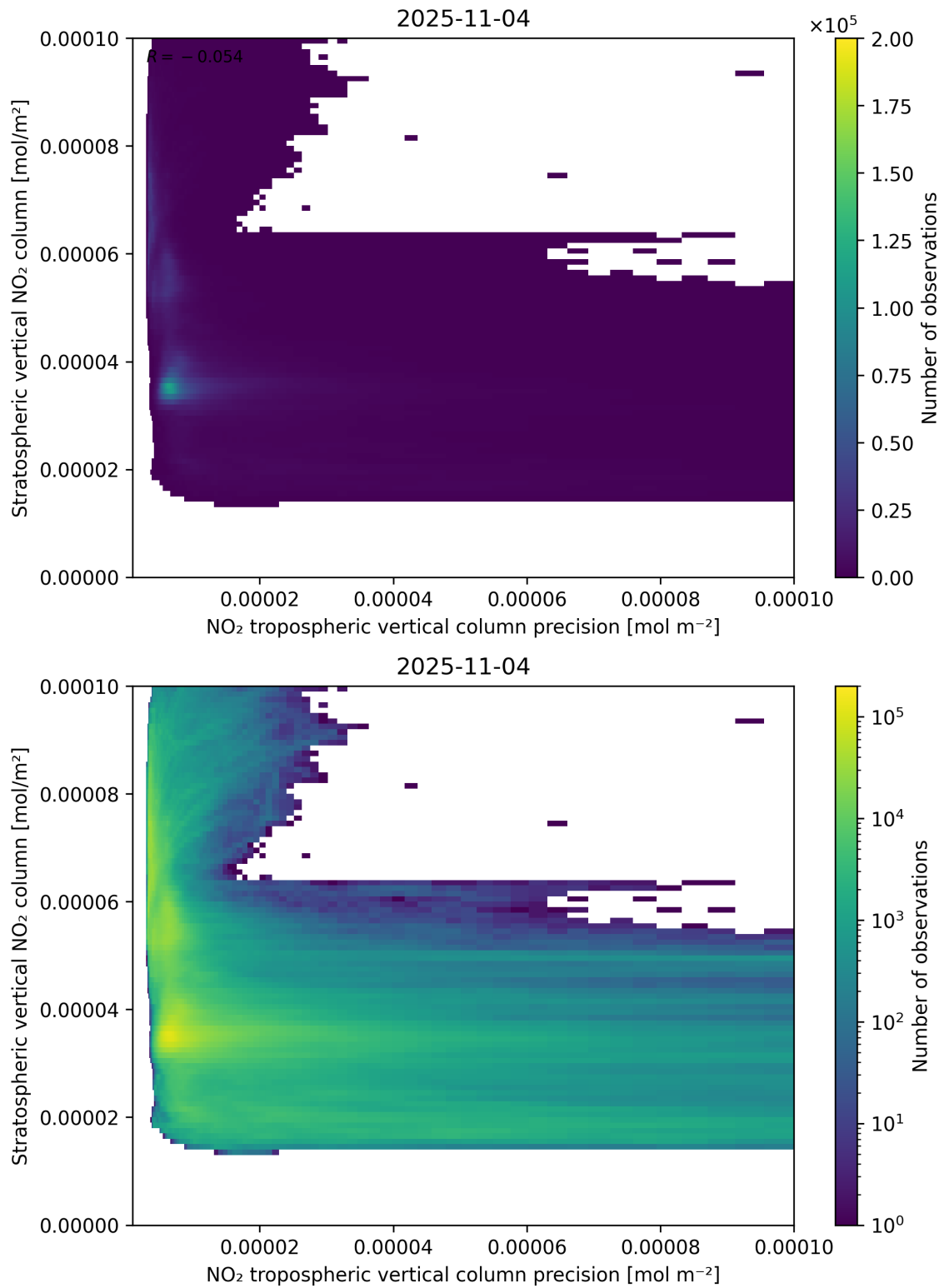
Figure 135: Scatter density plot of “NO 2 tropospheric vertical column precision” against “Stratospheric vertical NO 2 column” for 2025-11-03 to 2025-11-05.
