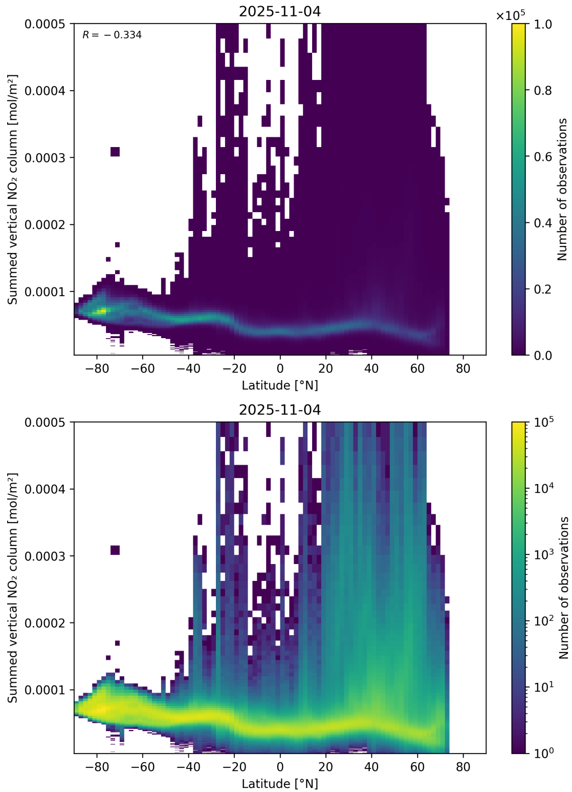
Figure 88: Scatter density plot of “Latitude” against “Summed vertical NO 2 column” for 2025-11-03 to 2025-11-05.
