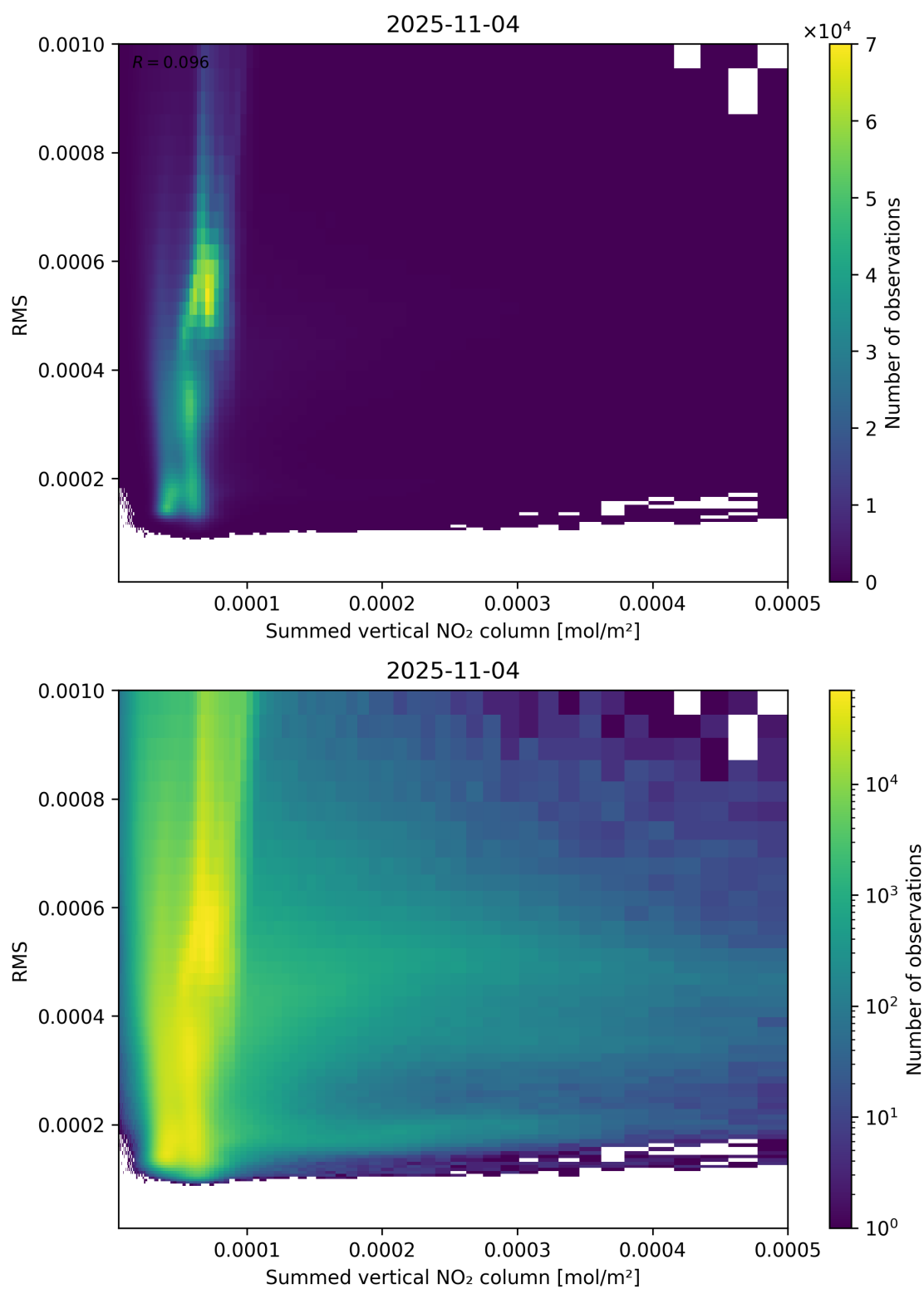
Figure 109: Scatter density plot of “Summed vertical NO 2 column” against “RMS” for 2025-11-03 to 2025-11-05.
