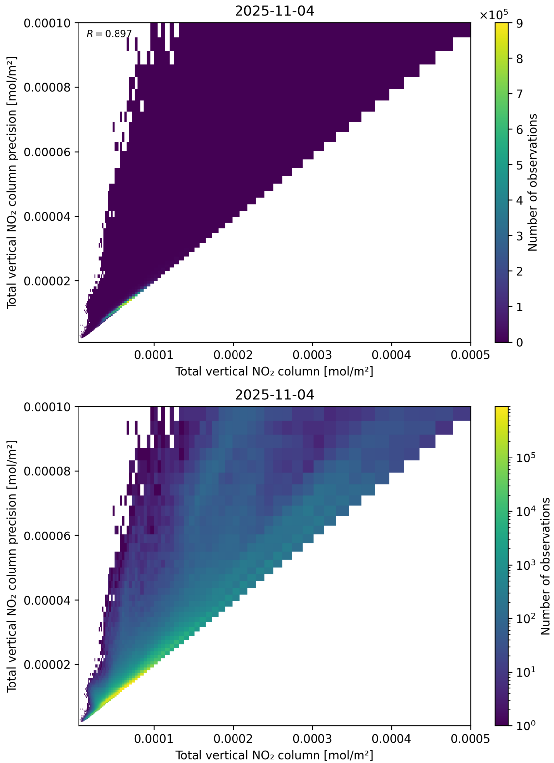
Figure 114: Scatter density plot of “Total vertical NO 2 column” against “Total vertical NO 2 column precision” for 2025-11-03 to 2025-11-05.
