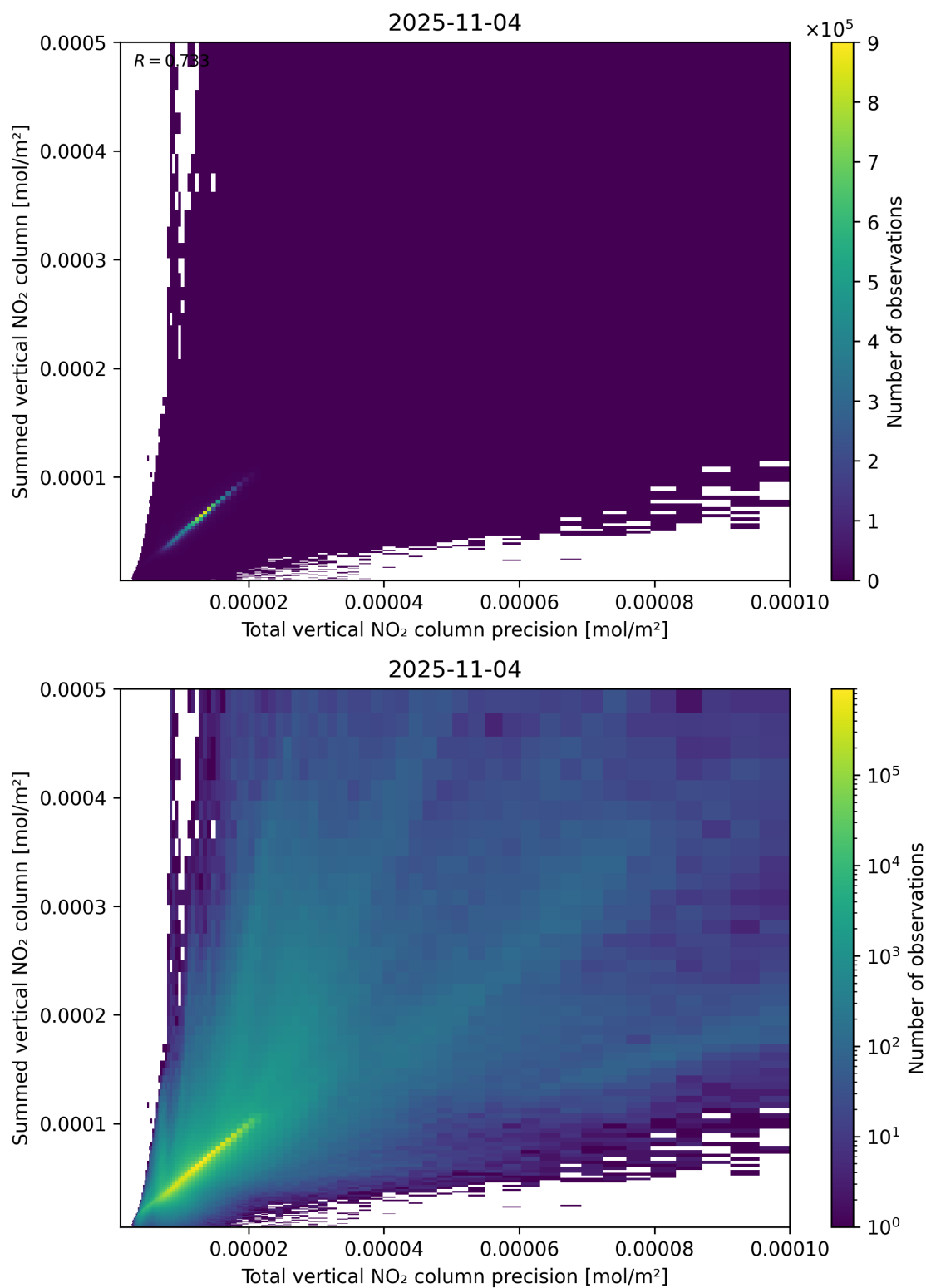
Figure 117: Scatter density plot of “Total vertical NO 2 column precision” against “Summed vertical NO 2 column” for 2025-11-03 to 2025-11-05.
