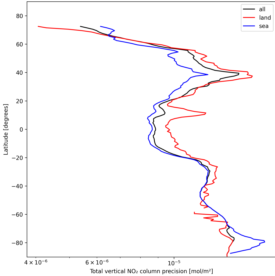
Figure 22: Zonal average of “Total vertical NO 2 column precision” for 2025-11-03 to 2025-11-05.
