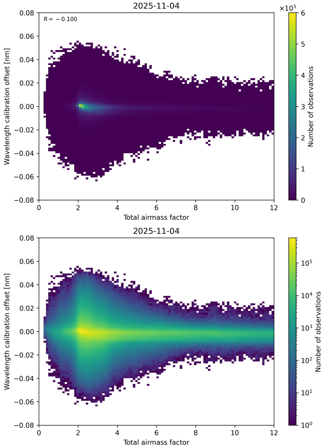
Figure 70: Scatter density plot of “Total airmass factor” against “Wavelength calibration offset” for 2025-11-03 to 2025-11-05.
