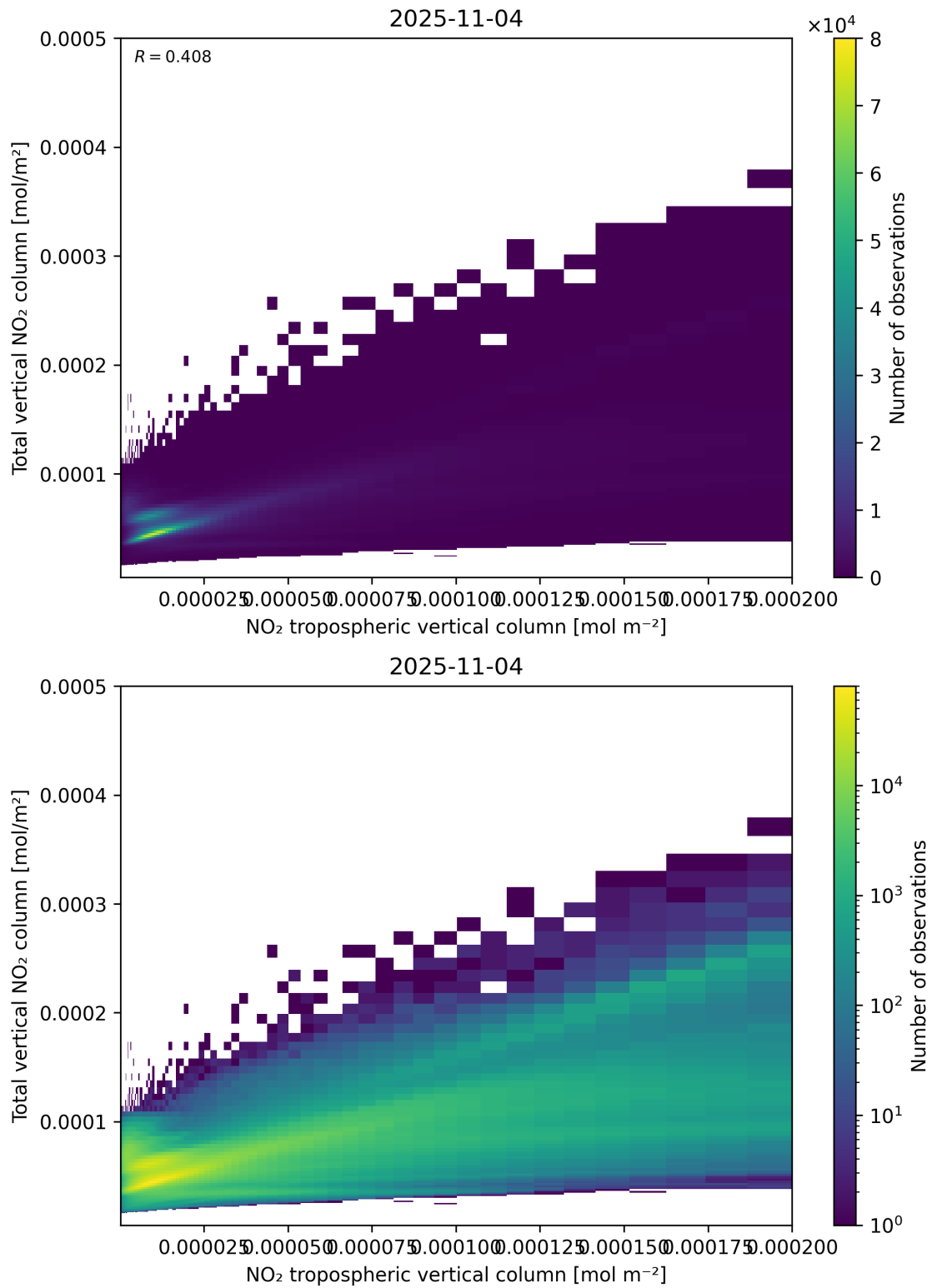
Figure 128: Scatter density plot of “NO 2 tropospheric vertical column” against “Total vertical NO 2 column” for 2025-11-03 to 2025-11-05.
