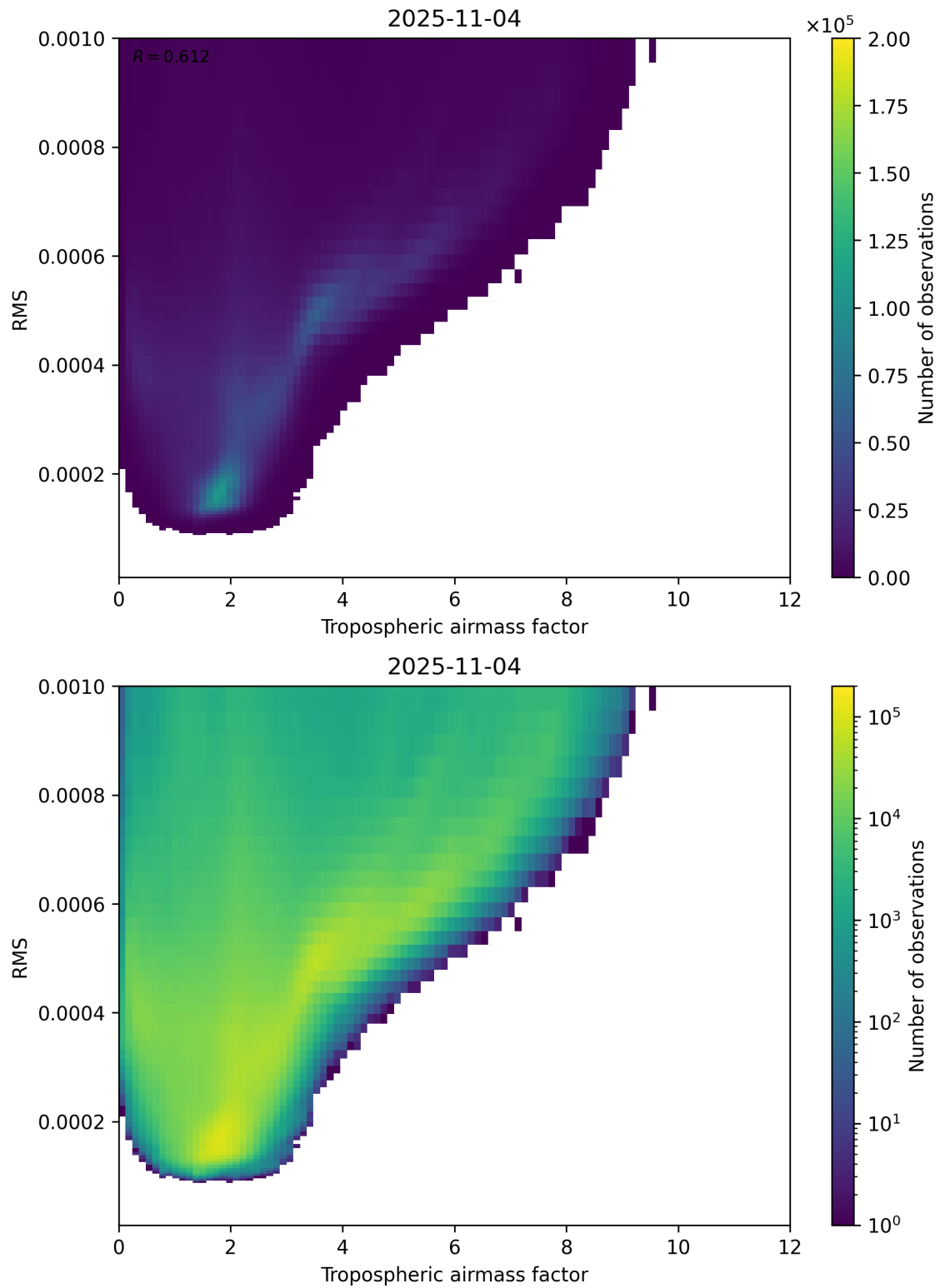
Figure 79: Scatter density plot of “Tropospheric airmass factor” against “RMS” for 2025-11-03 to 2025-11-05.
