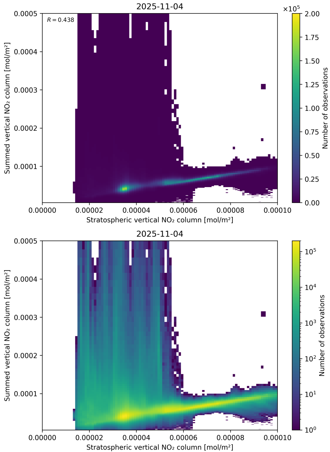
Figure 98: Scatter density plot of “Stratospheric vertical NO 2 column” against “Summed vertical NO 2 column” for 2025-11-03 to 2025-11-05.
