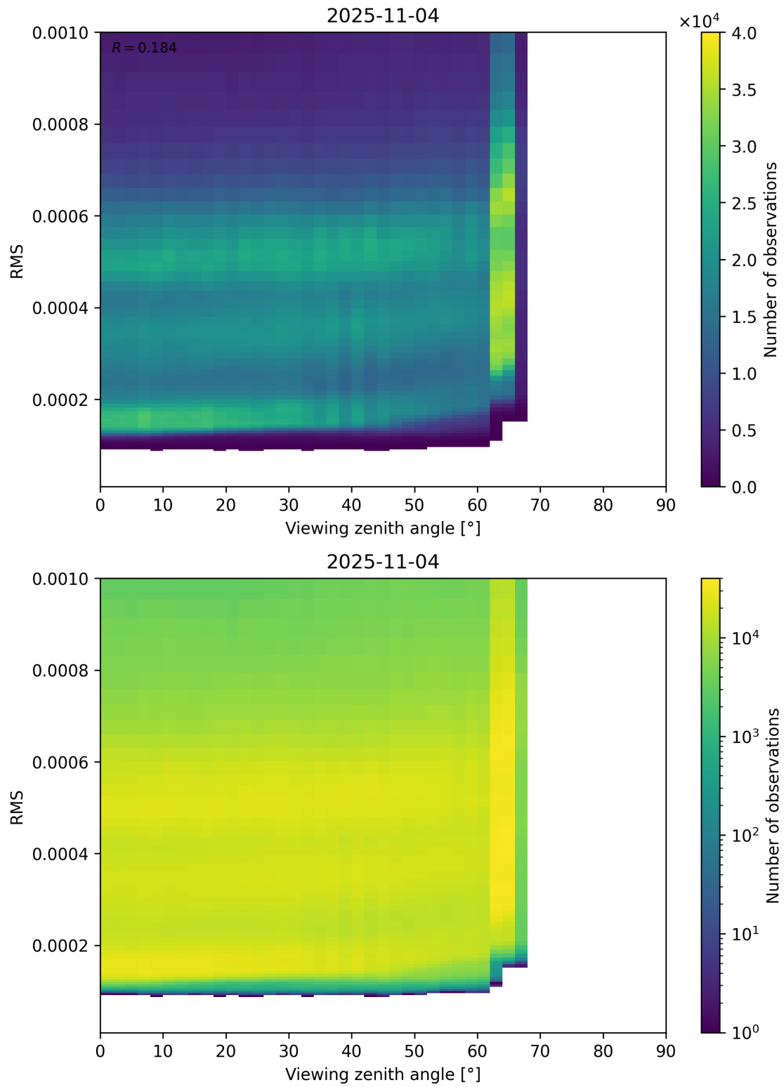
Figure 171: Scatter density plot of “Viewing zenith angle” against “RMS” for 2025-11-03 to 2025-11-05.
