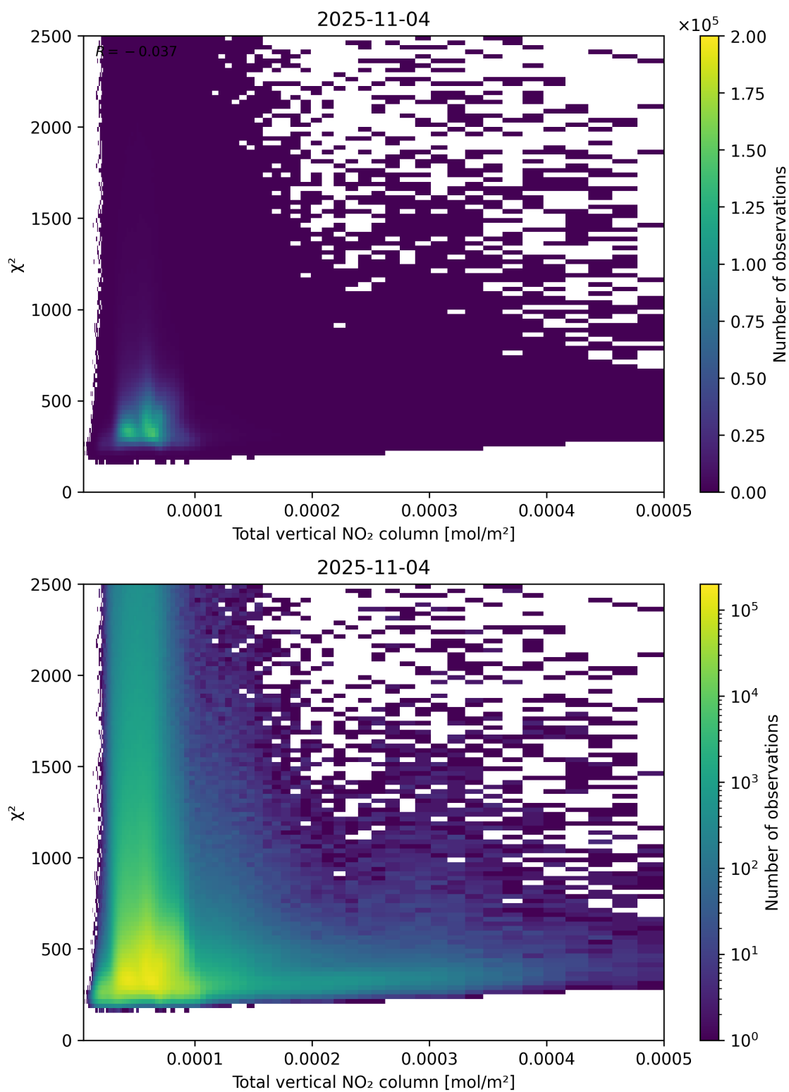
Figure 111: Scatter density plot of “Total vertical NO 2 column” against “ \chi^2 ” for 2025-11-03 to 2025-11-05.
