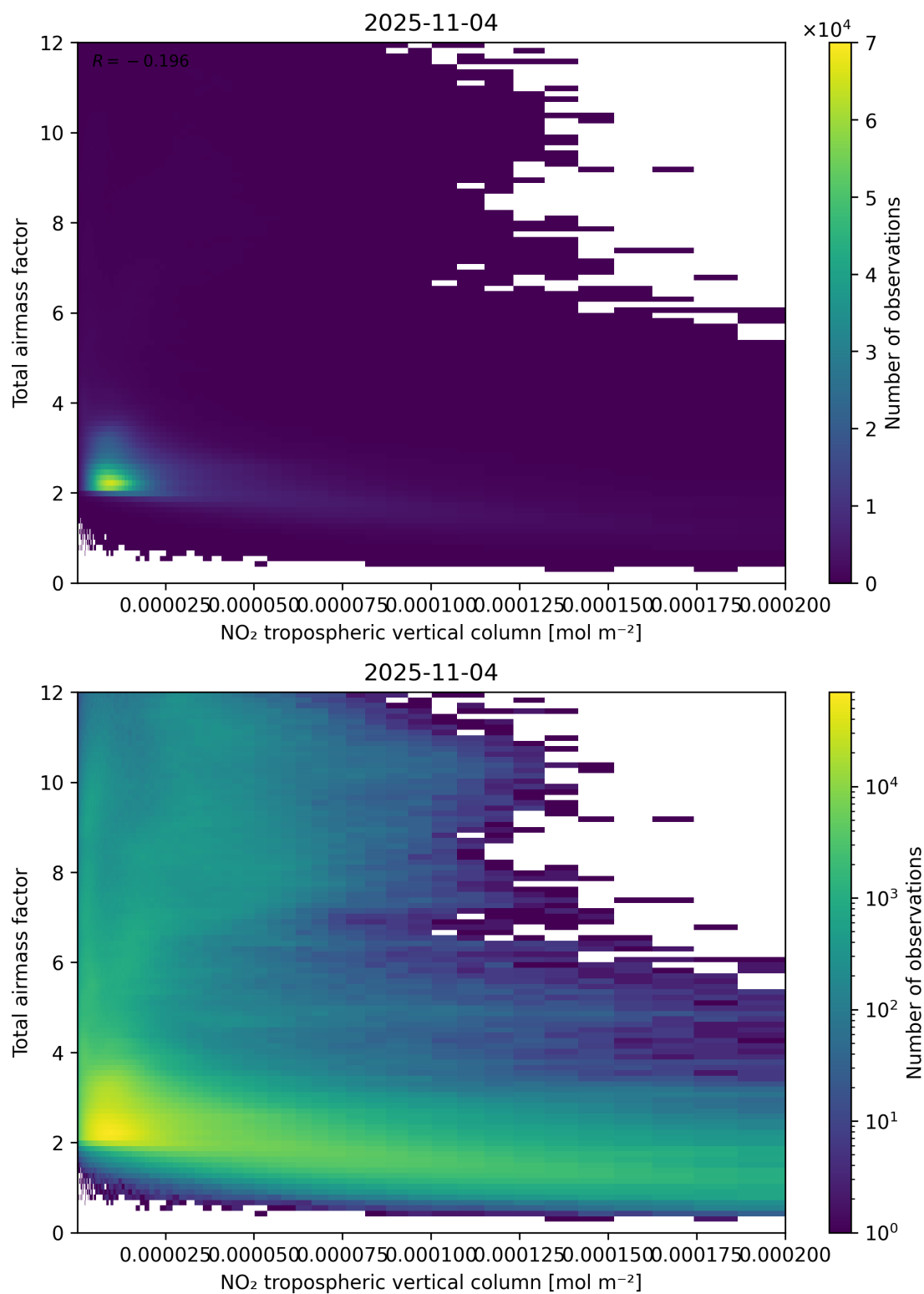
Figure 122: Scatter density plot of “NO 2 tropospheric vertical column” against “Total air mass factor” for 2025-11-03 to 2025-11-05.
