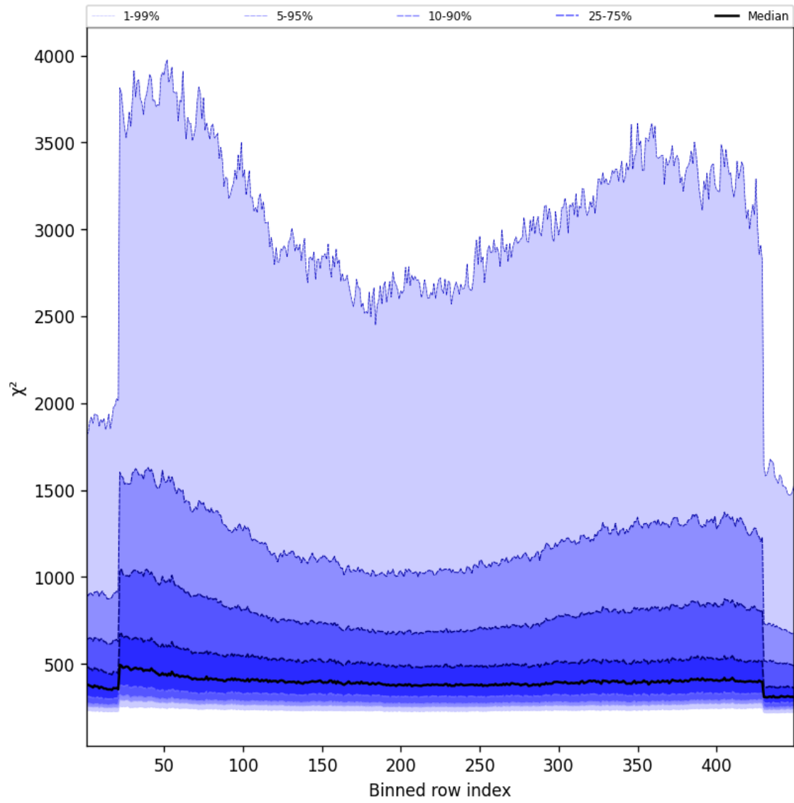
Figure 59: Along track statistics of “ \chi^2 ” for 2025-11-03 to 2025-11-05
