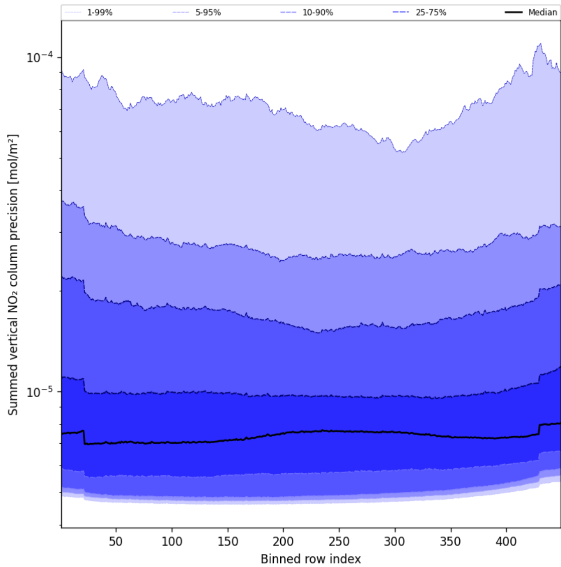
Figure 58: Along track statistics of “Summed vertical NO 2 column precision” for 2025-11-03 to 2025-11-05
