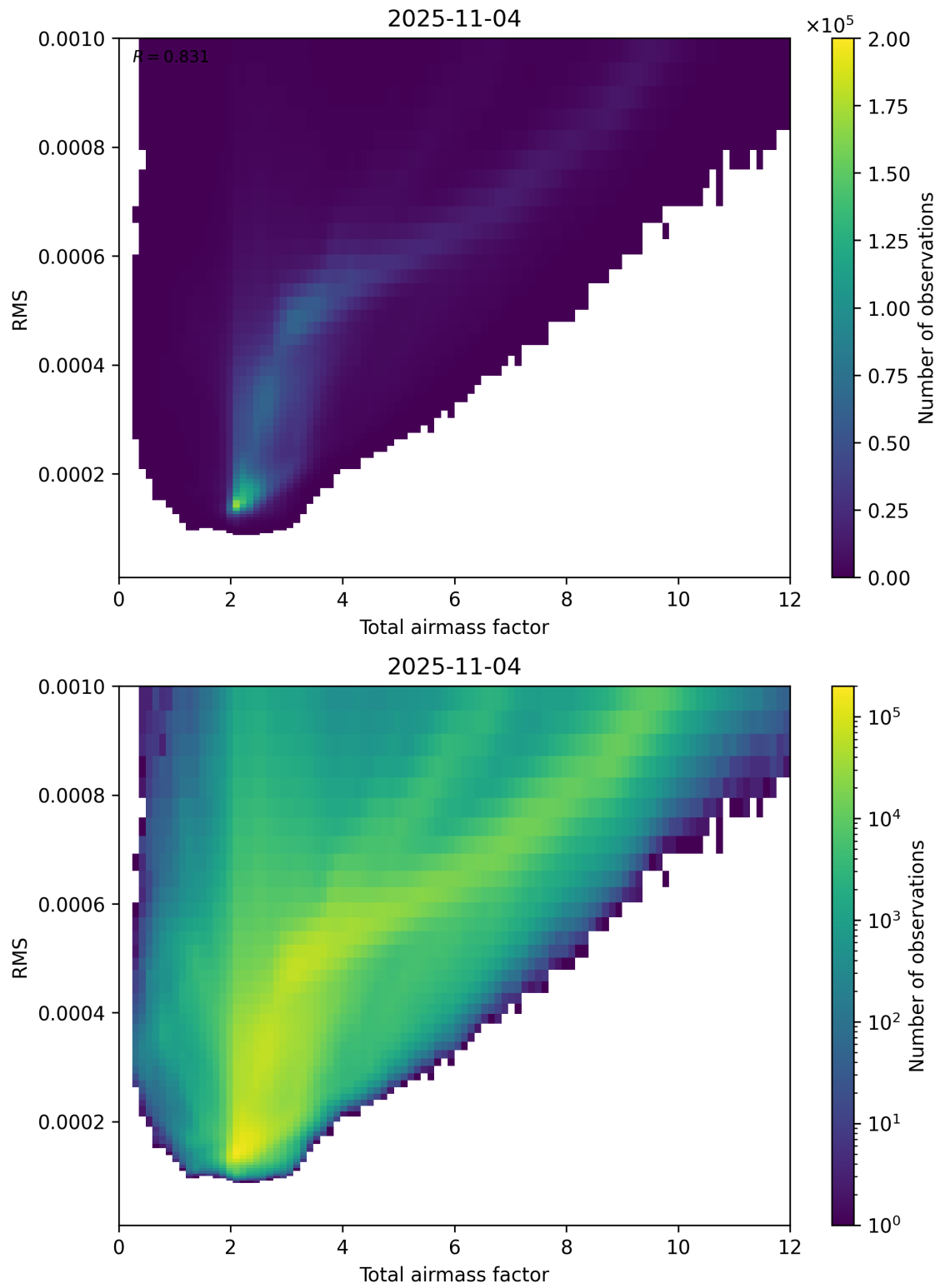
Figure 69: Scatter density plot of “Total airmass factor” against “RMS” for 2025-11-03 to 2025-11-05.
