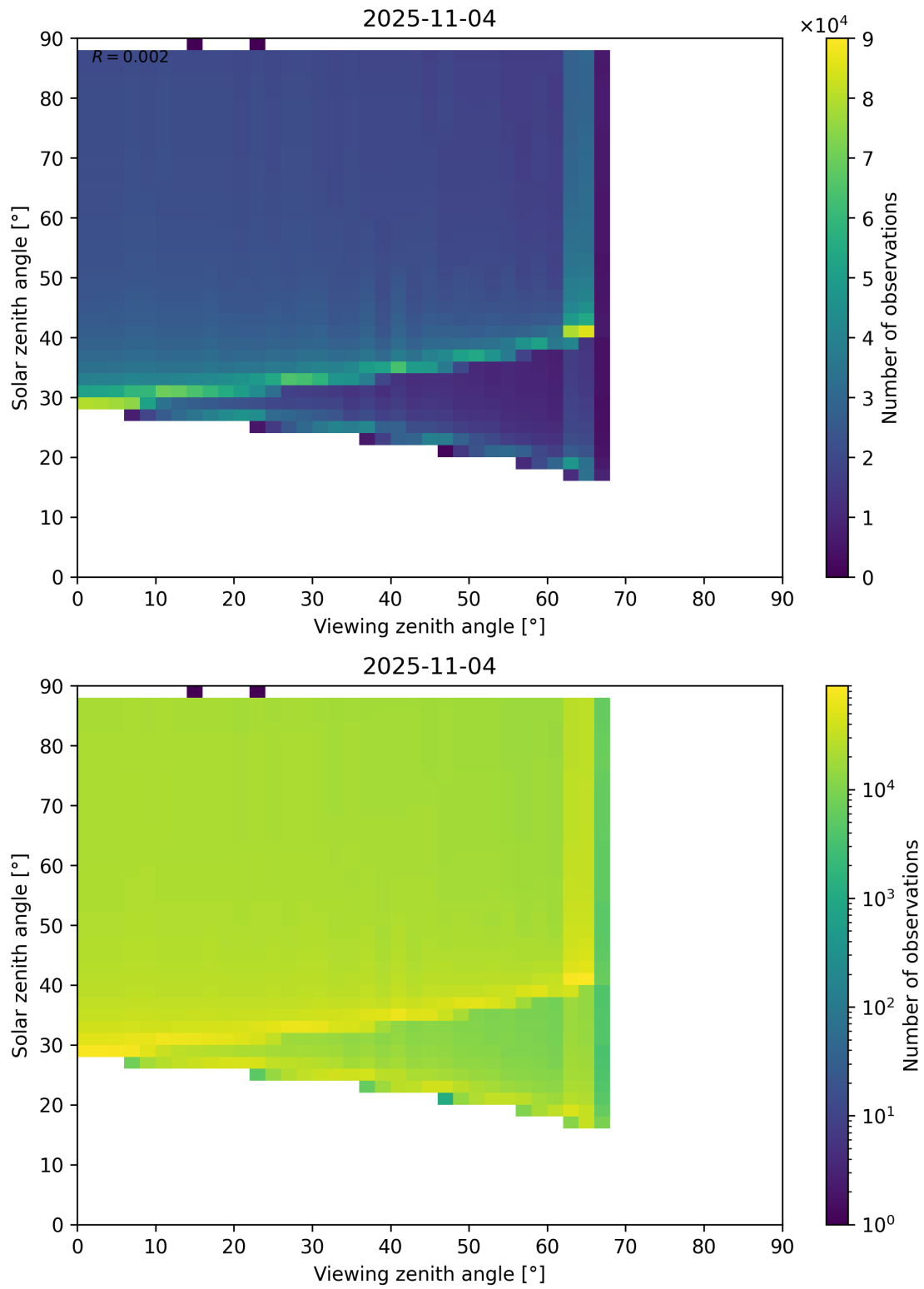
Figure 172: Scatter density plot of “Viewing zenith angle” against “Solar zenith angle” for 2025-11-03 to 2025-11-05.
