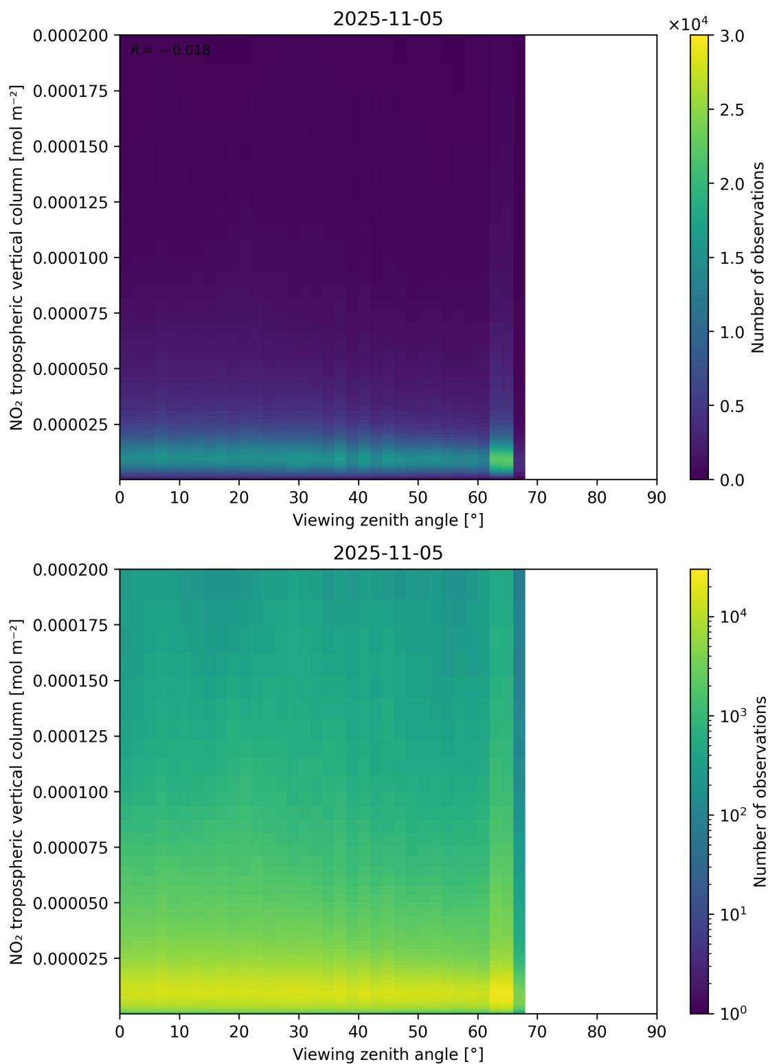
Figure 169: Scatter density plot of “Viewing zenith angle” against “NO 2 tropospheric vertical column” for 2025-11-04 to 2025-11-06.
