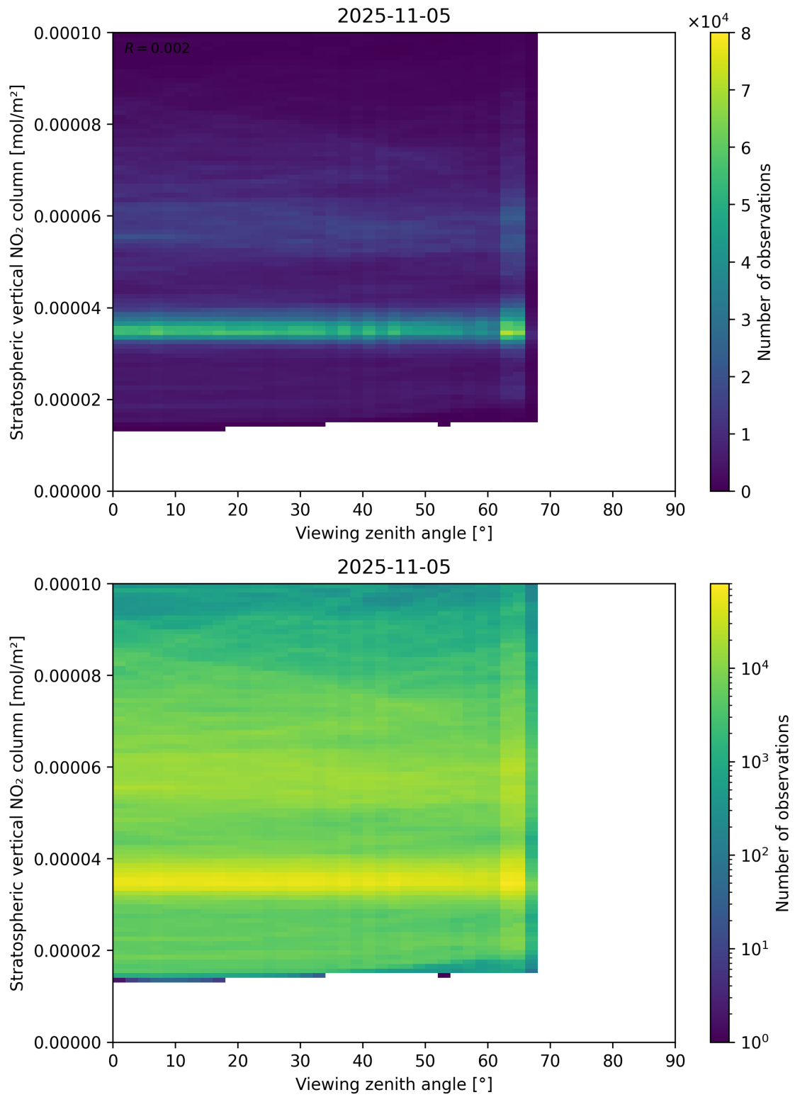
Figure 164: Scatter density plot of “Viewing zenith angle” against “Stratospheric vertical NO 2 column” for 2025-11-04 to 2025-11-06.
