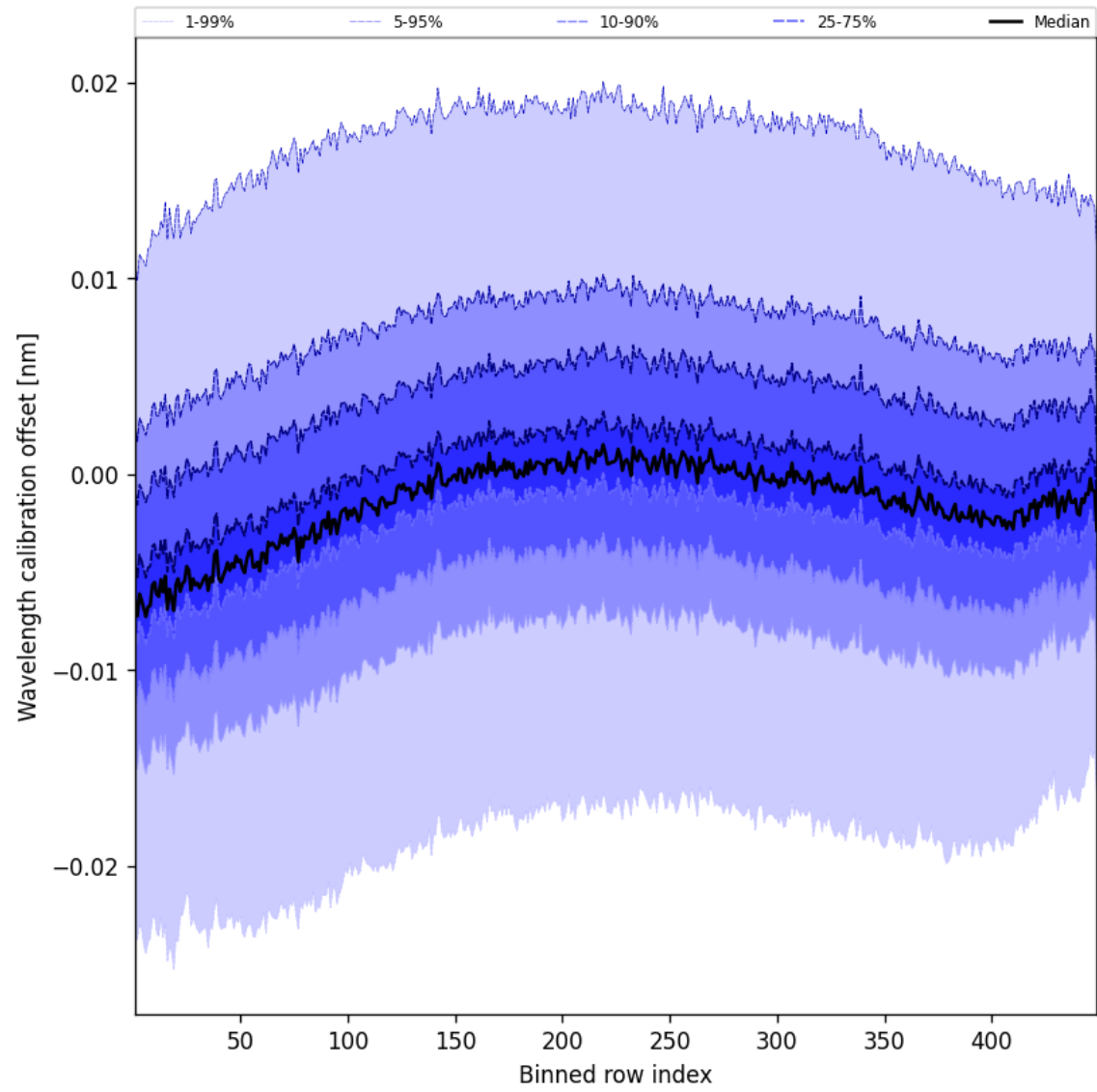
Figure 52: Along track statistics of “Wavelength calibration offset” for 2025-11-04 to 2025-11-06
