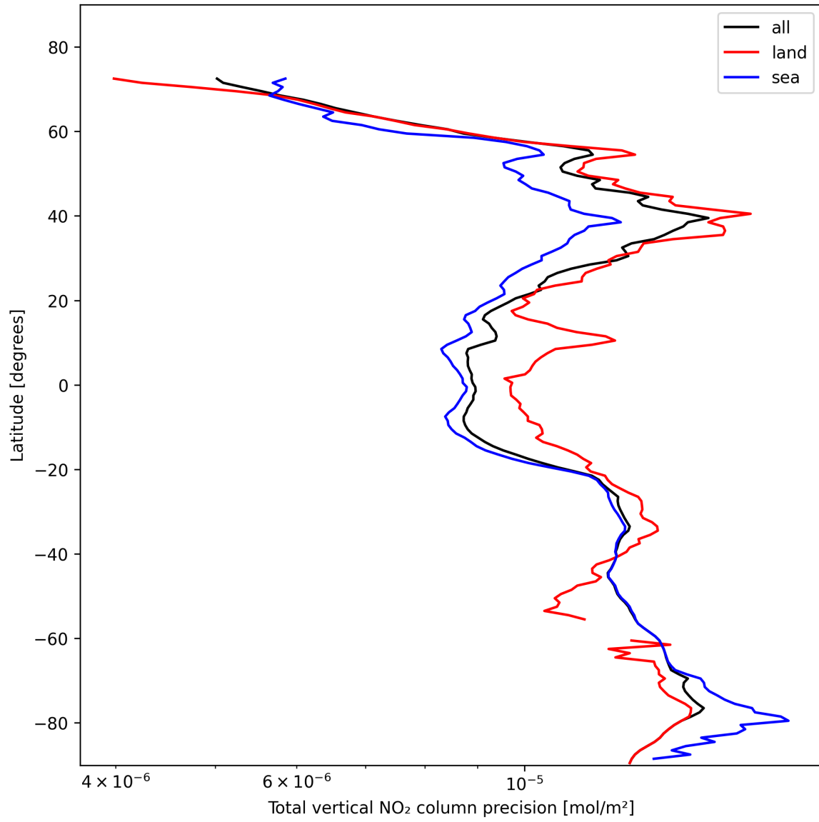
Figure 22: Zonal average of “Total vertical NO 2 column precision” for 2025-11-04 to 2025-11-06.
