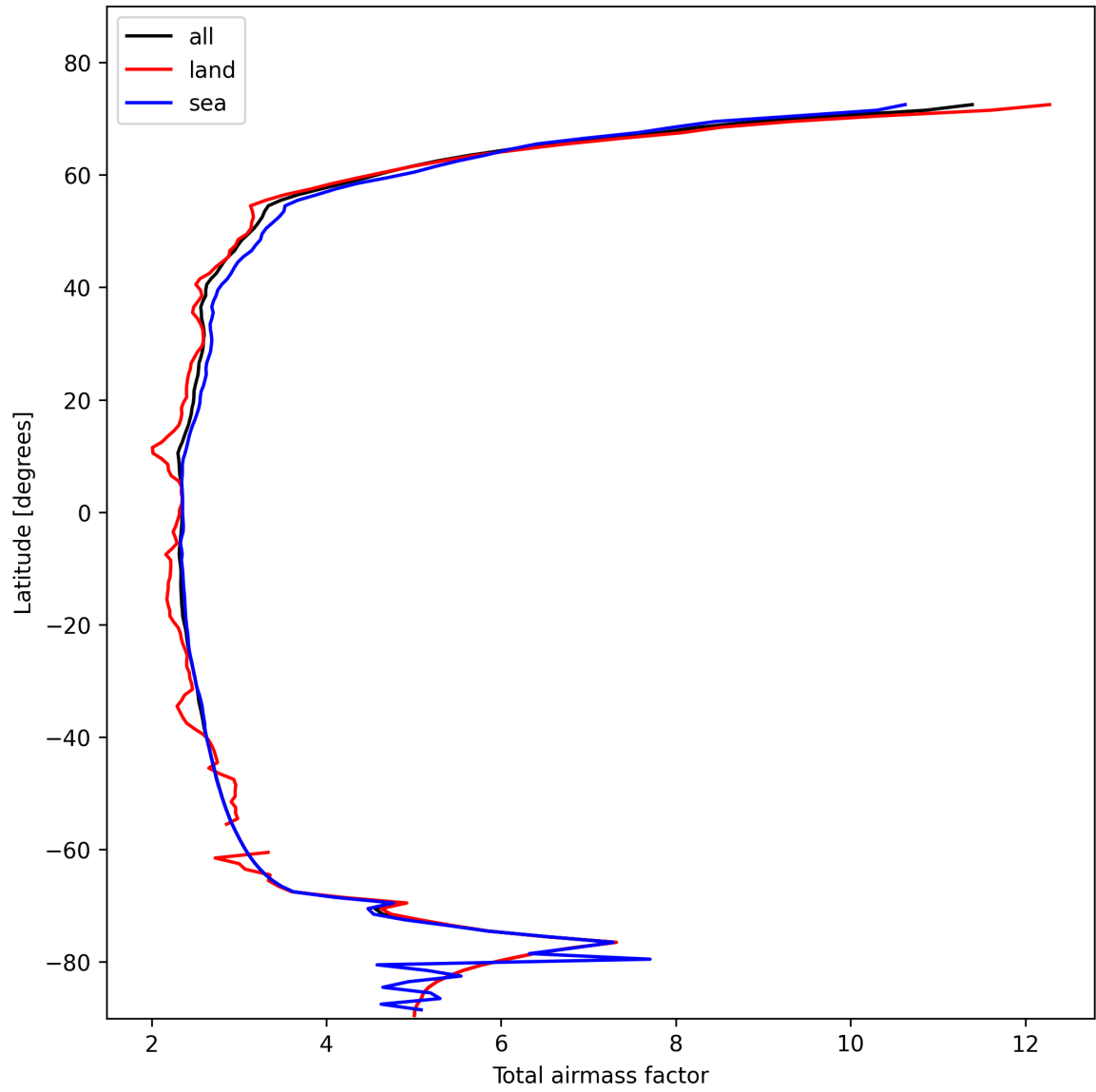
Figure 15: Zonal average of “Total airmass factor” for 2025-11-04 to 2025-11-06.
