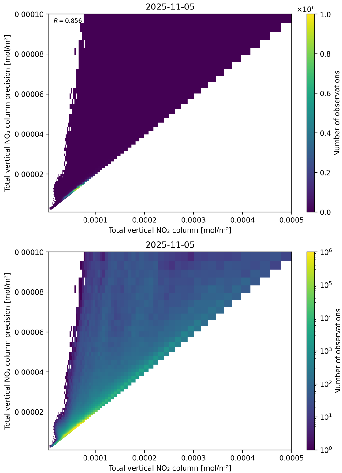
Figure 114: Scatter density plot of “Total vertical NO 2 column” against “Total vertical NO 2 column precision” for 2025-11-04 to 2025-11-06.
