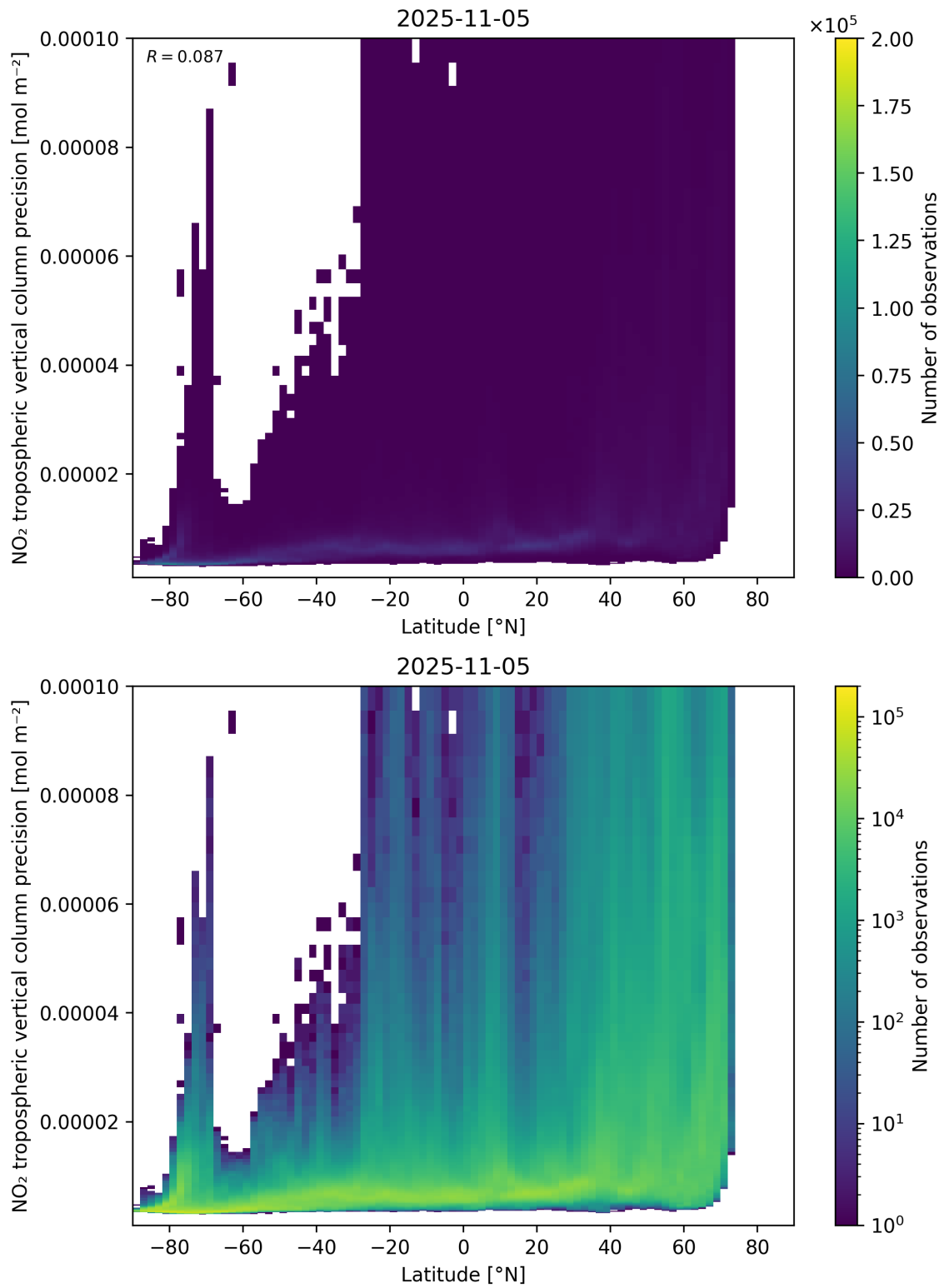
Figure 93: Scatter density plot of “Latitude” against “NO 2 tropospheric vertical column precision” for 2025-11-04 to 2025-11-06.
