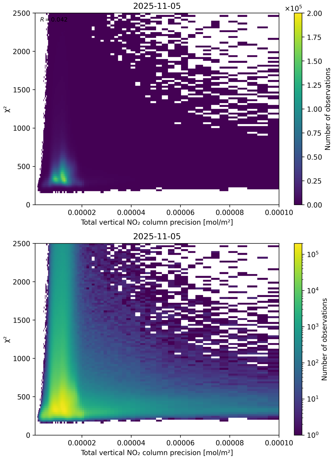
Figure 116: Scatter density plot of “Total vertical NO 2 column precision” against “ \chi^2 ” for 2025-11-04 to 2025-11-06.
