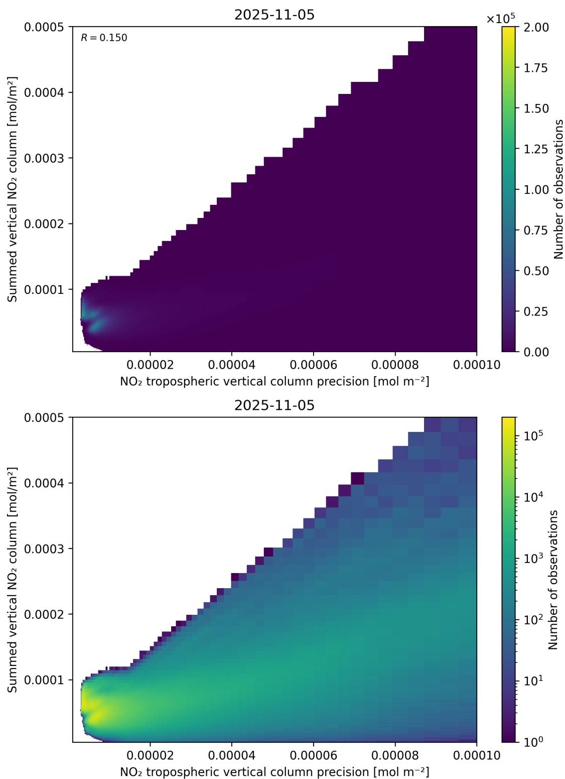
Figure 136: Scatter density plot of “NO 2 tropospheric vertical column precision” against “Summed vertical NO 2 column” for 2025-11-04 to 2025-11-06.
