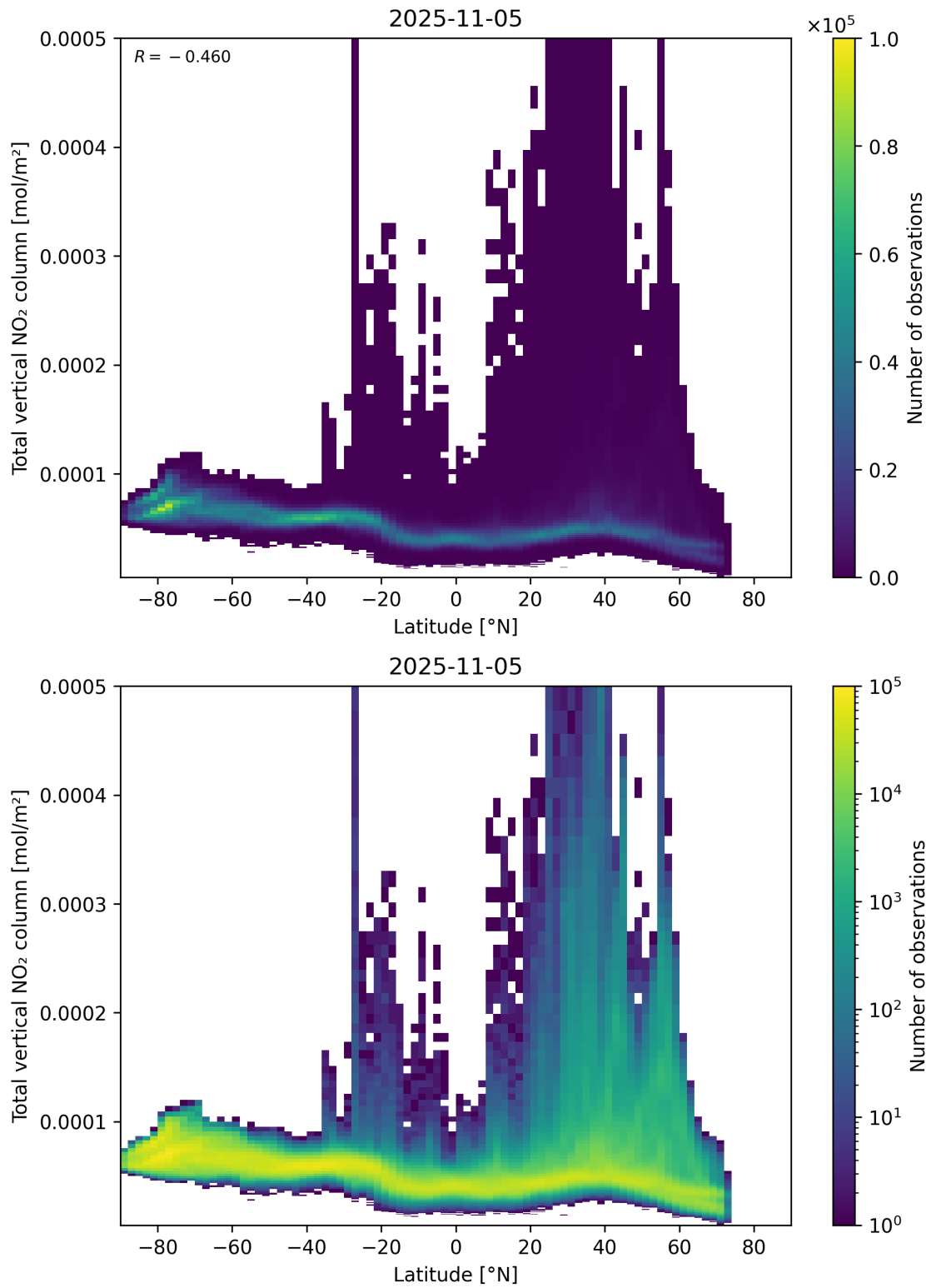
Figure 90: Scatter density plot of “Latitude” against “Total vertical NO 2 column” for 2025-11-04 to 2025-11-06.
