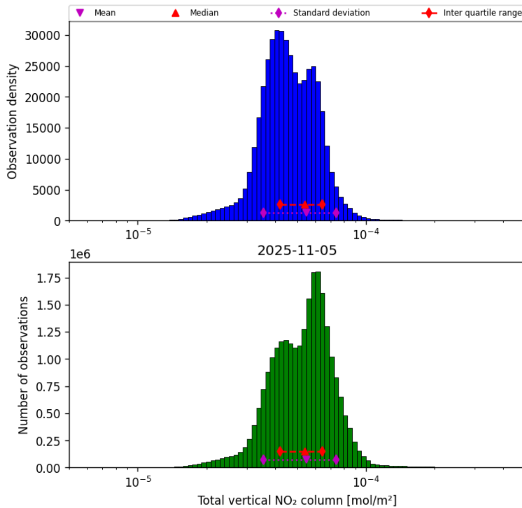
Figure 38: Histogram of “Total vertical NO 2 column” for 2025-11-04 to 2025-11-06
