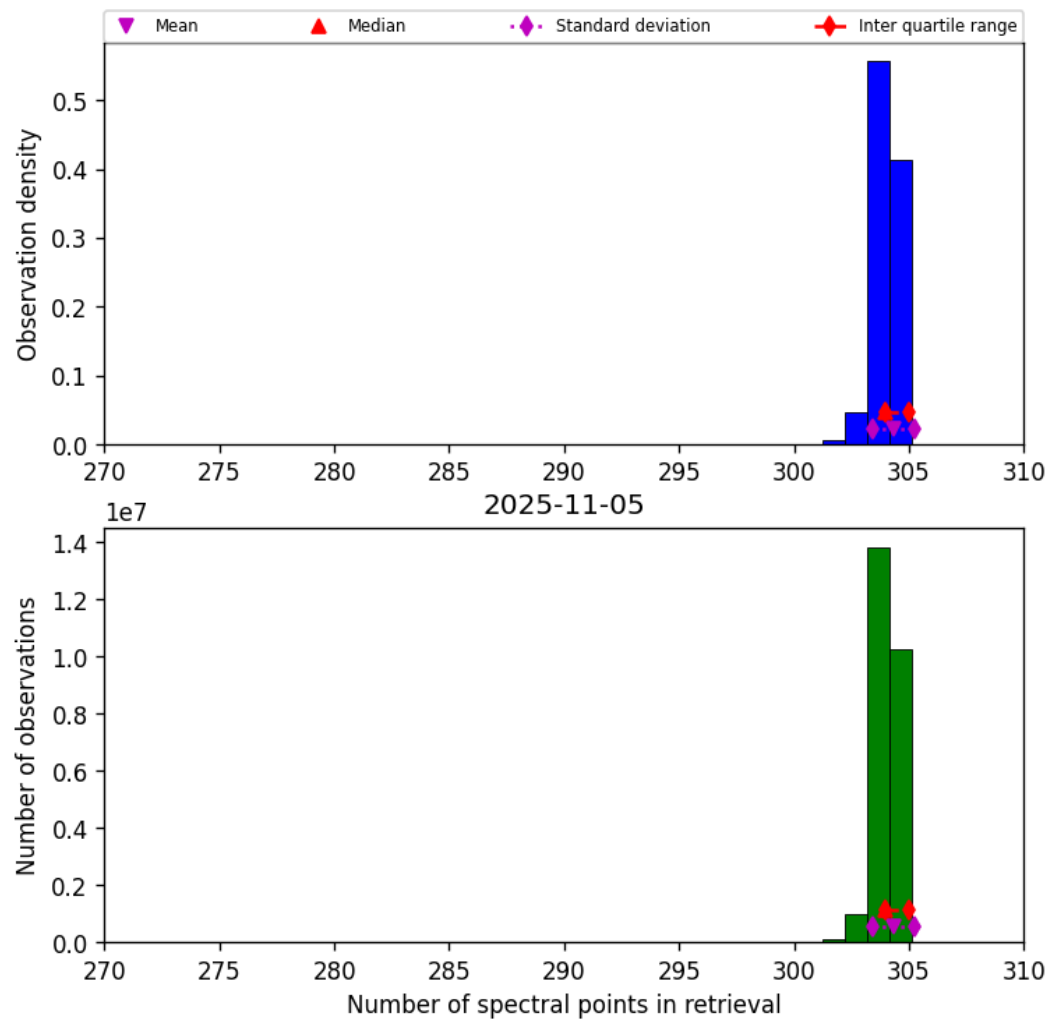
Figure 33: Histogram of “Number of spectral points in retrieval” for 2025-11-04 to 2025-11-06
