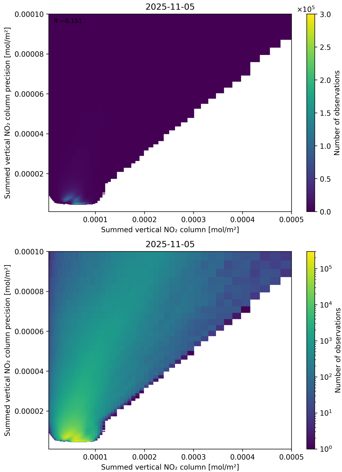
Figure 105: Scatter density plot of “Summed vertical NO 2 column” against “Summed vertical NO 2 column precision” for 2025-11-04 to 2025-11-06.
