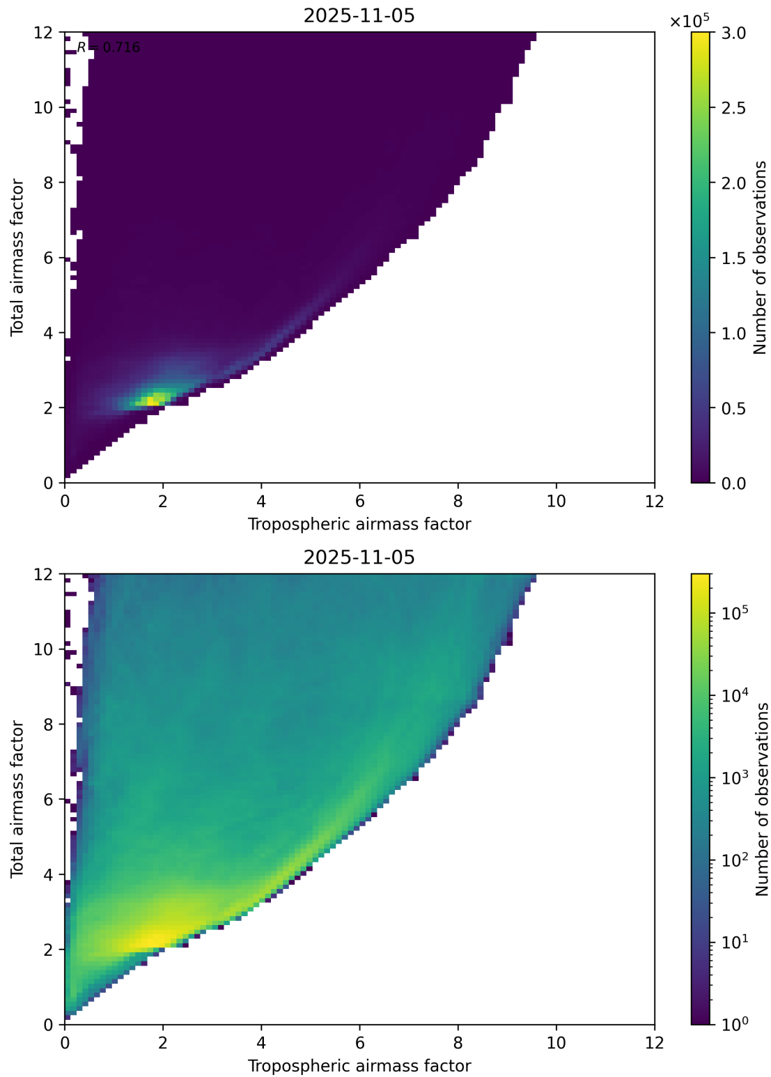
Figure 72: Scatter density plot of “Tropospheric airmass factor” against “Total airmass factor” for 2025-11-04 to 2025-11-06.
