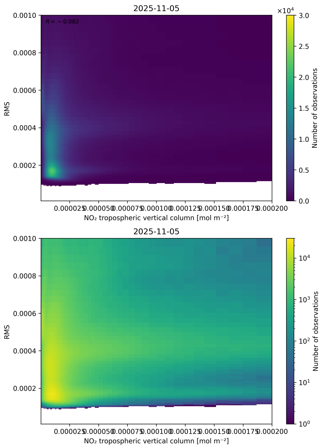
Figure 142: Scatter density plot of “NO 2 tropospheric vertical column” against “RMS” for 2025-11-04 to 2025-11-06.
