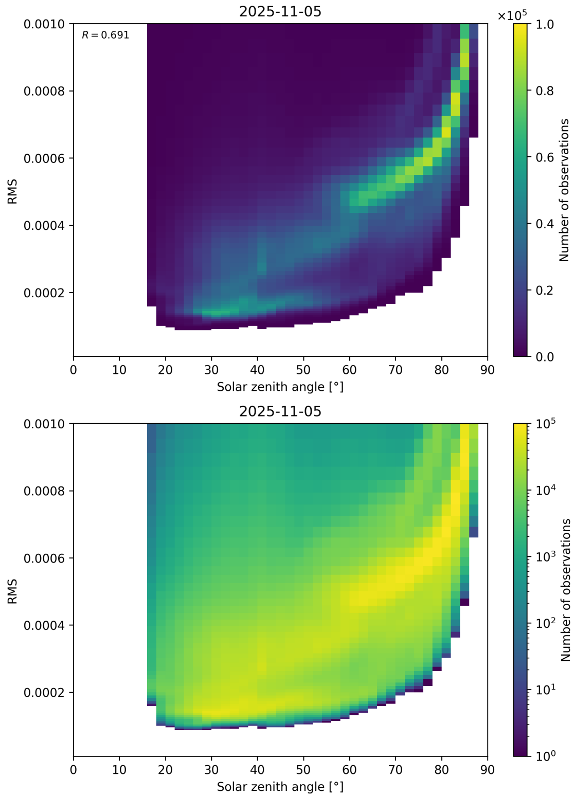
Figure 157: Scatter density plot of “Solar zenith angle” against “RMS” for 2025-11-04 to 2025-11-06.
