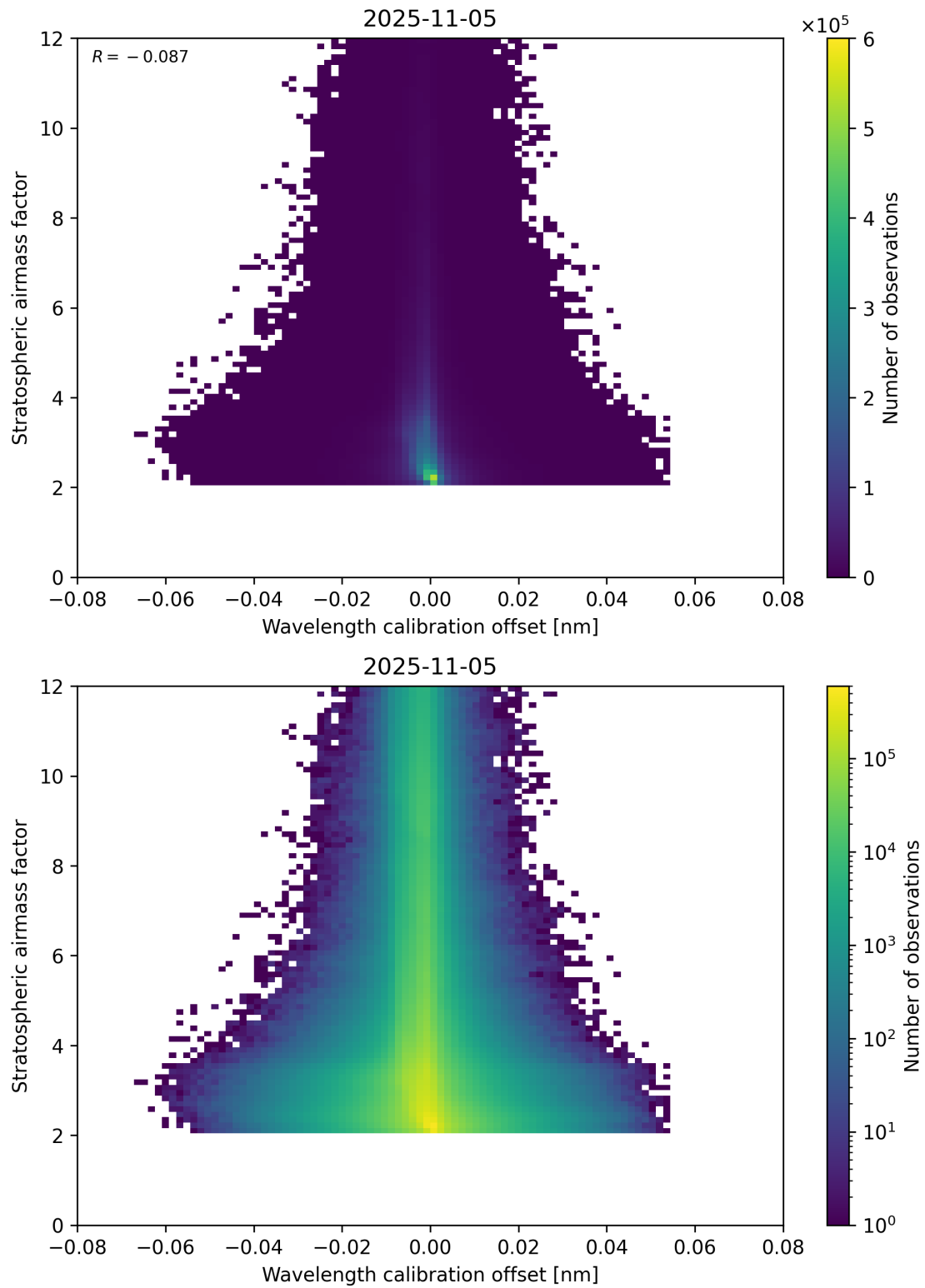
Figure 174: Scatter density plot of “Wavelength calibration offset” against “Stratospheric airmass factor” for 2025-11-04 to 2025-11-06.
