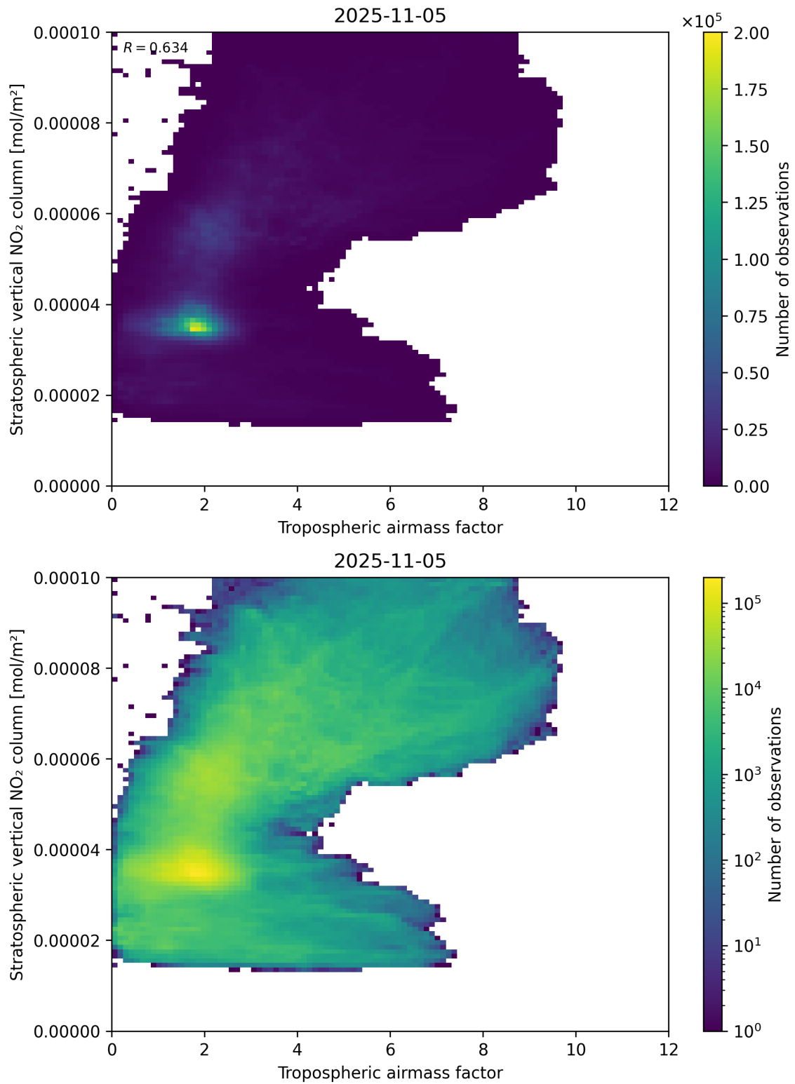
Figure 74: Scatter density plot of “Tropospheric air mass factor” against “Stratospheric vertical NO 2 column” for 2025-11-04 to 2025-11-06.
