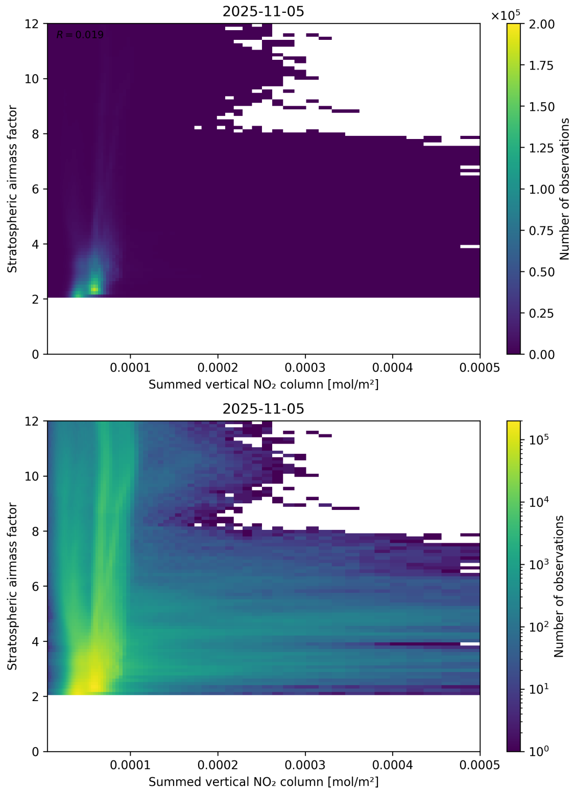
Figure 103: Scatter density plot of “Summed vertical NO 2 column” against “Stratospheric airmass factor” for 2025-11-04 to 2025-11-06.
