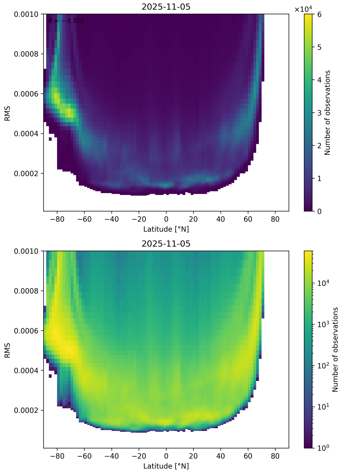
Figure 94: Scatter density plot of “Latitude” against “RMS” for 2025-11-04 to 2025-11-06.
