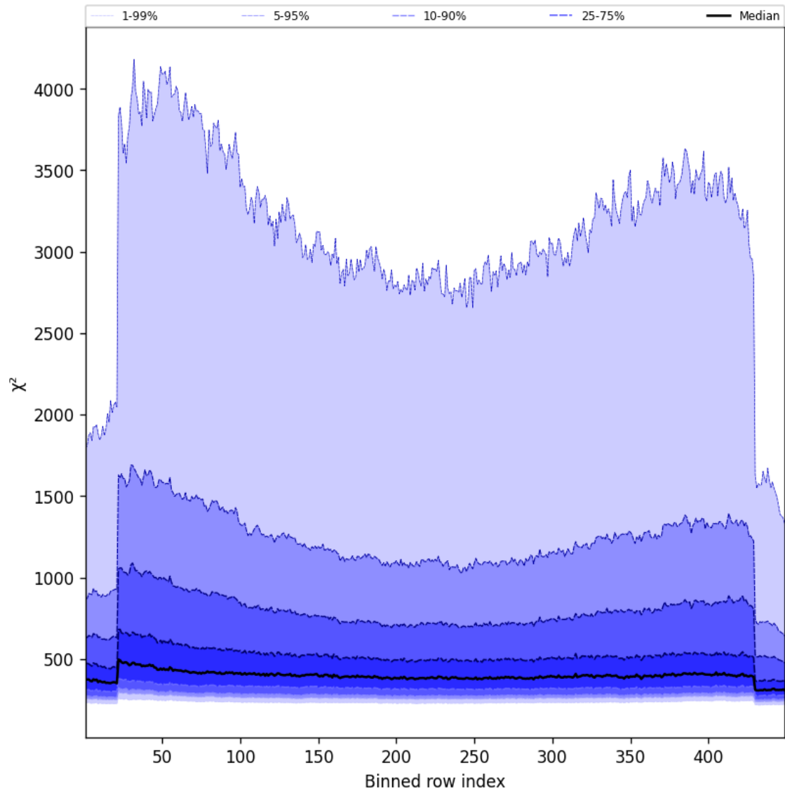
Figure 59: Along track statistics of “ \chi^2 ” for 2025-11-04 to 2025-11-06
