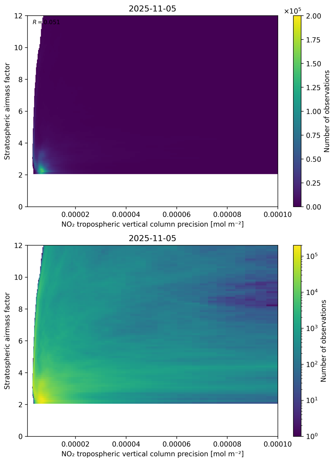
Figure 131: Scatter density plot of “NO 2 tropospheric vertical column precision” against “Stratospheric airmass factor” for 2025-11-04 to 2025-11-06.
