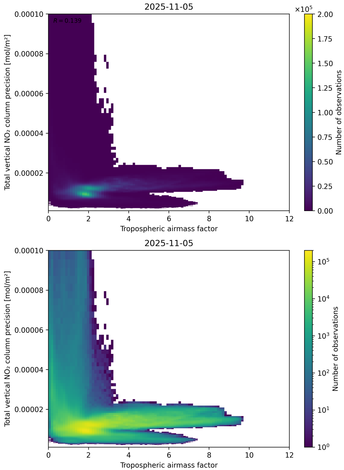
Figure 78: Scatter density plot of “Tropospheric airmass factor” against “Total vertical NO 2 column precision” for 2025-11-04 to 2025-11-06.
