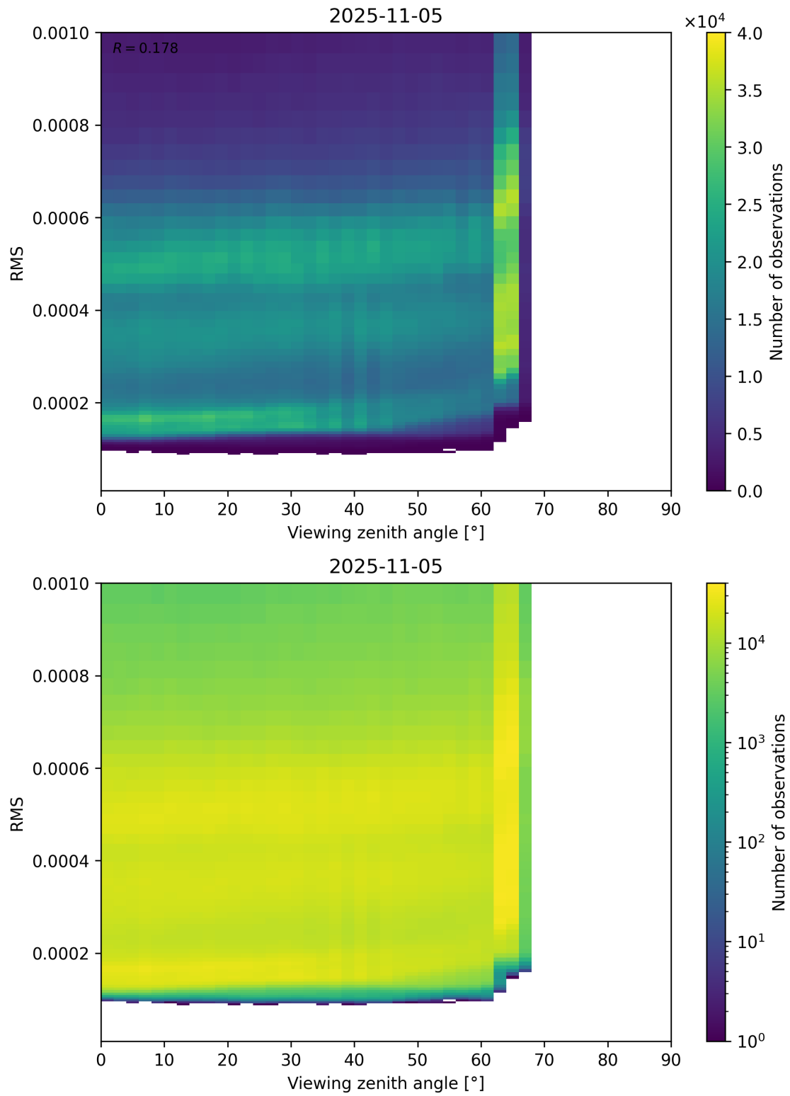
Figure 171: Scatter density plot of “Viewing zenith angle” against “RMS” for 2025-11-04 to 2025-11-06.
