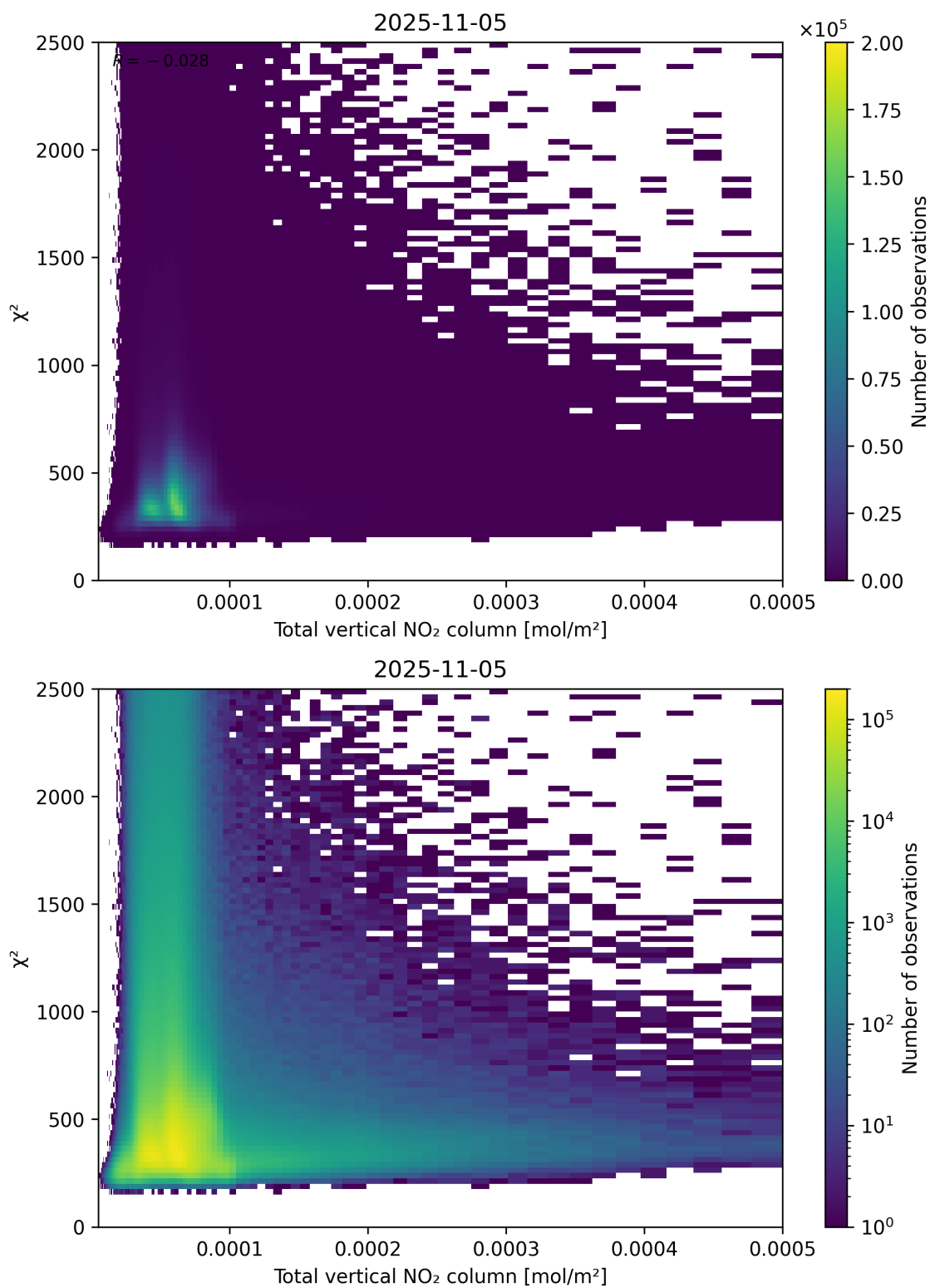
Figure 111: Scatter density plot of “Total vertical NO 2 column” against “ \chi^2 ” for 2025-11-04 to 2025-11-06.
