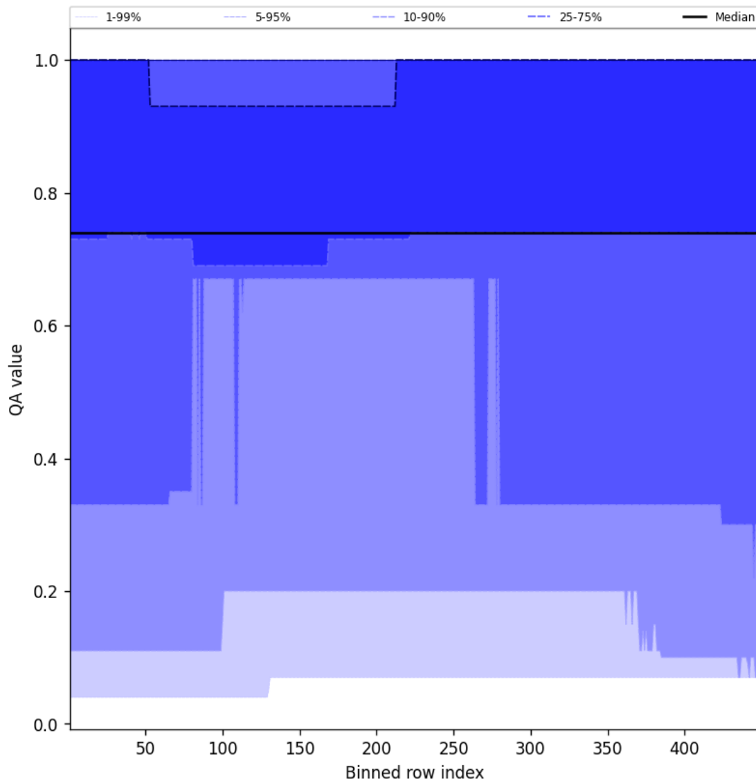
Figure 45: Along track statistics of “QA value” for 2025-11-04 to 2025-11-06
