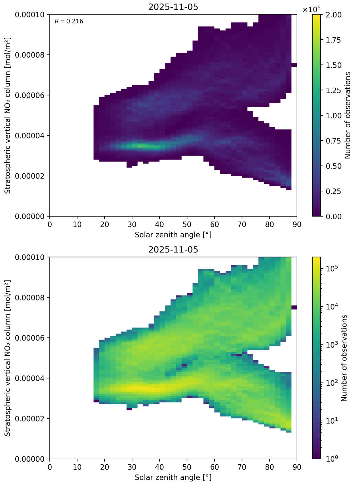
Figure 150: Scatter density plot of “Solar zenith angle” against “Stratospheric vertical NO 2 column” for 2025-11-04 to 2025-11-06.
