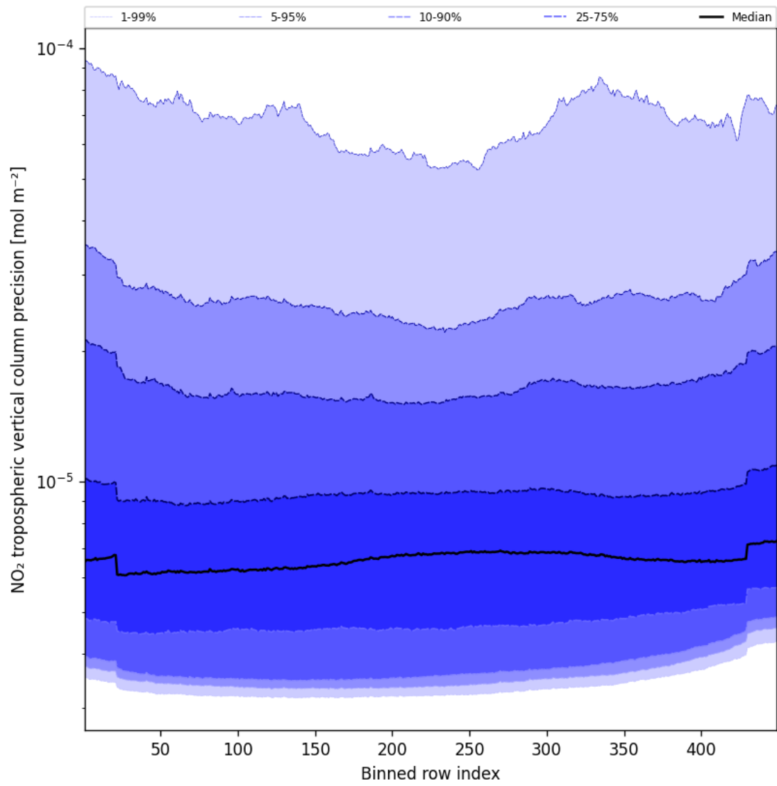
Figure 47: Along track statistics of “NO 2 tropospheric vertical column precision” for 2025-11-04 to 2025-11-06
