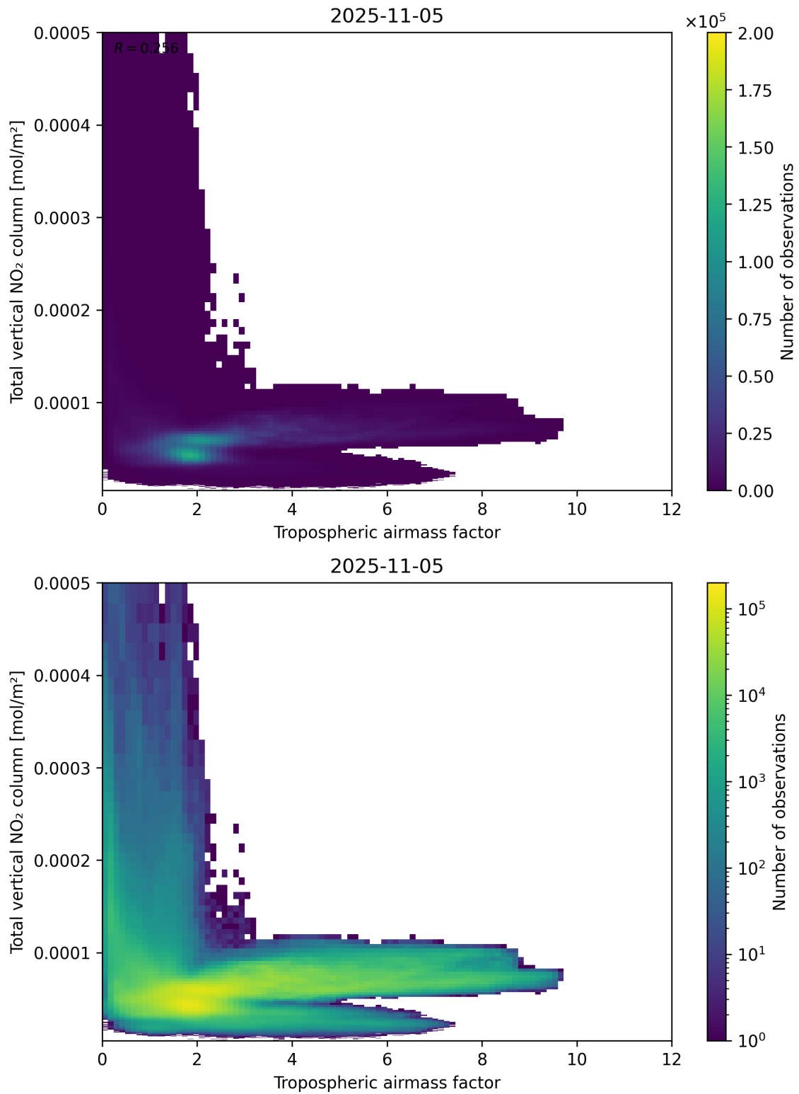
Figure 77: Scatter density plot of “Tropospheric airmass factor” against “Total vertical NO 2 column” for 2025-11-04 to 2025-11-06.
