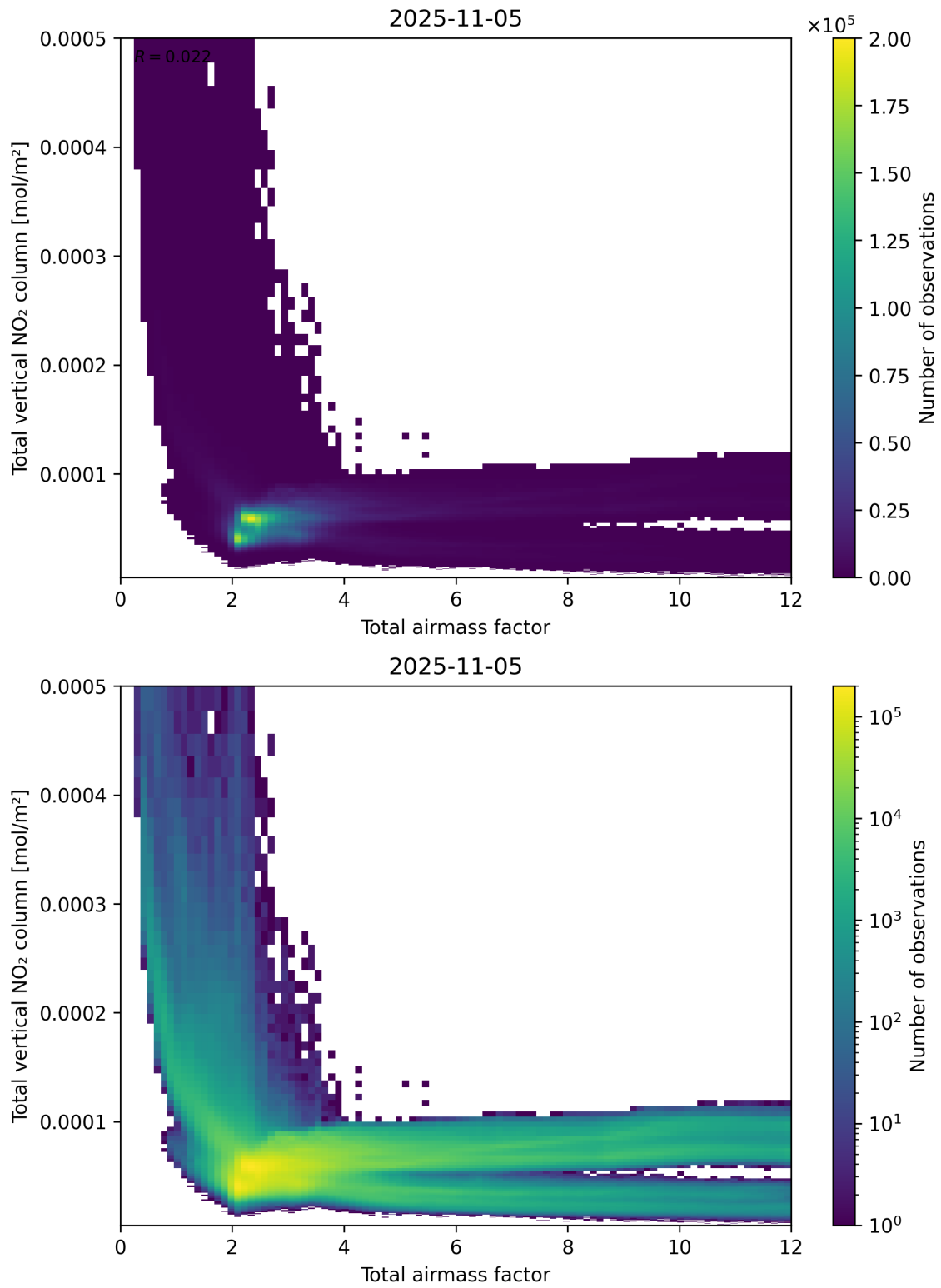
Figure 67: Scatter density plot of “Total airmass factor” against “Total vertical NO 2 column” for 2025-11-04 to 2025-11-06.
