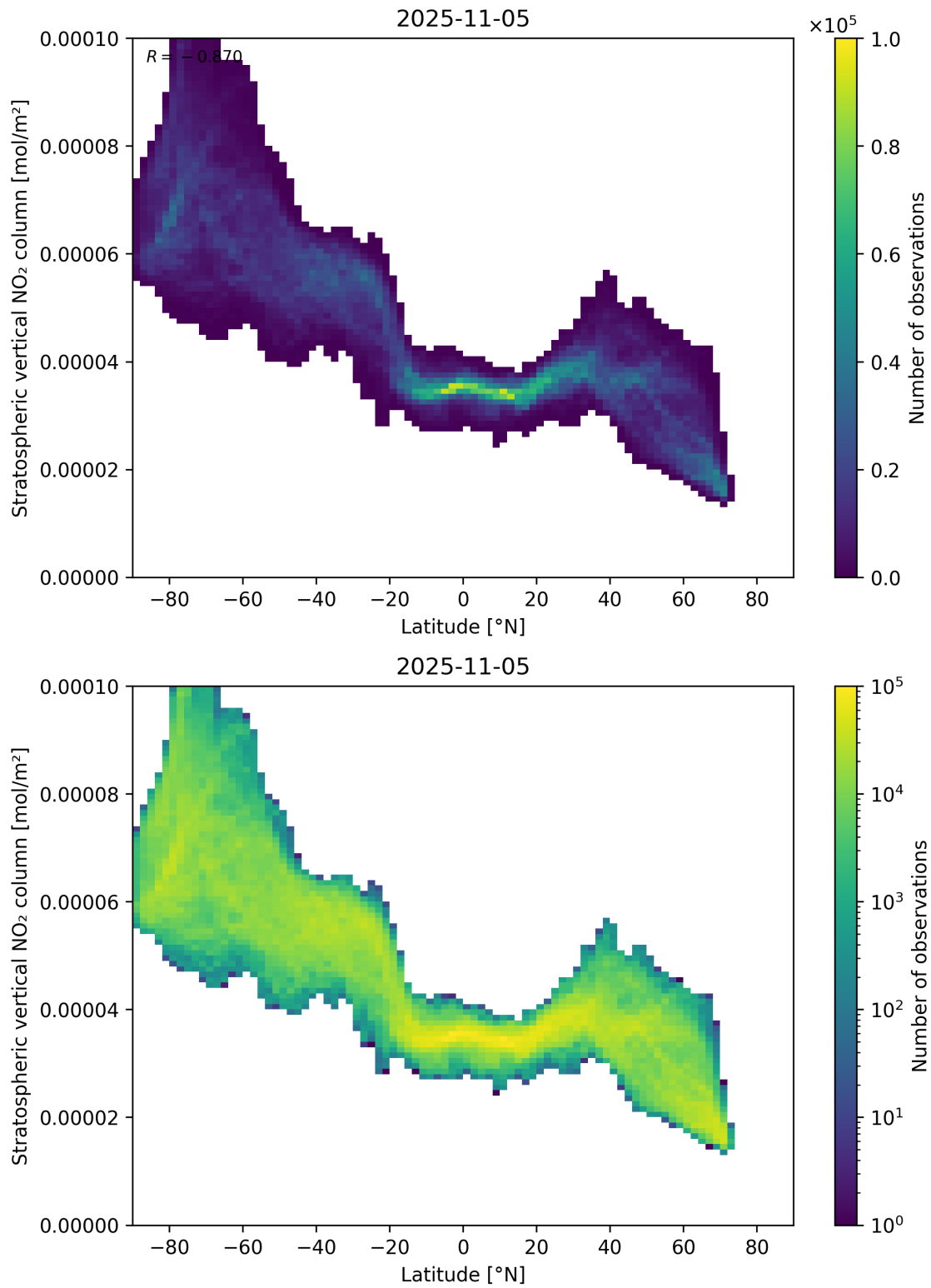
Figure 87: Scatter density plot of “Latitude” against “Stratospheric vertical NO 2 column” for 2025-11-04 to 2025-11-06.
