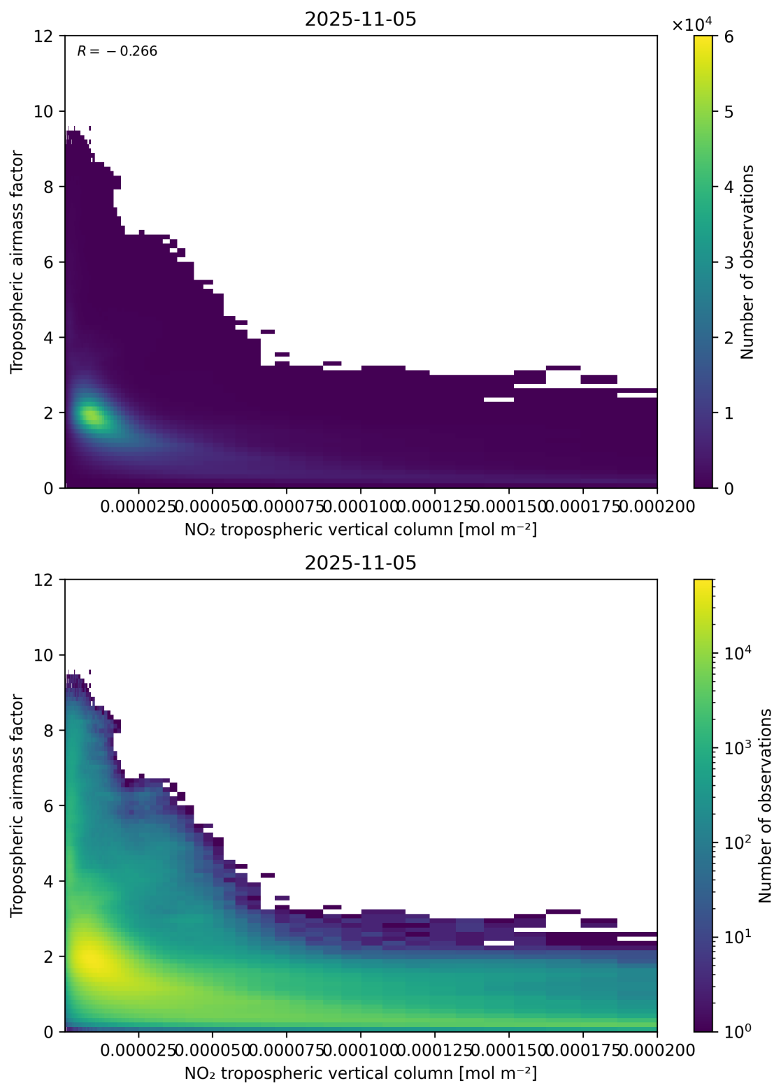
Figure 123: Scatter density plot of “NO 2 tropospheric vertical column” against “Tropospheric air mass factor” for 2025-11-04 to 2025-11-06.
