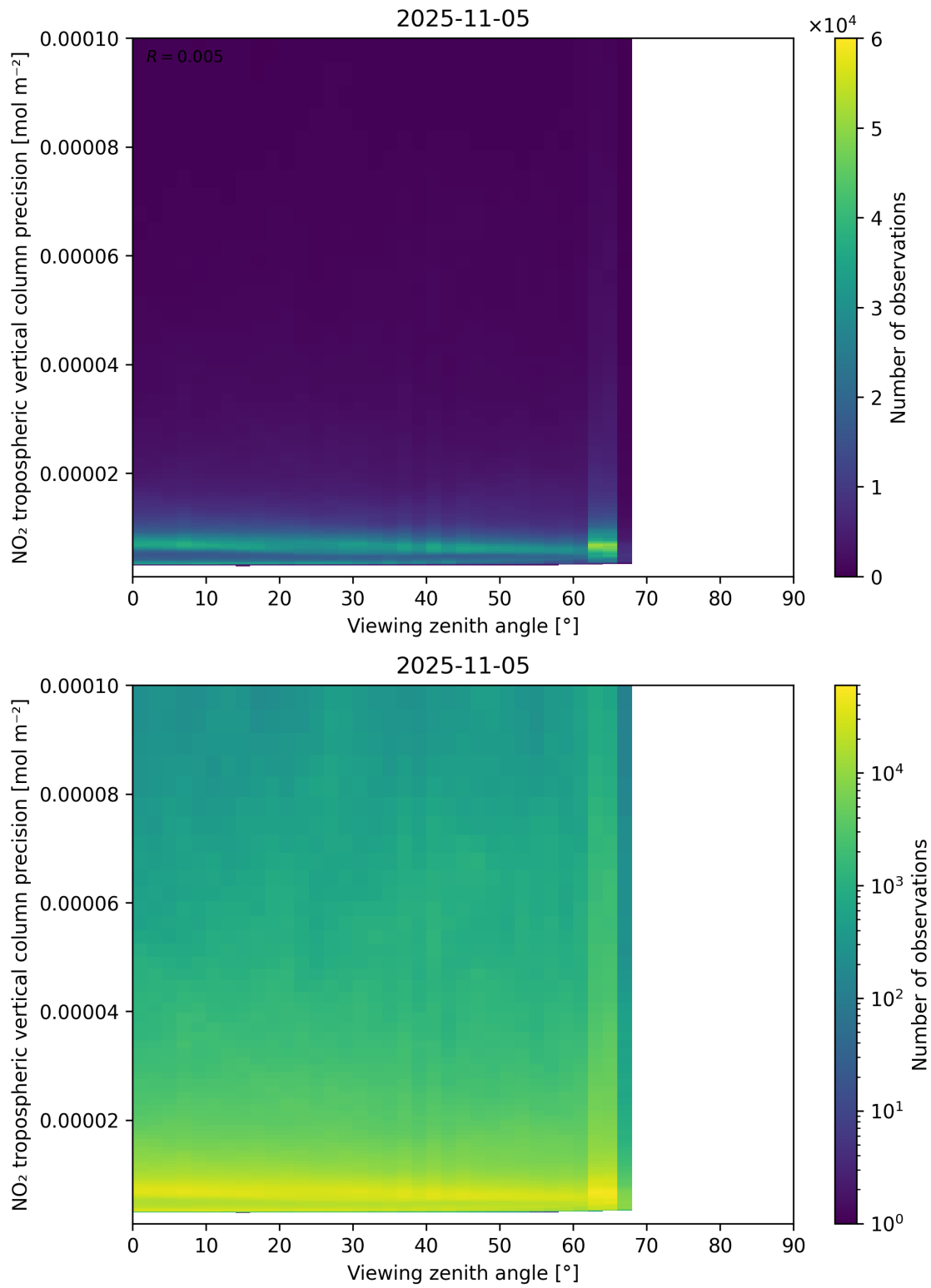
Figure 170: Scatter density plot of “Viewing zenith angle” against “NO 2 tropospheric vertical column precision” for 2025-11-04 to 2025-11-06.
