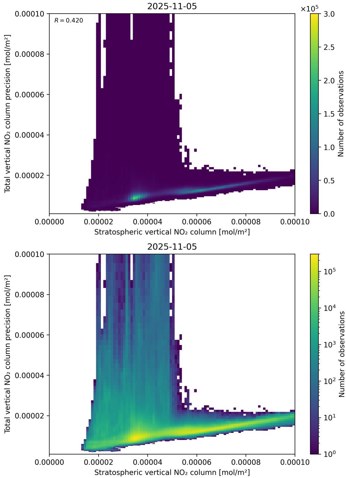
Figure 101: Scatter density plot of “Stratospheric vertical NO 2 column” against “Total vertical NO 2 column precision” for 2025-11-04 to 2025-11-06.
