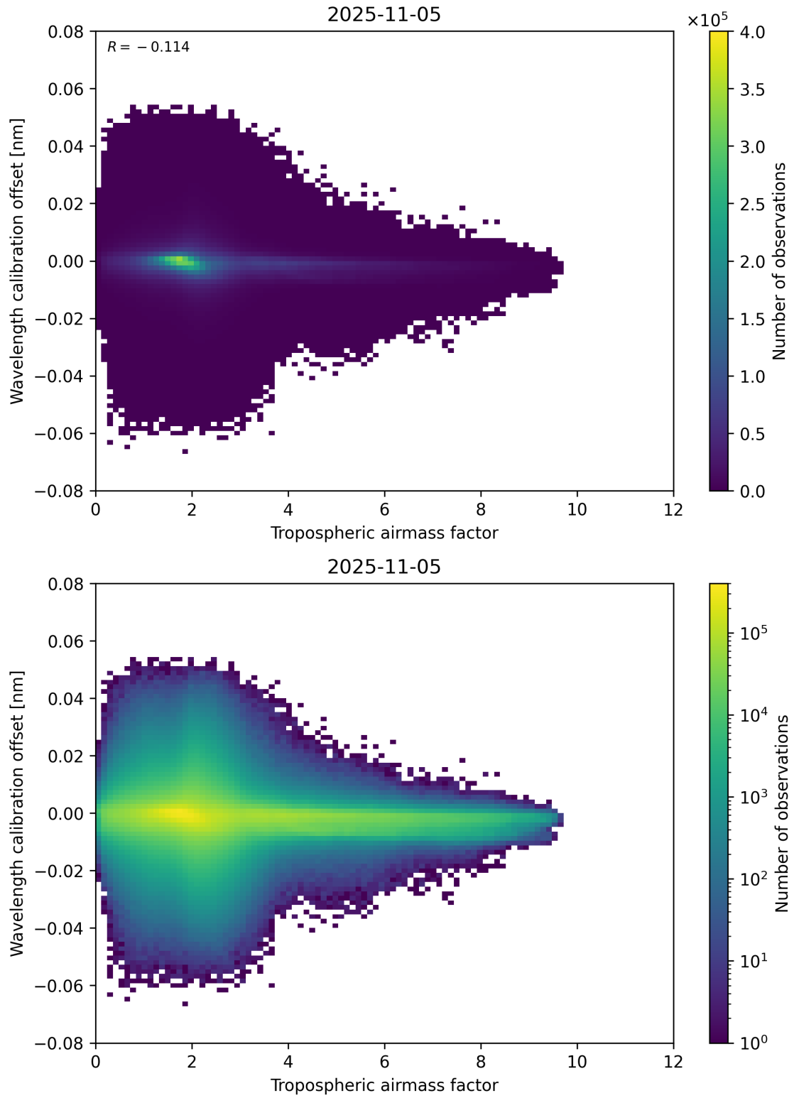
Figure 80: Scatter density plot of “Tropospheric airmass factor” against “Wavelength calibration offset” for 2025-11-04 to 2025-11-06.
