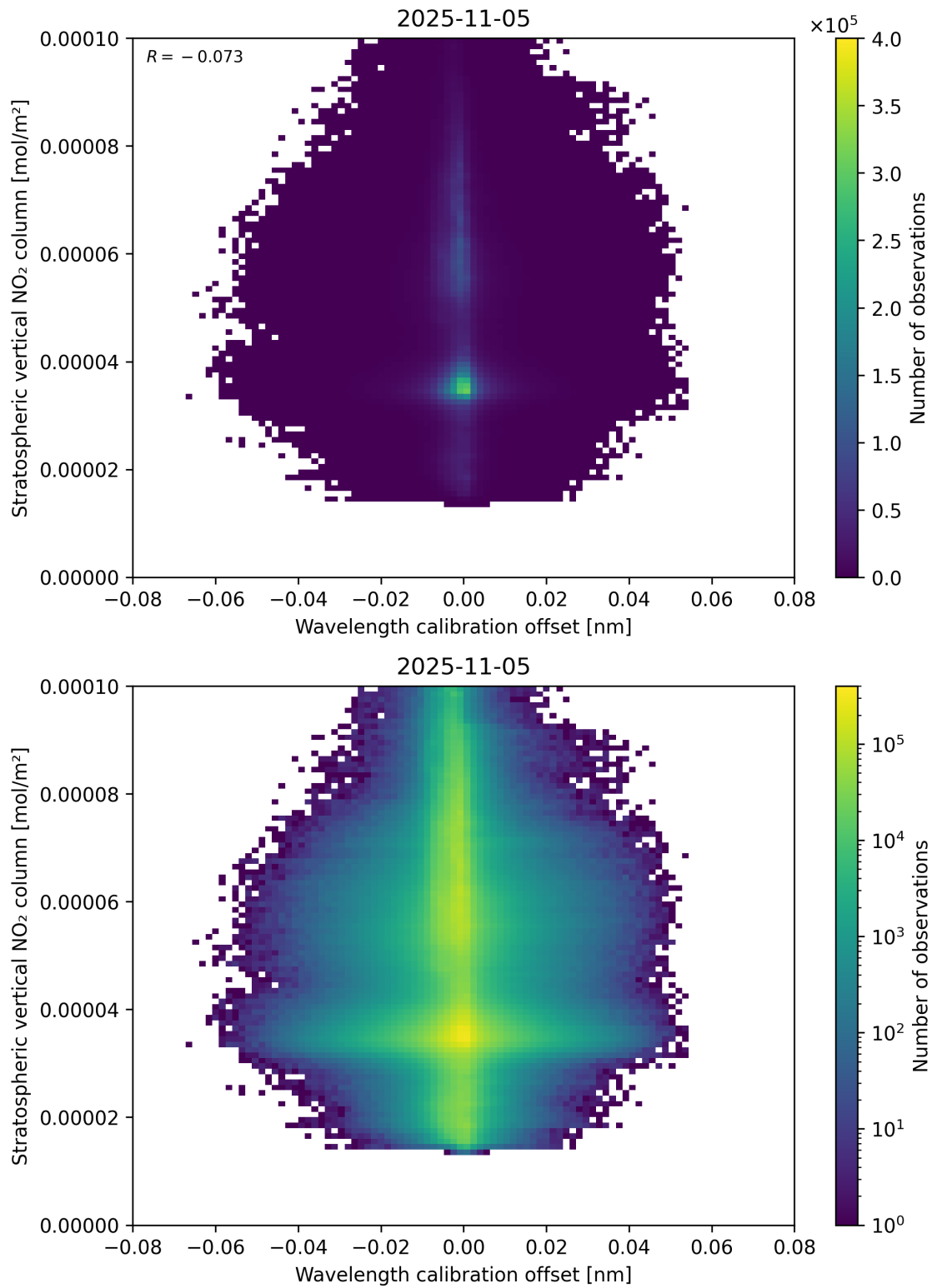
Figure 176: Scatter density plot of “Wavelength calibration offset” against “Stratospheric vertical NO 2 column” for 2025-11-04 to 2025-11-06.
