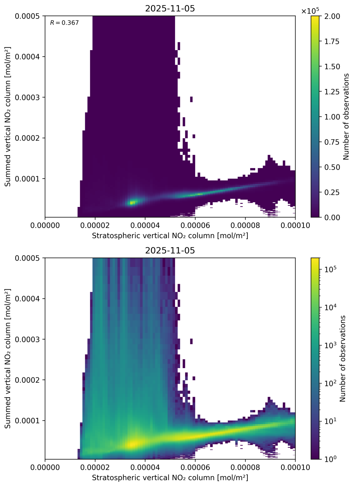
Figure 98: Scatter density plot of “Stratospheric vertical NO 2 column” against “Summed vertical NO 2 column” for 2025-11-04 to 2025-11-06.
