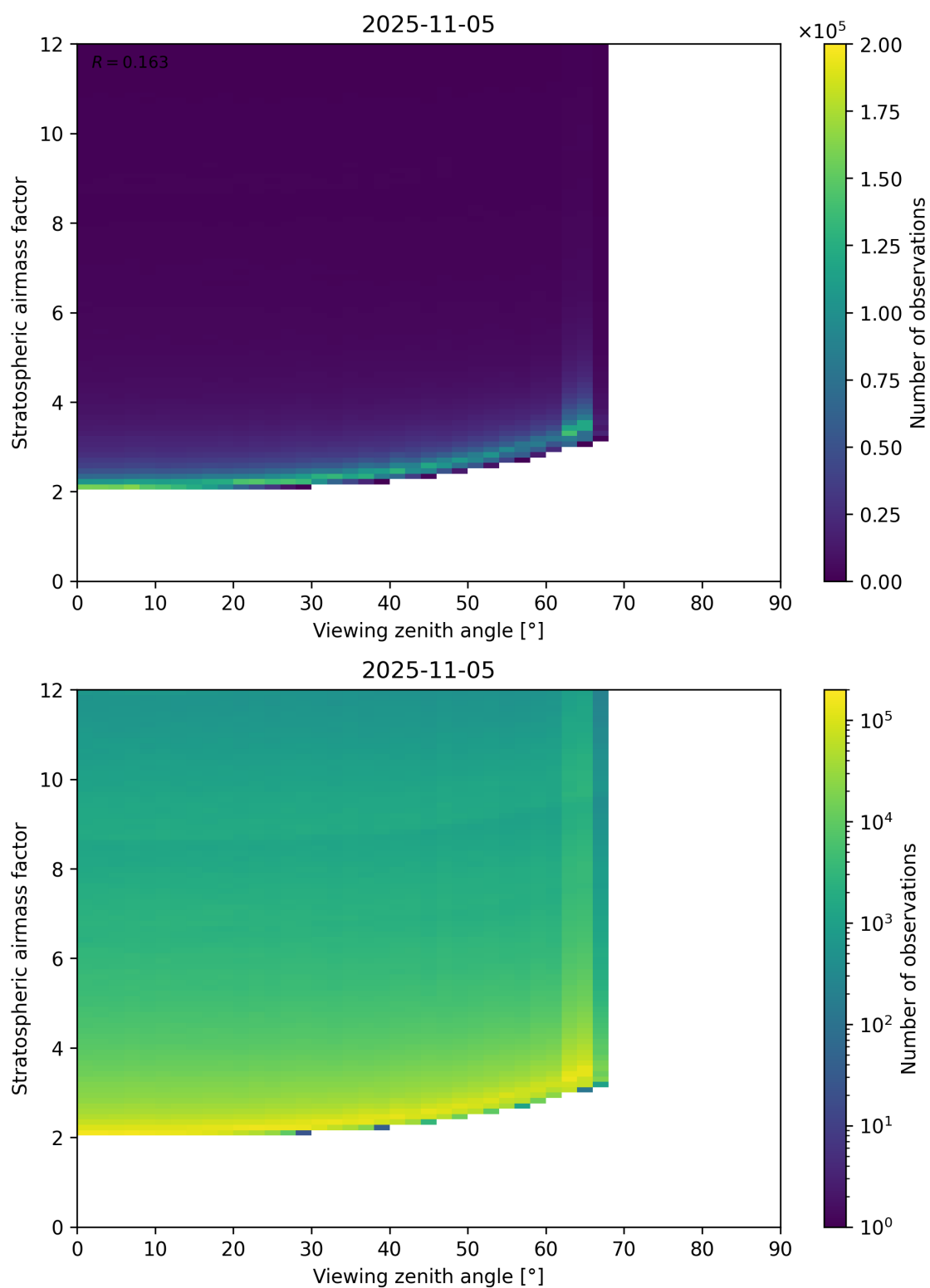
Figure 159: Scatter density plot of “Viewing zenith angle” against “Stratospheric airmass factor” for 2025-11-04 to 2025-11-06.
