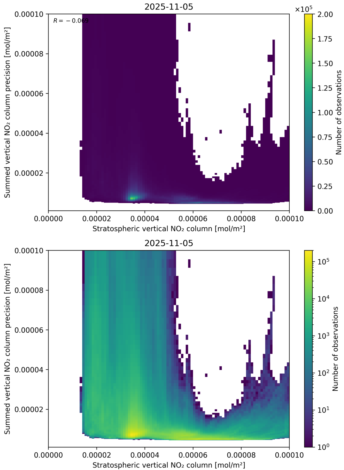
Figure 99: Scatter density plot of “Stratospheric vertical NO 2 column” against “Summed vertical NO 2 column precision” for 2025-11-04 to 2025-11-06.
