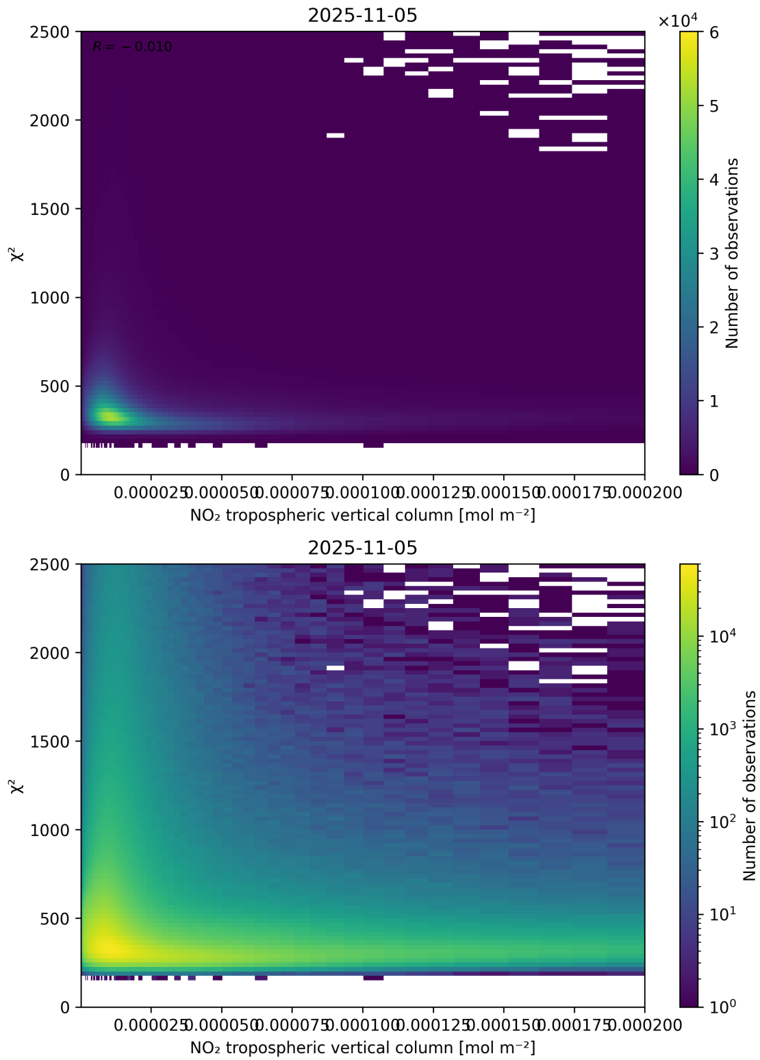
Figure 124: Scatter density plot of “NO 2 tropospheric vertical column” against “ \chi^2 ” for 2025-11-04 to 2025-11-06.
