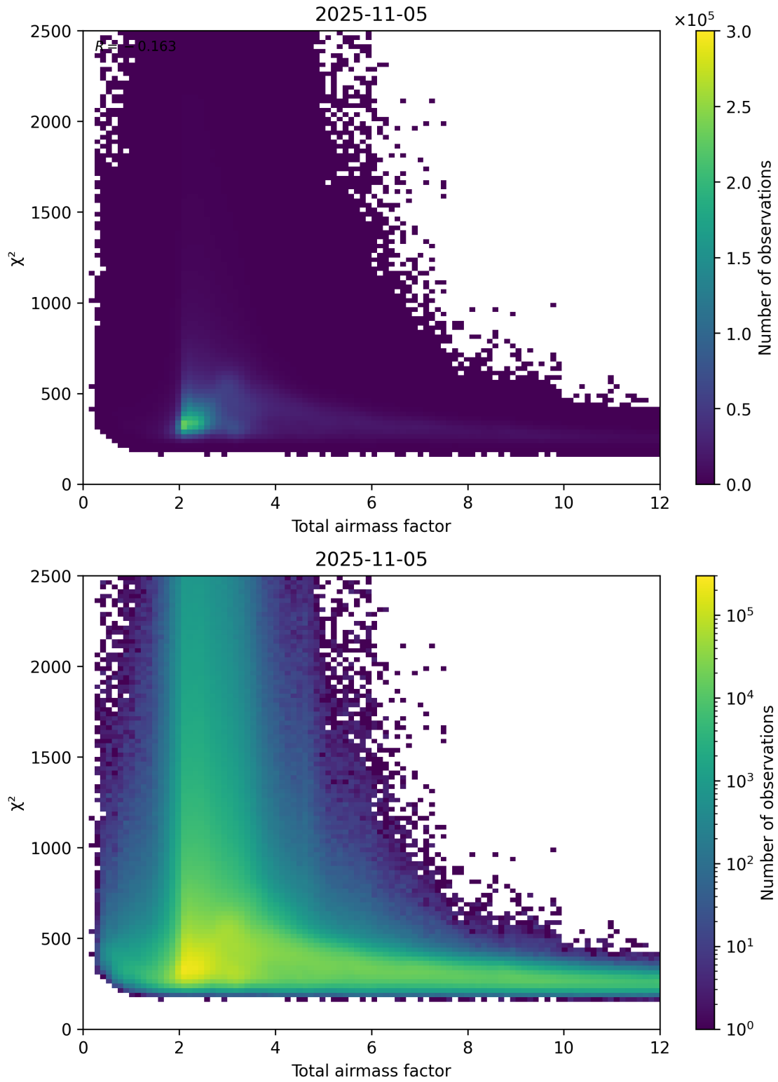
Figure 63: Scatter density plot of “Total airmass factor” against “ \chi^2 ” for 2025-11-04 to 2025-11-06.
