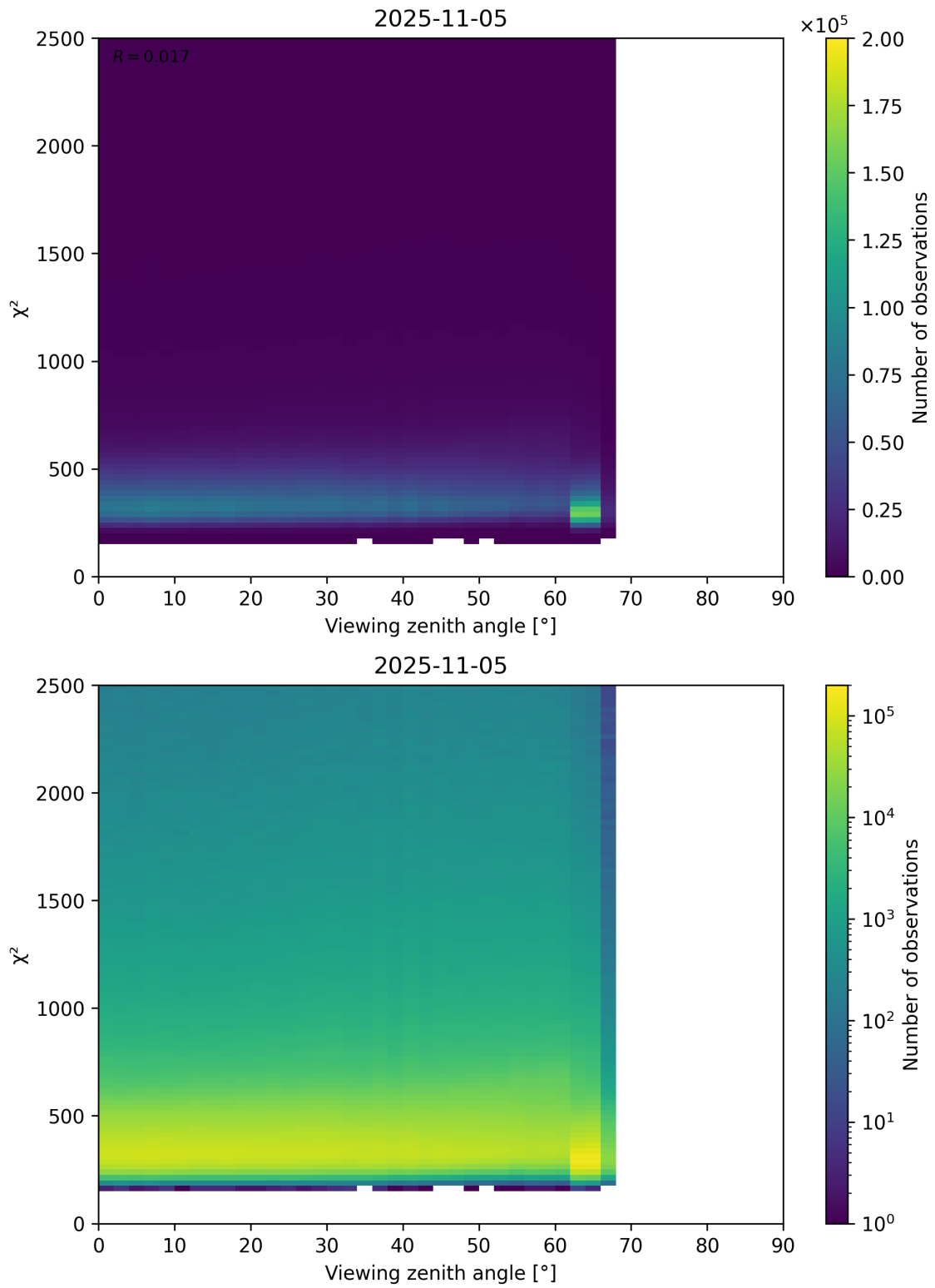
Figure 162: Scatter density plot of “Viewing zenith angle” against “ \chi^2 ” for 2025-11-04 to 2025-11-06.
