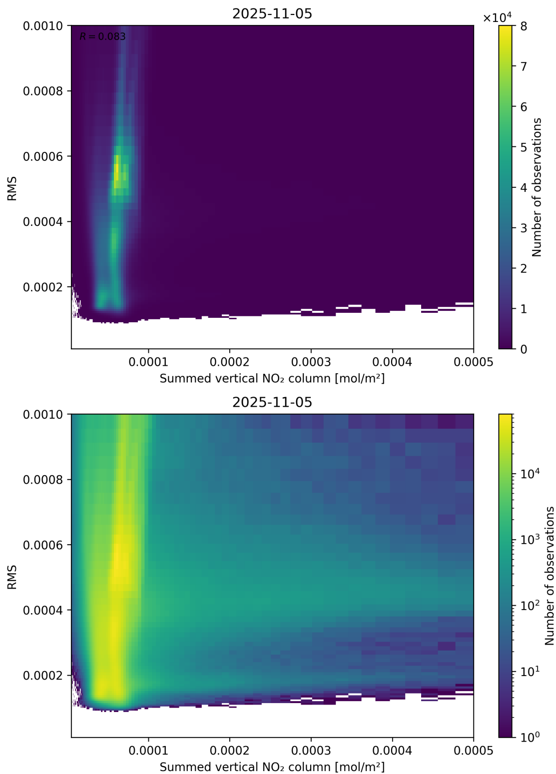
Figure 109: Scatter density plot of “Summed vertical NO 2 column” against “RMS” for 2025-11-04 to 2025-11-06.
