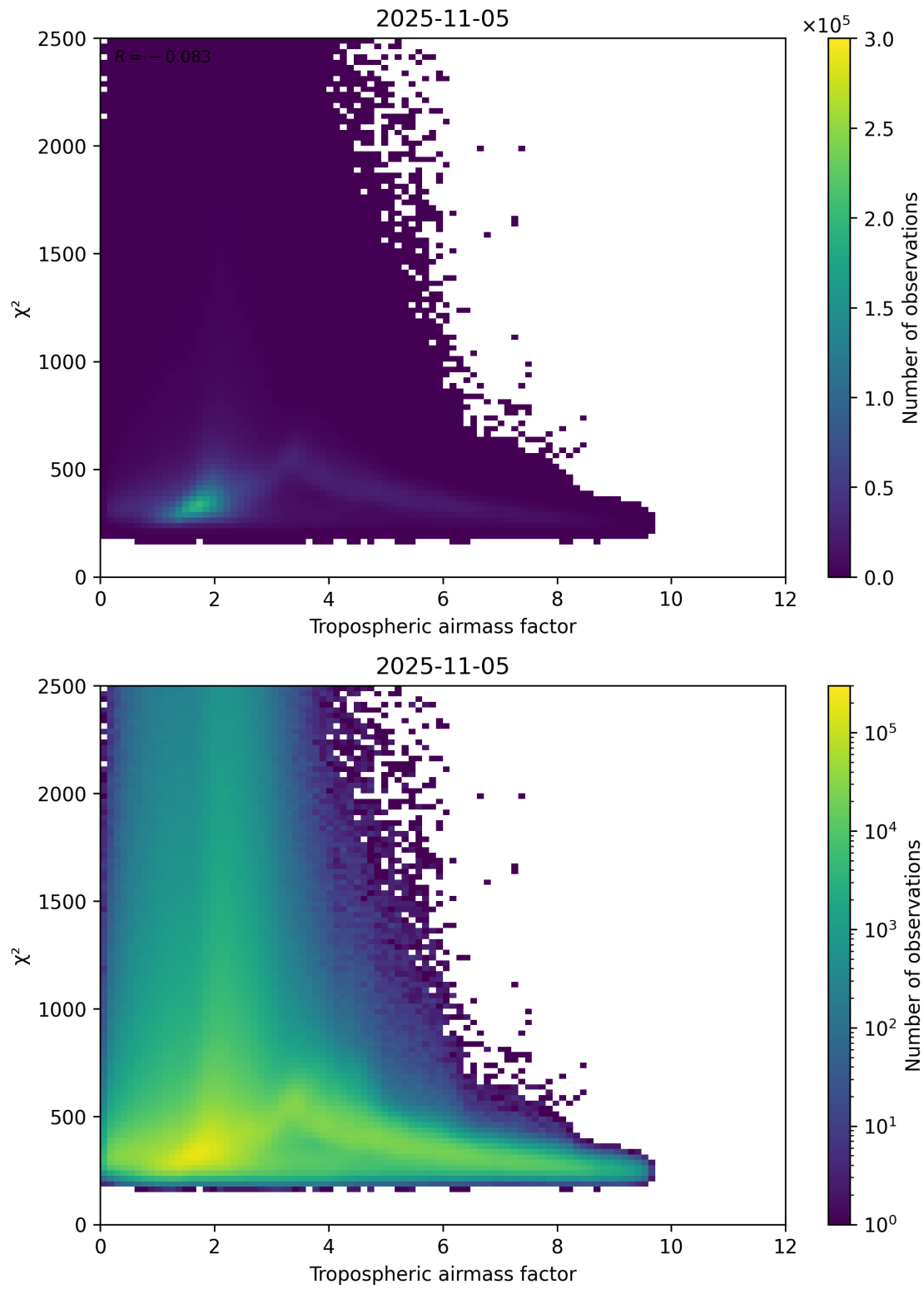
Figure 73: Scatter density plot of “Tropospheric airmass factor” against “ \chi^2 ” for 2025-11-04 to 2025-11-06.
