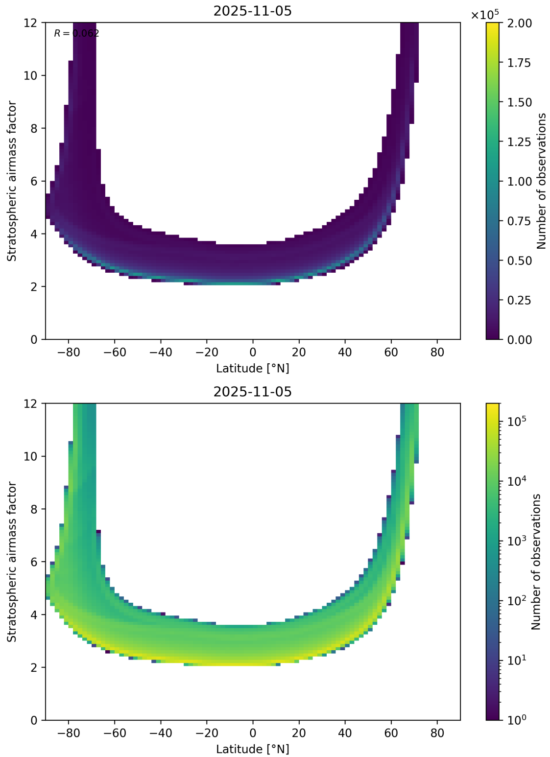
Figure 83: Scatter density plot of “Latitude” against “Stratospheric air mass factor” for 2025-11-04 to 2025-11-06.
