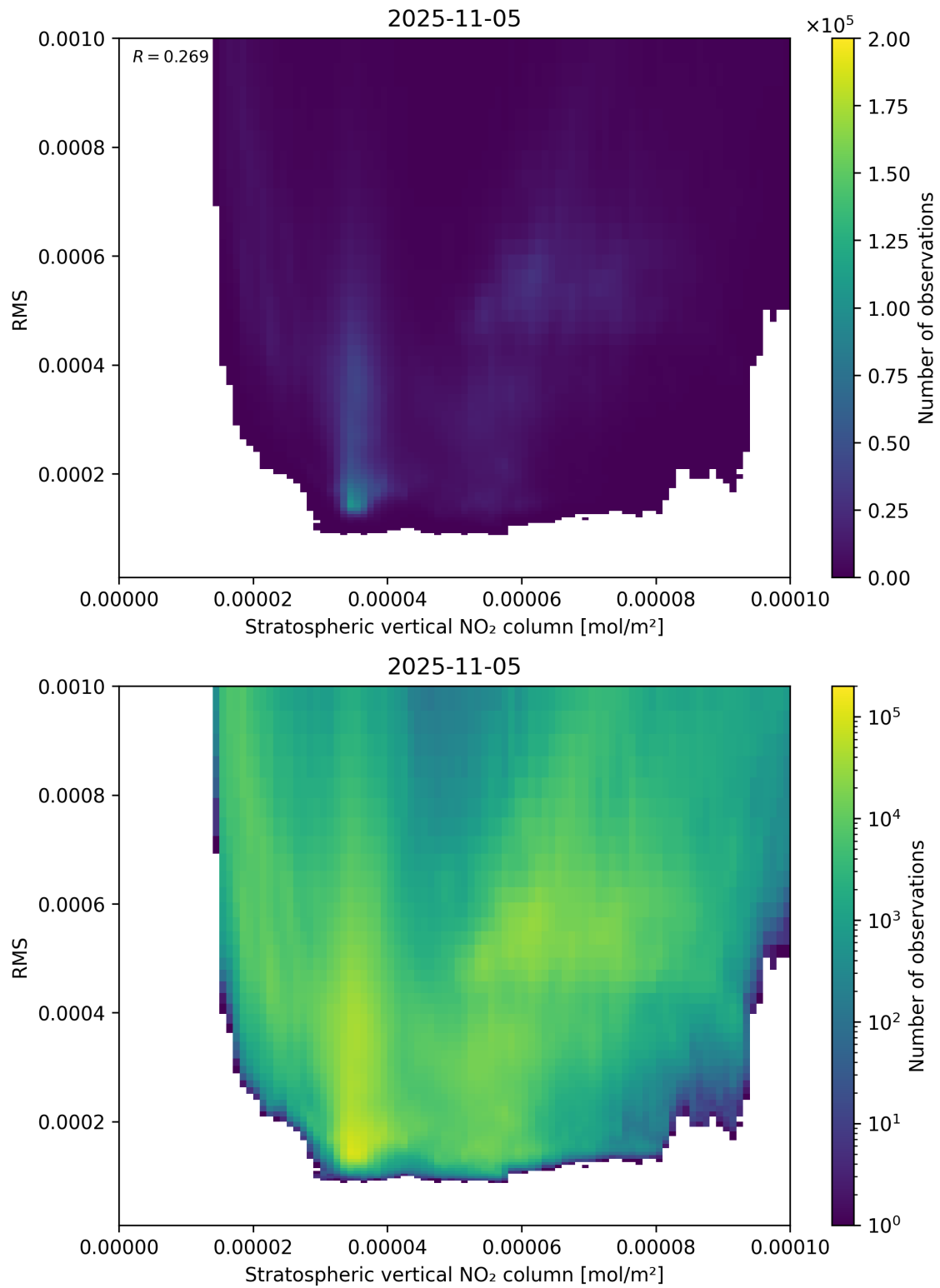
Figure 102: Scatter density plot of “Stratospheric vertical NO 2 column” against “RMS” for 2025-11-04 to 2025-11-06.
