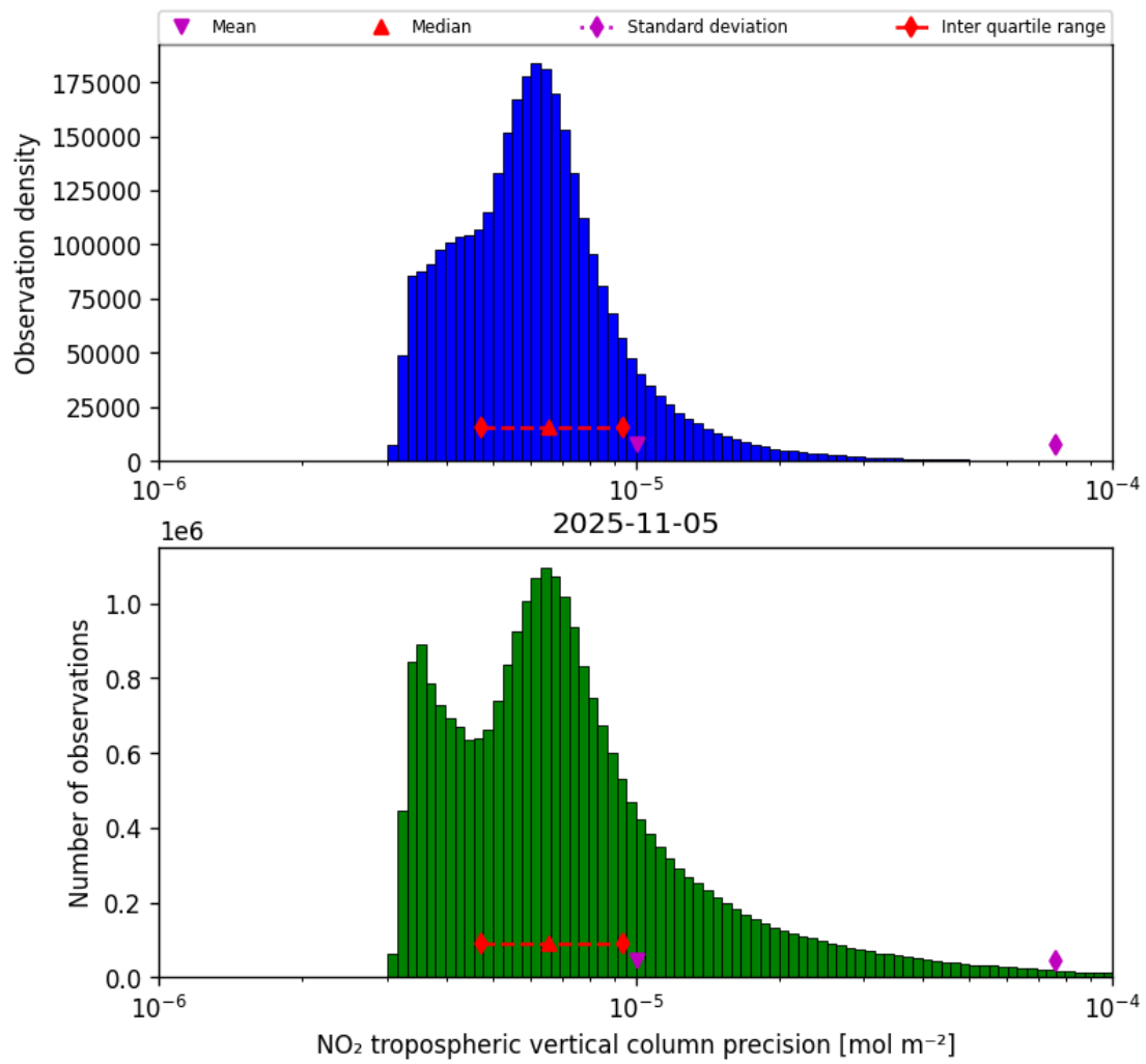
Figure 30: Histogram of “NO 2 tropospheric vertical column precision” for 2025-11-04 to 2025-11-06
