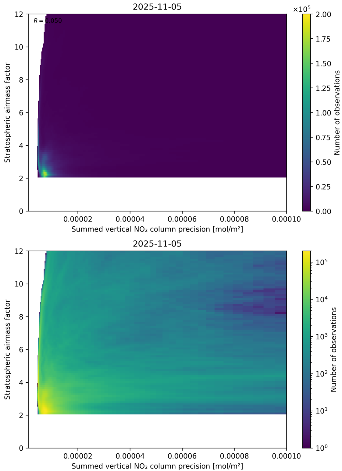
Figure 106: Scatter density plot of “Summed vertical NO 2 column precision” against “Stratospheric airmass factor” for 2025-11-04 to 2025-11-06.
