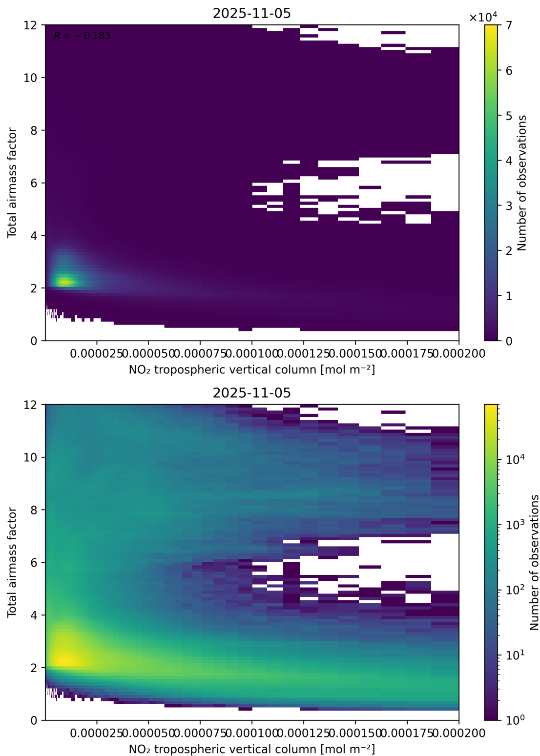
Figure 122: Scatter density plot of “NO 2 tropospheric vertical column” against “Total air mass factor” for 2025-11-04 to 2025-11-06.
