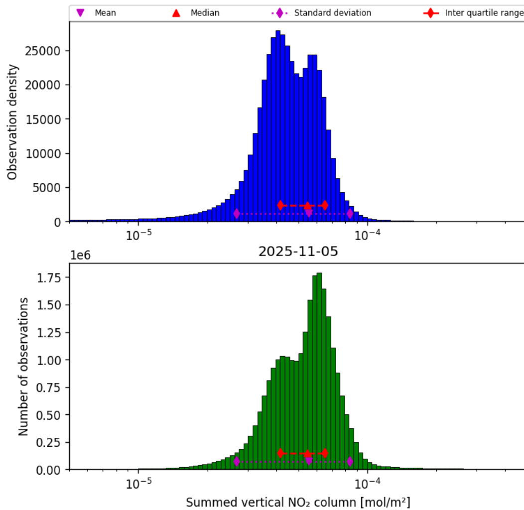
Figure 40: Histogram of “Summed vertical NO 2 column” for 2025-11-04 to 2025-11-06
