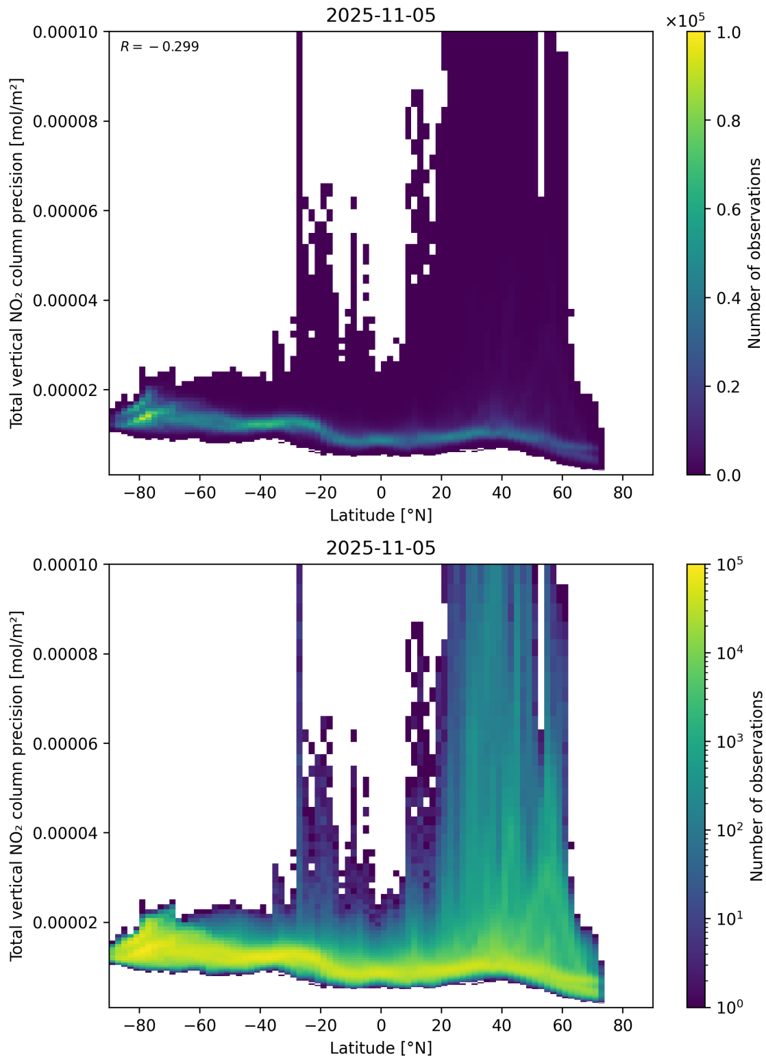
Figure 91: Scatter density plot of “Latitude” against “Total vertical NO 2 column precision” for 2025-11-04 to 2025-11-06.
