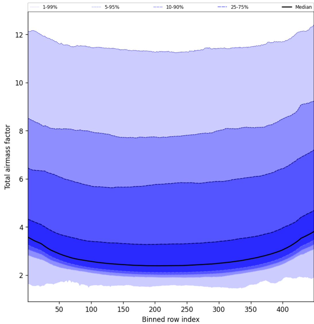
Figure 49: Along track statistics of “Total airmass factor” for 2025-11-04 to 2025-11-06
