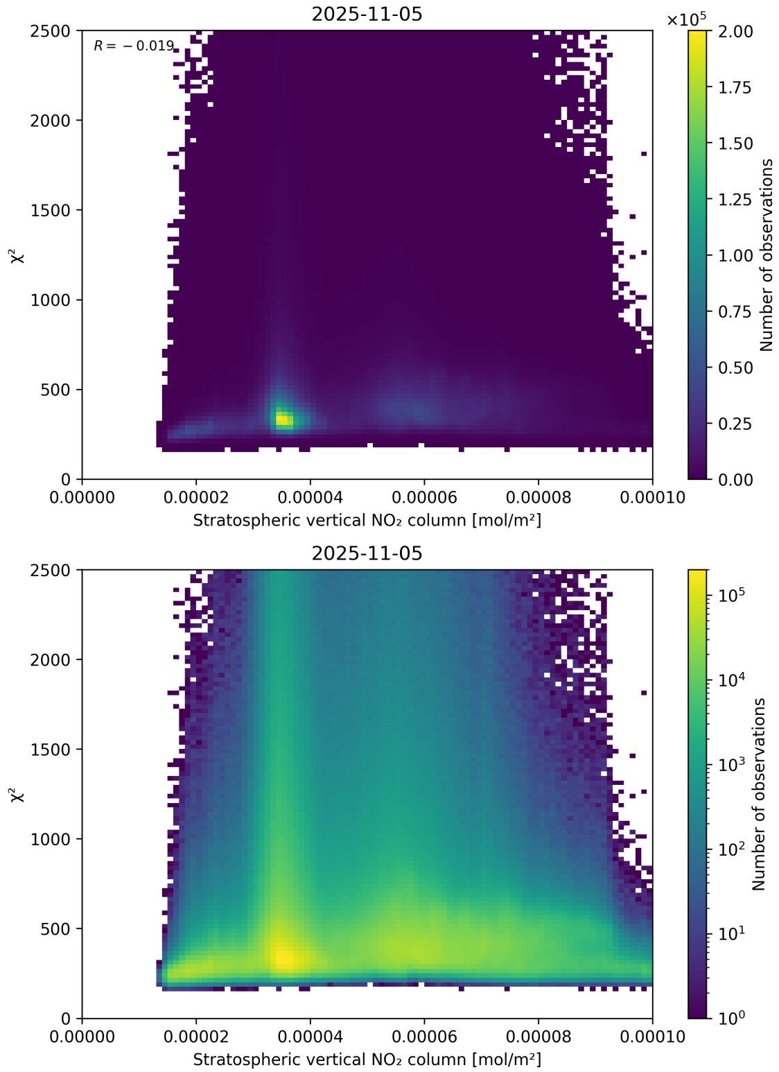
Figure 97: Scatter density plot of “Stratospheric vertical NO 2 column” against “ \chi^2 ” for 2025-11-04 to 2025-11-06.
