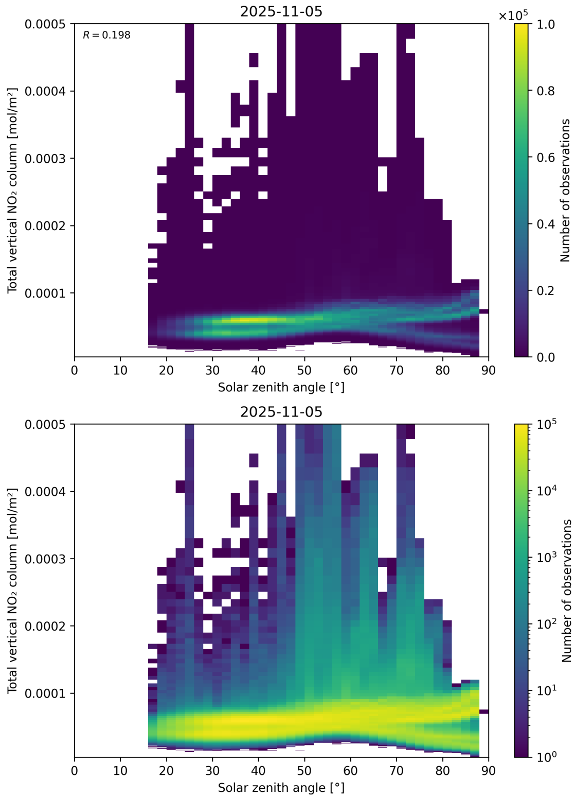
Figure 153: Scatter density plot of “Solar zenith angle” against “Total vertical NO 2 column” for 2025-11-04 to 2025-11-06.
