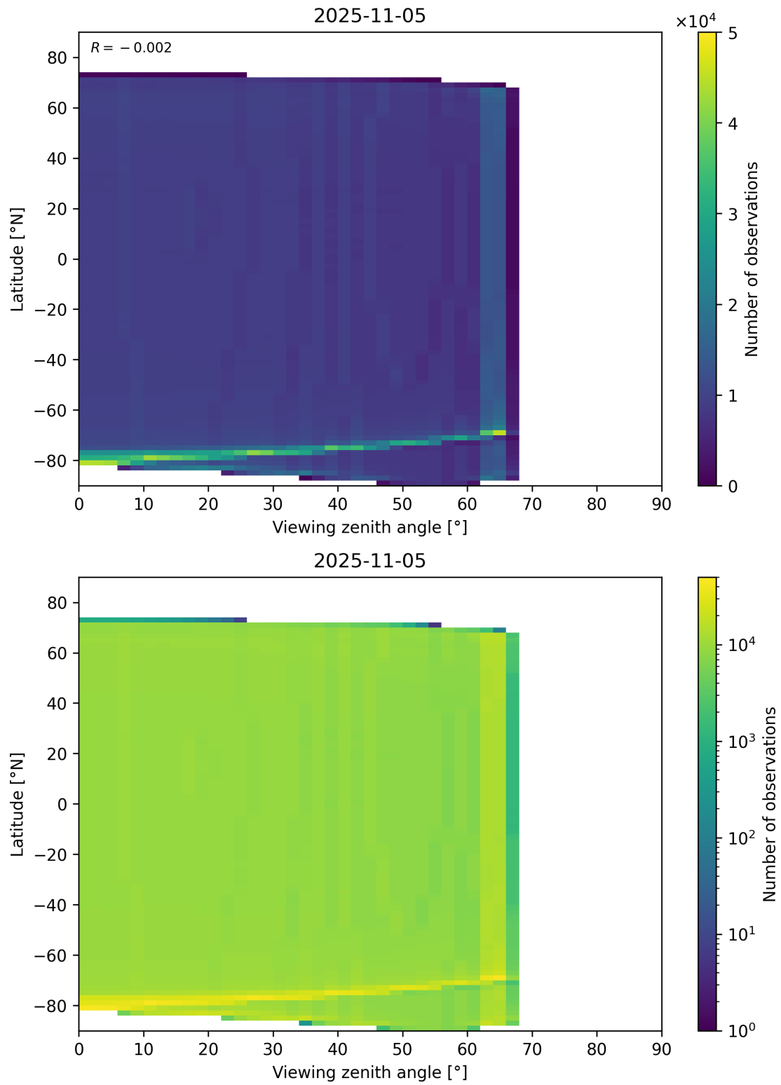
Figure 163: Scatter density plot of “Viewing zenith angle” against “Latitude” for 2025-11-04 to 2025-11-06.
