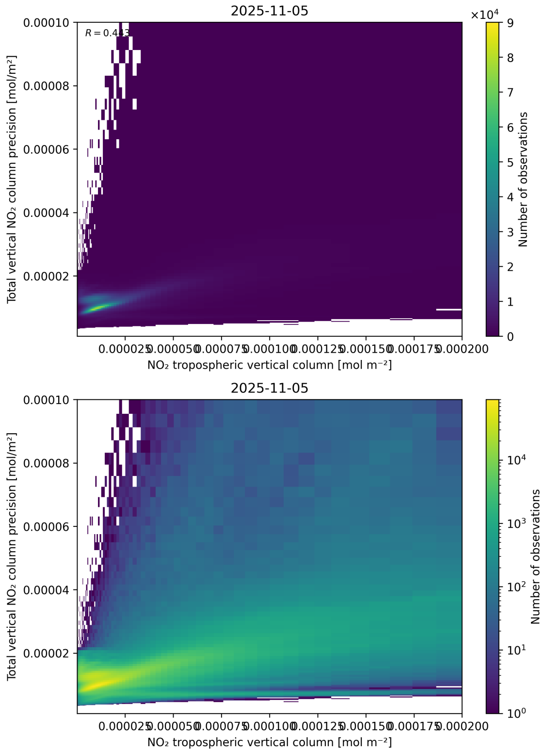
Figure 129: Scatter density plot of “NO 2 tropospheric vertical column” against “Total vertical NO 2 column precision” for 2025-11-04 to 2025-11-06.
