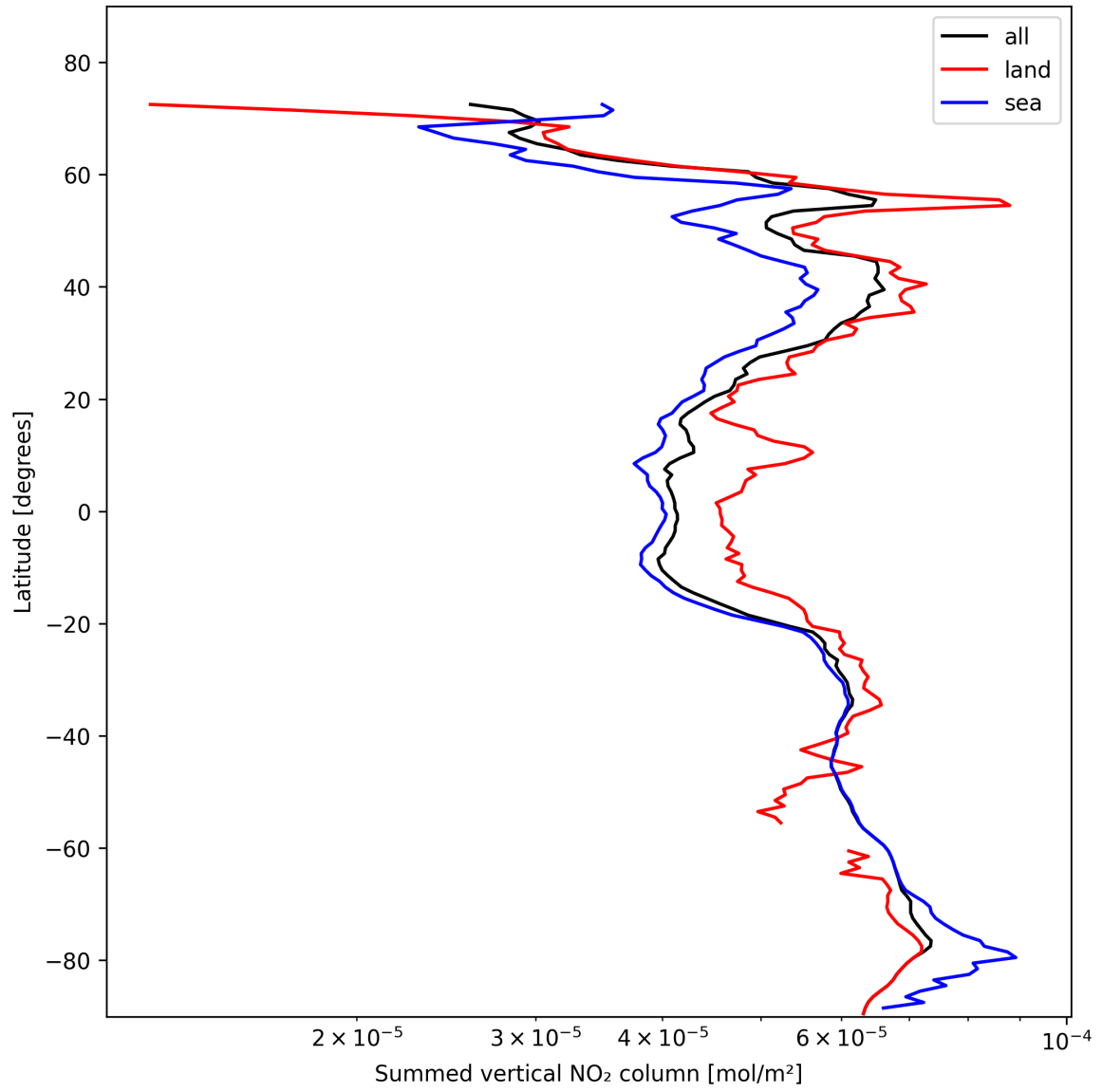
Figure 23: Zonal average of “Summed vertical NO 2 column” for 2025-11-04 to 2025-11-06.
