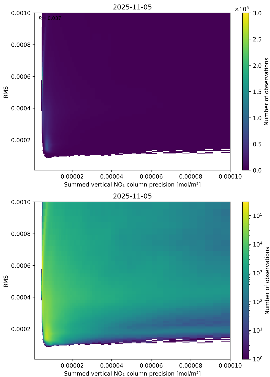
Figure 108: Scatter density plot of “Summed vertical NO 2 column precision” against “RMS” for 2025-11-04 to 2025-11-06.
