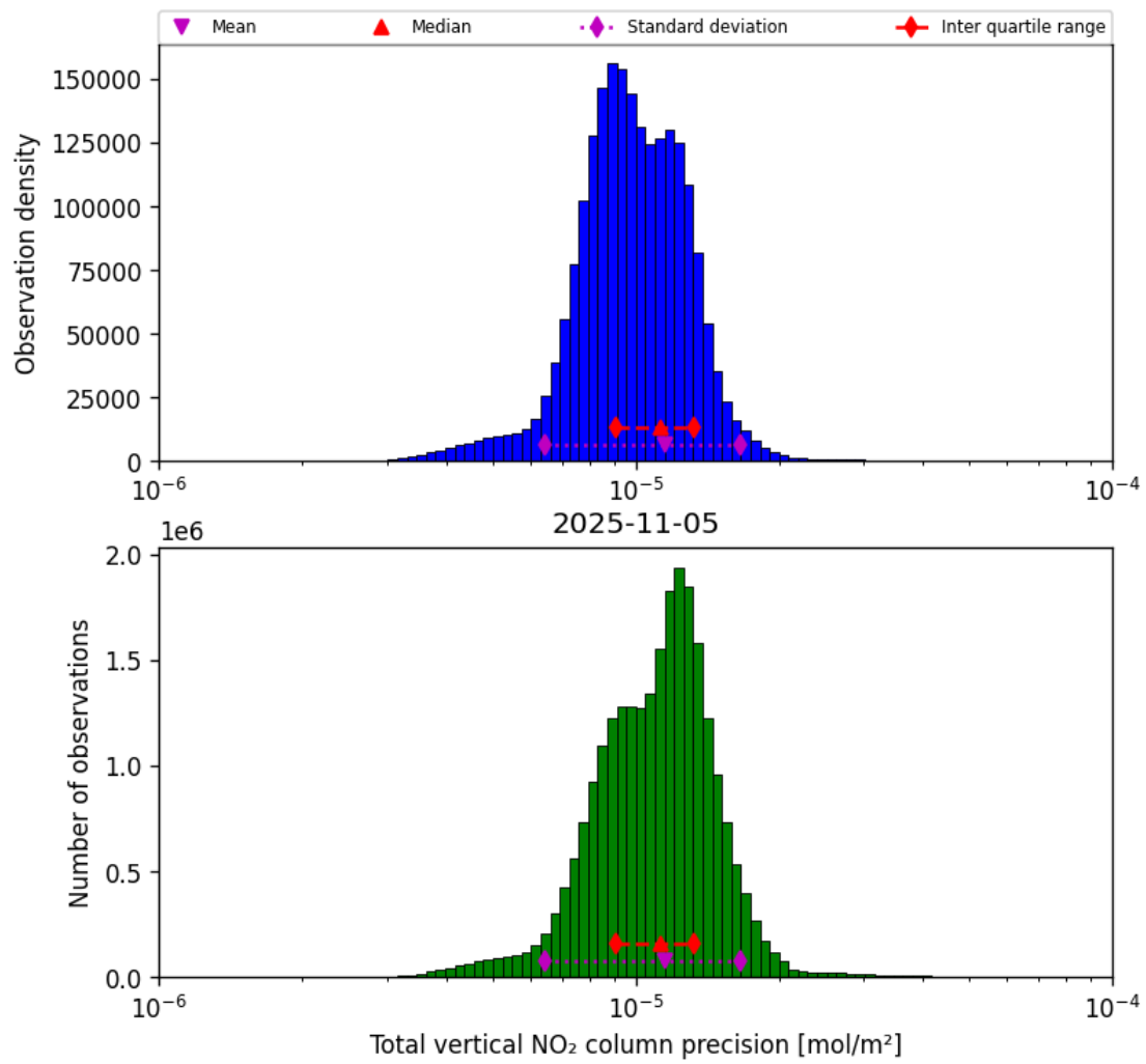
Figure 39: Histogram of “Total vertical NO 2 column precision” for 2025-11-04 to 2025-11-06
