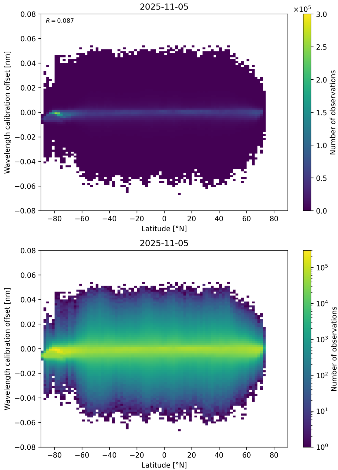
Figure 95: Scatter density plot of “Latitude” against “Wavelength calibration offset” for 2025-11-04 to 2025-11-06.
