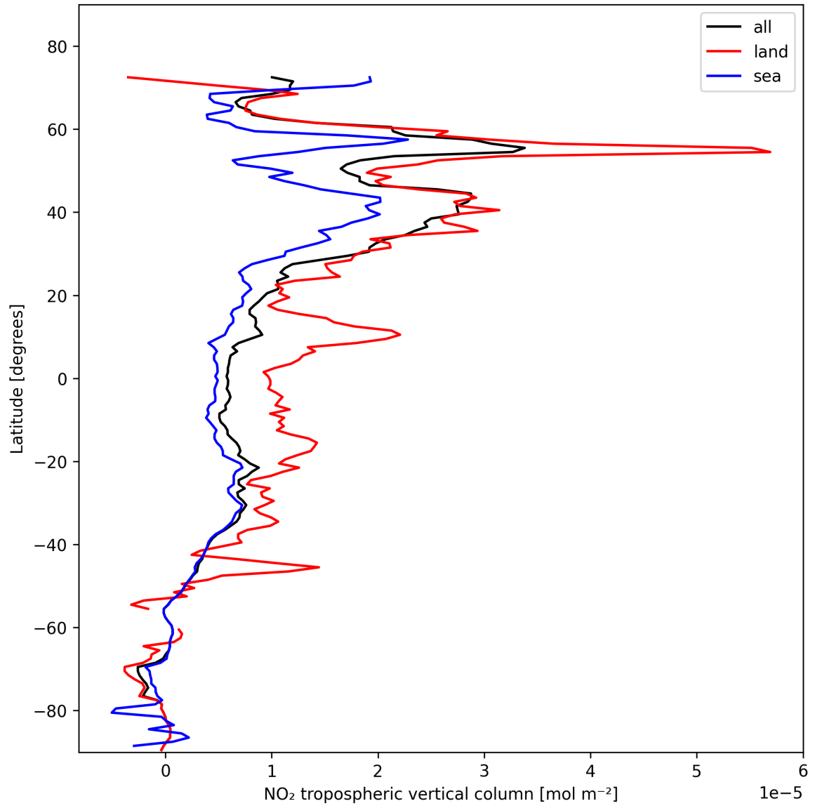
Figure 12: Zonal average of “NO 2 tropospheric vertical column” for 2025-11-04 to 2025-11-06.
