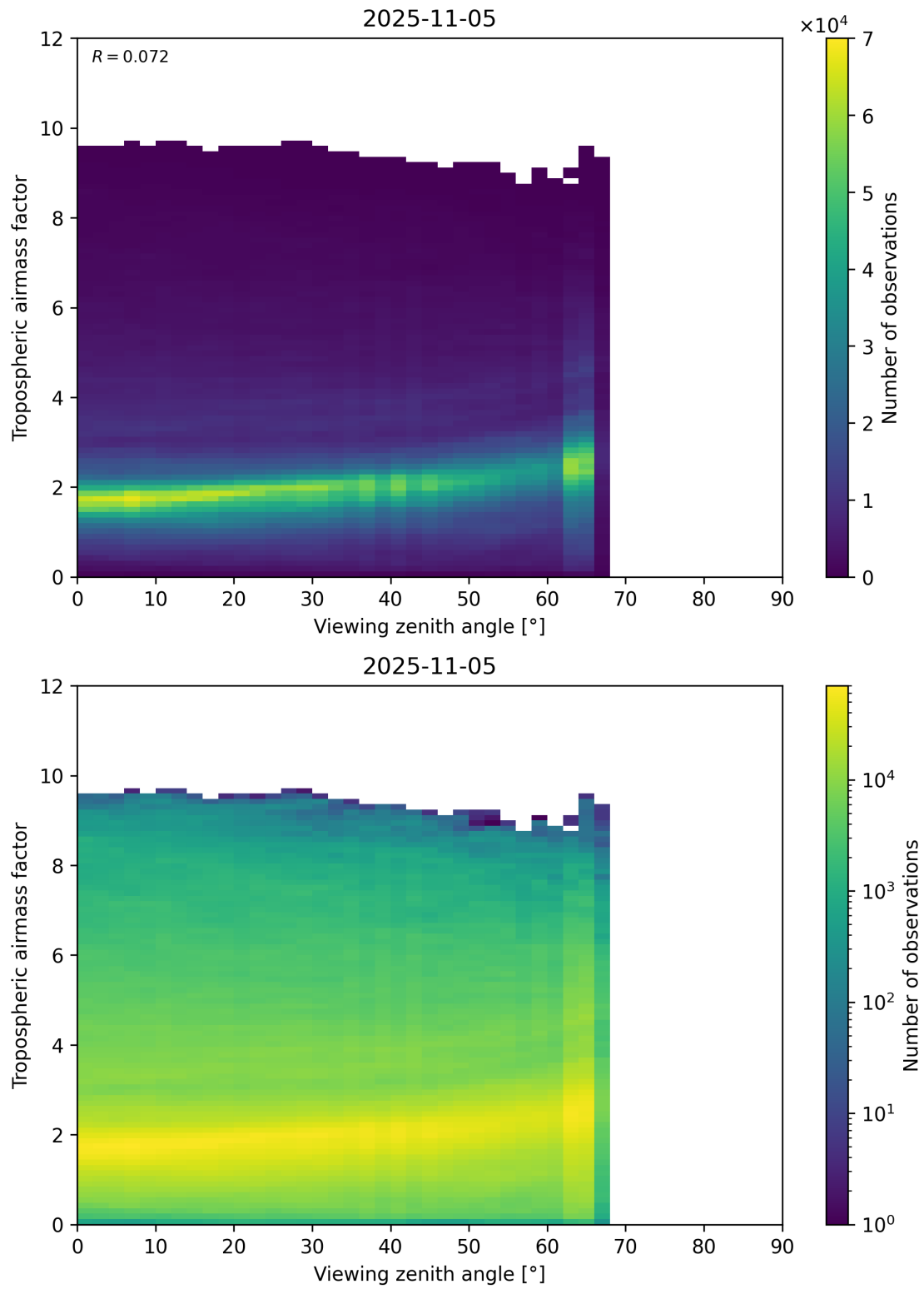
Figure 161: Scatter density plot of “Viewing zenith angle” against “Tropospheric airmass factor” for 2025-11-04 to 2025-11-06.
