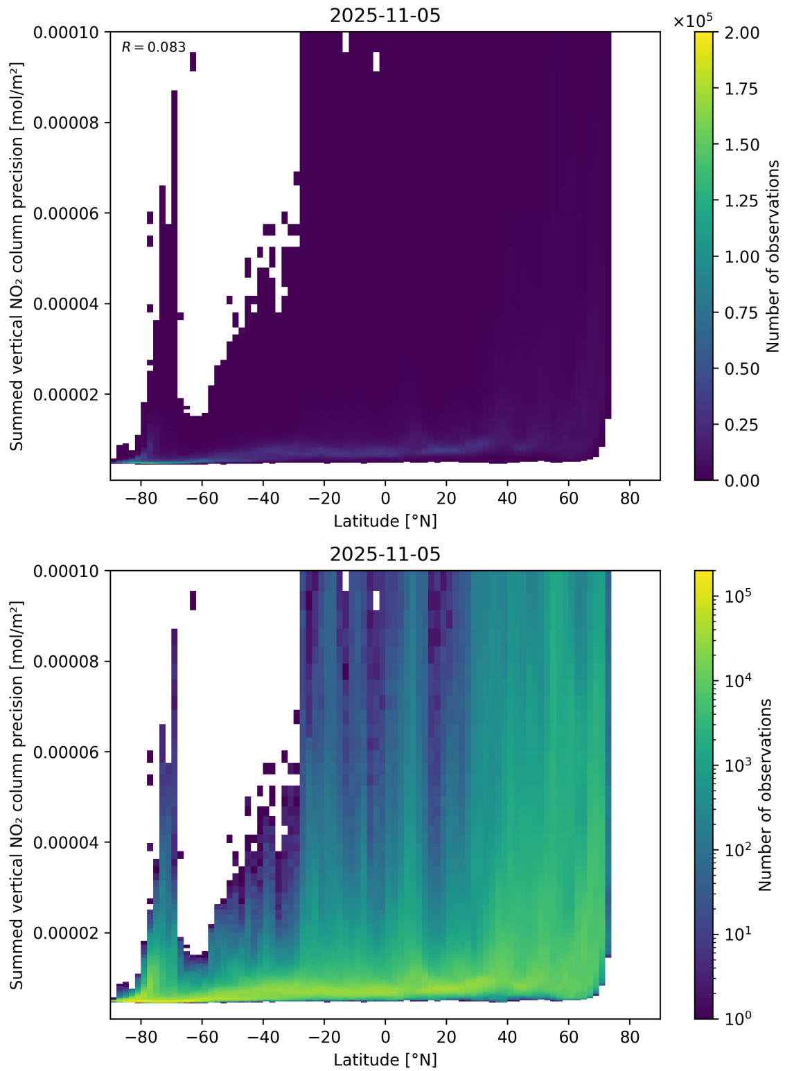
Figure 89: Scatter density plot of “Latitude” against “Summed vertical NO 2 column precision” for 2025-11-04 to 2025-11-06.
