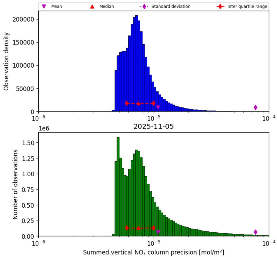
Figure 41: Histogram of “Summed vertical NO 2 column precision” for 2025-11-04 to 2025-11-06
