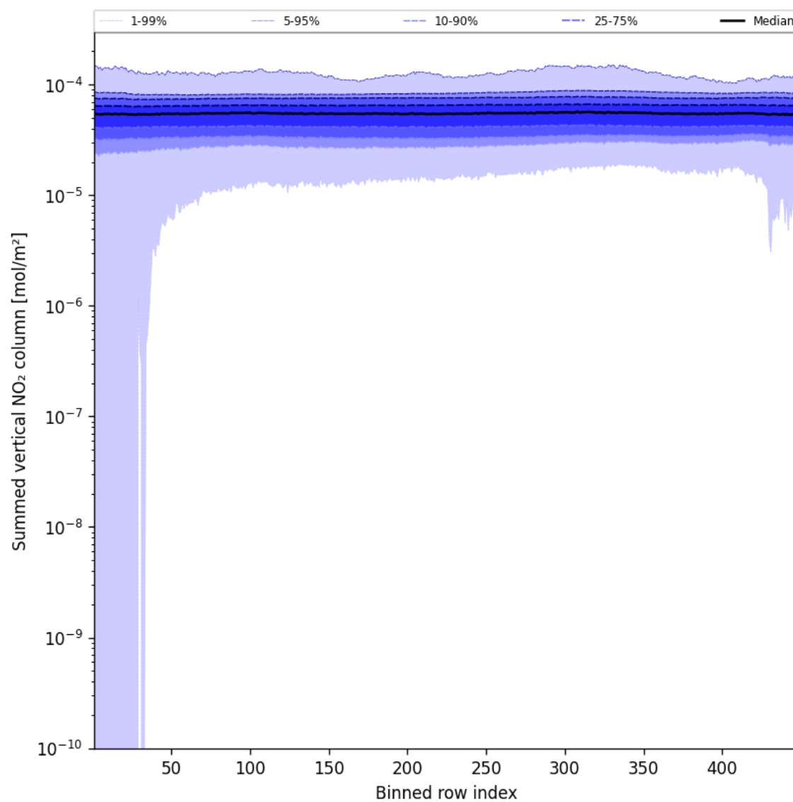
Figure 57: Along track statistics of “Summed vertical NO 2 column” for 2025-11-04 to 2025-11-06
