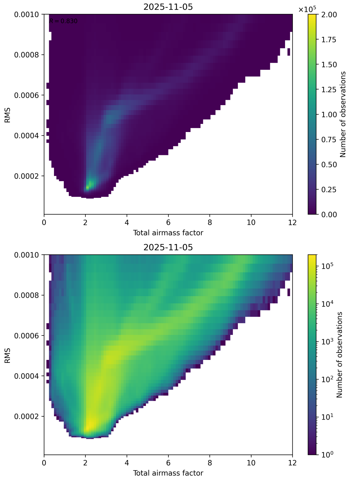
Figure 69: Scatter density plot of “Total airmass factor” against “RMS” for 2025-11-04 to 2025-11-06.
