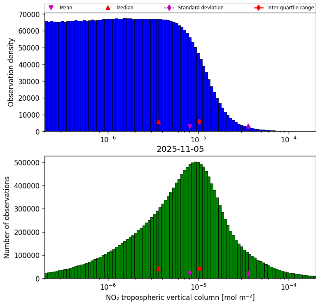
Figure 29: Histogram of “NO 2 tropospheric vertical column” for 2025-11-04 to 2025-11-06
