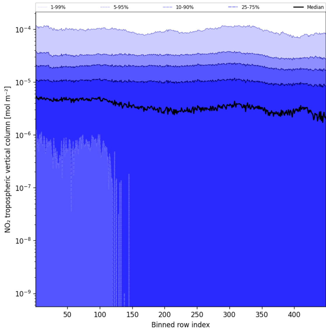
Figure 46: Along track statistics of “NO 2 tropospheric vertical column” for 2025-11-04 to 2025-11-06
