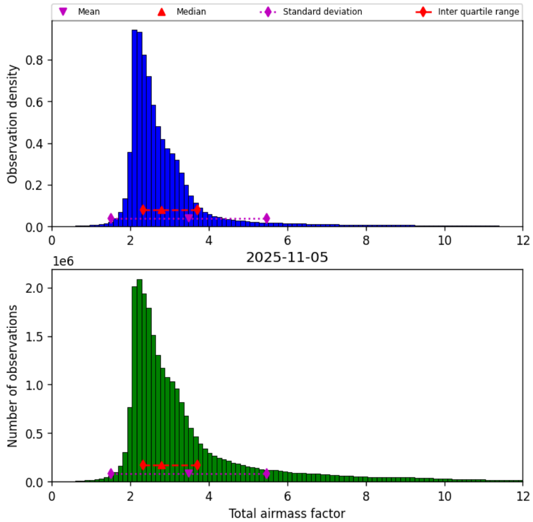
Figure 32: Histogram of “Total airmass factor” for 2025-11-04 to 2025-11-06
