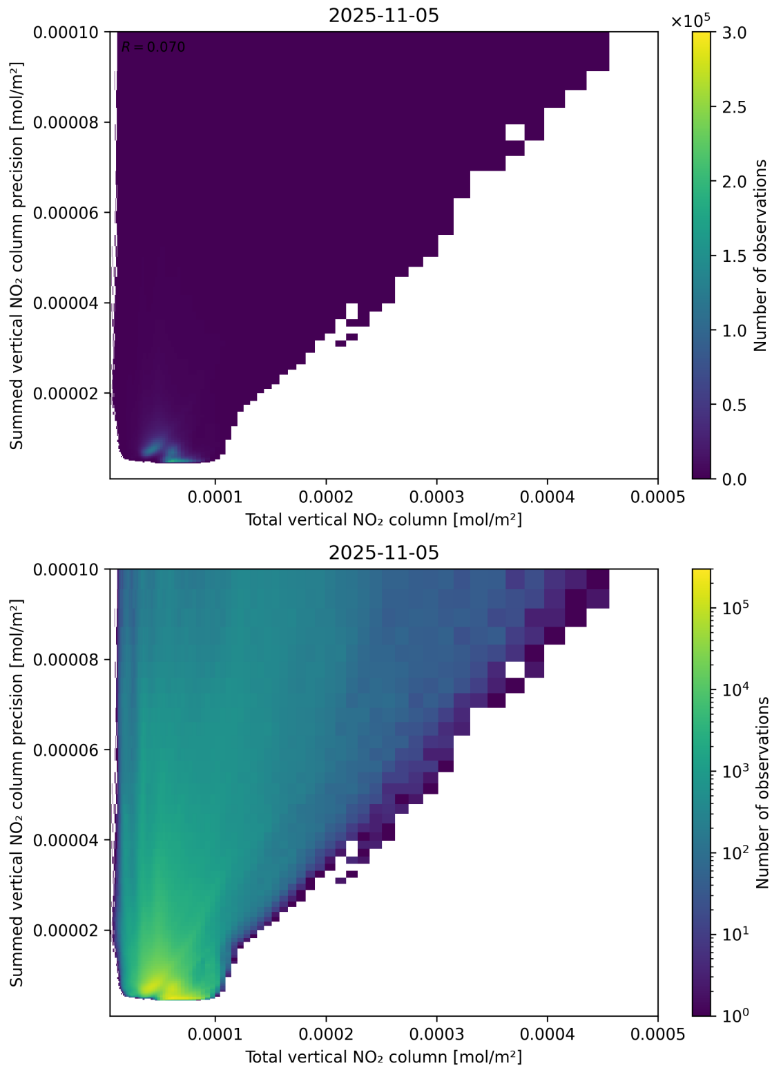
Figure 113: Scatter density plot of “Total vertical NO 2 column” against “Summed vertical NO 2 column precision” for 2025-11-04 to 2025-11-06.
