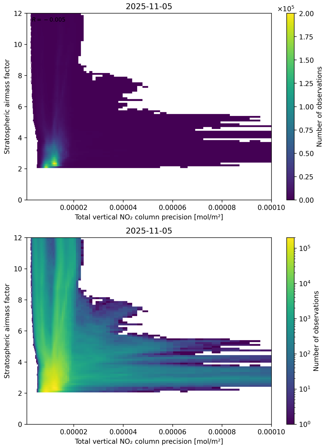
Figure 115: Scatter density plot of “Total vertical NO 2 column precision” against “Stratospheric airmass factor” for 2025-11-04 to 2025-11-06.
