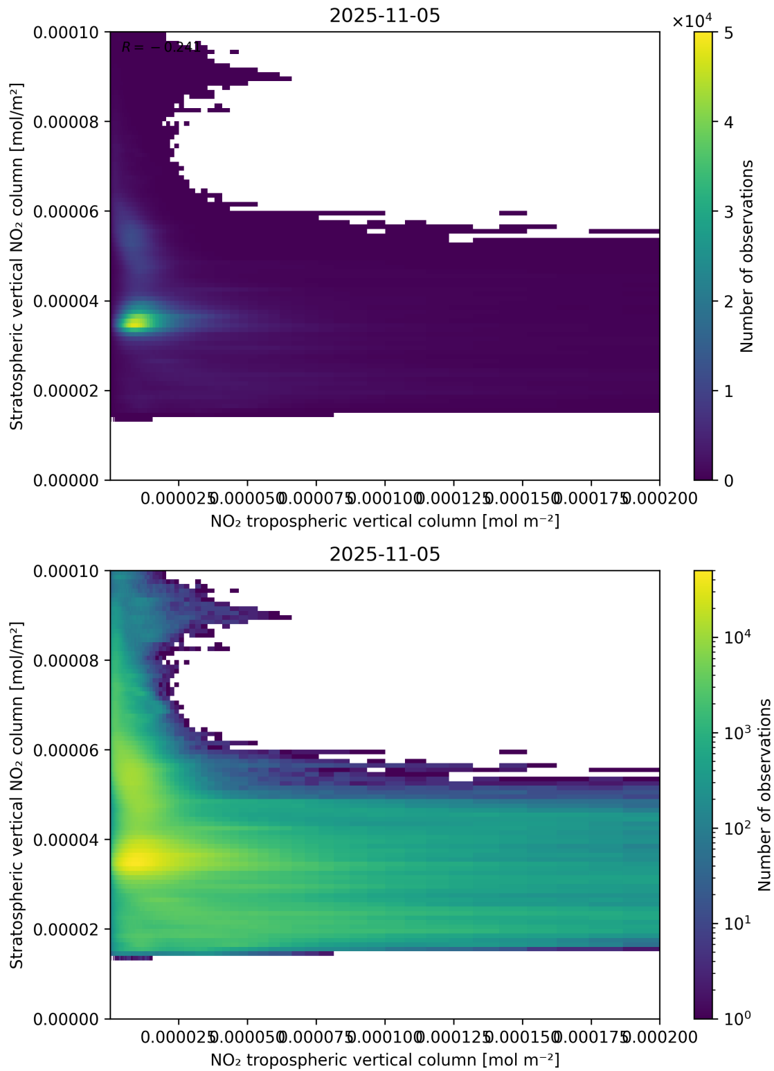
Figure 125: Scatter density plot of “NO 2 tropospheric vertical column” against “Stratospheric vertical NO 2 column” for 2025-11-04 to 2025-11-06.
