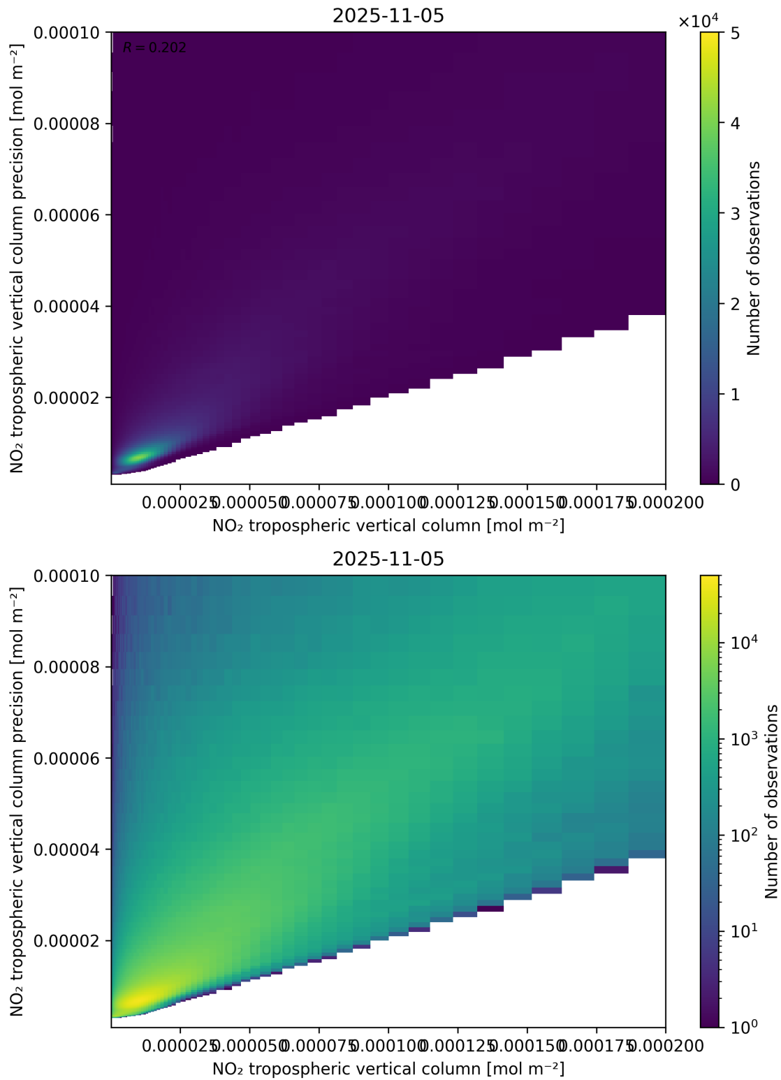
Figure 130: Scatter density plot of “NO 2 tropospheric vertical column” against “NO 2 tropospheric vertical column precision” for 2025-11-04 to 2025-11-06.
