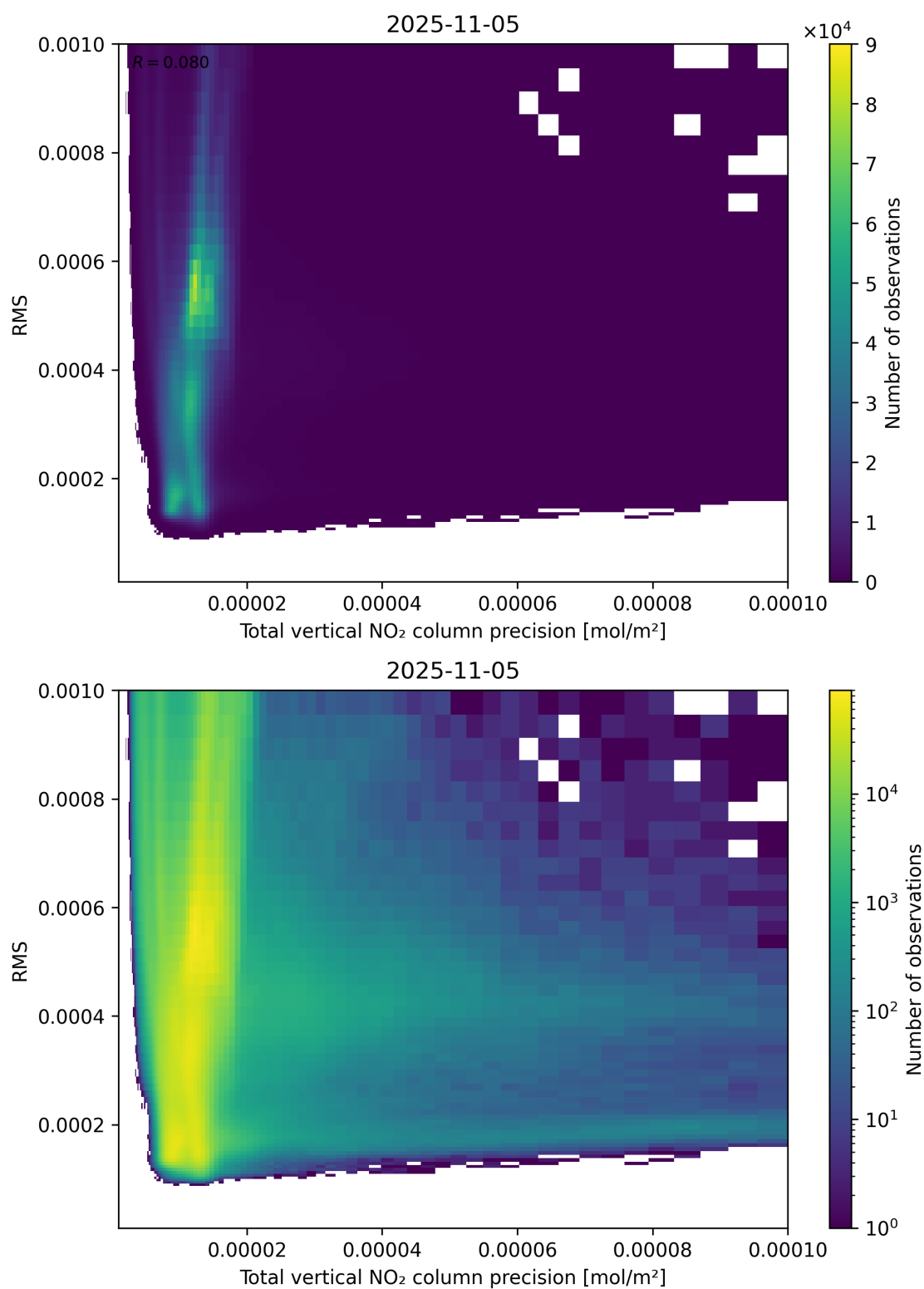
Figure 119: Scatter density plot of “Total vertical NO 2 column precision” against “RMS” for 2025-11-04 to 2025-11-06.
