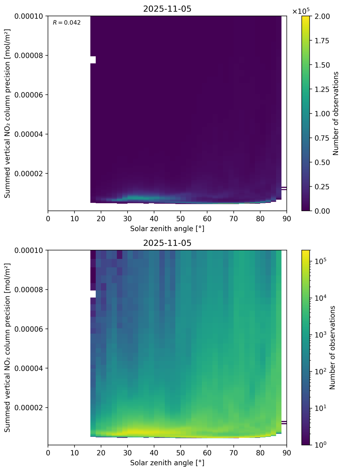
Figure 152: Scatter density plot of “Solar zenith angle” against “Summed vertical NO 2 column precision” for 2025-11-04 to 2025-11-06.
