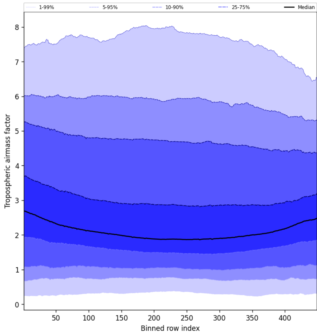
Figure 48: Along track statistics of “Tropospheric airmass factor” for 2025-11-04 to 2025-11-06
