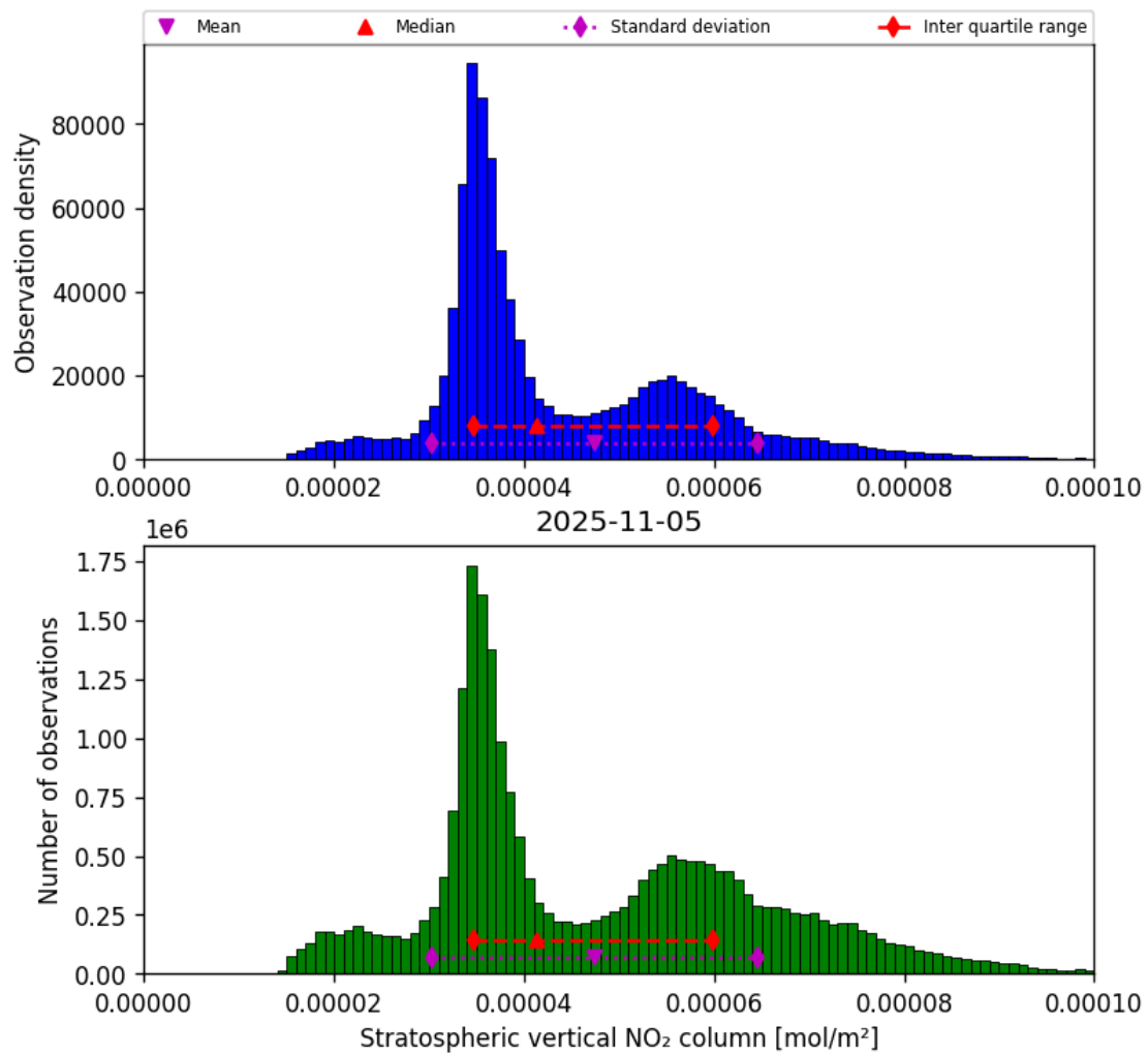
Figure 36: Histogram of “Stratospheric vertical NO 2 column” for 2025-11-04 to 2025-11-06
