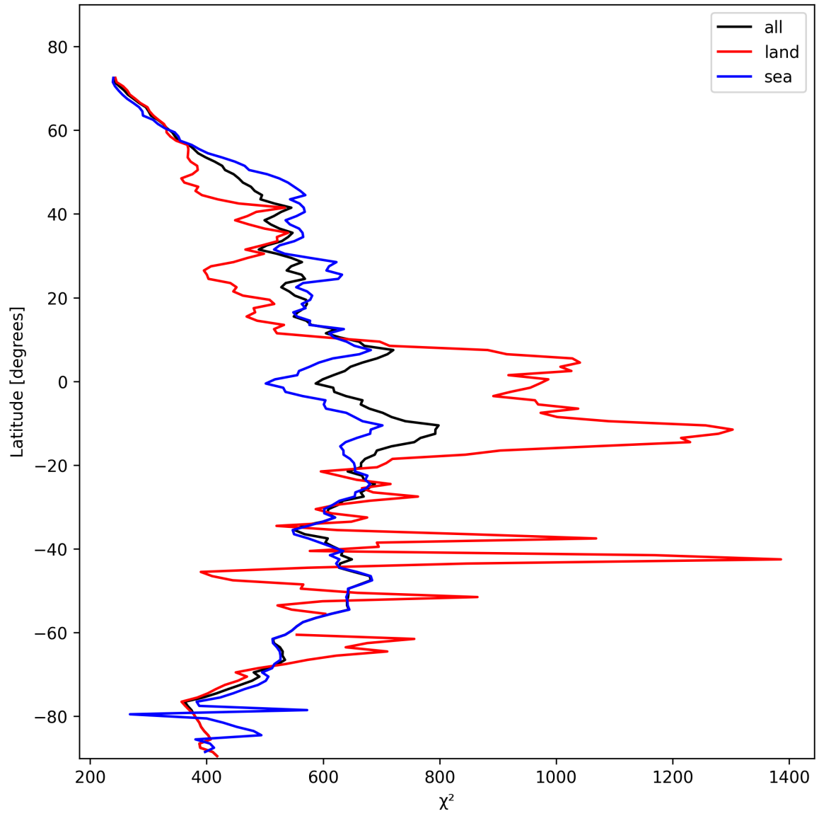
Figure 25: Zonal average of “ \chi^2 ” for 2025-11-04 to 2025-11-06.
