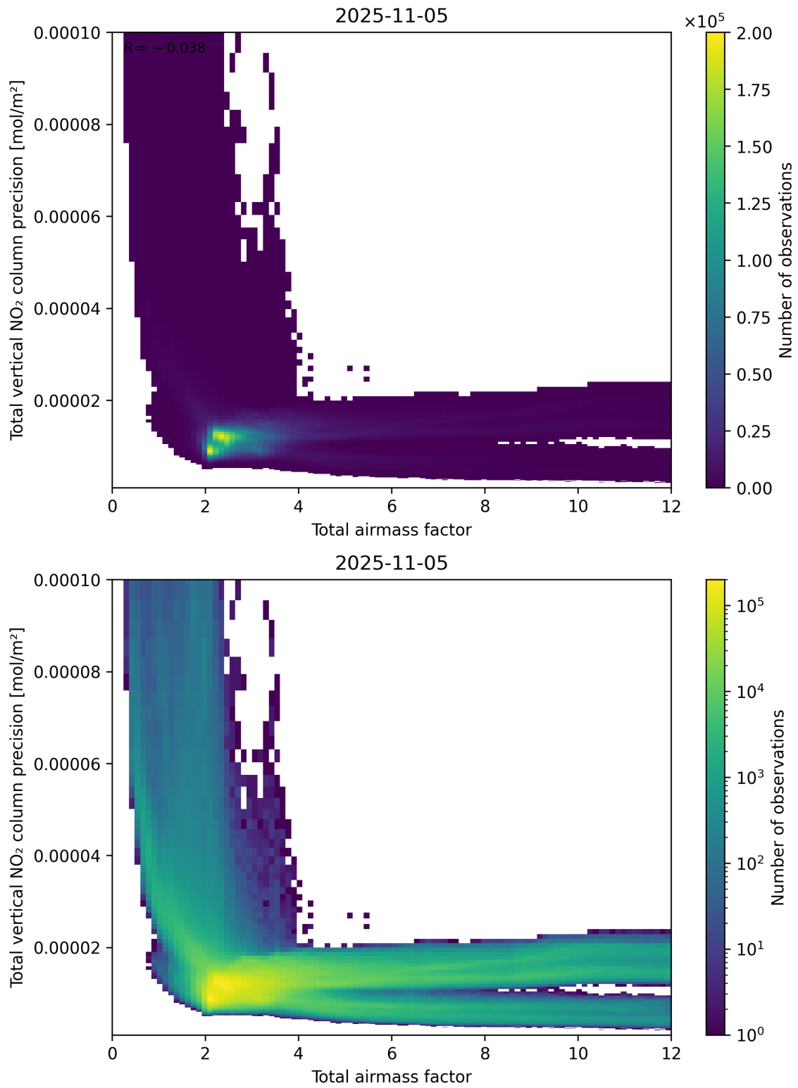
Figure 68: Scatter density plot of “Total airmass factor” against “Total vertical NO 2 column precision” for 2025-11-04 to 2025-11-06.
