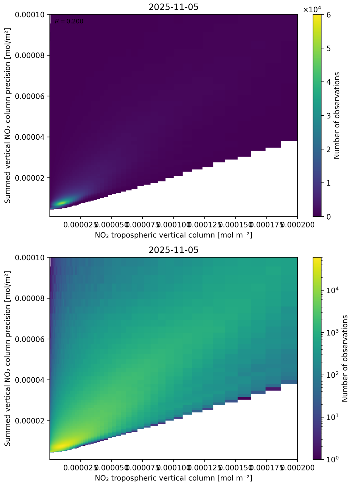
Figure 127: Scatter density plot of “NO 2 tropospheric vertical column” against “Summed vertical NO 2 column precision” for 2025-11-04 to 2025-11-06.
