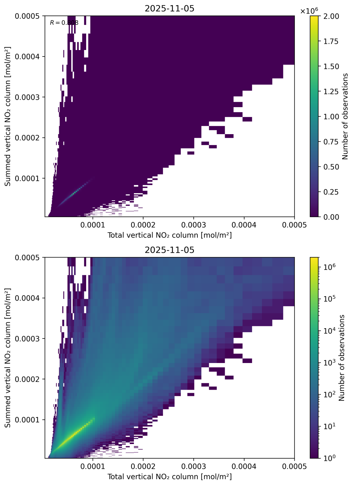
Figure 112: Scatter density plot of “Total vertical NO 2 column” against “Summed vertical NO 2 column” for 2025-11-04 to 2025-11-06.
