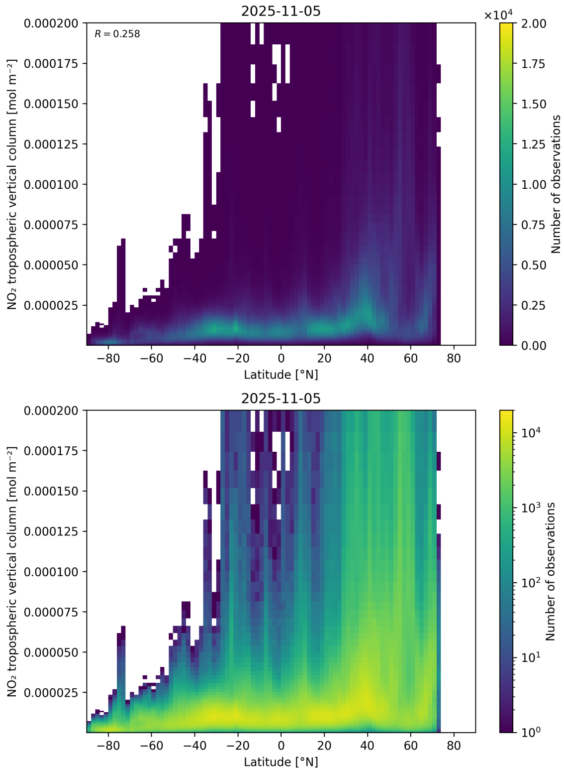
Figure 92: Scatter density plot of “Latitude” against “NO 2 tropospheric vertical column” for 2025-11-04 to 2025-11-06.
