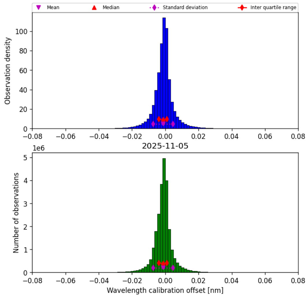
Figure 35: Histogram of “Wavelength calibration offset” for 2025-11-04 to 2025-11-06
