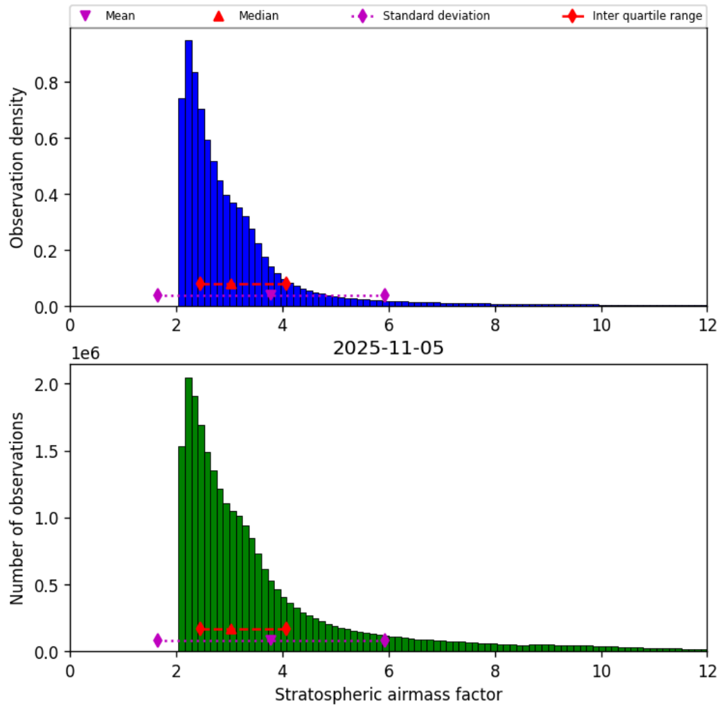
Figure 44: Histogram of “Stratospheric airmass factor” for 2025-11-04 to 2025-11-06
