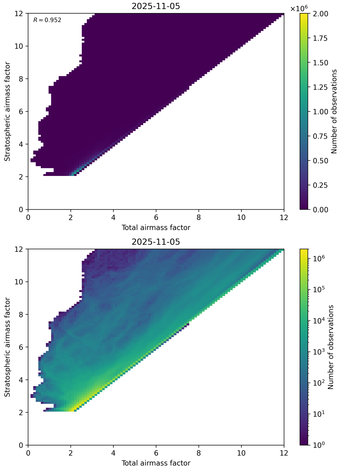
Figure 62: Scatter density plot of “Total airmass factor” against “Stratospheric airmass factor” for 2025-11-04 to 2025-11-06.
