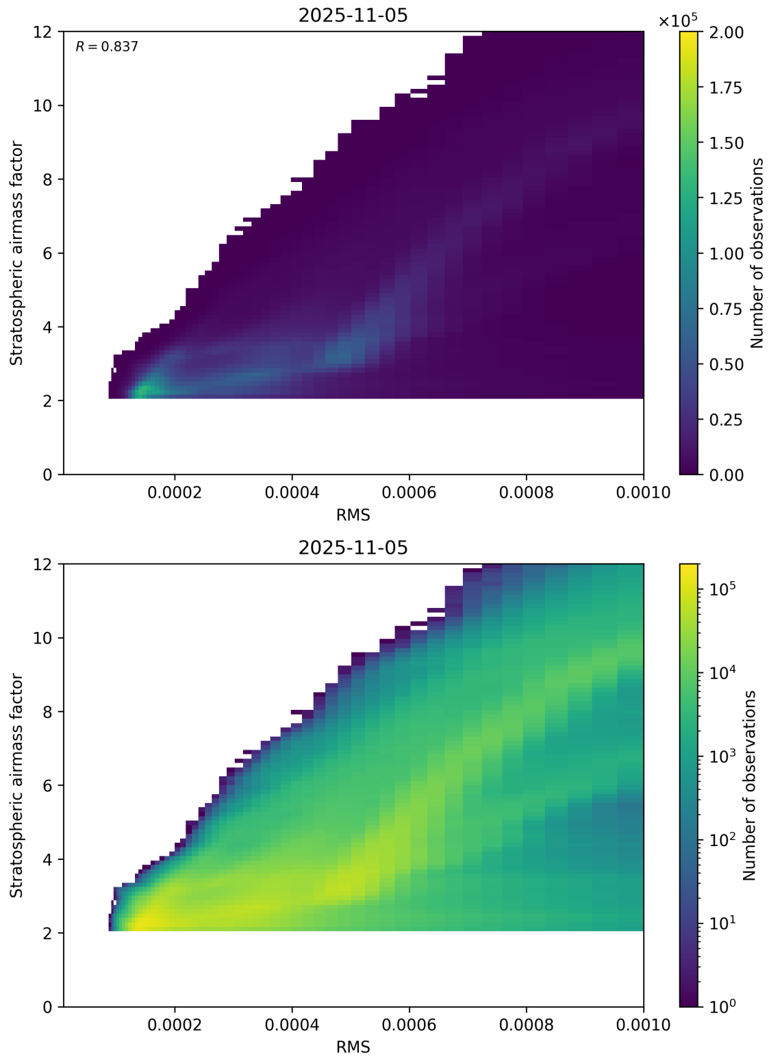
Figure 144: Scatter density plot of “RMS” against “Stratospheric airmass factor” for 2025-11-04 to 2025-11-06.
