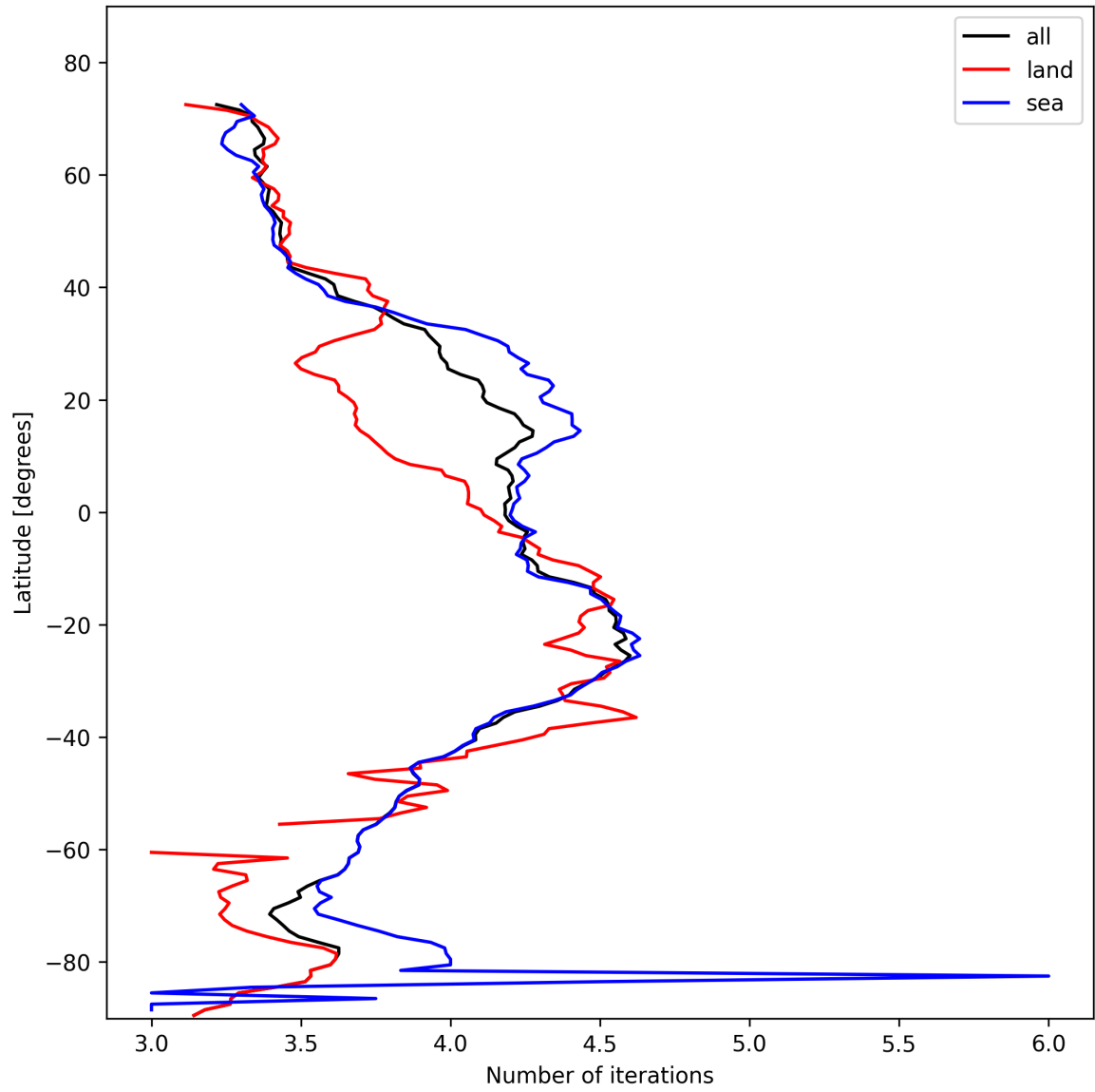
Figure 17: Zonal average of “Number of iterations” for 2025-11-04 to 2025-11-06.
