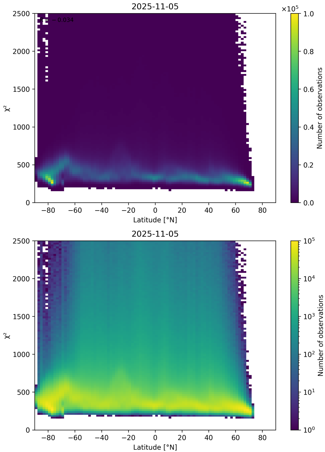
Figure 86: Scatter density plot of “Latitude” against “ \chi^2 ” for 2025-11-04 to 2025-11-06.
