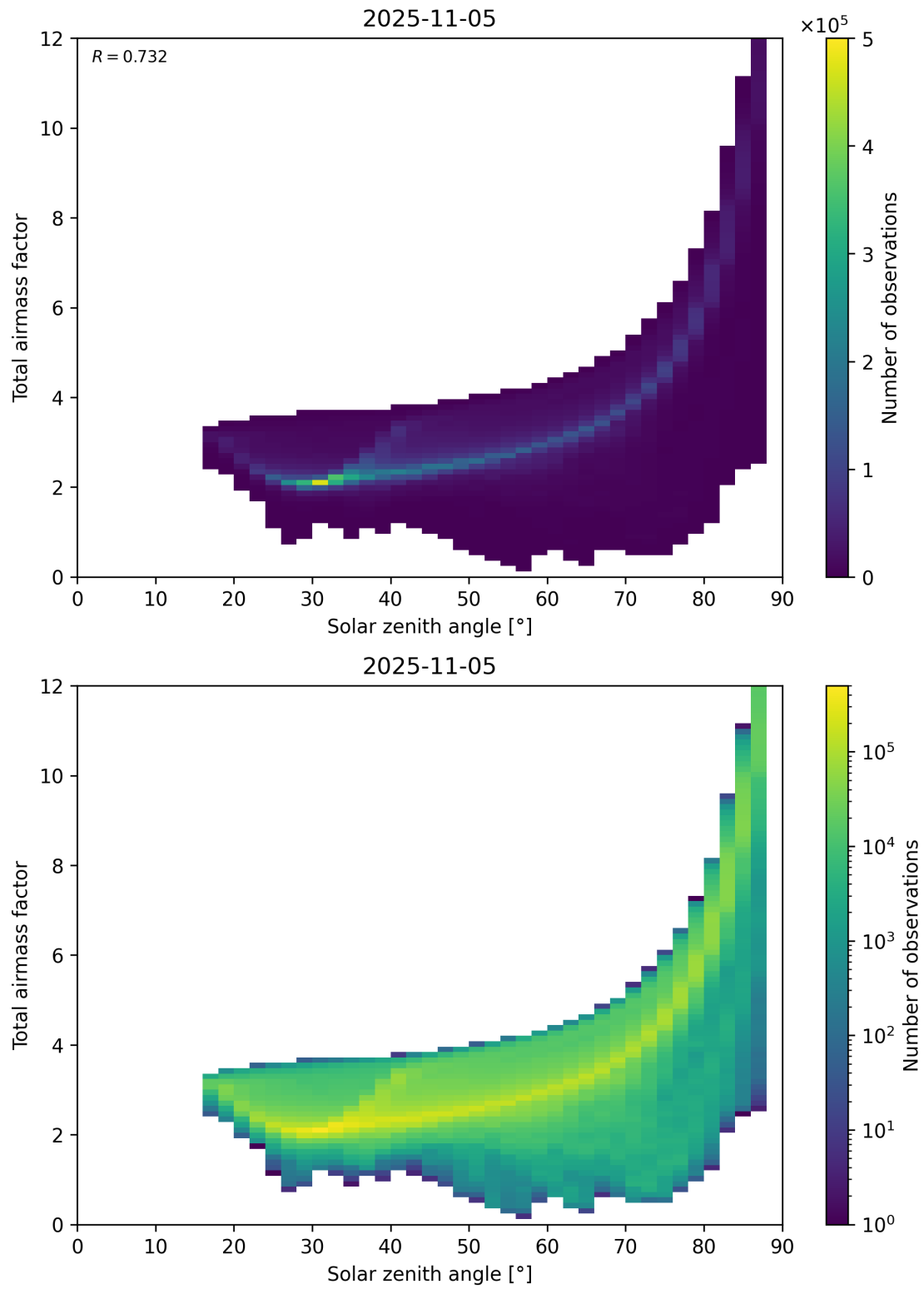
Figure 146: Scatter density plot of “Solar zenith angle” against “Total airmass factor” for 2025-11-04 to 2025-11-06.
