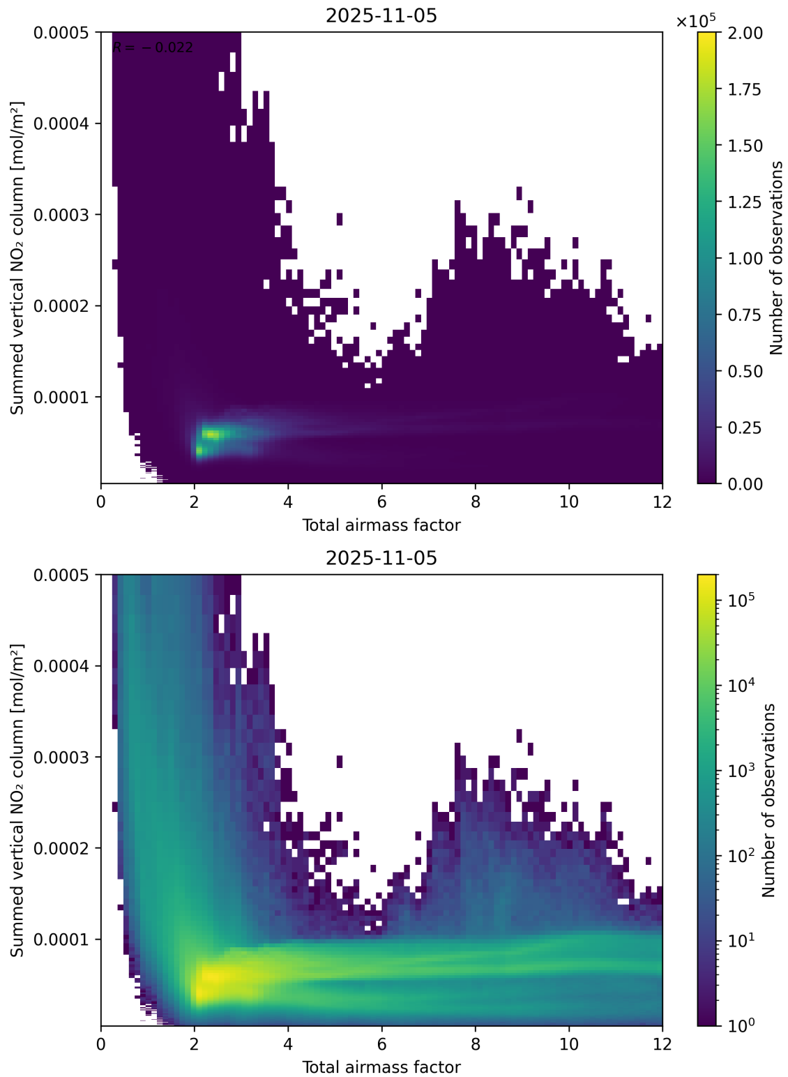
Figure 65: Scatter density plot of “Total airmass factor” against “Summed vertical NO 2 column” for 2025-11-04 to 2025-11-06.
