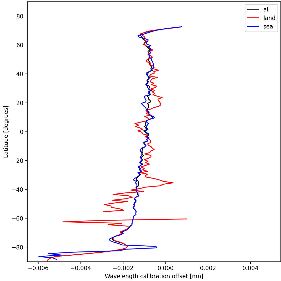
Figure 18: Zonal average of “Wavelength calibration offset” for 2025-11-04 to 2025-11-06.
