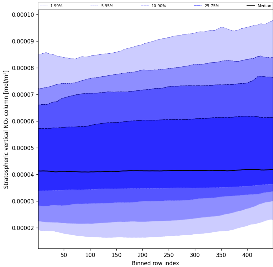
Figure 53: Along track statistics of “Stratospheric vertical NO 2 column” for 2025-11-04 to 2025-11-06
