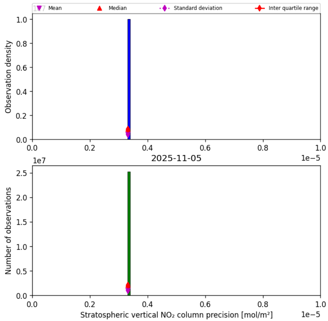
Figure 37: Histogram of “Stratospheric vertical NO 2 column precision” for 2025-11-04 to 2025-11-06
