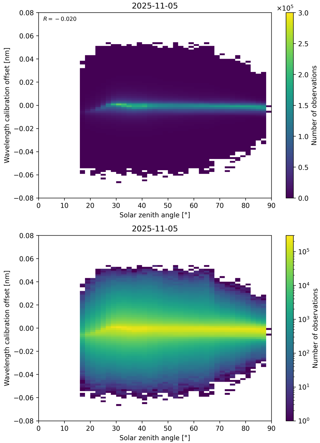
Figure 158: Scatter density plot of “Solar zenith angle” against “Wavelength calibration offset” for 2025-11-04 to 2025-11-06.
