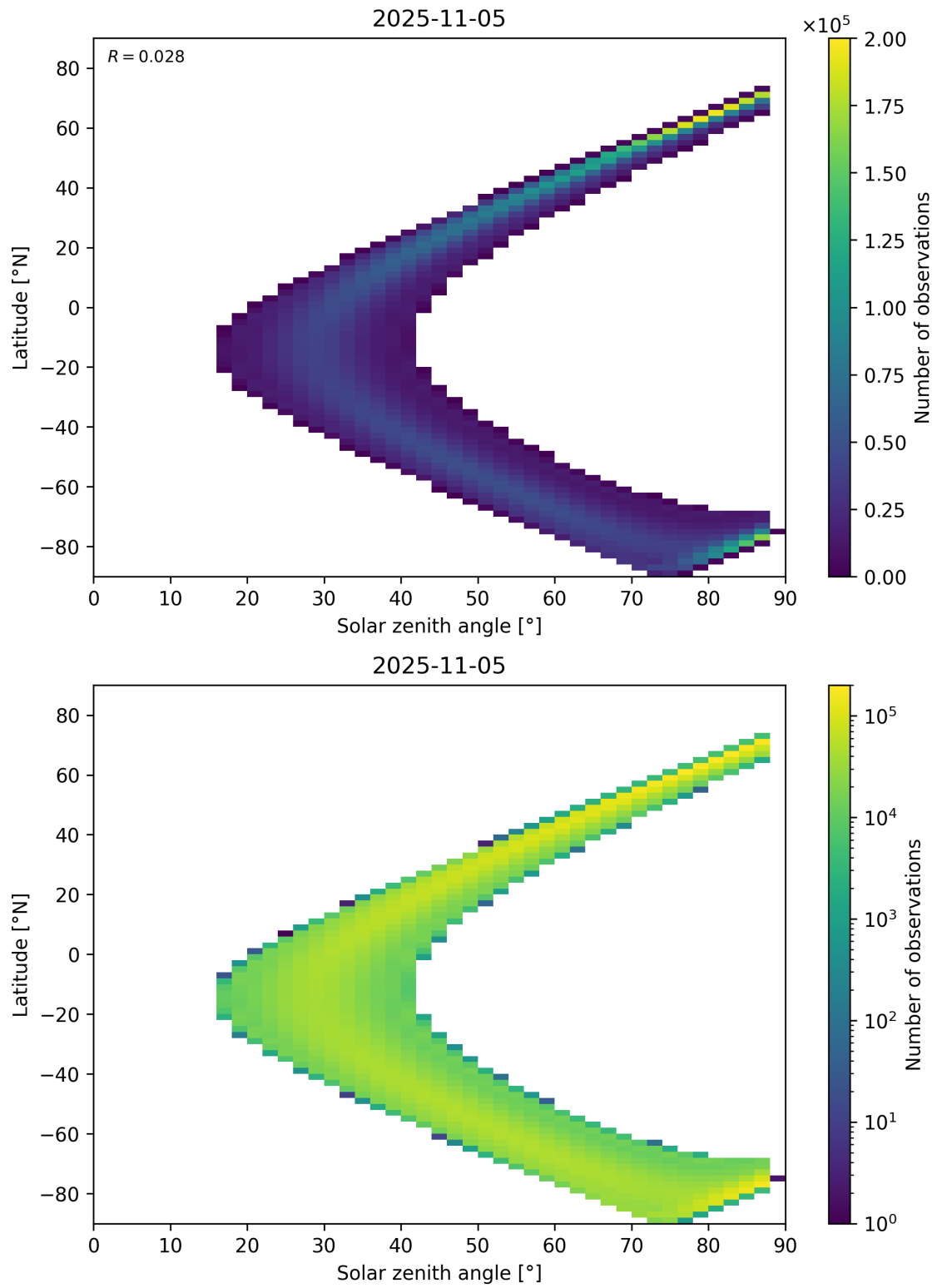
Figure 149: Scatter density plot of “Solar zenith angle” against “Latitude” for 2025-11-04 to 2025-11-06.
