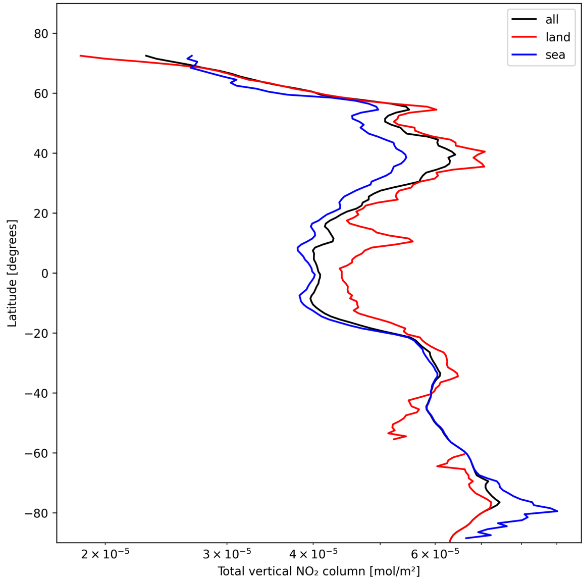
Figure 21: Zonal average of “Total vertical NO 2 column” for 2025-11-04 to 2025-11-06.
