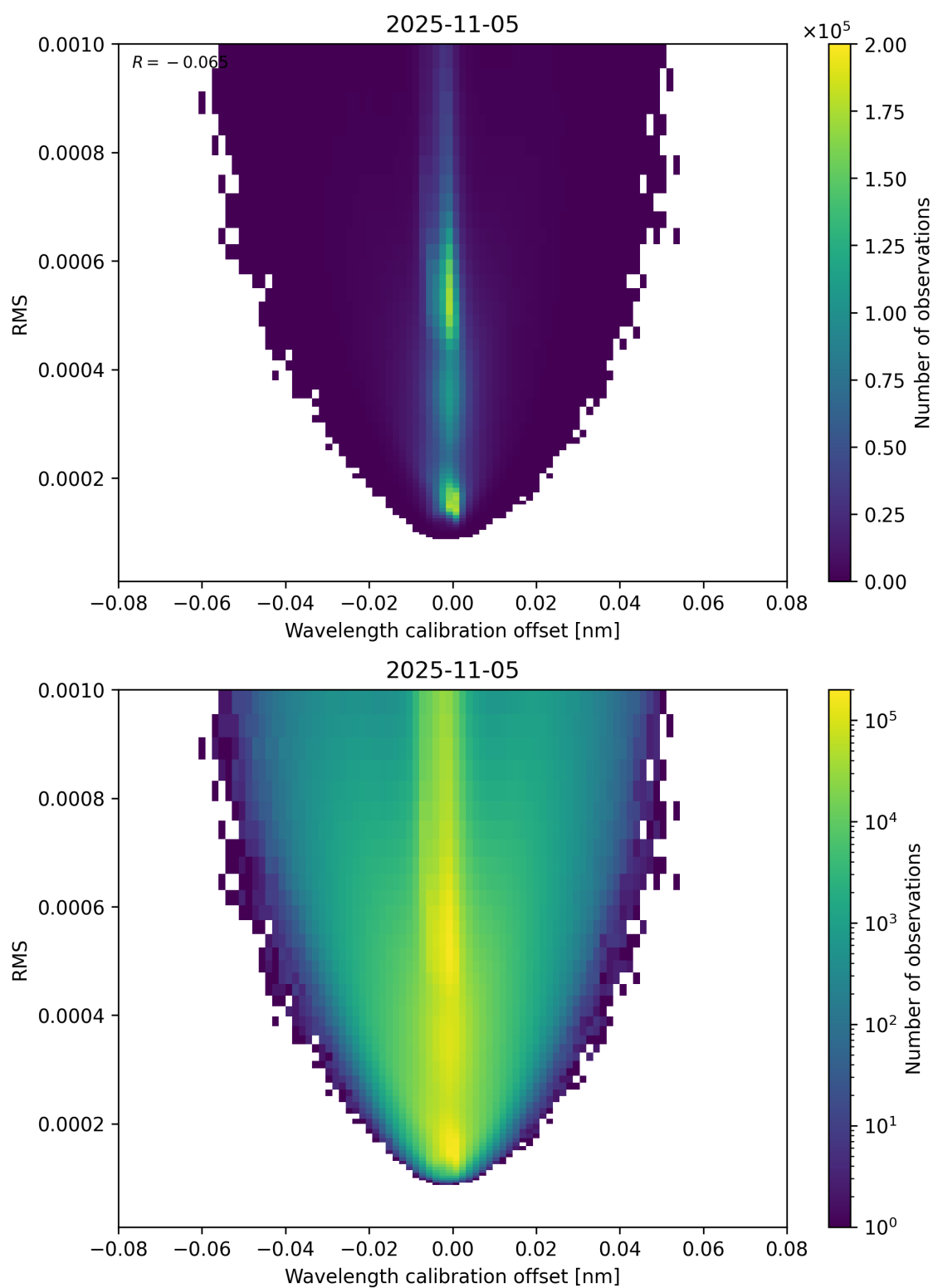
Figure 181: Scatter density plot of “Wavelength calibration offset” against “RMS” for 2025-11-04 to 2025-11-06.
