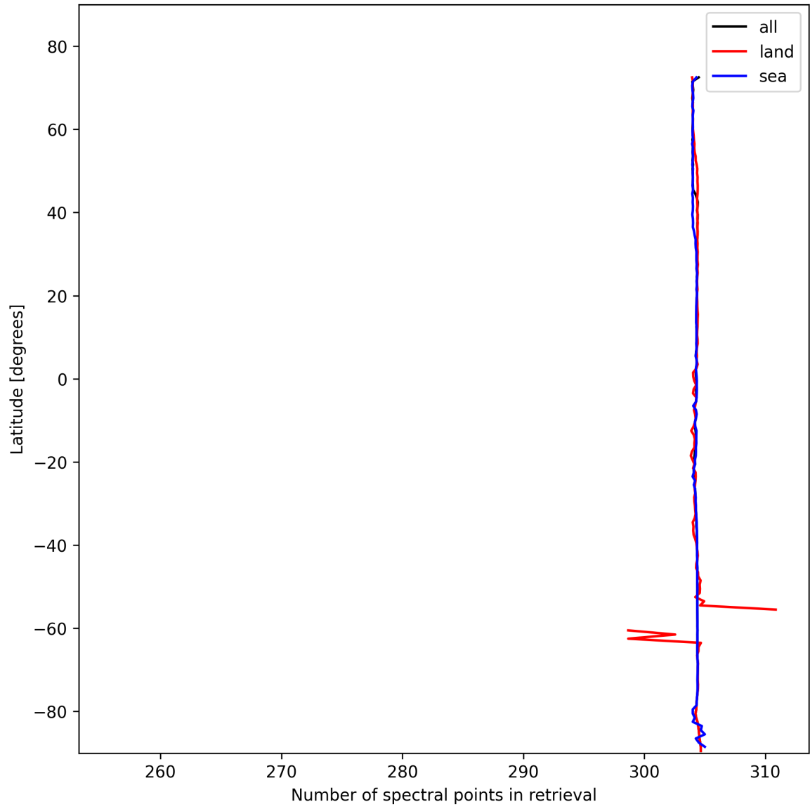
Figure 16: Zonal average of “Number of spectral points in retrieval” for 2025-11-04 to 2025-11-06.
