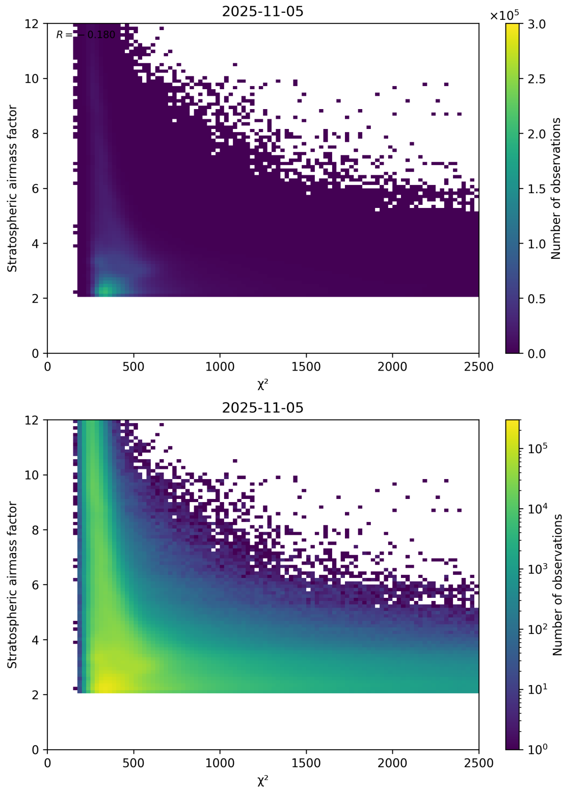
Figure 81: Scatter density plot of “ \chi^2 ” against “Stratospheric airmass factor” for 2025-11-04 to 2025-11-06.
