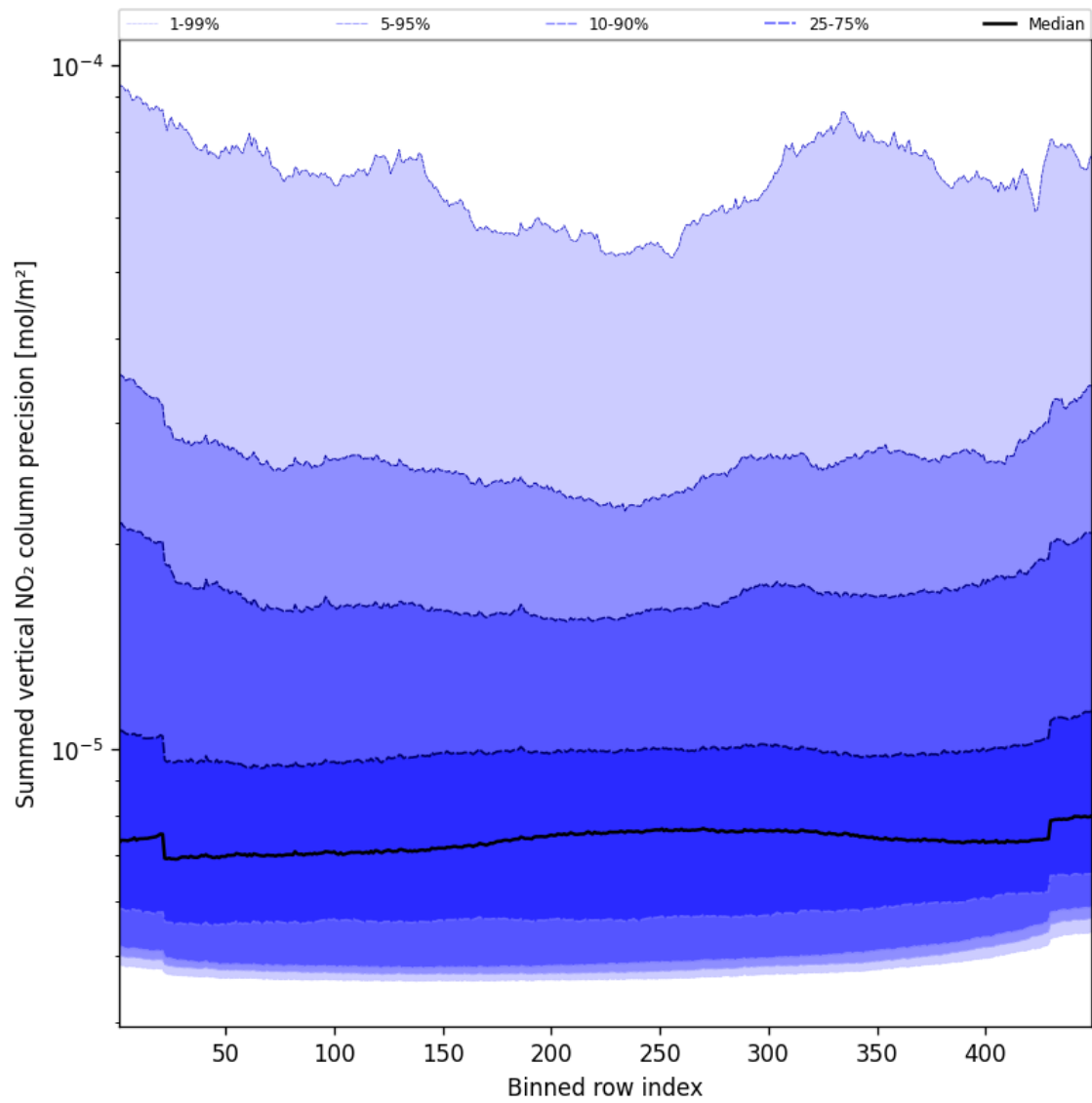
Figure 58: Along track statistics of “Summed vertical NO 2 column precision” for 2025-11-04 to 2025-11-06
