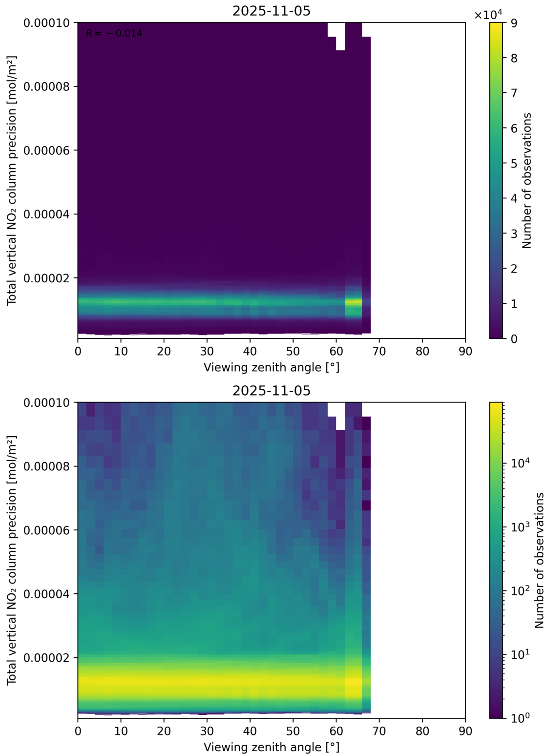
Figure 168: Scatter density plot of “Viewing zenith angle” against “Total vertical NO 2 column precision” for 2025-11-04 to 2025-11-06.
