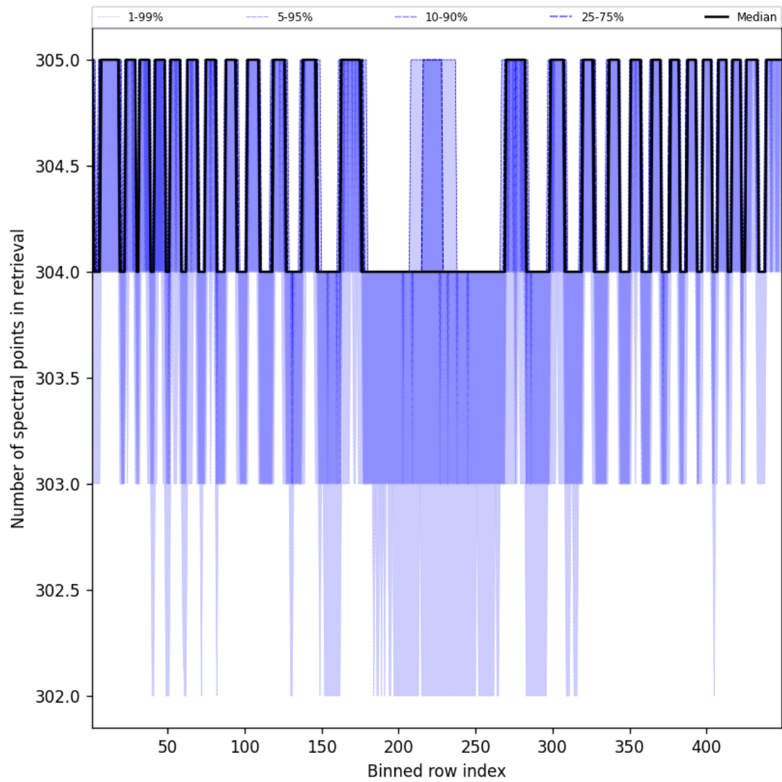
Figure 50: Along track statistics of “Number of spectral points in retrieval” for 2025-11-04 to 2025-11-06
