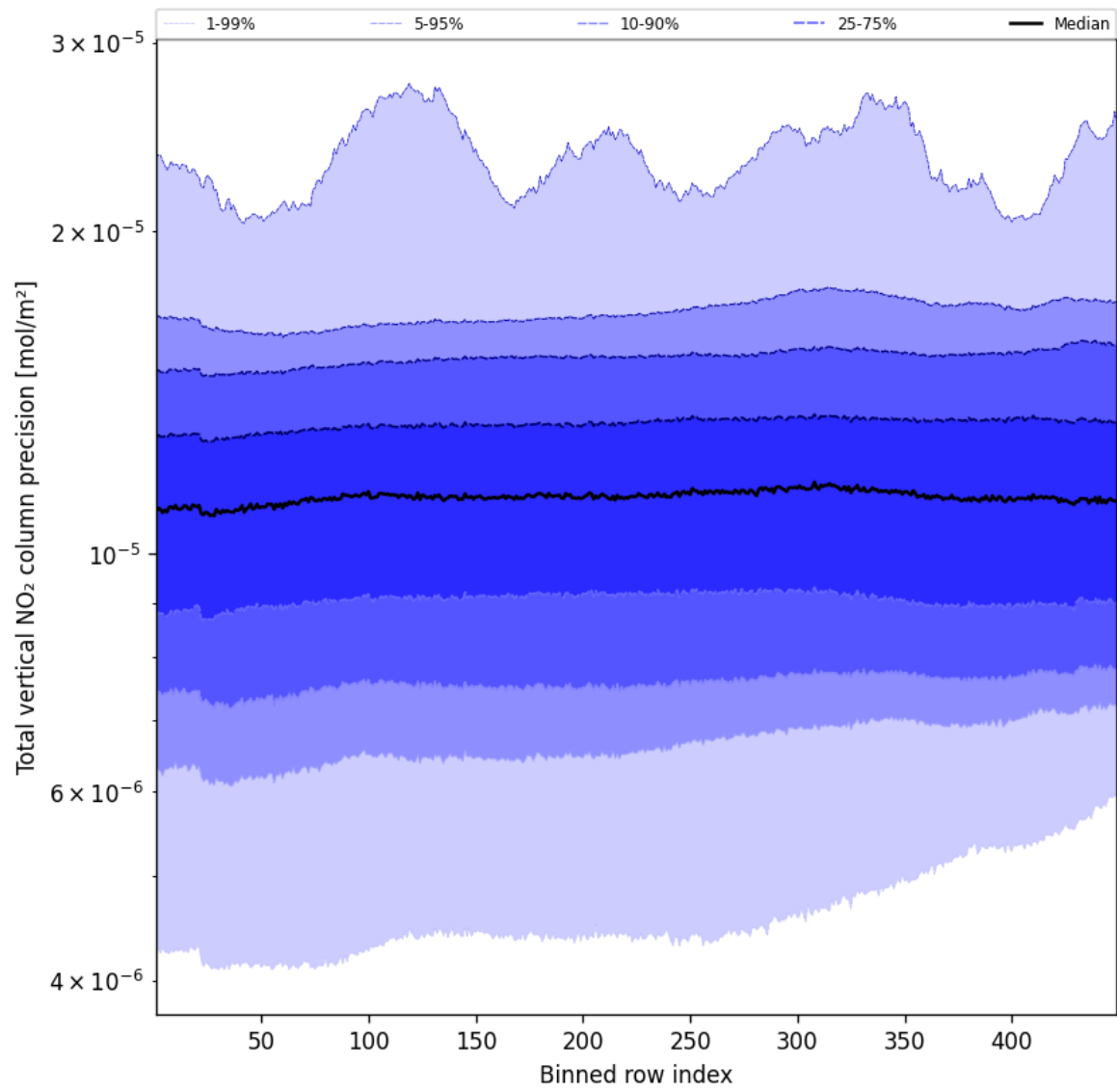
Figure 56: Along track statistics of “Total vertical NO 2 column precision” for 2025-11-04 to 2025-11-06
