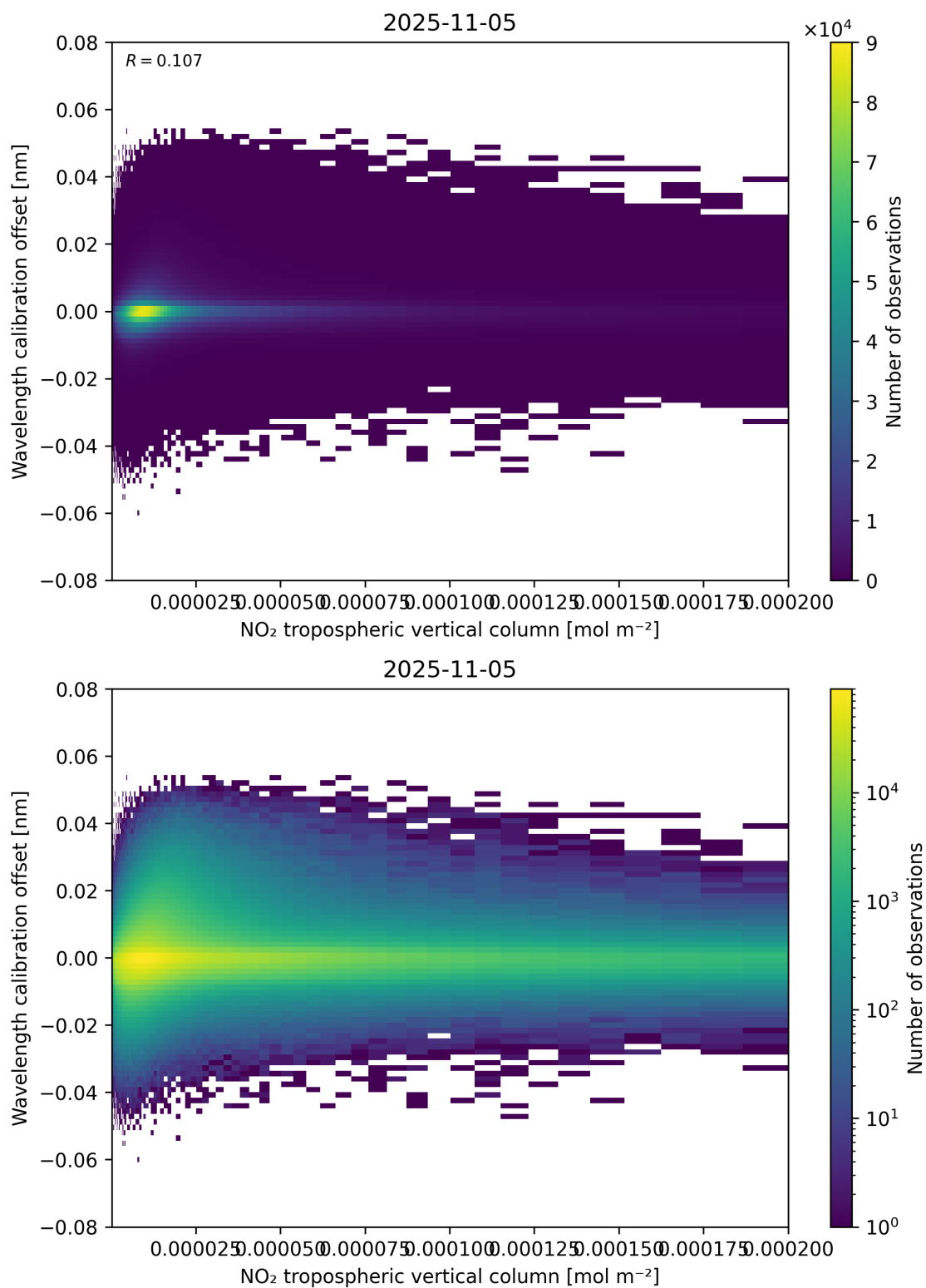
Figure 143: Scatter density plot of “NO 2 tropospheric vertical column” against “Wavelength calibration offset” for 2025-11-04 to 2025-11-06.
