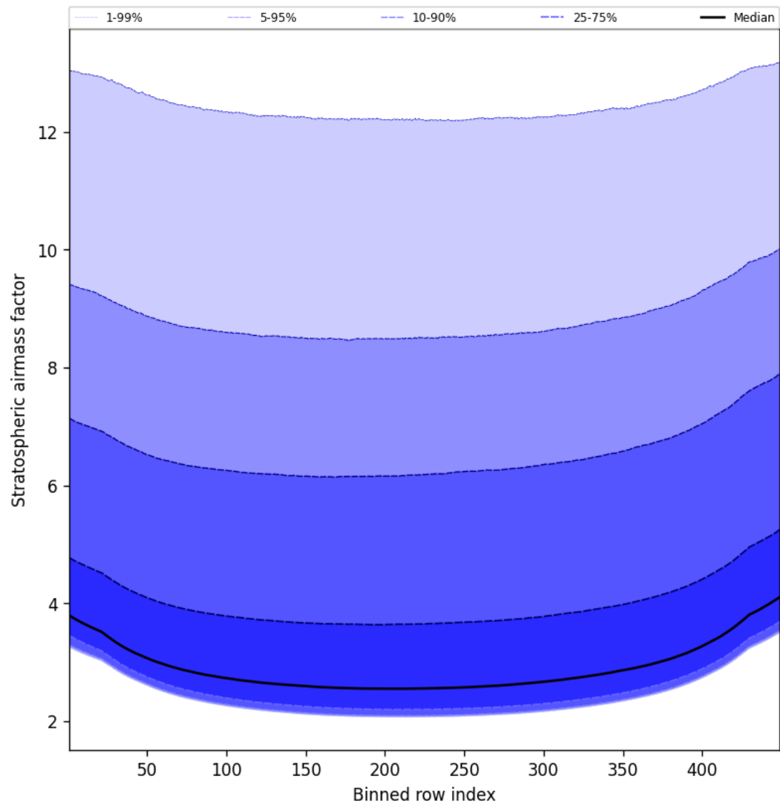
Figure 61: Along track statistics of “Stratospheric airmass factor” for 2025-11-04 to 2025-11-06
