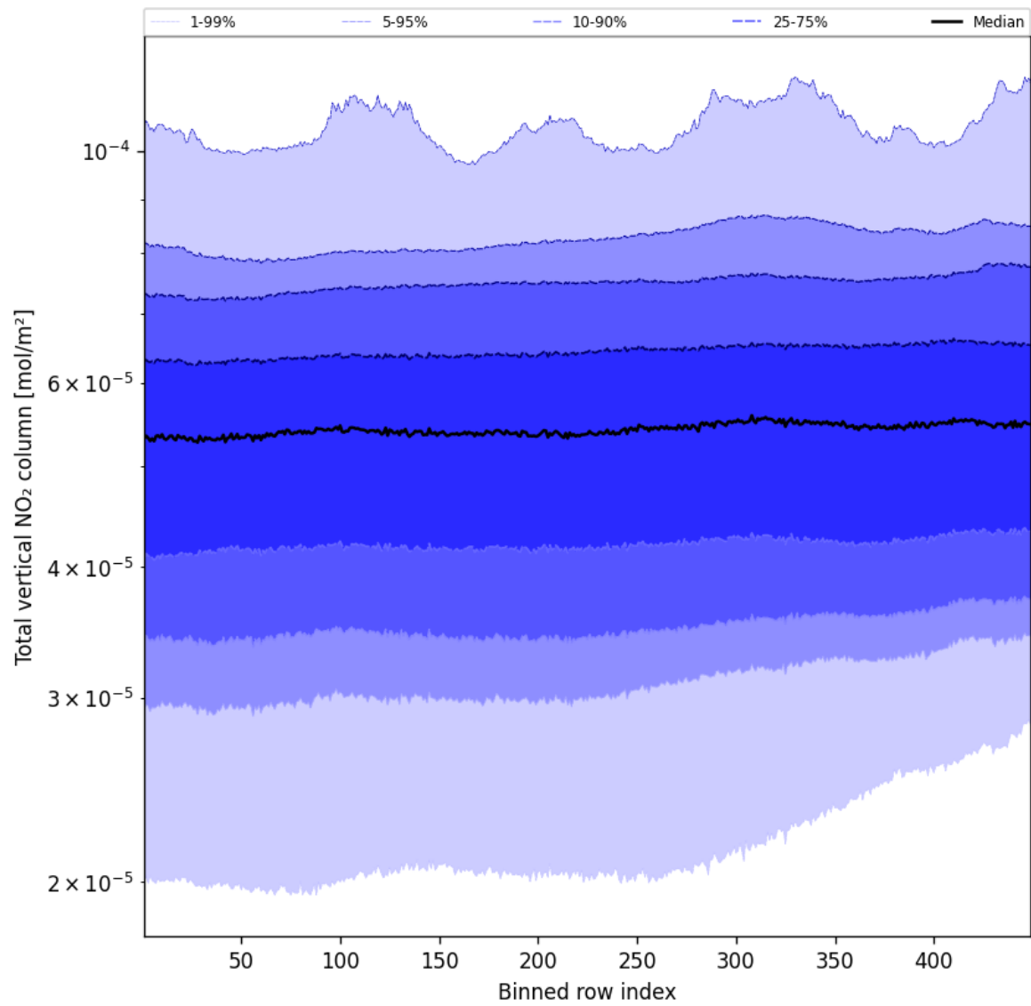
Figure 55: Along track statistics of “Total vertical NO 2 column” for 2025-11-04 to 2025-11-06
