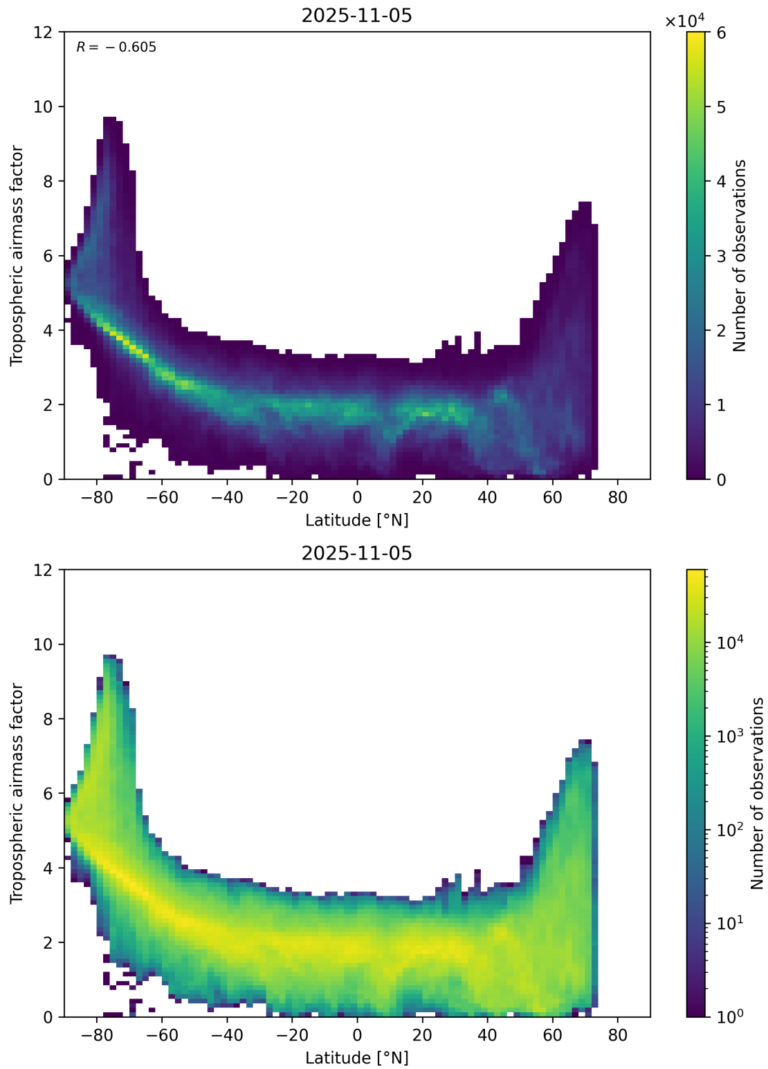
Figure 85: Scatter density plot of “Latitude” against “Tropospheric airmass factor” for 2025-11-04 to 2025-11-06.
