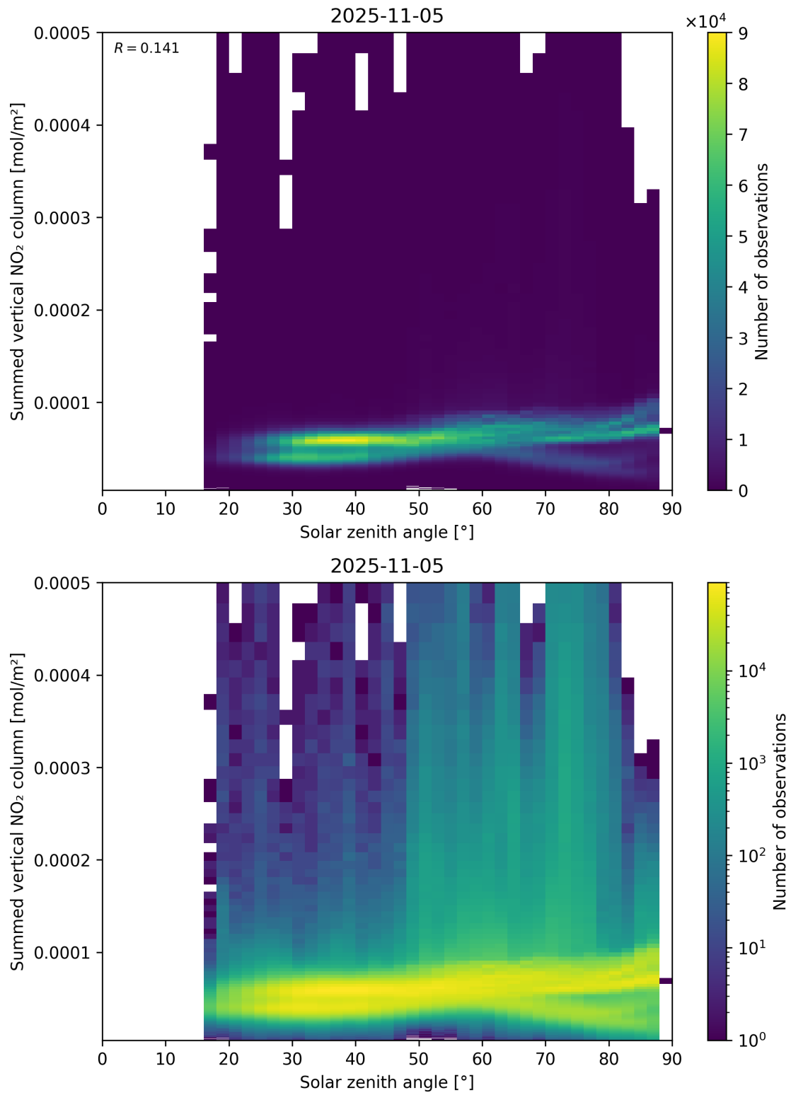
Figure 151: Scatter density plot of “Solar zenith angle” against “Summed vertical NO 2 column” for 2025-11-04 to 2025-11-06.
