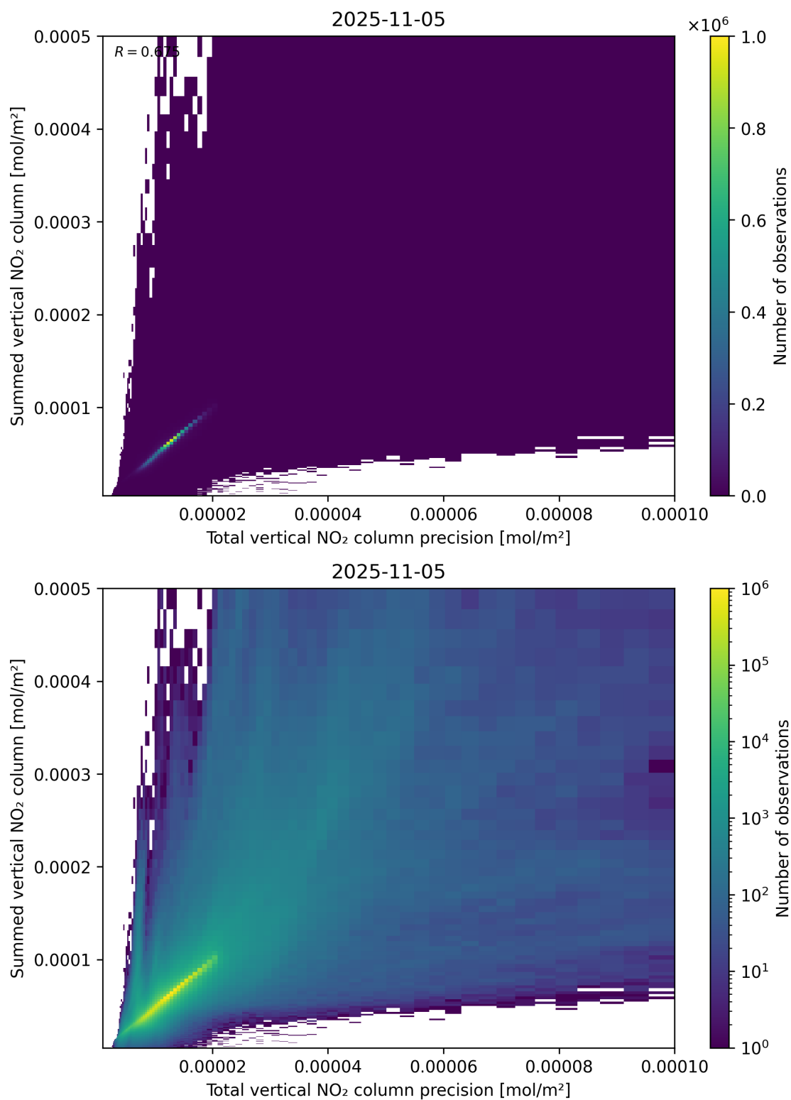
Figure 117: Scatter density plot of “Total vertical NO 2 column precision” against “Summed vertical NO 2 column” for 2025-11-04 to 2025-11-06.
