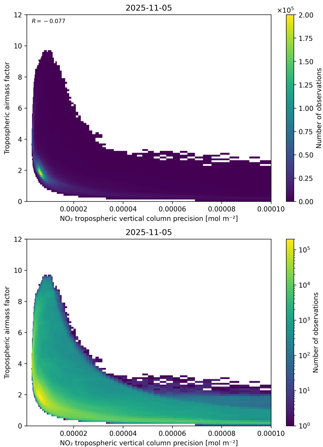
Figure 133: Scatter density plot of “NO 2 tropospheric vertical column precision” against “Tropospheric air mass factor” for 2025-11-04 to 2025-11-06.
