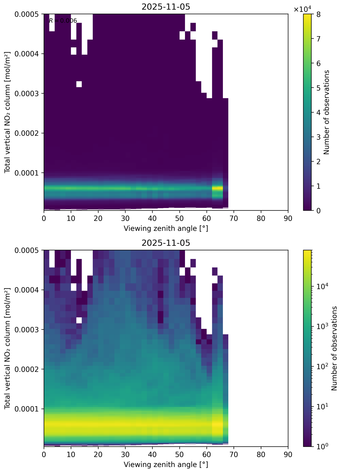
Figure 167: Scatter density plot of “Viewing zenith angle” against “Total vertical NO 2 column” for 2025-11-04 to 2025-11-06.
