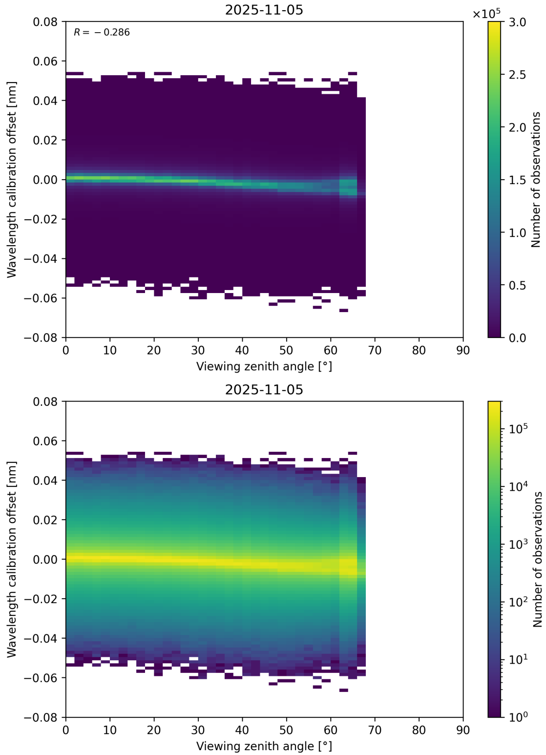
Figure 173: Scatter density plot of “Viewing zenith angle” against “Wavelength calibration offset” for 2025-11-04 to 2025-11-06.
