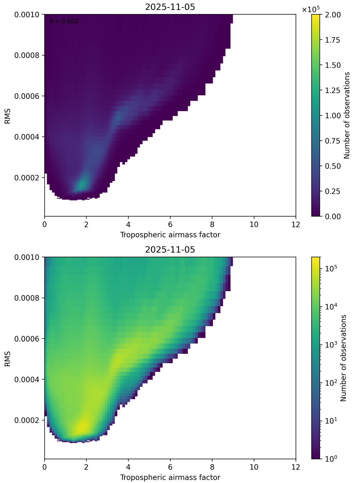
Figure 79: Scatter density plot of “Tropospheric airmass factor” against “RMS” for 2025-11-04 to 2025-11-06.
