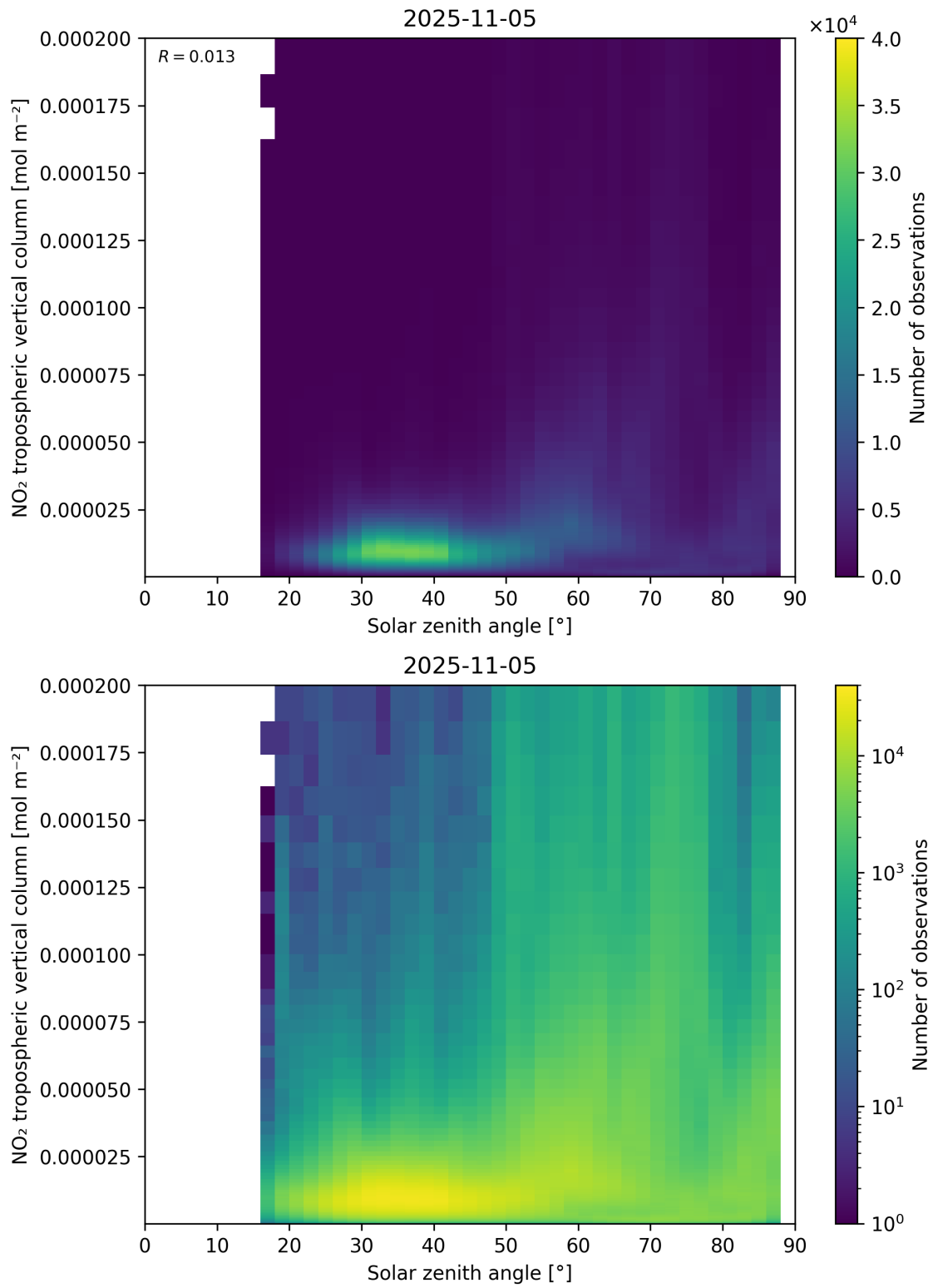
Figure 155: Scatter density plot of “Solar zenith angle” against “NO 2 tropospheric vertical column” for 2025-11-04 to 2025-11-06.
