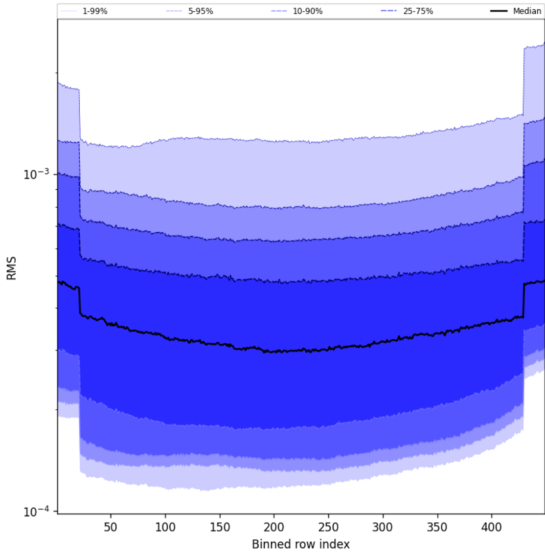
Figure 60: Along track statistics of “RMS” for 2025-11-04 to 2025-11-06
