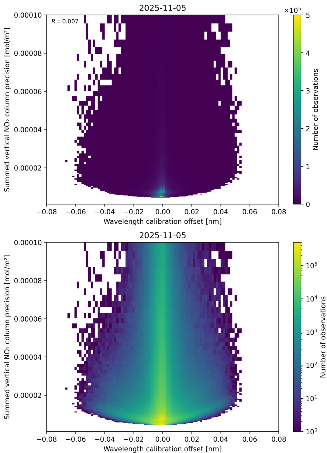
Figure 178: Scatter density plot of “Wavelength calibration offset” against “Summed vertical NO 2 column precision” for 2025-11-04 to 2025-11-06.
