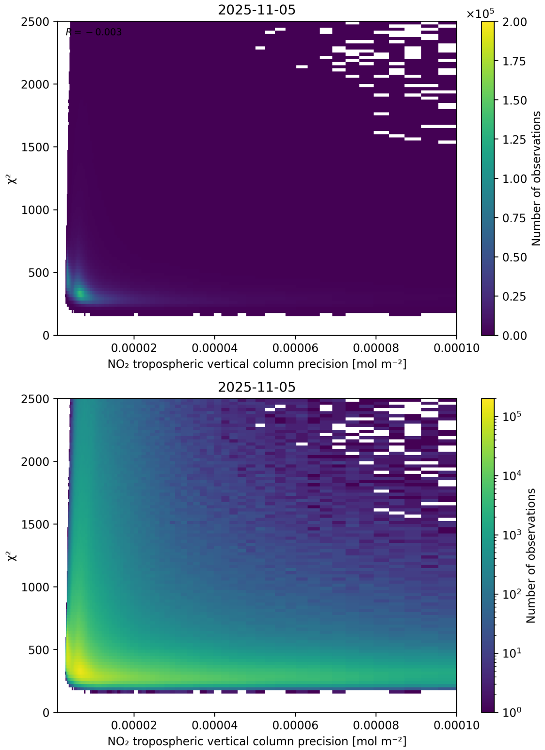
Figure 134: Scatter density plot of “NO 2 tropospheric vertical column precision” against “ \chi^2 ” for 2025-11-04 to 2025-11-06.
