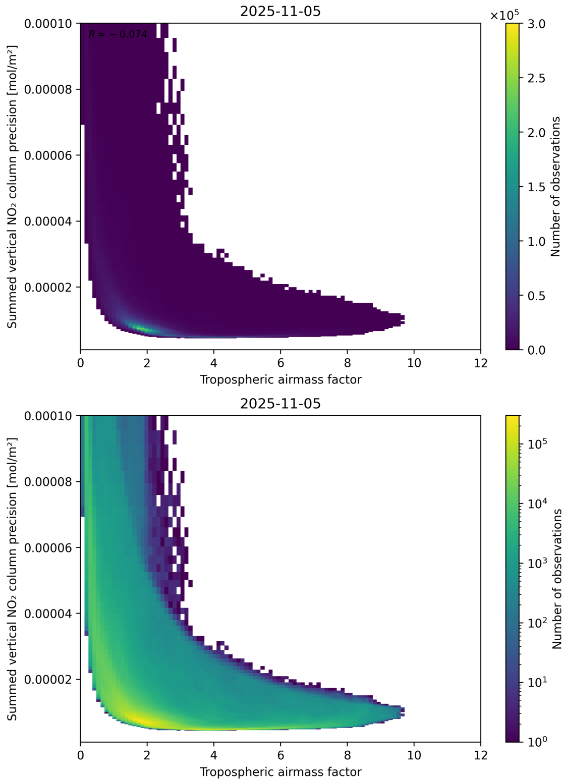
Figure 76: Scatter density plot of “Tropospheric air mass factor” against “Summed vertical NO 2 column precision” for 2025-11-04 to 2025-11-06.
