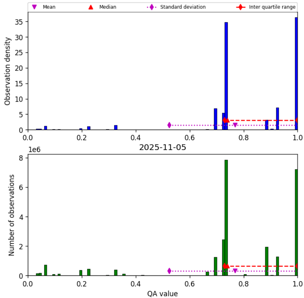
Figure 28: Histogram of “QA value” for 2025-11-04 to 2025-11-06
