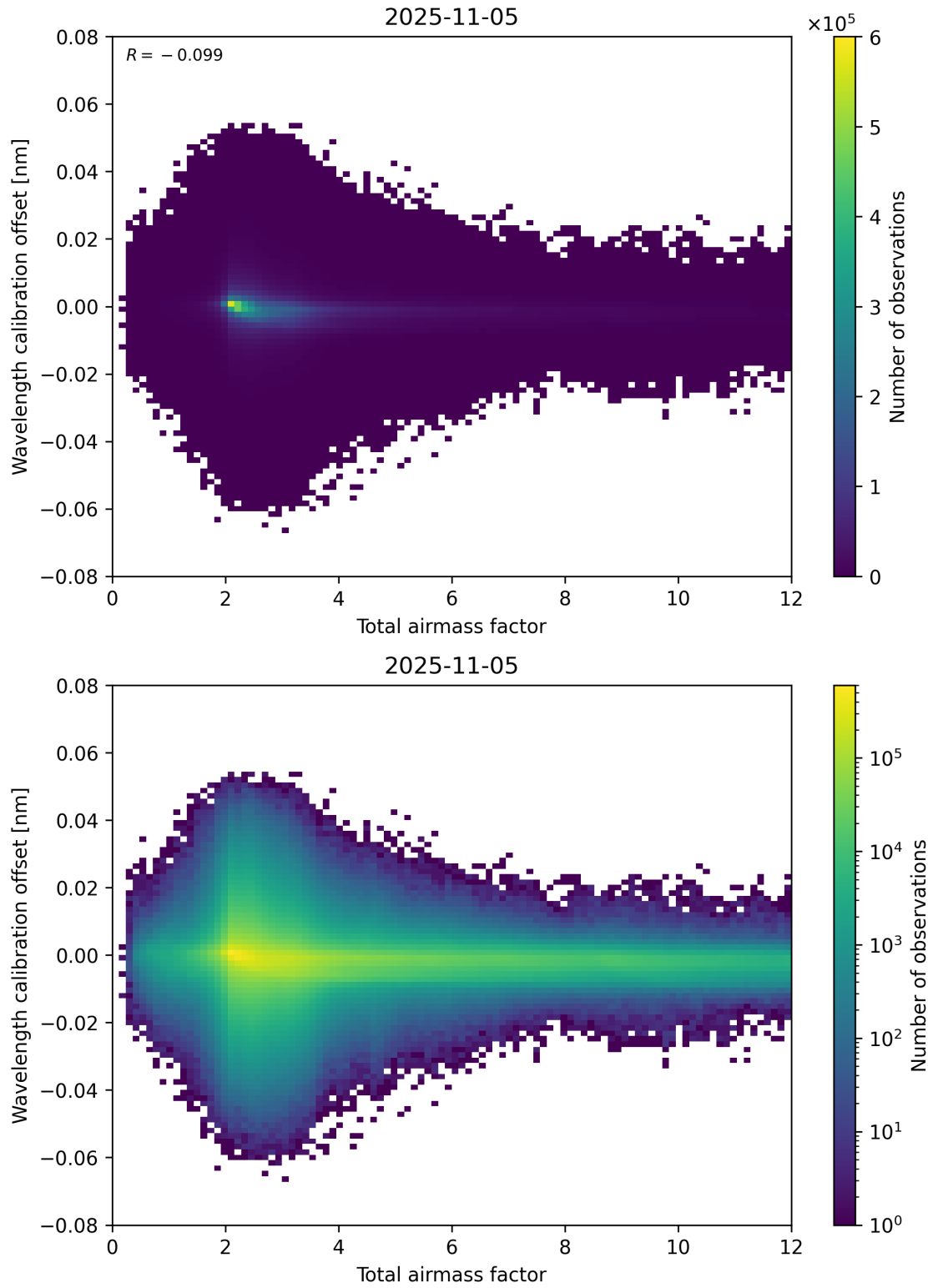
Figure 70: Scatter density plot of “Total airmass factor” against “Wavelength calibration offset” for 2025-11-04 to 2025-11-06.
