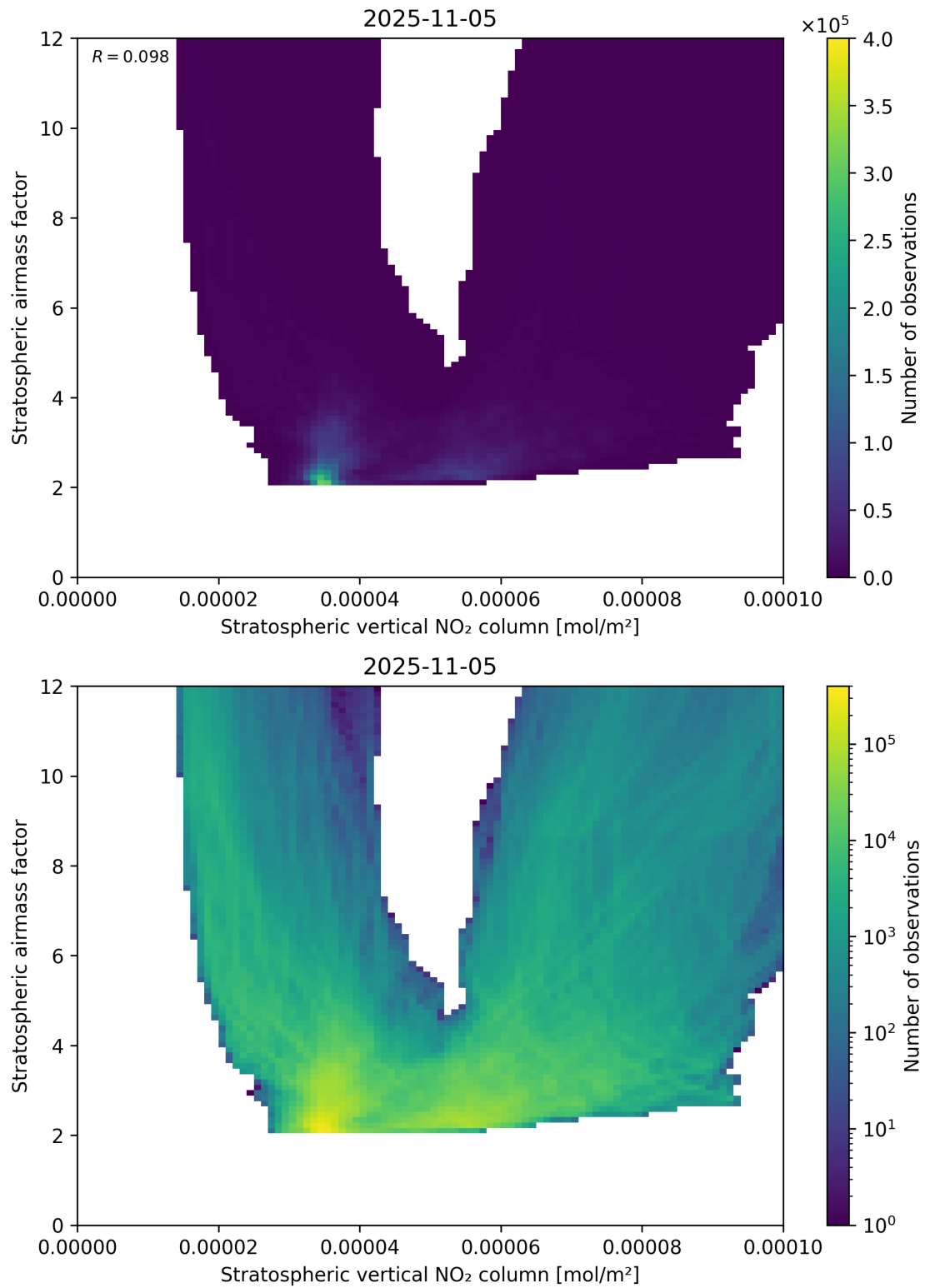
Figure 96: Scatter density plot of “Stratospheric vertical NO 2 column” against “Stratospheric airmass factor” for 2025-11-04 to 2025-11-06.
