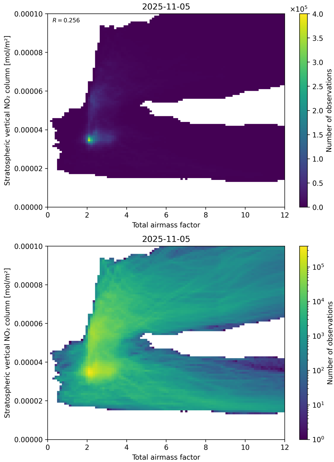
Figure 64: Scatter density plot of “Total airmass factor” against “Stratospheric vertical NO 2 column” for 2025-11-04 to 2025-11-06.
