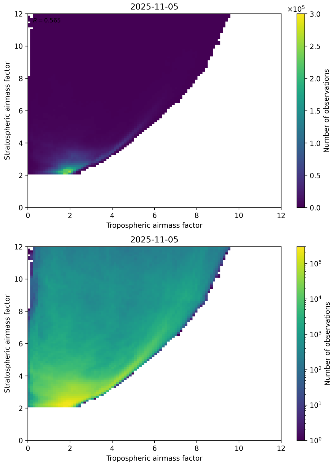
Figure 71: Scatter density plot of “Tropospheric airmass factor” against “Stratospheric airmass factor” for 2025-11-04 to 2025-11-06.
