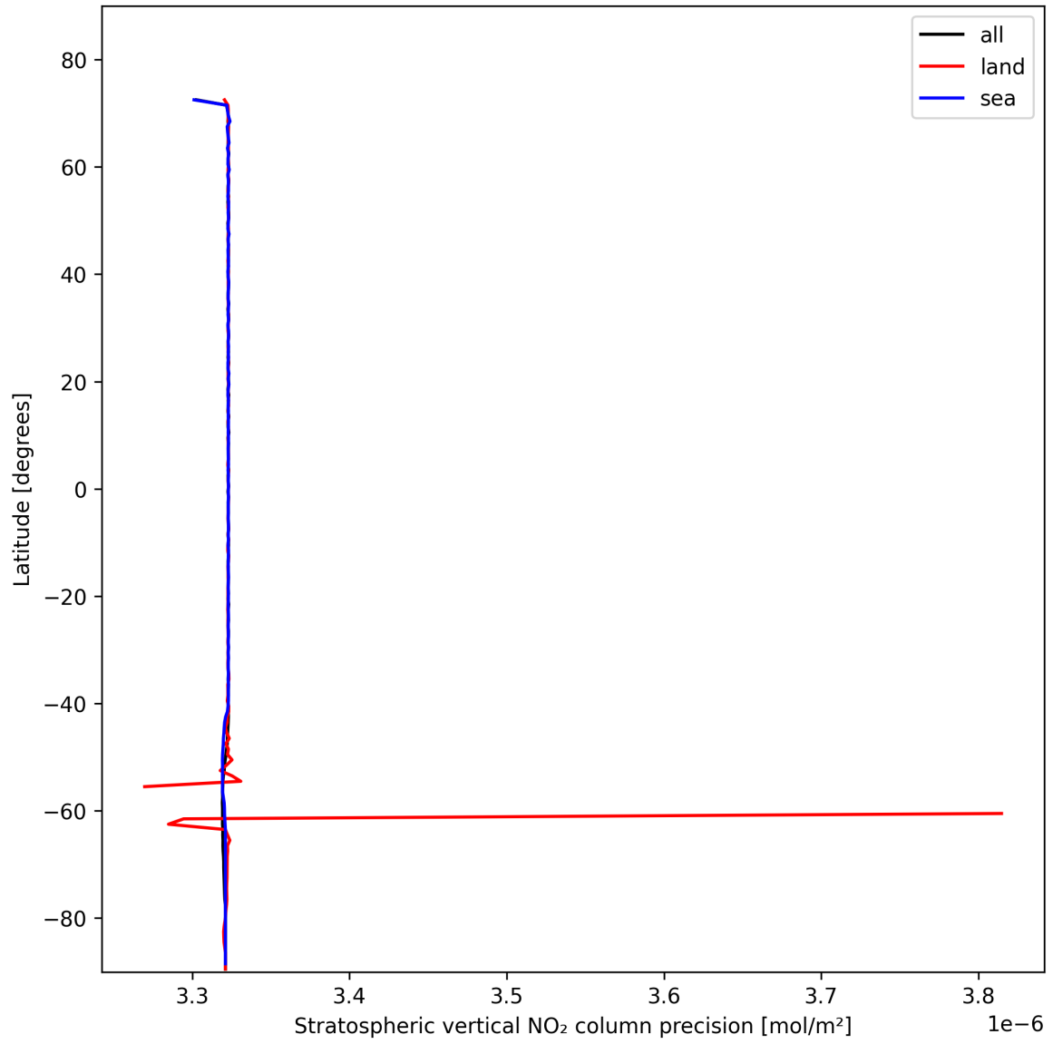
Figure 20: Zonal average of “Stratospheric vertical NO 2 column precision” for 2025-11-04 to 2025-11-06.
