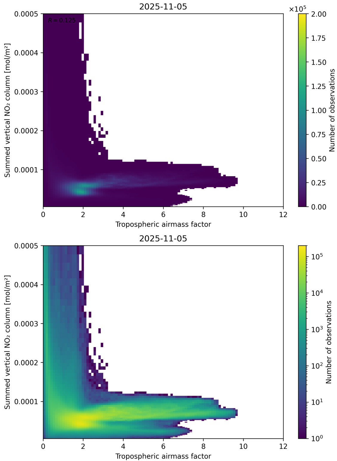
Figure 75: Scatter density plot of “Tropospheric air mass factor” against “Summed vertical NO 2 column” for 2025-11-04 to 2025-11-06.
