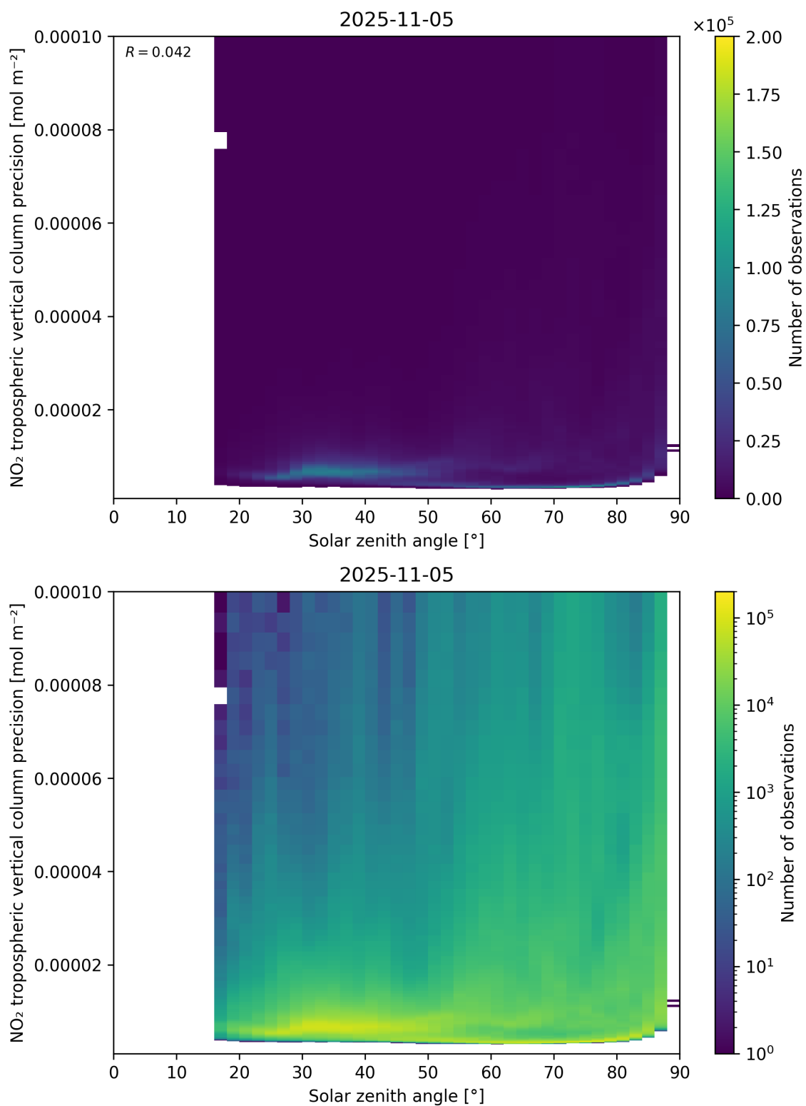
Figure 156: Scatter density plot of “Solar zenith angle” against “NO 2 tropospheric vertical column precision” for 2025-11-04 to 2025-11-06.
