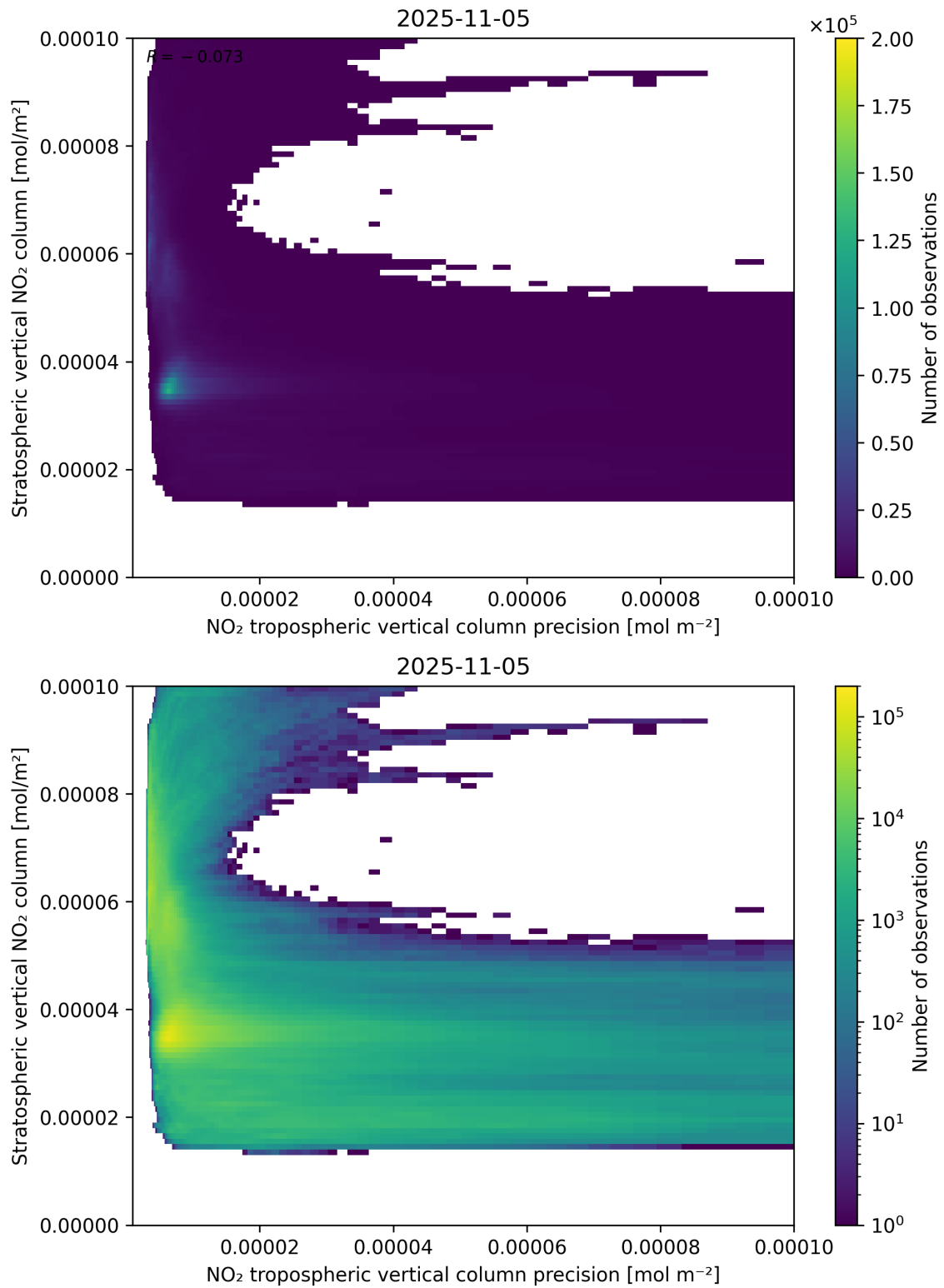
Figure 135: Scatter density plot of “NO 2 tropospheric vertical column precision” against “Stratospheric vertical NO 2 column” for 2025-11-04 to 2025-11-06.
