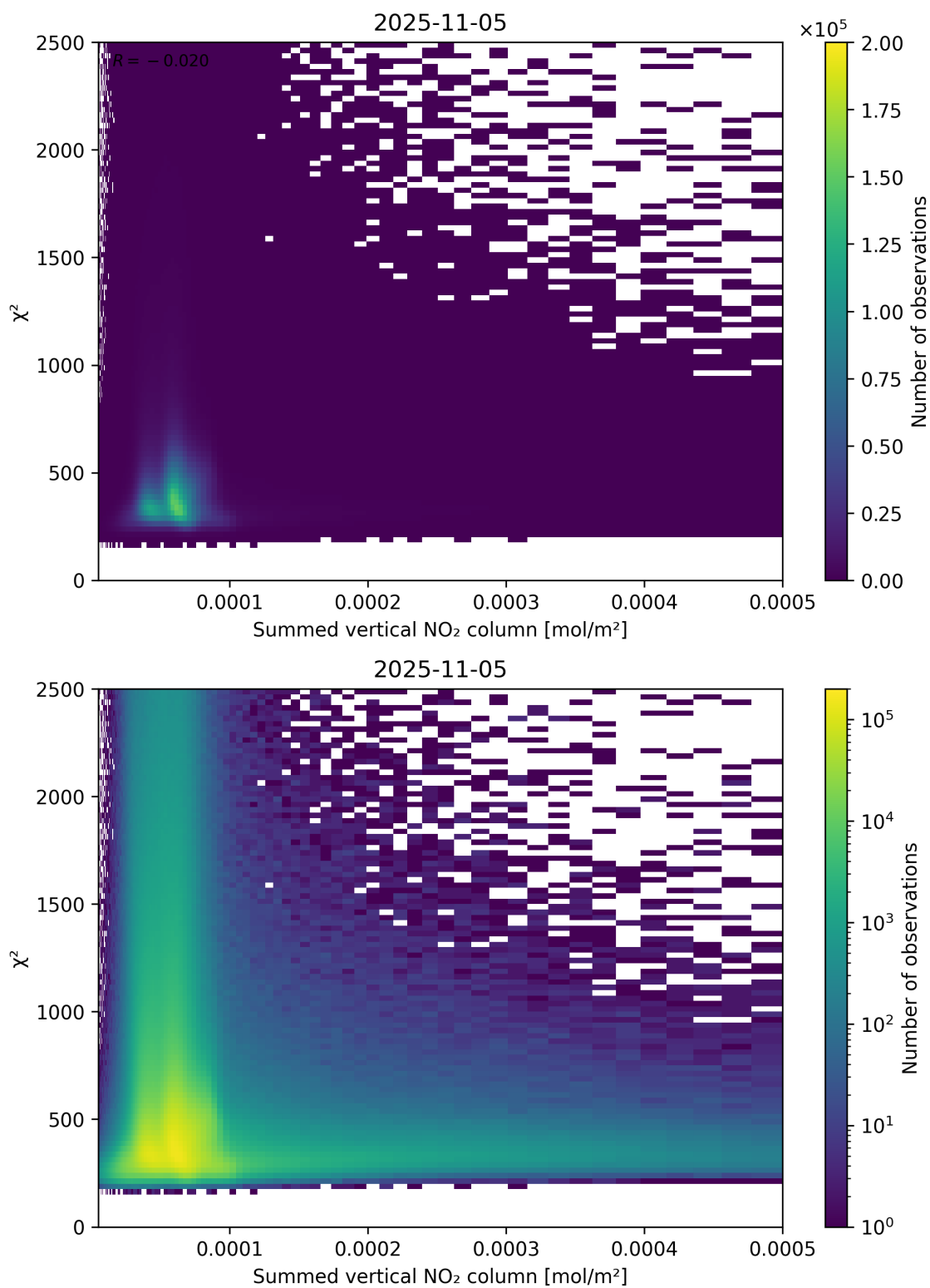
Figure 104: Scatter density plot of “Summed vertical NO 2 column” against “ \chi^2 ” for 2025-11-04 to 2025-11-06.
