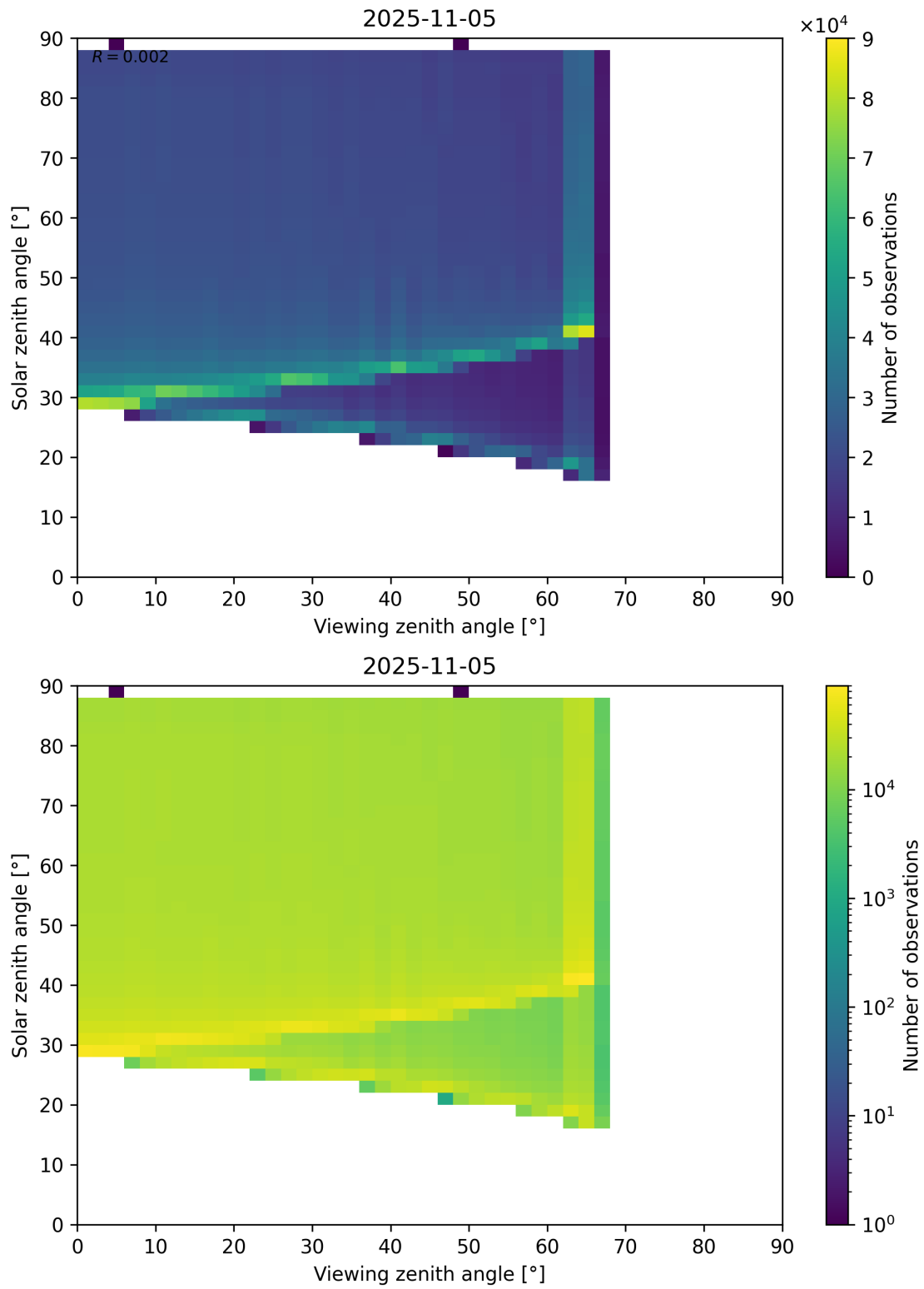
Figure 172: Scatter density plot of “Viewing zenith angle” against “Solar zenith angle” for 2025-11-04 to 2025-11-06.
