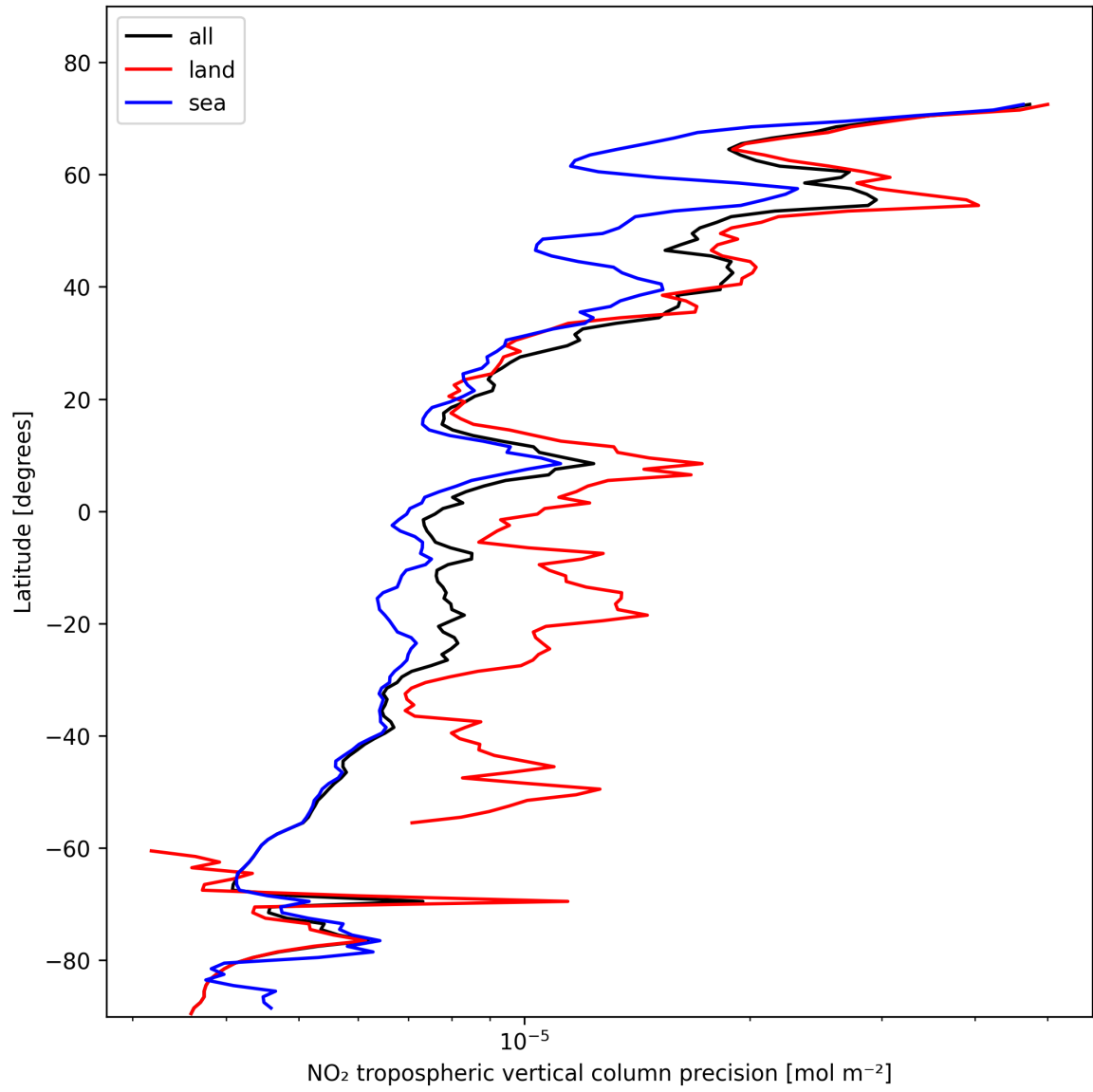
Figure 13: Zonal average of “NO 2 tropospheric vertical column precision” for 2025-11-04 to 2025-11-06.
