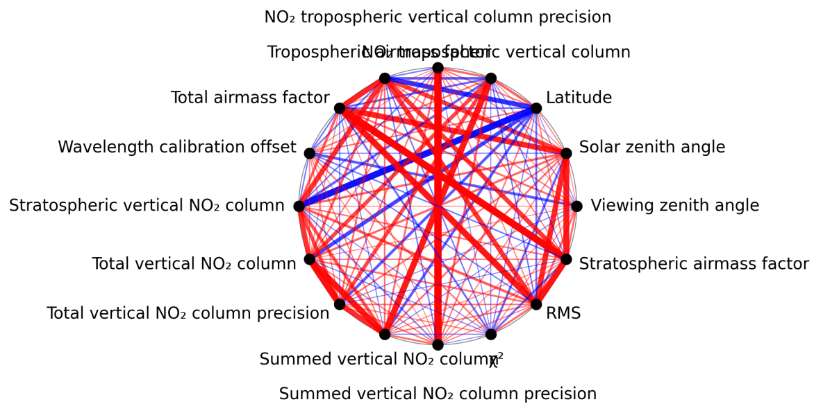
Figure 1: Map of correlation graph for 2025-11-04 to 2025-11-06.
