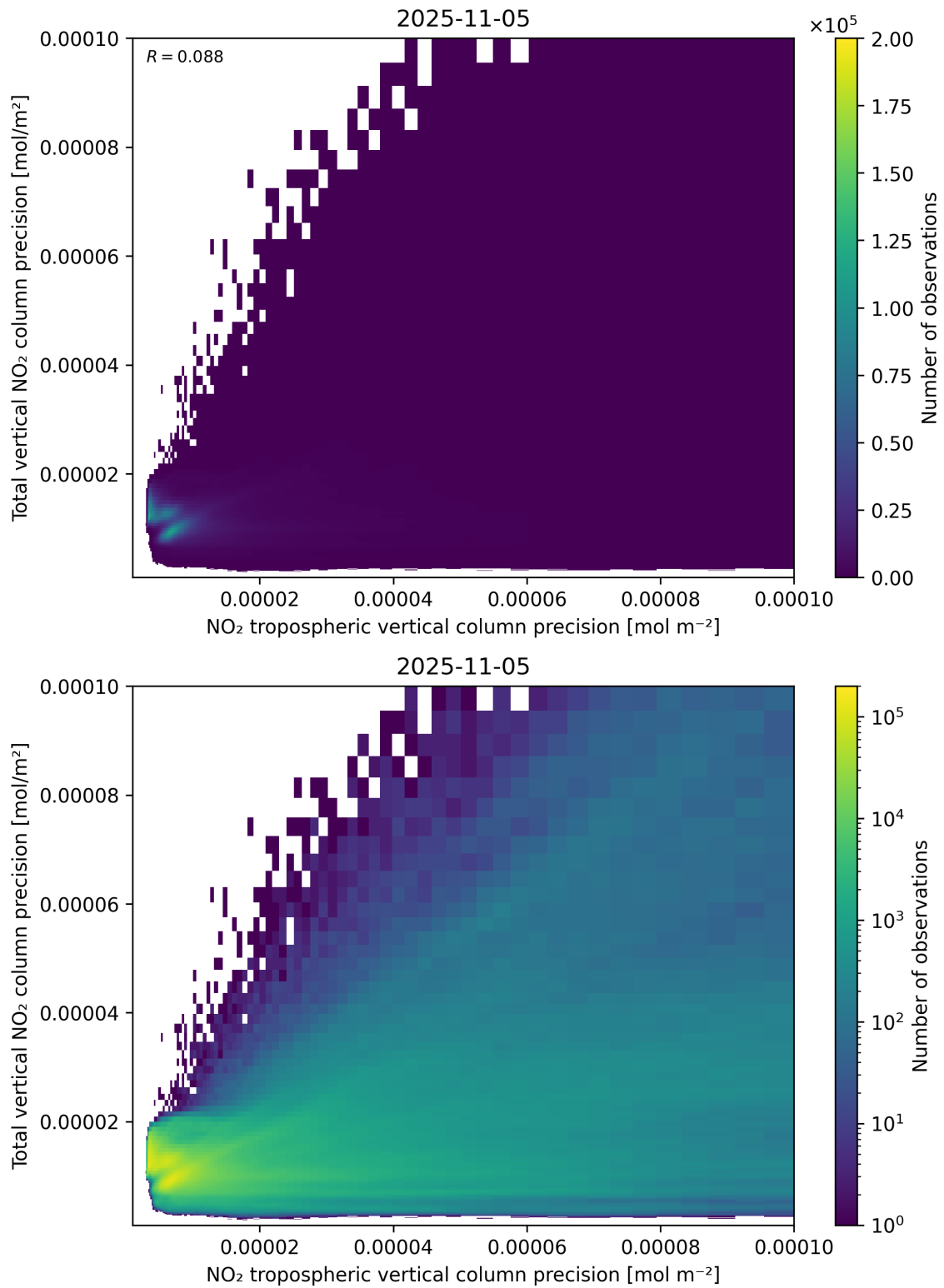
Figure 139: Scatter density plot of “NO 2 tropospheric vertical column precision” against “Total vertical NO 2 column precision” for 2025-11-04 to 2025-11-06.
