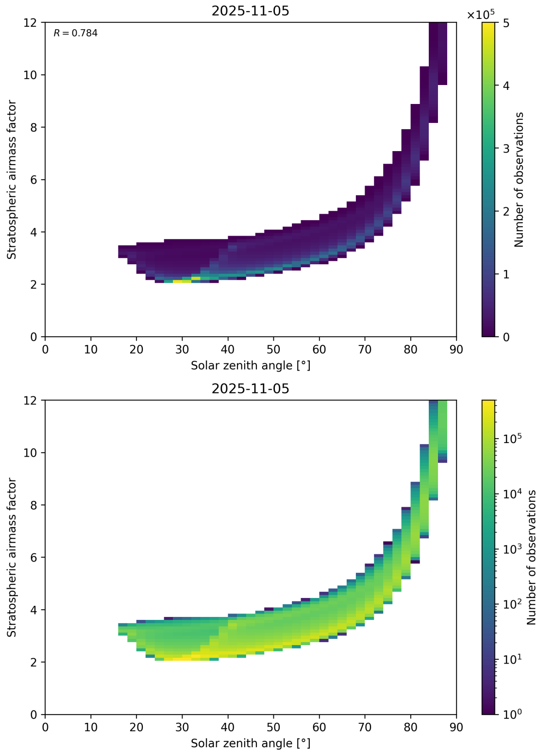
Figure 145: Scatter density plot of “Solar zenith angle” against “Stratospheric airmass factor” for 2025-11-04 to 2025-11-06.
