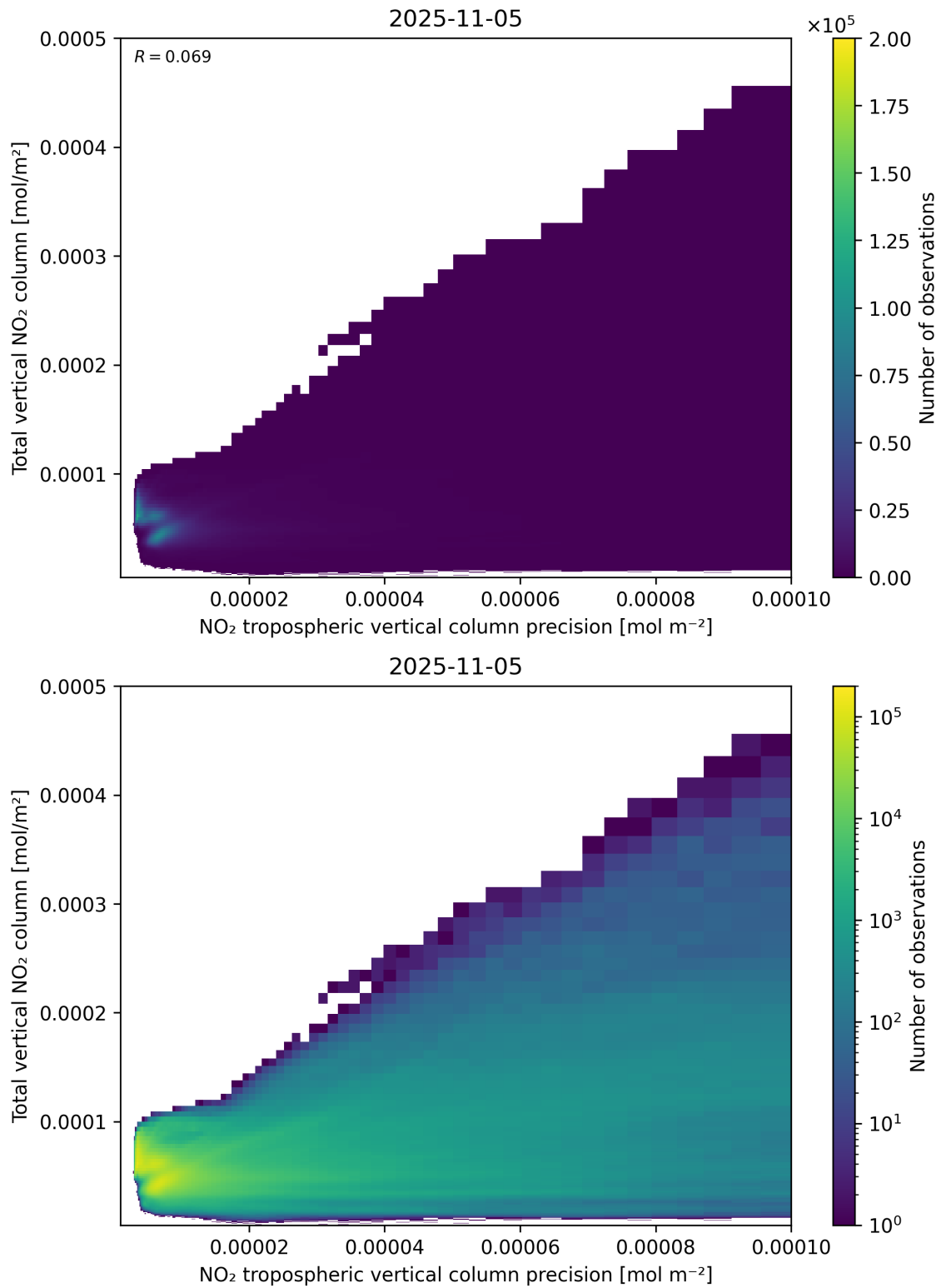
Figure 138: Scatter density plot of “NO 2 tropospheric vertical column precision” against “Total vertical NO 2 column” for 2025-11-04 to 2025-11-06.
