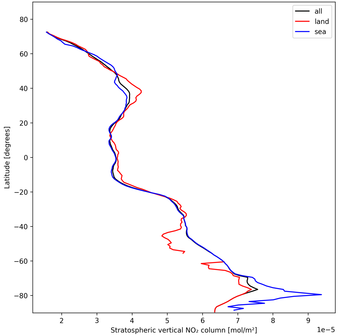
Figure 19: Zonal average of “Stratospheric vertical NO 2 column” for 2025-11-04 to 2025-11-06.
