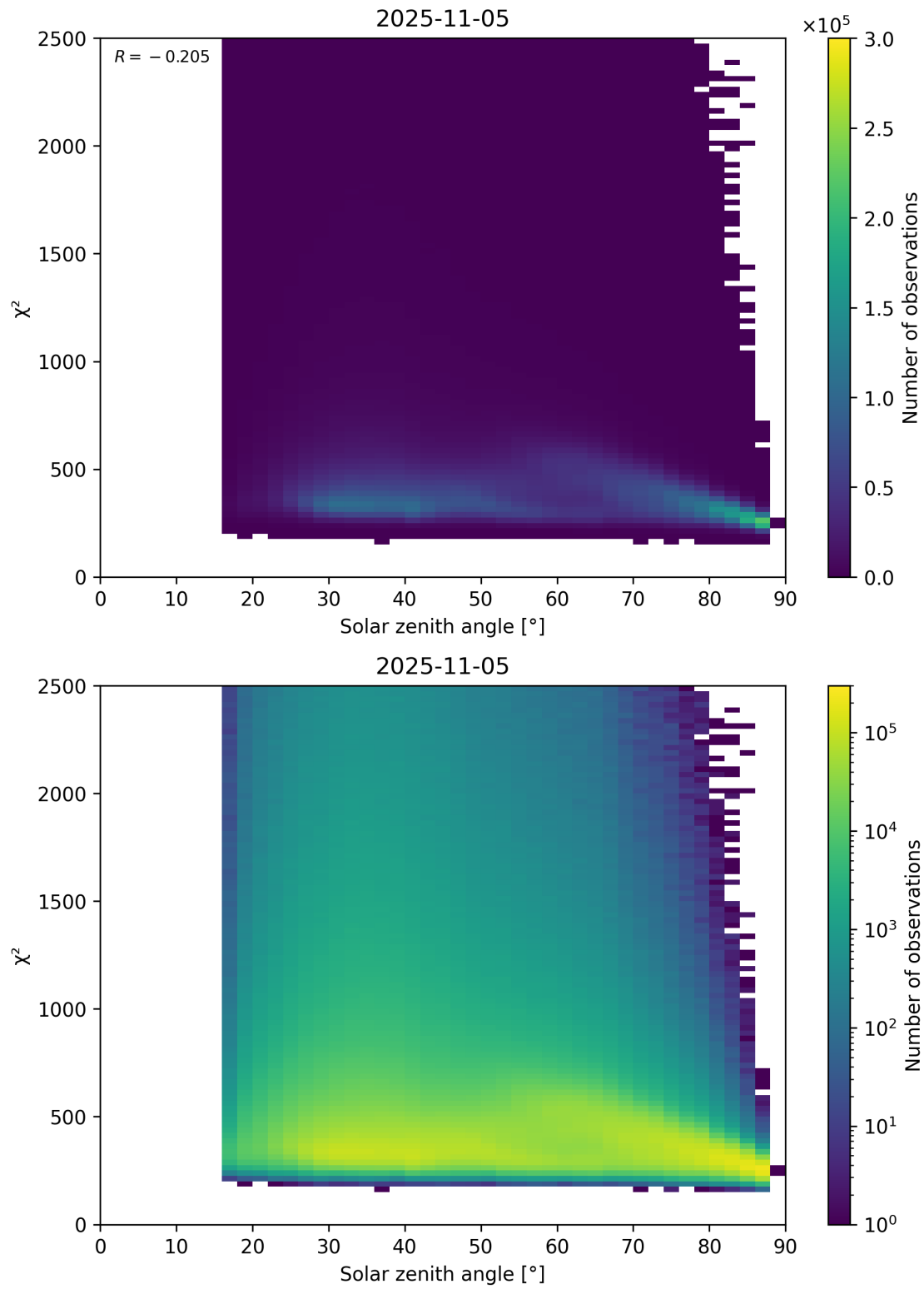
Figure 148: Scatter density plot of “Solar zenith angle” against “ \chi^2 ” for 2025-11-04 to 2025-11-06.
