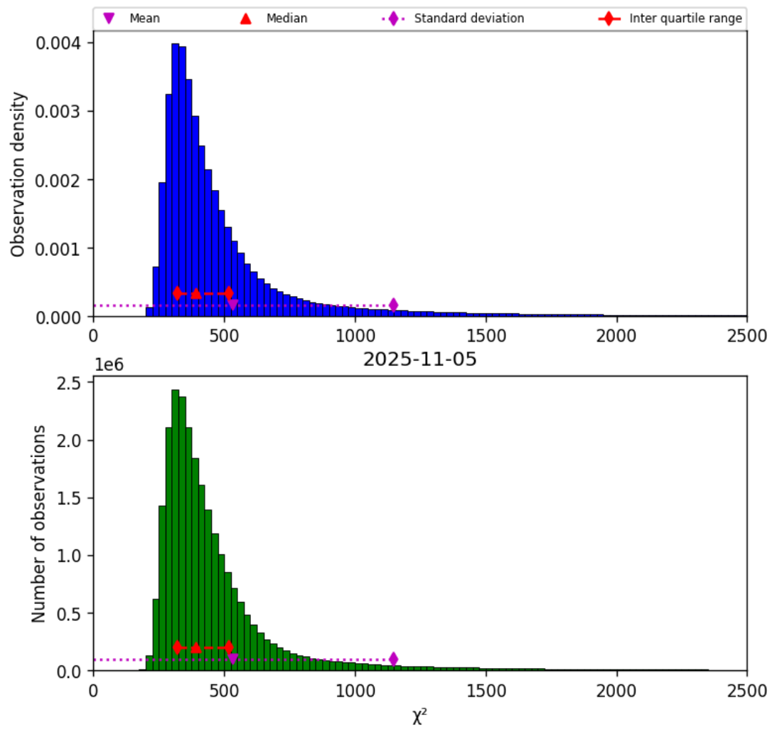
Figure 42: Histogram of “ \chi^2 ” for 2025-11-04 to 2025-11-06
