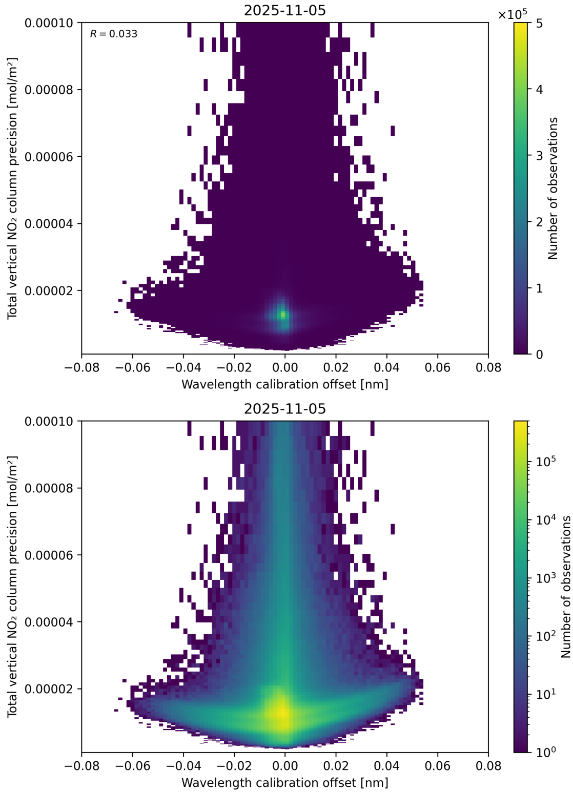
Figure 180: Scatter density plot of “Wavelength calibration offset” against “Total vertical NO 2 column precision” for 2025-11-04 to 2025-11-06.
