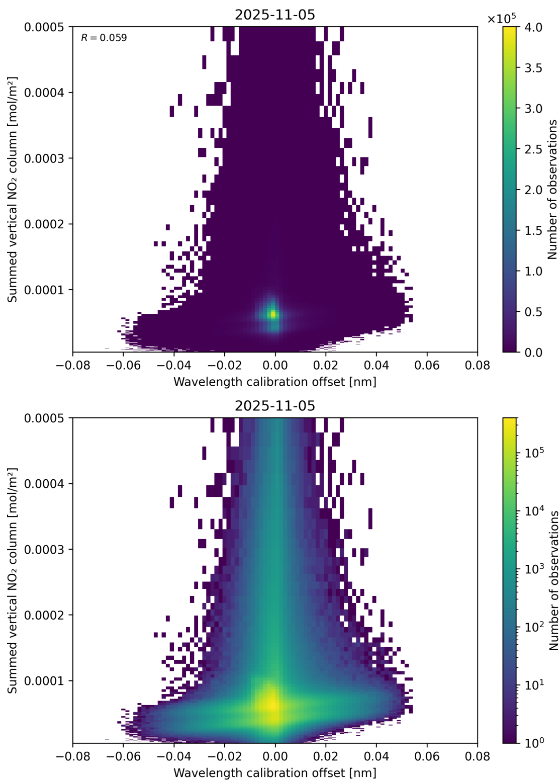
Figure 177: Scatter density plot of “Wavelength calibration offset” against “Summed vertical NO 2 column” for 2025-11-04 to 2025-11-06.
