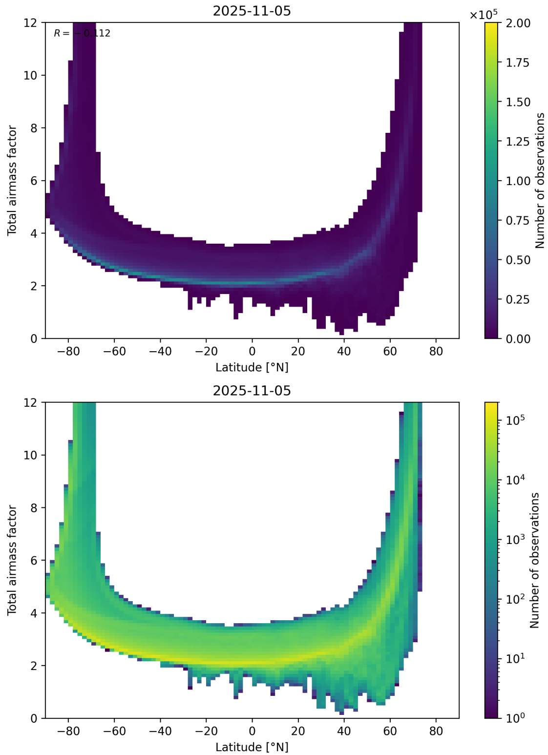
Figure 84: Scatter density plot of “Latitude” against “Total airmass factor” for 2025-11-04 to 2025-11-06.
