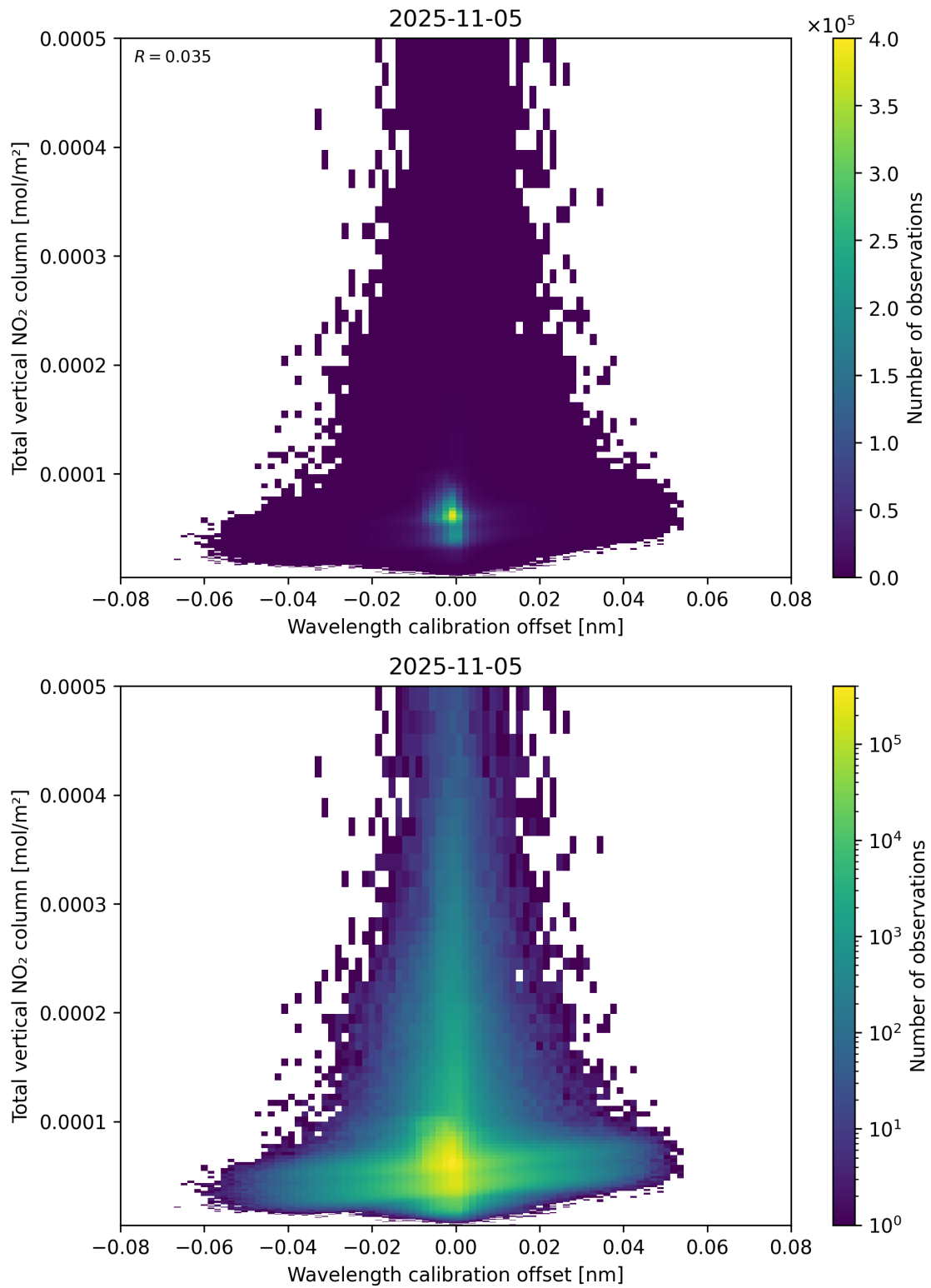
Figure 179: Scatter density plot of “Wavelength calibration offset” against “Total vertical NO 2 column” for 2025-11-04 to 2025-11-06.
