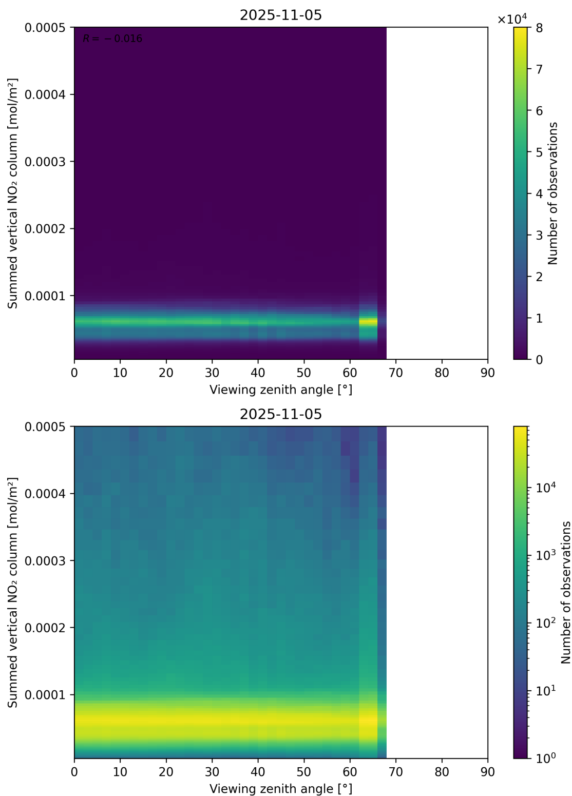
Figure 165: Scatter density plot of “Viewing zenith angle” against “Summed vertical NO 2 column” for 2025-11-04 to 2025-11-06.
