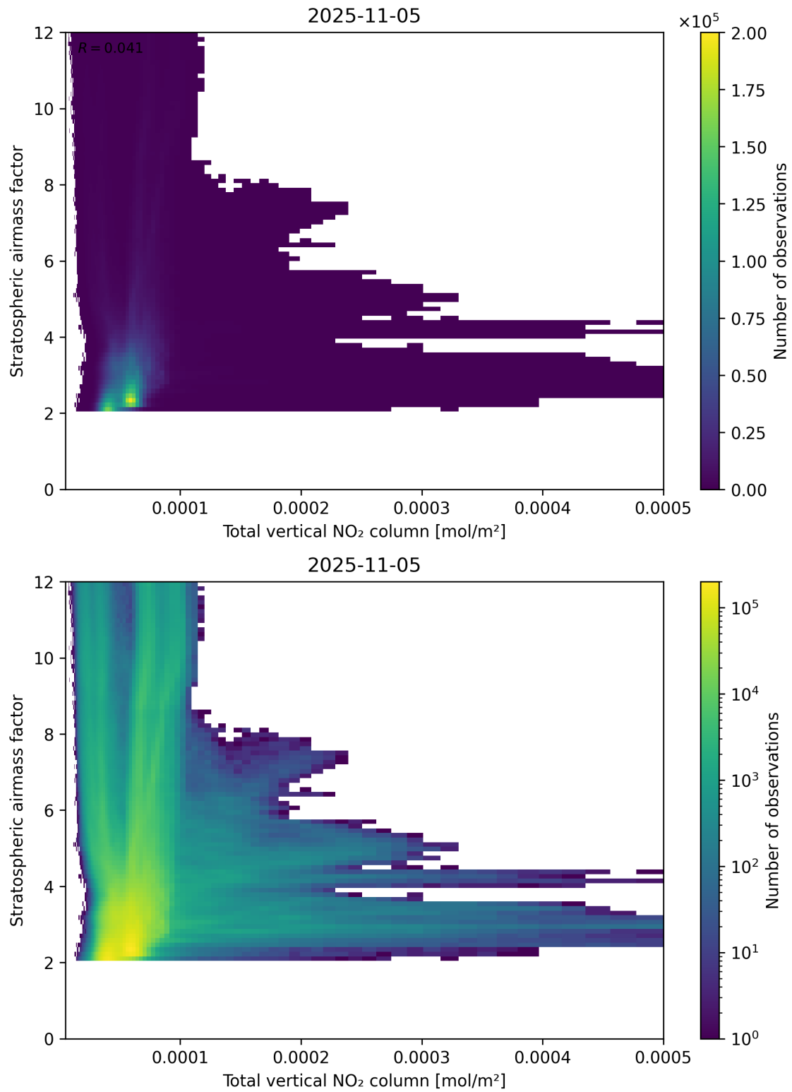
Figure 110: Scatter density plot of “Total vertical NO 2 column” against “Stratospheric airmass factor” for 2025-11-04 to 2025-11-06.
