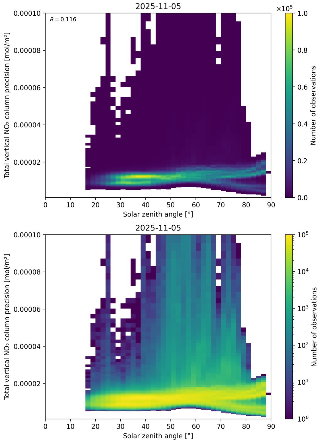
Figure 154: Scatter density plot of “Solar zenith angle” against “Total vertical NO 2 column precision” for 2025-11-04 to 2025-11-06.
