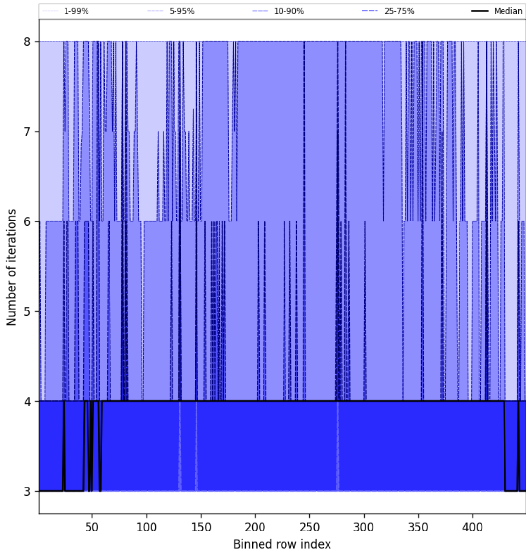
Figure 51: Along track statistics of “Number of iterations” for 2025-11-04 to 2025-11-06
