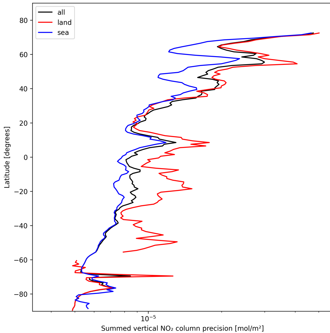
Figure 24: Zonal average of “Summed vertical NO 2 column precision” for 2025-11-04 to 2025-11-06.
