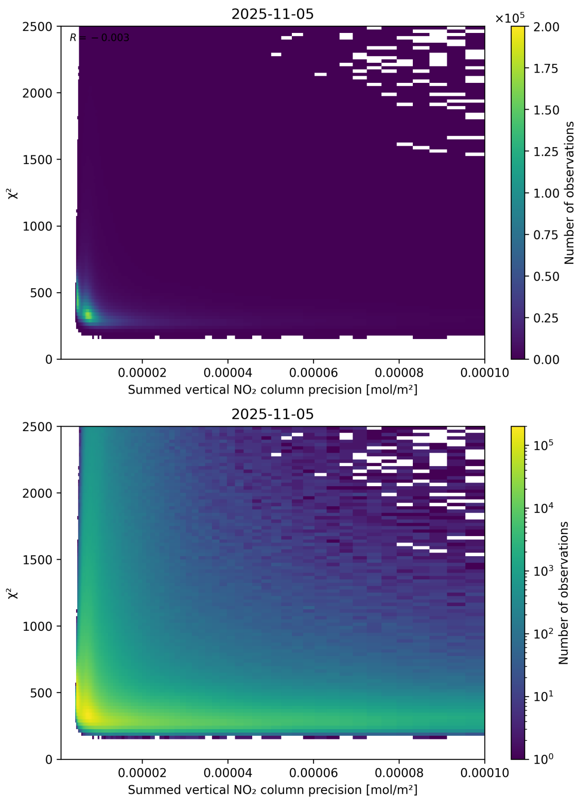
Figure 107: Scatter density plot of “Summed vertical NO 2 column precision” against “ \chi^2 ” for 2025-11-04 to 2025-11-06.
