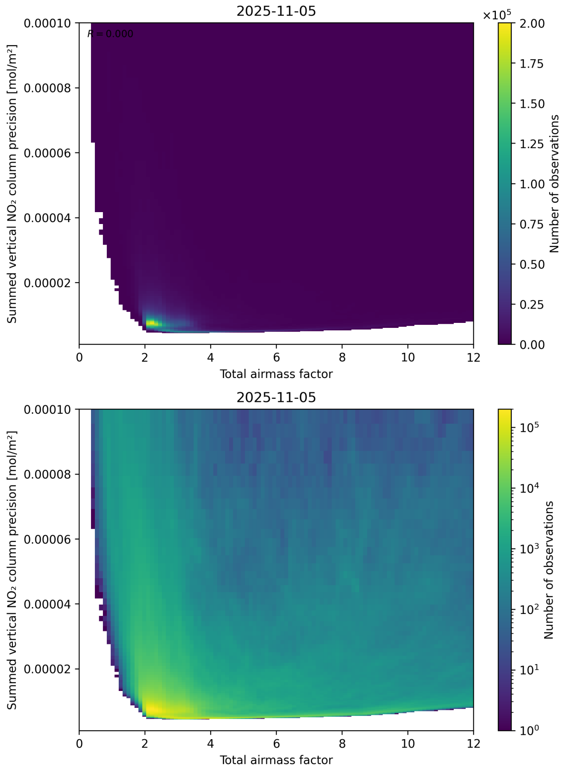
Figure 66: Scatter density plot of “Total airmass factor” against “Summed vertical NO 2 column precision” for 2025-11-04 to 2025-11-06.
