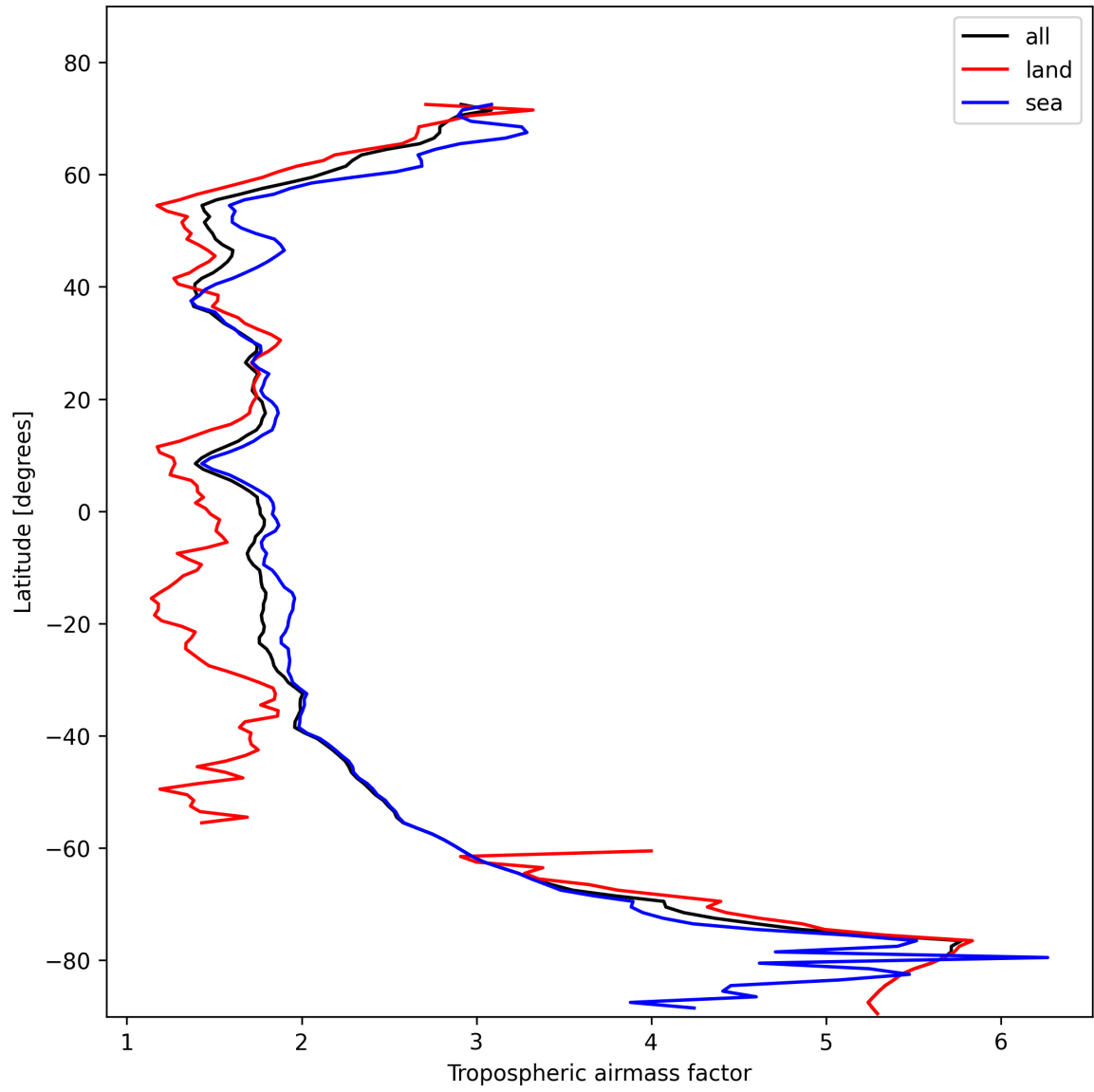
Figure 14: Zonal average of “Tropospheric airmass factor” for 2025-11-04 to 2025-11-06.
