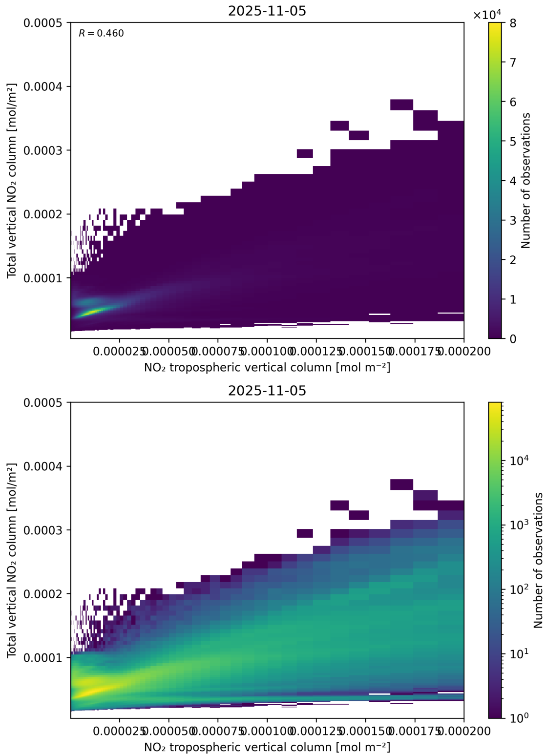
Figure 128: Scatter density plot of “NO 2 tropospheric vertical column” against “Total vertical NO 2 column” for 2025-11-04 to 2025-11-06.
