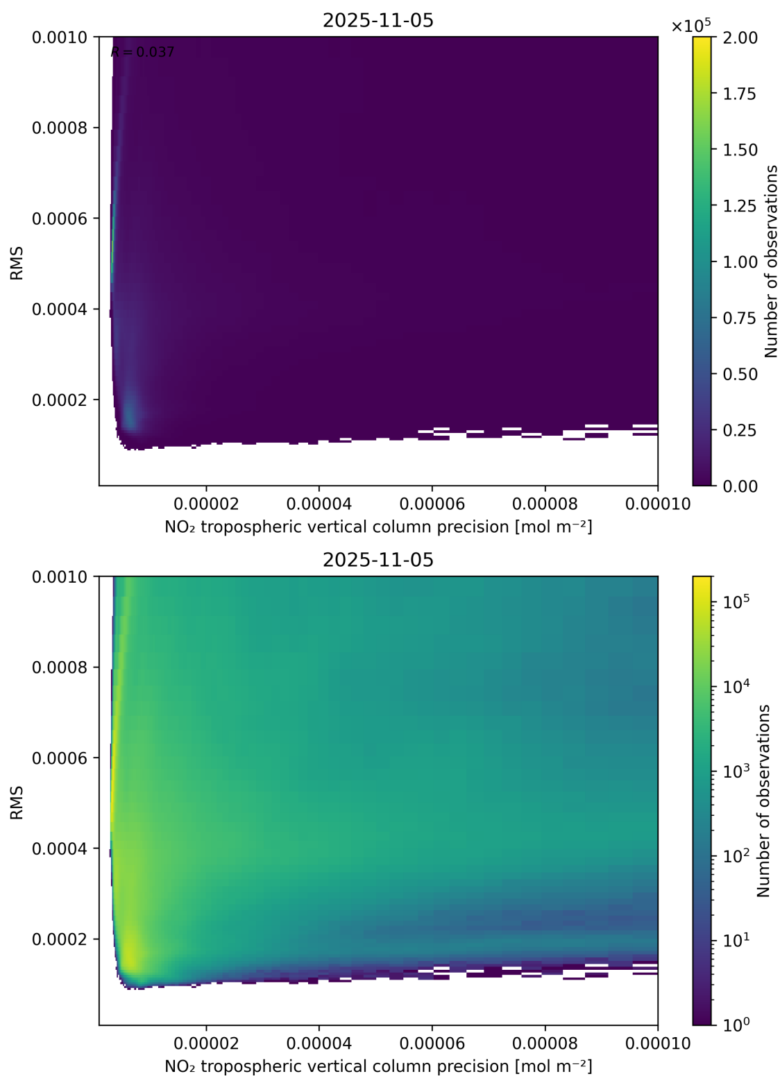
Figure 140: Scatter density plot of “NO 2 tropospheric vertical column precision” against “RMS” for 2025-11-04 to 2025-11-06.
