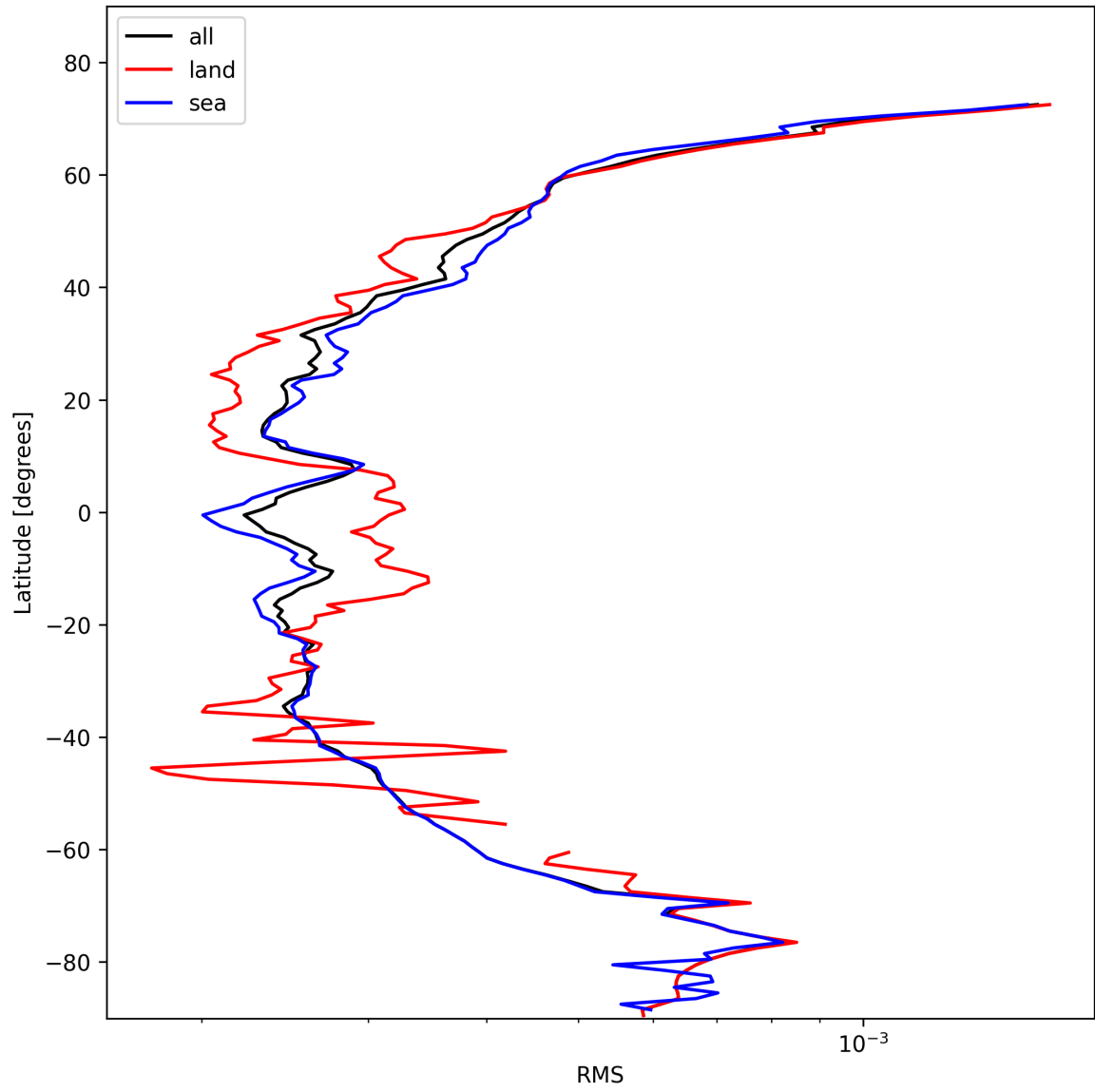
Figure 26: Zonal average of “RMS” for 2025-11-04 to 2025-11-06.
