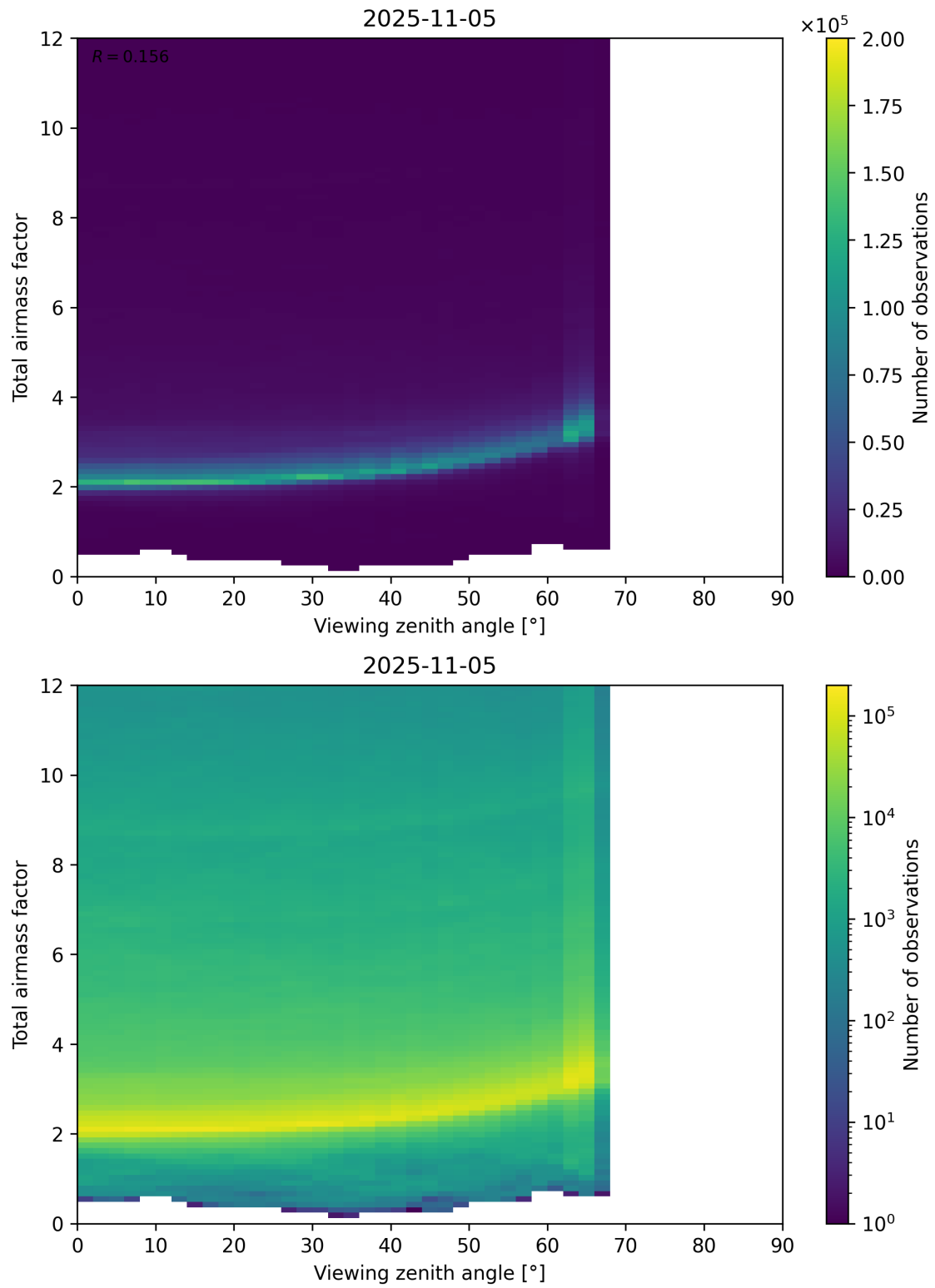
Figure 160: Scatter density plot of “Viewing zenith angle” against “Total airmass factor” for 2025-11-04 to 2025-11-06.
