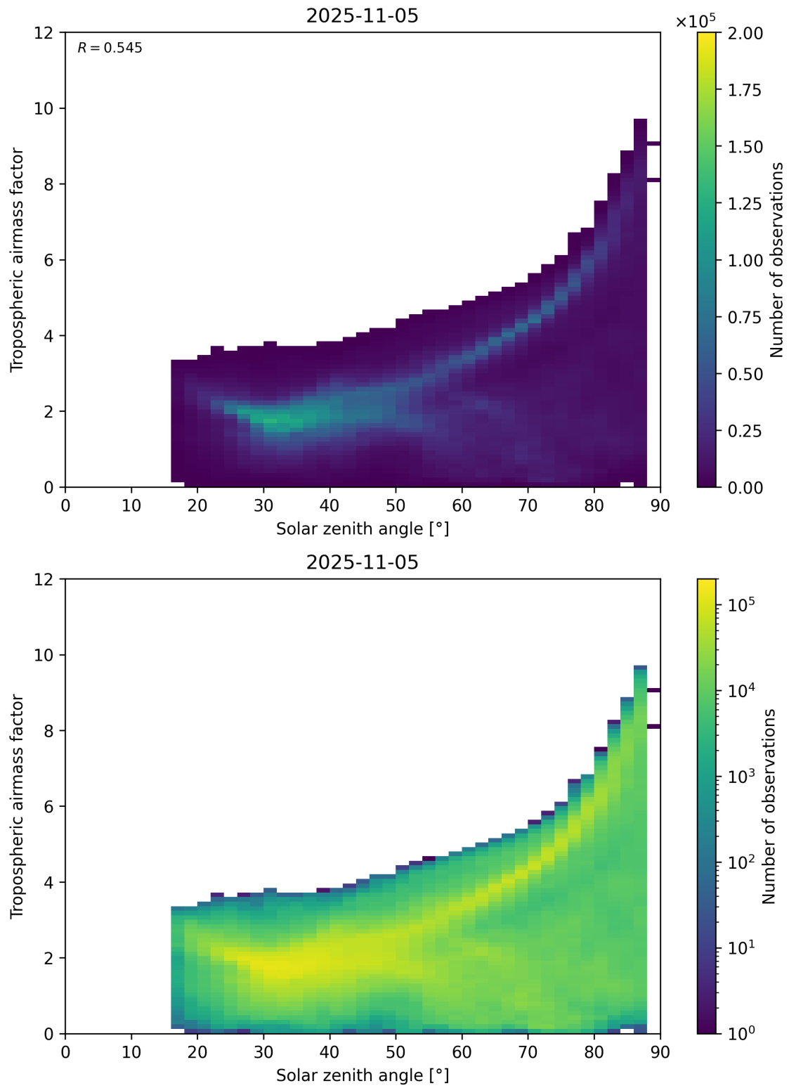
Figure 147: Scatter density plot of “Solar zenith angle” against “Tropospheric airmass factor” for 2025-11-04 to 2025-11-06.
