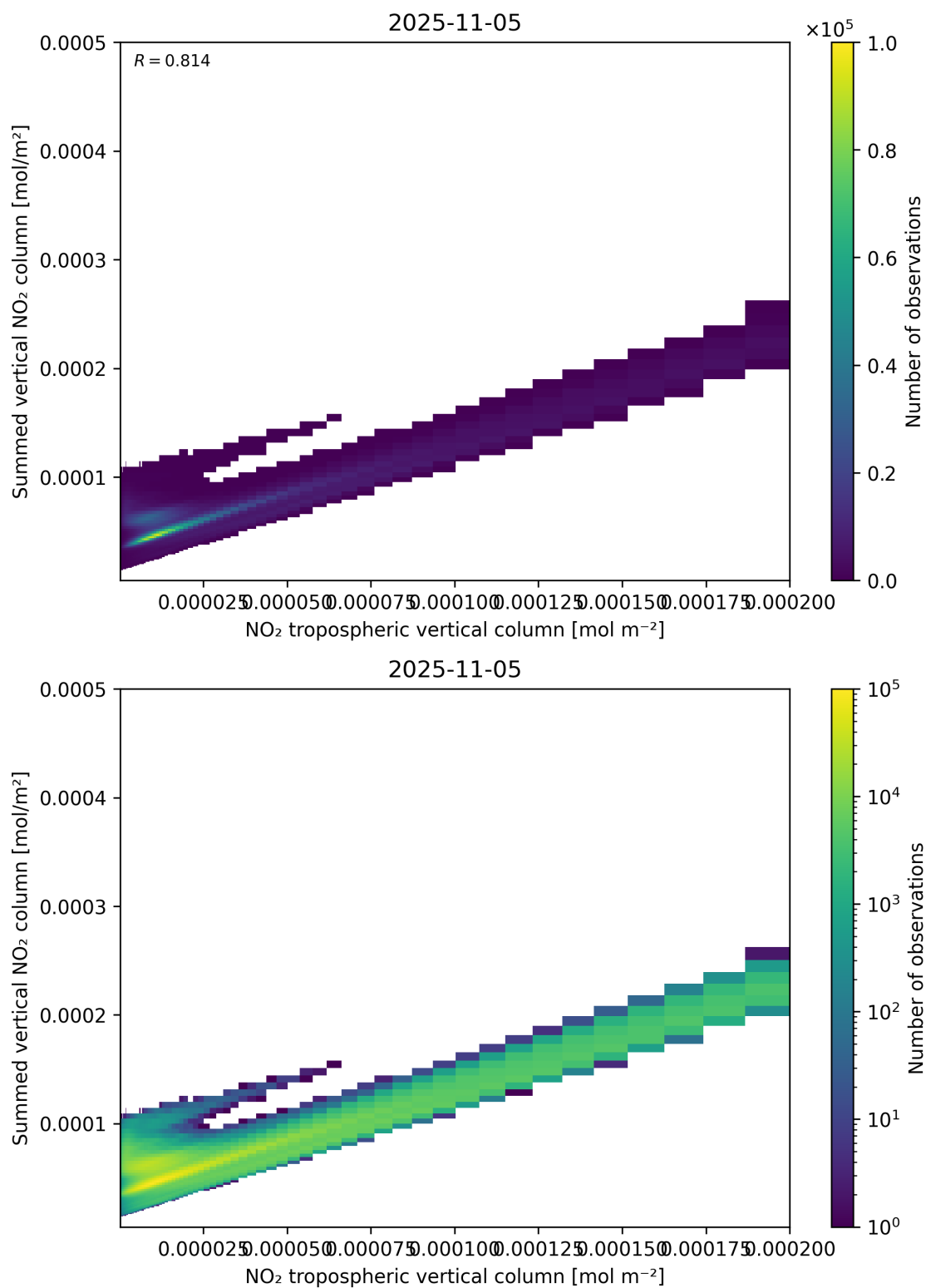
Figure 126: Scatter density plot of “NO 2 tropospheric vertical column” against “Summed vertical NO 2 column” for 2025-11-04 to 2025-11-06.
