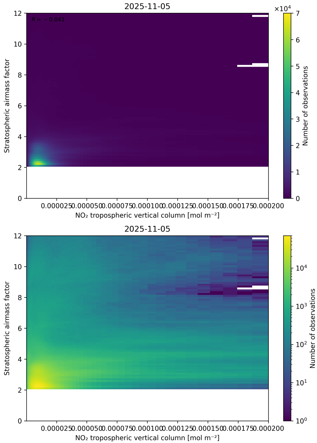
Figure 121: Scatter density plot of “NO 2 tropospheric vertical column” against “Stratospheric airmass factor” for 2025-11-04 to 2025-11-06.
