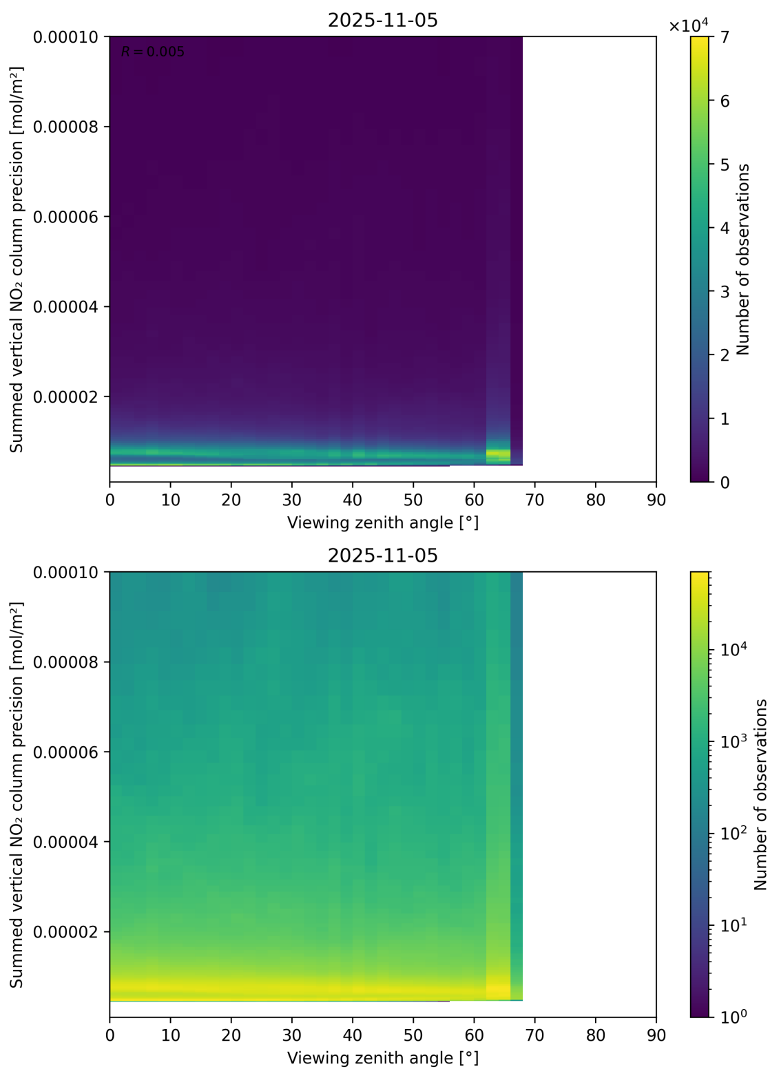
Figure 166: Scatter density plot of “Viewing zenith angle” against “Summed vertical NO 2 column precision” for 2025-11-04 to 2025-11-06.
