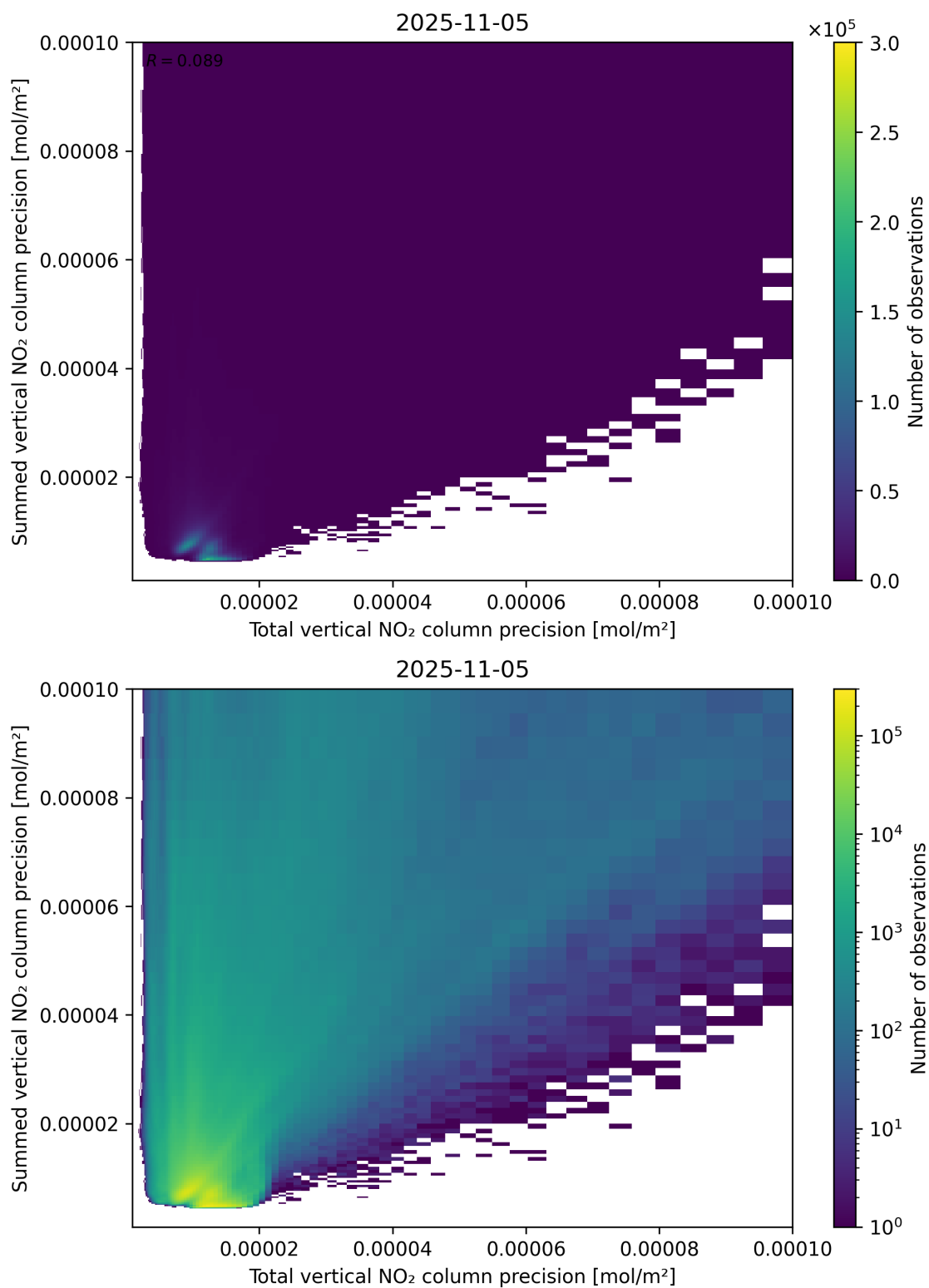
Figure 118: Scatter density plot of “Total vertical NO 2 column precision” against “Summed vertical NO 2 column precision” for 2025-11-04 to 2025-11-06.
