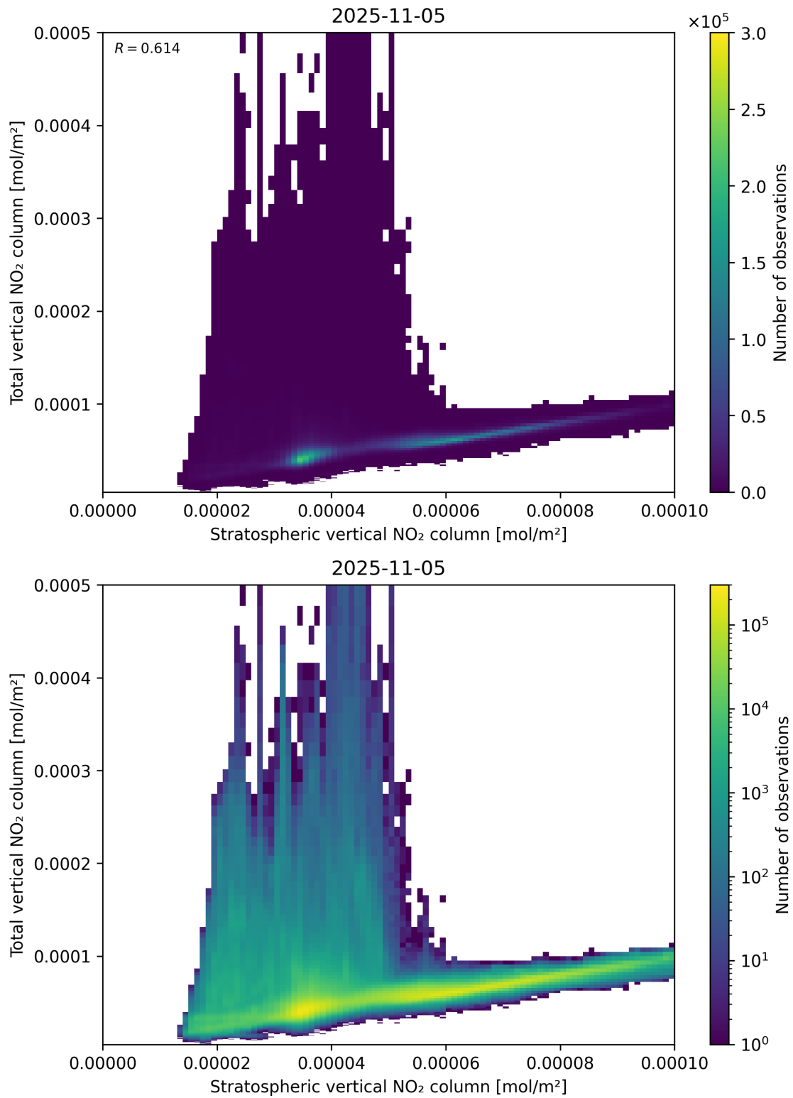
Figure 100: Scatter density plot of “Stratospheric vertical NO 2 column” against “Total vertical NO 2 column” for 2025-11-04 to 2025-11-06.
