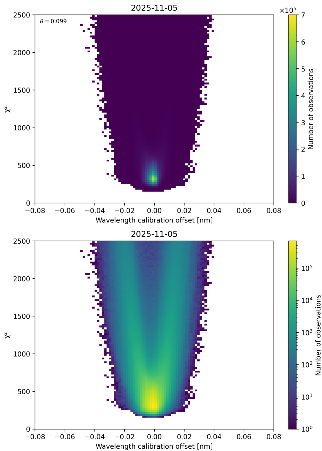
Figure 175: Scatter density plot of “Wavelength calibration offset” against “ \chi^2 ” for 2025-11-04 to 2025-11-06.
