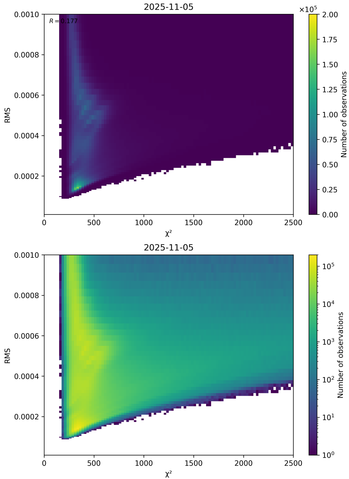
Figure 82: Scatter density plot of “ \chi^2 ” against “RMS” for 2025-11-04 to 2025-11-06.
