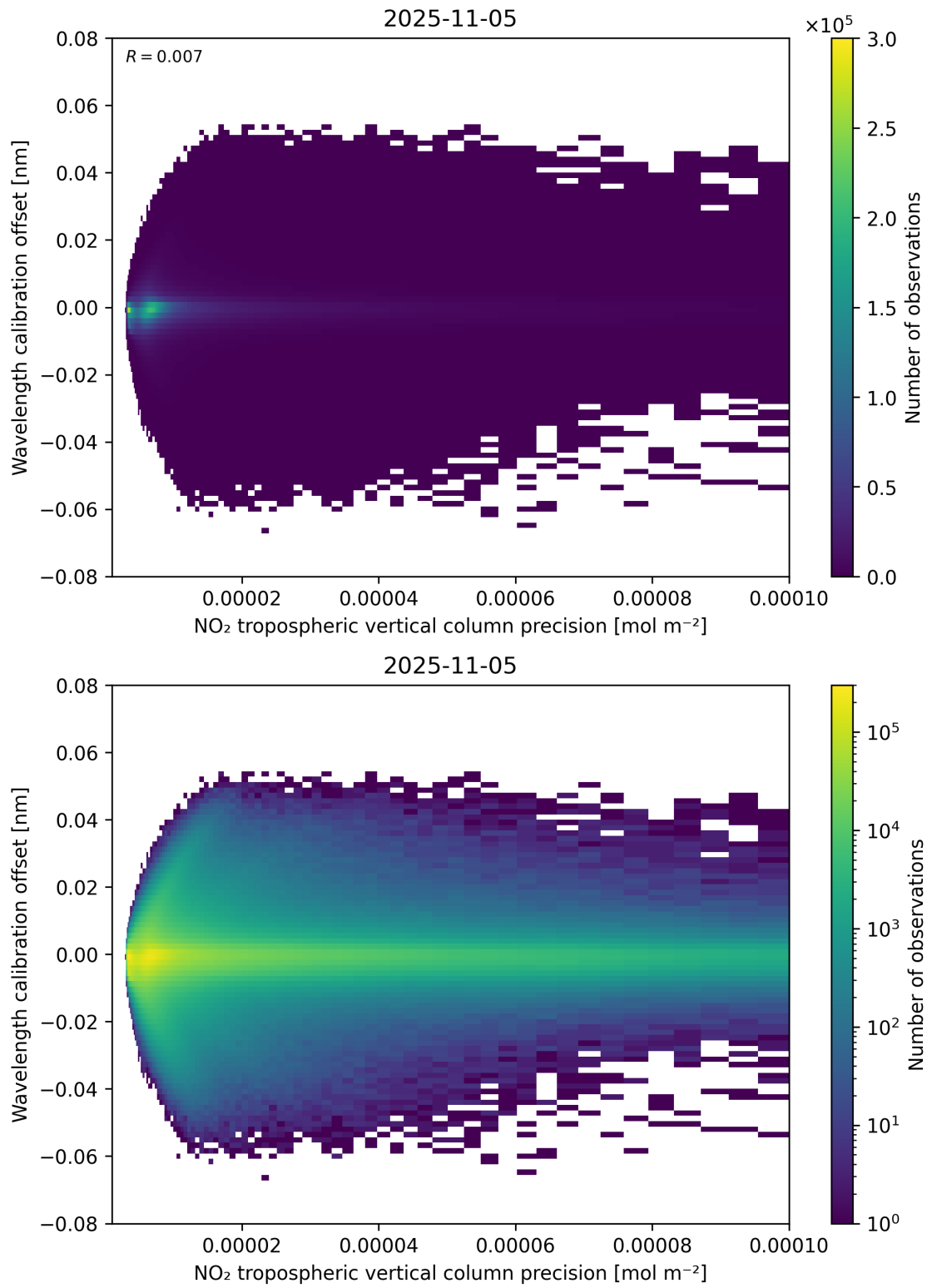
Figure 141: Scatter density plot of “NO 2 tropospheric vertical column precision” against “Wavelength calibration offset” for 2025-11-04 to 2025-11-06.
