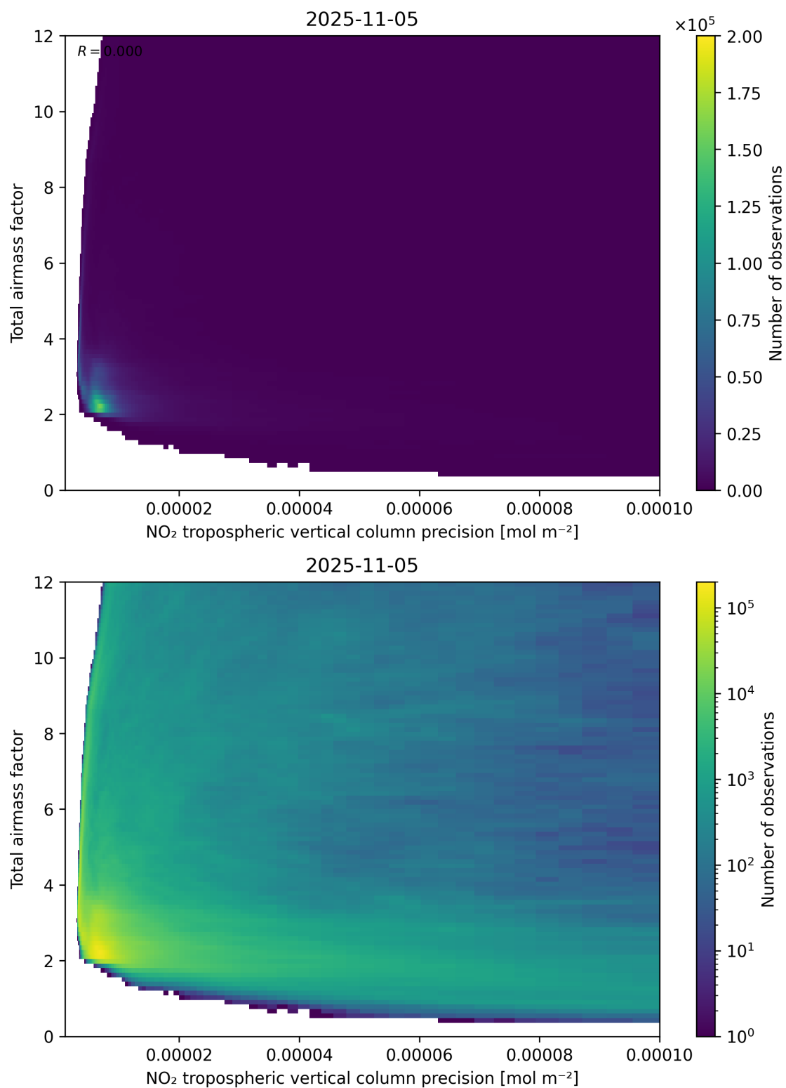
Figure 132: Scatter density plot of “NO 2 tropospheric vertical column precision” against “Total air mass factor” for 2025-11-04 to 2025-11-06.
