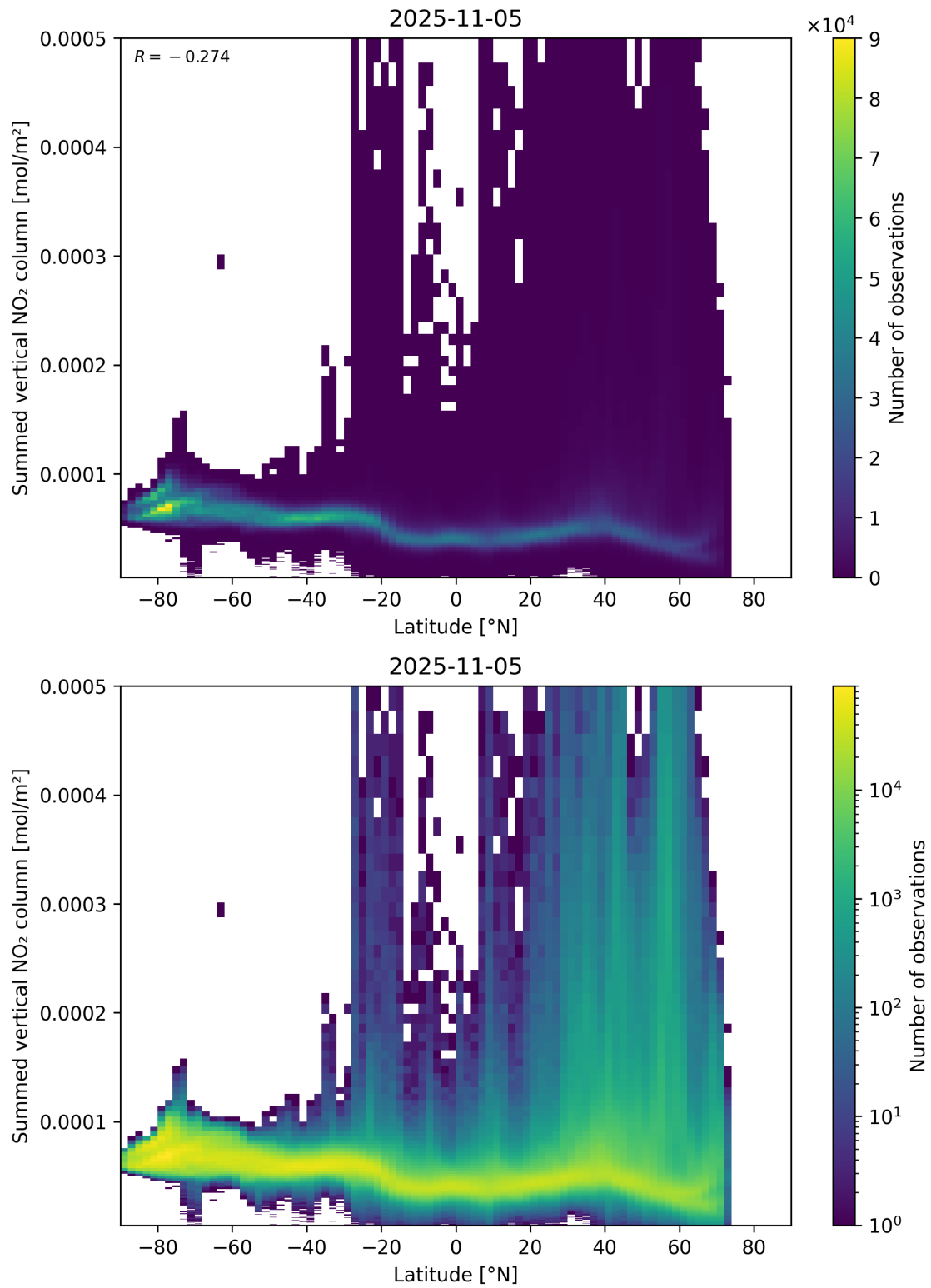
Figure 88: Scatter density plot of “Latitude” against “Summed vertical NO 2 column” for 2025-11-04 to 2025-11-06.
