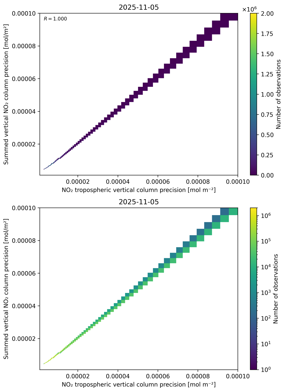
Figure 137: Scatter density plot of “NO 2 tropospheric vertical column precision” against “Summed vertical NO 2 column precision” for 2025-11-04 to 2025-11-06.
