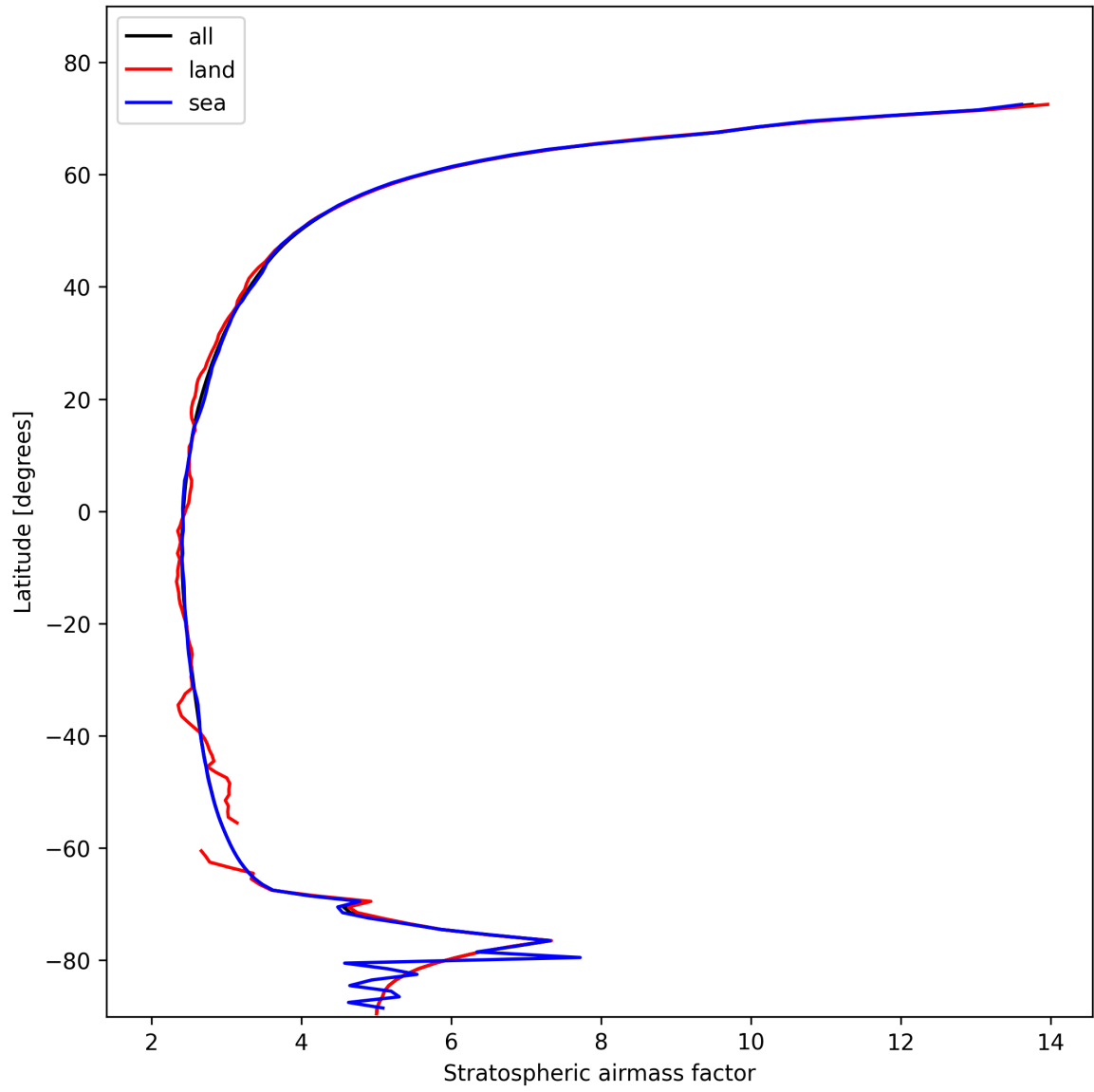
Figure 27: Zonal average of “Stratospheric air mass factor” for 2025-11-04 to 2025-11-06.
