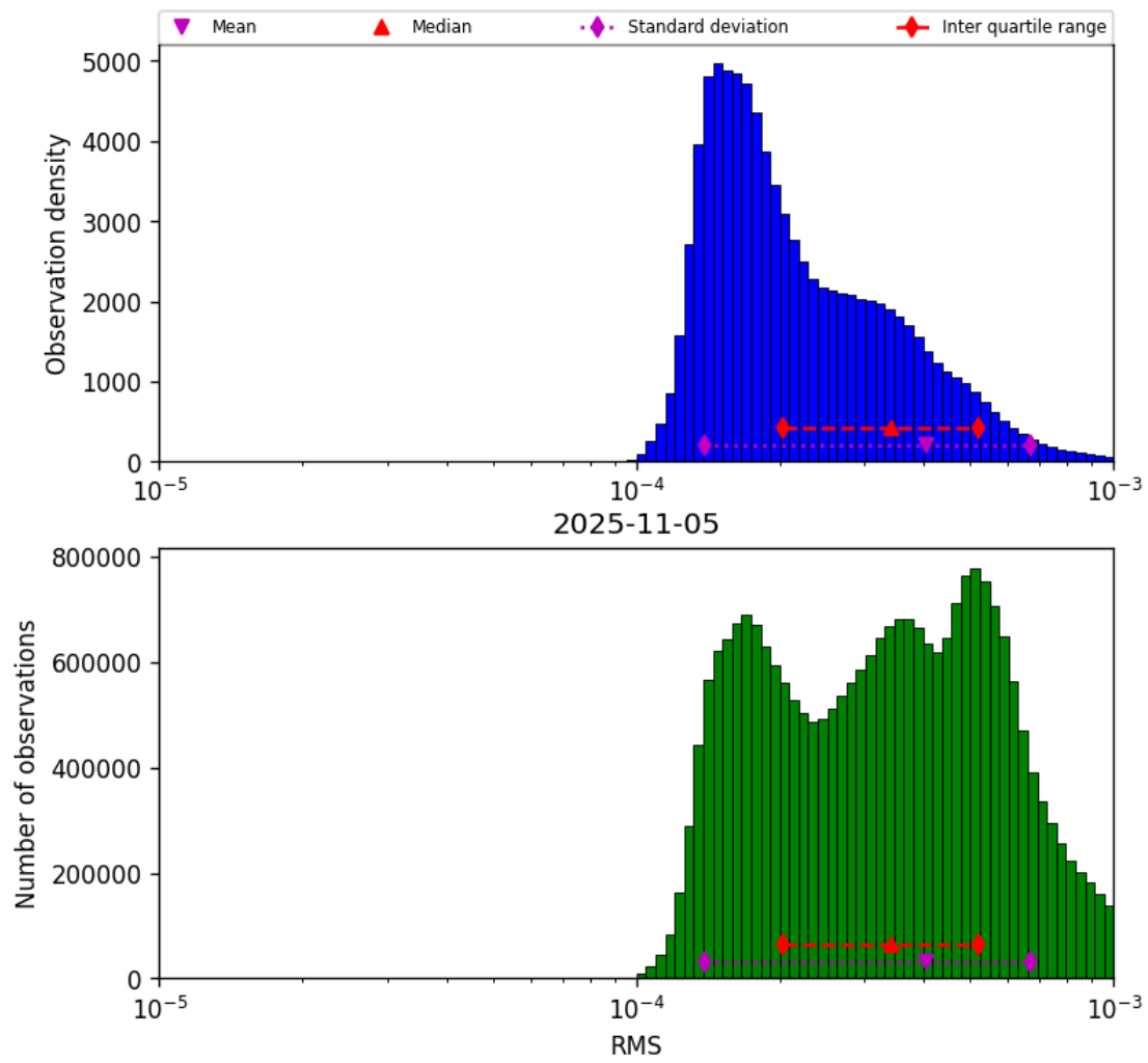
Figure 43: Histogram of “RMS” for 2025-11-04 to 2025-11-06
