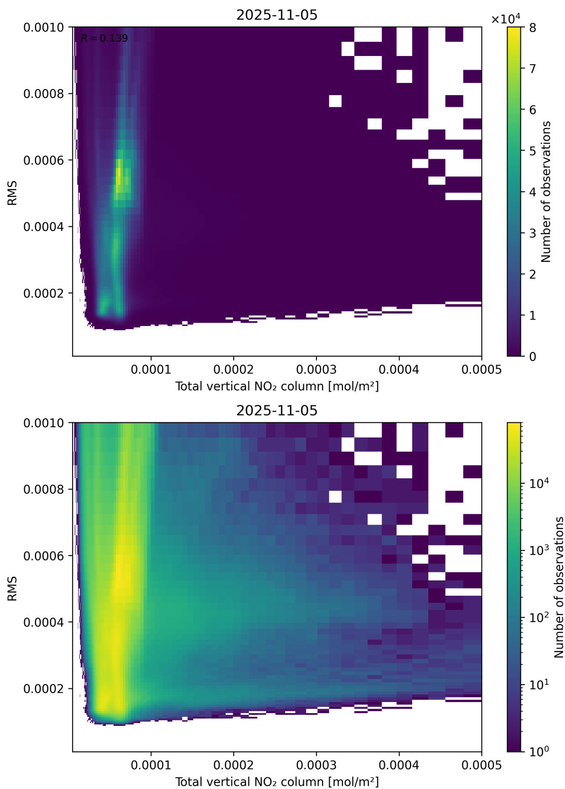
Figure 120: Scatter density plot of “Total vertical NO 2 column” against “RMS” for 2025-11-04 to 2025-11-06.
