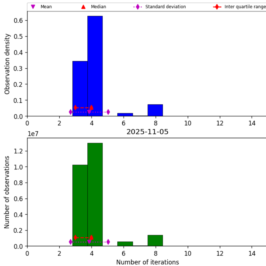
Figure 34: Histogram of “Number of iterations” for 2025-11-04 to 2025-11-06
