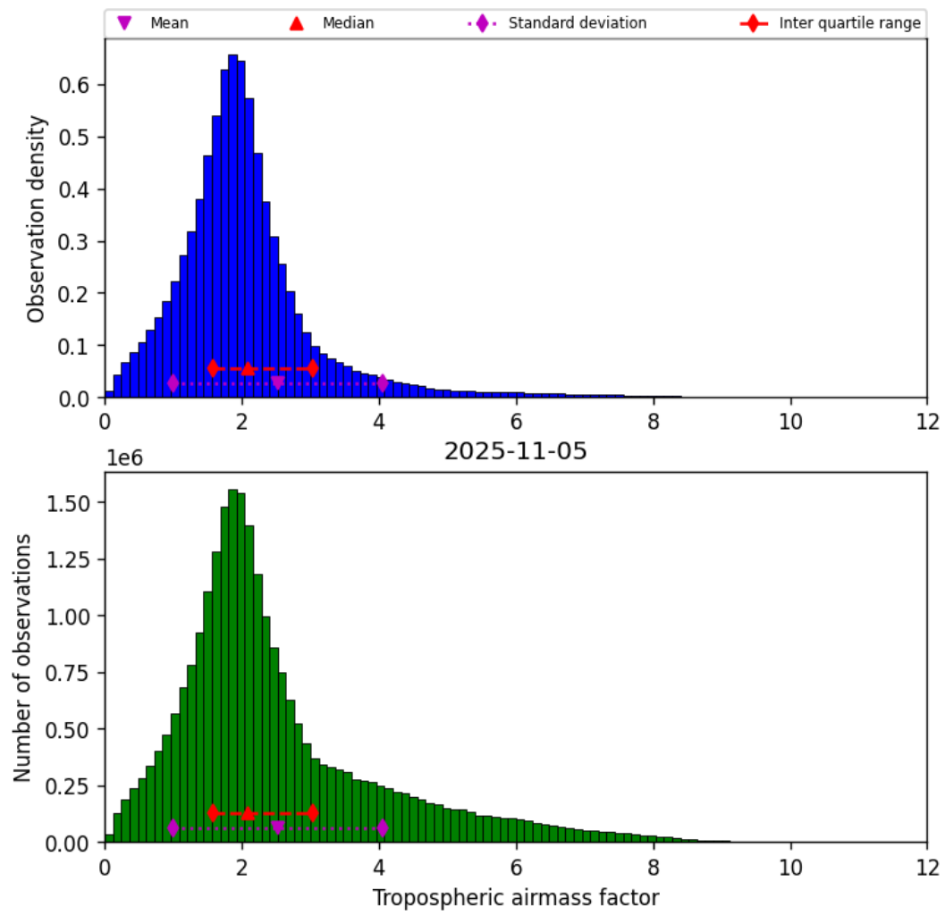
Figure 31: Histogram of “Tropospheric airmass factor” for 2025-11-04 to 2025-11-06
