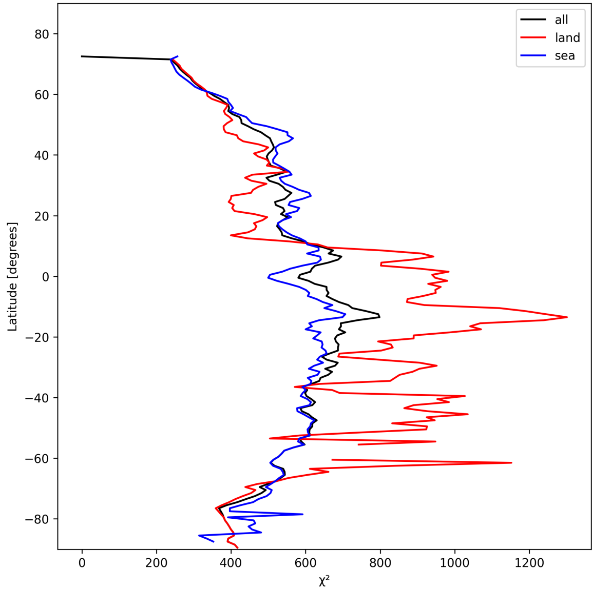
Figure 25: Zonal average of “ \chi^2 ” for 2025-11-05 to 2025-11-07.
