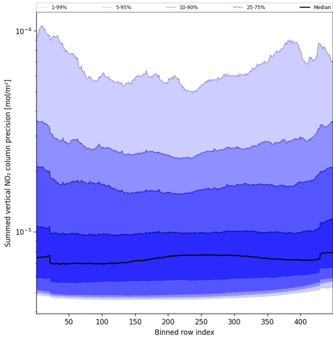
Figure 58: Along track statistics of “Summed vertical NO 2 column precision” for 2025-11-05 to 2025-11-07
