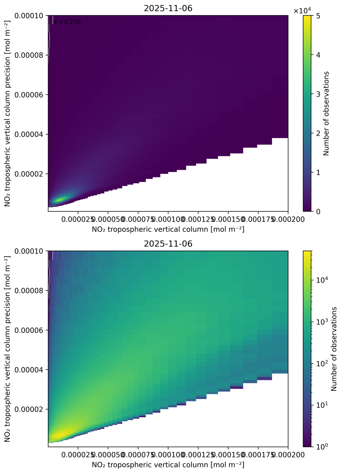
Figure 130: Scatter density plot of “NO 2 tropospheric vertical column” against “NO 2 tropospheric vertical column precision” for 2025-11-05 to 2025-11-07.
