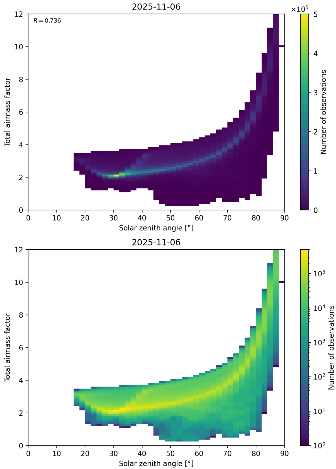
Figure 146: Scatter density plot of “Solar zenith angle” against “Total airmass factor” for 2025-11-05 to 2025-11-07.
