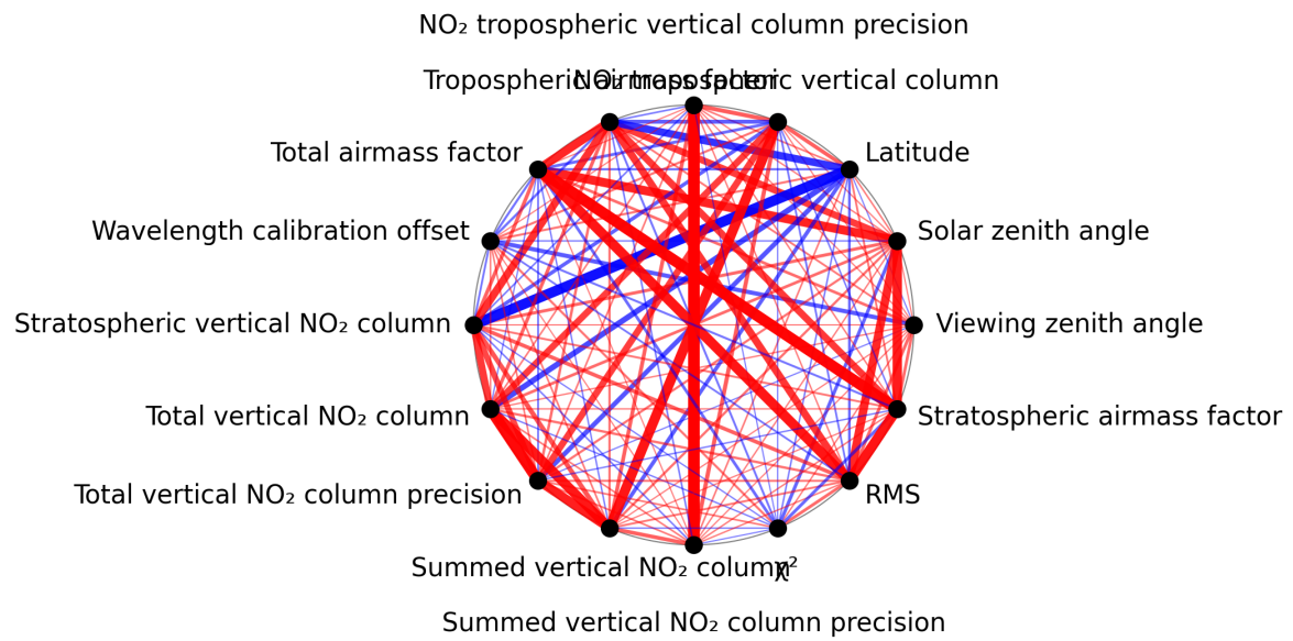
Figure 1: Map of correlation graph for 2025-11-05 to 2025-11-07.
