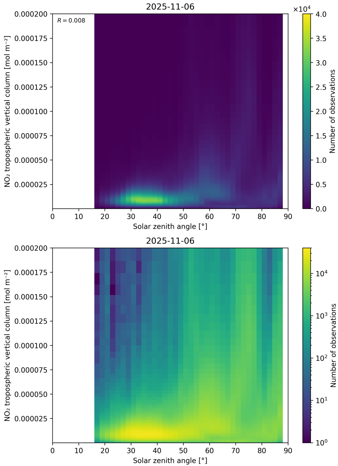
Figure 155: Scatter density plot of “Solar zenith angle” against “NO 2 tropospheric vertical column” for 2025-11-05 to 2025-11-07.
