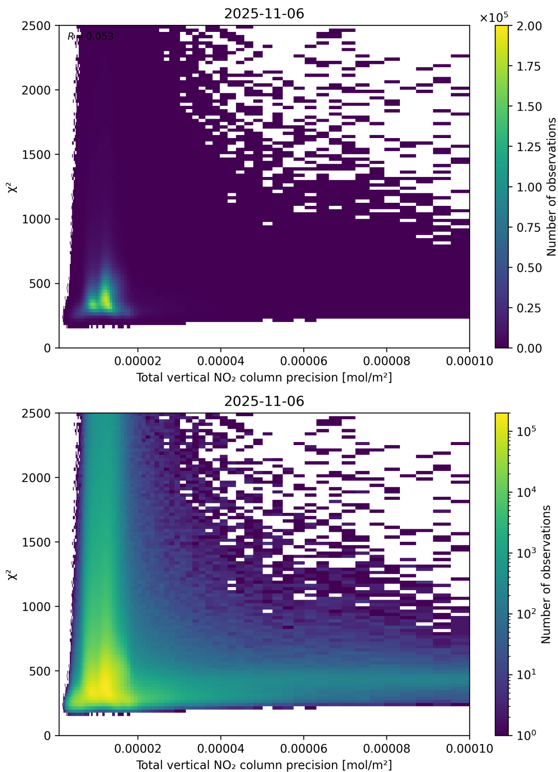
Figure 116: Scatter density plot of “Total vertical NO 2 column precision” against “ \chi^2 ” for 2025-11-05 to 2025-11-07.
