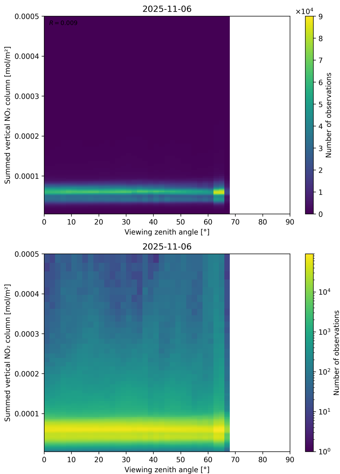
Figure 165: Scatter density plot of “Viewing zenith angle” against “Summed vertical NO 2 column” for 2025-11-05 to 2025-11-07.
