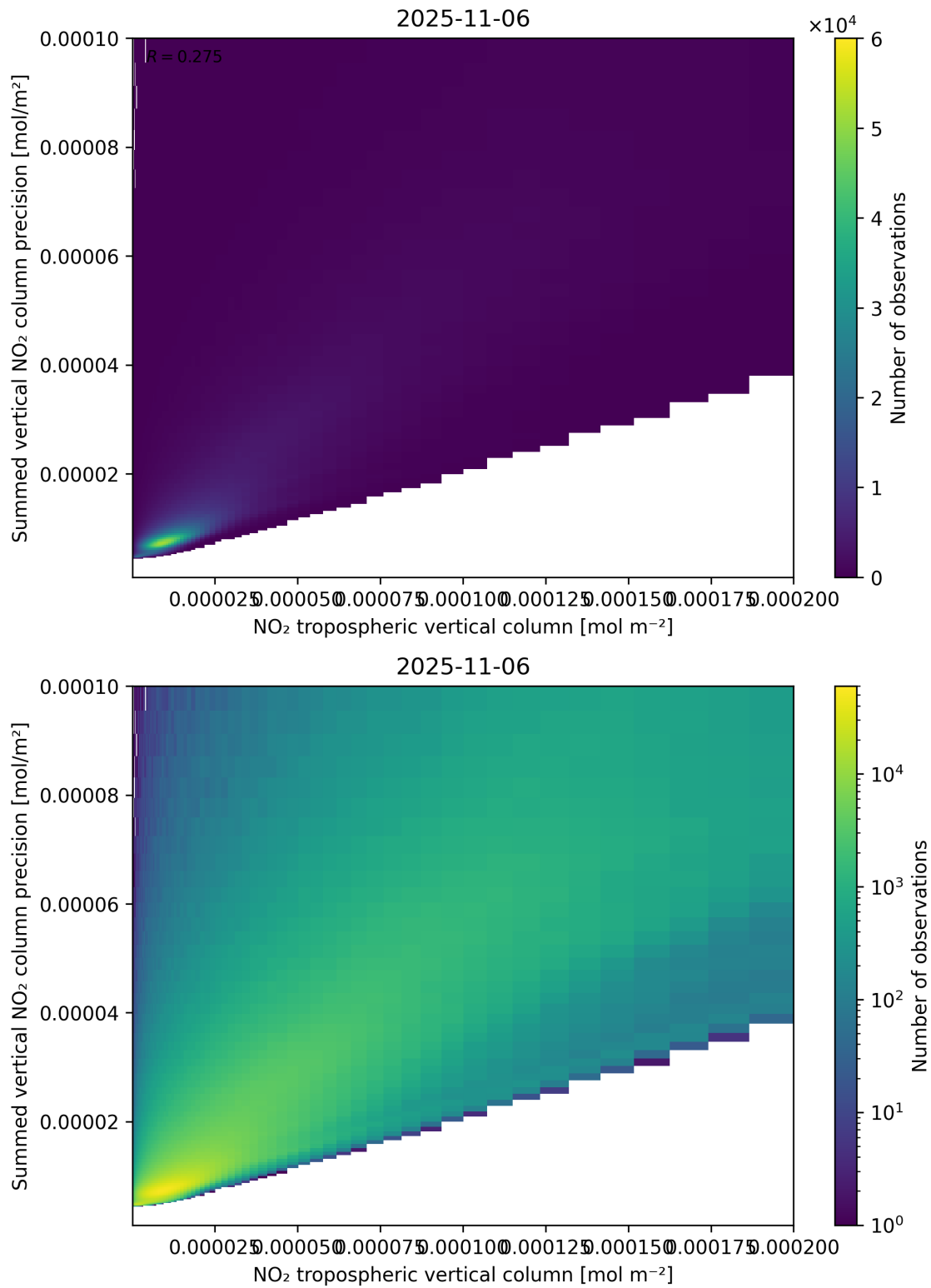
Figure 127: Scatter density plot of “NO 2 tropospheric vertical column” against “Summed vertical NO 2 column precision” for 2025-11-05 to 2025-11-07.
