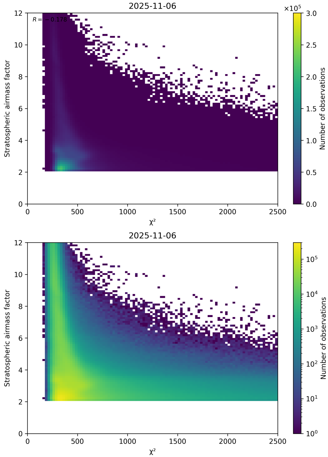
Figure 81: Scatter density plot of “ \chi^2 ” against “Stratospheric airmass factor” for 2025-11-05 to 2025-11-07.
