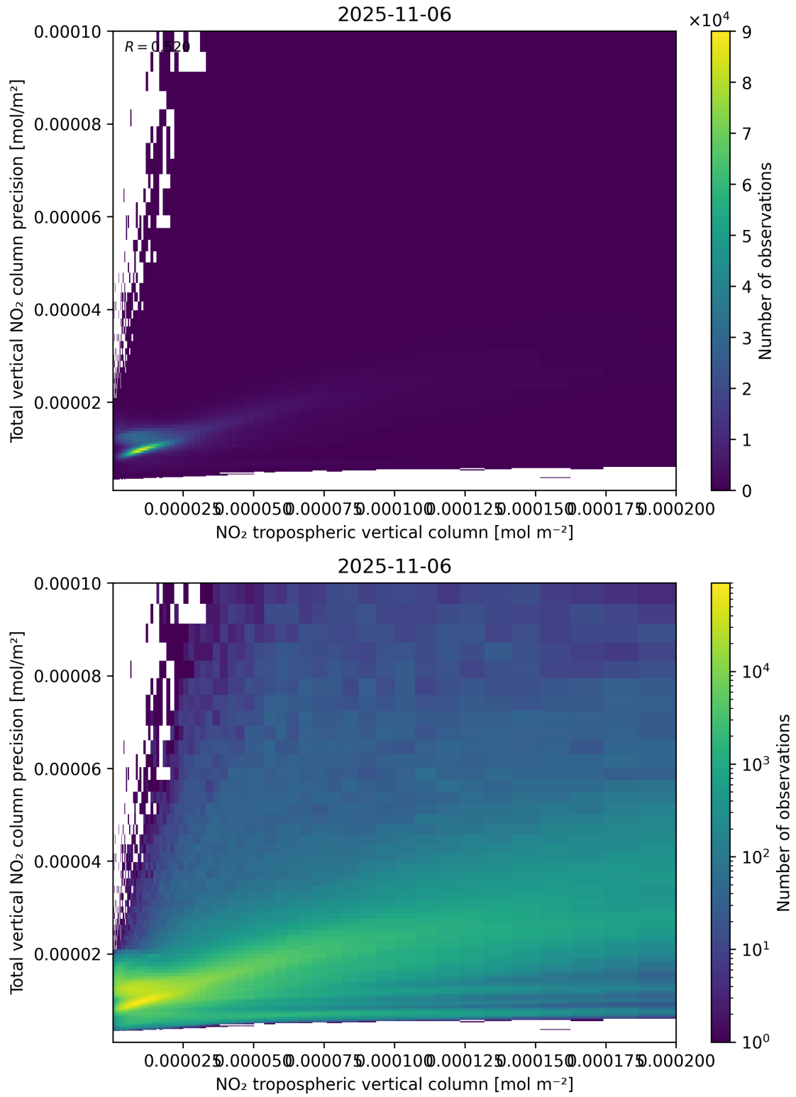
Figure 129: Scatter density plot of “NO 2 tropospheric vertical column” against “Total vertical NO 2 column precision” for 2025-11-05 to 2025-11-07.
