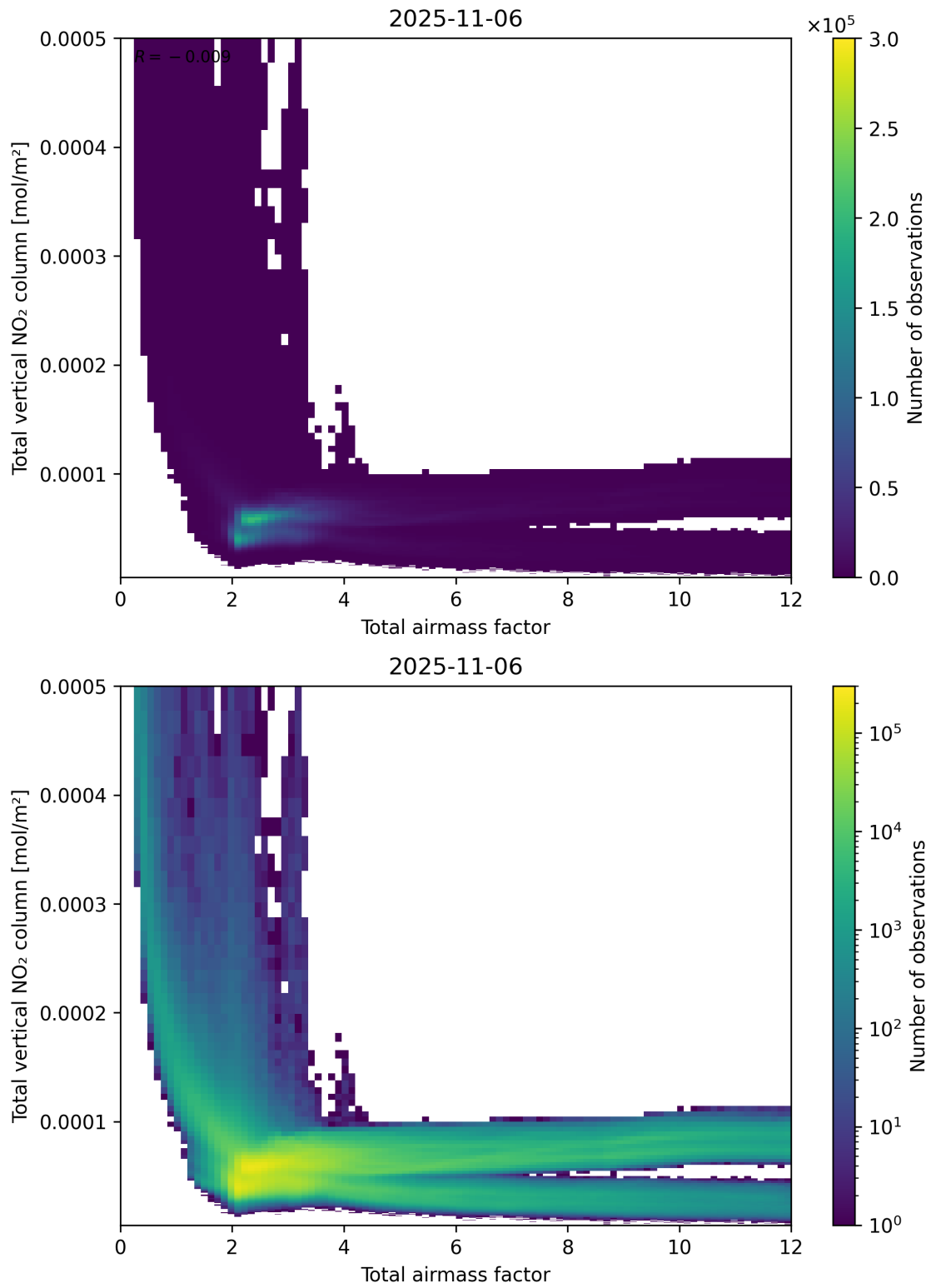
Figure 67: Scatter density plot of “Total airmass factor” against “Total vertical NO 2 column” for 2025-11-05 to 2025-11-07.
