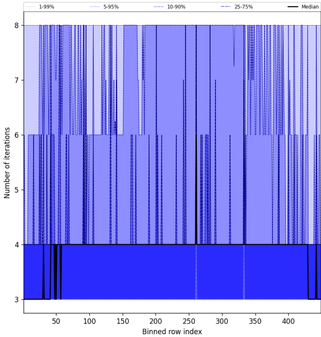
Figure 51: Along track statistics of “Number of iterations” for 2025-11-05 to 2025-11-07
