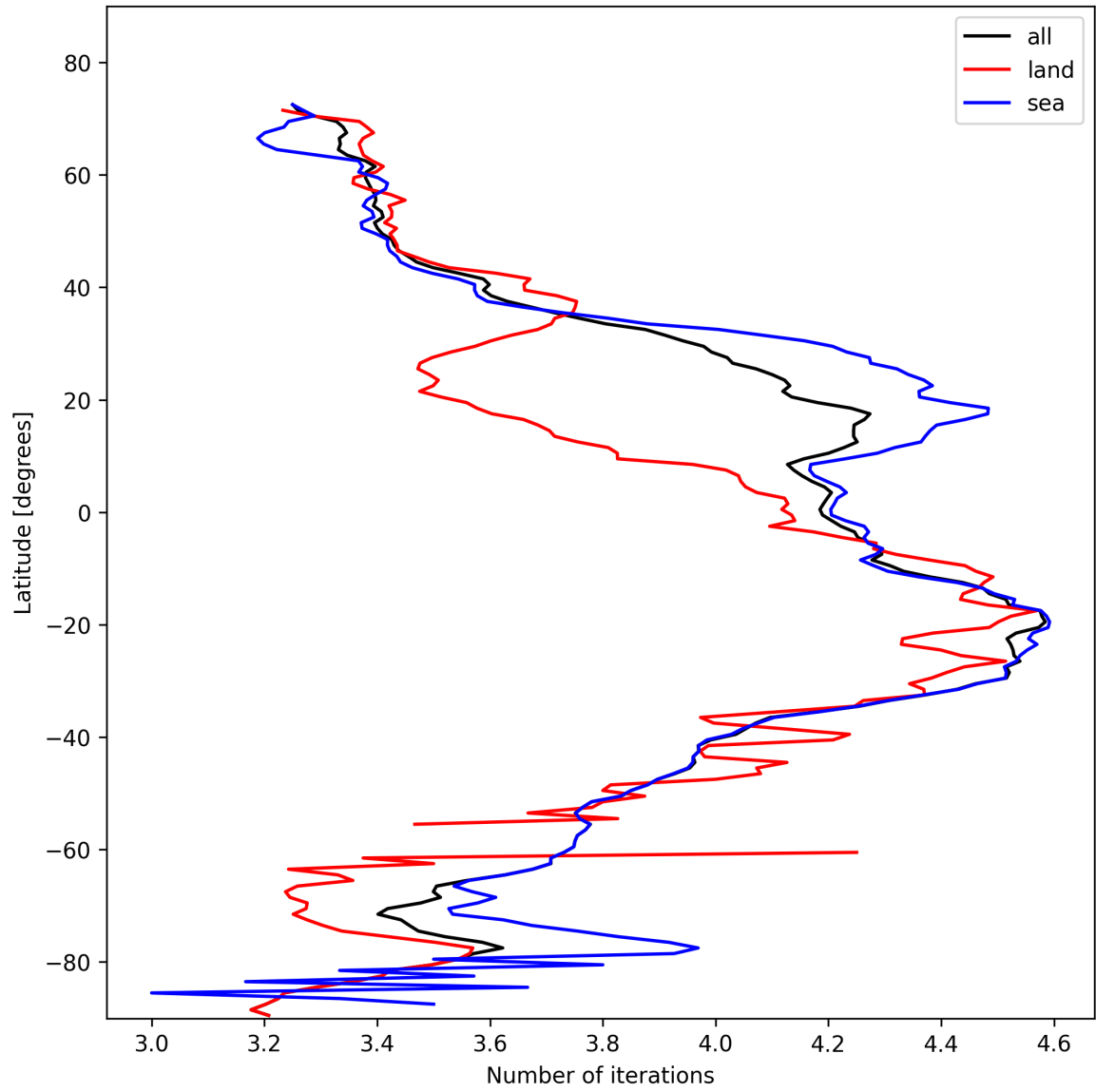
Figure 17: Zonal average of “Number of iterations” for 2025-11-05 to 2025-11-07.
