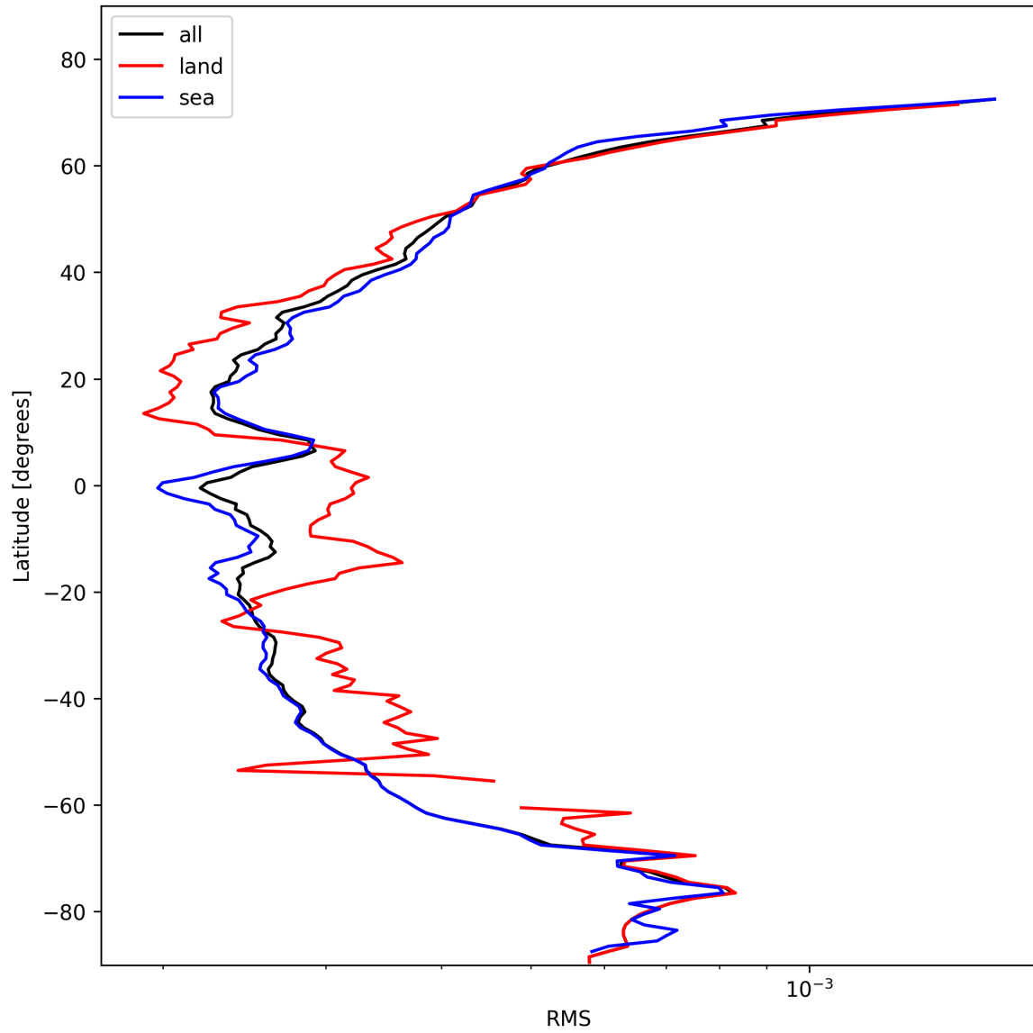
Figure 26: Zonal average of “RMS” for 2025-11-05 to 2025-11-07.
