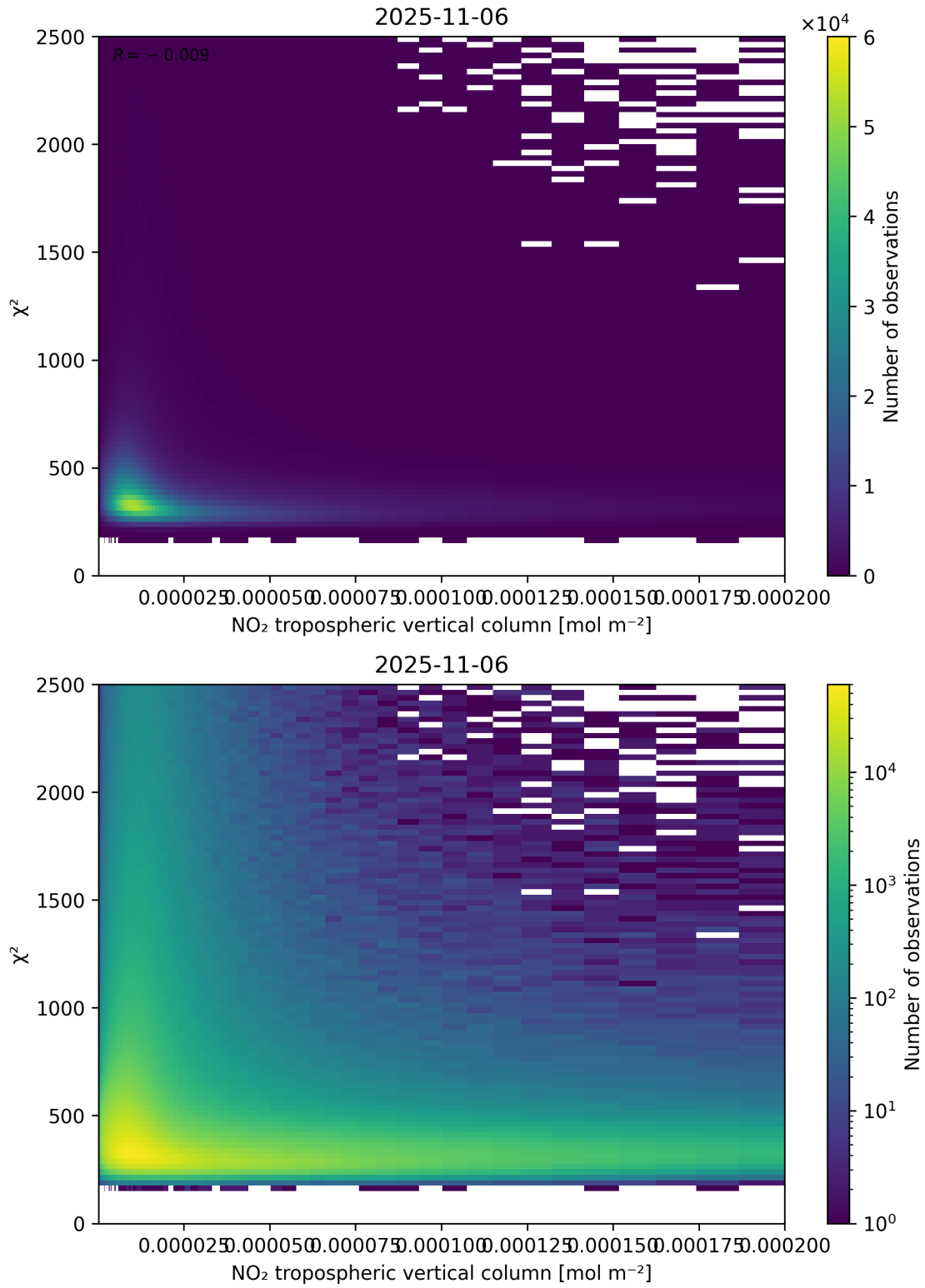
Figure 124: Scatter density plot of “NO 2 tropospheric vertical column” against “ \chi^2 ” for 2025-11-05 to 2025-11-07.
