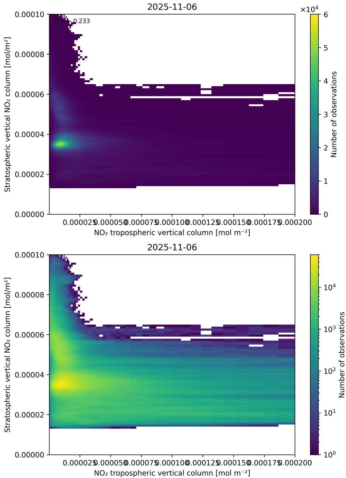
Figure 125: Scatter density plot of “NO 2 tropospheric vertical column” against “Stratospheric vertical NO 2 column” for 2025-11-05 to 2025-11-07.
