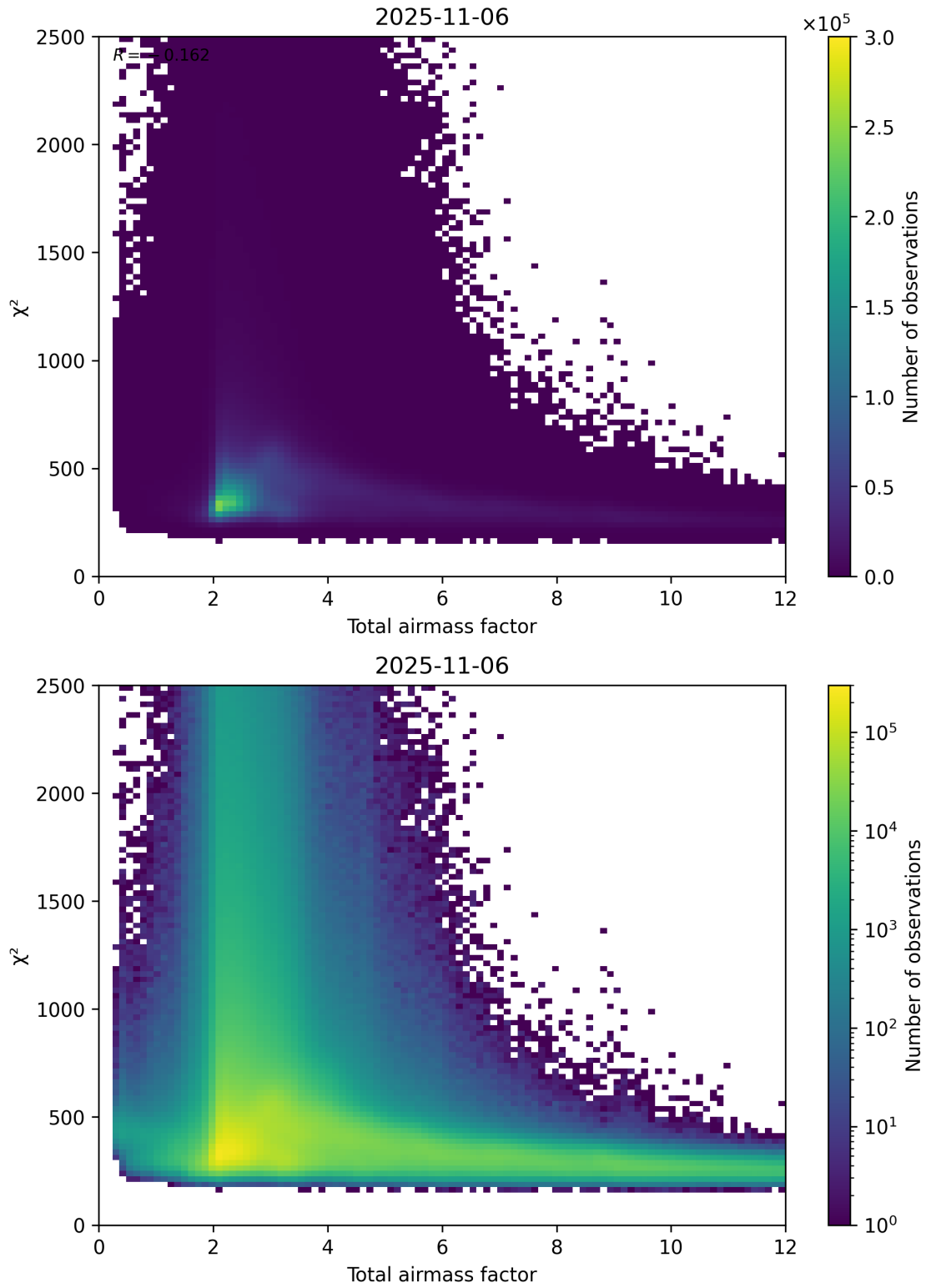
Figure 63: Scatter density plot of “Total airmass factor” against “ \chi^2 ” for 2025-11-05 to 2025-11-07.
