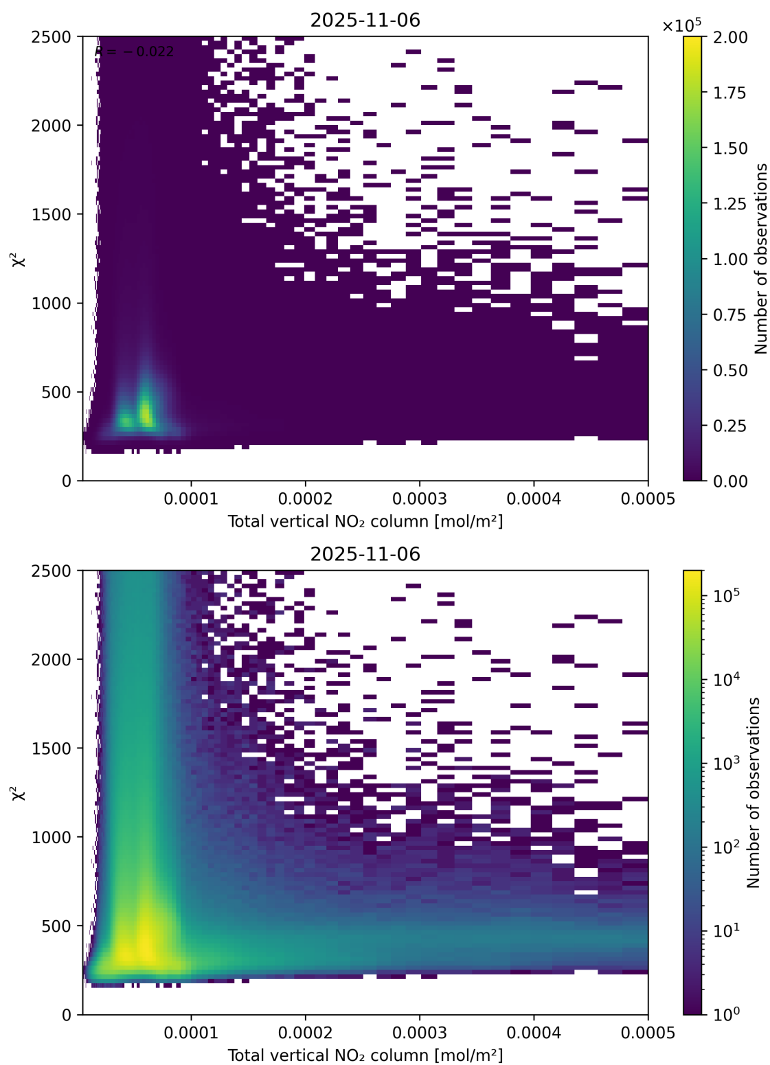
Figure 111: Scatter density plot of “Total vertical NO 2 column” against “ \chi^2 ” for 2025-11-05 to 2025-11-07.
