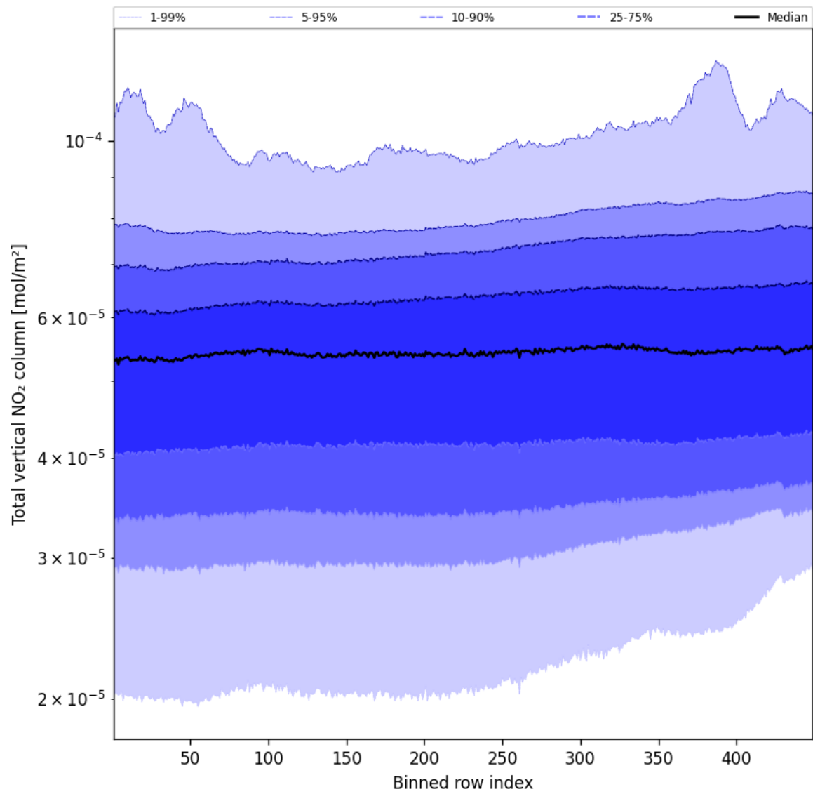
Figure 55: Along track statistics of “Total vertical NO 2 column” for 2025-11-05 to 2025-11-07
