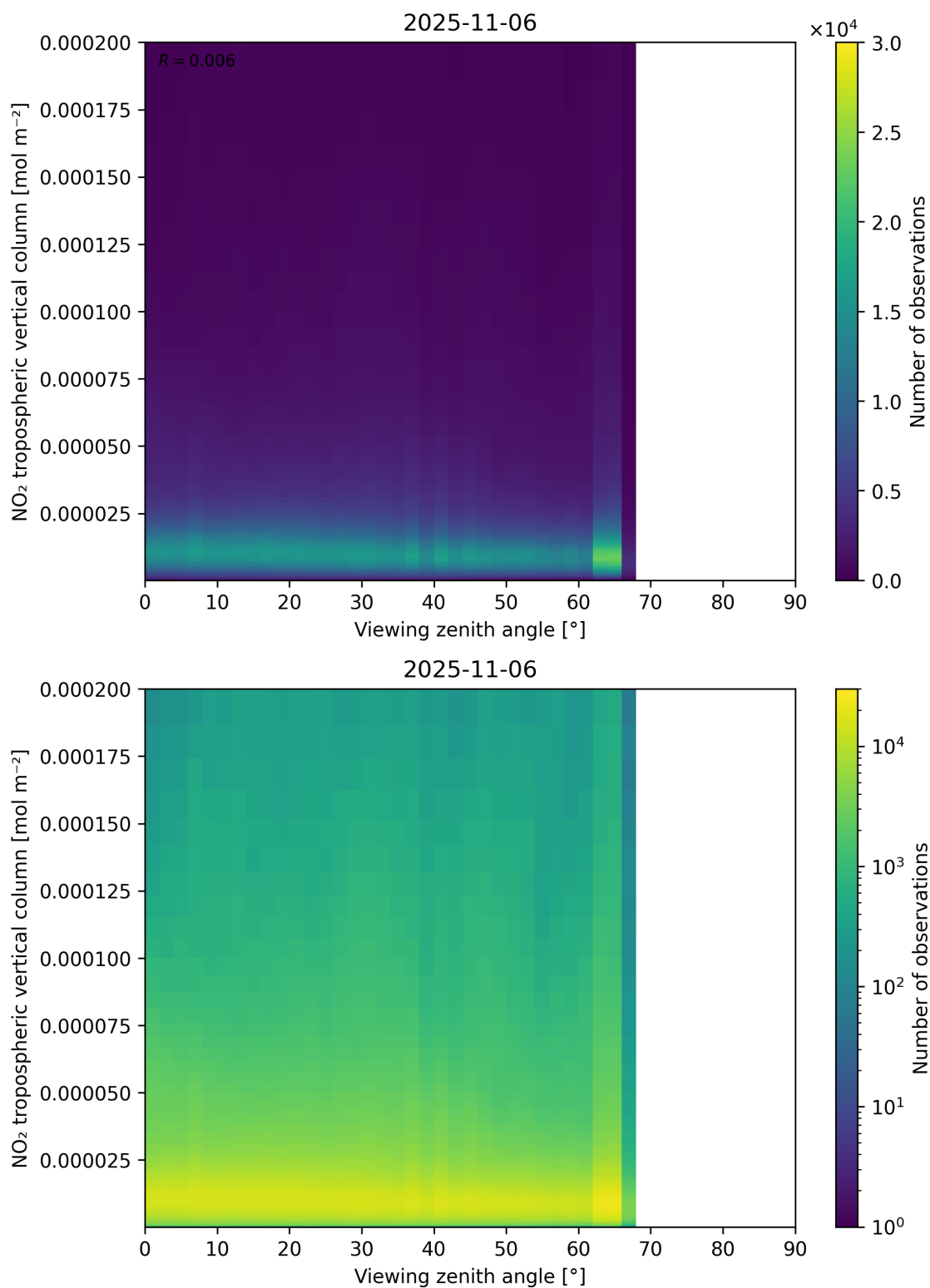
Figure 169: Scatter density plot of “Viewing zenith angle” against “NO 2 tropospheric vertical column” for 2025-11-05 to 2025-11-07.
