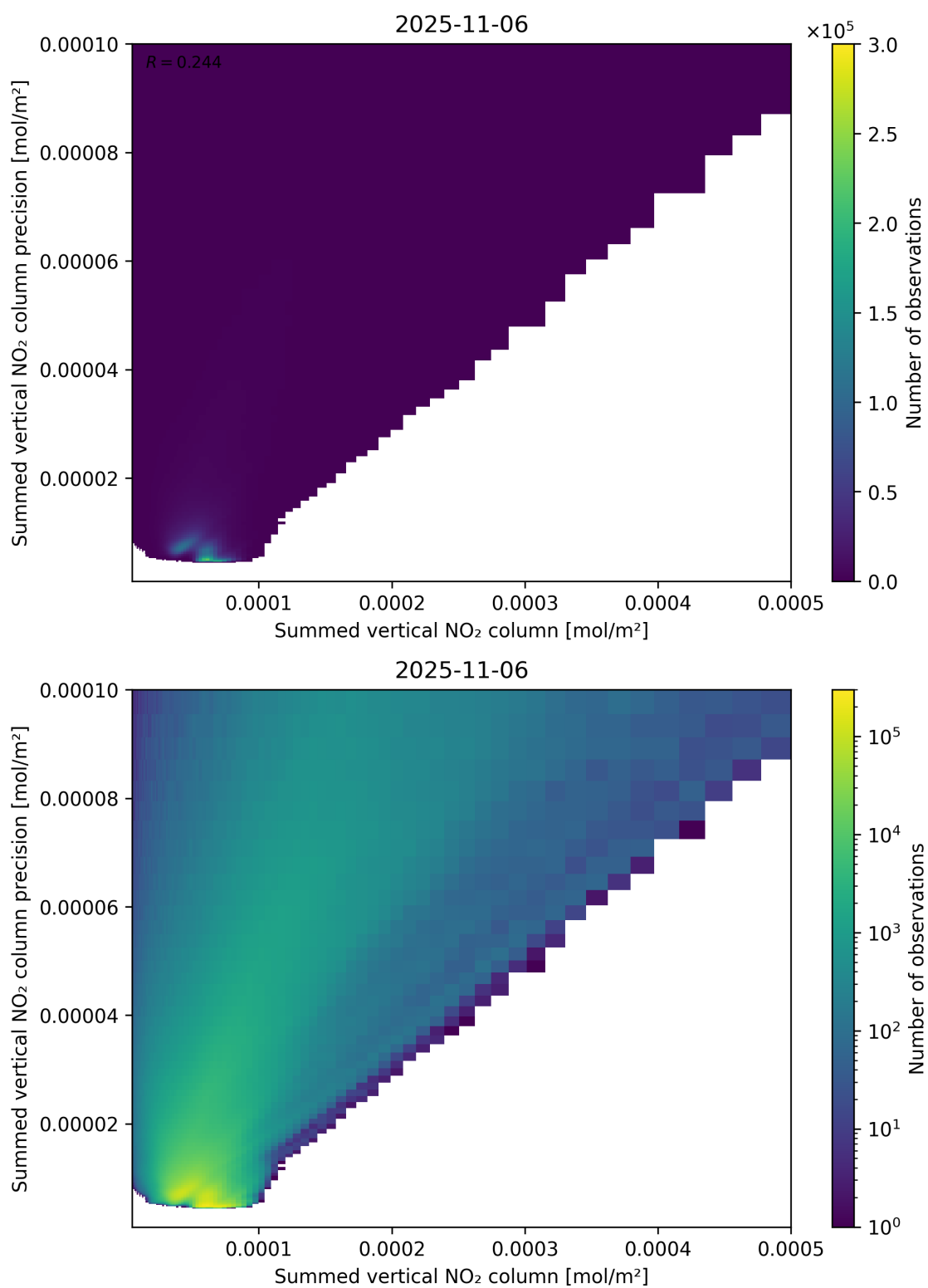
Figure 105: Scatter density plot of “Summed vertical NO 2 column” against “Summed vertical NO 2 column precision” for 2025-11-05 to 2025-11-07.
