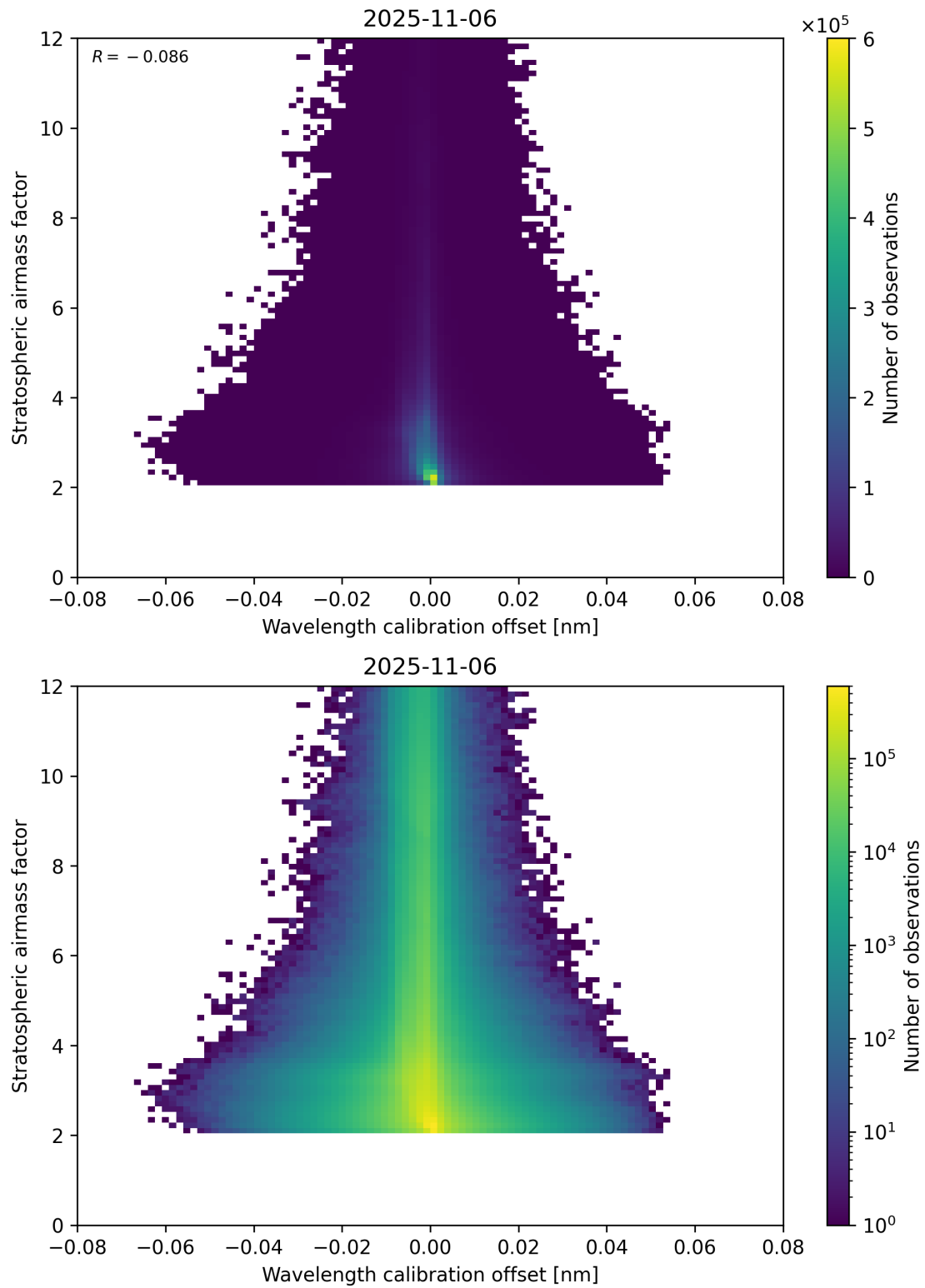
Figure 174: Scatter density plot of “Wavelength calibration offset” against “Stratospheric airmass factor” for 2025-11-05 to 2025-11-07.
