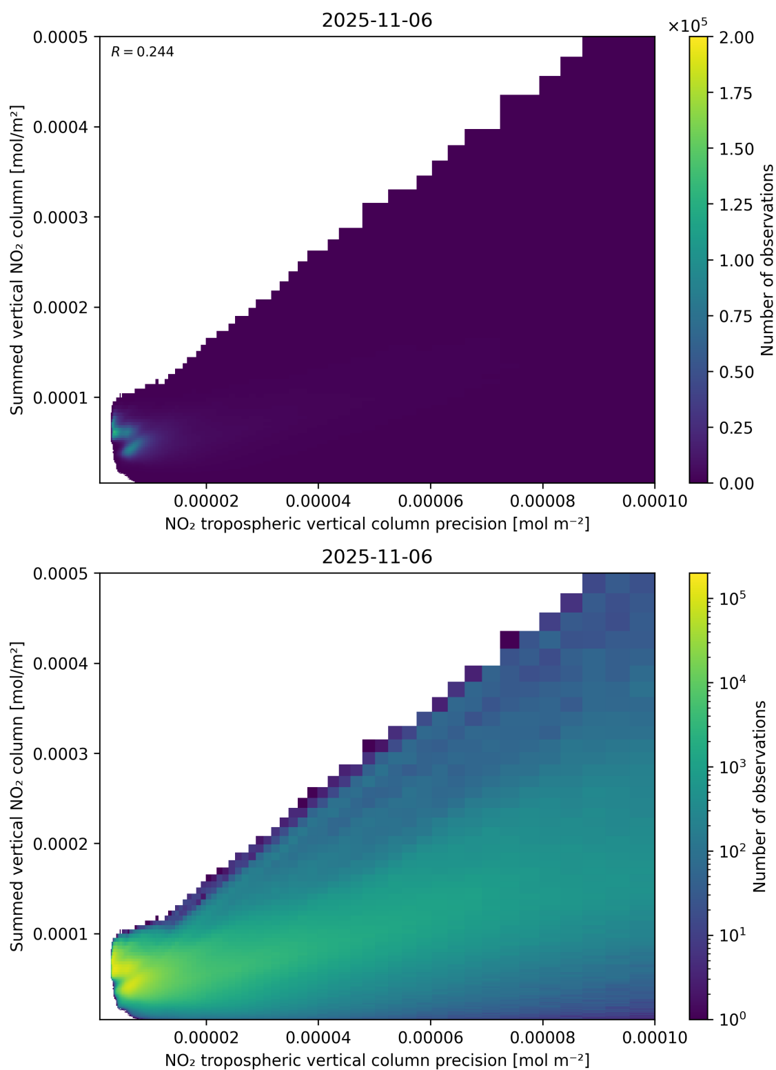
Figure 136: Scatter density plot of “NO 2 tropospheric vertical column precision” against “Summed vertical NO 2 column” for 2025-11-05 to 2025-11-07.
