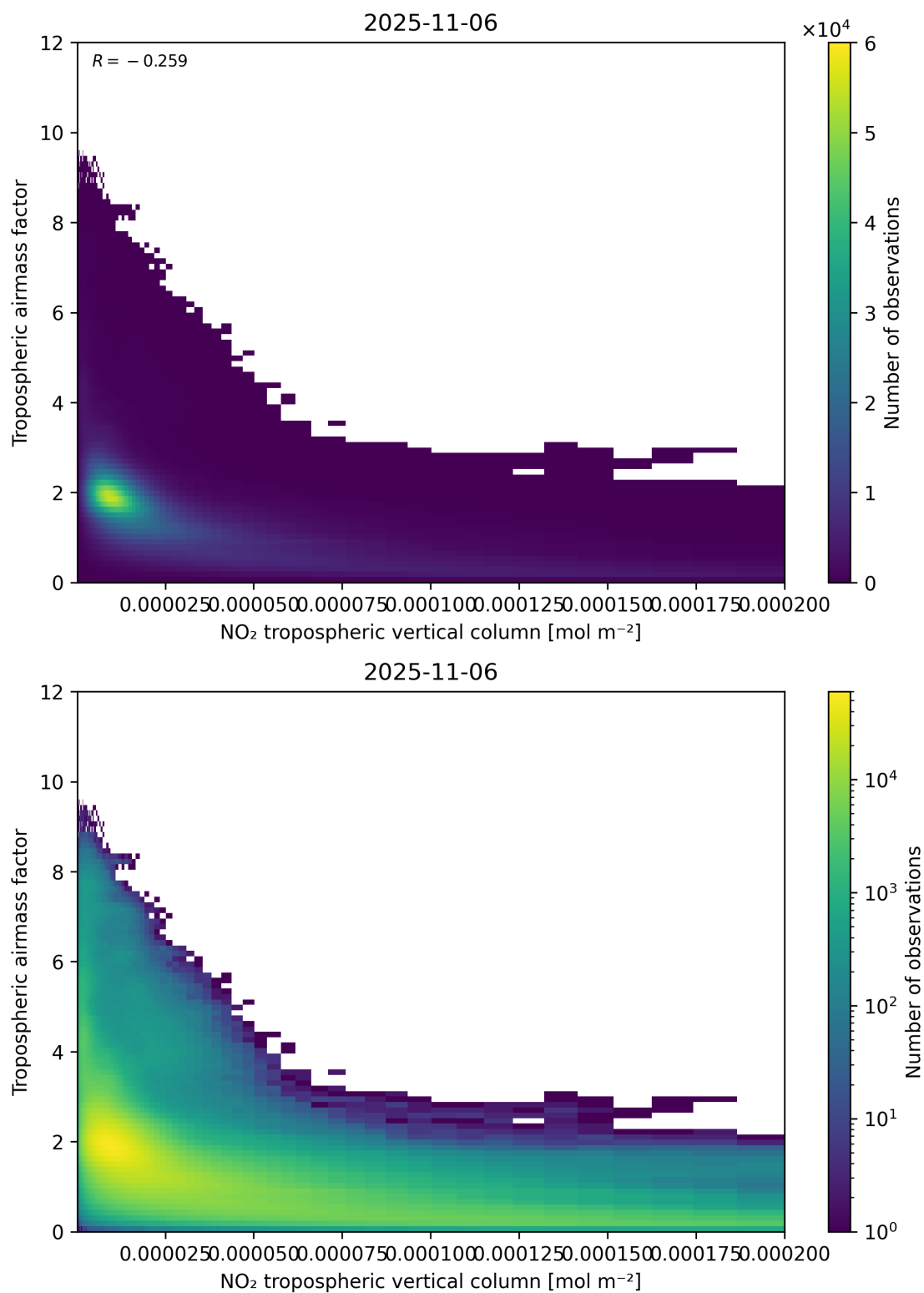
Figure 123: Scatter density plot of “NO 2 tropospheric vertical column” against “Tropospheric air mass factor” for 2025-11-05 to 2025-11-07.
