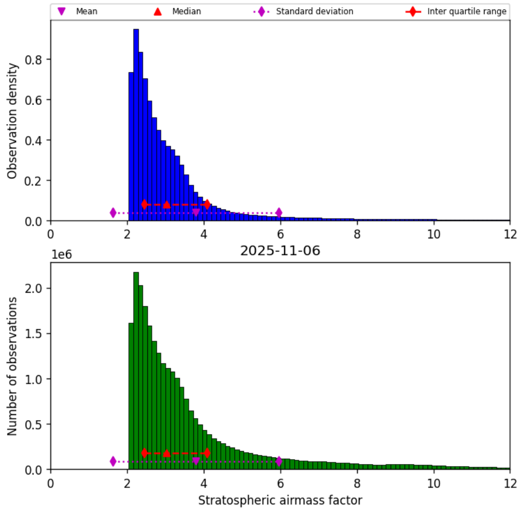
Figure 44: Histogram of “Stratospheric airmass factor” for 2025-11-05 to 2025-11-07
