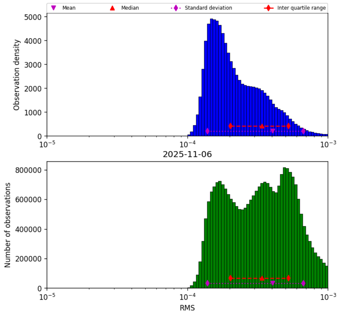
Figure 43: Histogram of “RMS” for 2025-11-05 to 2025-11-07
