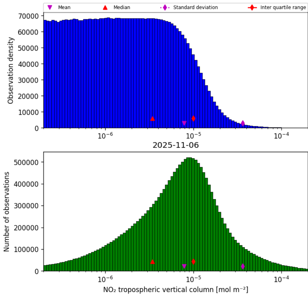
Figure 29: Histogram of “NO 2 tropospheric vertical column” for 2025-11-05 to 2025-11-07
