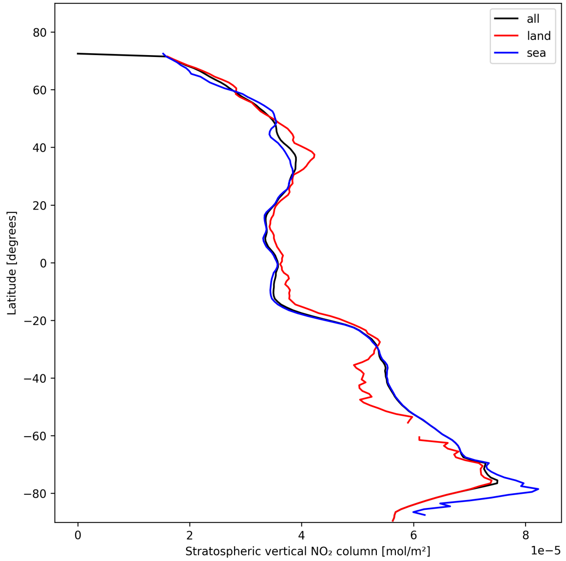
Figure 19: Zonal average of “Stratospheric vertical NO 2 column” for 2025-11-05 to 2025-11-07.
