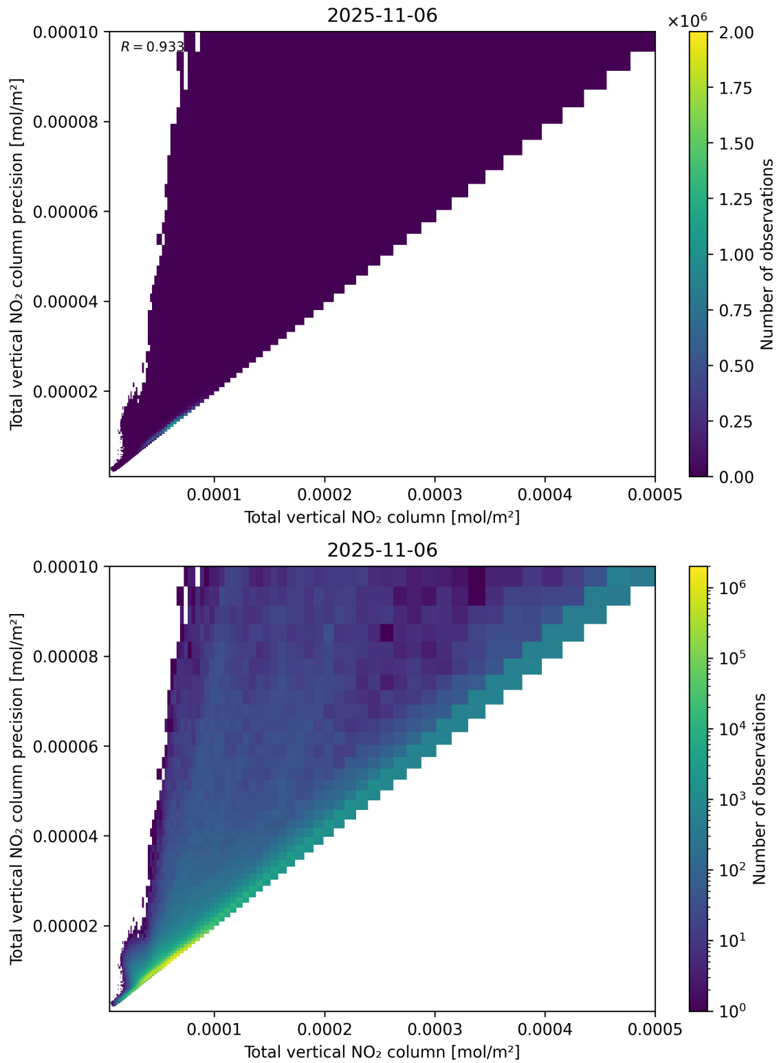
Figure 114: Scatter density plot of “Total vertical NO 2 column” against “Total vertical NO 2 column precision” for 2025-11-05 to 2025-11-07.
