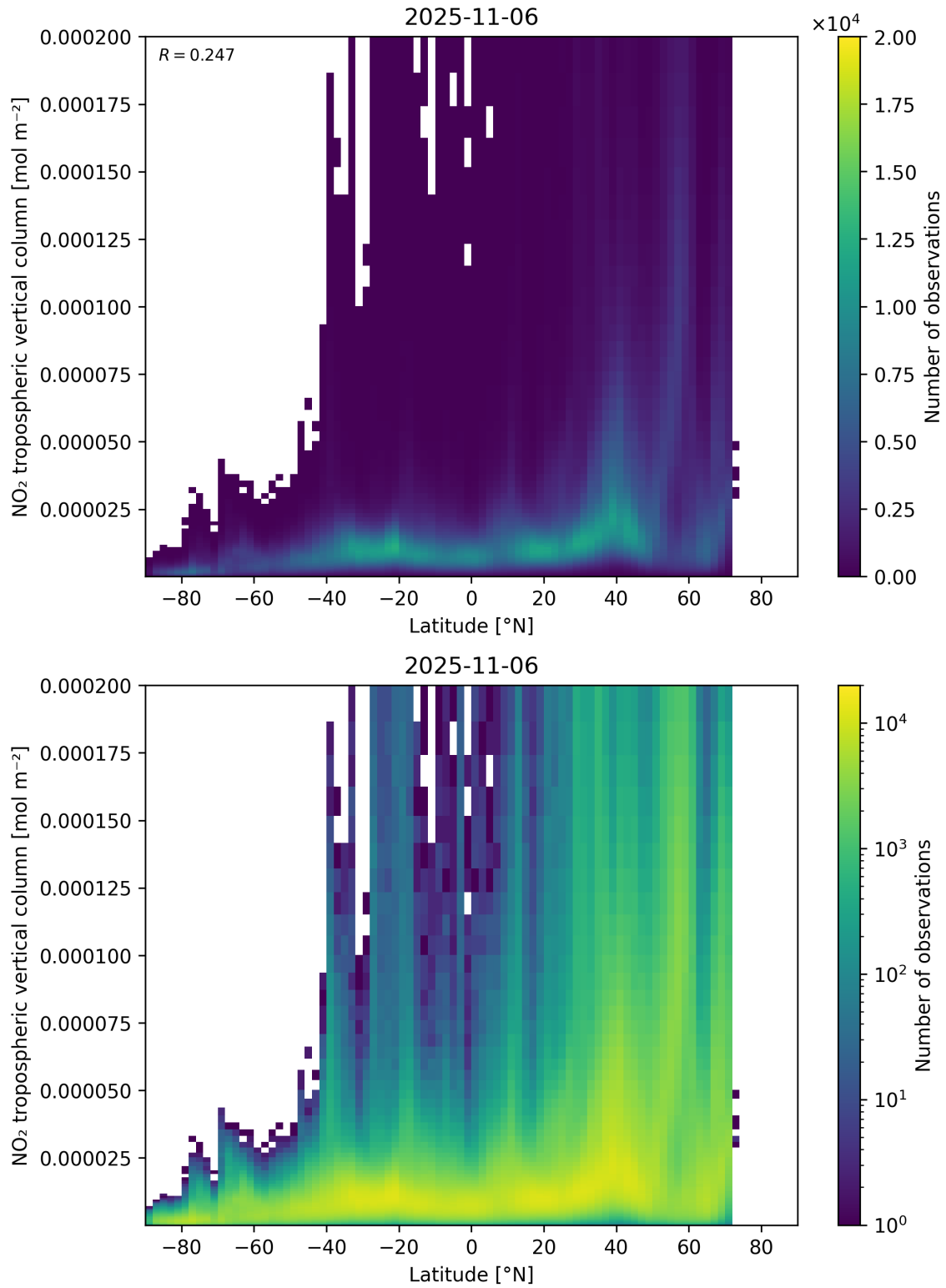
Figure 92: Scatter density plot of “Latitude” against “NO 2 tropospheric vertical column” for 2025-11-05 to 2025-11-07.
