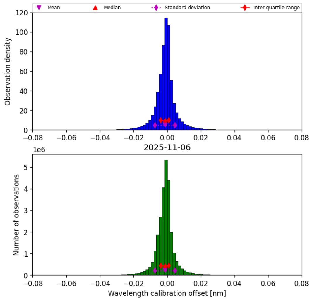
Figure 35: Histogram of “Wavelength calibration offset” for 2025-11-05 to 2025-11-07
