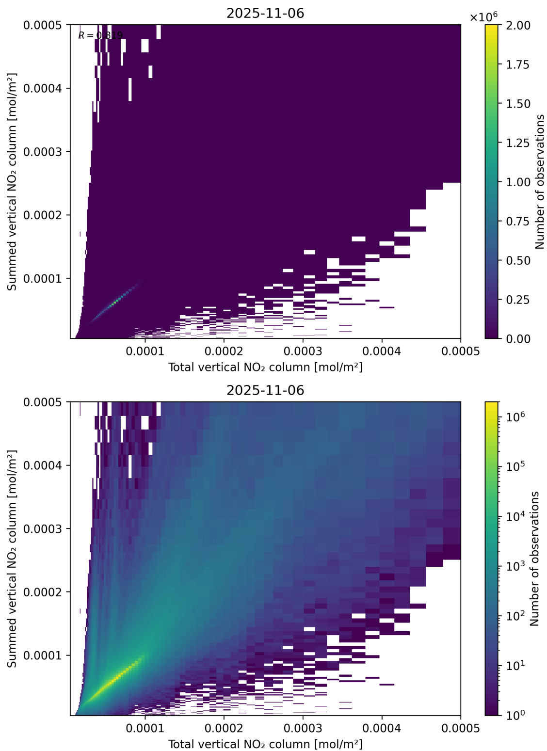
Figure 112: Scatter density plot of “Total vertical NO 2 column” against “Summed vertical NO 2 column” for 2025-11-05 to 2025-11-07.
