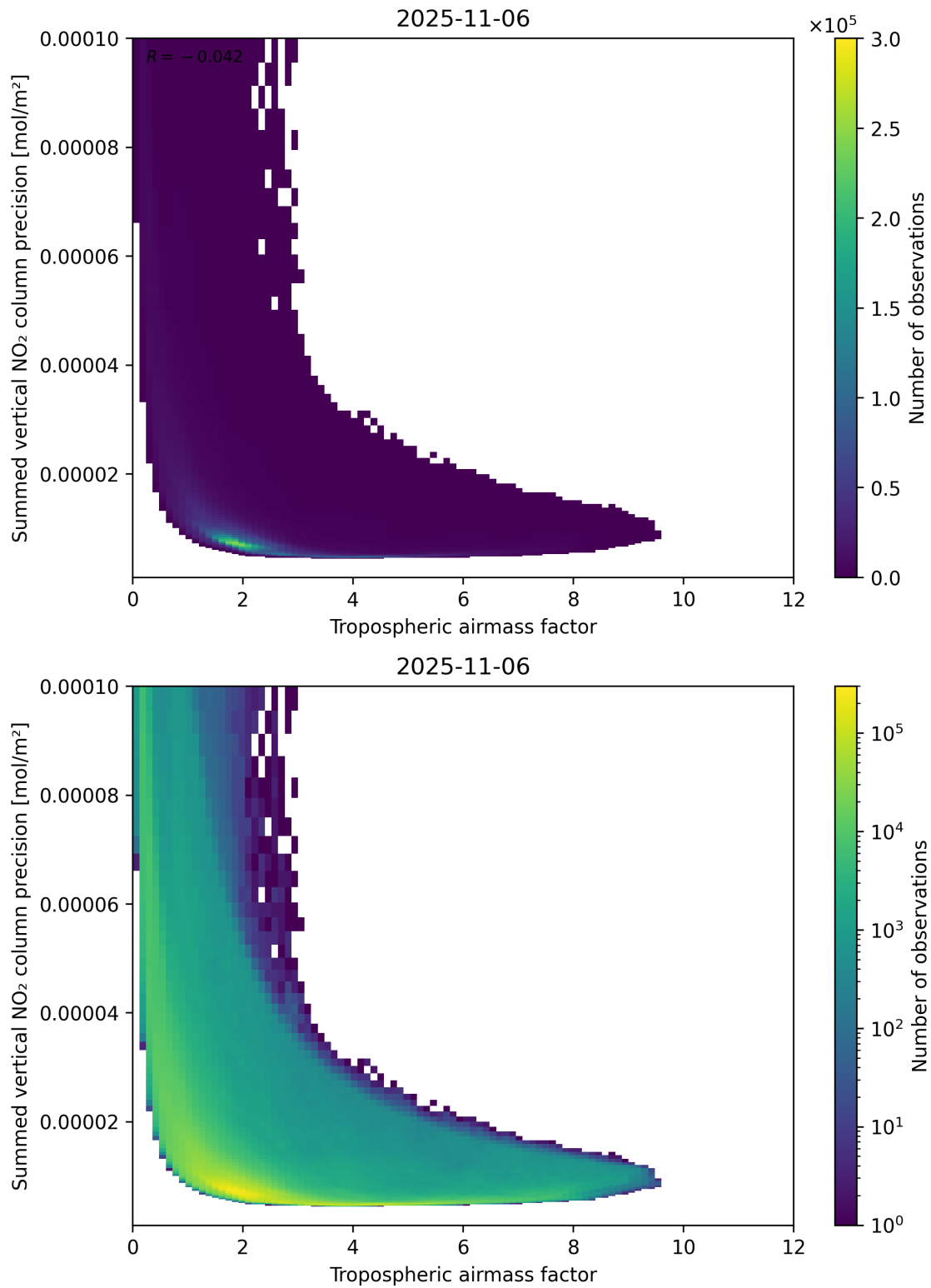
Figure 76: Scatter density plot of “Tropospheric airmass factor” against “Summed vertical NO 2 column precision” for 2025-11-05 to 2025-11-07.
