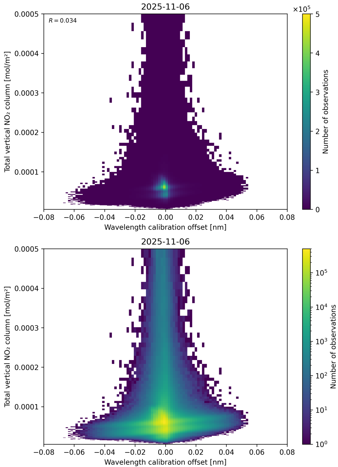
Figure 179: Scatter density plot of “Wavelength calibration offset” against “Total vertical NO 2 column” for 2025-11-05 to 2025-11-07.
