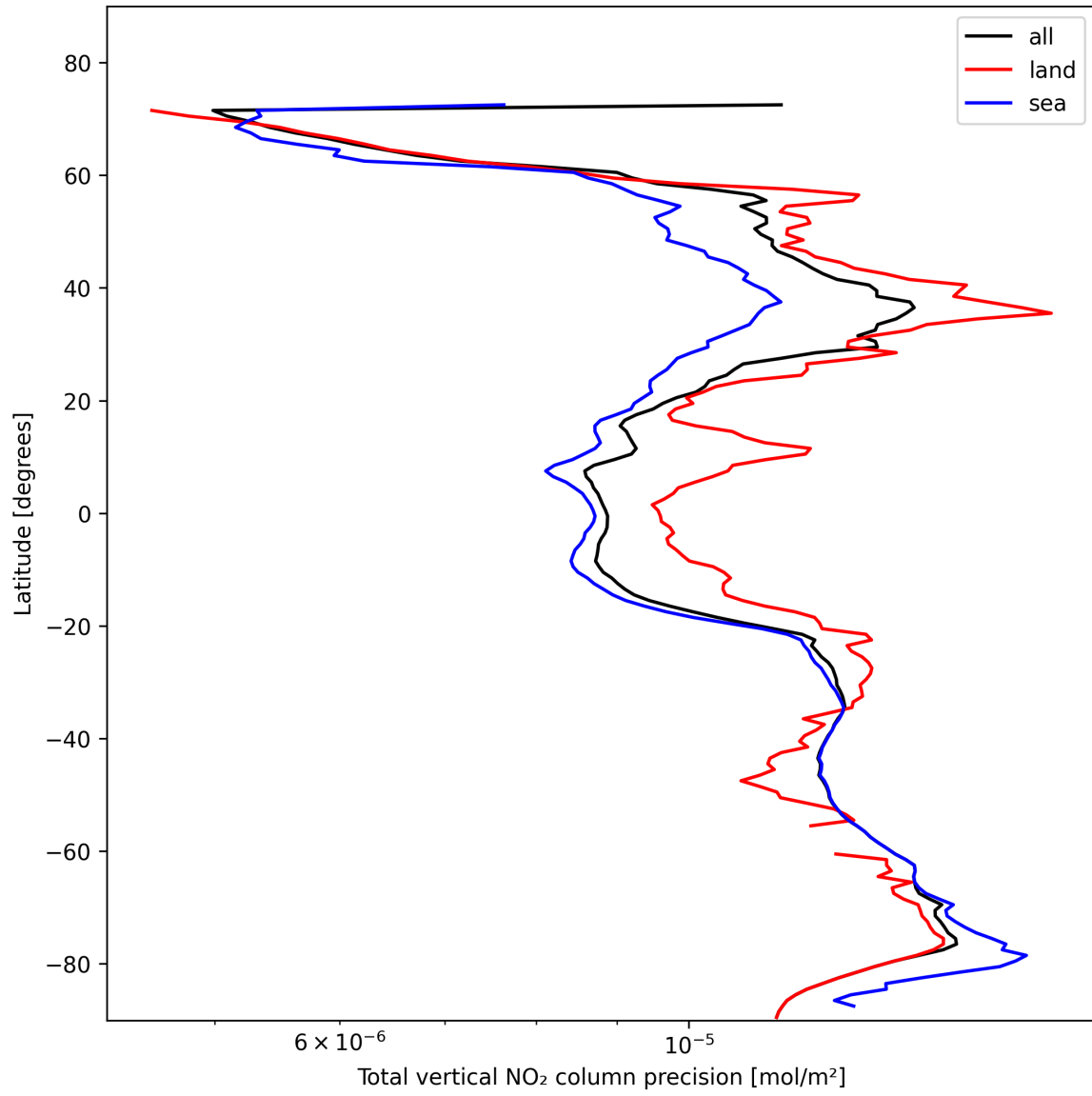
Figure 22: Zonal average of “Total vertical NO 2 column precision” for 2025-11-05 to 2025-11-07.
