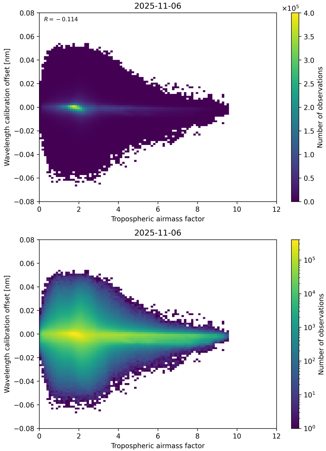
Figure 80: Scatter density plot of “Tropospheric airmass factor” against “Wavelength calibration offset” for 2025-11-05 to 2025-11-07.
