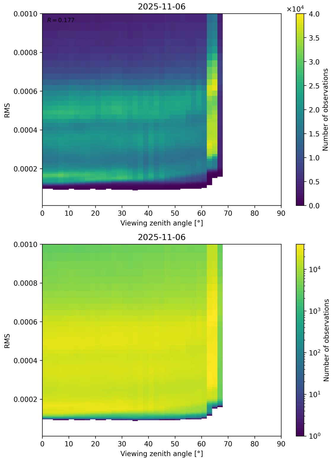
Figure 171: Scatter density plot of “Viewing zenith angle” against “RMS” for 2025-11-05 to 2025-11-07.
