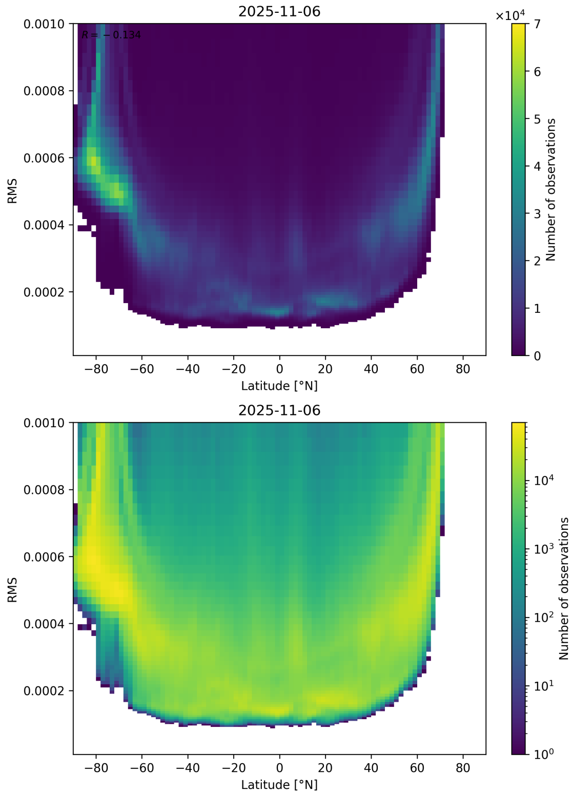
Figure 94: Scatter density plot of “Latitude” against “RMS” for 2025-11-05 to 2025-11-07.
