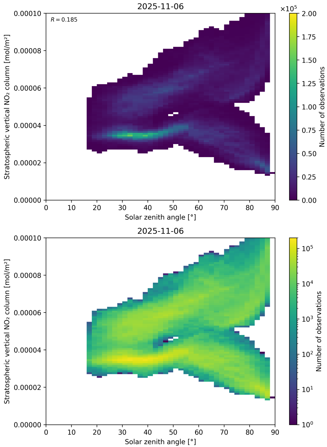
Figure 150: Scatter density plot of “Solar zenith angle” against “Stratospheric vertical NO 2 column” for 2025-11-05 to 2025-11-07.
