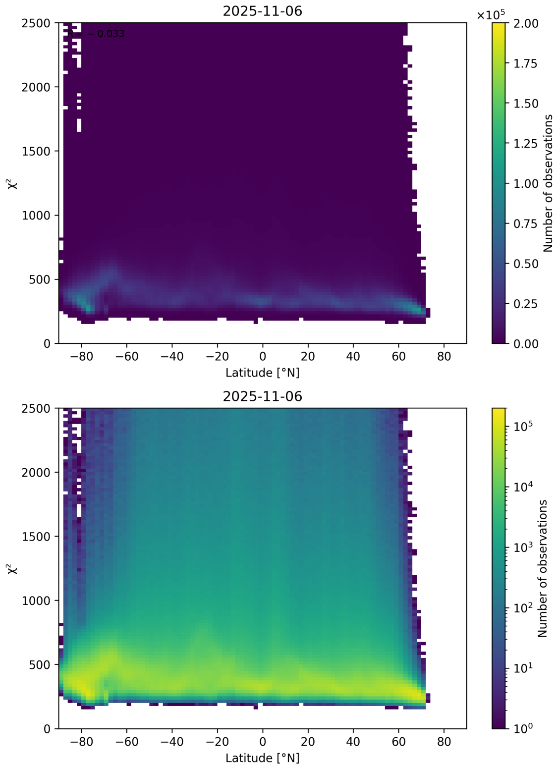
Figure 86: Scatter density plot of “Latitude” against “ \chi^2 ” for 2025-11-05 to 2025-11-07.
