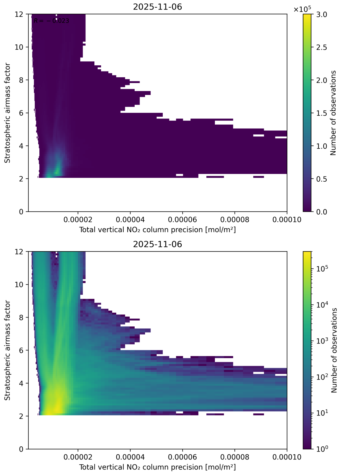
Figure 115: Scatter density plot of “Total vertical NO 2 column precision” against “Stratospheric airmass factor” for 2025-11-05 to 2025-11-07.
