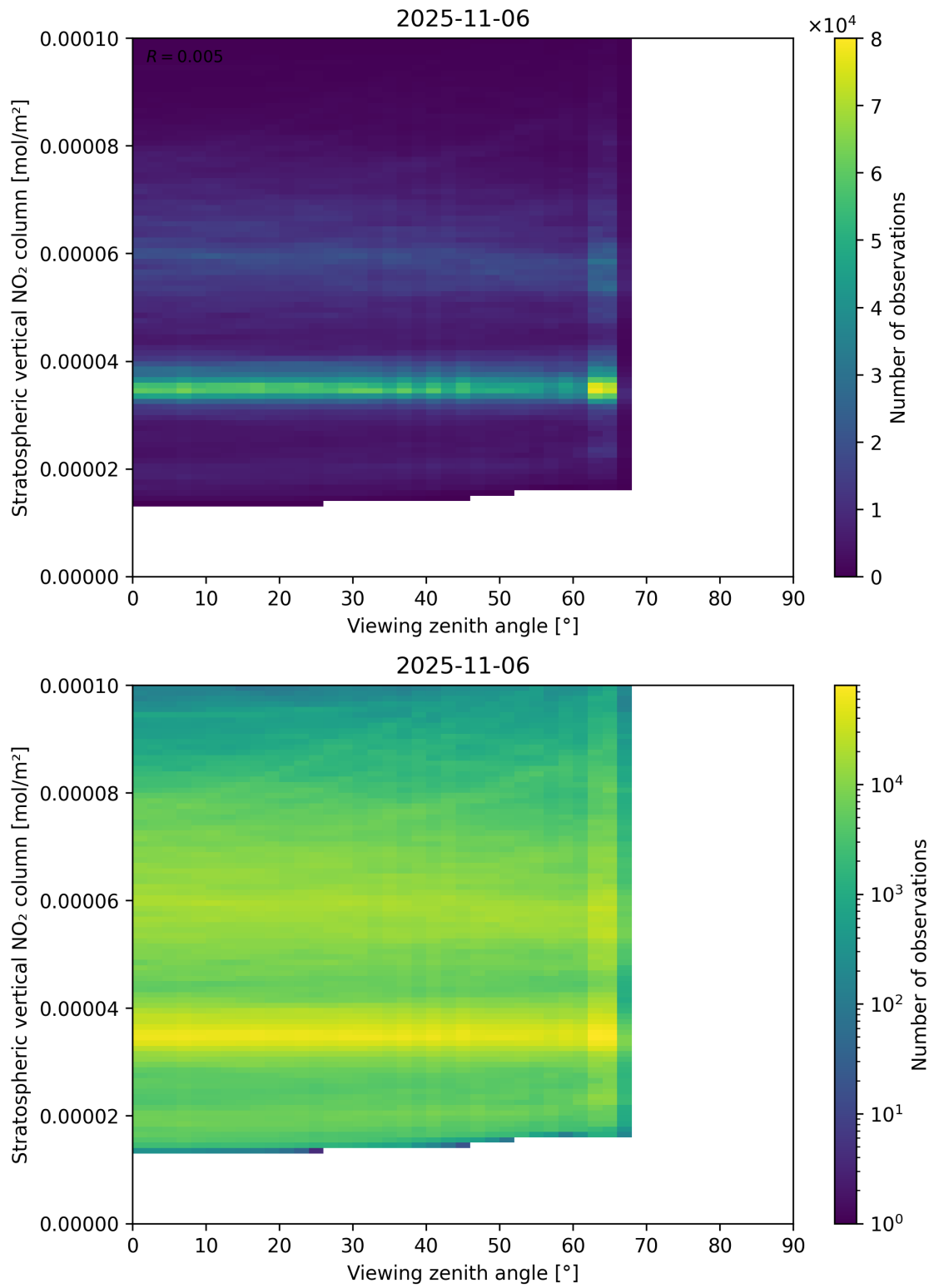
Figure 164: Scatter density plot of “Viewing zenith angle” against “Stratospheric vertical NO 2 column” for 2025-11-05 to 2025-11-07.
