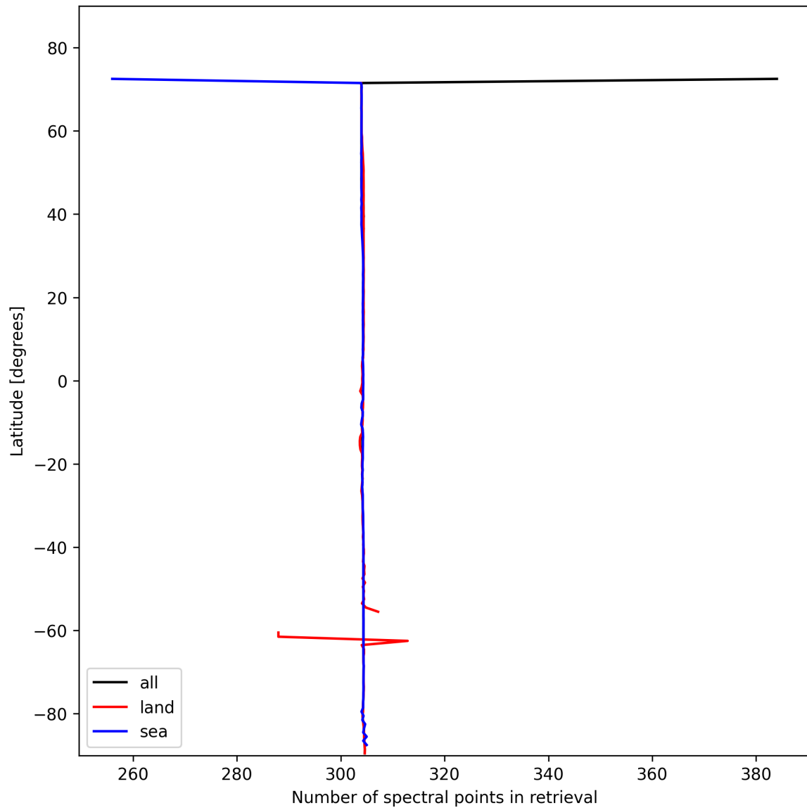
Figure 16: Zonal average of “Number of spectral points in retrieval” for 2025-11-05 to 2025-11-07.
