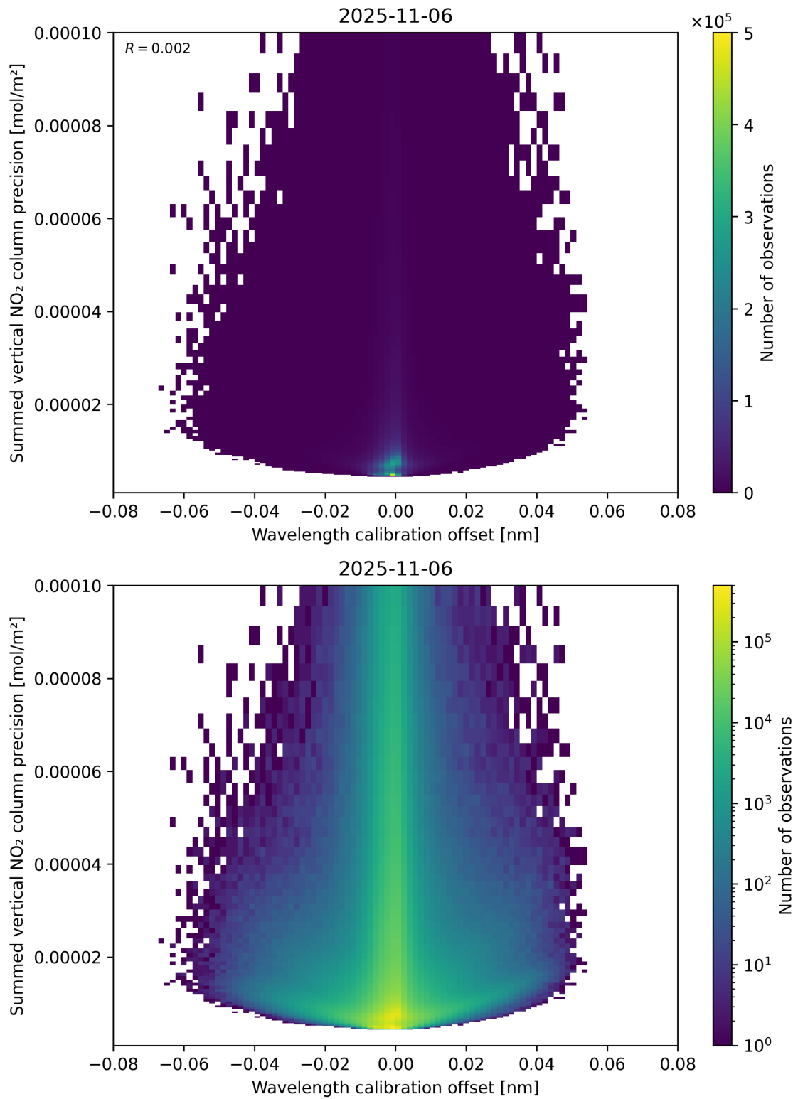
Figure 178: Scatter density plot of “Wavelength calibration offset” against “Summed vertical NO 2 column precision” for 2025-11-05 to 2025-11-07.
