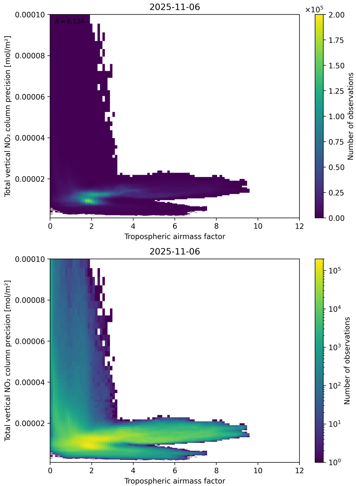
Figure 78: Scatter density plot of “Tropospheric air mass factor” against “Total vertical NO 2 column precision” for 2025-11-05 to 2025-11-07.
