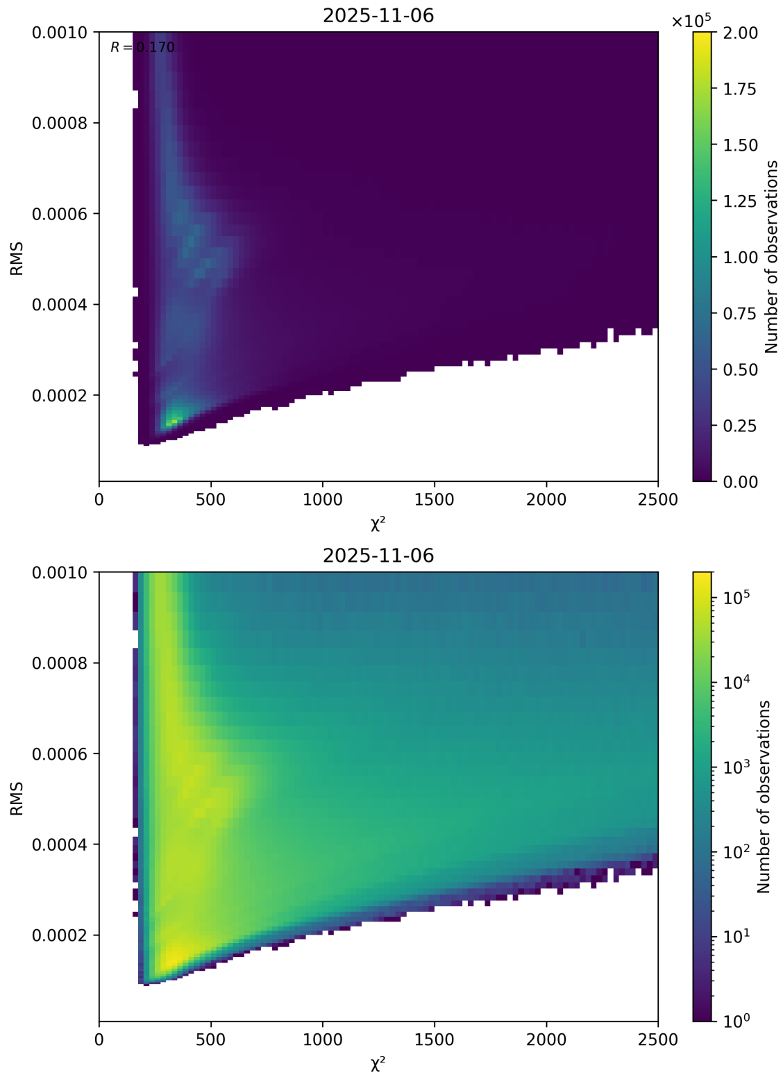
Figure 82: Scatter density plot of “ \chi^2 ” against “RMS” for 2025-11-05 to 2025-11-07.
