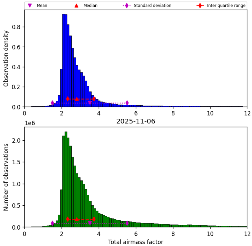
Figure 32: Histogram of “Total airmass factor” for 2025-11-05 to 2025-11-07
