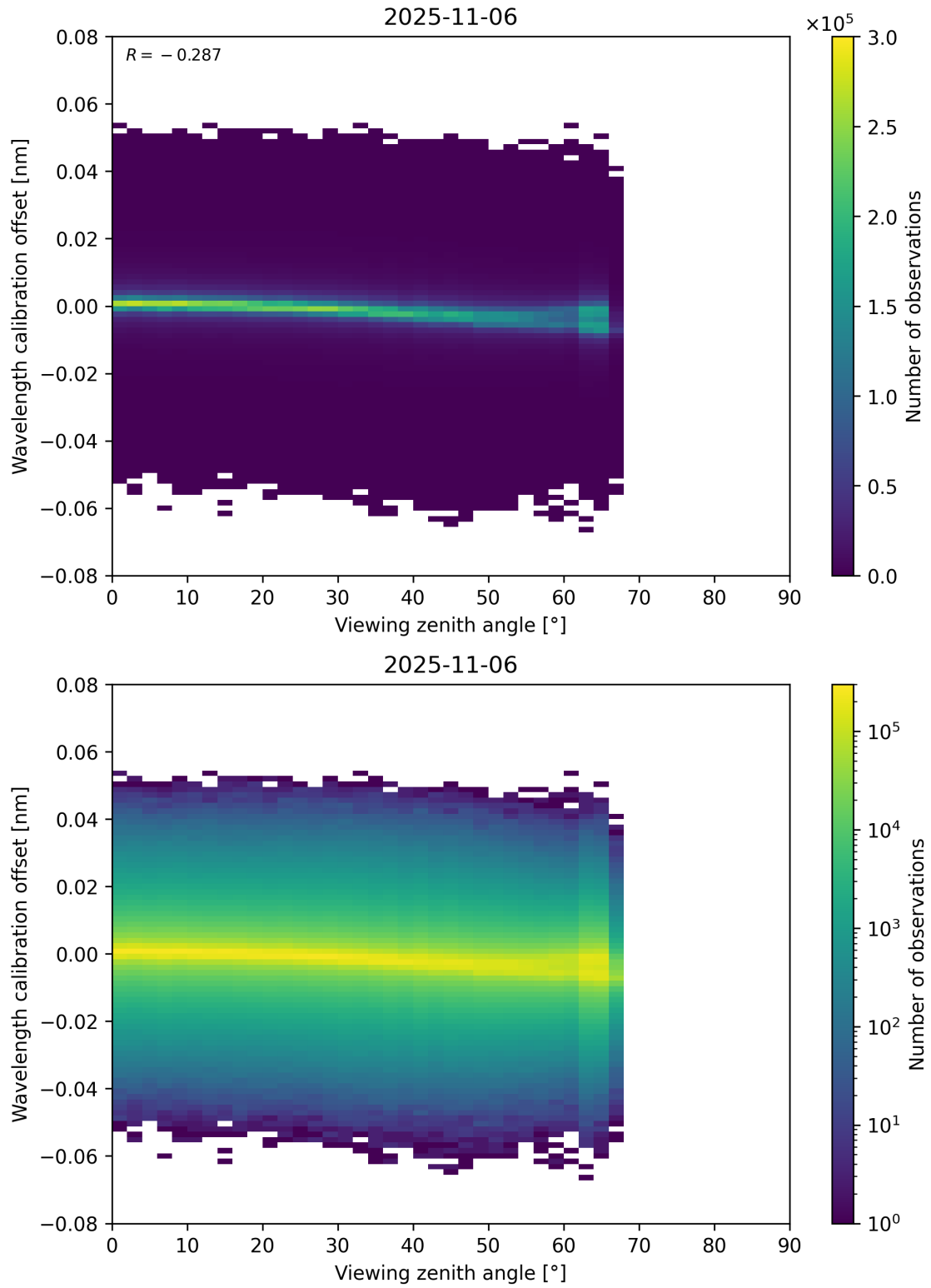
Figure 173: Scatter density plot of “Viewing zenith angle” against “Wavelength calibration offset” for 2025-11-05 to 2025-11-07.
