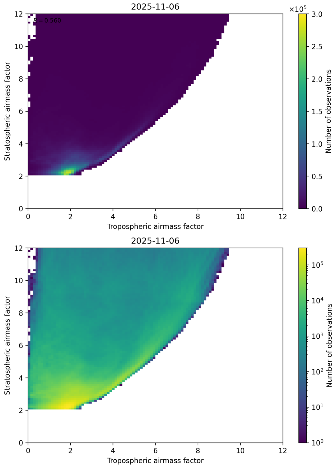
Figure 71: Scatter density plot of “Tropospheric airmass factor” against “Stratospheric airmass factor” for 2025-11-05 to 2025-11-07.
