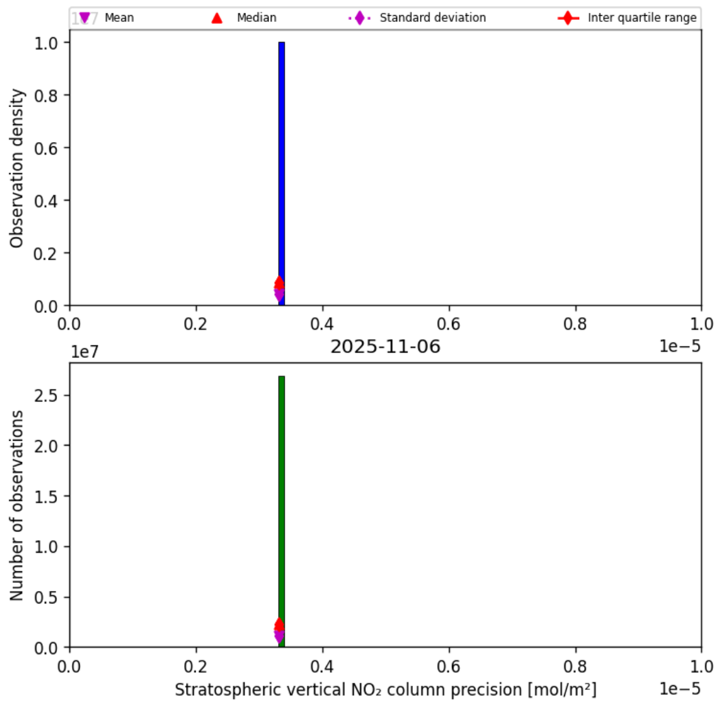
Figure 37: Histogram of “Stratospheric vertical NO 2 column precision” for 2025-11-05 to 2025-11-07
