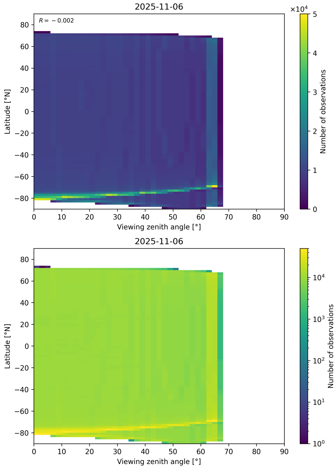
Figure 163: Scatter density plot of “Viewing zenith angle” against “Latitude” for 2025-11-05 to 2025-11-07.
