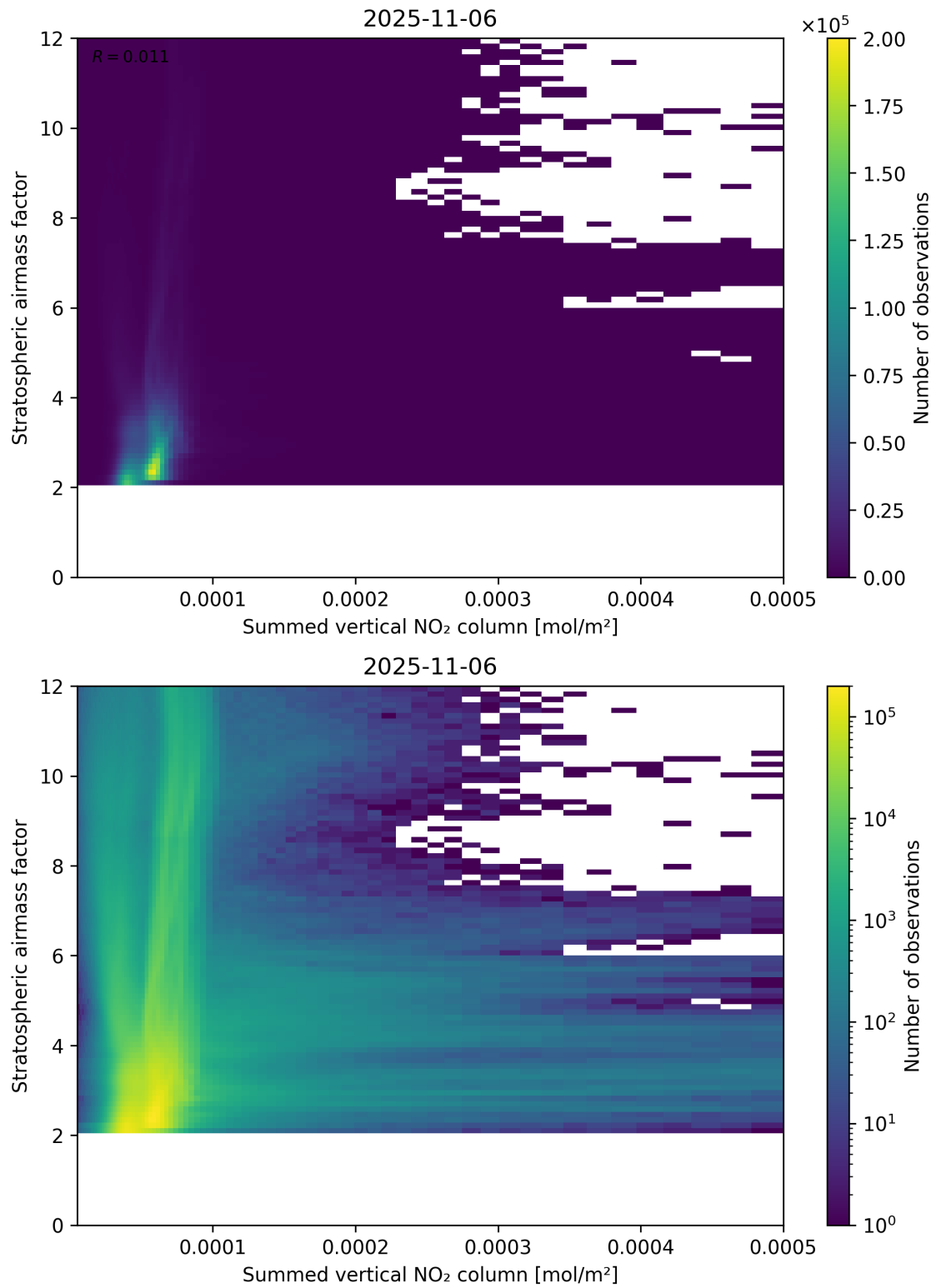
Figure 103: Scatter density plot of “Summed vertical NO 2 column” against “Stratospheric air mass factor” for 2025-11-05 to 2025-11-07.
