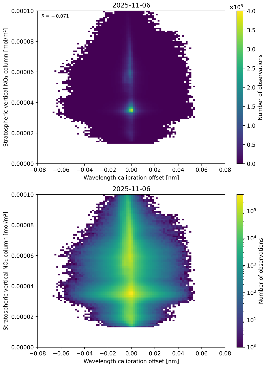
Figure 176: Scatter density plot of “Wavelength calibration offset” against “Stratospheric vertical NO 2 column” for 2025-11-05 to 2025-11-07.
