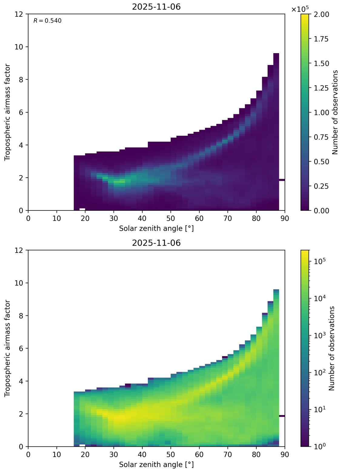
Figure 147: Scatter density plot of “Solar zenith angle” against “Tropospheric airmass factor” for 2025-11-05 to 2025-11-07.
