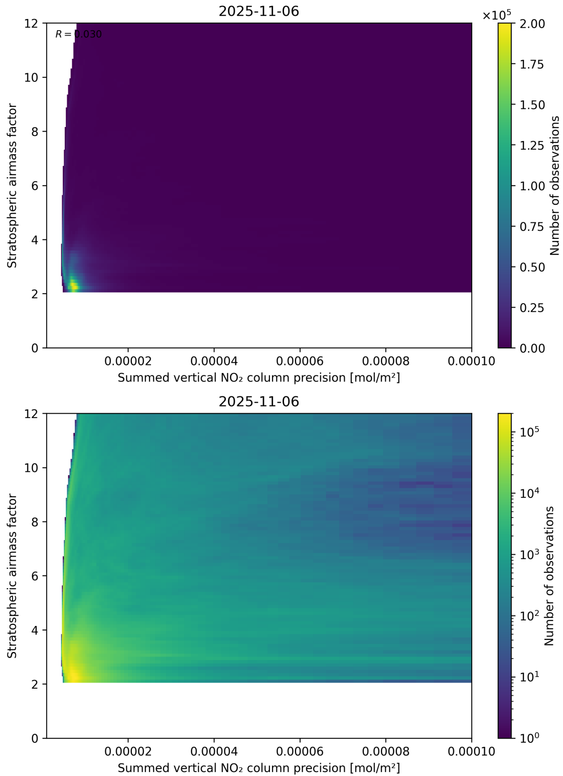
Figure 106: Scatter density plot of “Summed vertical NO 2 column precision” against “Stratospheric airmass factor” for 2025-11-05 to 2025-11-07.
