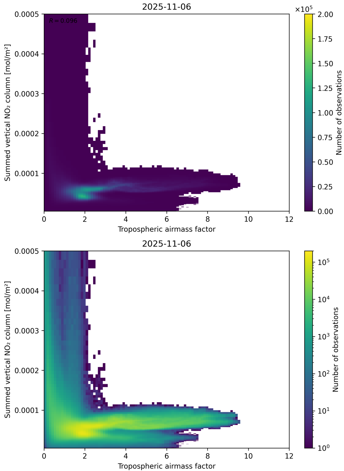
Figure 75: Scatter density plot of “Tropospheric air mass factor” against “Summed vertical NO 2 column” for 2025-11-05 to 2025-11-07.
