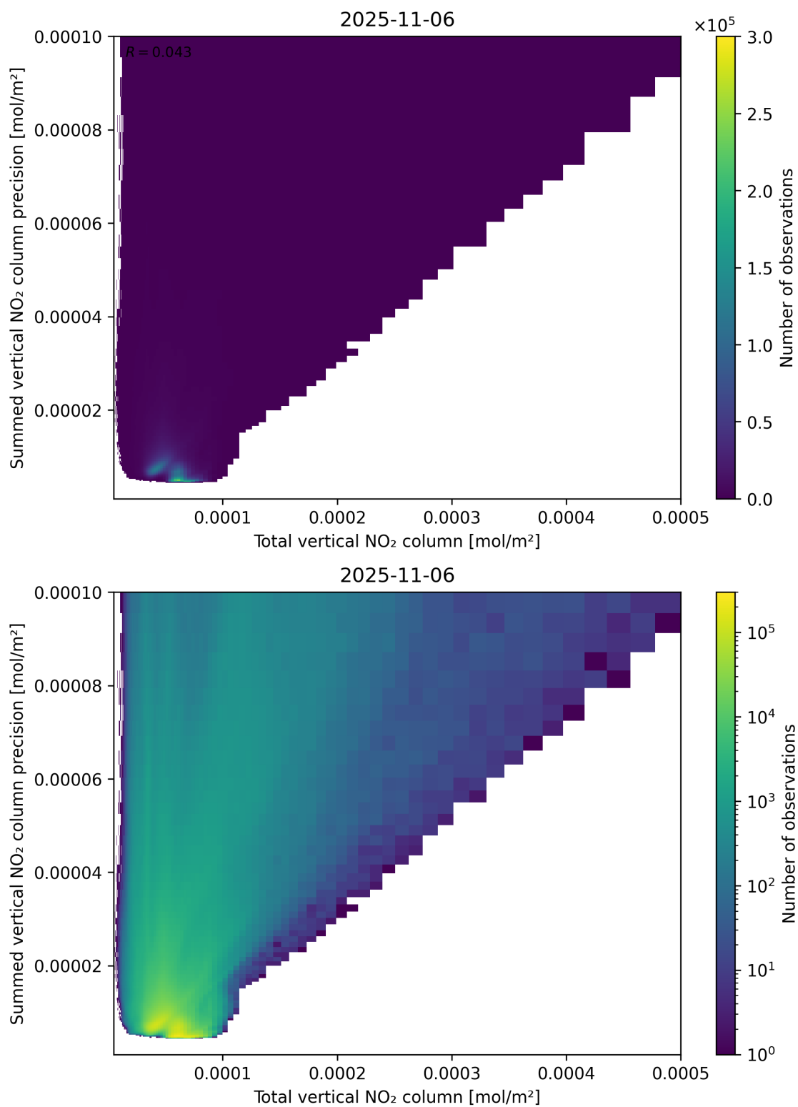
Figure 113: Scatter density plot of “Total vertical NO 2 column” against “Summed vertical NO 2 column precision” for 2025-11-05 to 2025-11-07.
