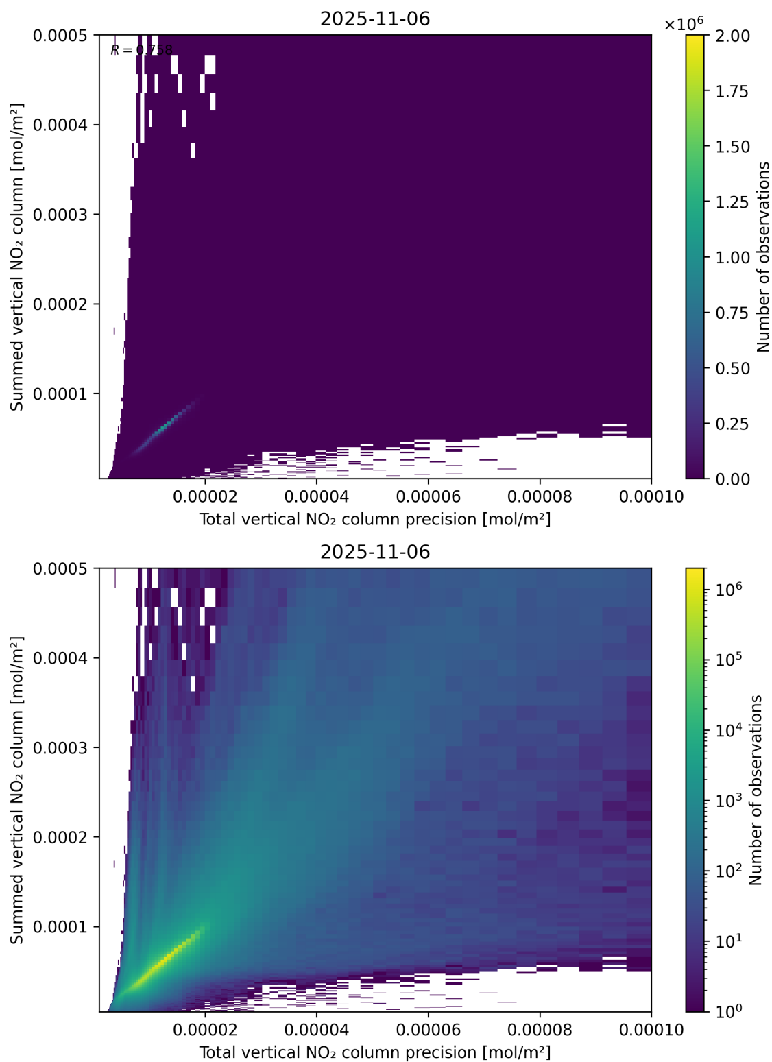
Figure 117: Scatter density plot of “Total vertical NO 2 column precision” against “Summed vertical NO 2 column” for 2025-11-05 to 2025-11-07.
