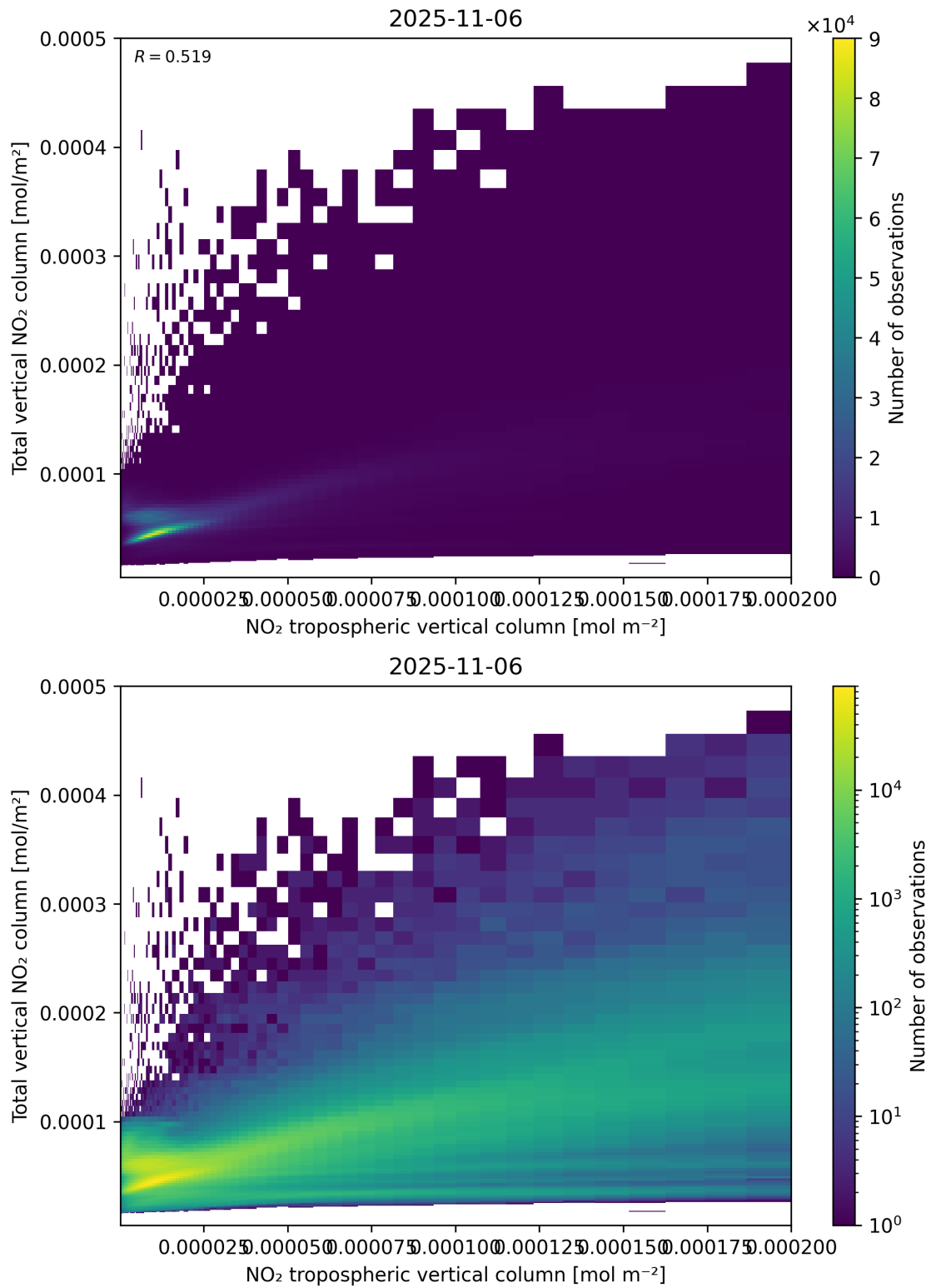
Figure 128: Scatter density plot of “NO 2 tropospheric vertical column” against “Total vertical NO 2 column” for 2025-11-05 to 2025-11-07.
