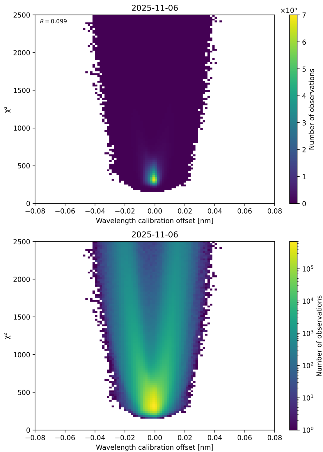
Figure 175: Scatter density plot of “Wavelength calibration offset” against “ \chi^2 ” for 2025-11-05 to 2025-11-07.
