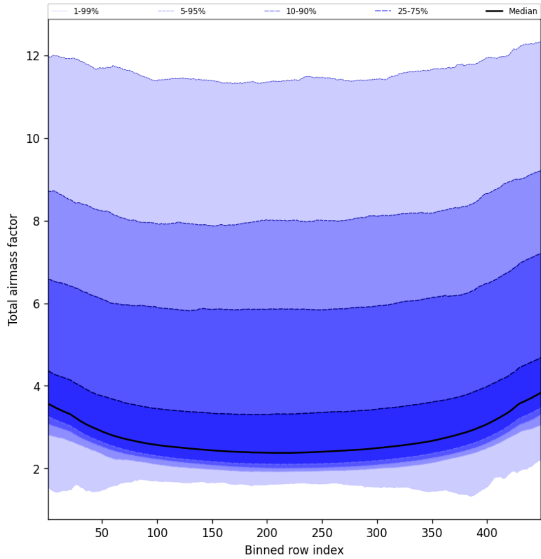
Figure 49: Along track statistics of “Total airmass factor” for 2025-11-05 to 2025-11-07
