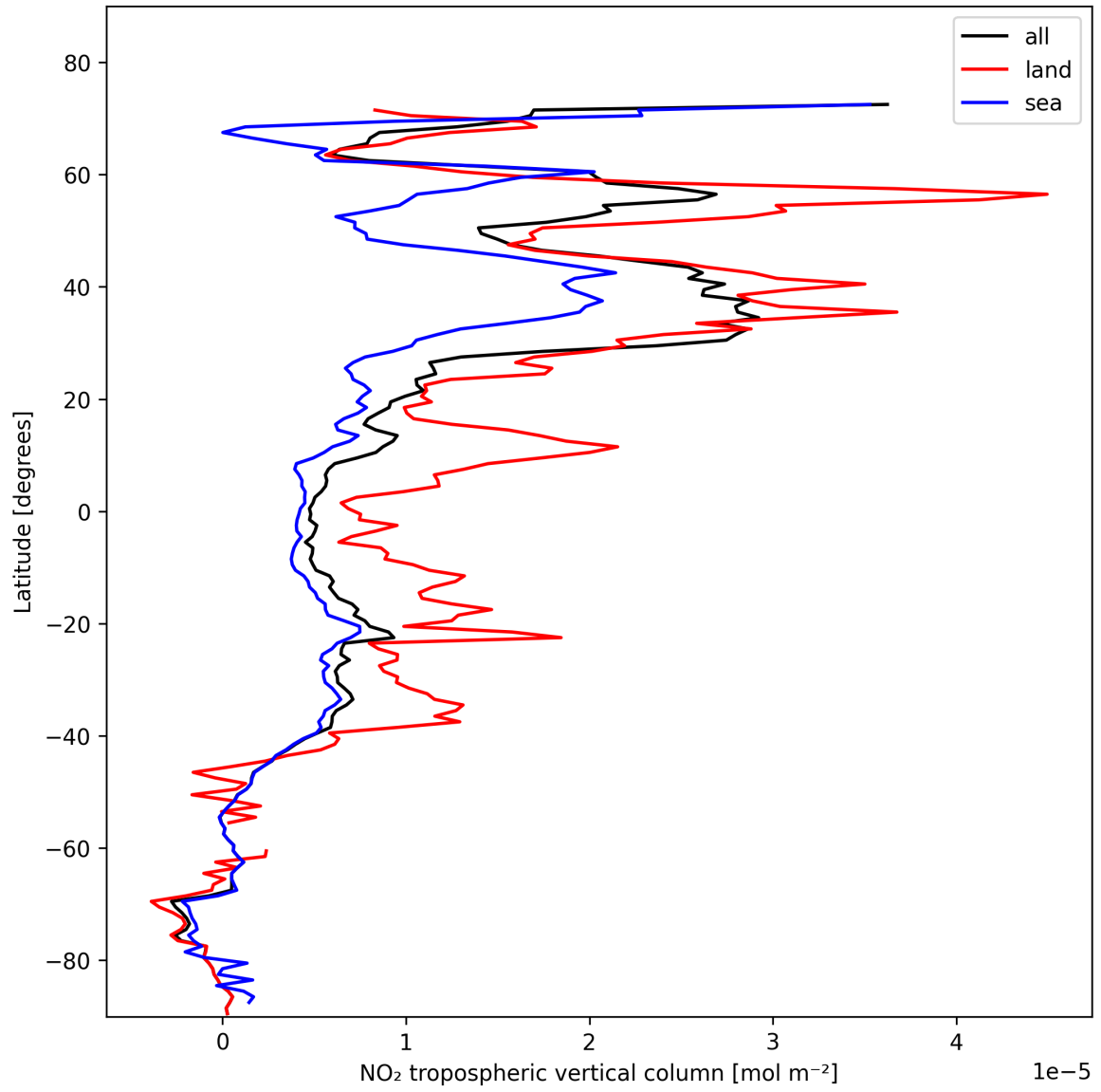
Figure 12: Zonal average of “NO 2 tropospheric vertical column” for 2025-11-05 to 2025-11-07.
