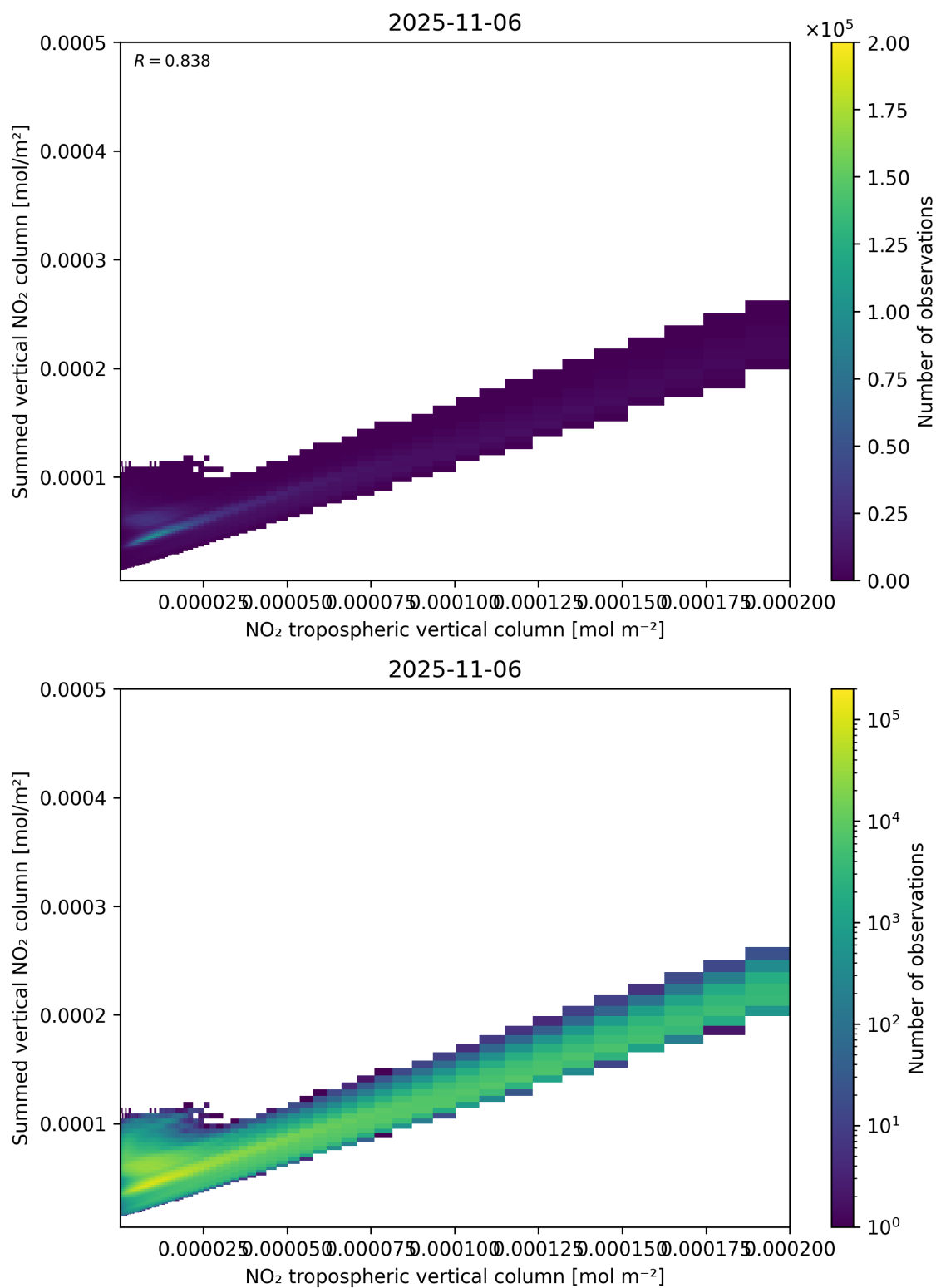
Figure 126: Scatter density plot of “NO 2 tropospheric vertical column” against “Summed vertical NO 2 column” for 2025-11-05 to 2025-11-07.
