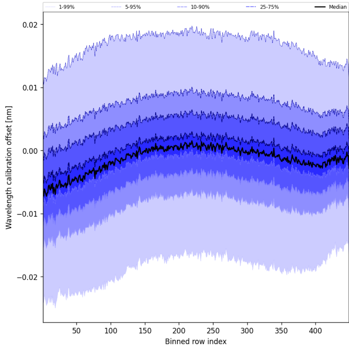
Figure 52: Along track statistics of “Wavelength calibration offset” for 2025-11-05 to 2025-11-07
