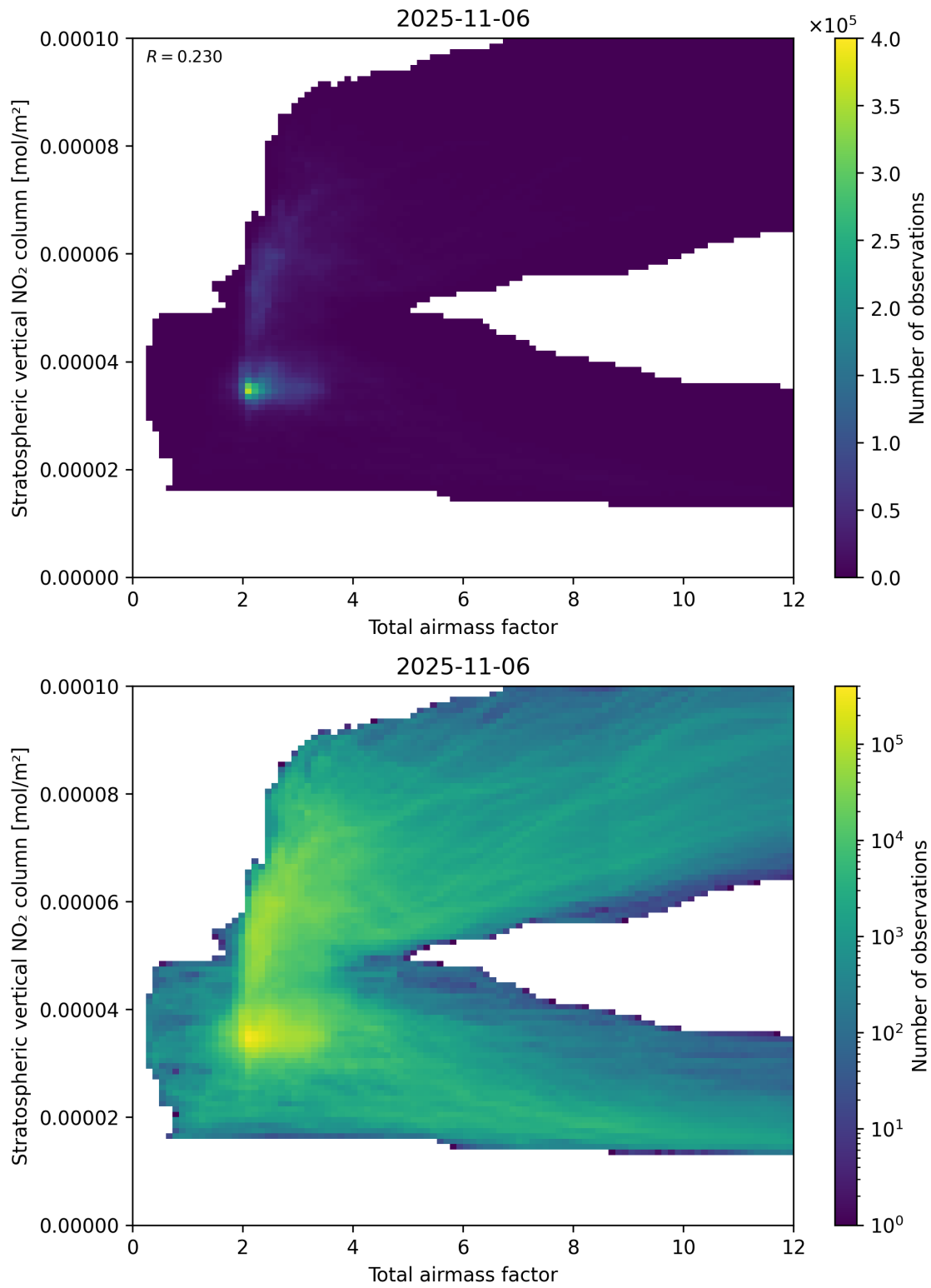
Figure 64: Scatter density plot of “Total airmass factor” against “Stratospheric vertical NO 2 column” for 2025-11-05 to 2025-11-07.
