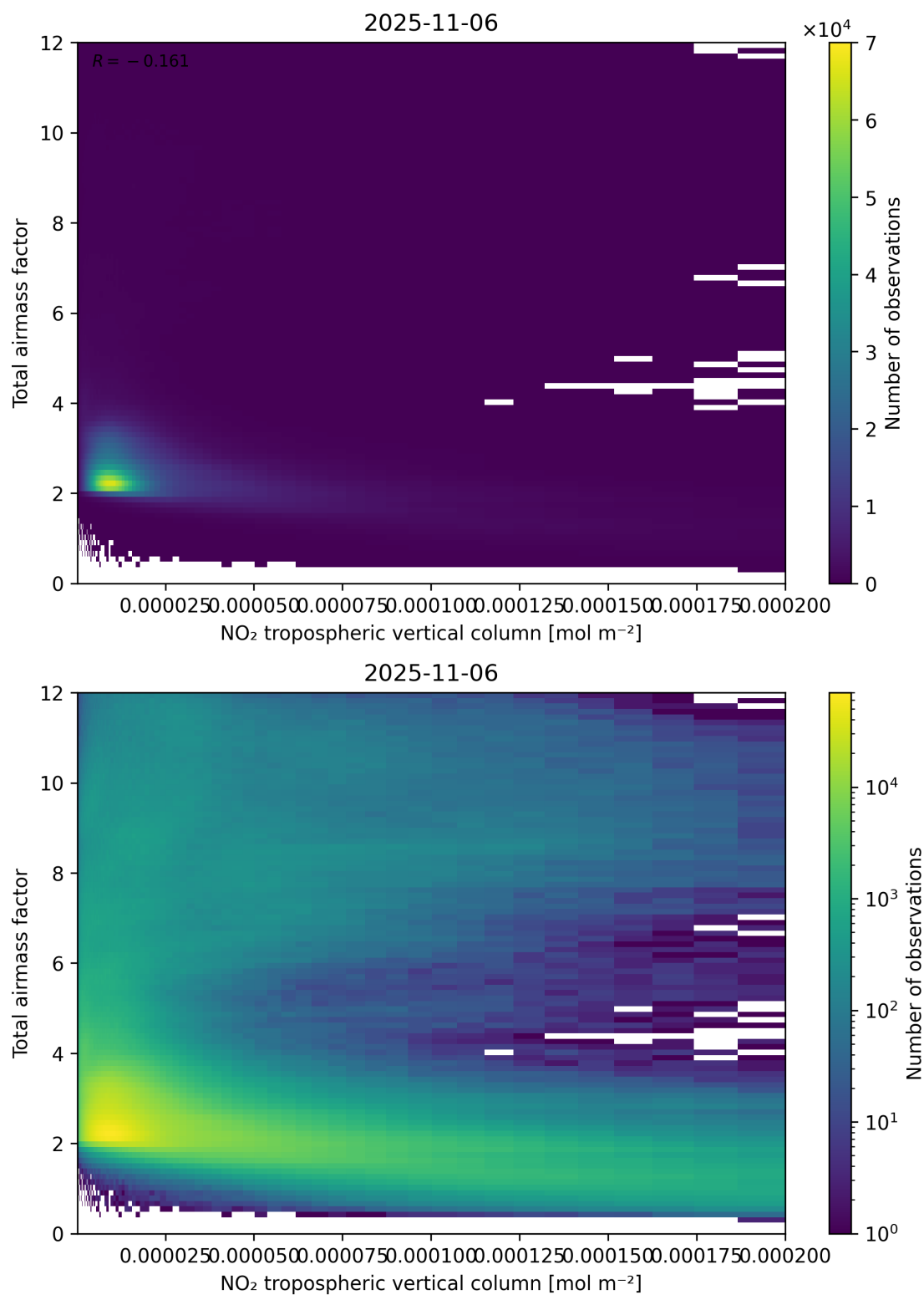
Figure 122: Scatter density plot of “NO 2 tropospheric vertical column” against “Total air mass factor” for 2025-11-05 to 2025-11-07.
