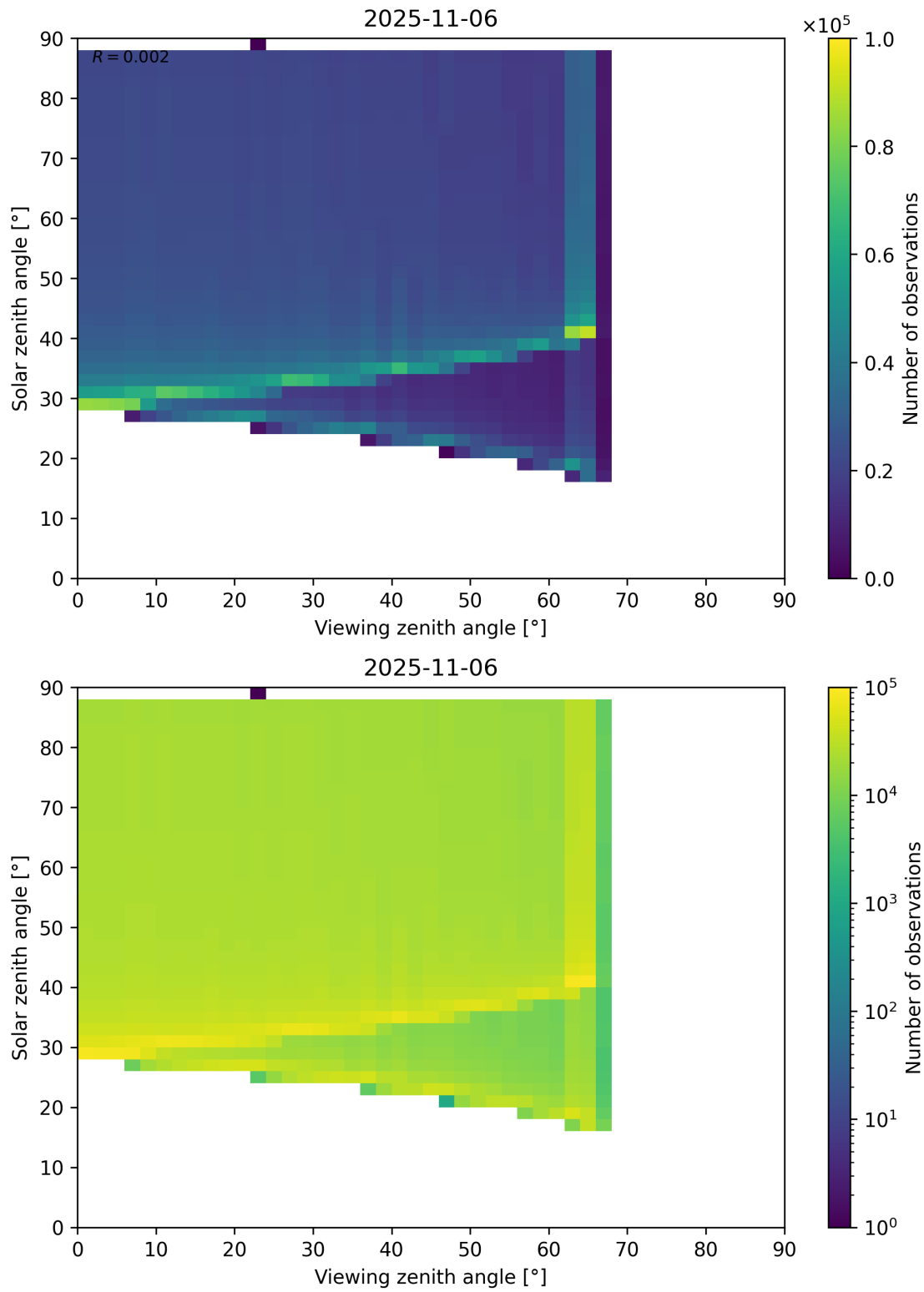
Figure 172: Scatter density plot of “Viewing zenith angle” against “Solar zenith angle” for 2025-11-05 to 2025-11-07.
