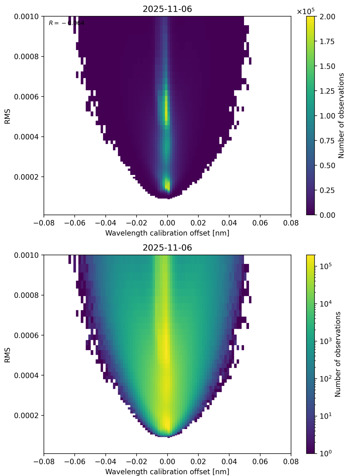
Figure 181: Scatter density plot of “Wavelength calibration offset” against “RMS” for 2025-11-05 to 2025-11-07.
