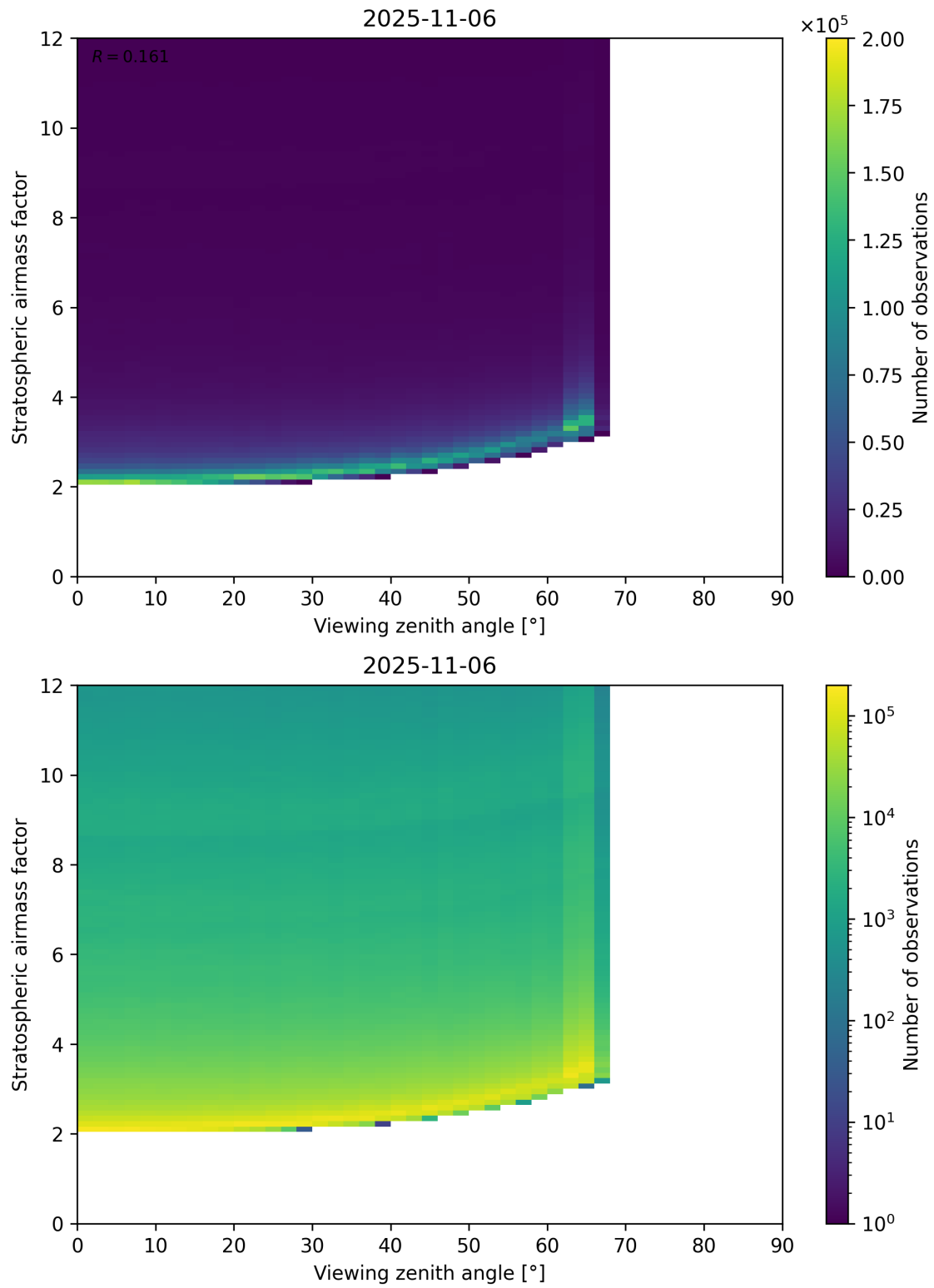
Figure 159: Scatter density plot of “Viewing zenith angle” against “Stratospheric airmass factor” for 2025-11-05 to 2025-11-07.
