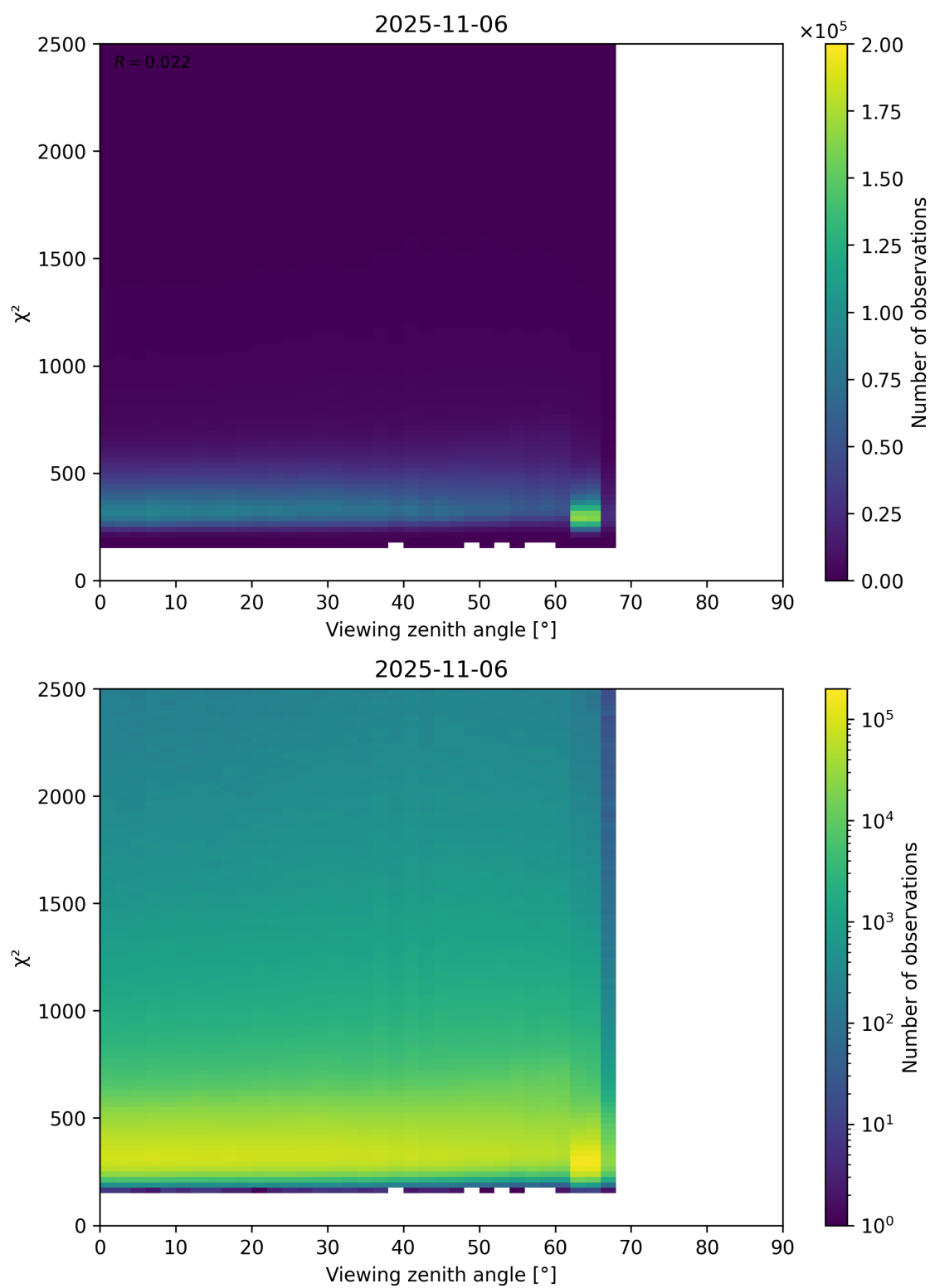
Figure 162: Scatter density plot of “Viewing zenith angle” against “ \chi^2 ” for 2025-11-05 to 2025-11-07.
