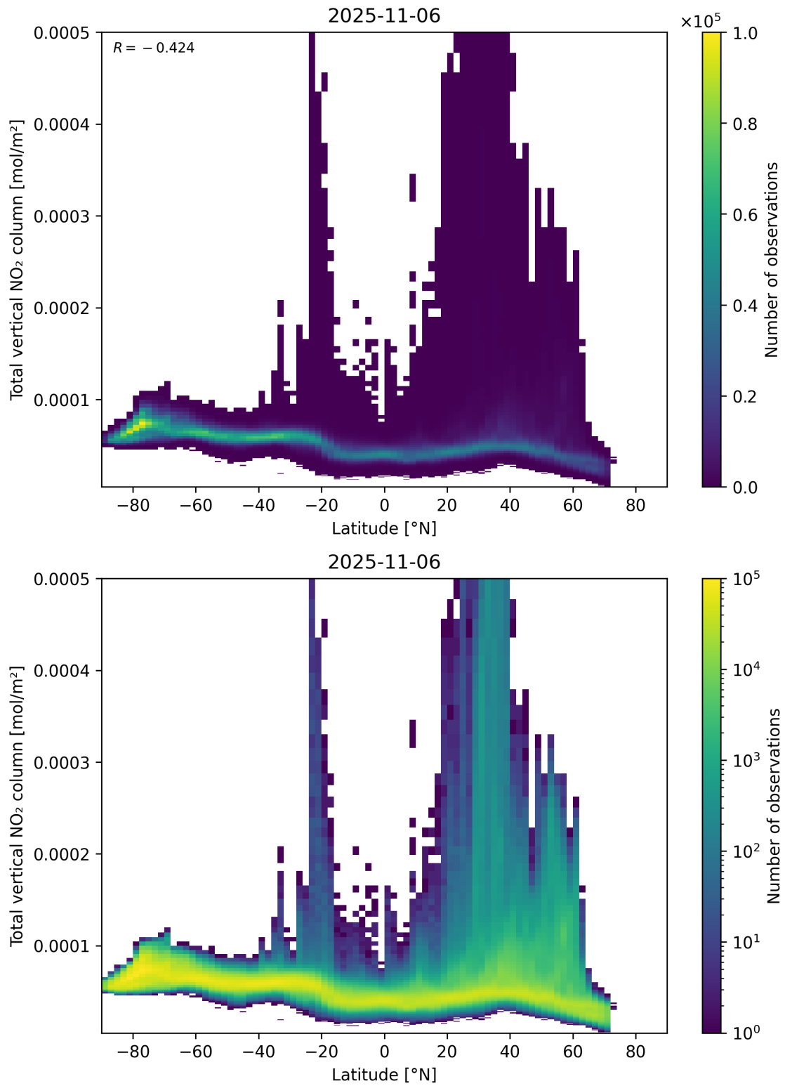
Figure 90: Scatter density plot of “Latitude” against “Total vertical NO 2 column” for 2025-11-05 to 2025-11-07.
