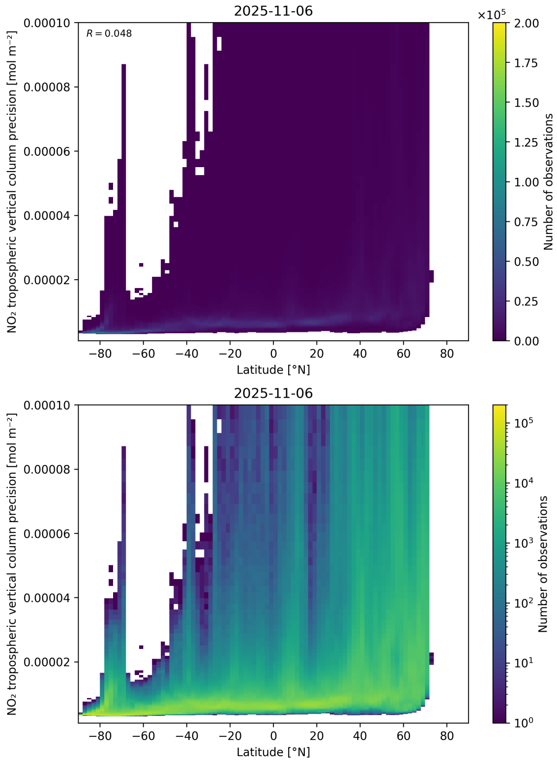
Figure 93: Scatter density plot of “Latitude” against “NO 2 tropospheric vertical column precision” for 2025-11-05 to 2025-11-07.
