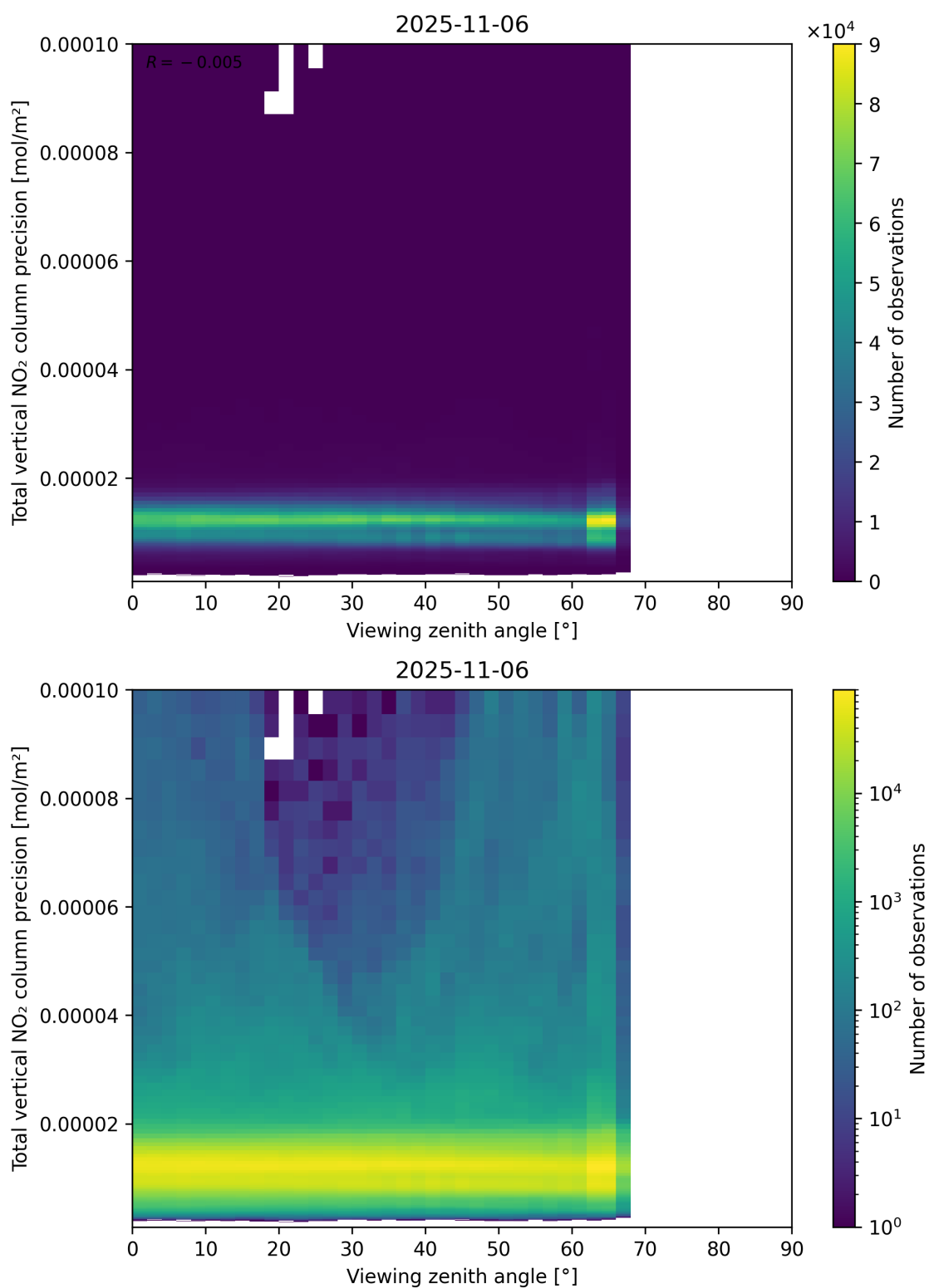
Figure 168: Scatter density plot of “Viewing zenith angle” against “Total vertical NO 2 column precision” for 2025-11-05 to 2025-11-07.
