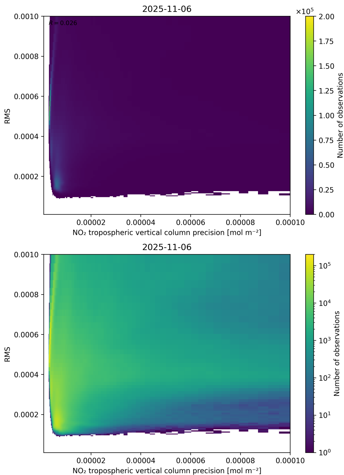
Figure 140: Scatter density plot of “NO 2 tropospheric vertical column precision” against “RMS” for 2025-11-05 to 2025-11-07.
