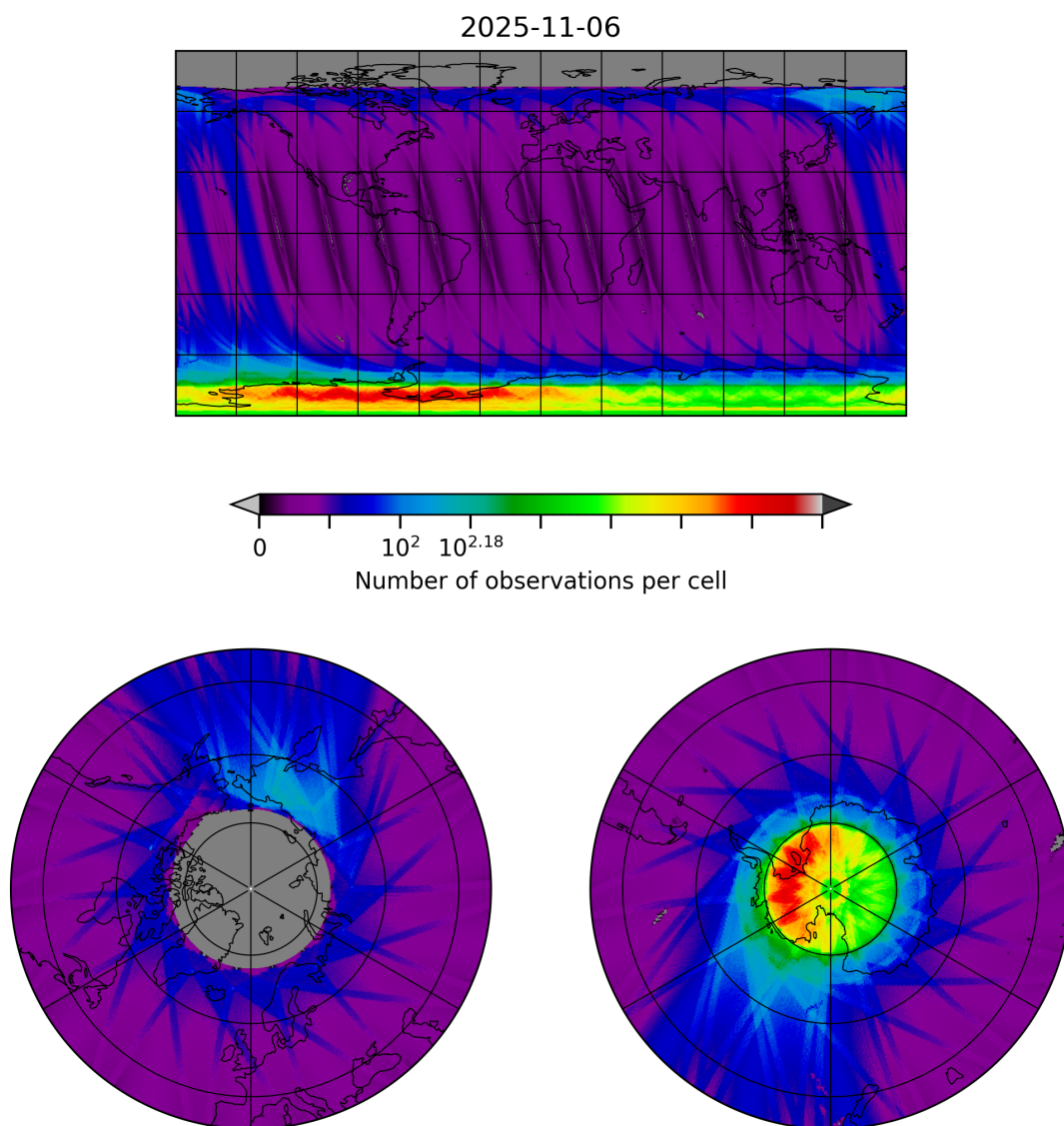
Figure 10: Map of the number of observations for 2025-11-05 to 2025-11-07
