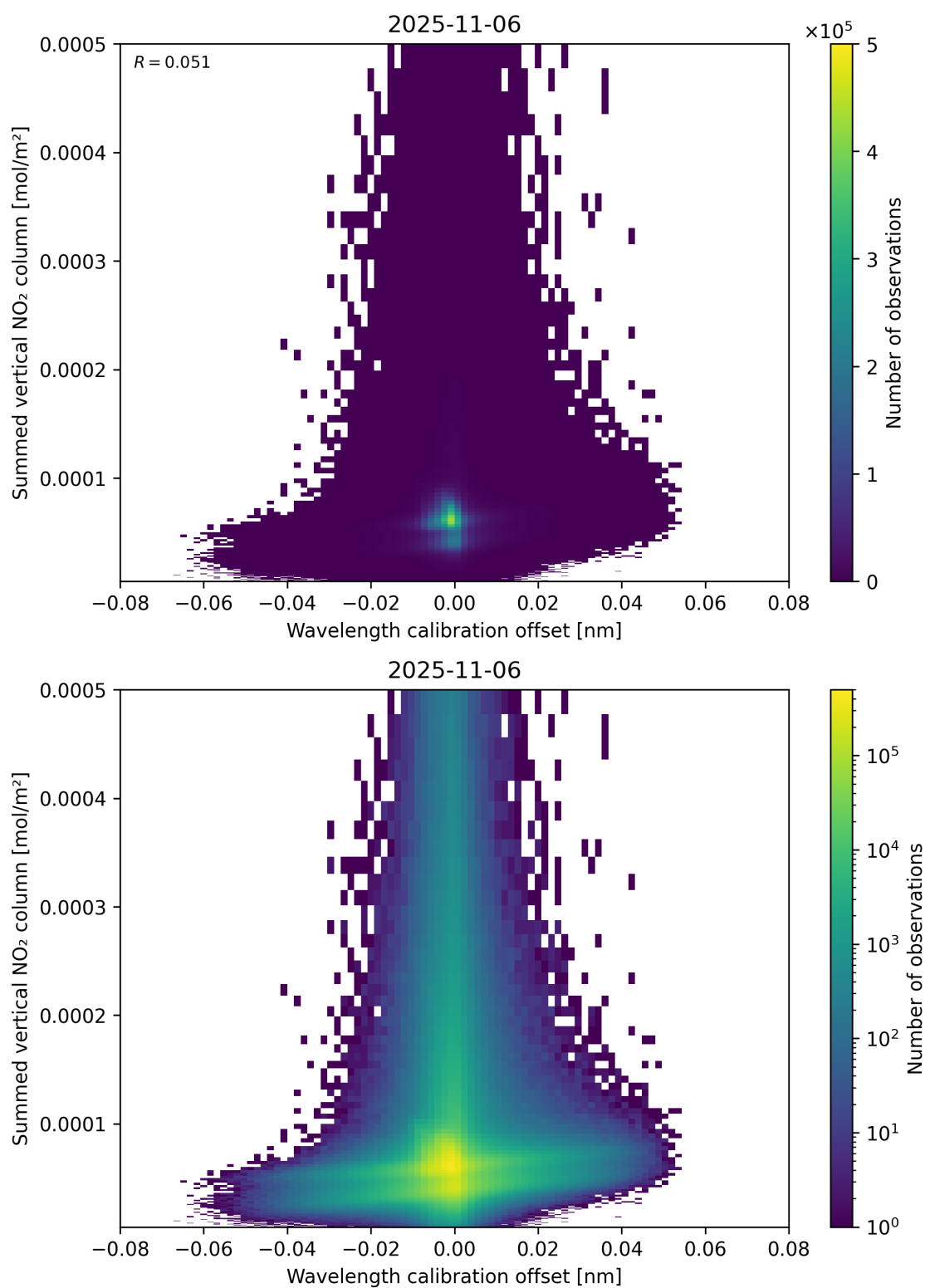
Figure 177: Scatter density plot of “Wavelength calibration offset” against “Summed vertical NO 2 column” for 2025-11-05 to 2025-11-07.
