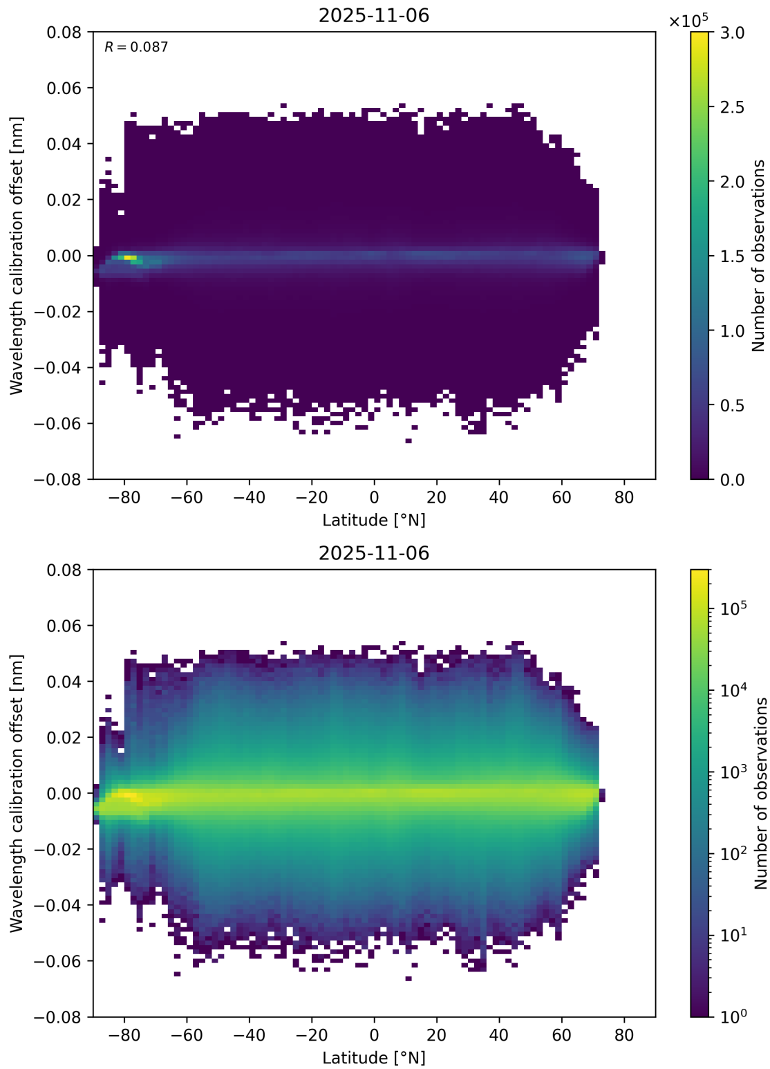
Figure 95: Scatter density plot of “Latitude” against “Wavelength calibration offset” for 2025-11-05 to 2025-11-07.
