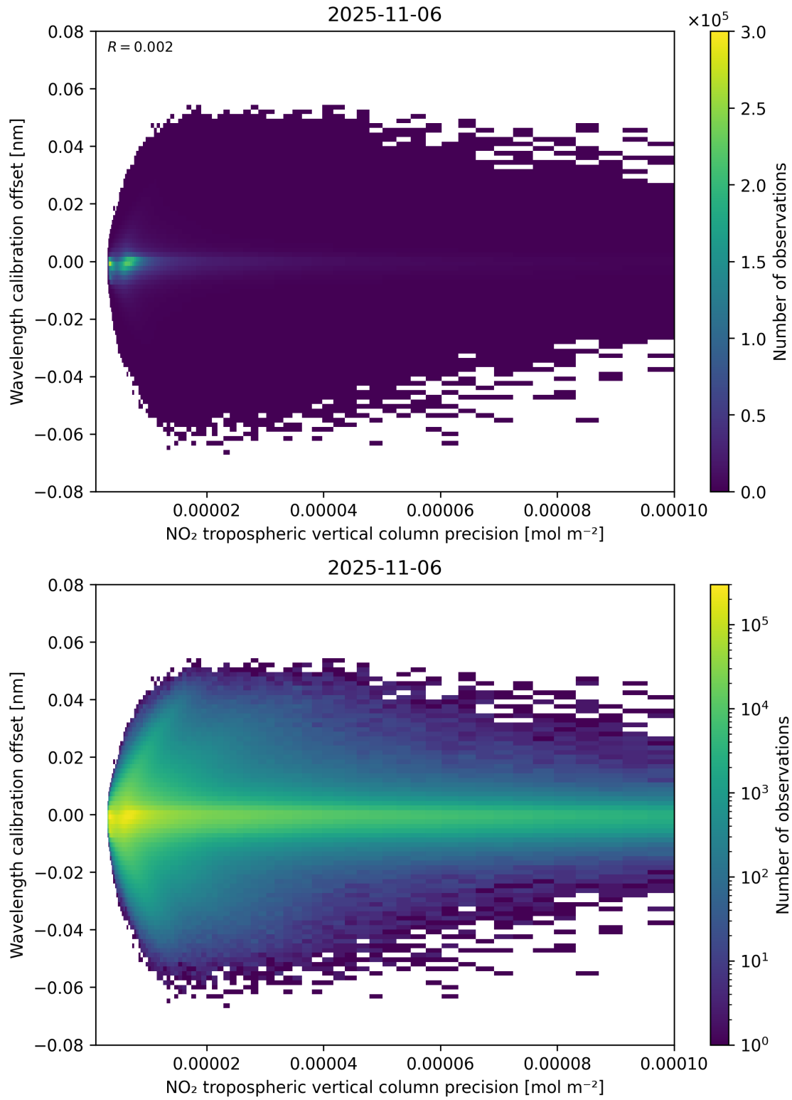
Figure 141: Scatter density plot of “NO 2 tropospheric vertical column precision” against “Wavelength calibration offset” for 2025-11-05 to 2025-11-07.
