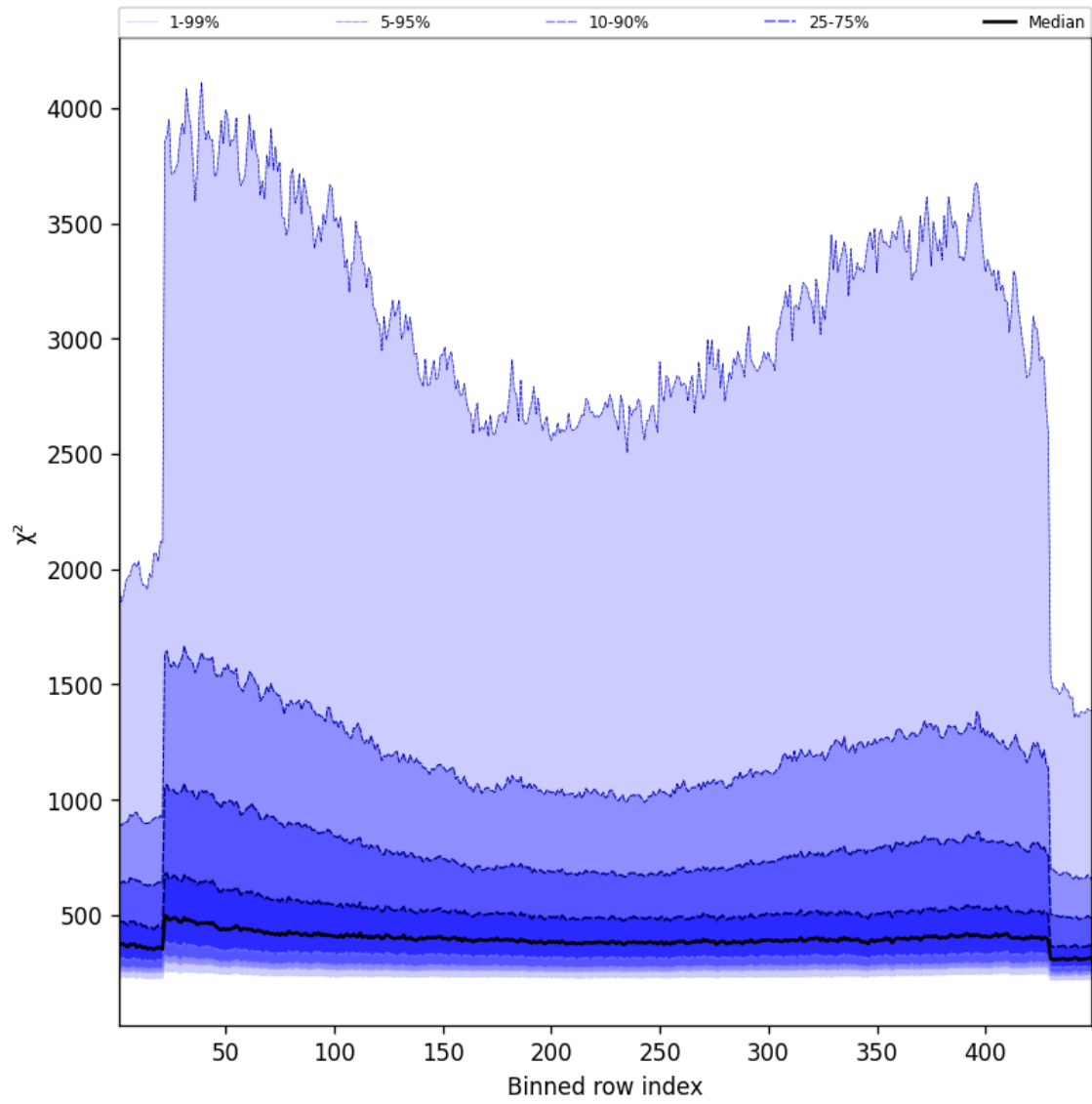
Figure 59: Along track statistics of “ \chi^2 ” for 2025-11-05 to 2025-11-07
