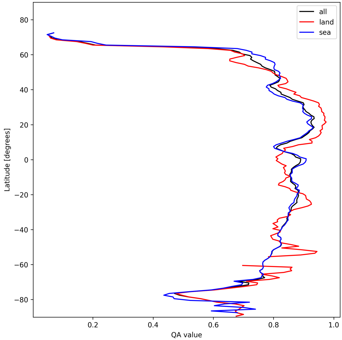
Figure 11: Zonal average of “QA value” for 2025-11-05 to 2025-11-07.
