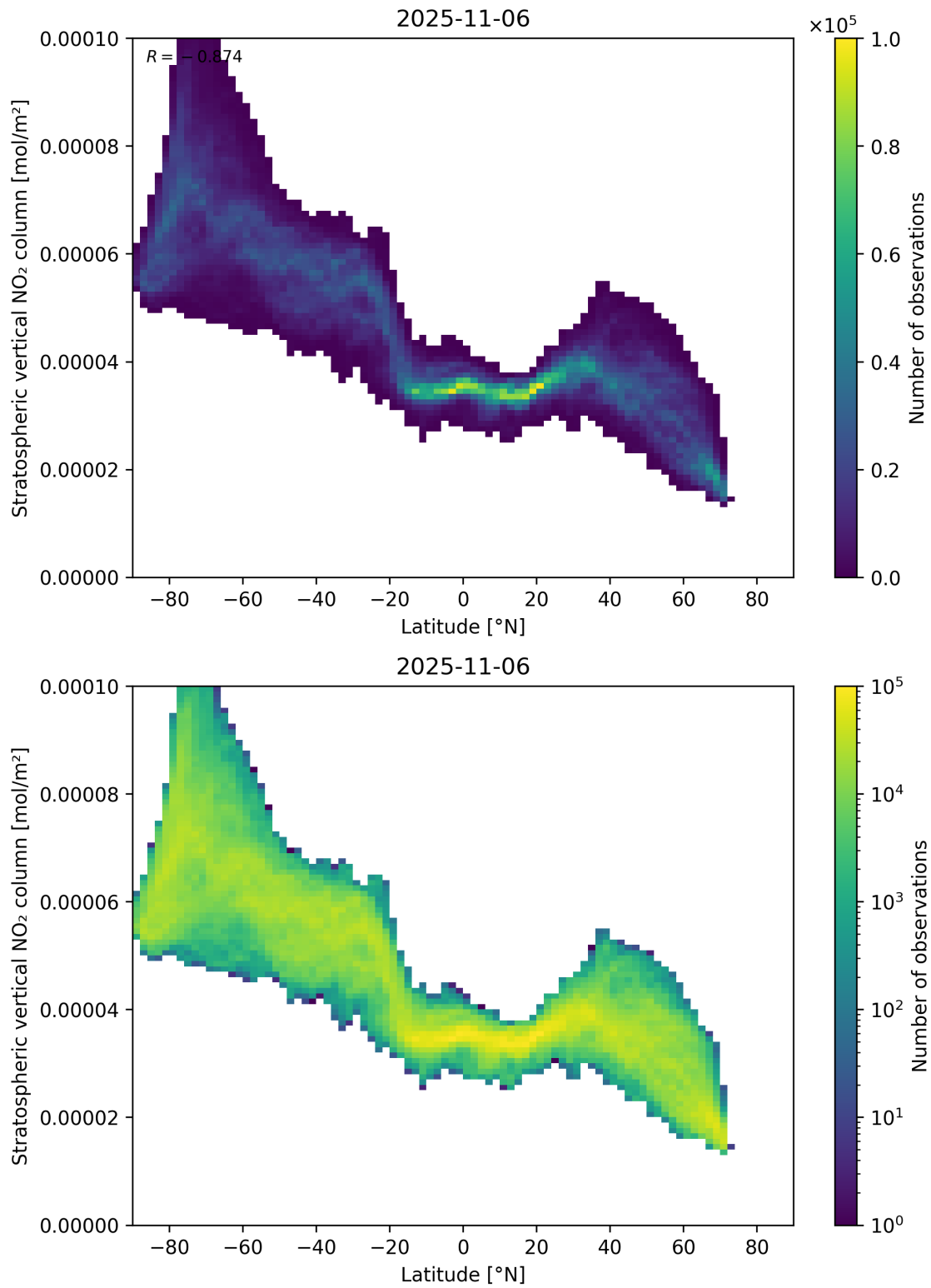
Figure 87: Scatter density plot of “Latitude” against “Stratospheric vertical NO 2 column” for 2025-11-05 to 2025-11-07.
