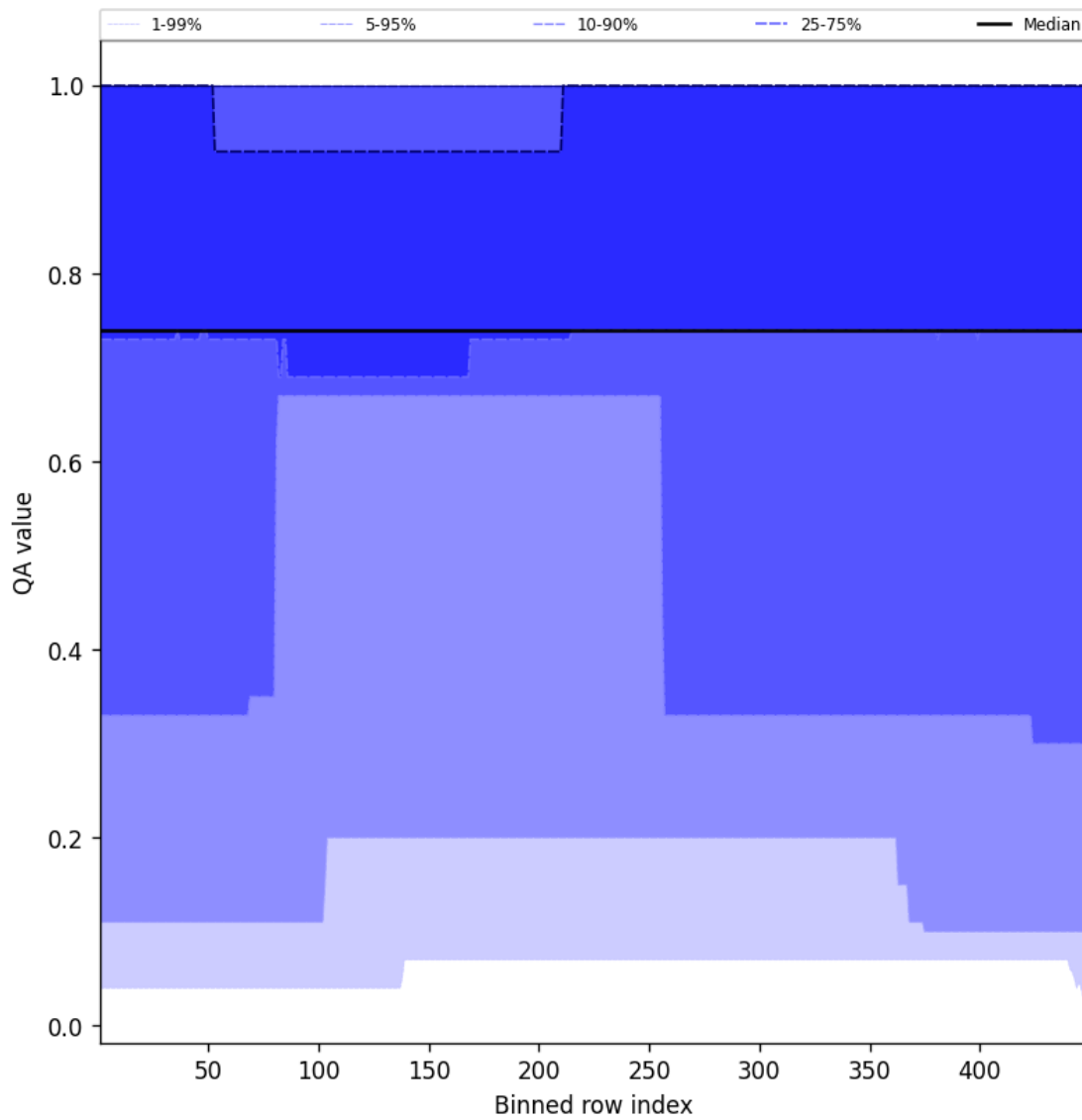
Figure 45: Along track statistics of “QA value” for 2025-11-05 to 2025-11-07
