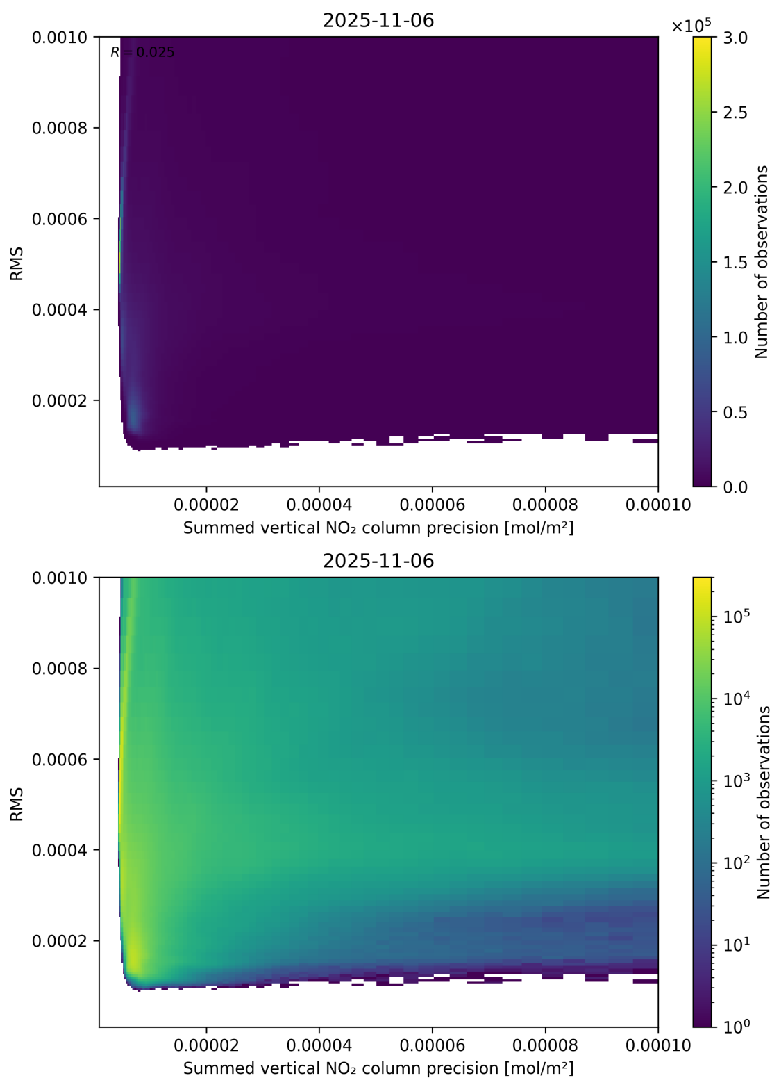
Figure 108: Scatter density plot of “Summed vertical NO 2 column precision” against “RMS” for 2025-11-05 to 2025-11-07.
