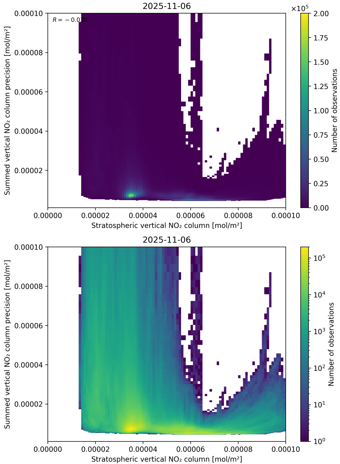
Figure 99: Scatter density plot of “Stratospheric vertical NO 2 column” against “Summed vertical NO 2 column precision” for 2025-11-05 to 2025-11-07.
