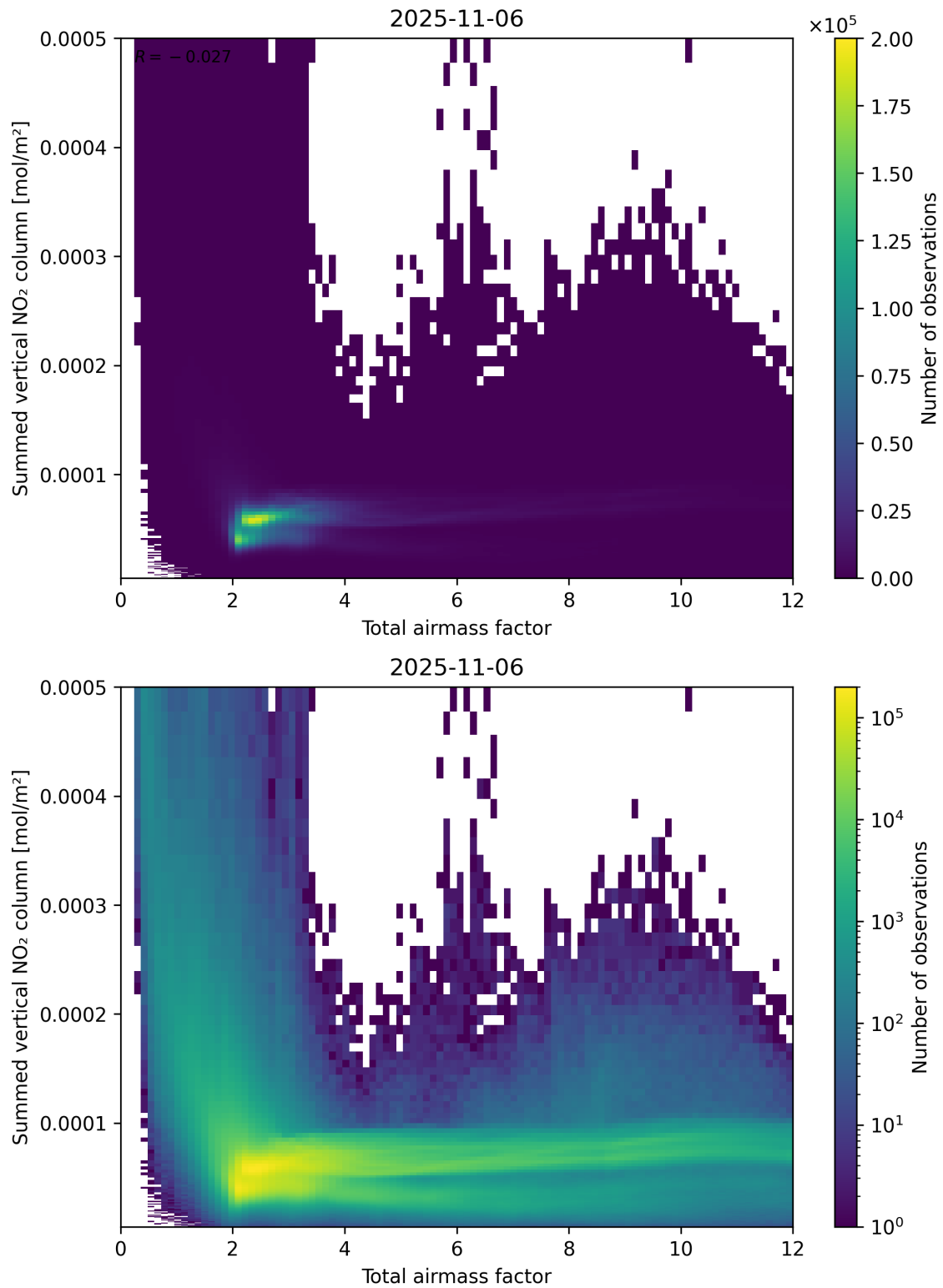
Figure 65: Scatter density plot of “Total airmass factor” against “Summed vertical NO 2 column” for 2025-11-05 to 2025-11-07.
