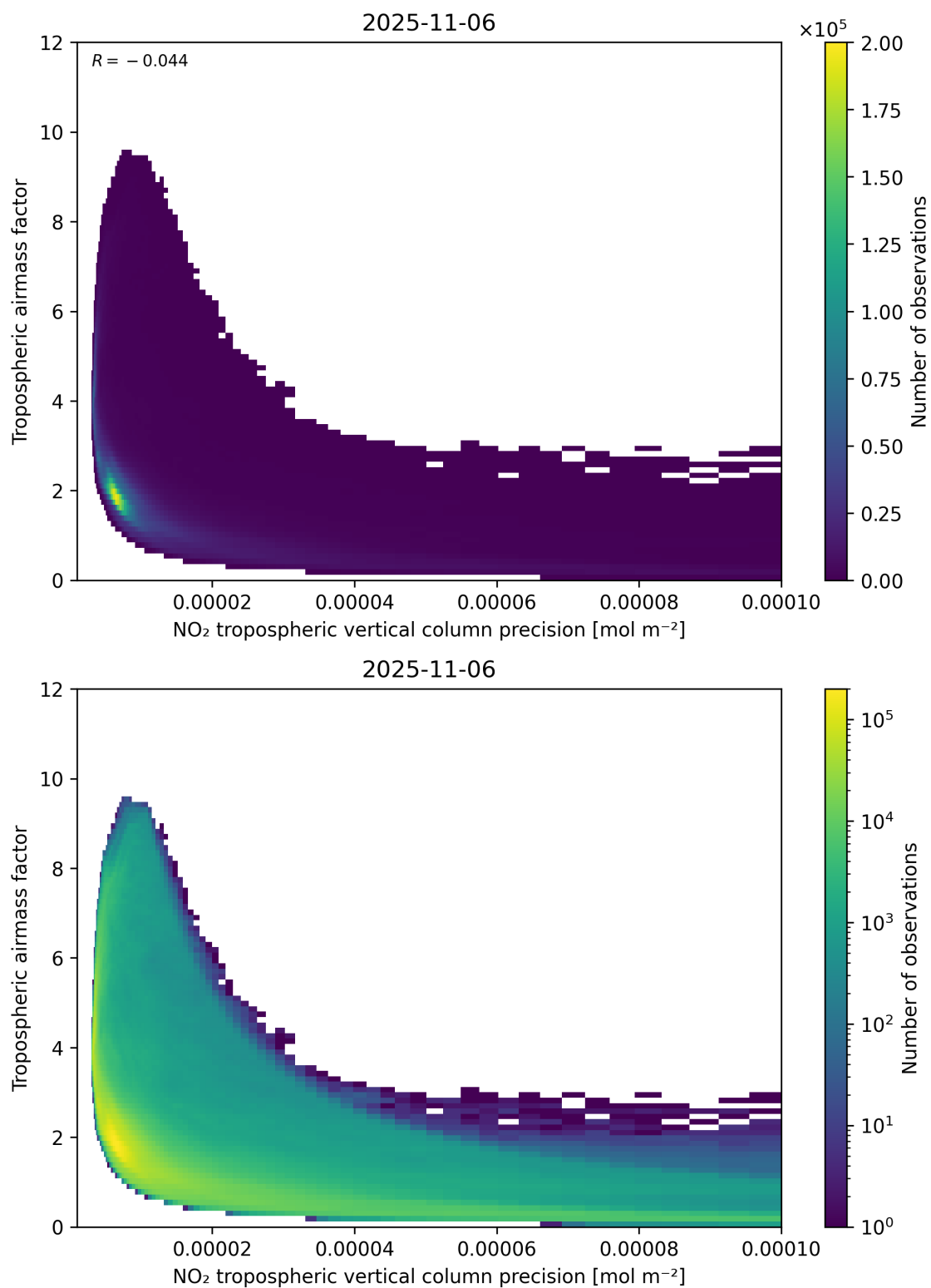
Figure 133: Scatter density plot of “NO 2 tropospheric vertical column precision” against “Tropospheric airmass factor” for 2025-11-05 to 2025-11-07.
