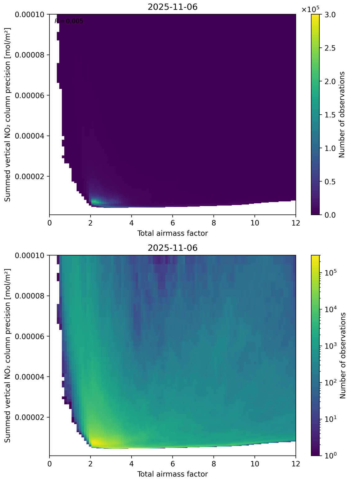
Figure 66: Scatter density plot of “Total airmass factor” against “Summed vertical NO 2 column precision” for 2025-11-05 to 2025-11-07.
