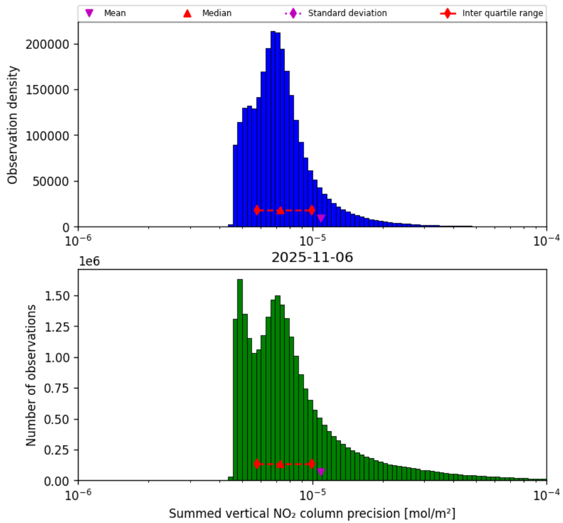
Figure 41: Histogram of “Summed vertical NO 2 column precision” for 2025-11-05 to 2025-11-07
