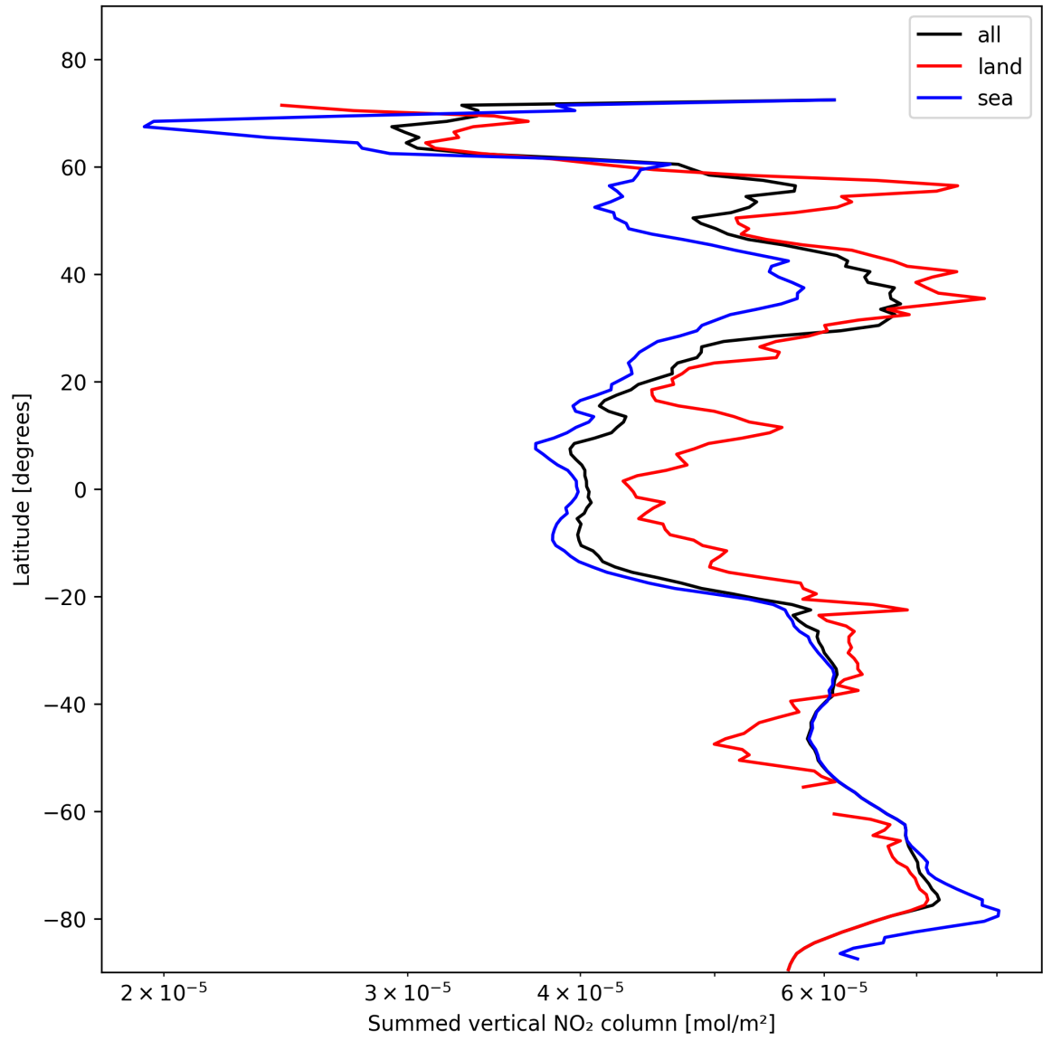
Figure 23: Zonal average of “Summed vertical NO 2 column” for 2025-11-05 to 2025-11-07.
