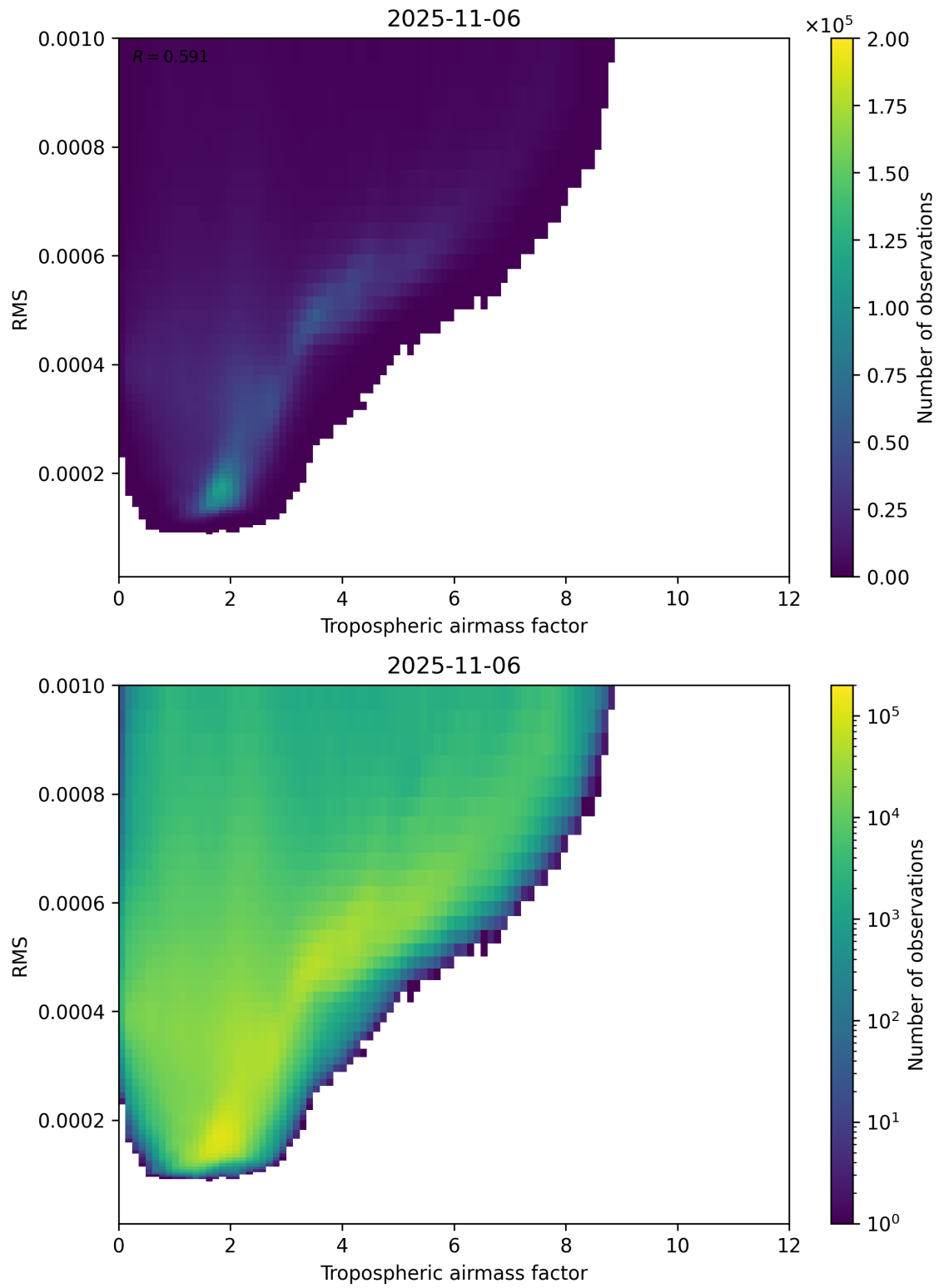
Figure 79: Scatter density plot of “Tropospheric airmass factor” against “RMS” for 2025-11-05 to 2025-11-07.
