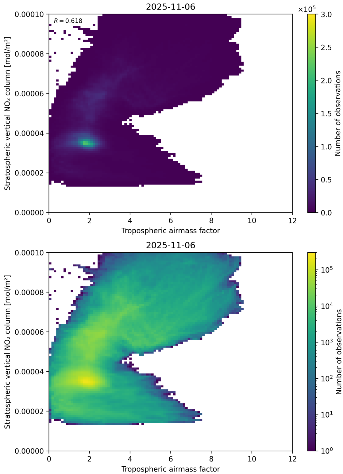
Figure 74: Scatter density plot of “Tropospheric air mass factor” against “Stratospheric vertical NO 2 column” for 2025-11-05 to 2025-11-07.
