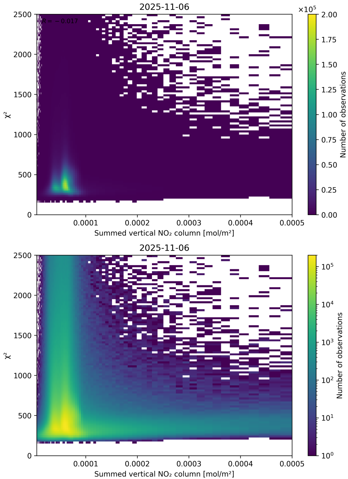
Figure 104: Scatter density plot of “Summed vertical NO 2 column” against “ \chi^2 ” for 2025-11-05 to 2025-11-07.
