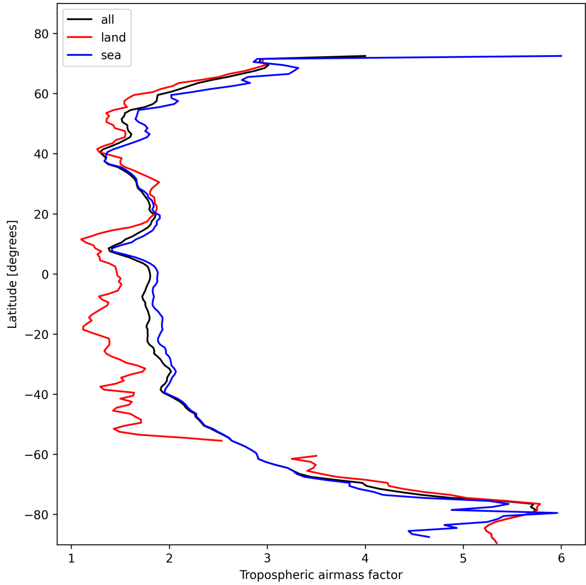
Figure 14: Zonal average of “Tropospheric airmass factor” for 2025-11-05 to 2025-11-07.
