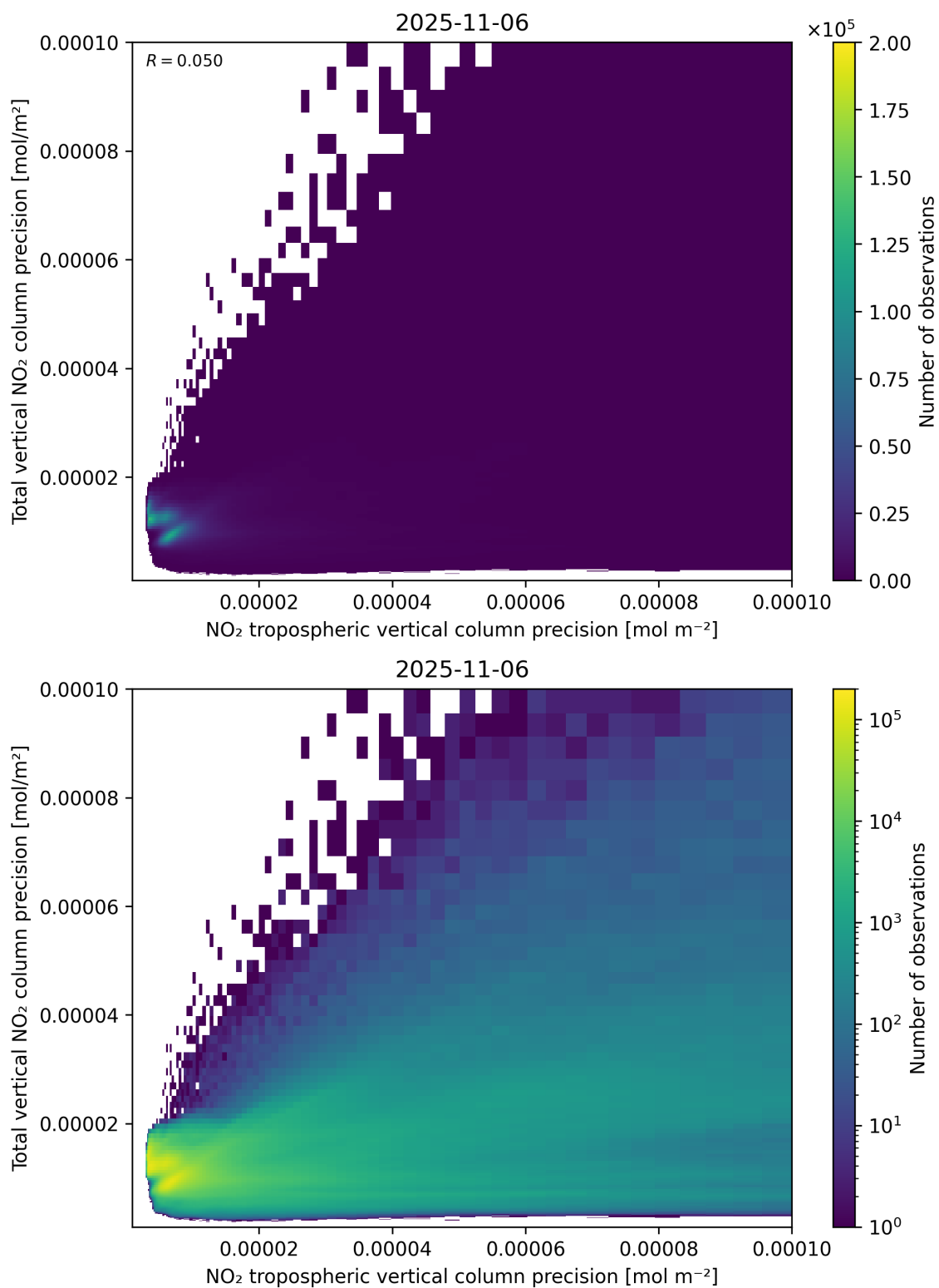
Figure 139: Scatter density plot of “NO 2 tropospheric vertical column precision” against “Total vertical NO 2 column precision” for 2025-11-05 to 2025-11-07.
