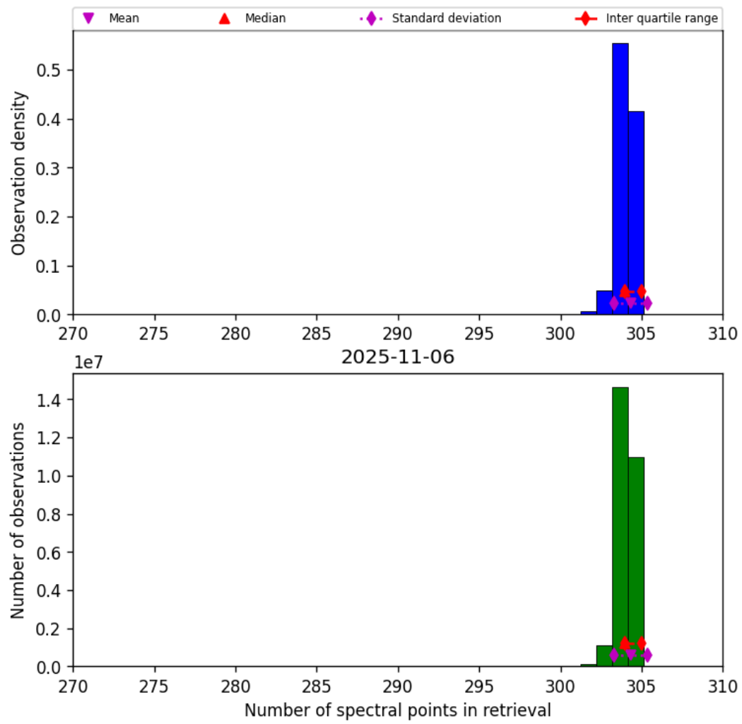
Figure 33: Histogram of “Number of spectral points in retrieval” for 2025-11-05 to 2025-11-07
