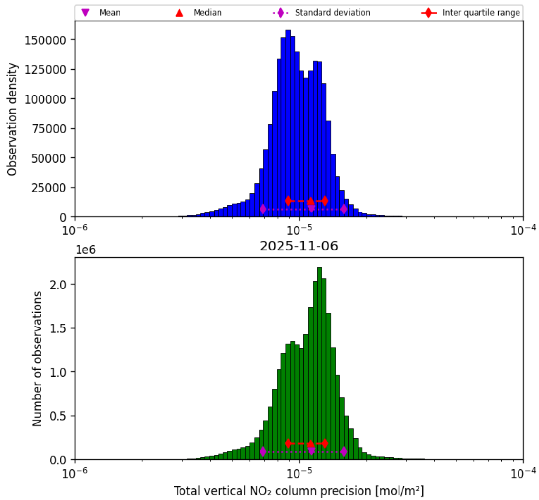
Figure 39: Histogram of "Total vertical NO 2 column precision" for 2025-11-05 to 2025-11-07
