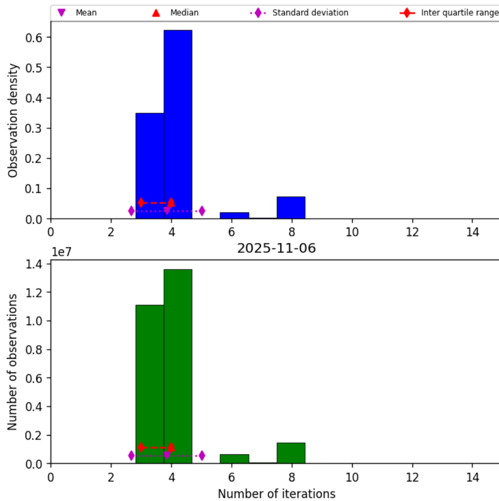
Figure 34: Histogram of "Number of iterations" for 2025-11-05 to 2025-11-07
