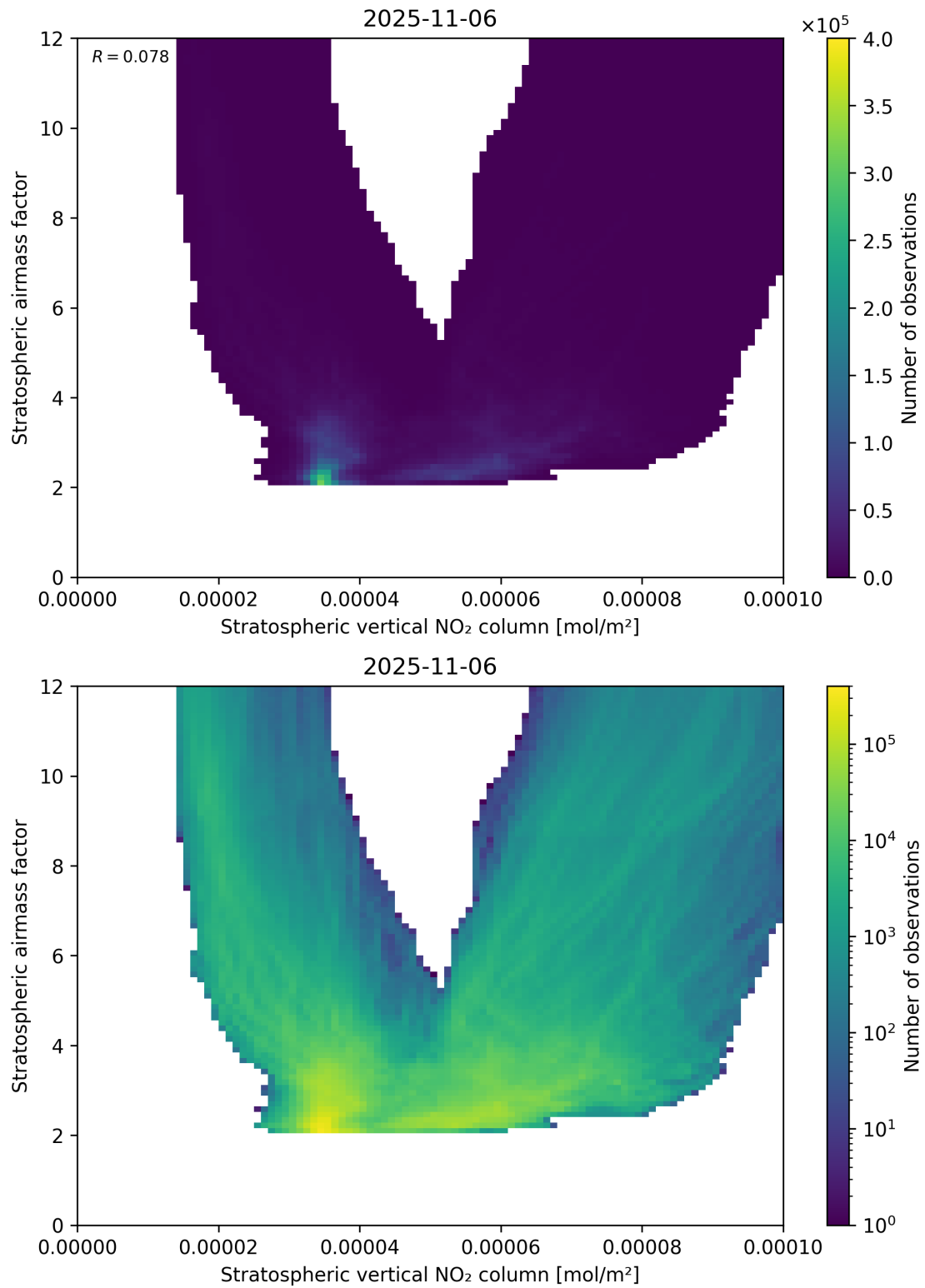
Figure 96: Scatter density plot of “Stratospheric vertical NO 2 column” against “Stratospheric airmass factor” for 2025-11-05 to 2025-11-07.
