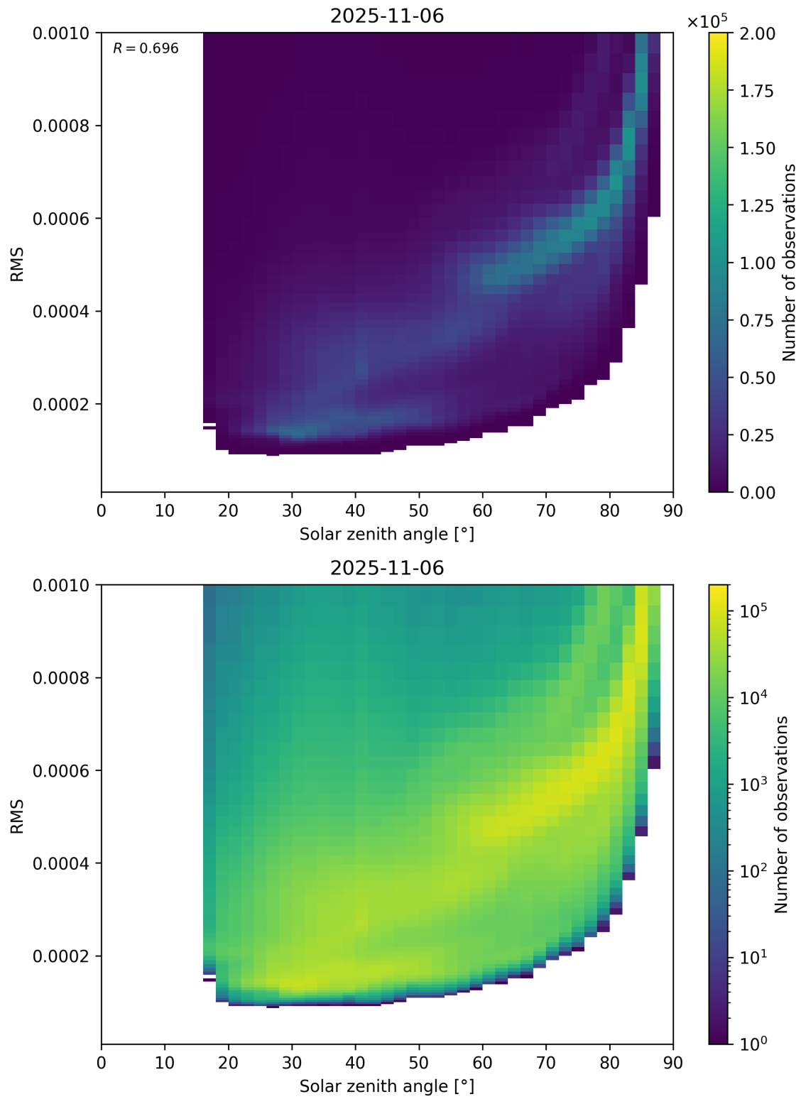
Figure 157: Scatter density plot of “Solar zenith angle” against “RMS” for 2025-11-05 to 2025-11-07.
