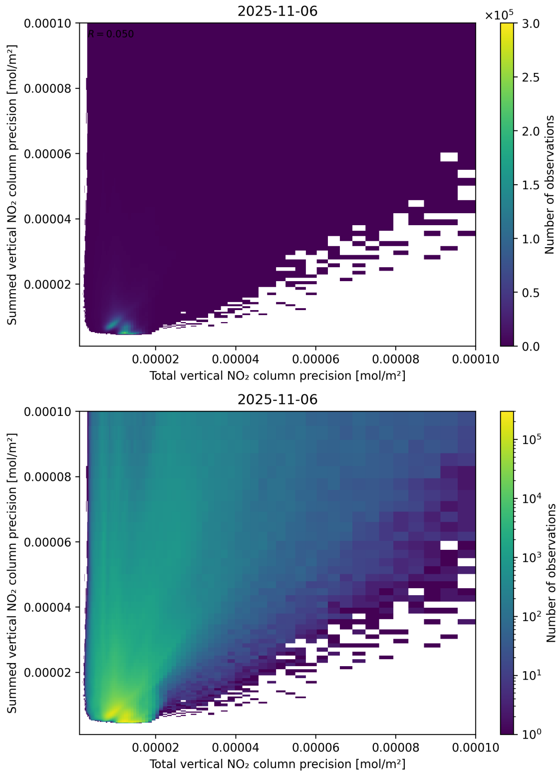
Figure 118: Scatter density plot of “Total vertical NO 2 column precision” against “Summed vertical NO 2 column precision” for 2025-11-05 to 2025-11-07.
