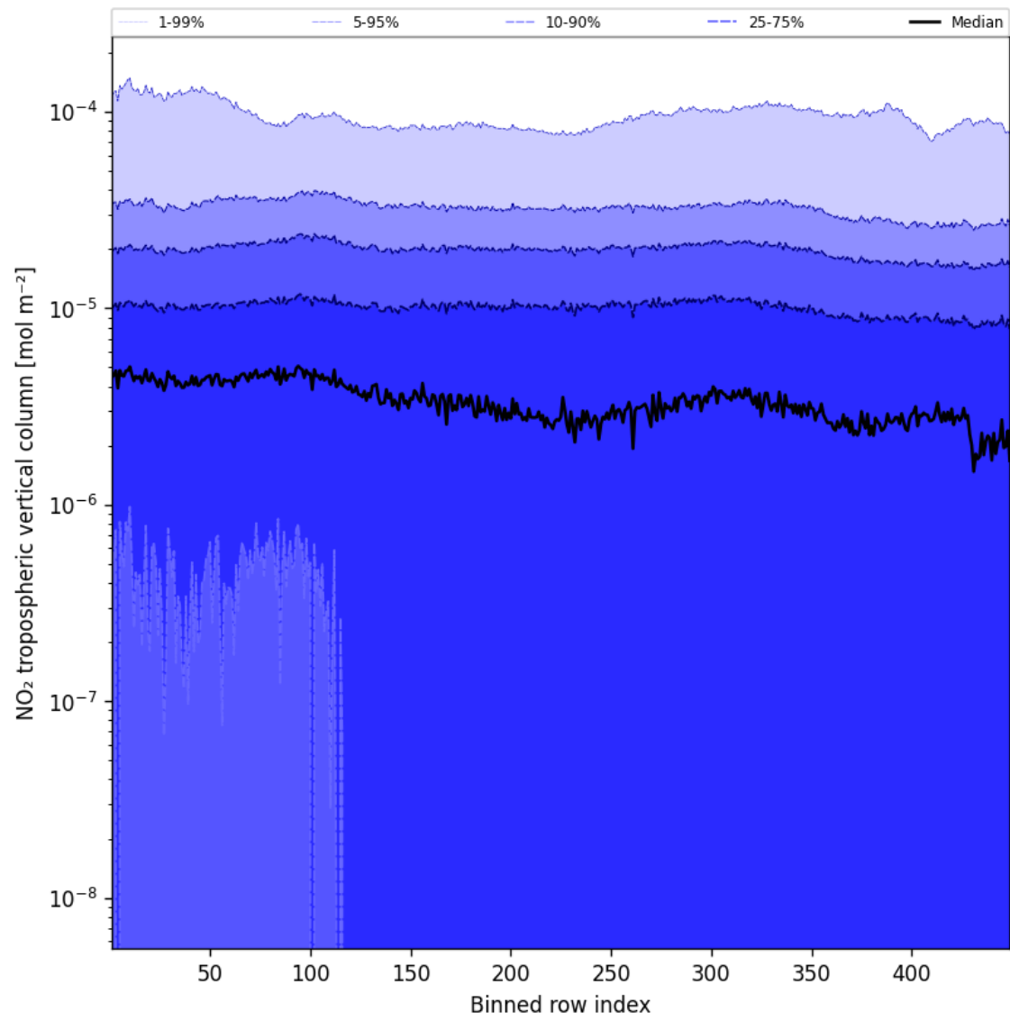
Figure 46: Along track statistics of “NO 2 tropospheric vertical column” for 2025-11-05 to 2025-11-07
