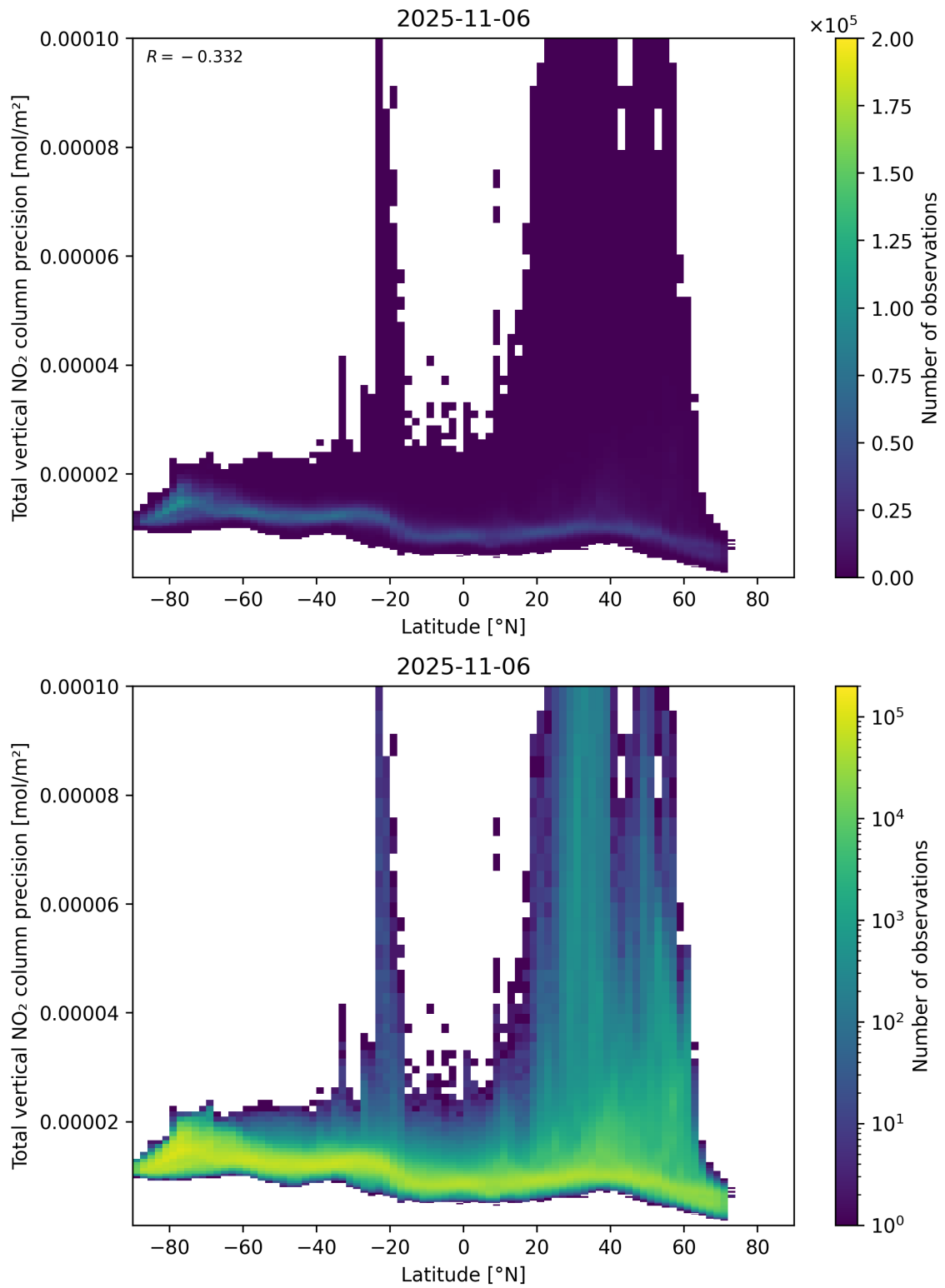
Figure 91: Scatter density plot of “Latitude” against “Total vertical NO 2 column precision” for 2025-11-05 to 2025-11-07.
