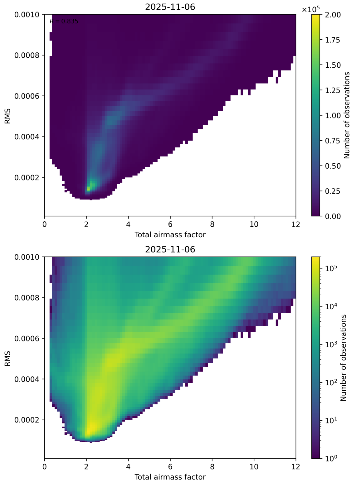
Figure 69: Scatter density plot of “Total airmass factor” against “RMS” for 2025-11-05 to 2025-11-07.
