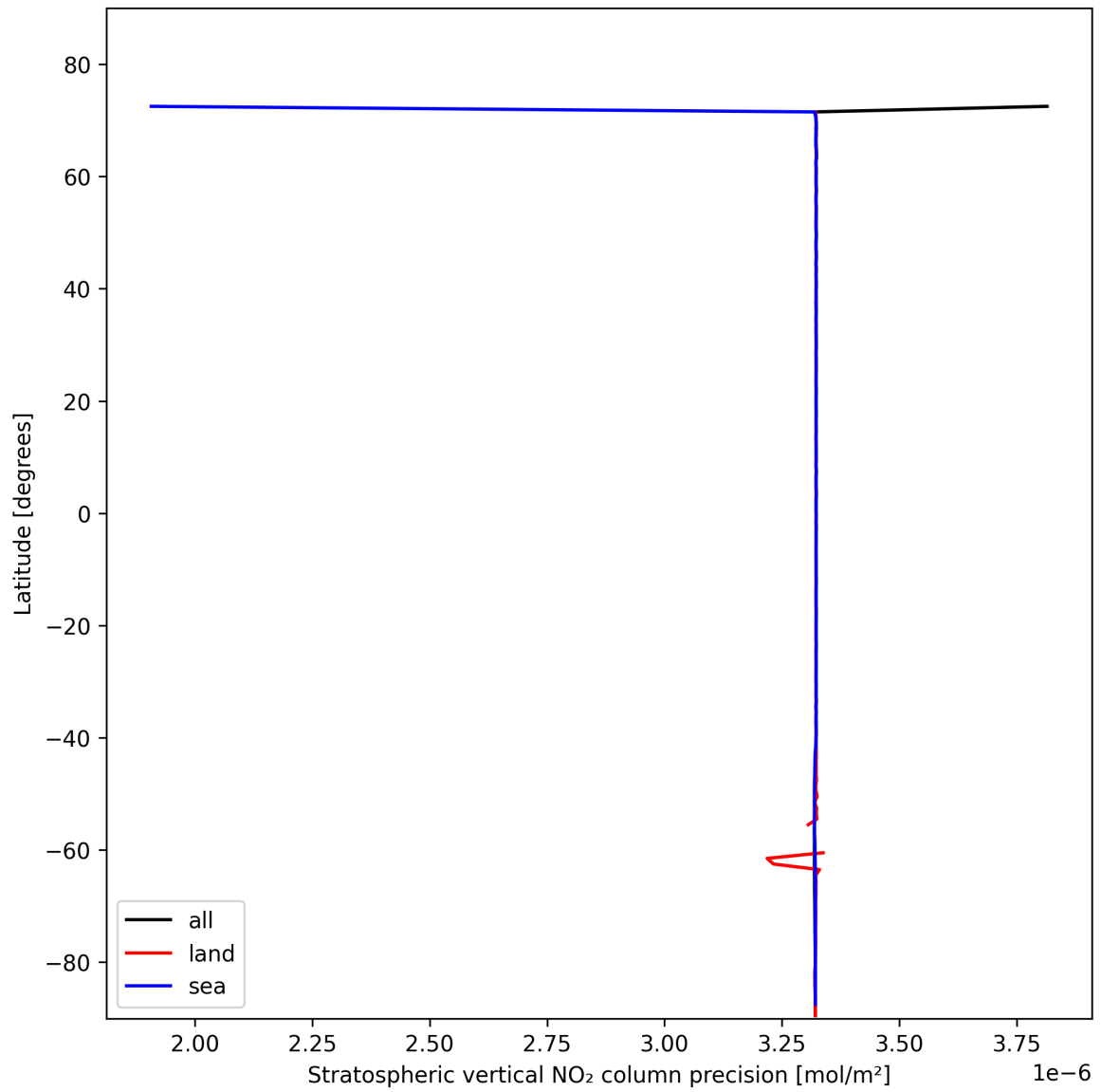
Figure 20: Zonal average of “Stratospheric vertical NO 2 column precision” for 2025-11-05 to 2025-11-07.
