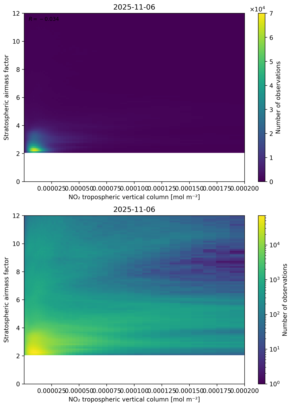
Figure 121: Scatter density plot of “NO 2 tropospheric vertical column” against “Stratospheric airmass factor” for 2025-11-05 to 2025-11-07.
