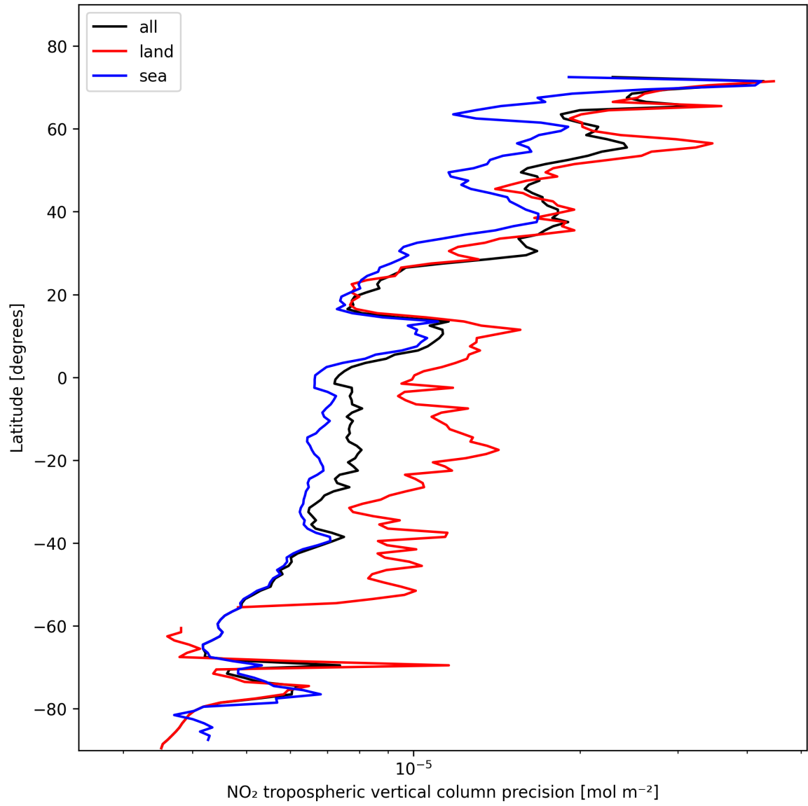
Figure 13: Zonal average of “NO 2 tropospheric vertical column precision” for 2025-11-05 to 2025-11-07.
