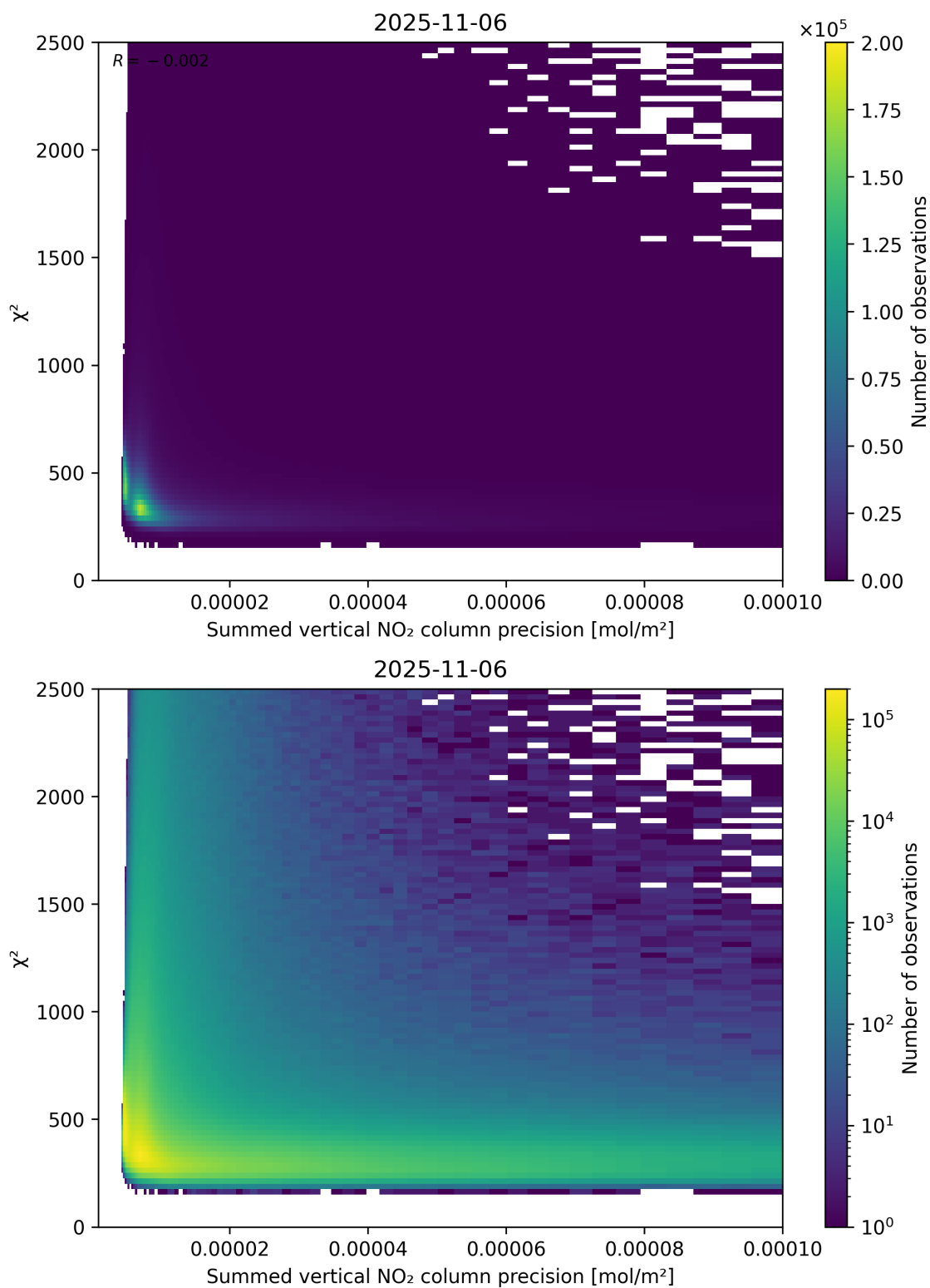
Figure 107: Scatter density plot of “Summed vertical NO 2 column precision” against “ \chi^2 ” for 2025-11-05 to 2025-11-07.
