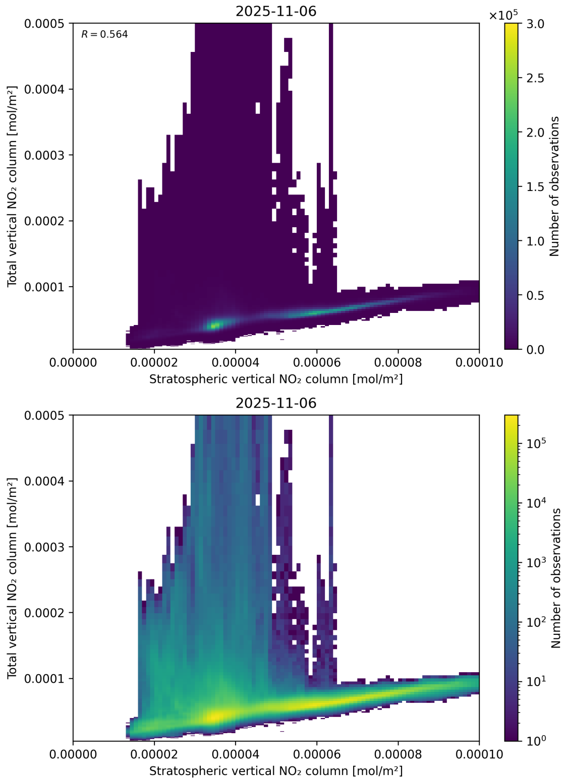
Figure 100: Scatter density plot of “Stratospheric vertical NO 2 column” against “Total vertical NO 2 column” for 2025-11-05 to 2025-11-07.
