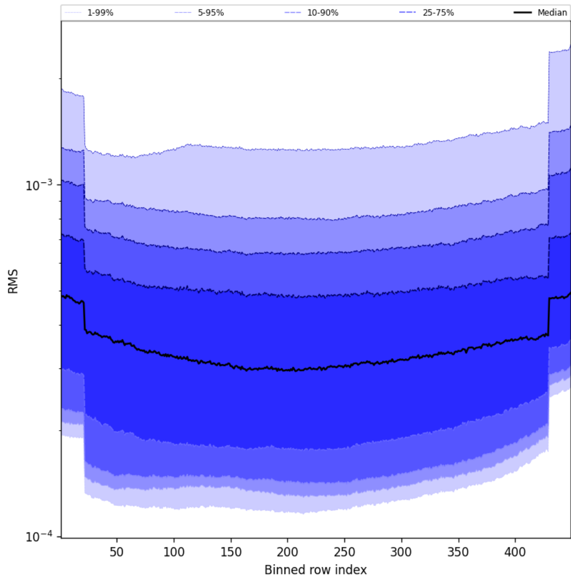
Figure 60: Along track statistics of “RMS” for 2025-11-05 to 2025-11-07
