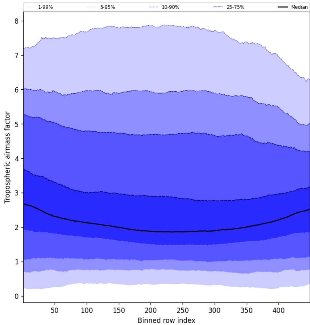
Figure 48: Along track statistics of “Tropospheric airmass factor” for 2025-11-05 to 2025-11-07
