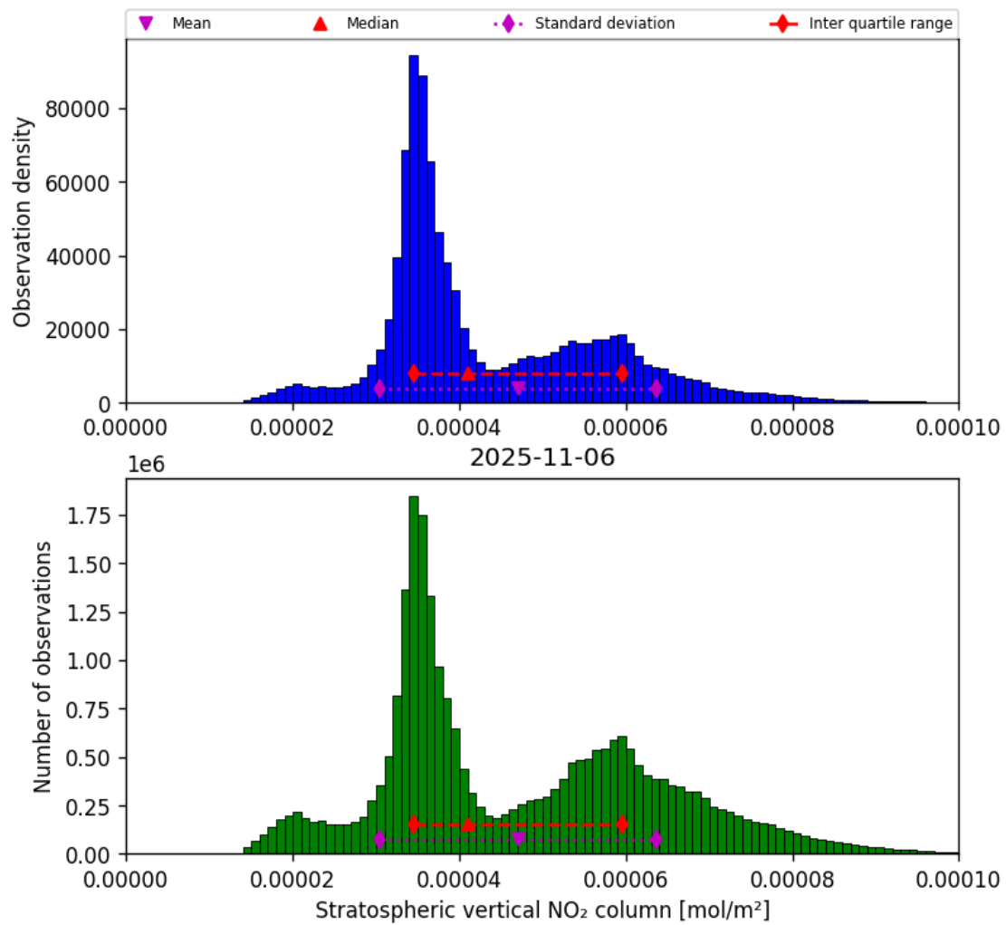
Figure 36: Histogram of “Stratospheric vertical NO 2 column” for 2025-11-05 to 2025-11-07
