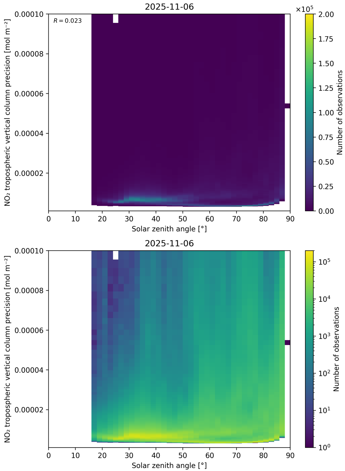
Figure 156: Scatter density plot of “Solar zenith angle” against “NO 2 tropospheric vertical column precision” for 2025-11-05 to 2025-11-07.
