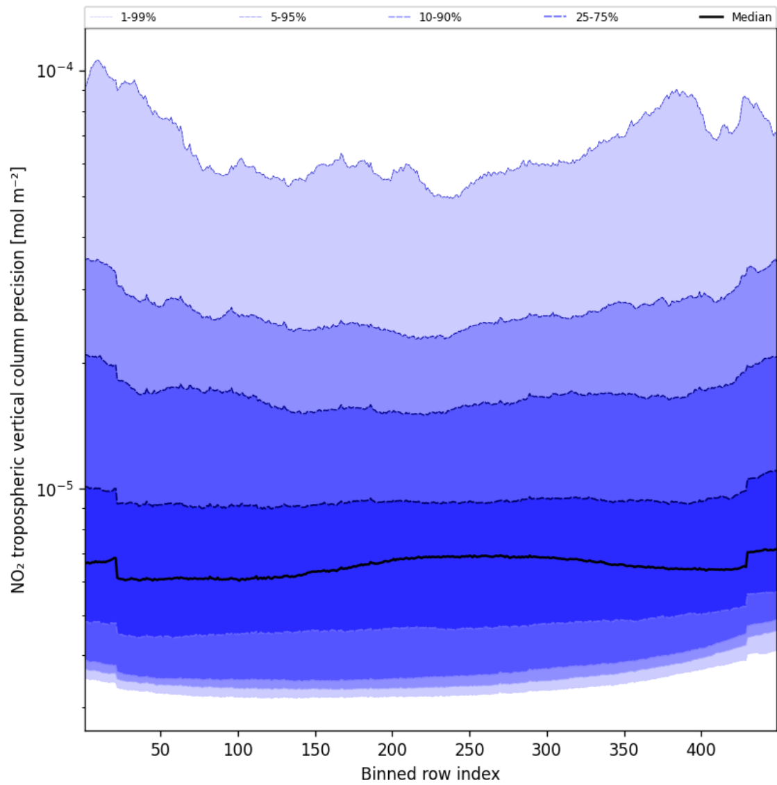
Figure 47: Along track statistics of “NO 2 tropospheric vertical column precision” for 2025-11-05 to 2025-11-07
