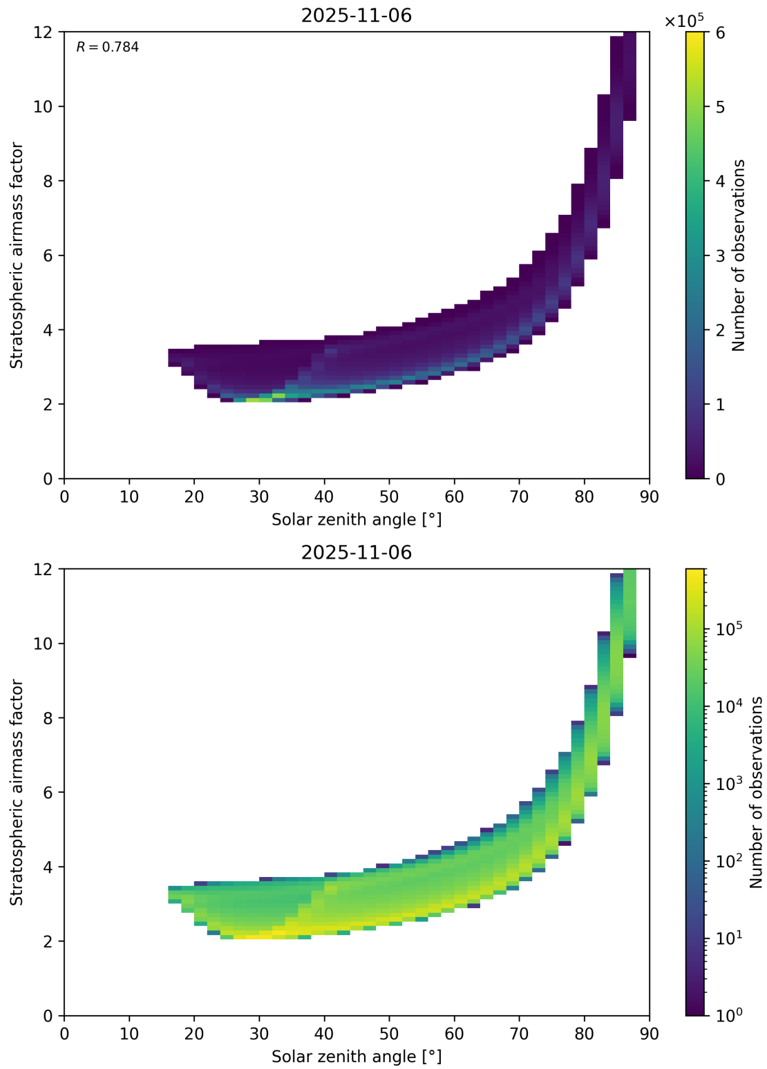
Figure 145: Scatter density plot of “Solar zenith angle” against “Stratospheric airmass factor” for 2025-11-05 to 2025-11-07.
