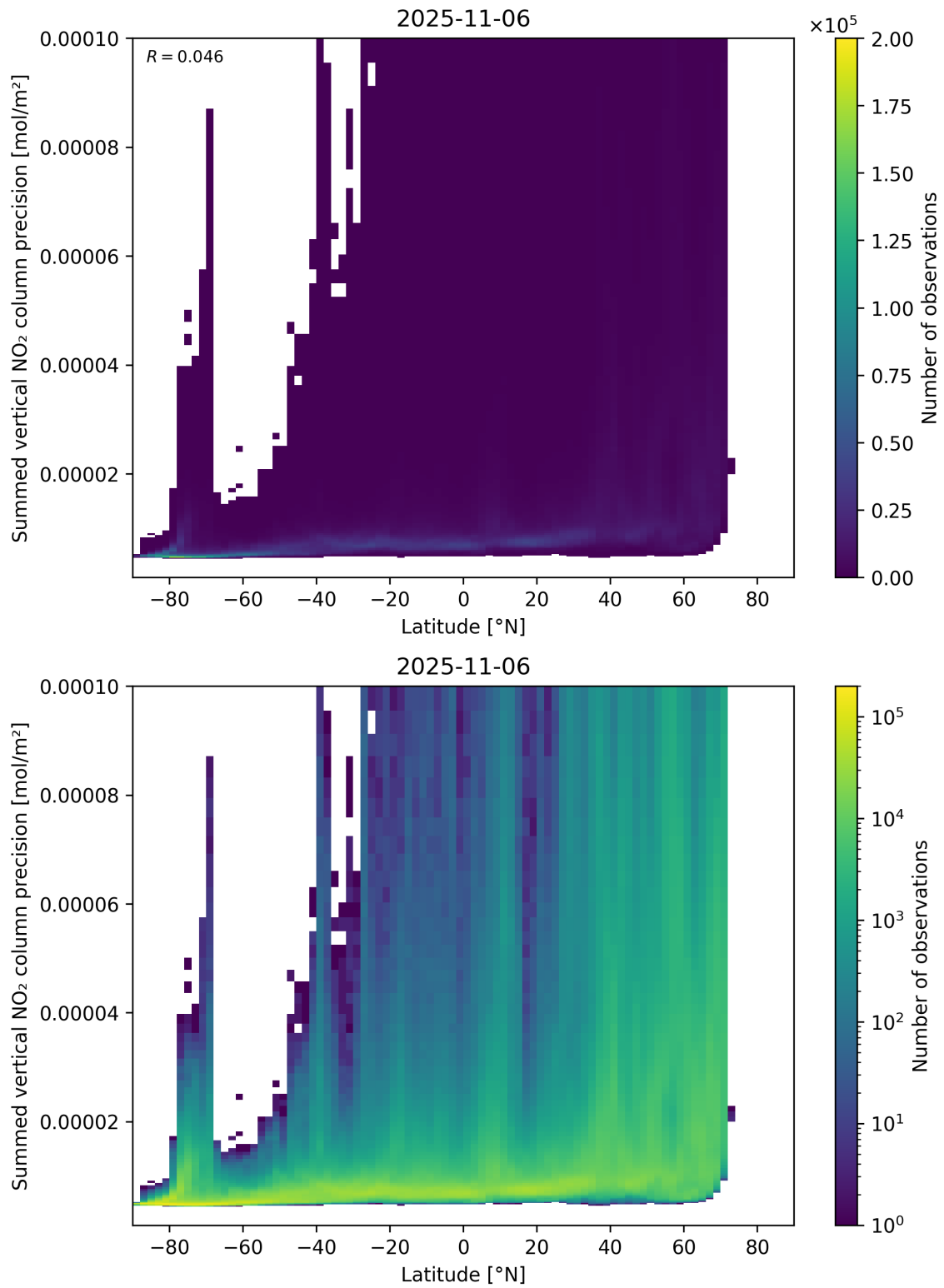
Figure 89: Scatter density plot of “Latitude” against “Summed vertical NO 2 column precision” for 2025-11-05 to 2025-11-07.
