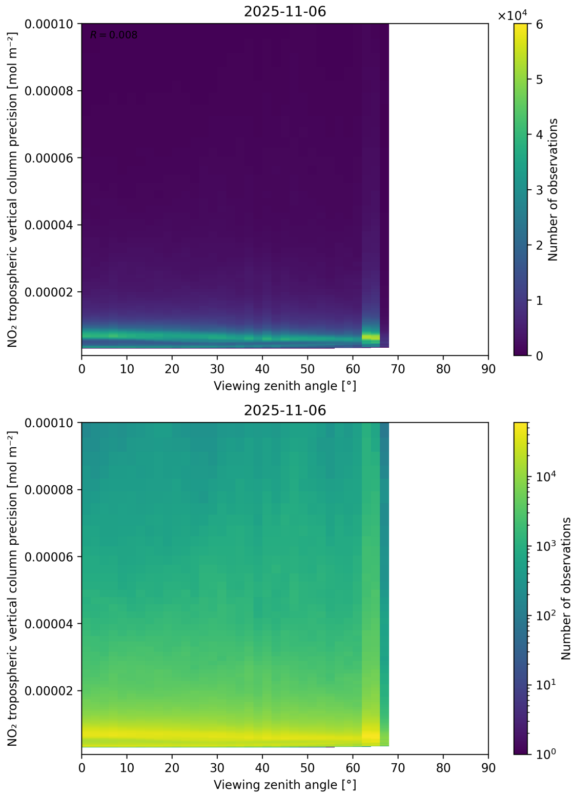
Figure 170: Scatter density plot of “Viewing zenith angle” against “NO 2 tropospheric vertical column precision” for 2025-11-05 to 2025-11-07.
