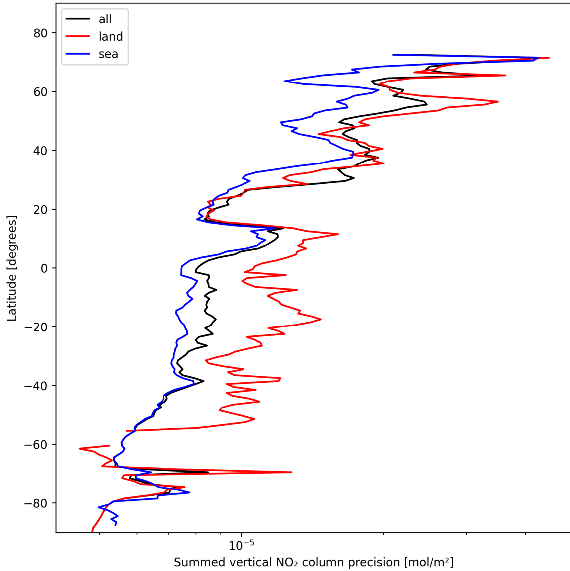
Figure 24: Zonal average of “Summed vertical NO 2 column precision” for 2025-11-05 to 2025-11-07.
