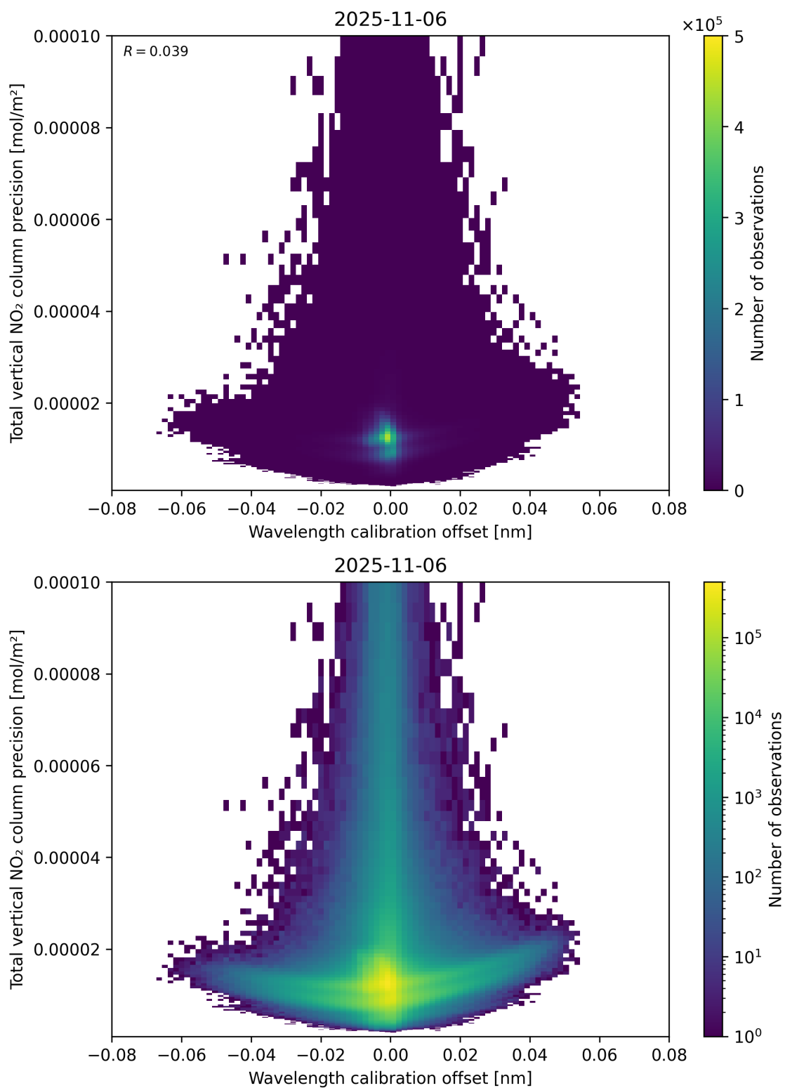
Figure 180: Scatter density plot of “Wavelength calibration offset” against “Total vertical NO 2 column precision” for 2025-11-05 to 2025-11-07.
