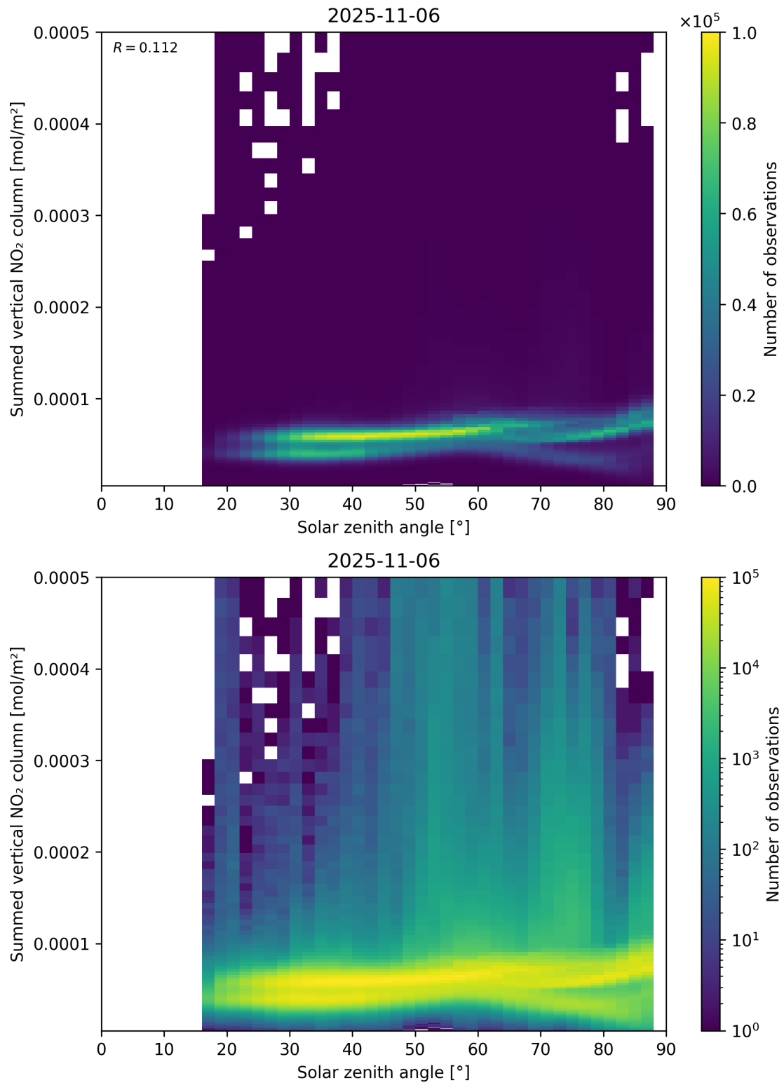
Figure 151: Scatter density plot of “Solar zenith angle” against “Summed vertical NO 2 column” for 2025-11-05 to 2025-11-07.
