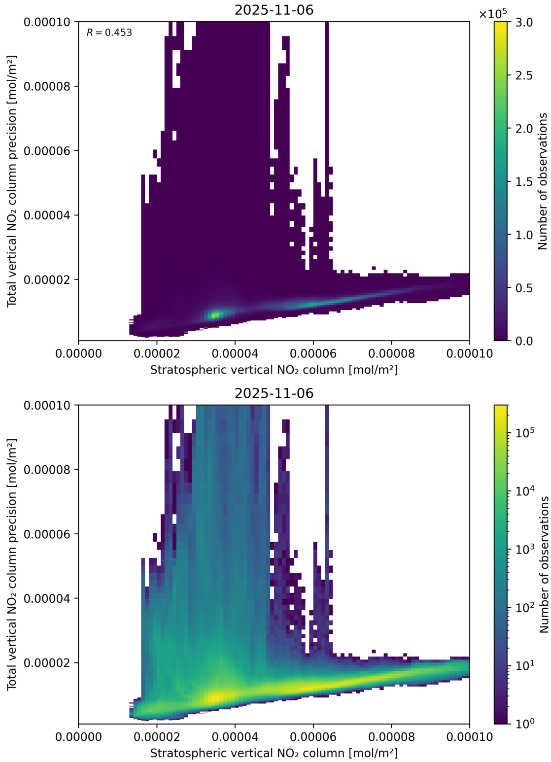
Figure 101: Scatter density plot of “Stratospheric vertical NO 2 column” against “Total vertical NO 2 column precision” for 2025-11-05 to 2025-11-07.
