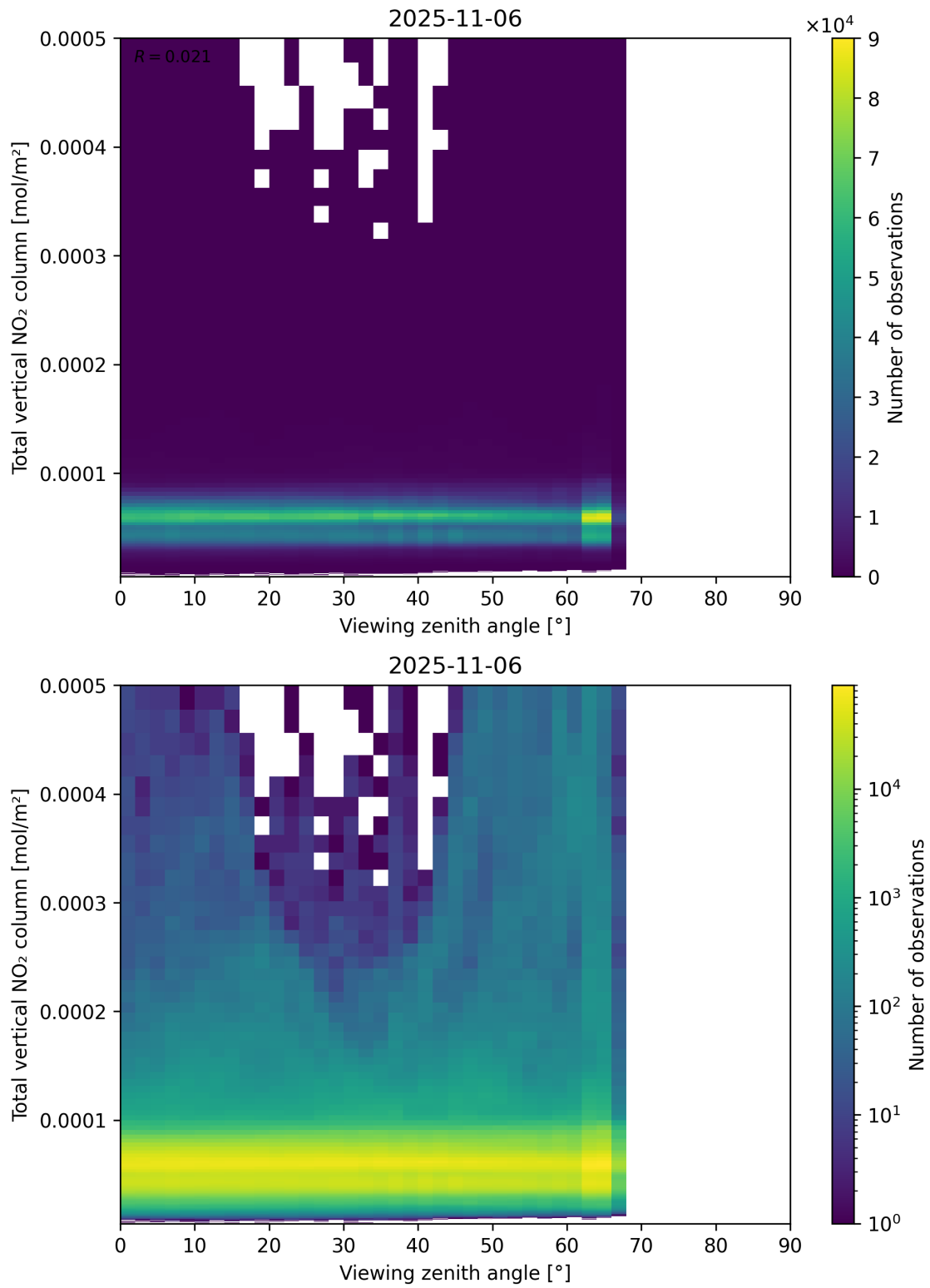
Figure 167: Scatter density plot of “Viewing zenith angle” against “Total vertical NO 2 column” for 2025-11-05 to 2025-11-07.
