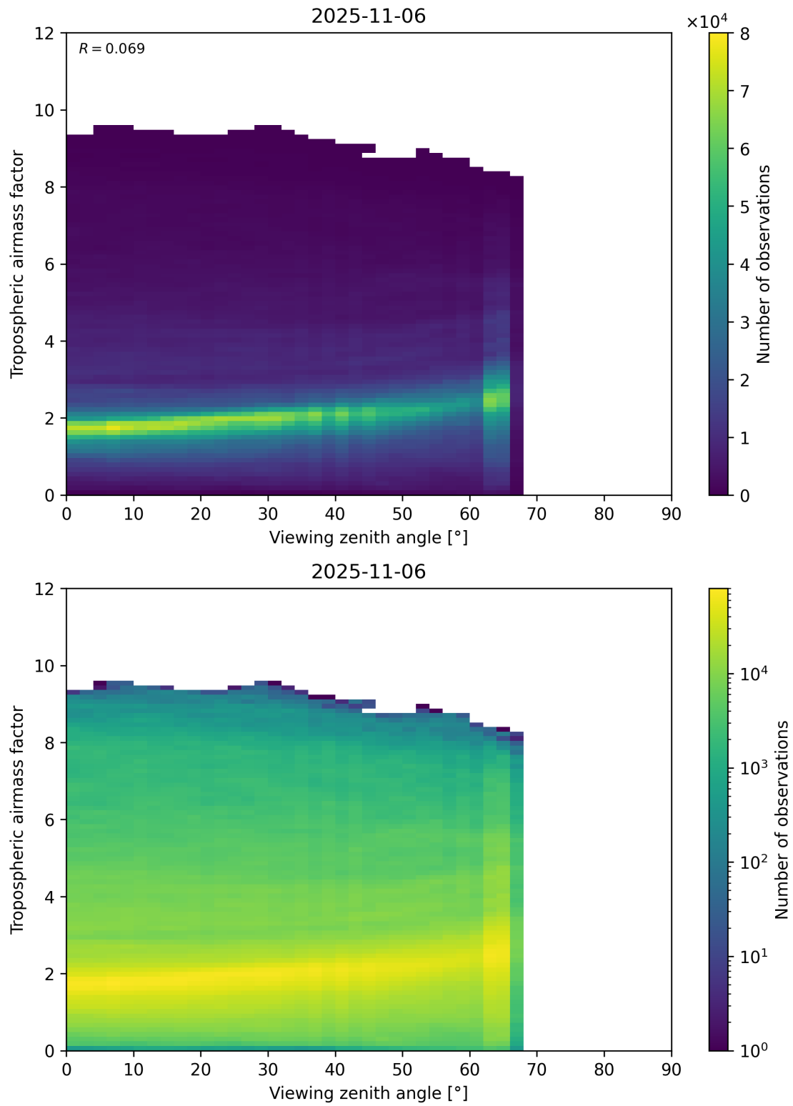
Figure 161: Scatter density plot of “Viewing zenith angle” against “Tropospheric airmass factor” for 2025-11-05 to 2025-11-07.
