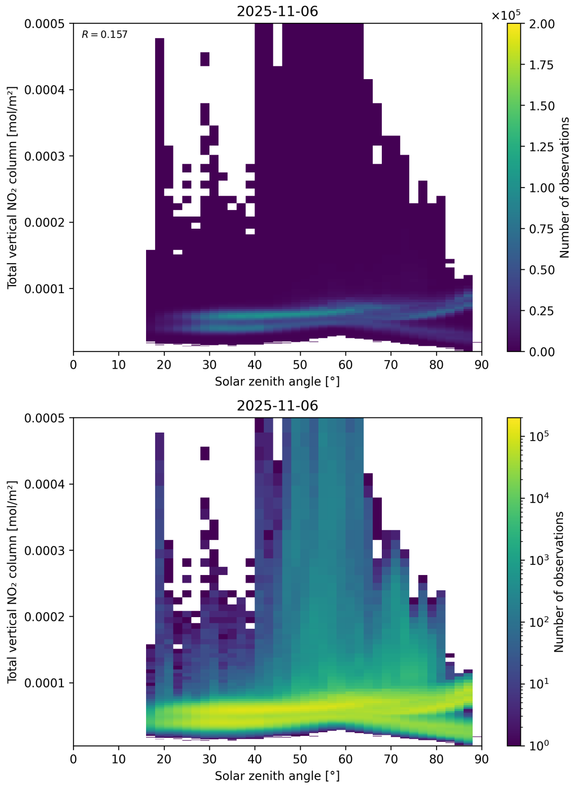
Figure 153: Scatter density plot of “Solar zenith angle” against “Total vertical NO 2 column” for 2025-11-05 to 2025-11-07.
