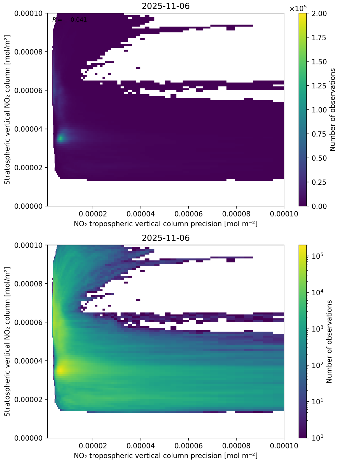
Figure 135: Scatter density plot of “NO 2 tropospheric vertical column precision” against “Stratospheric vertical NO 2 column” for 2025-11-05 to 2025-11-07.
