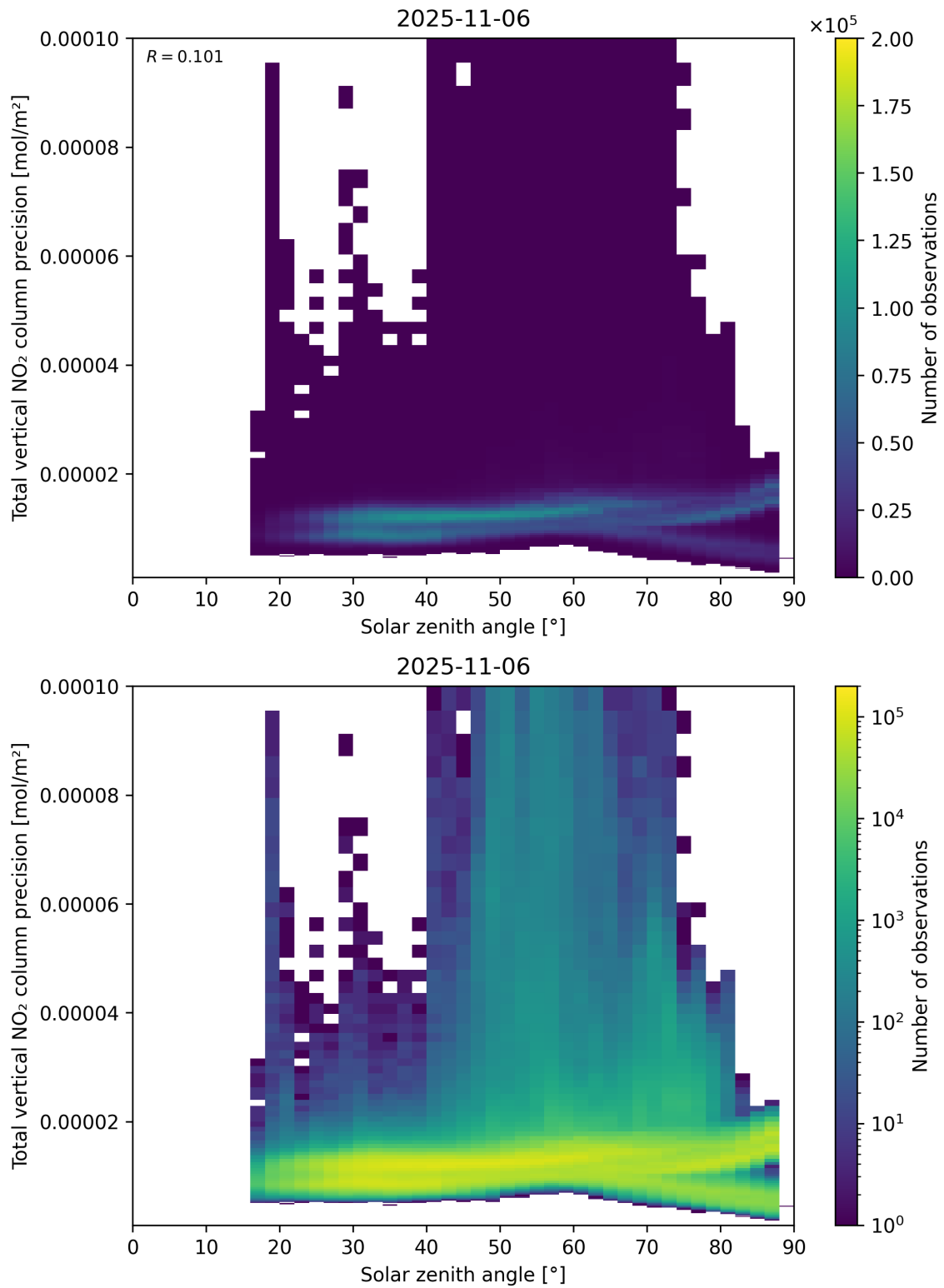
Figure 154: Scatter density plot of “Solar zenith angle” against “Total vertical NO 2 column precision” for 2025-11-05 to 2025-11-07.
