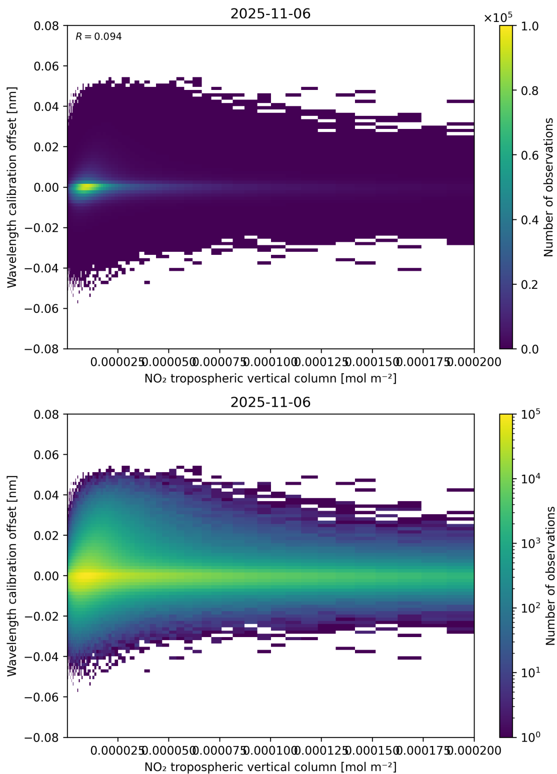
Figure 143: Scatter density plot of “NO 2 tropospheric vertical column” against “Wavelength calibration offset” for 2025-11-05 to 2025-11-07.
