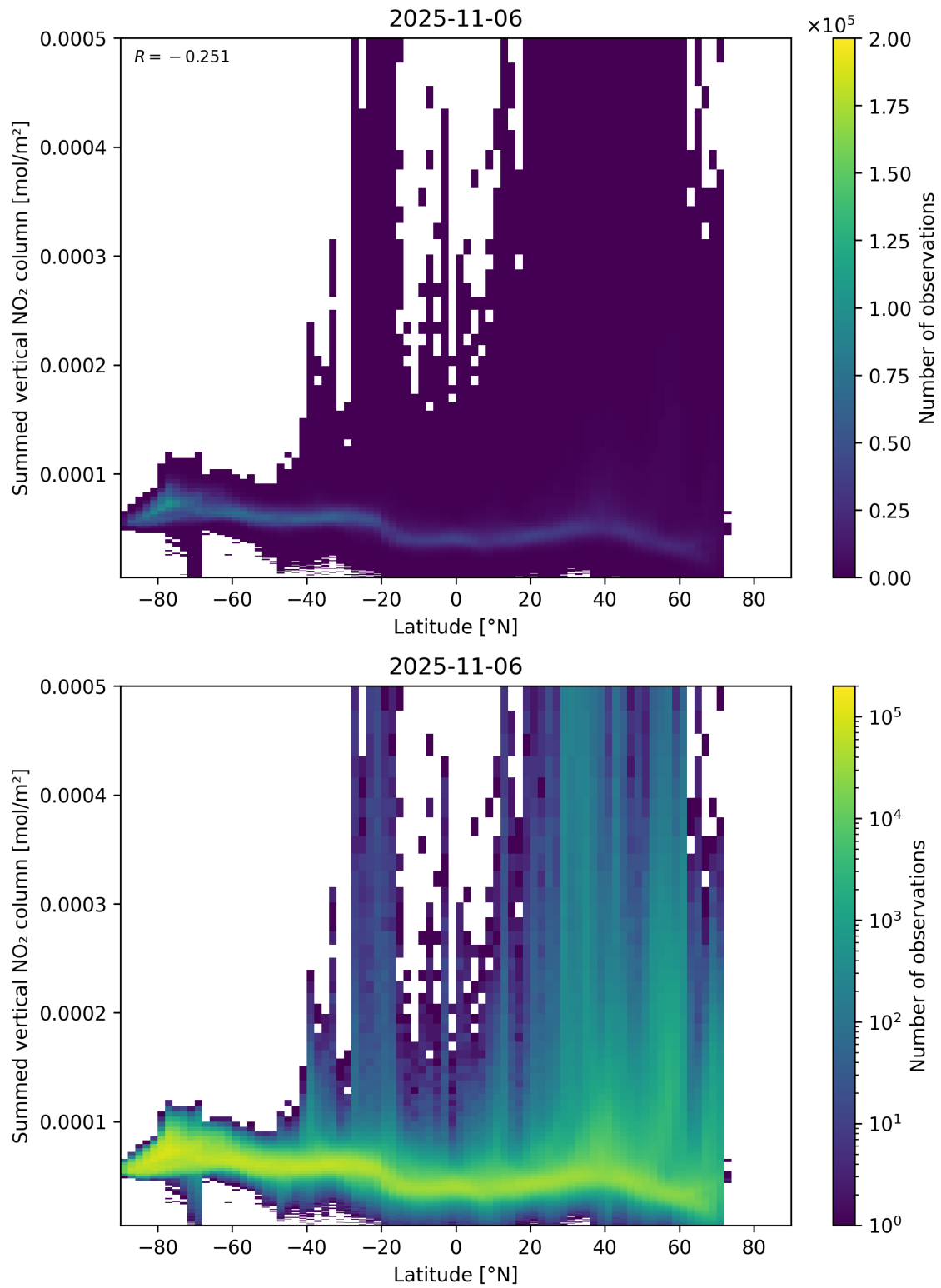
Figure 88: Scatter density plot of “Latitude” against “Summed vertical NO 2 column” for 2025-11-05 to 2025-11-07.
