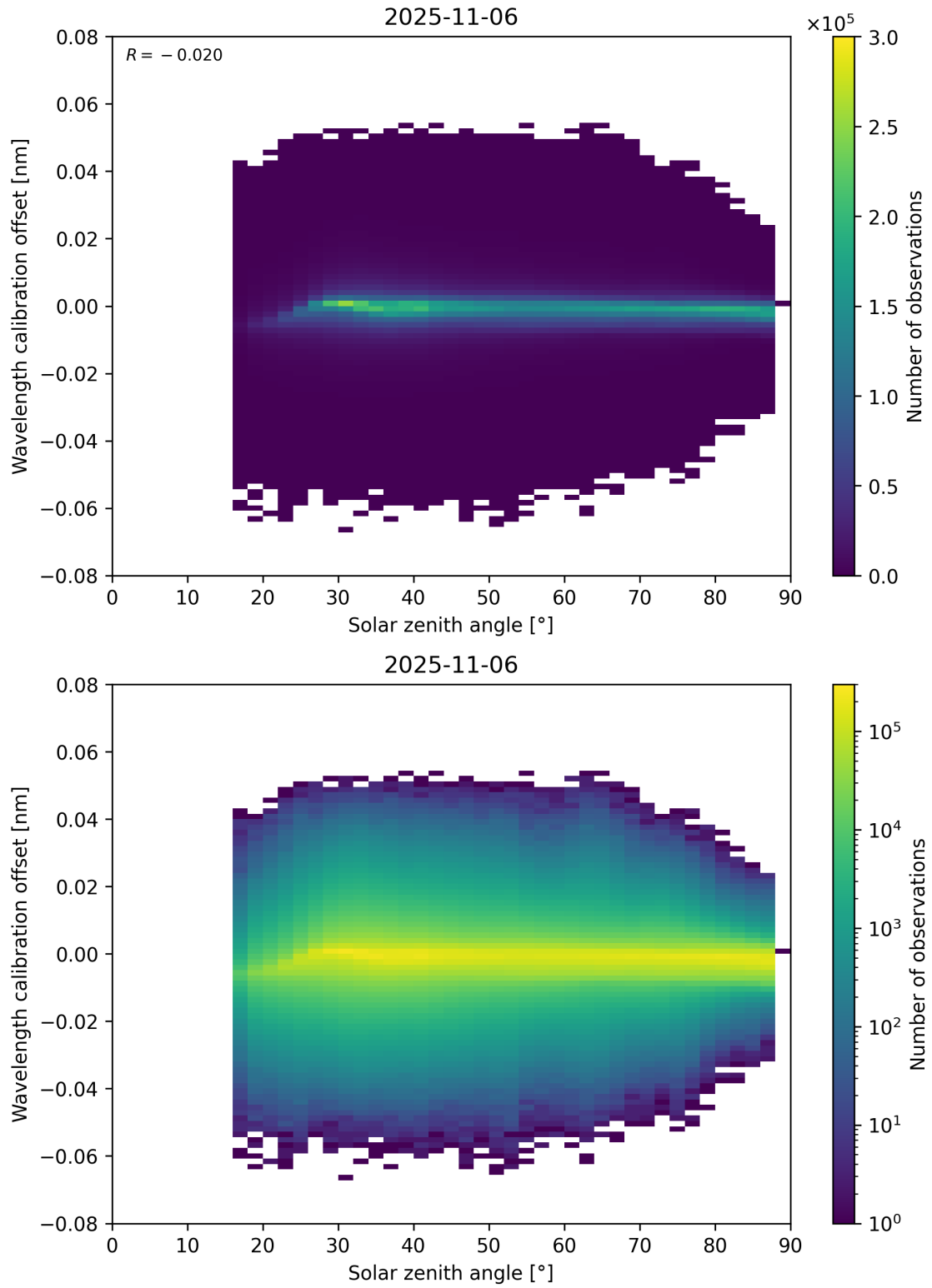
Figure 158: Scatter density plot of “Solar zenith angle” against “Wavelength calibration offset” for 2025-11-05 to 2025-11-07.
