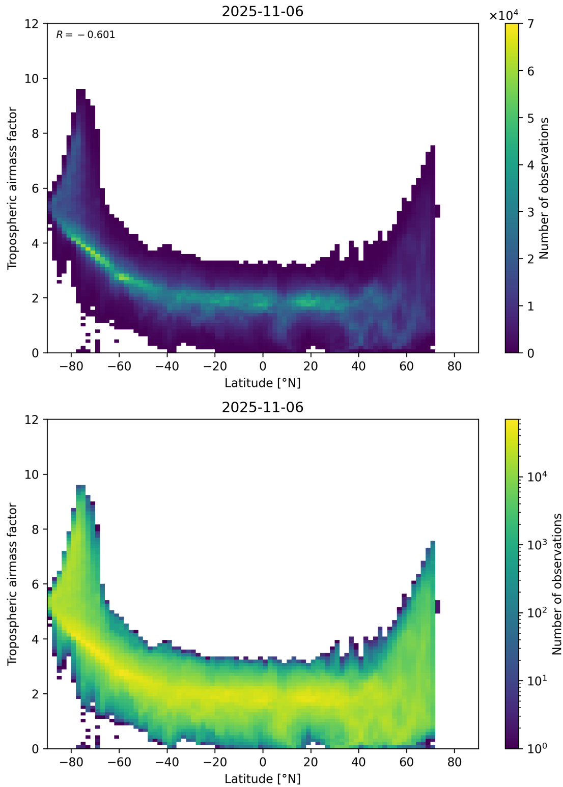
Figure 85: Scatter density plot of “Latitude” against “Tropospheric airmass factor” for 2025-11-05 to 2025-11-07.
