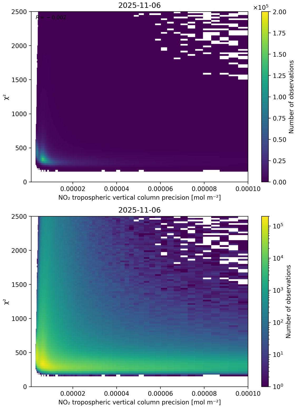
Figure 134: Scatter density plot of “NO 2 tropospheric vertical column precision” against “ \chi^2 ” for 2025-11-05 to 2025-11-07.
