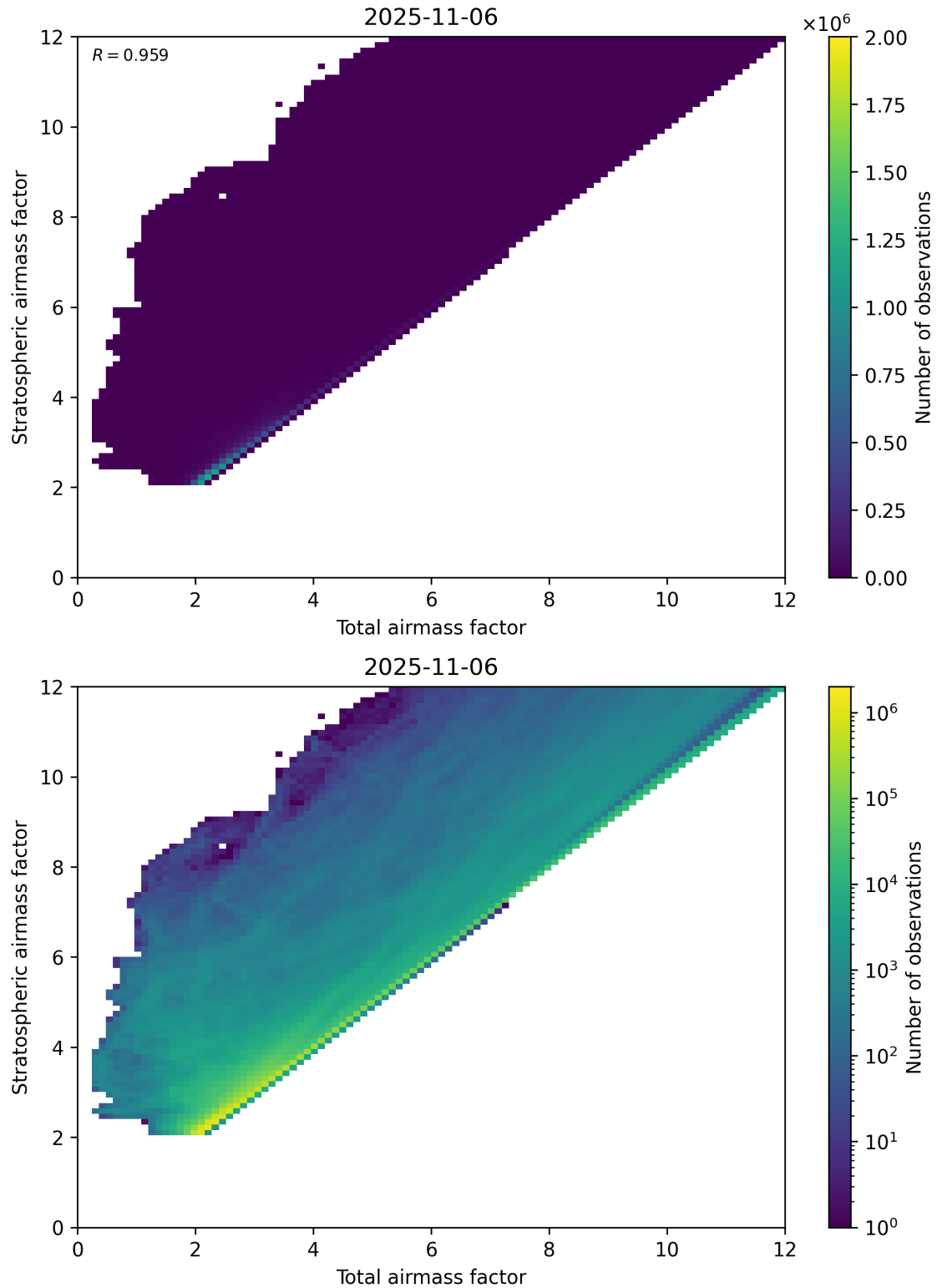
Figure 62: Scatter density plot of “Total airmass factor” against “Stratospheric airmass factor” for 2025-11-05 to 2025-11-07.
