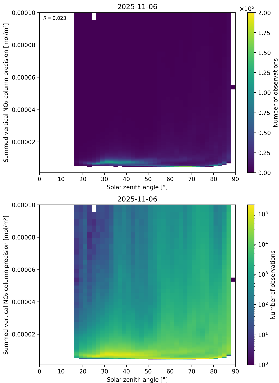
Figure 152: Scatter density plot of “Solar zenith angle” against “Summed vertical NO 2 column precision” for 2025-11-05 to 2025-11-07.
