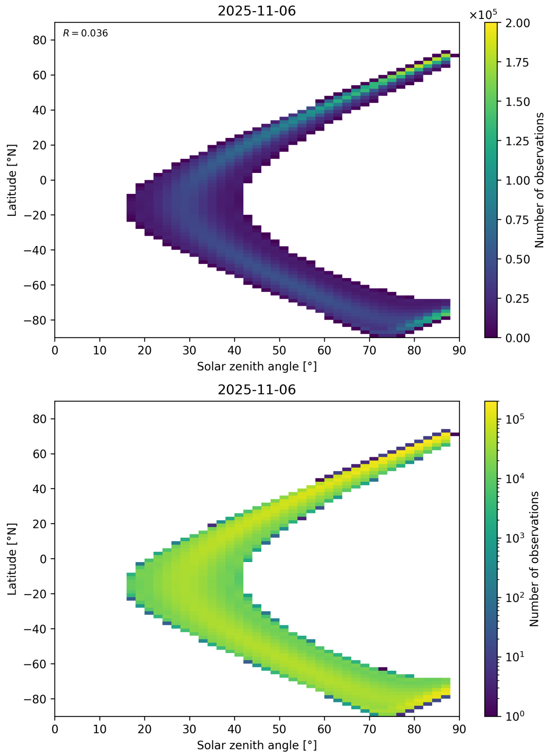
Figure 149: Scatter density plot of “Solar zenith angle” against “Latitude” for 2025-11-05 to 2025-11-07.
