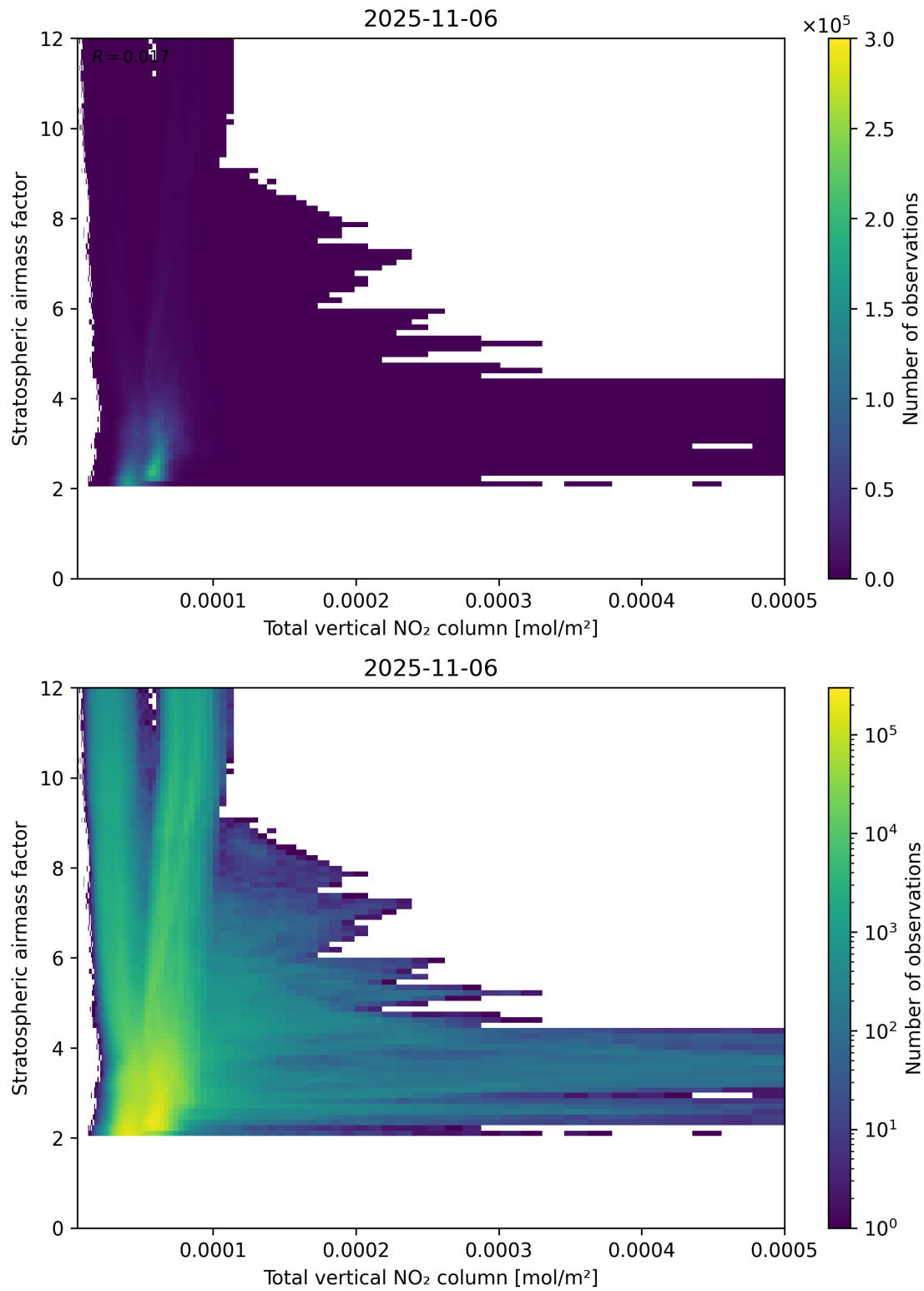
Figure 110: Scatter density plot of “Total vertical NO 2 column” against “Stratospheric airmass factor” for 2025-11-05 to 2025-11-07.
