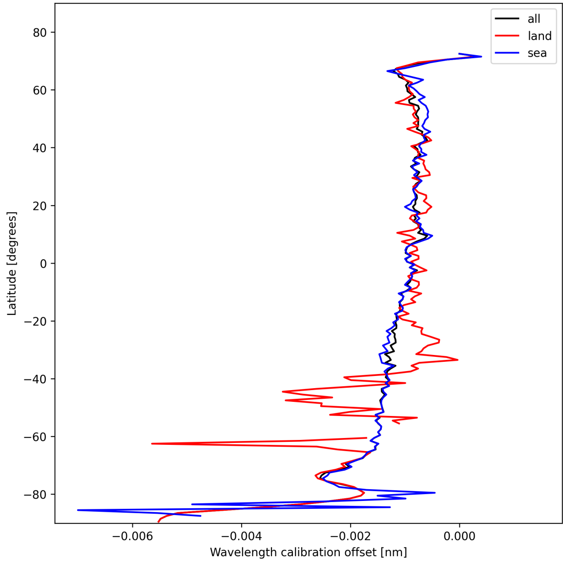
Figure 18: Zonal average of “Wavelength calibration offset” for 2025-11-05 to 2025-11-07.
