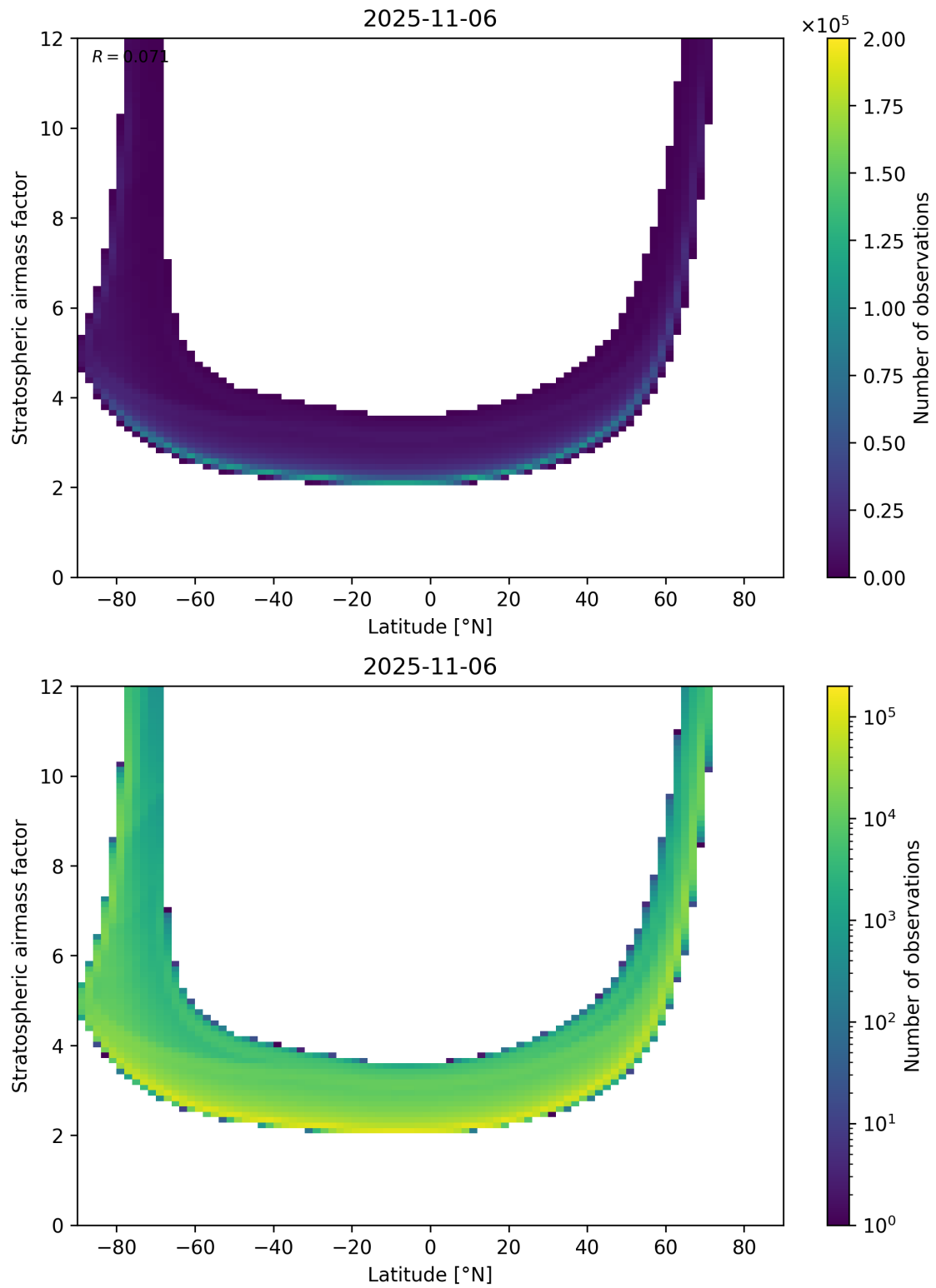
Figure 83: Scatter density plot of “Latitude” against “Stratospheric air mass factor” for 2025-11-05 to 2025-11-07.
