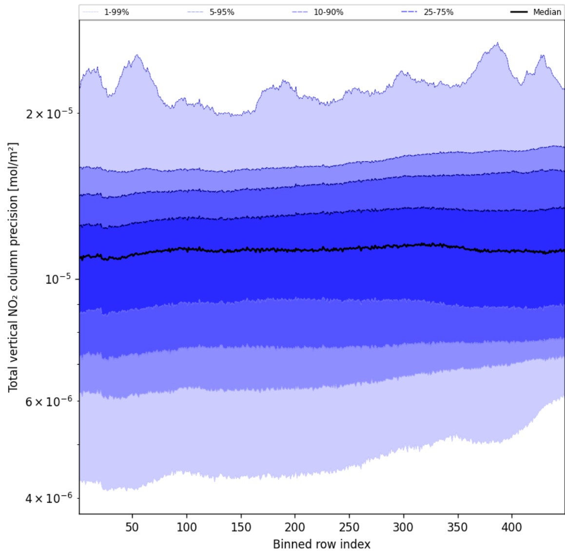
Figure 56: Along track statistics of "Total vertical NO 2 column precision" for 2025-11-05 to 2025-11-07
