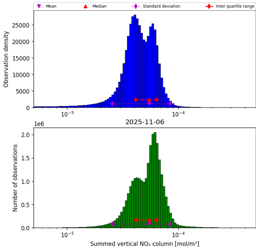
Figure 40: Histogram of “Summed vertical NO 2 column” for 2025-11-05 to 2025-11-07
