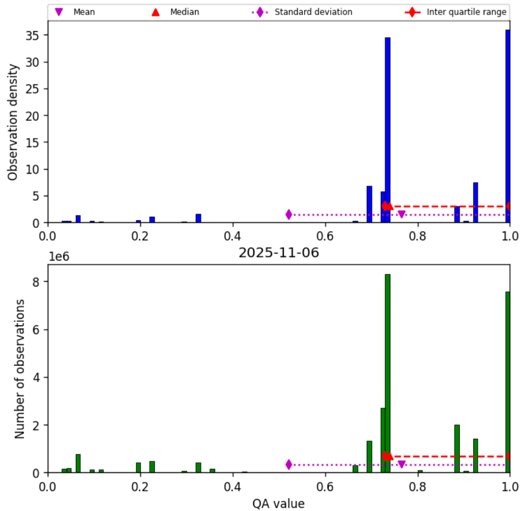
Figure 28: Histogram of “QA value” for 2025-11-05 to 2025-11-07
