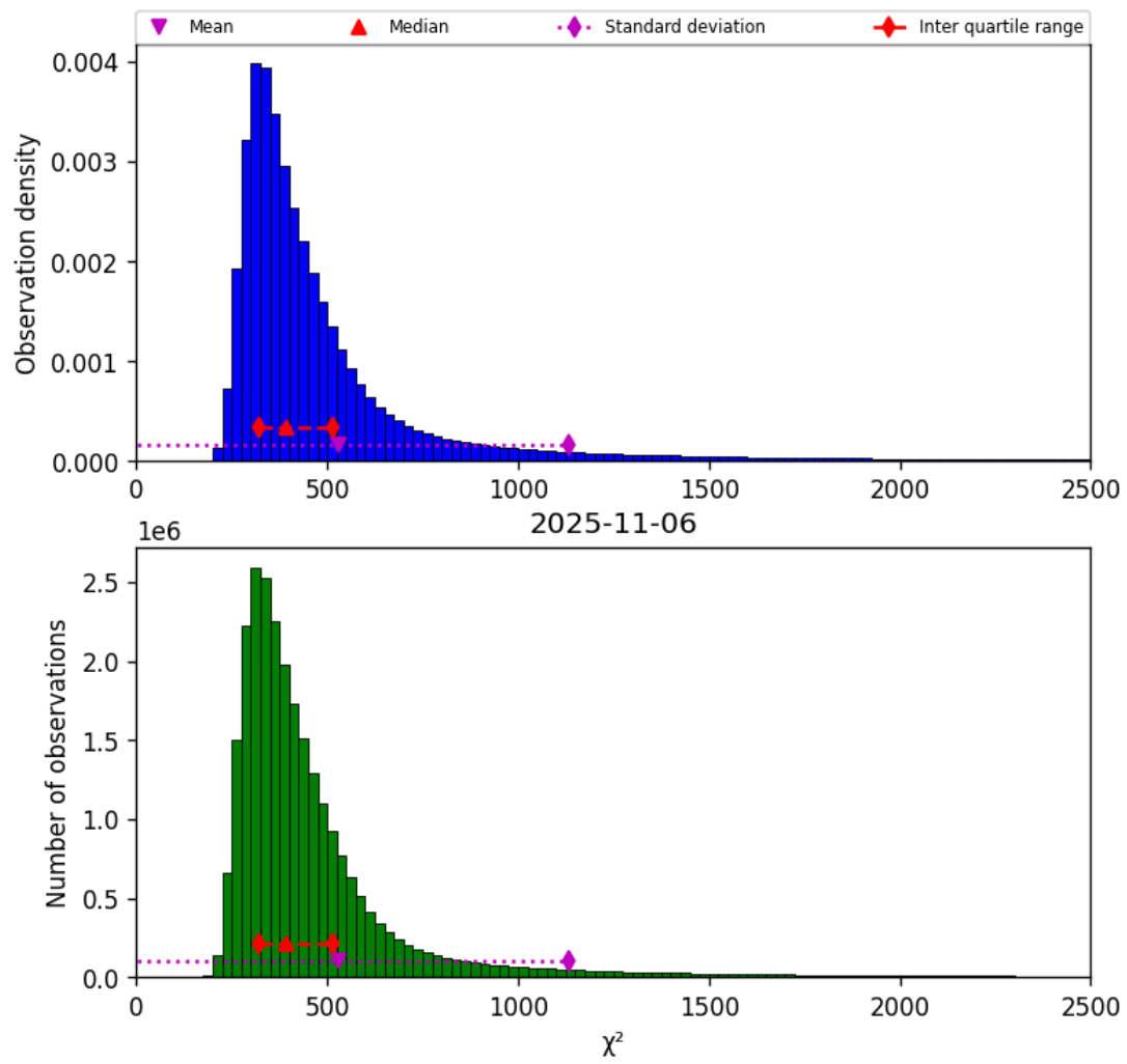
Figure 42: Histogram of “ \chi^2 ” for 2025-11-05 to 2025-11-07
