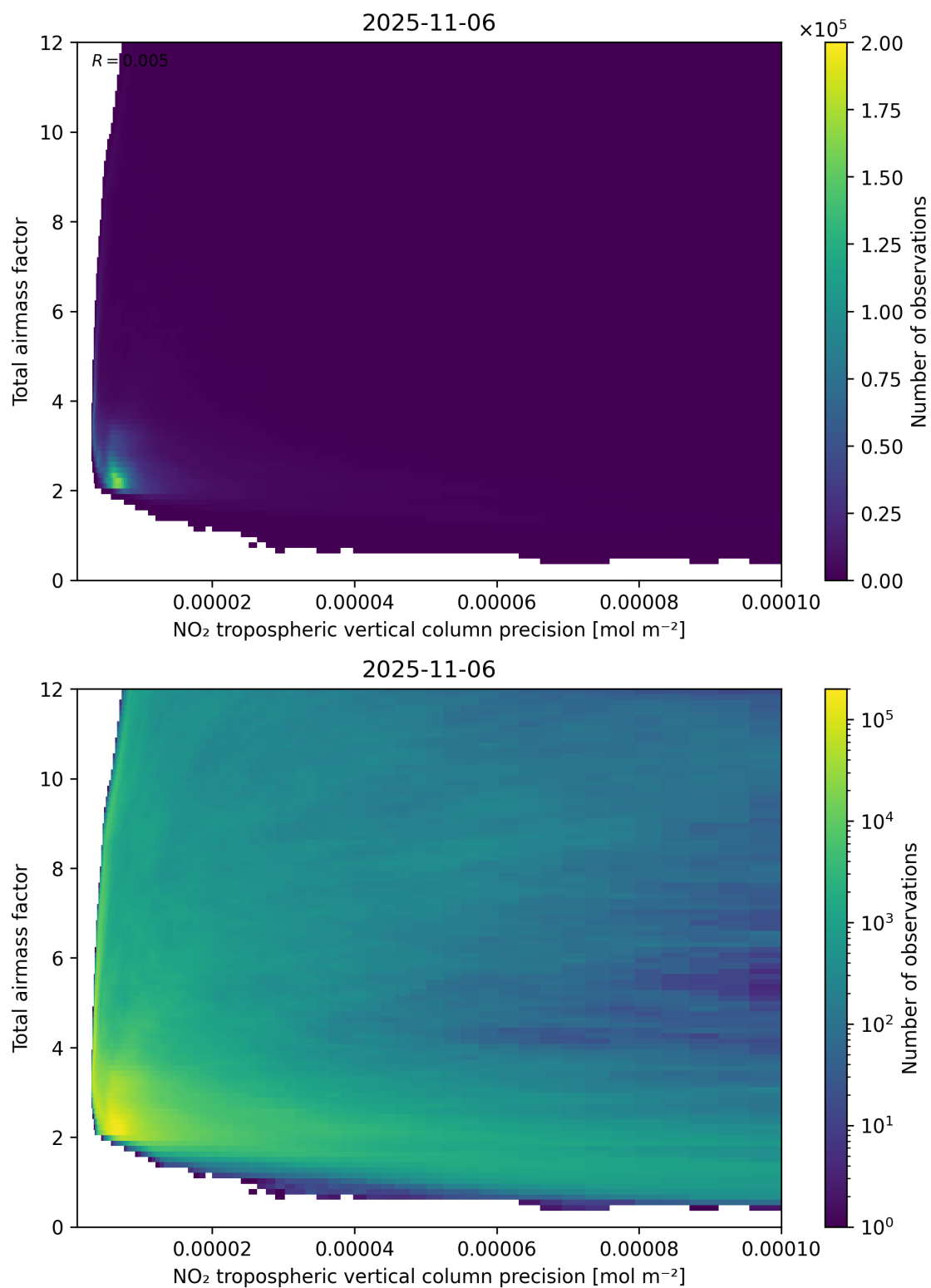
Figure 132: Scatter density plot of “NO 2 tropospheric vertical column precision” against “Total air mass factor” for 2025-11-05 to 2025-11-07.
