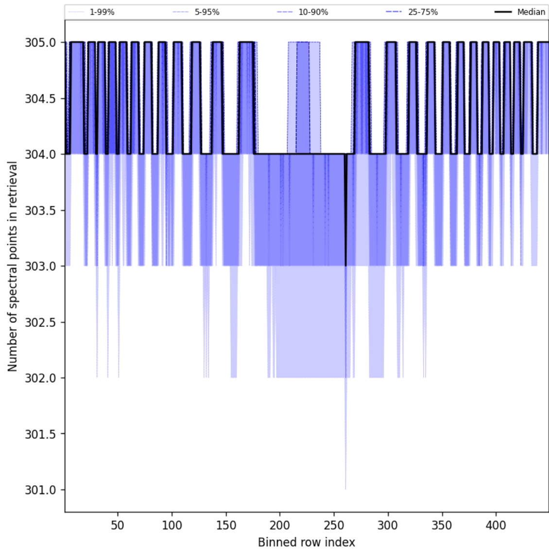
Figure 50: Along track statistics of “Number of spectral points in retrieval” for 2025-11-05 to 2025-11-07
