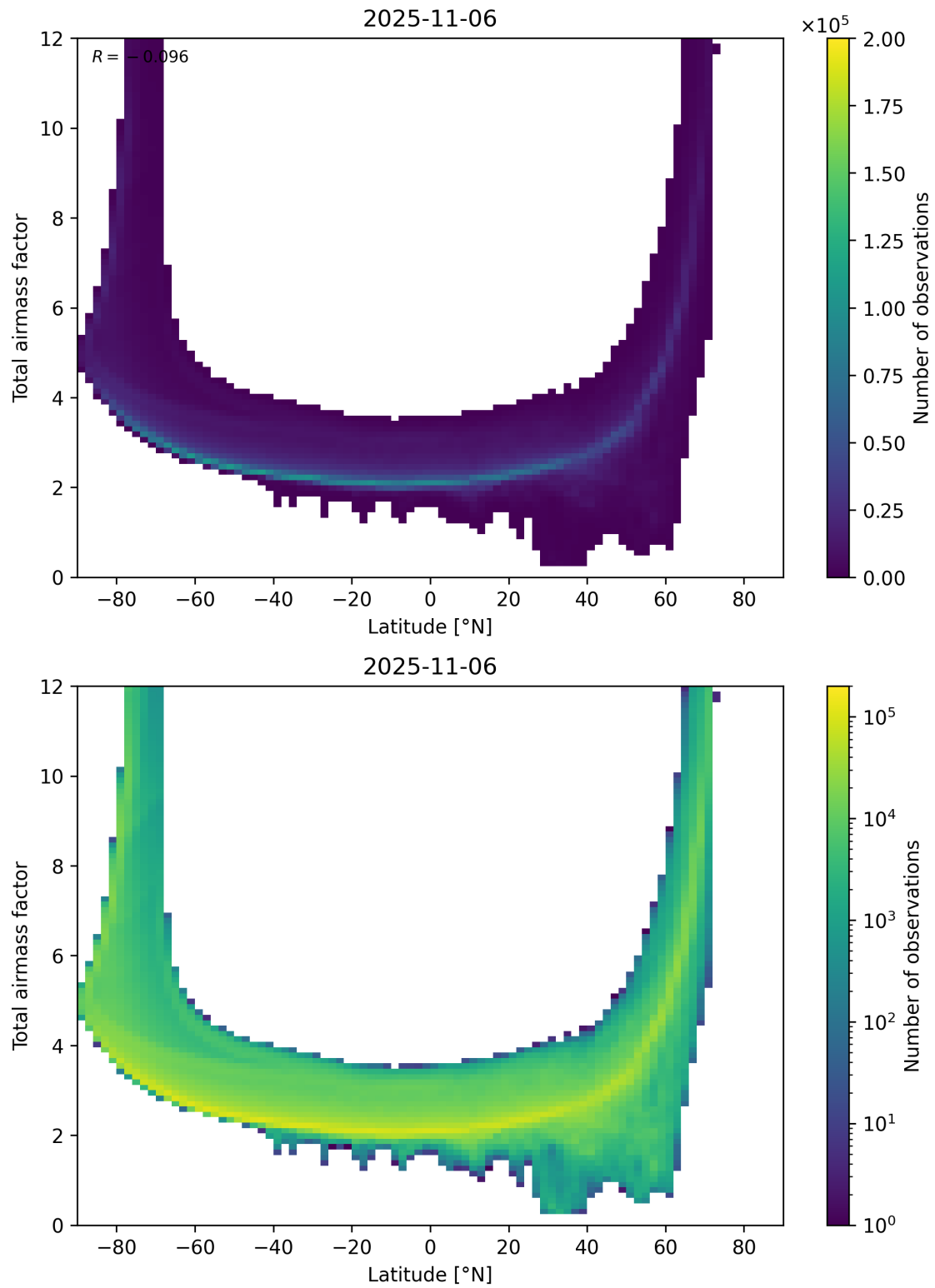
Figure 84: Scatter density plot of “Latitude” against “Total airmass factor” for 2025-11-05 to 2025-11-07.
