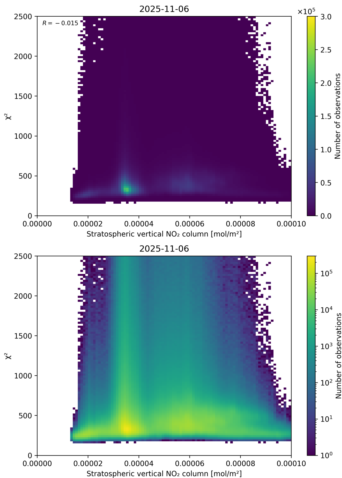
Figure 97: Scatter density plot of “Stratospheric vertical NO 2 column” against “ \chi^2 ” for 2025-11-05 to 2025-11-07.
