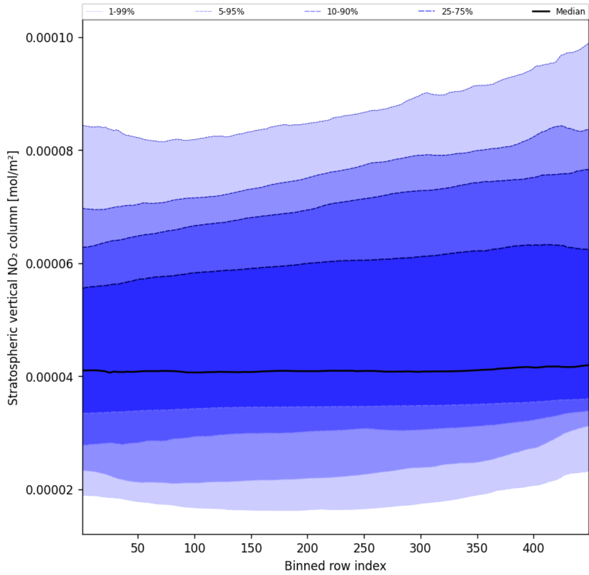
Figure 53: Along track statistics of “Stratospheric vertical NO 2 column” for 2025-11-05 to 2025-11-07
