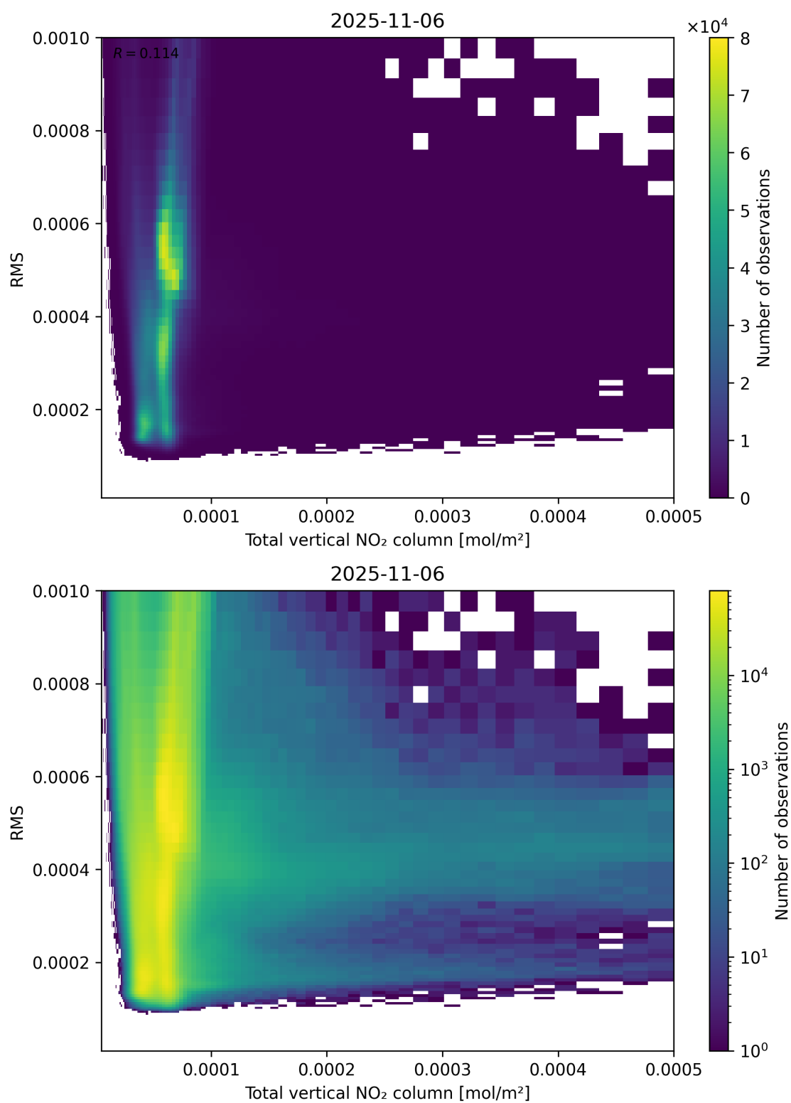
Figure 120: Scatter density plot of “Total vertical NO 2 column” against “RMS” for 2025-11-05 to 2025-11-07.
