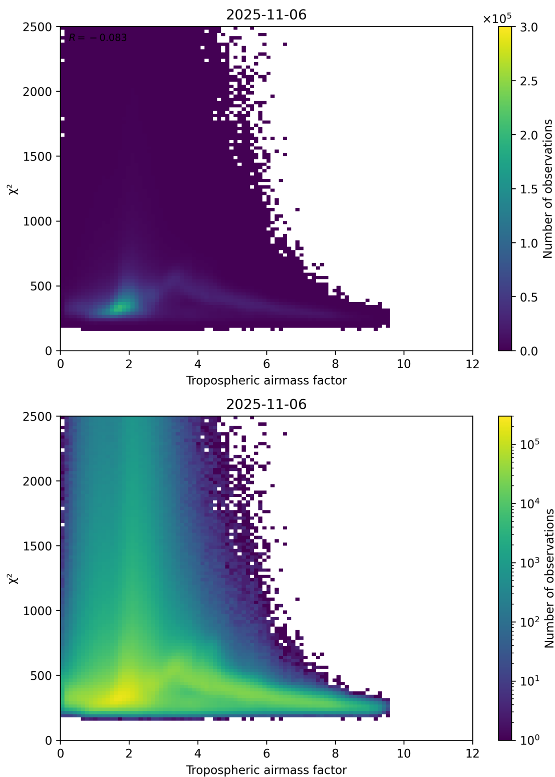
Figure 73: Scatter density plot of “Tropospheric airmass factor” against “ \chi^2 ” for 2025-11-05 to 2025-11-07.
