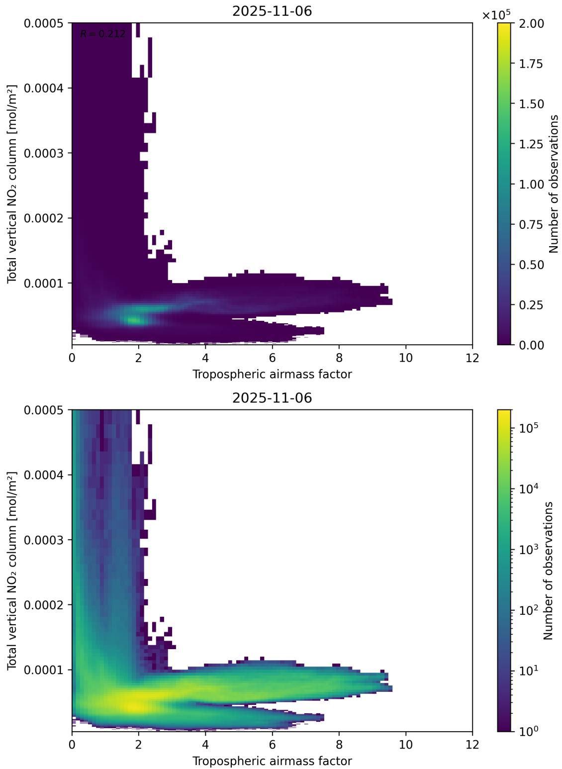
Figure 77: Scatter density plot of “Tropospheric airmass factor” against “Total vertical NO 2 column” for 2025-11-05 to 2025-11-07.
