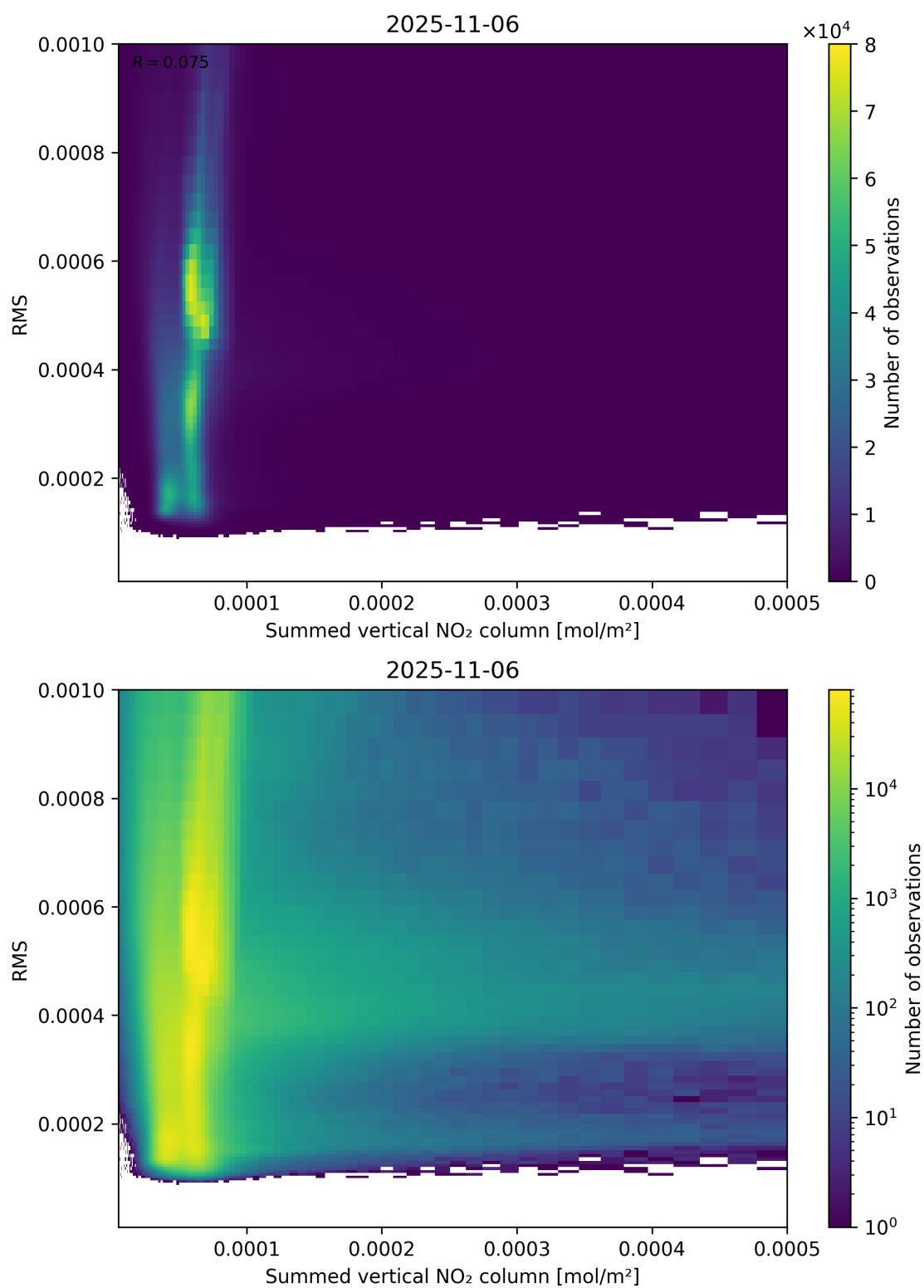
Figure 109: Scatter density plot of “Summed vertical NO 2 column” against “RMS” for 2025-11-05 to 2025-11-07.
