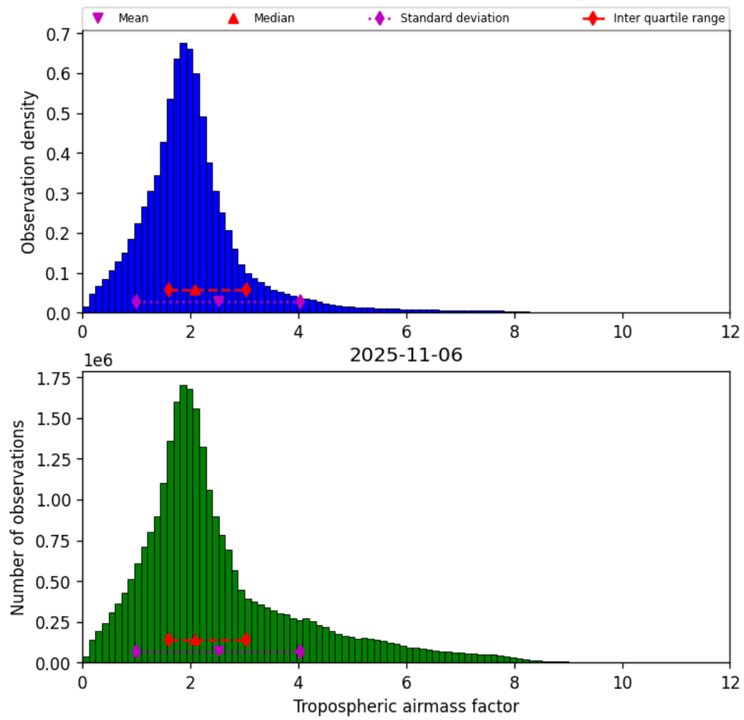
Figure 31: Histogram of “Tropospheric airmass factor” for 2025-11-05 to 2025-11-07
