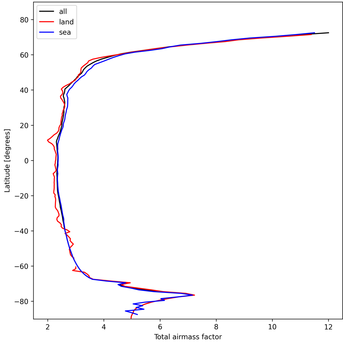
Figure 15: Zonal average of “Total airmass factor” for 2025-11-05 to 2025-11-07.
