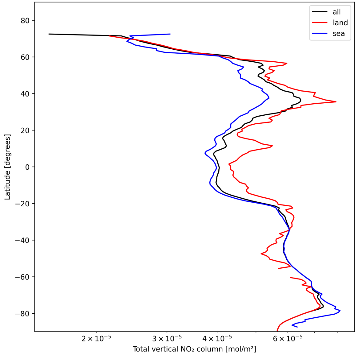
Figure 21: Zonal average of “Total vertical NO 2 column” for 2025-11-05 to 2025-11-07.
