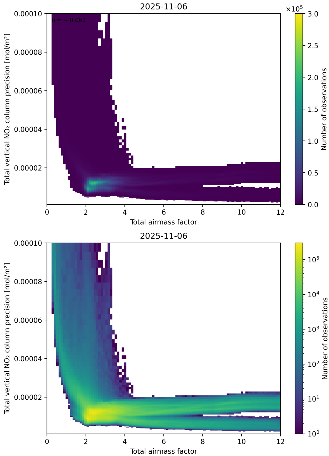
Figure 68: Scatter density plot of “Total airmass factor” against “Total vertical NO 2 column precision” for 2025-11-05 to 2025-11-07.
