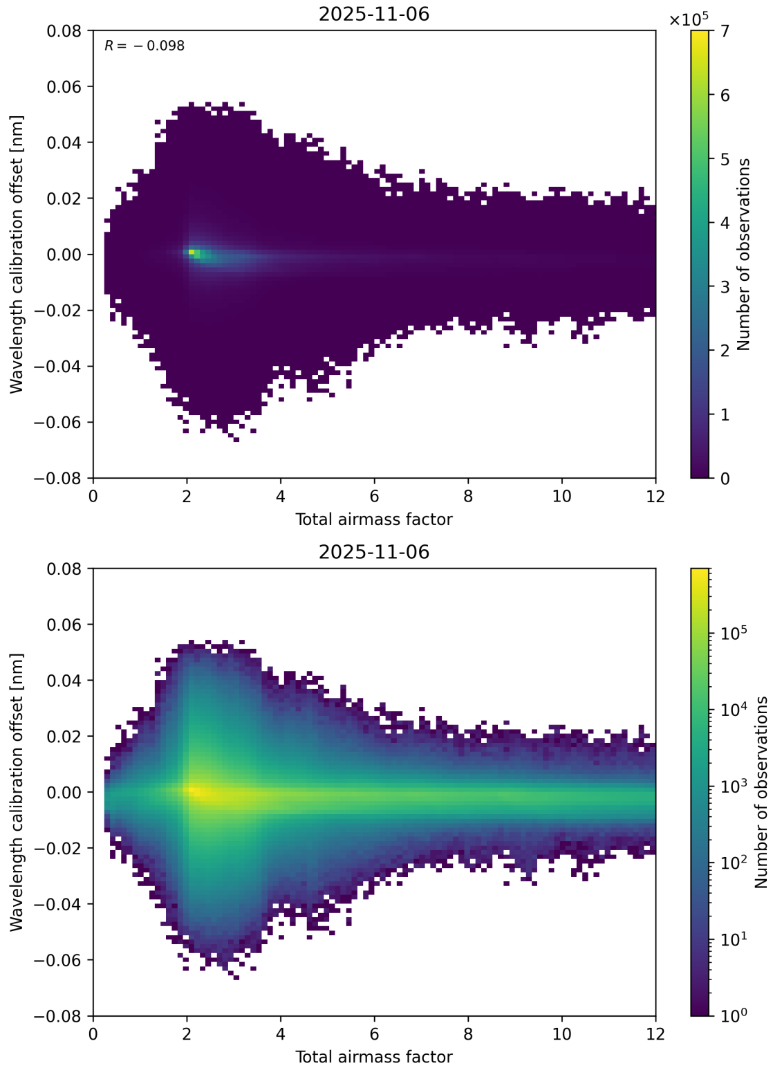
Figure 70: Scatter density plot of “Total airmass factor” against “Wavelength calibration offset” for 2025-11-05 to 2025-11-07.
