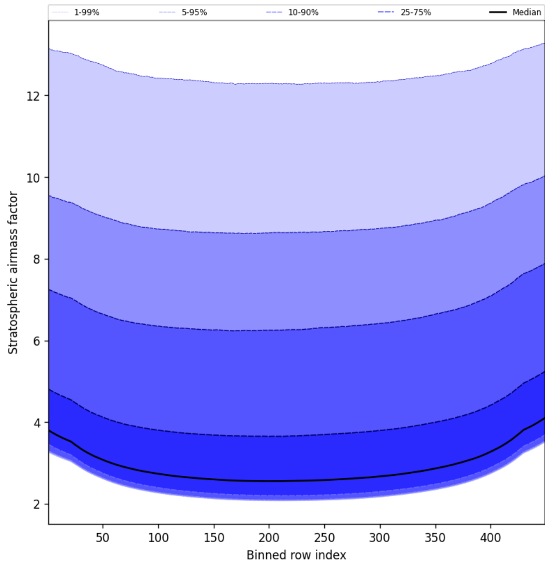
Figure 61: Along track statistics of “Stratospheric air mass factor” for 2025-11-05 to 2025-11-07
