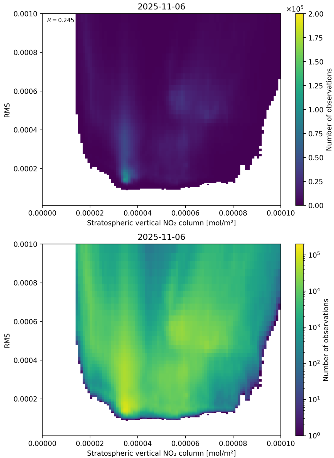
Figure 102: Scatter density plot of “Stratospheric vertical NO 2 column” against “RMS” for 2025-11-05 to 2025-11-07.
