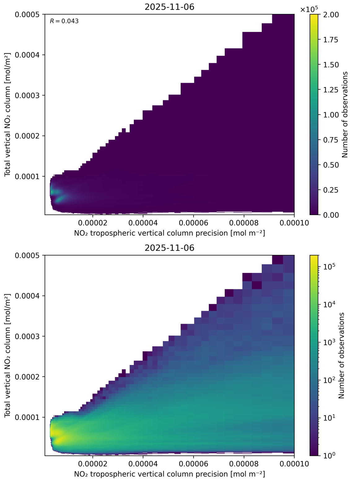
Figure 138: Scatter density plot of “NO 2 tropospheric vertical column precision” against “Total vertical NO 2 column” for 2025-11-05 to 2025-11-07.
