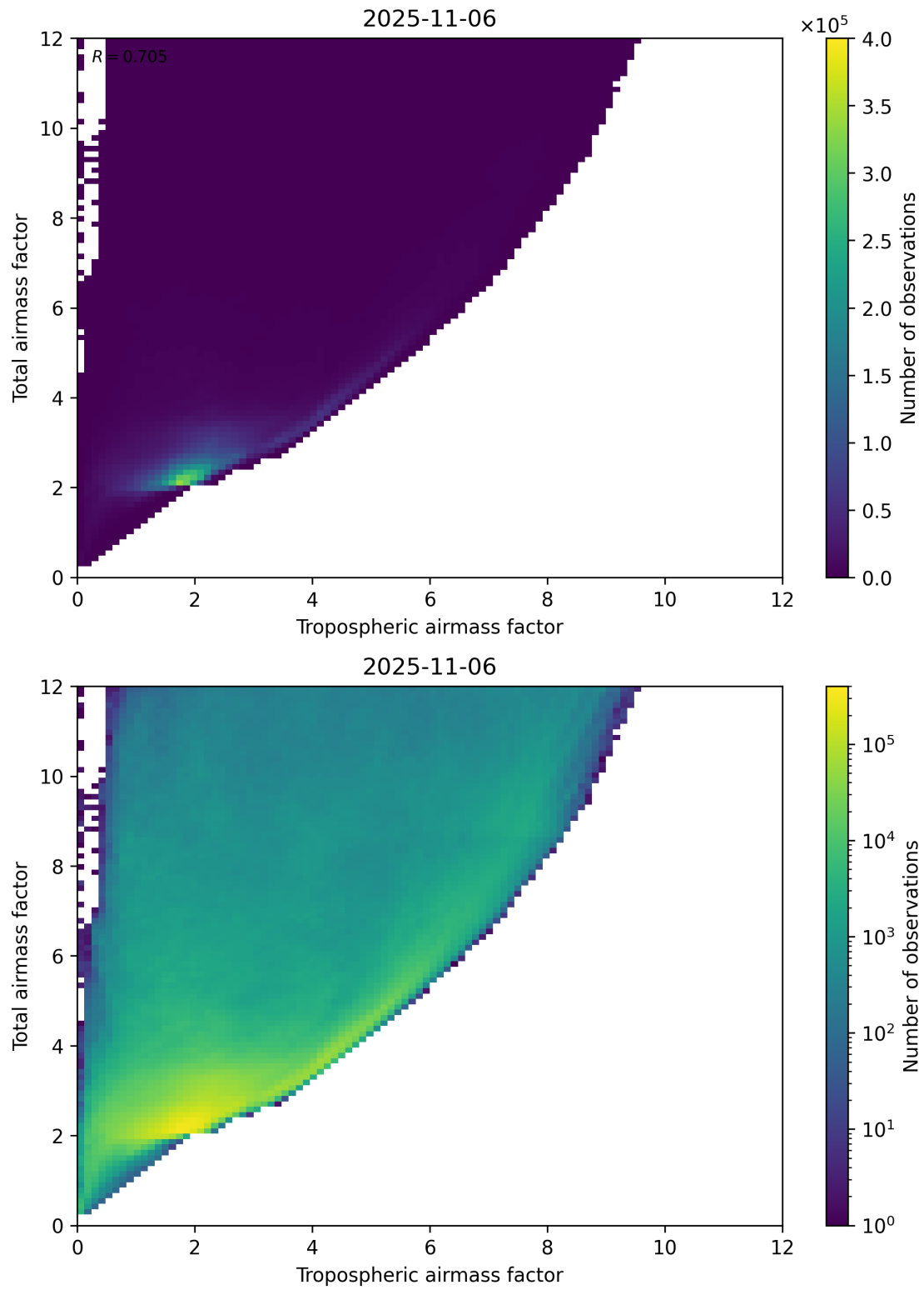
Figure 72: Scatter density plot of “Tropospheric airmass factor” against “Total airmass factor” for 2025-11-05 to 2025-11-07.
