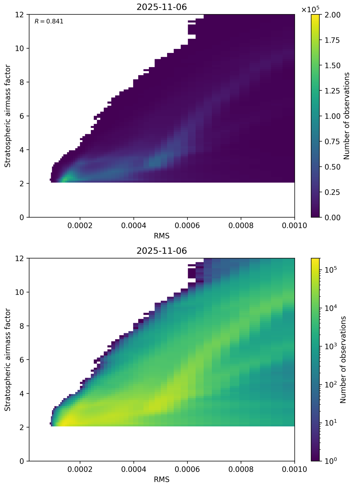
Figure 144: Scatter density plot of “RMS” against “Stratospheric airmass factor” for 2025-11-05 to 2025-11-07.
