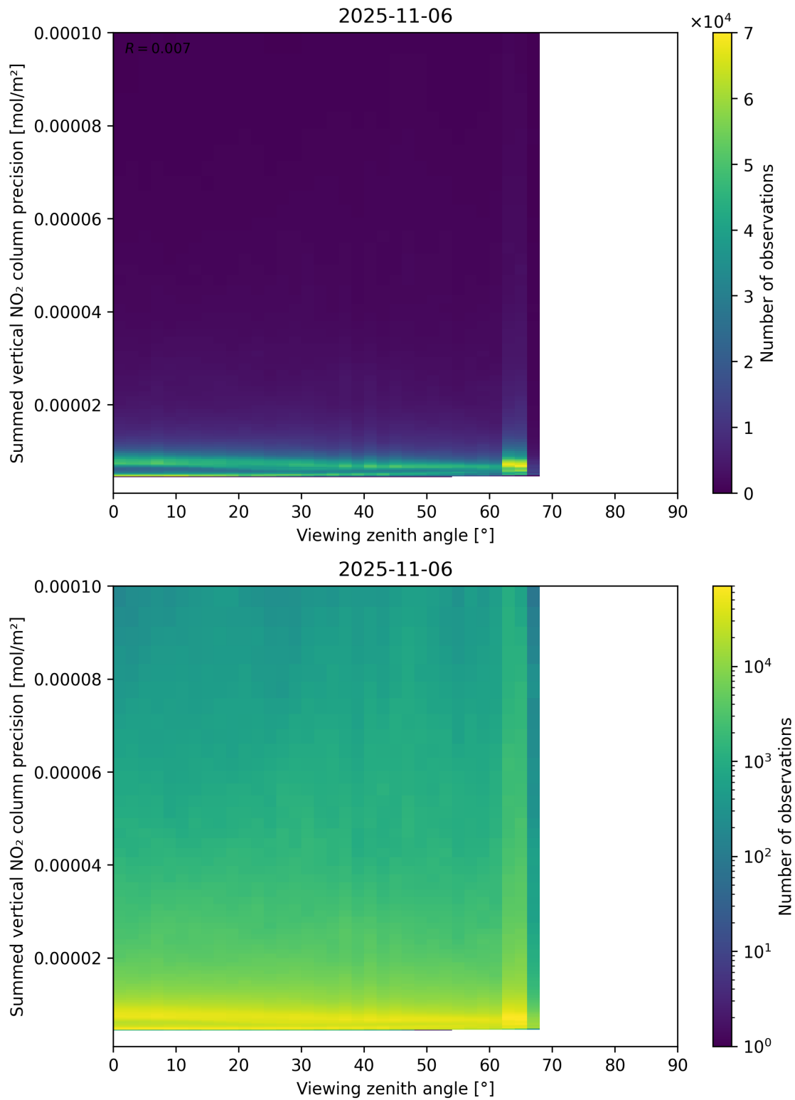
Figure 166: Scatter density plot of “Viewing zenith angle” against “Summed vertical NO 2 column precision” for 2025-11-05 to 2025-11-07.
