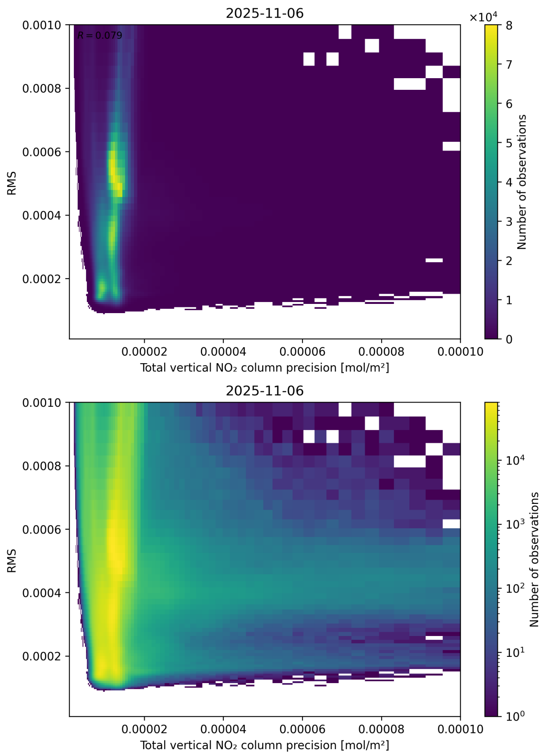
Figure 119: Scatter density plot of “Total vertical NO 2 column precision” against “RMS” for 2025-11-05 to 2025-11-07.
