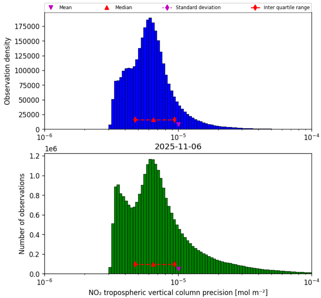
Figure 30: Histogram of "NO 2 tropospheric vertical column precision" for 2025-11-05 to 2025-11-07
