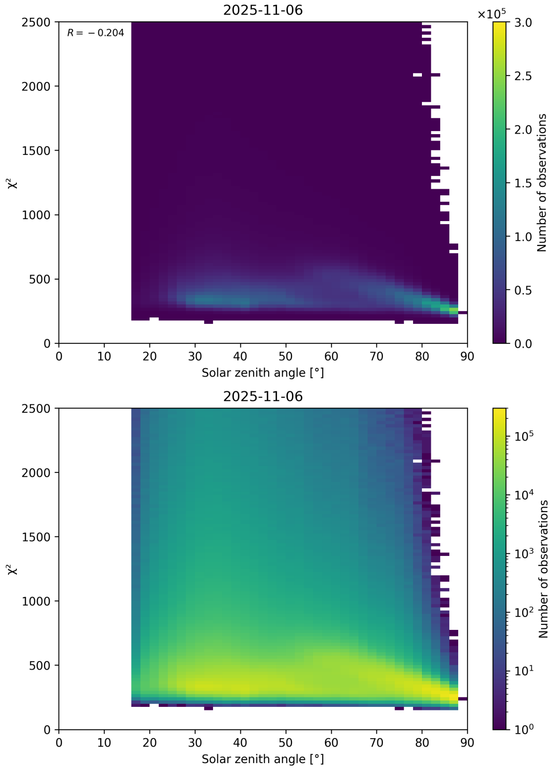
Figure 148: Scatter density plot of “Solar zenith angle” against “ \chi^2 ” for 2025-11-05 to 2025-11-07.
