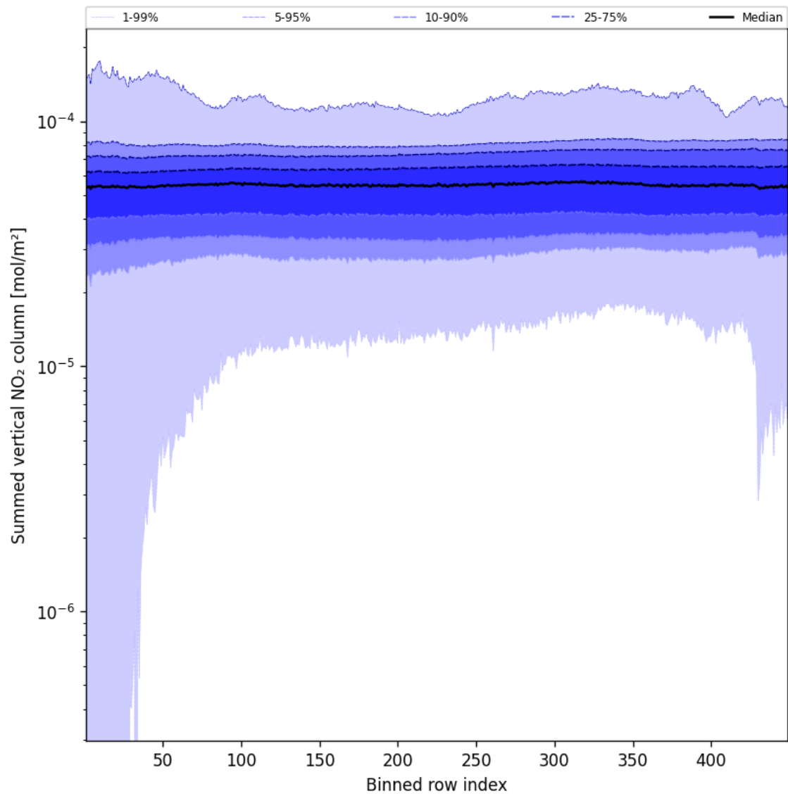
Figure 57: Along track statistics of “Summed vertical NO 2 column” for 2025-11-05 to 2025-11-07
