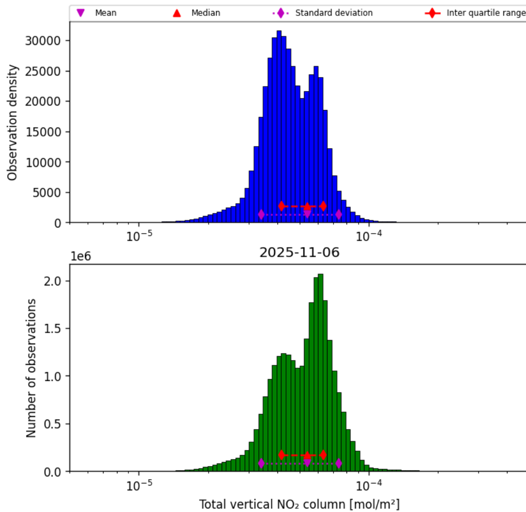
Figure 38: Histogram of “Total vertical NO 2 column” for 2025-11-05 to 2025-11-07
