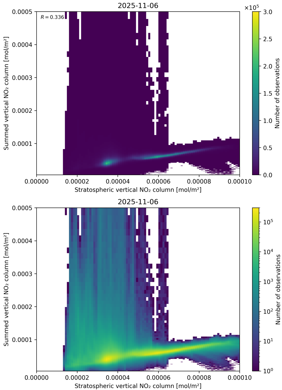
Figure 98: Scatter density plot of “Stratospheric vertical NO 2 column” against “Summed vertical NO 2 column” for 2025-11-05 to 2025-11-07.
