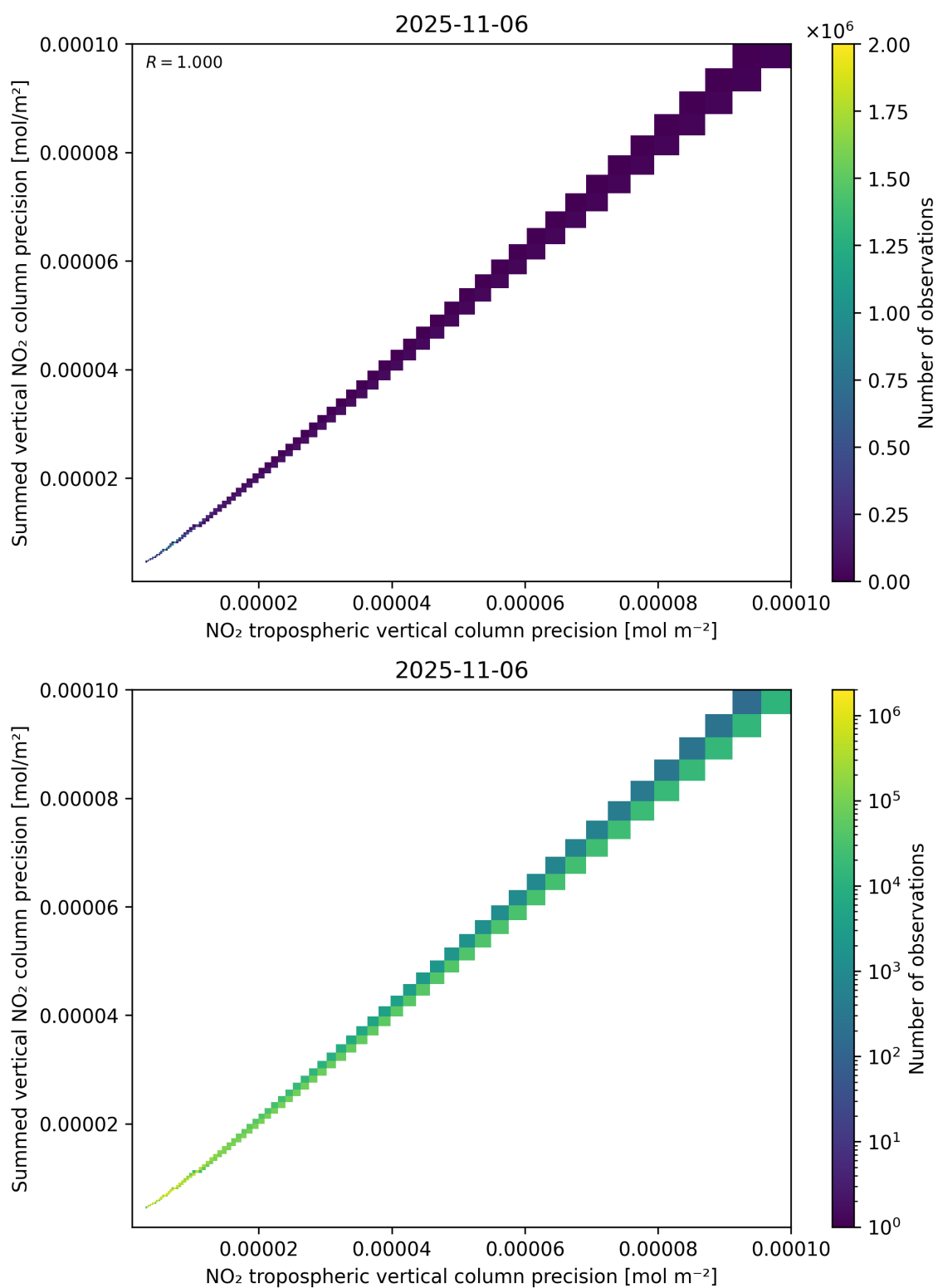
Figure 137: Scatter density plot of “NO 2 tropospheric vertical column precision” against “Summed vertical NO 2 column precision” for 2025-11-05 to 2025-11-07.
