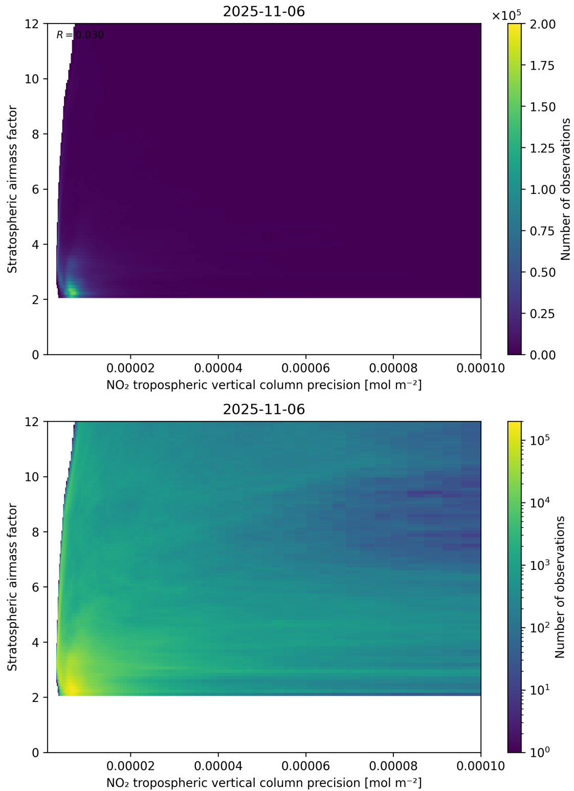
Figure 131: Scatter density plot of “NO 2 tropospheric vertical column precision” against “Stratospheric airmass factor” for 2025-11-05 to 2025-11-07.
