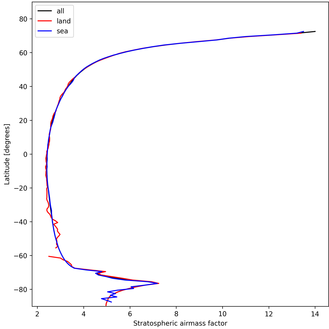
Figure 27: Zonal average of “Stratospheric airmass factor” for 2025-11-05 to 2025-11-07.
