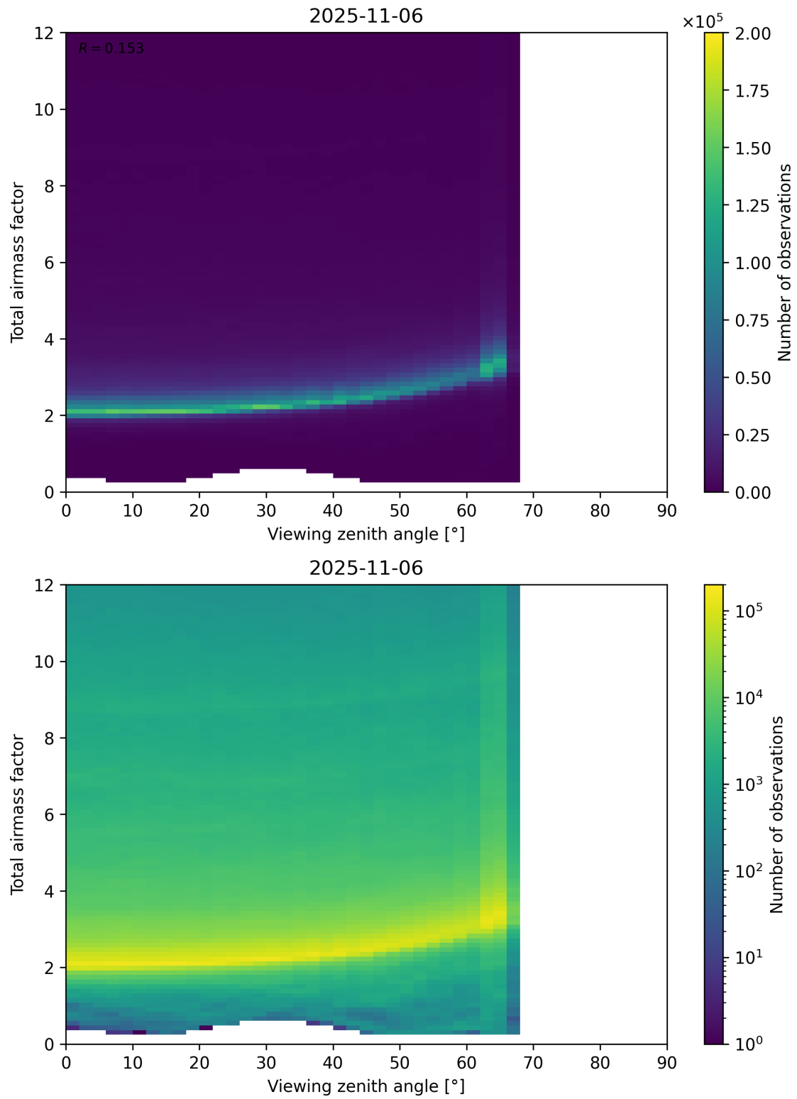
Figure 160: Scatter density plot of “Viewing zenith angle” against “Total airmass factor” for 2025-11-05 to 2025-11-07.
