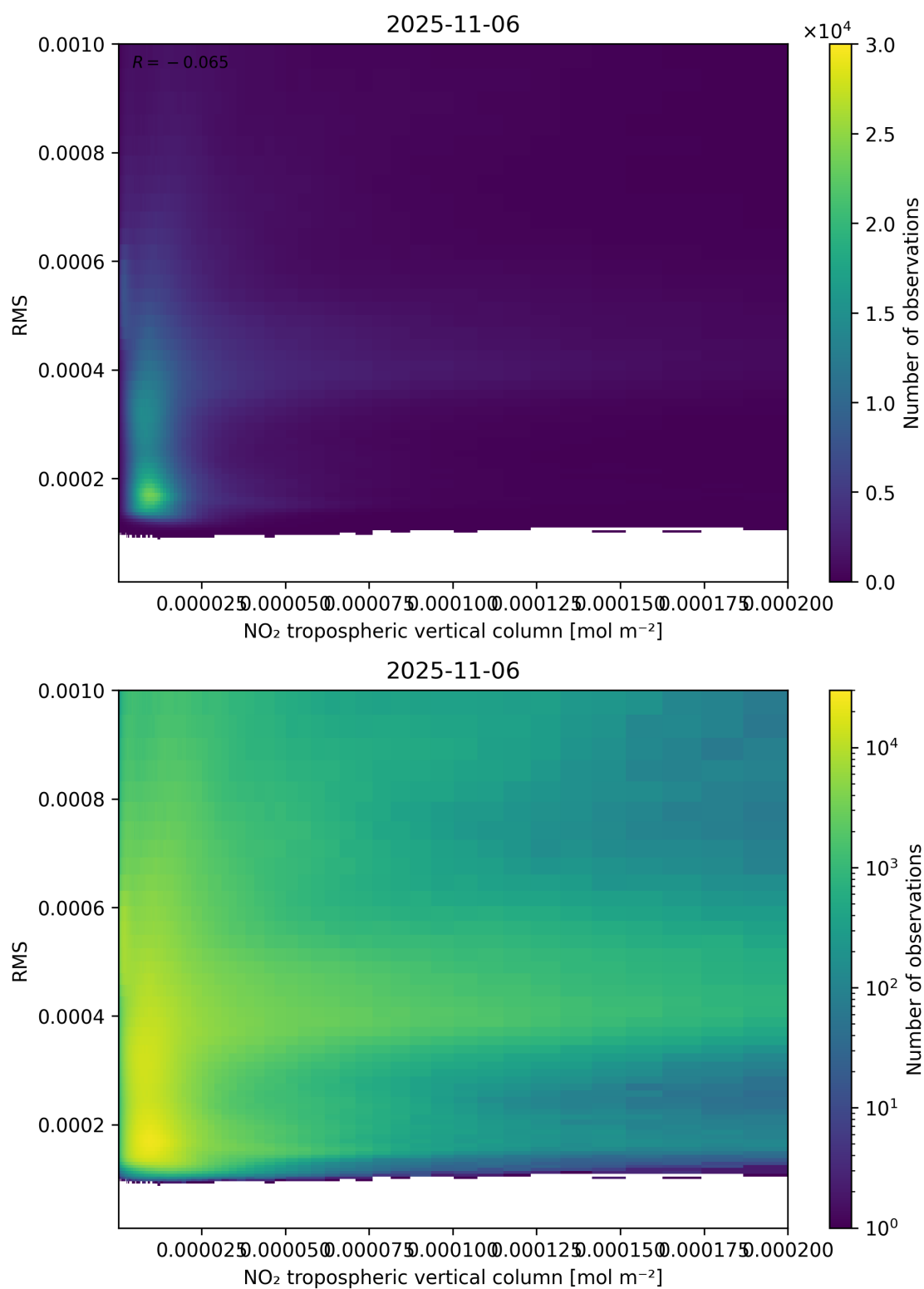
Figure 142: Scatter density plot of “NO 2 tropospheric vertical column” against “RMS” for 2025-11-05 to 2025-11-07.
