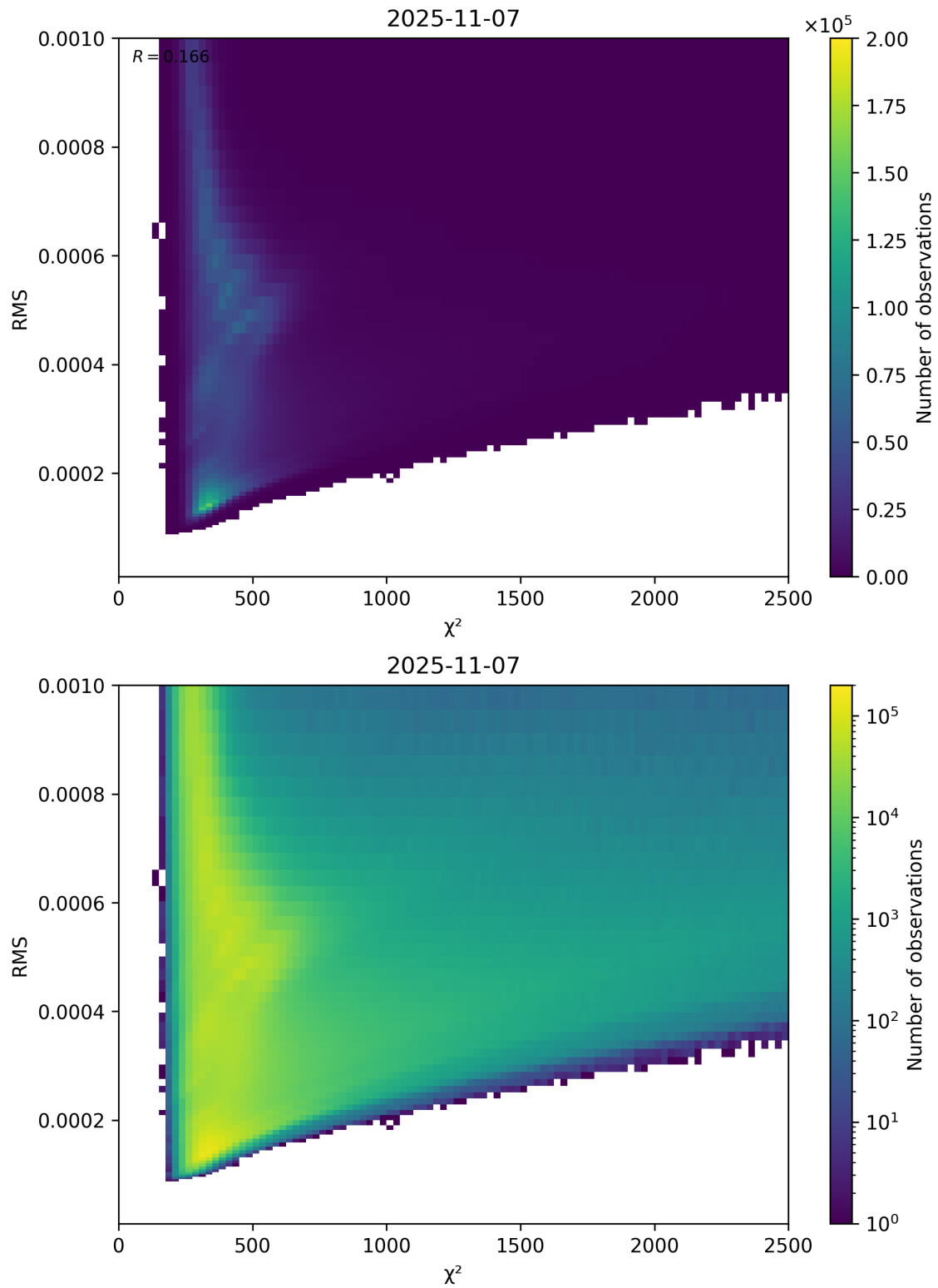
Figure 82: Scatter density plot of “ \chi^2 ” against “RMS” for 2025-11-07 to 2025-11-08.
