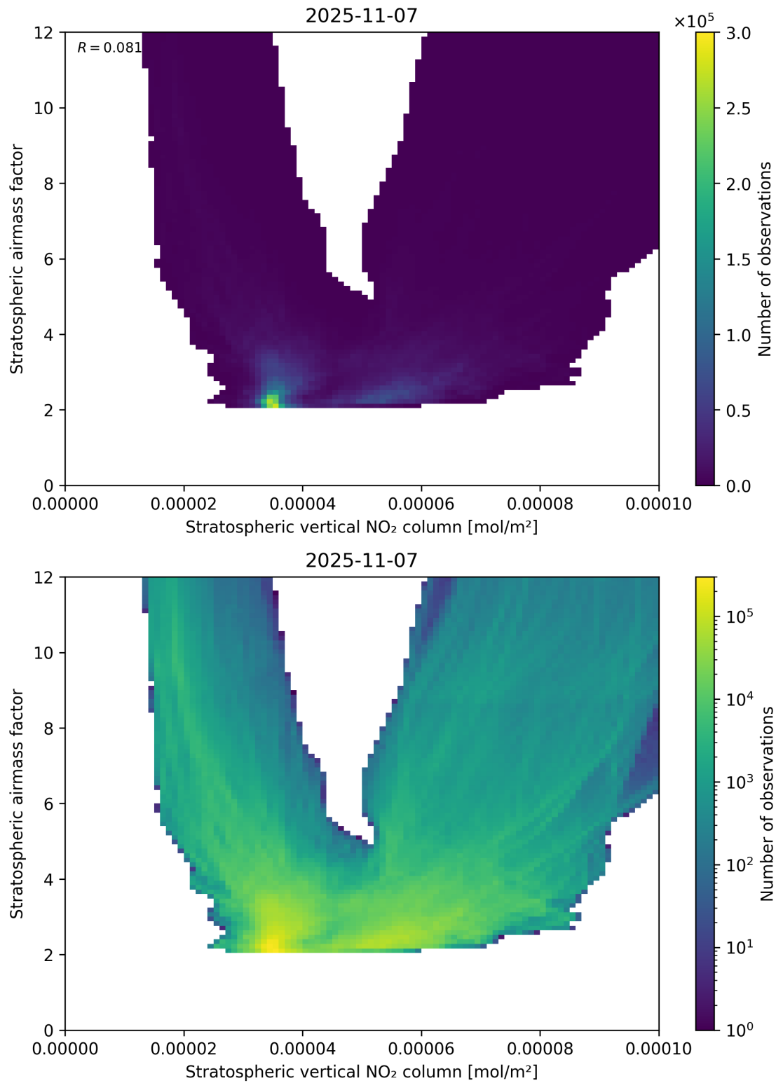
Figure 96: Scatter density plot of “Stratospheric vertical NO 2 column” against “Stratospheric airmass factor” for 2025-11-07 to 2025-11-08.
