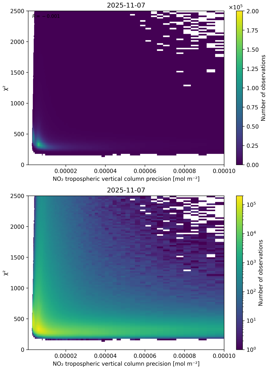
Figure 134: Scatter density plot of “NO 2 tropospheric vertical column precision” against “ \chi^2 ” for 2025-11-07 to 2025-11-08.
