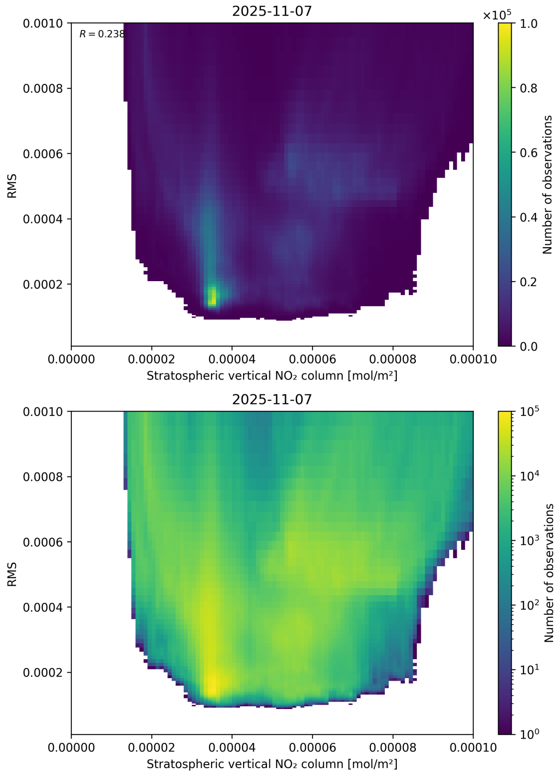
Figure 102: Scatter density plot of “Stratospheric vertical NO 2 column” against “RMS” for 2025-11-07 to 2025-11-08.
