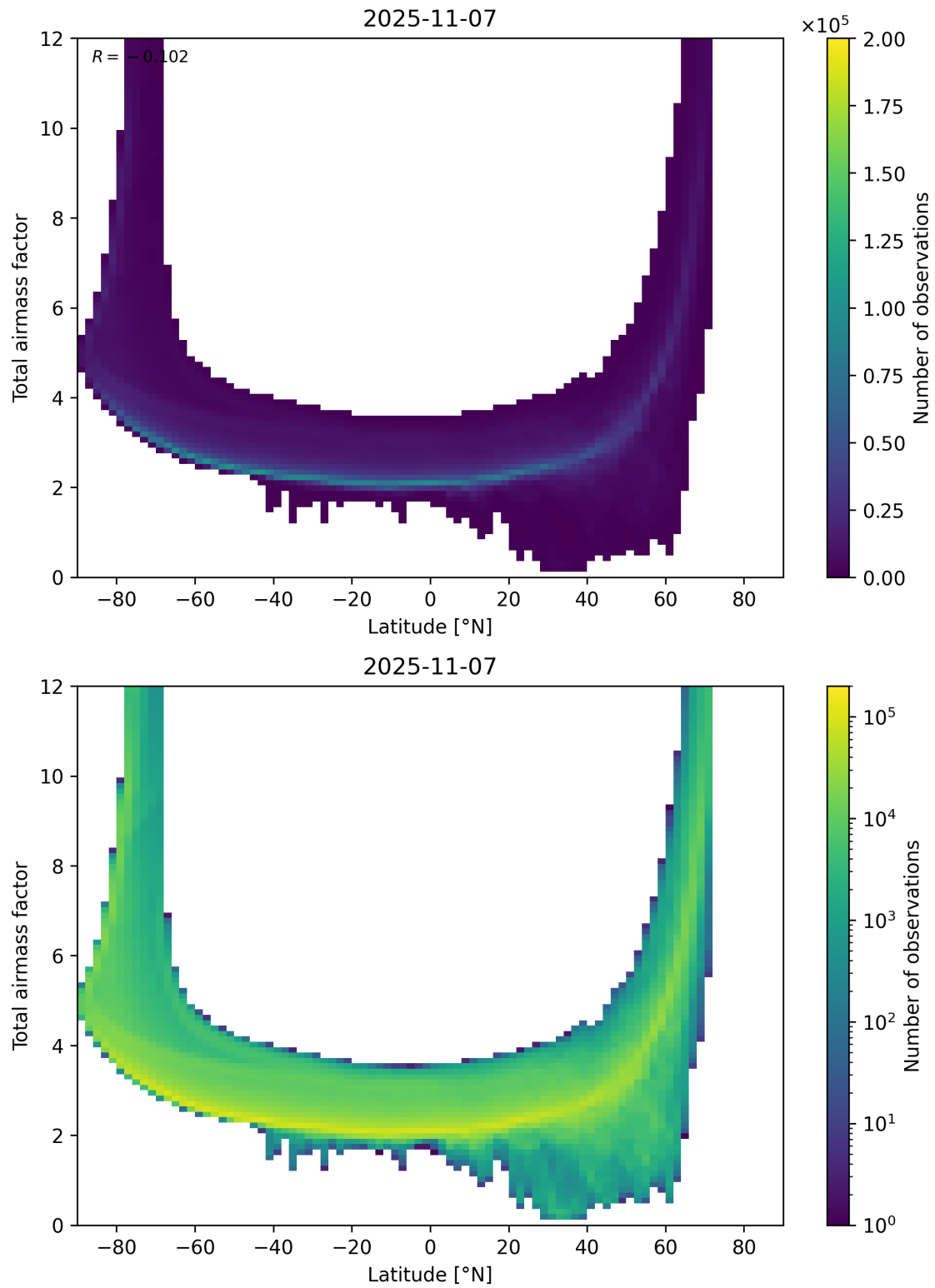
Figure 84: Scatter density plot of “Latitude” against “Total airmass factor” for 2025-11-07 to 2025-11-08.
