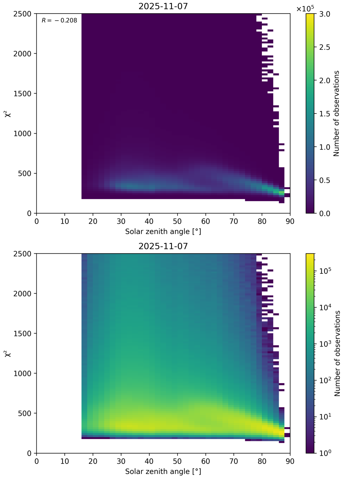
Figure 148: Scatter density plot of “Solar zenith angle” against “ \chi^2 ” for 2025-11-07 to 2025-11-08.
