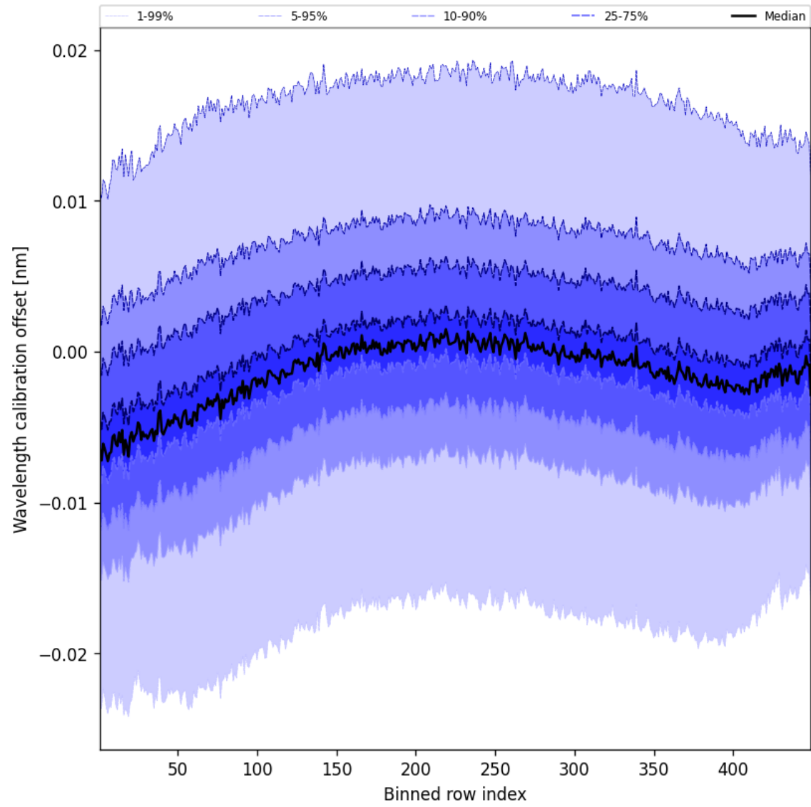
Figure 52: Along track statistics of “Wavelength calibration offset” for 2025-11-07 to 2025-11-08
