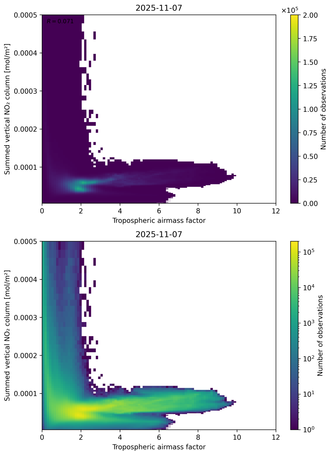
Figure 75: Scatter density plot of “Tropospheric air mass factor” against “Summed vertical NO 2 column” for 2025-11-07 to 2025-11-08.
