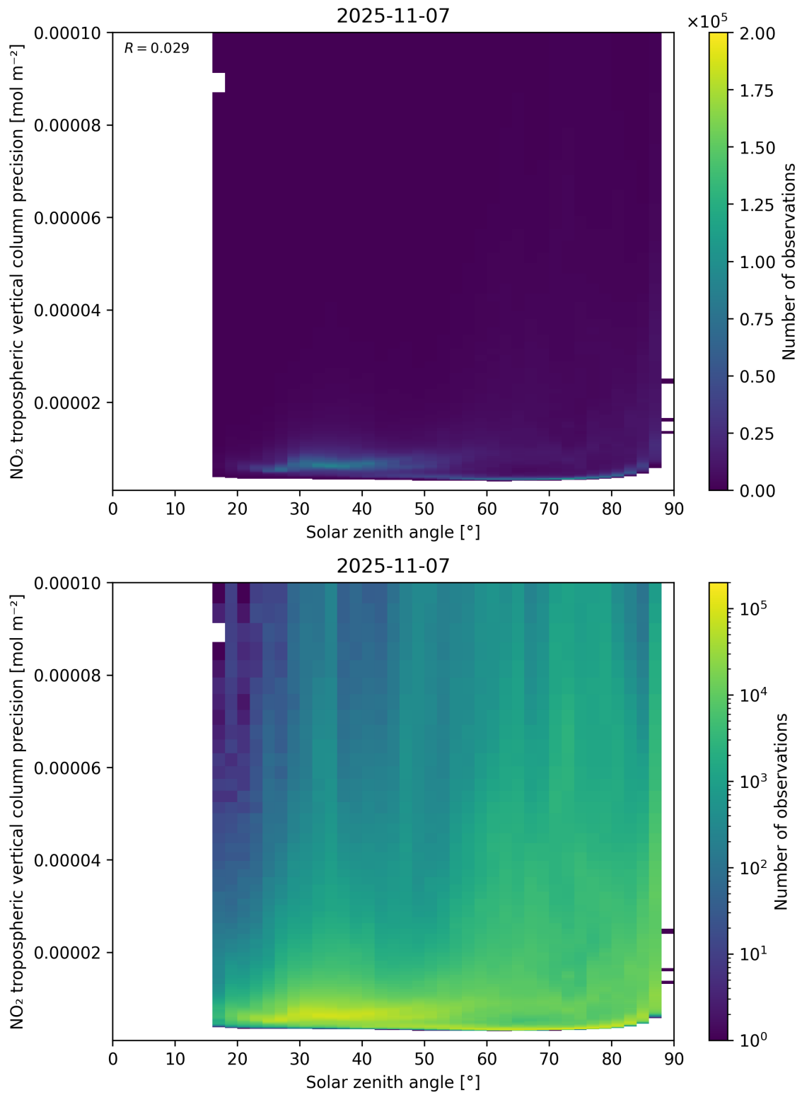
Figure 156: Scatter density plot of “Solar zenith angle” against “NO 2 tropospheric vertical column precision” for 2025-11-07 to 2025-11-08.
