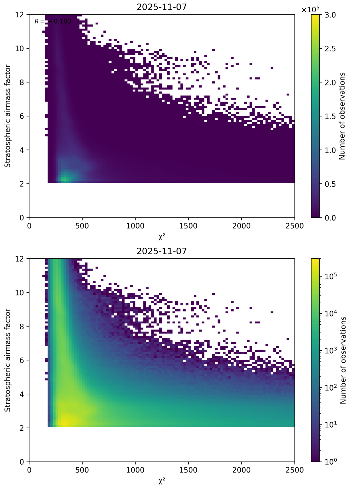
Figure 81: Scatter density plot of “ \chi^2 ” against “Stratospheric airmass factor” for 2025-11-07 to 2025-11-08.
