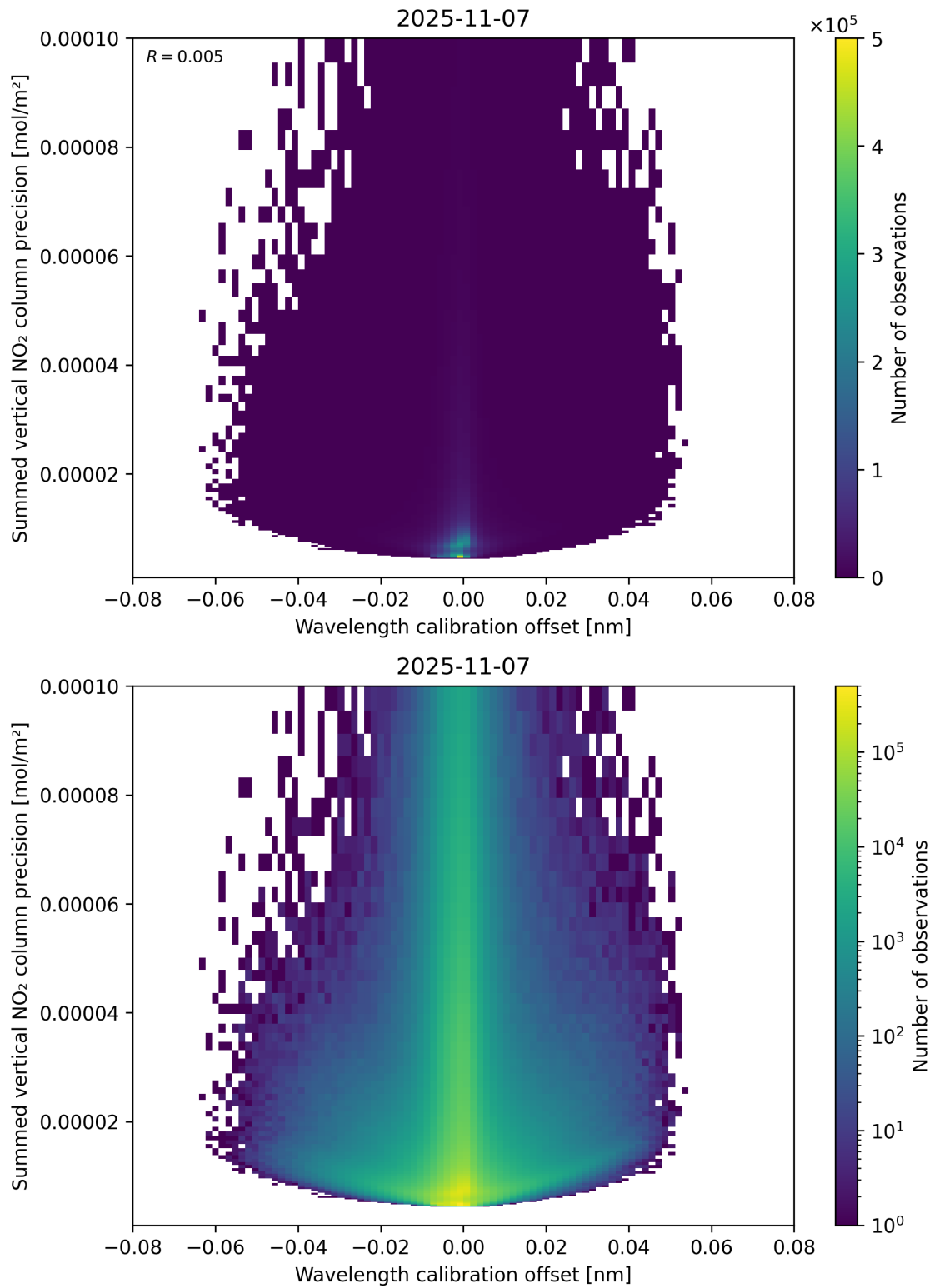
Figure 178: Scatter density plot of “Wavelength calibration offset” against “Summed vertical NO 2 column precision” for 2025-11-07 to 2025-11-08.
