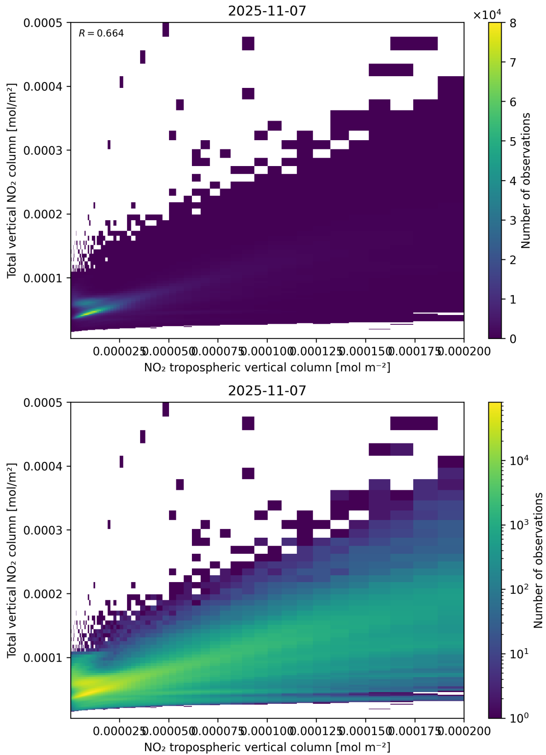
Figure 128: Scatter density plot of “NO 2 tropospheric vertical column” against “Total vertical NO 2 column” for 2025-11-07 to 2025-11-08.
