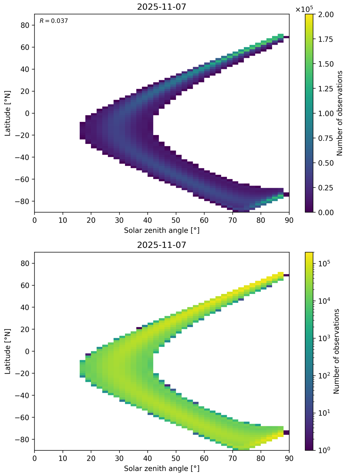
Figure 149: Scatter density plot of “Solar zenith angle” against “Latitude” for 2025-11-07 to 2025-11-08.
