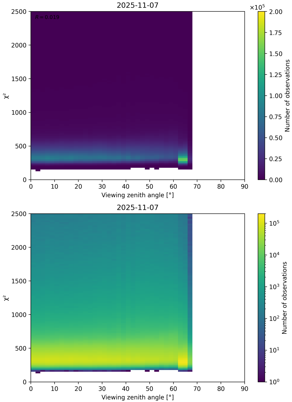
Figure 162: Scatter density plot of “Viewing zenith angle” against “ \chi^2 ” for 2025-11-07 to 2025-11-08.
