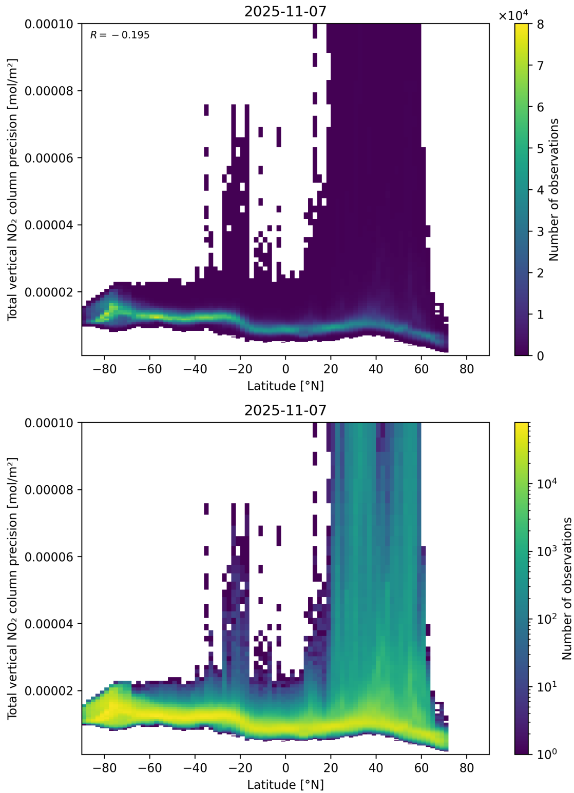
Figure 91: Scatter density plot of “Latitude” against “Total vertical NO 2 column precision” for 2025-11-07 to 2025-11-08.
