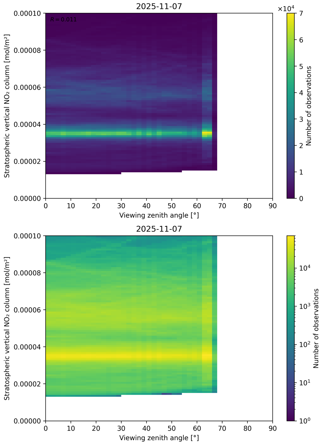
Figure 164: Scatter density plot of “Viewing zenith angle” against “Stratospheric vertical NO 2 column” for 2025-11-07 to 2025-11-08.
