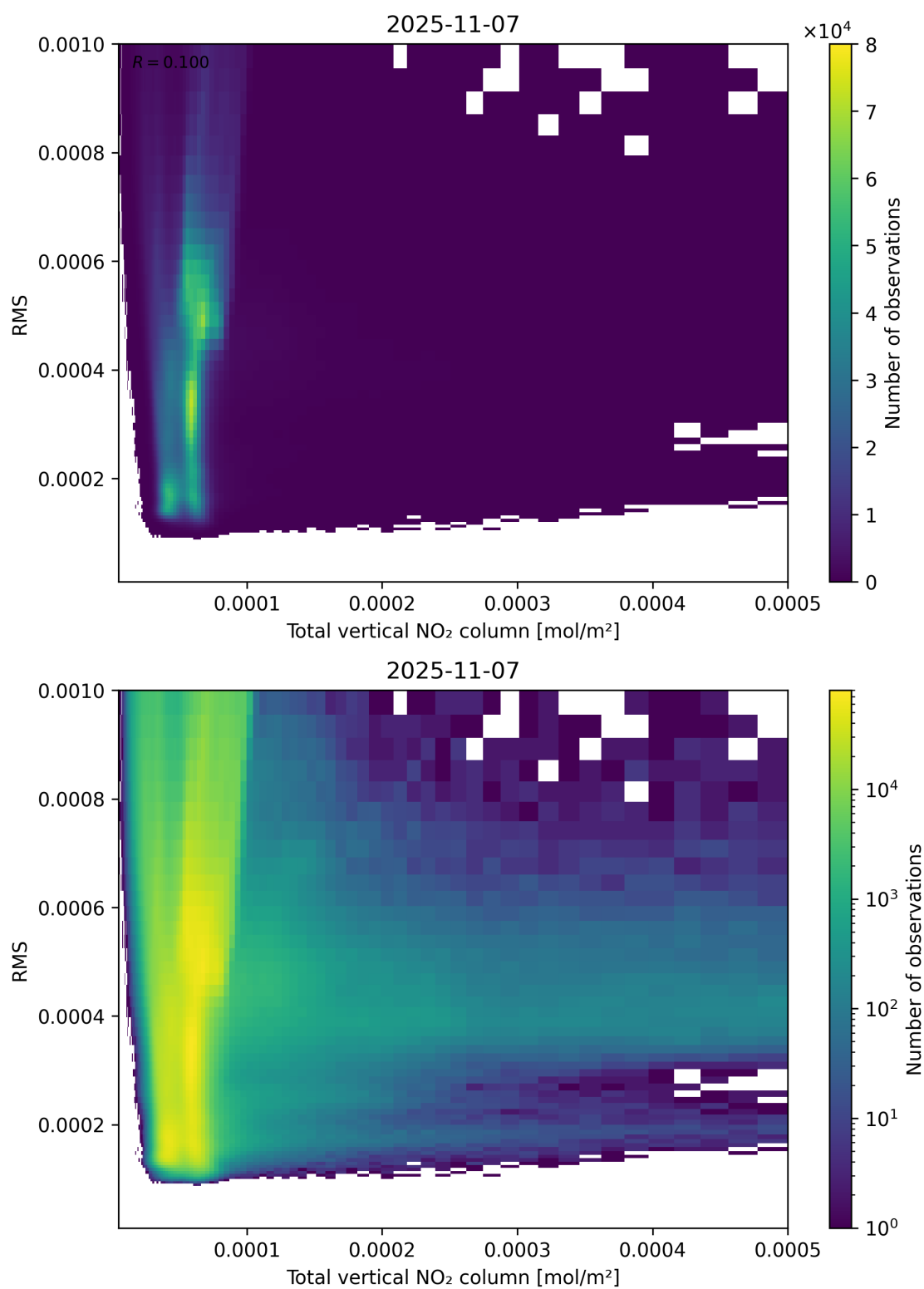
Figure 120: Scatter density plot of “Total vertical NO 2 column” against “RMS” for 2025-11-07 to 2025-11-08.
