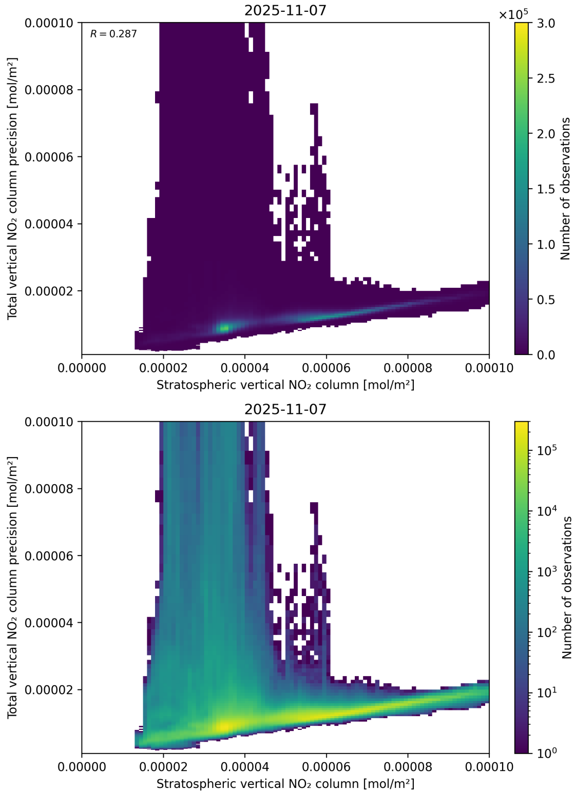
Figure 101: Scatter density plot of “Stratospheric vertical NO 2 column” against “Total vertical NO 2 column precision” for 2025-11-07 to 2025-11-08.
