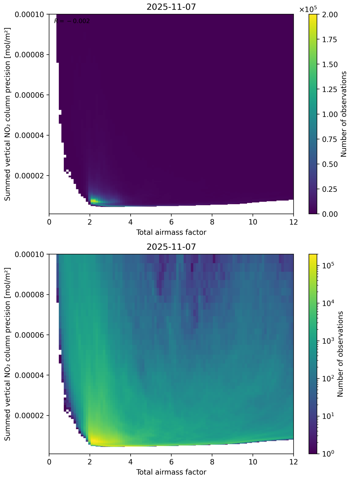
Figure 66: Scatter density plot of “Total airmass factor” against “Summed vertical NO 2 column precision” for 2025-11-07 to 2025-11-08.
