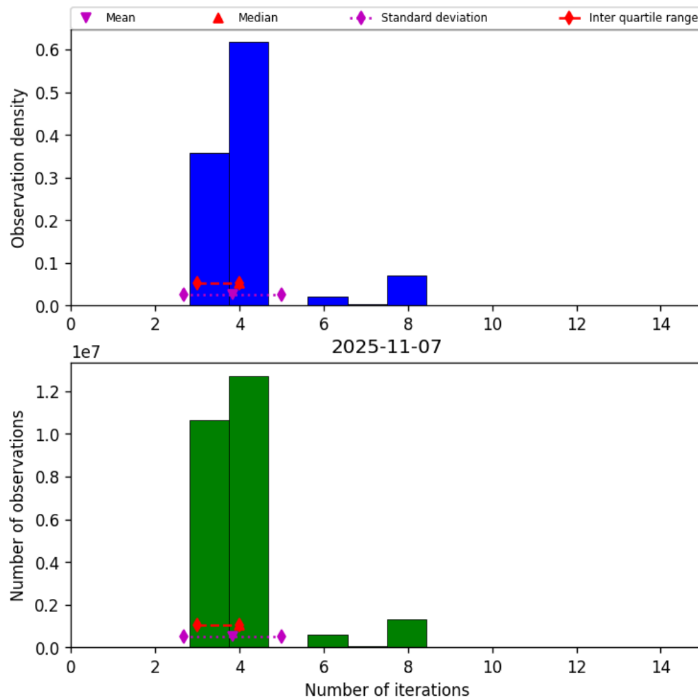
Figure 34: Histogram of “Number of iterations” for 2025-11-07 to 2025-11-08
