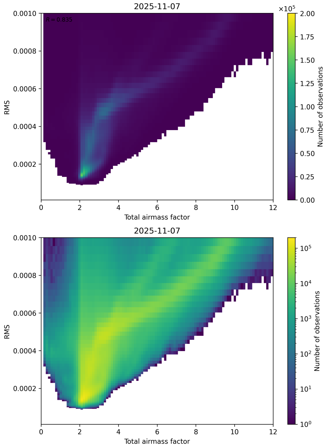
Figure 69: Scatter density plot of “Total airmass factor” against “RMS” for 2025-11-07 to 2025-11-08.
