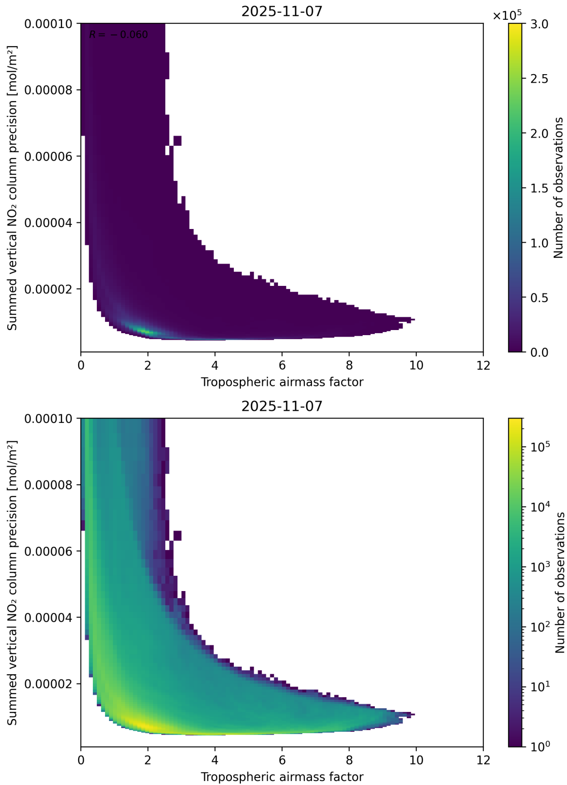
Figure 76: Scatter density plot of “Tropospheric air mass factor” against “Summed vertical NO 2 column precision” for 2025-11-07 to 2025-11-08.
