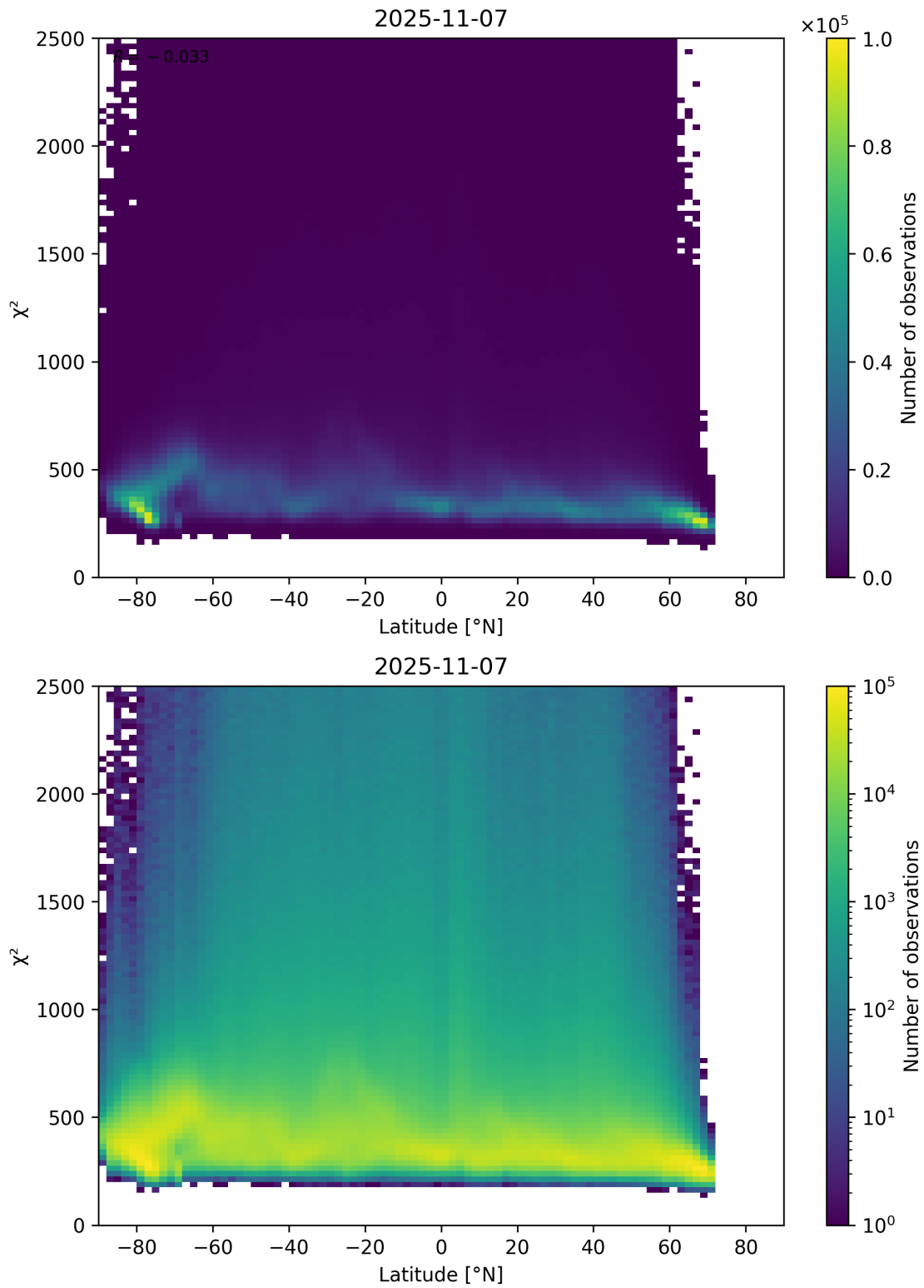
Figure 86: Scatter density plot of “Latitude” against “ \chi^2 ” for 2025-11-07 to 2025-11-08.
