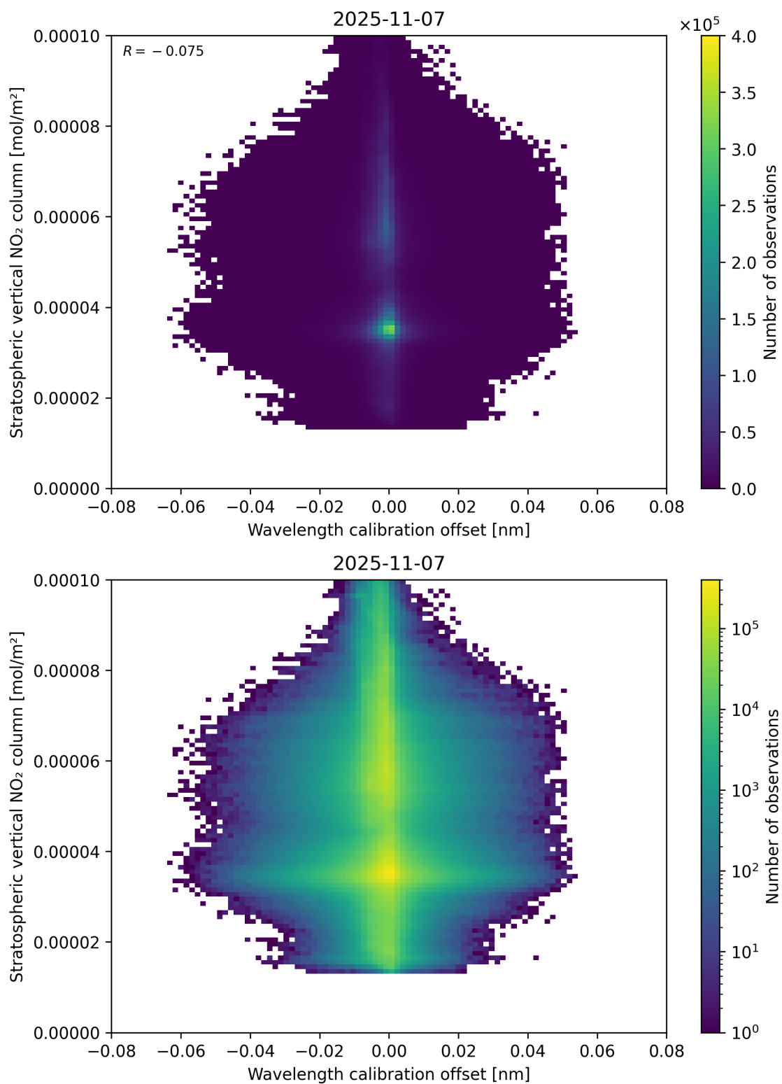
Figure 176: Scatter density plot of “Wavelength calibration offset” against “Stratospheric vertical NO 2 column” for 2025-11-07 to 2025-11-08.
