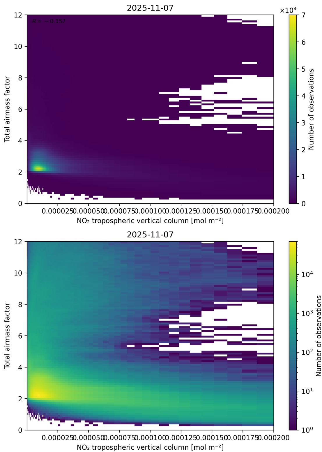
Figure 122: Scatter density plot of “NO 2 tropospheric vertical column” against “Total airmass factor” for 2025-11-07 to 2025-11-08.
