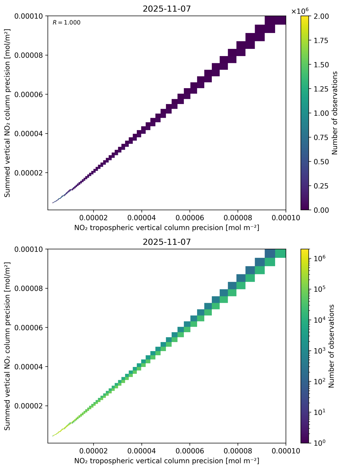
Figure 137: Scatter density plot of “NO 2 tropospheric vertical column precision” against “Summed vertical NO 2 column precision” for 2025-11-07 to 2025-11-08.
