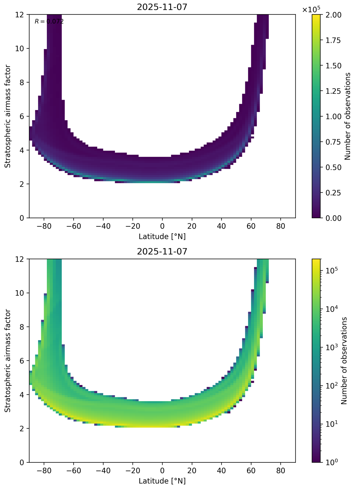
Figure 83: Scatter density plot of “Latitude” against “Stratospheric airmass factor” for 2025-11-07 to 2025-11-08.
