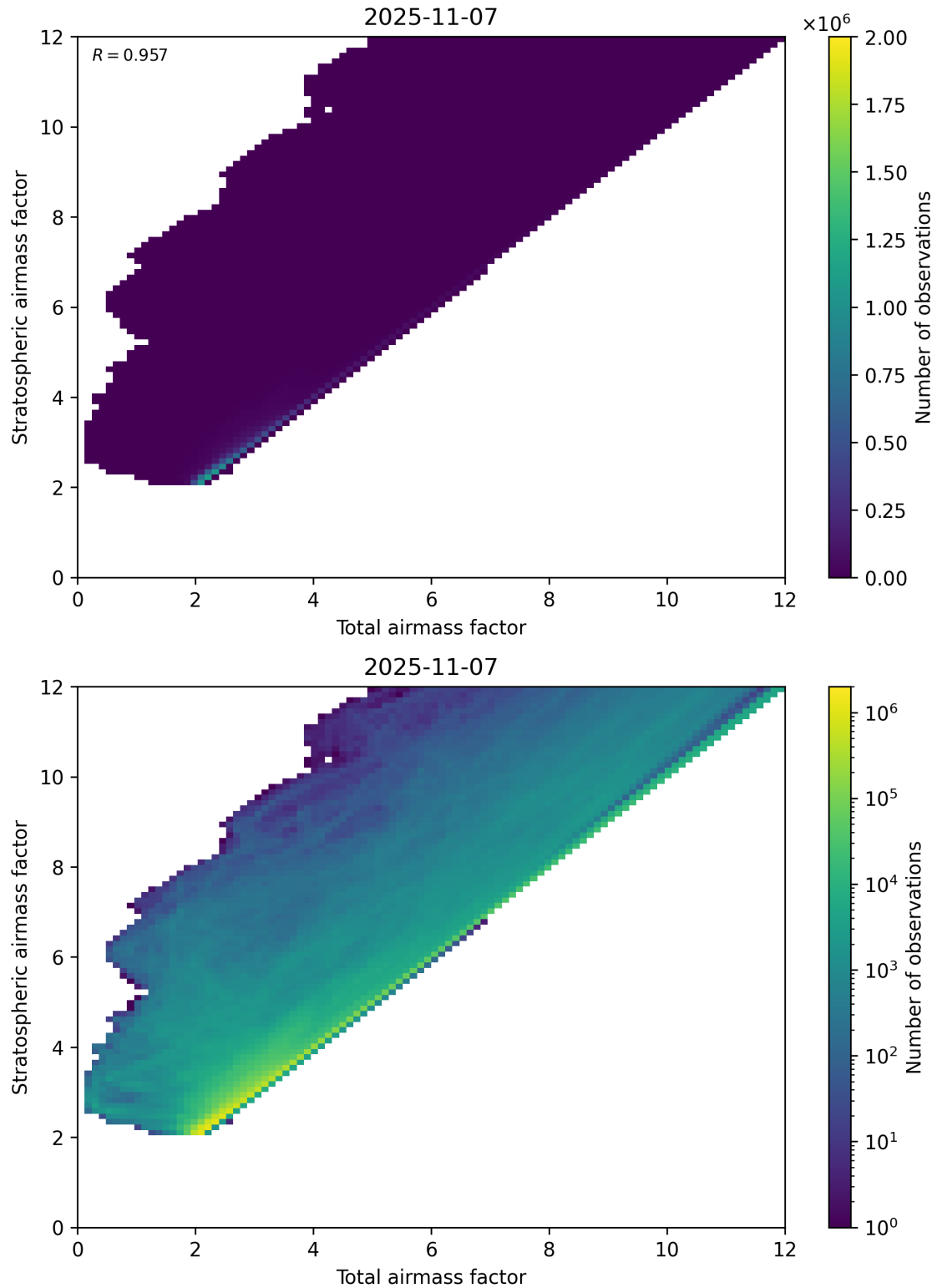
Figure 62: Scatter density plot of “Total airmass factor” against “Stratospheric airmass factor” for 2025-11-07 to 2025-11-08.
