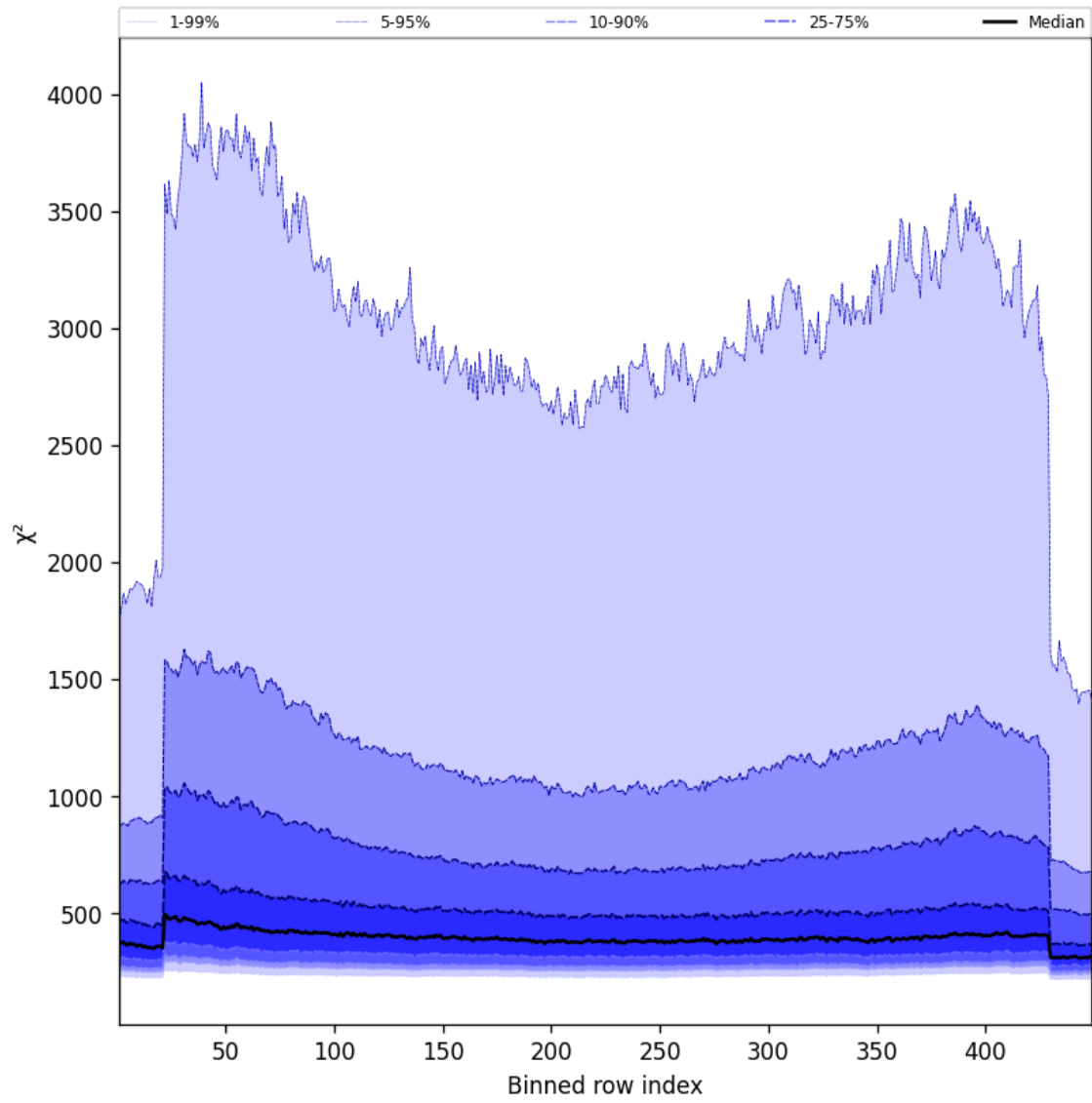
Figure 59: Along track statistics of “ \chi^2 ” for 2025-11-07 to 2025-11-08
