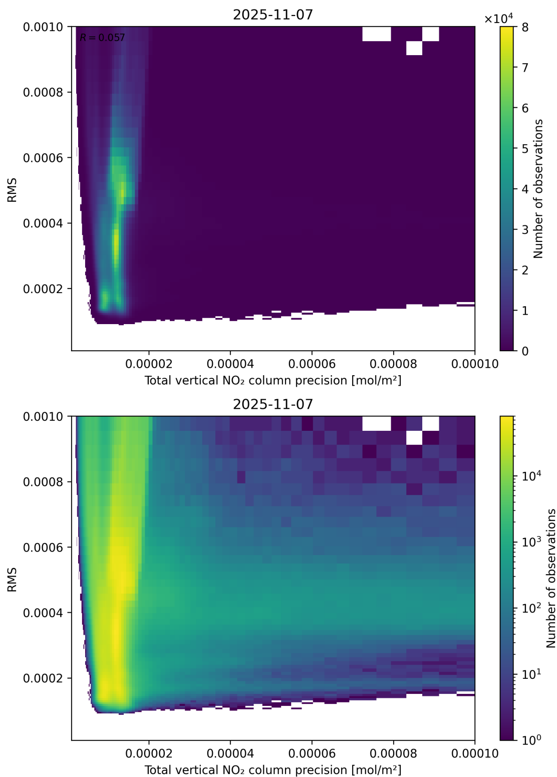
Figure 119: Scatter density plot of “Total vertical NO 2 column precision” against “RMS” for 2025-11-07 to 2025-11-08.
