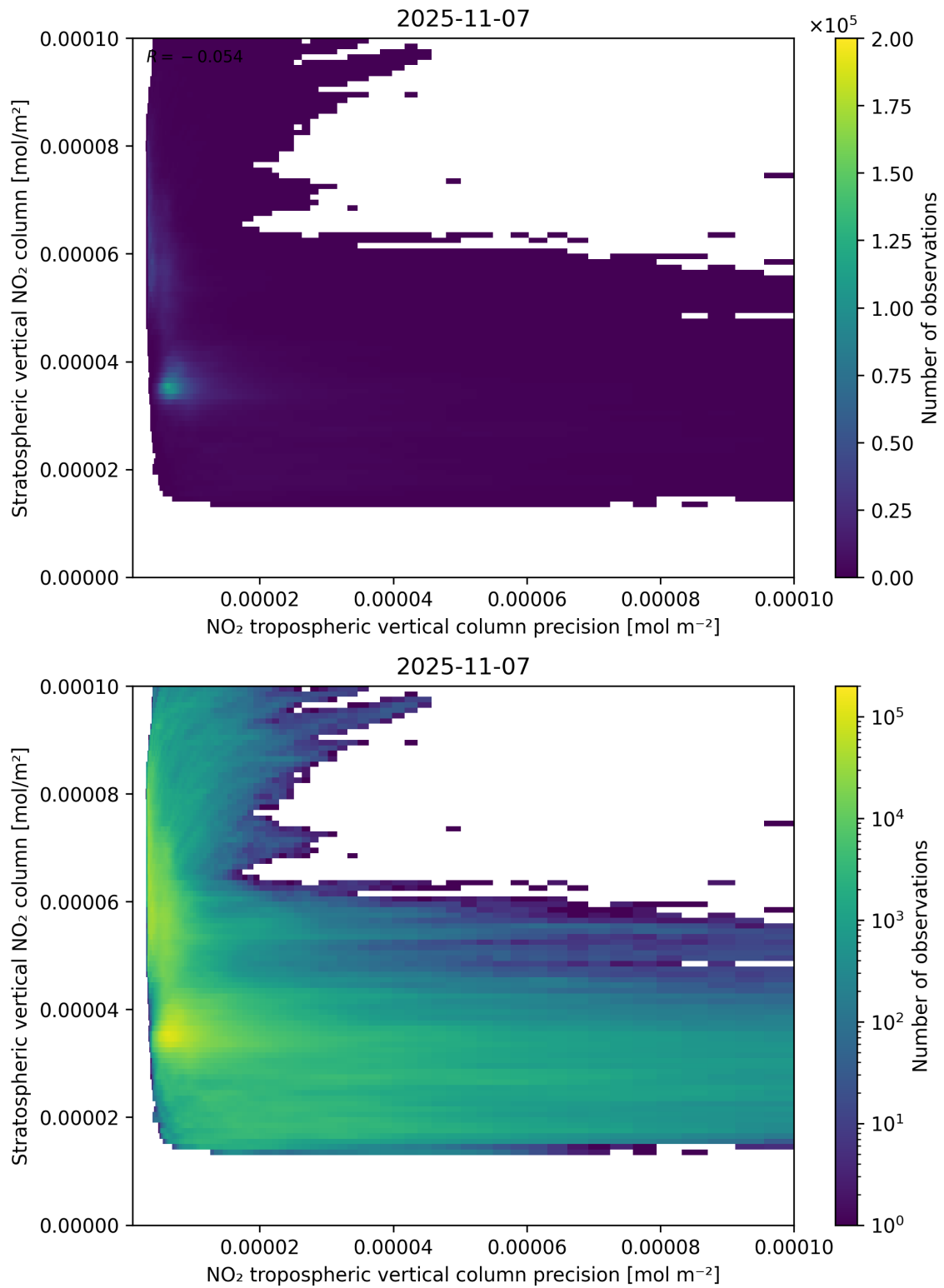
Figure 135: Scatter density plot of “NO 2 tropospheric vertical column precision” against “Stratospheric vertical NO 2 column” for 2025-11-07 to 2025-11-08.
