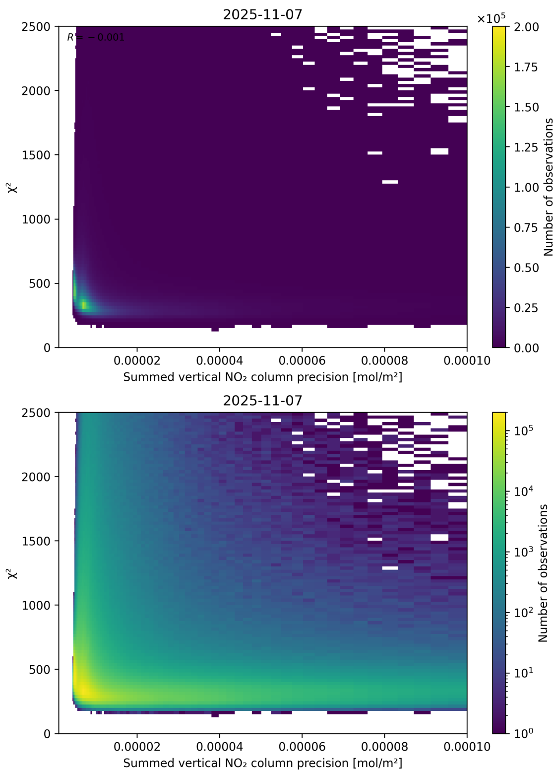
Figure 107: Scatter density plot of “Summed vertical NO 2 column precision” against “ \chi^2 ” for 2025-11-07 to 2025-11-08.
