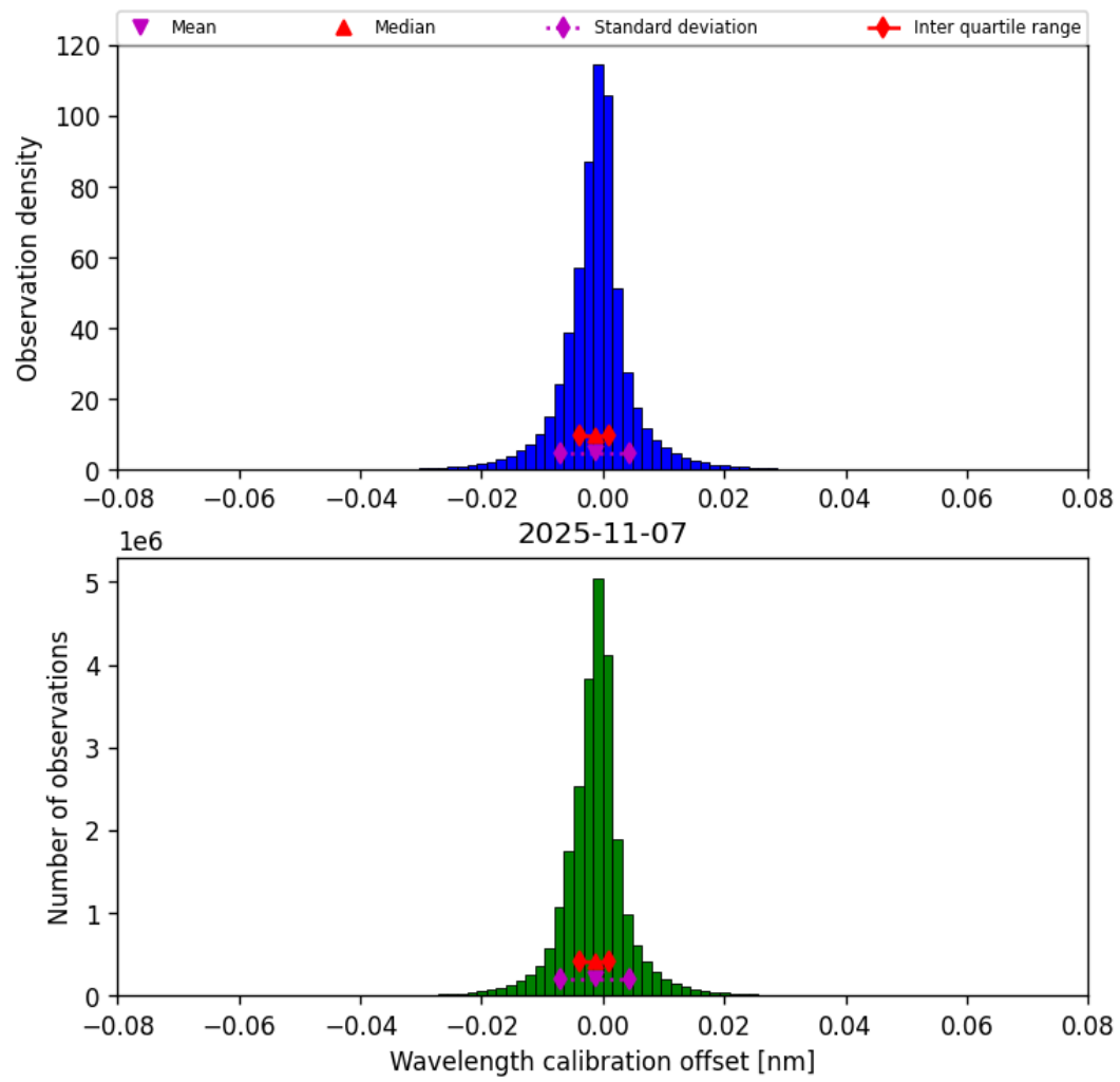
Figure 35: Histogram of “Wavelength calibration offset” for 2025-11-07 to 2025-11-08
