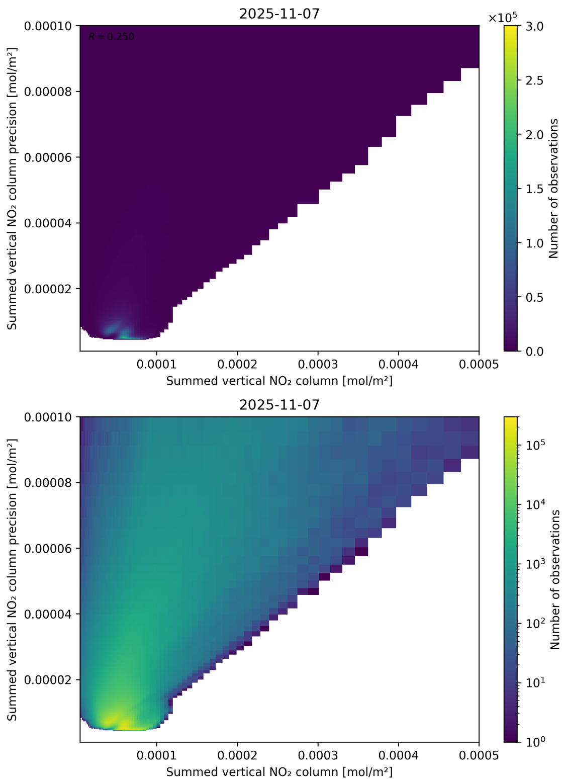
Figure 105: Scatter density plot of “Summed vertical NO 2 column” against “Summed vertical NO 2 column precision” for 2025-11-07 to 2025-11-08.
