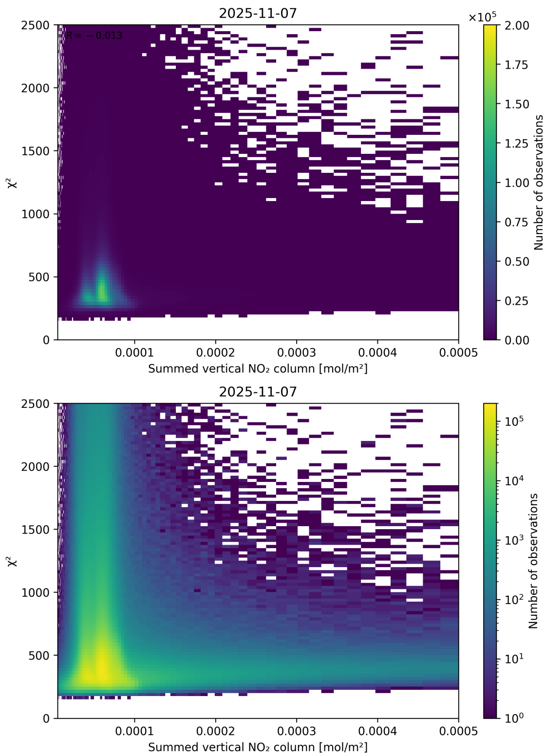
Figure 104: Scatter density plot of “Summed vertical NO 2 column” against “ \chi^2 ” for 2025-11-07 to 2025-11-08.
