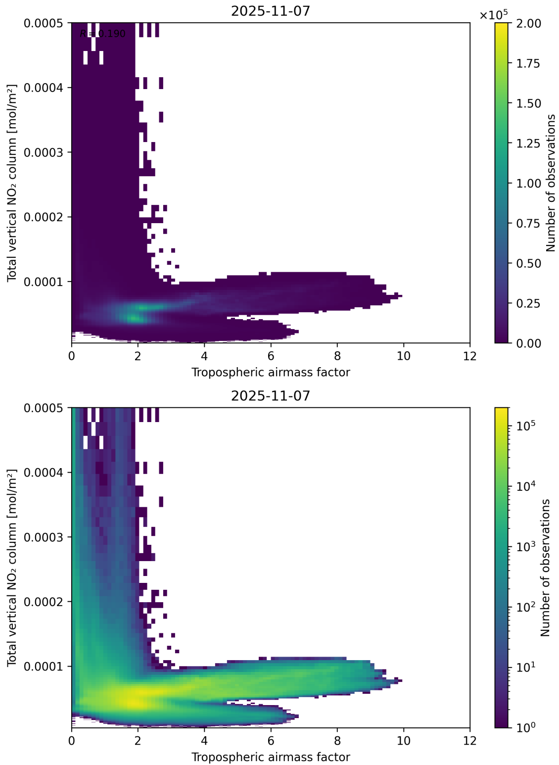
Figure 77: Scatter density plot of “Tropospheric airmass factor” against “Total vertical NO 2 column” for 2025-11-07 to 2025-11-08.
