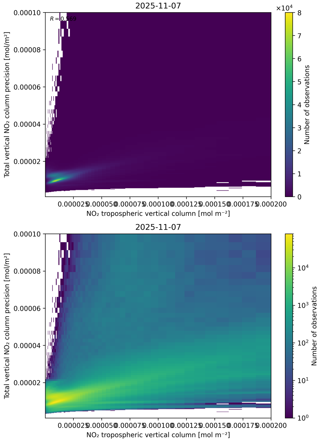
Figure 129: Scatter density plot of “NO 2 tropospheric vertical column” against “Total vertical NO 2 column precision” for 2025-11-07 to 2025-11-08.
