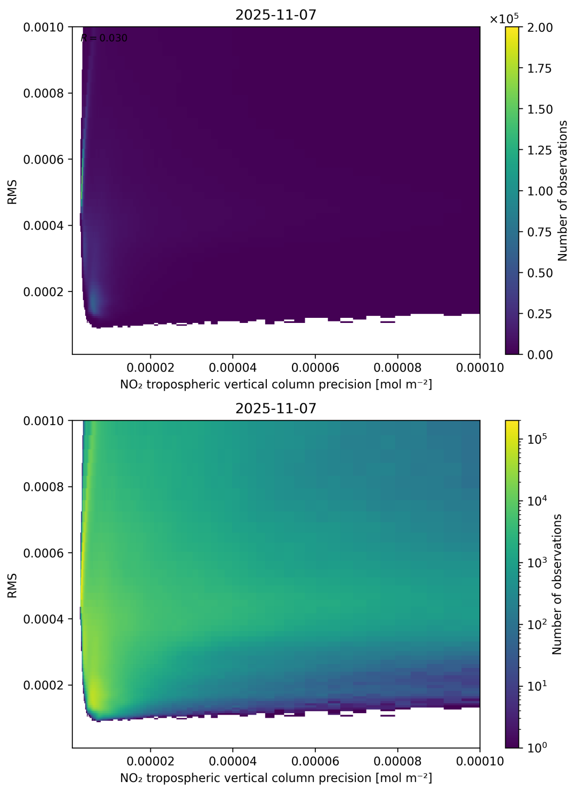
Figure 140: Scatter density plot of “NO 2 tropospheric vertical column precision” against “RMS” for 2025-11-07 to 2025-11-08.
