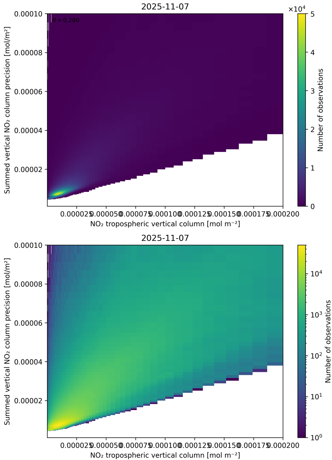
Figure 127: Scatter density plot of “NO 2 tropospheric vertical column” against “Summed vertical NO 2 column precision” for 2025-11-07 to 2025-11-08.
