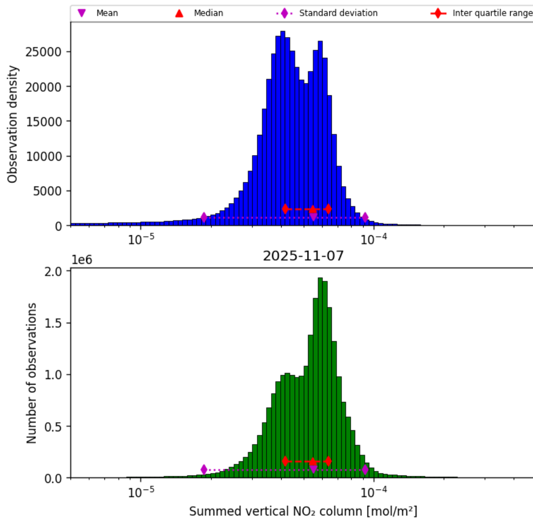
Figure 40: Histogram of “Summed vertical NO 2 column” for 2025-11-07 to 2025-11-08
