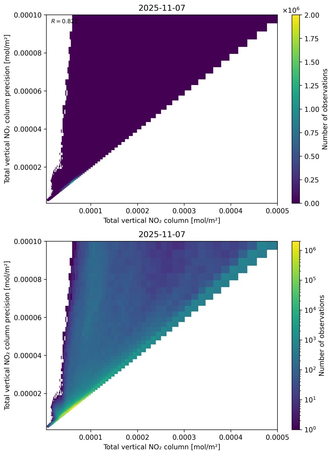
Figure 114: Scatter density plot of “Total vertical NO 2 column” against “Total vertical NO 2 column precision” for 2025-11-07 to 2025-11-08.
