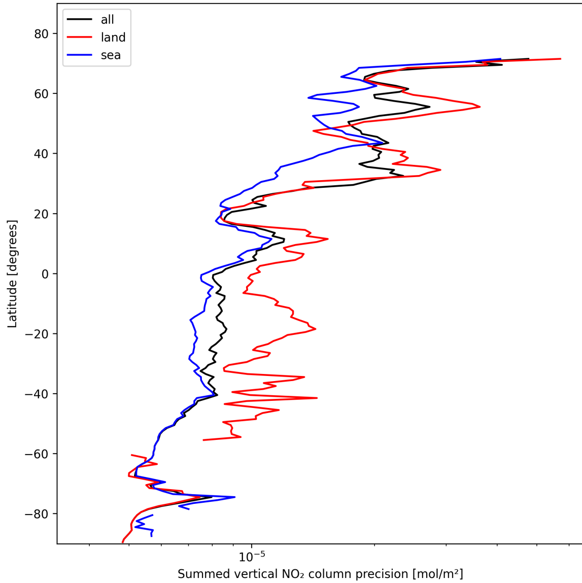
Figure 24: Zonal average of “Summed vertical NO 2 column precision” for 2025-11-07 to 2025-11-08.
