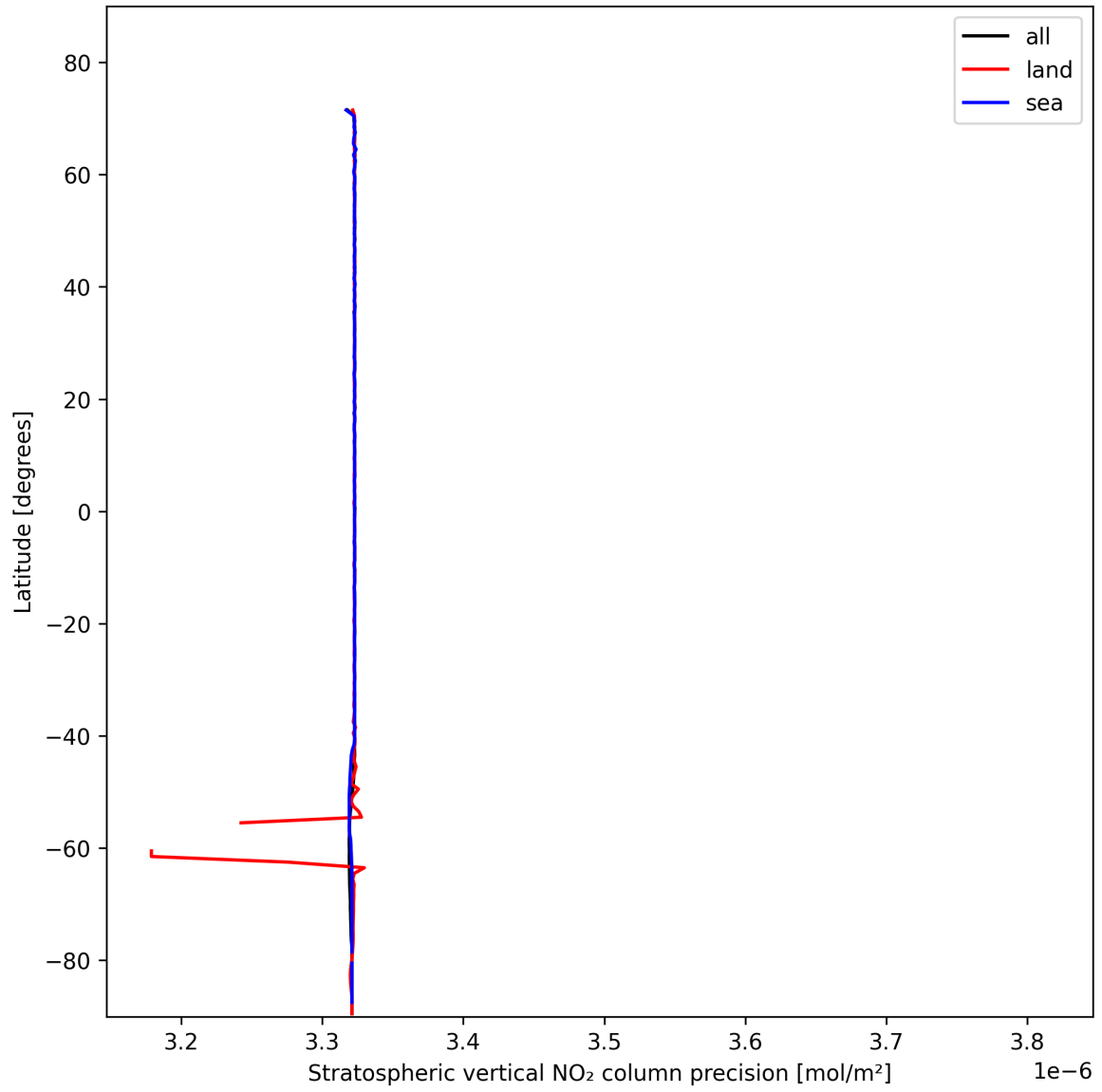
Figure 20: Zonal average of “Stratospheric vertical NO 2 column precision” for 2025-11-07 to 2025-11-08.
