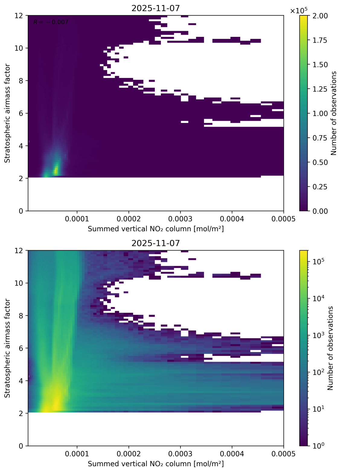
Figure 103: Scatter density plot of “Summed vertical NO 2 column” against “Stratospheric airmass factor” for 2025-11-07 to 2025-11-08.
