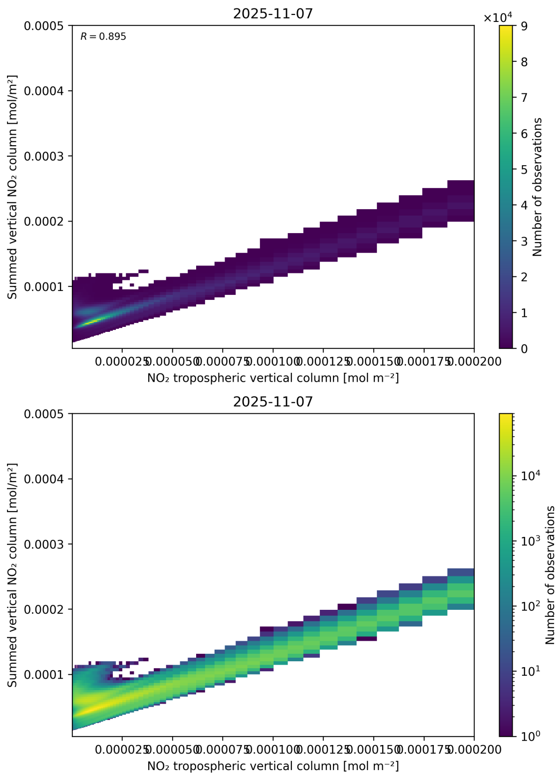
Figure 126: Scatter density plot of “NO 2 tropospheric vertical column” against “Summed vertical NO 2 column” for 2025-11-07 to 2025-11-08.
