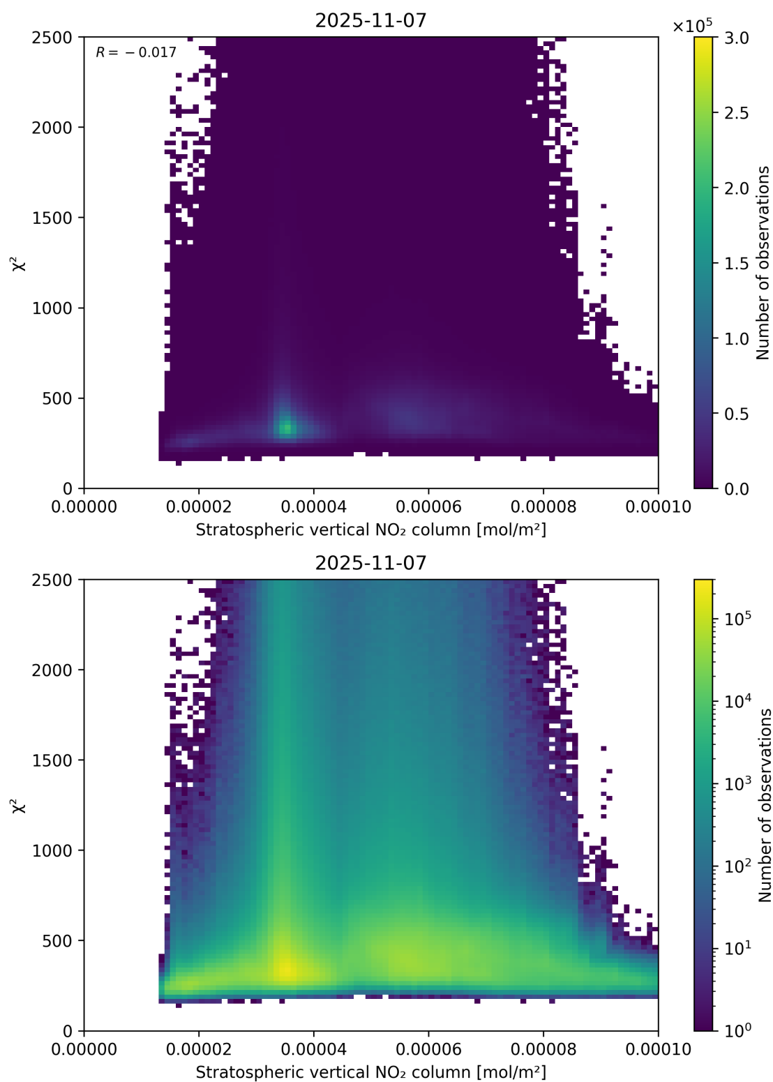
Figure 97: Scatter density plot of “Stratospheric vertical NO 2 column” against “ \chi^2 ” for 2025-11-07 to 2025-11-08.
