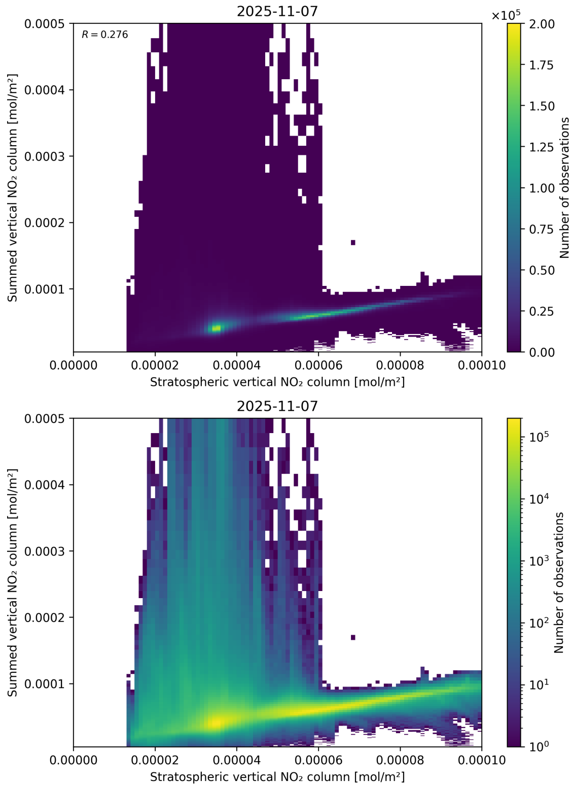
Figure 98: Scatter density plot of “Stratospheric vertical NO 2 column” against “Summed vertical NO 2 column” for 2025-11-07 to 2025-11-08.
