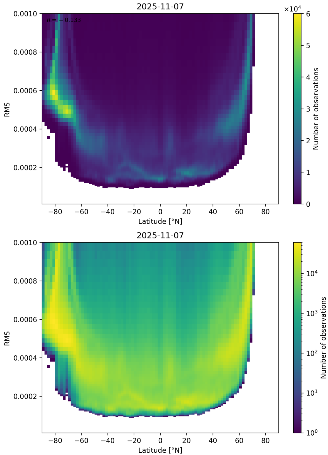
Figure 94: Scatter density plot of “Latitude” against “RMS” for 2025-11-07 to 2025-11-08.
