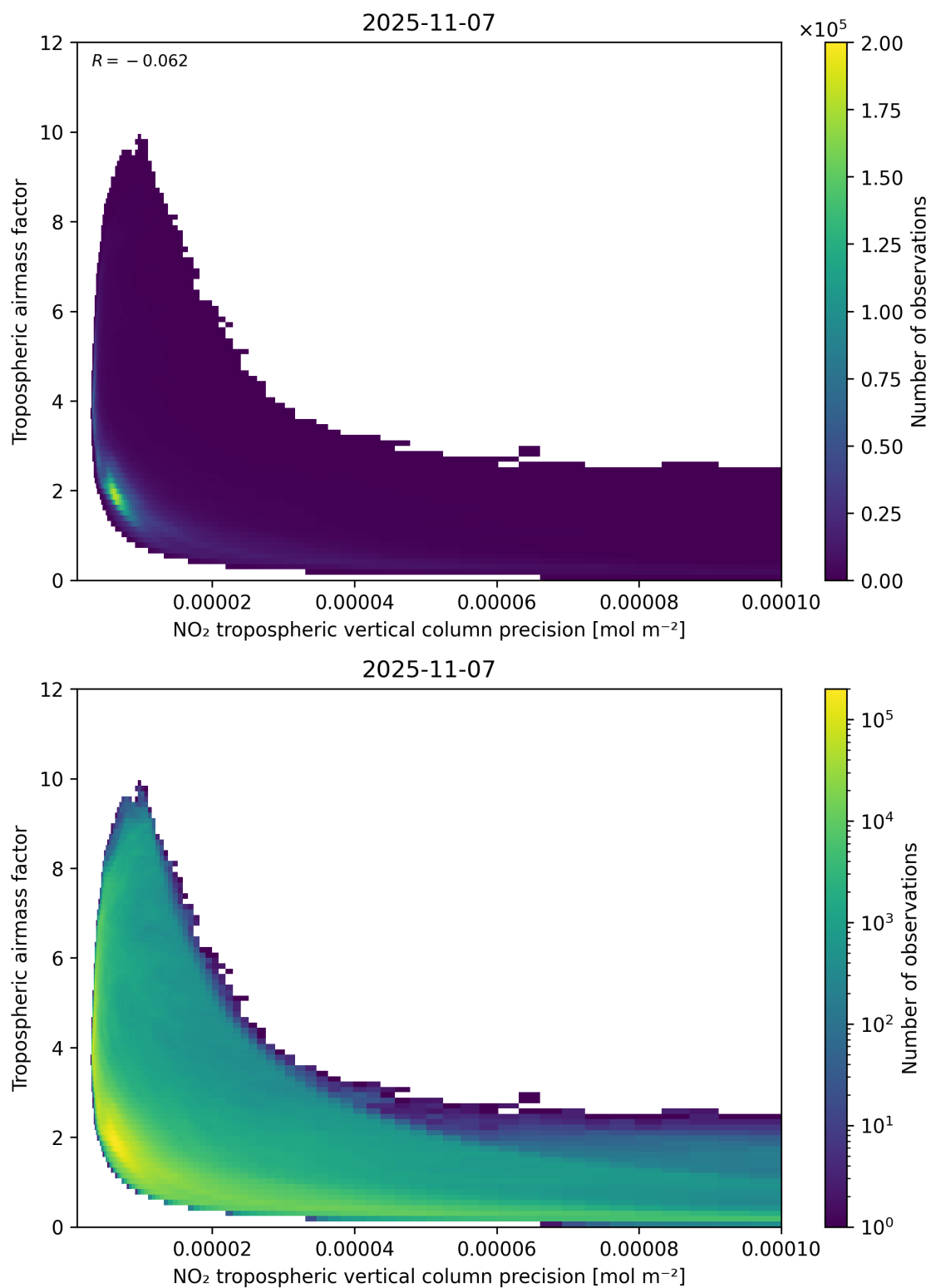
Figure 133: Scatter density plot of “NO 2 tropospheric vertical column precision” against “Tropospheric airmass factor” for 2025-11-07 to 2025-11-08.
