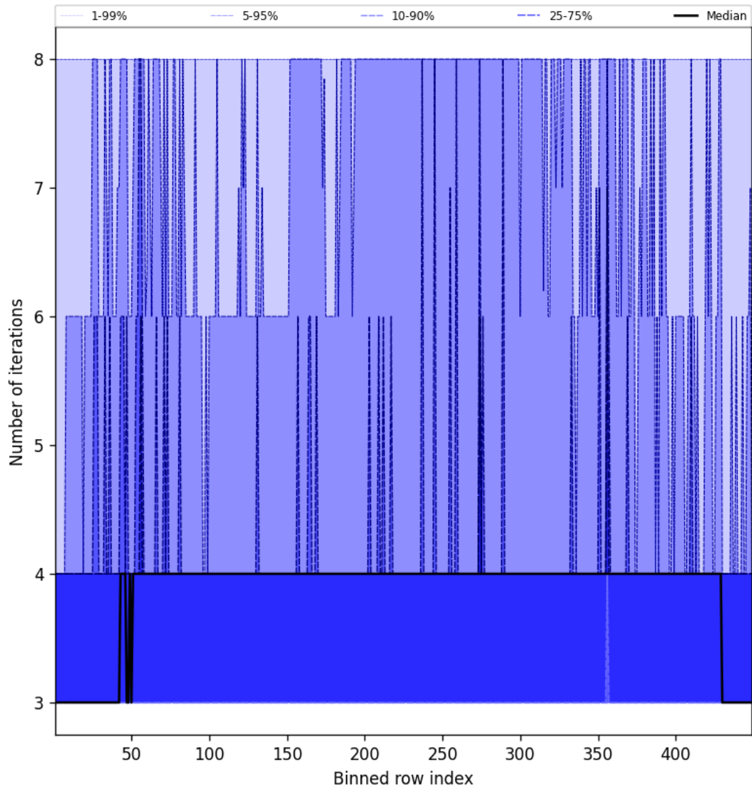
Figure 51: Along track statistics of “Number of iterations” for 2025-11-07 to 2025-11-08
