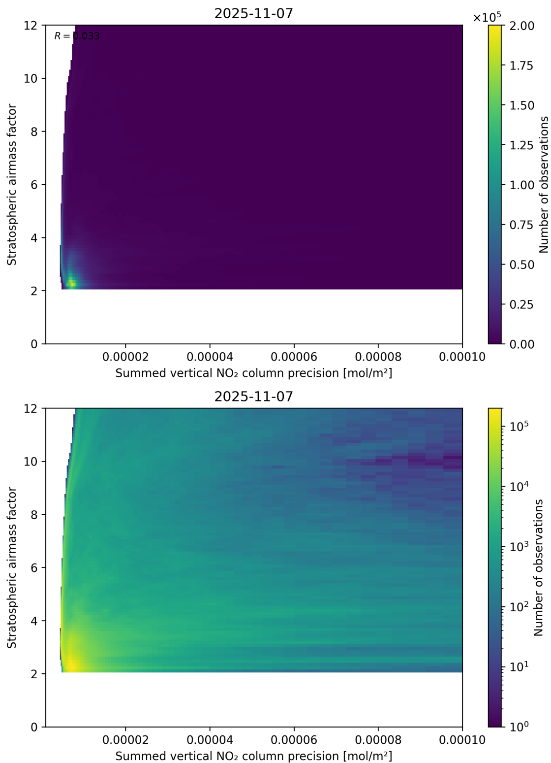
Figure 106: Scatter density plot of “Summed vertical NO 2 column precision” against “Stratospheric airmass factor” for 2025-11-07 to 2025-11-08.
