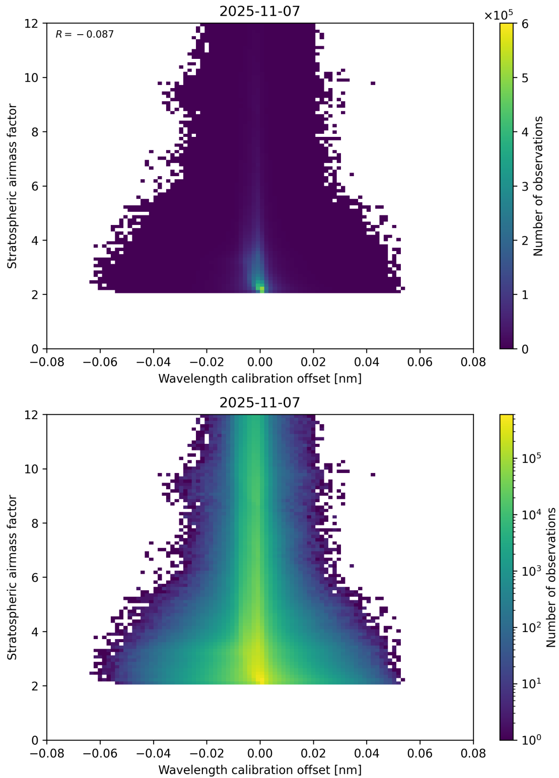
Figure 174: Scatter density plot of “Wavelength calibration offset” against “Stratospheric airmass factor” for 2025-11-07 to 2025-11-08.
