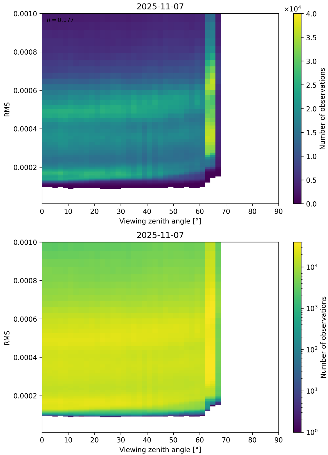
Figure 171: Scatter density plot of “Viewing zenith angle” against “RMS” for 2025-11-07 to 2025-11-08.
