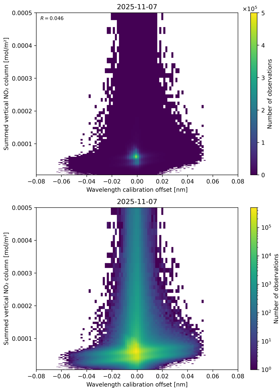
Figure 177: Scatter density plot of “Wavelength calibration offset” against “Summed vertical NO 2 column” for 2025-11-07 to 2025-11-08.
