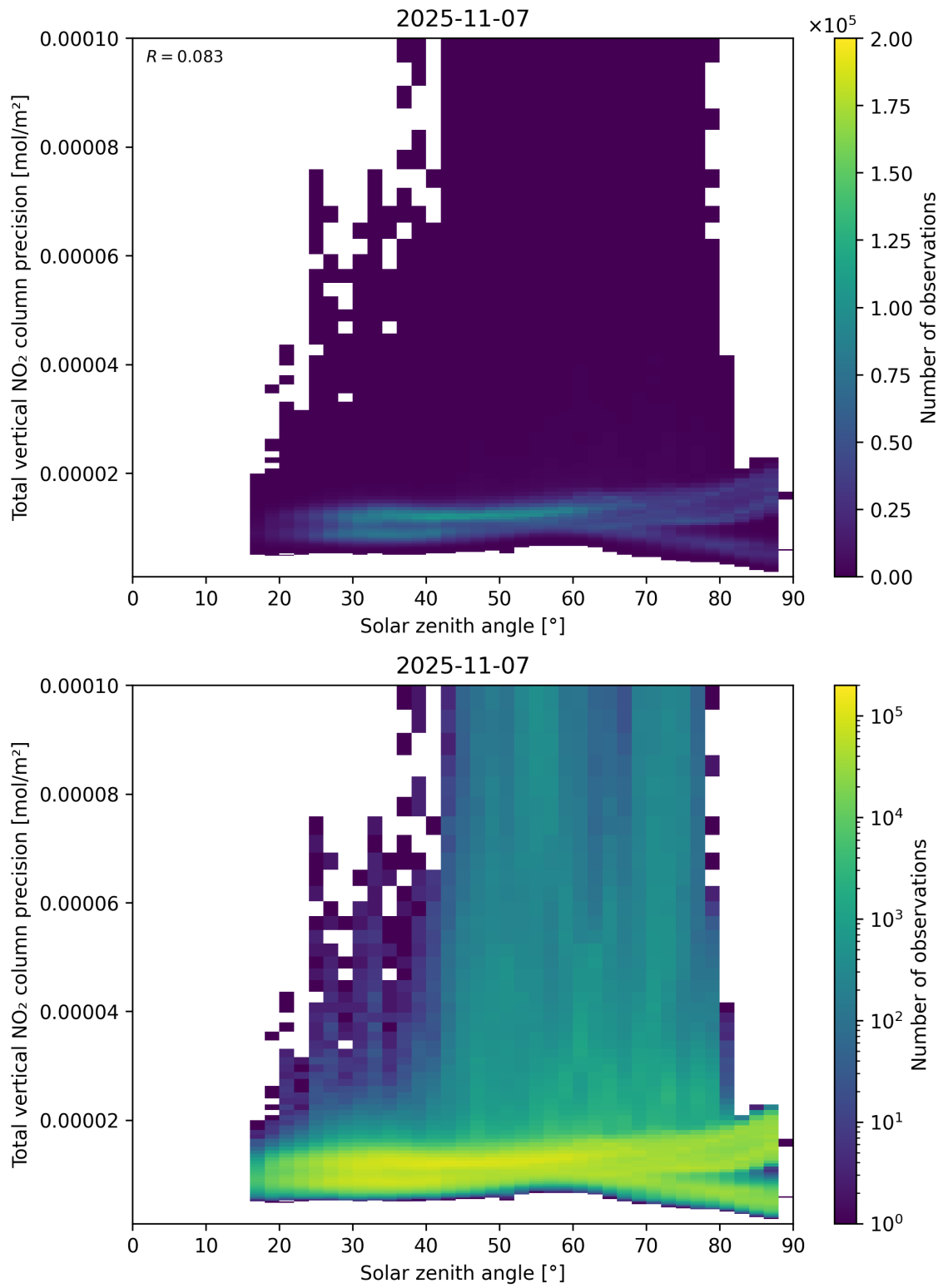
Figure 154: Scatter density plot of “Solar zenith angle” against “Total vertical NO 2 column precision” for 2025-11-07 to 2025-11-08.
