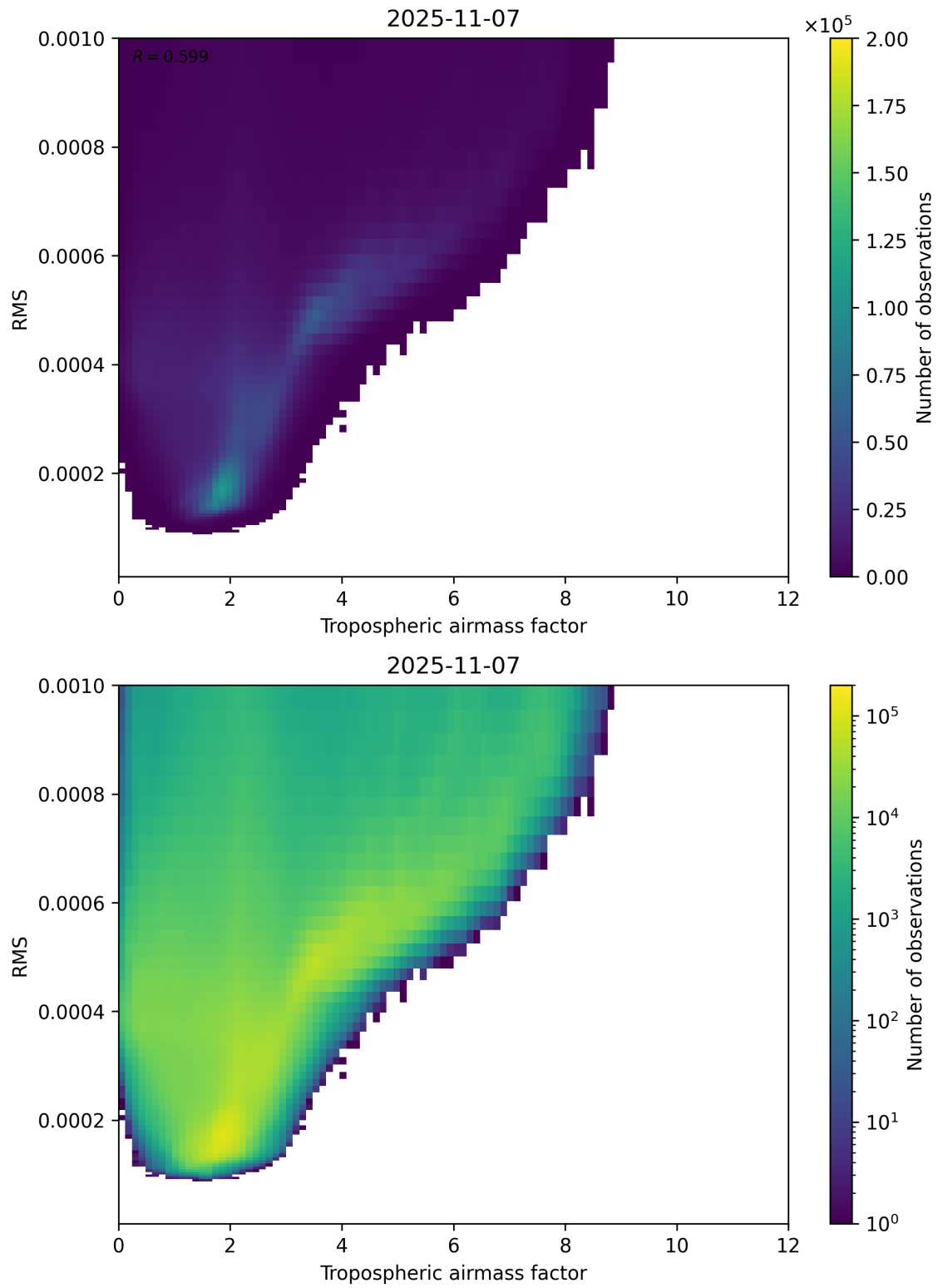
Figure 79: Scatter density plot of “Tropospheric airmass factor” against “RMS” for 2025-11-07 to 2025-11-08.
