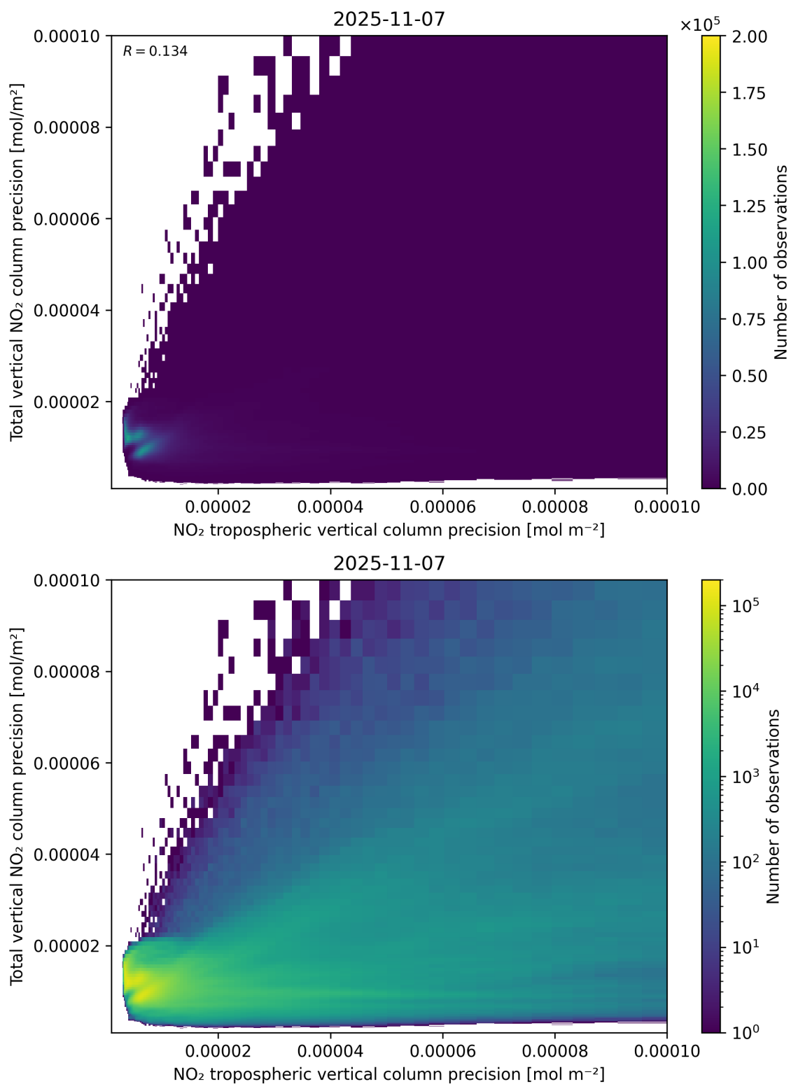
Figure 139: Scatter density plot of “NO 2 tropospheric vertical column precision” against “Total vertical NO 2 column precision” for 2025-11-07 to 2025-11-08.
