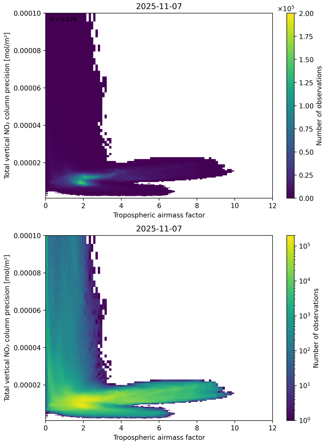
Figure 78: Scatter density plot of “Tropospheric air mass factor” against “Total vertical NO 2 column precision” for 2025-11-07 to 2025-11-08.
