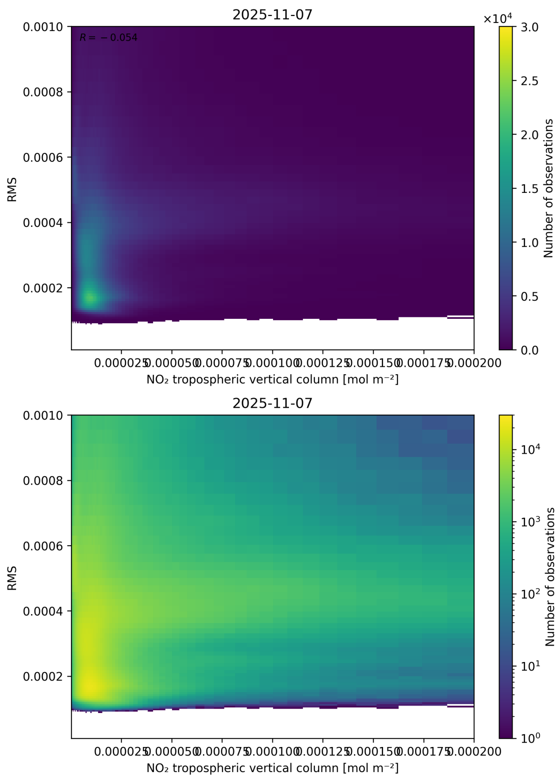
Figure 142: Scatter density plot of “NO 2 tropospheric vertical column” against “RMS” for 2025-11-07 to 2025-11-08.
