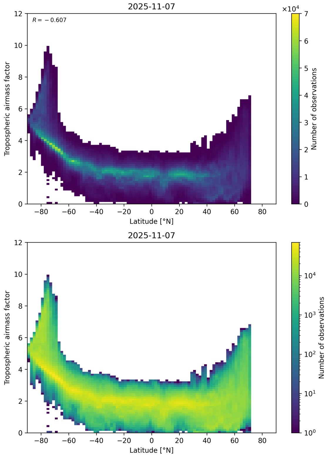
Figure 85: Scatter density plot of “Latitude” against “Tropospheric airmass factor” for 2025-11-07 to 2025-11-08.
