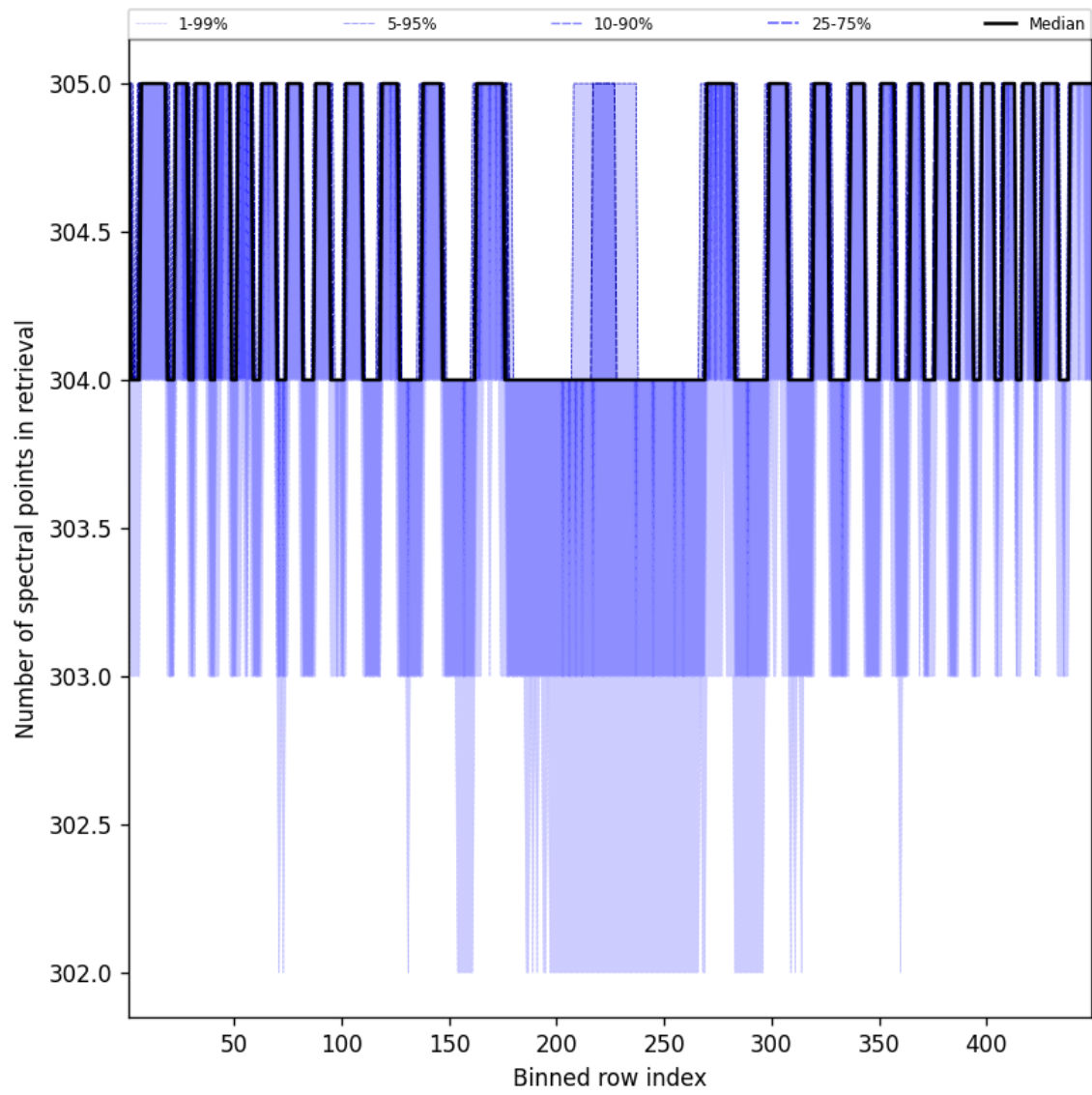
Figure 50: Along track statistics of “Number of spectral points in retrieval” for 2025-11-07 to 2025-11-08
