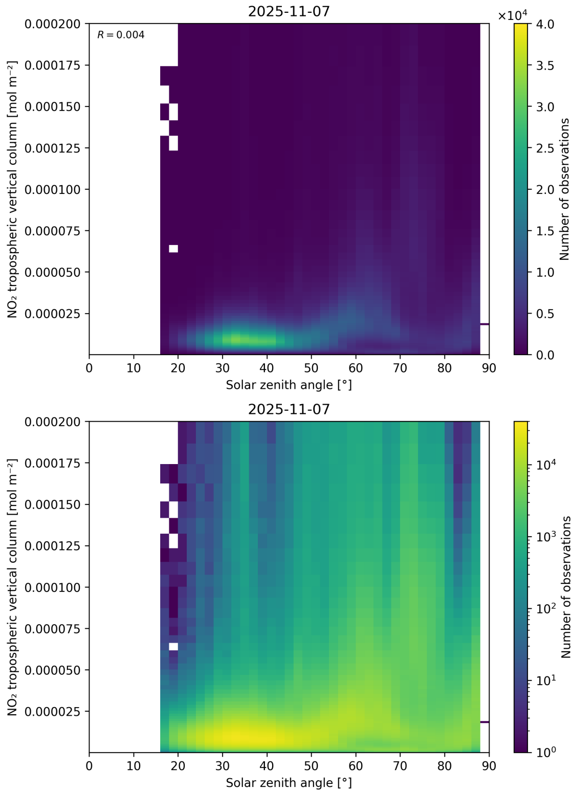
Figure 155: Scatter density plot of “Solar zenith angle” against “NO 2 tropospheric vertical column” for 2025-11-07 to 2025-11-08.
