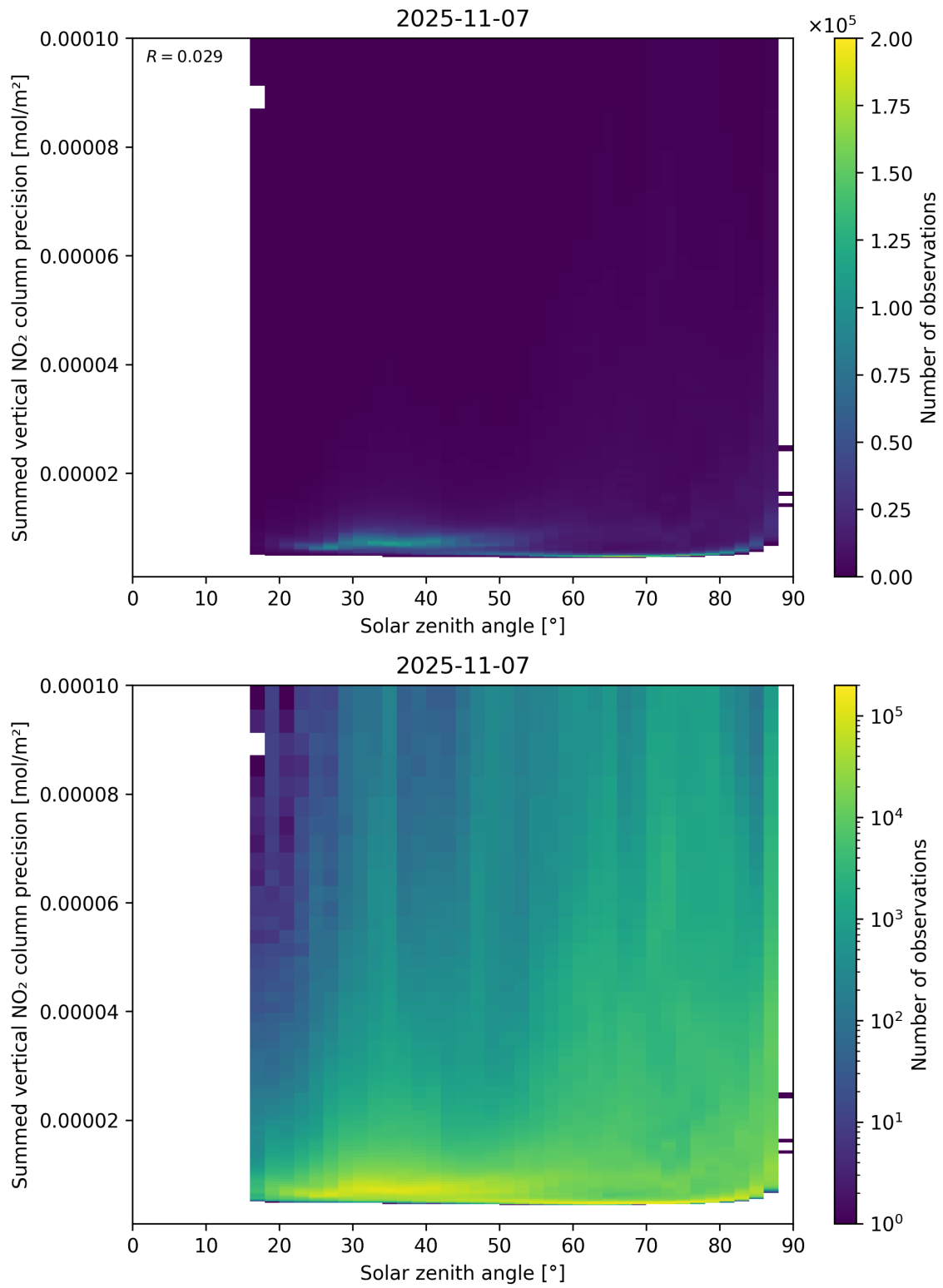
Figure 152: Scatter density plot of “Solar zenith angle” against “Summed vertical NO 2 column precision” for 2025-11-07 to 2025-11-08.
