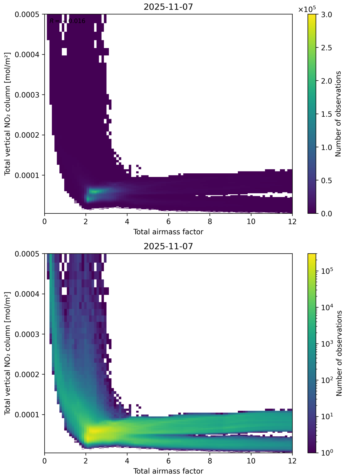
Figure 67: Scatter density plot of “Total airmass factor” against “Total vertical NO 2 column” for 2025-11-07 to 2025-11-08.
