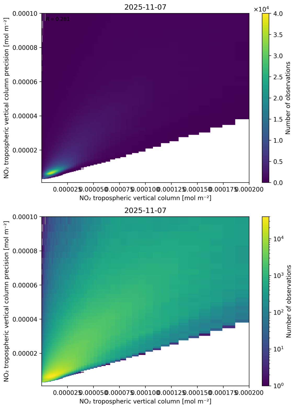
Figure 130: Scatter density plot of “NO 2 tropospheric vertical column” against “NO 2 tropospheric vertical column precision” for 2025-11-07 to 2025-11-08.
