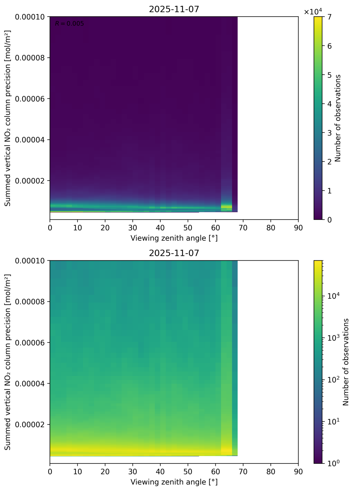
Figure 166: Scatter density plot of “Viewing zenith angle” against “Summed vertical NO 2 column precision” for 2025-11-07 to 2025-11-08.
