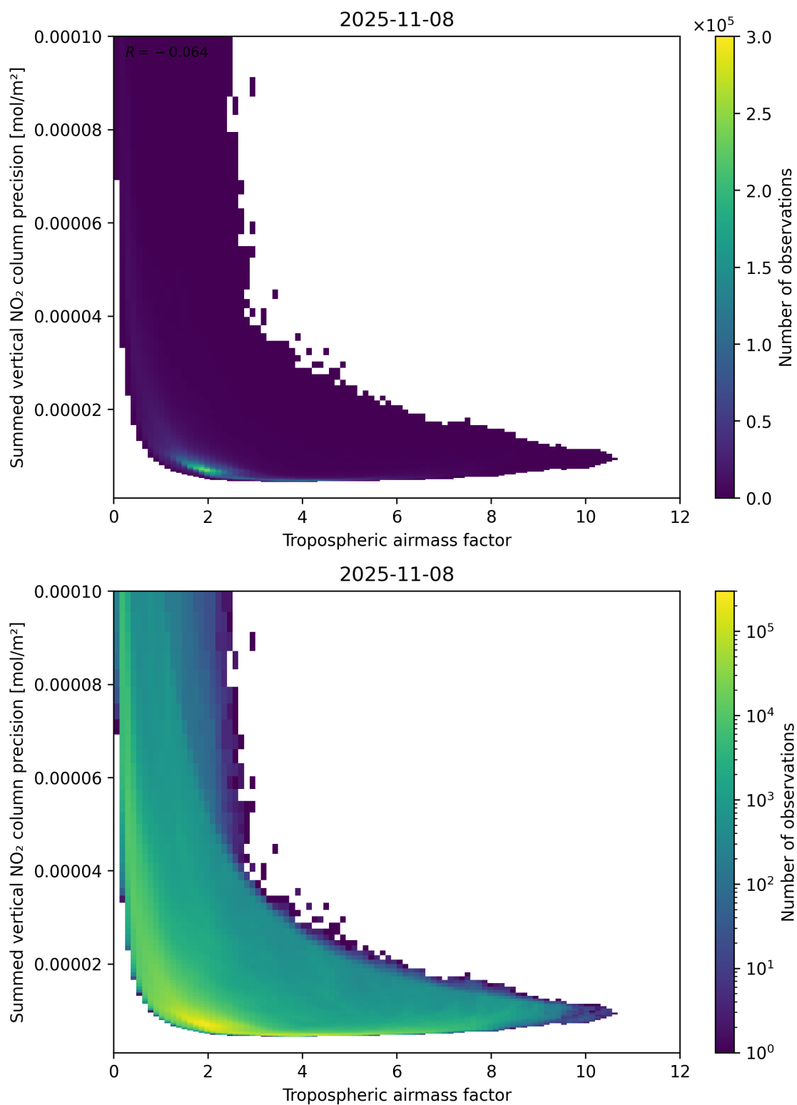
Figure 76: Scatter density plot of “Tropospheric air mass factor” against “Summed vertical NO 2 column precision” for 2025-11-07 to 2025-11-09.
