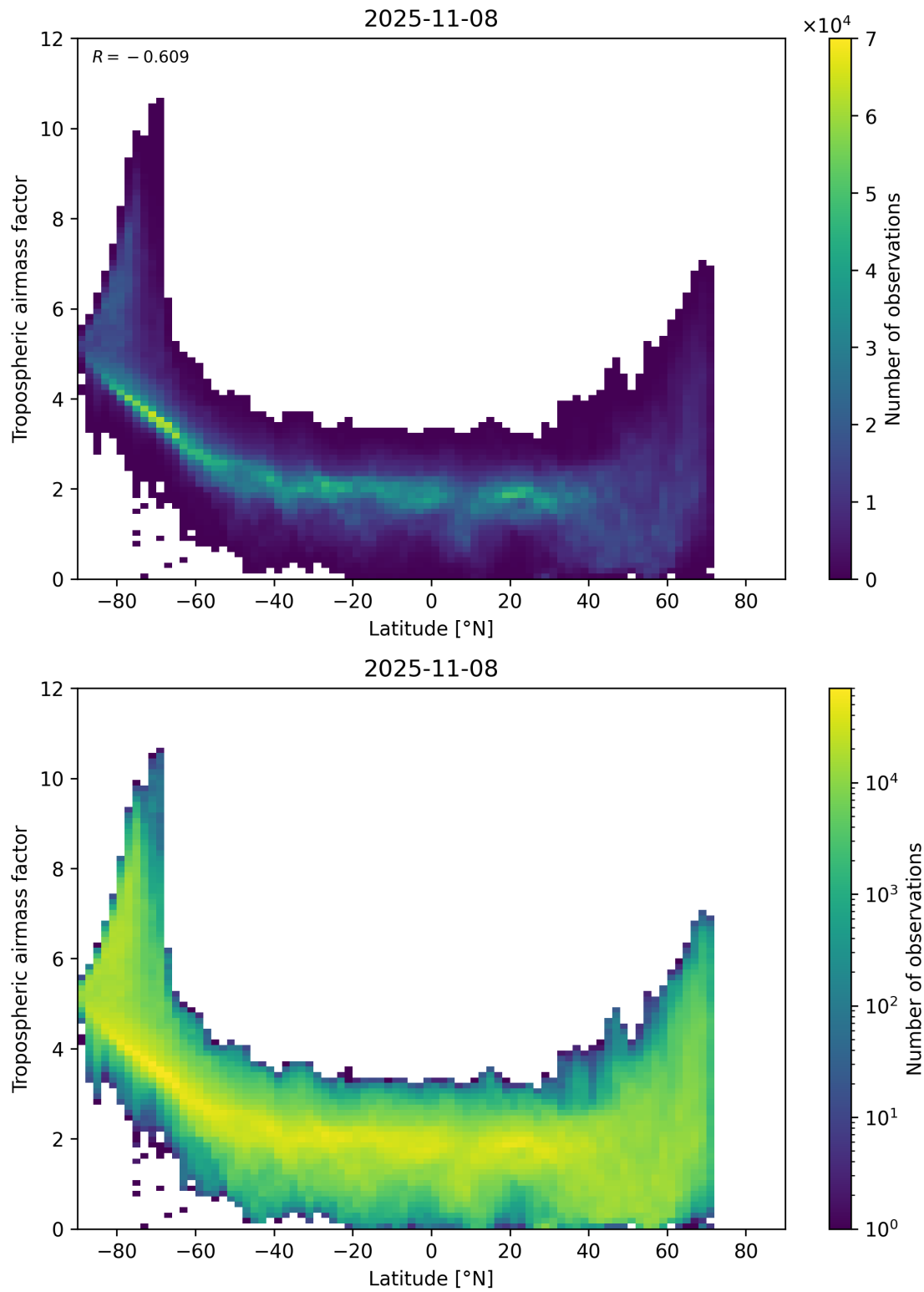
Figure 85: Scatter density plot of “Latitude” against “Tropospheric air mass factor” for 2025-11-07 to 2025-11-09.
