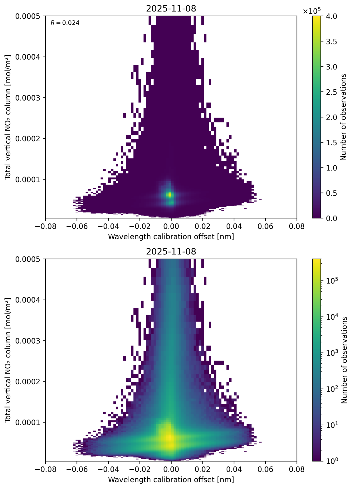
Figure 179: Scatter density plot of “Wavelength calibration offset” against “Total vertical NO 2 column” for 2025-11-07 to 2025-11-09.
