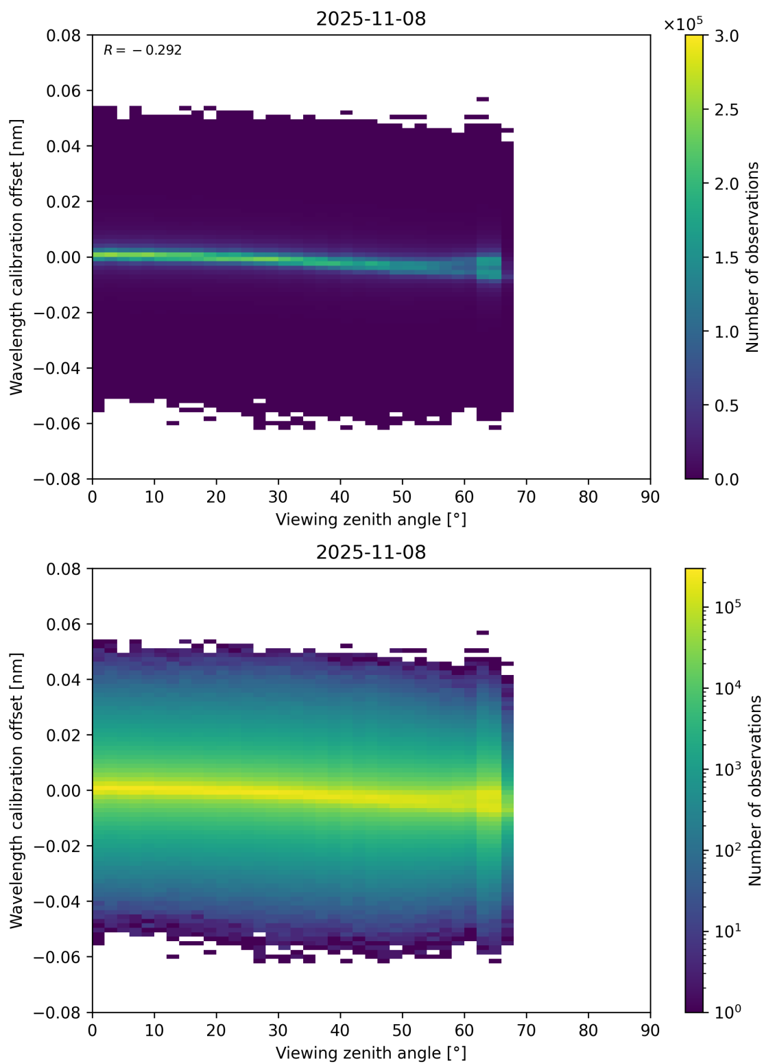
Figure 173: Scatter density plot of “Viewing zenith angle” against “Wavelength calibration offset” for 2025-11-07 to 2025-11-09.
