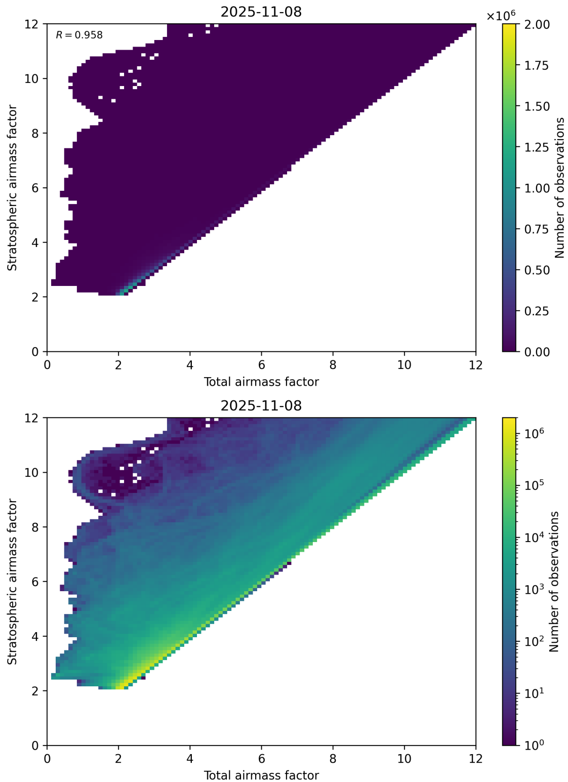
Figure 62: Scatter density plot of “Total airmass factor” against “Stratospheric airmass factor” for 2025-11-07 to 2025-11-09.
