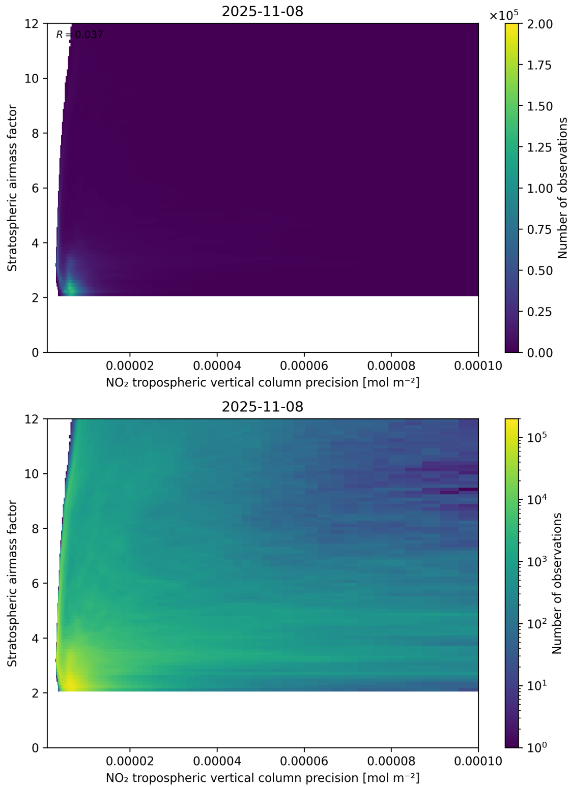
Figure 131: Scatter density plot of “NO 2 tropospheric vertical column precision” against “Stratospheric airmass factor” for 2025-11-07 to 2025-11-09.
