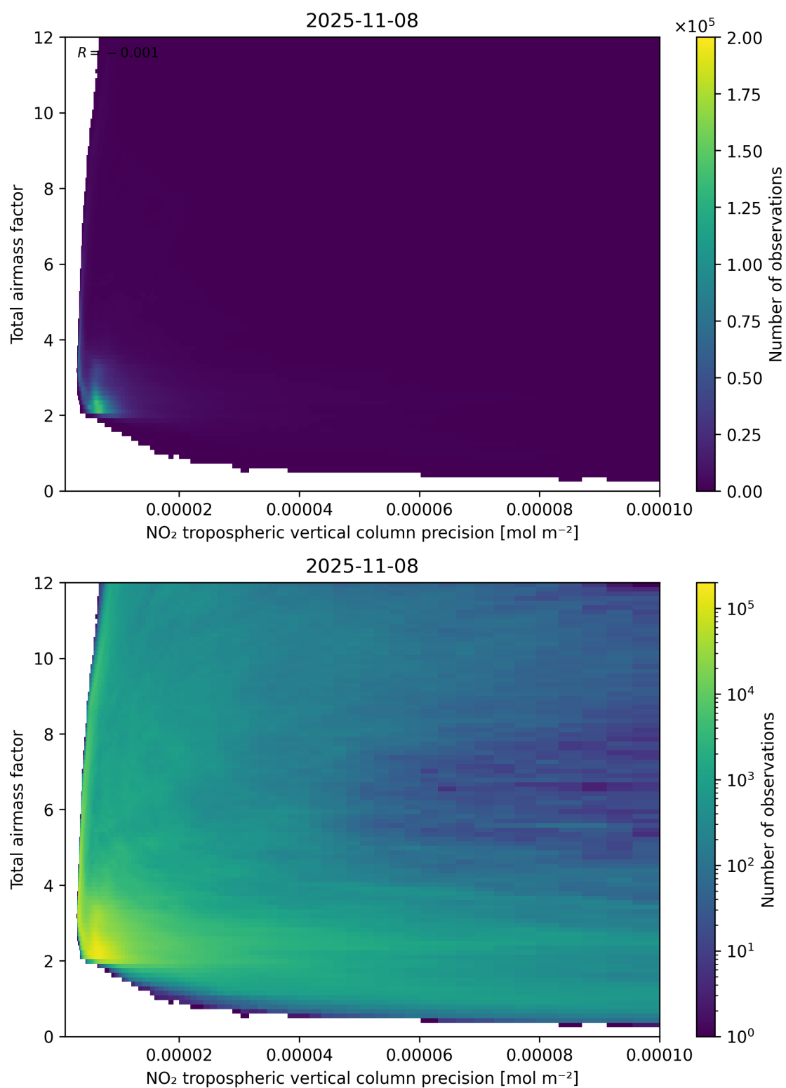
Figure 132: Scatter density plot of “NO 2 tropospheric vertical column precision” against “Total air mass factor” for 2025-11-07 to 2025-11-09.
