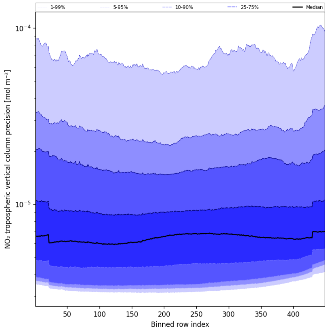
Figure 47: Along track statistics of “NO 2 tropospheric vertical column precision” for 2025-11-07 to 2025-11-09
