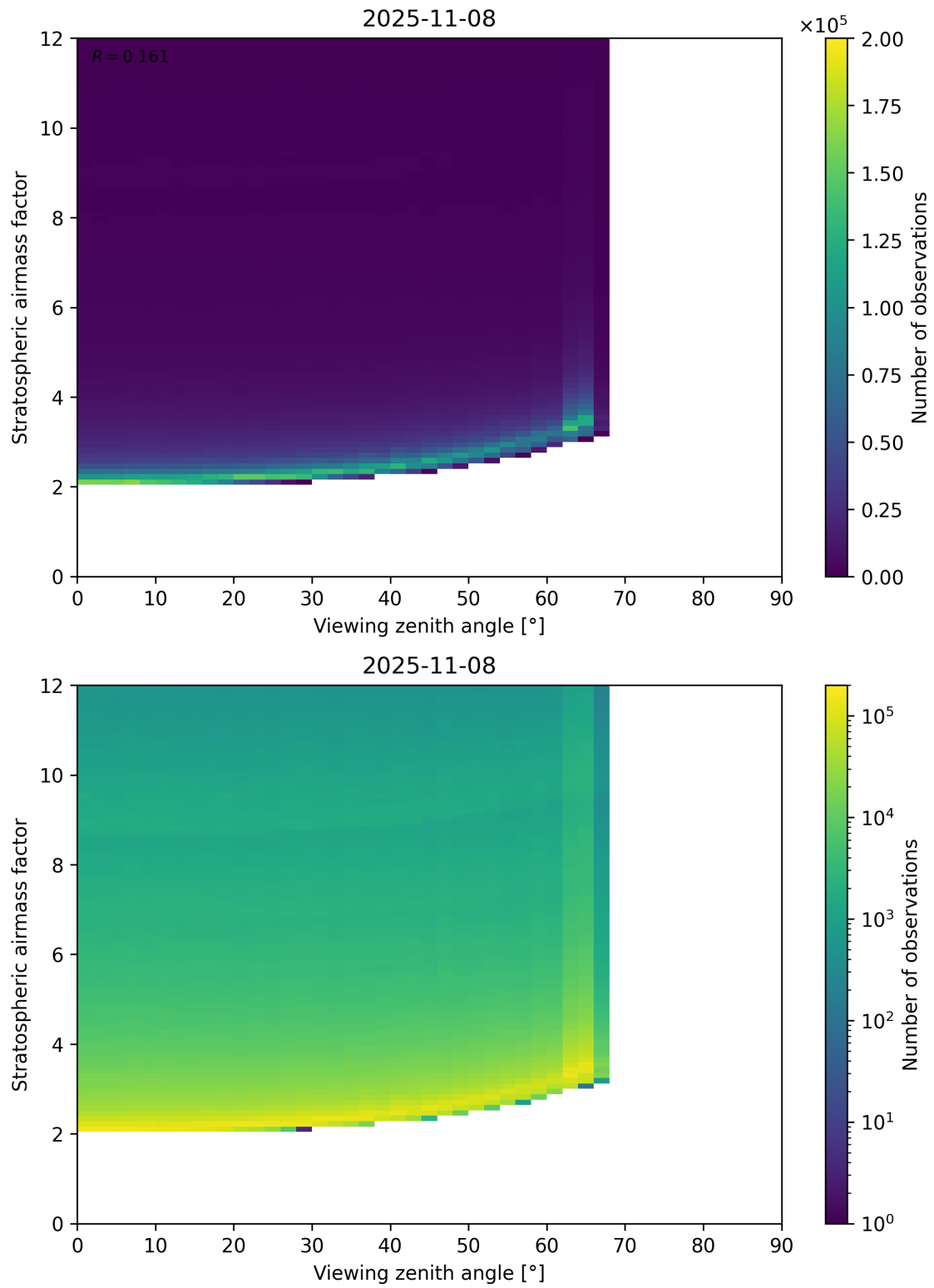
Figure 159: Scatter density plot of “Viewing zenith angle” against “Stratospheric airmass factor” for 2025-11-07 to 2025-11-09.
