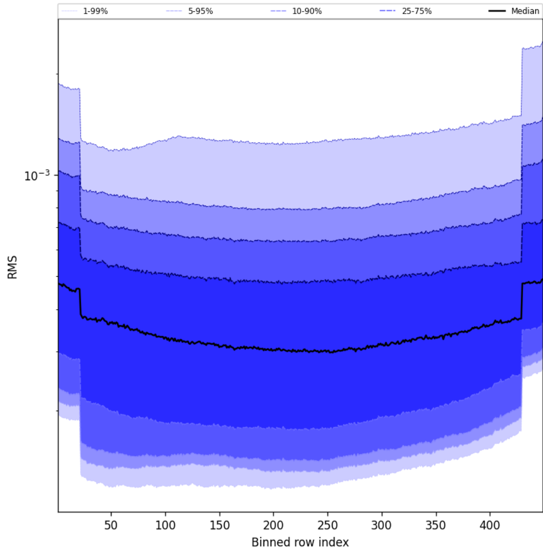
Figure 60: Along track statistics of “RMS” for 2025-11-07 to 2025-11-09
