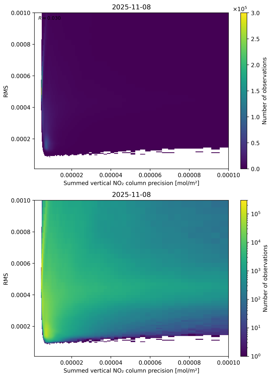
Figure 108: Scatter density plot of “Summed vertical NO 2 column precision” against “RMS” for 2025-11-07 to 2025-11-09.
