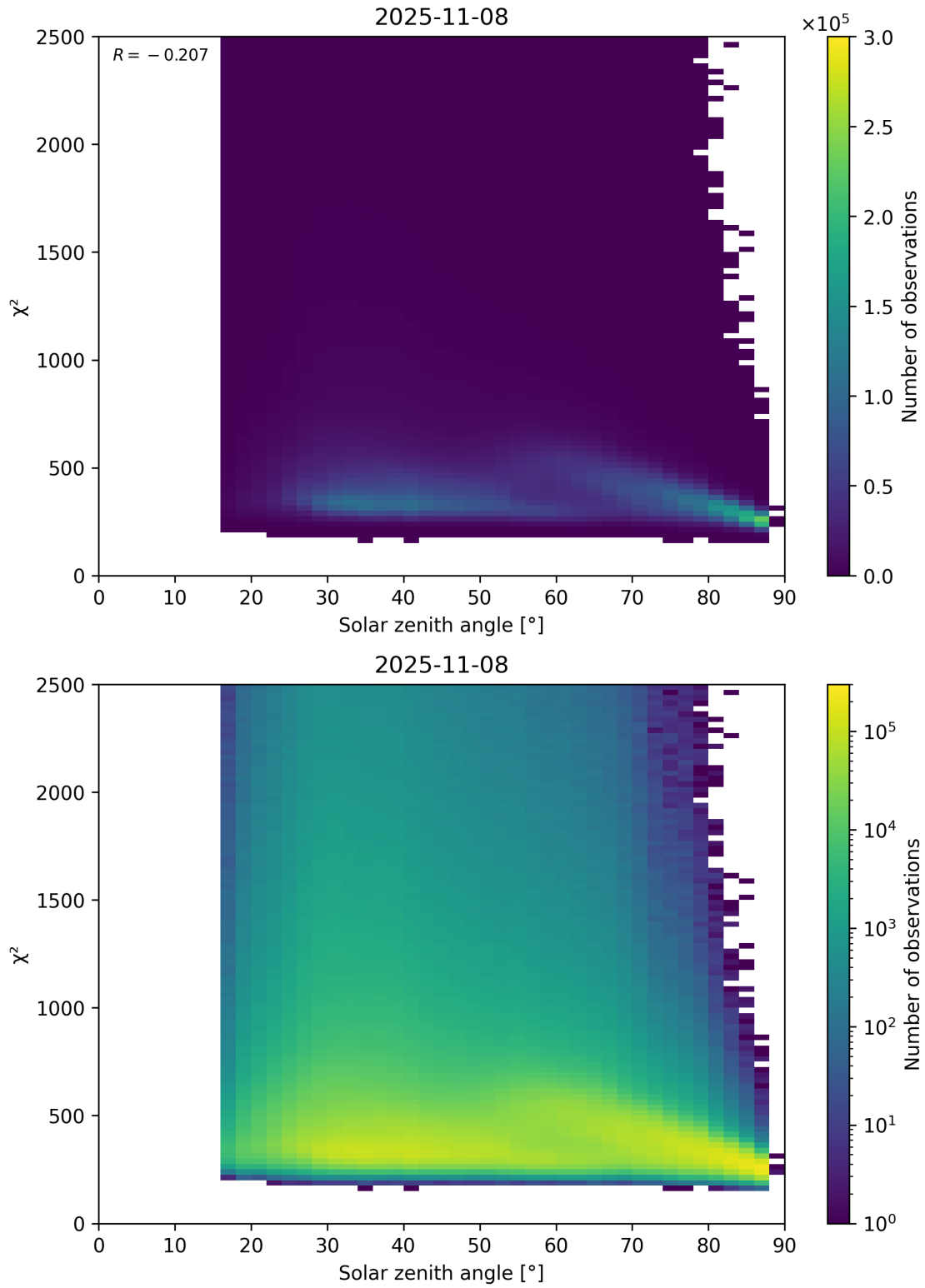
Figure 148: Scatter density plot of “Solar zenith angle” against “ \chi^2 ” for 2025-11-07 to 2025-11-09.
