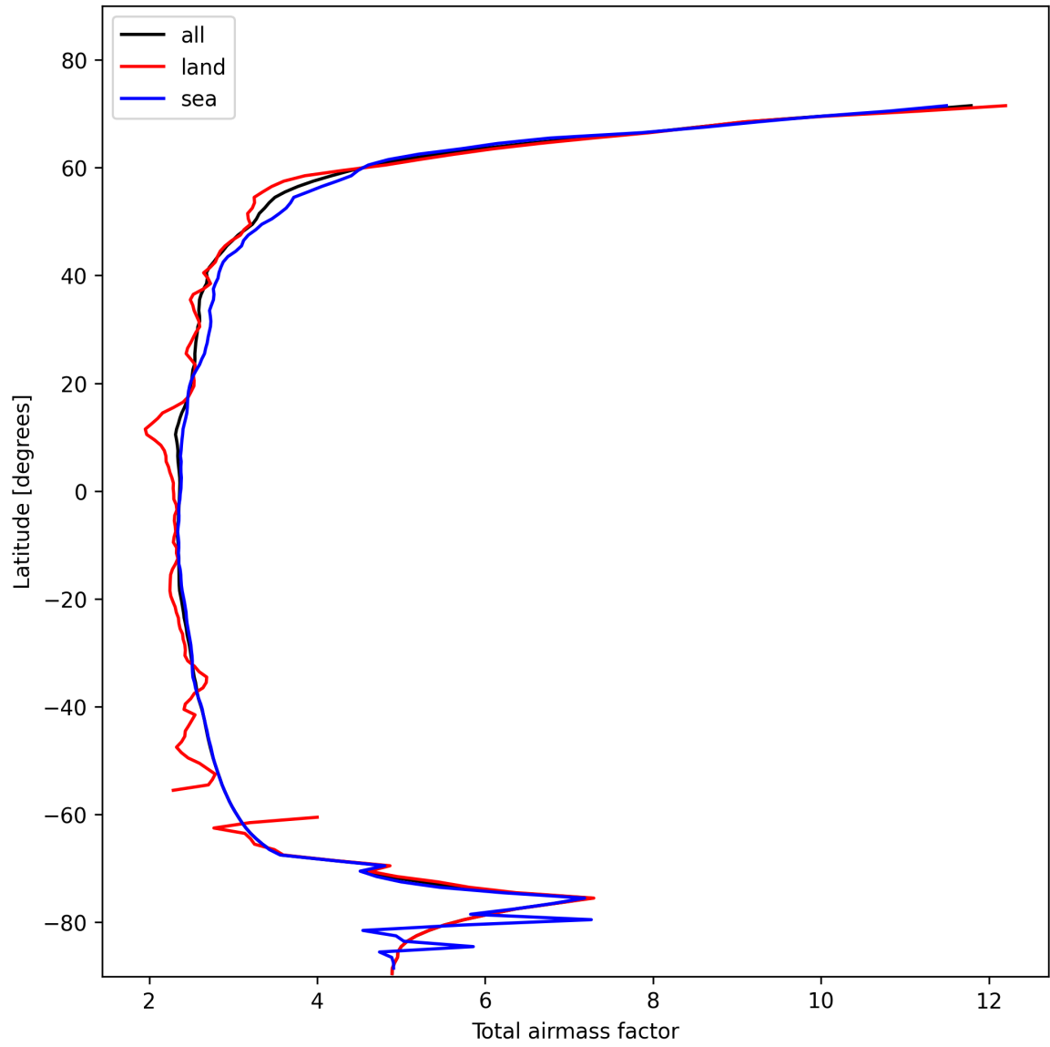
Figure 15: Zonal average of “Total airmass factor” for 2025-11-07 to 2025-11-09.
