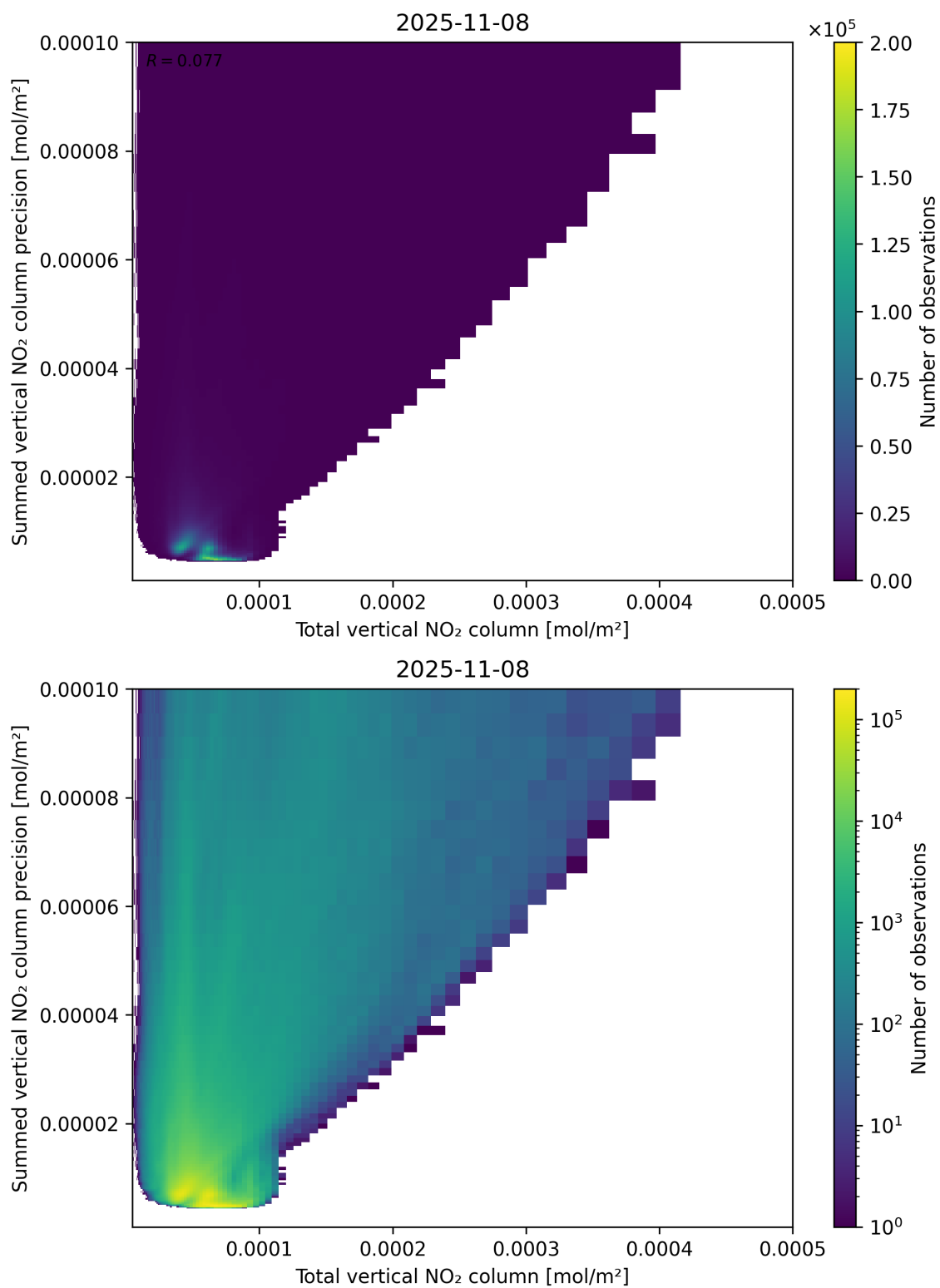
Figure 113: Scatter density plot of “Total vertical NO 2 column” against “Summed vertical NO 2 column precision” for 2025-11-07 to 2025-11-09.
