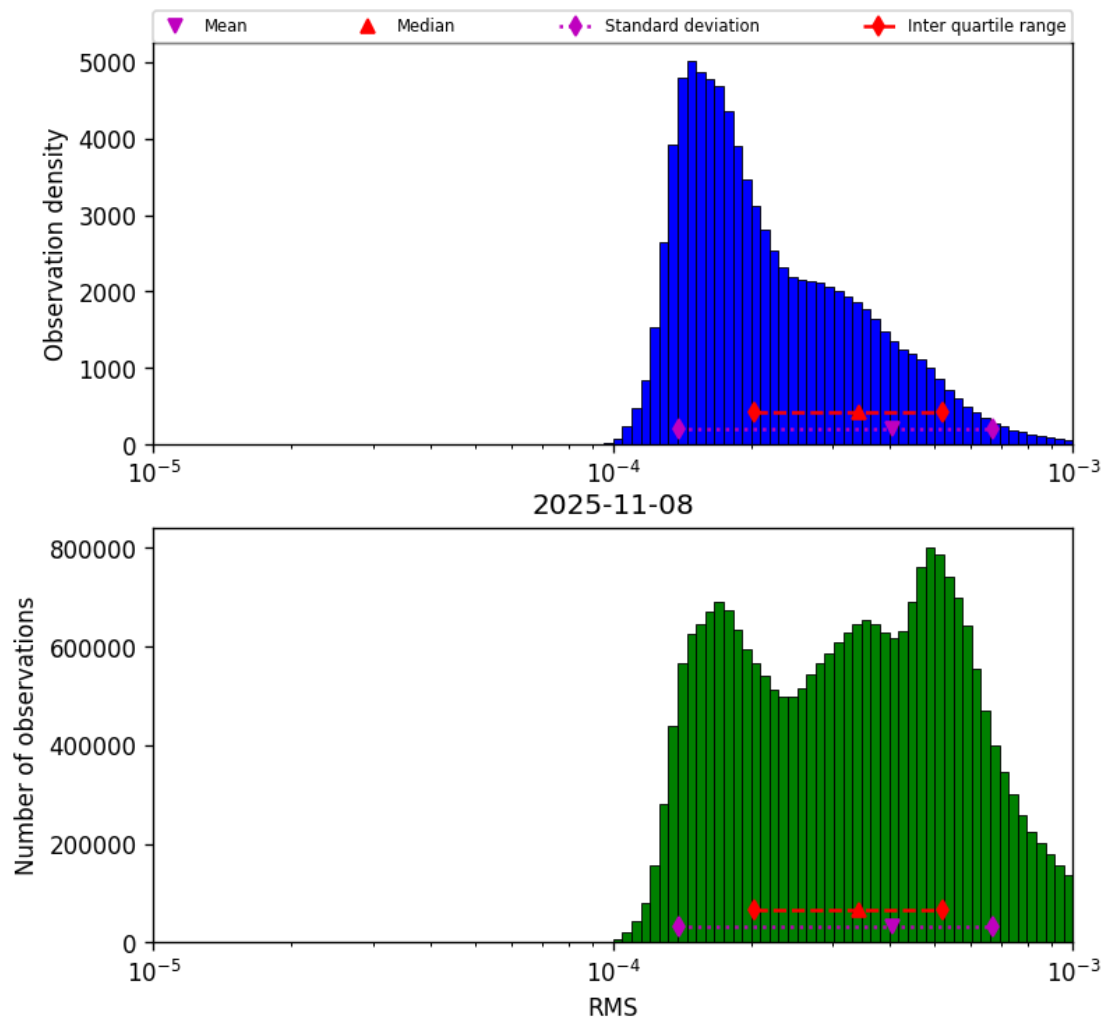
Figure 43: Histogram of “RMS” for 2025-11-07 to 2025-11-09
