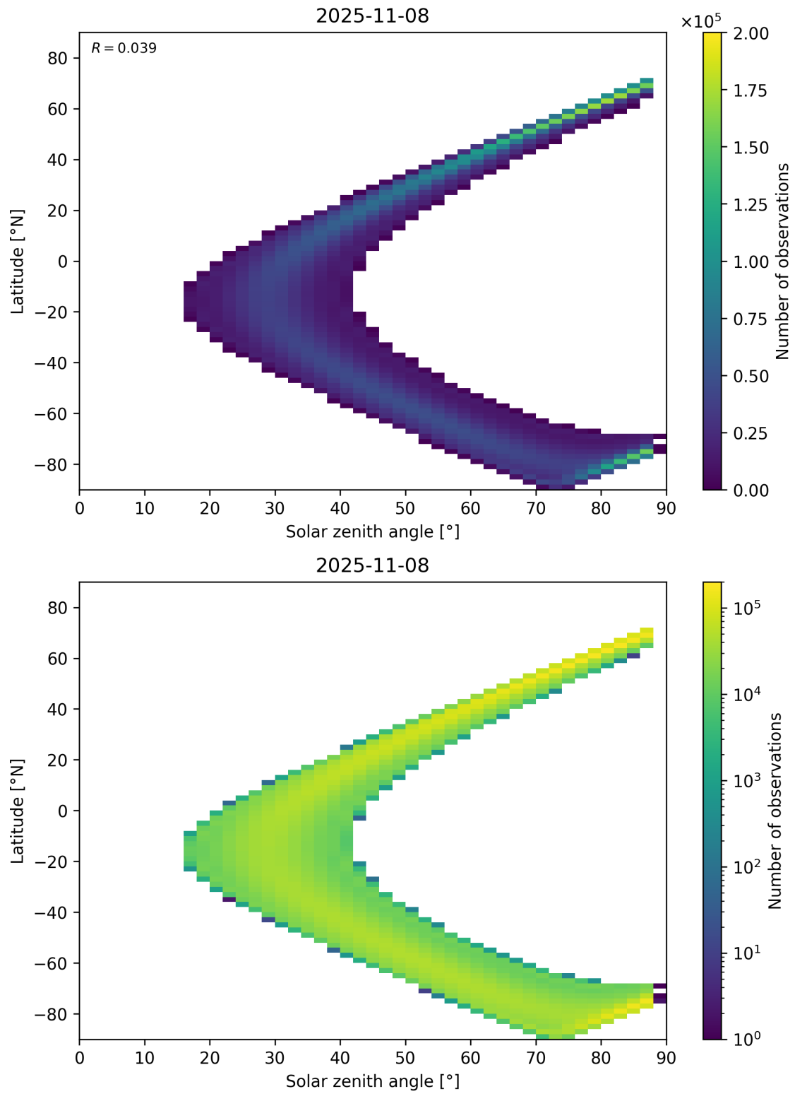
Figure 149: Scatter density plot of “Solar zenith angle” against “Latitude” for 2025-11-07 to 2025-11-09.
