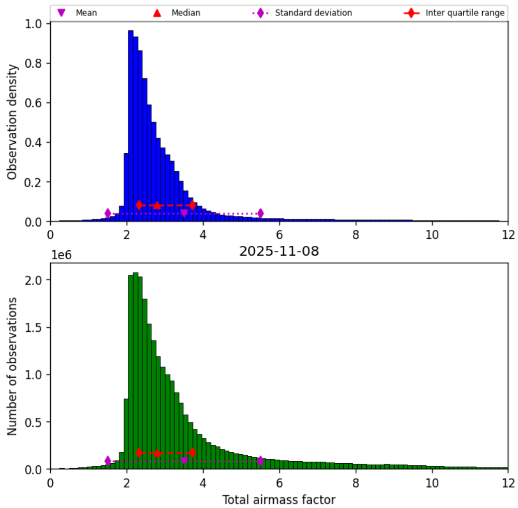
Figure 32: Histogram of “Total airmass factor” for 2025-11-07 to 2025-11-09
