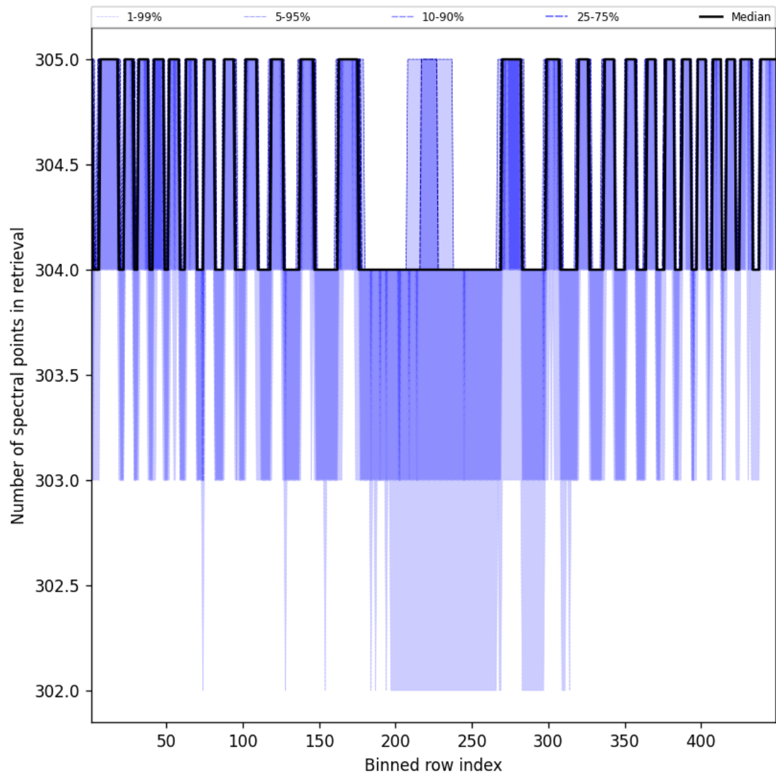
Figure 50: Along track statistics of “Number of spectral points in retrieval” for 2025-11-07 to 2025-11-09
