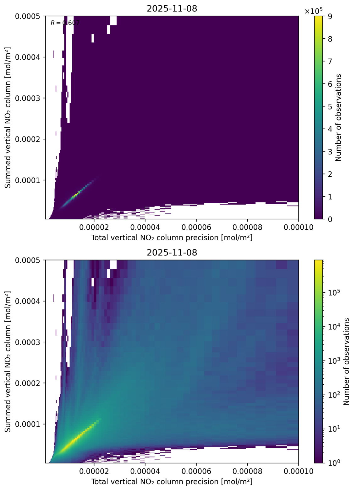
Figure 117: Scatter density plot of “Total vertical NO 2 column precision” against “Summed vertical NO 2 column” for 2025-11-07 to 2025-11-09.
