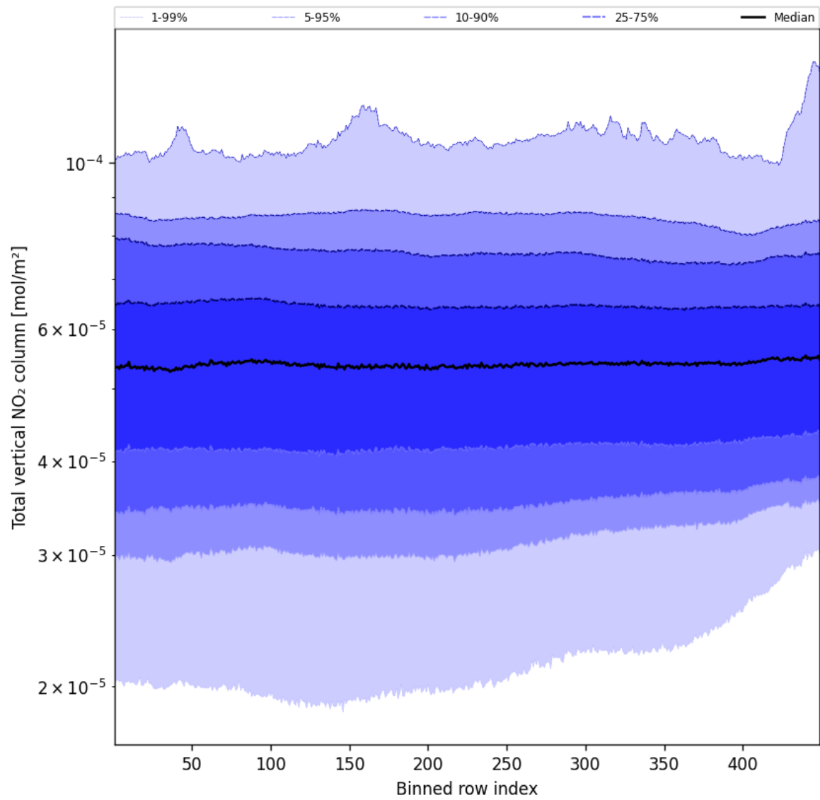
Figure 55: Along track statistics of “Total vertical NO 2 column” for 2025-11-07 to 2025-11-09
