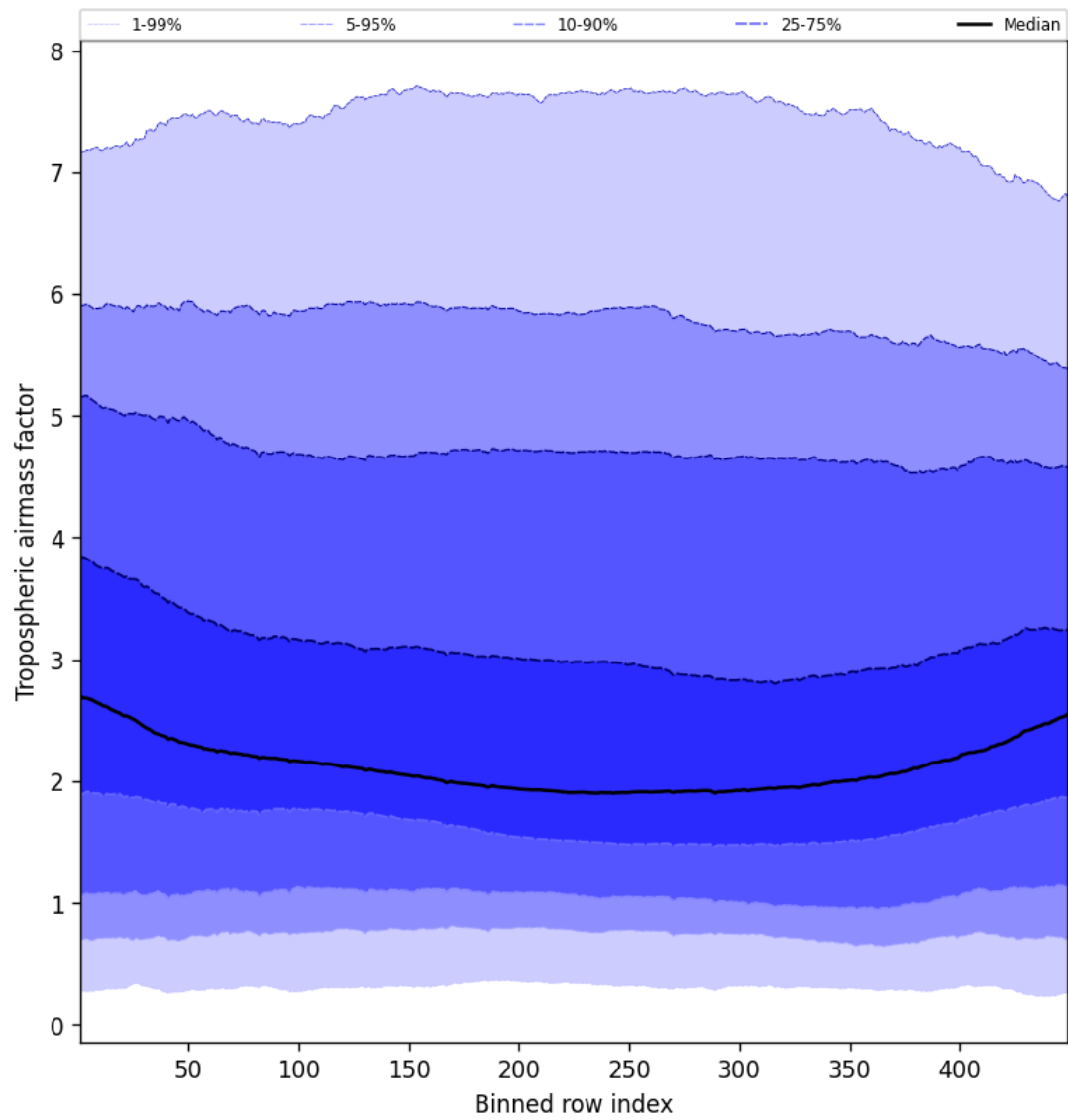
Figure 48: Along track statistics of “Tropospheric air mass factor” for 2025-11-07 to 2025-11-09
