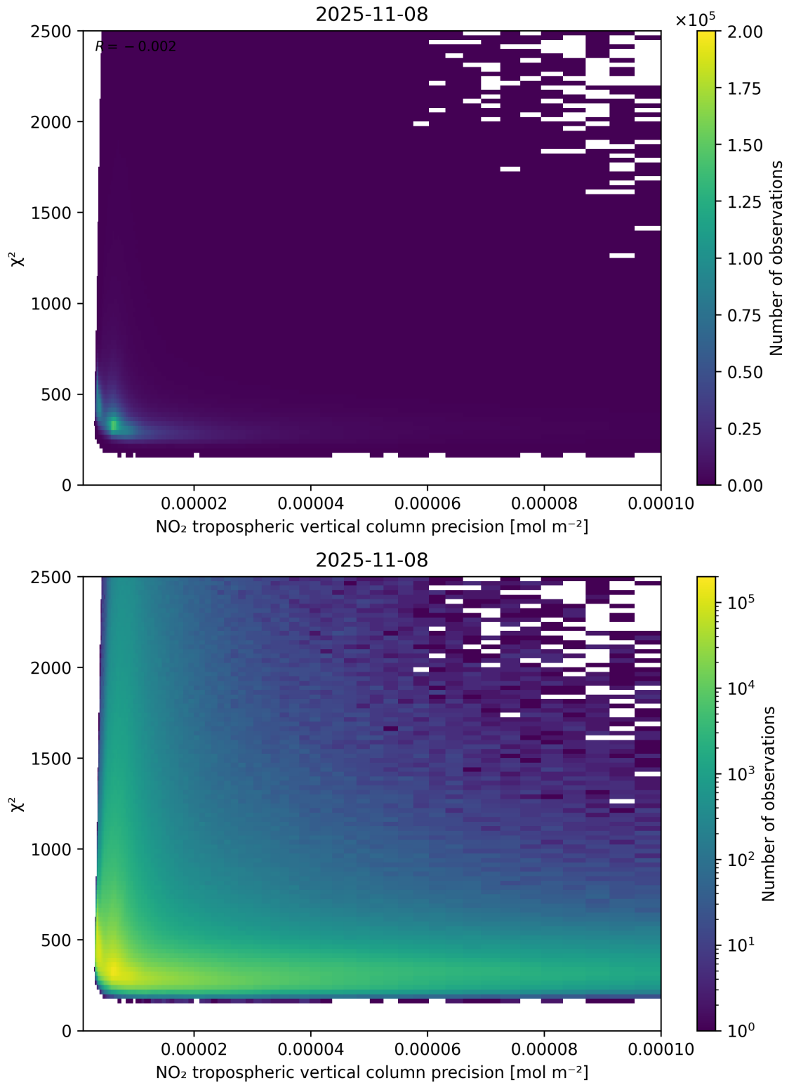
Figure 134: Scatter density plot of “NO 2 tropospheric vertical column precision” against “ \chi^2 ” for 2025-11-07 to 2025-11-09.
