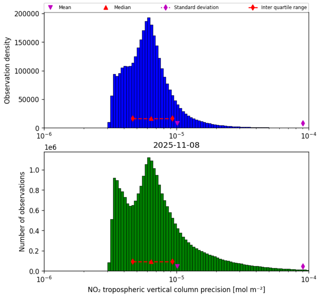
Figure 30: Histogram of “NO 2 tropospheric vertical column precision” for 2025-11-07 to 2025-11-09
