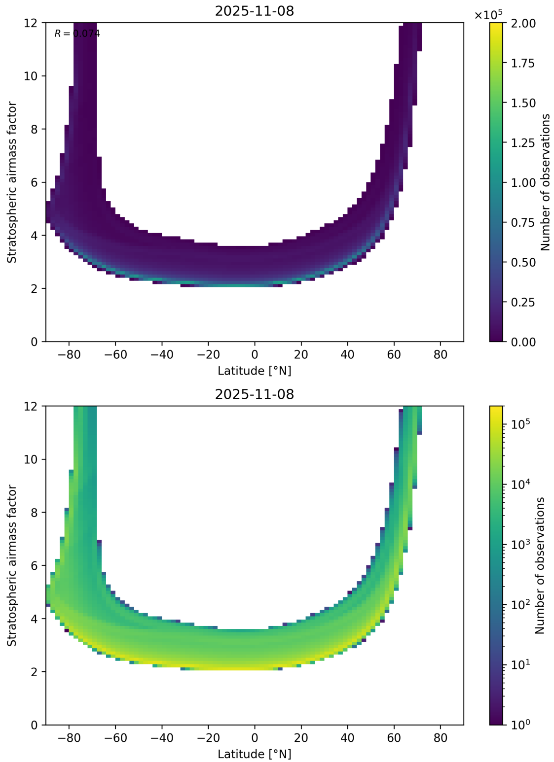
Figure 83: Scatter density plot of “Latitude” against “Stratospheric airmass factor” for 2025-11-07 to 2025-11-09.
