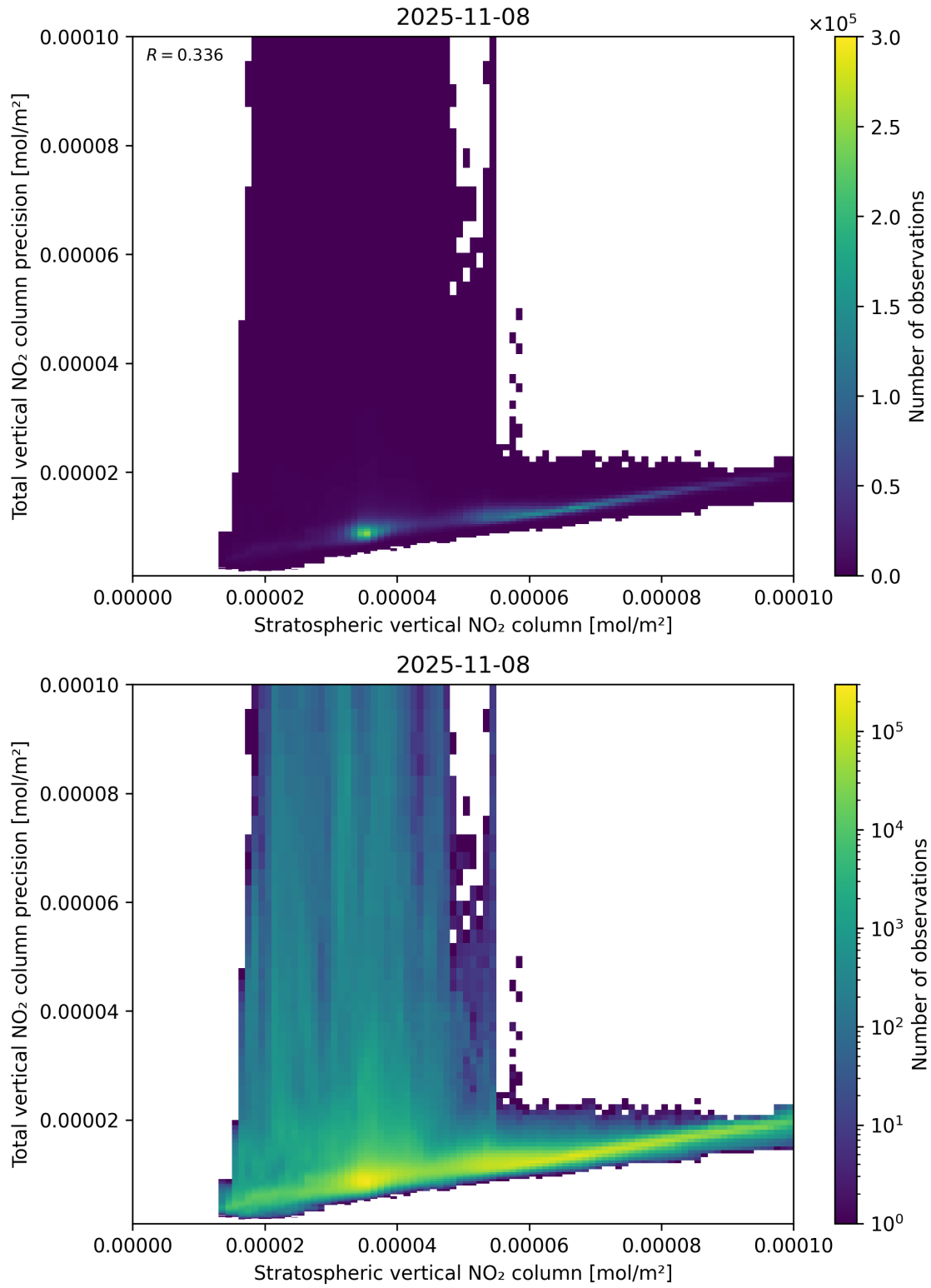
Figure 101: Scatter density plot of “Stratospheric vertical NO 2 column” against “Total vertical NO 2 column precision” for 2025-11-07 to 2025-11-09.
