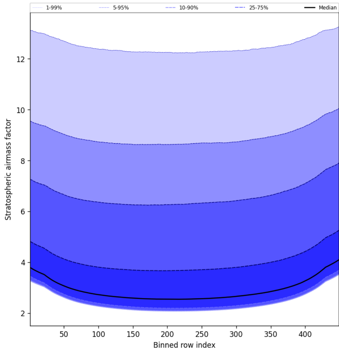
Figure 61: Along track statistics of “Stratospheric air mass factor” for 2025-11-07 to 2025-11-09
