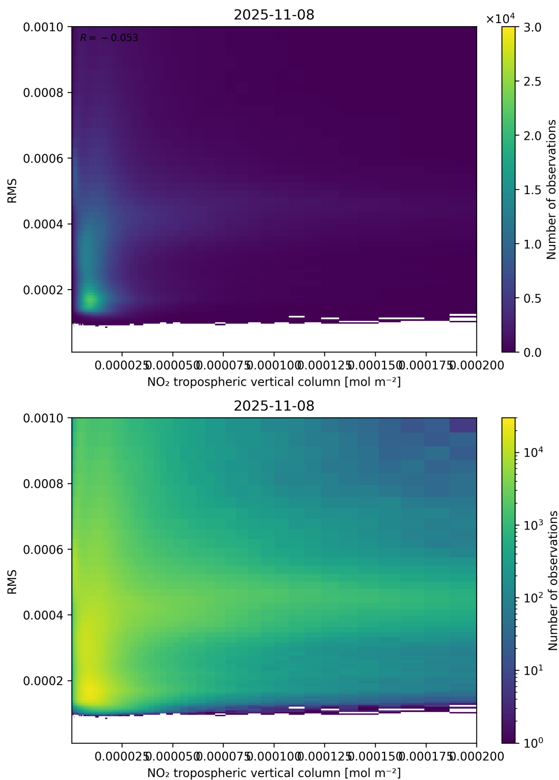
Figure 142: Scatter density plot of “NO 2 tropospheric vertical column” against “RMS” for 2025-11-07 to 2025-11-09.
