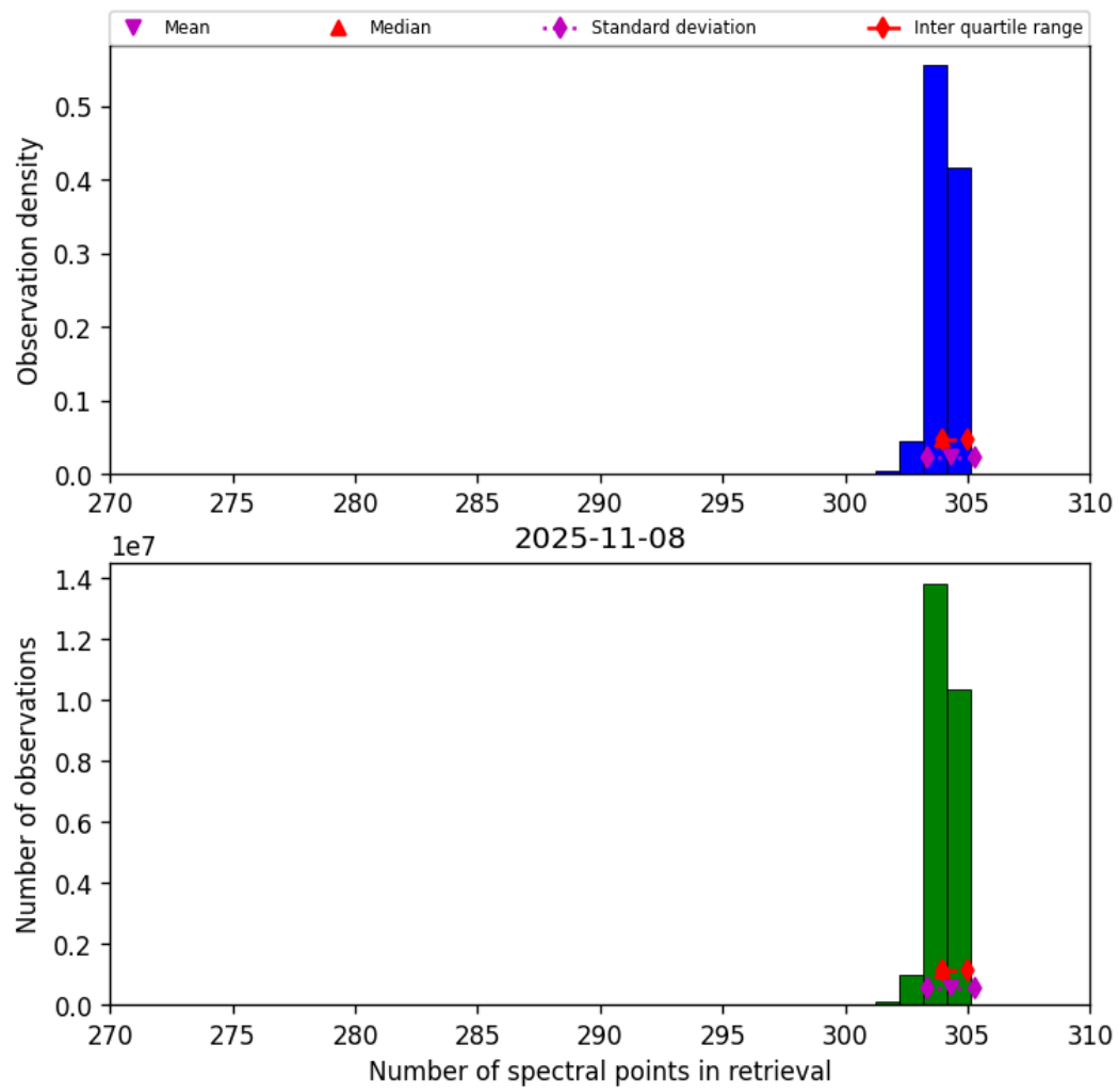
Figure 33: Histogram of “Number of spectral points in retrieval” for 2025-11-07 to 2025-11-09
