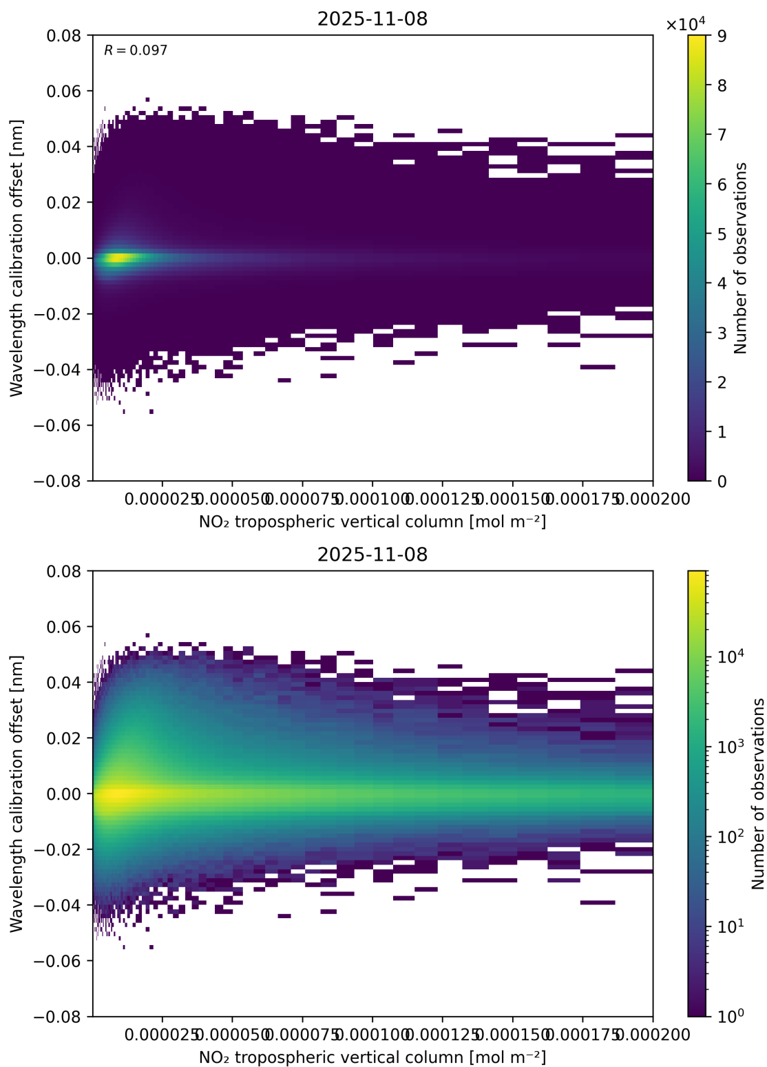
Figure 143: Scatter density plot of “NO 2 tropospheric vertical column” against “Wavelength calibration offset” for 2025-11-07 to 2025-11-09.
