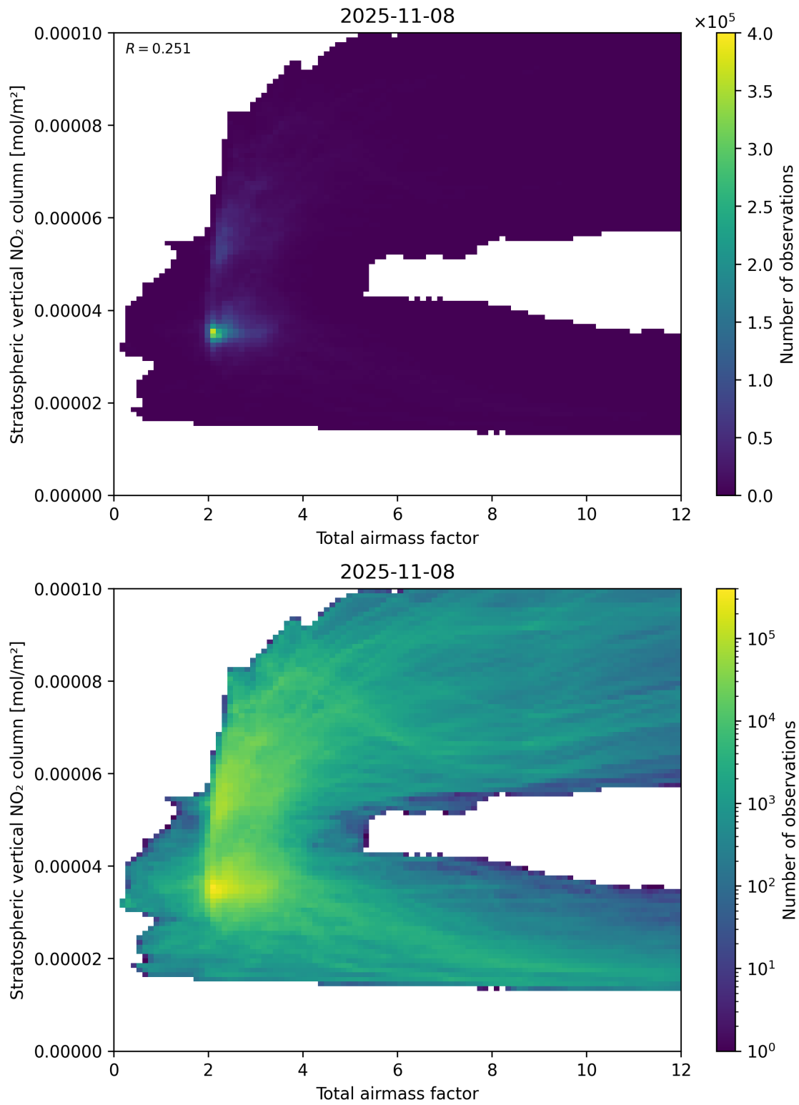
Figure 64: Scatter density plot of “Total airmass factor” against “Stratospheric vertical NO 2 column” for 2025-11-07 to 2025-11-09.
