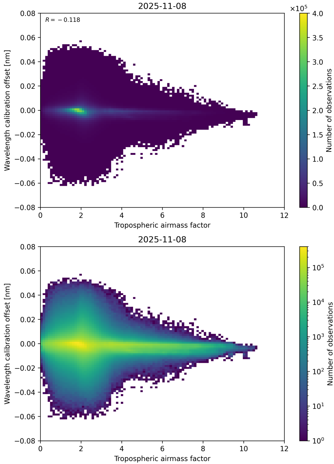
Figure 80: Scatter density plot of “Tropospheric airmass factor” against “Wavelength calibration offset” for 2025-11-07 to 2025-11-09.
