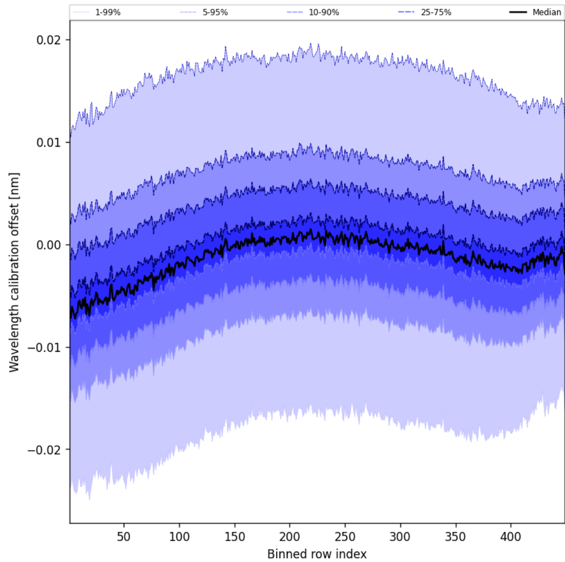
Figure 52: Along track statistics of “Wavelength calibration offset” for 2025-11-07 to 2025-11-09
