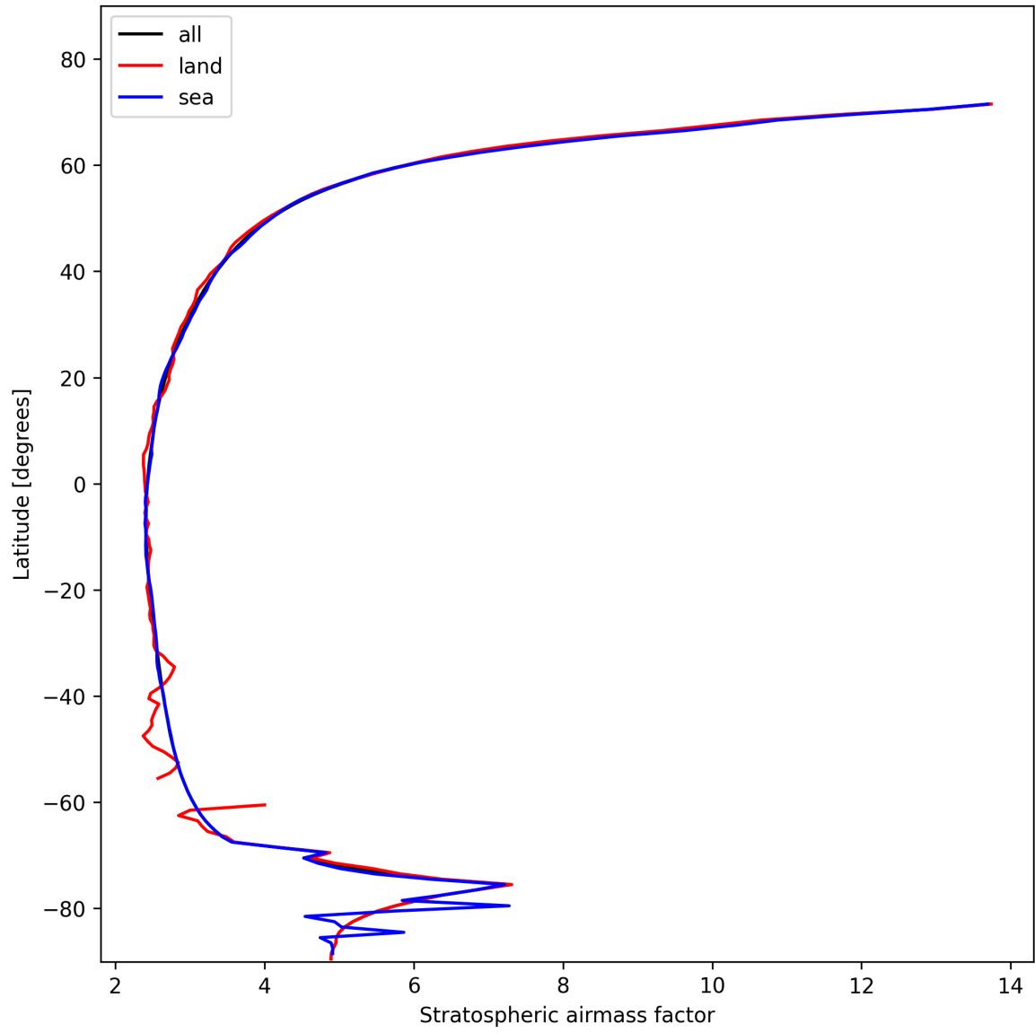
Figure 27: Zonal average of “Stratospheric air mass factor” for 2025-11-07 to 2025-11-09.
