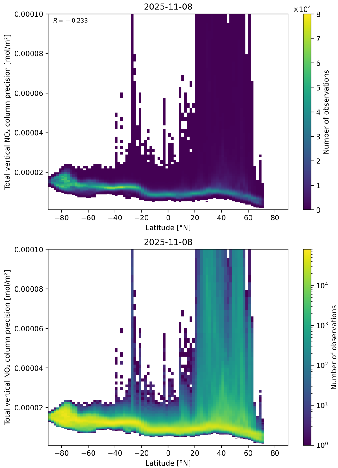
Figure 91: Scatter density plot of “Latitude” against “Total vertical NO 2 column precision” for 2025-11-07 to 2025-11-09.
