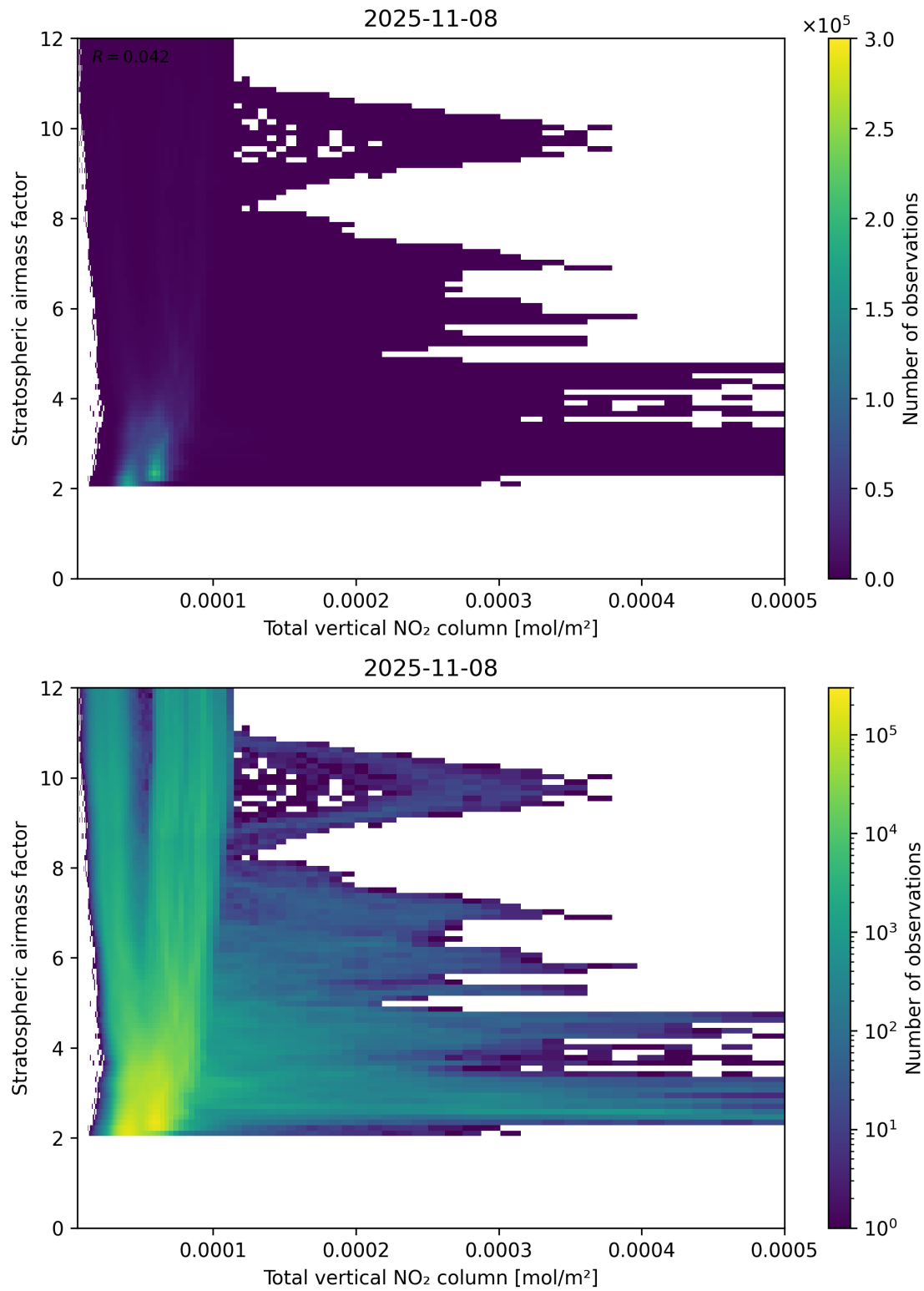
Figure 110: Scatter density plot of “Total vertical NO 2 column” against “Stratospheric airmass factor” for 2025-11-07 to 2025-11-09.
