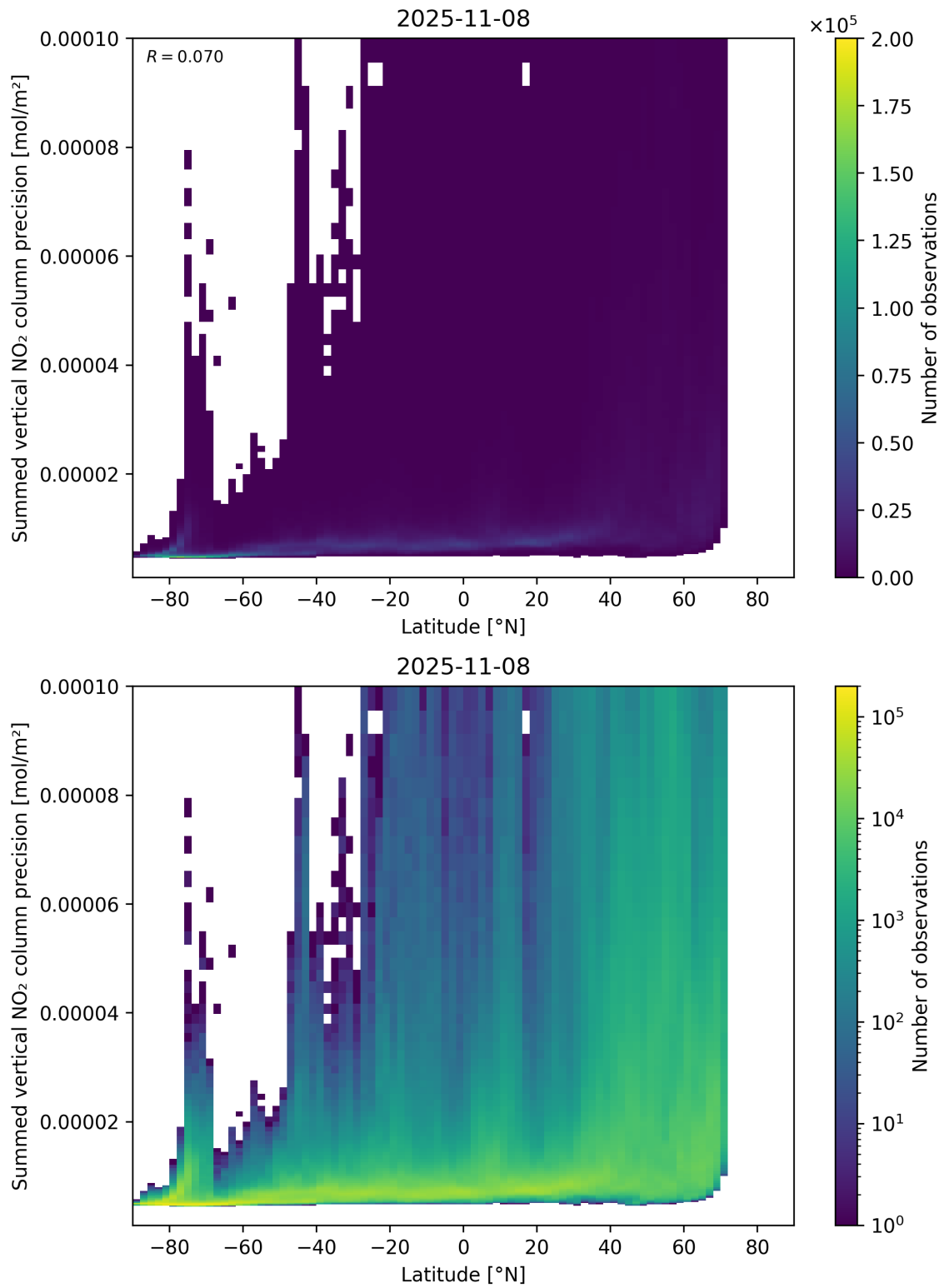
Figure 89: Scatter density plot of “Latitude” against “Summed vertical NO 2 column precision” for 2025-11-07 to 2025-11-09.
