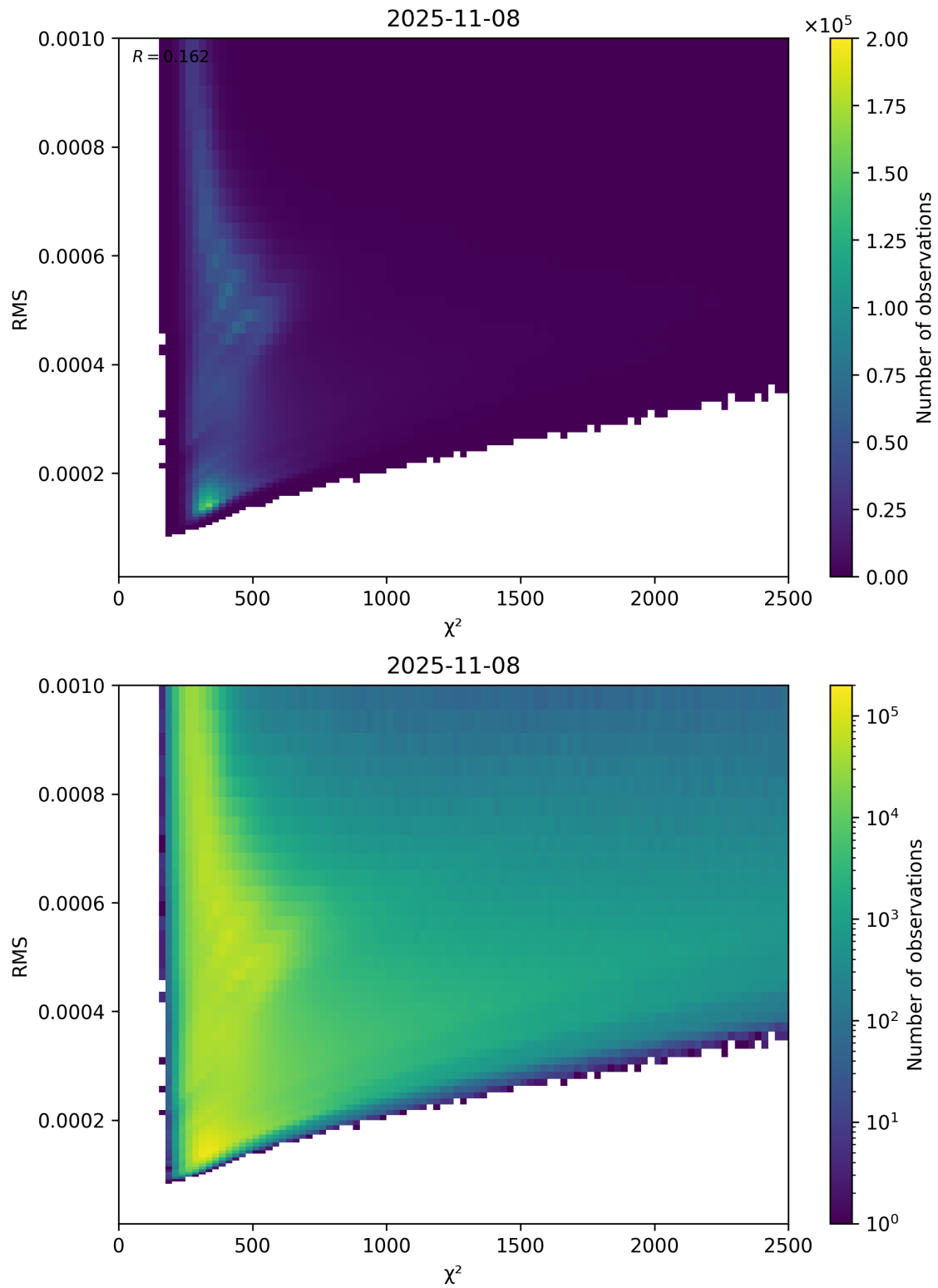
Figure 82: Scatter density plot of “ \chi^2 ” against “RMS” for 2025-11-07 to 2025-11-09.
