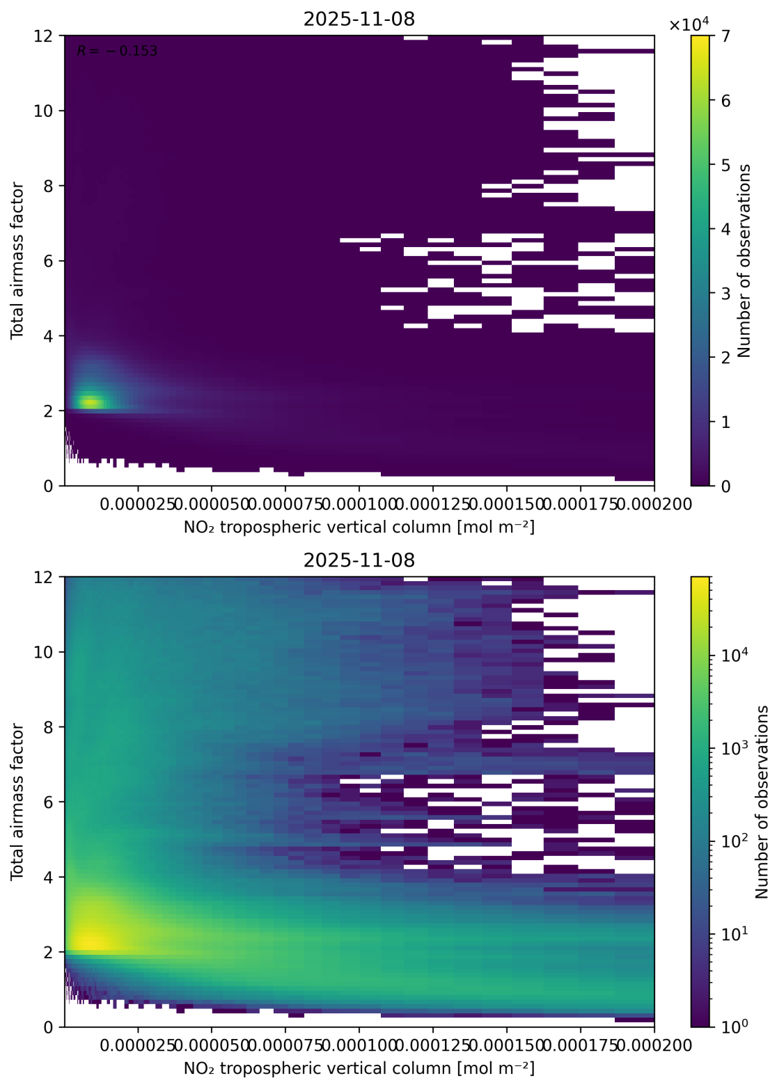
Figure 122: Scatter density plot of “NO 2 tropospheric vertical column” against “Total airmass factor” for 2025-11-07 to 2025-11-09.
