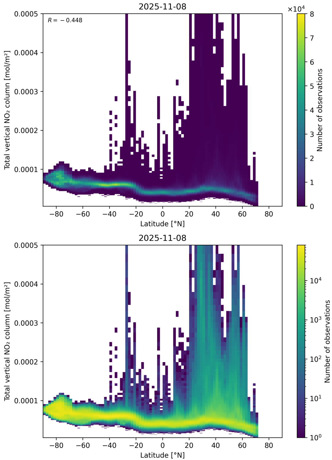
Figure 90: Scatter density plot of “Latitude” against “Total vertical NO 2 column” for 2025-11-07 to 2025-11-09.
