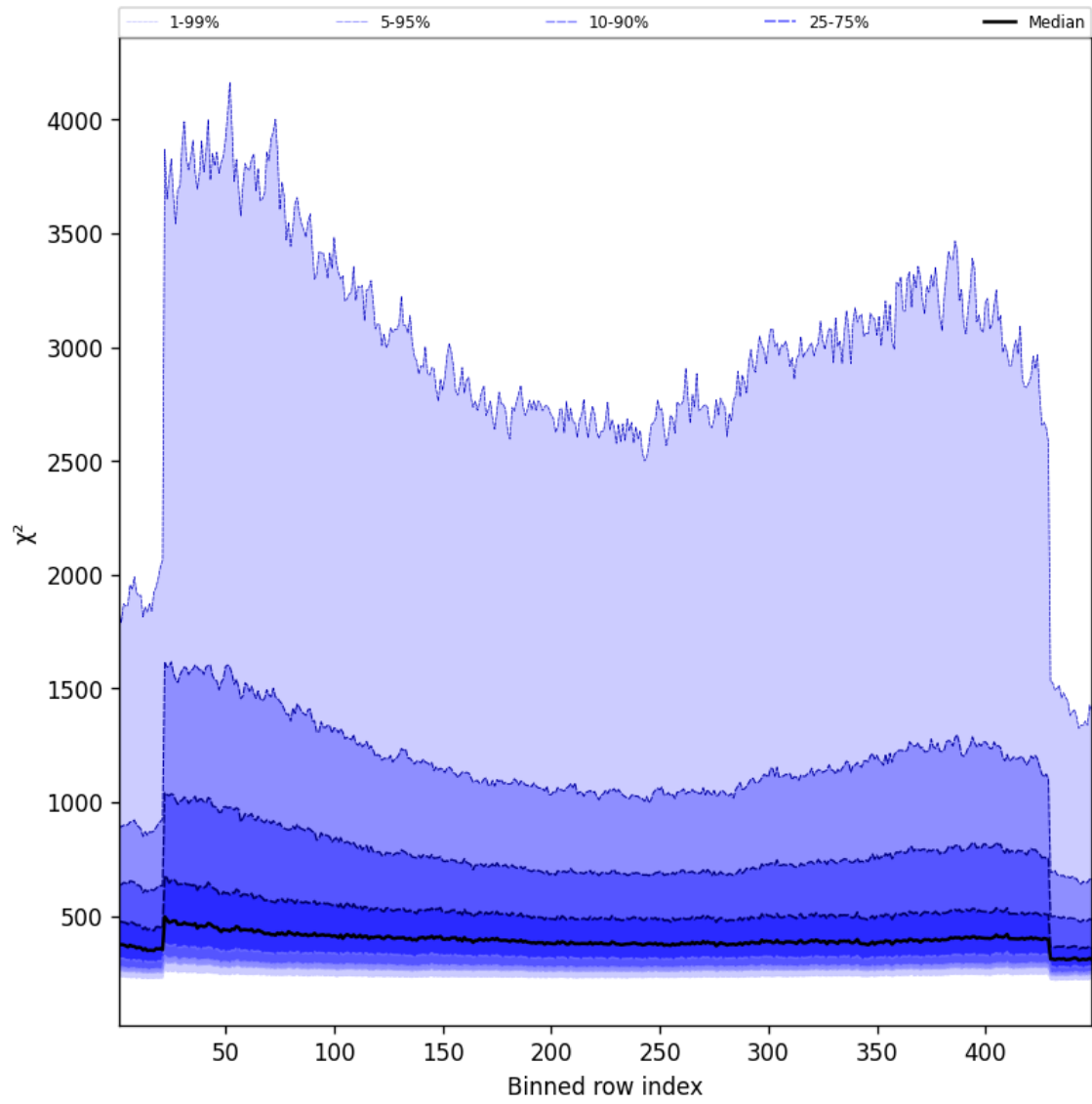
Figure 59: Along track statistics of “ \chi^2 ” for 2025-11-07 to 2025-11-09
