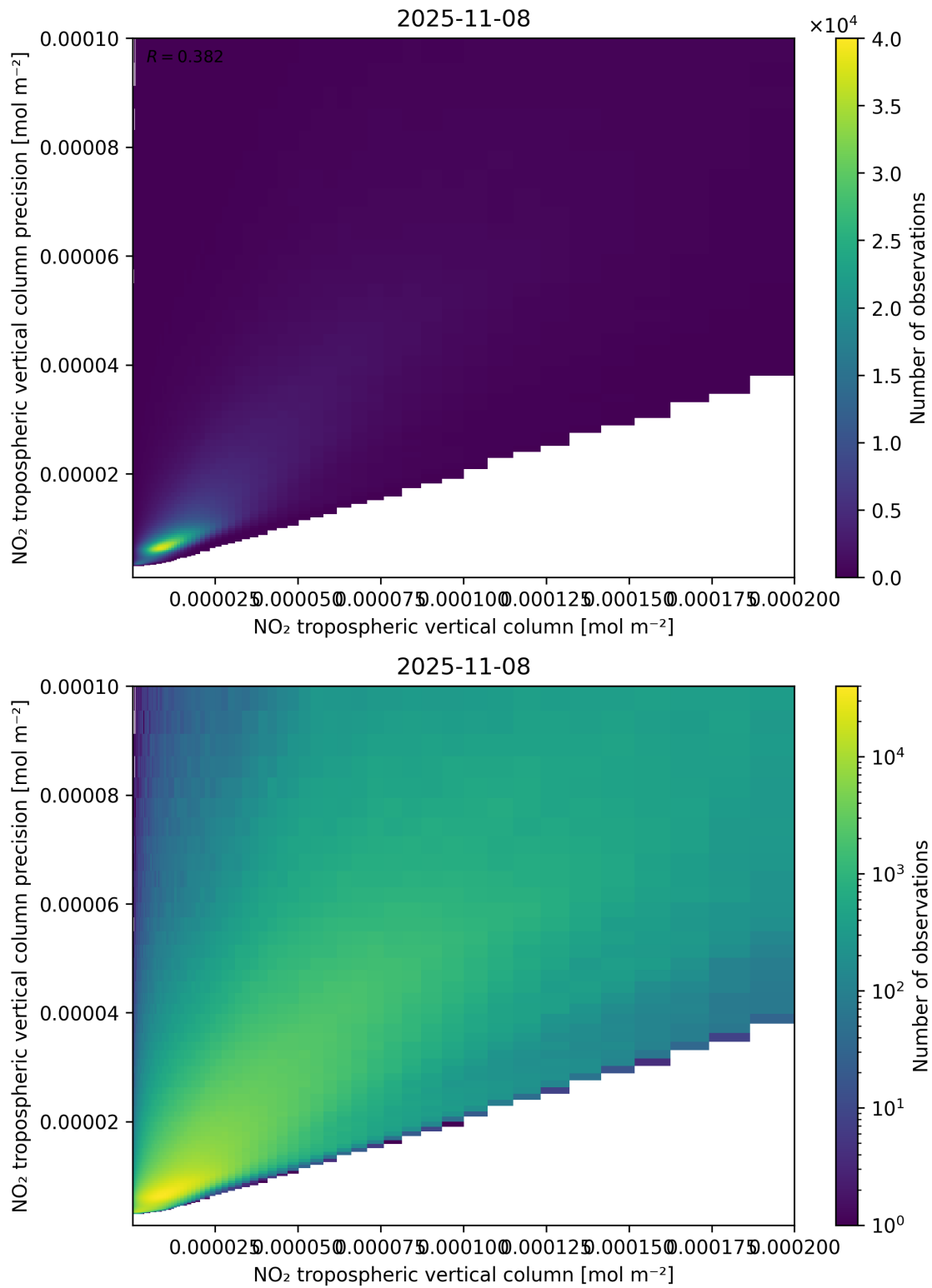
Figure 130: Scatter density plot of “NO 2 tropospheric vertical column” against “NO 2 tropospheric vertical column precision” for 2025-11-07 to 2025-11-09.
