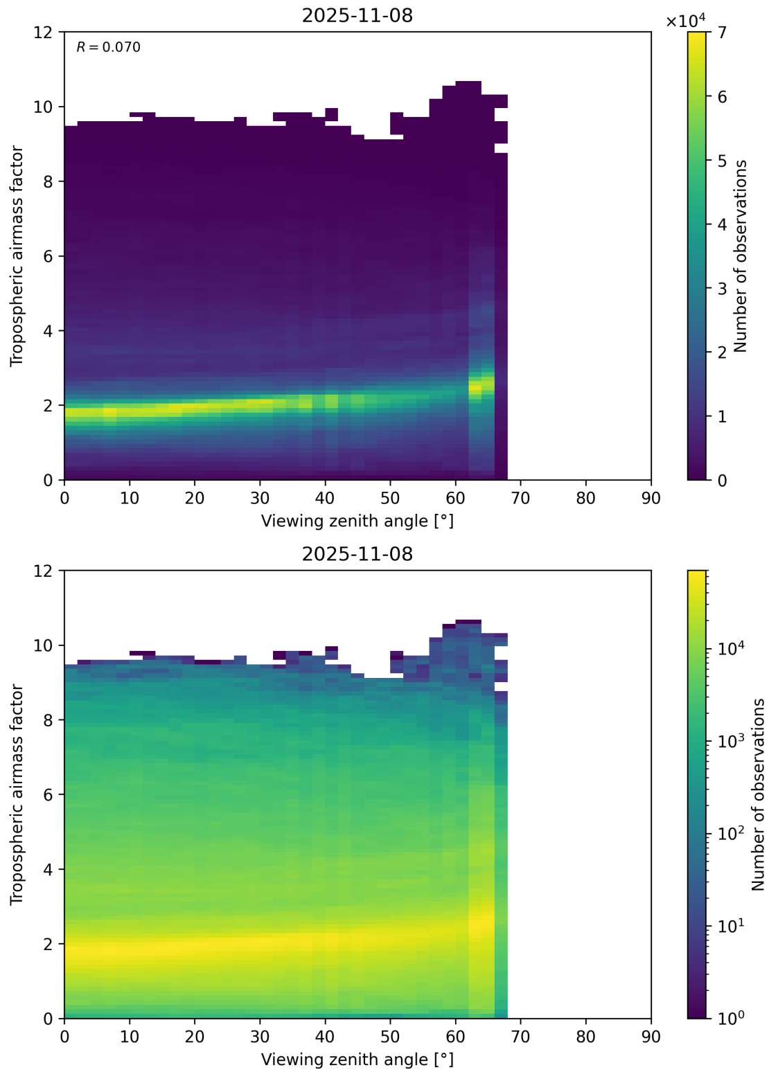
Figure 161: Scatter density plot of “Viewing zenith angle” against “Tropospheric airmass factor” for 2025-11-07 to 2025-11-09.
