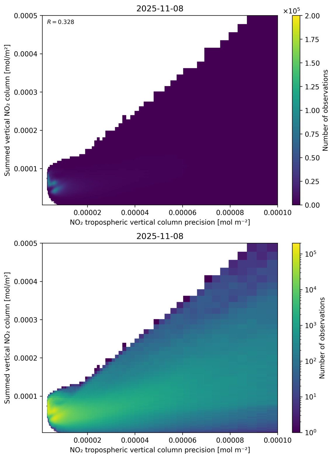
Figure 136: Scatter density plot of “NO 2 tropospheric vertical column precision” against “Summed vertical NO 2 column” for 2025-11-07 to 2025-11-09.
