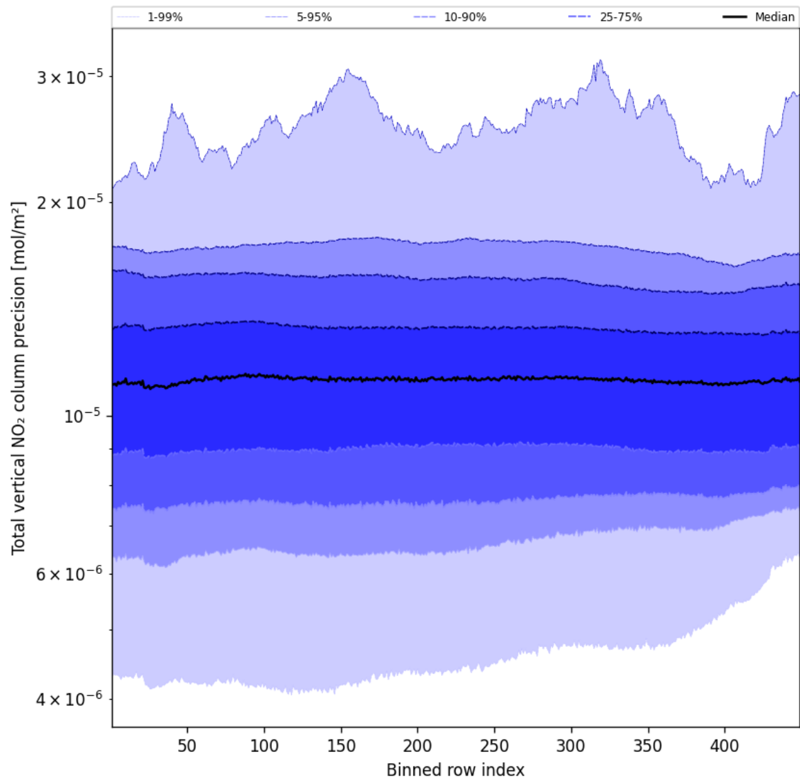
Figure 56: Along track statistics of “Total vertical NO 2 column precision” for 2025-11-07 to 2025-11-09
