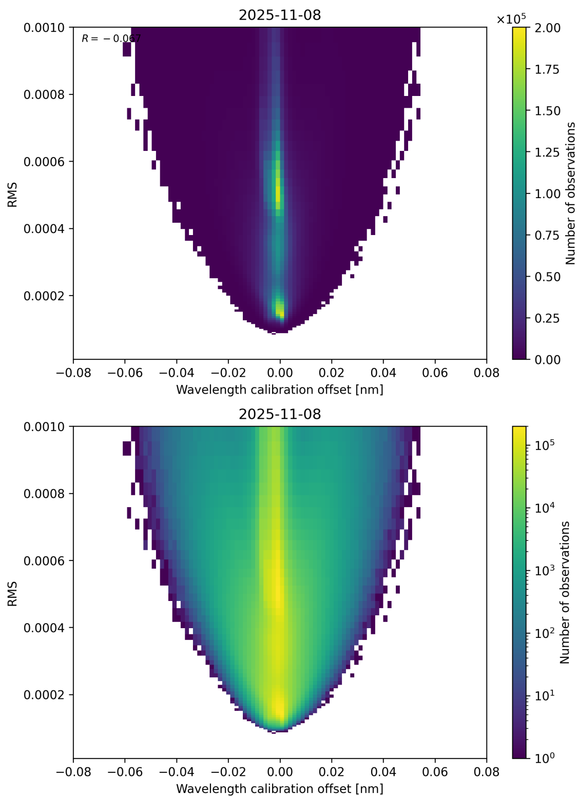
Figure 181: Scatter density plot of “Wavelength calibration offset” against “RMS” for 2025-11-07 to 2025-11-09.
