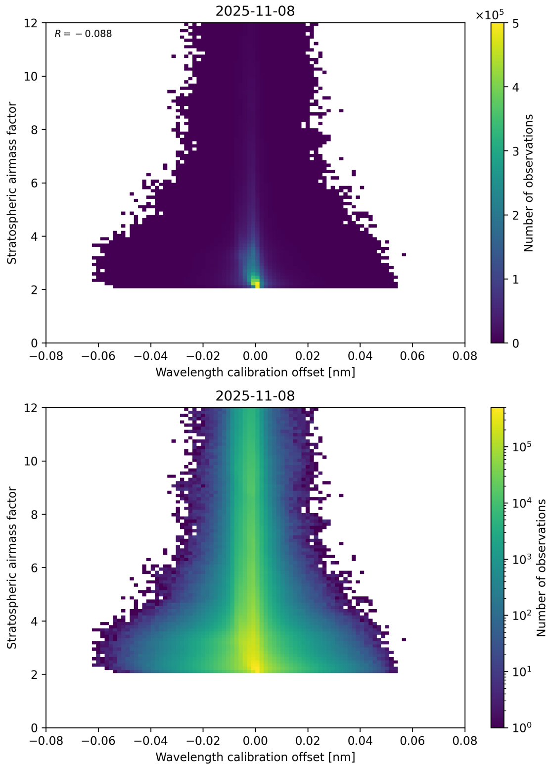
Figure 174: Scatter density plot of “Wavelength calibration offset” against “Stratospheric airmass factor” for 2025-11-07 to 2025-11-09.
