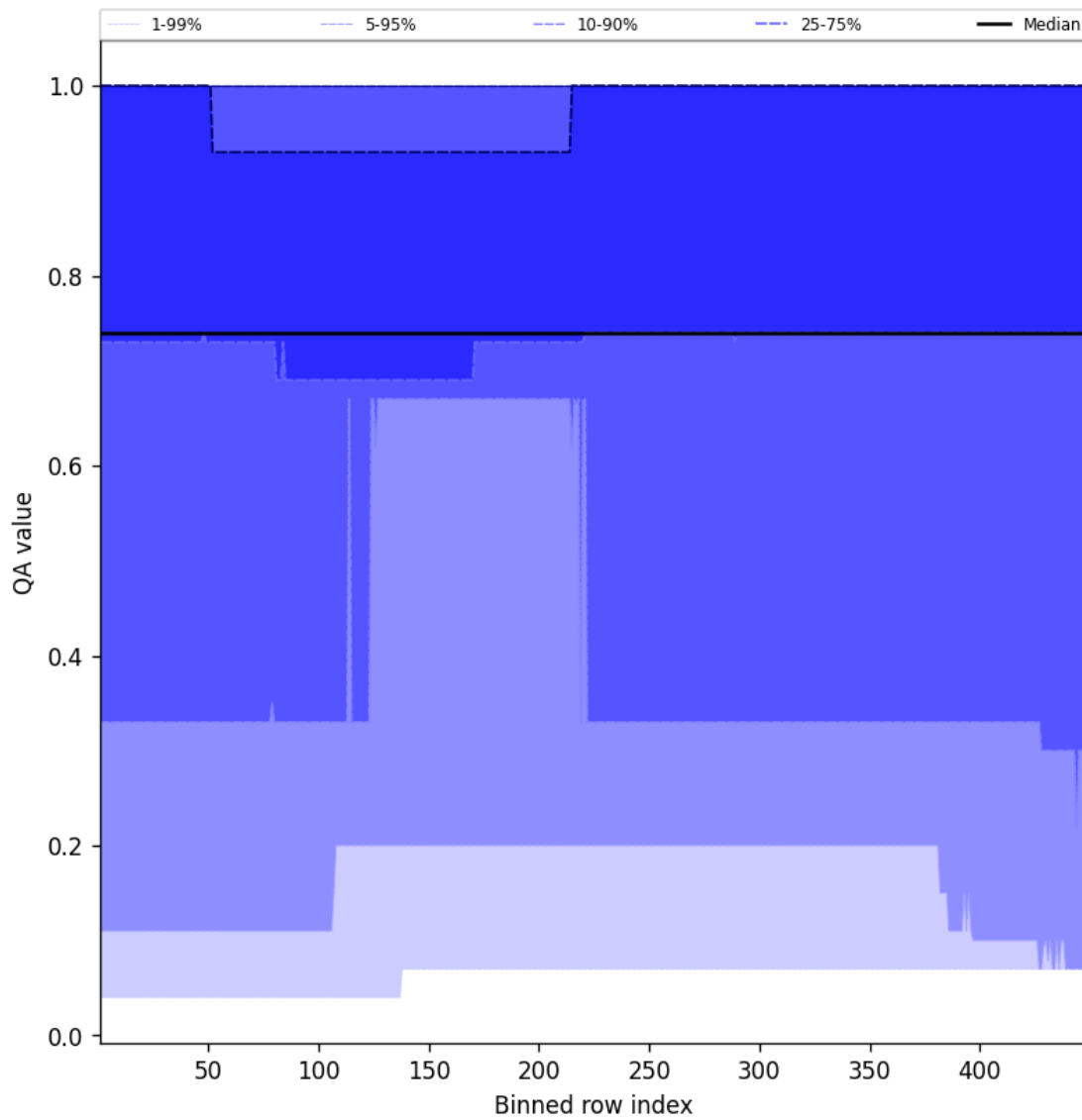
Figure 45: Along track statistics of “QA value” for 2025-11-07 to 2025-11-09
