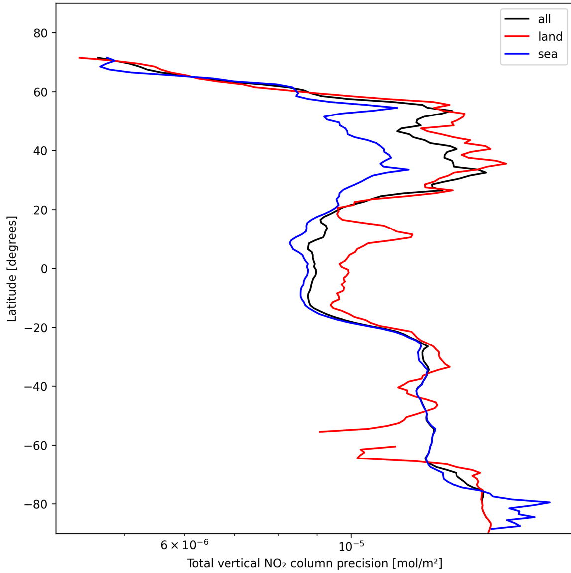
Figure 22: Zonal average of “Total vertical NO 2 column precision” for 2025-11-07 to 2025-11-09.
