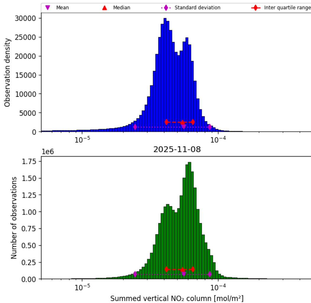
Figure 40: Histogram of “Summed vertical NO 2 column” for 2025-11-07 to 2025-11-09
