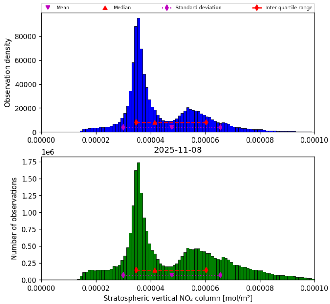
Figure 36: Histogram of “Stratospheric vertical NO 2 column” for 2025-11-07 to 2025-11-09
