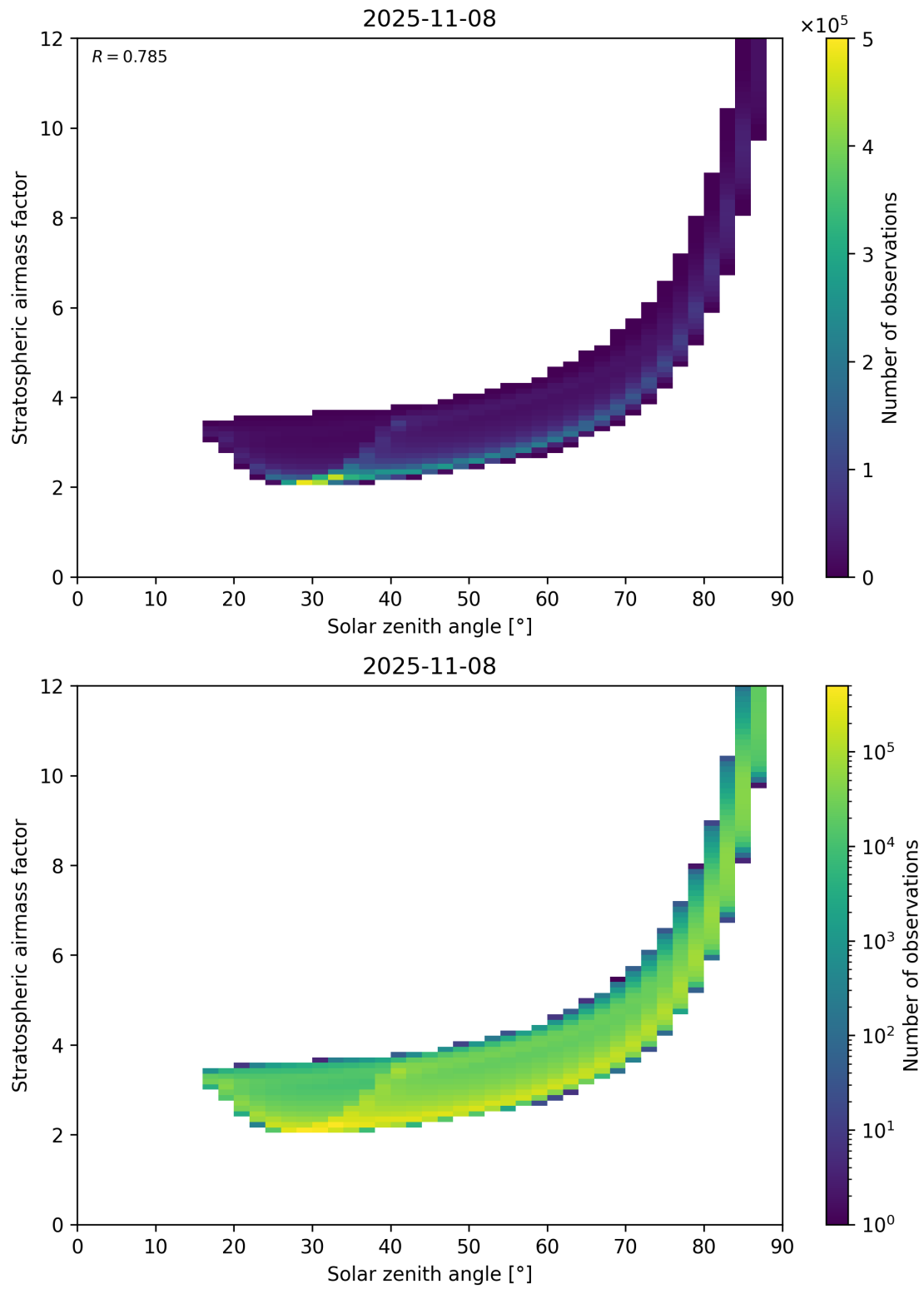
Figure 145: Scatter density plot of “Solar zenith angle” against “Stratospheric airmass factor” for 2025-11-07 to 2025-11-09.
