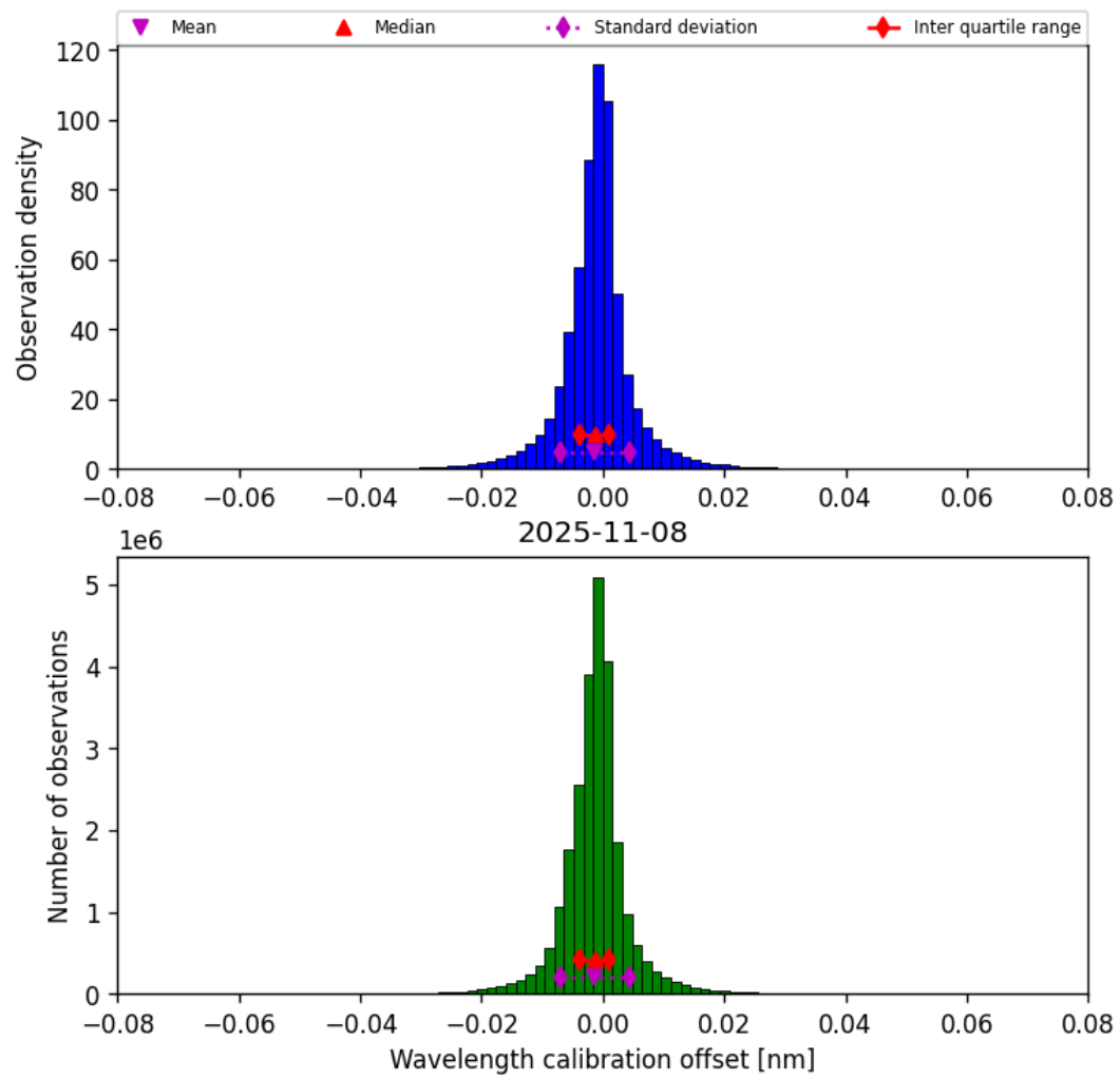
Figure 35: Histogram of “Wavelength calibration offset” for 2025-11-07 to 2025-11-09
