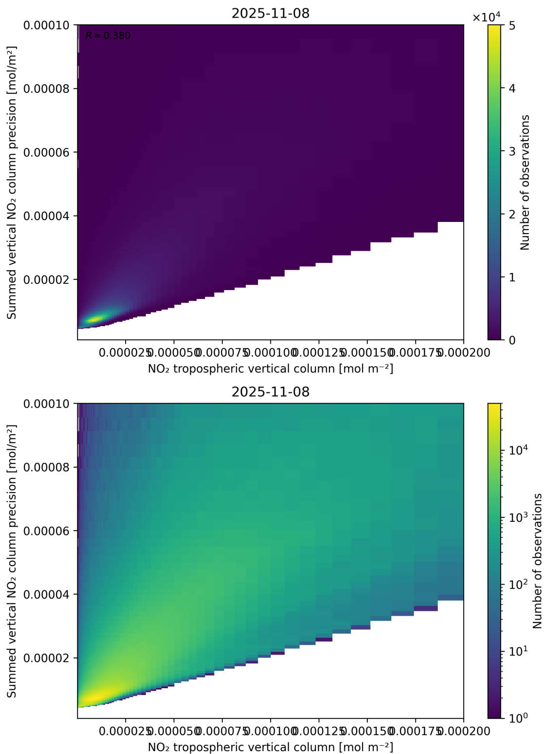
Figure 127: Scatter density plot of “NO 2 tropospheric vertical column” against “Summed vertical NO 2 column precision” for 2025-11-07 to 2025-11-09.
