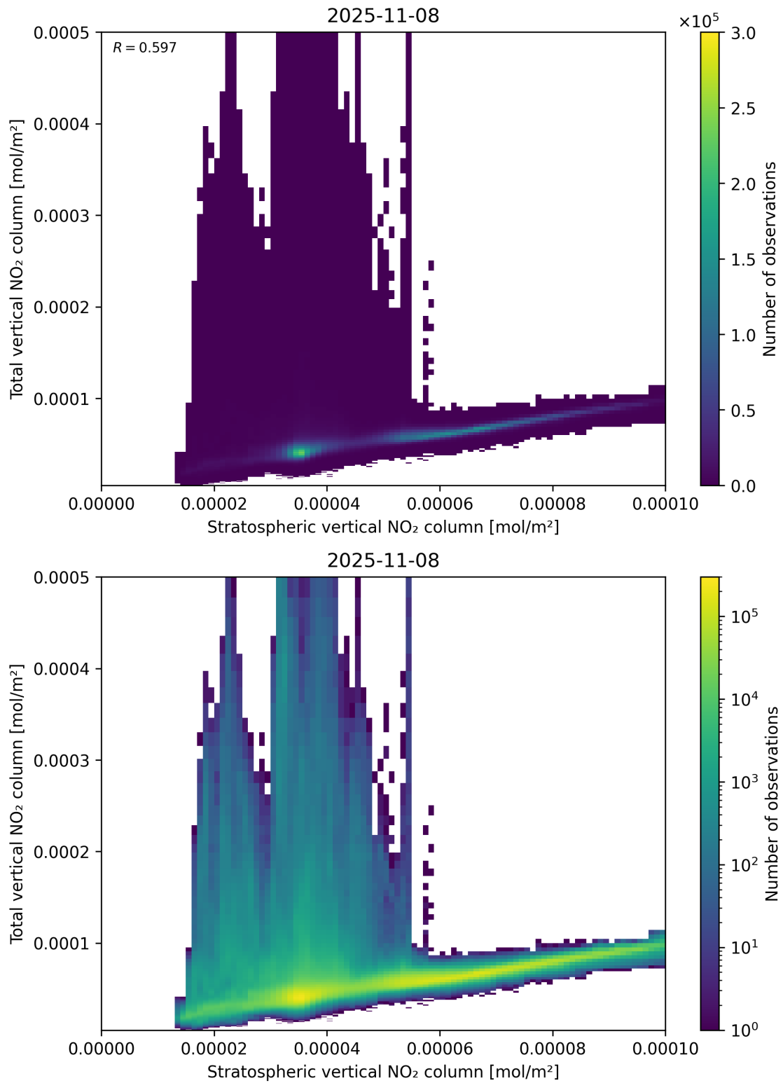
Figure 100: Scatter density plot of “Stratospheric vertical NO 2 column” against “Total vertical NO 2 column” for 2025-11-07 to 2025-11-09.
