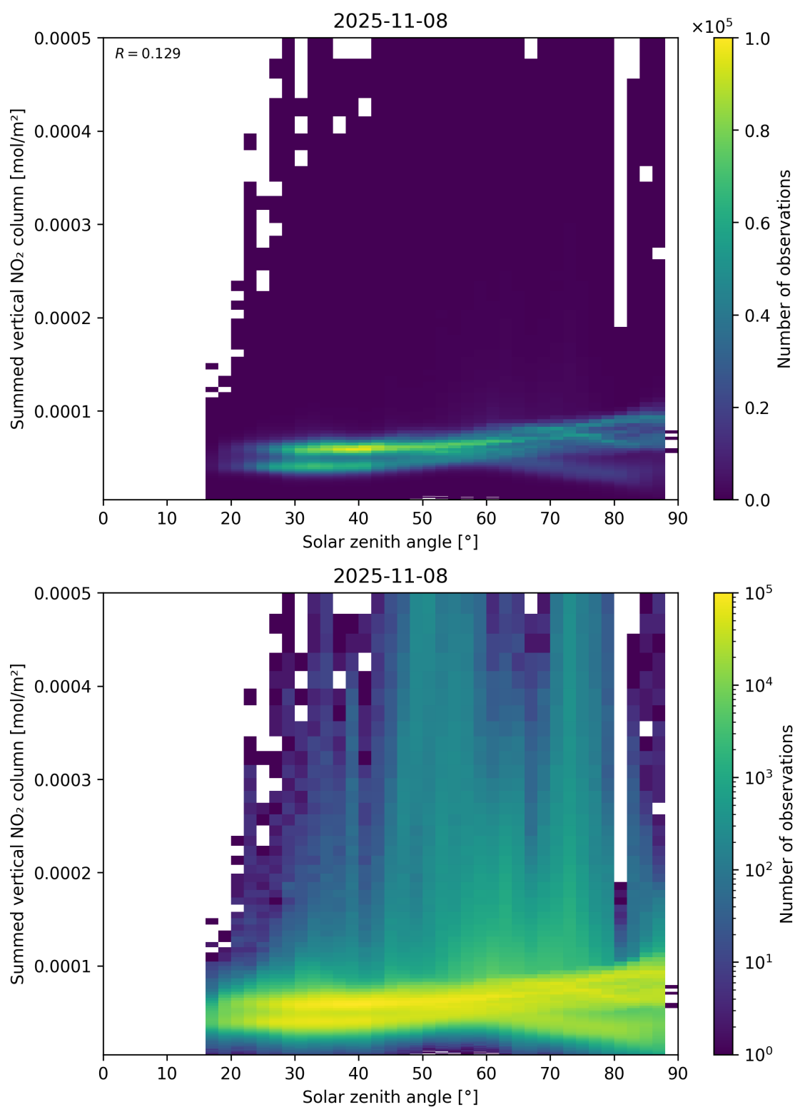
Figure 151: Scatter density plot of “Solar zenith angle” against “Summed vertical NO 2 column” for 2025-11-07 to 2025-11-09.
