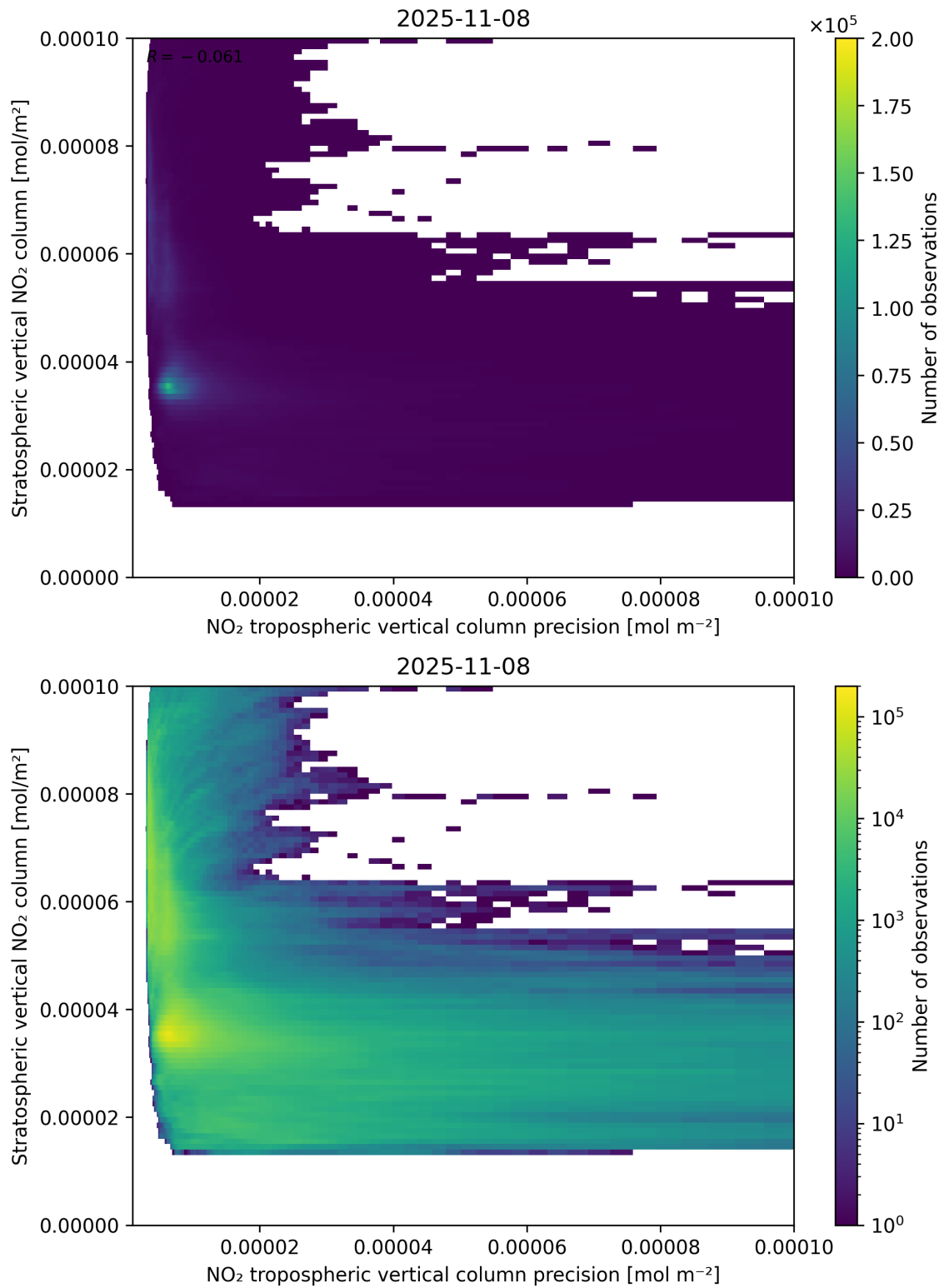
Figure 135: Scatter density plot of “NO 2 tropospheric vertical column precision” against “Stratospheric vertical NO 2 column” for 2025-11-07 to 2025-11-09.
