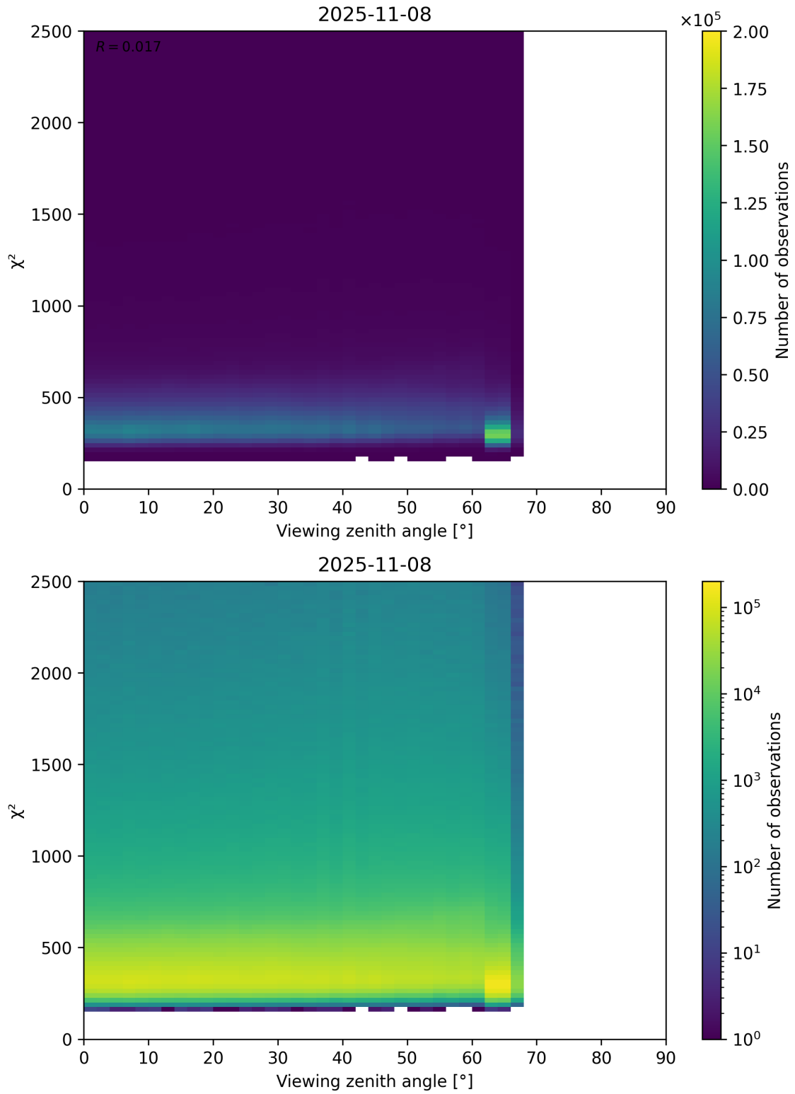
Figure 162: Scatter density plot of “Viewing zenith angle” against “ \chi^2 ” for 2025-11-07 to 2025-11-09.
