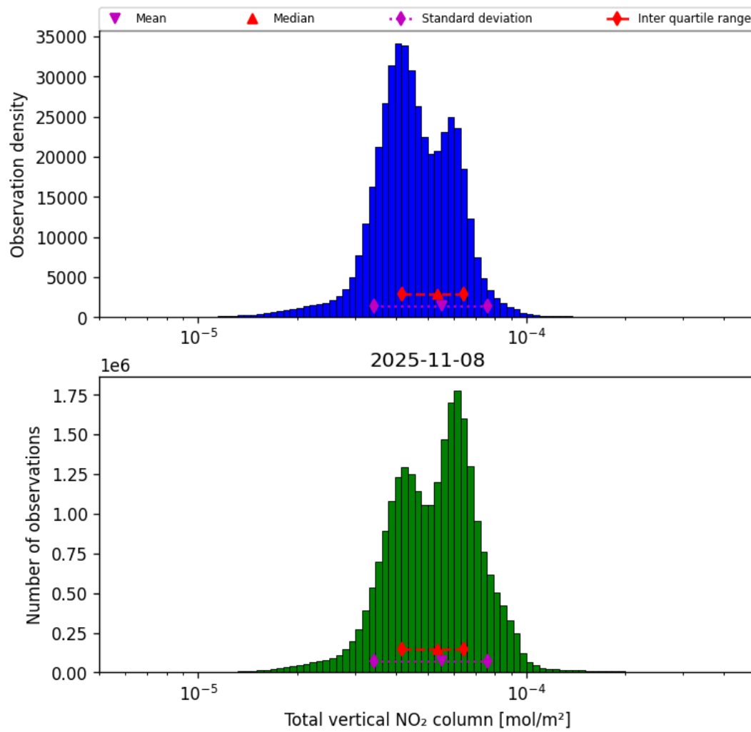
Figure 38: Histogram of “Total vertical NO 2 column” for 2025-11-07 to 2025-11-09
