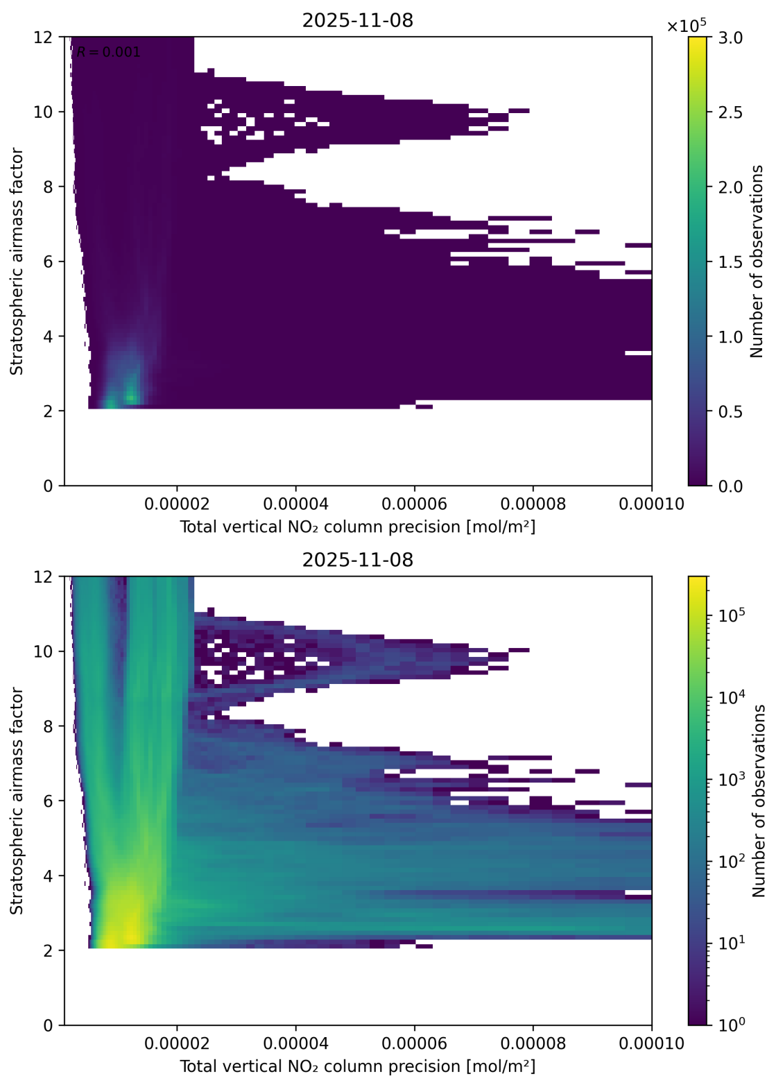
Figure 115: Scatter density plot of “Total vertical NO 2 column precision” against “Stratospheric air mass factor” for 2025-11-07 to 2025-11-09.
