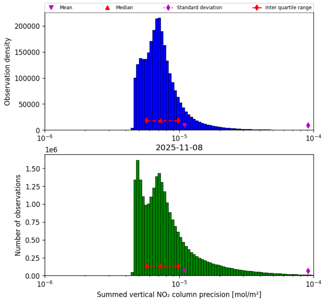
Figure 41: Histogram of “Summed vertical NO 2 column precision” for 2025-11-07 to 2025-11-09
