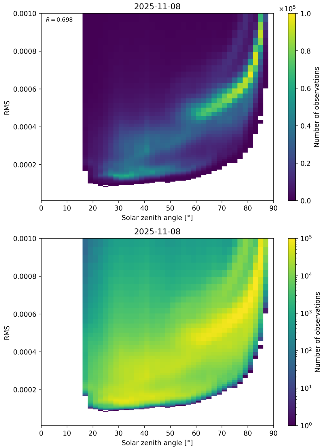
Figure 157: Scatter density plot of “Solar zenith angle” against “RMS” for 2025-11-07 to 2025-11-09.
