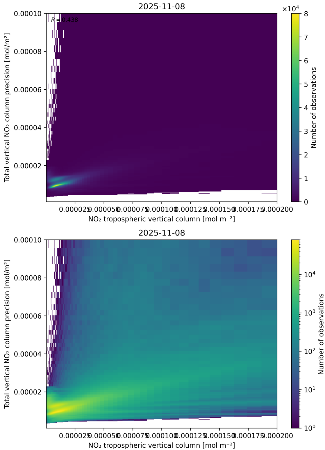
Figure 129: Scatter density plot of “NO 2 tropospheric vertical column” against “Total vertical NO 2 column precision” for 2025-11-07 to 2025-11-09.
