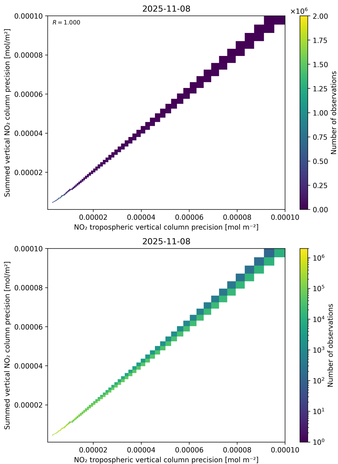
Figure 137: Scatter density plot of “NO 2 tropospheric vertical column precision” against “Summed vertical NO 2 column precision” for 2025-11-07 to 2025-11-09.
