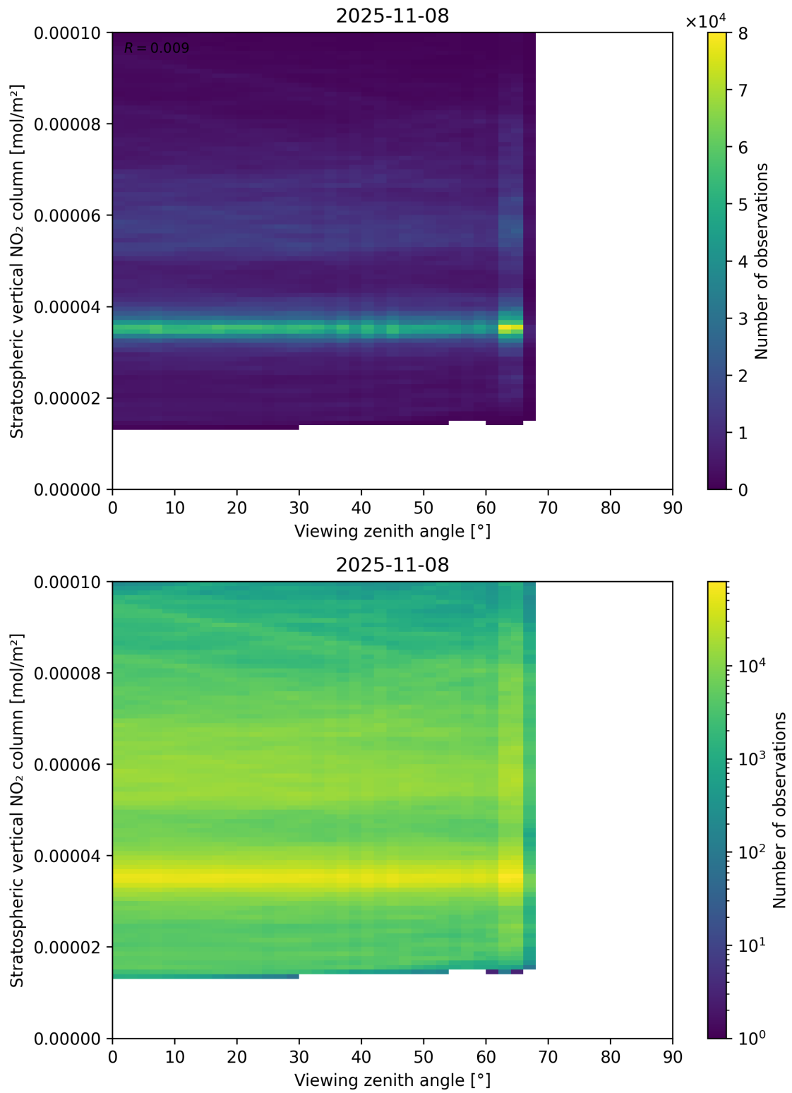
Figure 164: Scatter density plot of “Viewing zenith angle” against “Stratospheric vertical NO 2 column” for 2025-11-07 to 2025-11-09.
