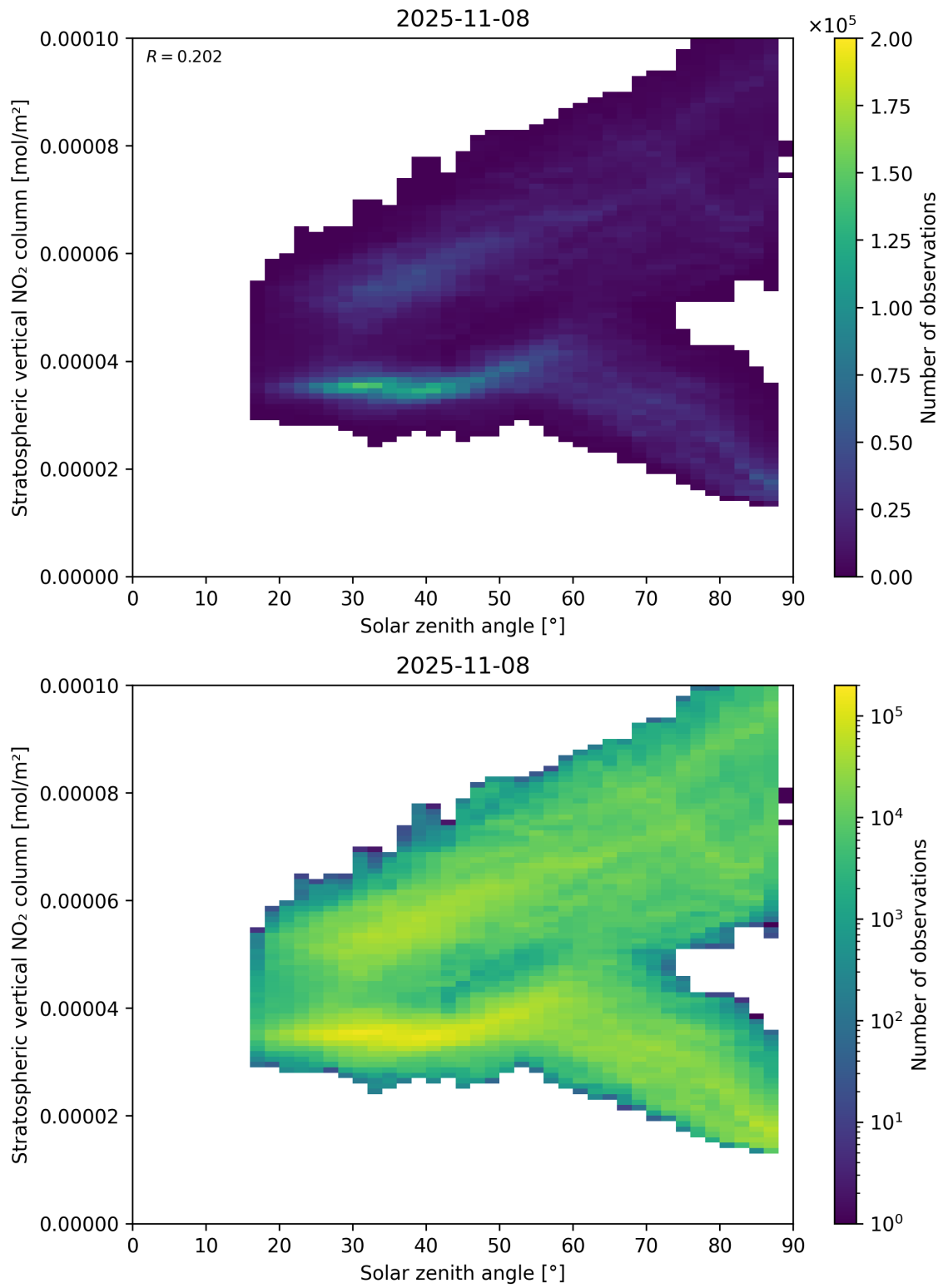
Figure 150: Scatter density plot of “Solar zenith angle” against “Stratospheric vertical NO 2 column” for 2025-11-07 to 2025-11-09.
