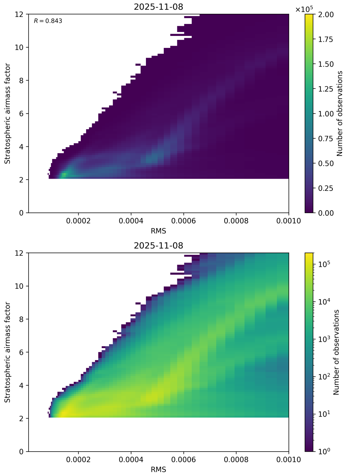
Figure 144: Scatter density plot of “RMS” against “Stratospheric airmass factor” for 2025-11-07 to 2025-11-09.
