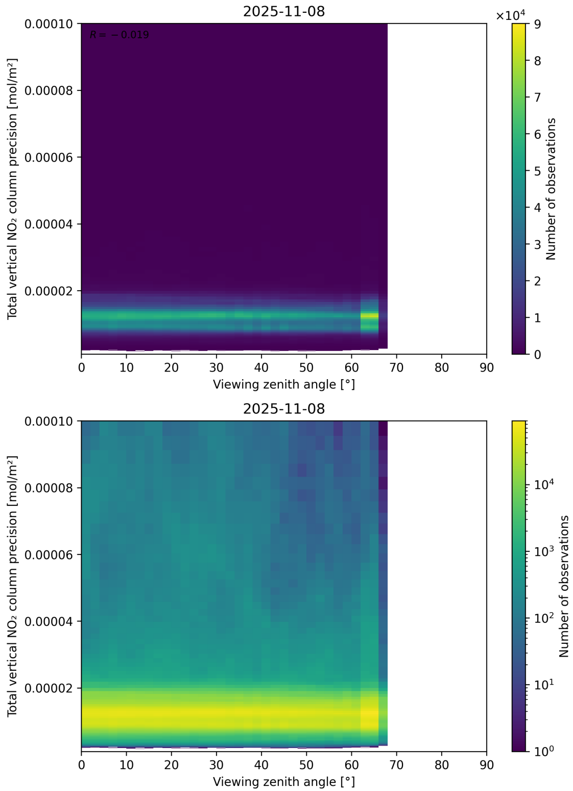
Figure 168: Scatter density plot of “Viewing zenith angle” against “Total vertical NO 2 column precision” for 2025-11-07 to 2025-11-09.
