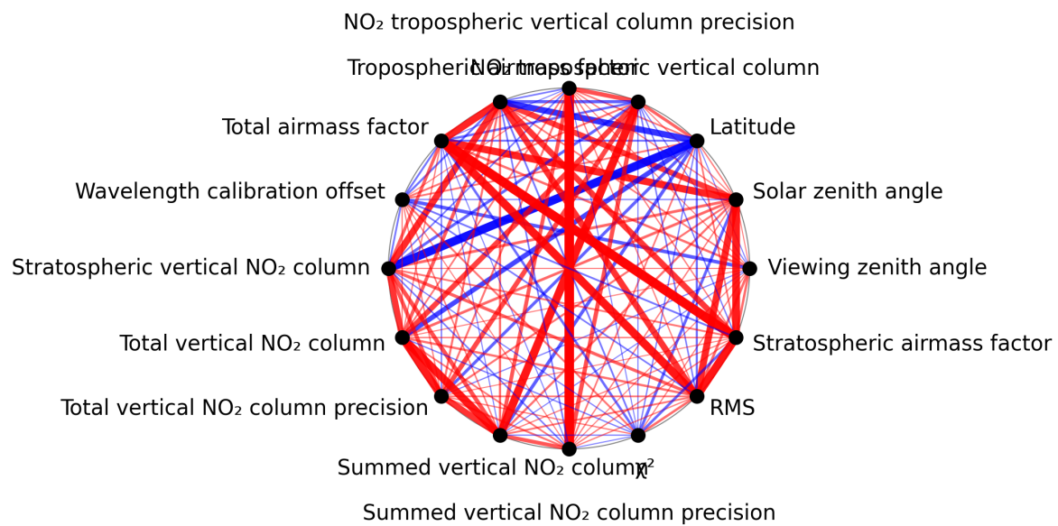
Figure 1: Map of correlation graph for 2025-11-07 to 2025-11-09.
