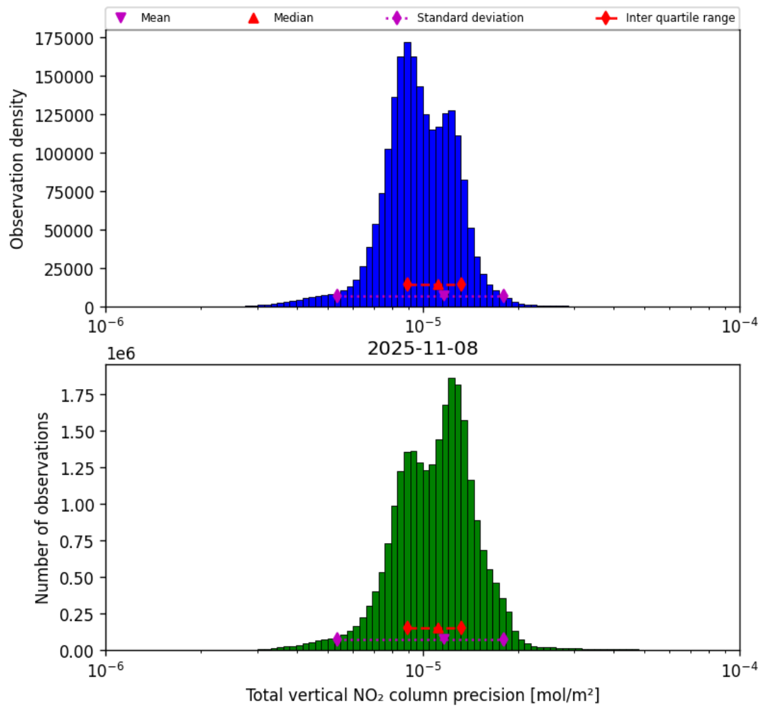
Figure 39: Histogram of “Total vertical NO 2 column precision” for 2025-11-07 to 2025-11-09
