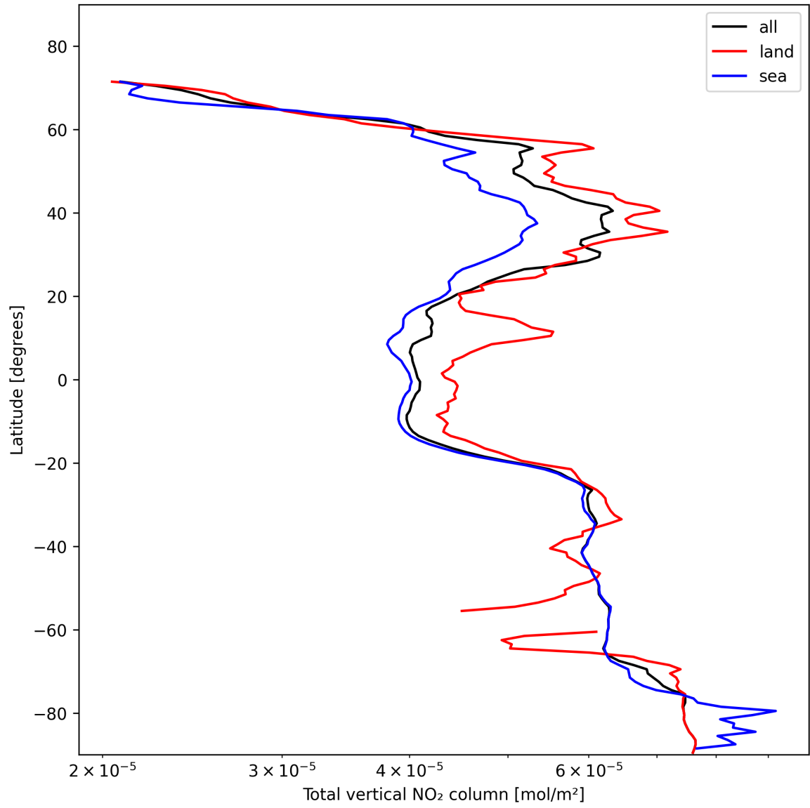
Figure 21: Zonal average of “Total vertical NO 2 column” for 2025-11-07 to 2025-11-09.
