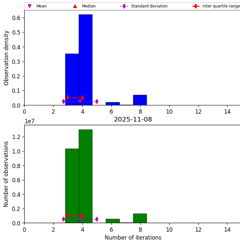
Figure 34: Histogram of “Number of iterations” for 2025-11-07 to 2025-11-09
