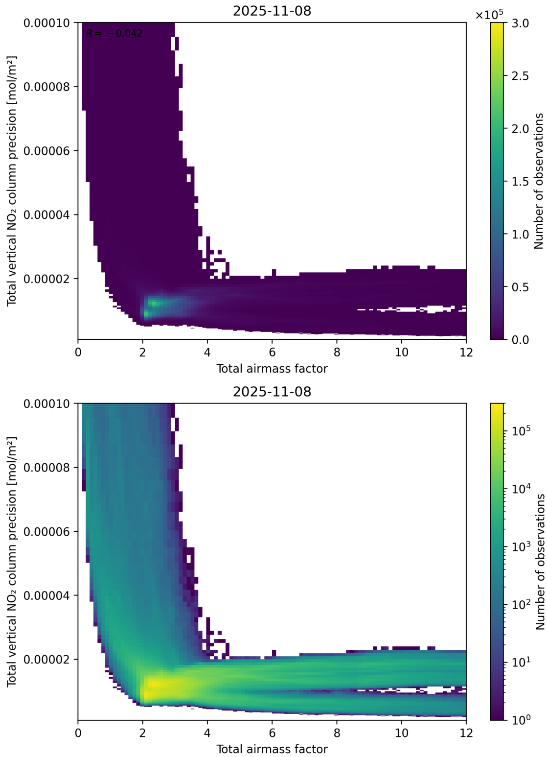
Figure 68: Scatter density plot of “Total airmass factor” against “Total vertical NO 2 column precision” for 2025-11-07 to 2025-11-09.
