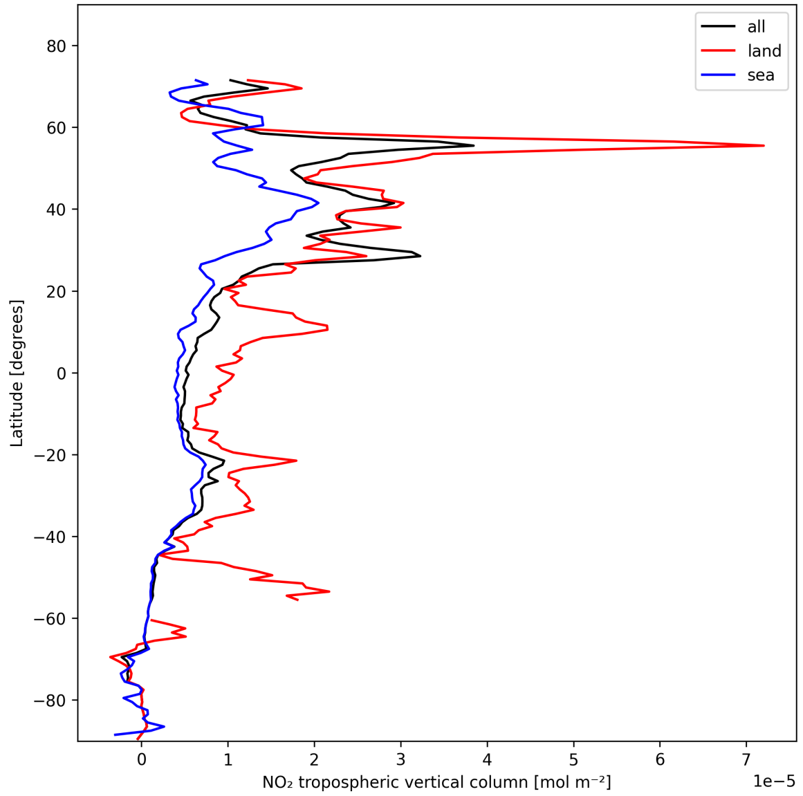
Figure 12: Zonal average of “NO 2 tropospheric vertical column” for 2025-11-07 to 2025-11-09.
