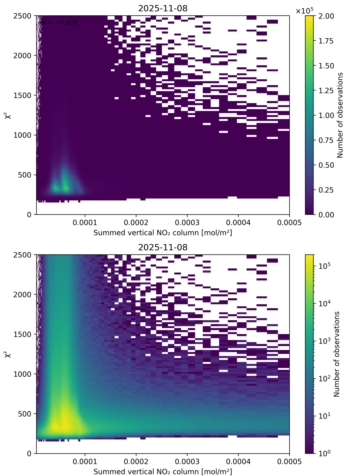
Figure 104: Scatter density plot of “Summed vertical NO 2 column” against “ \chi^2 ” for 2025-11-07 to 2025-11-09.
