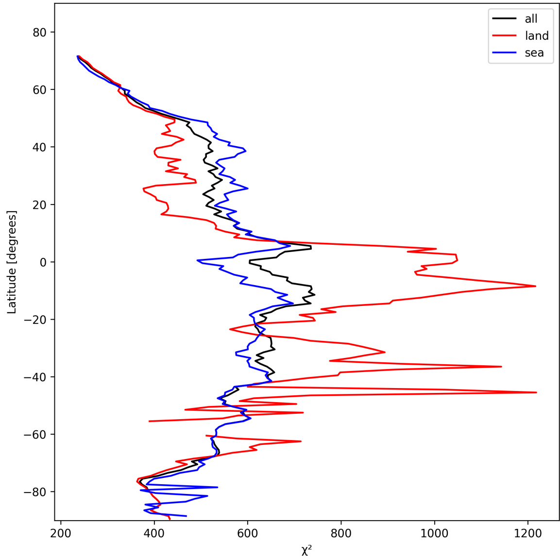
Figure 25: Zonal average of “ \chi^2 ” for 2025-11-07 to 2025-11-09.
