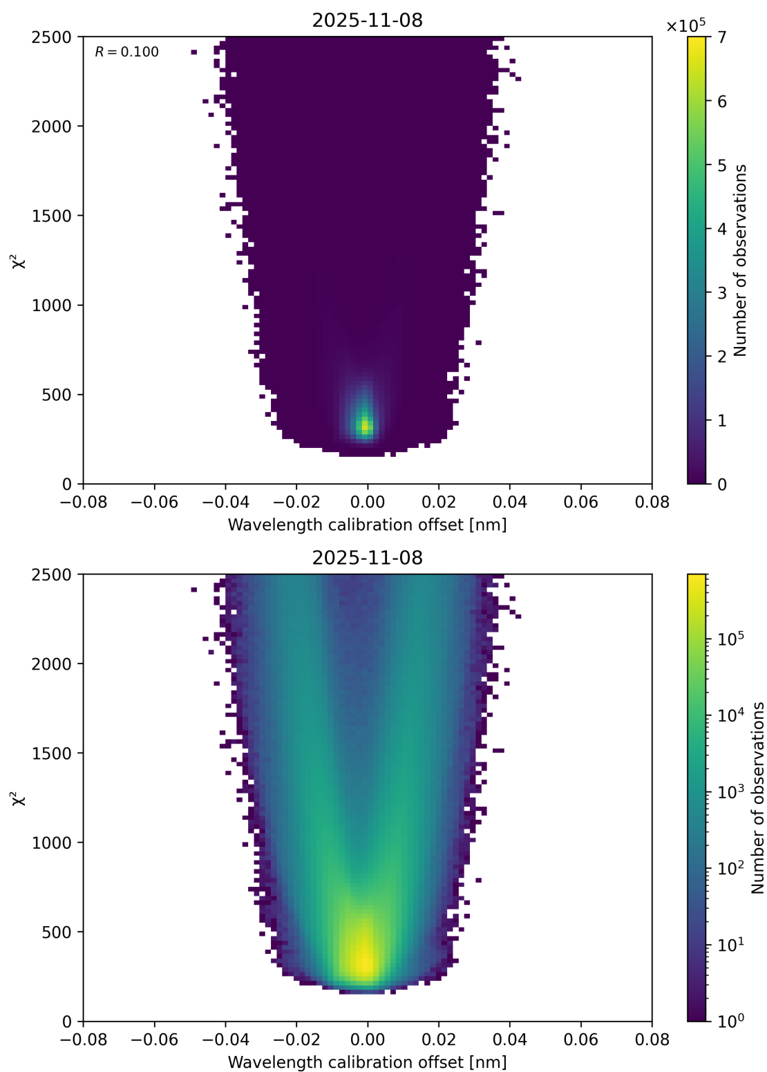
Figure 175: Scatter density plot of “Wavelength calibration offset” against “ \chi^2 ” for 2025-11-07 to 2025-11-09.
