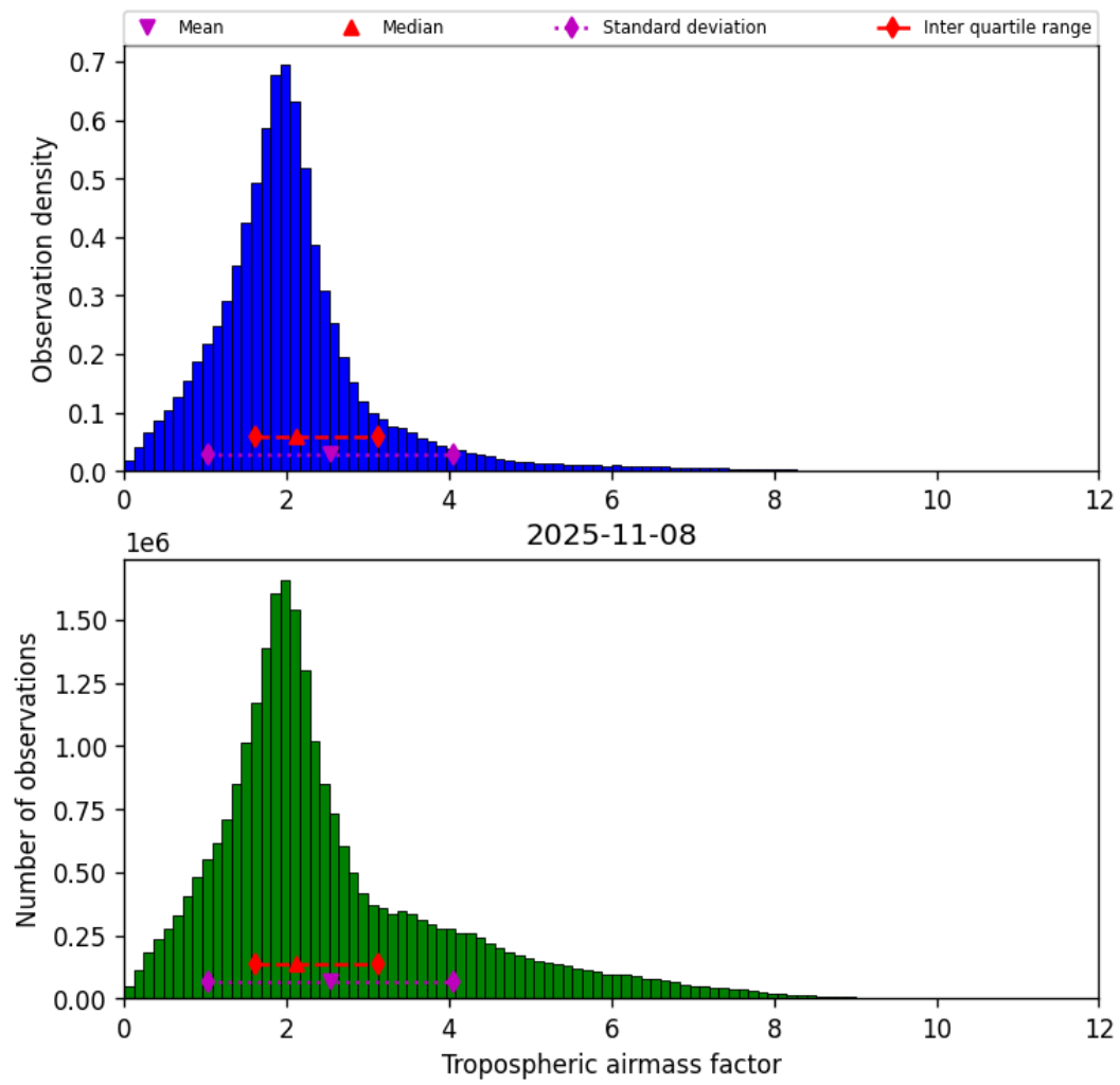
Figure 31: Histogram of “Tropospheric airmass factor” for 2025-11-07 to 2025-11-09
