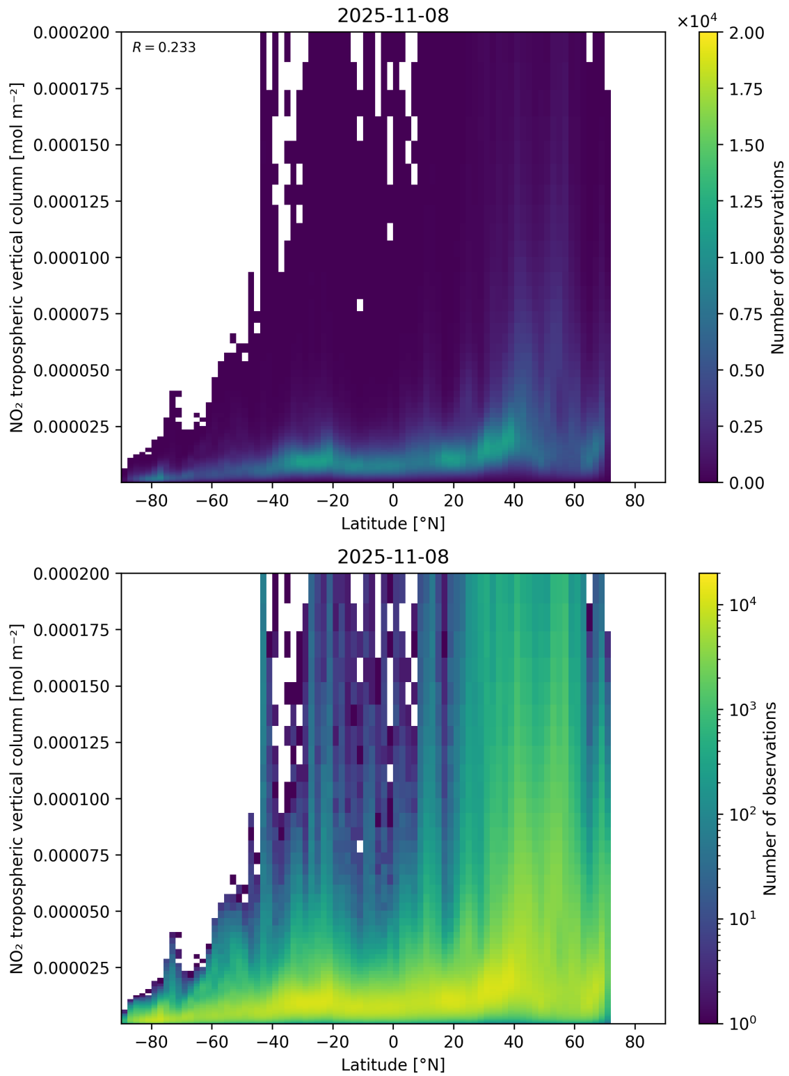
Figure 92: Scatter density plot of “Latitude” against “NO 2 tropospheric vertical column” for 2025-11-07 to 2025-11-09.
