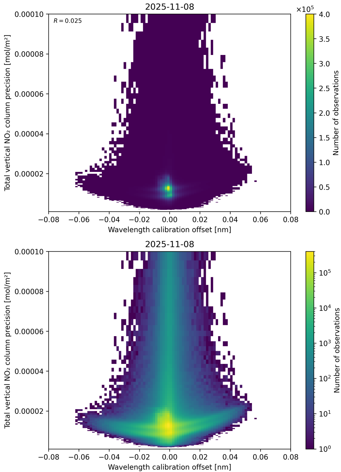
Figure 180: Scatter density plot of “Wavelength calibration offset” against “Total vertical NO 2 column precision” for 2025-11-07 to 2025-11-09.
