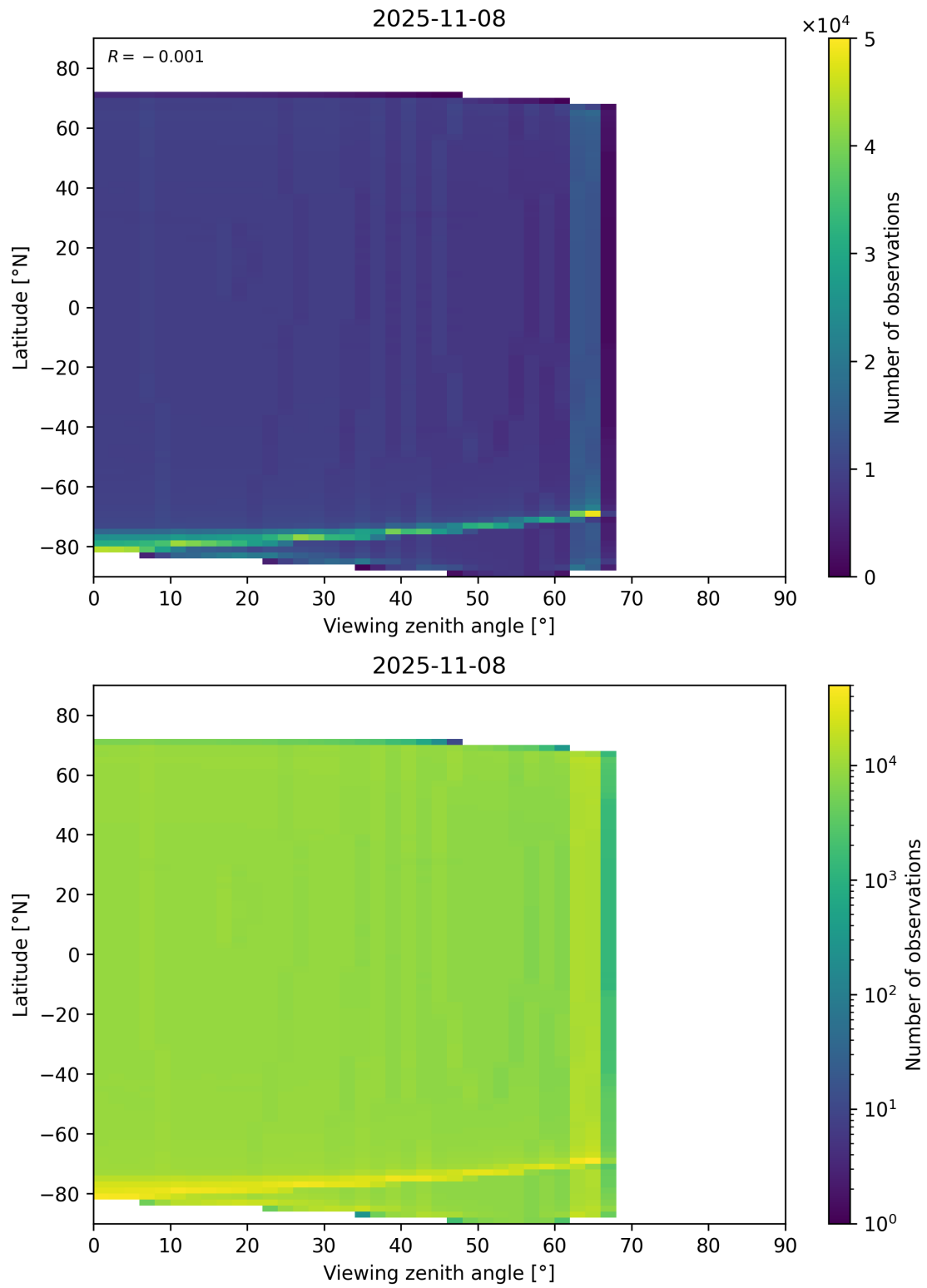
Figure 163: Scatter density plot of “Viewing zenith angle” against “Latitude” for 2025-11-07 to 2025-11-09.
