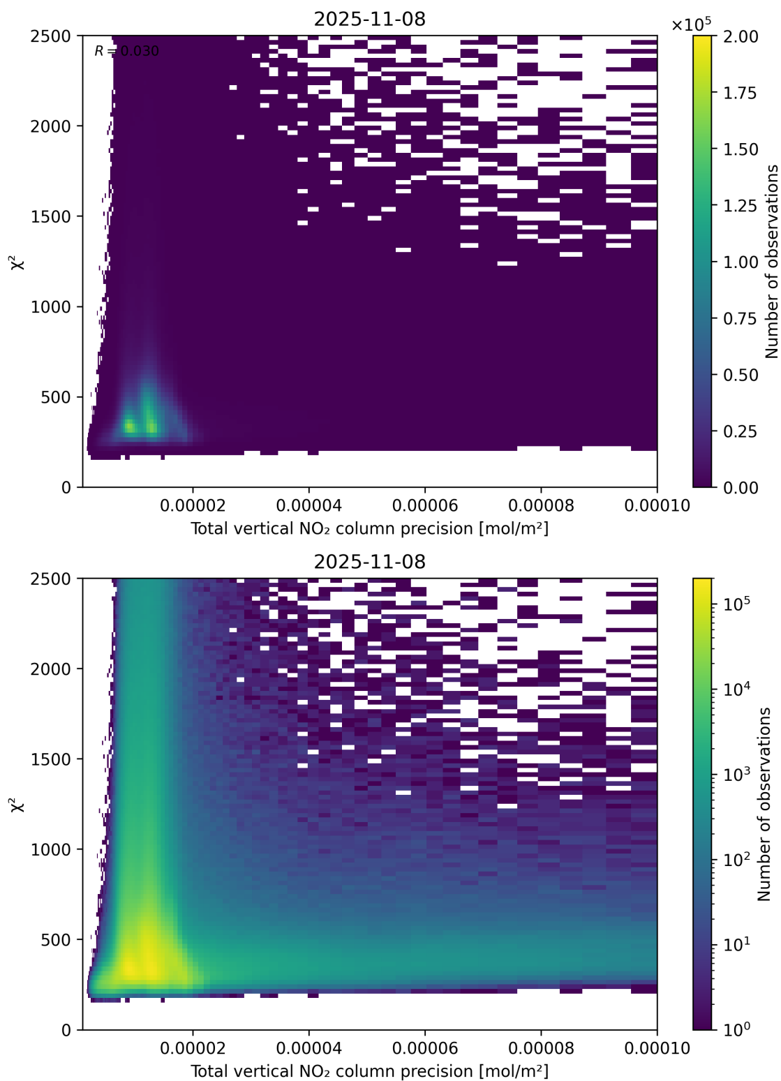
Figure 116: Scatter density plot of “Total vertical NO 2 column precision” against “ \chi^2 ” for 2025-11-07 to 2025-11-09.
