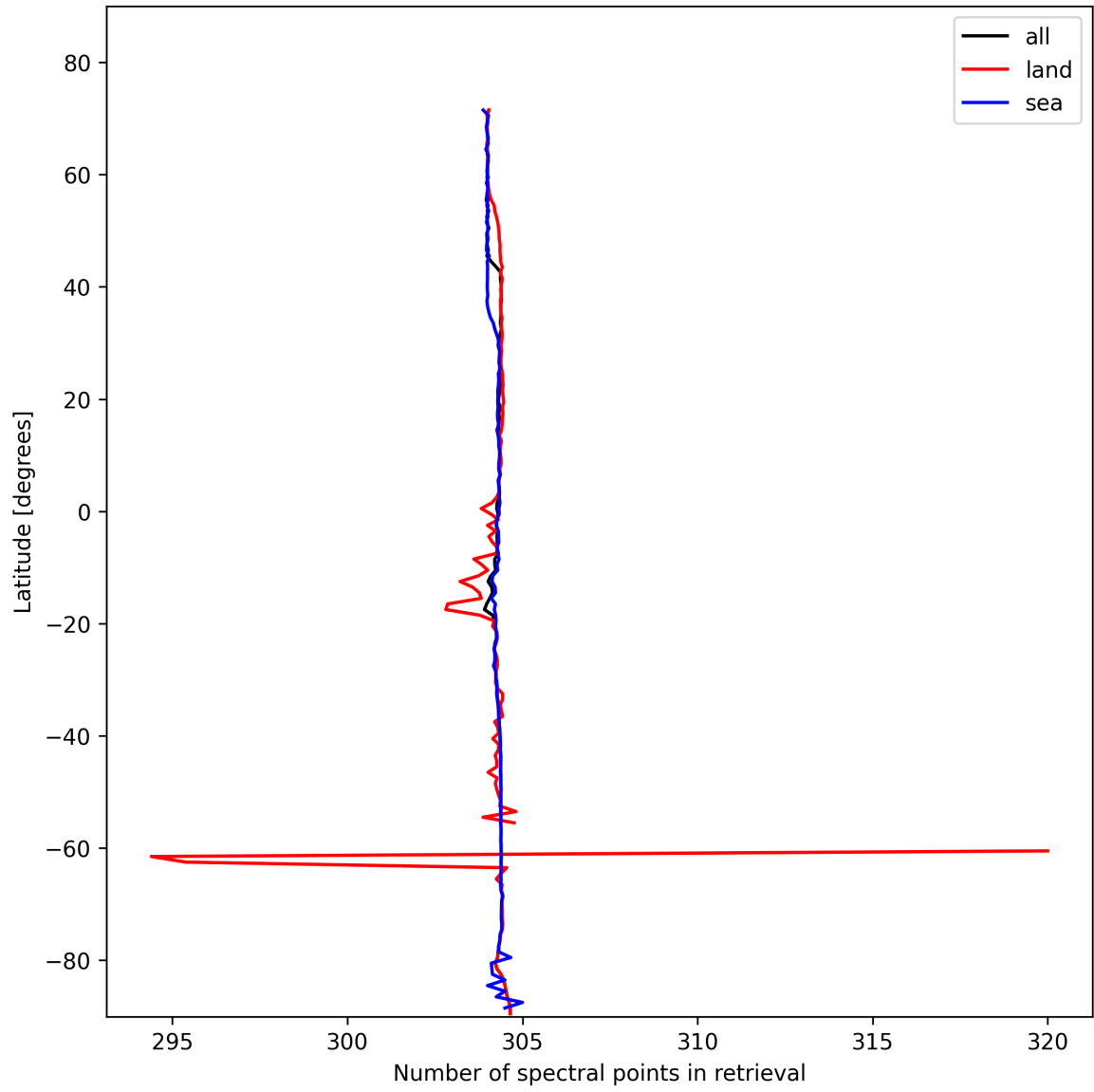
Figure 16: Zonal average of “Number of spectral points in retrieval” for 2025-11-07 to 2025-11-09.
