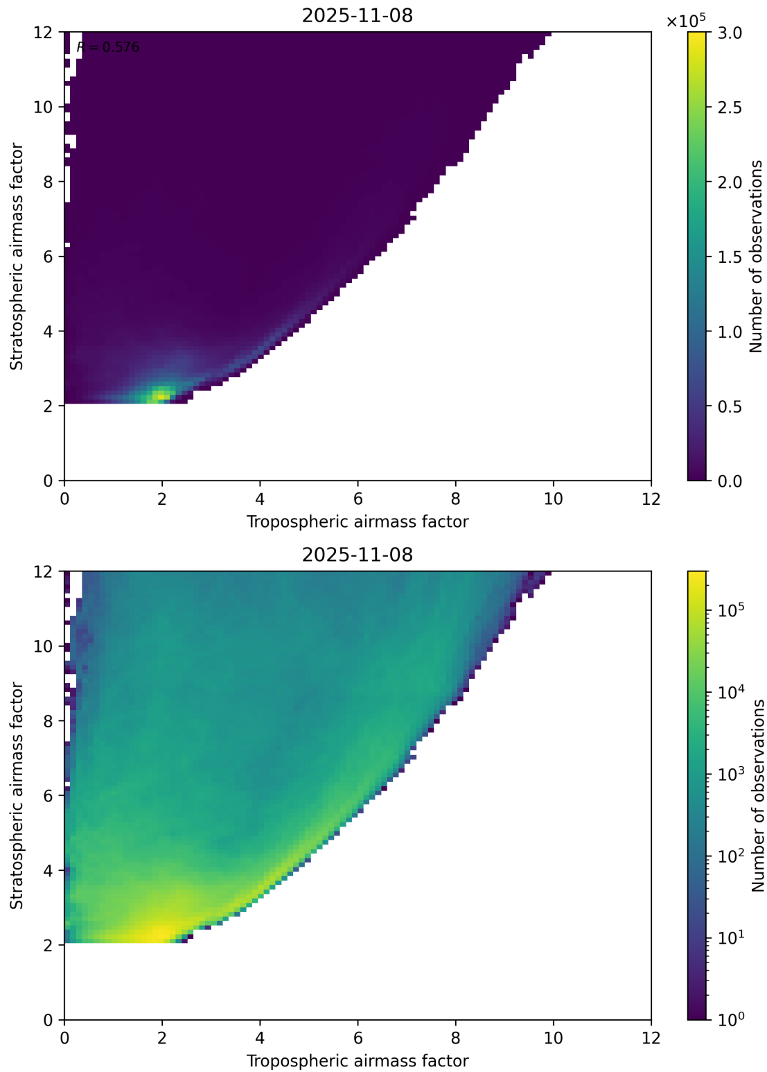
Figure 71: Scatter density plot of “Tropospheric airmass factor” against “Stratospheric airmass factor” for 2025-11-07 to 2025-11-09.
