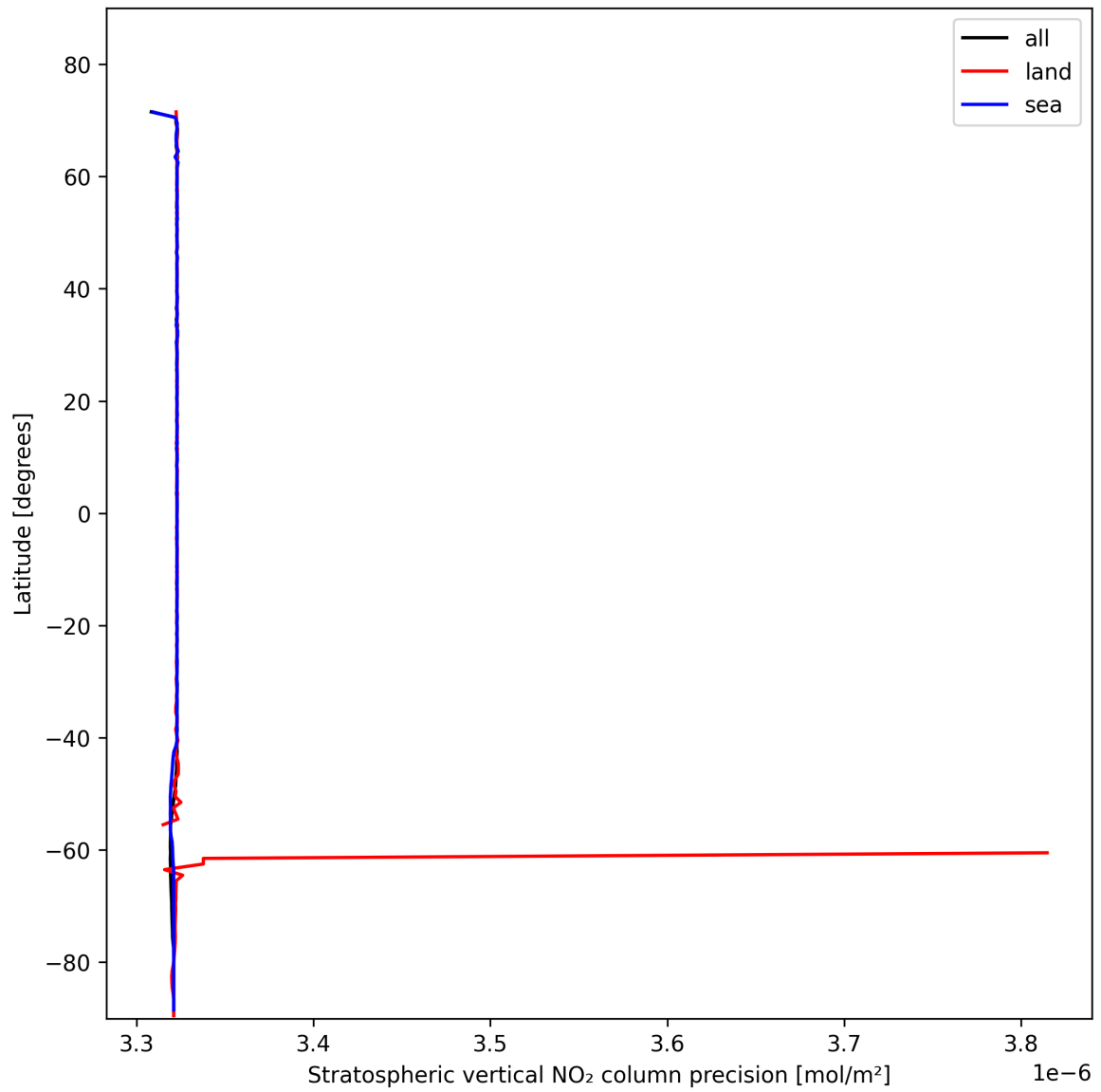
Figure 20: Zonal average of “Stratospheric vertical NO 2 column precision” for 2025-11-07 to 2025-11-09.
