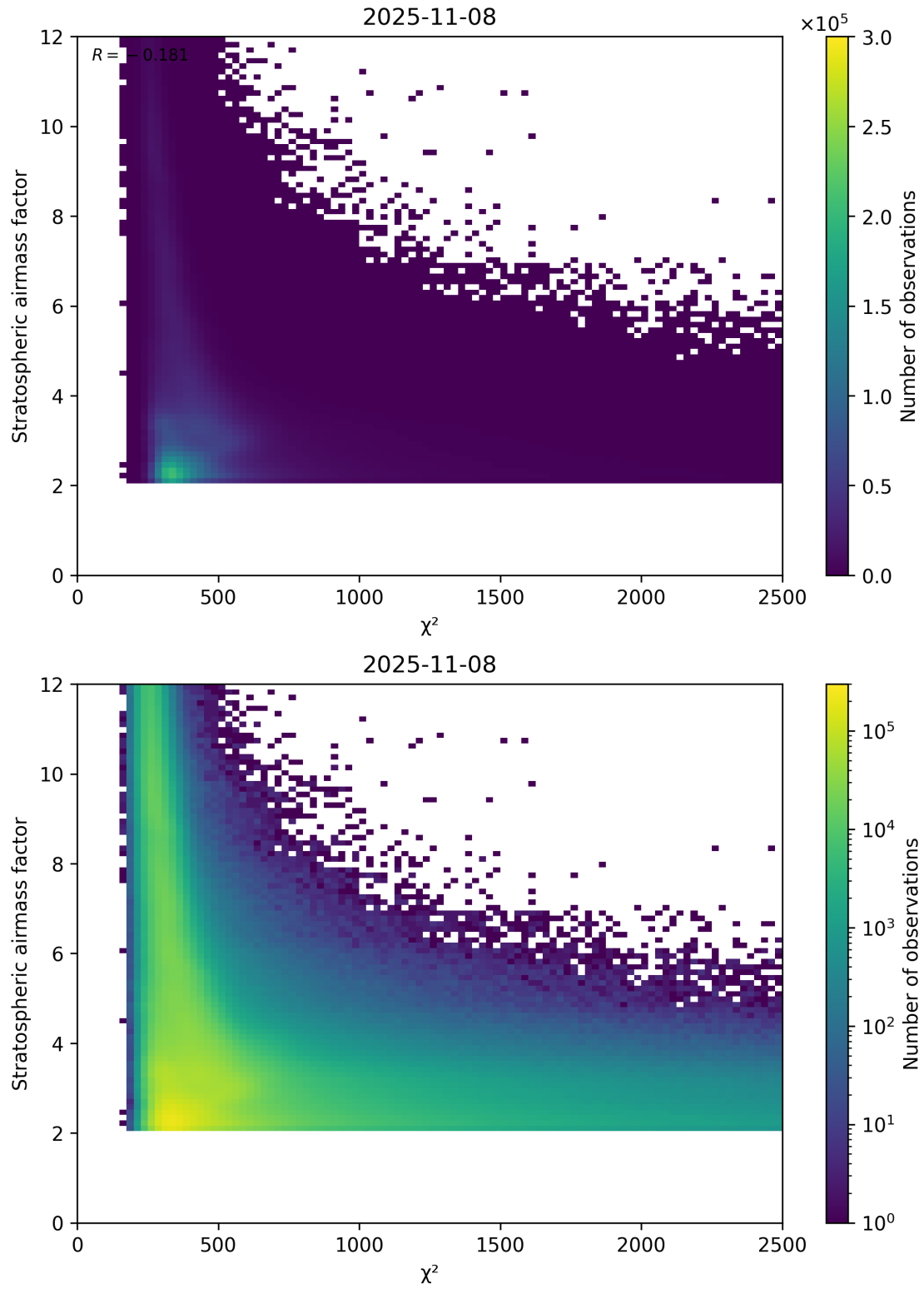
Figure 81: Scatter density plot of “ \chi^2 ” against “Stratospheric airmass factor” for 2025-11-07 to 2025-11-09.
