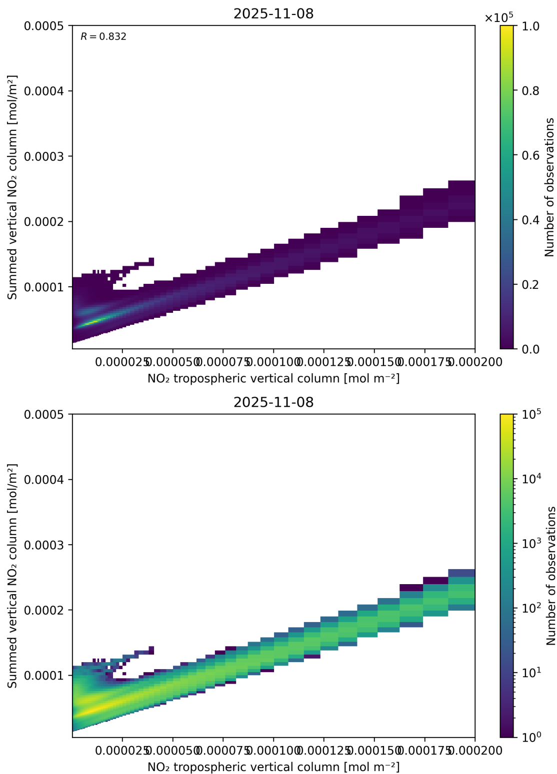
Figure 126: Scatter density plot of “NO 2 tropospheric vertical column” against “Summed vertical NO 2 column” for 2025-11-07 to 2025-11-09.
