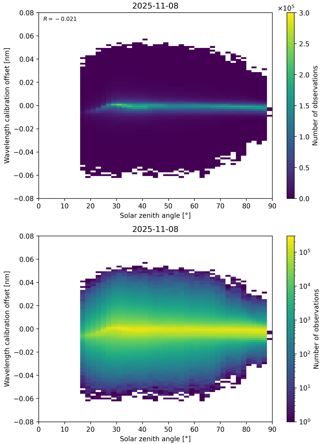
Figure 158: Scatter density plot of “Solar zenith angle” against “Wavelength calibration offset” for 2025-11-07 to 2025-11-09.
