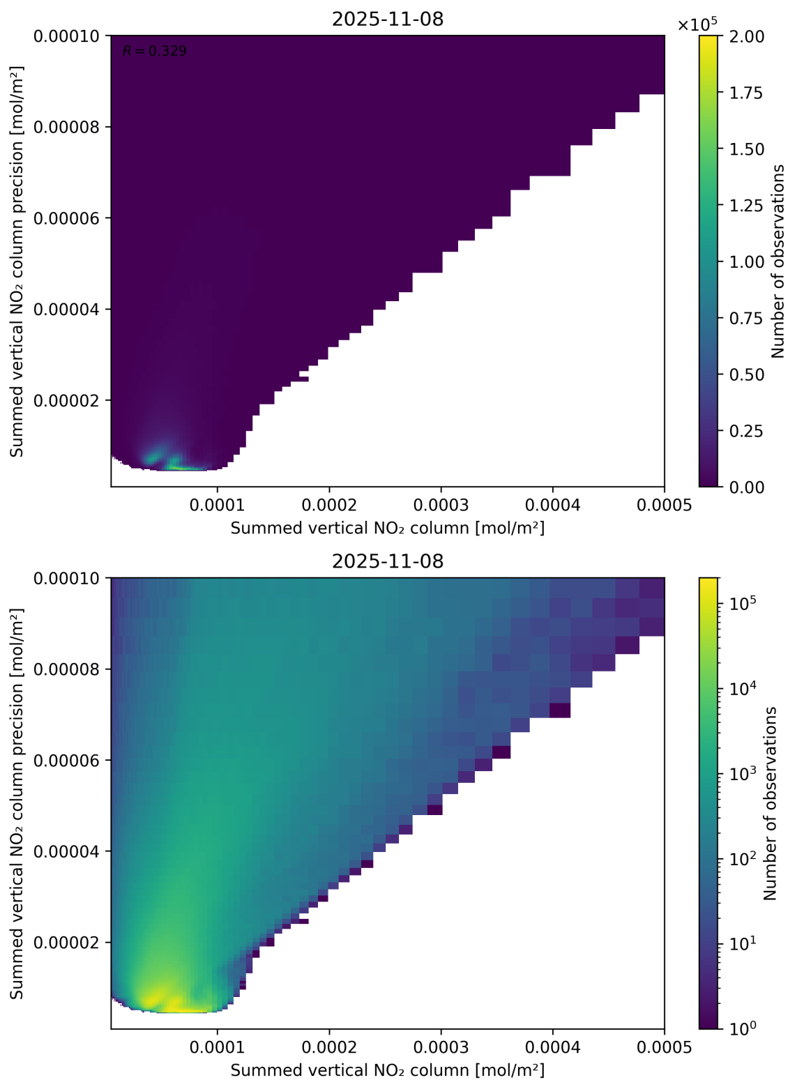
Figure 105: Scatter density plot of “Summed vertical NO 2 column” against “Summed vertical NO 2 column precision” for 2025-11-07 to 2025-11-09.
