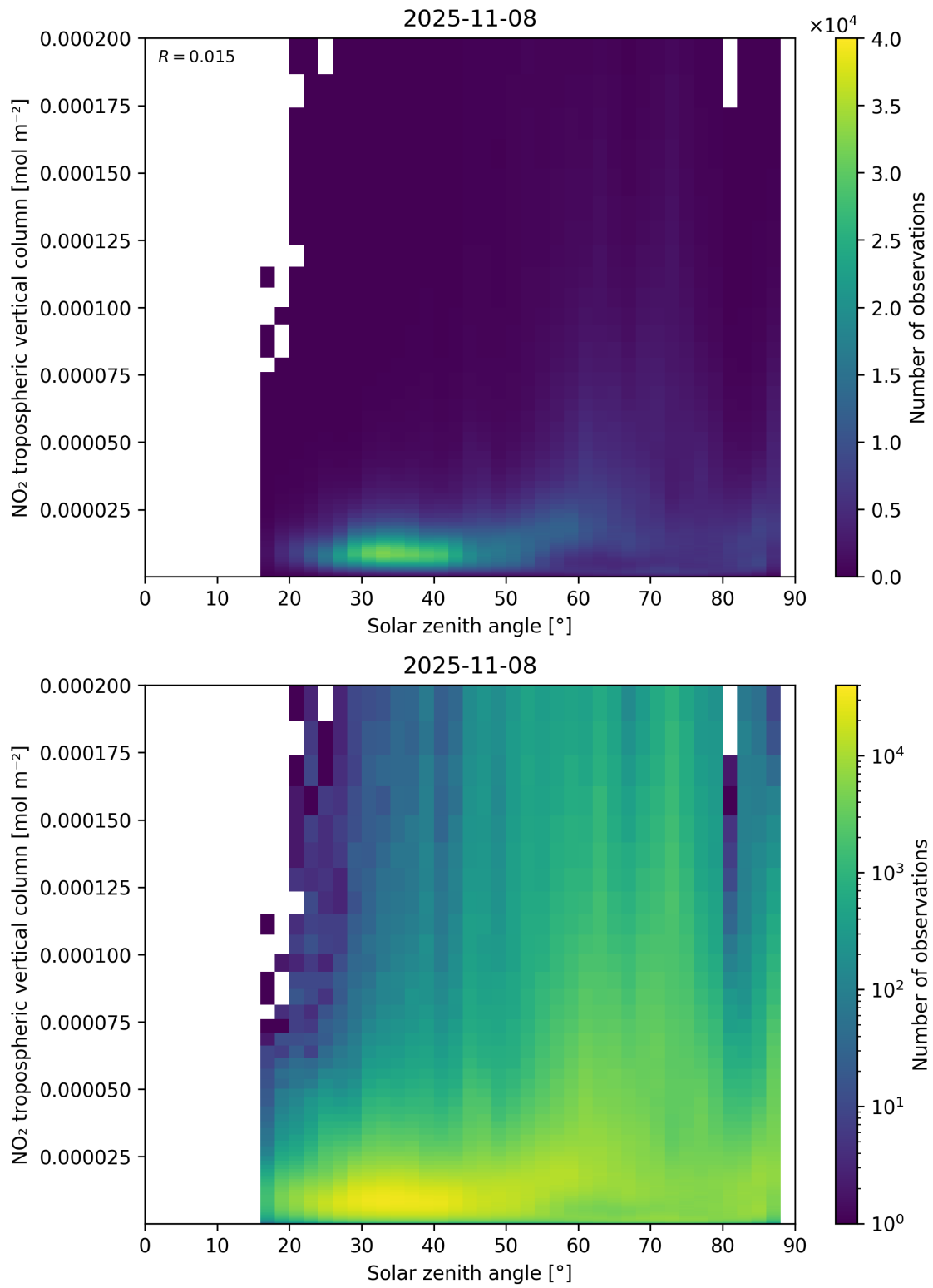
Figure 155: Scatter density plot of “Solar zenith angle” against “NO 2 tropospheric vertical column” for 2025-11-07 to 2025-11-09.
