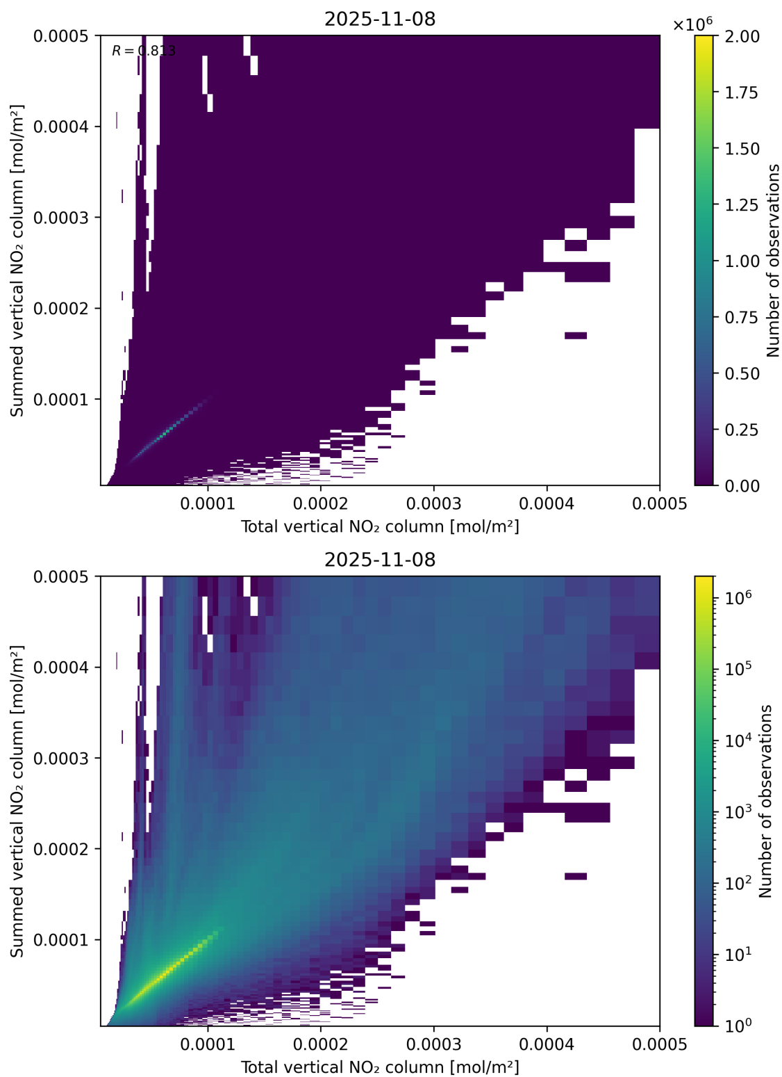
Figure 112: Scatter density plot of “Total vertical NO 2 column” against “Summed vertical NO 2 column” for 2025-11-07 to 2025-11-09.
