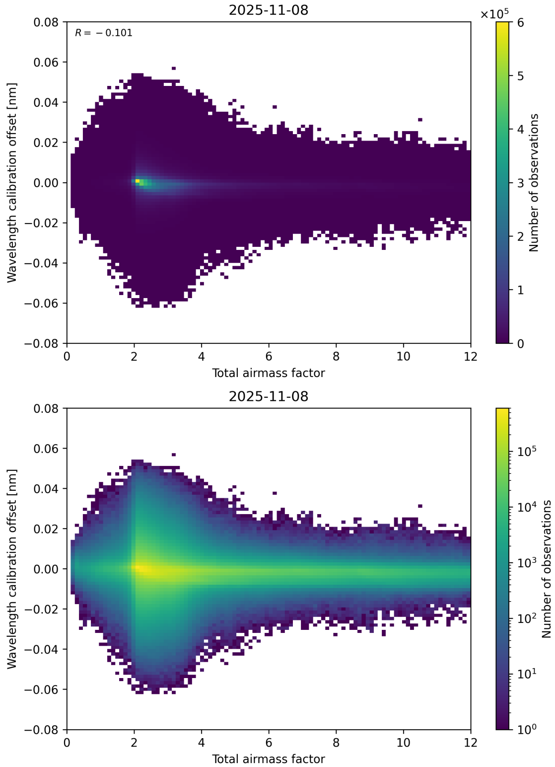
Figure 70: Scatter density plot of “Total airmass factor” against “Wavelength calibration offset” for 2025-11-07 to 2025-11-09.
