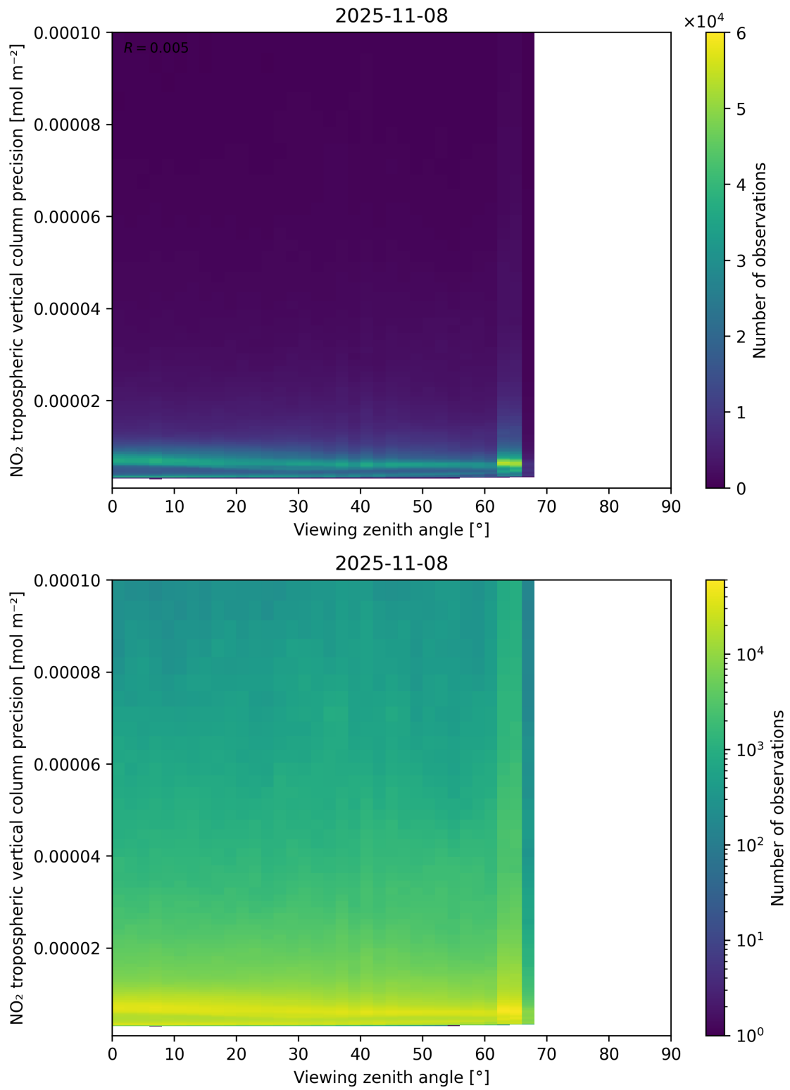
Figure 170: Scatter density plot of “Viewing zenith angle” against “NO 2 tropospheric vertical column precision” for 2025-11-07 to 2025-11-09.
