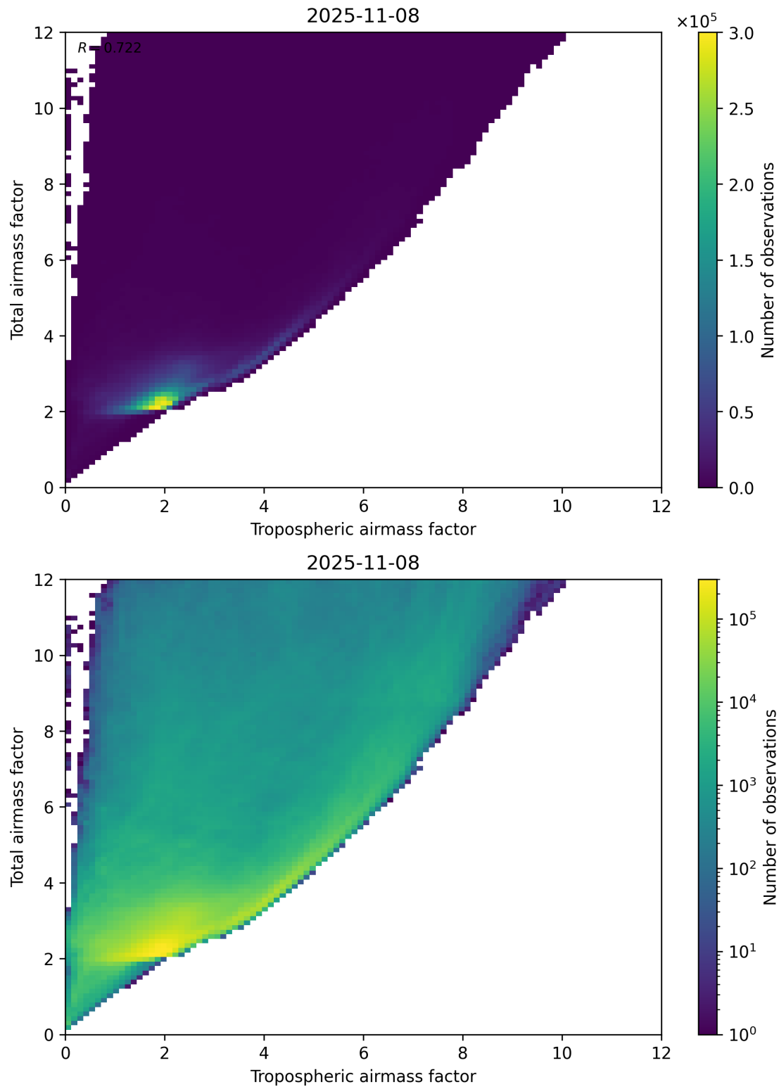
Figure 72: Scatter density plot of “Tropospheric airmass factor” against “Total airmass factor” for 2025-11-07 to 2025-11-09.
