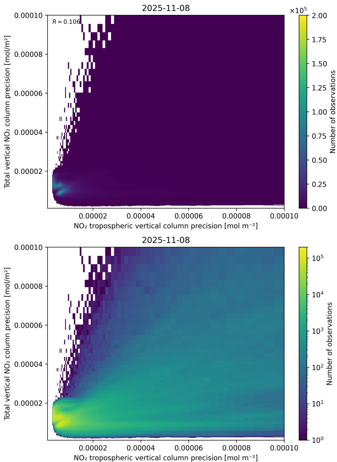
Figure 139: Scatter density plot of “NO 2 tropospheric vertical column precision” against “Total vertical NO 2 column precision” for 2025-11-07 to 2025-11-09.
