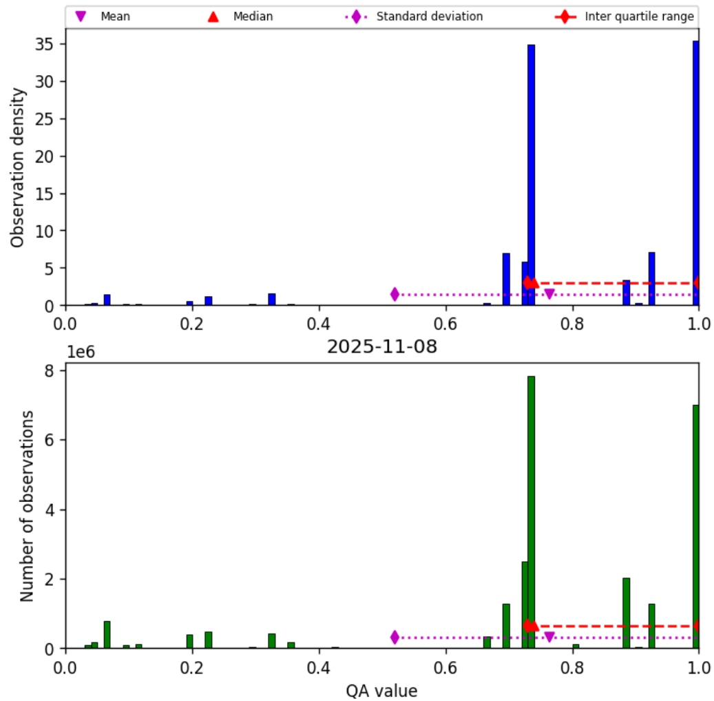
Figure 28: Histogram of “QA value” for 2025-11-07 to 2025-11-09
