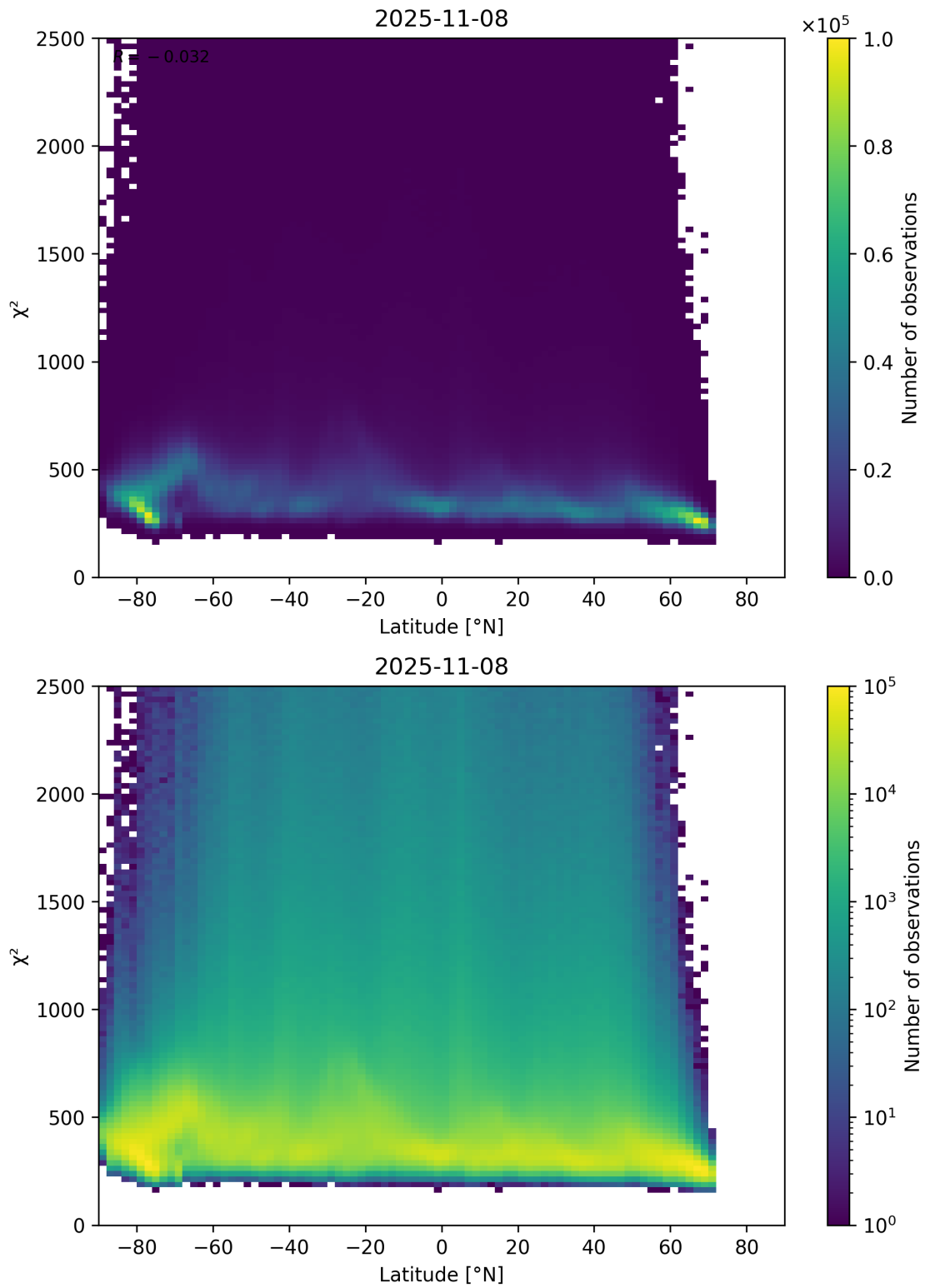
Figure 86: Scatter density plot of “Latitude” against “ \chi^2 ” for 2025-11-07 to 2025-11-09.
