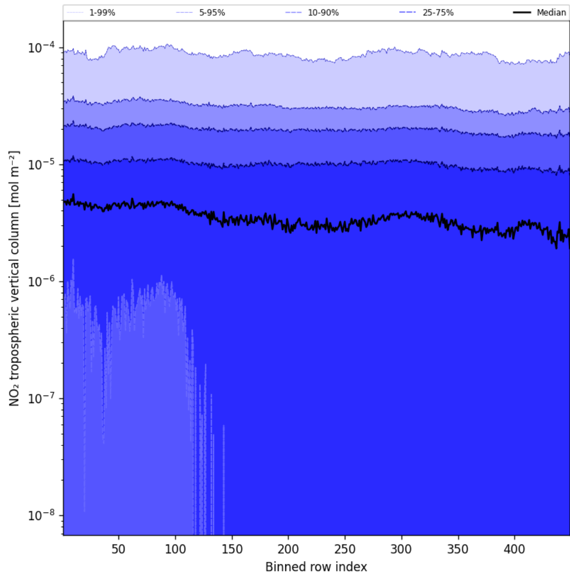
Figure 46: Along track statistics of “NO 2 tropospheric vertical column” for 2025-11-07 to 2025-11-09
