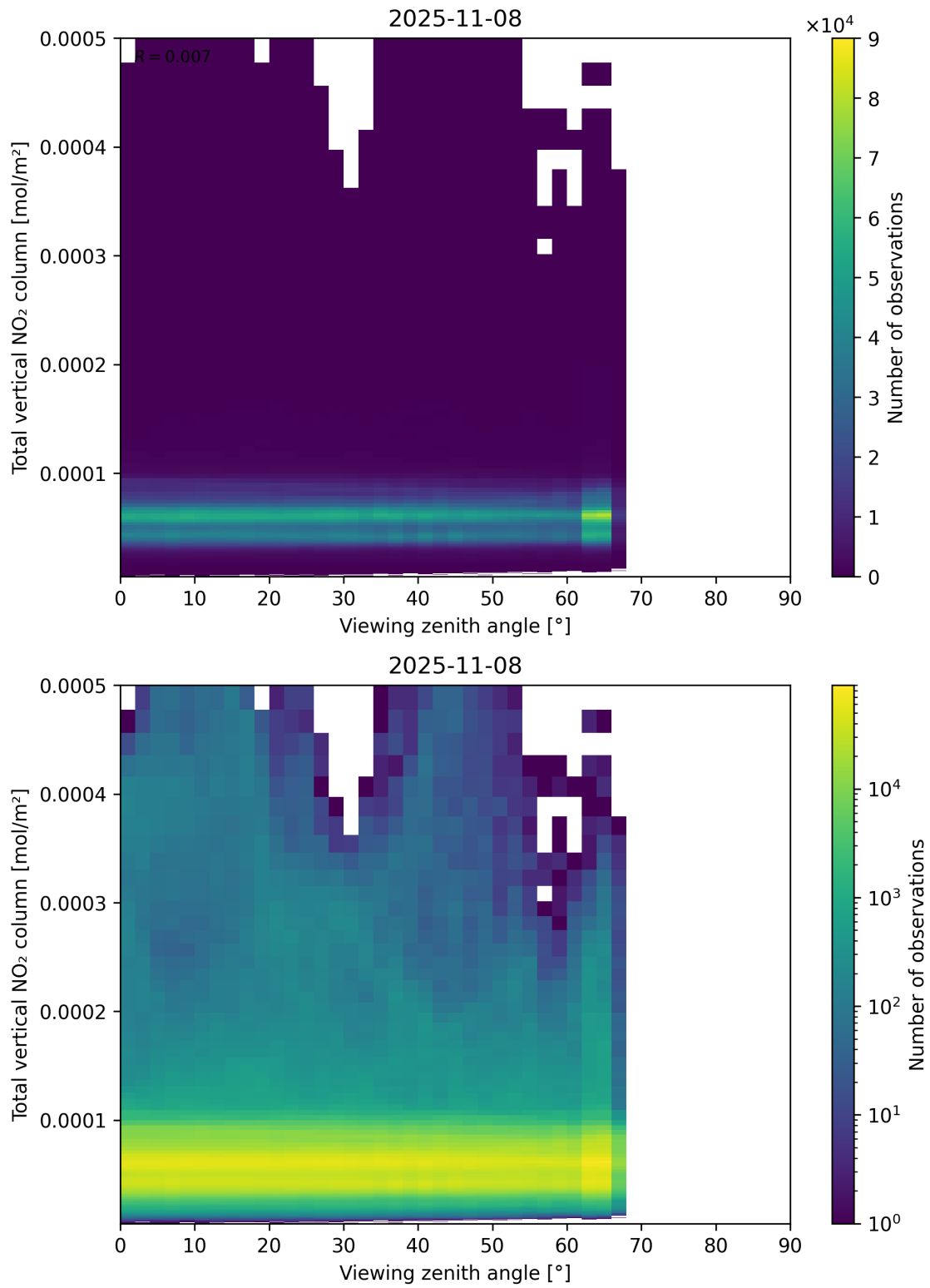
Figure 167: Scatter density plot of “Viewing zenith angle” against “Total vertical NO 2 column” for 2025-11-07 to 2025-11-09.
