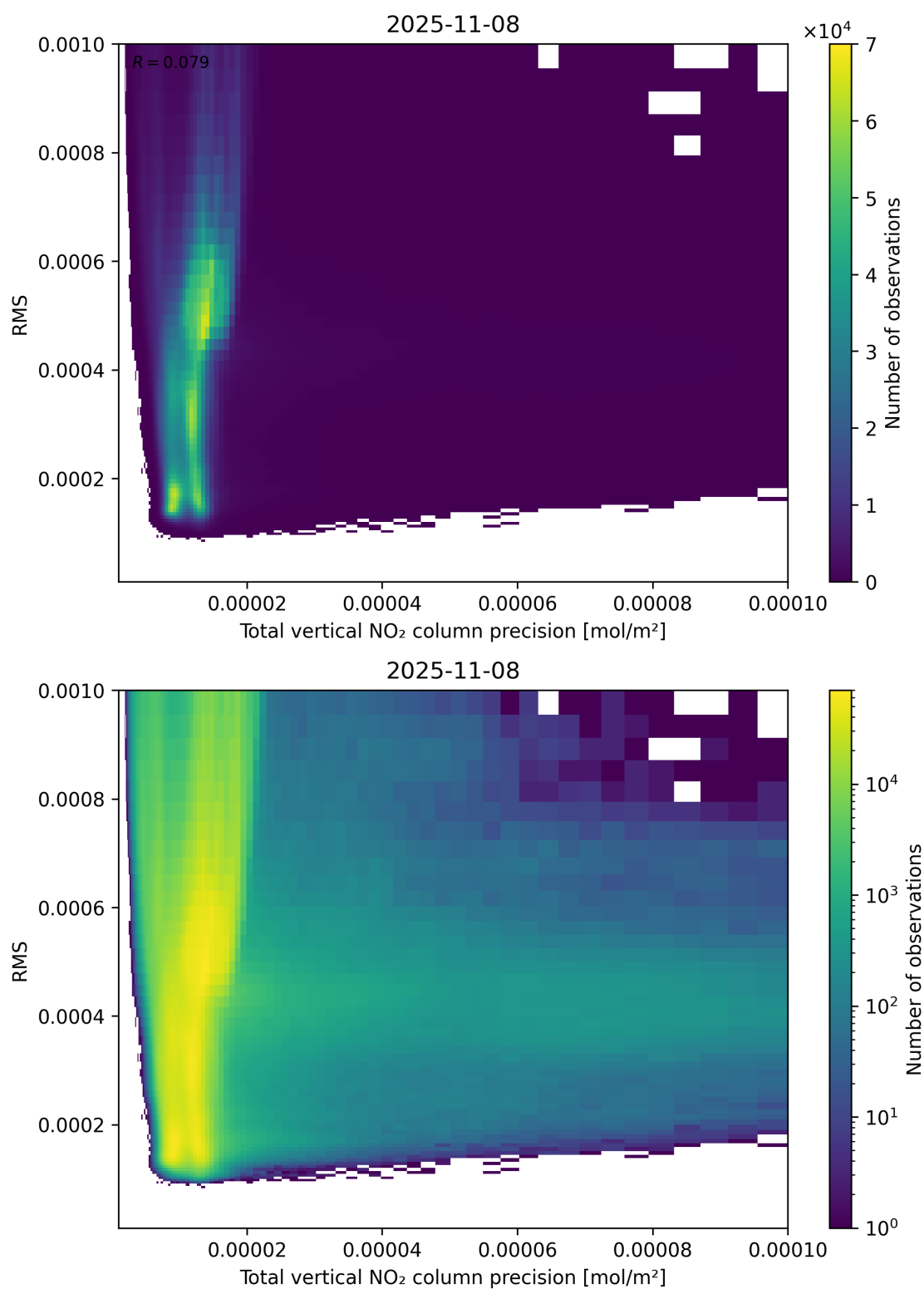
Figure 119: Scatter density plot of “Total vertical NO 2 column precision” against “RMS” for 2025-11-07 to 2025-11-09.
