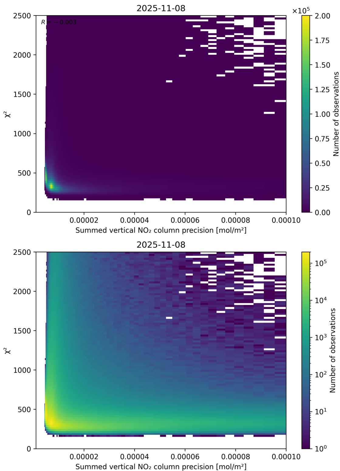
Figure 107: Scatter density plot of “Summed vertical NO 2 column precision” against “ \chi^2 ” for 2025-11-07 to 2025-11-09.
