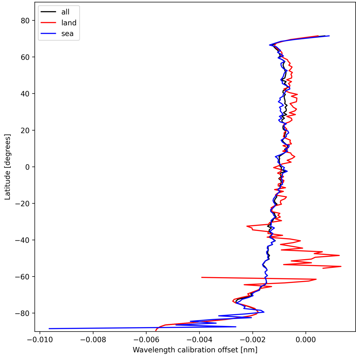
Figure 18: Zonal average of “Wavelength calibration offset” for 2025-11-07 to 2025-11-09.
