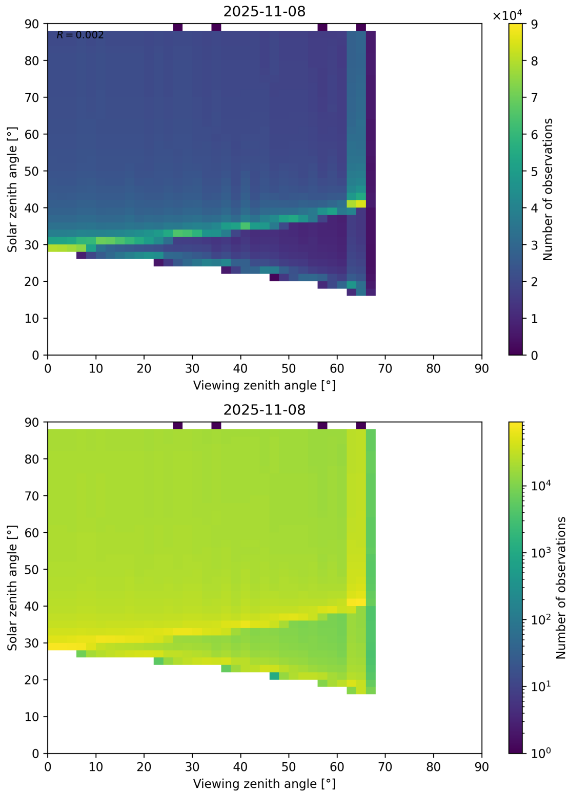
Figure 172: Scatter density plot of “Viewing zenith angle” against “Solar zenith angle” for 2025-11-07 to 2025-11-09.
