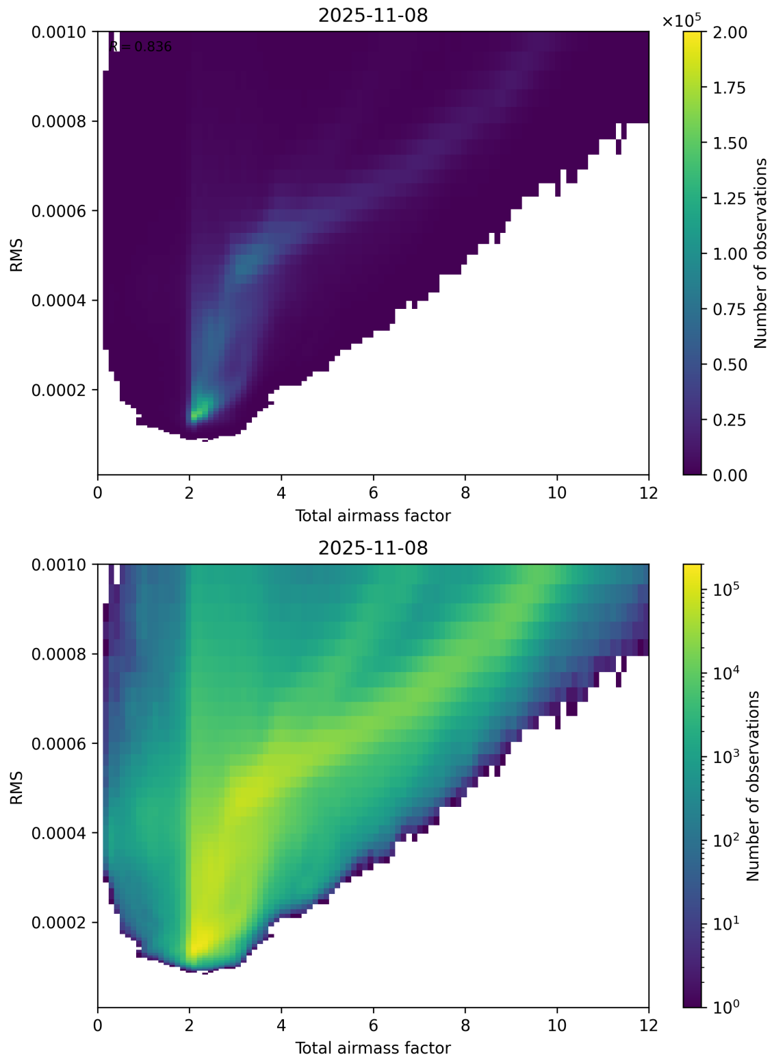
Figure 69: Scatter density plot of “Total airmass factor” against “RMS” for 2025-11-07 to 2025-11-09.
