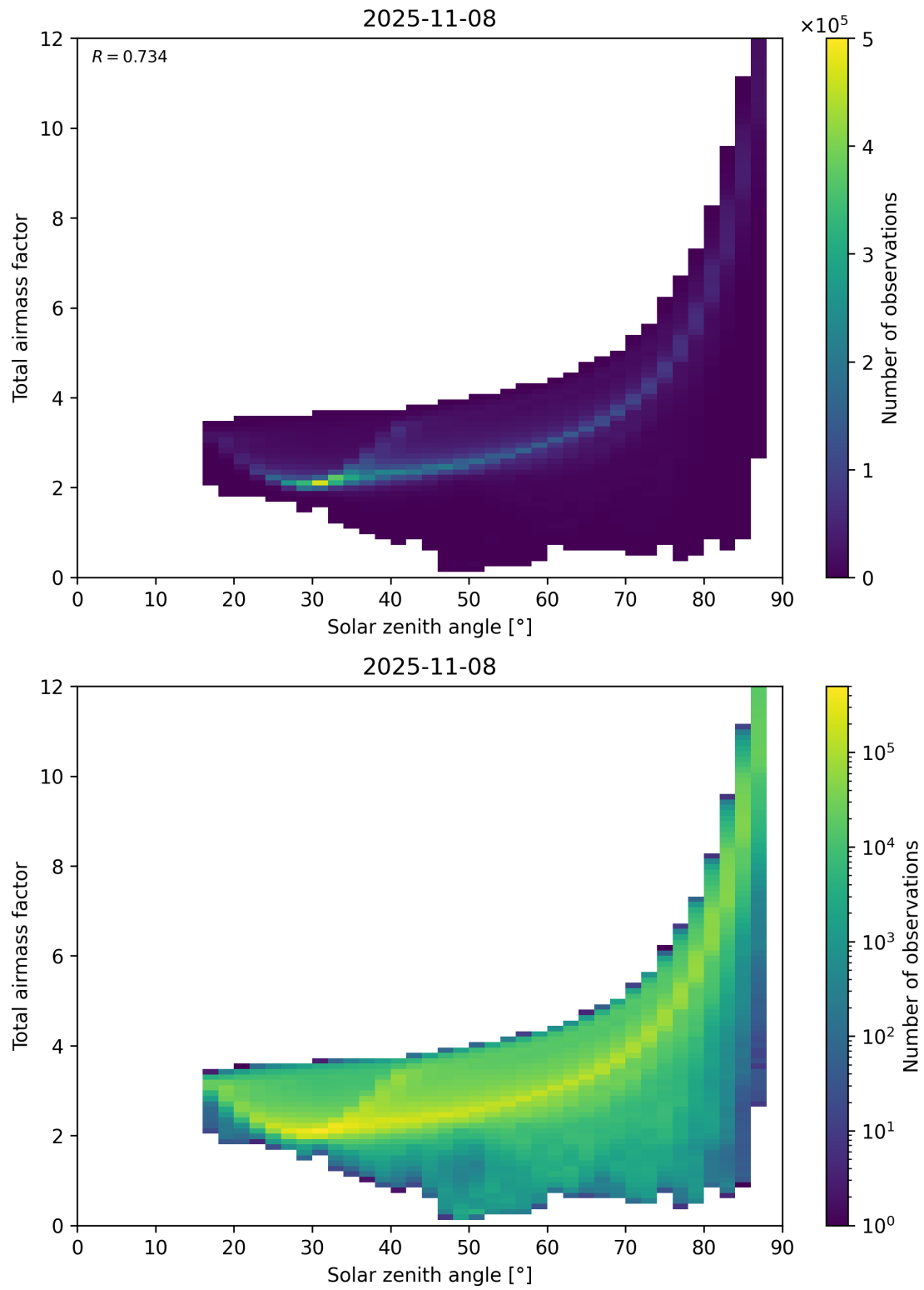
Figure 146: Scatter density plot of “Solar zenith angle” against “Total airmass factor” for 2025-11-07 to 2025-11-09.
