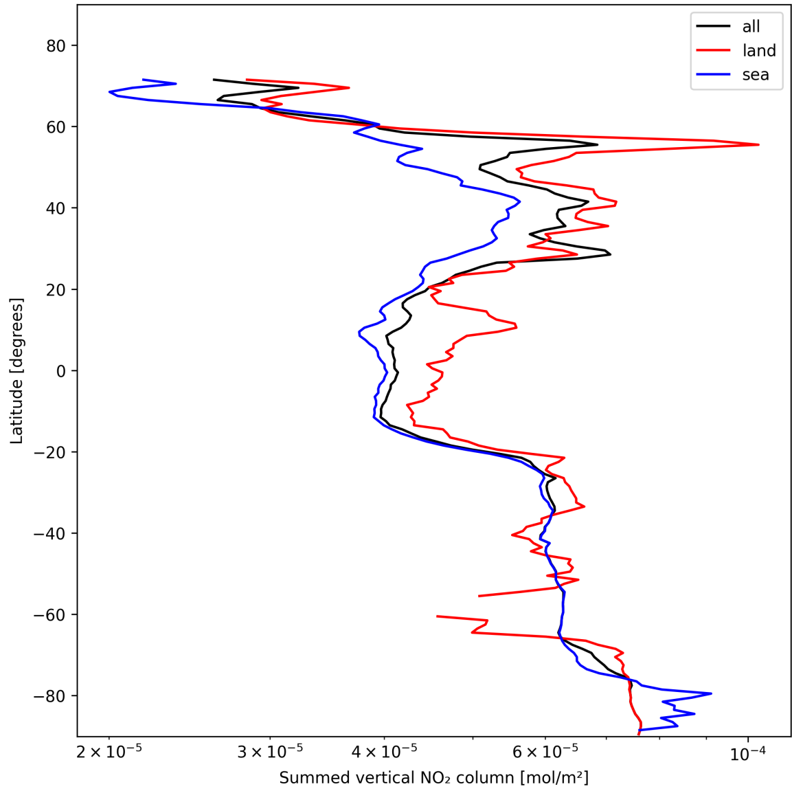
Figure 23: Zonal average of “Summed vertical NO 2 column” for 2025-11-07 to 2025-11-09.
