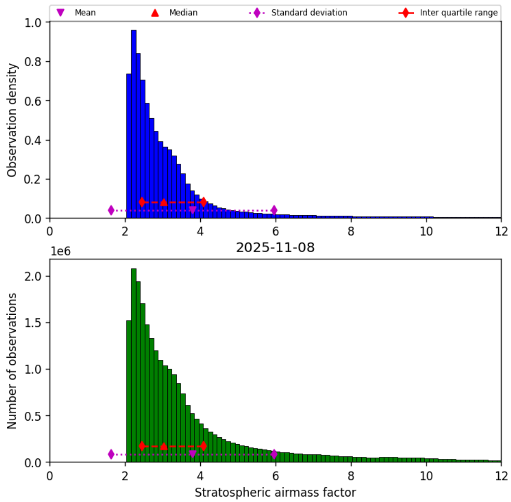
Figure 44: Histogram of “Stratospheric airmass factor” for 2025-11-07 to 2025-11-09
