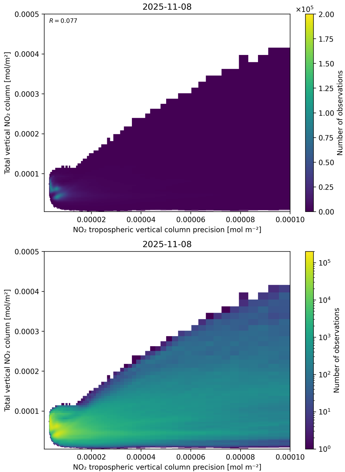
Figure 138: Scatter density plot of “NO 2 tropospheric vertical column precision” against “Total vertical NO 2 column” for 2025-11-07 to 2025-11-09.
