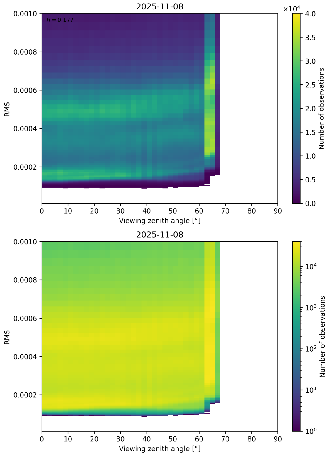
Figure 171: Scatter density plot of “Viewing zenith angle” against “RMS” for 2025-11-07 to 2025-11-09.
