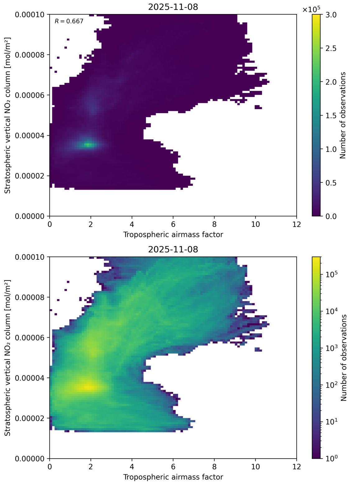
Figure 74: Scatter density plot of “Tropospheric air mass factor” against “Stratospheric vertical NO 2 column” for 2025-11-07 to 2025-11-09.
