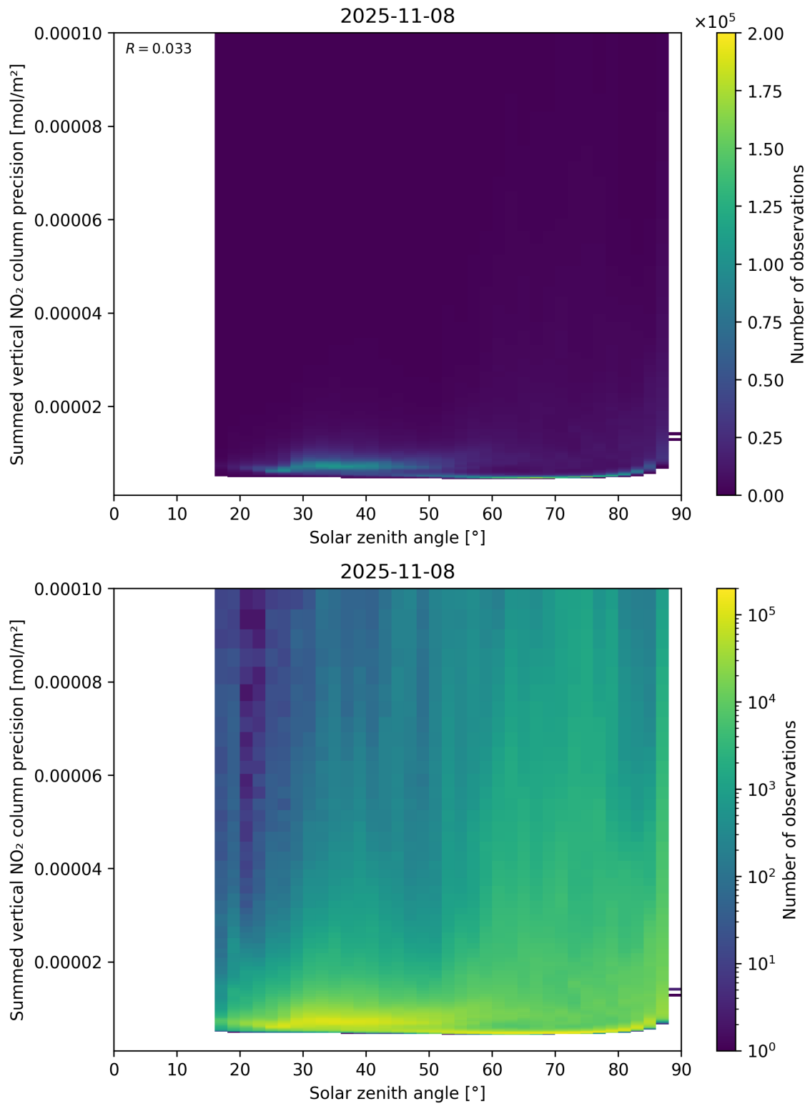
Figure 152: Scatter density plot of “Solar zenith angle” against “Summed vertical NO 2 column precision” for 2025-11-07 to 2025-11-09.
