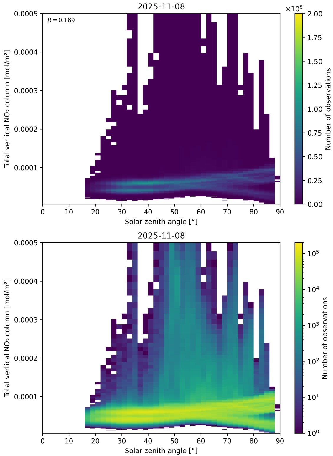
Figure 153: Scatter density plot of “Solar zenith angle” against “Total vertical NO 2 column” for 2025-11-07 to 2025-11-09.
