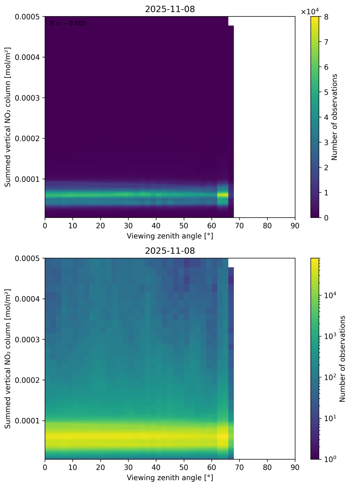
Figure 165: Scatter density plot of “Viewing zenith angle” against “Summed vertical NO 2 column” for 2025-11-07 to 2025-11-09.
