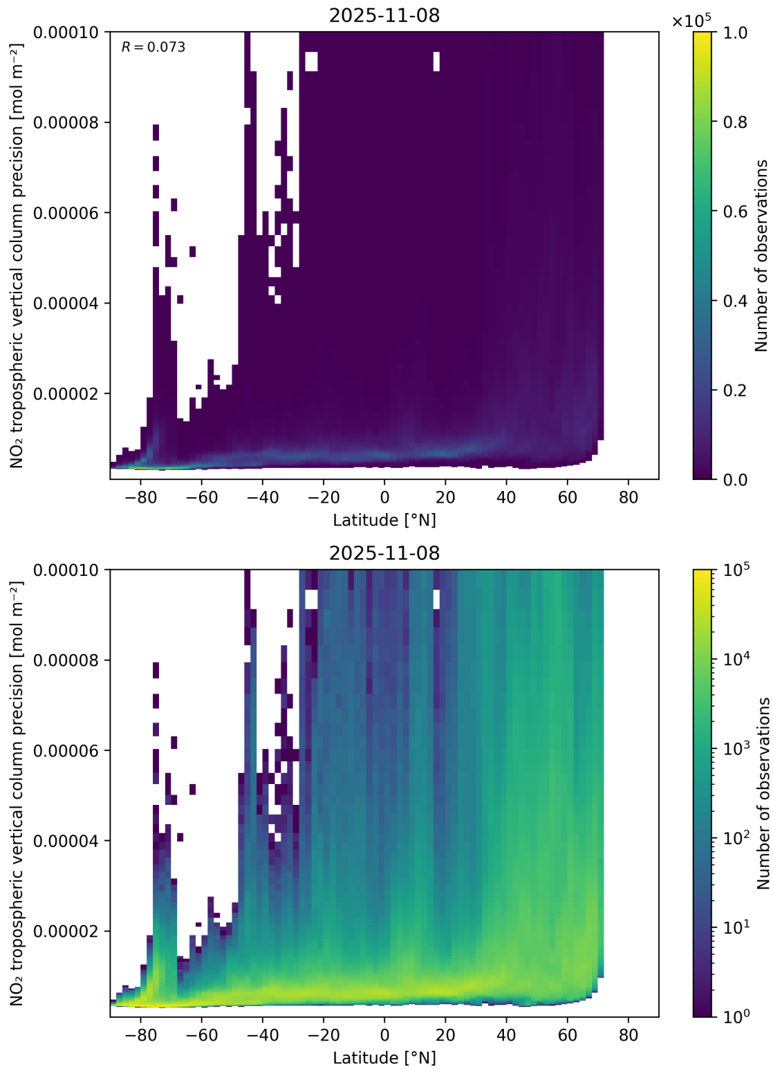
Figure 93: Scatter density plot of “Latitude” against “NO 2 tropospheric vertical column precision” for 2025-11-07 to 2025-11-09.
