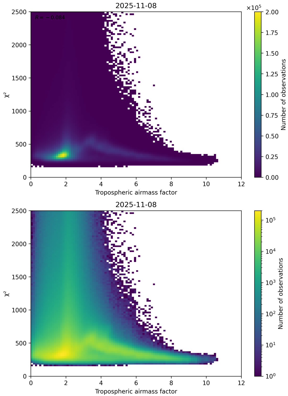
Figure 73: Scatter density plot of “Tropospheric airmass factor” against “ \chi^2 ” for 2025-11-07 to 2025-11-09.
