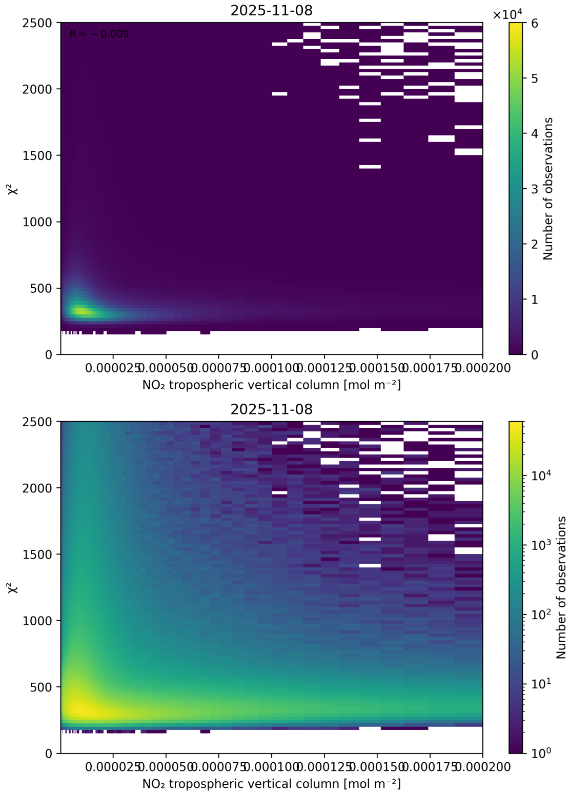
Figure 124: Scatter density plot of “NO 2 tropospheric vertical column” against “ \chi^2 ” for 2025-11-07 to 2025-11-09.
