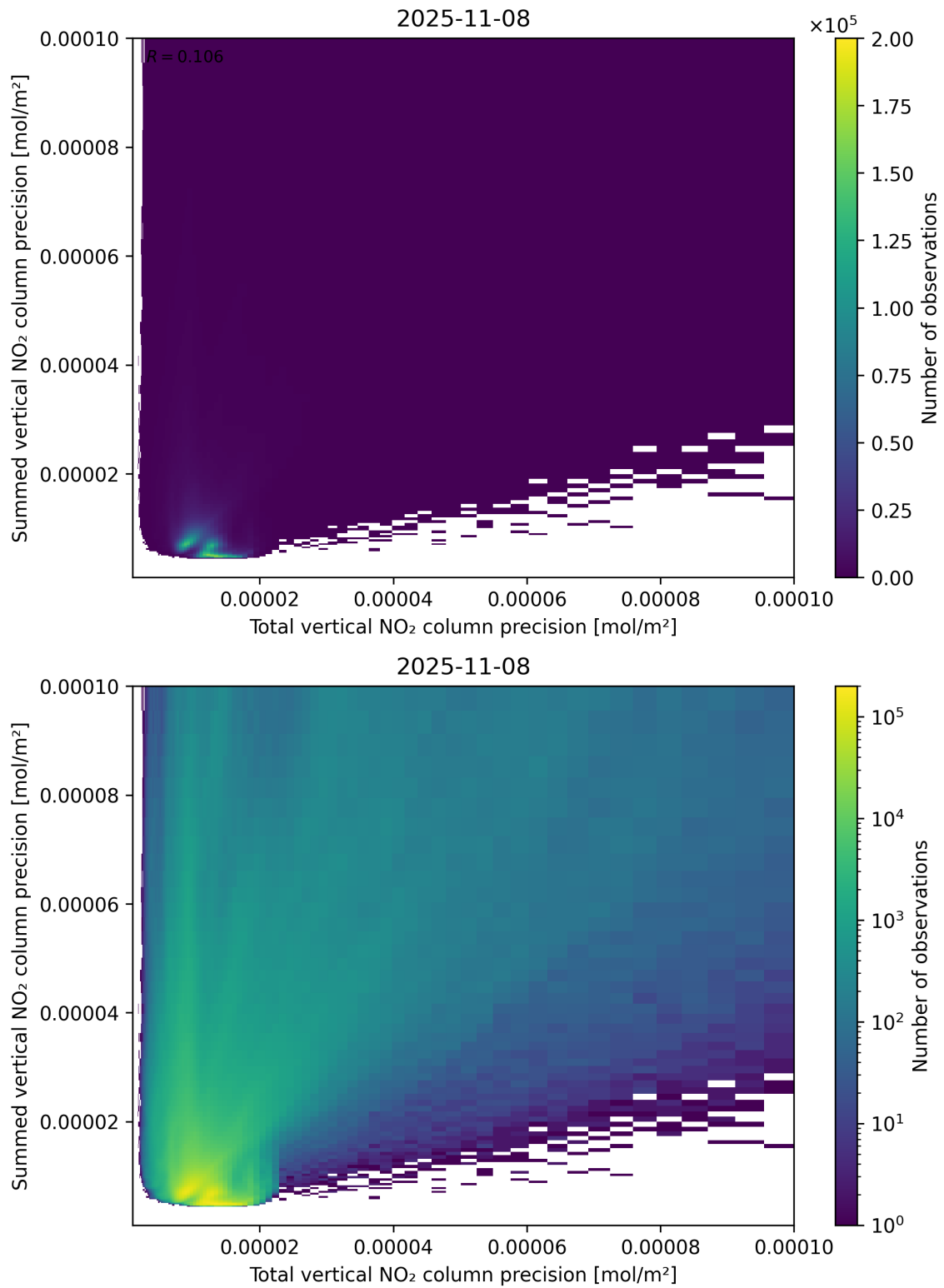
Figure 118: Scatter density plot of “Total vertical NO 2 column precision” against “Summed vertical NO 2 column precision” for 2025-11-07 to 2025-11-09.
