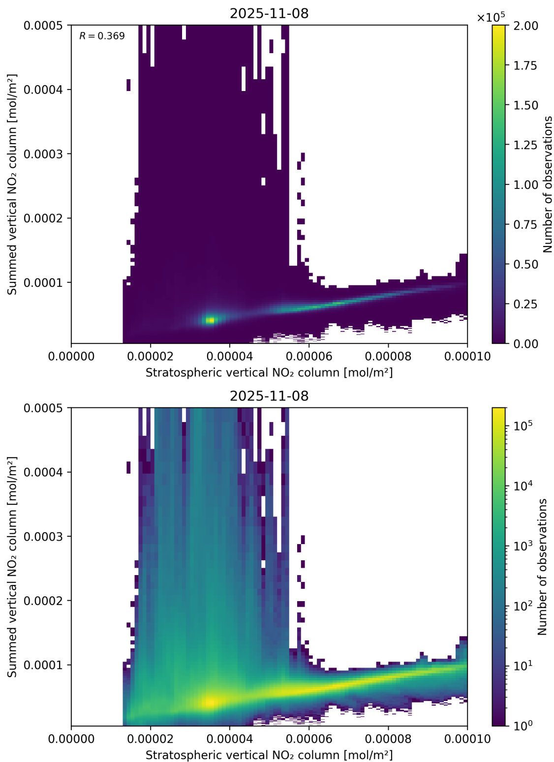
Figure 98: Scatter density plot of “Stratospheric vertical NO 2 column” against “Summed vertical NO 2 column” for 2025-11-07 to 2025-11-09.
