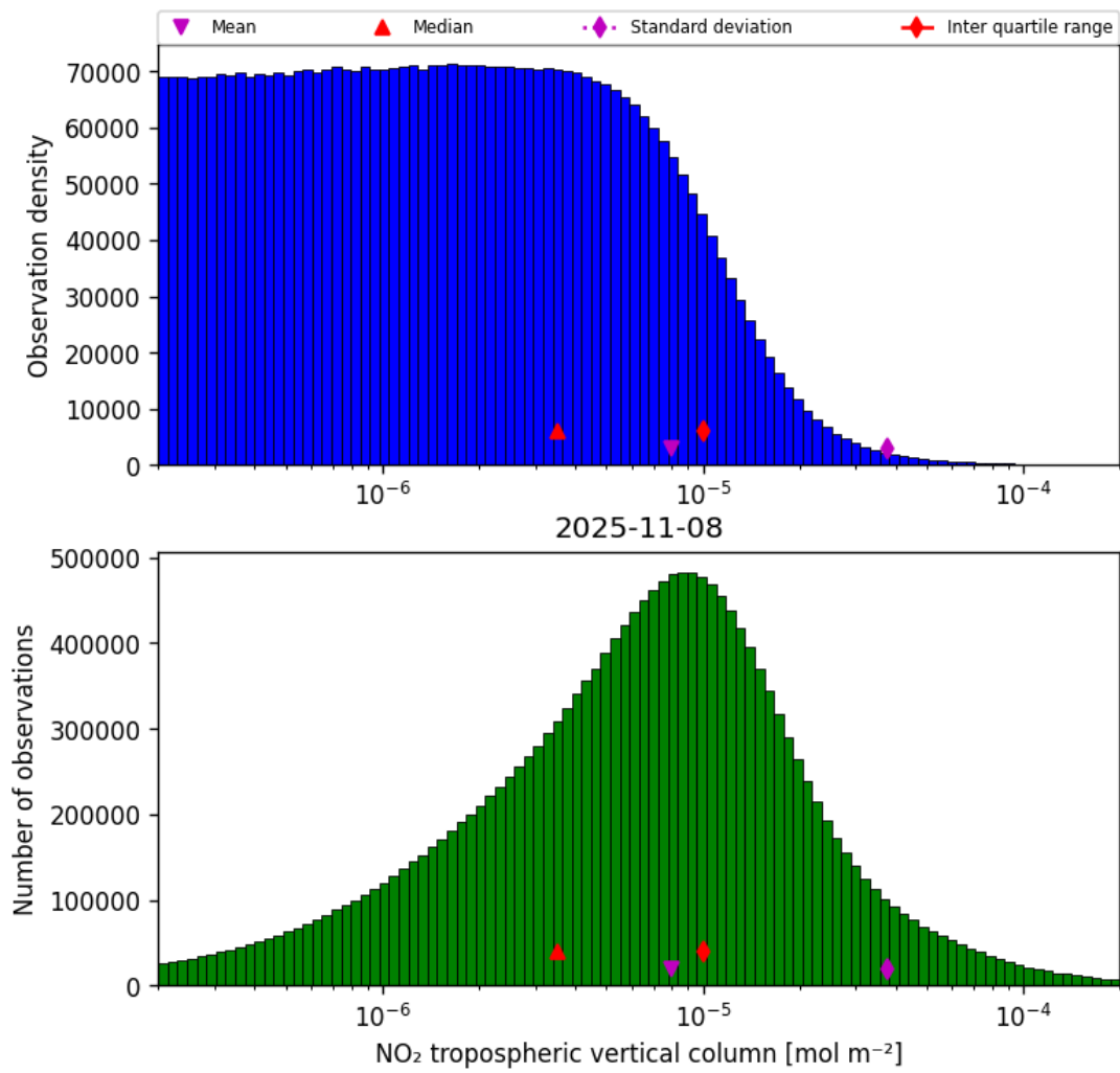
Figure 29: Histogram of “NO 2 tropospheric vertical column” for 2025-11-07 to 2025-11-09
