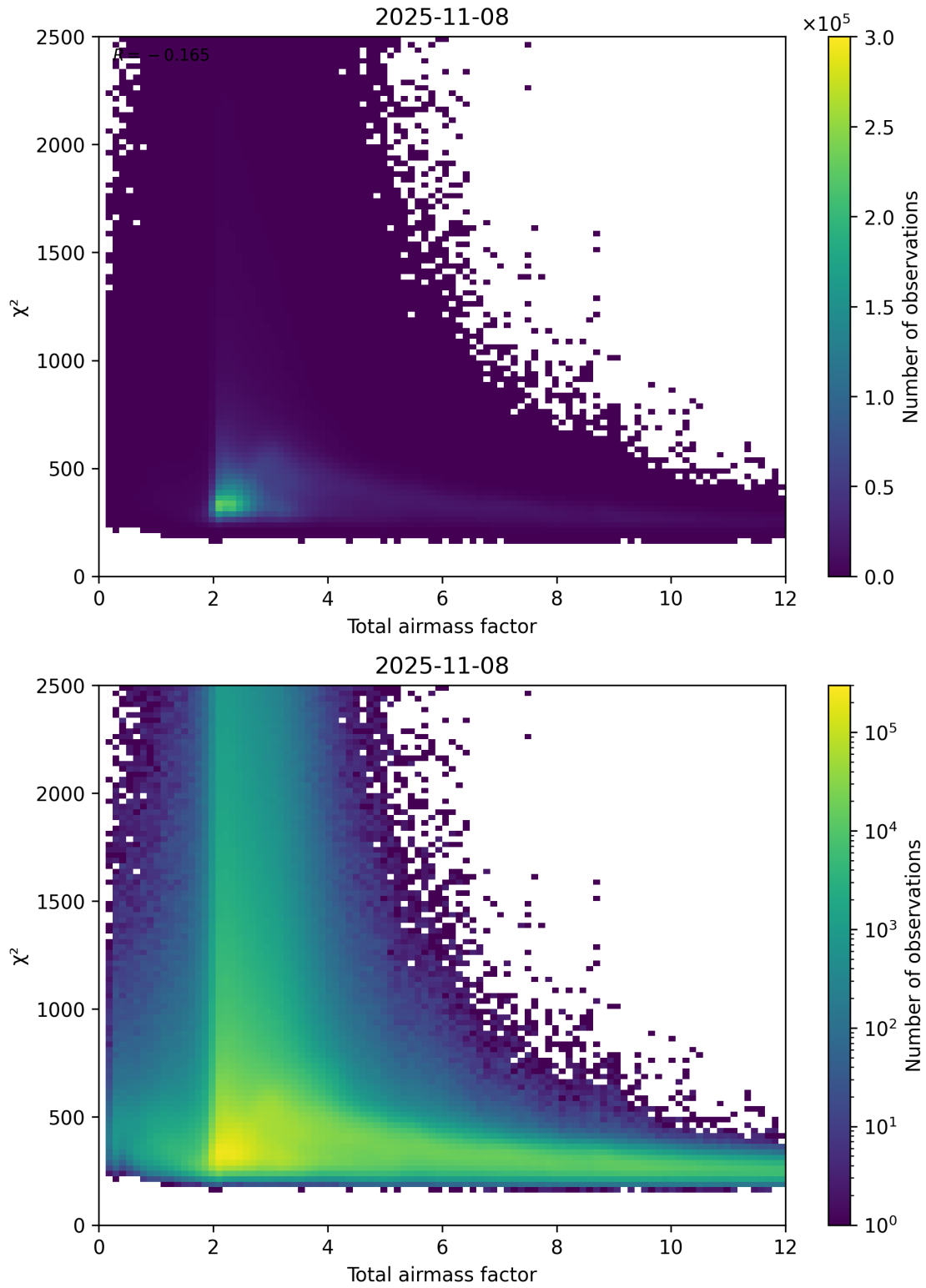
Figure 63: Scatter density plot of “Total airmass factor” against “ \chi^2 ” for 2025-11-07 to 2025-11-09.
