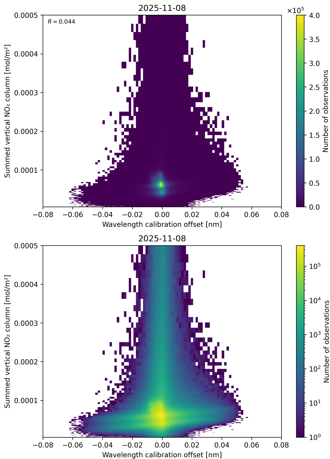
Figure 177: Scatter density plot of “Wavelength calibration offset” against “Summed vertical NO 2 column” for 2025-11-07 to 2025-11-09.
