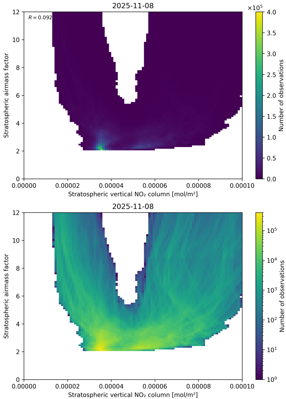
Figure 96: Scatter density plot of “Stratospheric vertical NO 2 column” against “Stratospheric airmass factor” for 2025-11-07 to 2025-11-09.
