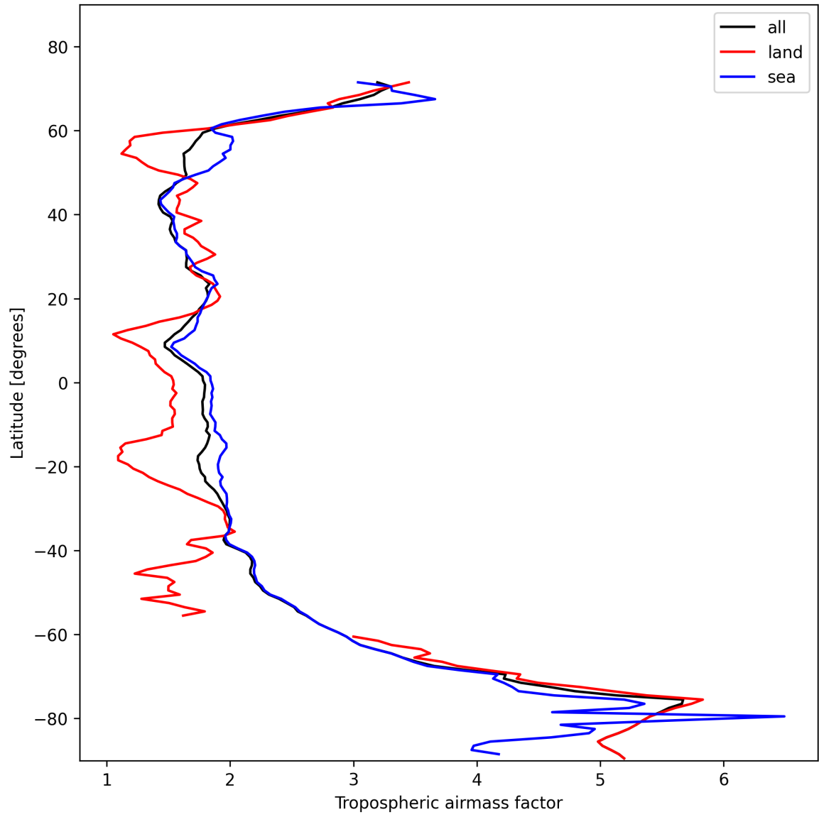
Figure 14: Zonal average of “Tropospheric airmass factor” for 2025-11-07 to 2025-11-09.
