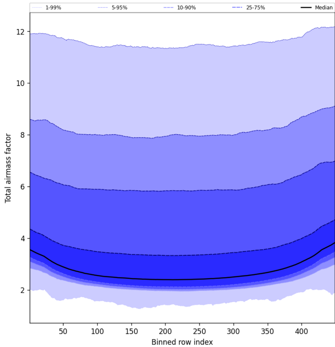
Figure 49: Along track statistics of “Total airmass factor” for 2025-11-07 to 2025-11-09
