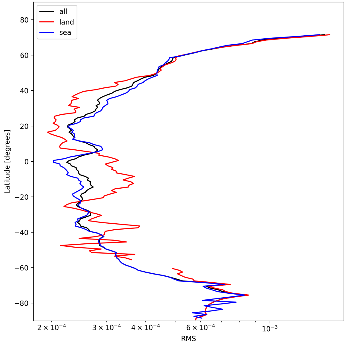
Figure 26: Zonal average of “RMS” for 2025-11-07 to 2025-11-09.
