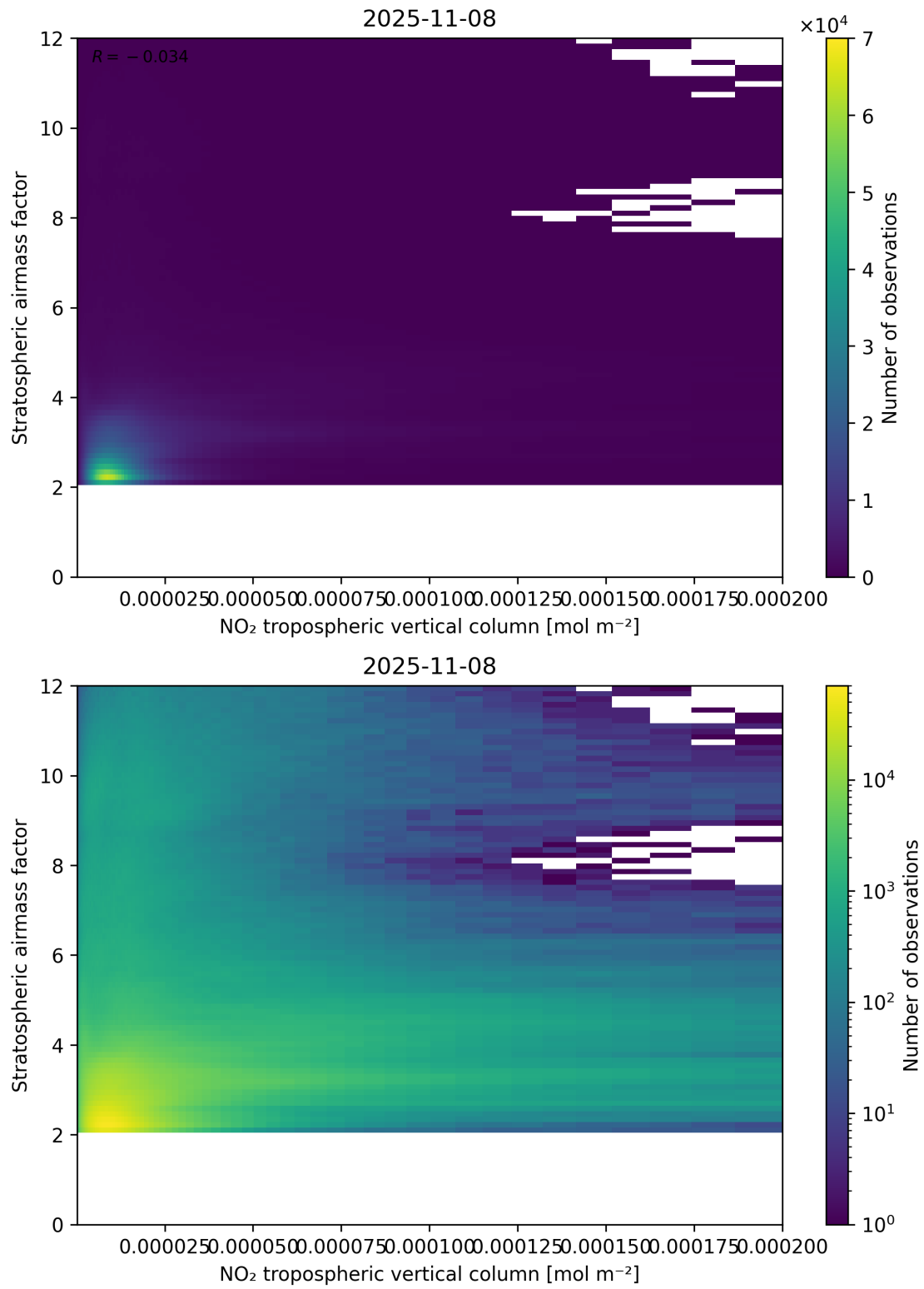
Figure 121: Scatter density plot of “NO 2 tropospheric vertical column” against “Stratospheric air mass factor” for 2025-11-07 to 2025-11-09.
