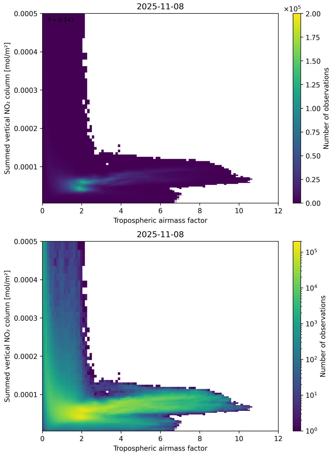
Figure 75: Scatter density plot of “Tropospheric air mass factor” against “Summed vertical NO 2 column” for 2025-11-07 to 2025-11-09.
