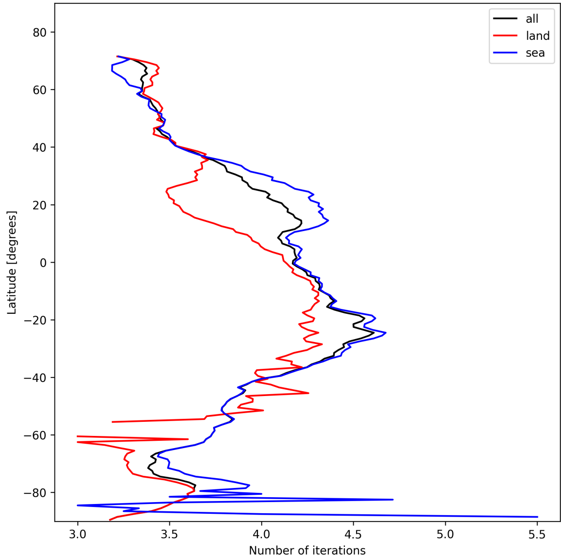
Figure 17: Zonal average of “Number of iterations” for 2025-11-07 to 2025-11-09.
