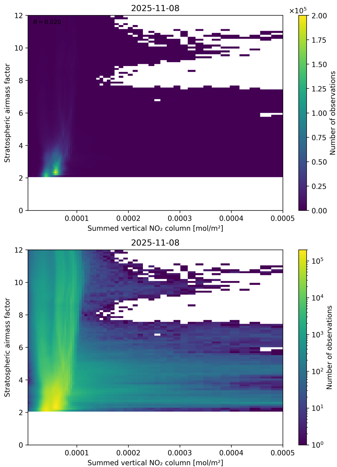
Figure 103: Scatter density plot of “Summed vertical NO 2 column” against “Stratospheric air mass factor” for 2025-11-07 to 2025-11-09.
