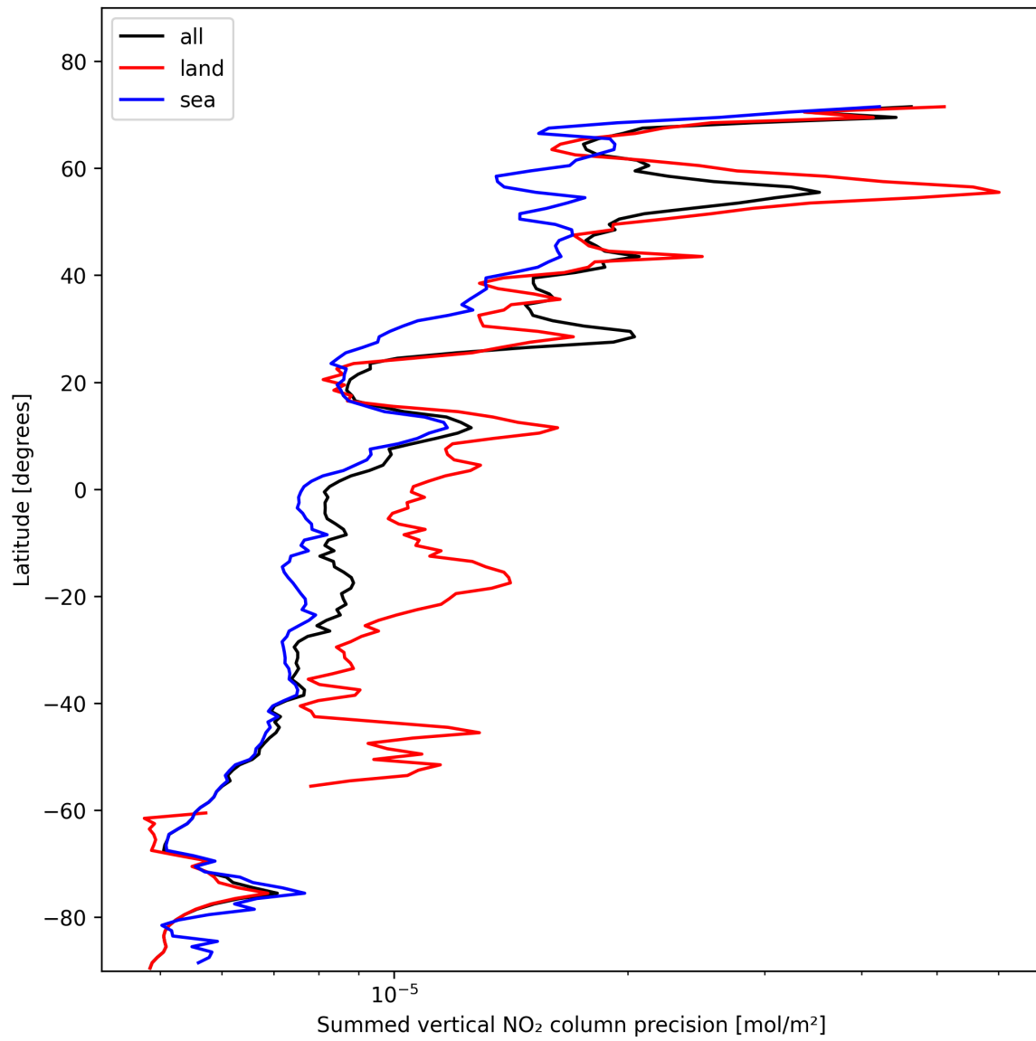
Figure 24: Zonal average of “Summed vertical NO 2 column precision” for 2025-11-07 to 2025-11-09.
