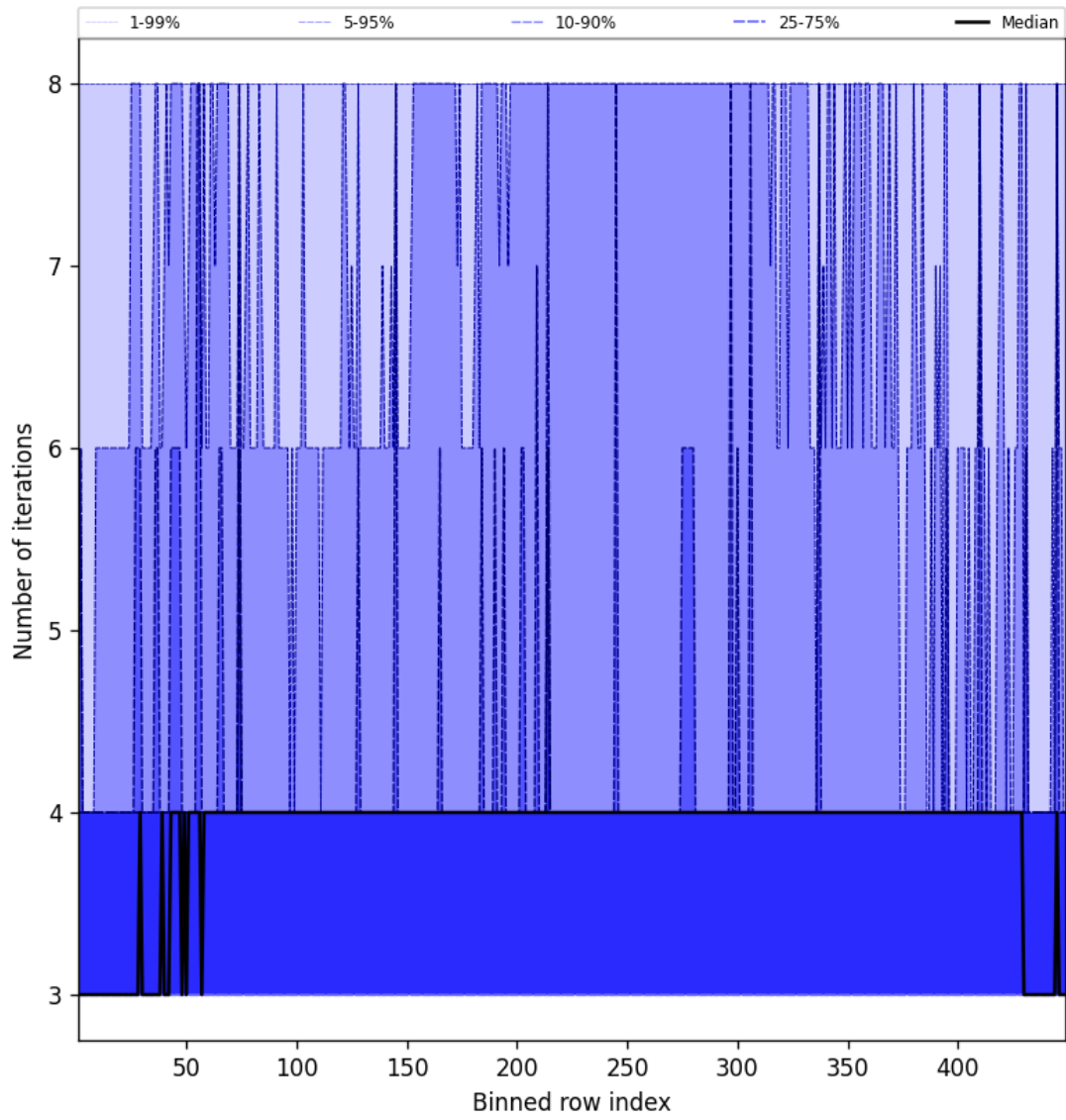
Figure 51: Along track statistics of “Number of iterations” for 2025-11-07 to 2025-11-09
