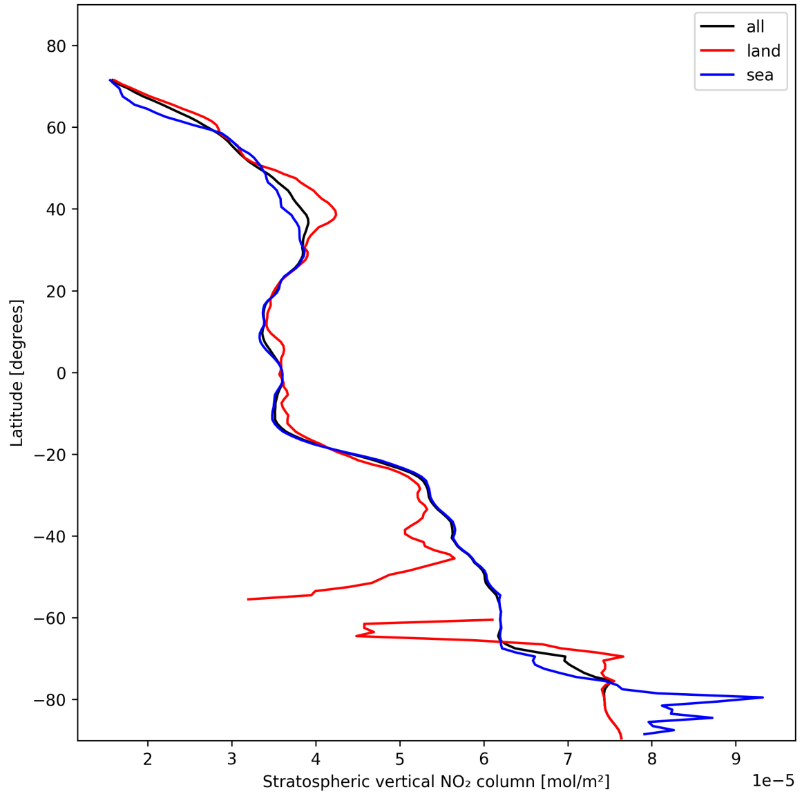
Figure 19: Zonal average of “Stratospheric vertical NO 2 column” for 2025-11-07 to 2025-11-09.
