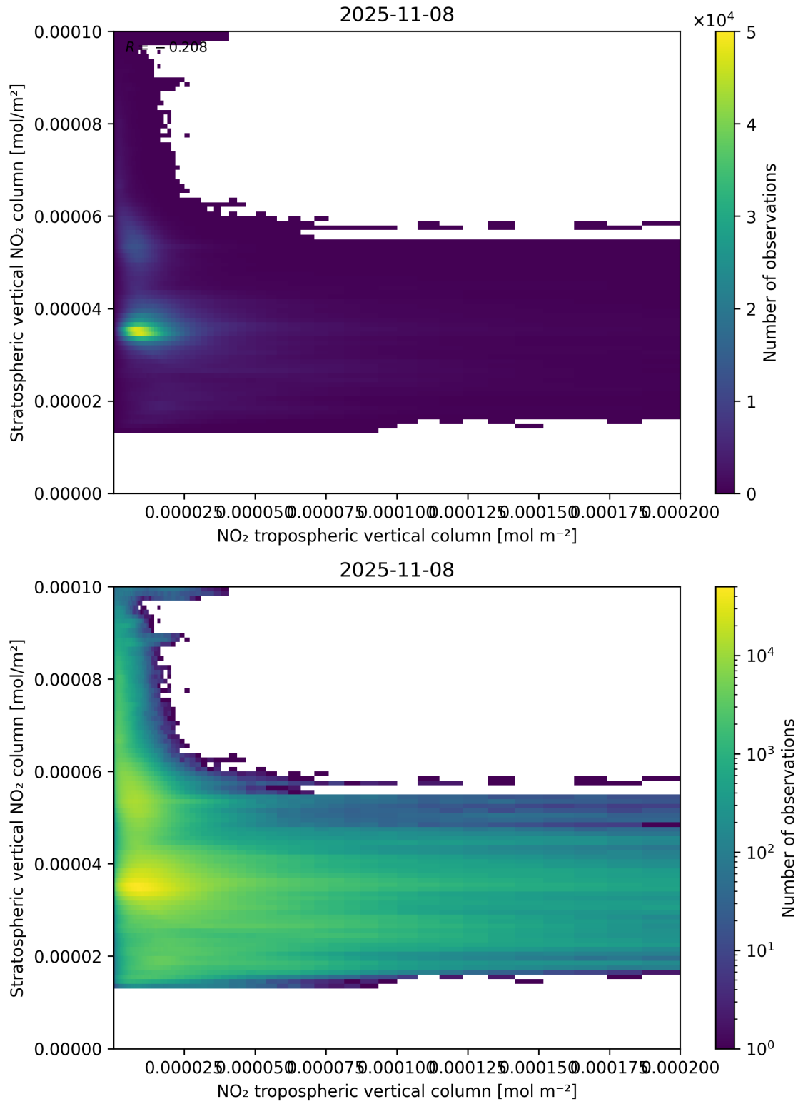
Figure 125: Scatter density plot of “NO 2 tropospheric vertical column” against “Stratospheric vertical NO 2 column” for 2025-11-07 to 2025-11-09.
