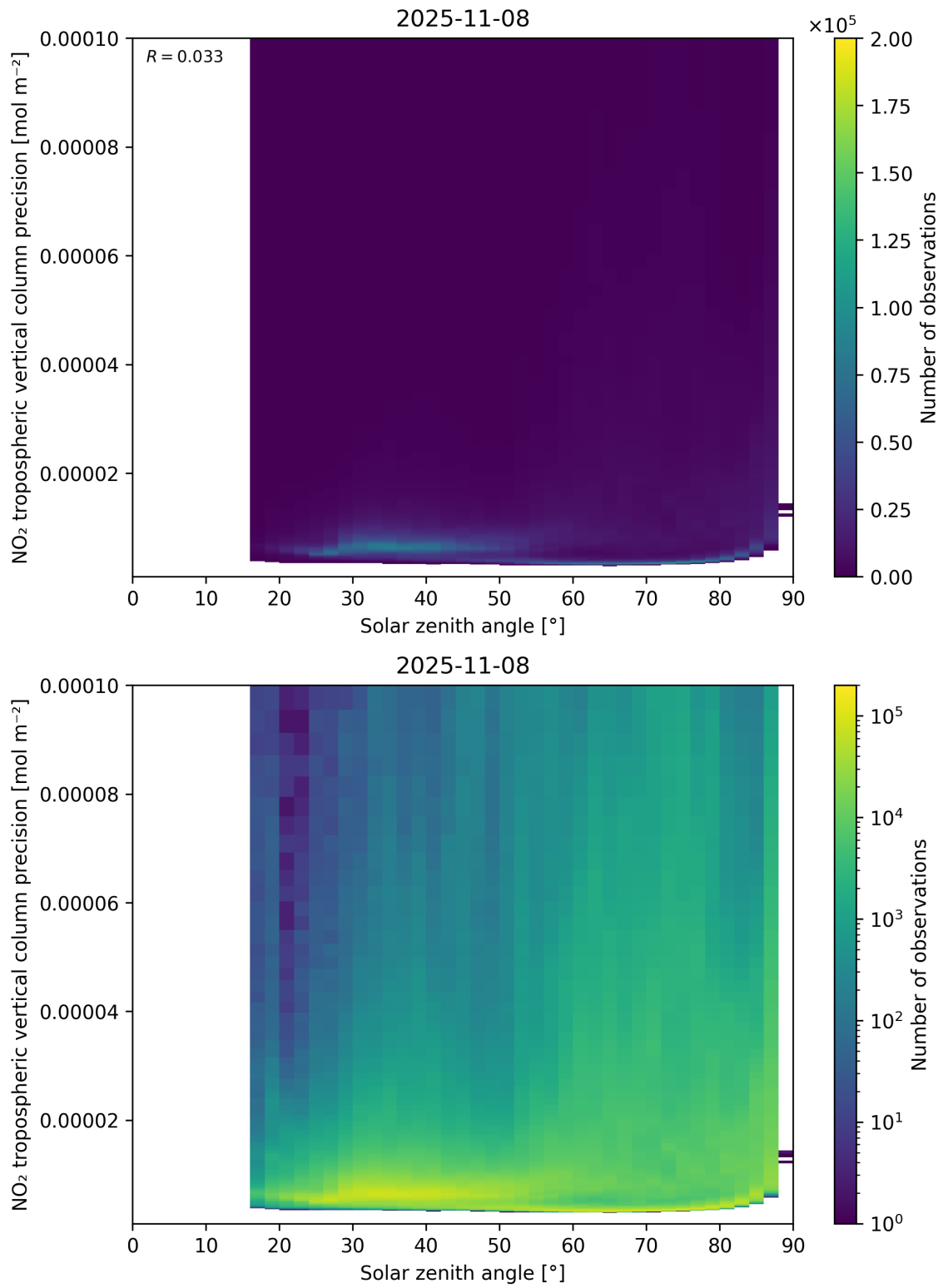
Figure 156: Scatter density plot of “Solar zenith angle” against “NO 2 tropospheric vertical column precision” for 2025-11-07 to 2025-11-09.
