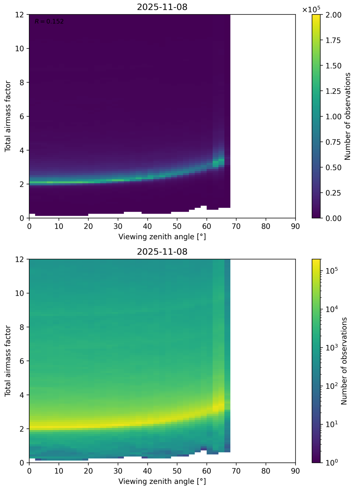
Figure 160: Scatter density plot of “Viewing zenith angle” against “Total airmass factor” for 2025-11-07 to 2025-11-09.
