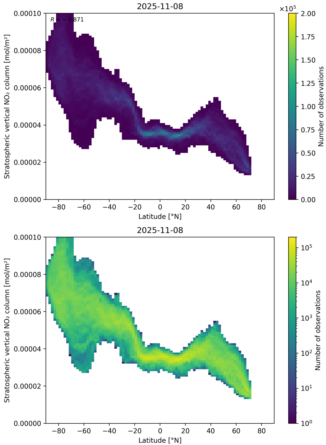
Figure 87: Scatter density plot of “Latitude” against “Stratospheric vertical NO 2 column” for 2025-11-07 to 2025-11-09.
