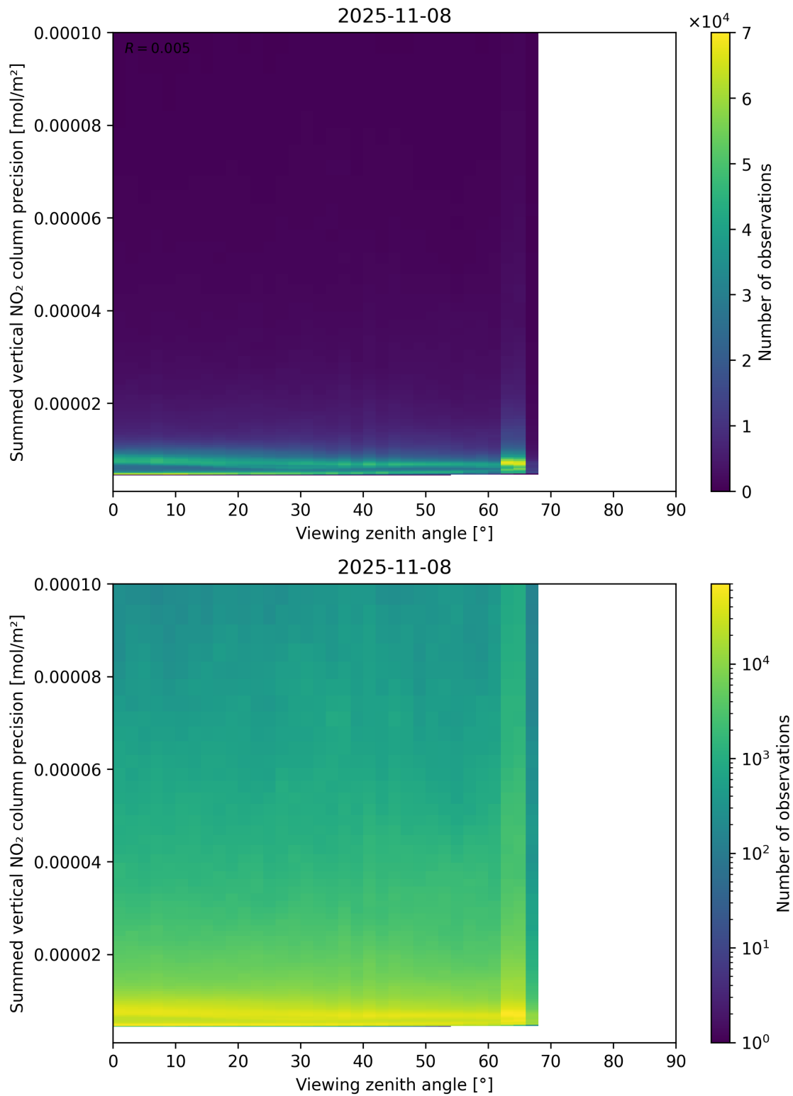
Figure 166: Scatter density plot of “Viewing zenith angle” against “Summed vertical NO 2 column precision” for 2025-11-07 to 2025-11-09.
