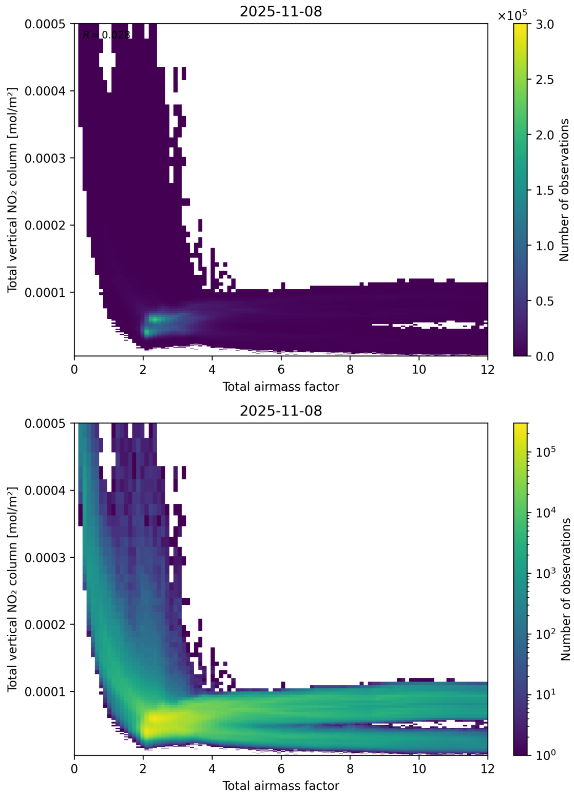
Figure 67: Scatter density plot of “Total airmass factor” against “Total vertical NO 2 column” for 2025-11-07 to 2025-11-09.
