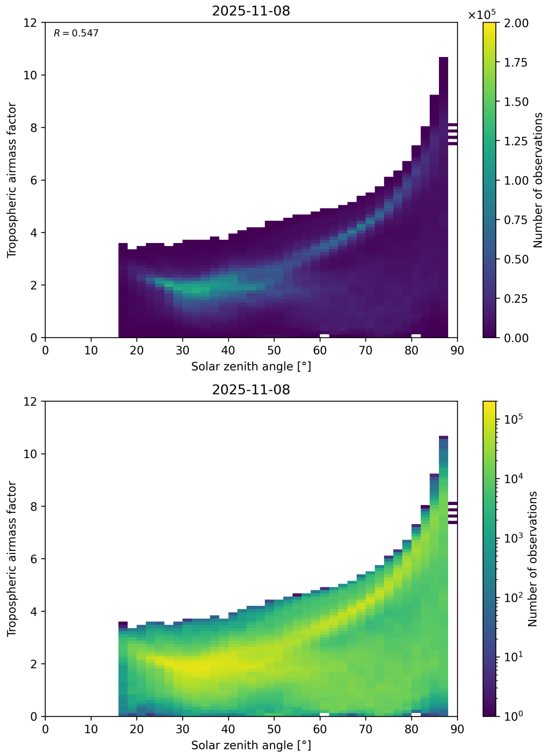
Figure 147: Scatter density plot of “Solar zenith angle” against “Tropospheric airmass factor” for 2025-11-07 to 2025-11-09.
