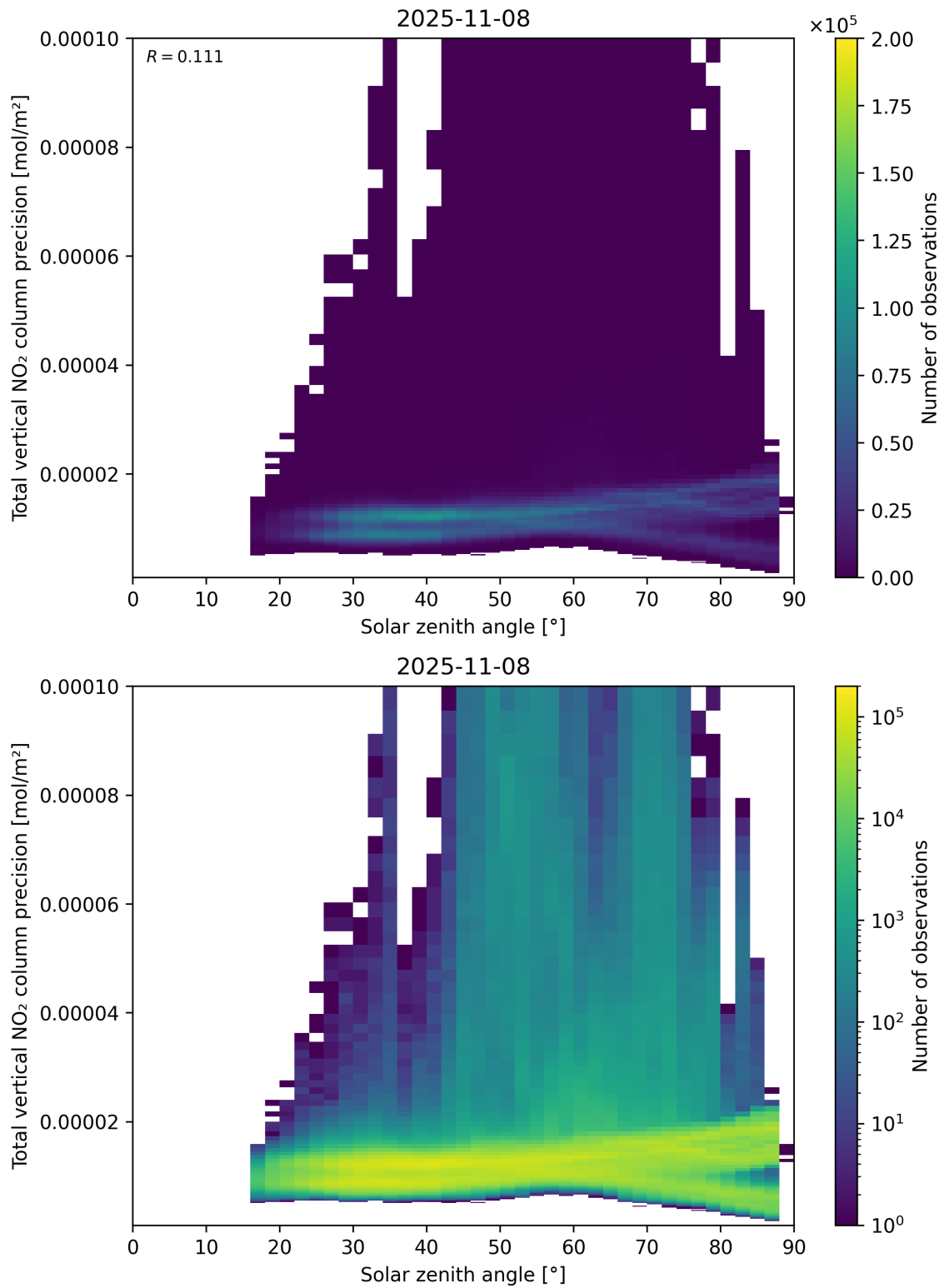
Figure 154: Scatter density plot of “Solar zenith angle” against “Total vertical NO 2 column precision” for 2025-11-07 to 2025-11-09.
