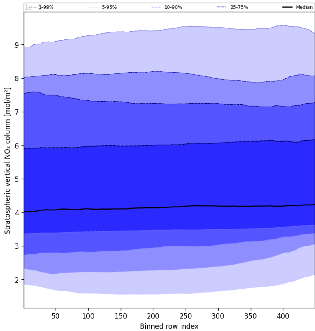
Figure 53: Along track statistics of “Stratospheric vertical NO 2 column” for 2025-11-07 to 2025-11-09
