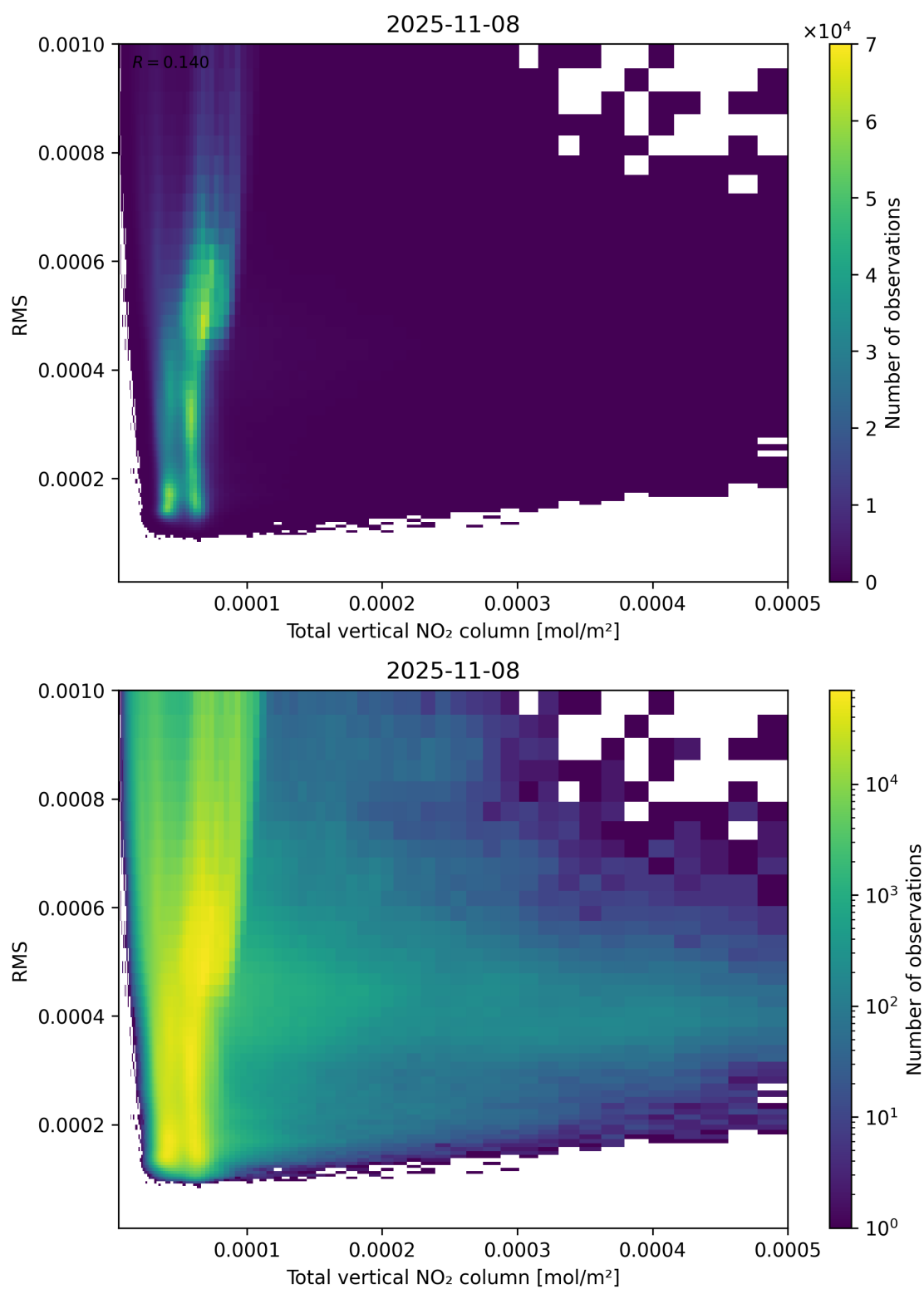
Figure 120: Scatter density plot of “Total vertical NO 2 column” against “RMS” for 2025-11-07 to 2025-11-09.
