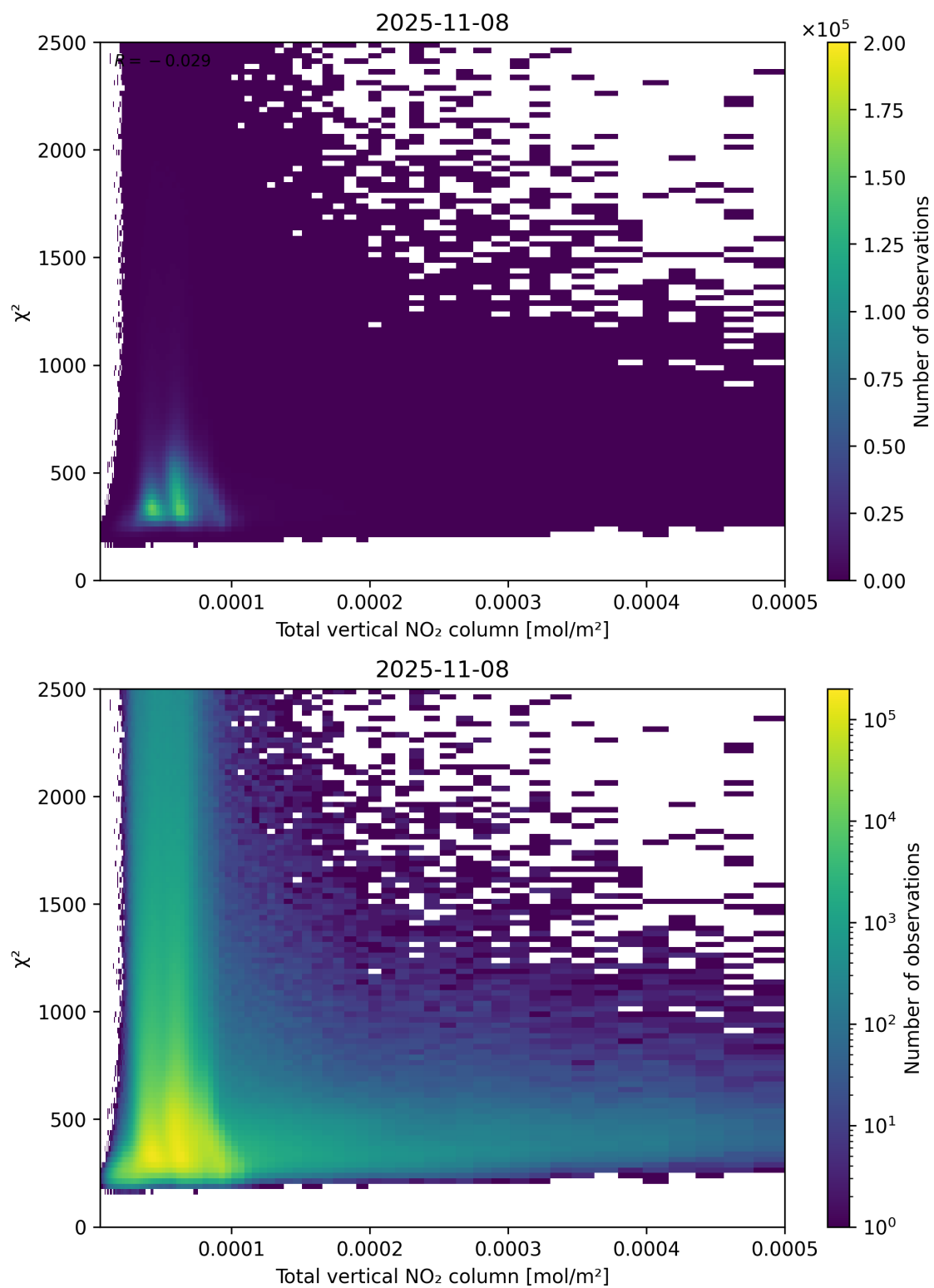
Figure 111: Scatter density plot of “Total vertical NO 2 column” against “ \chi^2 ” for 2025-11-07 to 2025-11-09.
