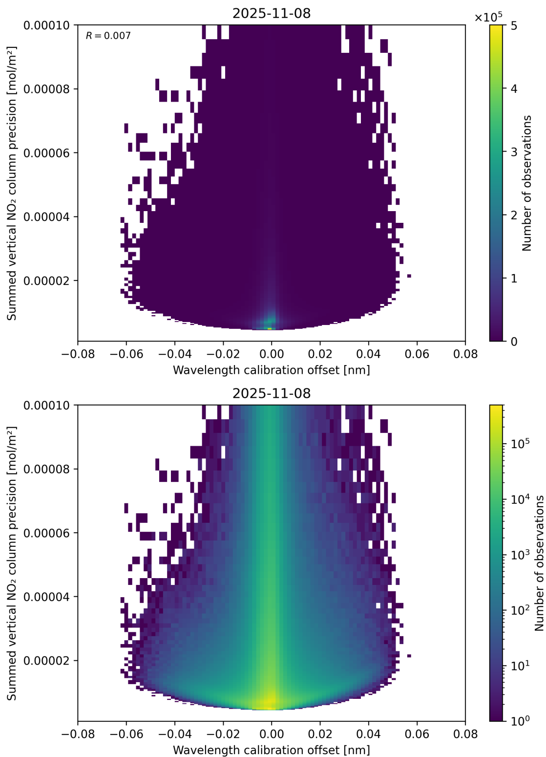
Figure 178: Scatter density plot of “Wavelength calibration offset” against “Summed vertical NO 2 column precision” for 2025-11-07 to 2025-11-09.
