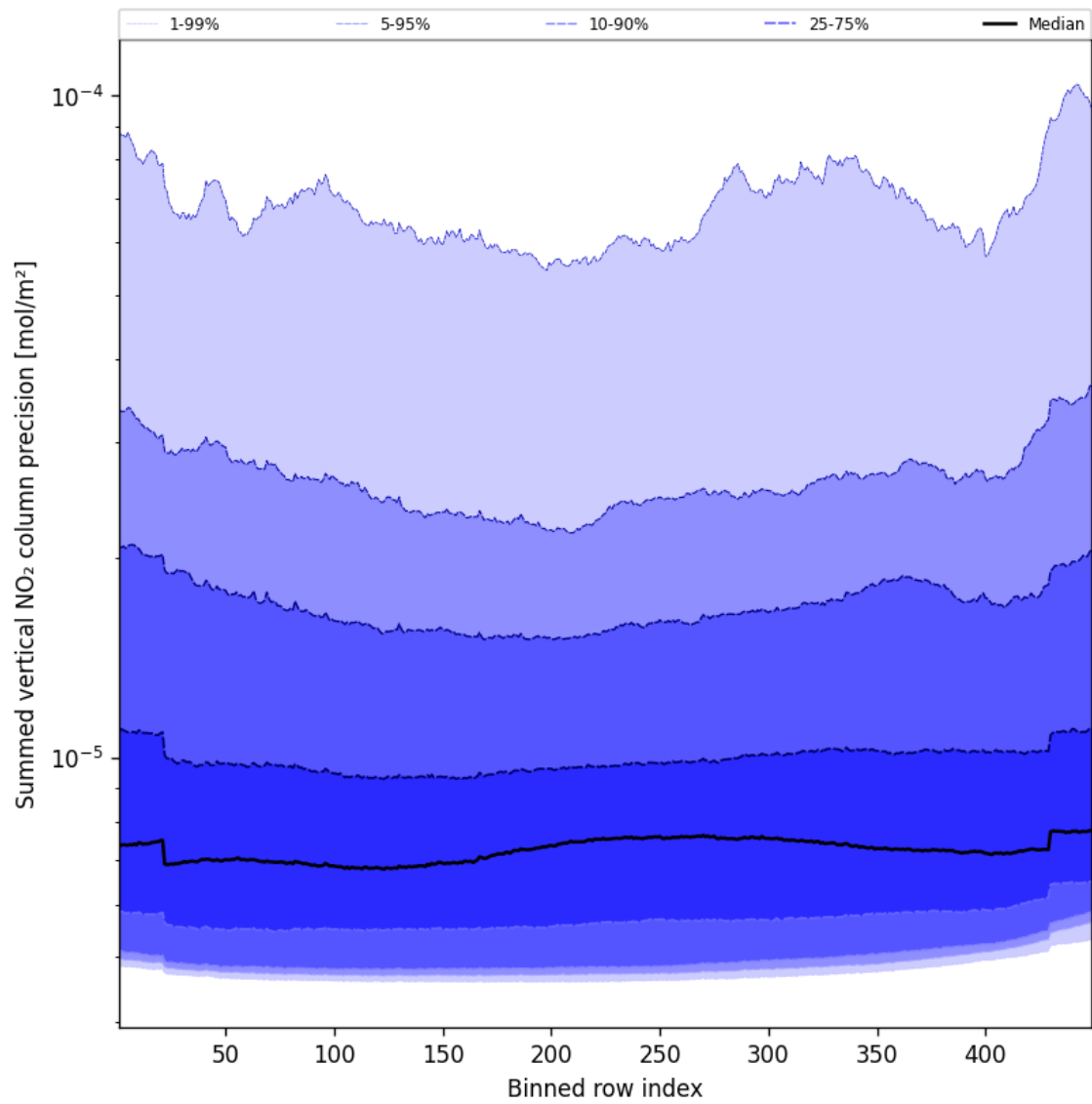
Figure 58: Along track statistics of “Summed vertical NO 2 column precision” for 2025-11-07 to 2025-11-09
