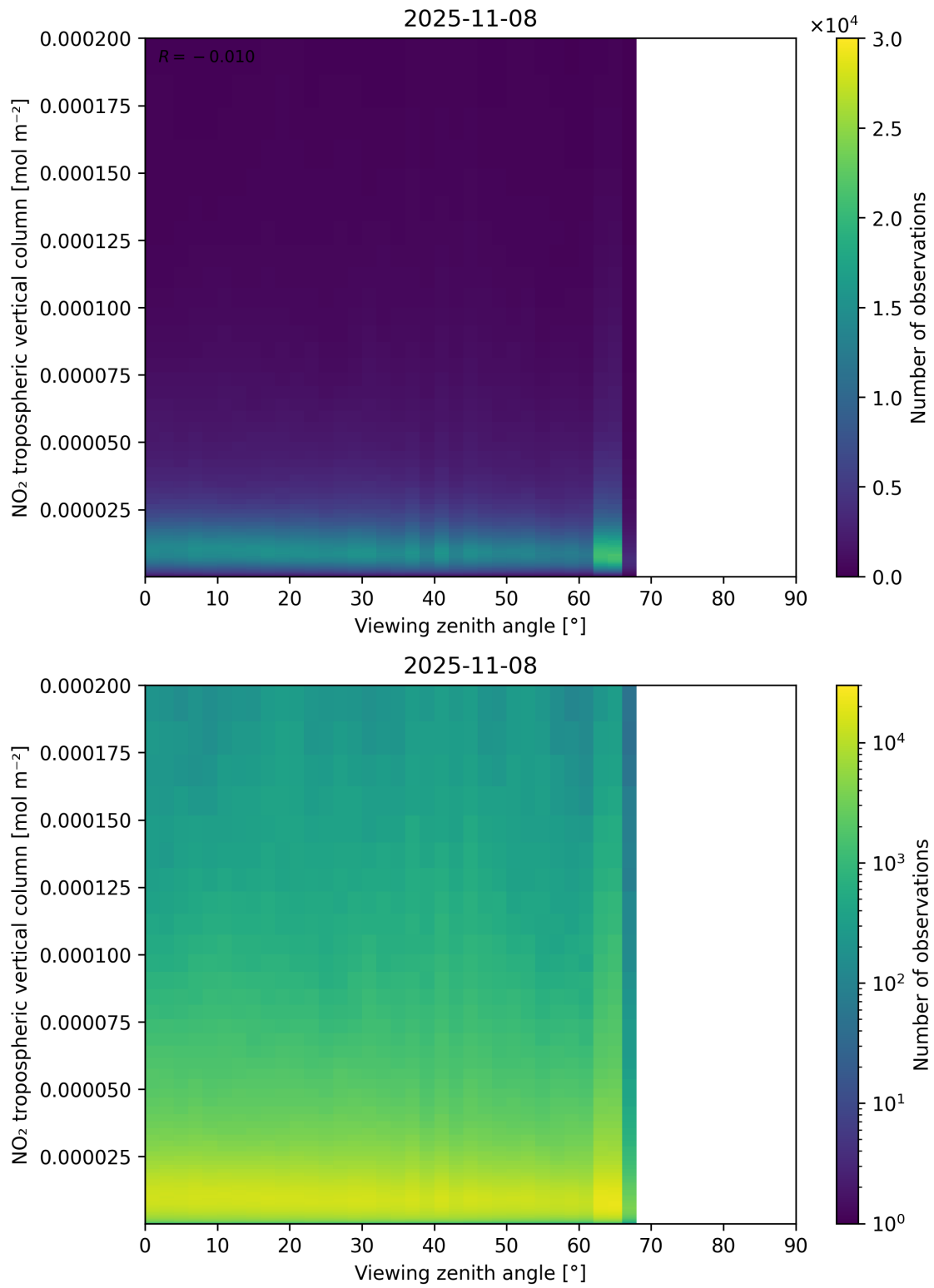
Figure 169: Scatter density plot of “Viewing zenith angle” against “NO 2 tropospheric vertical column” for 2025-11-07 to 2025-11-09.
