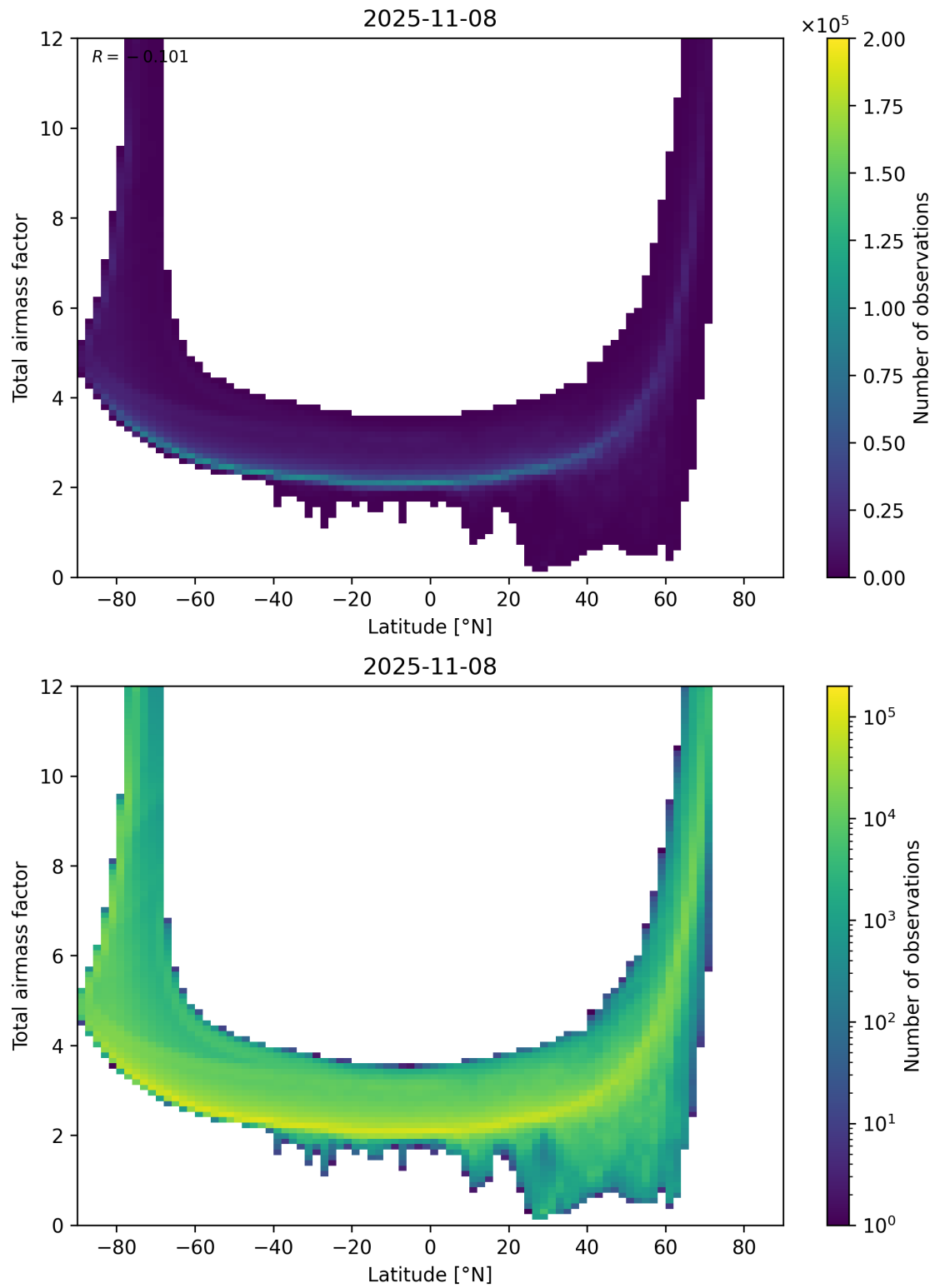
Figure 84: Scatter density plot of “Latitude” against “Total airmass factor” for 2025-11-07 to 2025-11-09.
