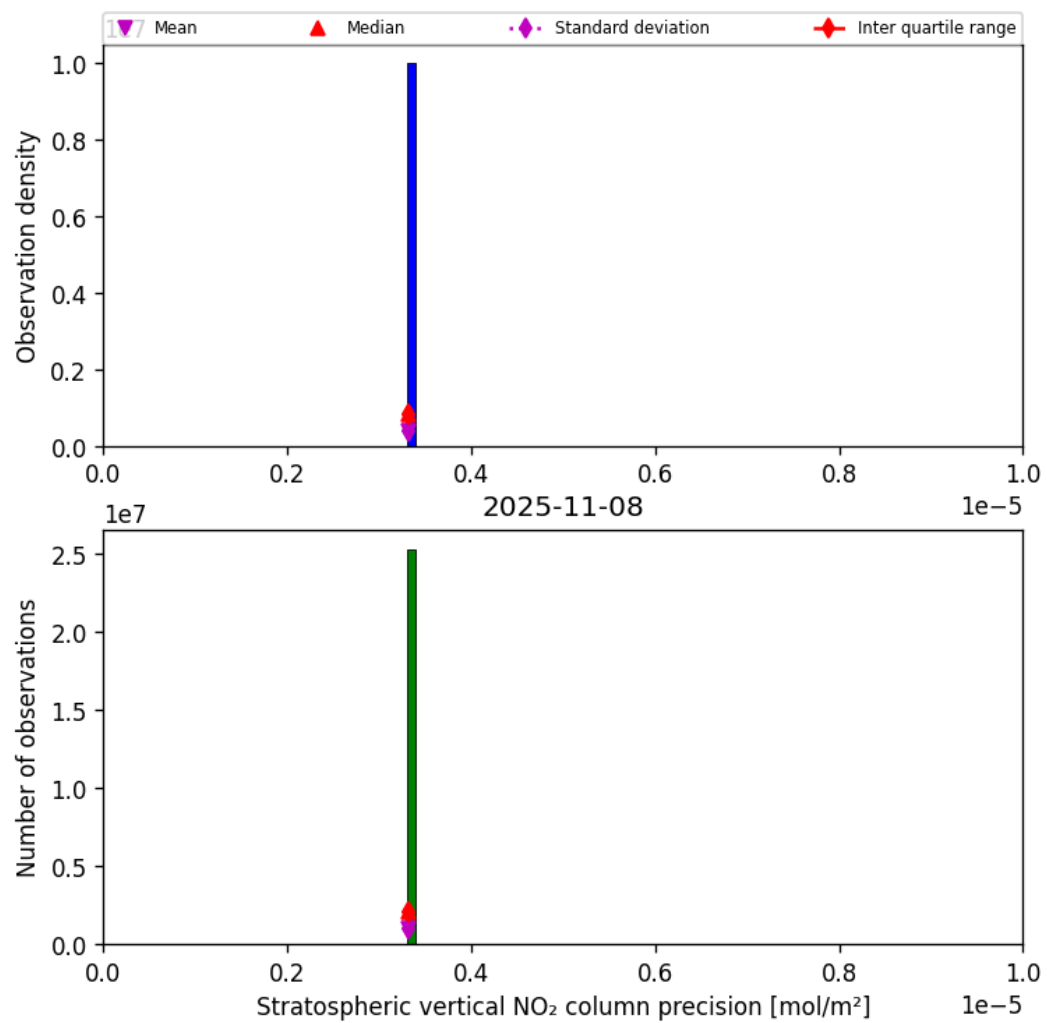
Figure 37: Histogram of “Stratospheric vertical NO 2 column precision” for 2025-11-07 to 2025-11-09
