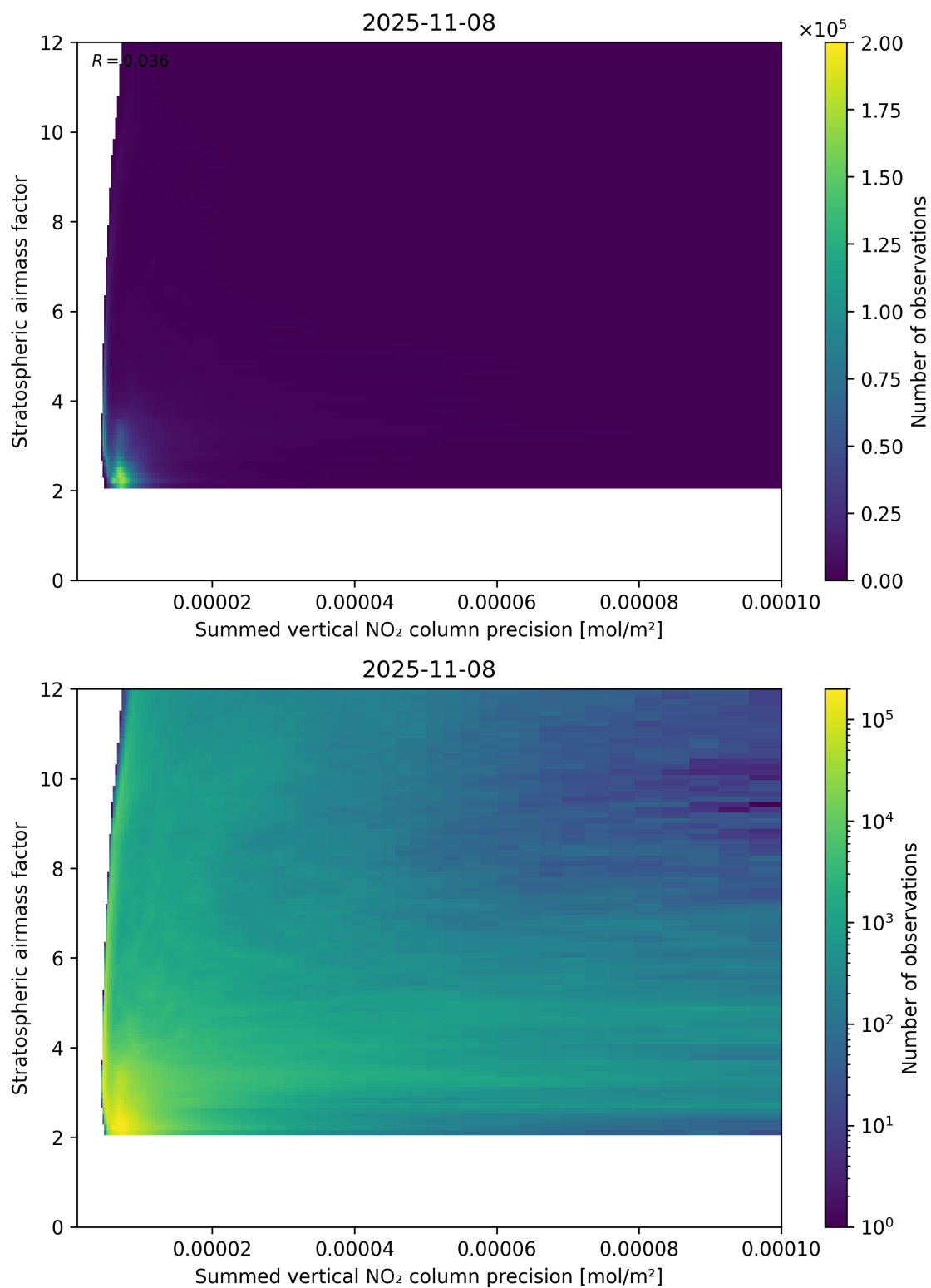
Figure 106: Scatter density plot of “Summed vertical NO 2 column precision” against “Stratospheric airmass factor” for 2025-11-07 to 2025-11-09.
