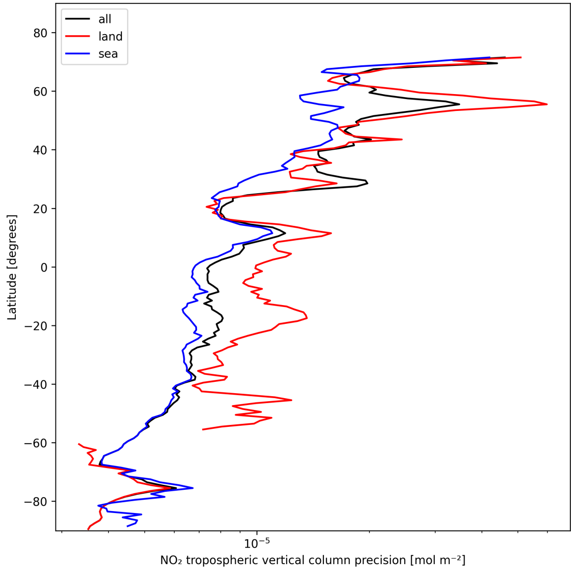
Figure 13: Zonal average of “NO 2 tropospheric vertical column precision” for 2025-11-07 to 2025-11-09.
