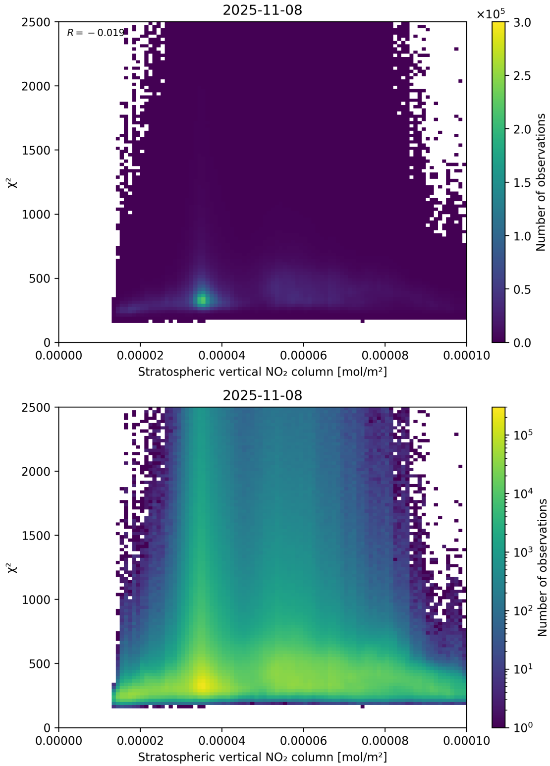
Figure 97: Scatter density plot of “Stratospheric vertical NO 2 column” against “ \chi^2 ” for 2025-11-07 to 2025-11-09.
