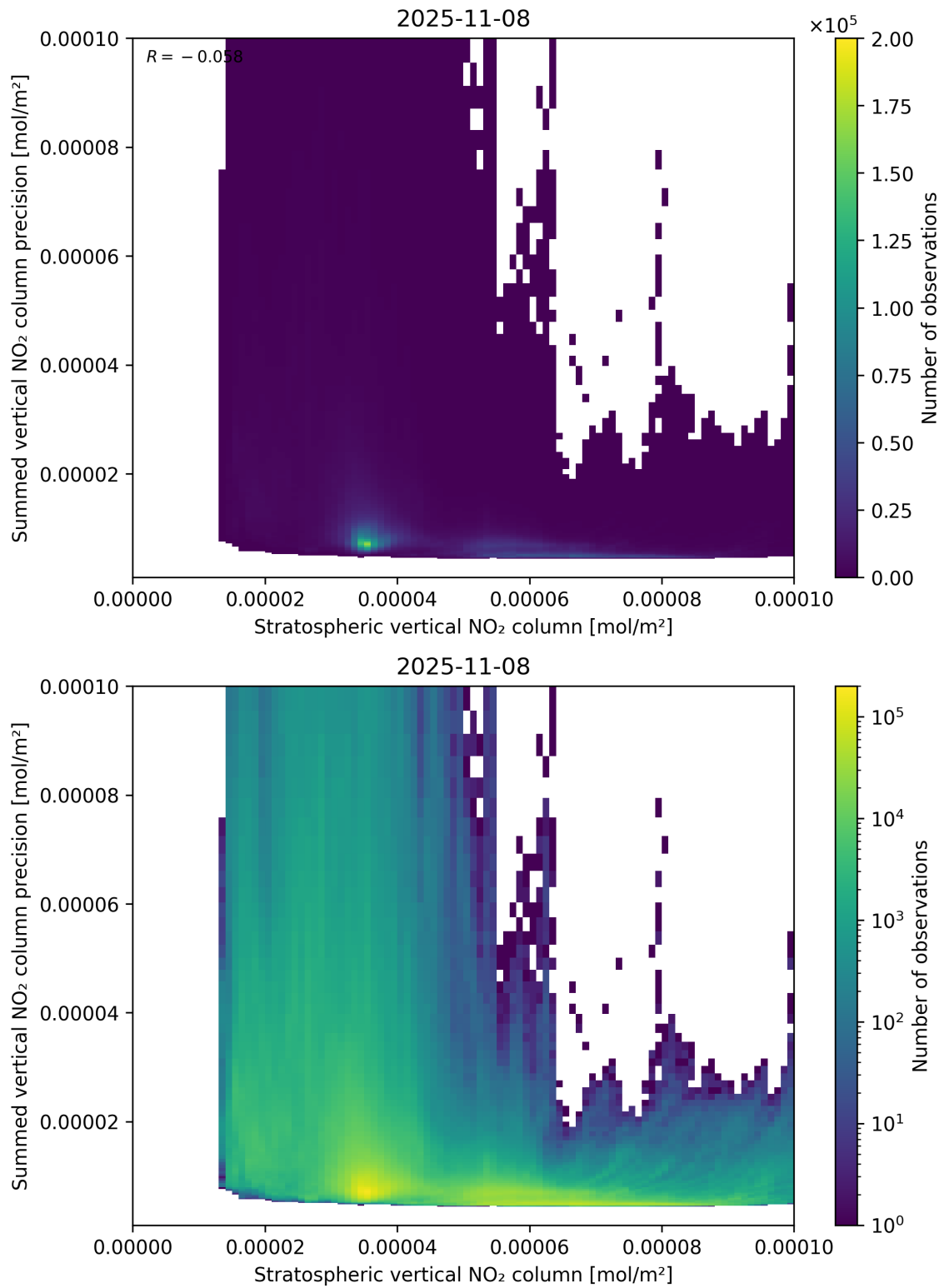
Figure 99: Scatter density plot of “Stratospheric vertical NO 2 column” against “Summed vertical NO 2 column precision” for 2025-11-07 to 2025-11-09.
