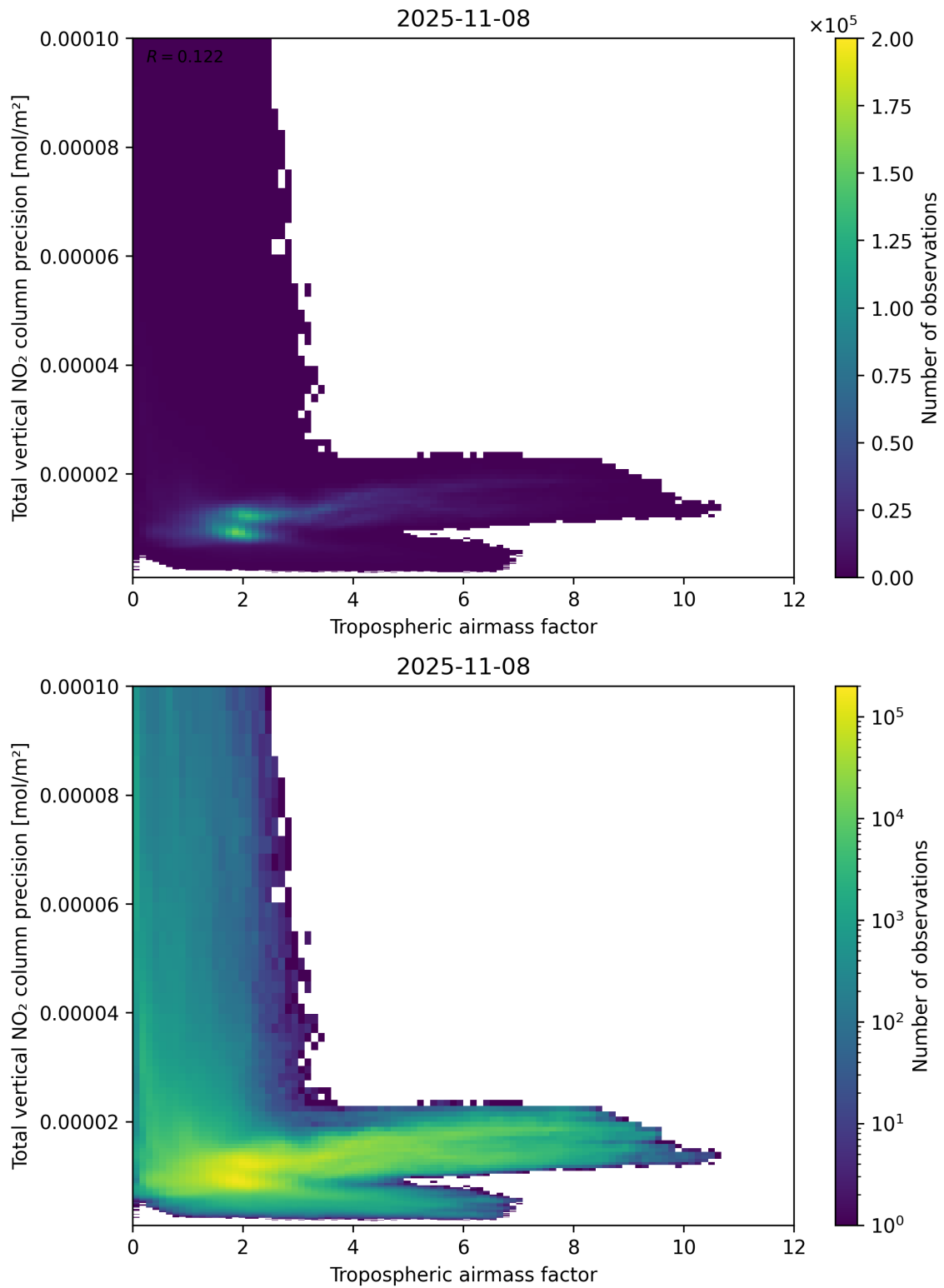
Figure 78: Scatter density plot of “Tropospheric air mass factor” against “Total vertical NO 2 column precision” for 2025-11-07 to 2025-11-09.
