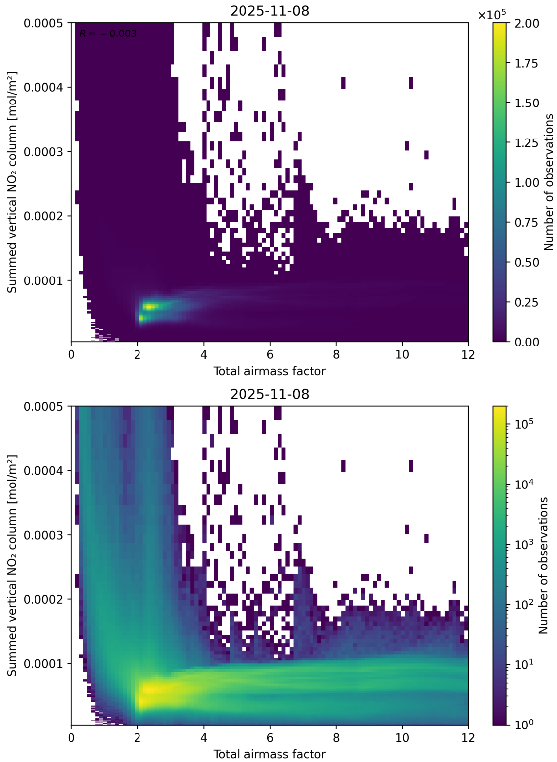
Figure 65: Scatter density plot of “Total airmass factor” against “Summed vertical NO 2 column” for 2025-11-07 to 2025-11-09.
