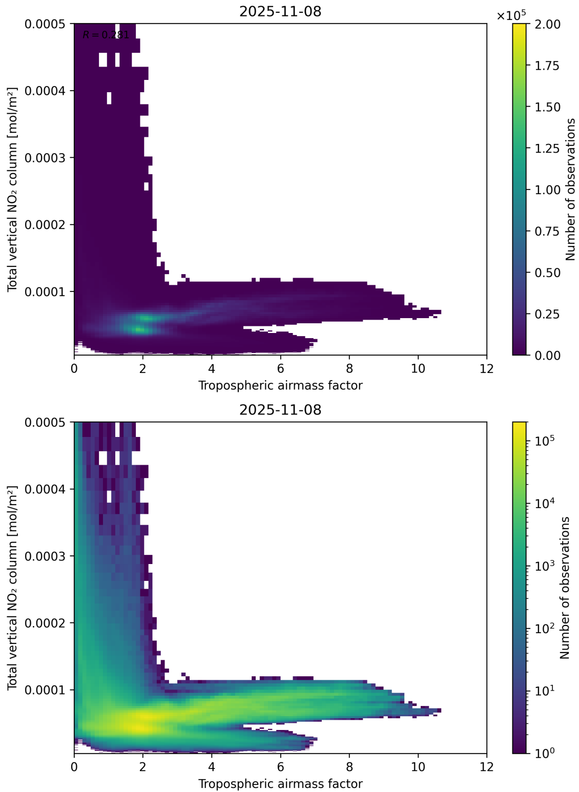
Figure 77: Scatter density plot of “Tropospheric airmass factor” against “Total vertical NO 2 column” for 2025-11-07 to 2025-11-09.
