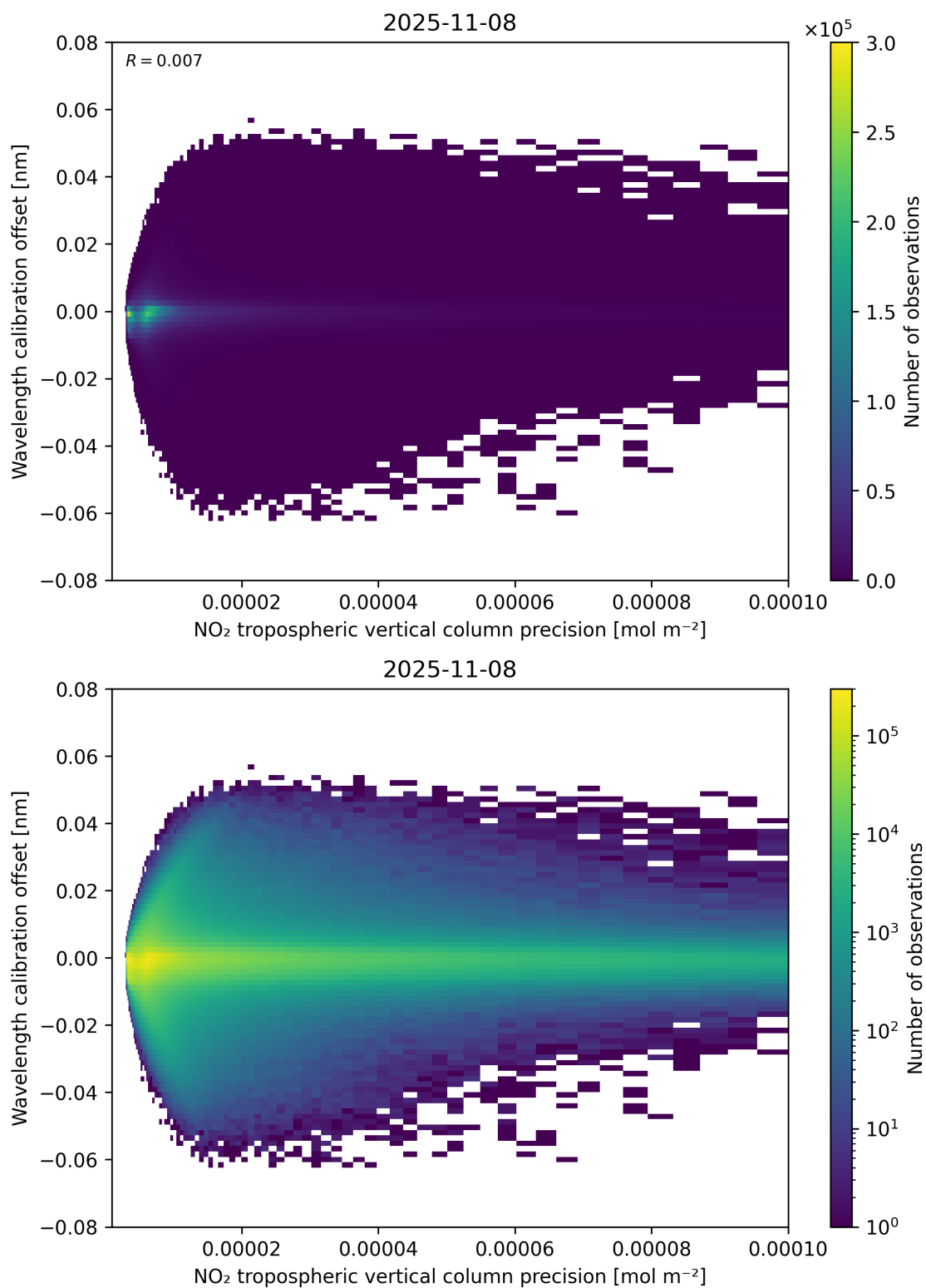
Figure 141: Scatter density plot of “NO 2 tropospheric vertical column precision” against “Wavelength calibration offset” for 2025-11-07 to 2025-11-09.
