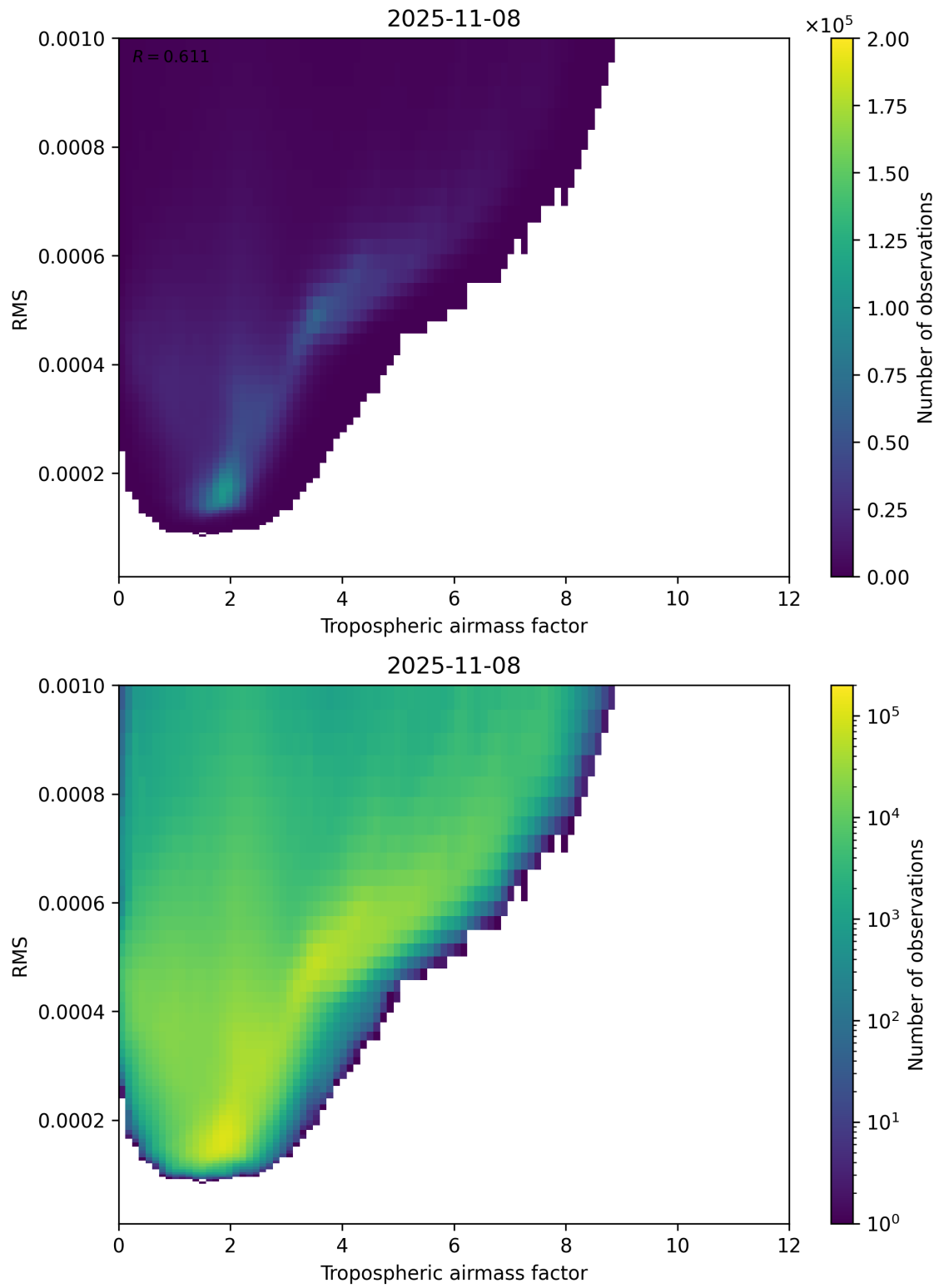
Figure 79: Scatter density plot of “Tropospheric airmass factor” against “RMS” for 2025-11-07 to 2025-11-09.
