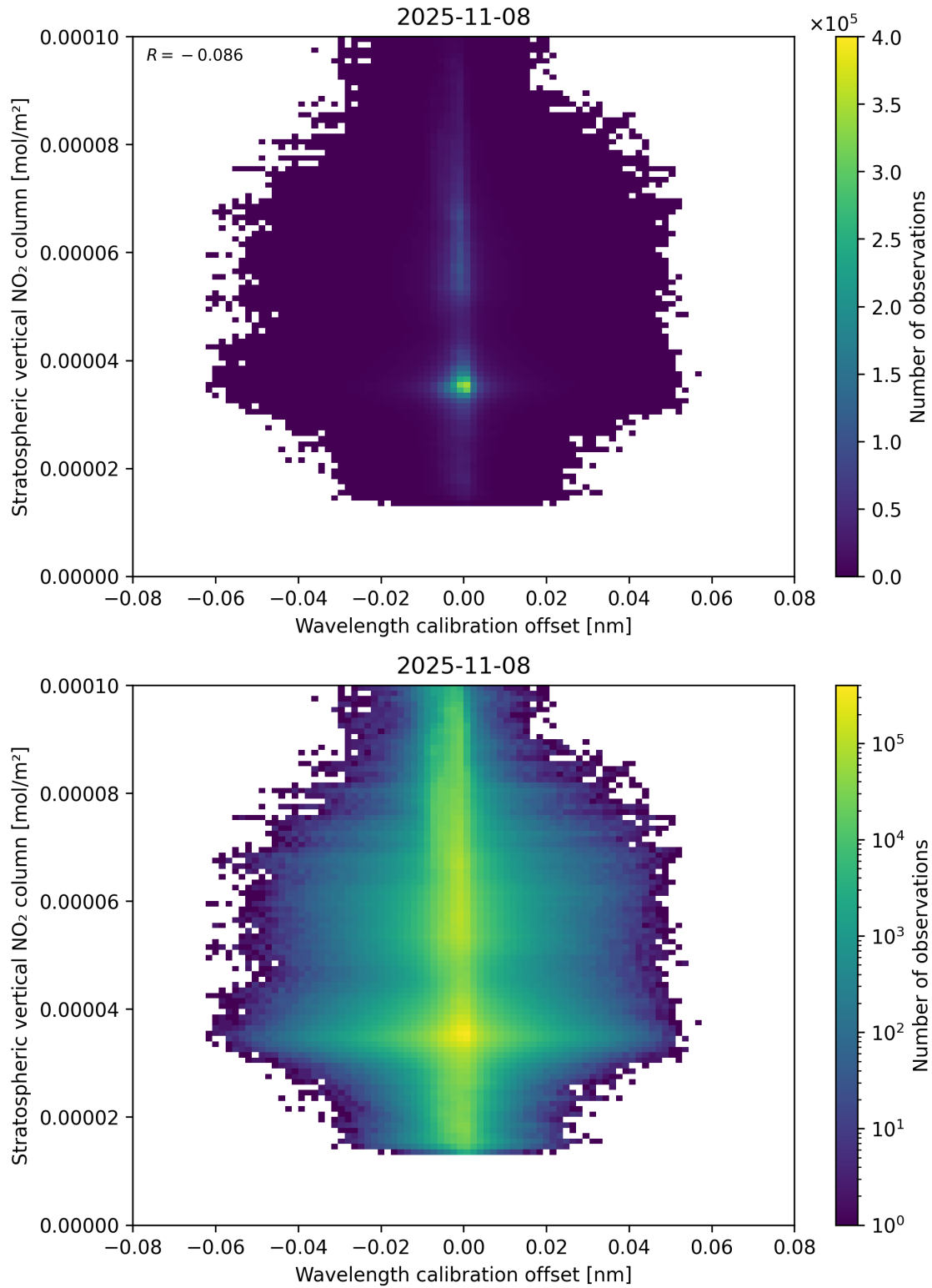
Figure 176: Scatter density plot of “Wavelength calibration offset” against “Stratospheric vertical NO 2 column” for 2025-11-07 to 2025-11-09.
