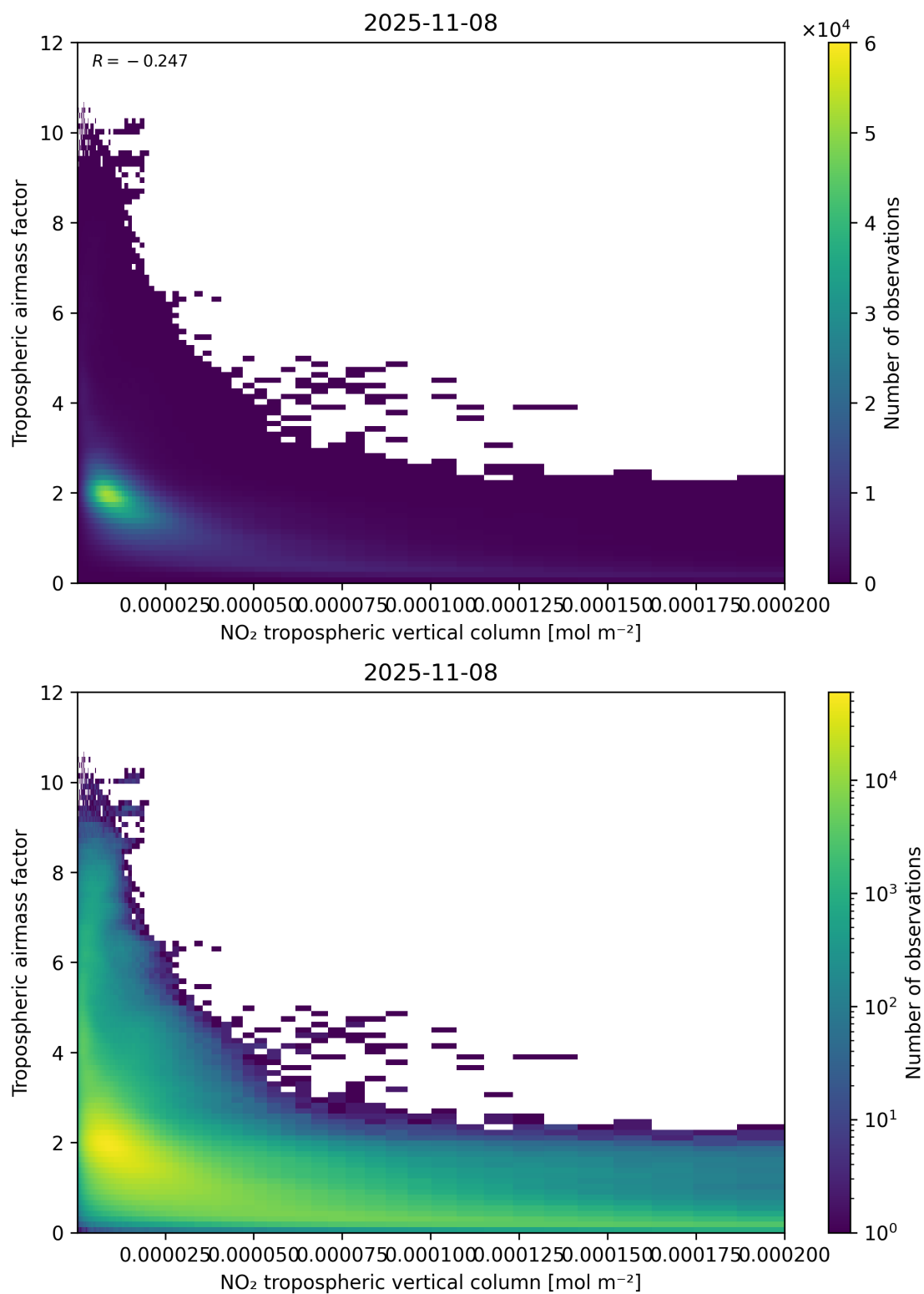
Figure 123: Scatter density plot of “NO 2 tropospheric vertical column” against “Tropospheric air mass factor” for 2025-11-07 to 2025-11-09.
