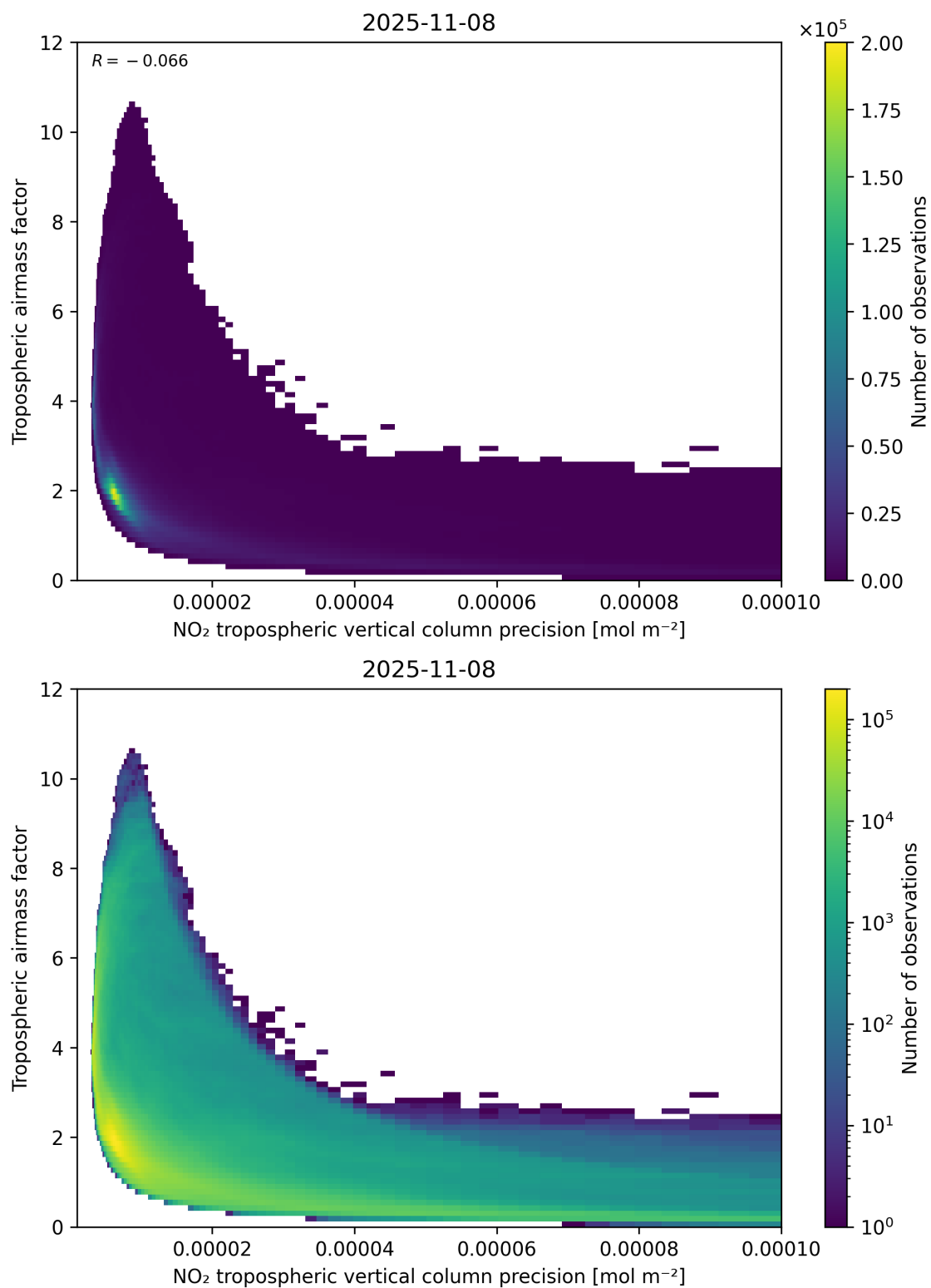
Figure 133: Scatter density plot of “NO 2 tropospheric vertical column precision” against “Tropospheric air mass factor” for 2025-11-07 to 2025-11-09.
