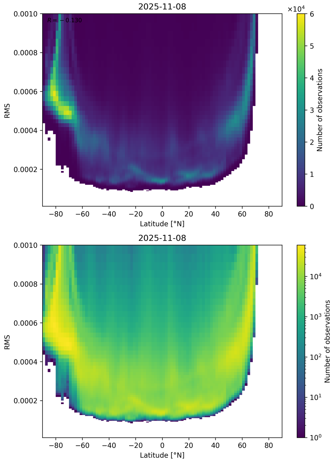
Figure 94: Scatter density plot of “Latitude” against “RMS” for 2025-11-07 to 2025-11-09.
