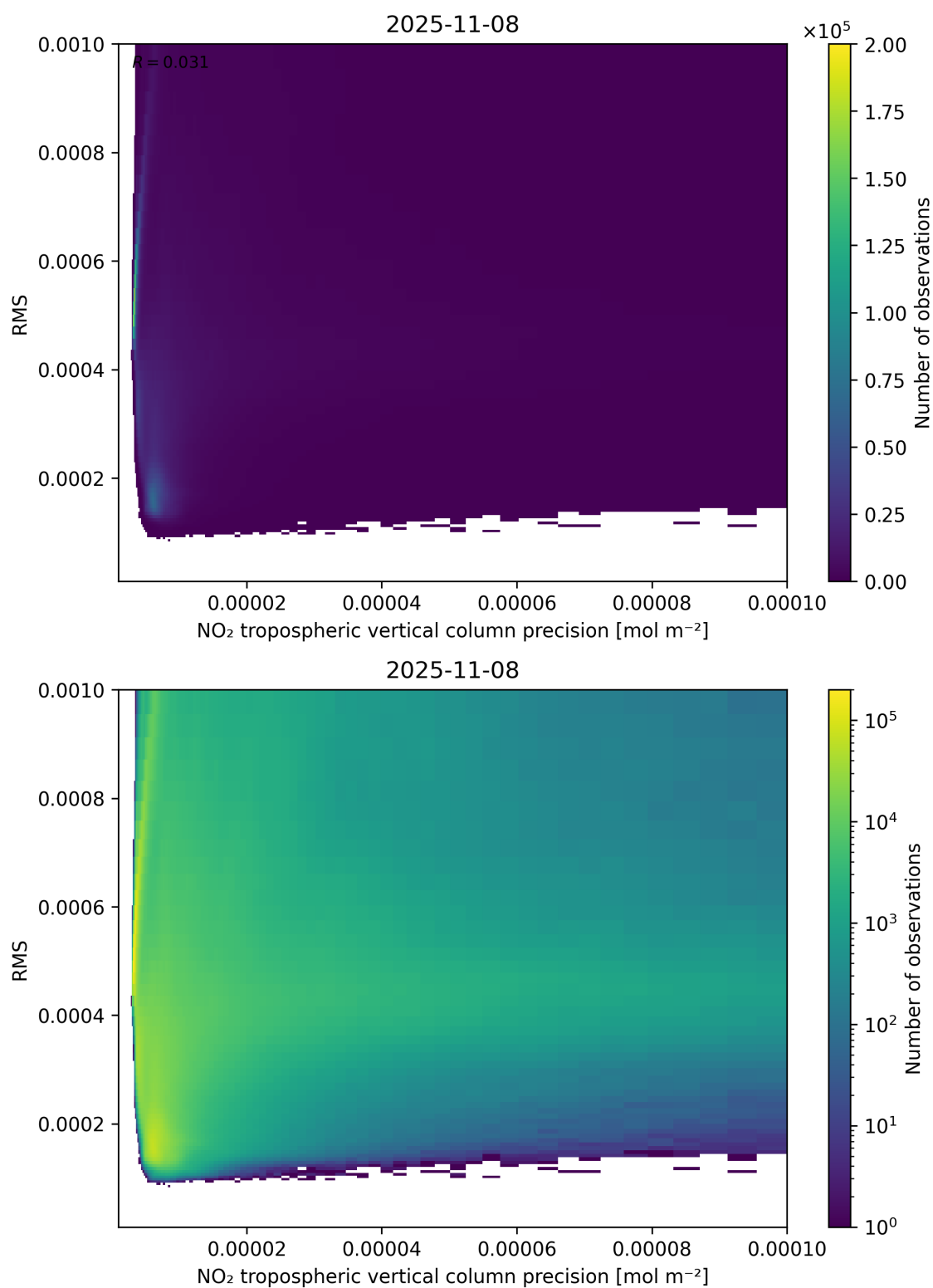
Figure 140: Scatter density plot of “NO 2 tropospheric vertical column precision” against “RMS” for 2025-11-07 to 2025-11-09.
