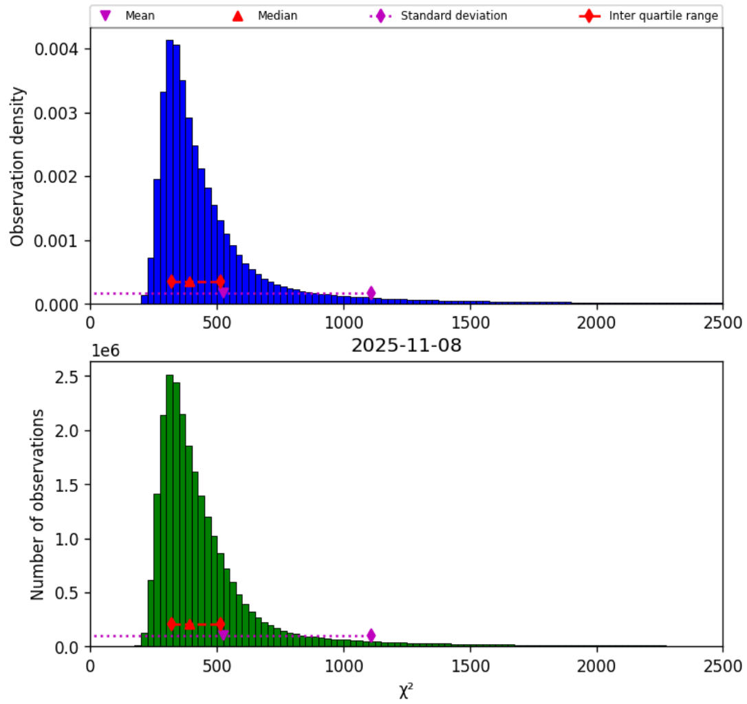
Figure 42: Histogram of “ \chi^2 ” for 2025-11-07 to 2025-11-09
