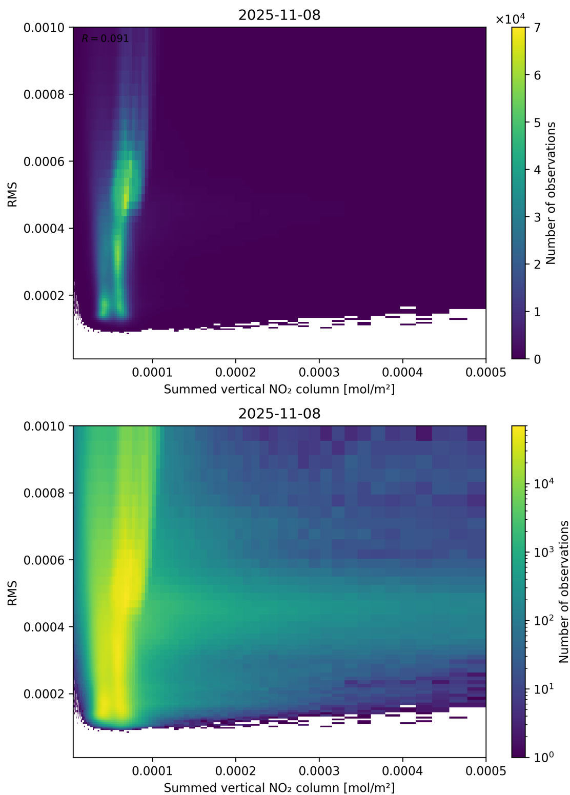
Figure 109: Scatter density plot of “Summed vertical NO 2 column” against “RMS” for 2025-11-07 to 2025-11-09.
