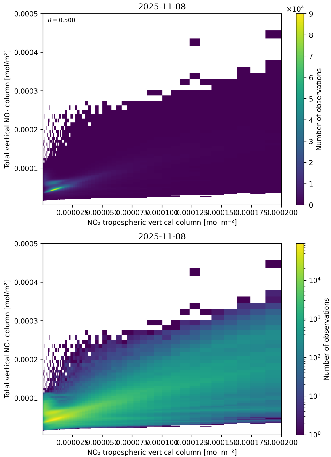
Figure 128: Scatter density plot of “NO 2 tropospheric vertical column” against “Total vertical NO 2 column” for 2025-11-07 to 2025-11-09.
