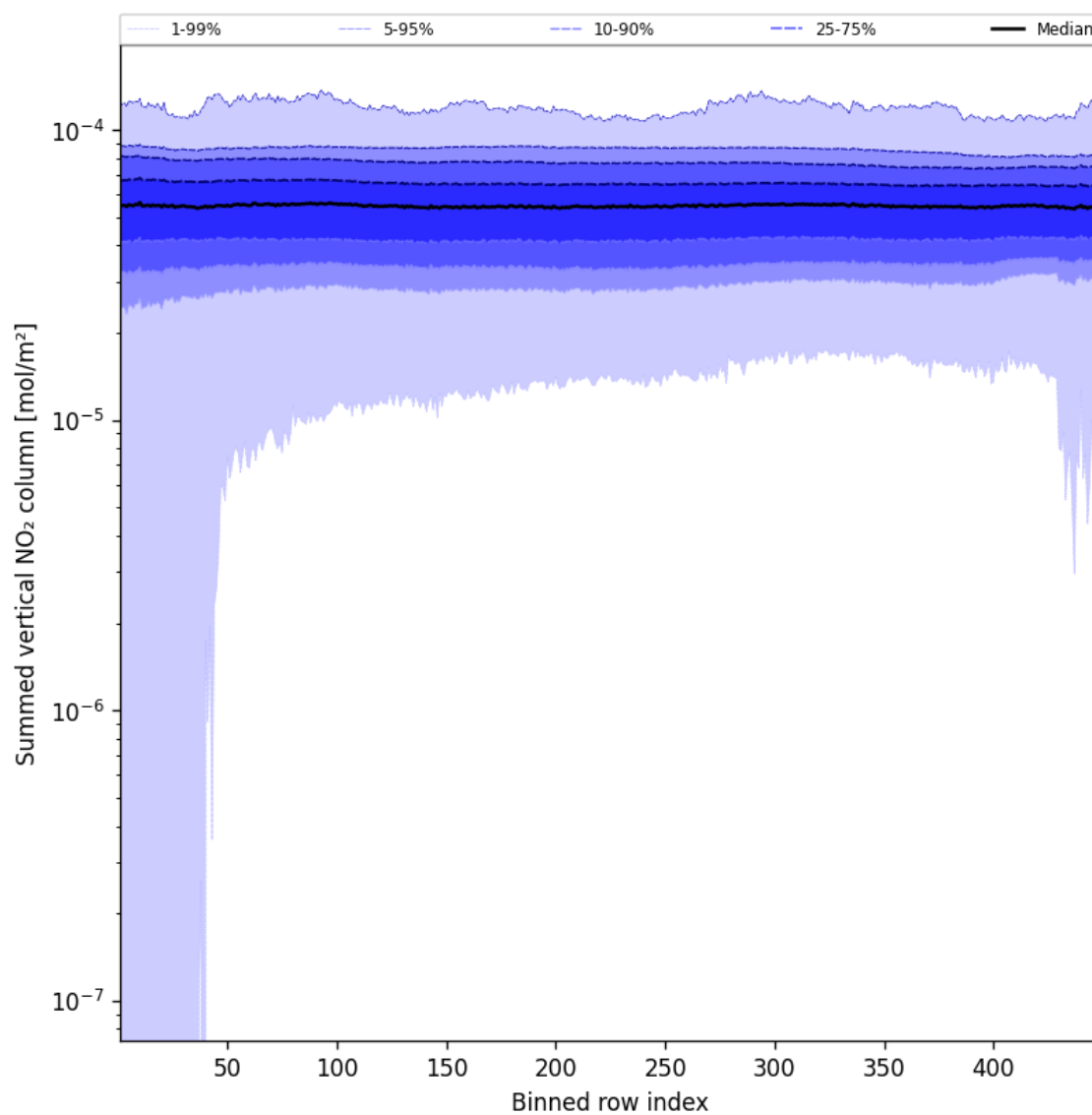
Figure 57: Along track statistics of “Summed vertical NO 2 column” for 2025-11-07 to 2025-11-09
