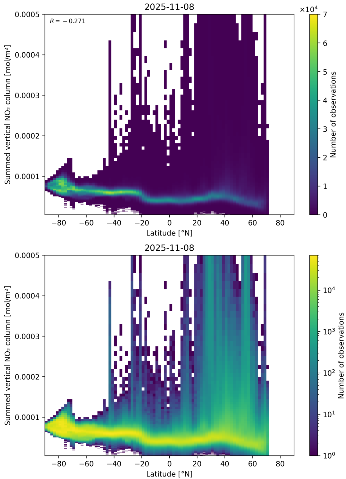
Figure 88: Scatter density plot of “Latitude” against “Summed vertical NO 2 column” for 2025-11-07 to 2025-11-09.
