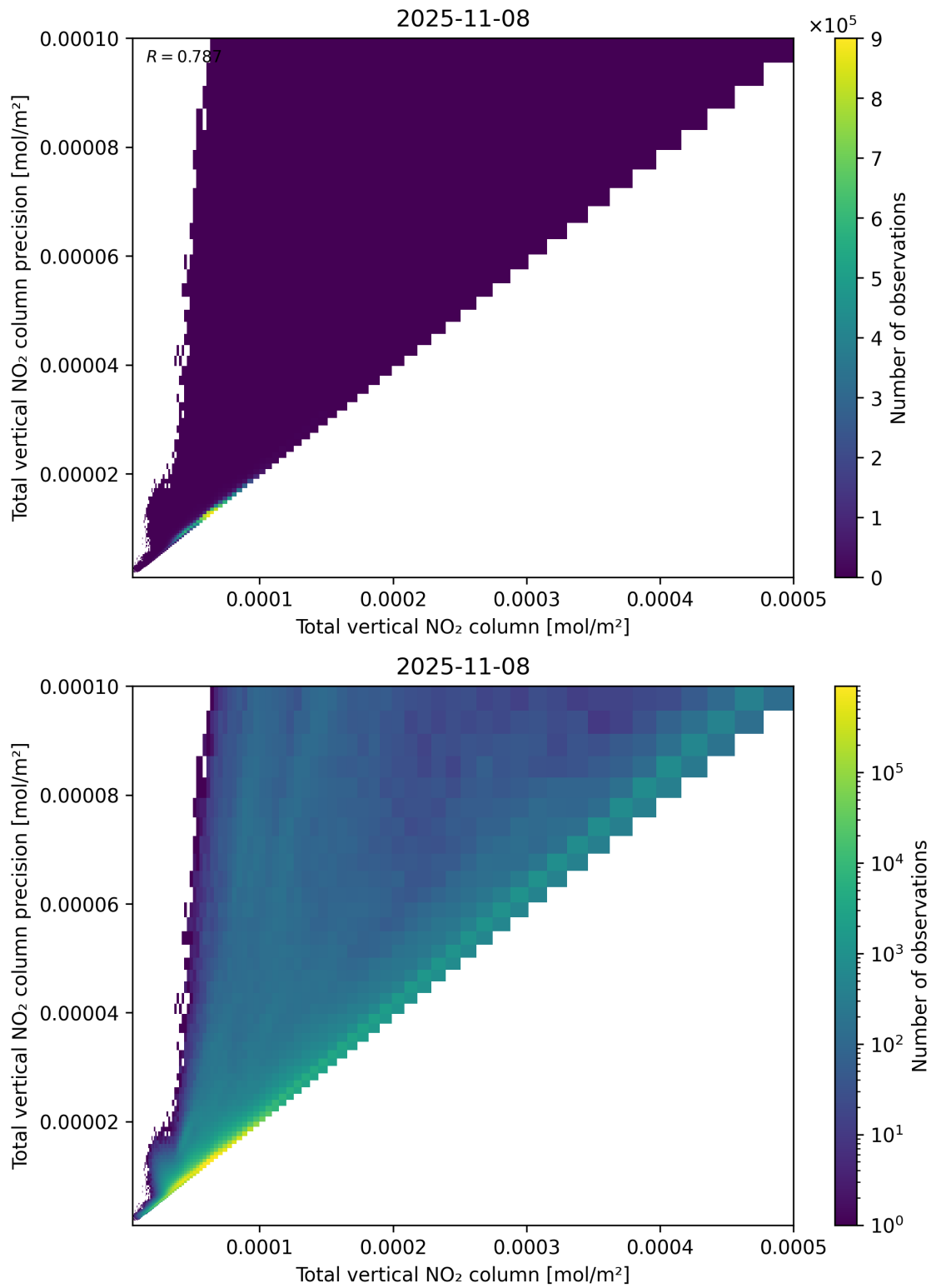
Figure 114: Scatter density plot of “Total vertical NO 2 column” against “Total vertical NO 2 column precision” for 2025-11-07 to 2025-11-09.
