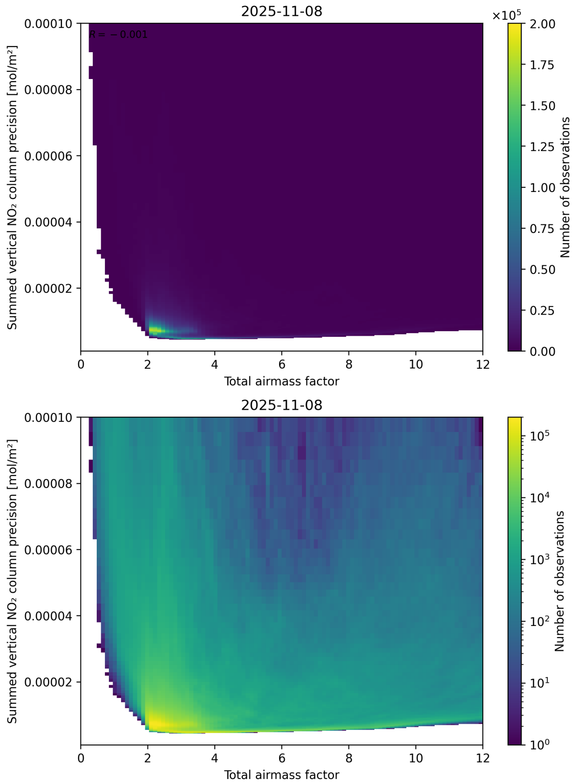
Figure 66: Scatter density plot of “Total airmass factor” against “Summed vertical NO 2 column precision” for 2025-11-07 to 2025-11-09.
