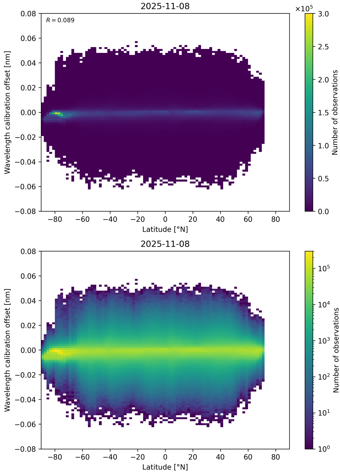
Figure 95: Scatter density plot of “Latitude” against “Wavelength calibration offset” for 2025-11-07 to 2025-11-09.
