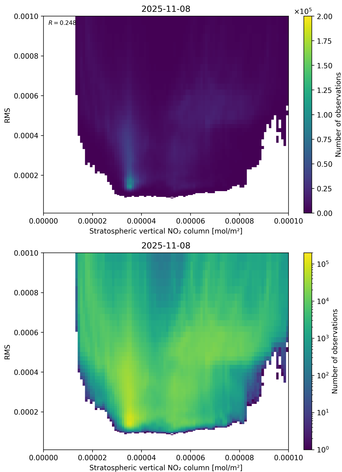
Figure 102: Scatter density plot of “Stratospheric vertical NO 2 column” against “RMS” for 2025-11-07 to 2025-11-09.
