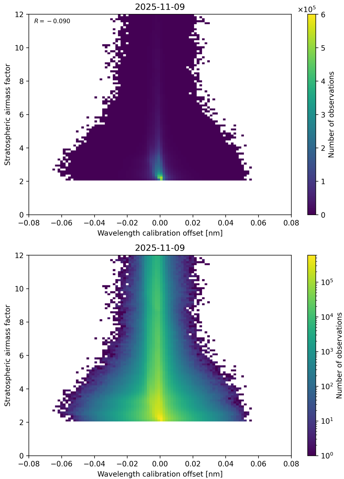
Figure 174: Scatter density plot of “Wavelength calibration offset” against “Stratospheric airmass factor” for 2025-11-08 to 2025-11-10.
