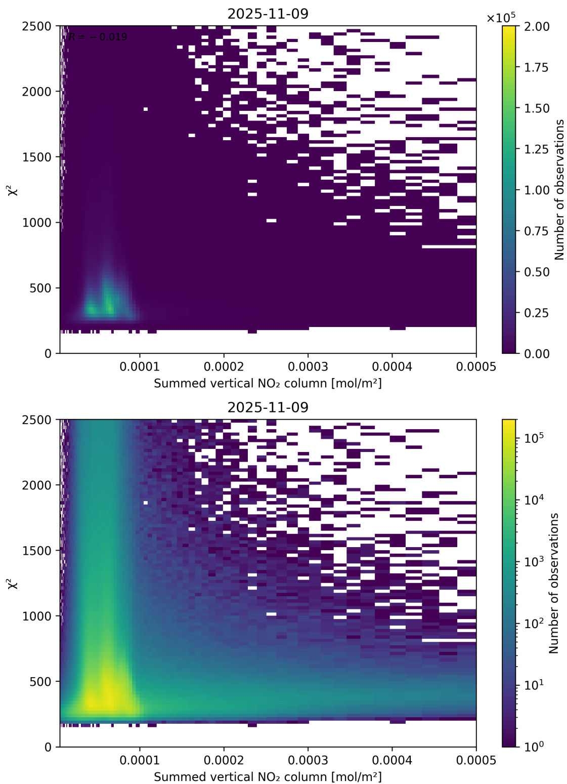
Figure 104: Scatter density plot of “Summed vertical NO 2 column” against “ \chi^2 ” for 2025-11-08 to 2025-11-10.
