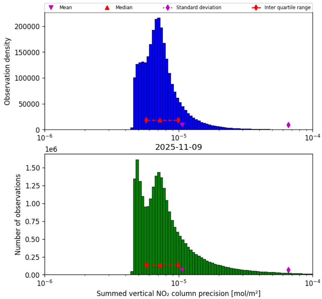
Figure 41: Histogram of “Summed vertical NO 2 column precision” for 2025-11-08 to 2025-11-10
