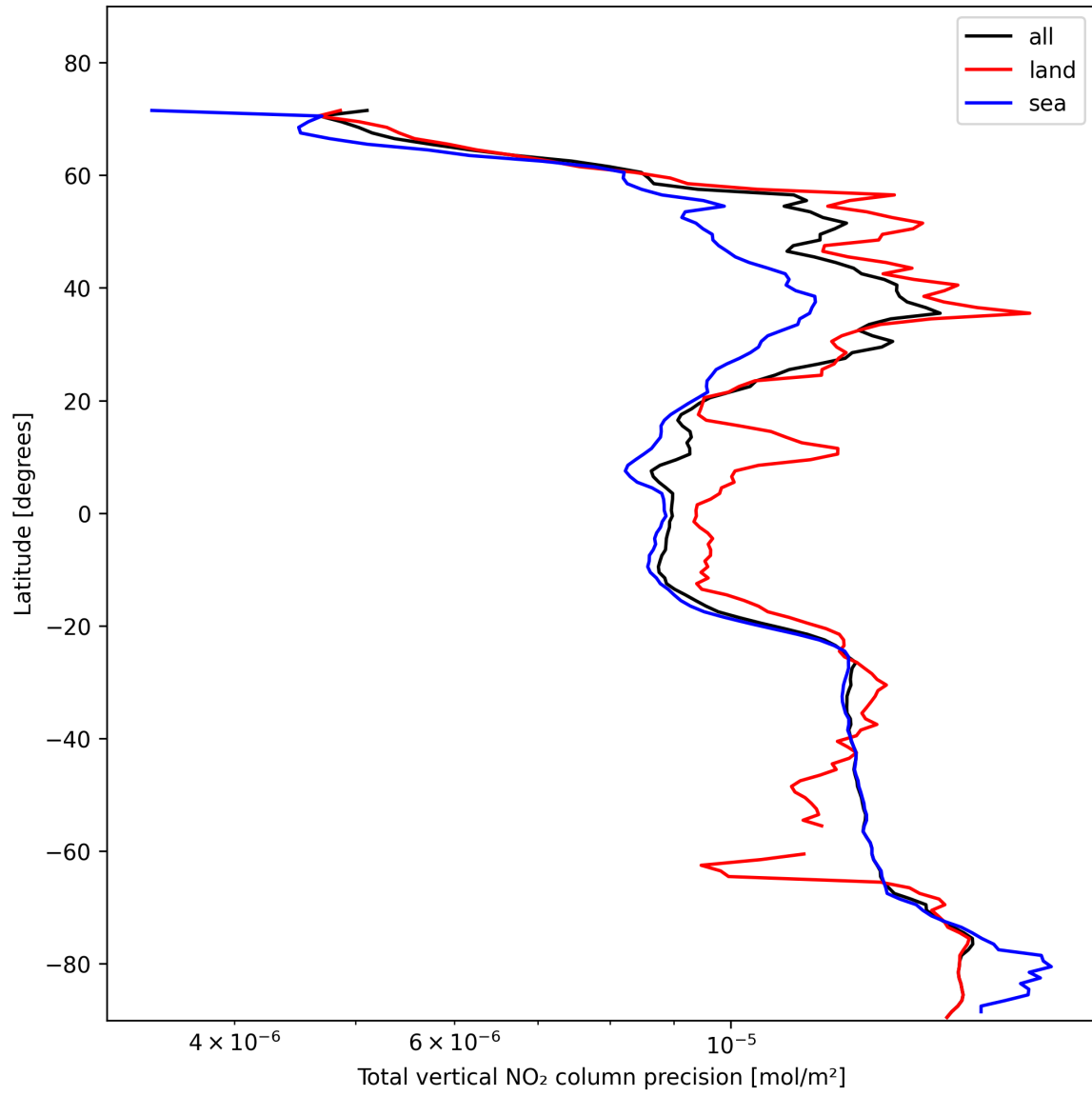
Figure 22: Zonal average of “Total vertical NO 2 column precision” for 2025-11-08 to 2025-11-10.
