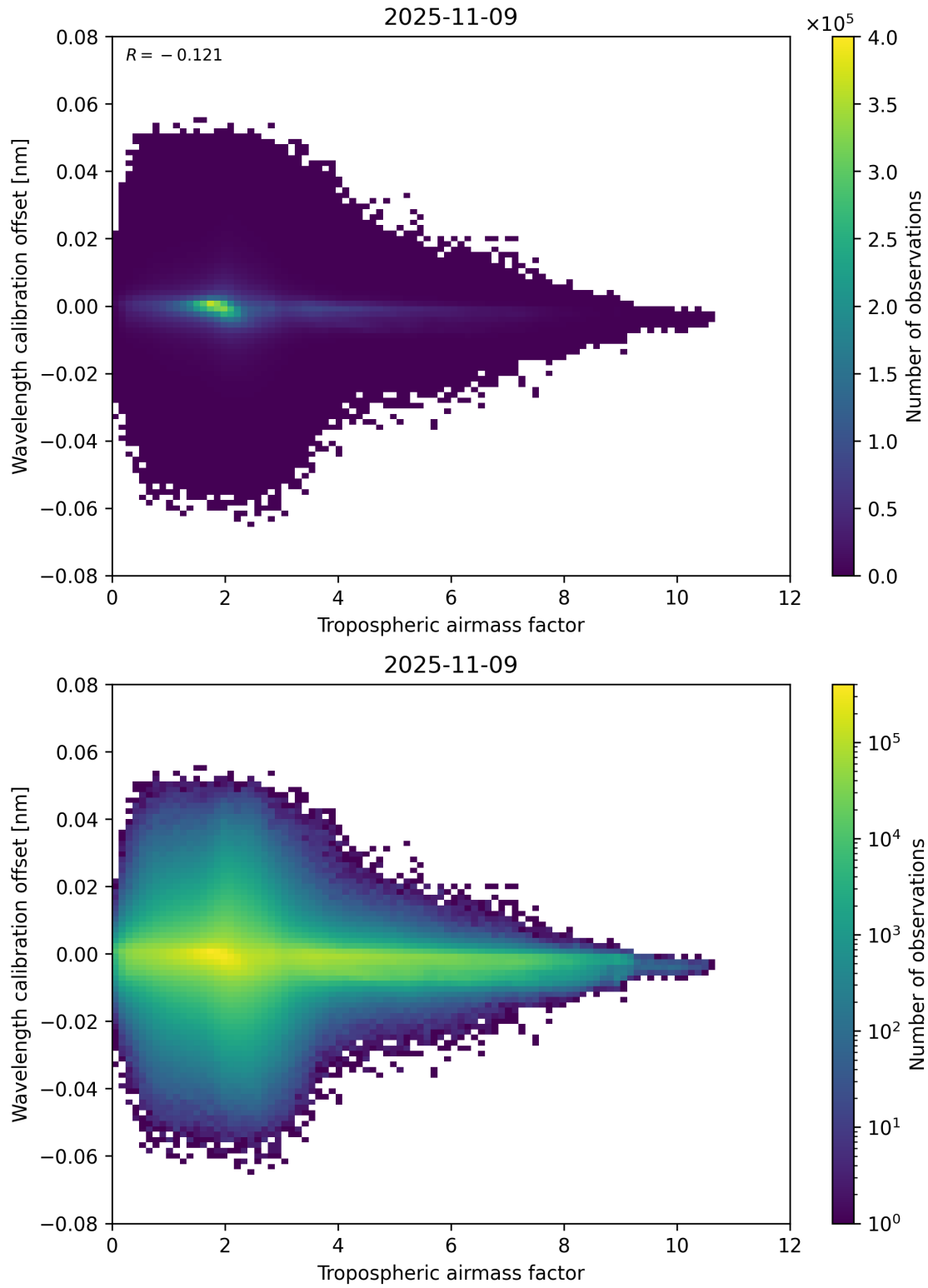
Figure 80: Scatter density plot of “Tropospheric airmass factor” against “Wavelength calibration offset” for 2025-11-08 to 2025-11-10.
