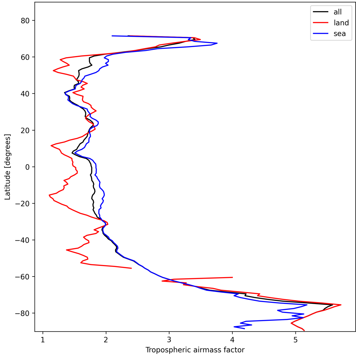
Figure 14: Zonal average of “Tropospheric airmass factor” for 2025-11-08 to 2025-11-10.
