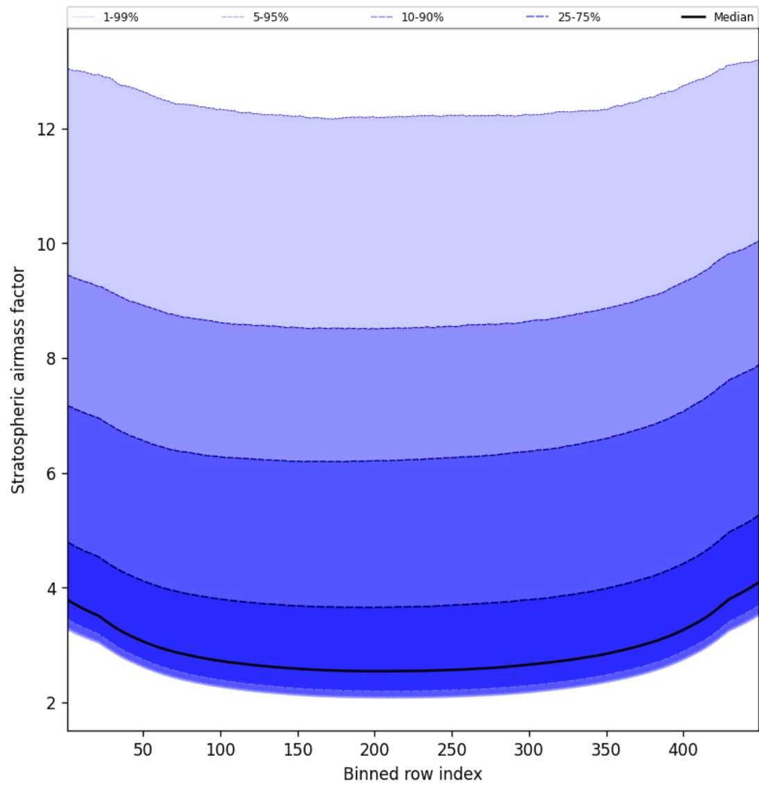
Figure 61: Along track statistics of “Stratospheric airmass factor” for 2025-11-08 to 2025-11-10
