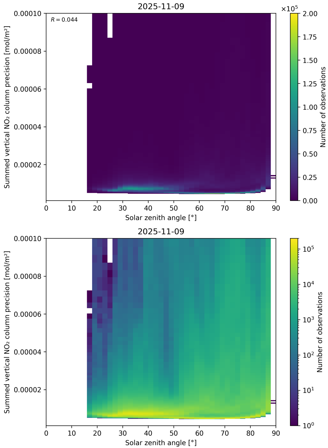
Figure 152: Scatter density plot of “Solar zenith angle” against “Summed vertical NO 2 column precision” for 2025-11-08 to 2025-11-10.
