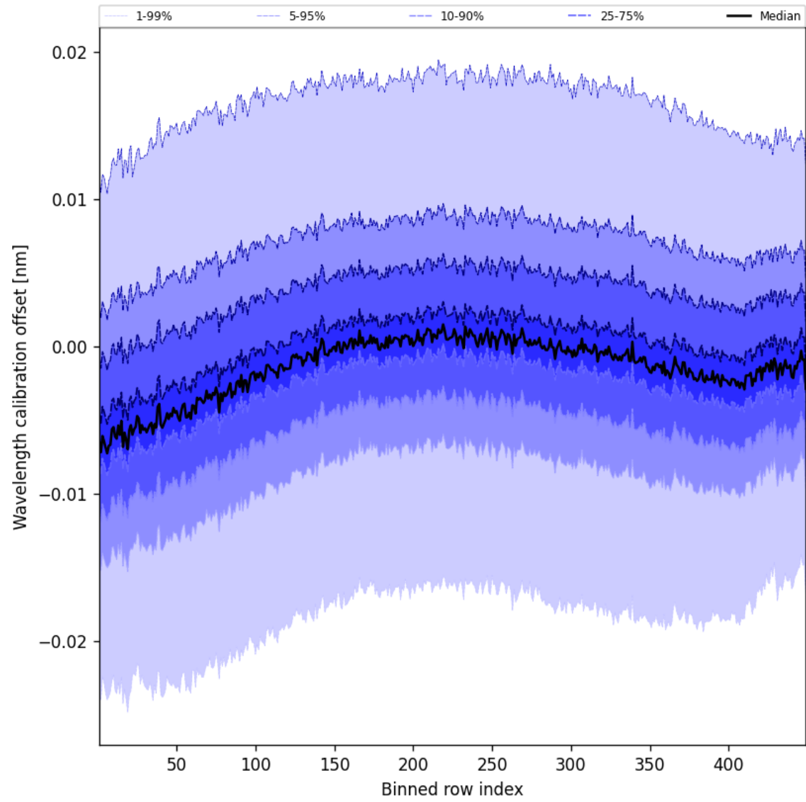
Figure 52: Along track statistics of “Wavelength calibration offset” for 2025-11-08 to 2025-11-10
