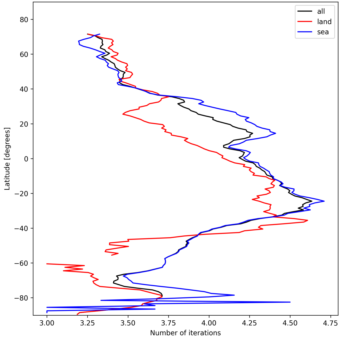
Figure 17: Zonal average of “Number of iterations” for 2025-11-08 to 2025-11-10.
