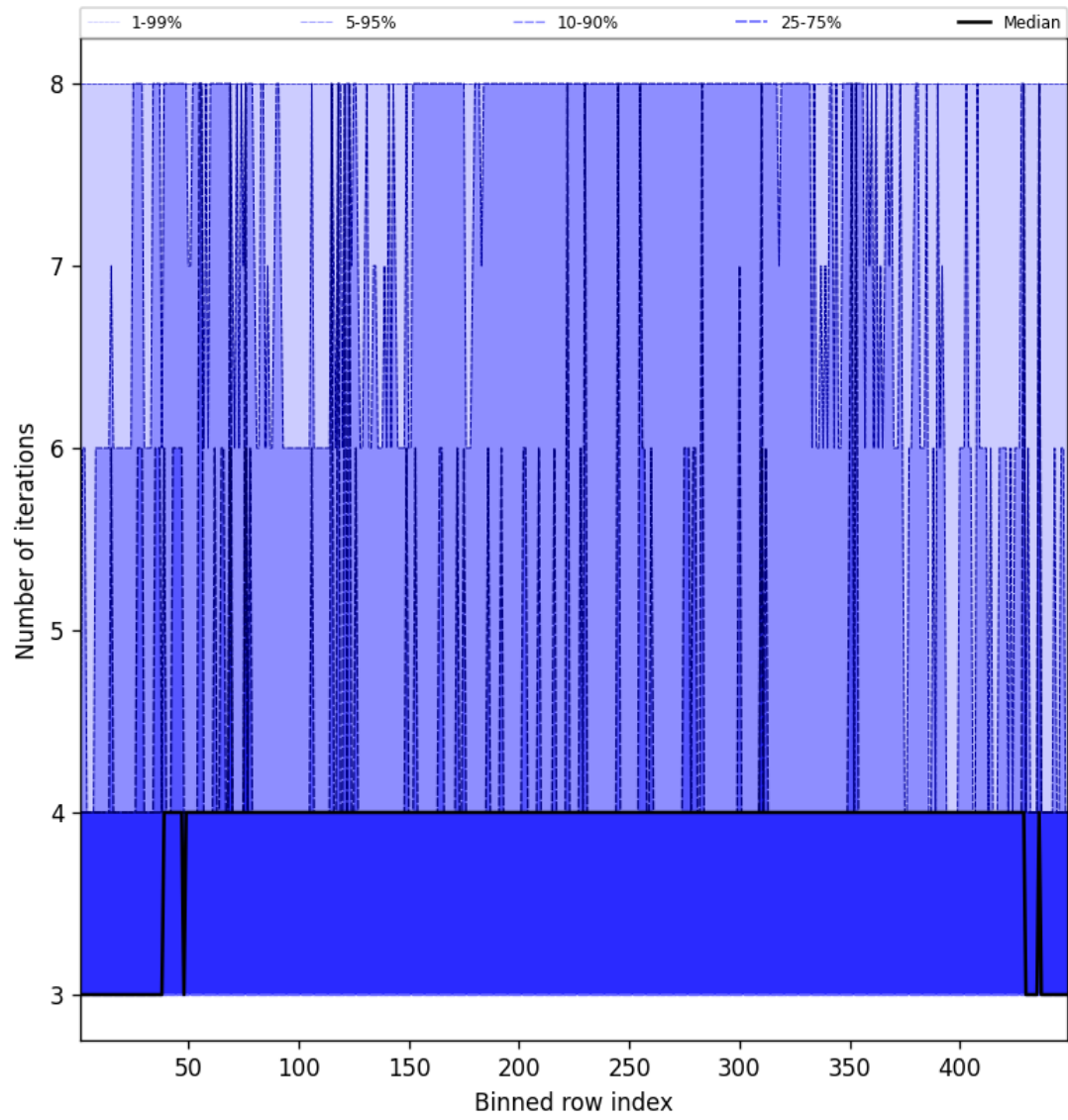
Figure 51: Along track statistics of “Number of iterations” for 2025-11-08 to 2025-11-10
