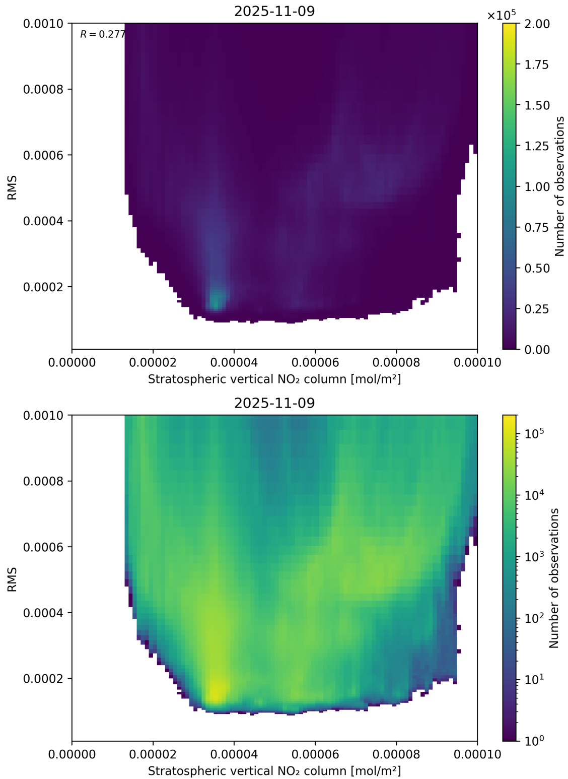
Figure 102: Scatter density plot of “Stratospheric vertical NO 2 column” against “RMS” for 2025-11-08 to 2025-11-10.
