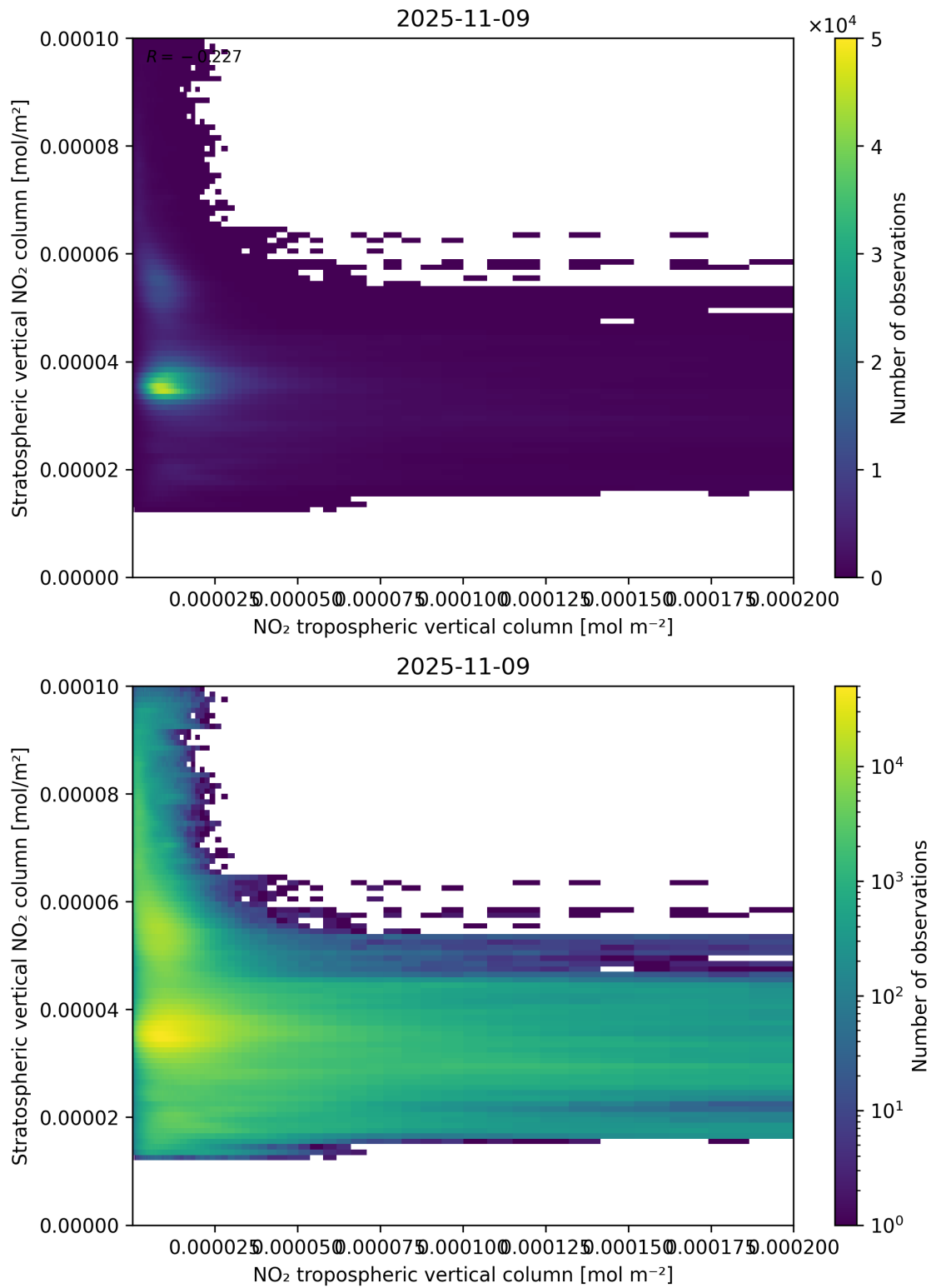
Figure 125: Scatter density plot of “NO 2 tropospheric vertical column” against “Stratospheric vertical NO 2 column” for 2025-11-08 to 2025-11-10.
