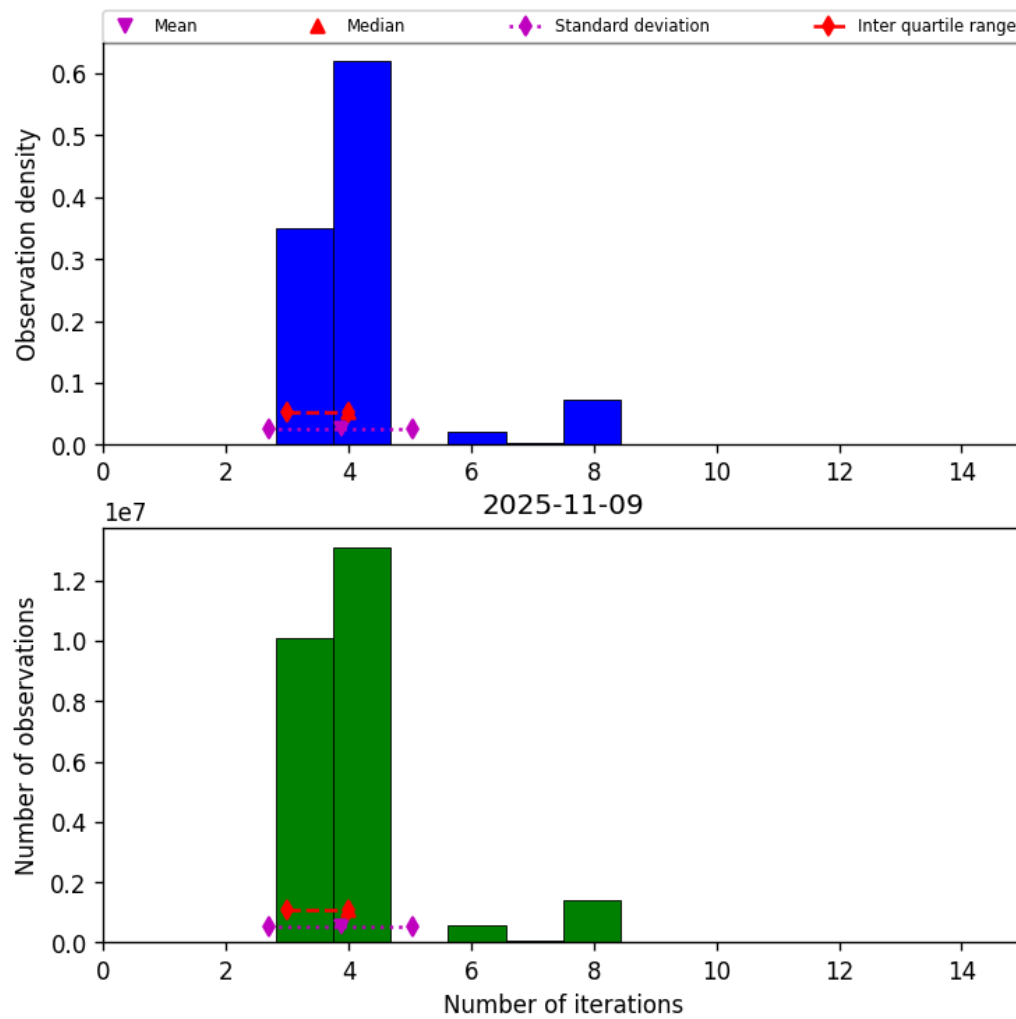
Figure 34: Histogram of “Number of iterations” for 2025-11-08 to 2025-11-10
