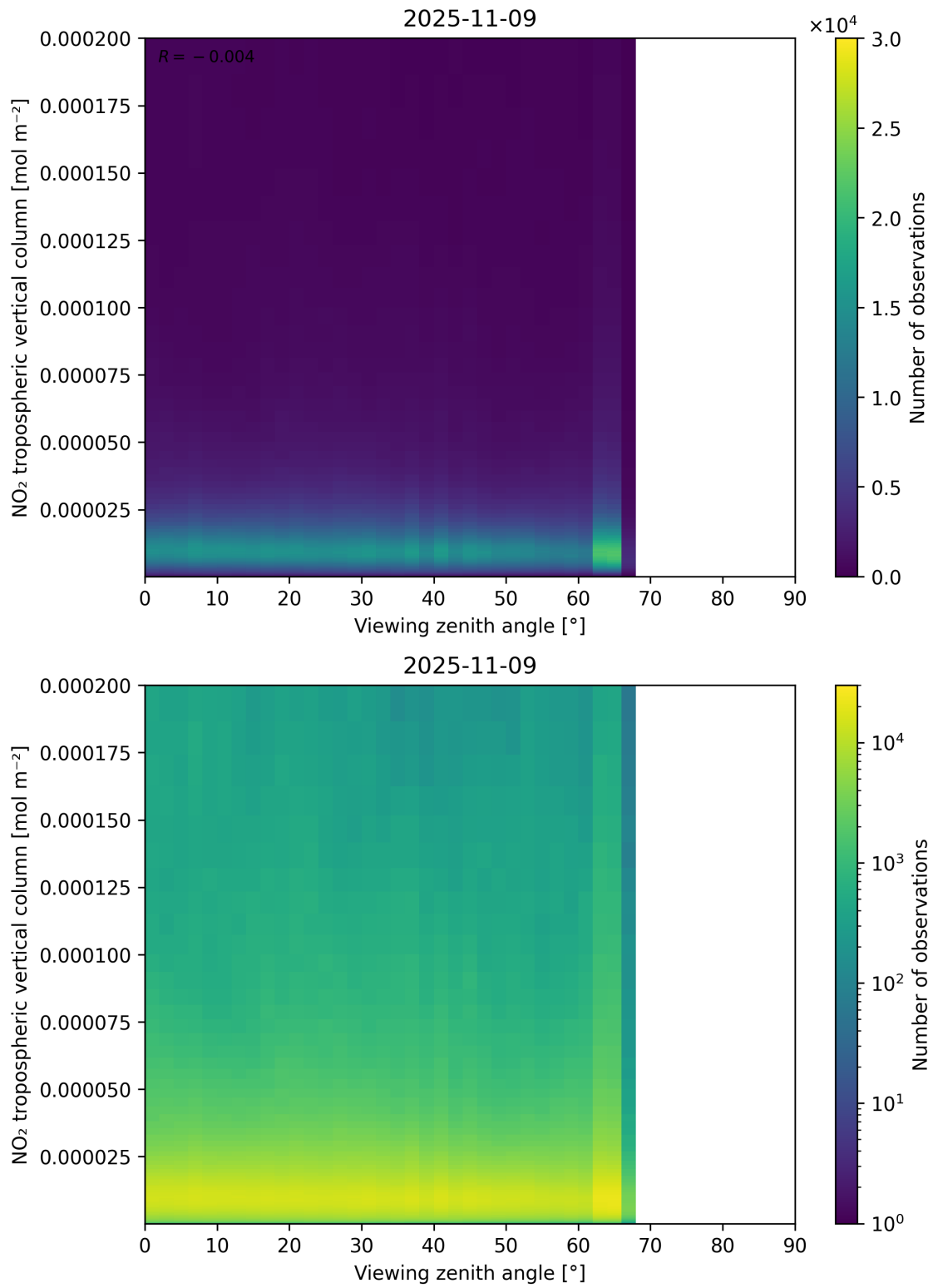
Figure 169: Scatter density plot of “Viewing zenith angle” against “NO 2 tropospheric vertical column” for 2025-11-08 to 2025-11-10.
