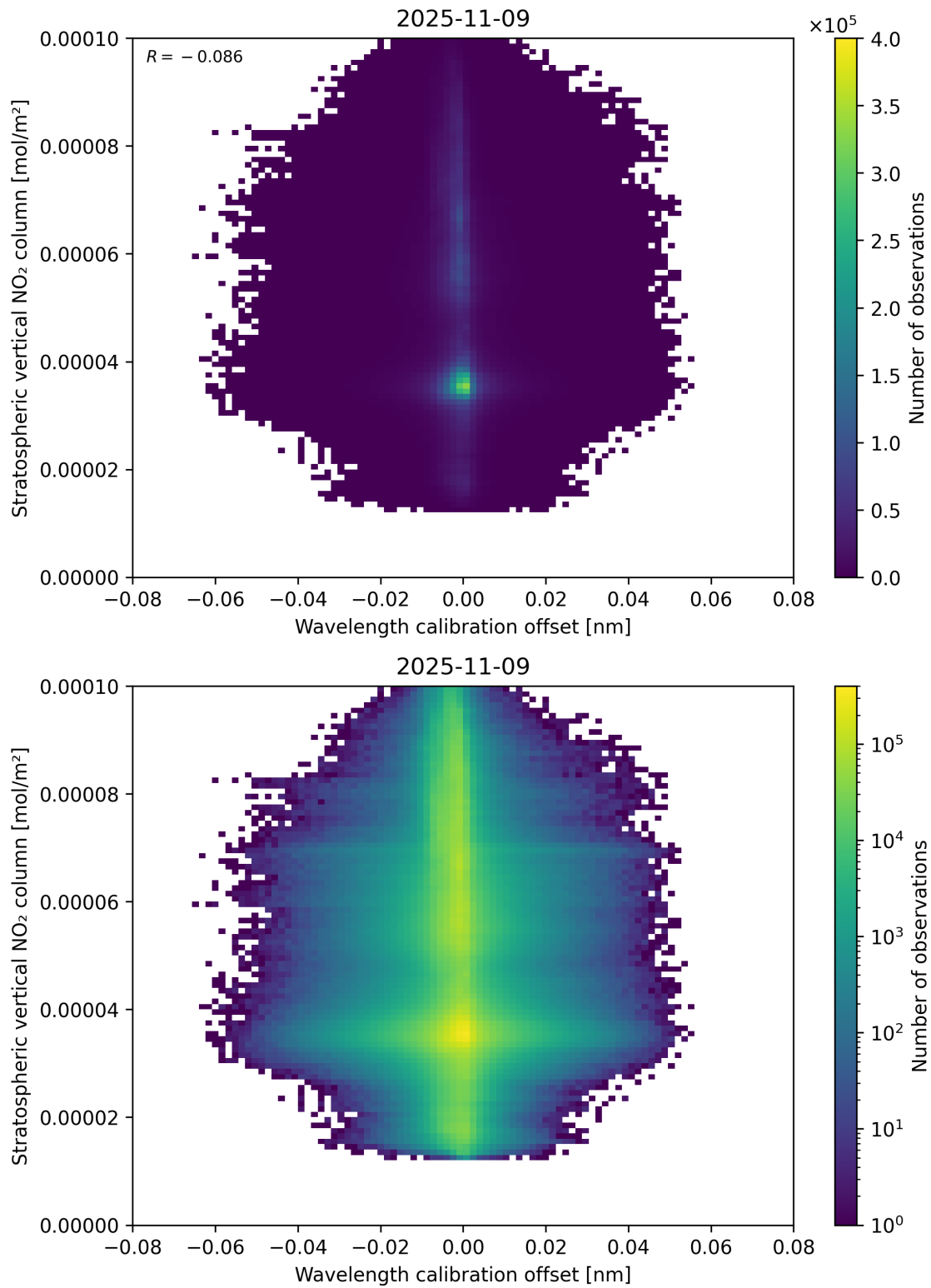
Figure 176: Scatter density plot of “Wavelength calibration offset” against “Stratospheric vertical NO 2 column” for 2025-11-08 to 2025-11-10.
