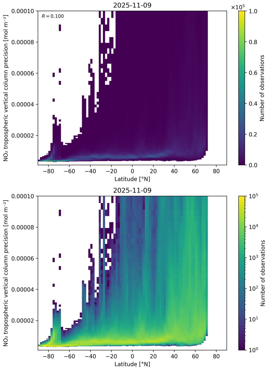
Figure 93: Scatter density plot of “Latitude” against “NO 2 tropospheric vertical column precision” for 2025-11-08 to 2025-11-10.
