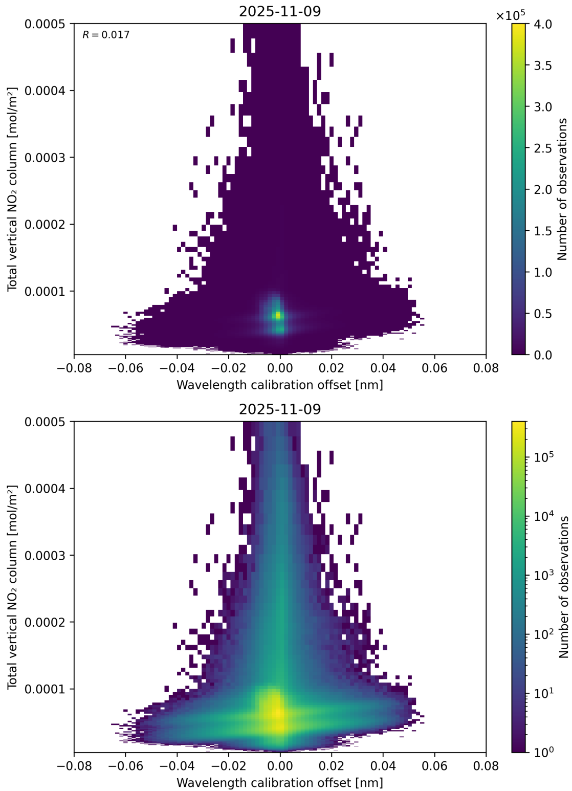
Figure 179: Scatter density plot of “Wavelength calibration offset” against “Total vertical NO 2 column” for 2025-11-08 to 2025-11-10.
