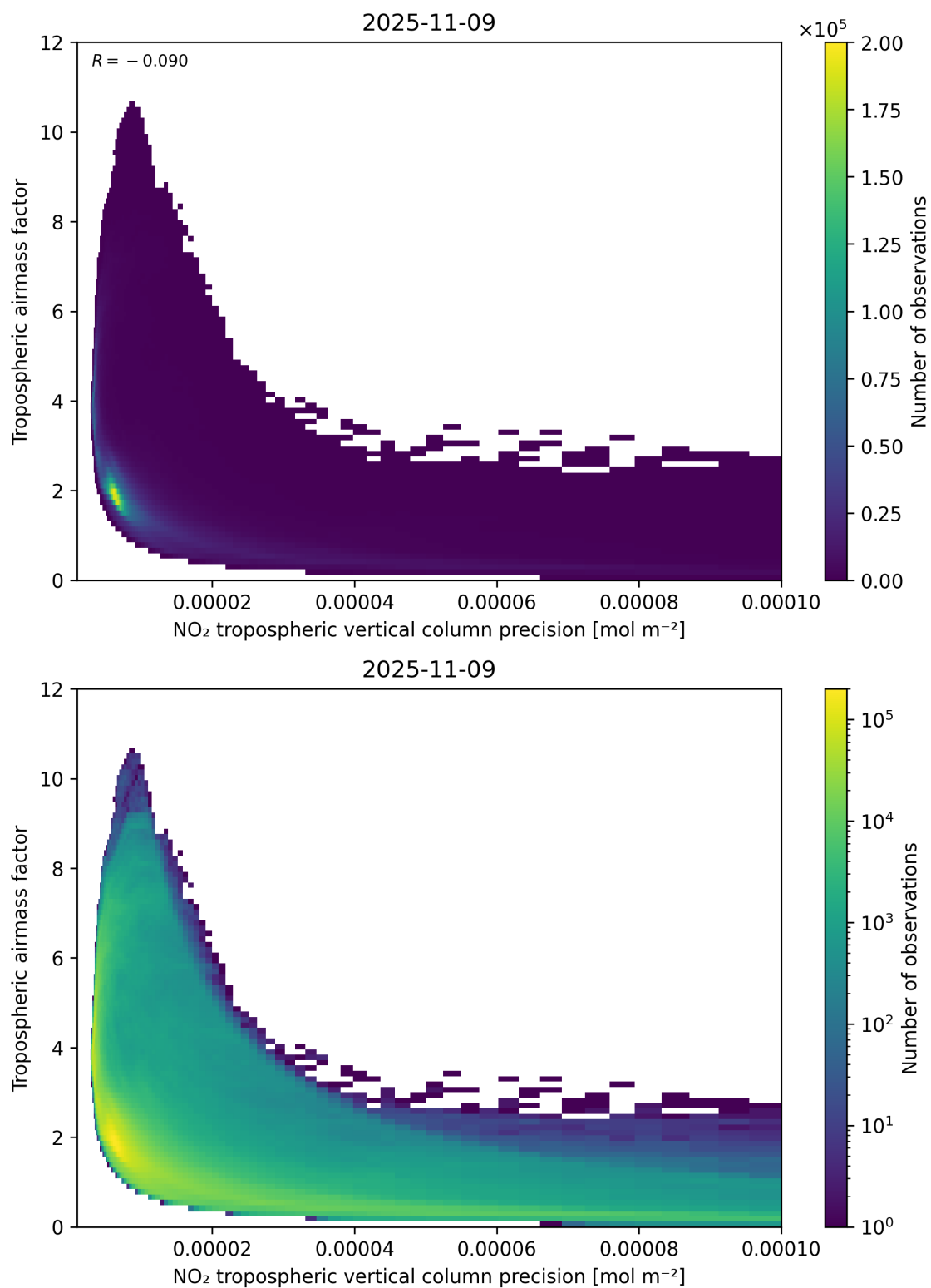
Figure 133: Scatter density plot of “NO 2 tropospheric vertical column precision” against “Tropospheric airmass factor” for 2025-11-08 to 2025-11-10.
