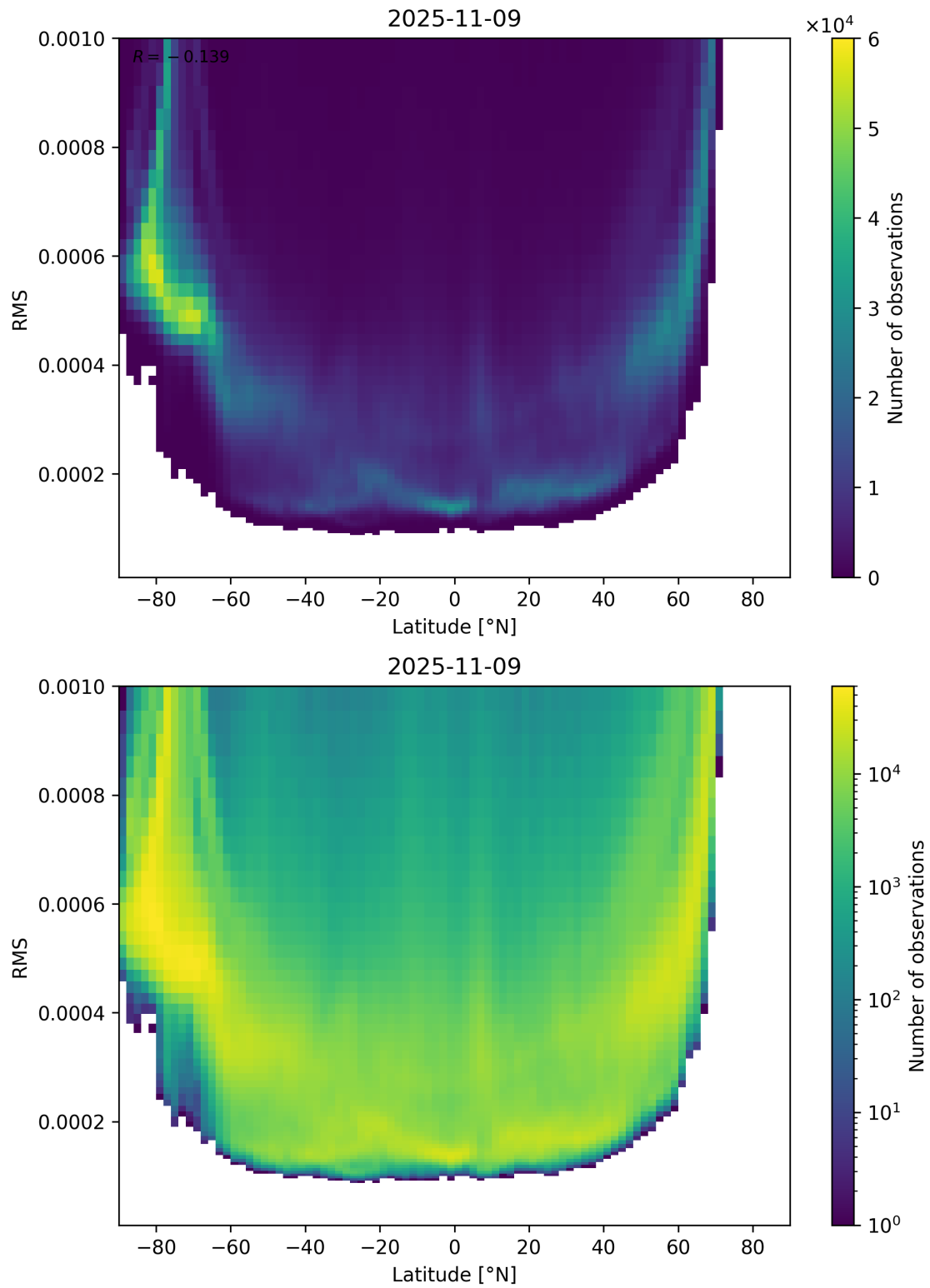
Figure 94: Scatter density plot of “Latitude” against “RMS” for 2025-11-08 to 2025-11-10.
