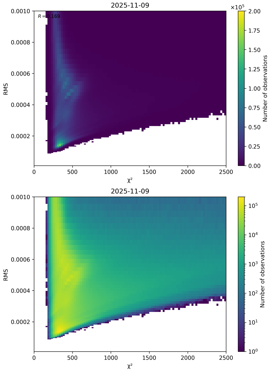
Figure 82: Scatter density plot of “ \chi^2 ” against “RMS” for 2025-11-08 to 2025-11-10.
