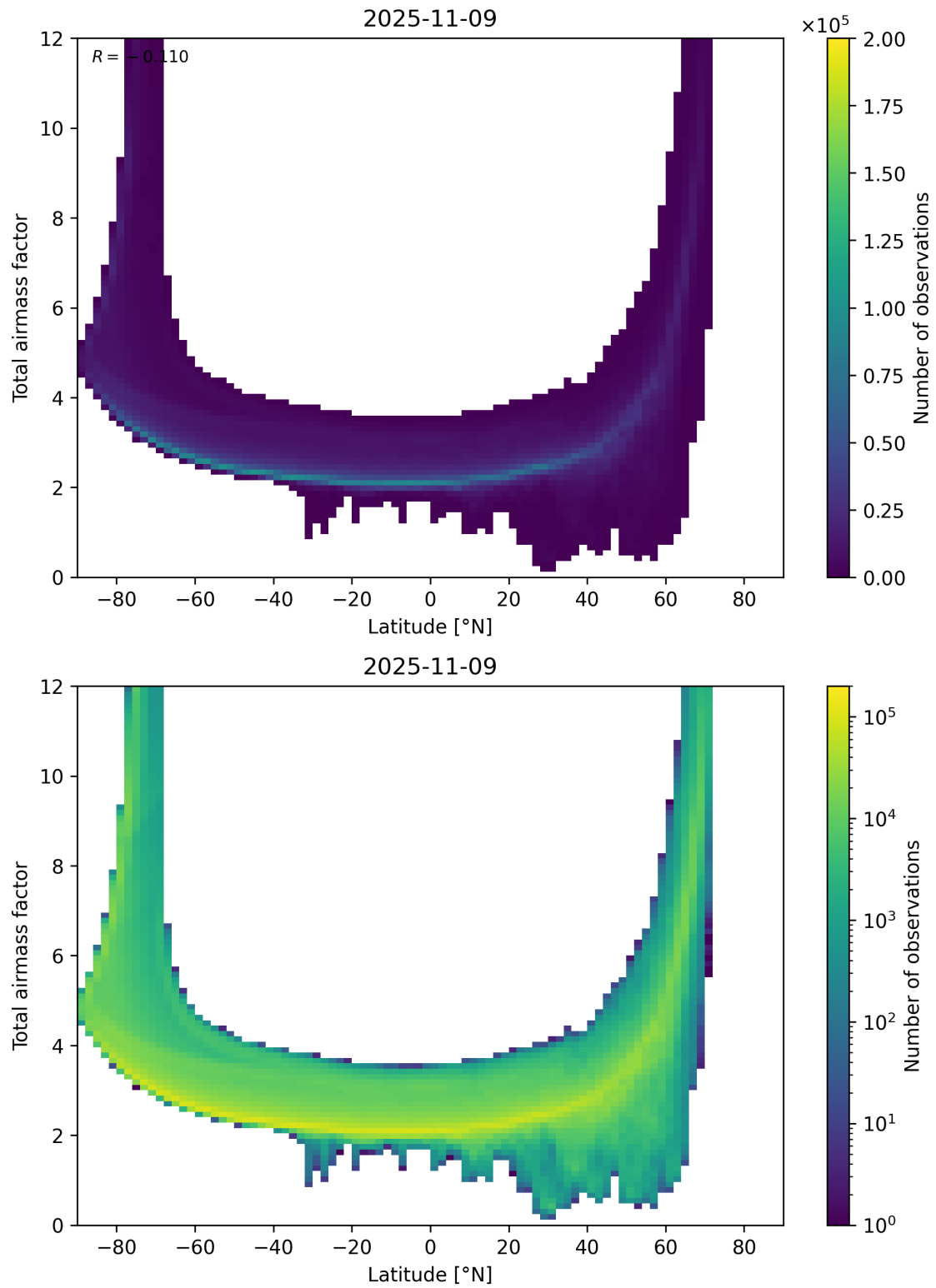
Figure 84: Scatter density plot of “Latitude” against “Total airmass factor” for 2025-11-08 to 2025-11-10.
