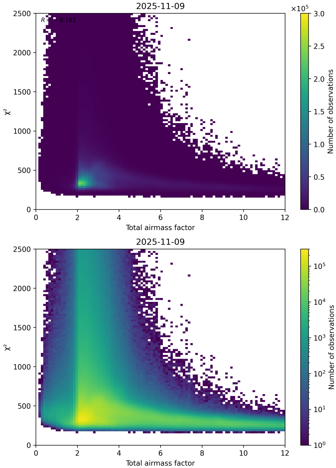
Figure 63: Scatter density plot of “Total airmass factor” against “ \chi^2 ” for 2025-11-08 to 2025-11-10.
