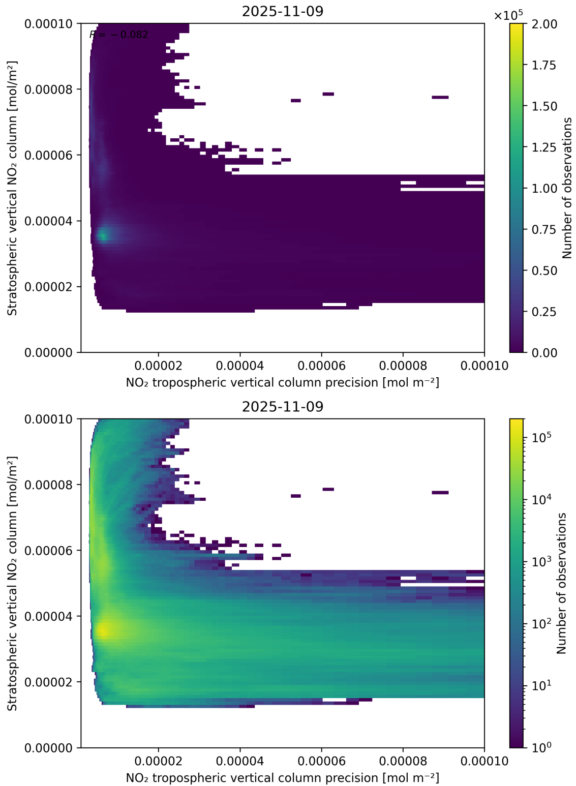
Figure 135: Scatter density plot of “NO 2 tropospheric vertical column precision” against “Stratospheric vertical NO 2 column” for 2025-11-08 to 2025-11-10.
