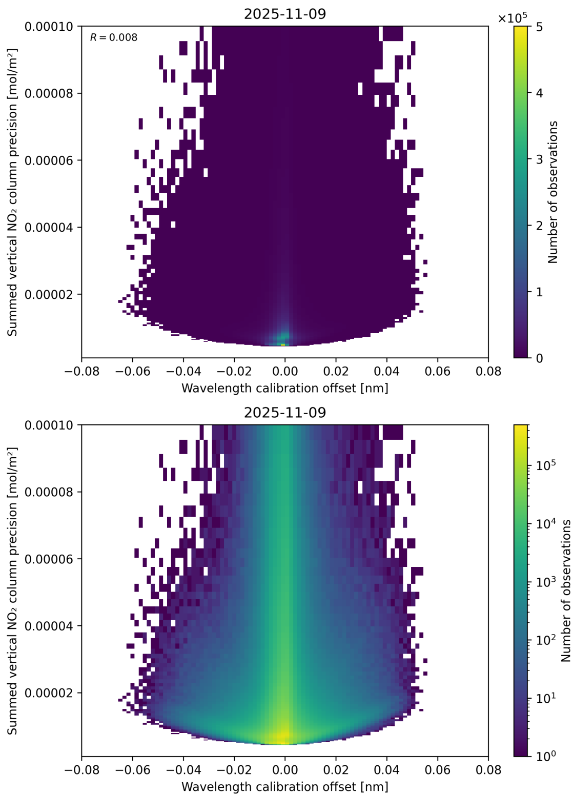
Figure 178: Scatter density plot of “Wavelength calibration offset” against “Summed vertical NO 2 column precision” for 2025-11-08 to 2025-11-10.
