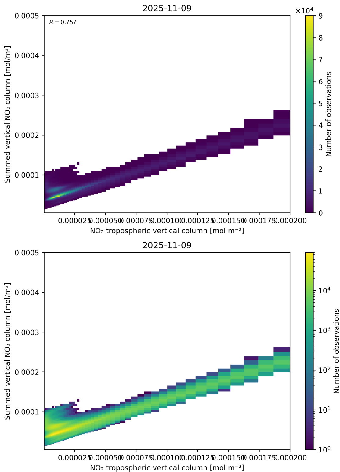
Figure 126: Scatter density plot of “NO 2 tropospheric vertical column” against “Summed vertical NO 2 column” for 2025-11-08 to 2025-11-10.
