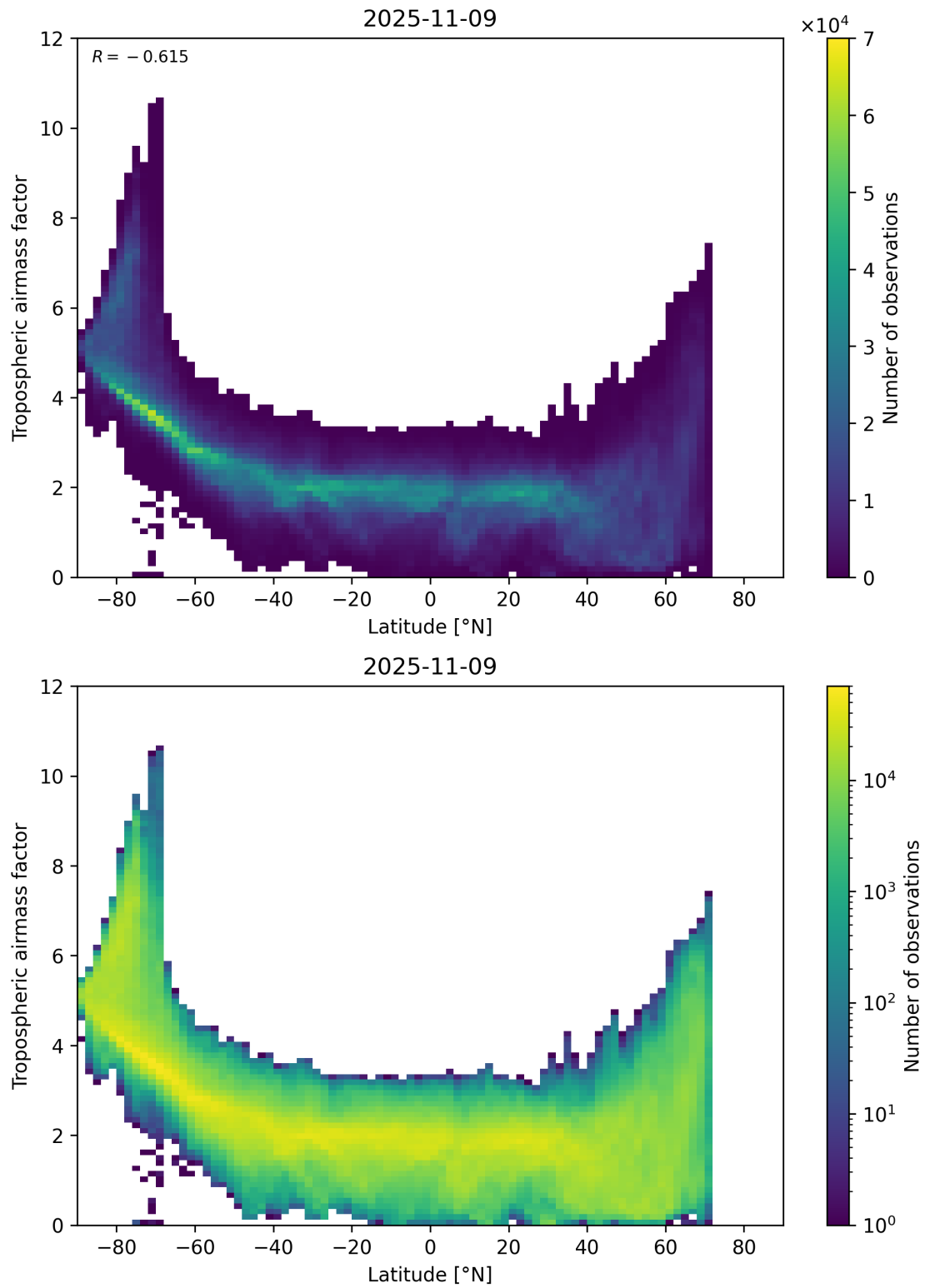
Figure 85: Scatter density plot of “Latitude” against “Tropospheric air mass factor” for 2025-11-08 to 2025-11-10.
