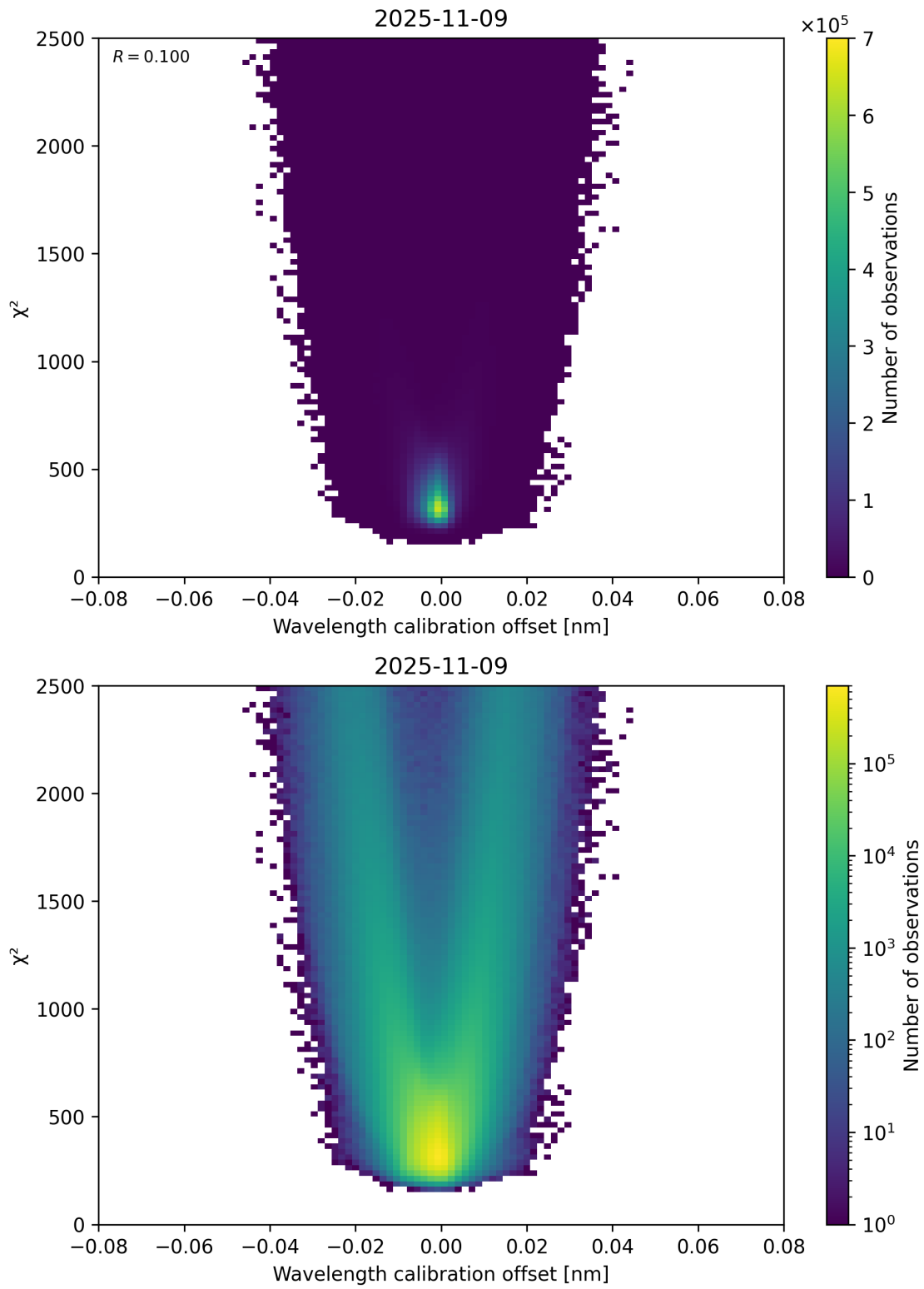
Figure 175: Scatter density plot of “Wavelength calibration offset” against “ \chi^2 ” for 2025-11-08 to 2025-11-10.
