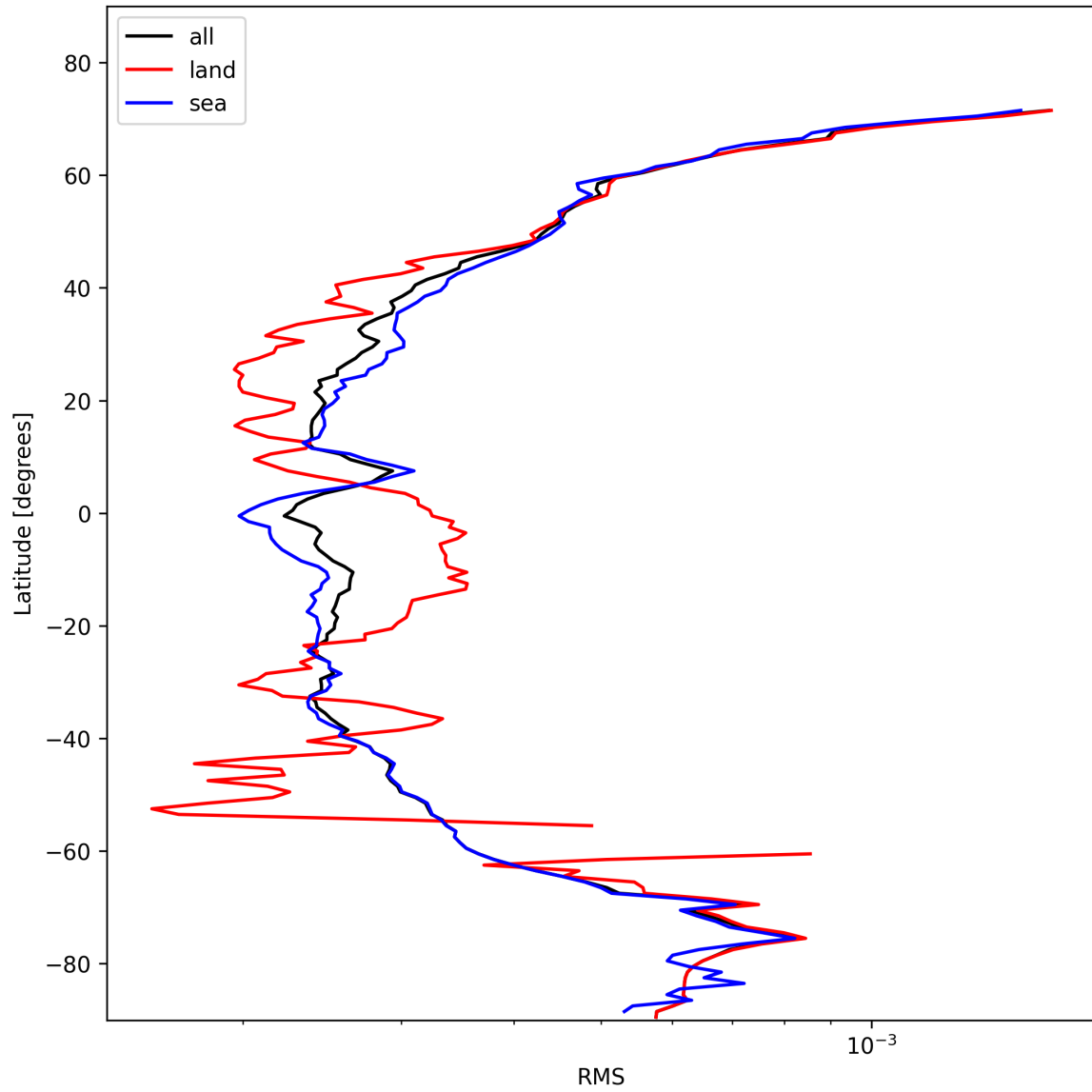
Figure 26: Zonal average of “RMS” for 2025-11-08 to 2025-11-10.
