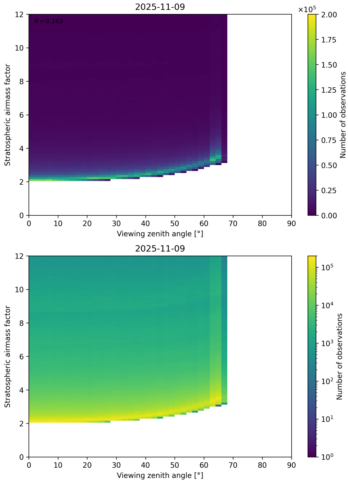
Figure 159: Scatter density plot of “Viewing zenith angle” against “Stratospheric airmass factor” for 2025-11-08 to 2025-11-10.
