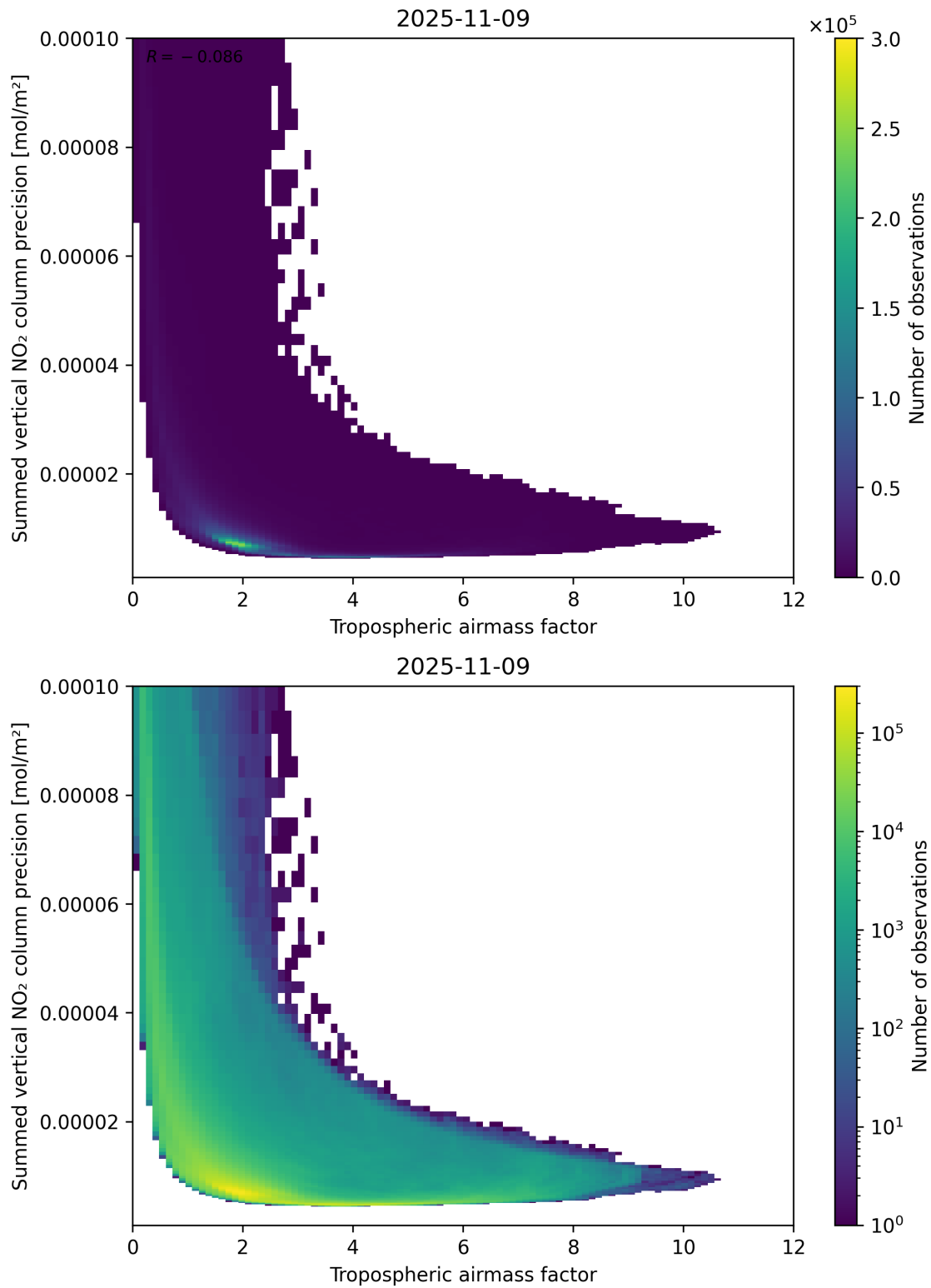
Figure 76: Scatter density plot of “Tropospheric air mass factor” against “Summed vertical NO 2 column precision” for 2025-11-08 to 2025-11-10.
