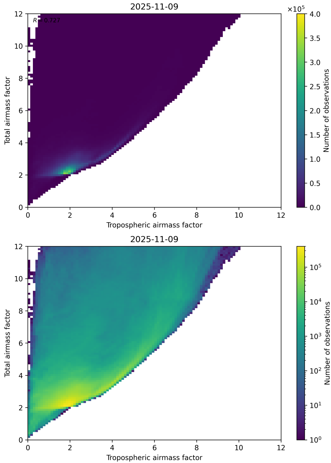
Figure 72: Scatter density plot of “Tropospheric airmass factor” against “Total airmass factor” for 2025-11-08 to 2025-11-10.
