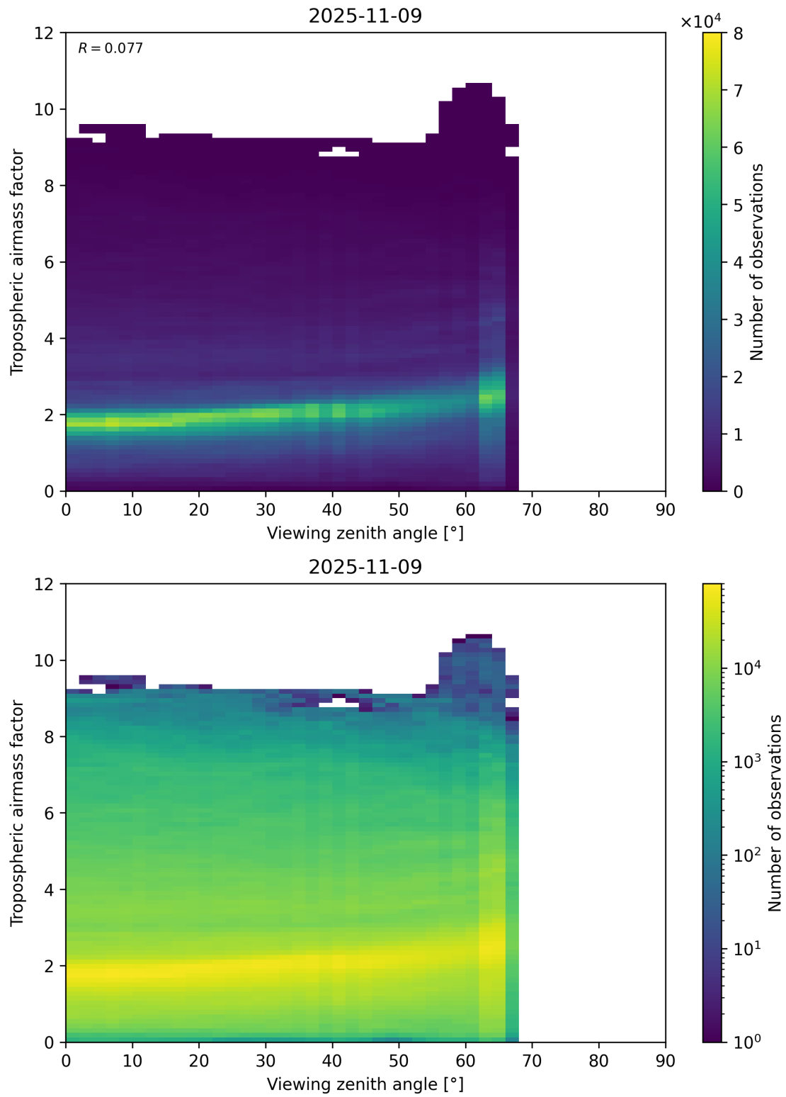
Figure 161: Scatter density plot of “Viewing zenith angle” against “Tropospheric airmass factor” for 2025-11-08 to 2025-11-10.
