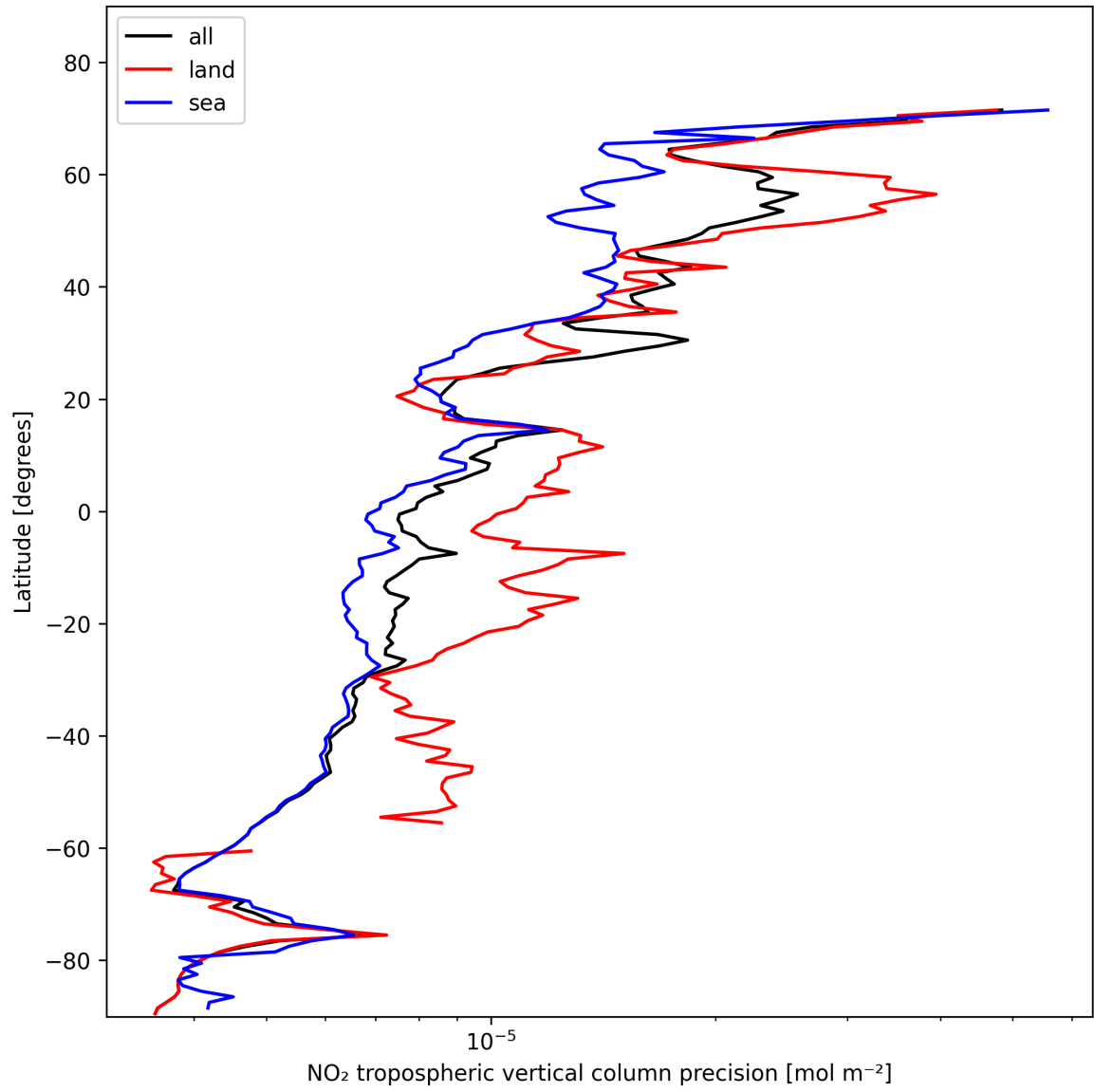
Figure 13: Zonal average of “NO 2 tropospheric vertical column precision” for 2025-11-08 to 2025-11-10.
