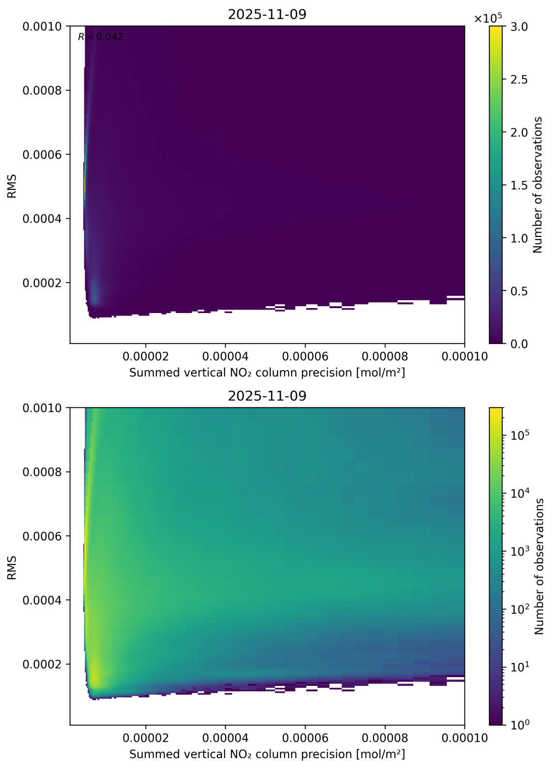
Figure 108: Scatter density plot of “Summed vertical NO 2 column precision” against “RMS” for 2025-11-08 to 2025-11-10.
