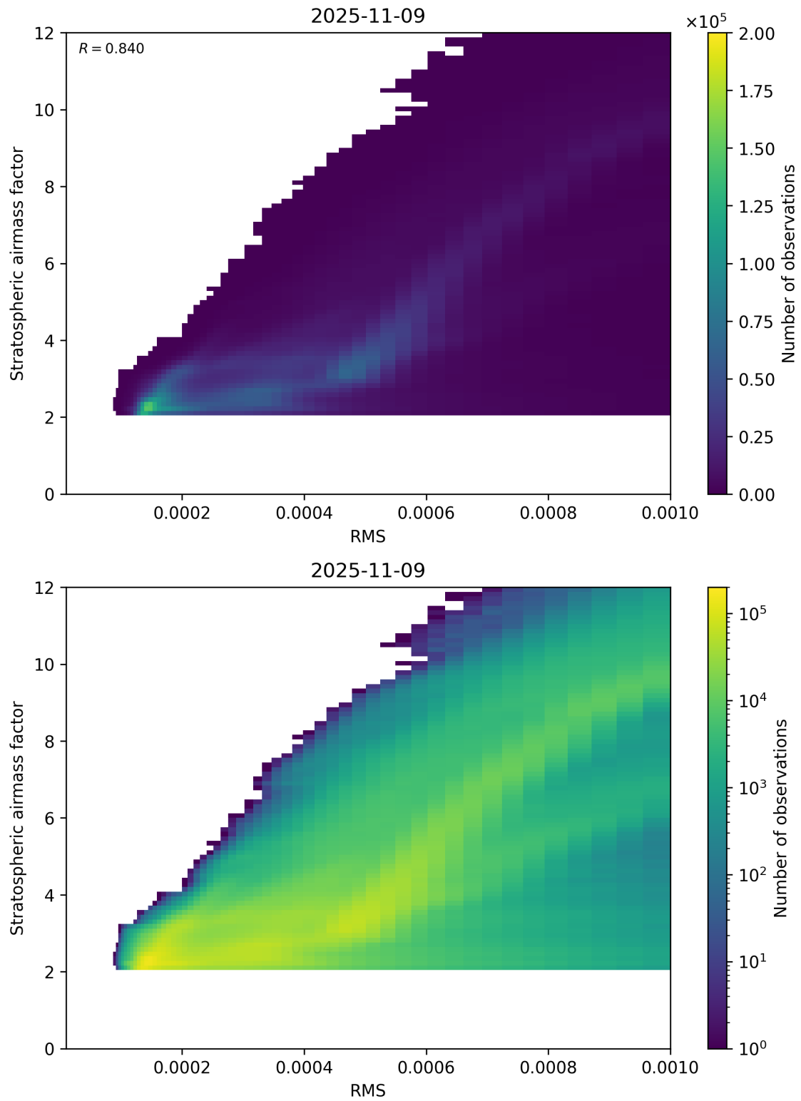
Figure 144: Scatter density plot of “RMS” against “Stratospheric airmass factor” for 2025-11-08 to 2025-11-10.
