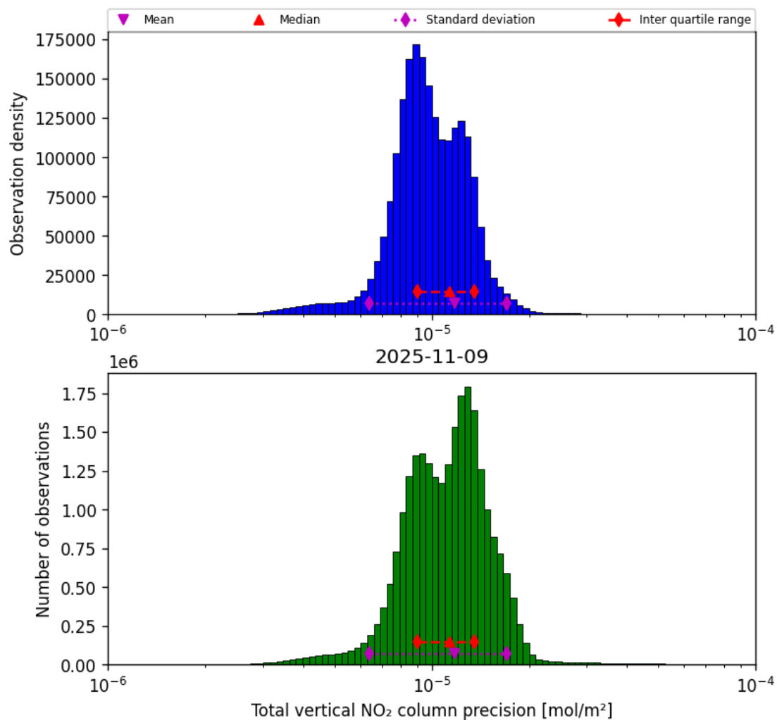
Figure 39: Histogram of “Total vertical NO 2 column precision” for 2025-11-08 to 2025-11-10
