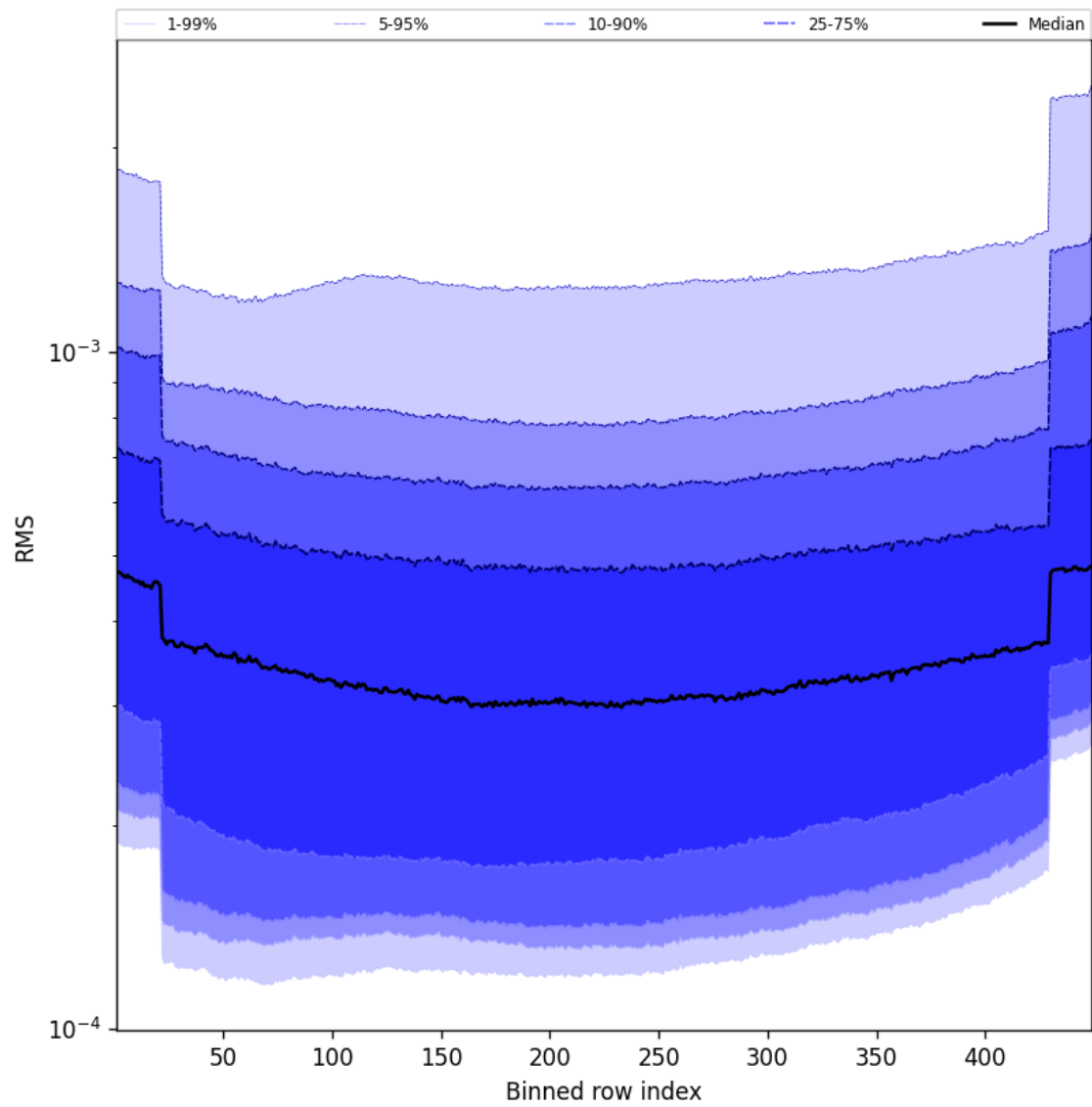
Figure 60: Along track statistics of “RMS” for 2025-11-08 to 2025-11-10
