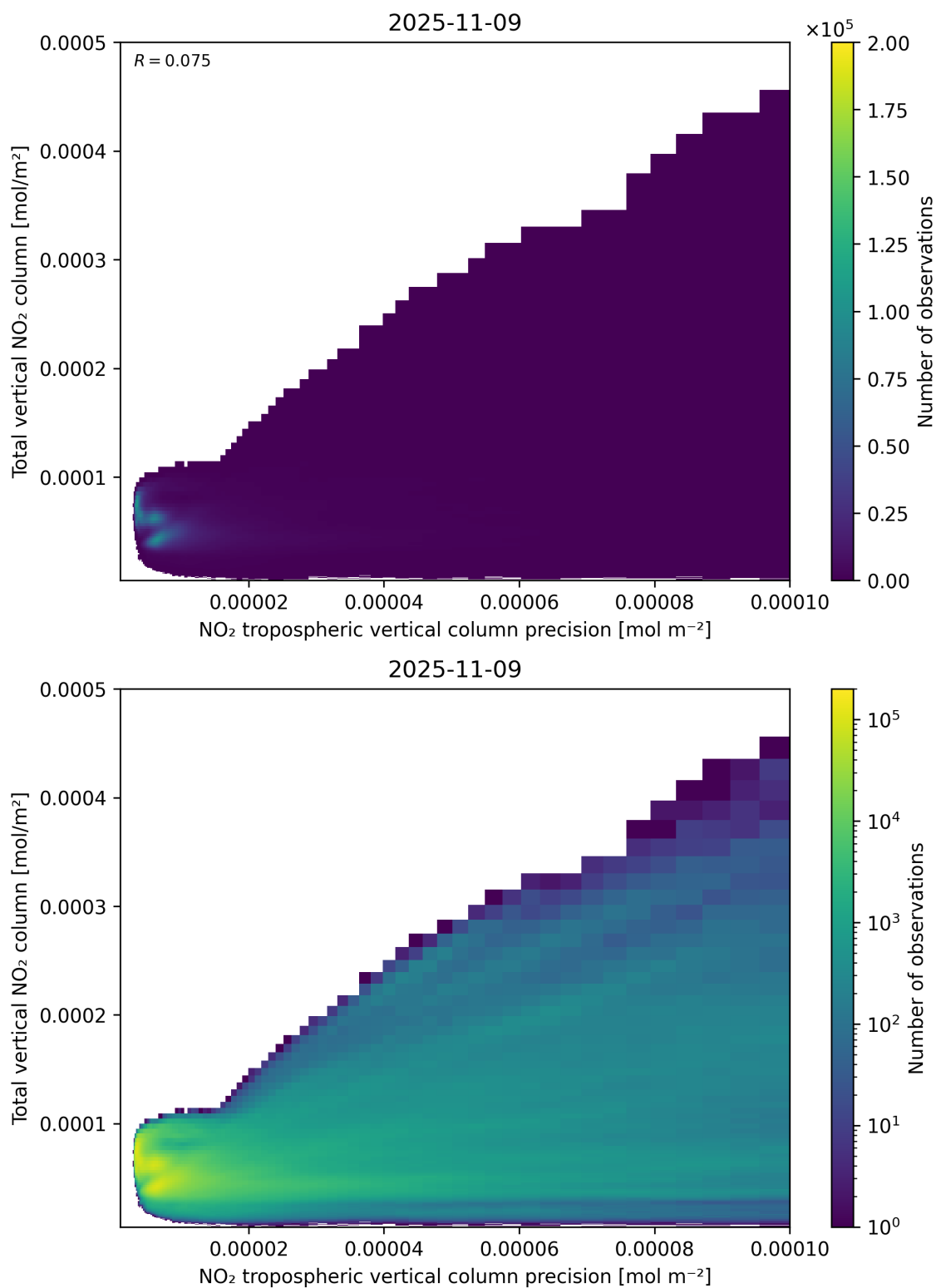
Figure 138: Scatter density plot of “NO 2 tropospheric vertical column precision” against “Total vertical NO 2 column” for 2025-11-08 to 2025-11-10.
