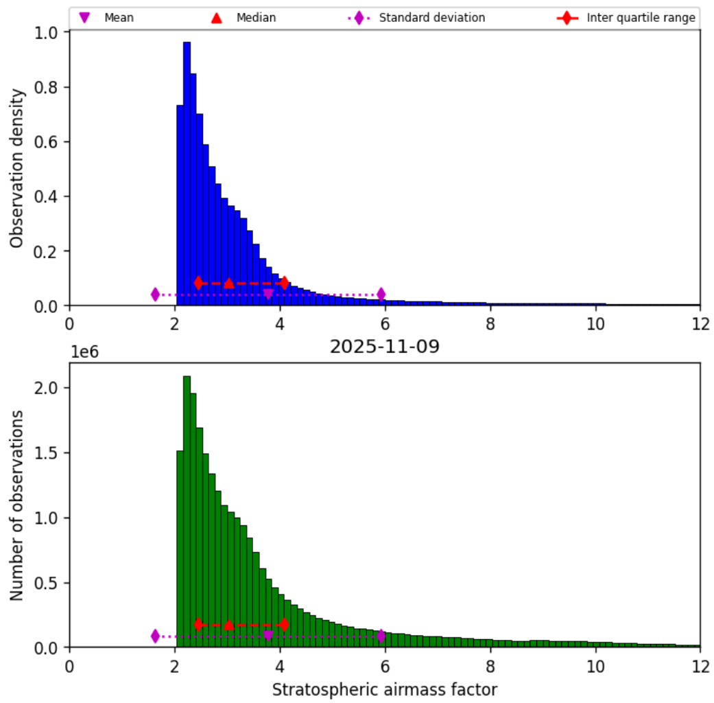
Figure 44: Histogram of “Stratospheric airmass factor” for 2025-11-08 to 2025-11-10
