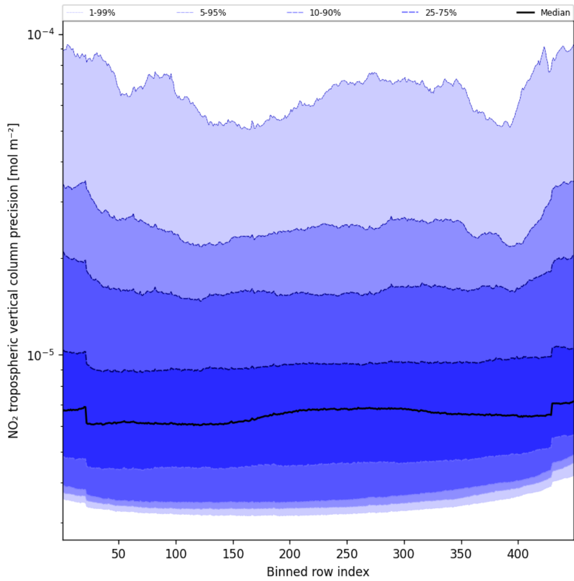
Figure 47: Along track statistics of “NO 2 tropospheric vertical column precision” for 2025-11-08 to 2025-11-10
