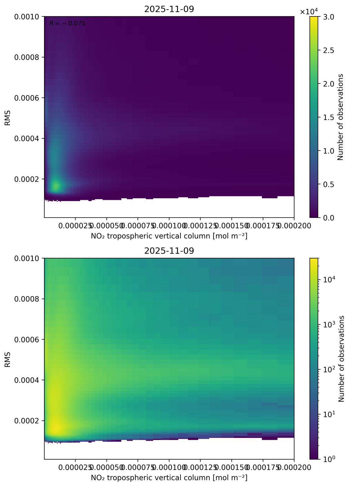
Figure 142: Scatter density plot of “NO 2 tropospheric vertical column” against “RMS” for 2025-11-08 to 2025-11-10.
