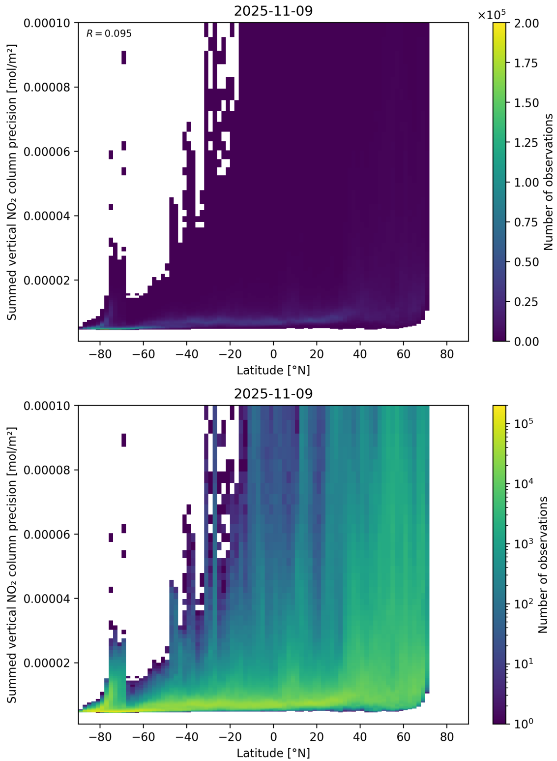
Figure 89: Scatter density plot of “Latitude” against “Summed vertical NO 2 column precision” for 2025-11-08 to 2025-11-10.
