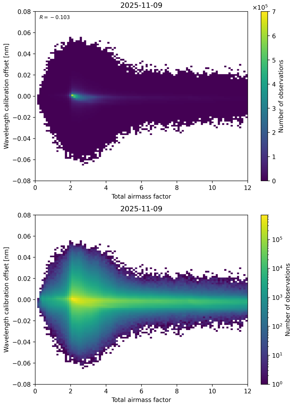
Figure 70: Scatter density plot of “Total airmass factor” against “Wavelength calibration offset” for 2025-11-08 to 2025-11-10.
