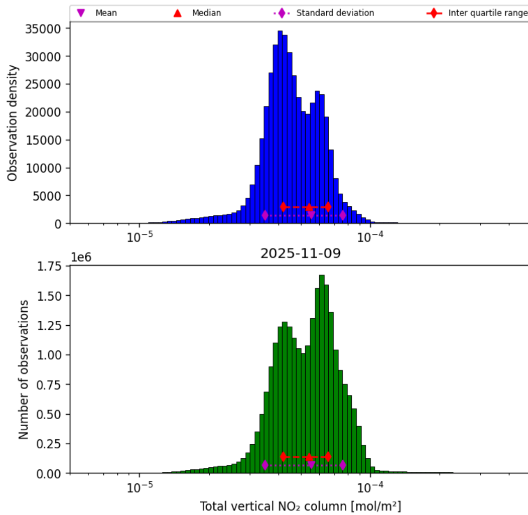
Figure 38: Histogram of “Total vertical NO 2 column” for 2025-11-08 to 2025-11-10
