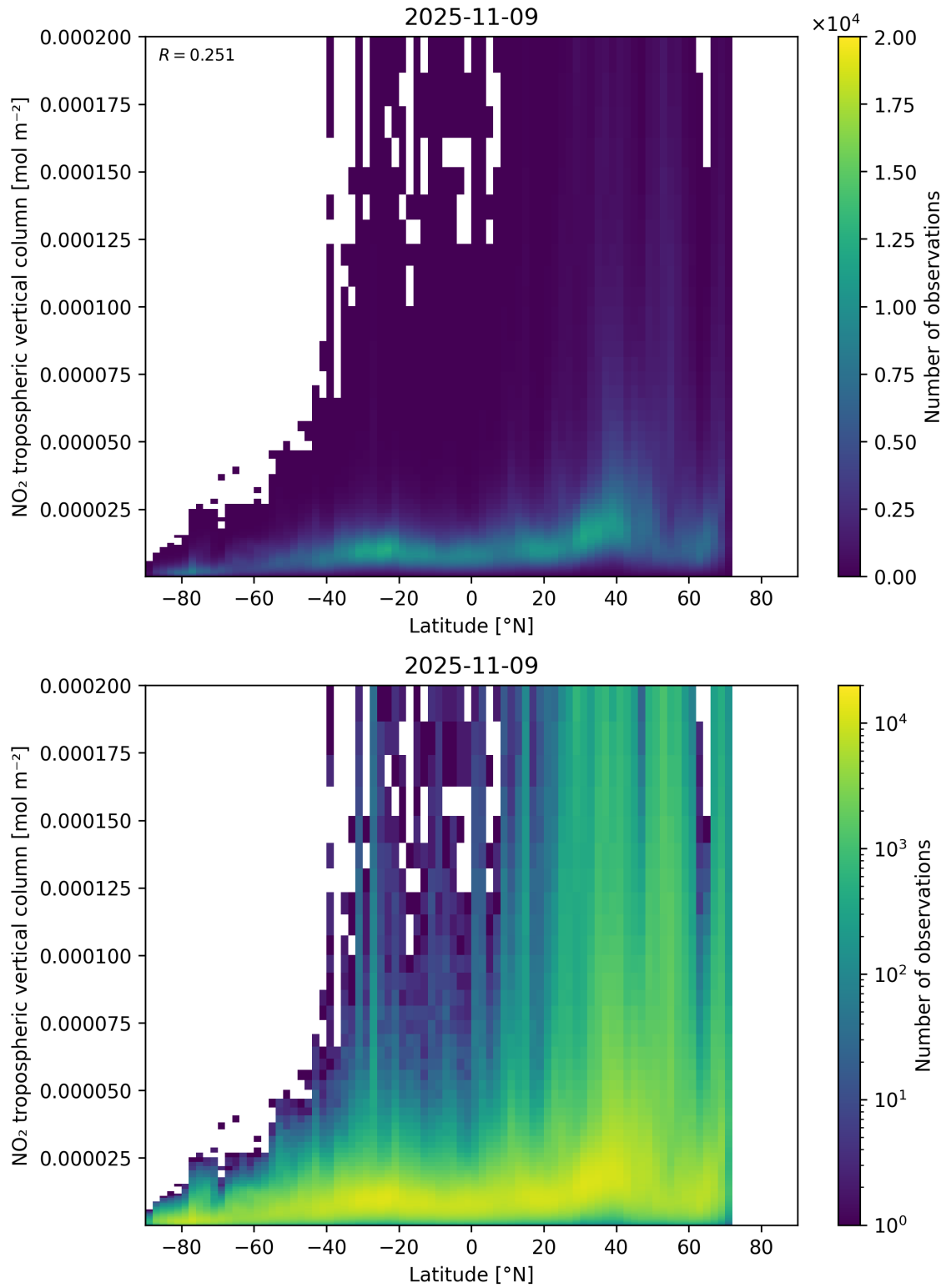
Figure 92: Scatter density plot of “Latitude” against “NO 2 tropospheric vertical column” for 2025-11-08 to 2025-11-10.
