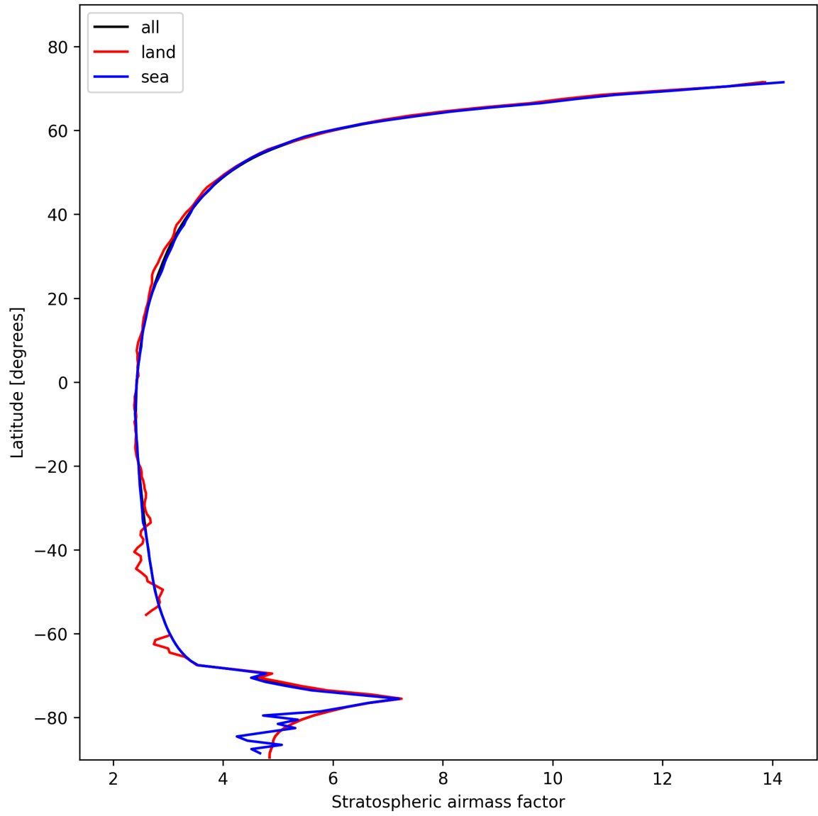
Figure 27: Zonal average of “Stratospheric airmass factor” for 2025-11-08 to 2025-11-10.
