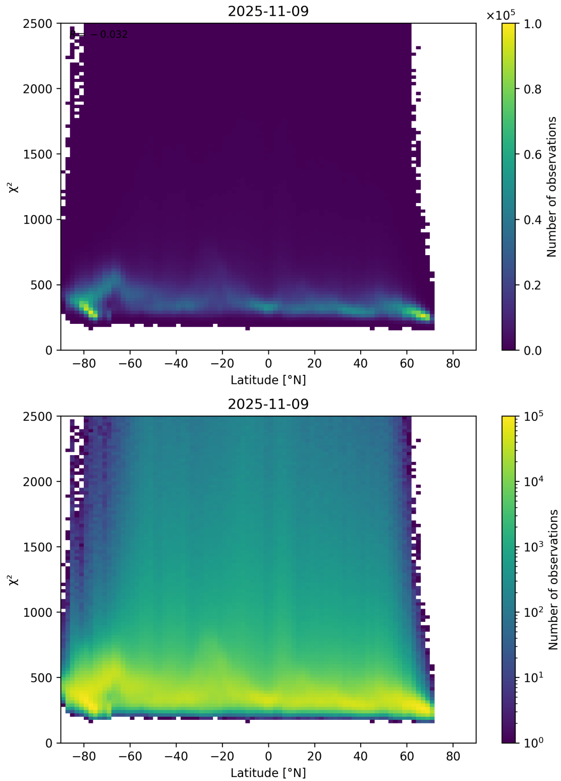
Figure 86: Scatter density plot of “Latitude” against “ \chi^2 ” for 2025-11-08 to 2025-11-10.
