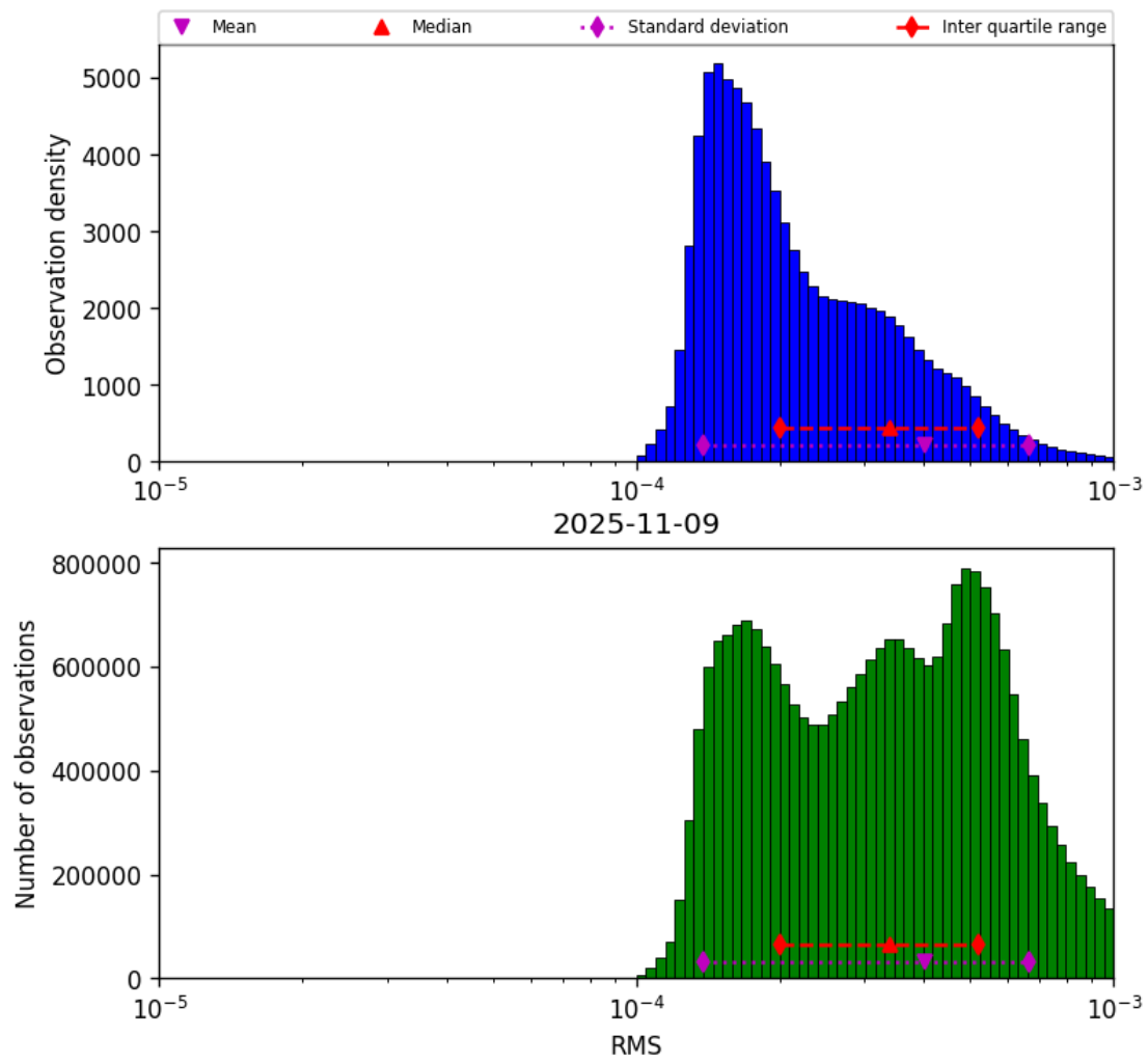
Figure 43: Histogram of “RMS” for 2025-11-08 to 2025-11-10
