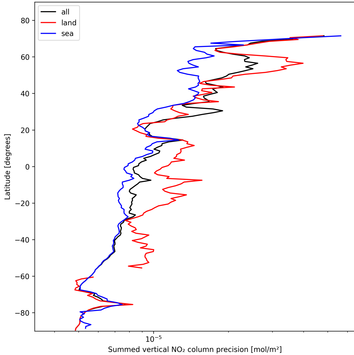
Figure 24: Zonal average of “Summed vertical NO 2 column precision” for 2025-11-08 to 2025-11-10.
