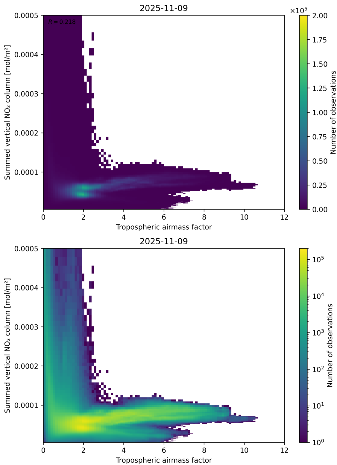
Figure 75: Scatter density plot of “Tropospheric airmass factor” against “Summed vertical NO 2 column” for 2025-11-08 to 2025-11-10.
