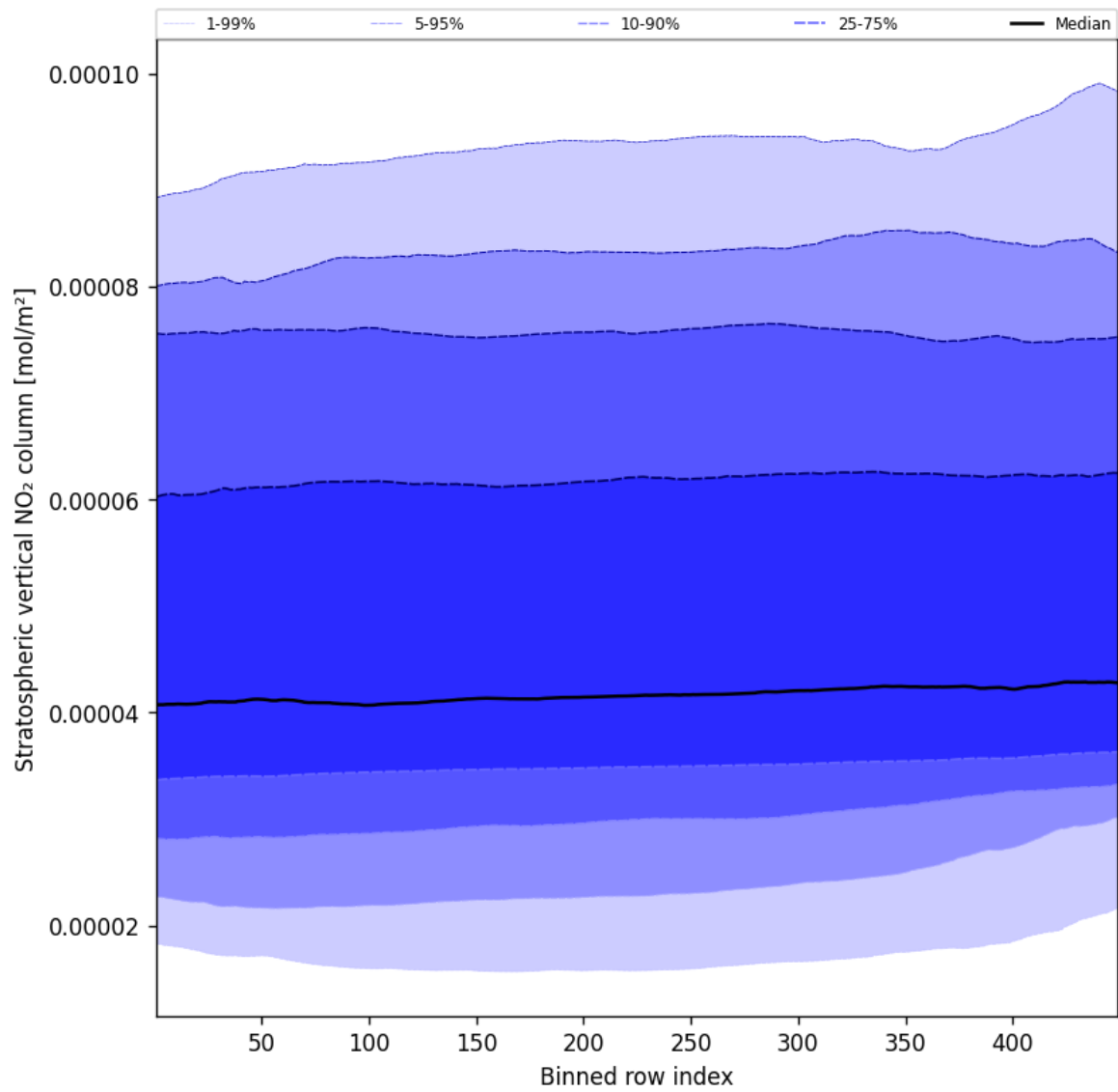
Figure 53: Along track statistics of “Stratospheric vertical NO 2 column” for 2025-11-08 to 2025-11-10
