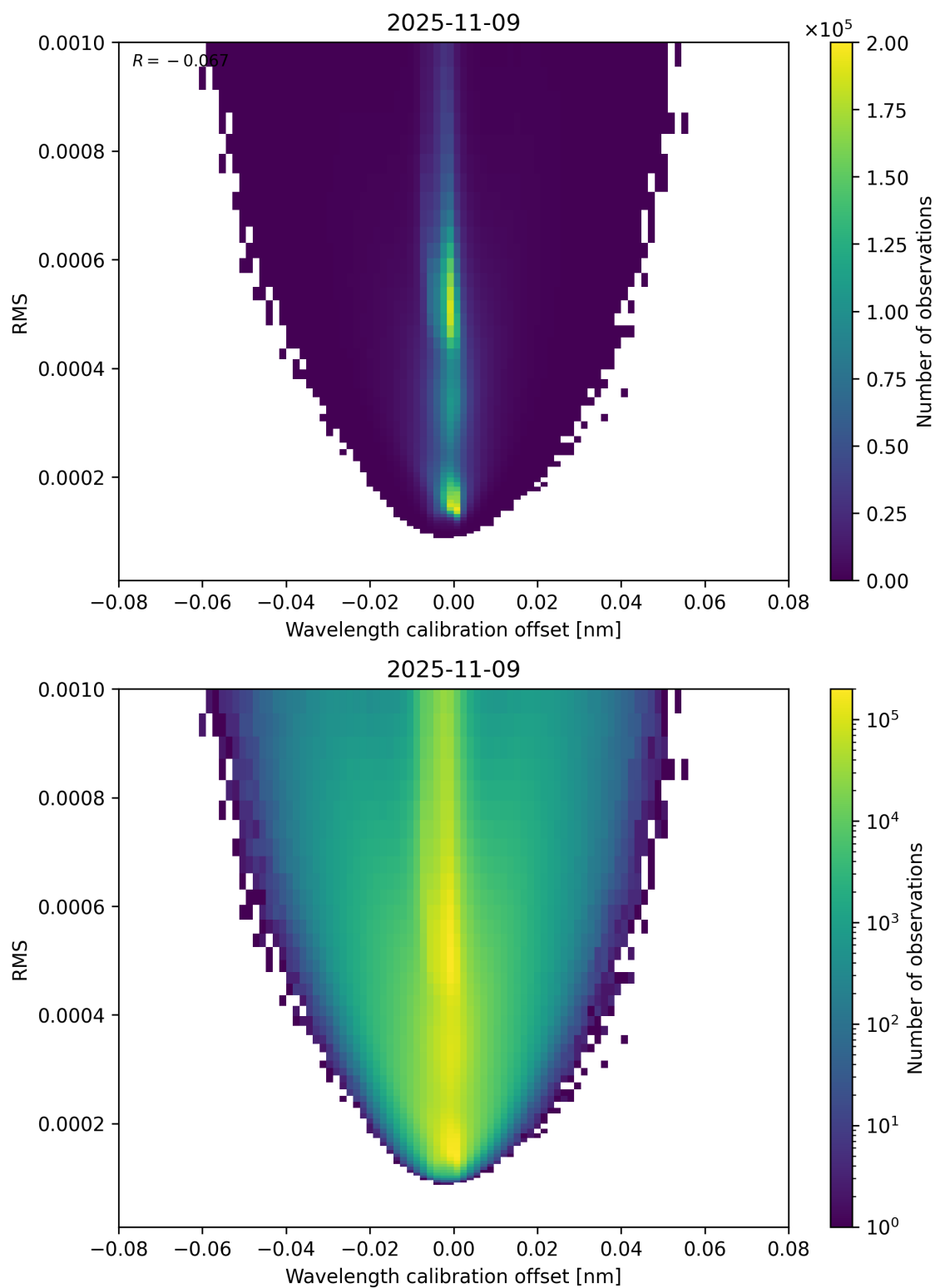
Figure 181: Scatter density plot of “Wavelength calibration offset” against “RMS” for 2025-11-08 to 2025-11-10.
