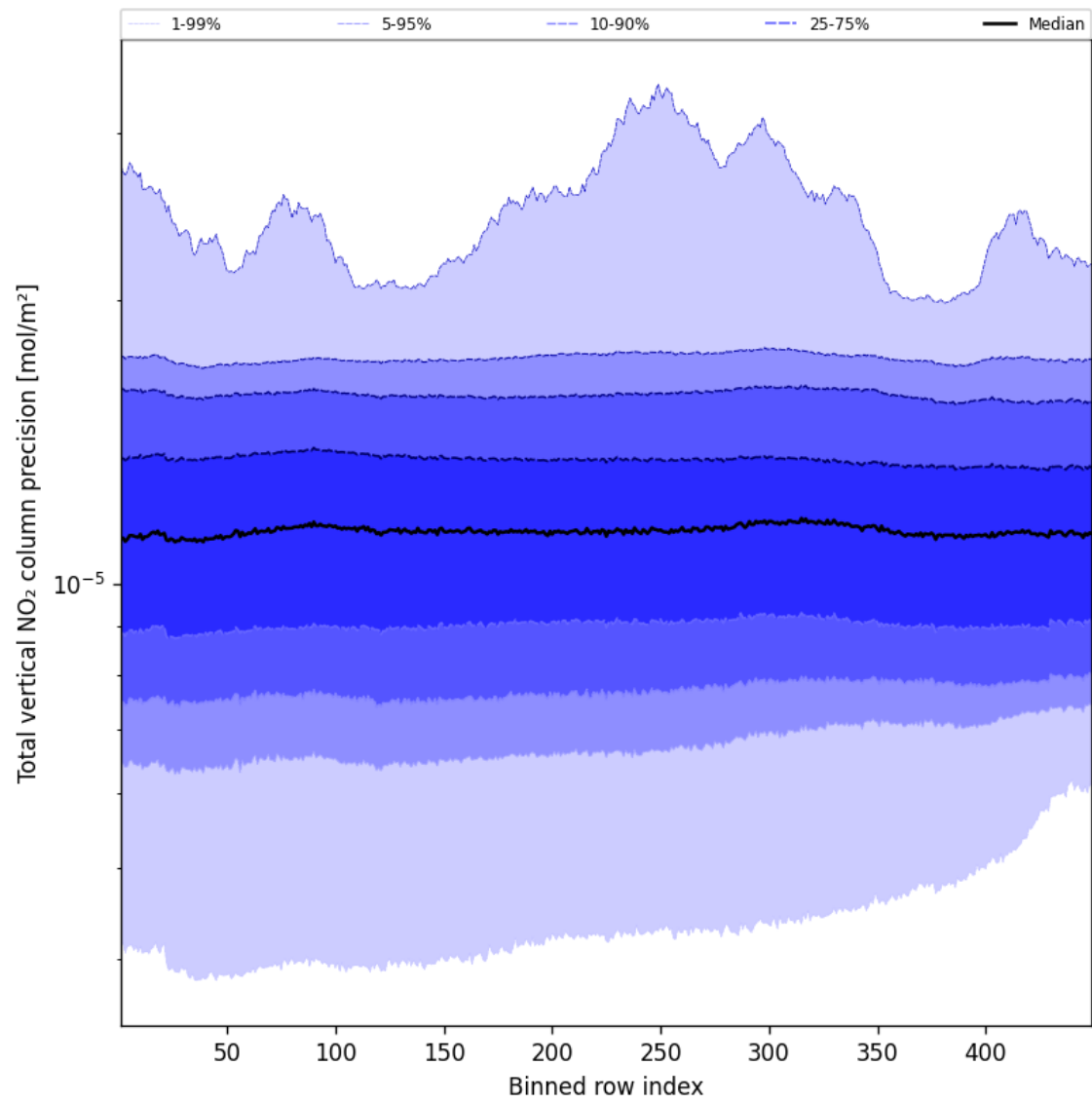
Figure 56: Along track statistics of “Total vertical NO 2 column precision” for 2025-11-08 to 2025-11-10
