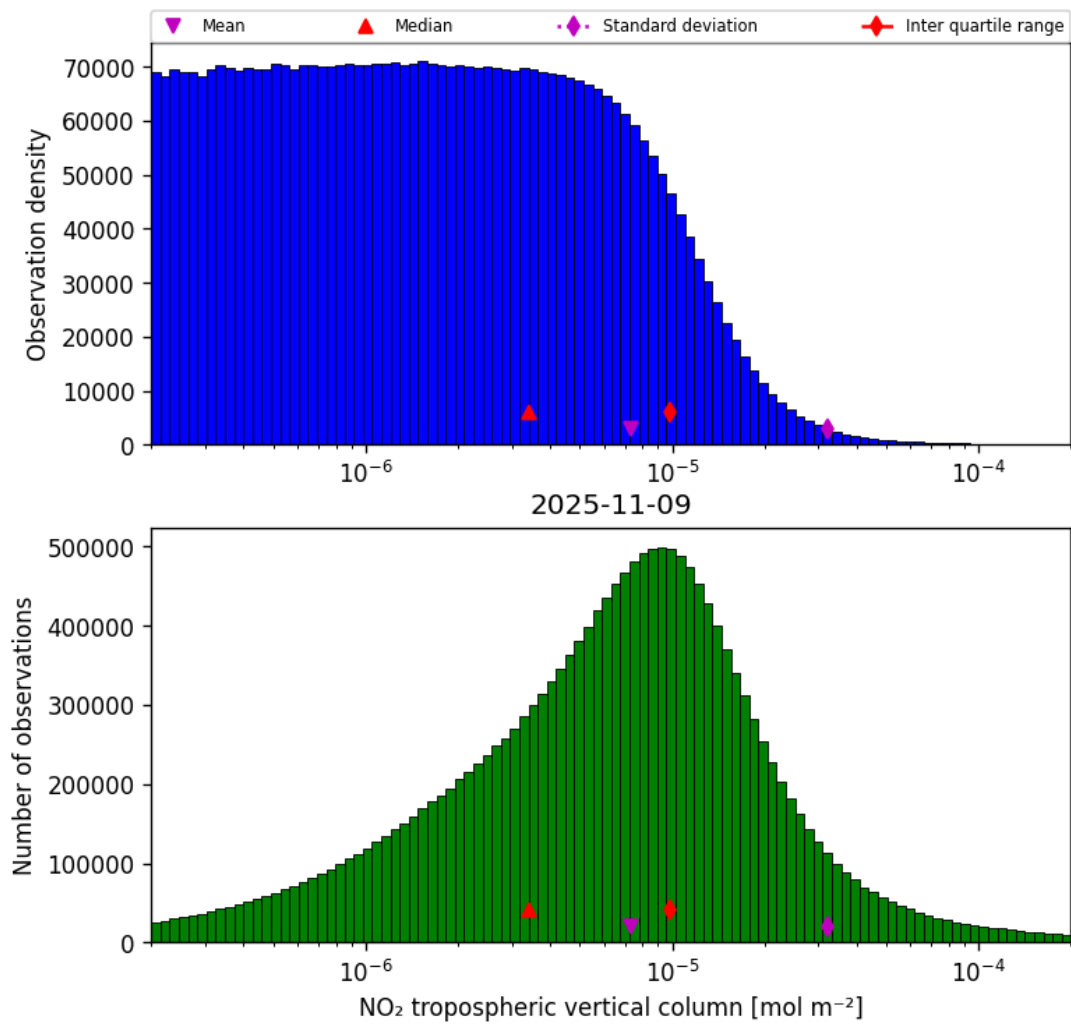
Figure 29: Histogram of “NO 2 tropospheric vertical column” for 2025-11-08 to 2025-11-10
