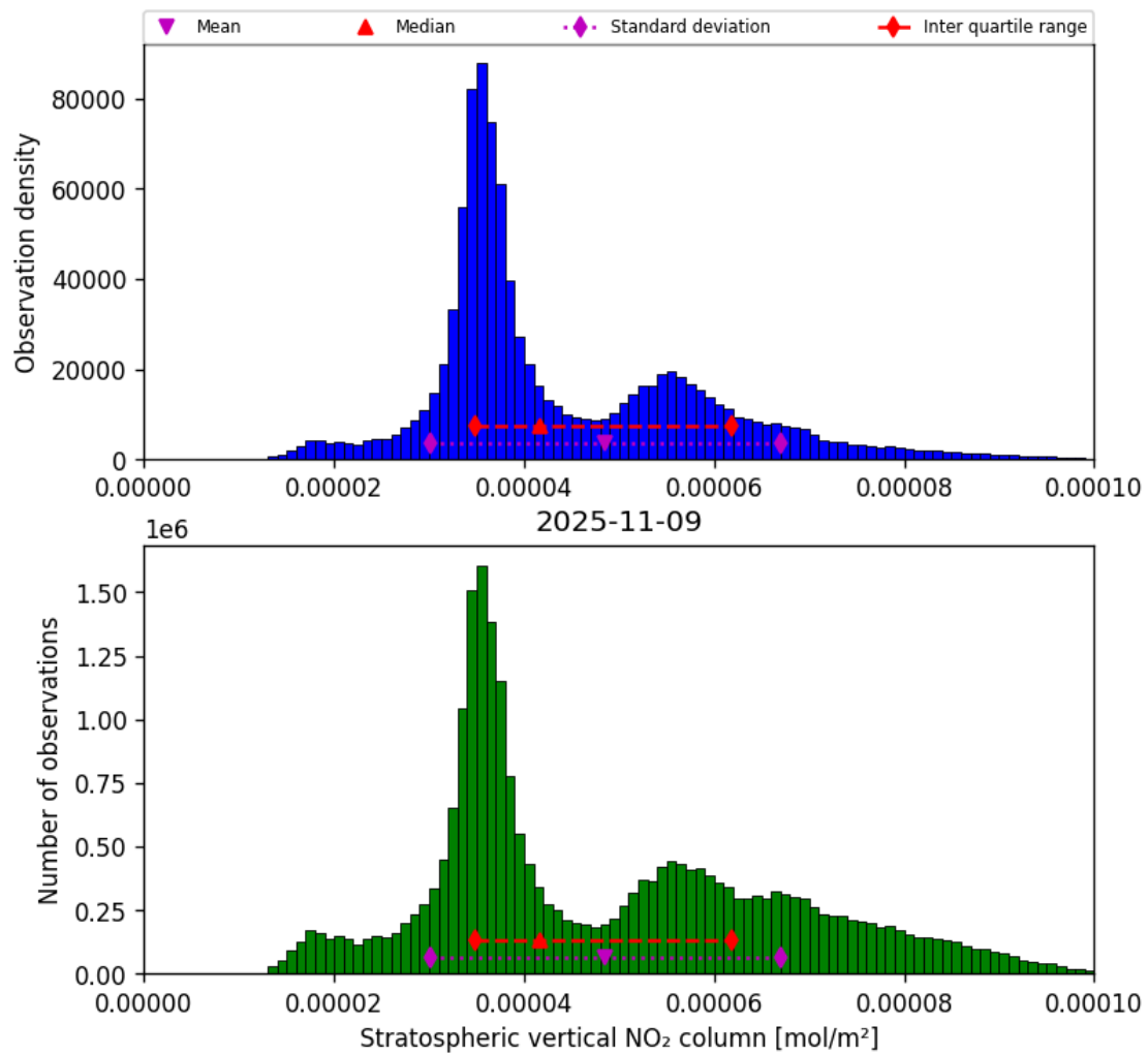
Figure 36: Histogram of “Stratospheric vertical NO 2 column” for 2025-11-08 to 2025-11-10
