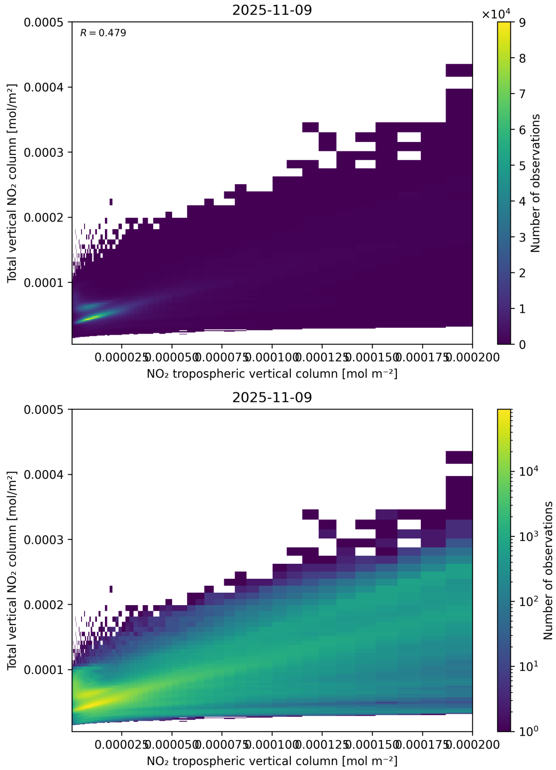
Figure 128: Scatter density plot of “NO 2 tropospheric vertical column” against “Total vertical NO 2 column” for 2025-11-08 to 2025-11-10.
