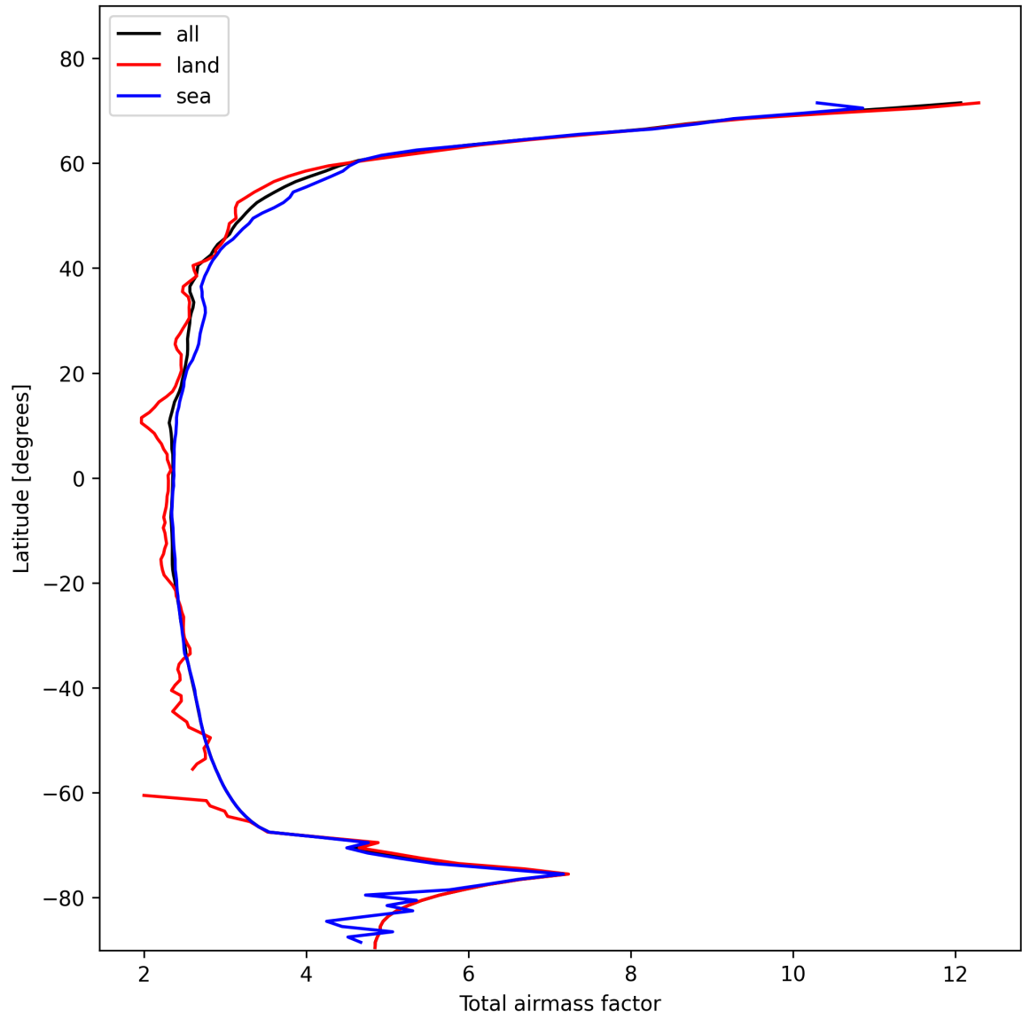
Figure 15: Zonal average of “Total airmass factor” for 2025-11-08 to 2025-11-10.
