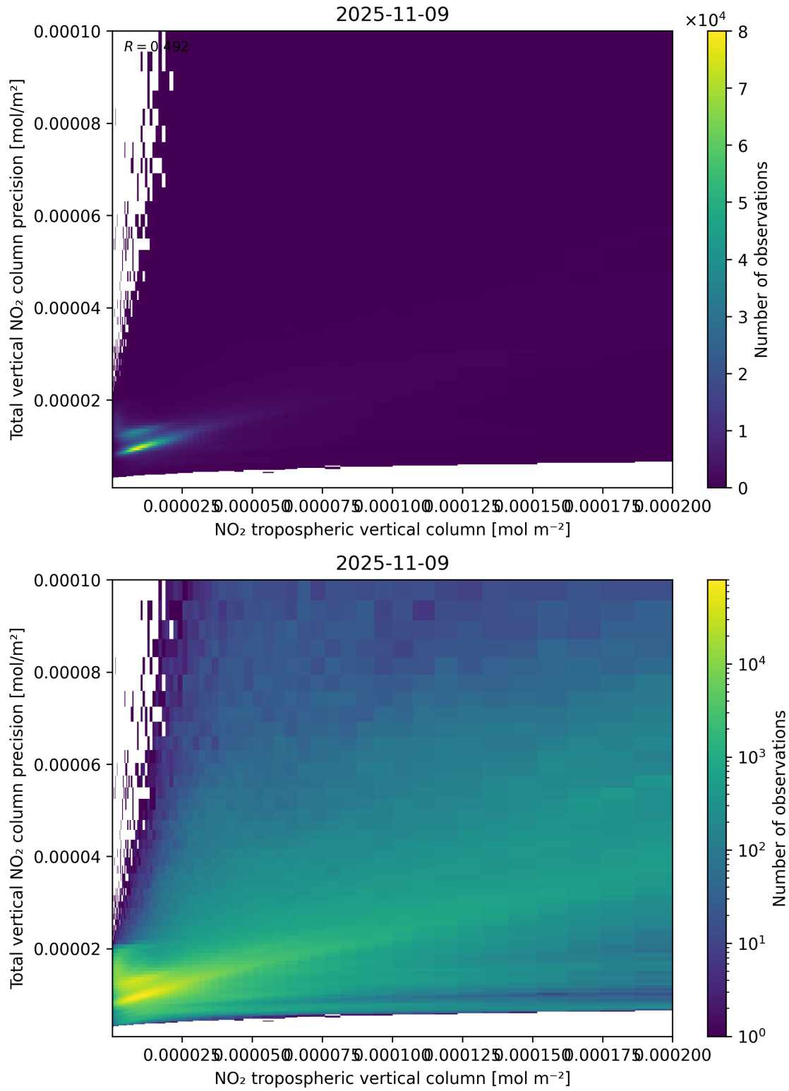
Figure 129: Scatter density plot of “NO 2 tropospheric vertical column” against “Total vertical NO 2 column precision” for 2025-11-08 to 2025-11-10.
