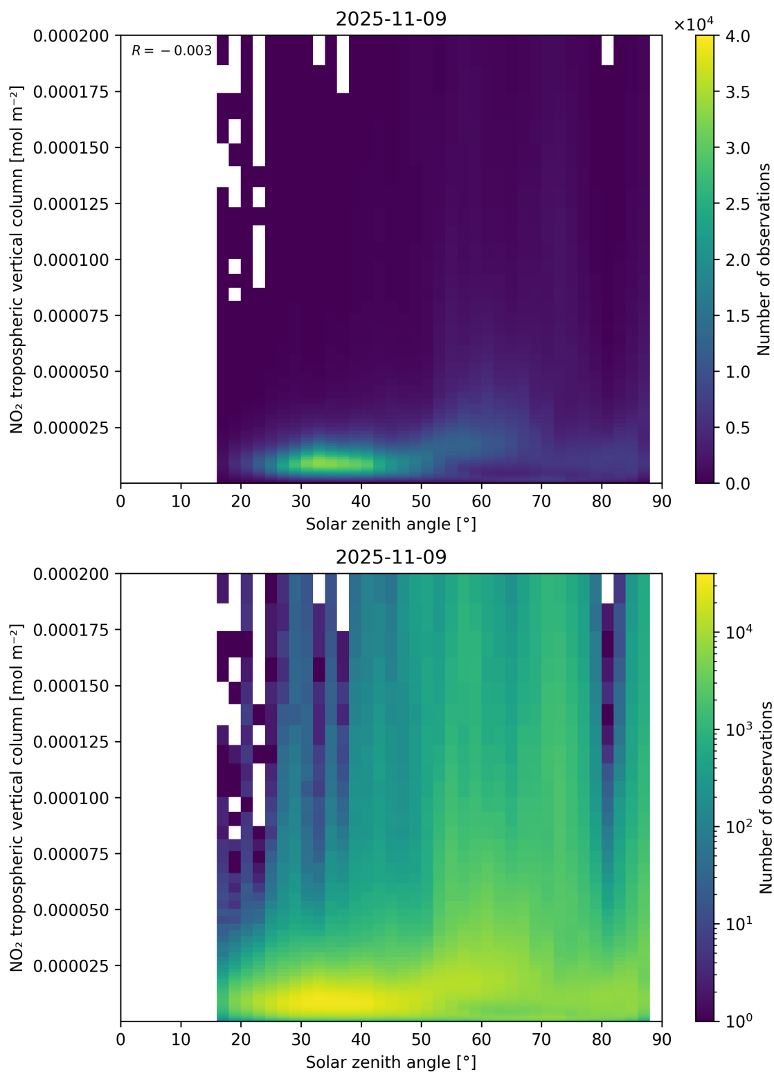
Figure 155: Scatter density plot of “Solar zenith angle” against “NO 2 tropospheric vertical column” for 2025-11-08 to 2025-11-10.
