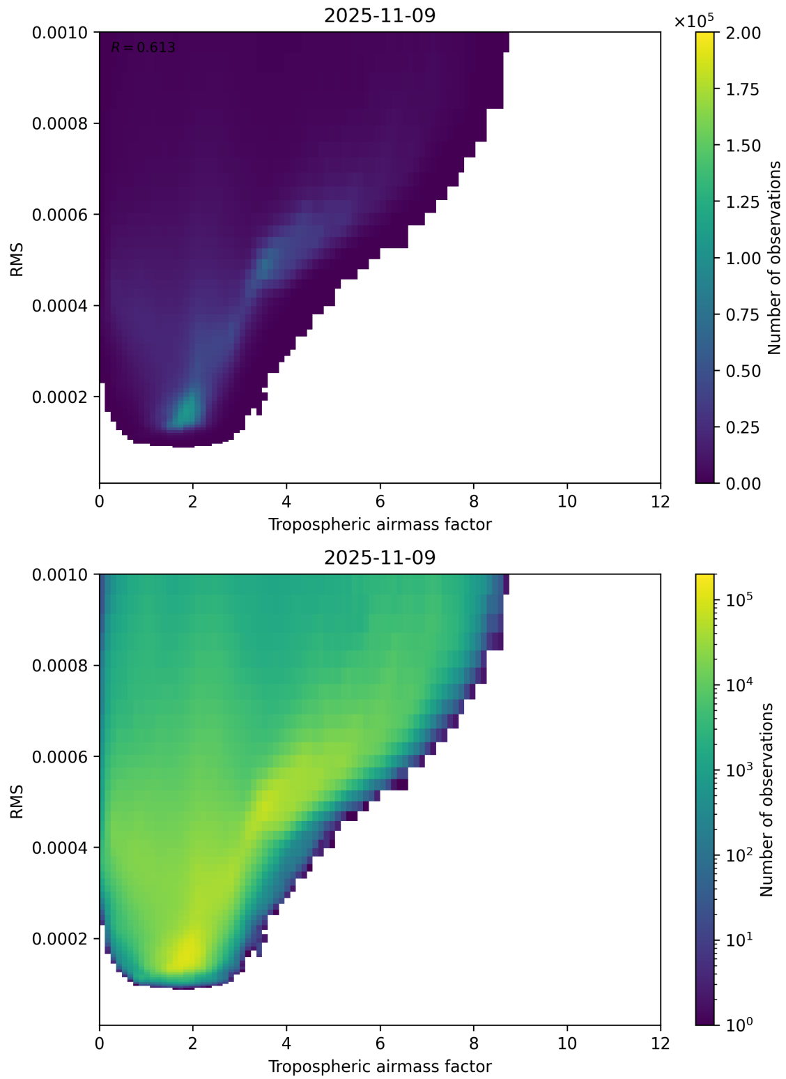
Figure 79: Scatter density plot of “Tropospheric airmass factor” against “RMS” for 2025-11-08 to 2025-11-10.
