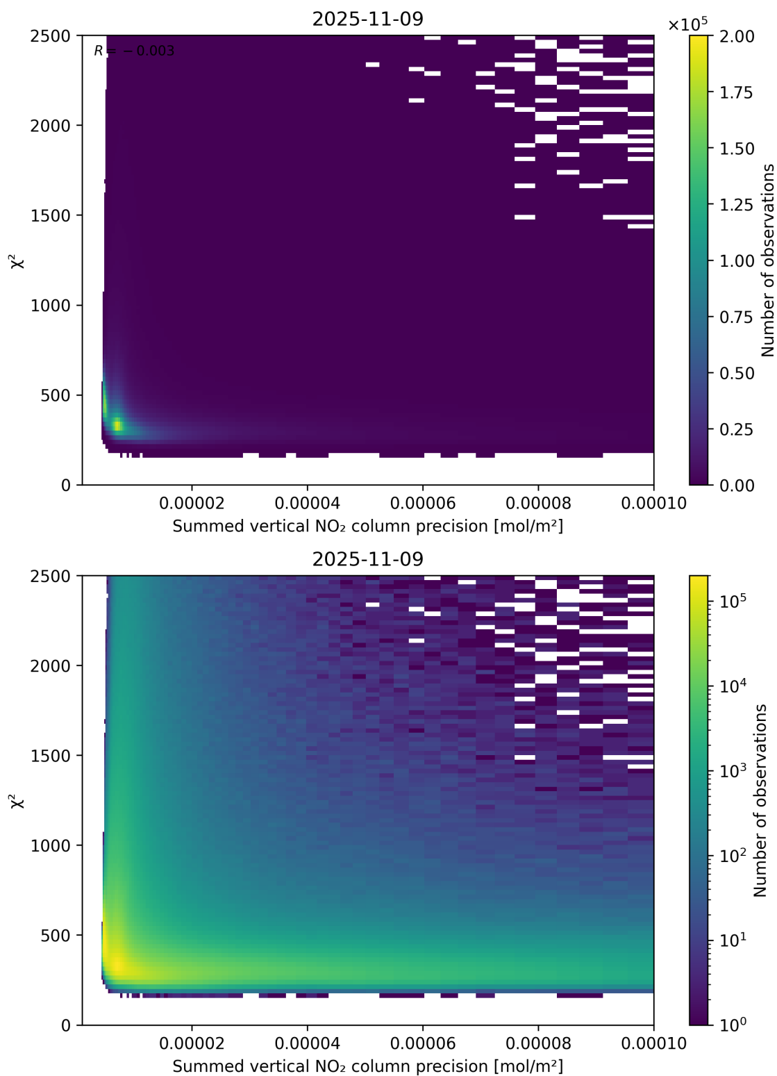
Figure 107: Scatter density plot of “Summed vertical NO 2 column precision” against “ \chi^2 ” for 2025-11-08 to 2025-11-10.
