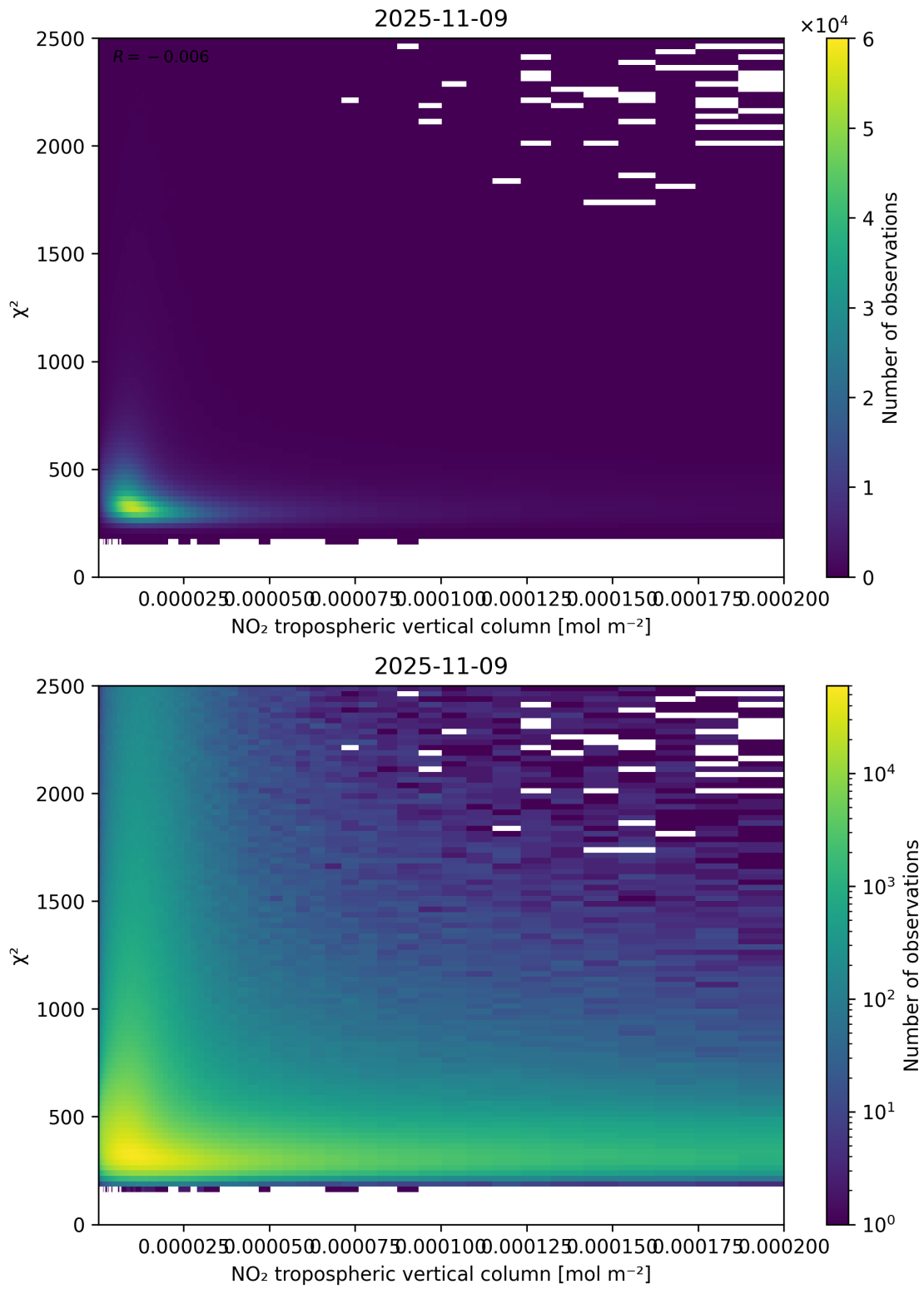
Figure 124: Scatter density plot of “NO 2 tropospheric vertical column” against “ \chi^2 ” for 2025-11-08 to 2025-11-10.
