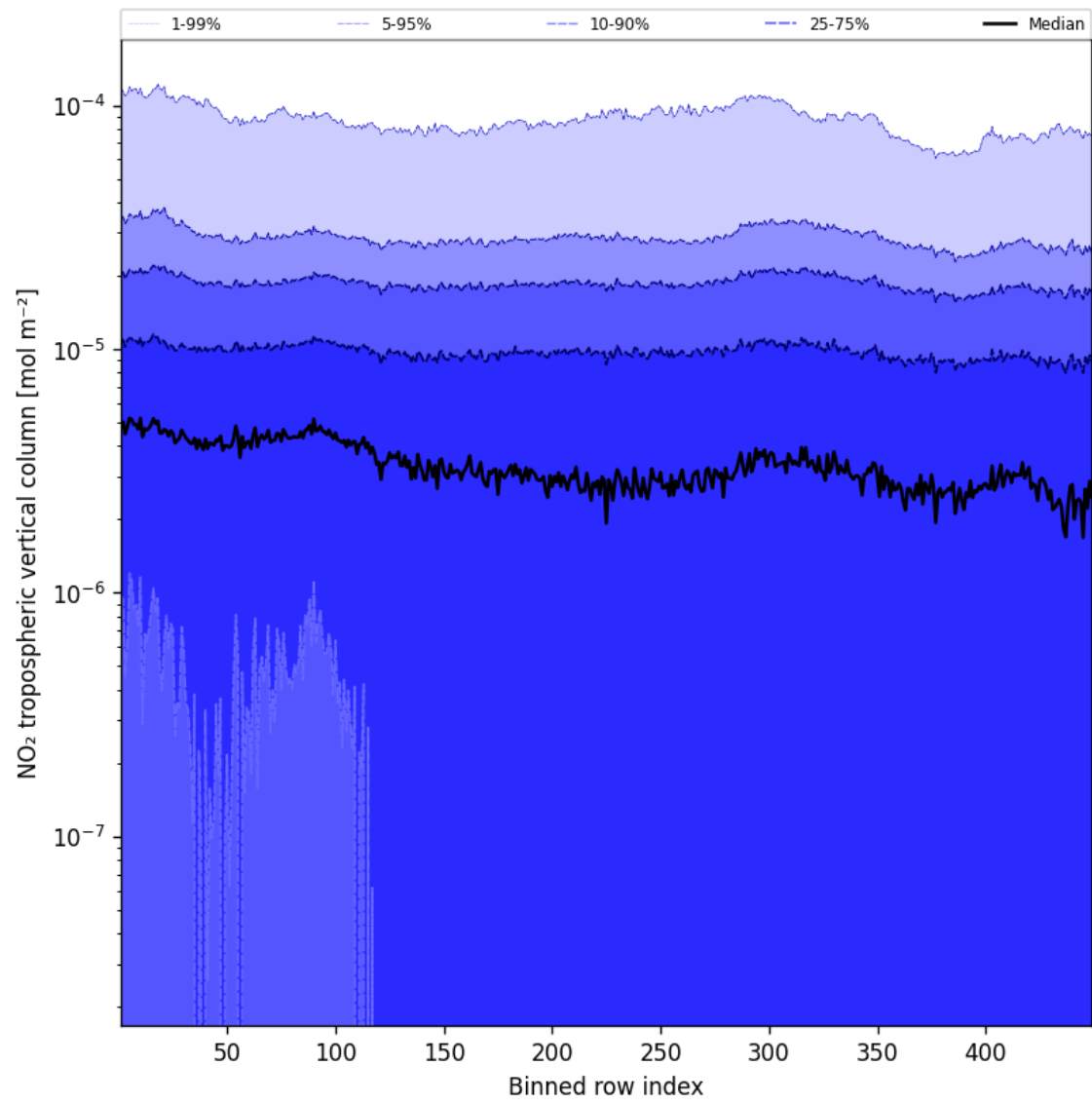
Figure 46: Along track statistics of “NO 2 tropospheric vertical column” for 2025-11-08 to 2025-11-10
