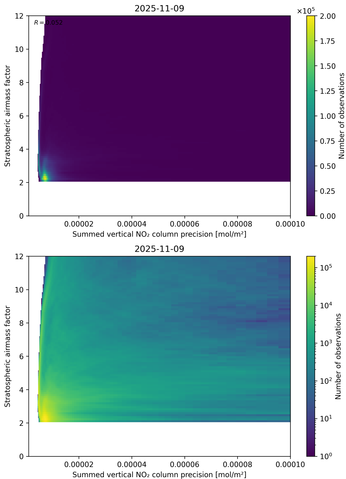
Figure 106: Scatter density plot of “Summed vertical NO 2 column precision” against “Stratospheric airmass factor” for 2025-11-08 to 2025-11-10.
