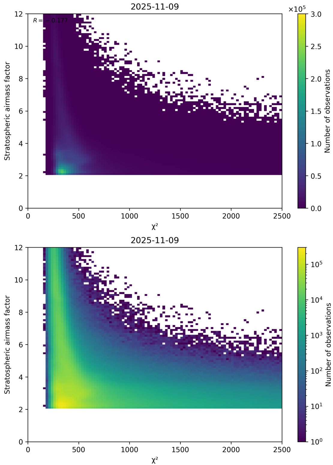
Figure 81: Scatter density plot of “ \chi^2 ” against “Stratospheric airmass factor” for 2025-11-08 to 2025-11-10.
