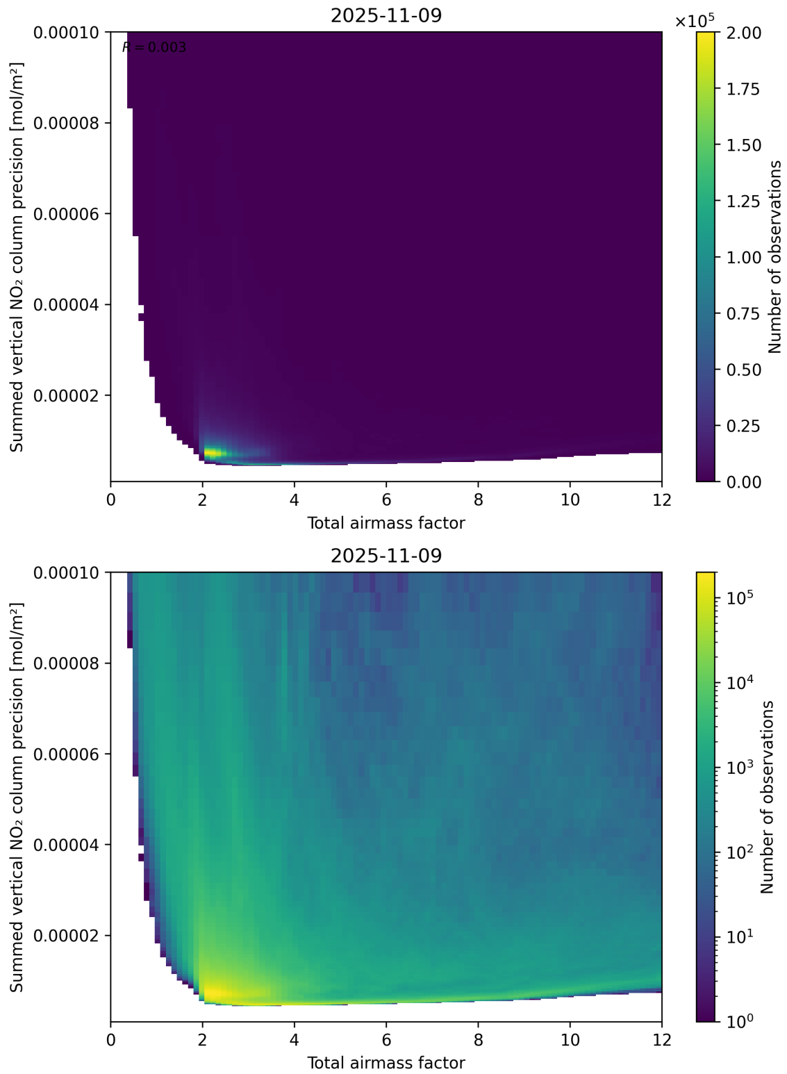
Figure 66: Scatter density plot of “Total airmass factor” against “Summed vertical NO 2 column precision” for 2025-11-08 to 2025-11-10.
