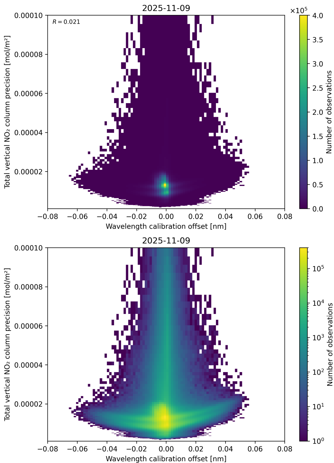
Figure 180: Scatter density plot of “Wavelength calibration offset” against “Total vertical NO 2 column precision” for 2025-11-08 to 2025-11-10.
