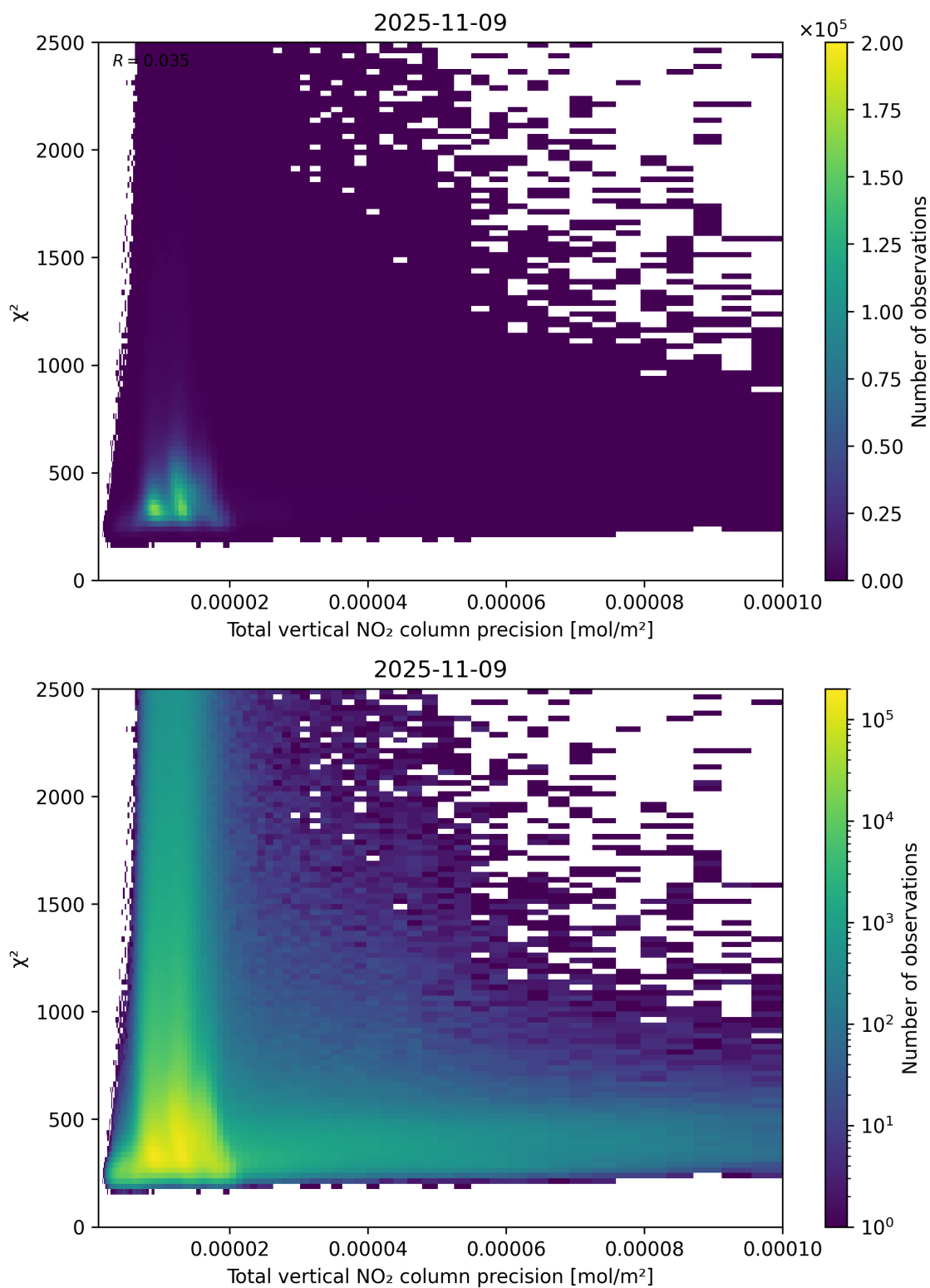
Figure 116: Scatter density plot of “Total vertical NO 2 column precision” against “ \chi^2 ” for 2025-11-08 to 2025-11-10.
