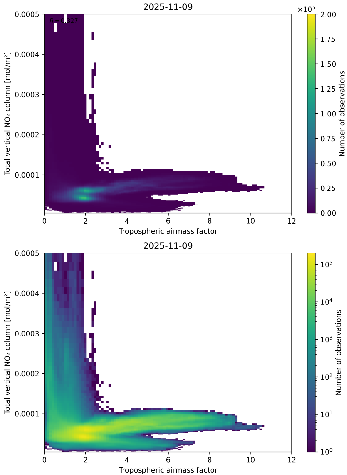
Figure 77: Scatter density plot of “Tropospheric airmass factor” against “Total vertical NO 2 column” for 2025-11-08 to 2025-11-10.
