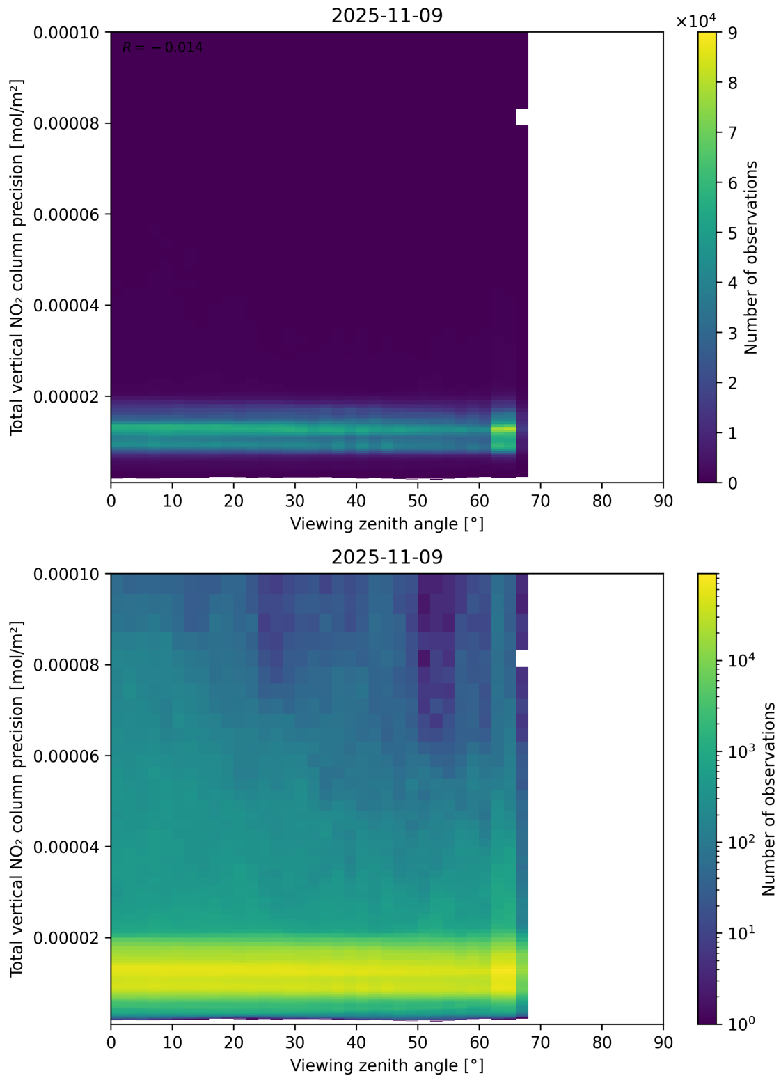
Figure 168: Scatter density plot of “Viewing zenith angle” against “Total vertical NO 2 column precision” for 2025-11-08 to 2025-11-10.
