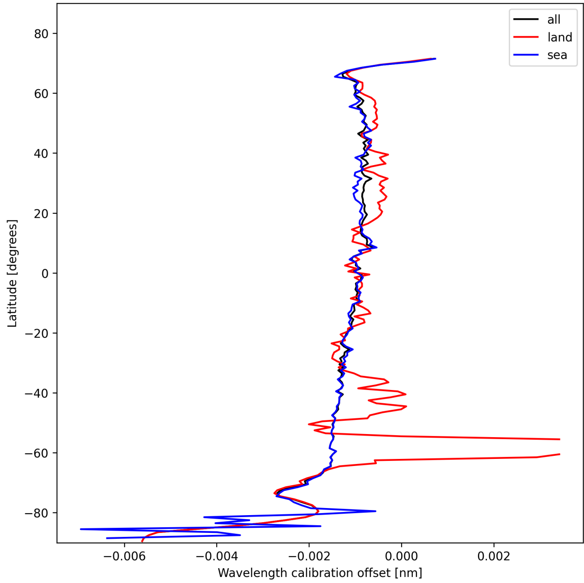
Figure 18: Zonal average of “Wavelength calibration offset” for 2025-11-08 to 2025-11-10.
