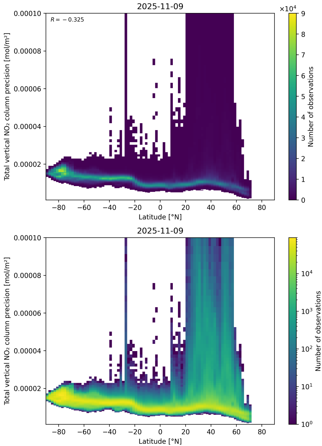
Figure 91: Scatter density plot of “Latitude” against “Total vertical NO 2 column precision” for 2025-11-08 to 2025-11-10.
