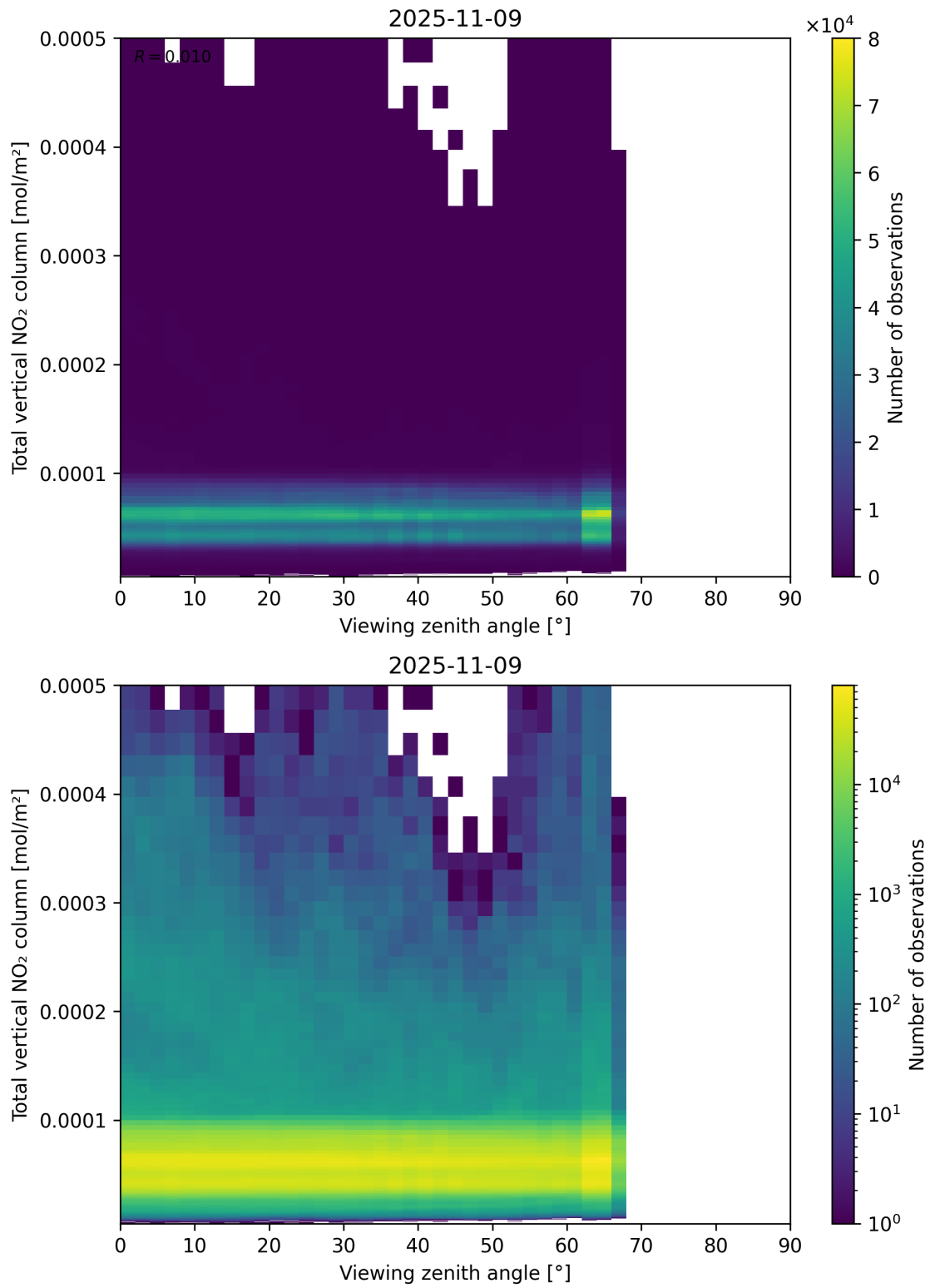
Figure 167: Scatter density plot of “Viewing zenith angle” against “Total vertical NO 2 column” for 2025-11-08 to 2025-11-10.
