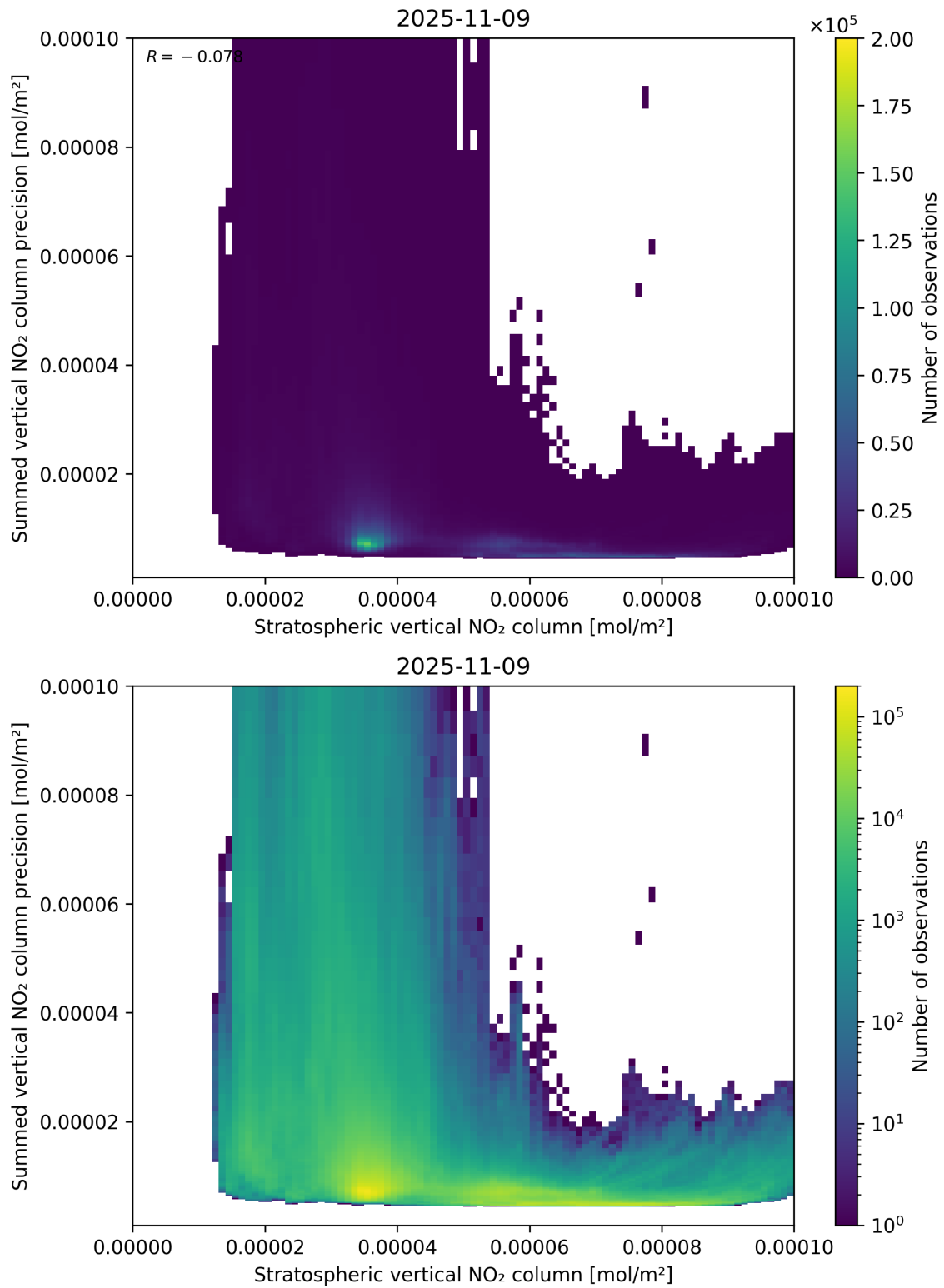
Figure 99: Scatter density plot of “Stratospheric vertical NO 2 column” against “Summed vertical NO 2 column precision” for 2025-11-08 to 2025-11-10.
