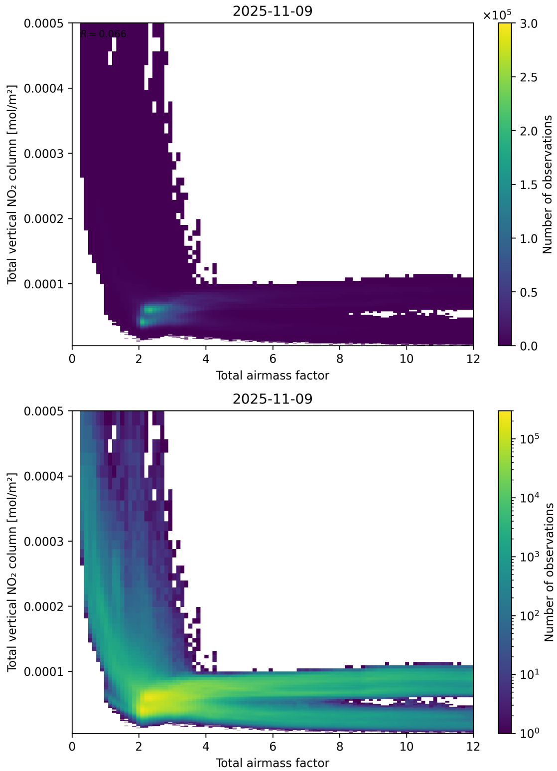
Figure 67: Scatter density plot of “Total airmass factor” against “Total vertical NO 2 column” for 2025-11-08 to 2025-11-10.
