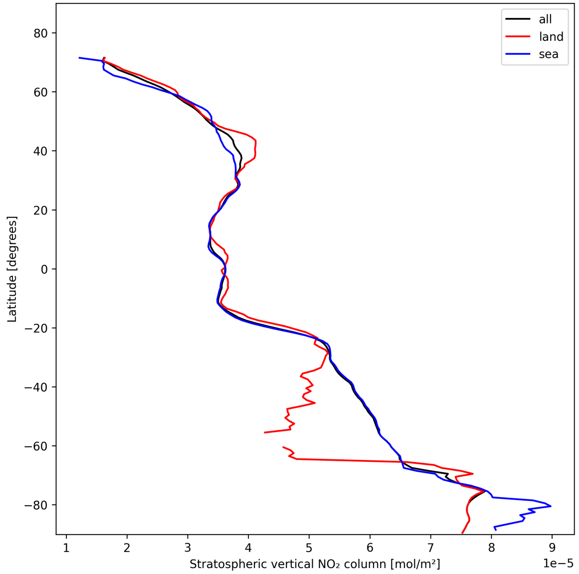
Figure 19: Zonal average of “Stratospheric vertical NO 2 column” for 2025-11-08 to 2025-11-10.
