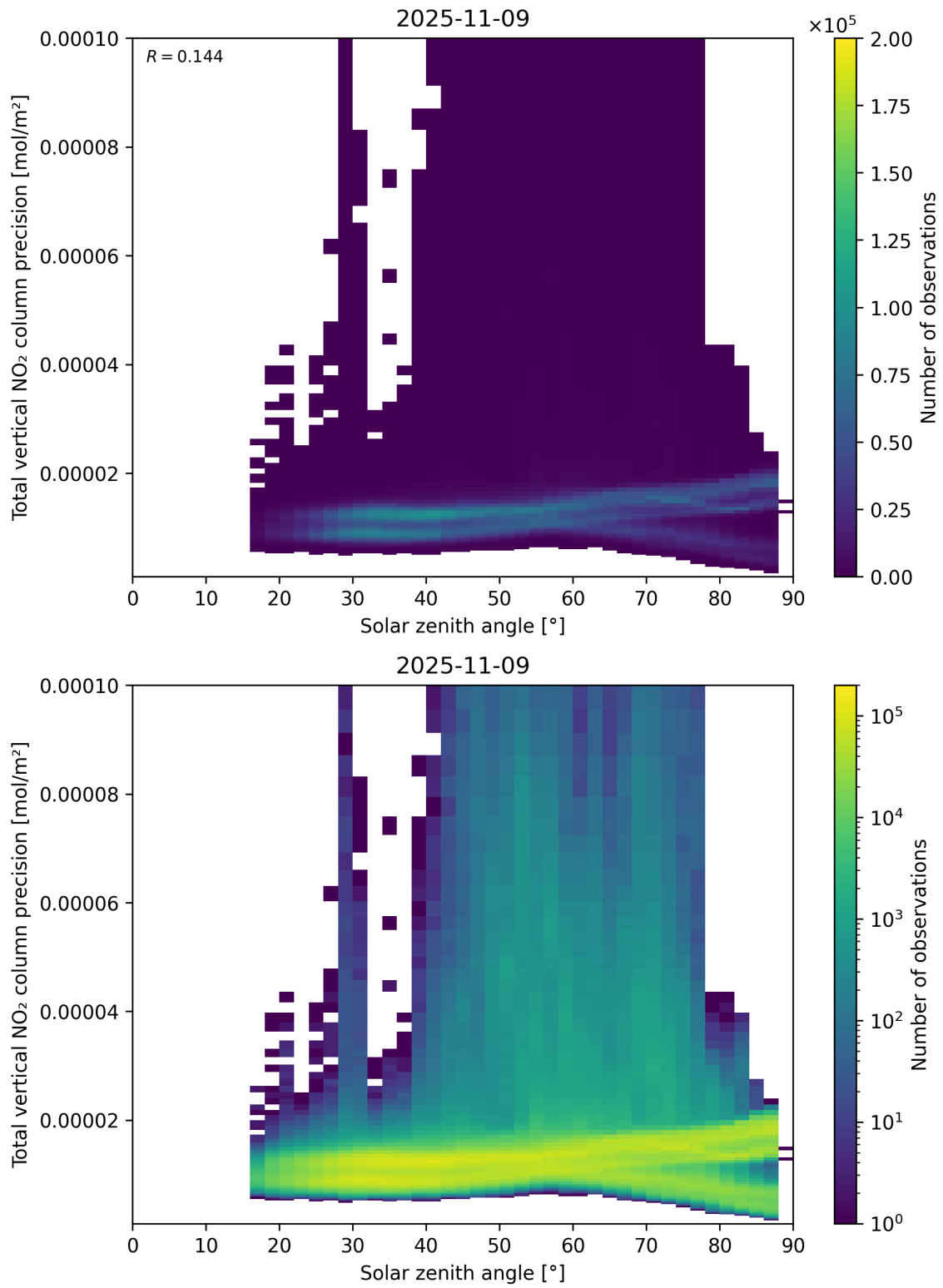
Figure 154: Scatter density plot of “Solar zenith angle” against “Total vertical NO 2 column precision” for 2025-11-08 to 2025-11-10.
