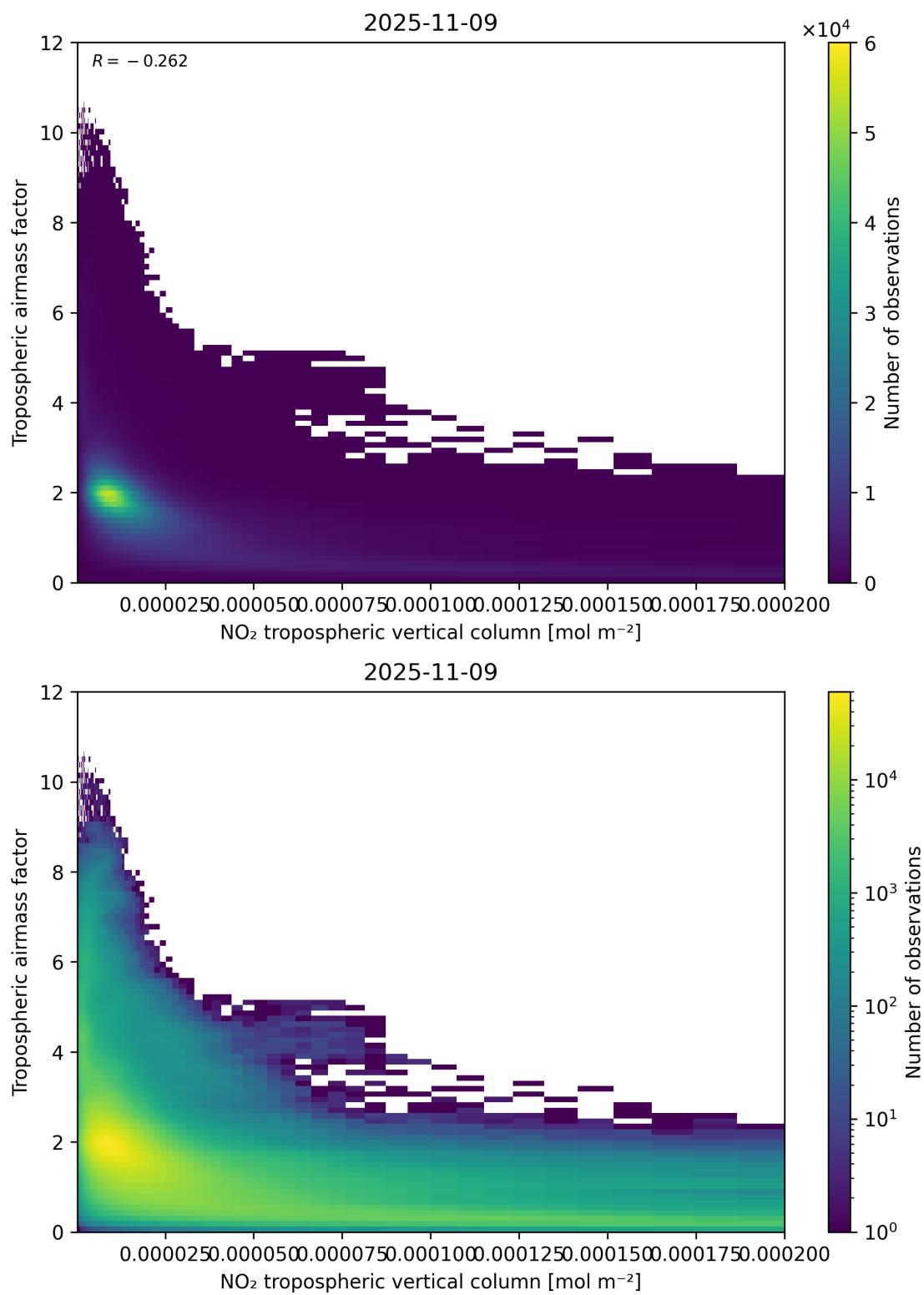
Figure 123: Scatter density plot of “NO 2 tropospheric vertical column” against “Tropospheric air mass factor” for 2025-11-08 to 2025-11-10.
