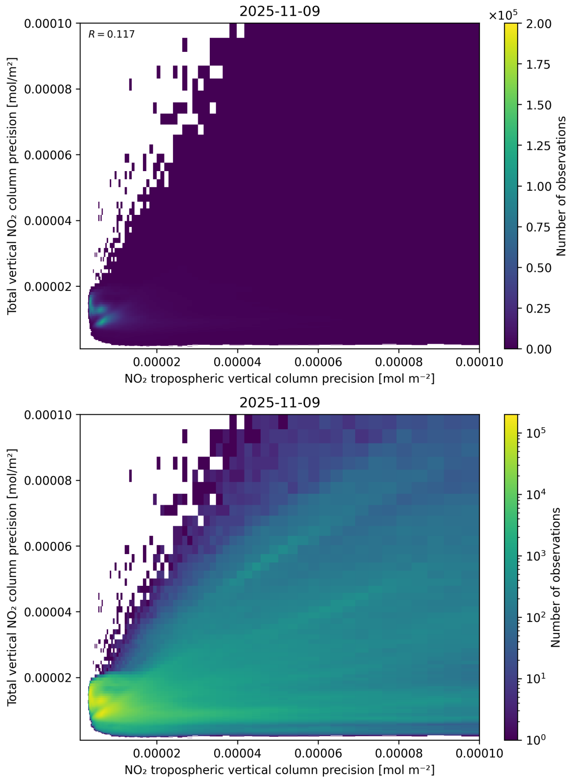
Figure 139: Scatter density plot of “NO 2 tropospheric vertical column precision” against “Total vertical NO 2 column precision” for 2025-11-08 to 2025-11-10.
