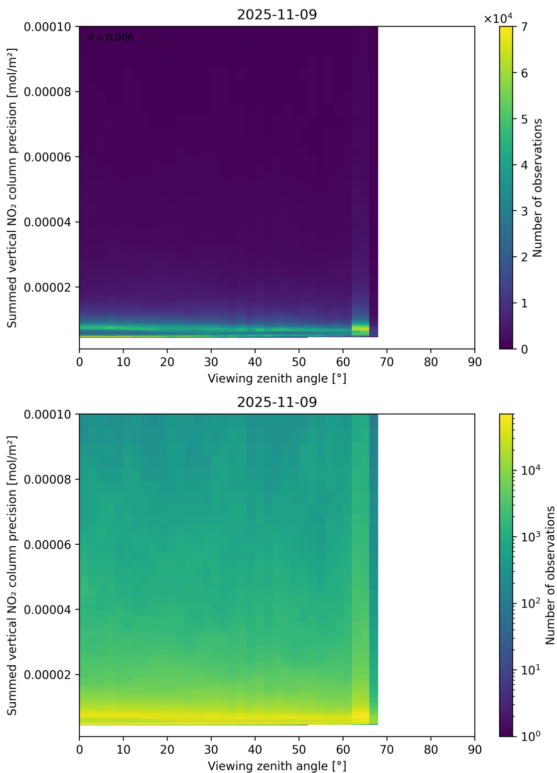
Figure 166: Scatter density plot of “Viewing zenith angle” against “Summed vertical NO 2 column precision” for 2025-11-08 to 2025-11-10.
