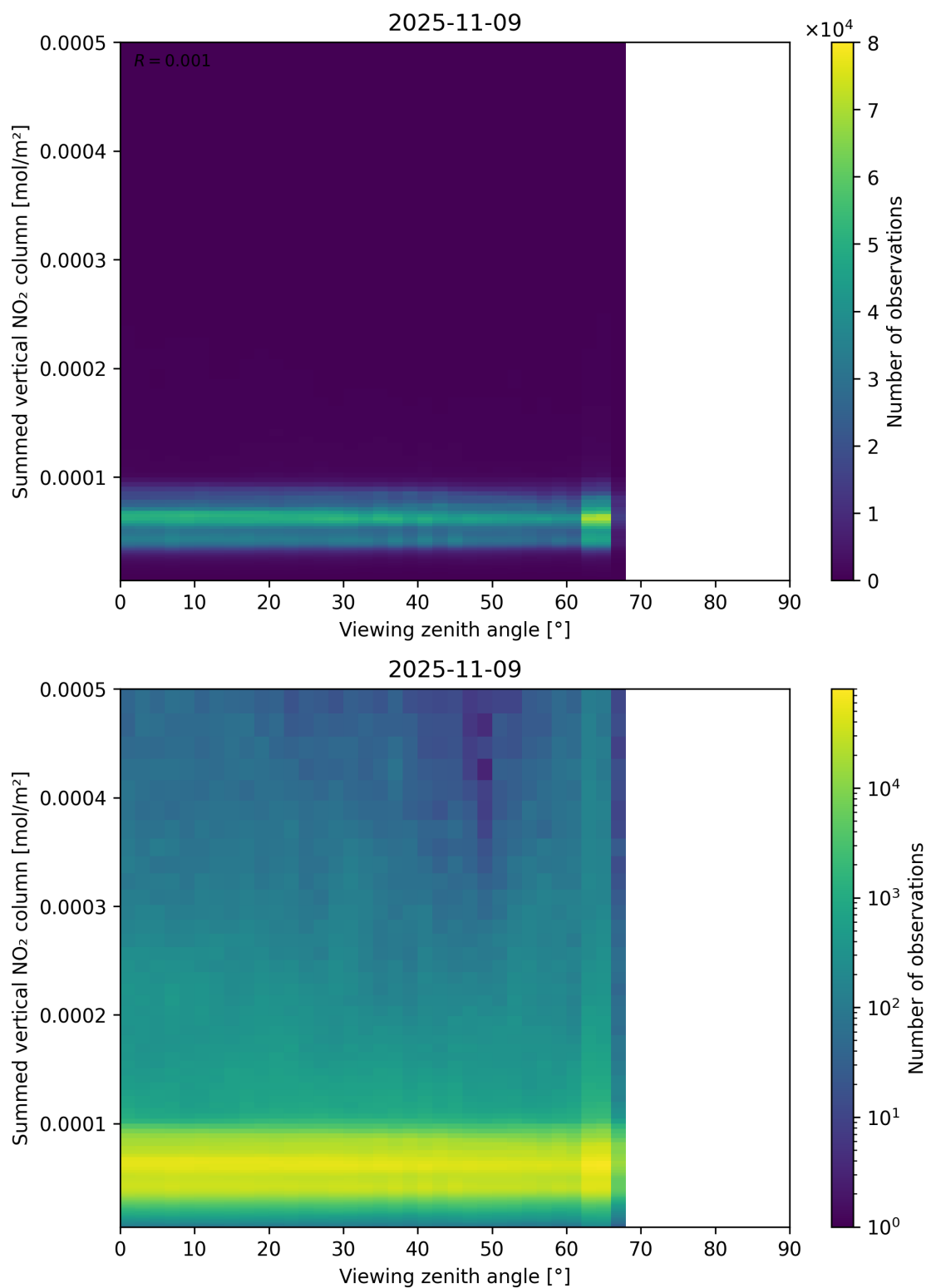
Figure 165: Scatter density plot of “Viewing zenith angle” against “Summed vertical NO 2 column” for 2025-11-08 to 2025-11-10.
