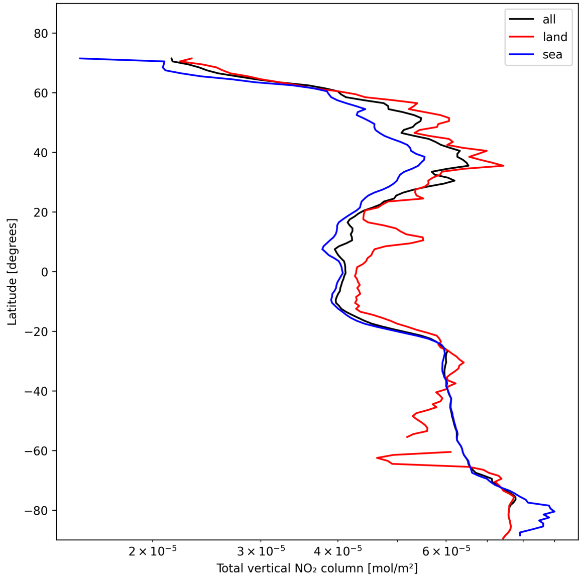
Figure 21: Zonal average of “Total vertical NO 2 column” for 2025-11-08 to 2025-11-10.
