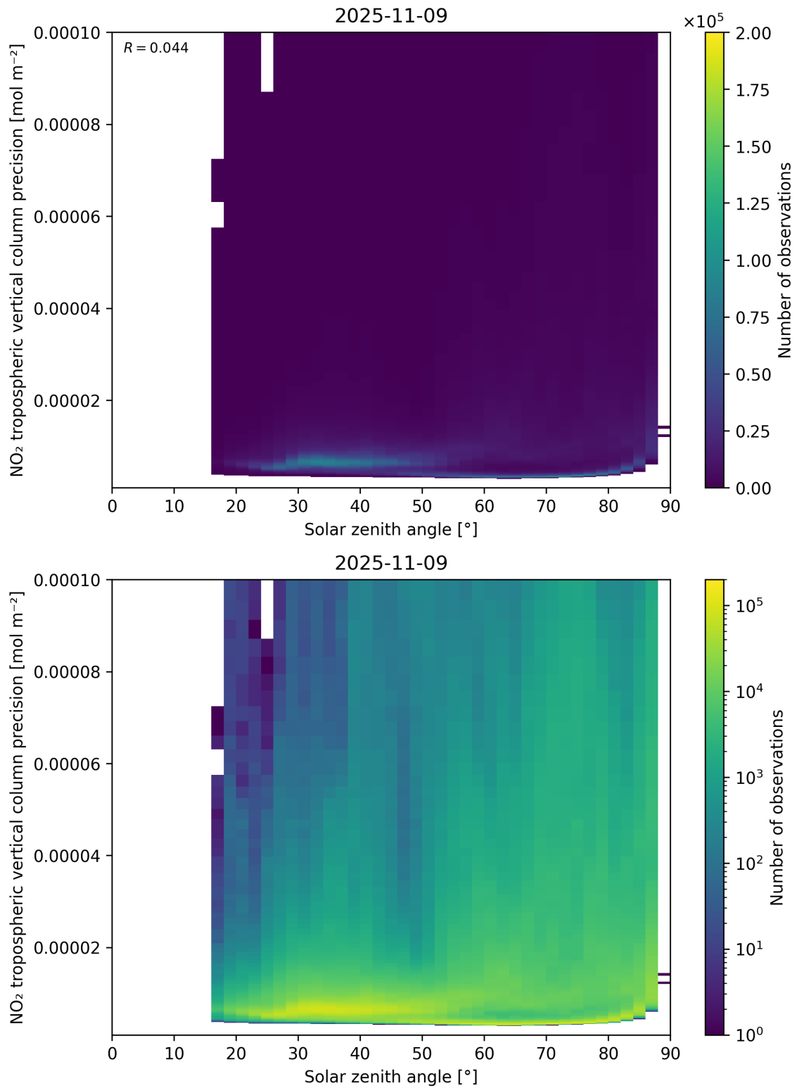
Figure 156: Scatter density plot of “Solar zenith angle” against “NO 2 tropospheric vertical column precision” for 2025-11-08 to 2025-11-10.
