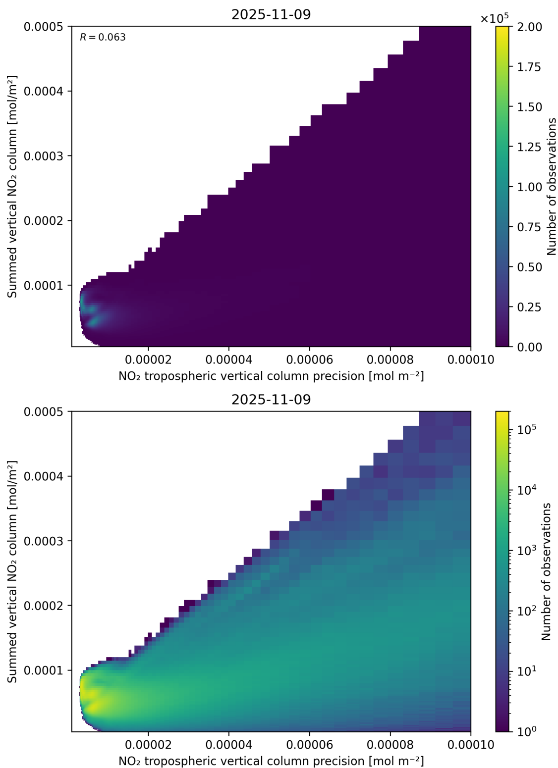
Figure 136: Scatter density plot of “NO 2 tropospheric vertical column precision” against “Summed vertical NO 2 column” for 2025-11-08 to 2025-11-10.
