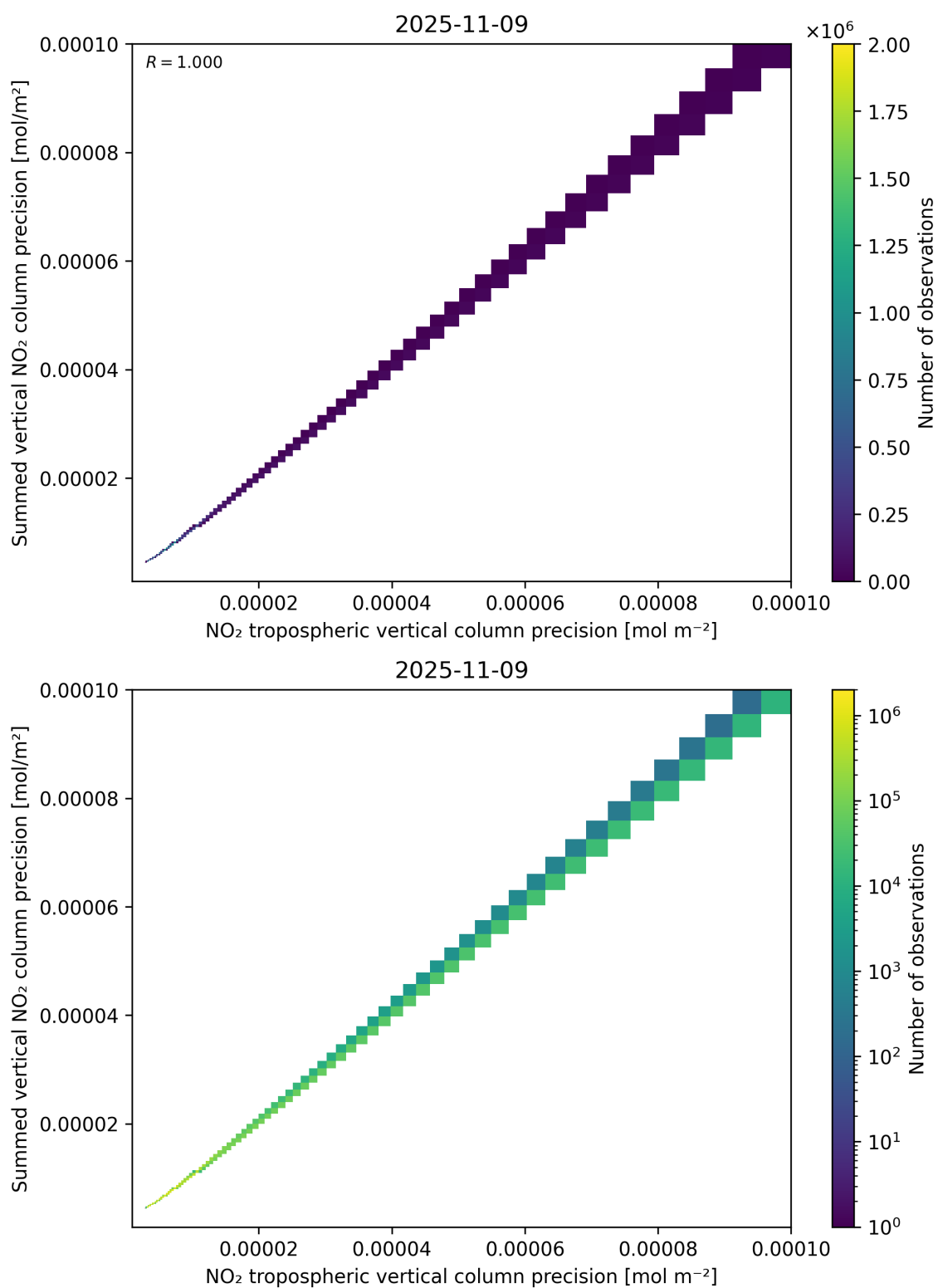
Figure 137: Scatter density plot of “NO 2 tropospheric vertical column precision” against “Summed vertical NO 2 column precision” for 2025-11-08 to 2025-11-10.
