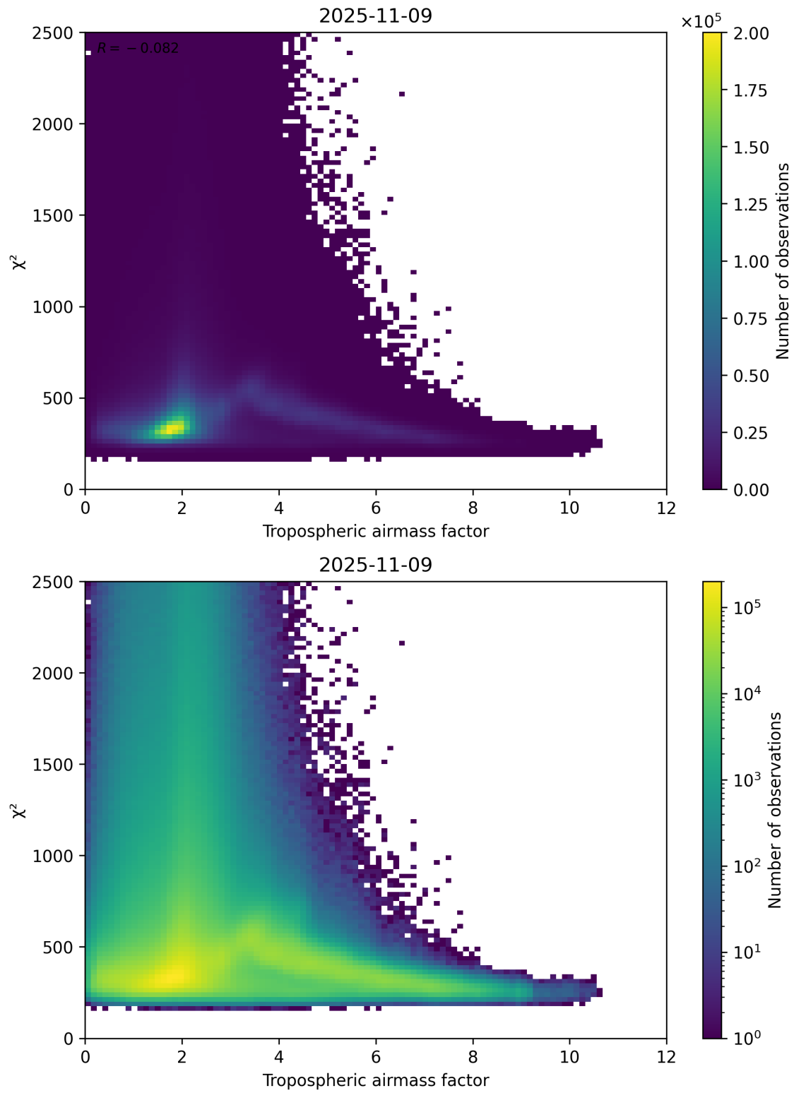
Figure 73: Scatter density plot of “Tropospheric airmass factor” against “ \chi^2 ” for 2025-11-08 to 2025-11-10.
