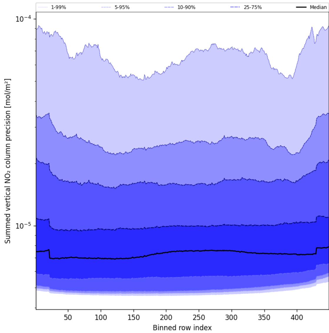
Figure 58: Along track statistics of “Summed vertical NO 2 column precision” for 2025-11-08 to 2025-11-10
