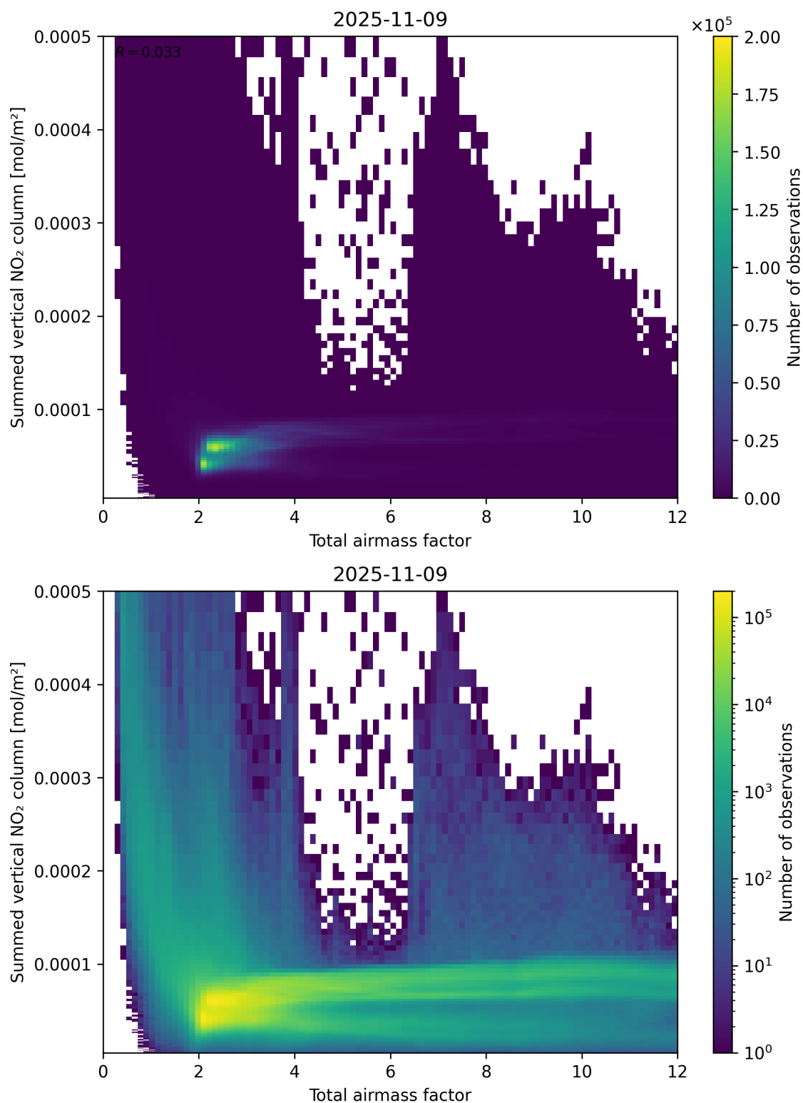
Figure 65: Scatter density plot of “Total airmass factor” against “Summed vertical NO 2 column” for 2025-11-08 to 2025-11-10.
