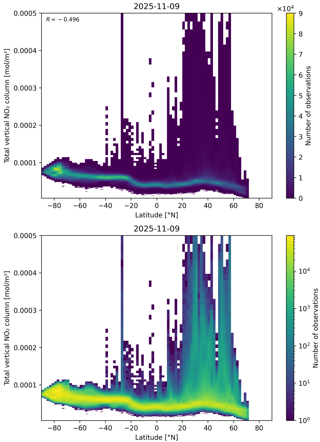
Figure 90: Scatter density plot of “Latitude” against “Total vertical NO 2 column” for 2025-11-08 to 2025-11-10.
