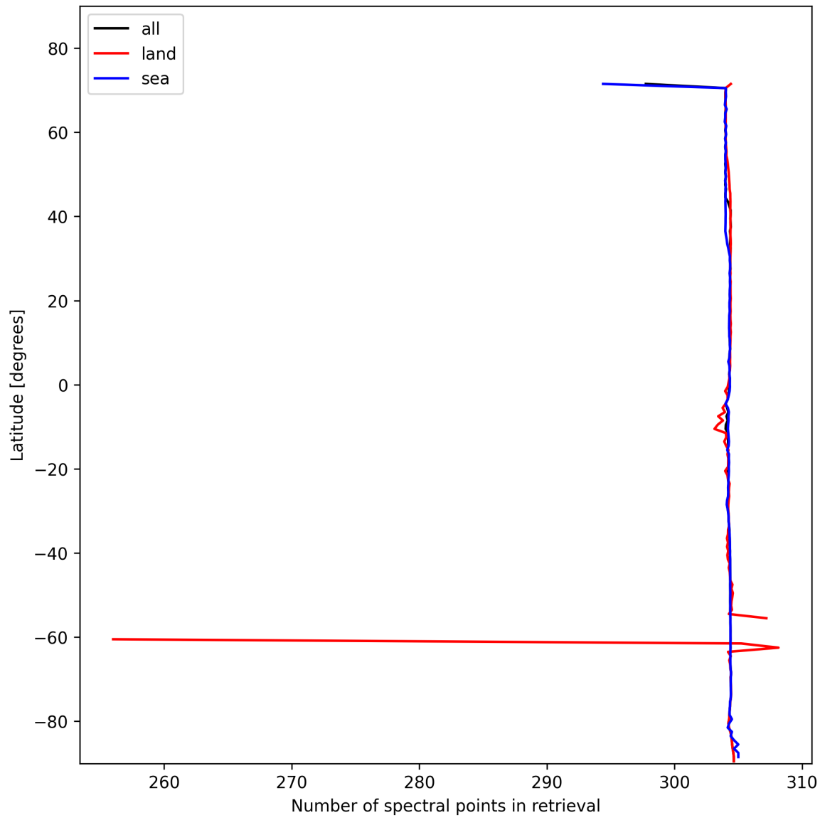
Figure 16: Zonal average of “Number of spectral points in retrieval” for 2025-11-08 to 2025-11-10.
