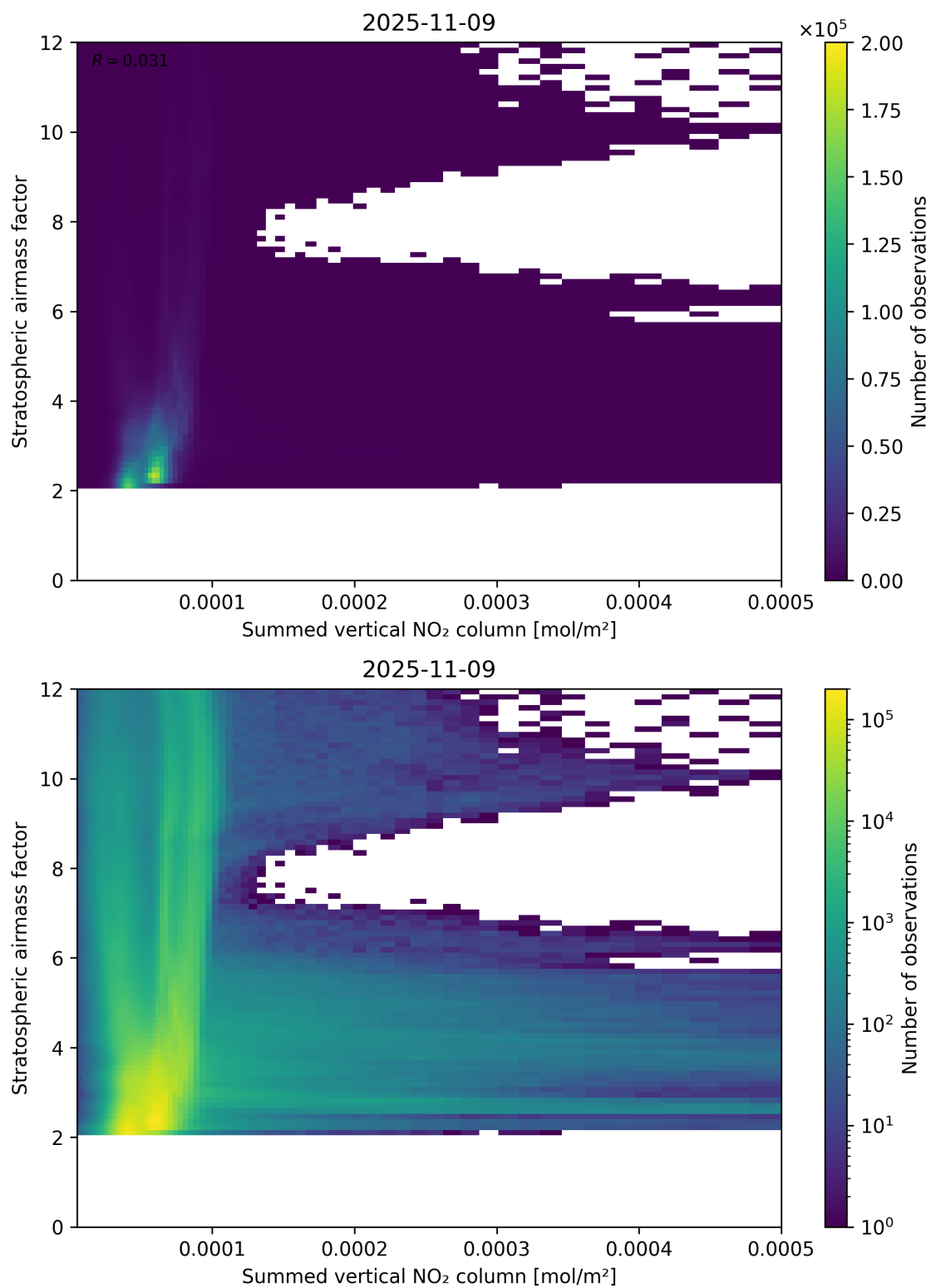
Figure 103: Scatter density plot of “Summed vertical NO 2 column” against “Stratospheric airmass factor” for 2025-11-08 to 2025-11-10.
