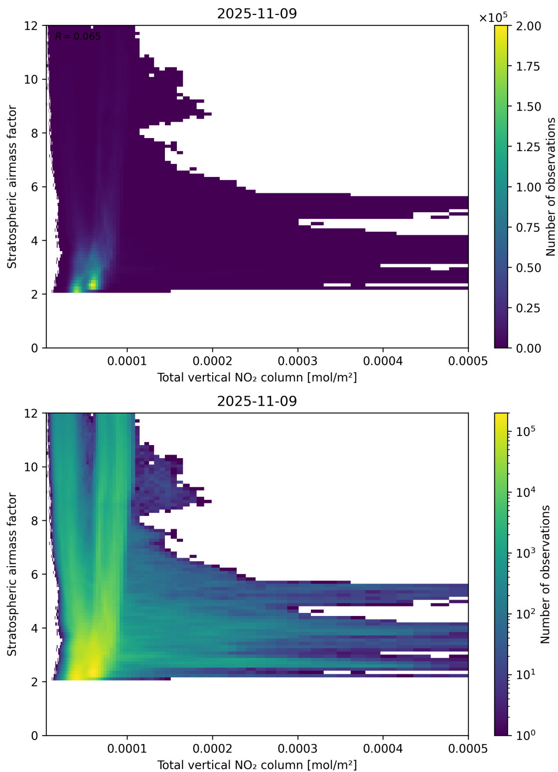
Figure 110: Scatter density plot of “Total vertical NO 2 column” against “Stratospheric airmass factor” for 2025-11-08 to 2025-11-10.
