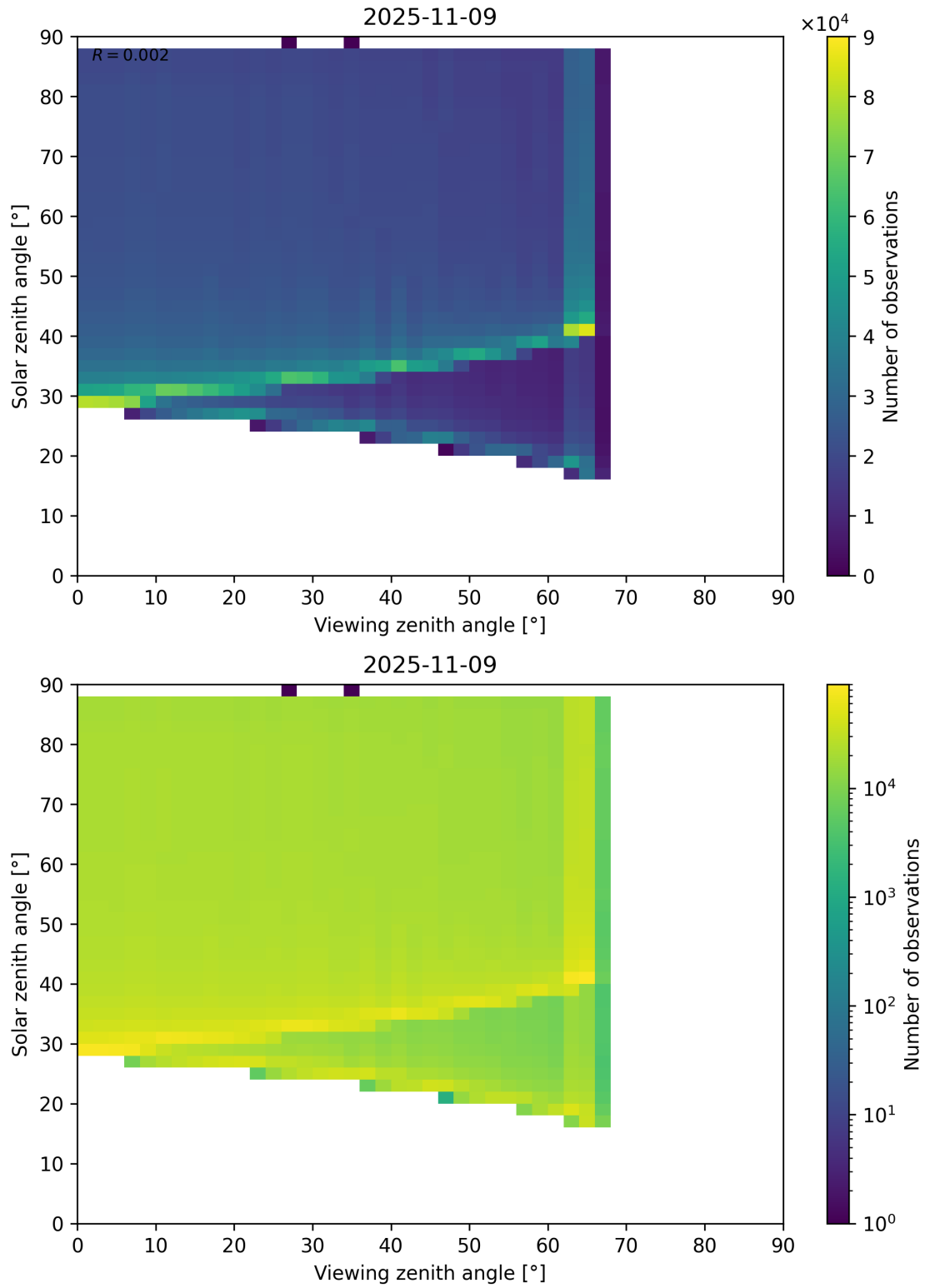
Figure 172: Scatter density plot of “Viewing zenith angle” against “Solar zenith angle” for 2025-11-08 to 2025-11-10.
