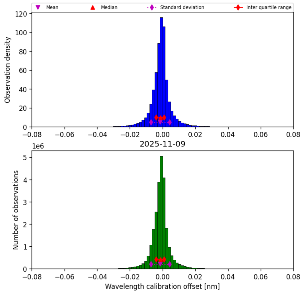
Figure 35: Histogram of “Wavelength calibration offset” for 2025-11-08 to 2025-11-10
