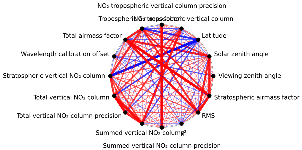
Figure 1: Map of correlation graph for 2025-11-08 to 2025-11-10.
