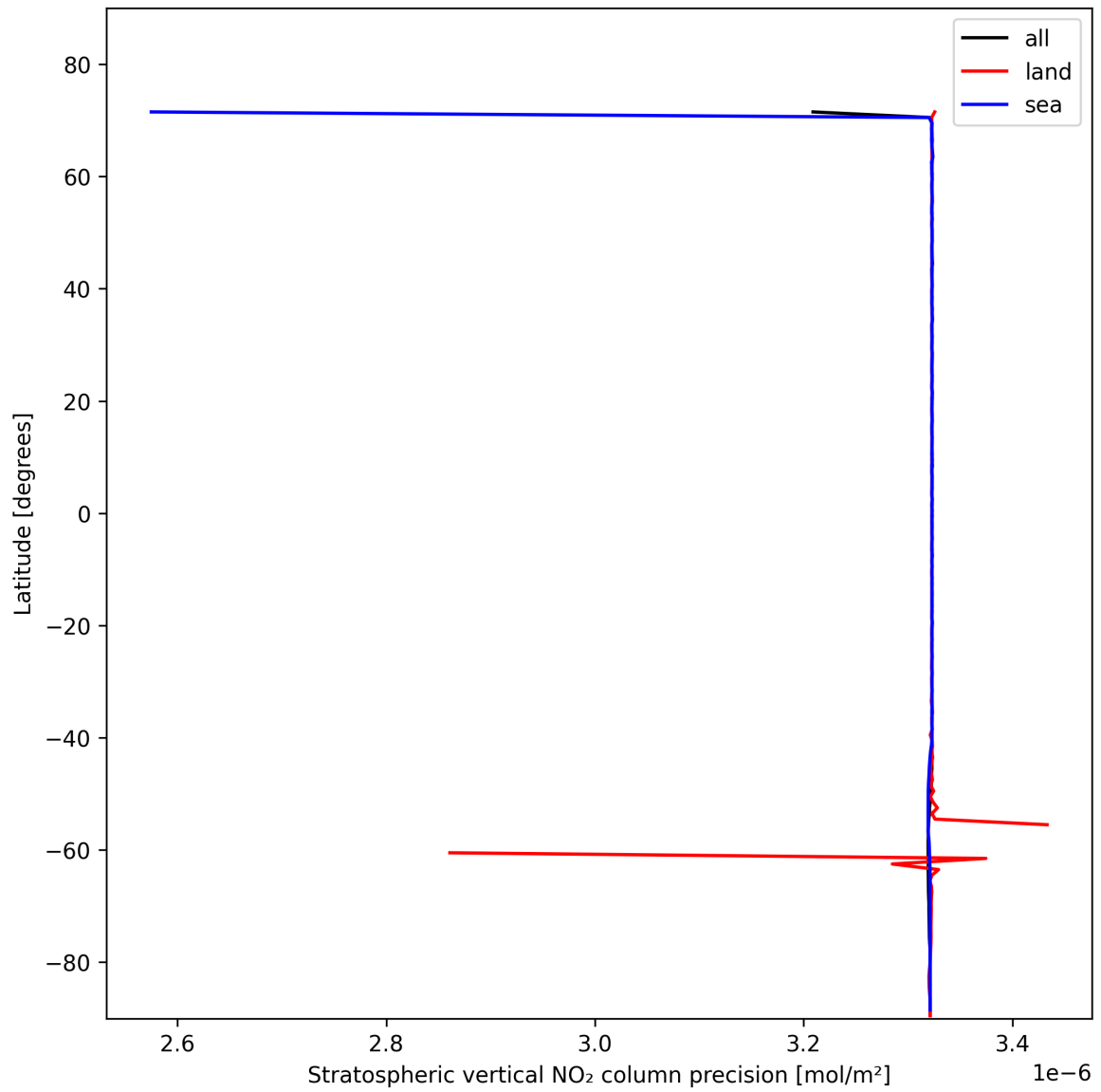
Figure 20: Zonal average of “Stratospheric vertical NO 2 column precision” for 2025-11-08 to 2025-11-10.
