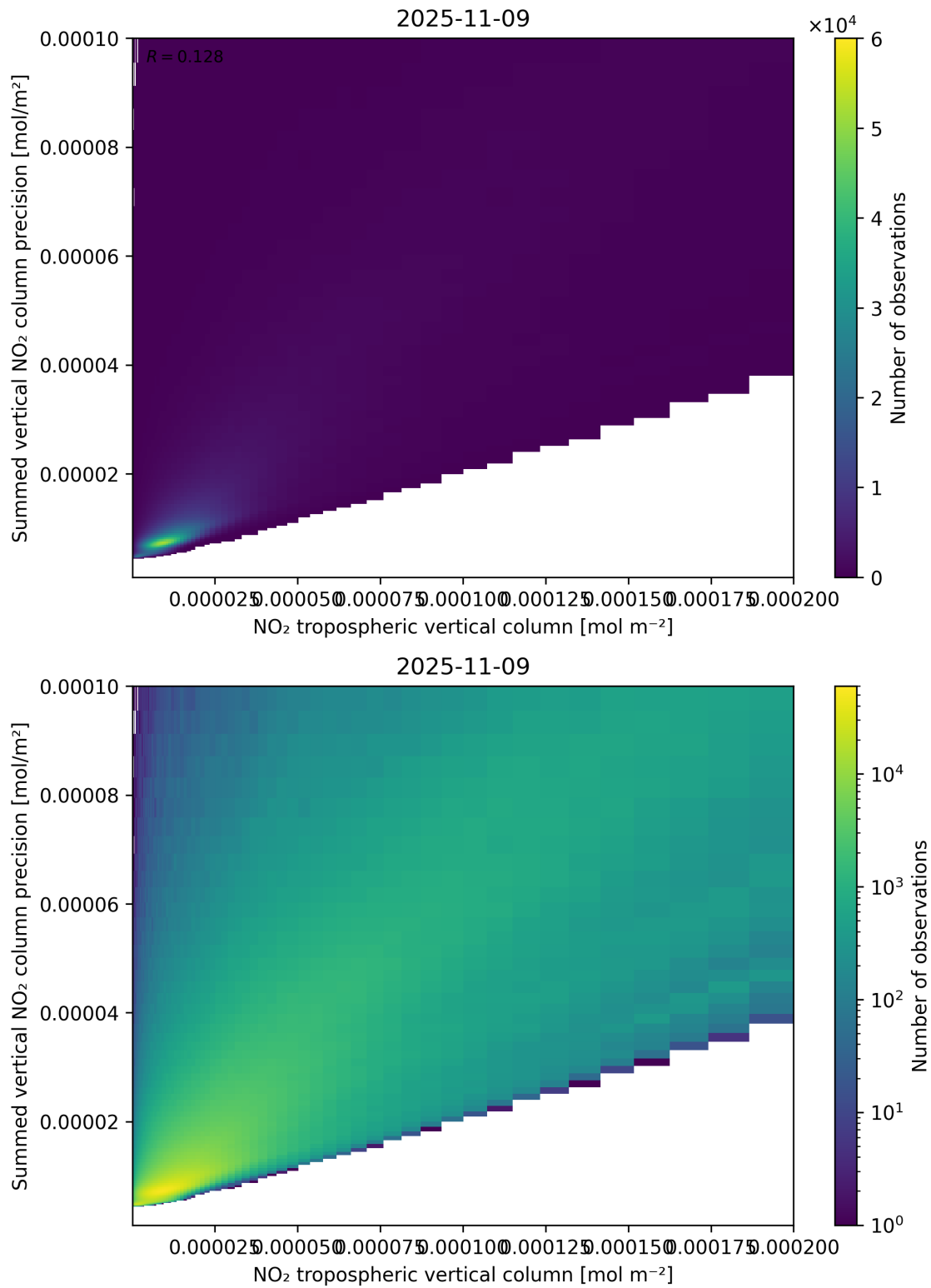
Figure 127: Scatter density plot of “NO 2 tropospheric vertical column” against “Summed vertical NO 2 column precision” for 2025-11-08 to 2025-11-10.
