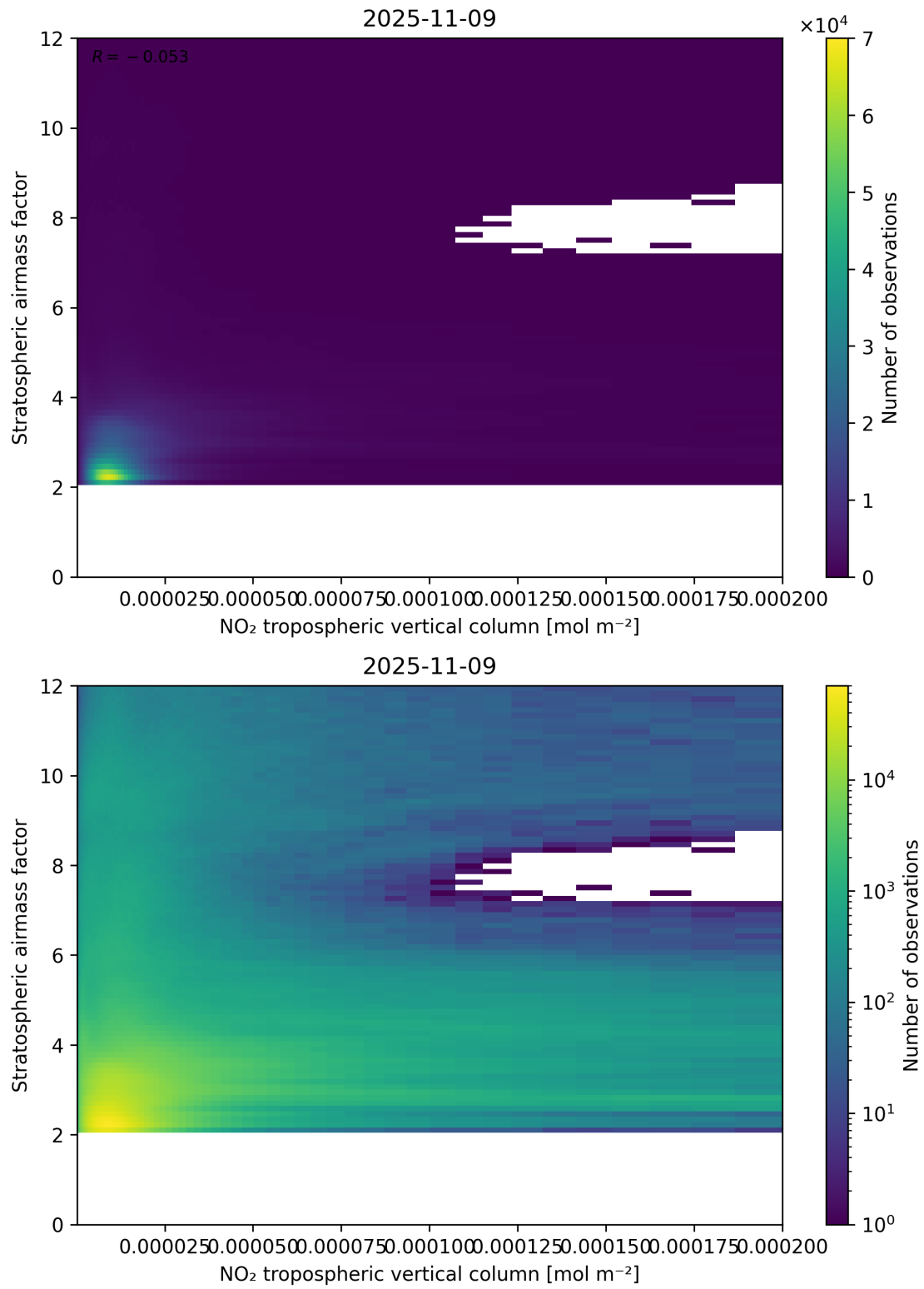
Figure 121: Scatter density plot of “NO 2 tropospheric vertical column” against “Stratospheric air mass factor” for 2025-11-08 to 2025-11-10.
