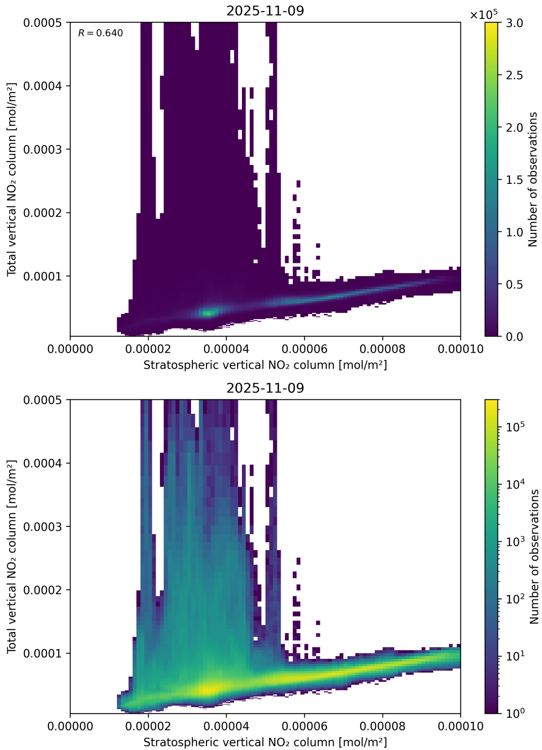
Figure 100: Scatter density plot of “Stratospheric vertical NO 2 column” against “Total vertical NO 2 column” for 2025-11-08 to 2025-11-10.
