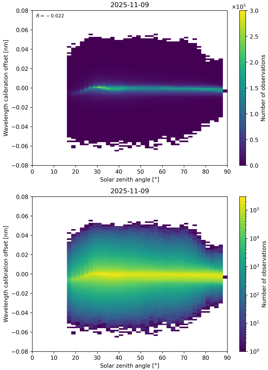
Figure 158: Scatter density plot of “Solar zenith angle” against “Wavelength calibration offset” for 2025-11-08 to 2025-11-10.
