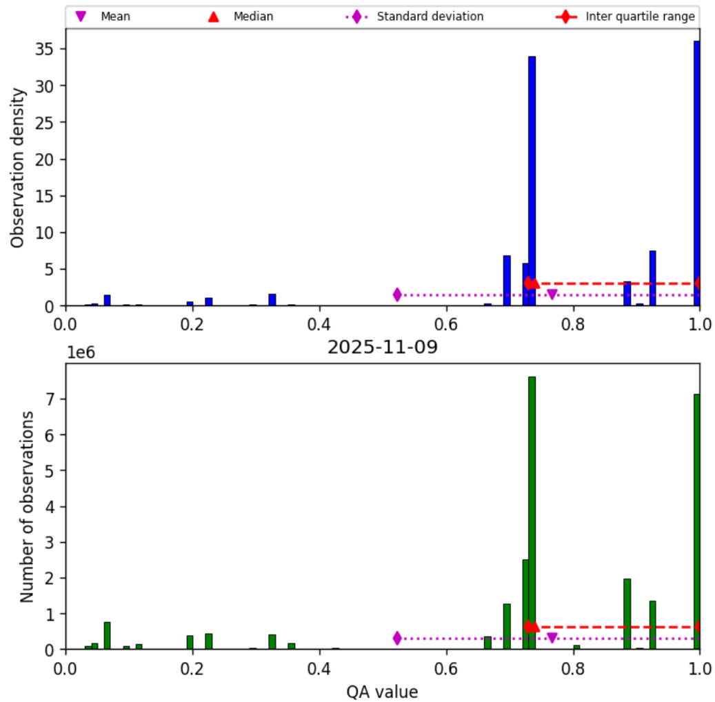
Figure 28: Histogram of “QA value” for 2025-11-08 to 2025-11-10
