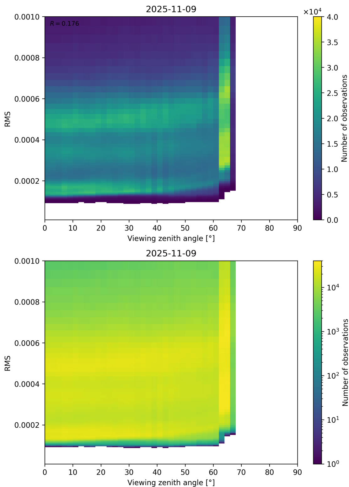
Figure 171: Scatter density plot of “Viewing zenith angle” against “RMS” for 2025-11-08 to 2025-11-10.
