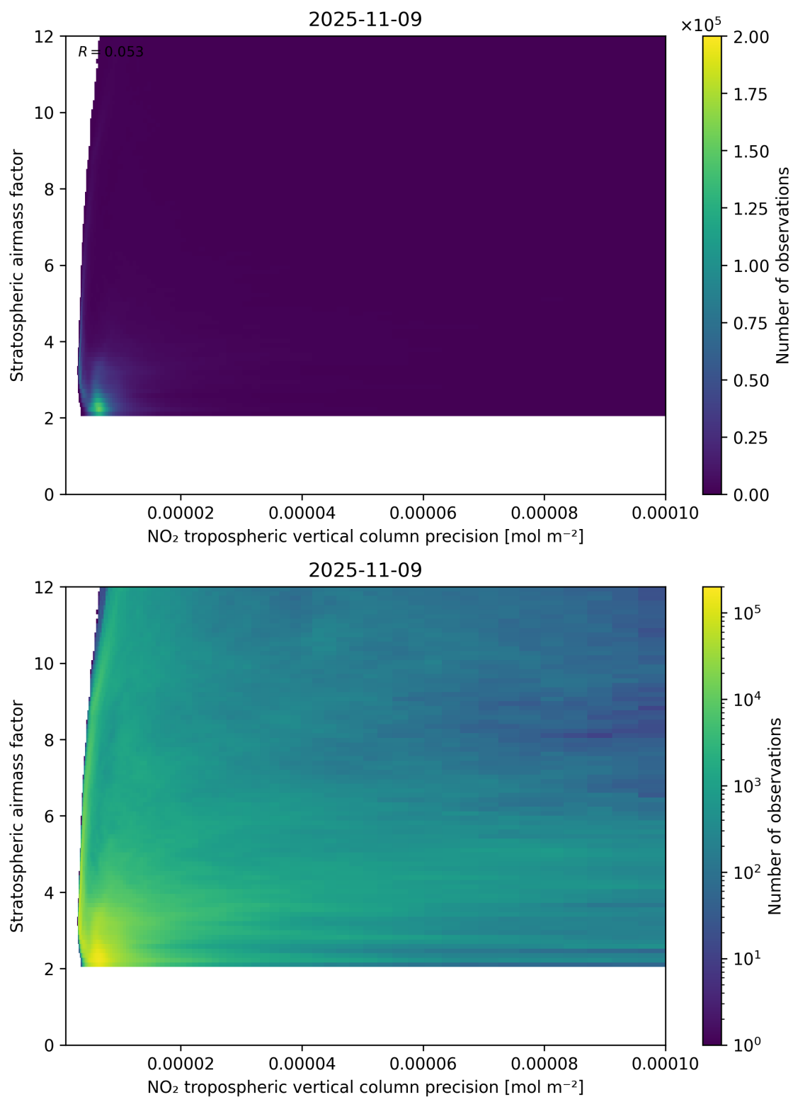
Figure 131: Scatter density plot of “NO 2 tropospheric vertical column precision” against “Stratospheric airmass factor” for 2025-11-08 to 2025-11-10.
