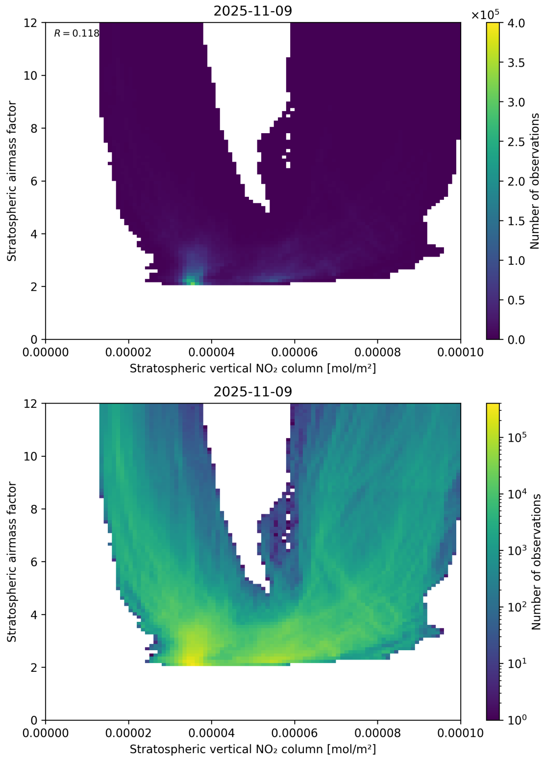
Figure 96: Scatter density plot of “Stratospheric vertical NO 2 column” against “Stratospheric airmass factor” for 2025-11-08 to 2025-11-10.
