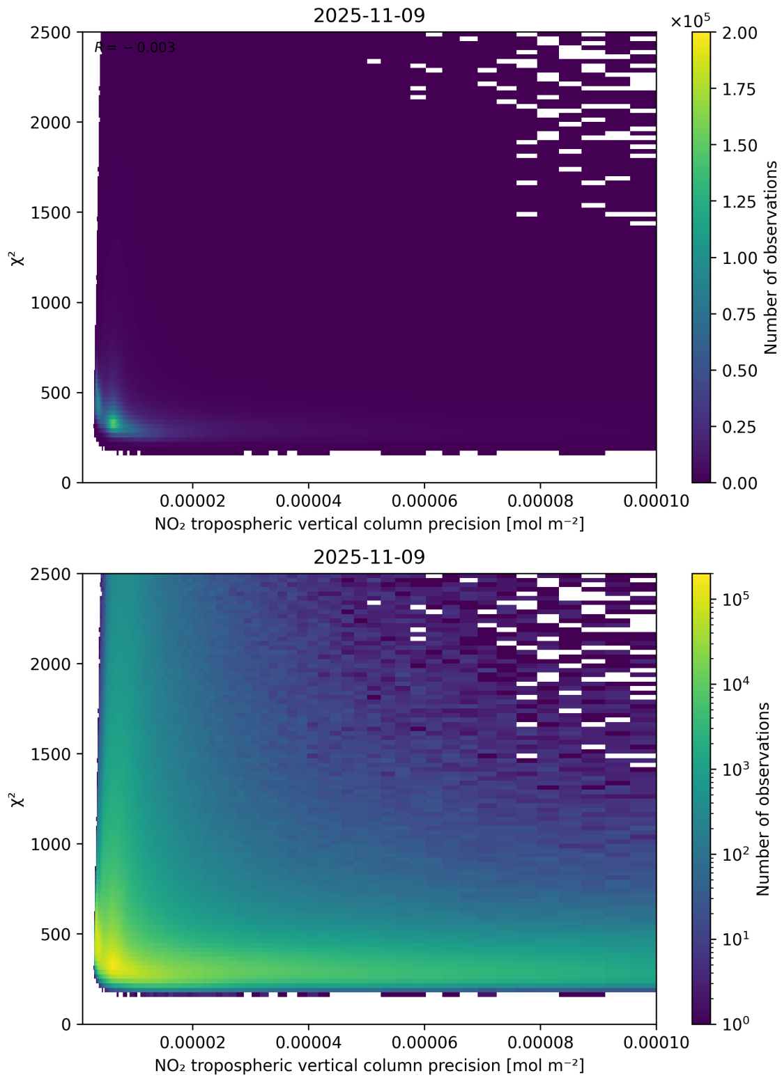
Figure 134: Scatter density plot of “NO 2 tropospheric vertical column precision” against “ \chi^2 ” for 2025-11-08 to 2025-11-10.
