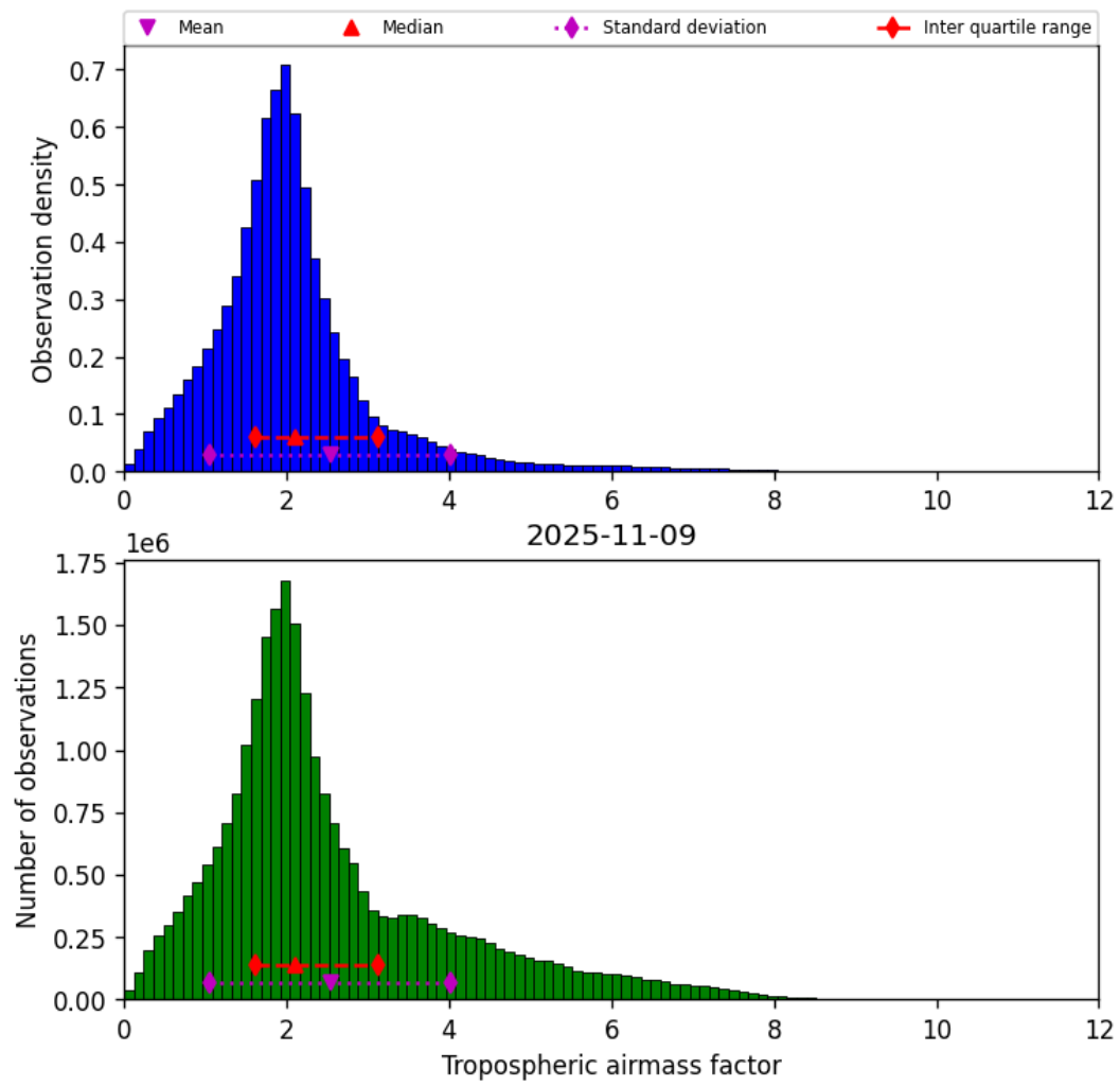
Figure 31: Histogram of “Tropospheric airmass factor” for 2025-11-08 to 2025-11-10
