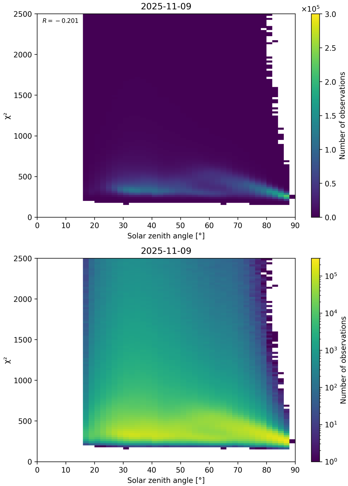
Figure 148: Scatter density plot of “Solar zenith angle” against “ \chi^2 ” for 2025-11-08 to 2025-11-10.
