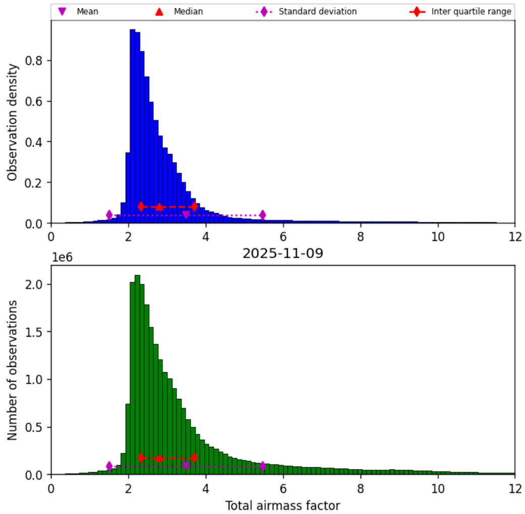
Figure 32: Histogram of “Total airmass factor” for 2025-11-08 to 2025-11-10
