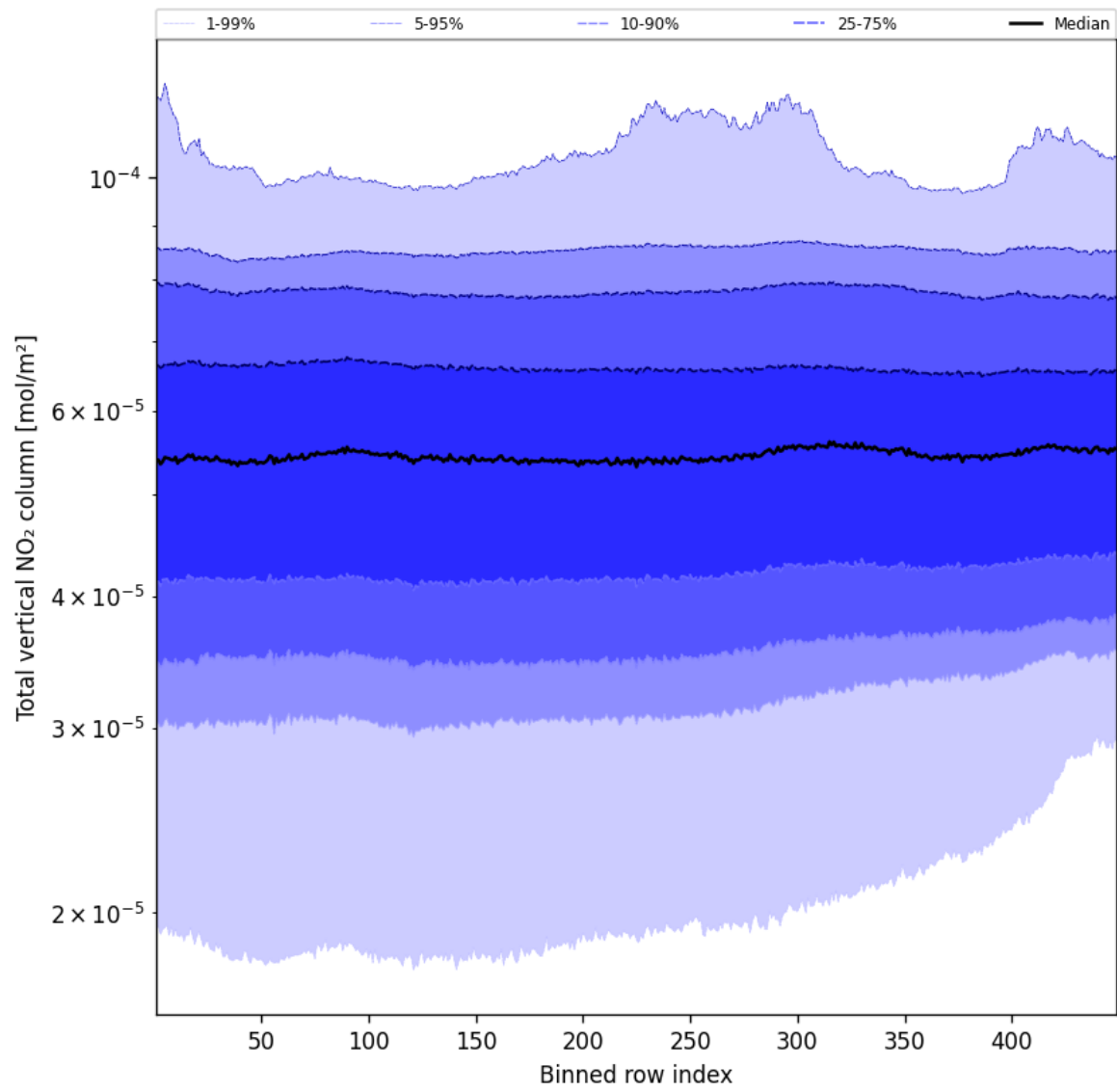
Figure 55: Along track statistics of “Total vertical NO 2 column” for 2025-11-08 to 2025-11-10
