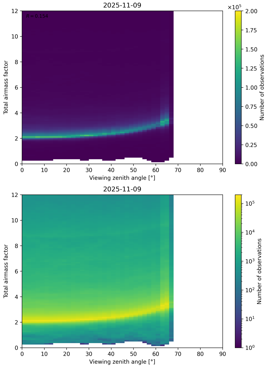
Figure 160: Scatter density plot of “Viewing zenith angle” against “Total airmass factor” for 2025-11-08 to 2025-11-10.
