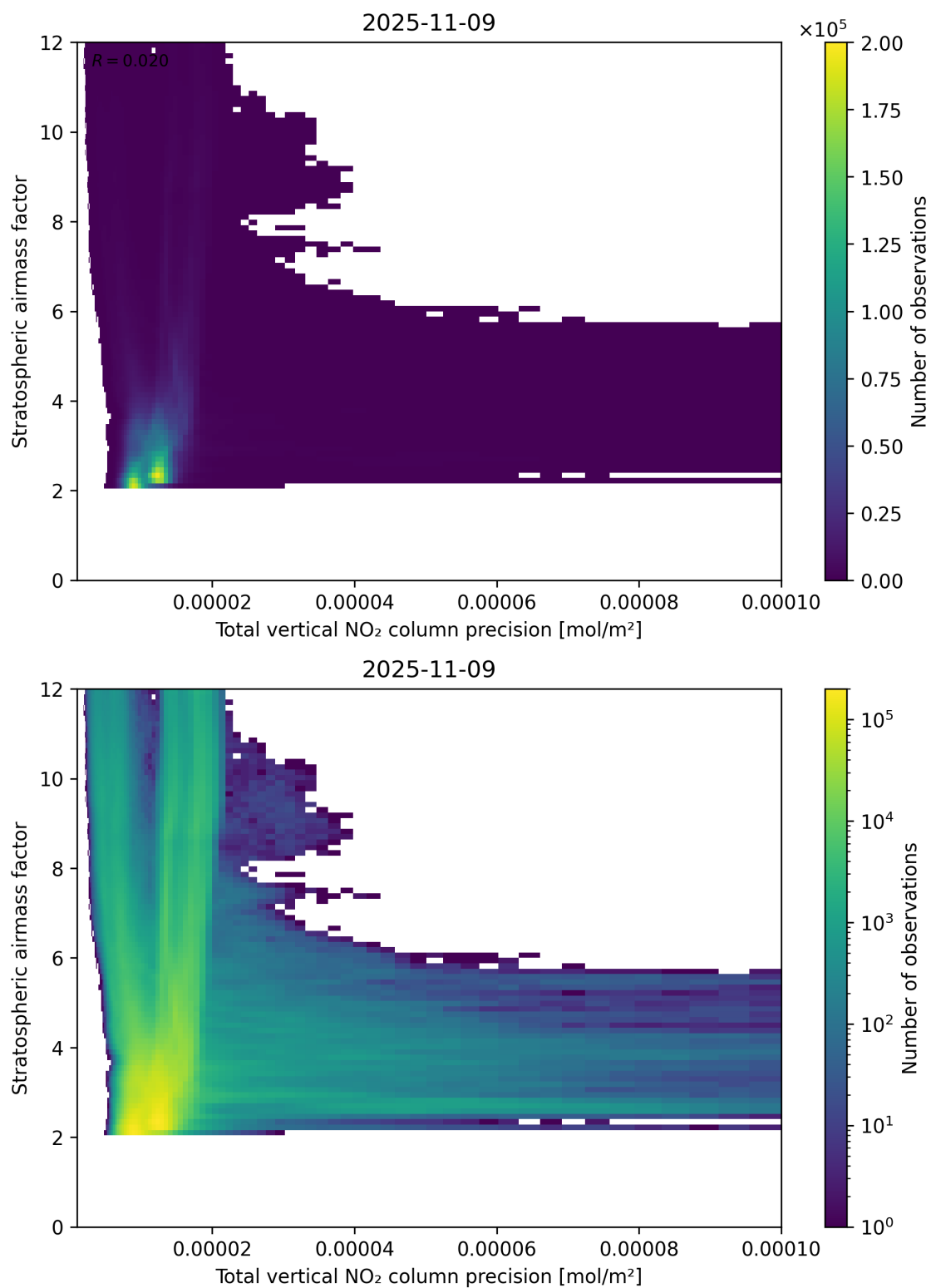
Figure 115: Scatter density plot of “Total vertical NO 2 column precision” against “Stratospheric air mass factor” for 2025-11-08 to 2025-11-10.
