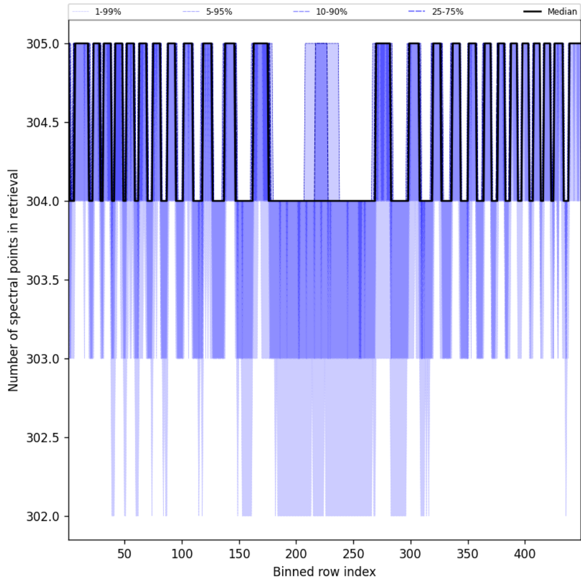
Figure 50: Along track statistics of “Number of spectral points in retrieval” for 2025-11-08 to 2025-11-10
