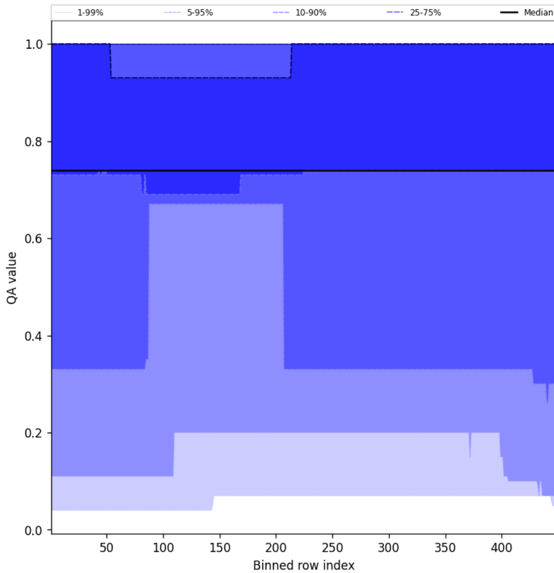
Figure 45: Along track statistics of “QA value” for 2025-11-08 to 2025-11-10
