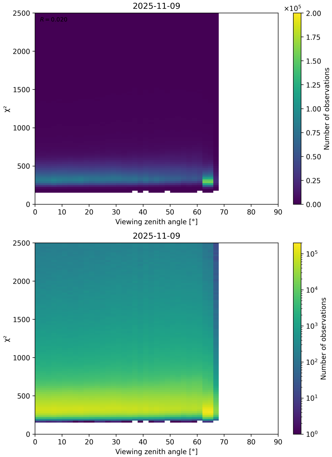
Figure 162: Scatter density plot of “Viewing zenith angle” against “ \chi^2 ” for 2025-11-08 to 2025-11-10.
