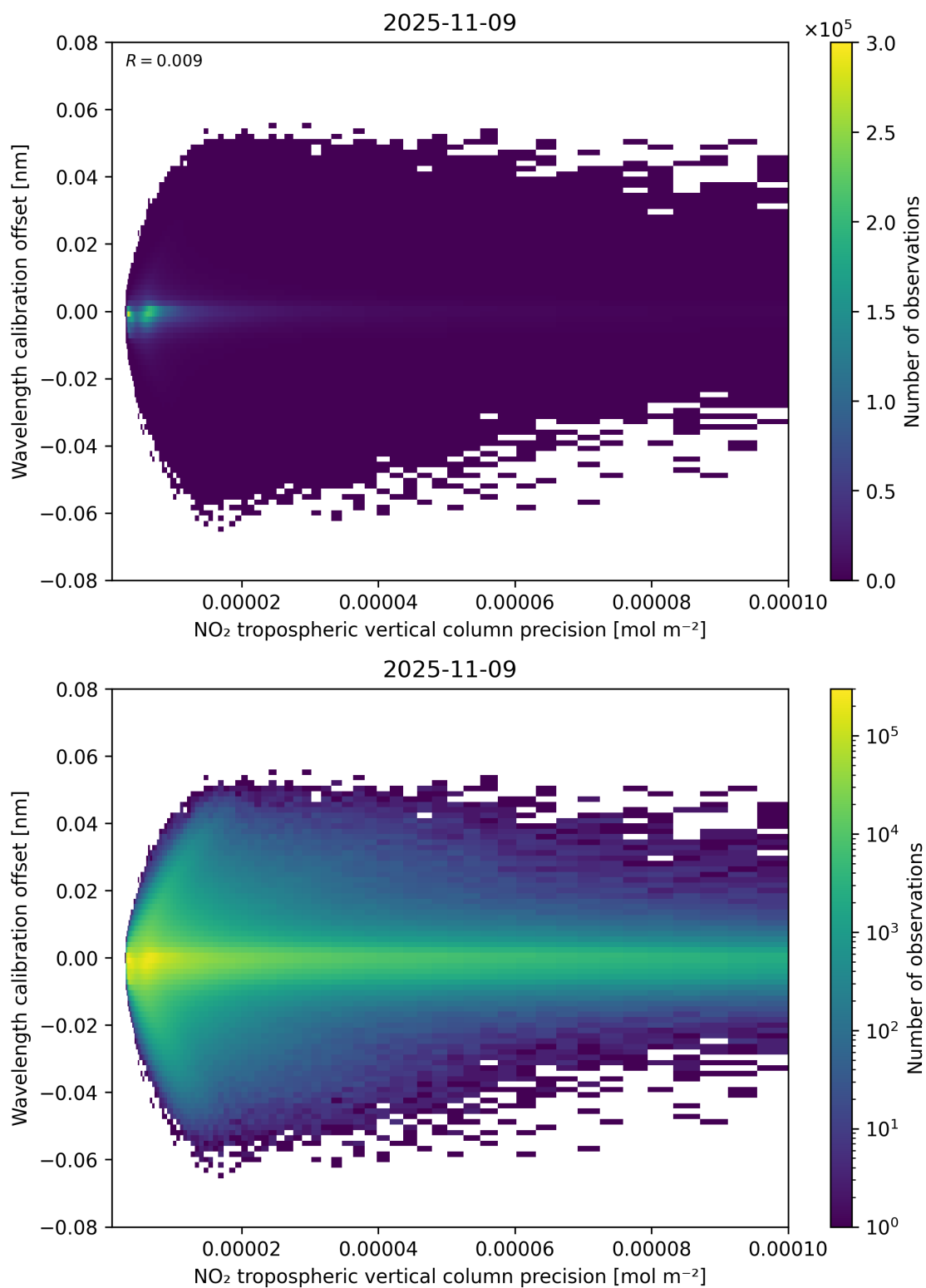
Figure 141: Scatter density plot of “NO 2 tropospheric vertical column precision” against “Wavelength calibration offset” for 2025-11-08 to 2025-11-10.
