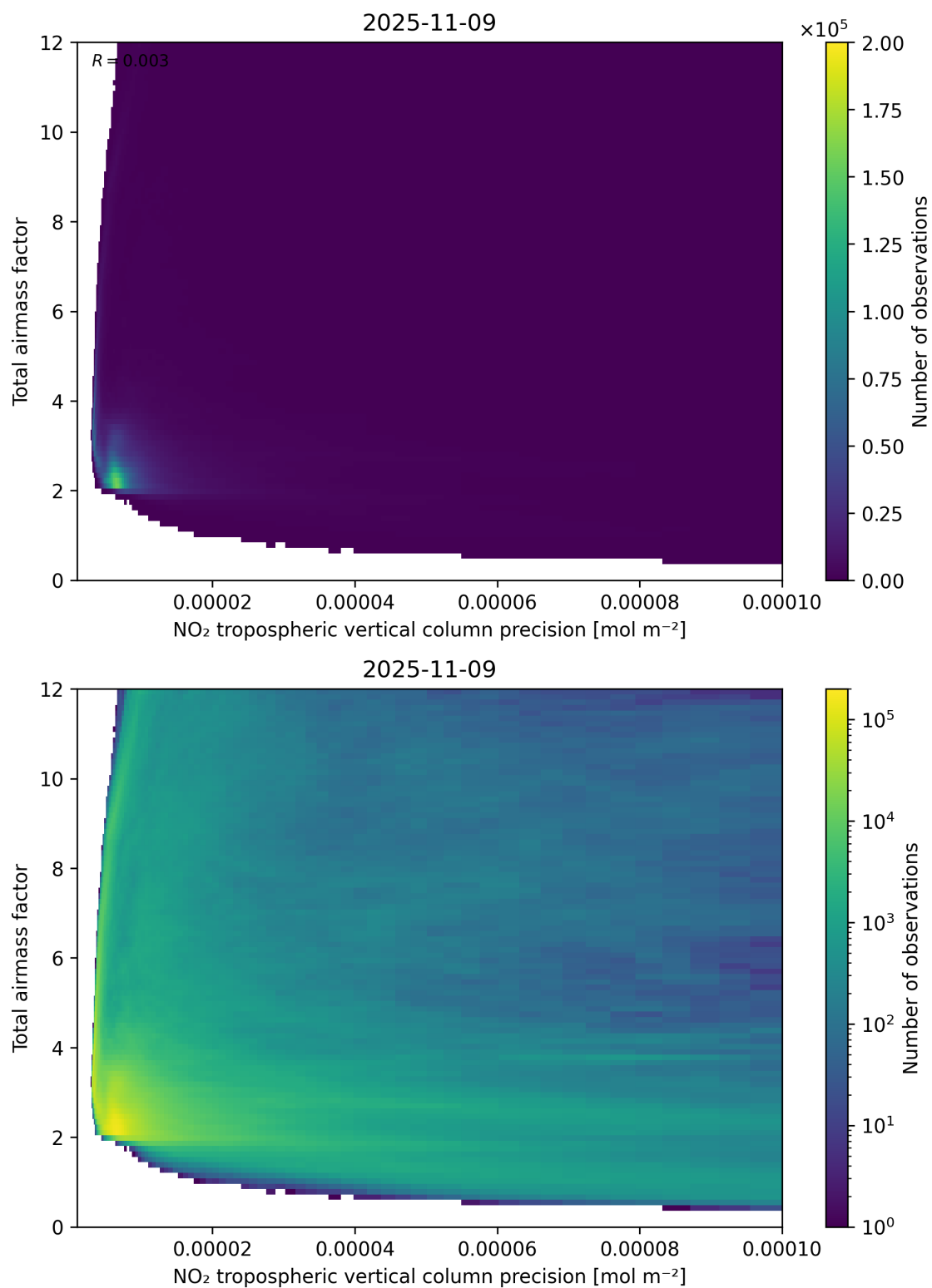
Figure 132: Scatter density plot of “NO 2 tropospheric vertical column precision” against “Total air mass factor” for 2025-11-08 to 2025-11-10.
