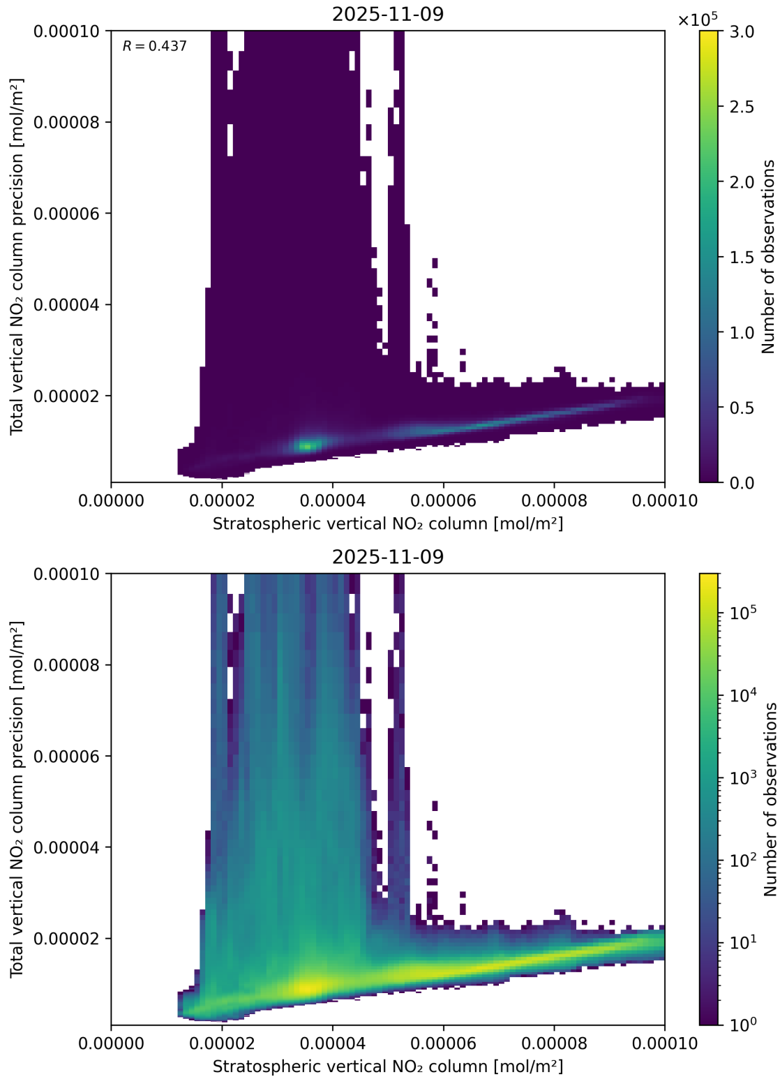
Figure 101: Scatter density plot of “Stratospheric vertical NO 2 column” against “Total vertical NO 2 column precision” for 2025-11-08 to 2025-11-10.
