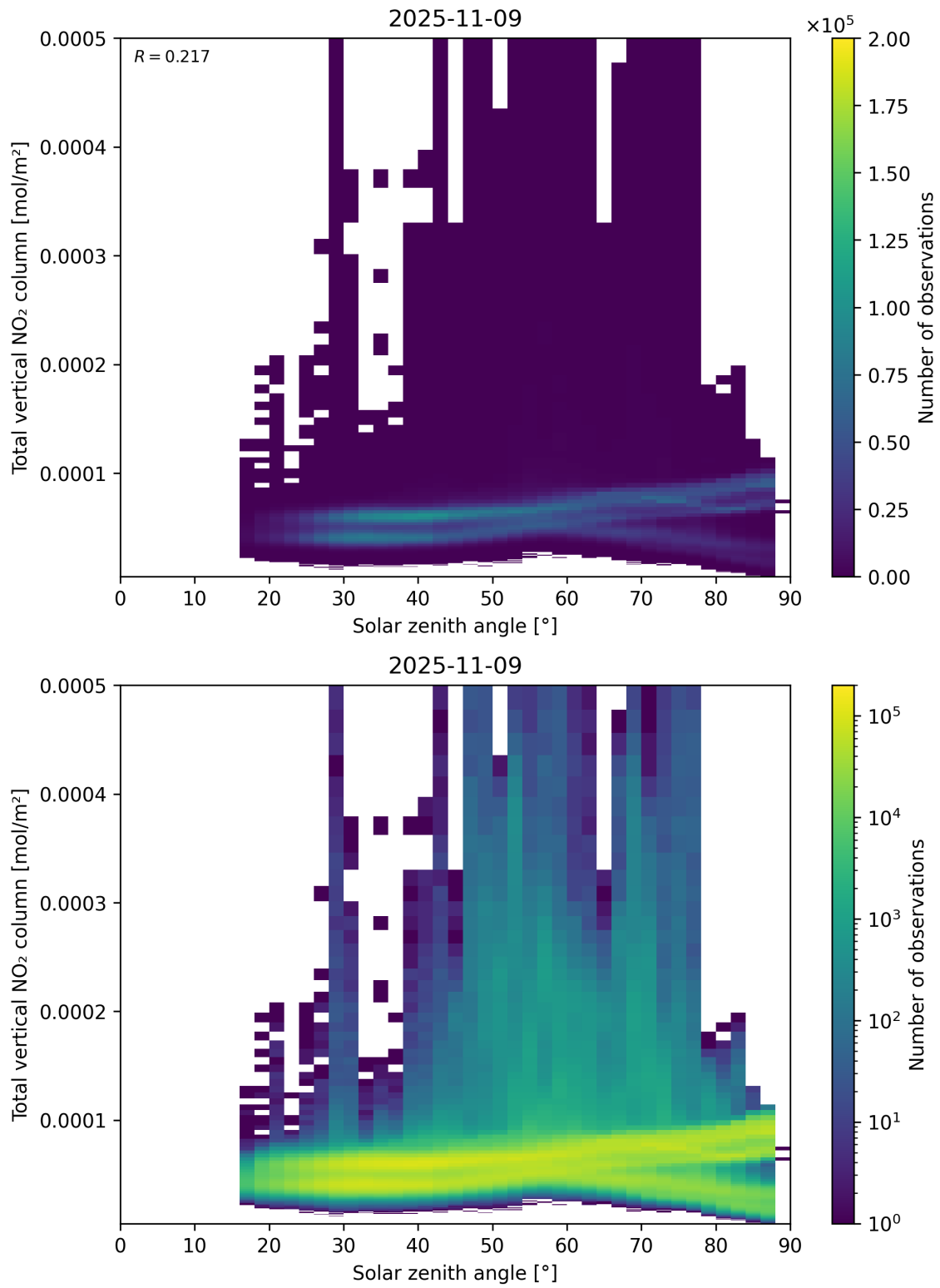
Figure 153: Scatter density plot of “Solar zenith angle” against “Total vertical NO 2 column” for 2025-11-08 to 2025-11-10.
