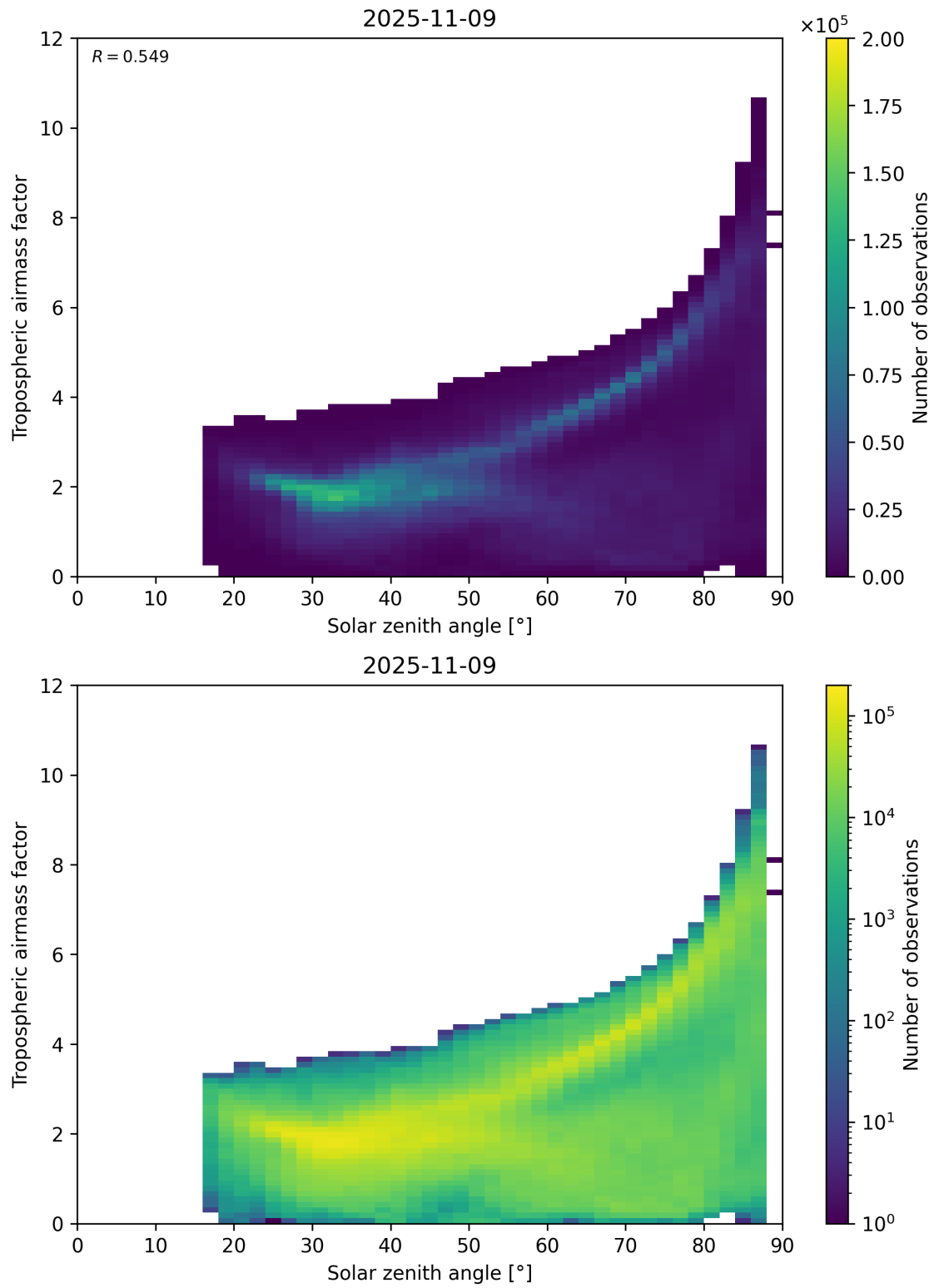
Figure 147: Scatter density plot of “Solar zenith angle” against “Tropospheric airmass factor” for 2025-11-08 to 2025-11-10.
