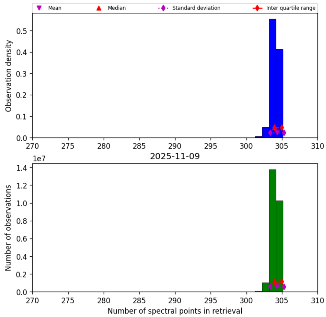
Figure 33: Histogram of “Number of spectral points in retrieval” for 2025-11-08 to 2025-11-10
