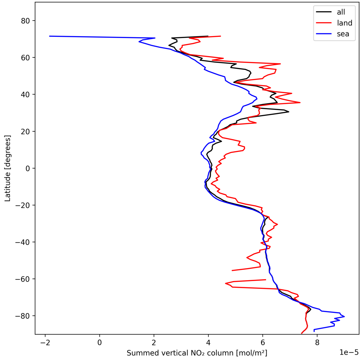
Figure 23: Zonal average of “Summed vertical NO 2 column” for 2025-11-08 to 2025-11-10.
