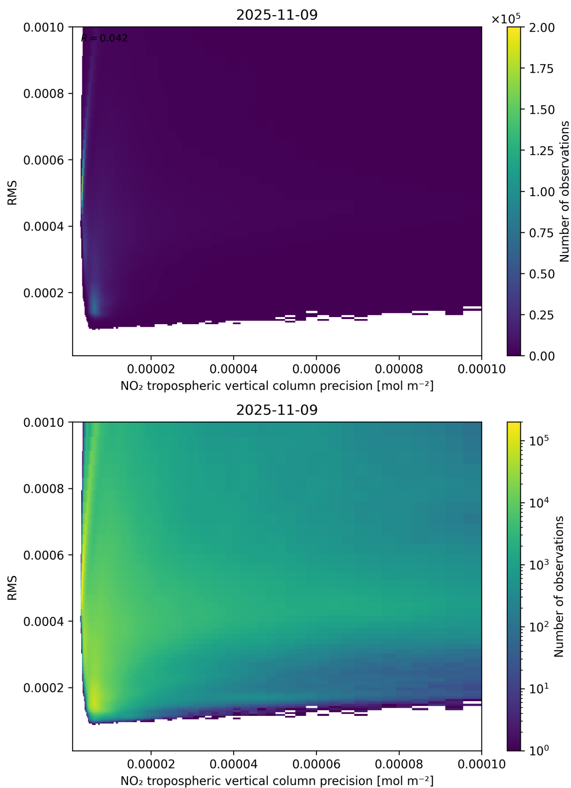
Figure 140: Scatter density plot of “NO 2 tropospheric vertical column precision” against “RMS” for 2025-11-08 to 2025-11-10.
