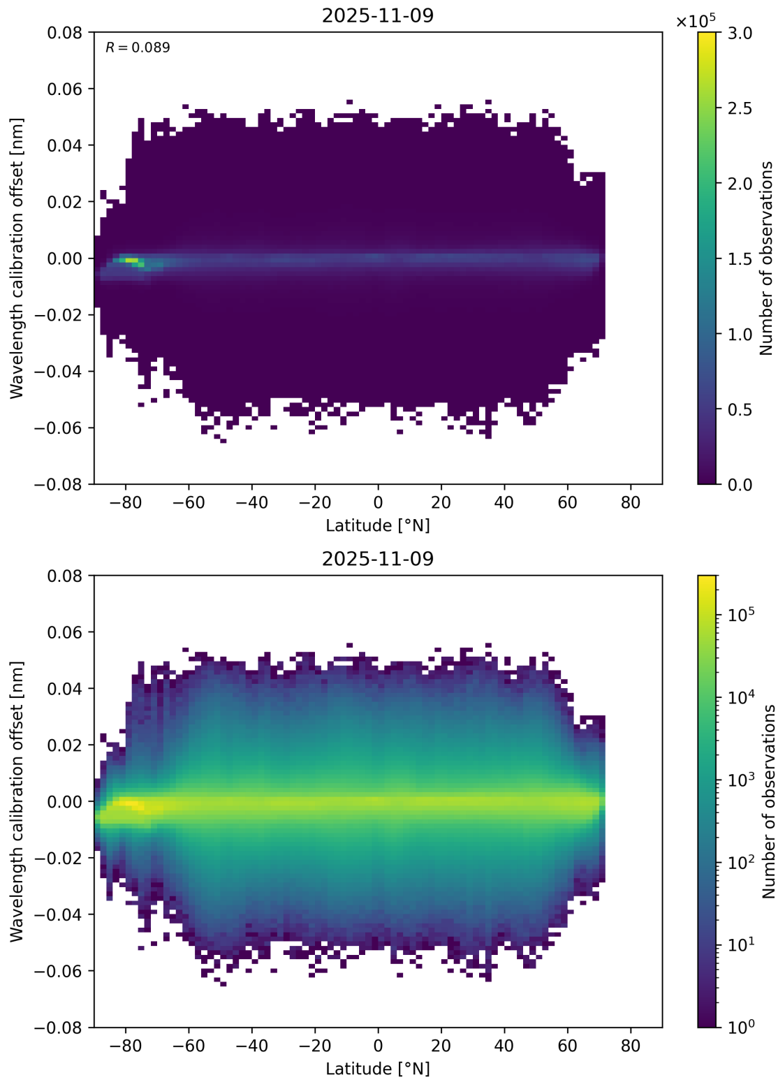
Figure 95: Scatter density plot of “Latitude” against “Wavelength calibration offset” for 2025-11-08 to 2025-11-10.
