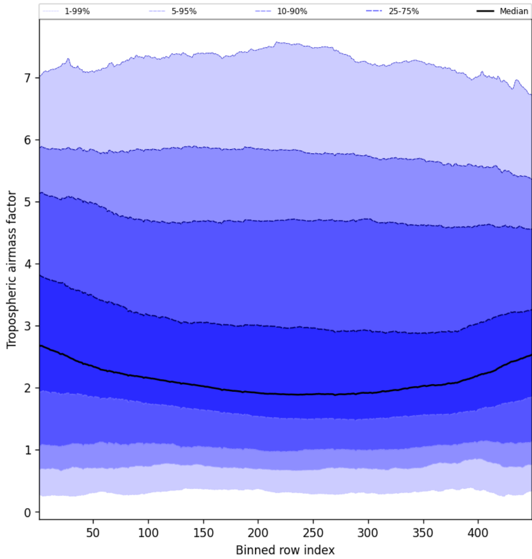
Figure 48: Along track statistics of “Tropospheric airmass factor” for 2025-11-08 to 2025-11-10
