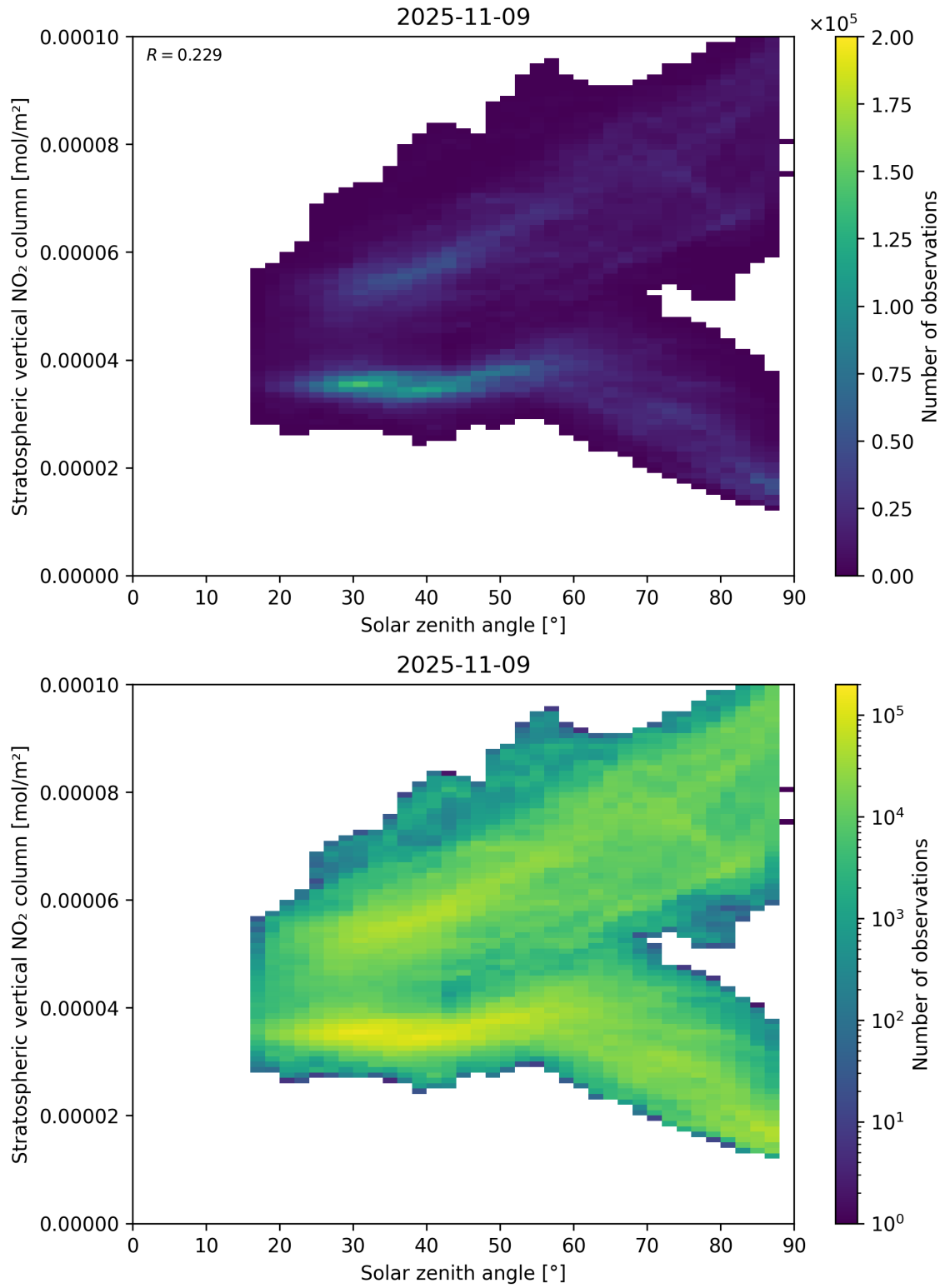
Figure 150: Scatter density plot of “Solar zenith angle” against “Stratospheric vertical NO 2 column” for 2025-11-08 to 2025-11-10.
