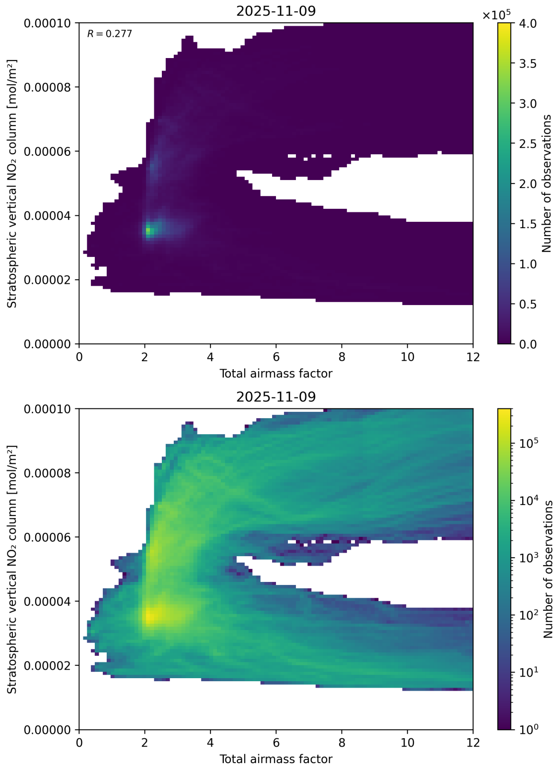
Figure 64: Scatter density plot of “Total airmass factor” against “Stratospheric vertical NO 2 column” for 2025-11-08 to 2025-11-10.
