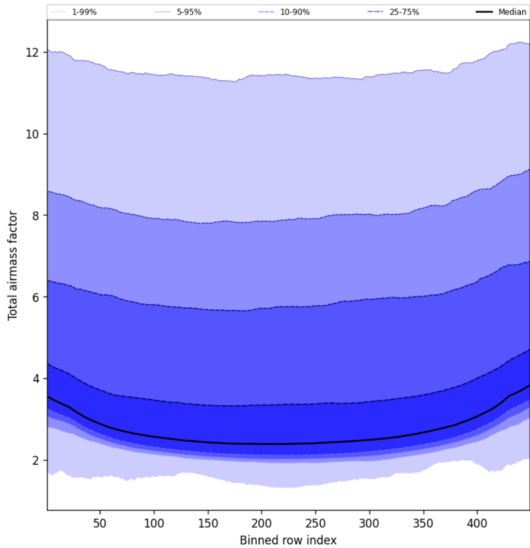
Figure 49: Along track statistics of “Total airmass factor” for 2025-11-08 to 2025-11-10
