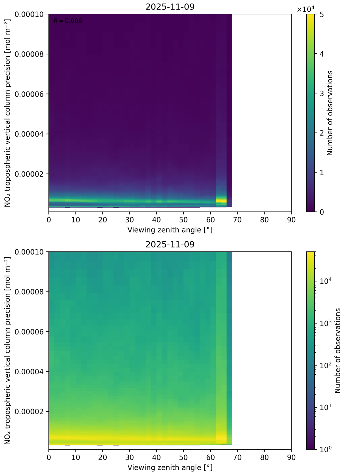
Figure 170: Scatter density plot of “Viewing zenith angle” against “NO 2 tropospheric vertical column precision” for 2025-11-08 to 2025-11-10.
