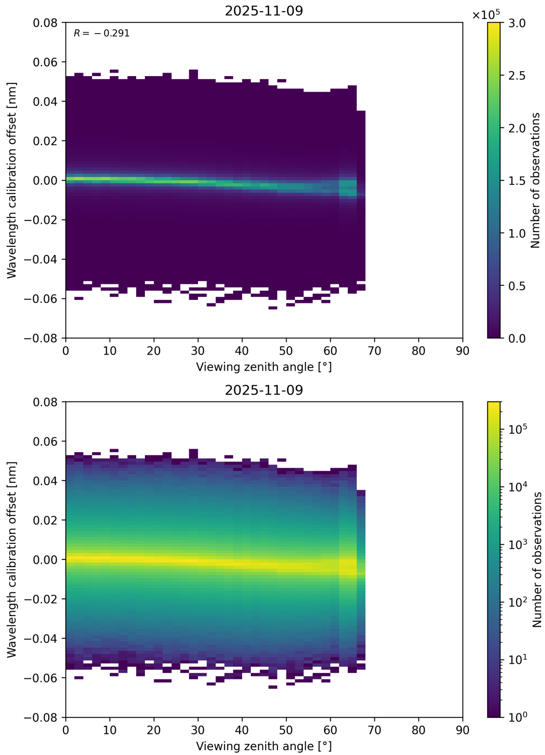
Figure 173: Scatter density plot of “Viewing zenith angle” against “Wavelength calibration offset” for 2025-11-08 to 2025-11-10.
