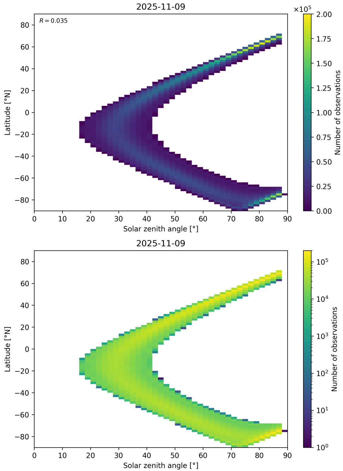
Figure 149: Scatter density plot of “Solar zenith angle” against “Latitude” for 2025-11-08 to 2025-11-10.
