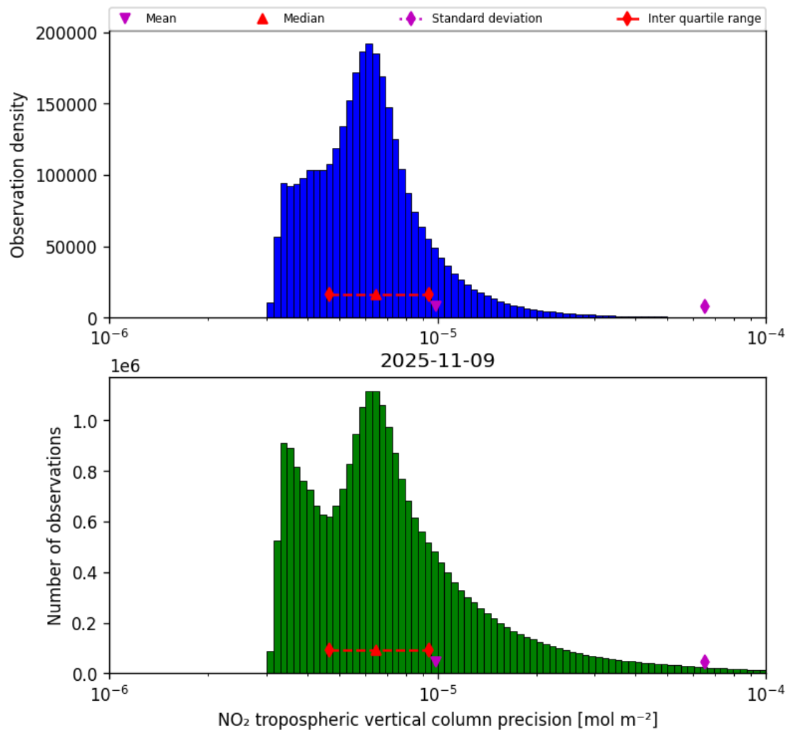
Figure 30: Histogram of “NO 2 tropospheric vertical column precision” for 2025-11-08 to 2025-11-10
