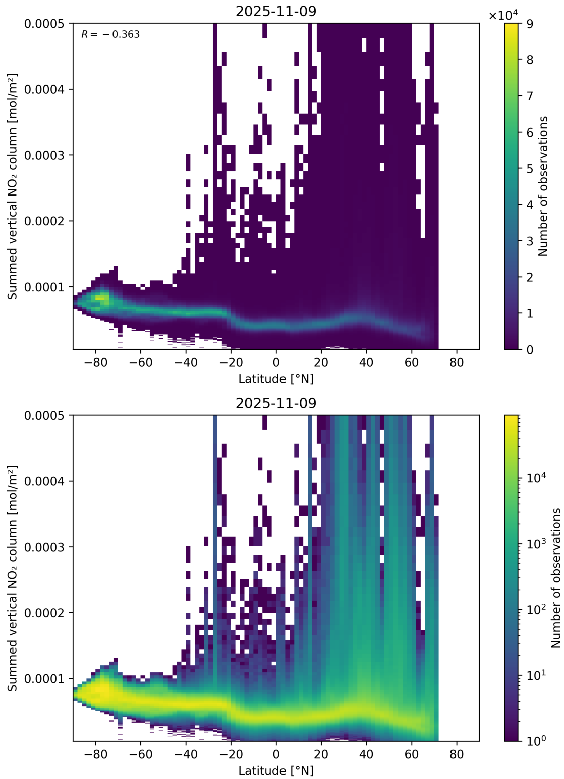
Figure 88: Scatter density plot of “Latitude” against “Summed vertical NO 2 column” for 2025-11-08 to 2025-11-10.
