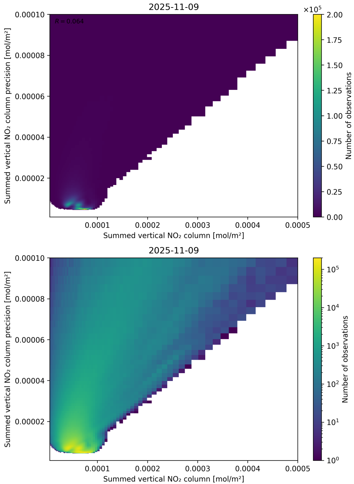
Figure 105: Scatter density plot of “Summed vertical NO 2 column” against “Summed vertical NO 2 column precision” for 2025-11-08 to 2025-11-10.
