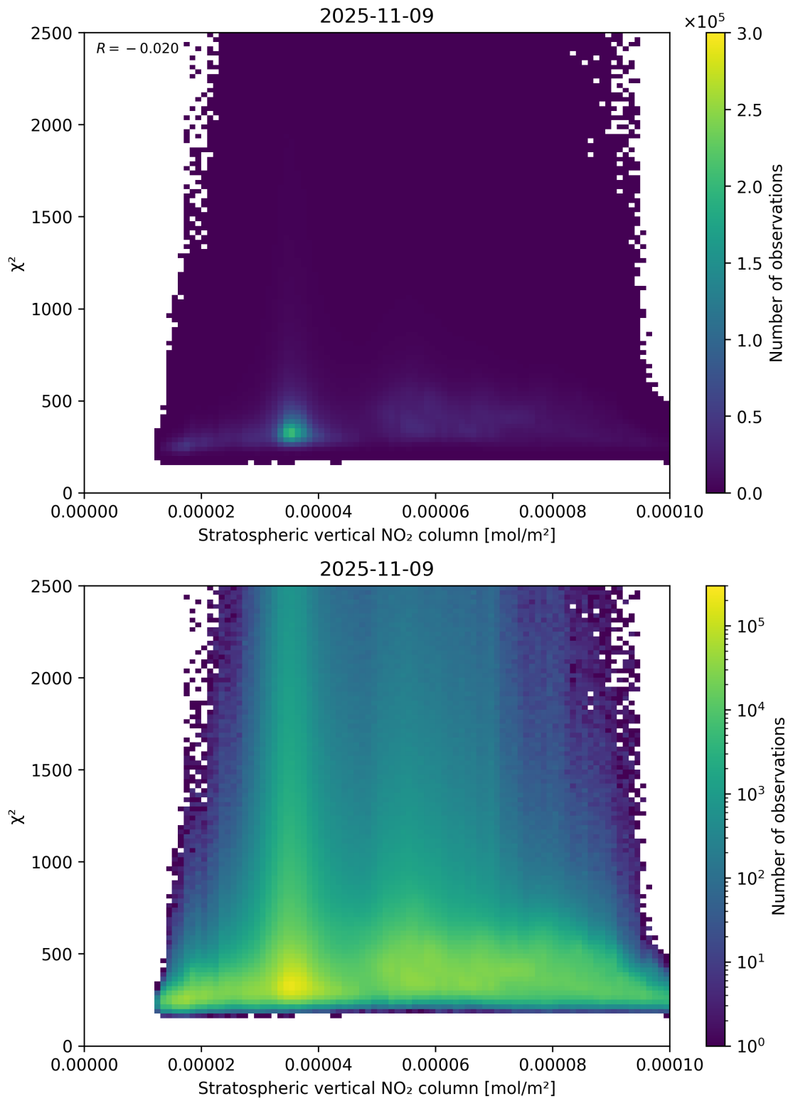
Figure 97: Scatter density plot of “Stratospheric vertical NO 2 column” against “ \chi^2 ” for 2025-11-08 to 2025-11-10.
