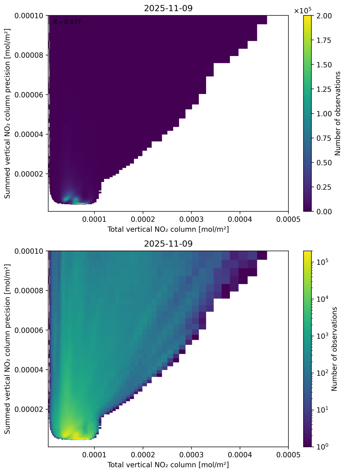
Figure 113: Scatter density plot of “Total vertical NO 2 column” against “Summed vertical NO 2 column precision” for 2025-11-08 to 2025-11-10.
