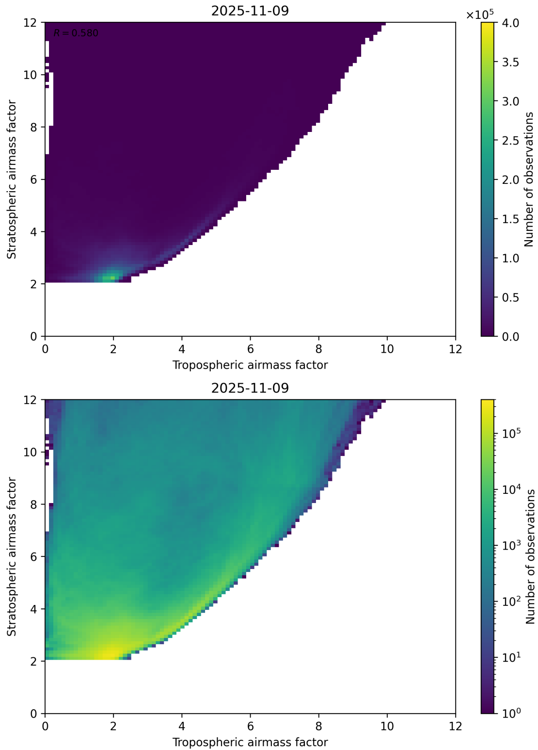
Figure 71: Scatter density plot of “Tropospheric airmass factor” against “Stratospheric airmass factor” for 2025-11-08 to 2025-11-10.
