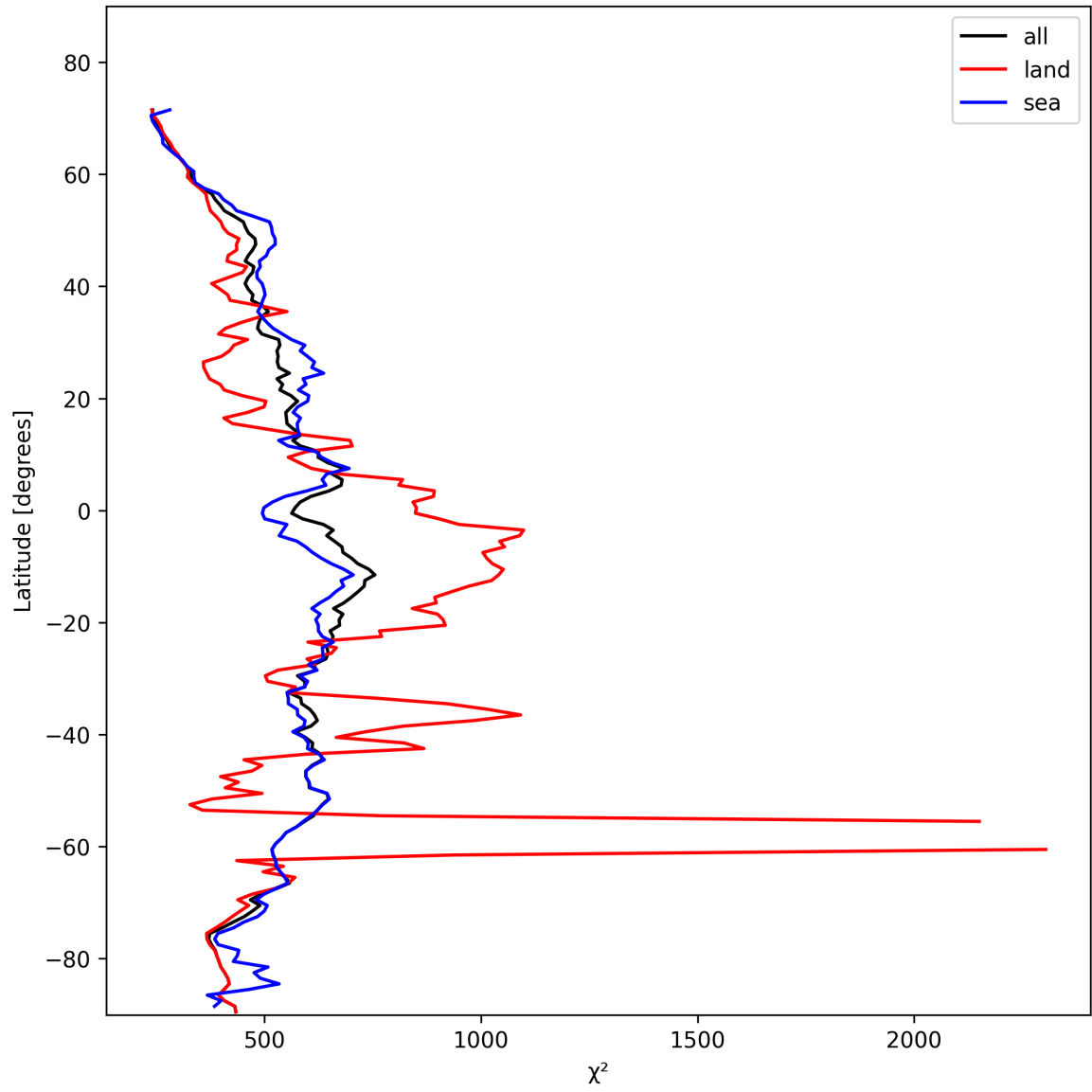
Figure 25: Zonal average of “ \chi^2 ” for 2025-11-08 to 2025-11-10.
