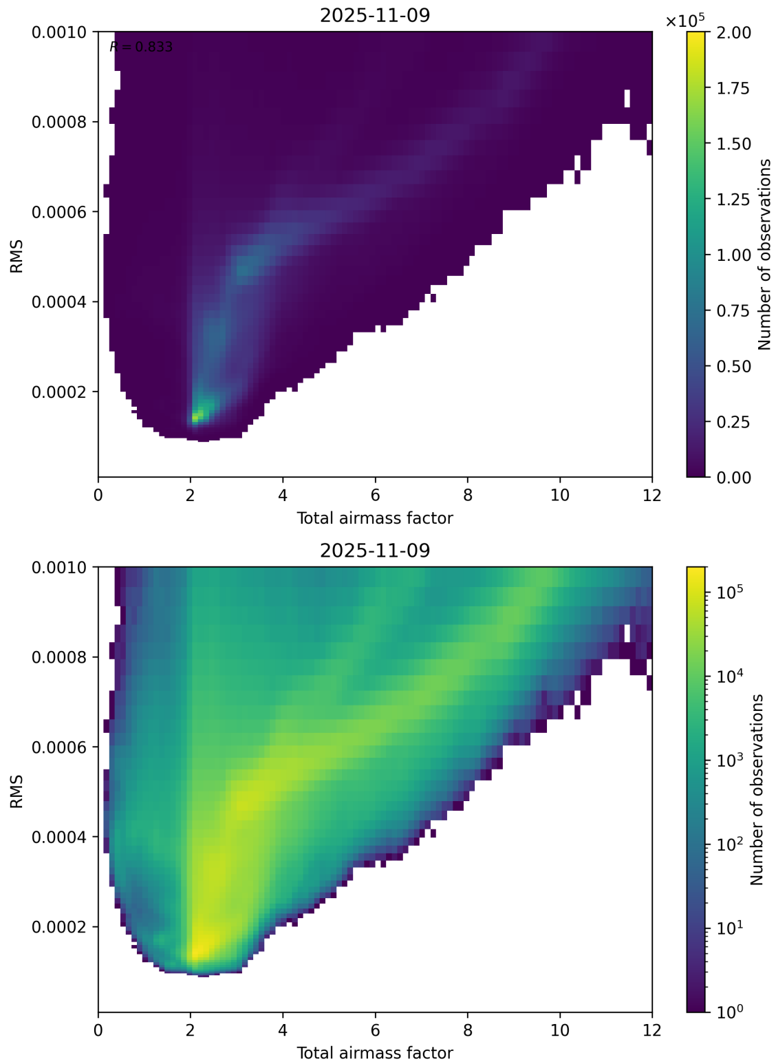
Figure 69: Scatter density plot of “Total airmass factor” against “RMS” for 2025-11-08 to 2025-11-10.
