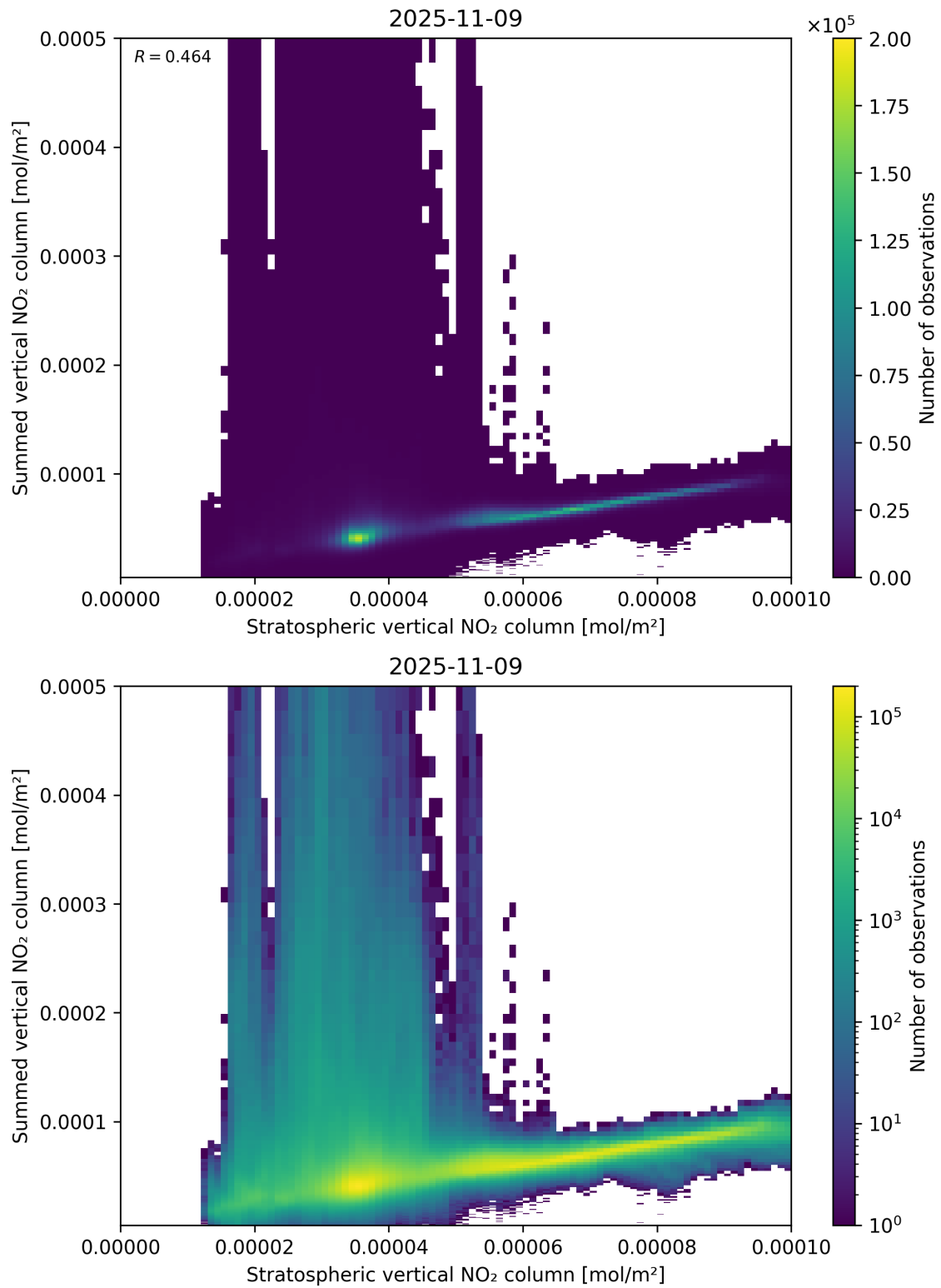
Figure 98: Scatter density plot of “Stratospheric vertical NO 2 column” against “Summed vertical NO 2 column” for 2025-11-08 to 2025-11-10.
