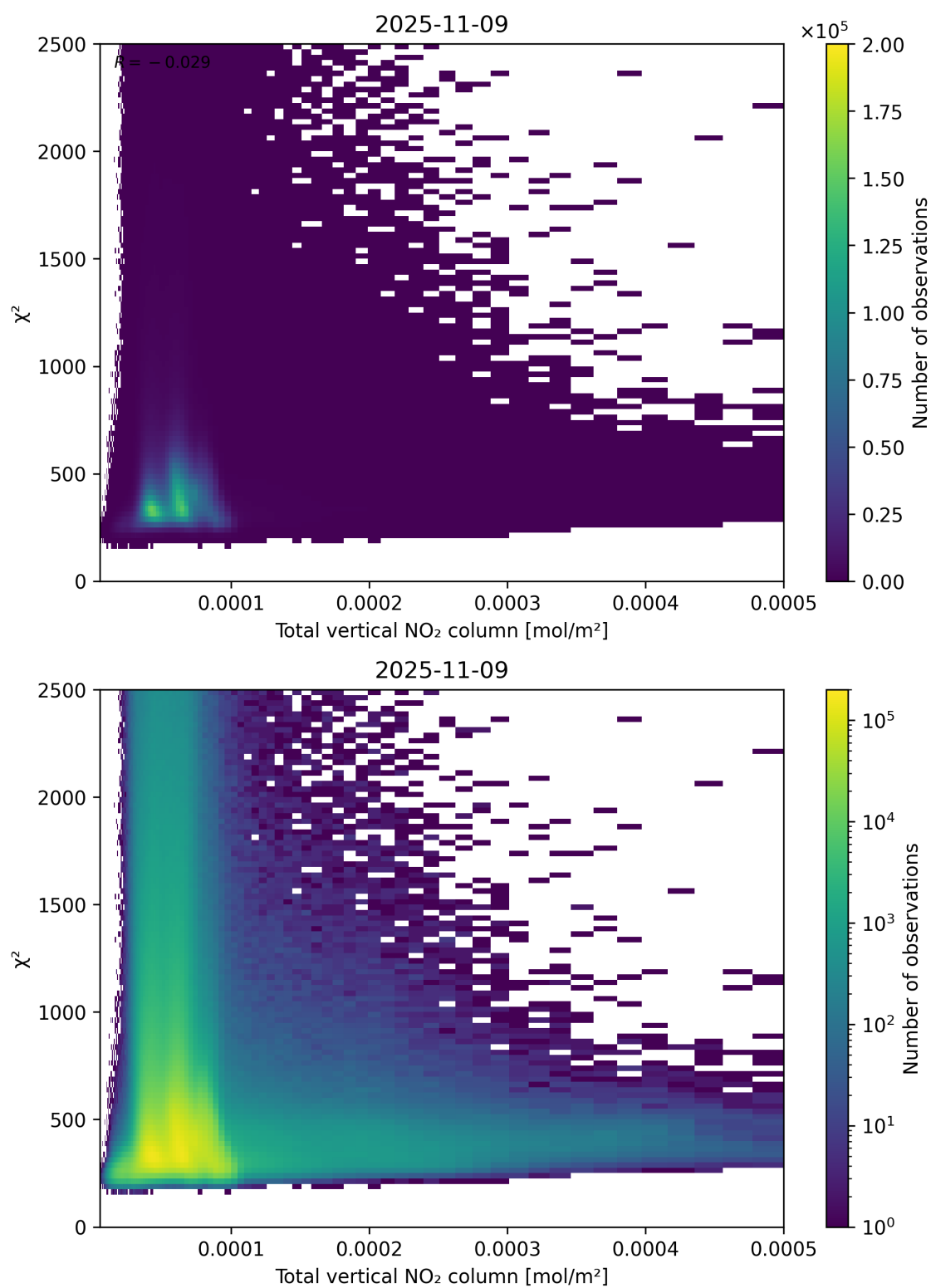
Figure 111: Scatter density plot of “Total vertical NO 2 column” against “ \chi^2 ” for 2025-11-08 to 2025-11-10.
