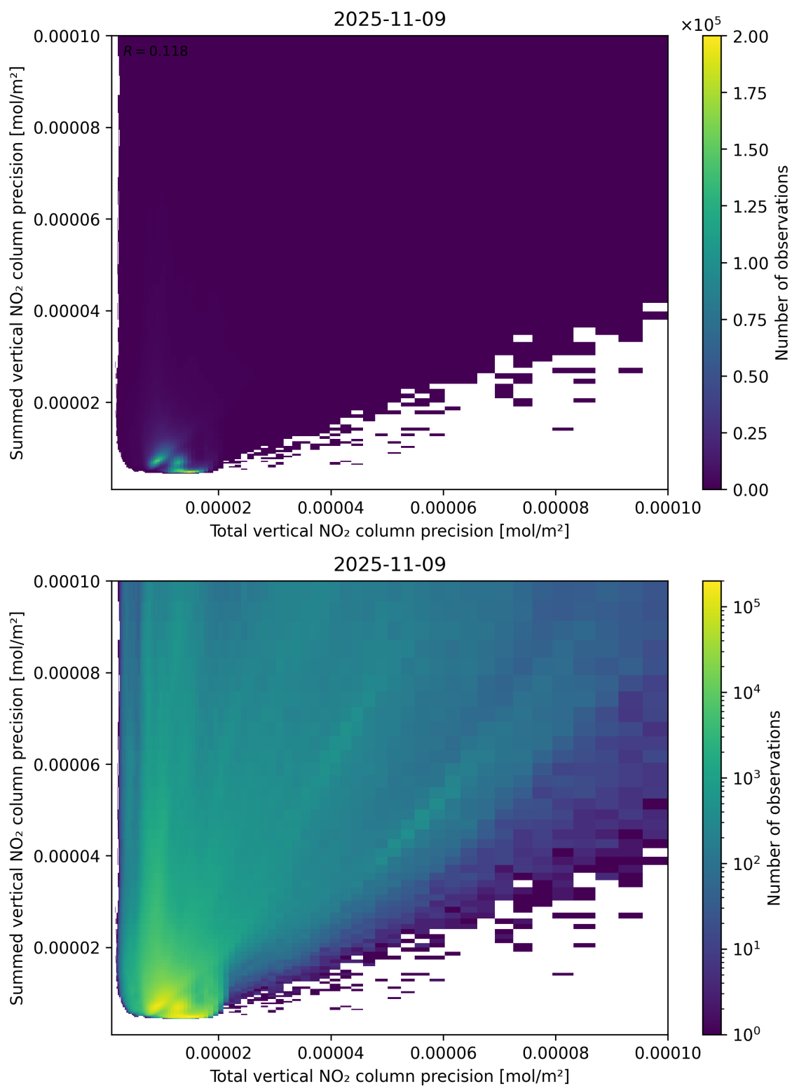
Figure 118: Scatter density plot of “Total vertical NO 2 column precision” against “Summed vertical NO 2 column precision” for 2025-11-08 to 2025-11-10.
