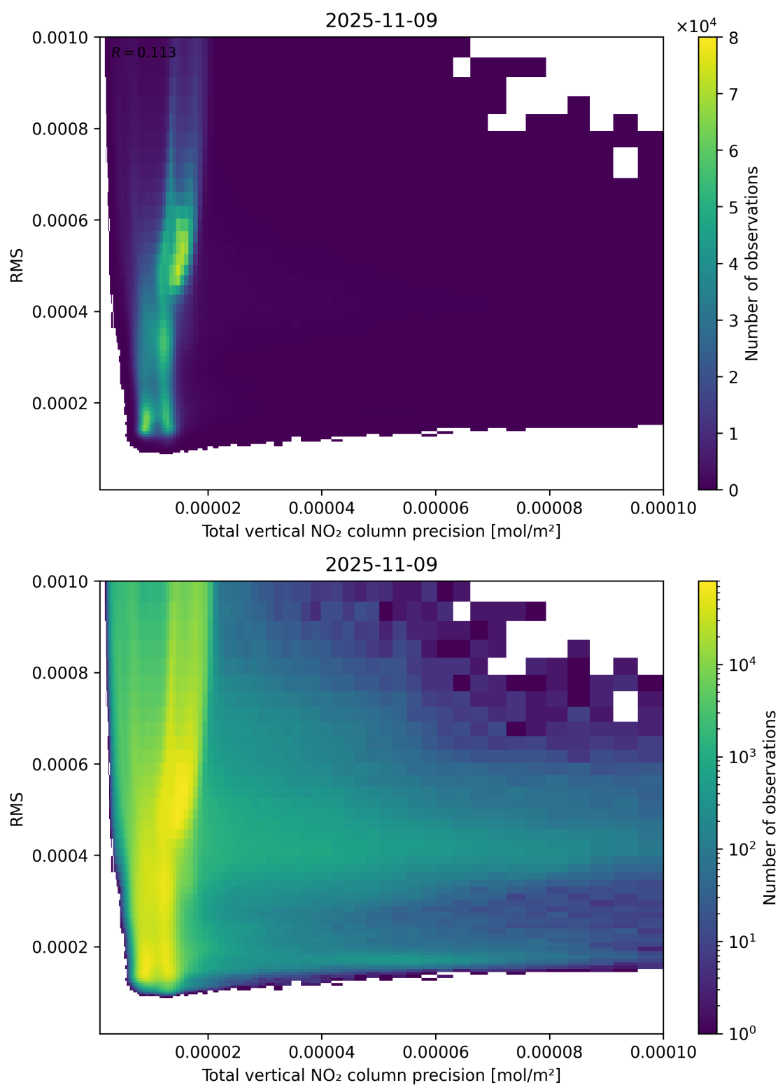
Figure 119: Scatter density plot of “Total vertical NO 2 column precision” against “RMS” for 2025-11-08 to 2025-11-10.
