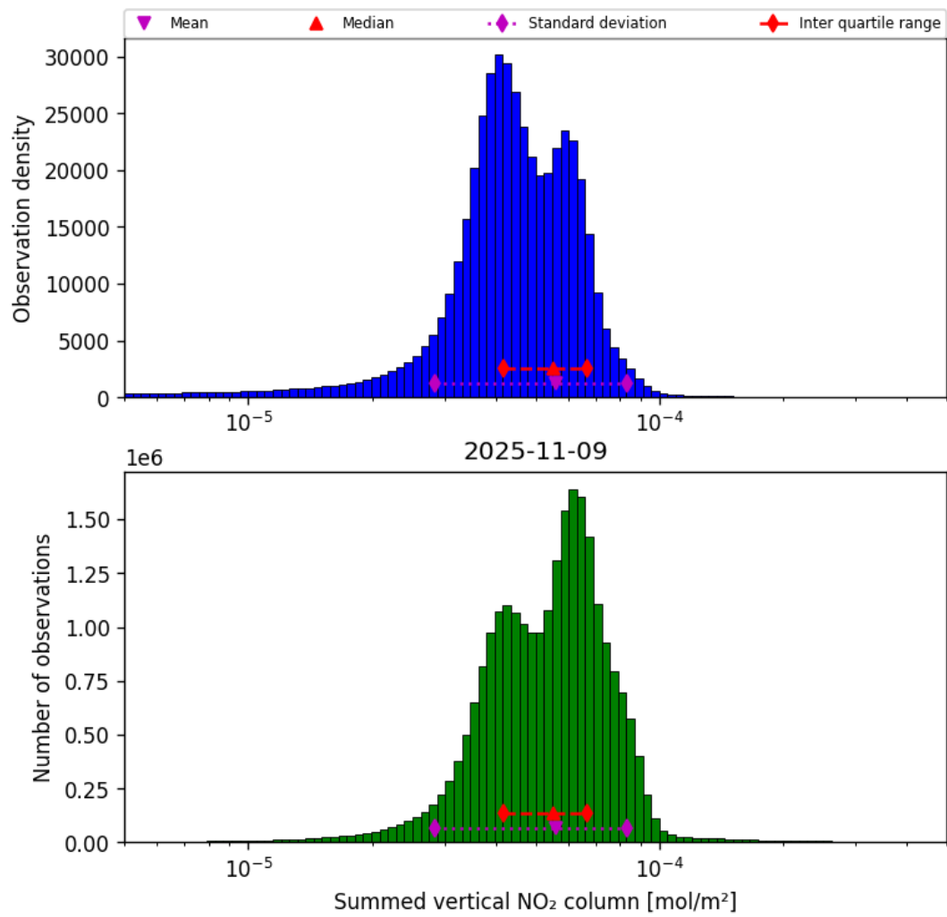
Figure 40: Histogram of “Summed vertical NO 2 column” for 2025-11-08 to 2025-11-10
