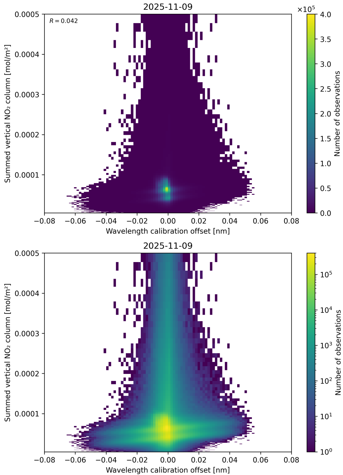
Figure 177: Scatter density plot of “Wavelength calibration offset” against “Summed vertical NO 2 column” for 2025-11-08 to 2025-11-10.
