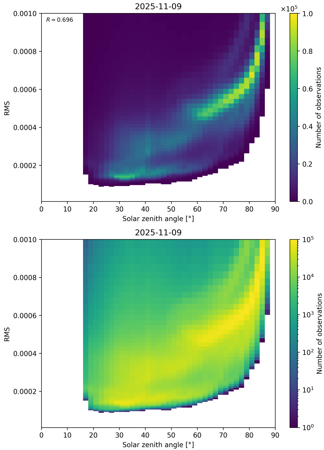
Figure 157: Scatter density plot of “Solar zenith angle” against “RMS” for 2025-11-08 to 2025-11-10.
