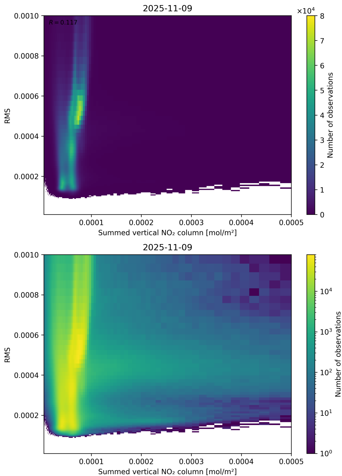
Figure 109: Scatter density plot of “Summed vertical NO 2 column” against “RMS” for 2025-11-08 to 2025-11-10.
