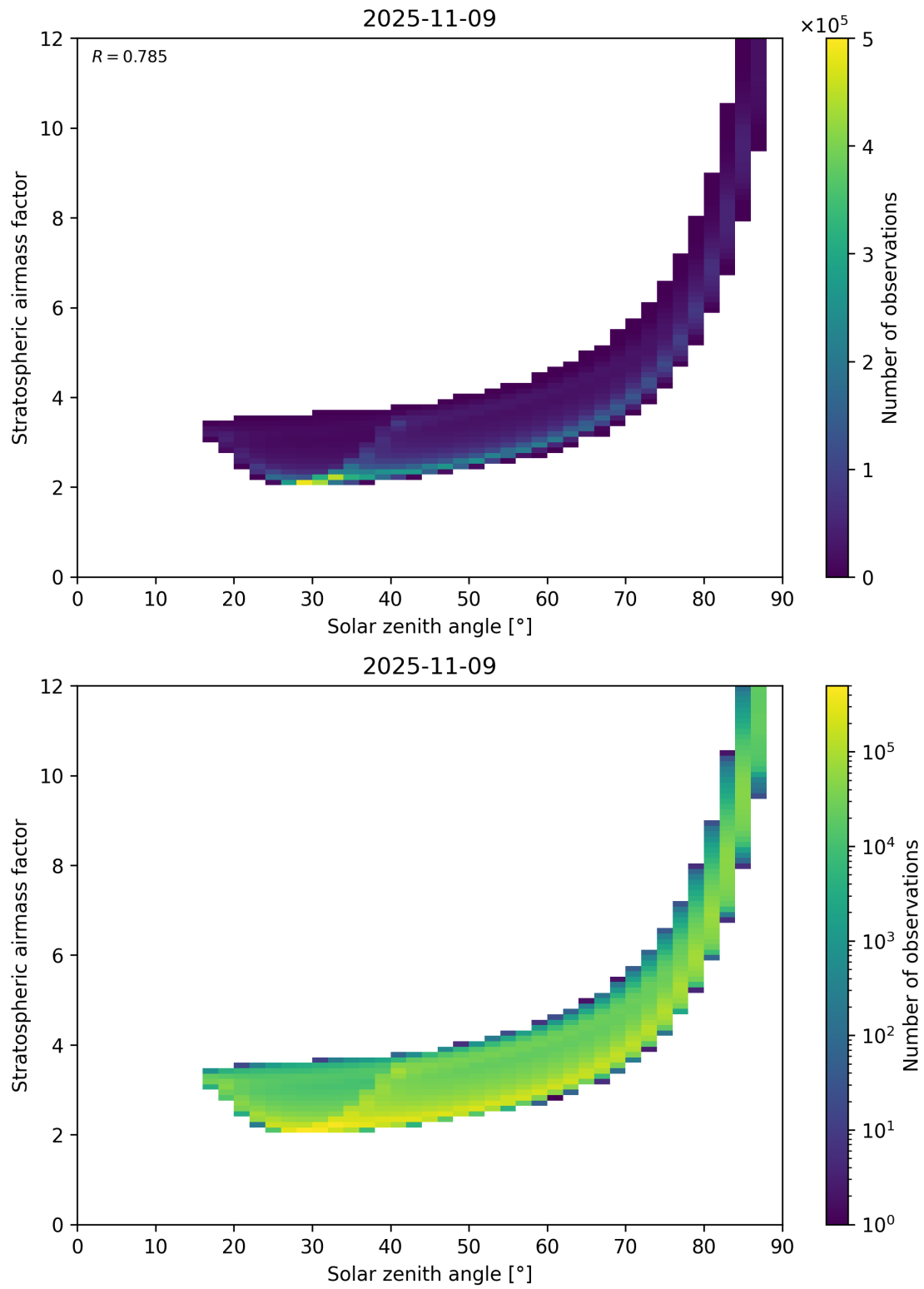
Figure 145: Scatter density plot of “Solar zenith angle” against “Stratospheric airmass factor” for 2025-11-08 to 2025-11-10.
