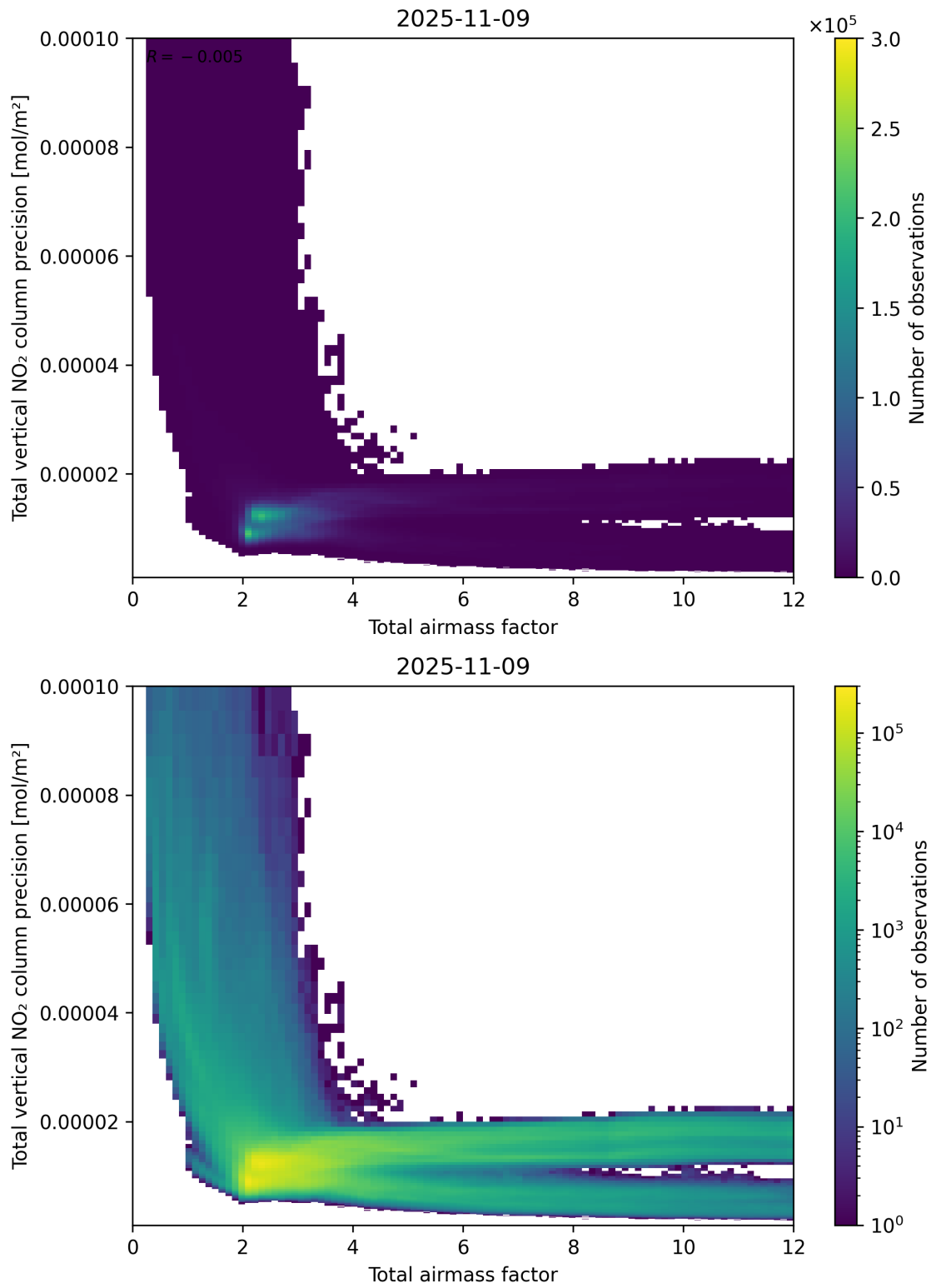
Figure 68: Scatter density plot of “Total airmass factor” against “Total vertical NO 2 column precision” for 2025-11-08 to 2025-11-10.
