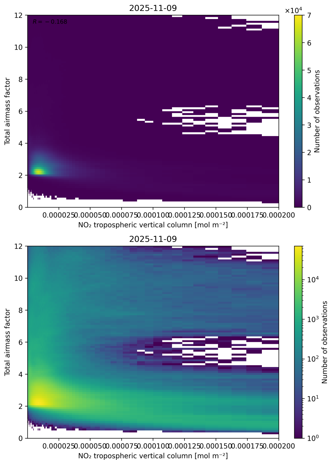
Figure 122: Scatter density plot of “NO 2 tropospheric vertical column” against “Total airmass factor” for 2025-11-08 to 2025-11-10.
