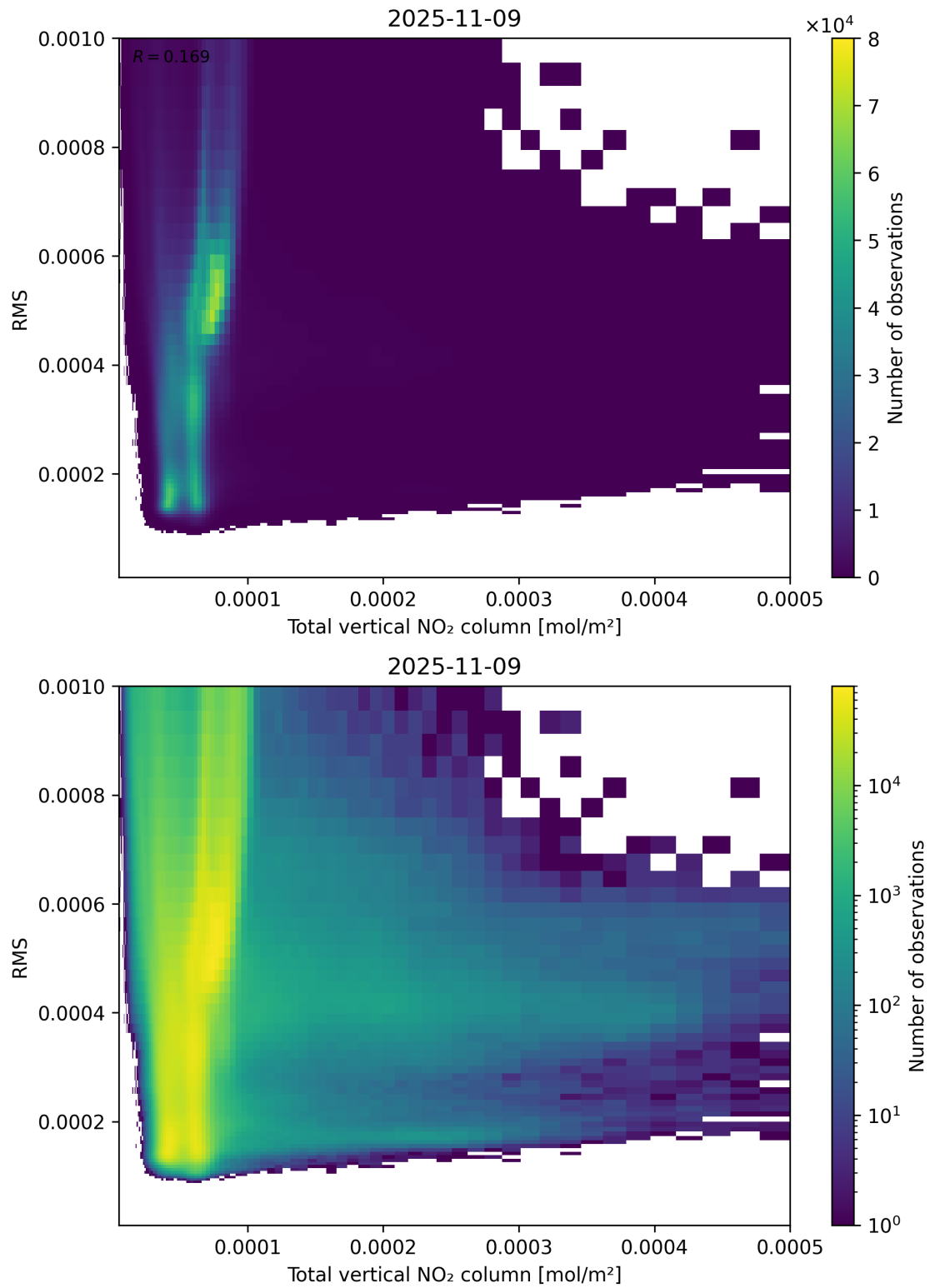
Figure 120: Scatter density plot of “Total vertical NO 2 column” against “RMS” for 2025-11-08 to 2025-11-10.
