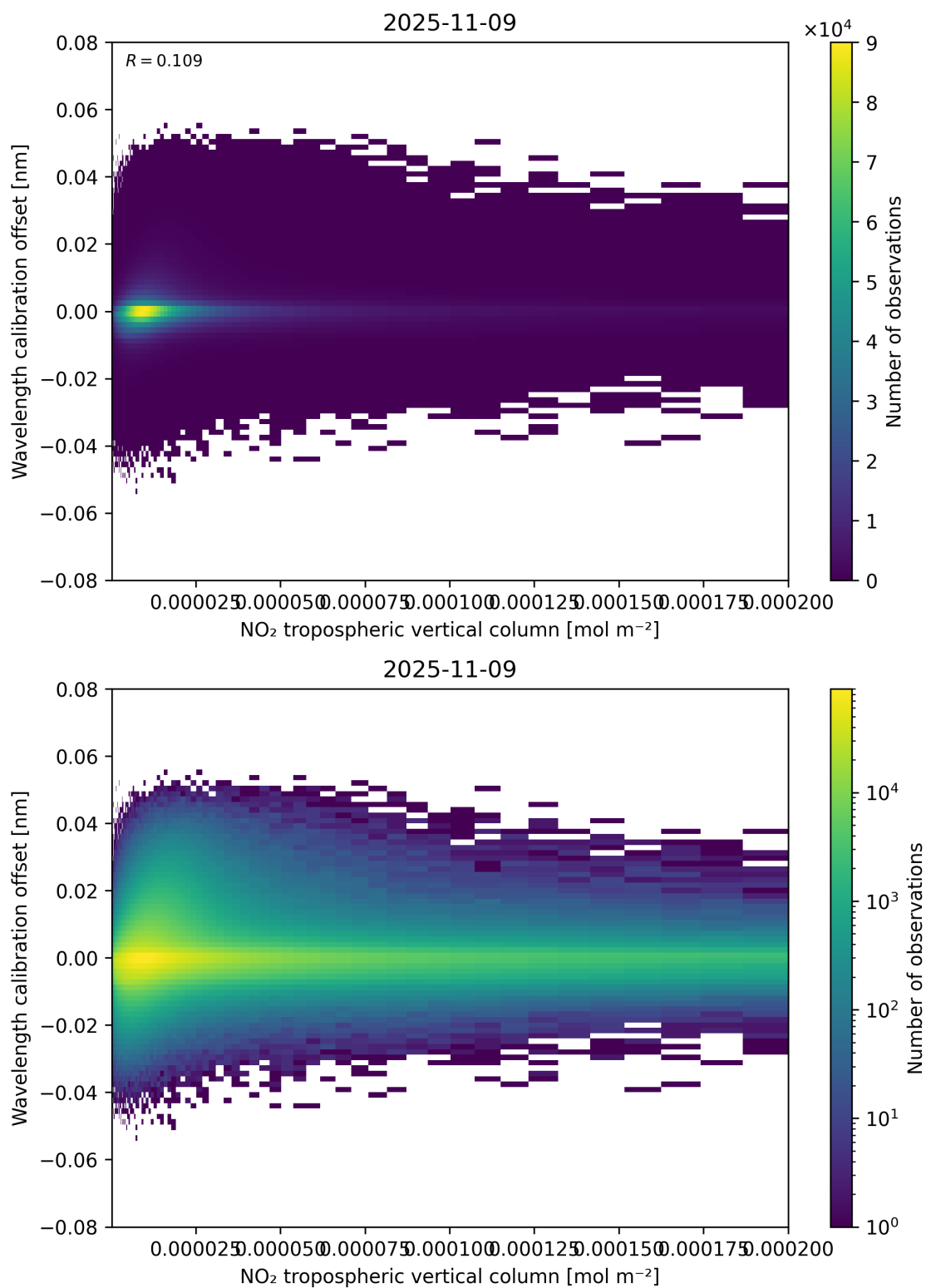
Figure 143: Scatter density plot of “NO 2 tropospheric vertical column” against “Wavelength calibration offset” for 2025-11-08 to 2025-11-10.
