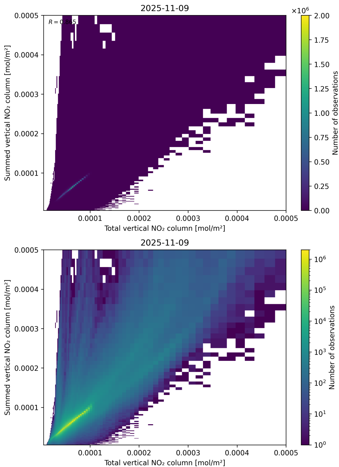
Figure 112: Scatter density plot of “Total vertical NO 2 column” against “Summed vertical NO 2 column” for 2025-11-08 to 2025-11-10.
