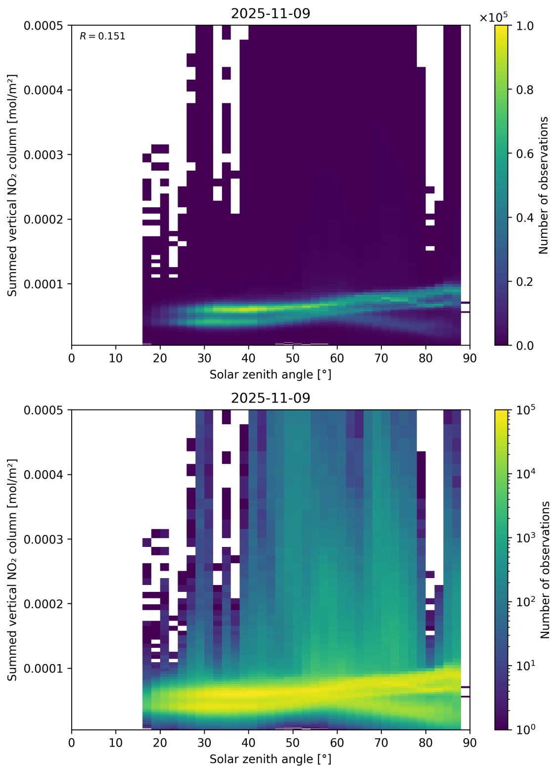
Figure 151: Scatter density plot of “Solar zenith angle” against “Summed vertical NO 2 column” for 2025-11-08 to 2025-11-10.
