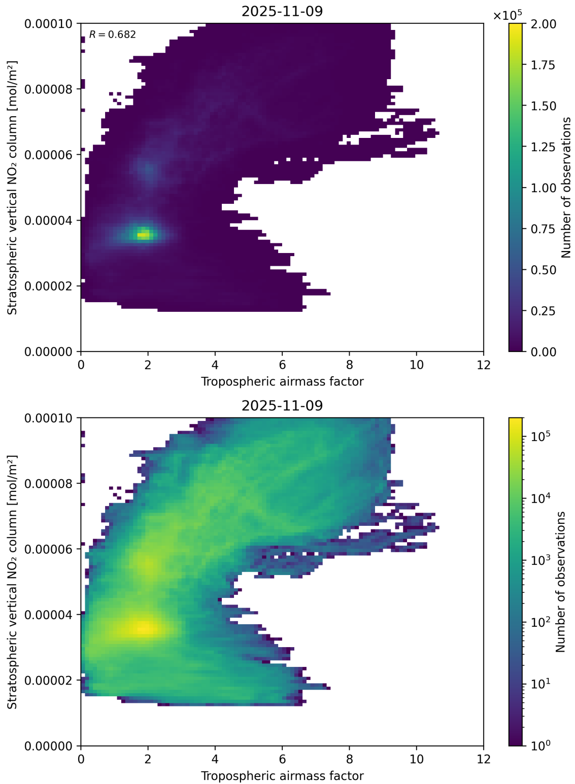
Figure 74: Scatter density plot of “Tropospheric air mass factor” against “Stratospheric vertical NO 2 column” for 2025-11-08 to 2025-11-10.
