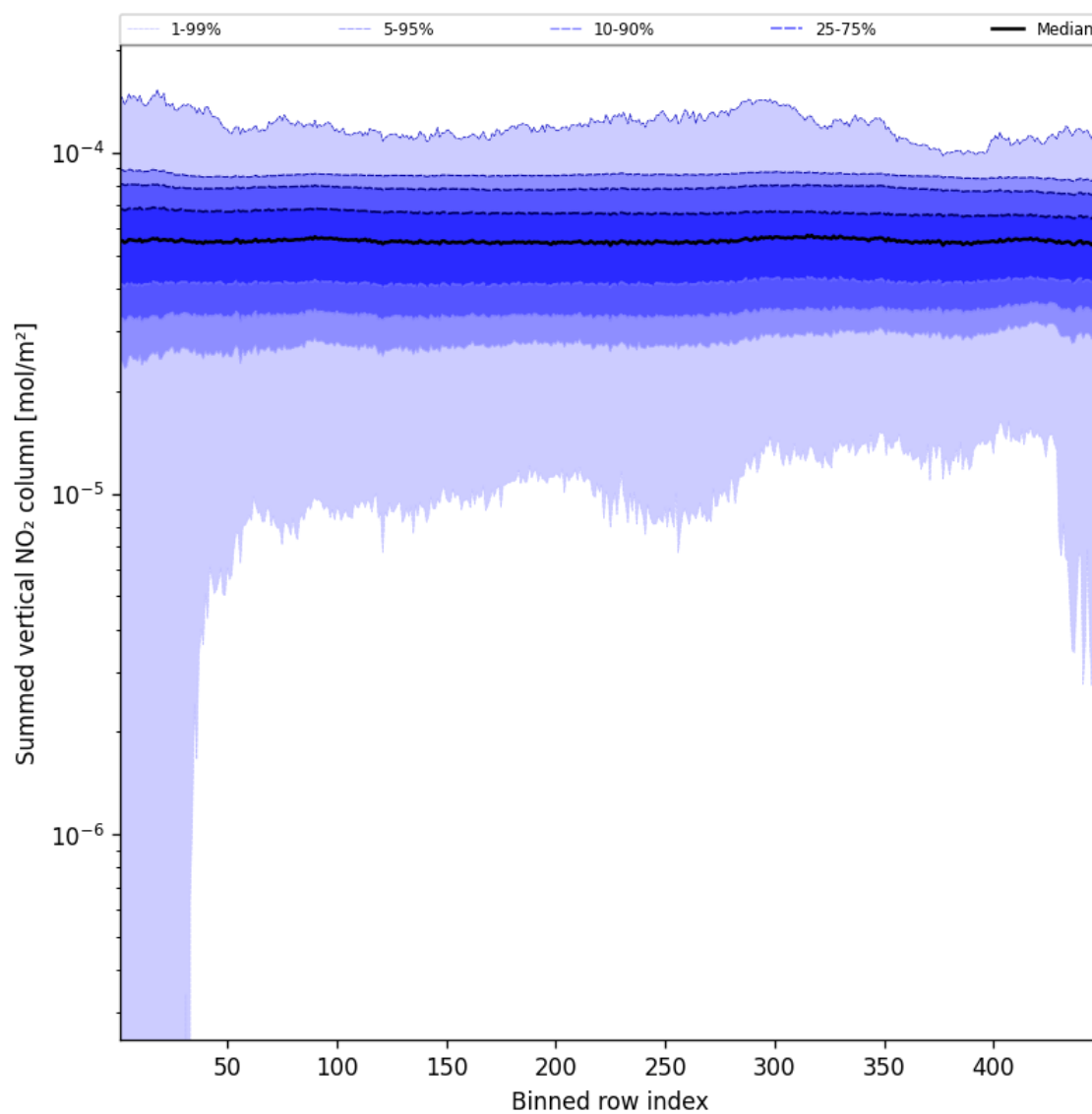
Figure 57: Along track statistics of “Summed vertical NO 2 column” for 2025-11-08 to 2025-11-10
