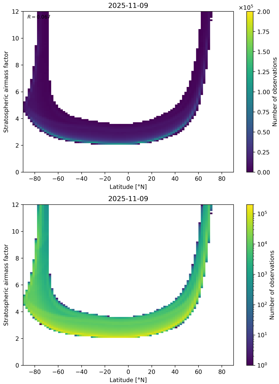
Figure 83: Scatter density plot of “Latitude” against “Stratospheric air mass factor” for 2025-11-08 to 2025-11-10.
