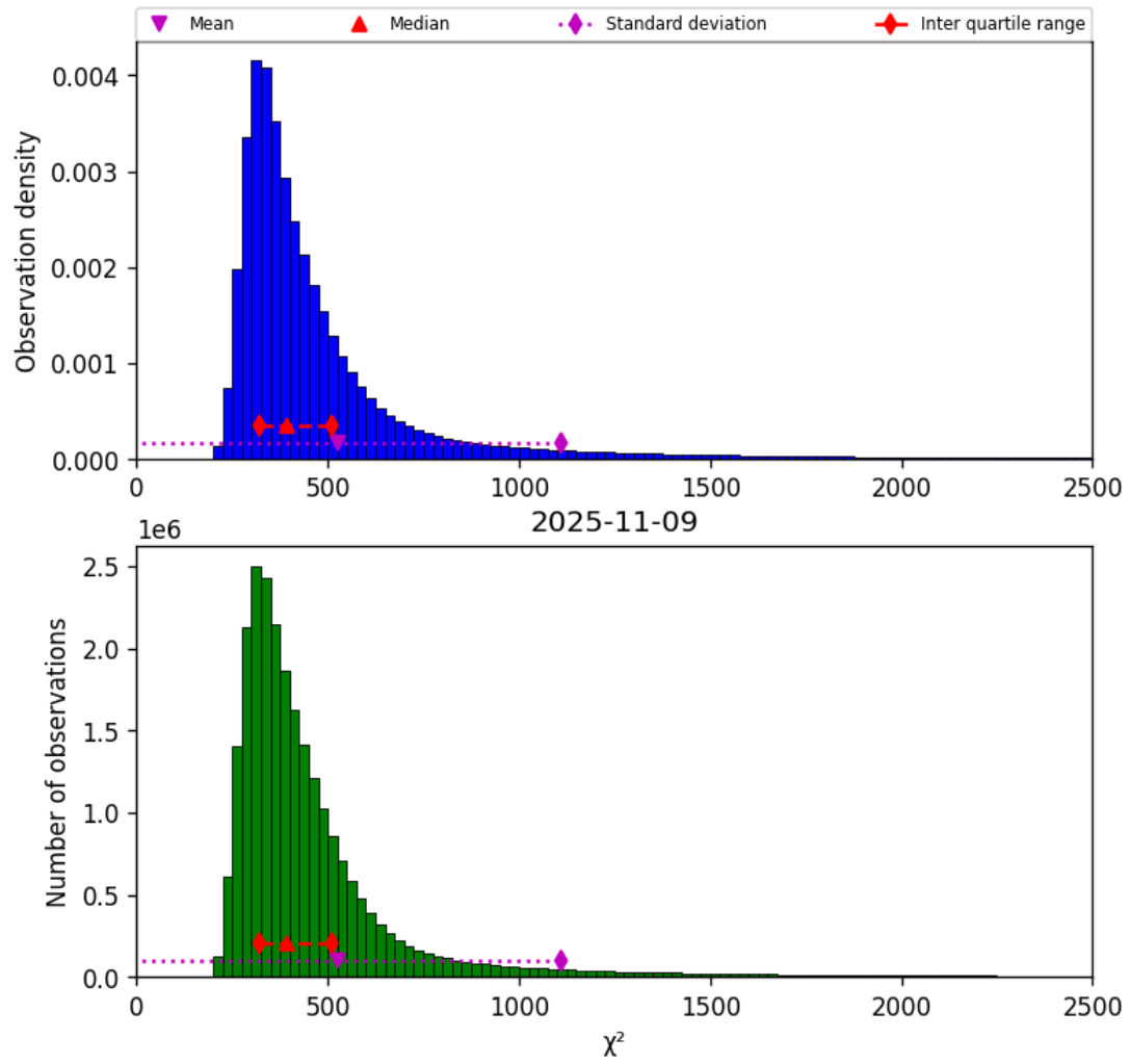
Figure 42: Histogram of “ \chi^2 ” for 2025-11-08 to 2025-11-10
