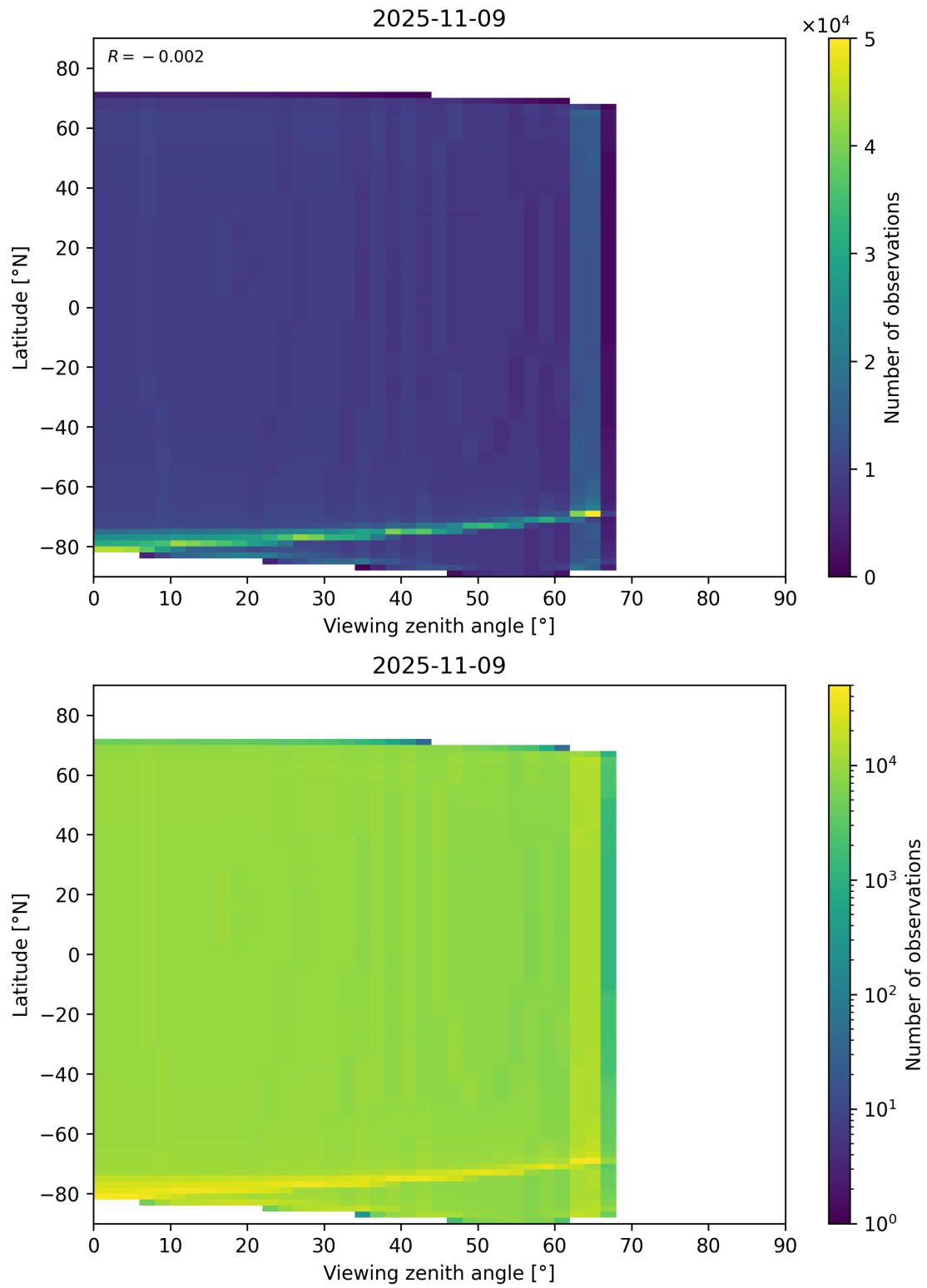
Figure 163: Scatter density plot of “Viewing zenith angle” against “Latitude” for 2025-11-08 to 2025-11-10.
