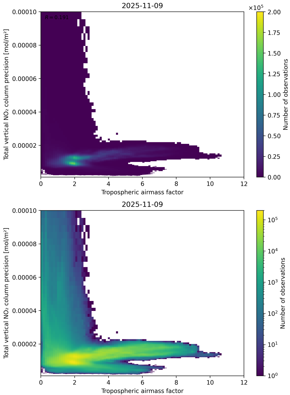
Figure 78: Scatter density plot of “Tropospheric air mass factor” against “Total vertical NO 2 column precision” for 2025-11-08 to 2025-11-10.
