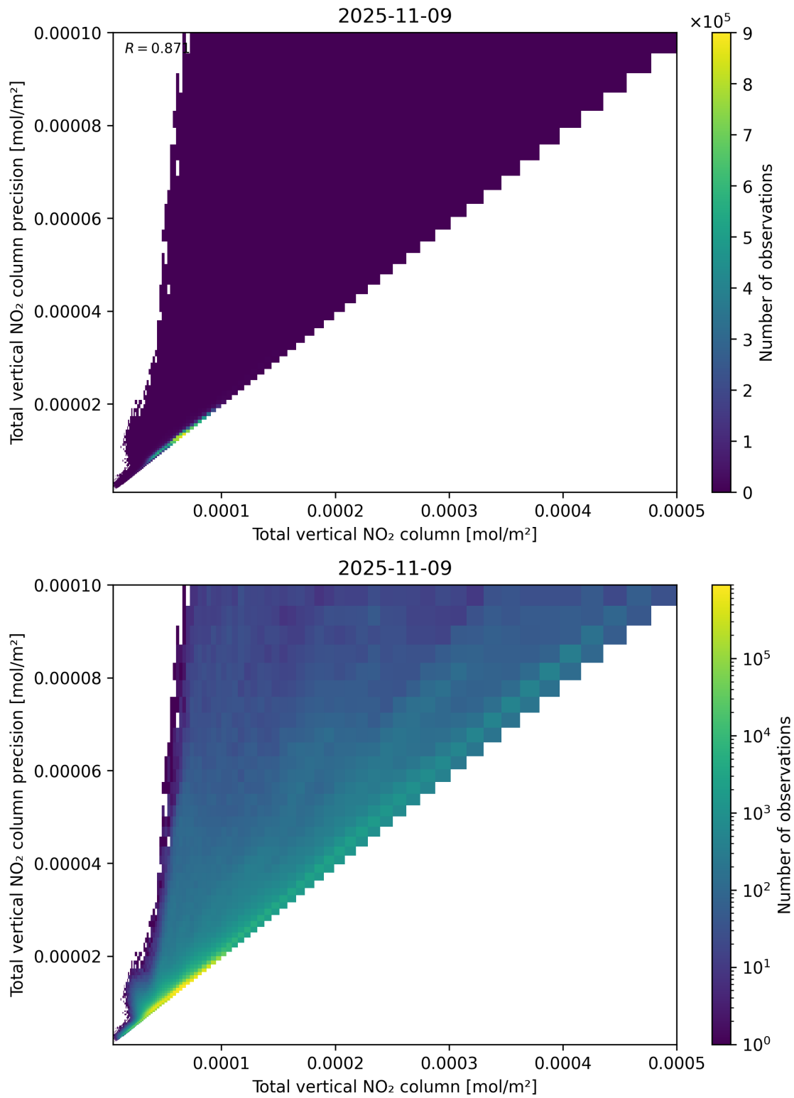
Figure 114: Scatter density plot of “Total vertical NO 2 column” against “Total vertical NO 2 column precision” for 2025-11-08 to 2025-11-10.
