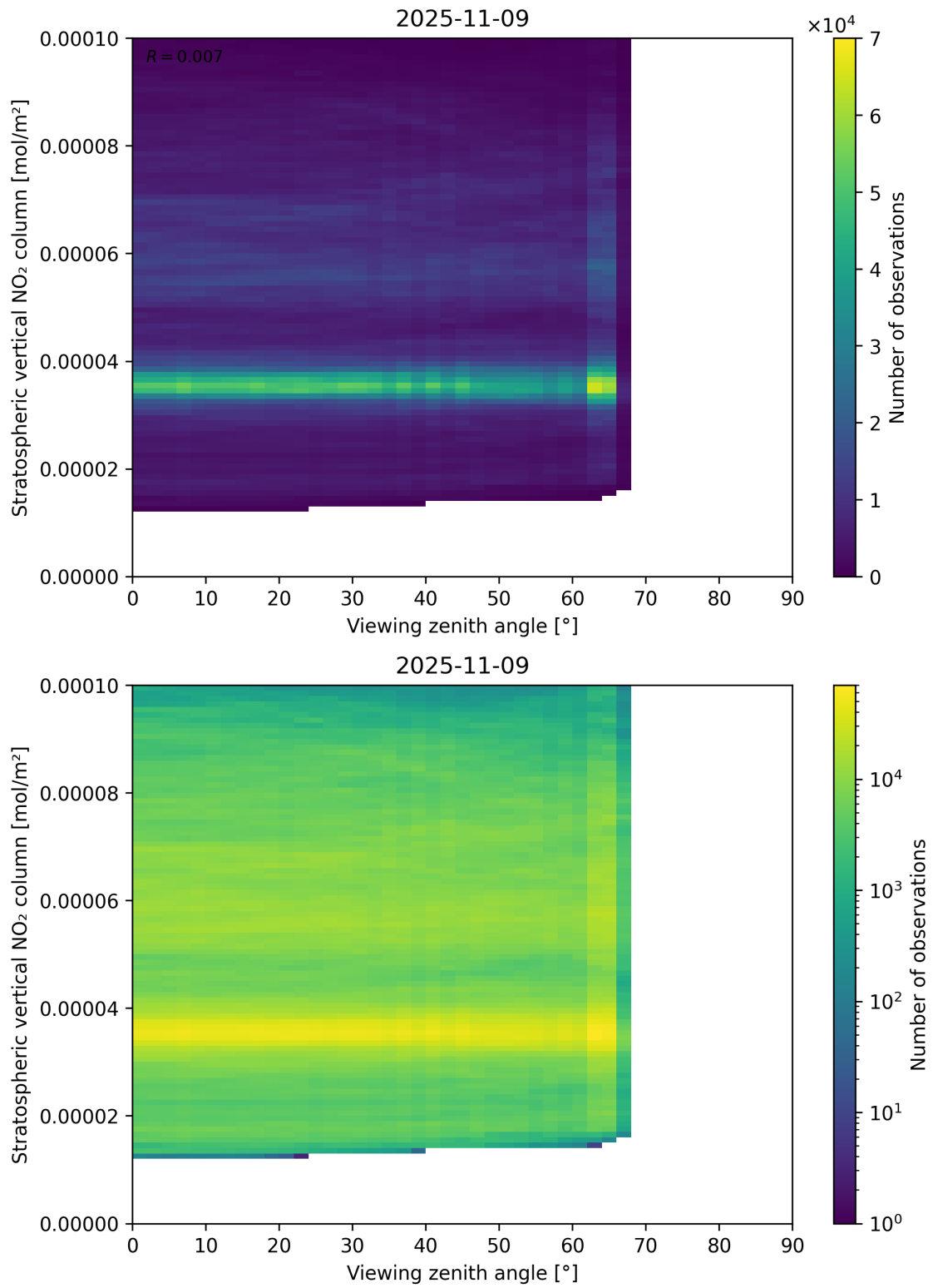
Figure 164: Scatter density plot of “Viewing zenith angle” against “Stratospheric vertical NO 2 column” for 2025-11-08 to 2025-11-10.
