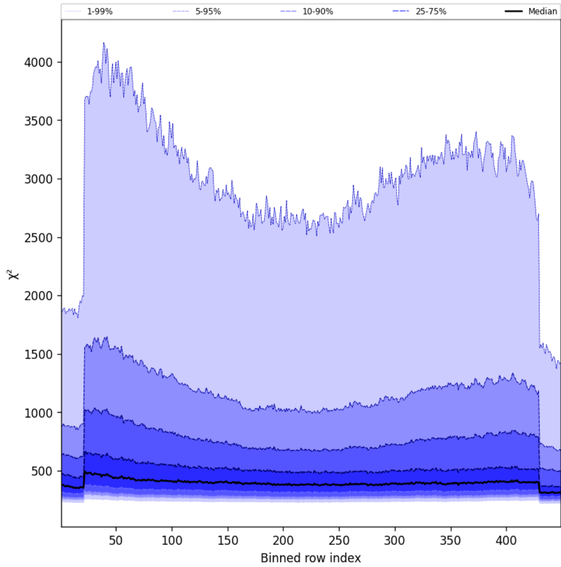
Figure 59: Along track statistics of “ \chi^2 ” for 2025-11-08 to 2025-11-10
