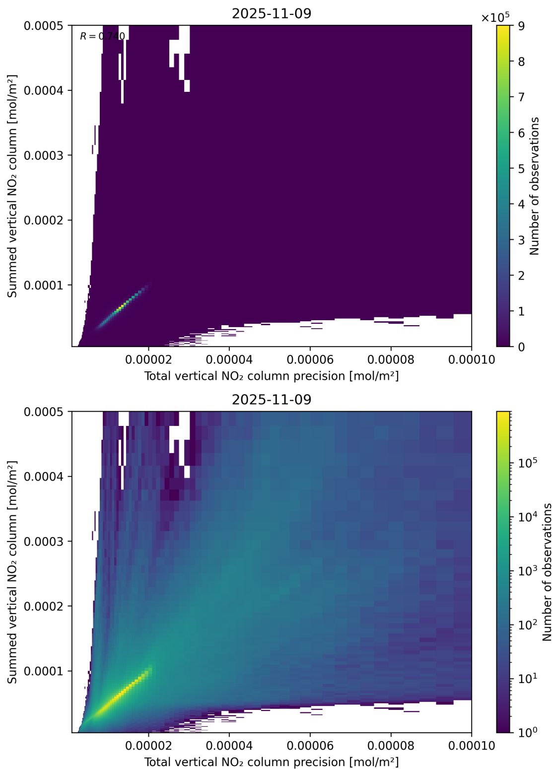
Figure 117: Scatter density plot of “Total vertical NO 2 column precision” against “Summed vertical NO 2 column” for 2025-11-08 to 2025-11-10.
