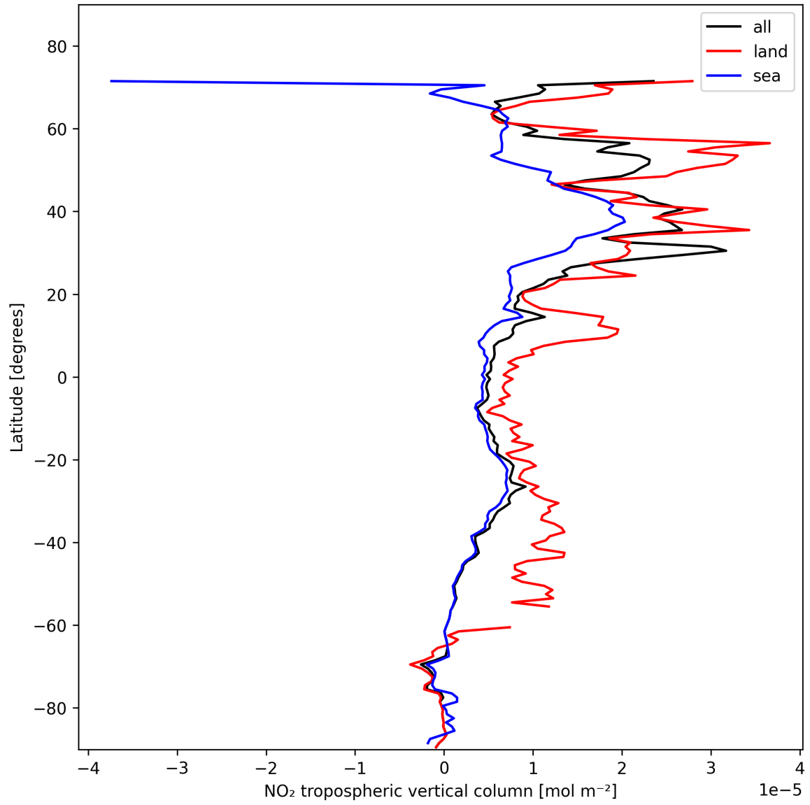
Figure 12: Zonal average of “NO 2 tropospheric vertical column” for 2025-11-08 to 2025-11-10.
