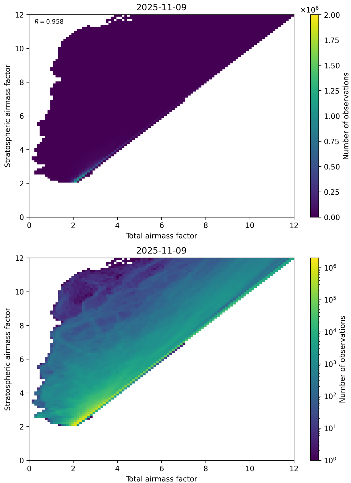
Figure 62: Scatter density plot of “Total airmass factor” against “Stratospheric airmass factor” for 2025-11-08 to 2025-11-10.
