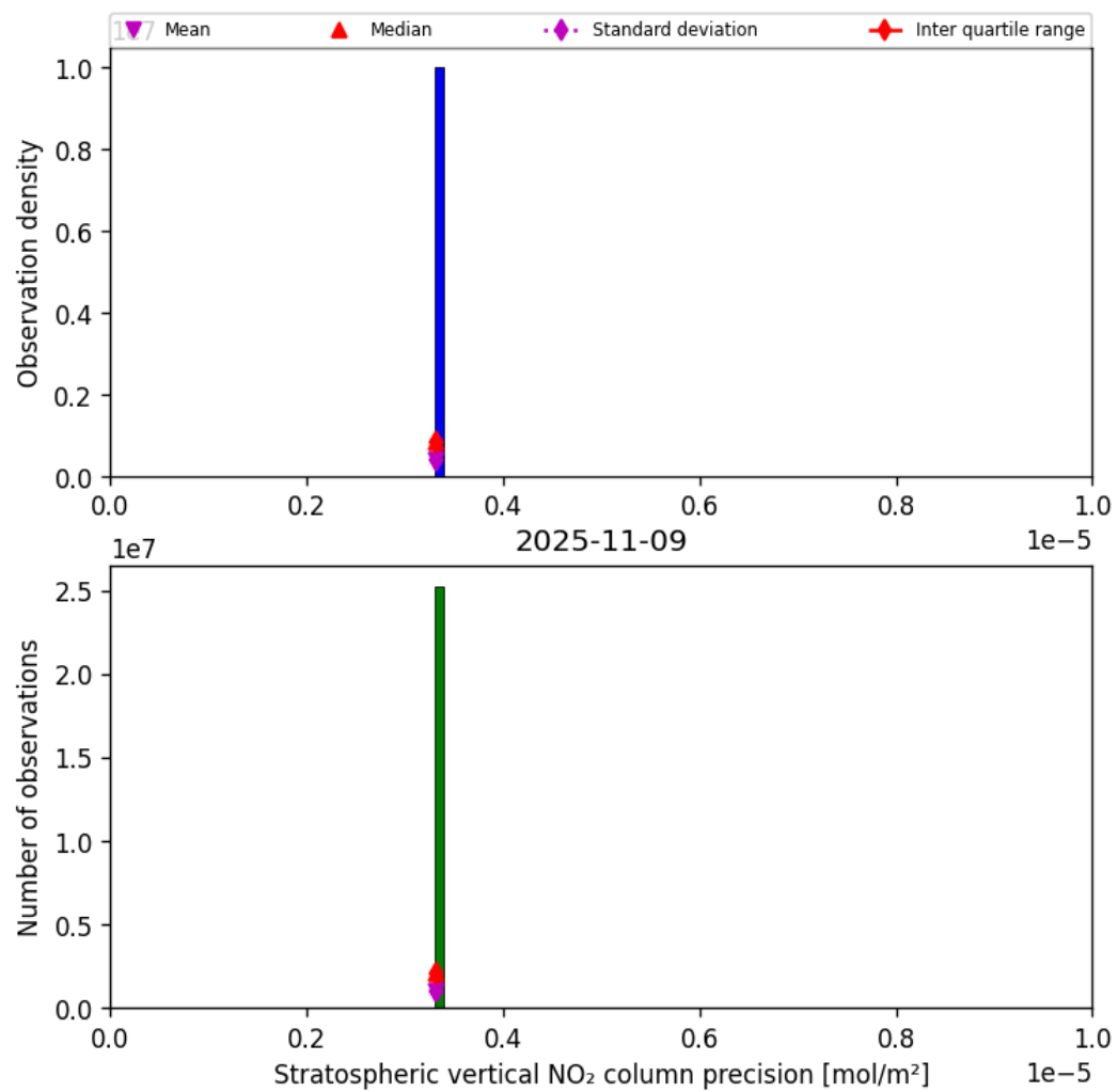
Figure 37: Histogram of “Stratospheric vertical NO 2 column precision” for 2025-11-08 to 2025-11-10
