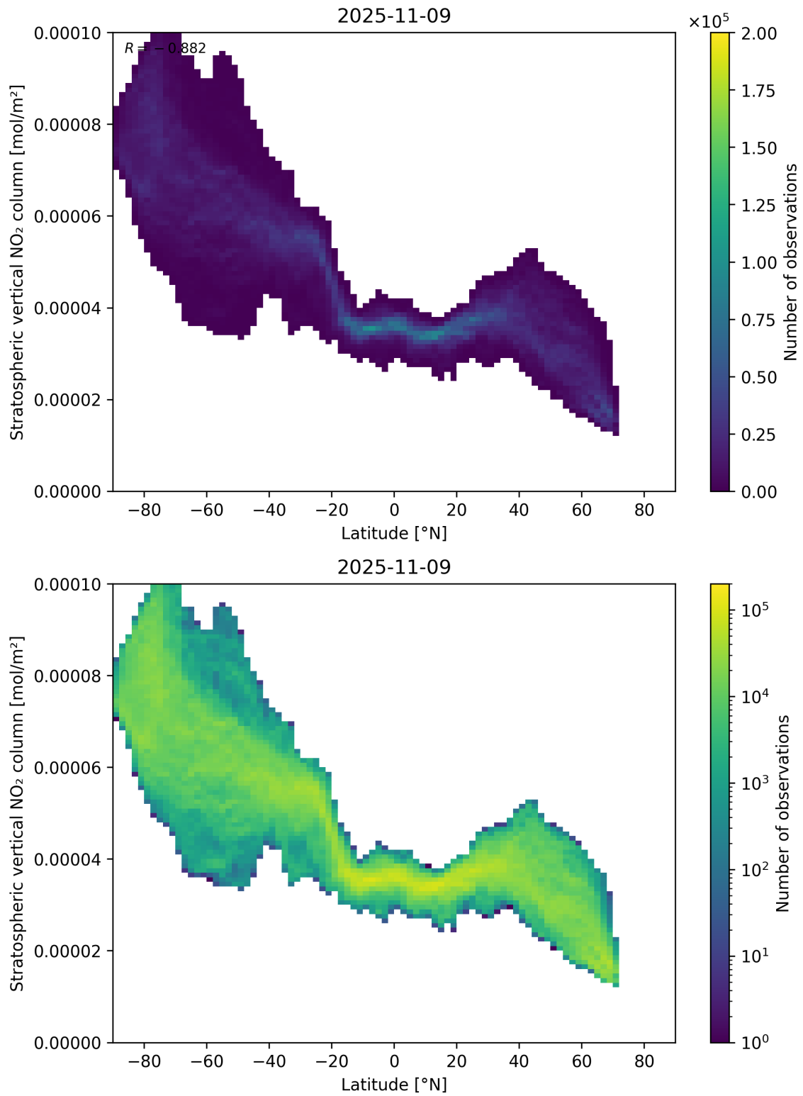
Figure 87: Scatter density plot of “Latitude” against “Stratospheric vertical NO 2 column” for 2025-11-08 to 2025-11-10.
