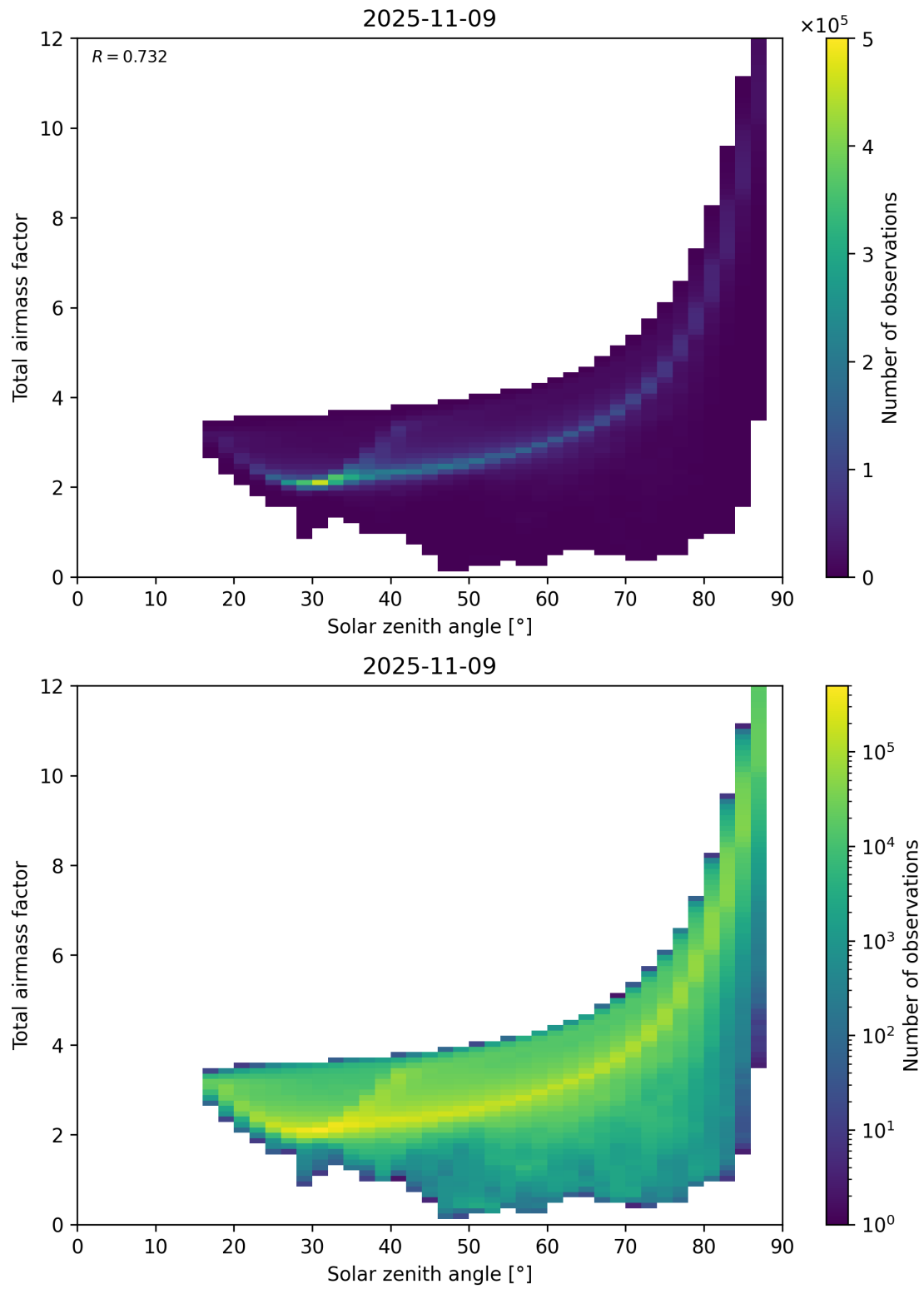
Figure 146: Scatter density plot of “Solar zenith angle” against “Total airmass factor” for 2025-11-08 to 2025-11-10.
