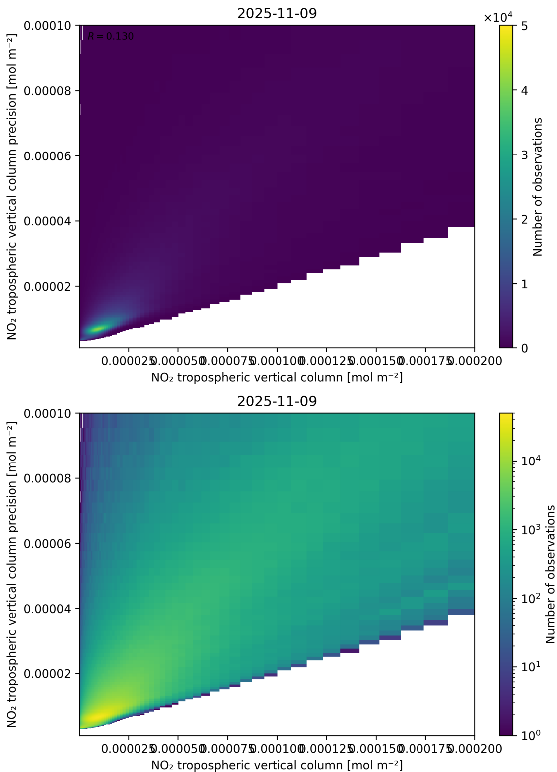
Figure 130: Scatter density plot of “NO 2 tropospheric vertical column” against “NO 2 tropospheric vertical column precision” for 2025-11-08 to 2025-11-10.
