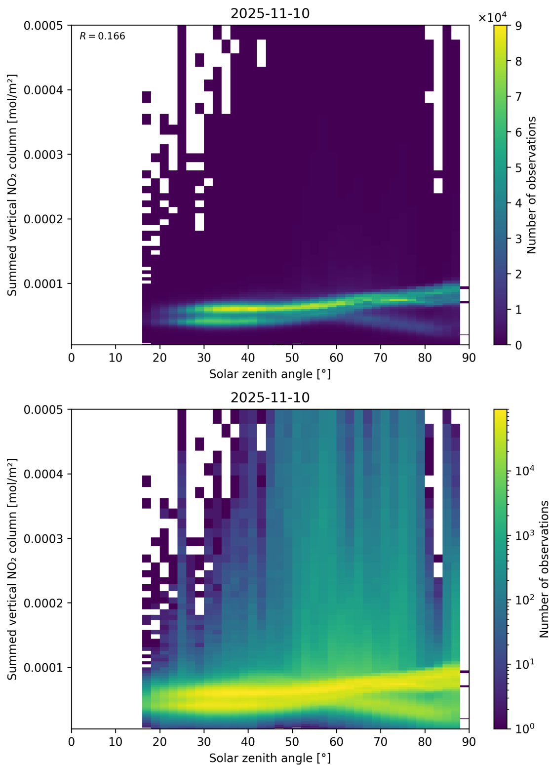
Figure 151: Scatter density plot of “Solar zenith angle” against “Summed vertical NO 2 column” for 2025-11-09 to 2025-11-11.
