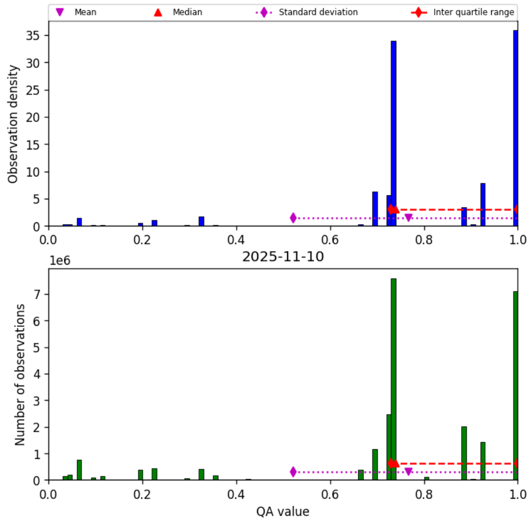
Figure 28: Histogram of “QA value” for 2025-11-09 to 2025-11-11
