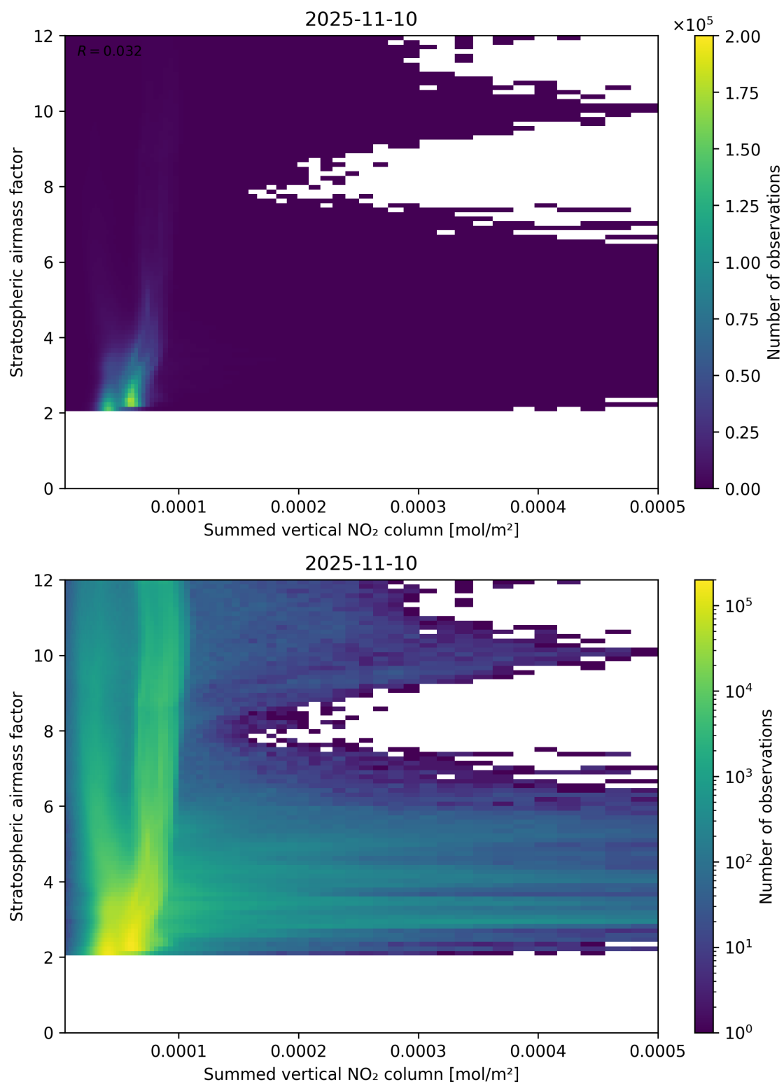
Figure 103: Scatter density plot of “Summed vertical NO 2 column” against “Stratospheric air mass factor” for 2025-11-09 to 2025-11-11.
