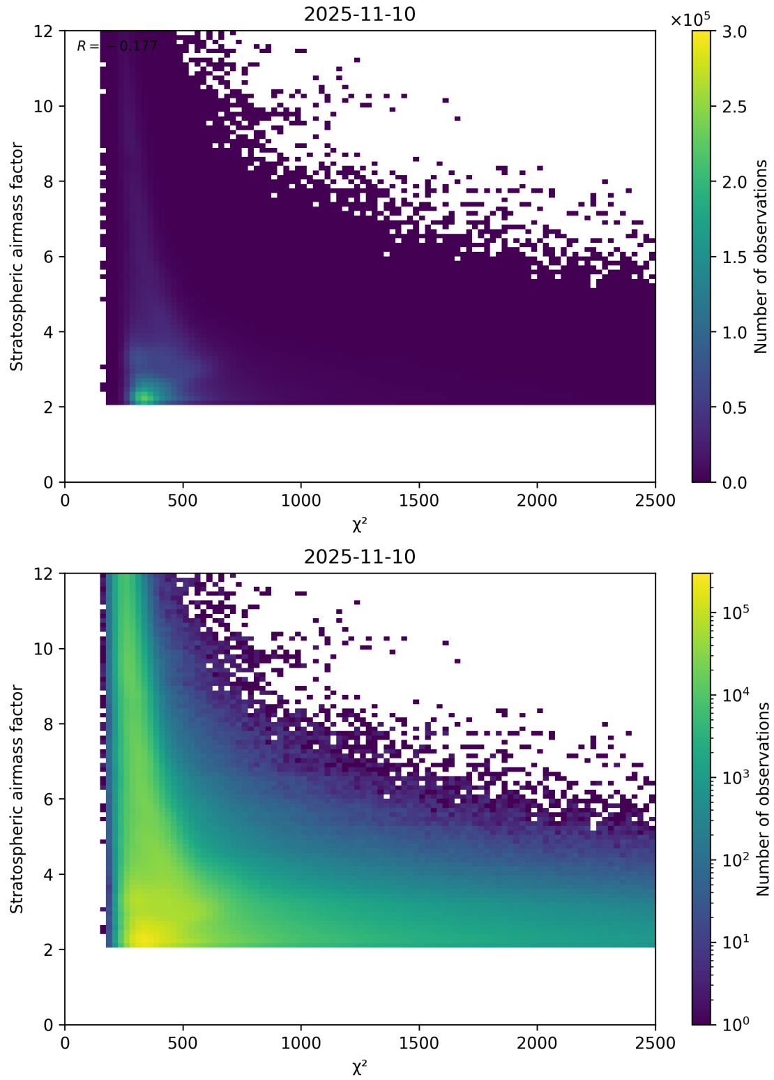
Figure 81: Scatter density plot of “ \chi^2 ” against “Stratospheric airmass factor” for 2025-11-09 to 2025-11-11.
