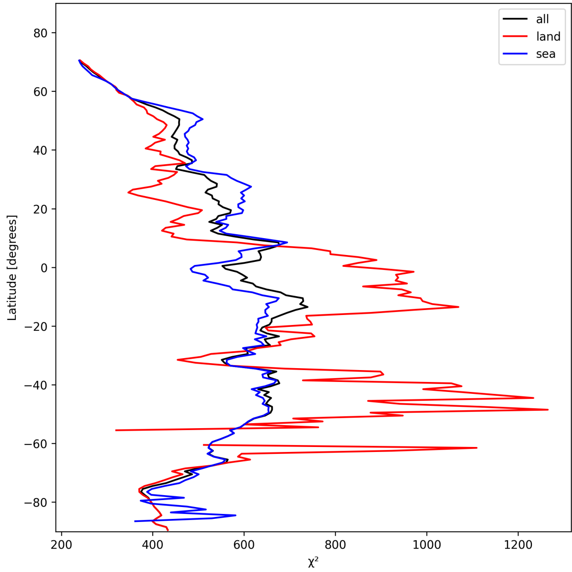
Figure 25: Zonal average of “ \chi^2 ” for 2025-11-09 to 2025-11-11.
