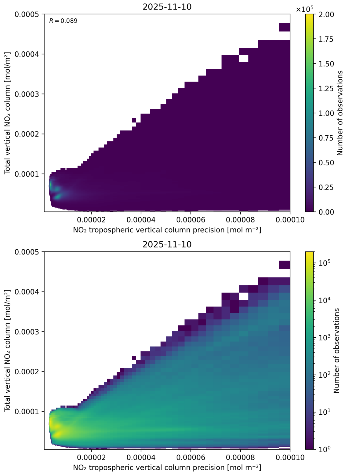
Figure 138: Scatter density plot of “NO 2 tropospheric vertical column precision” against “Total vertical NO 2 column” for 2025-11-09 to 2025-11-11.
