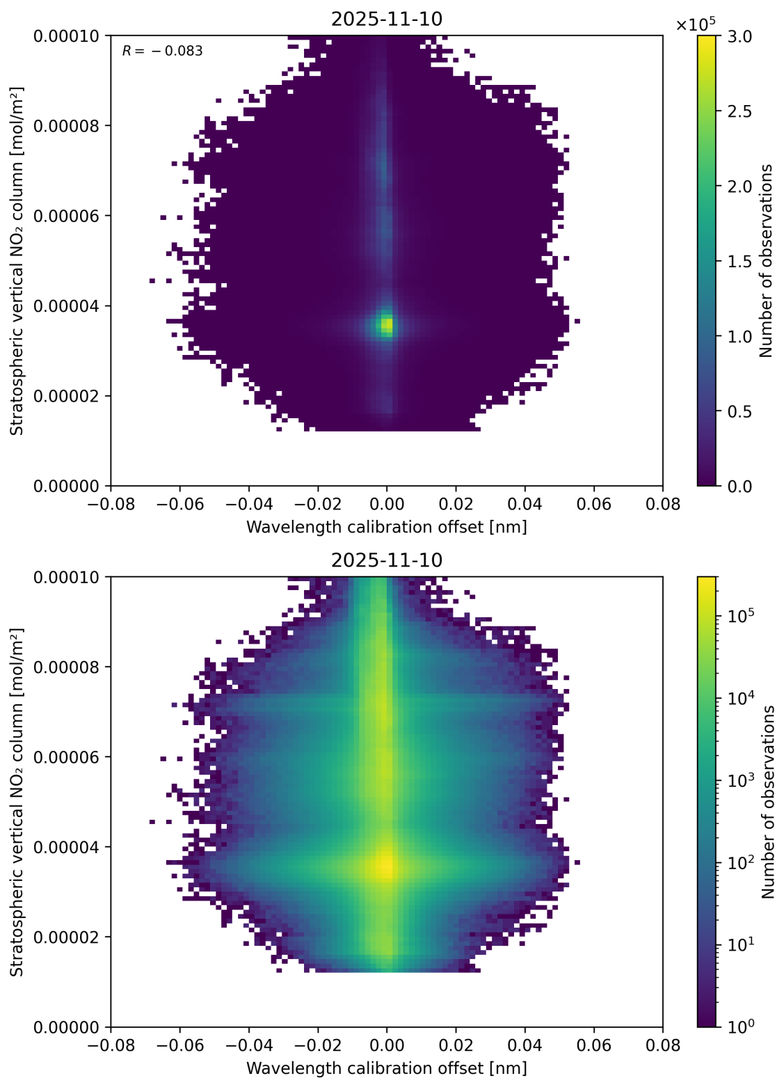
Figure 176: Scatter density plot of “Wavelength calibration offset” against “Stratospheric vertical NO 2 column” for 2025-11-09 to 2025-11-11.
