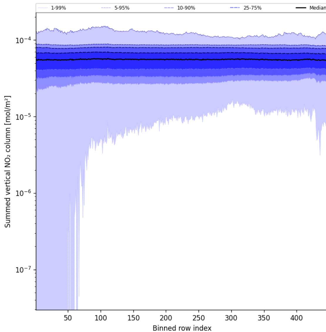
Figure 57: Along track statistics of “Summed vertical NO 2 column” for 2025-11-09 to 2025-11-11
