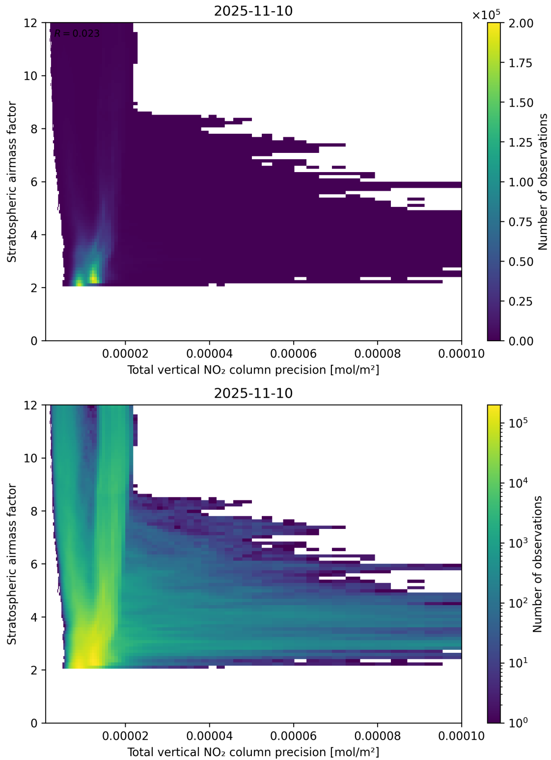
Figure 115: Scatter density plot of “Total vertical NO 2 column precision” against “Stratospheric air mass factor” for 2025-11-09 to 2025-11-11.
