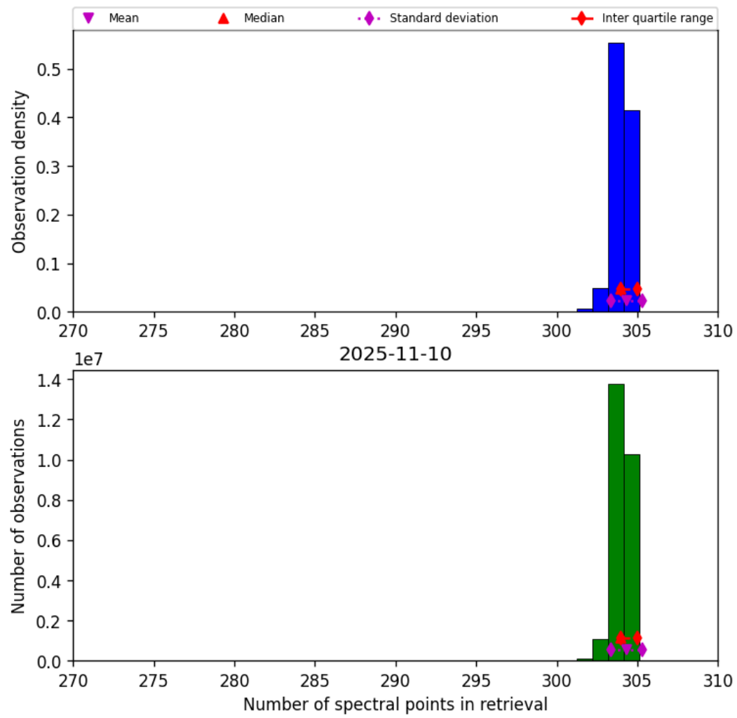
Figure 33: Histogram of “Number of spectral points in retrieval” for 2025-11-09 to 2025-11-11
