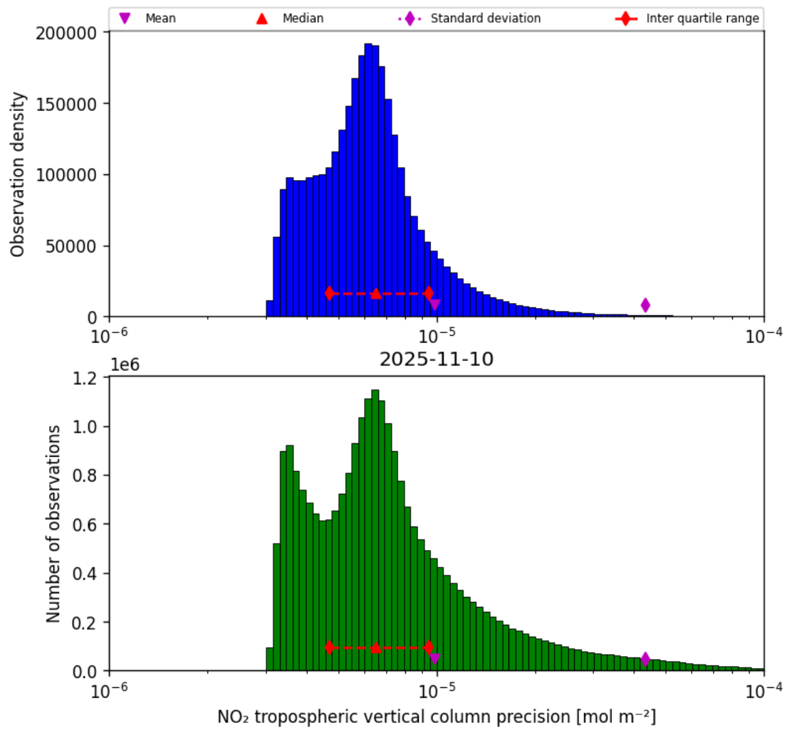
Figure 30: Histogram of “NO 2 tropospheric vertical column precision” for 2025-11-09 to 2025-11-11
