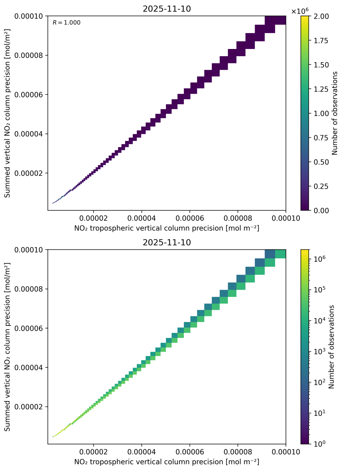
Figure 137: Scatter density plot of “NO 2 tropospheric vertical column precision” against “Summed vertical NO 2 column precision” for 2025-11-09 to 2025-11-11.
