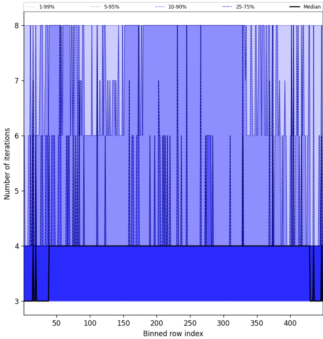
Figure 51: Along track statistics of “Number of iterations” for 2025-11-09 to 2025-11-11
