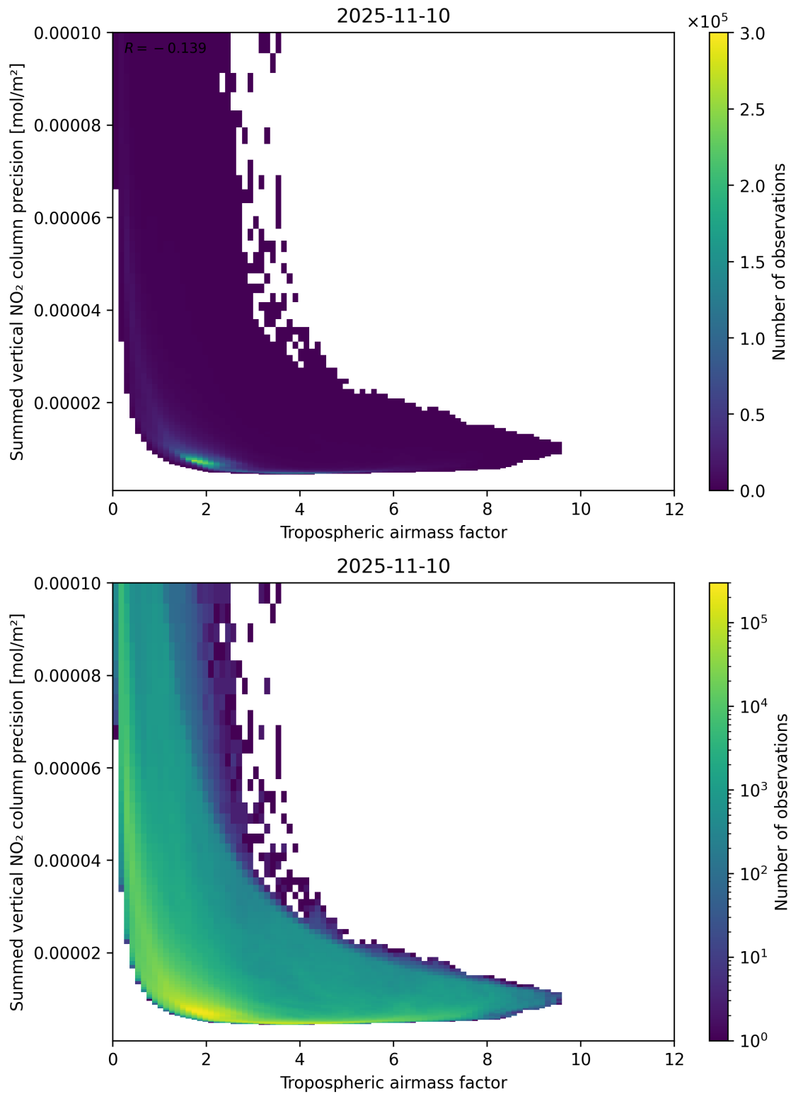
Figure 76: Scatter density plot of “Tropospheric air mass factor” against “Summed vertical NO 2 column precision” for 2025-11-09 to 2025-11-11.
