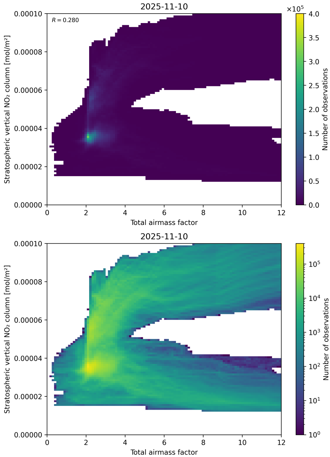
Figure 64: Scatter density plot of “Total airmass factor” against “Stratospheric vertical \text{NO}_2 column” for 2025-11-09 to 2025-11-11.
