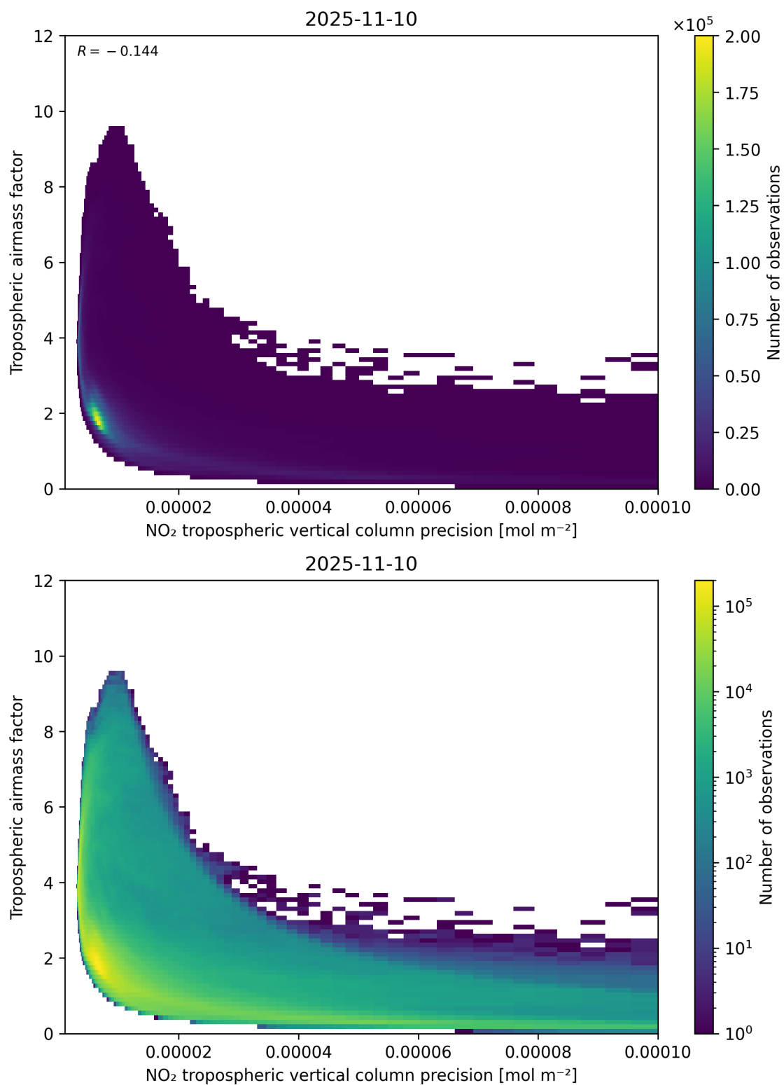
Figure 133: Scatter density plot of “NO 2 tropospheric vertical column precision” against “Tropospheric air mass factor” for 2025-11-09 to 2025-11-11.
