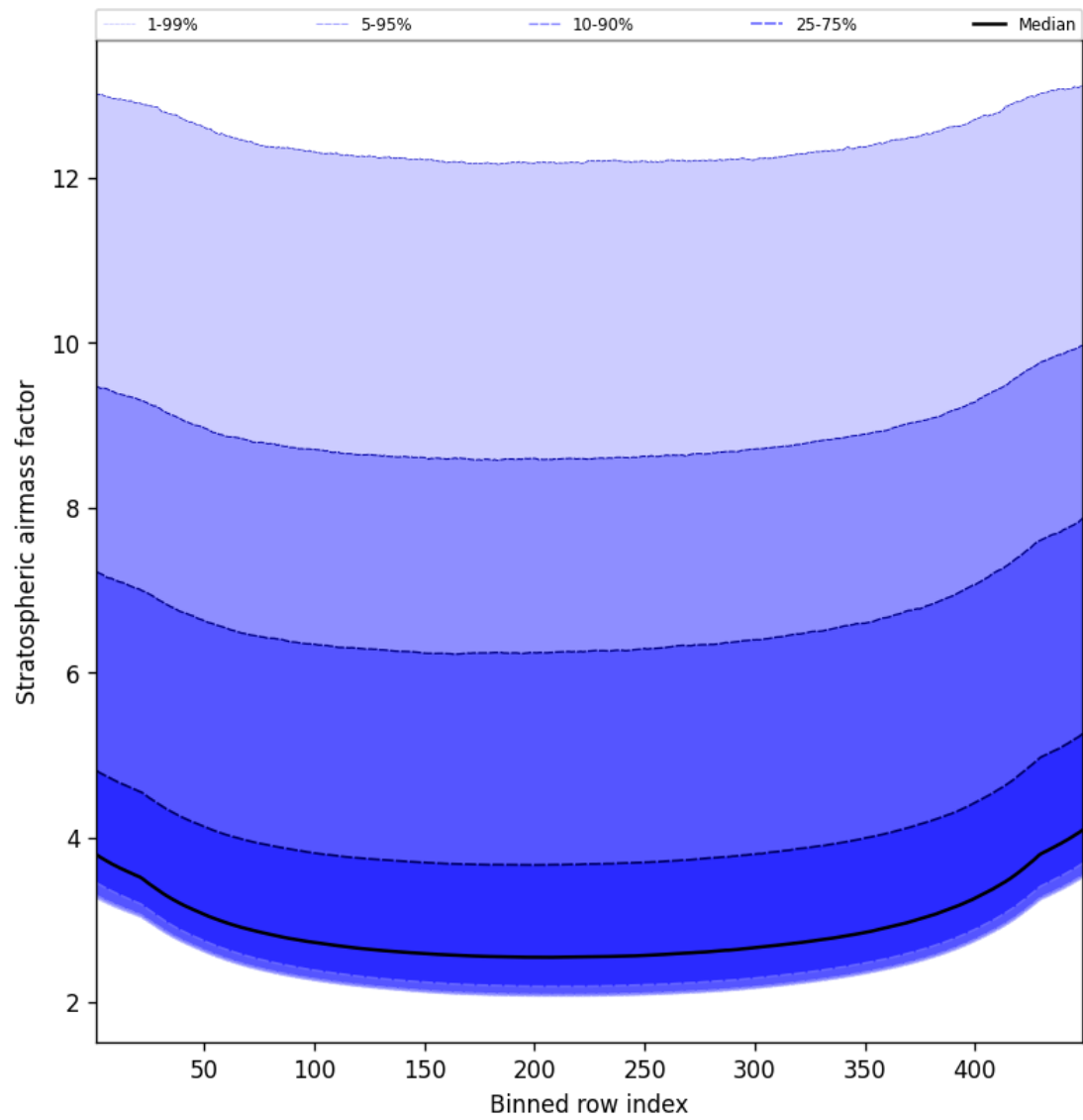
Figure 61: Along track statistics of “Stratospheric air mass factor” for 2025-11-09 to 2025-11-11
