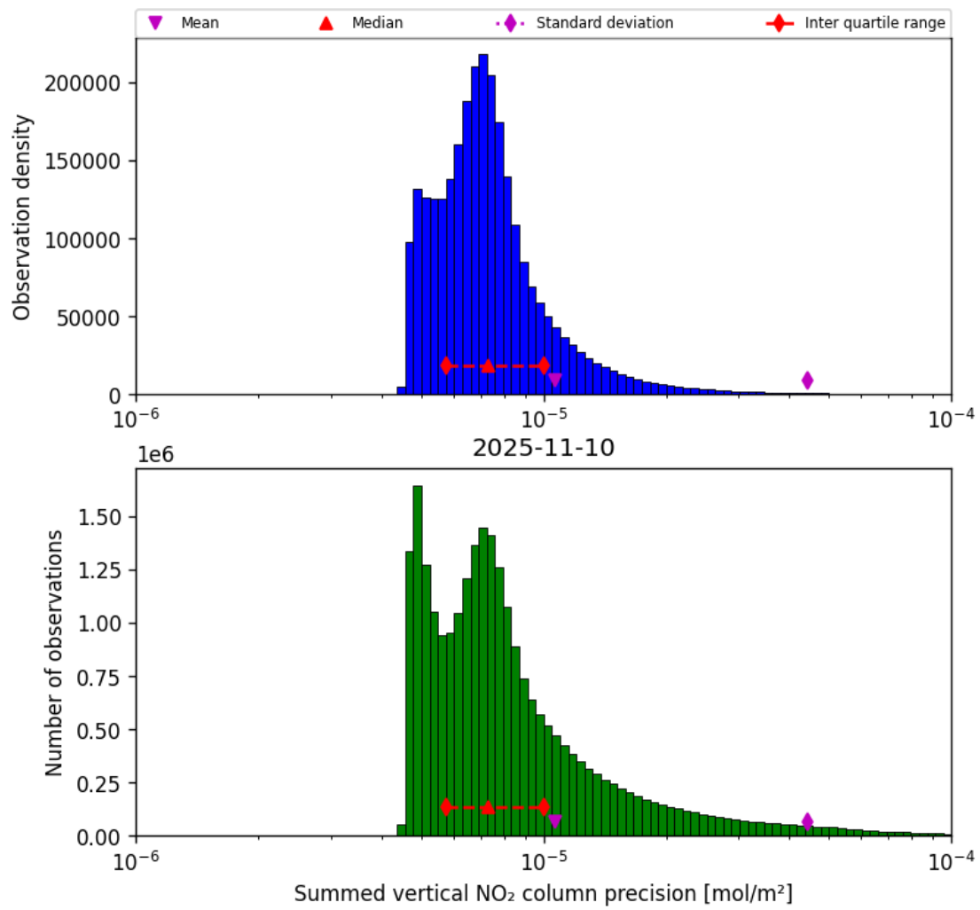
Figure 41: Histogram of “Summed vertical NO 2 column precision” for 2025-11-09 to 2025-11-11
