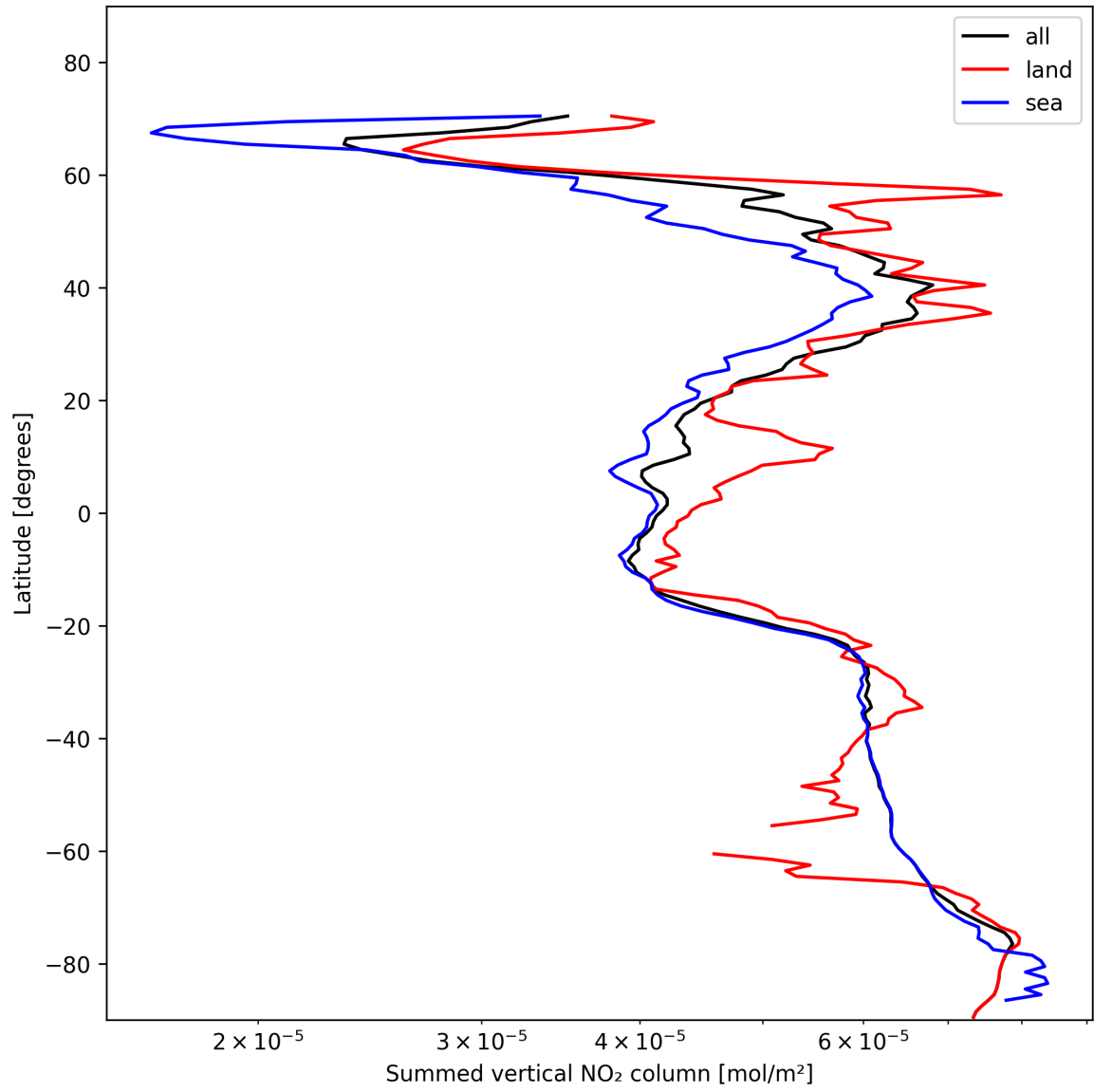
Figure 23: Zonal average of “Summed vertical NO 2 column” for 2025-11-09 to 2025-11-11.
