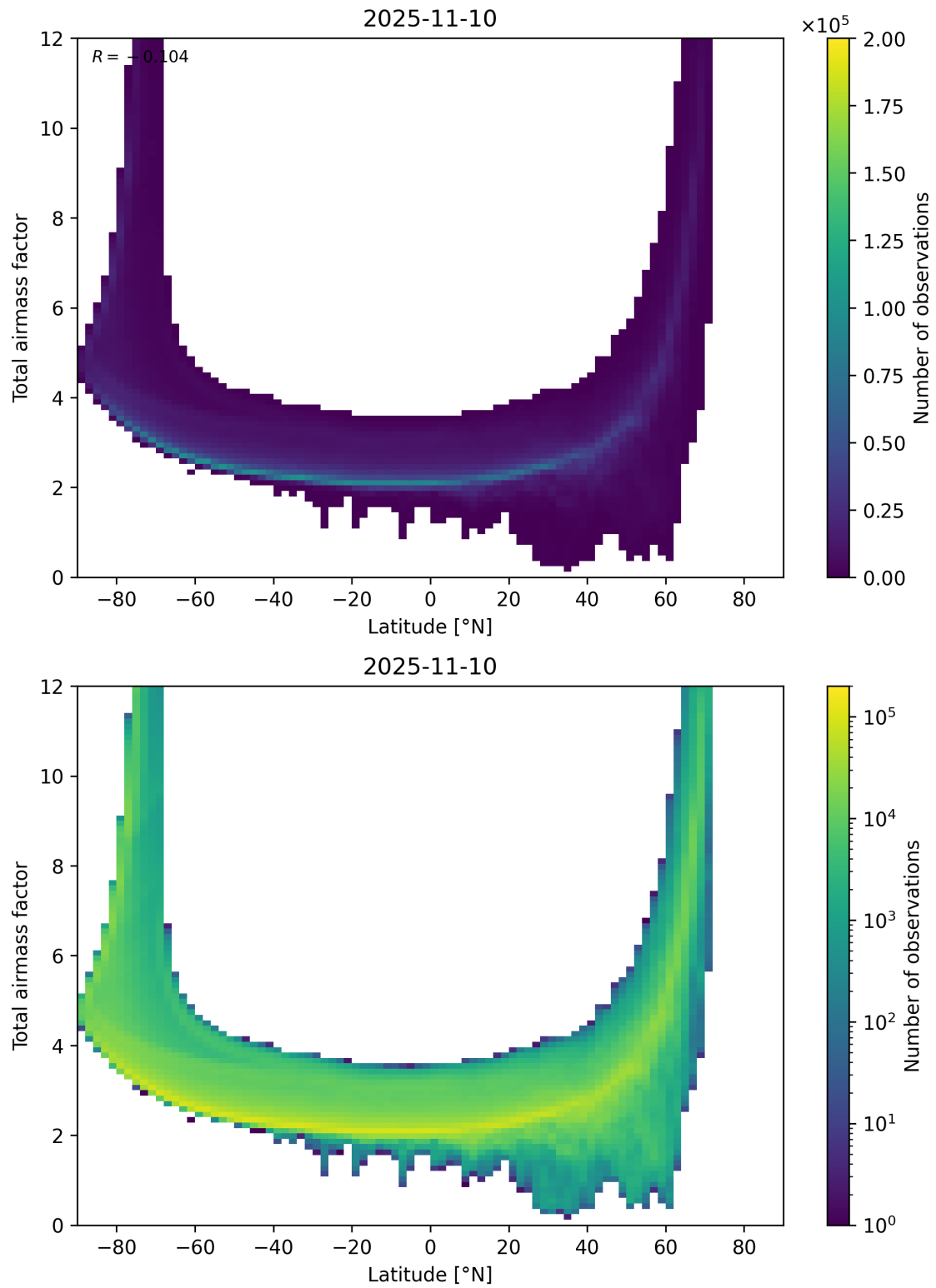
Figure 84: Scatter density plot of “Latitude” against “Total airmass factor” for 2025-11-09 to 2025-11-11.
