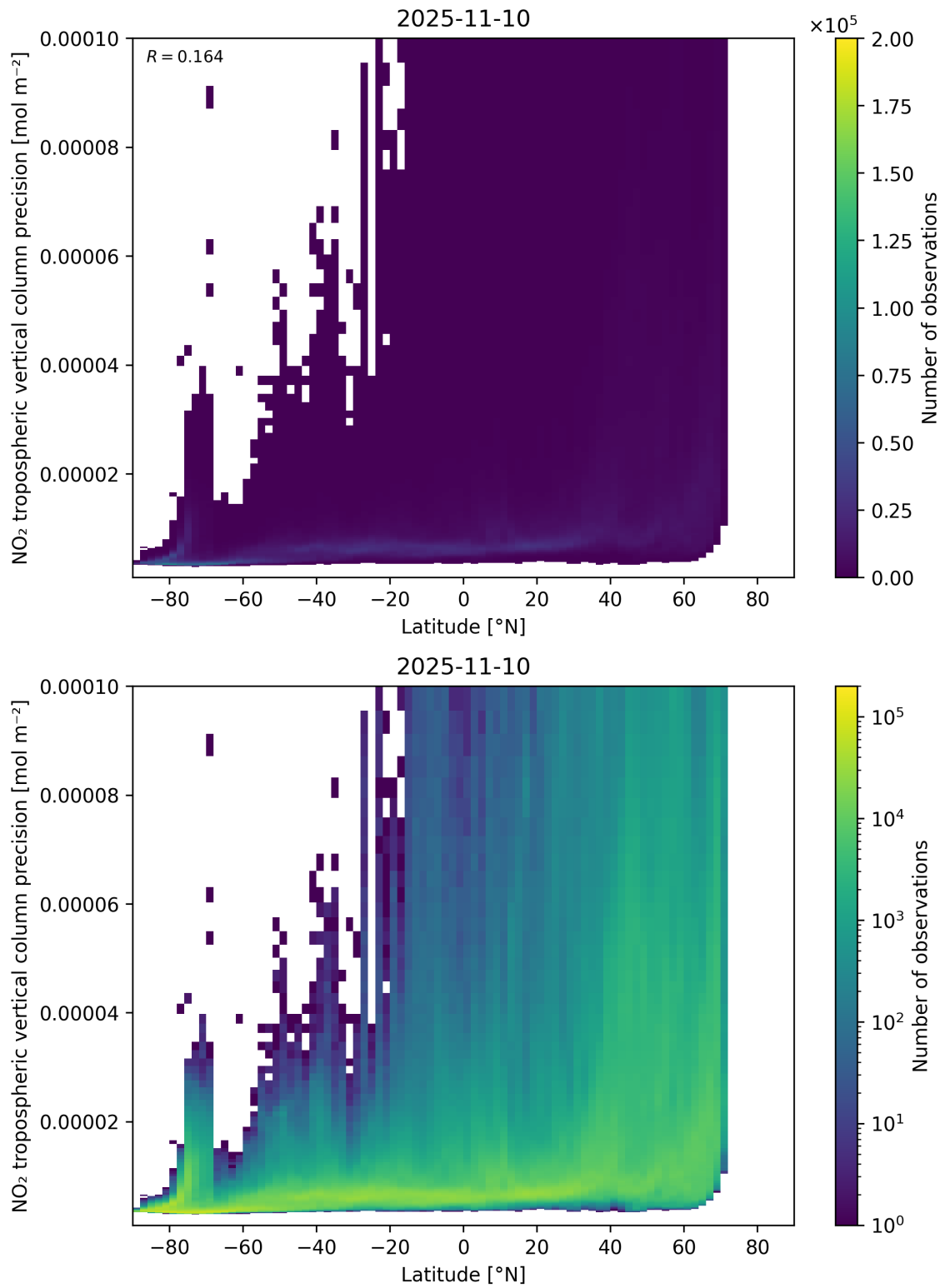
Figure 93: Scatter density plot of “Latitude” against “NO 2 tropospheric vertical column precision” for 2025-11-09 to 2025-11-11.
