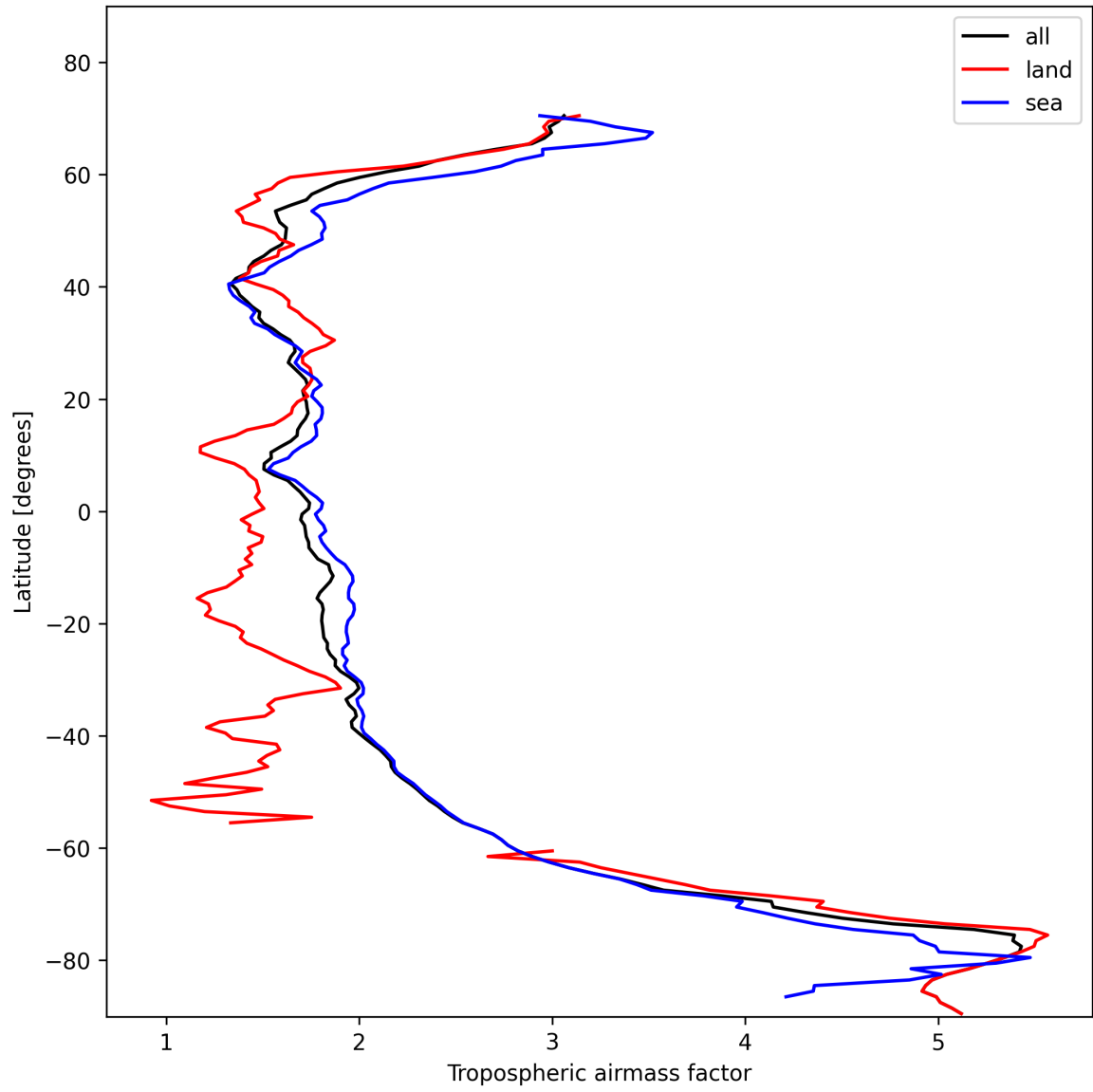
Figure 14: Zonal average of “Tropospheric airmass factor” for 2025-11-09 to 2025-11-11.
