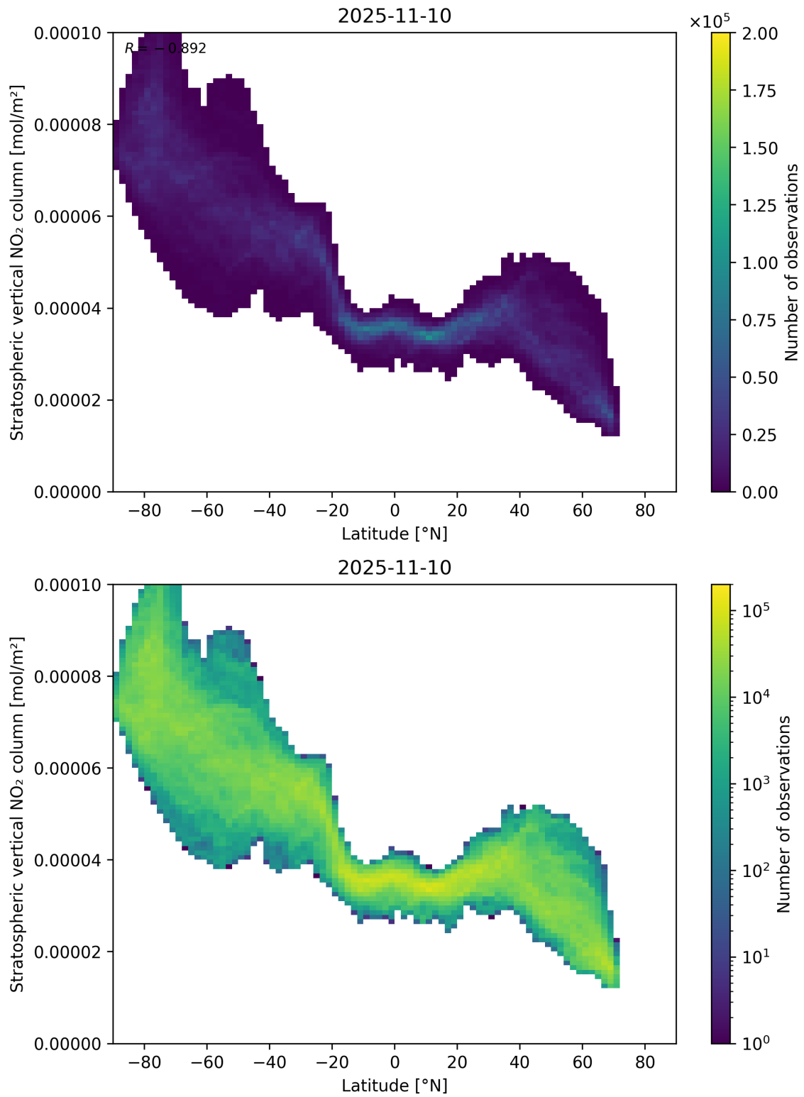
Figure 87: Scatter density plot of “Latitude” against “Stratospheric vertical NO 2 column” for 2025-11-09 to 2025-11-11.
