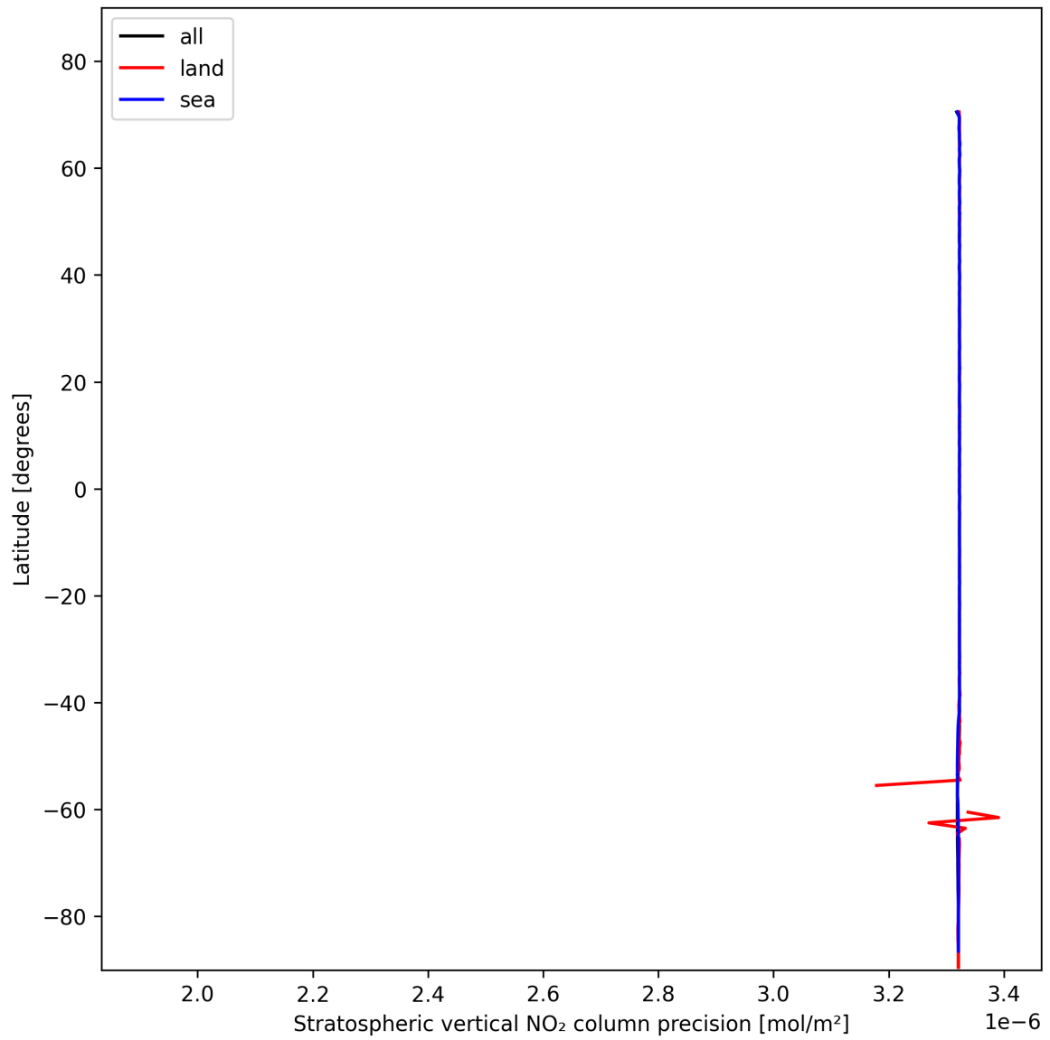
Figure 20: Zonal average of “Stratospheric vertical NO 2 column precision” for 2025-11-09 to 2025-11-11.
