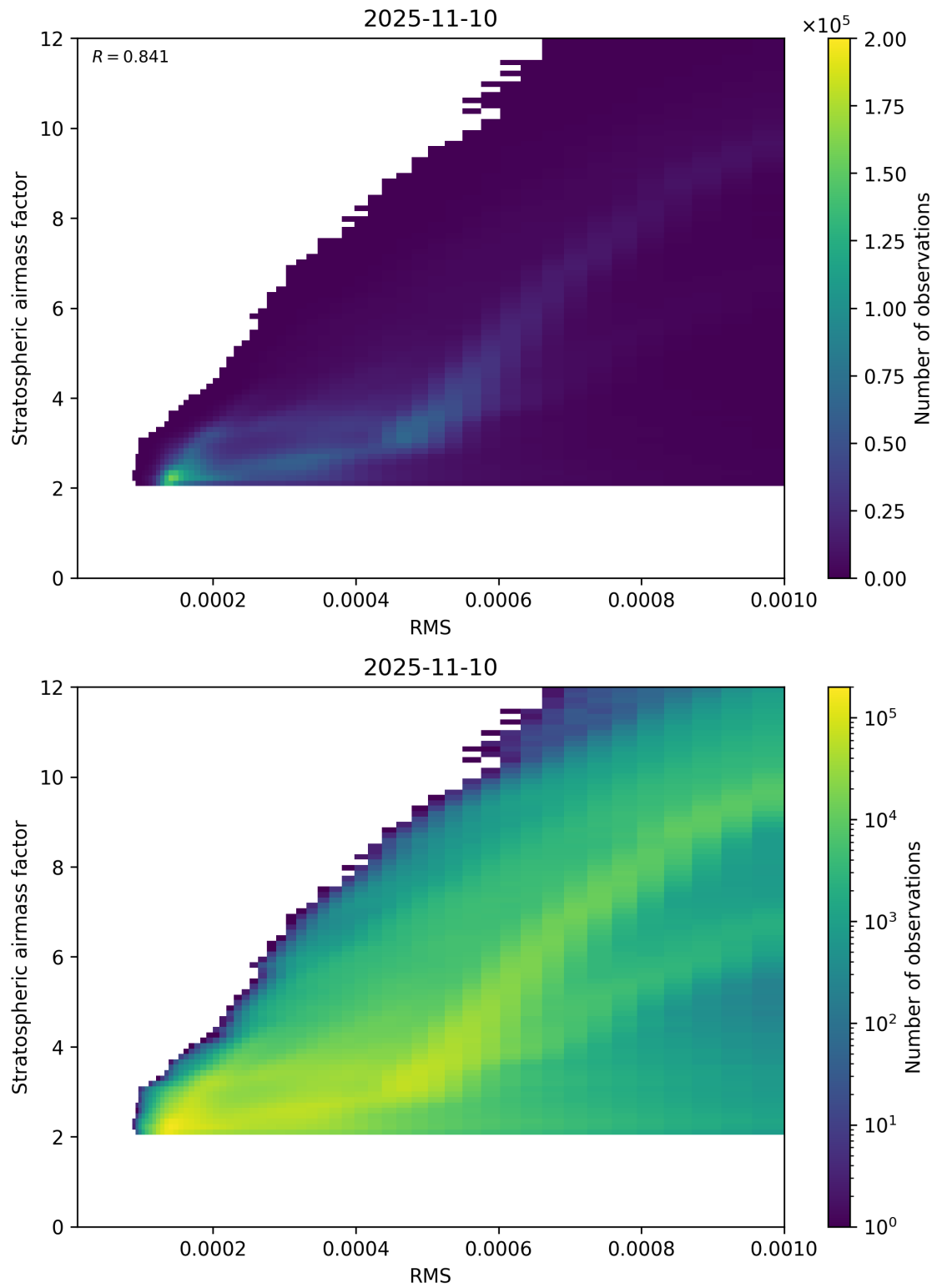
Figure 144: Scatter density plot of “RMS” against “Stratospheric airmass factor” for 2025-11-09 to 2025-11-11.
