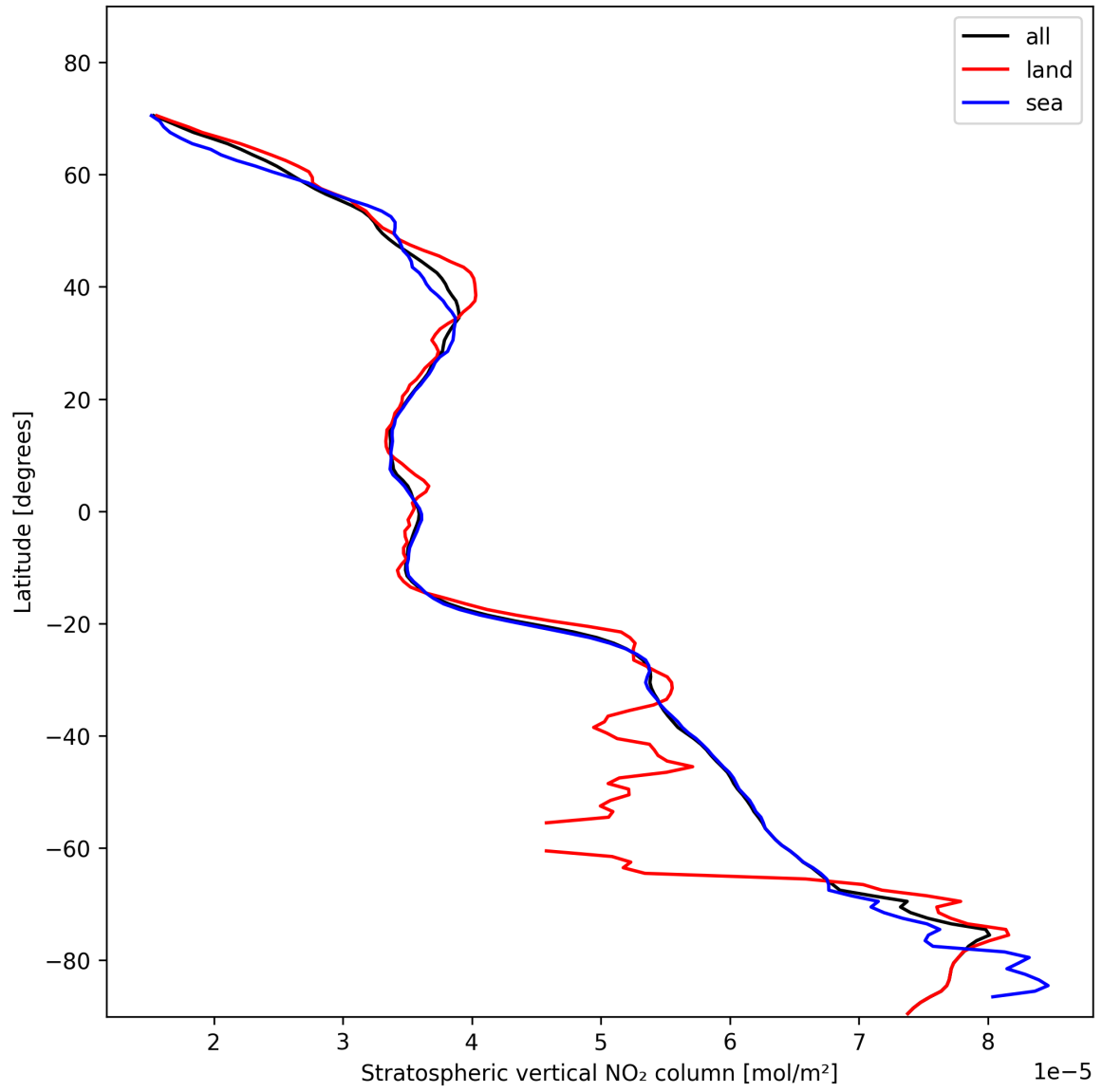
Figure 19: Zonal average of “Stratospheric vertical NO 2 column” for 2025-11-09 to 2025-11-11.
