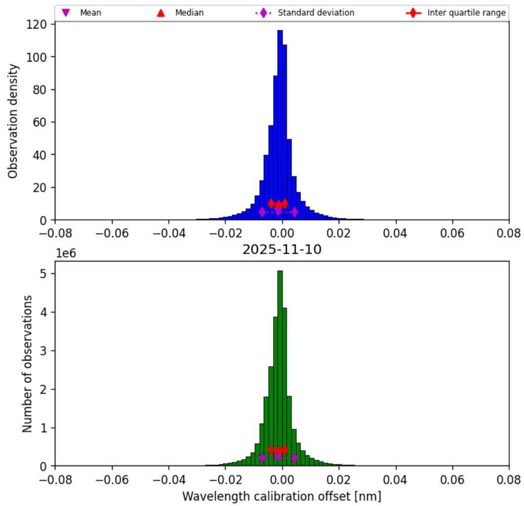
Figure 35: Histogram of “Wavelength calibration offset” for 2025-11-09 to 2025-11-11
