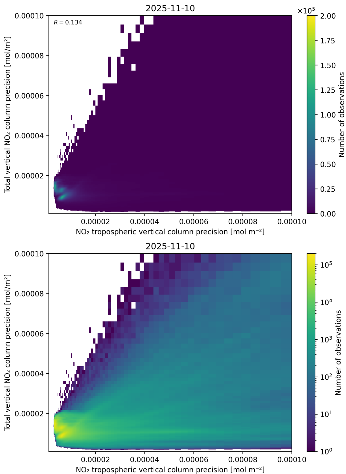
Figure 139: Scatter density plot of “NO 2 tropospheric vertical column precision” against “Total vertical NO 2 column precision” for 2025-11-09 to 2025-11-11.
