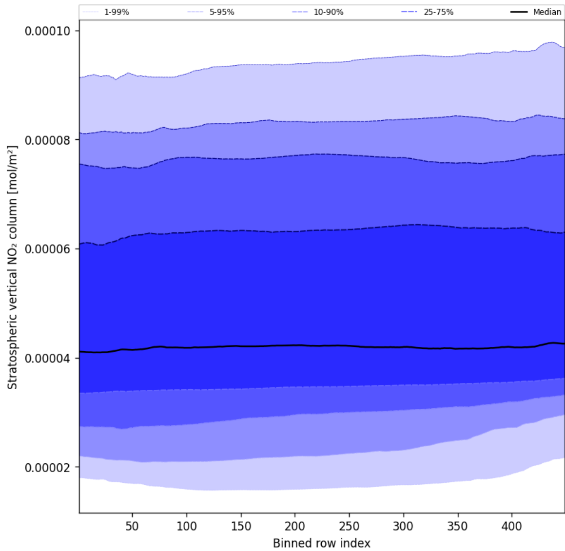
Figure 53: Along track statistics of “Stratospheric vertical NO 2 column” for 2025-11-09 to 2025-11-11
