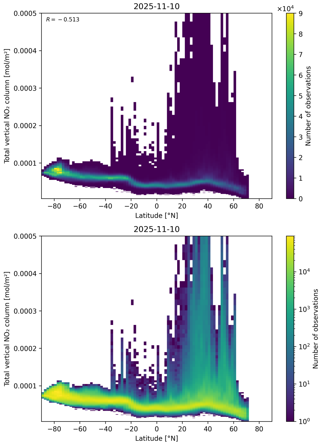
Figure 90: Scatter density plot of “Latitude” against “Total vertical NO 2 column” for 2025-11-09 to 2025-11-11.
