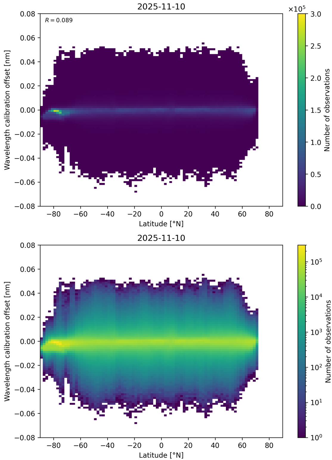
Figure 95: Scatter density plot of “Latitude” against “Wavelength calibration offset” for 2025-11-09 to 2025-11-11.
