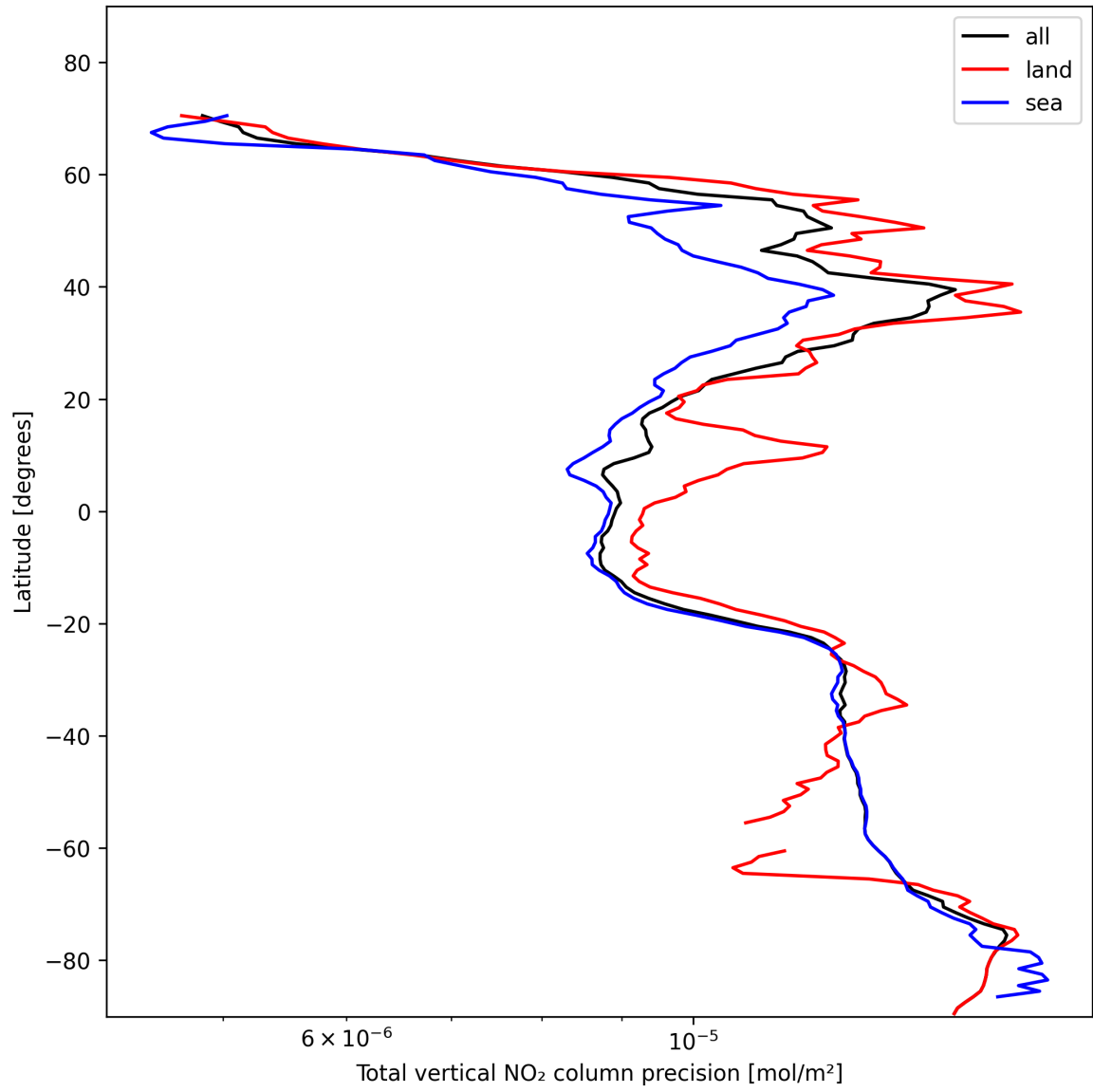
Figure 22: Zonal average of “Total vertical NO 2 column precision” for 2025-11-09 to 2025-11-11.
