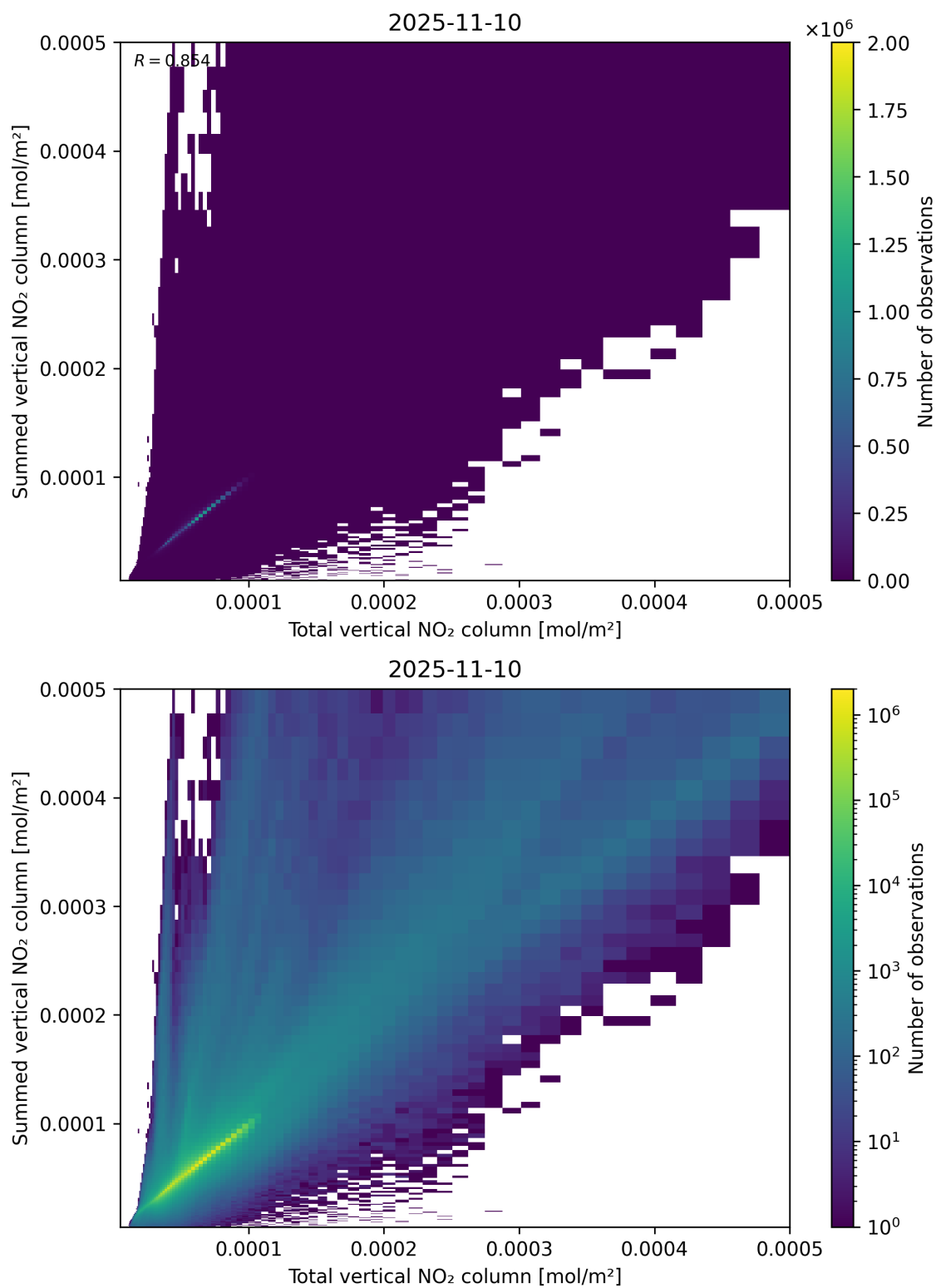
Figure 112: Scatter density plot of “Total vertical NO 2 column” against “Summed vertical NO 2 column” for 2025-11-09 to 2025-11-11.
