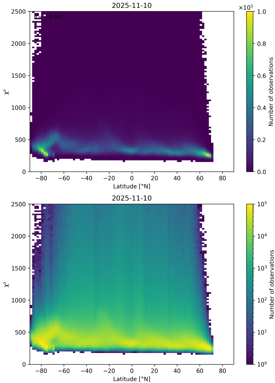
Figure 86: Scatter density plot of “Latitude” against “ \chi^2 ” for 2025-11-09 to 2025-11-11.
