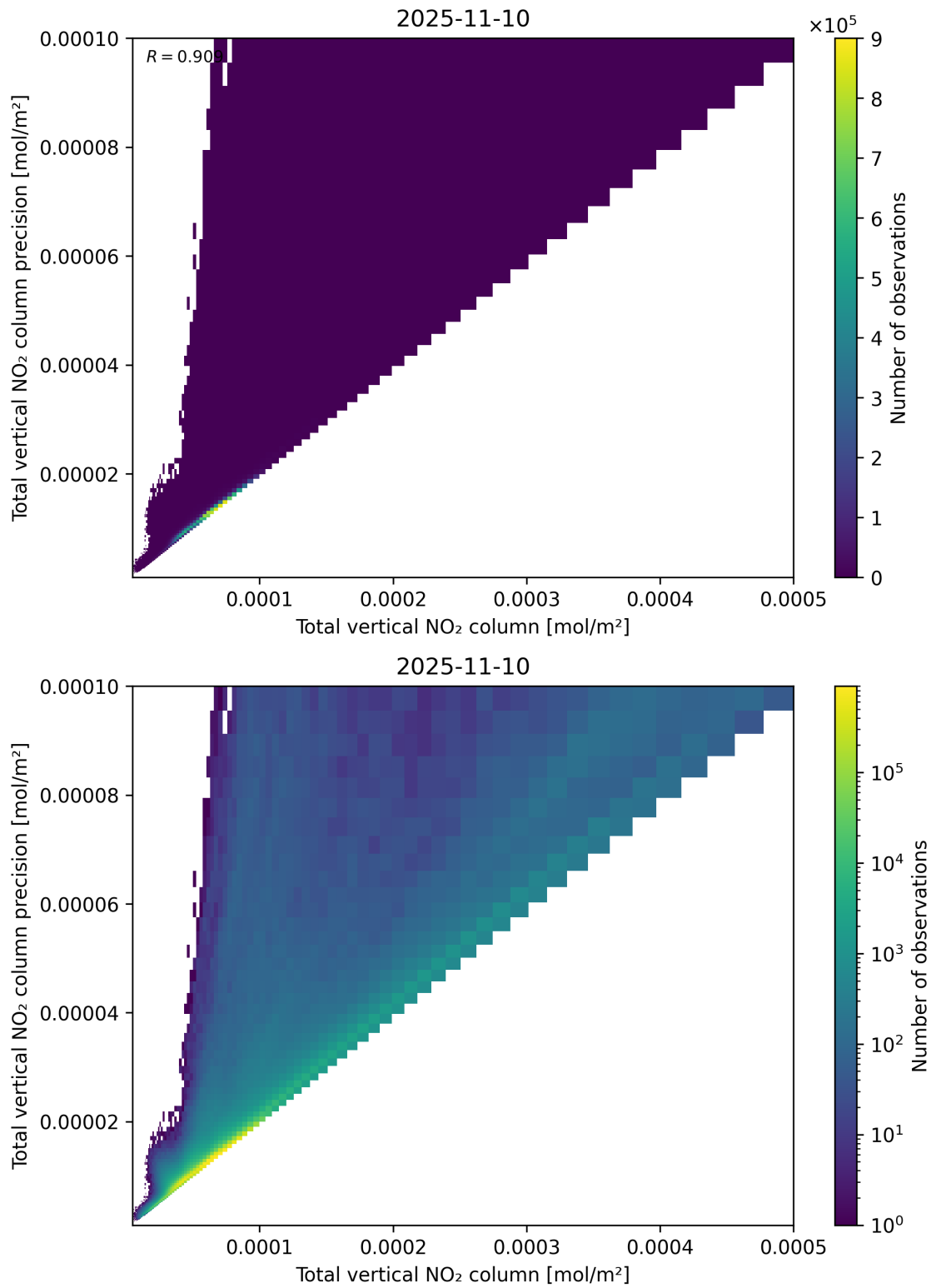
Figure 114: Scatter density plot of “Total vertical NO 2 column” against “Total vertical NO 2 column precision” for 2025-11-09 to 2025-11-11.
