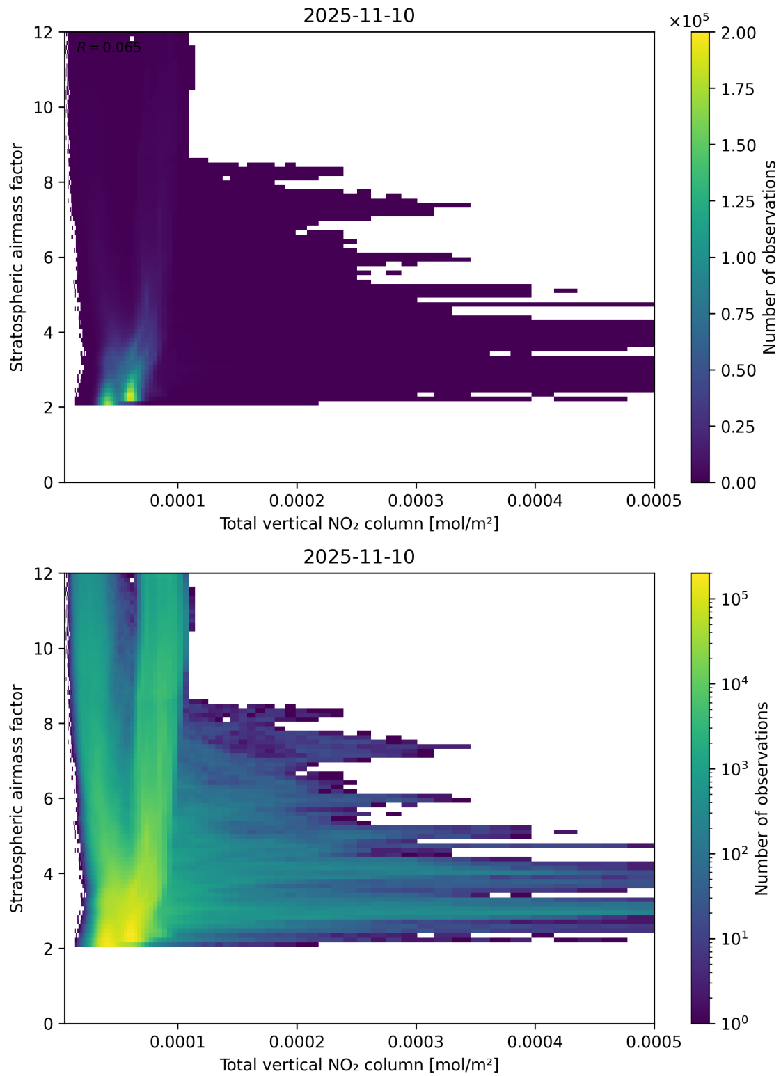
Figure 110: Scatter density plot of “Total vertical NO 2 column” against “Stratospheric airmass factor” for 2025-11-09 to 2025-11-11.
