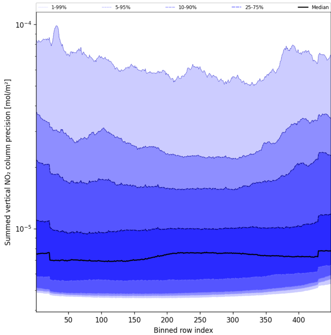
Figure 58: Along track statistics of “Summed vertical NO 2 column precision” for 2025-11-09 to 2025-11-11
