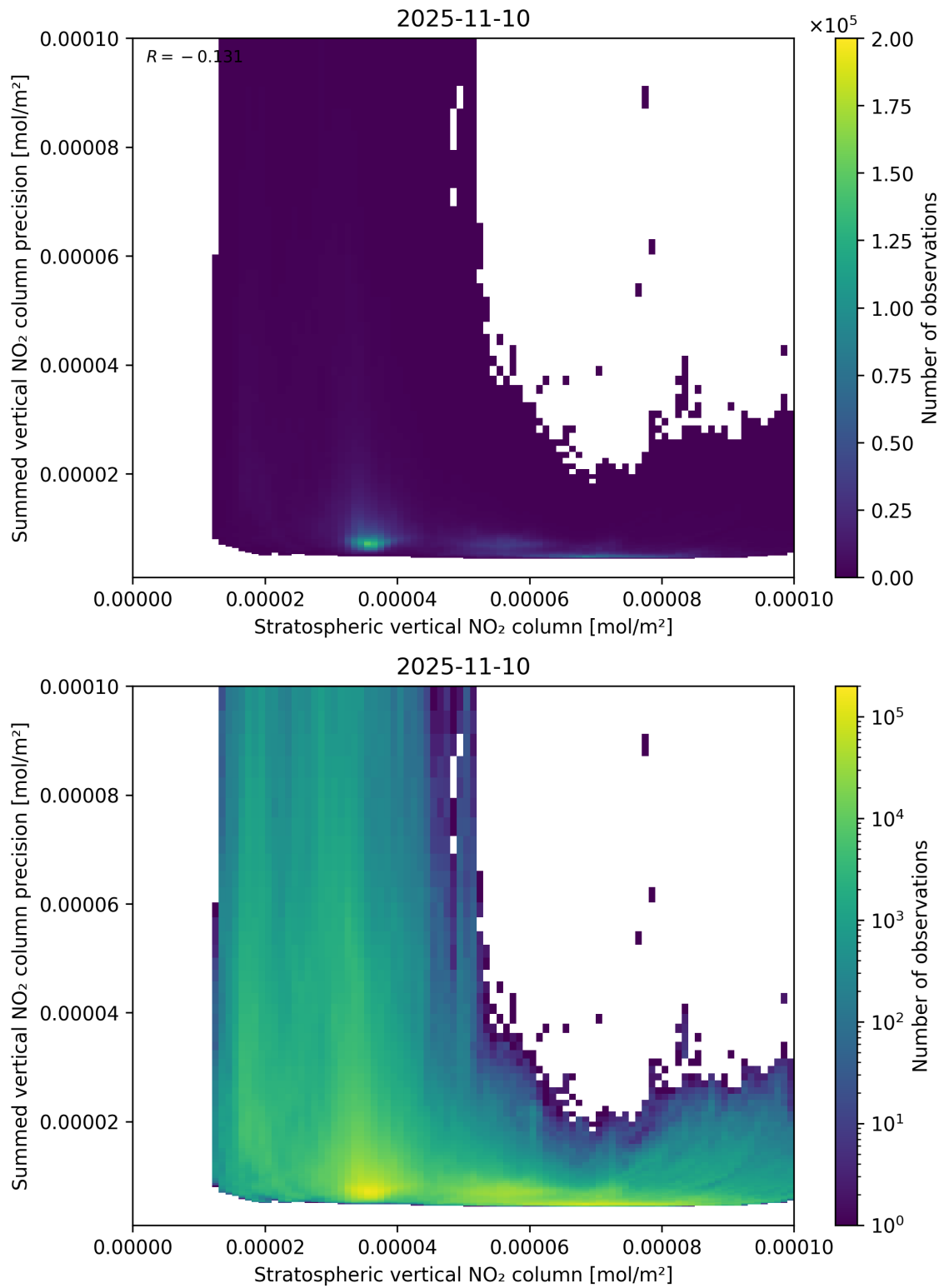
Figure 99: Scatter density plot of “Stratospheric vertical NO 2 column” against “Summed vertical NO 2 column precision” for 2025-11-09 to 2025-11-11.
