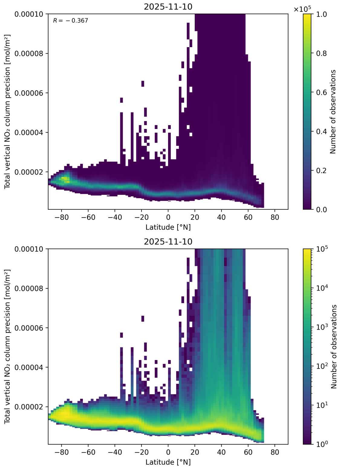
Figure 91: Scatter density plot of “Latitude” against “Total vertical NO 2 column precision” for 2025-11-09 to 2025-11-11.
