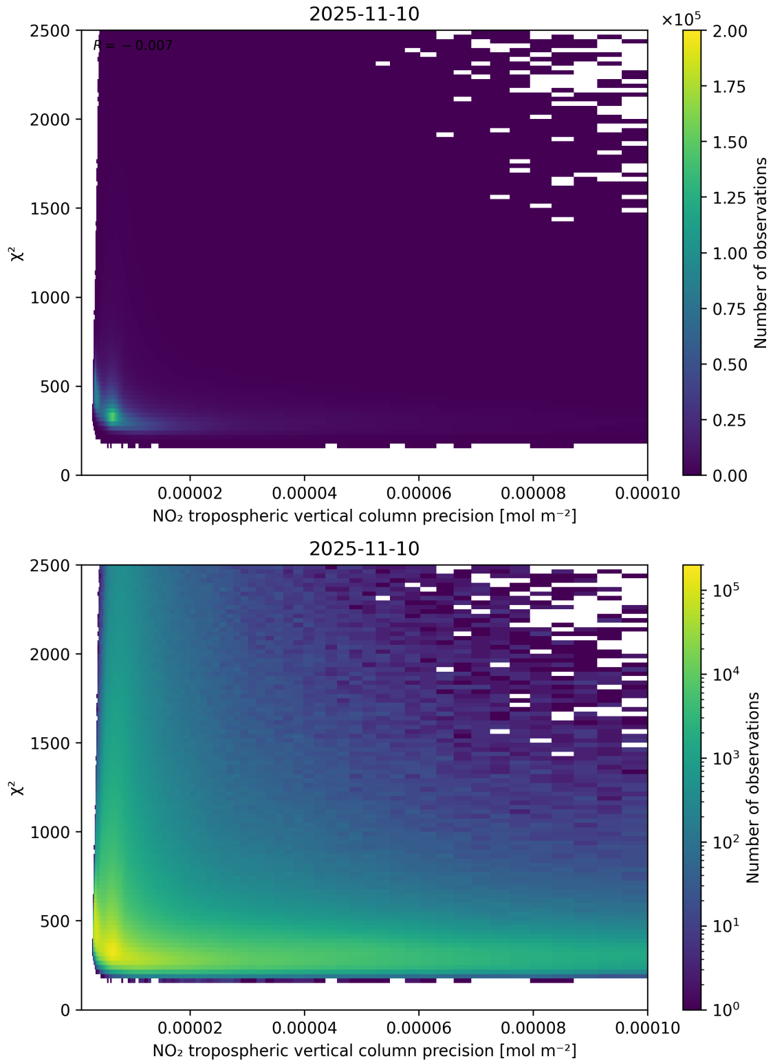
Figure 134: Scatter density plot of “NO 2 tropospheric vertical column precision” against “ \chi^2 ” for 2025-11-09 to 2025-11-11.
