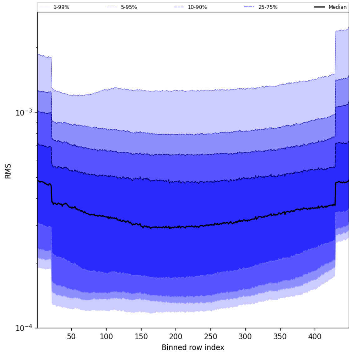
Figure 60: Along track statistics of “RMS” for 2025-11-09 to 2025-11-11
