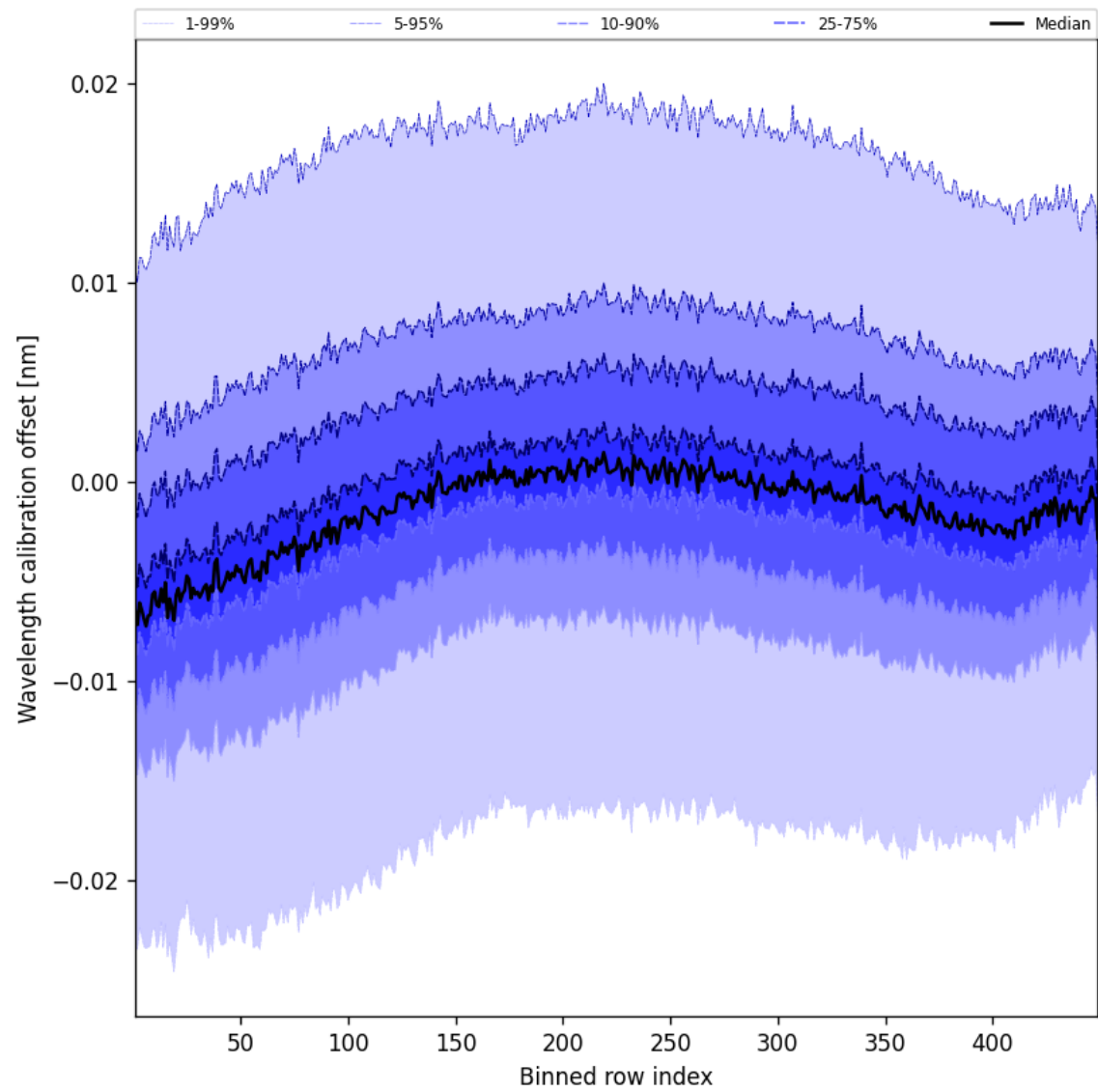
Figure 52: Along track statistics of “Wavelength calibration offset” for 2025-11-09 to 2025-11-11
