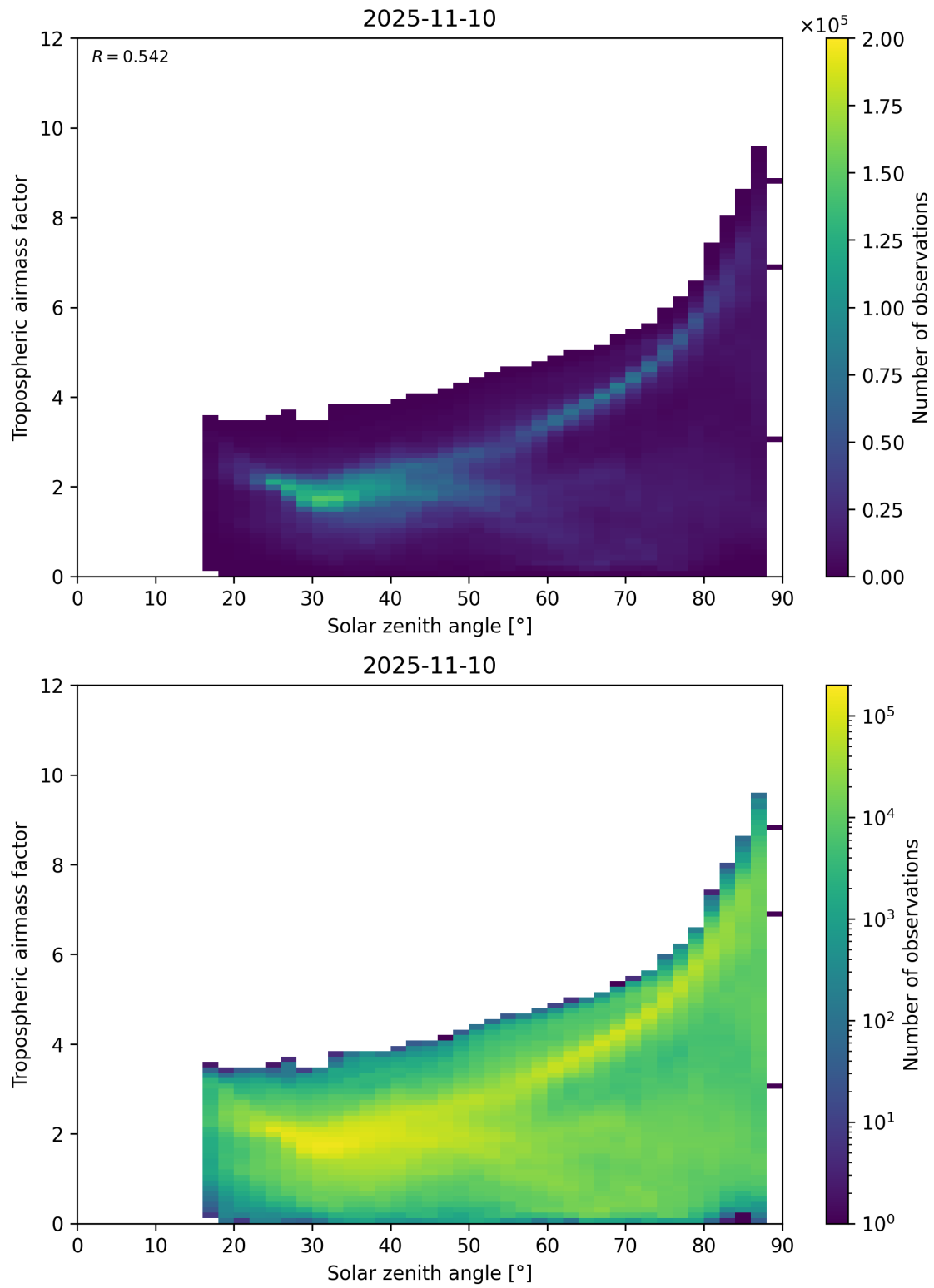
Figure 147: Scatter density plot of “Solar zenith angle” against “Tropospheric airmass factor” for 2025-11-09 to 2025-11-11.
