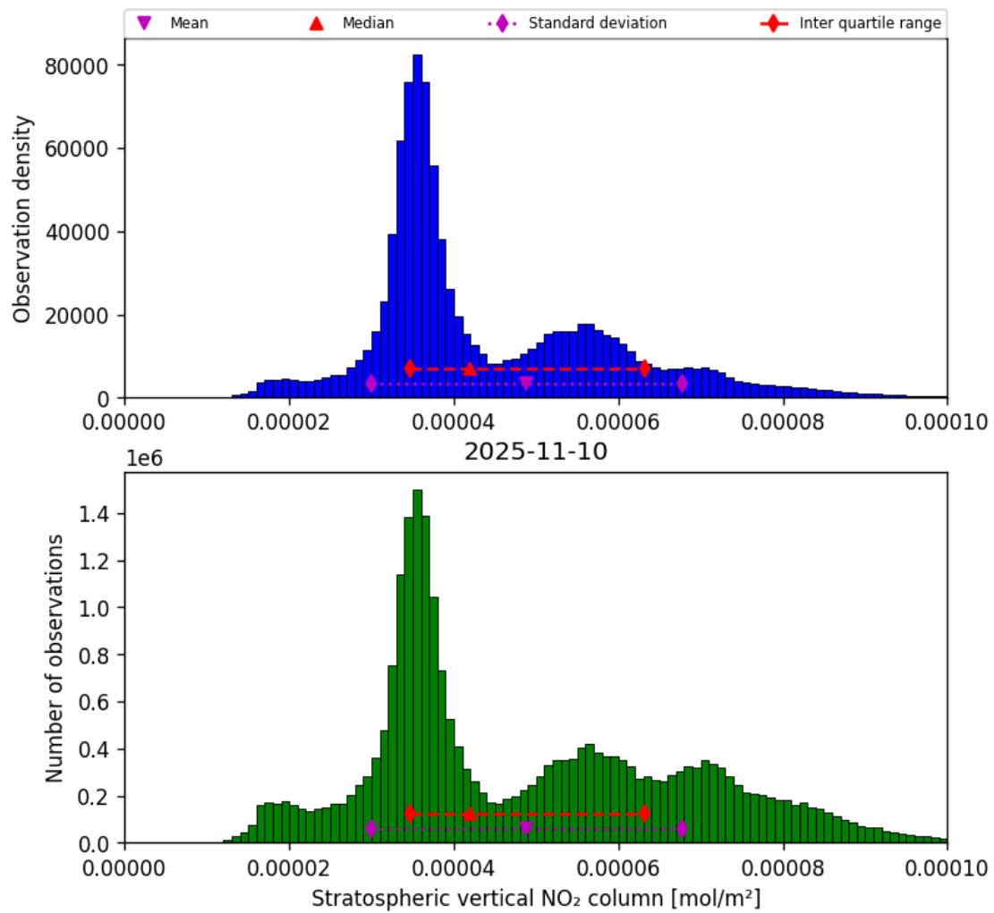
Figure 36: Histogram of “Stratospheric vertical NO 2 column” for 2025-11-09 to 2025-11-11
