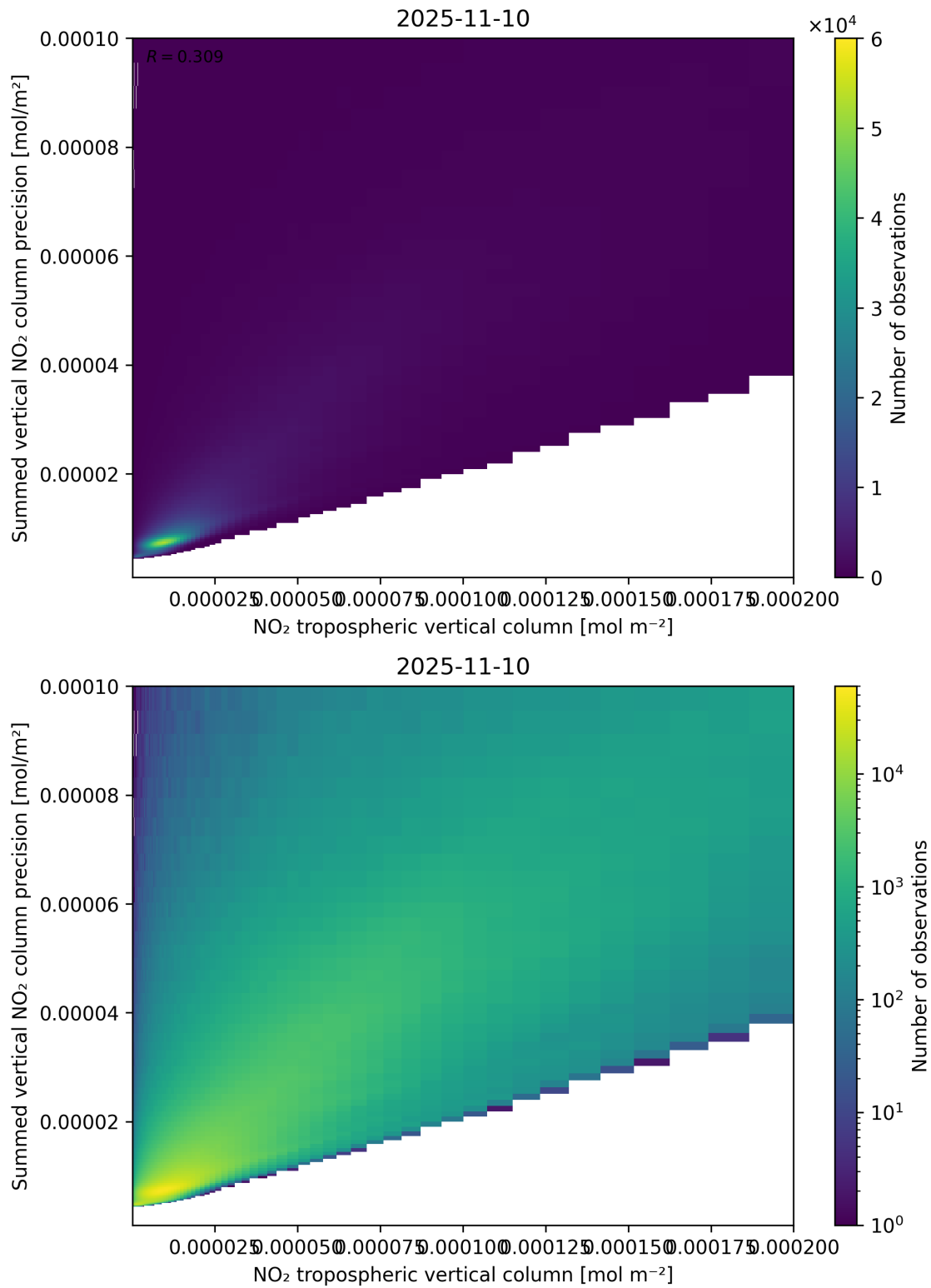
Figure 127: Scatter density plot of “NO 2 tropospheric vertical column” against “Summed vertical NO 2 column precision” for 2025-11-09 to 2025-11-11.
