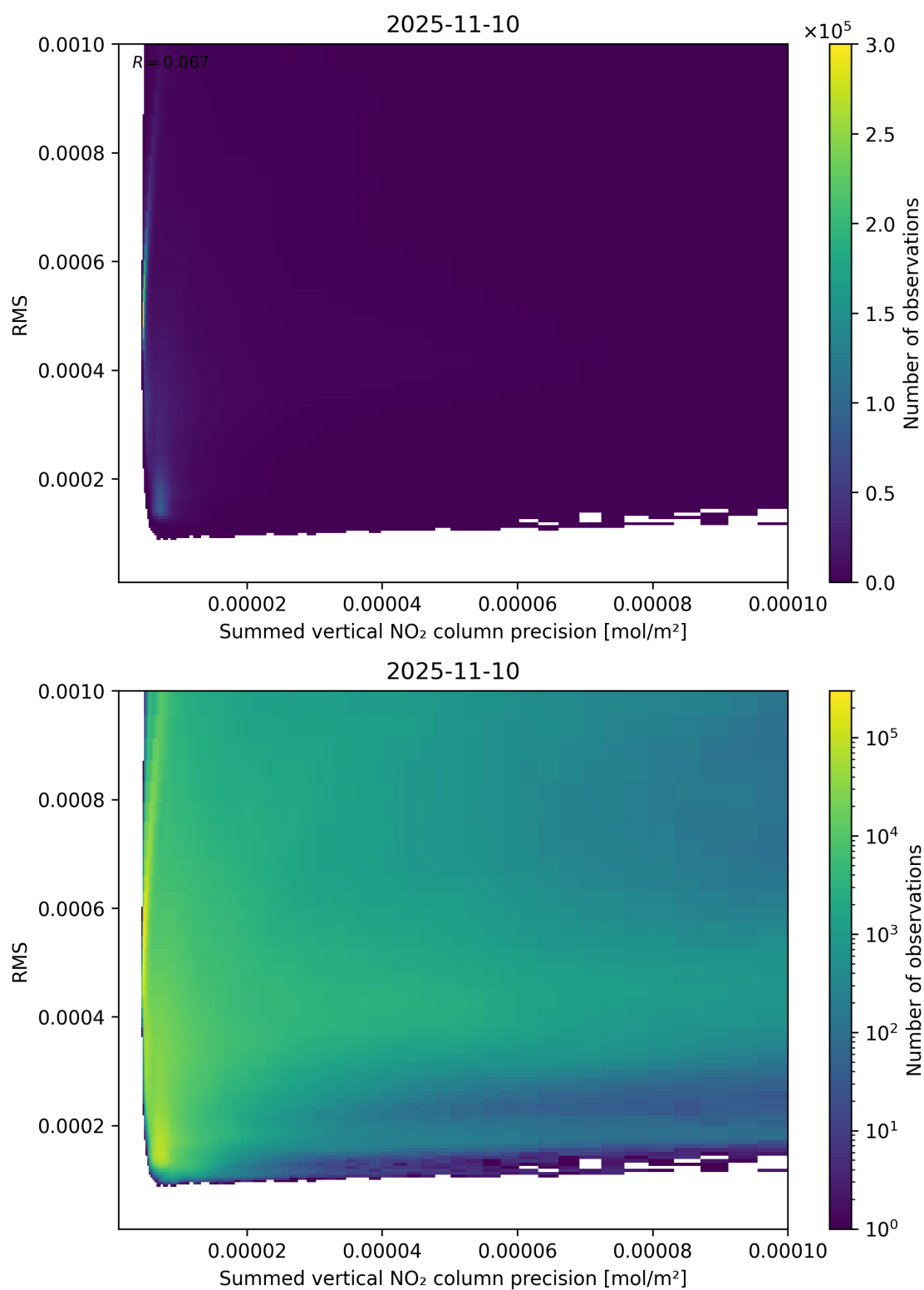
Figure 108: Scatter density plot of “Summed vertical NO 2 column precision” against “RMS” for 2025-11-09 to 2025-11-11.
