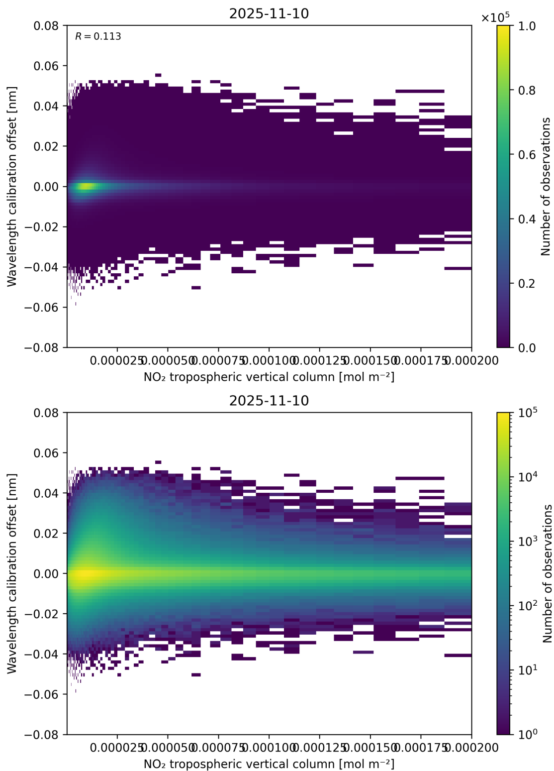
Figure 143: Scatter density plot of “NO 2 tropospheric vertical column” against “Wavelength calibration offset” for 2025-11-09 to 2025-11-11.
