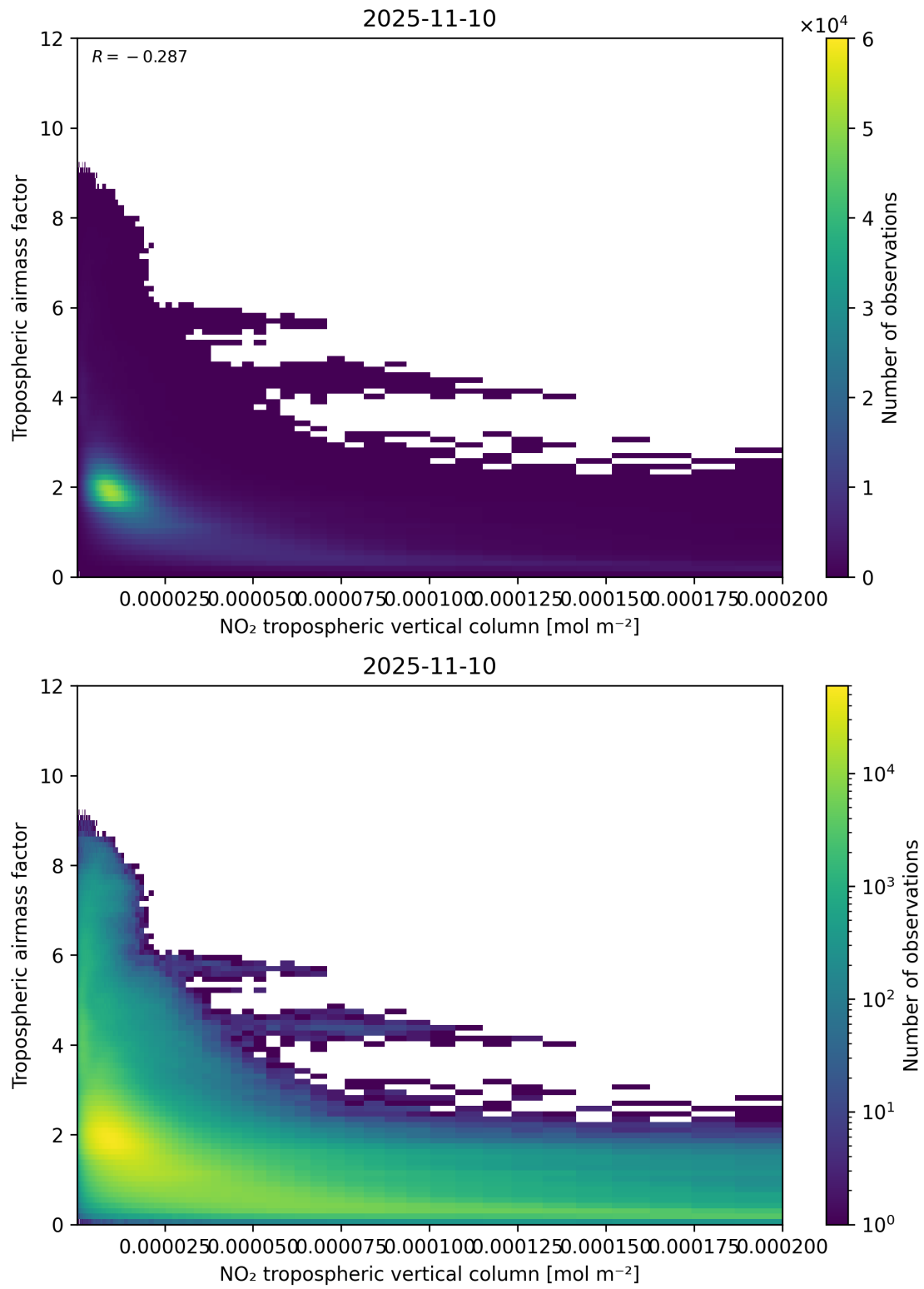
Figure 123: Scatter density plot of “NO 2 tropospheric vertical column” against “Tropospheric air mass factor” for 2025-11-09 to 2025-11-11.
