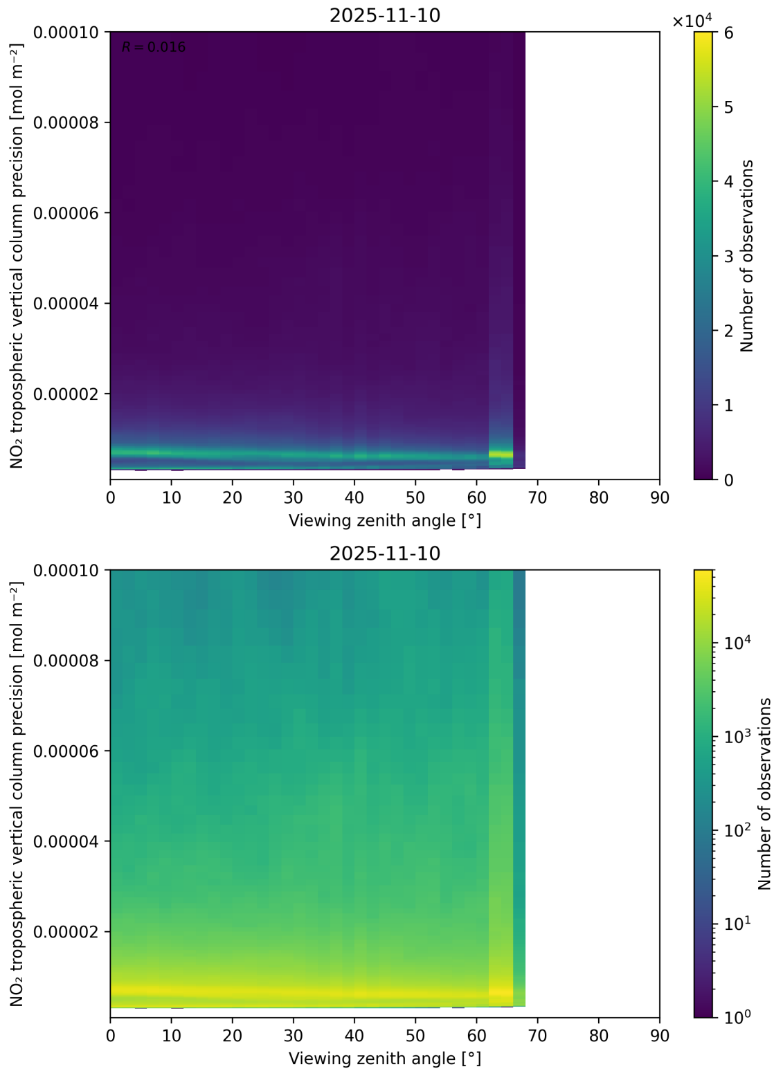
Figure 170: Scatter density plot of “Viewing zenith angle” against “NO 2 tropospheric vertical column precision” for 2025-11-09 to 2025-11-11.
