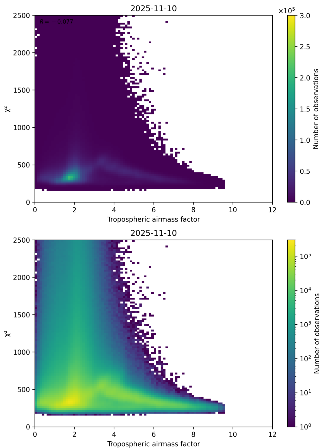
Figure 73: Scatter density plot of “Tropospheric airmass factor” against “ \chi^2 ” for 2025-11-09 to 2025-11-11.
