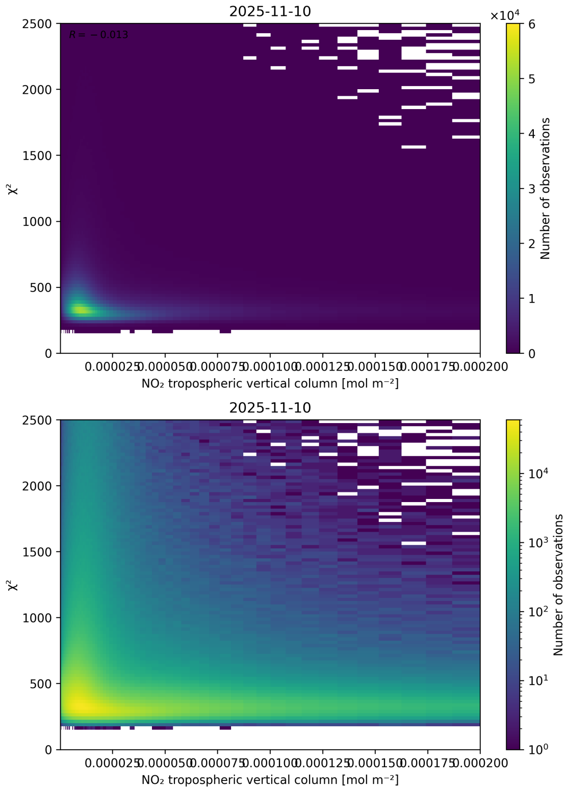
Figure 124: Scatter density plot of “NO 2 tropospheric vertical column” against “ \chi^2 ” for 2025-11-09 to 2025-11-11.
