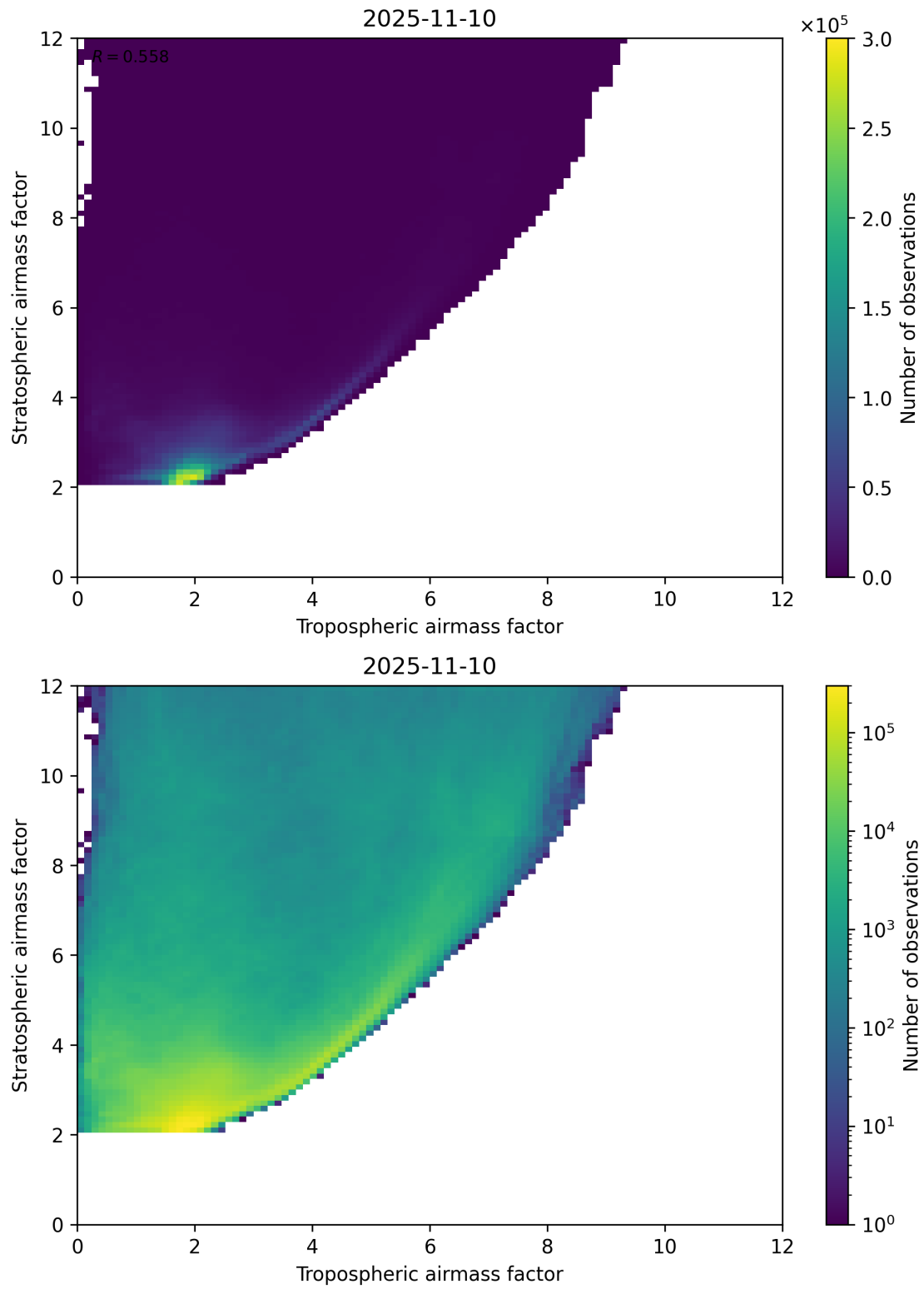
Figure 71: Scatter density plot of “Tropospheric airmass factor” against “Stratospheric airmass factor” for 2025-11-09 to 2025-11-11.
