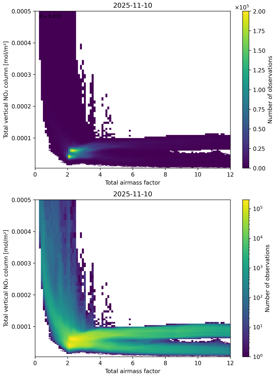
Figure 67: Scatter density plot of “Total airmass factor” against “Total vertical NO 2 column” for 2025-11-09 to 2025-11-11.
