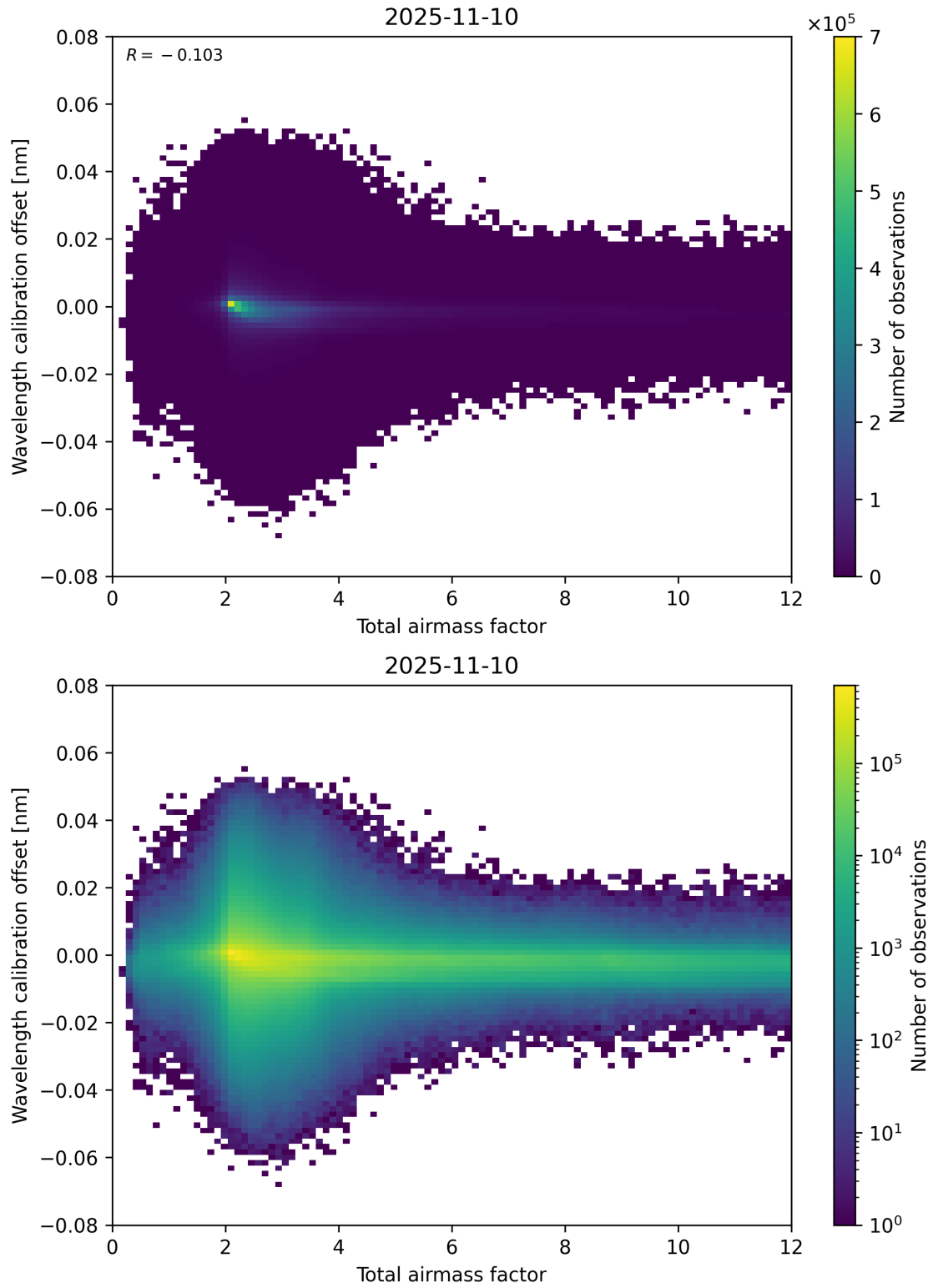
Figure 70: Scatter density plot of “Total airmass factor” against “Wavelength calibration offset” for 2025-11-09 to 2025-11-11.
