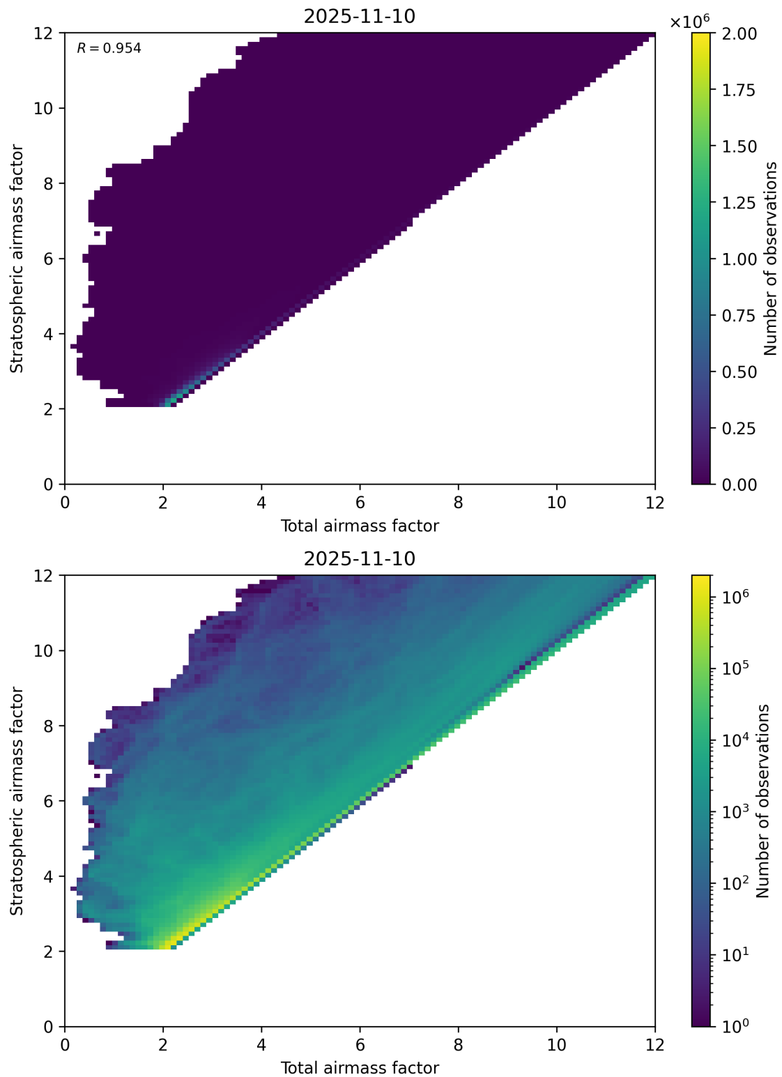
Figure 62: Scatter density plot of “Total airmass factor” against “Stratospheric airmass factor” for 2025-11-09 to 2025-11-11.
