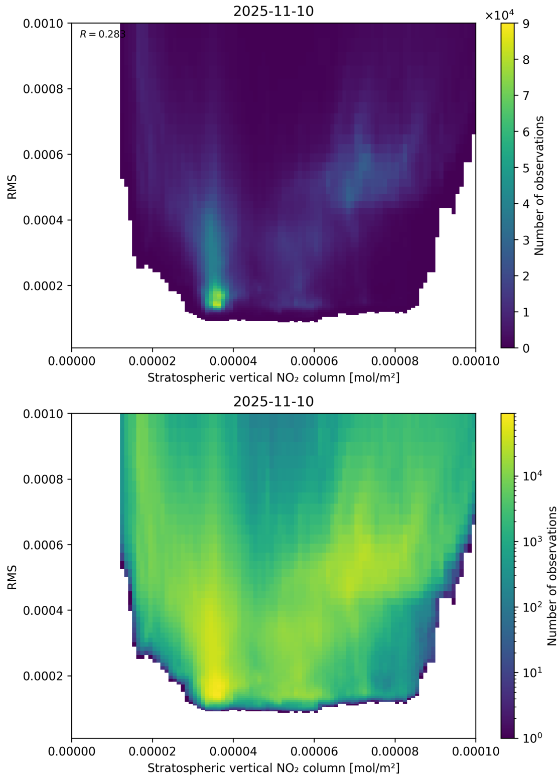
Figure 102: Scatter density plot of “Stratospheric vertical NO 2 column” against “RMS” for 2025-11-09 to 2025-11-11.
