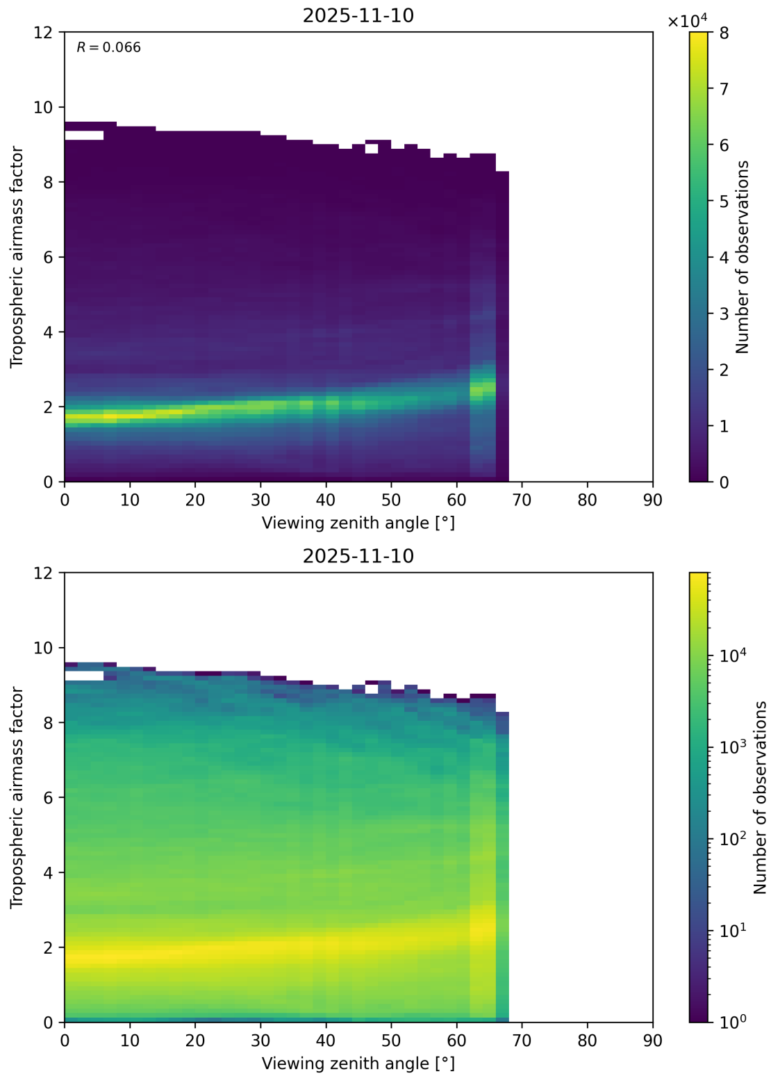
Figure 161: Scatter density plot of “Viewing zenith angle” against “Tropospheric airmass factor” for 2025-11-09 to 2025-11-11.
