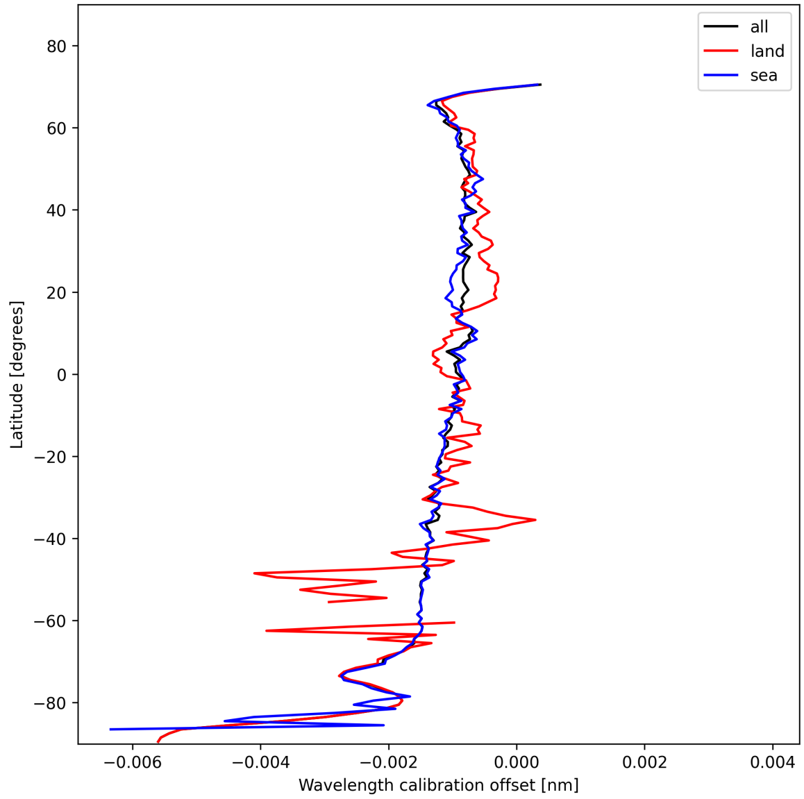
Figure 18: Zonal average of “Wavelength calibration offset” for 2025-11-09 to 2025-11-11.
