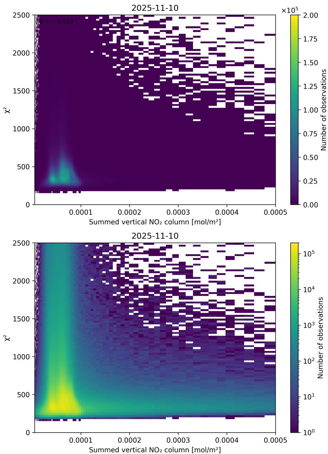
Figure 104: Scatter density plot of “Summed vertical NO 2 column” against “ \chi^2 ” for 2025-11-09 to 2025-11-11.
