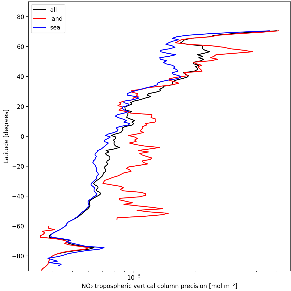
Figure 13: Zonal average of “NO 2 tropospheric vertical column precision” for 2025-11-09 to 2025-11-11.
