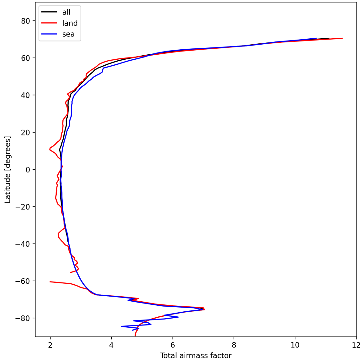
Figure 15: Zonal average of “Total airmass factor” for 2025-11-09 to 2025-11-11.
