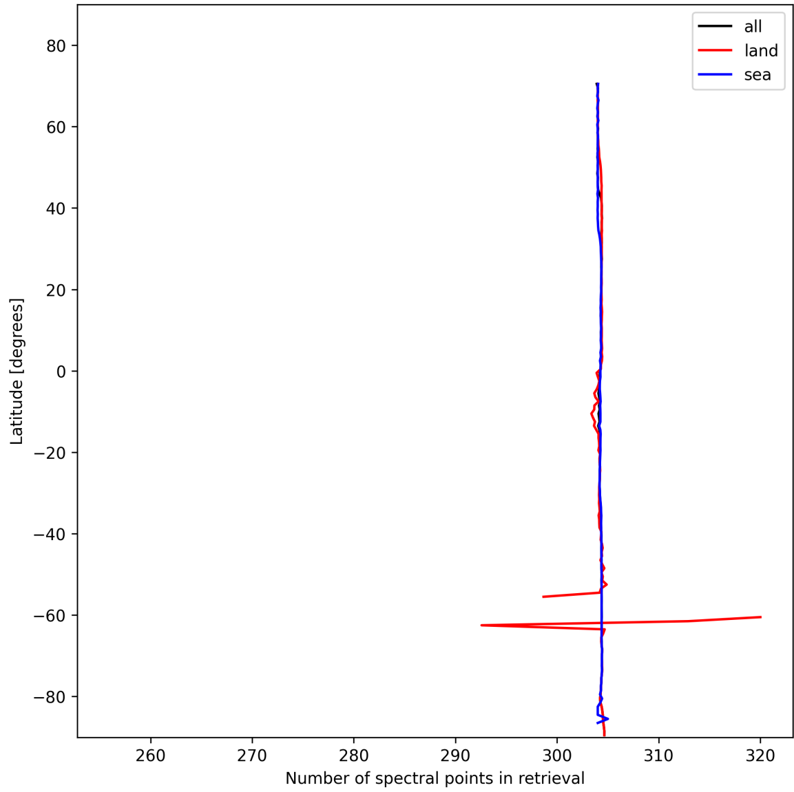
Figure 16: Zonal average of “Number of spectral points in retrieval” for 2025-11-09 to 2025-11-11.
