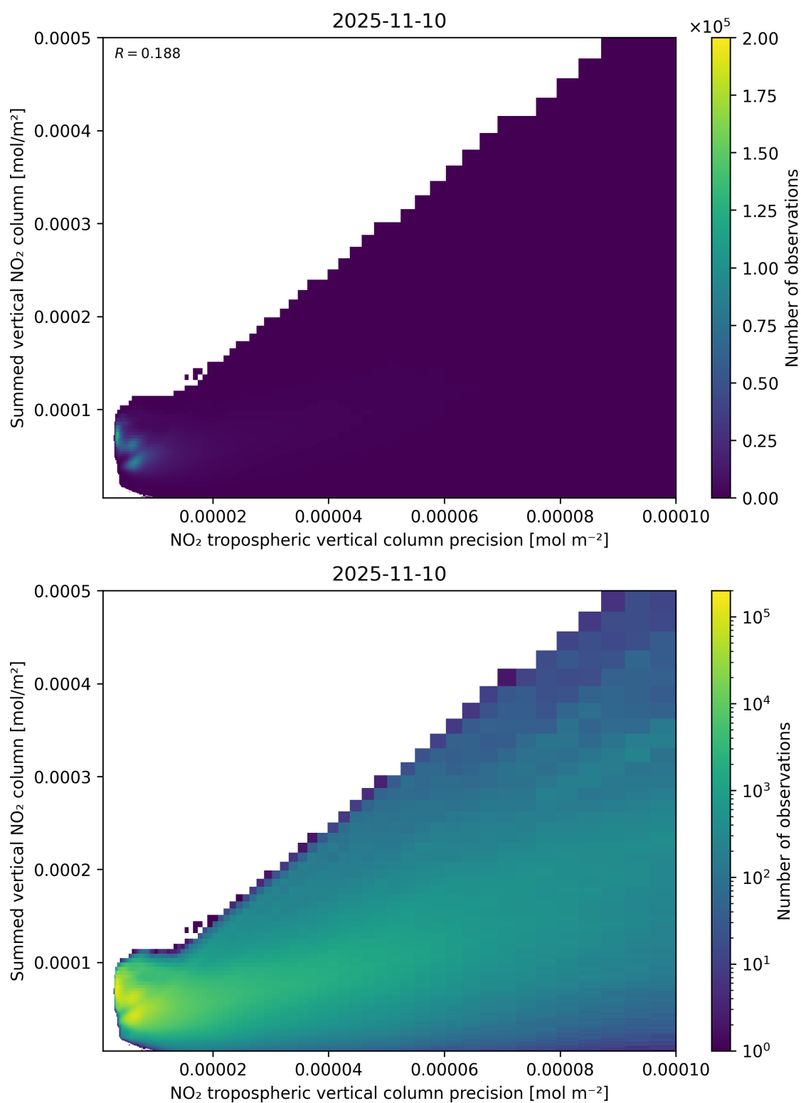
Figure 136: Scatter density plot of “NO 2 tropospheric vertical column precision” against “Summed vertical NO 2 column” for 2025-11-09 to 2025-11-11.
