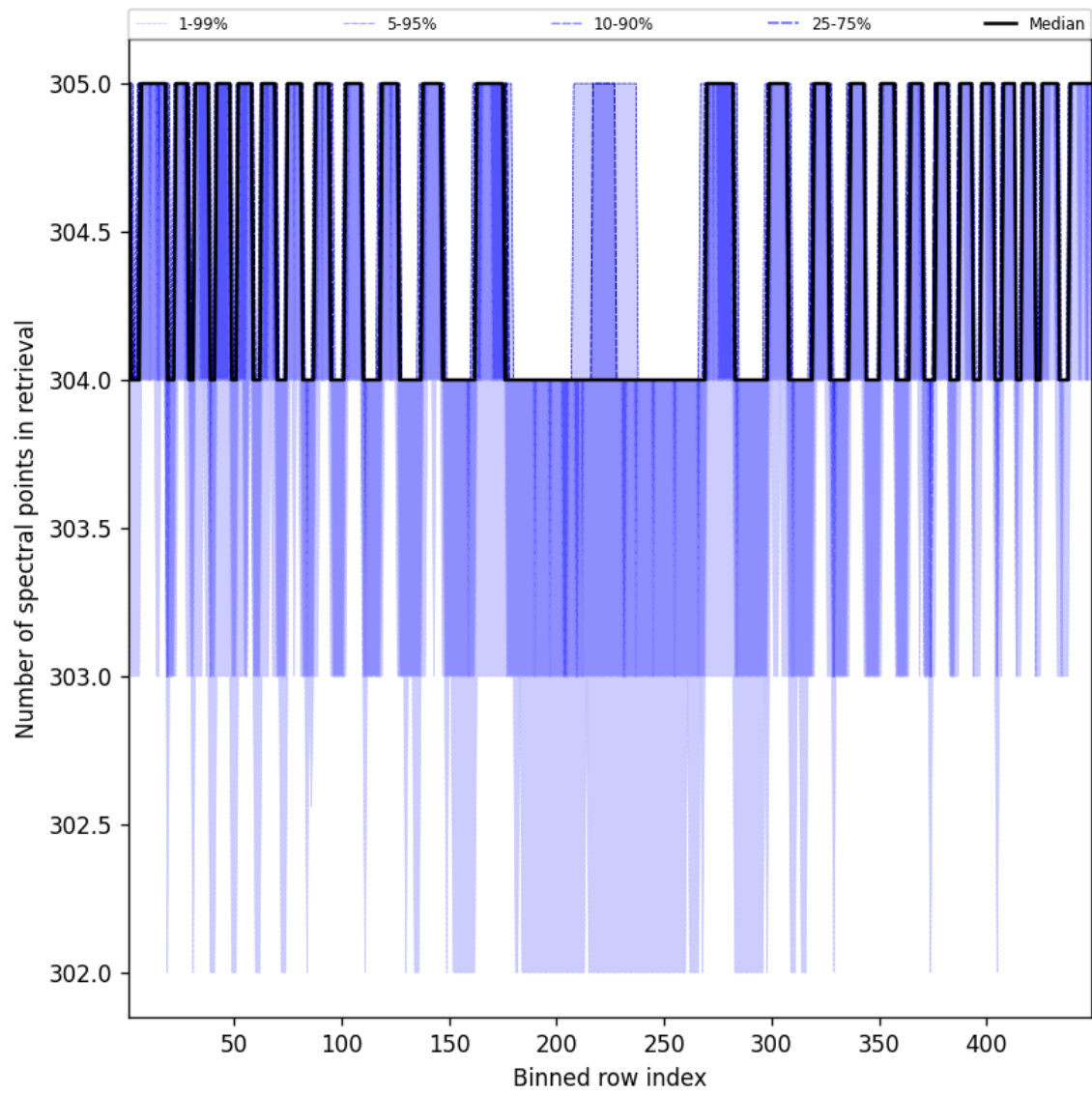
Figure 50: Along track statistics of “Number of spectral points in retrieval” for 2025-11-09 to 2025-11-11
