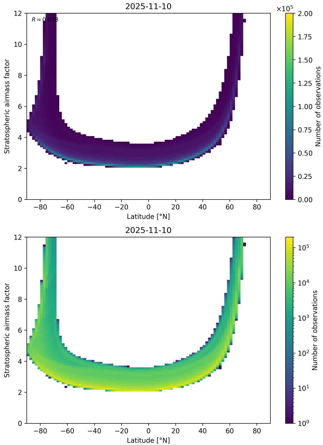
Figure 83: Scatter density plot of “Latitude” against “Stratospheric airmass factor” for 2025-11-09 to 2025-11-11.
