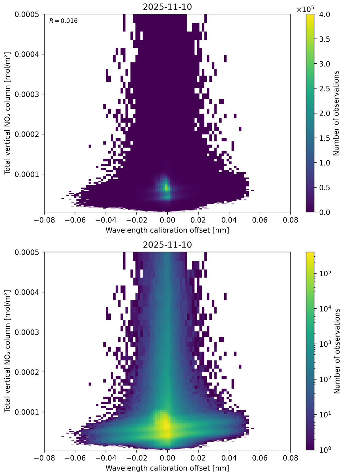
Figure 179: Scatter density plot of “Wavelength calibration offset” against “Total vertical NO 2 column” for 2025-11-09 to 2025-11-11.
