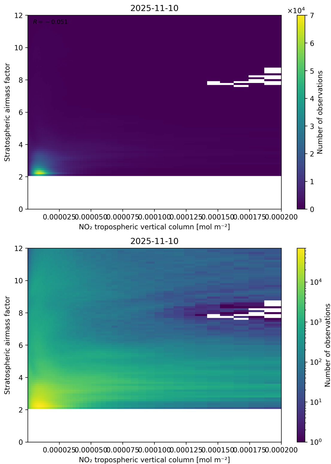
Figure 121: Scatter density plot of “NO 2 tropospheric vertical column” against “Stratospheric airmass factor” for 2025-11-09 to 2025-11-11.
