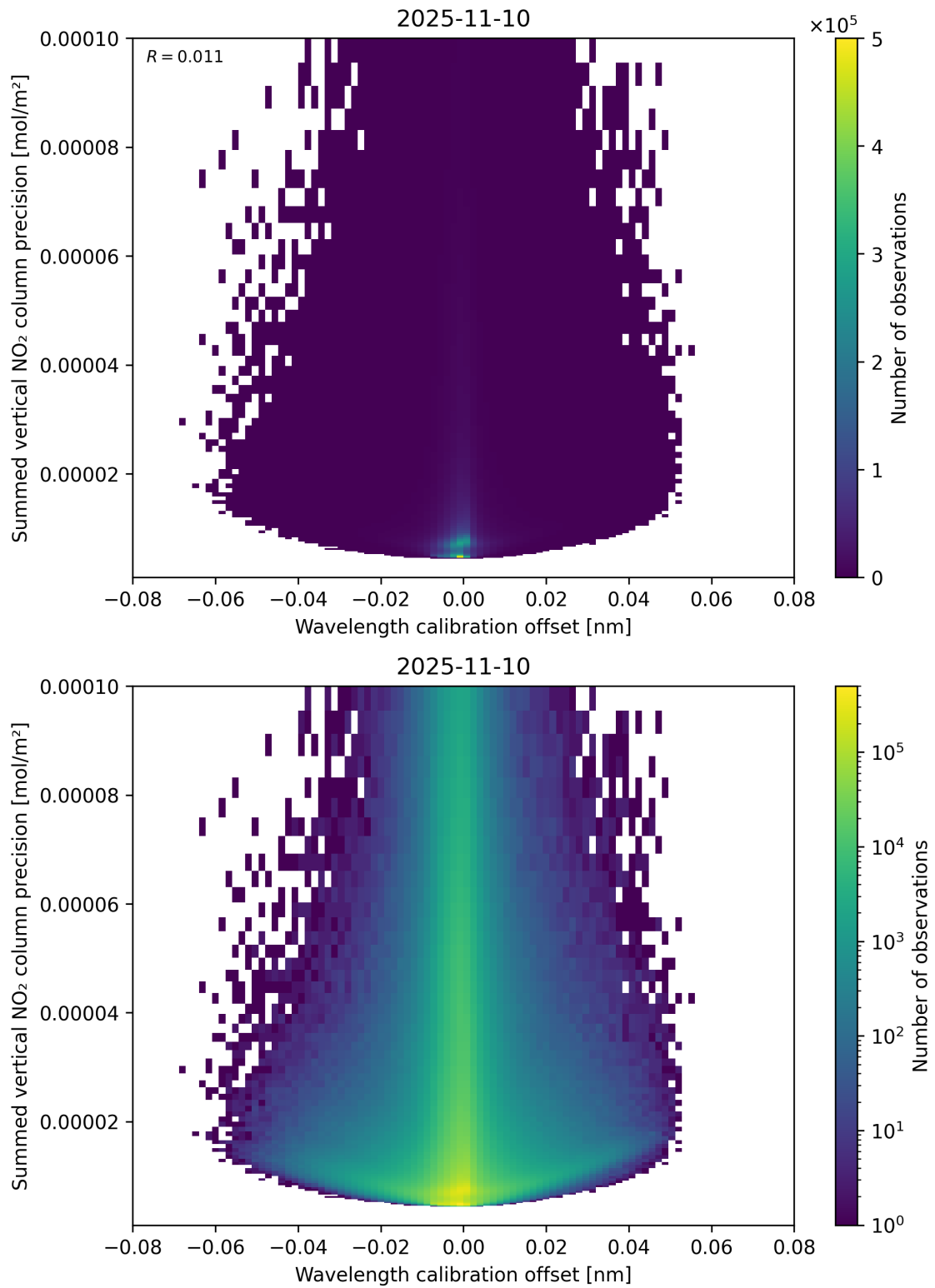
Figure 178: Scatter density plot of “Wavelength calibration offset” against “Summed vertical NO 2 column precision” for 2025-11-09 to 2025-11-11.
