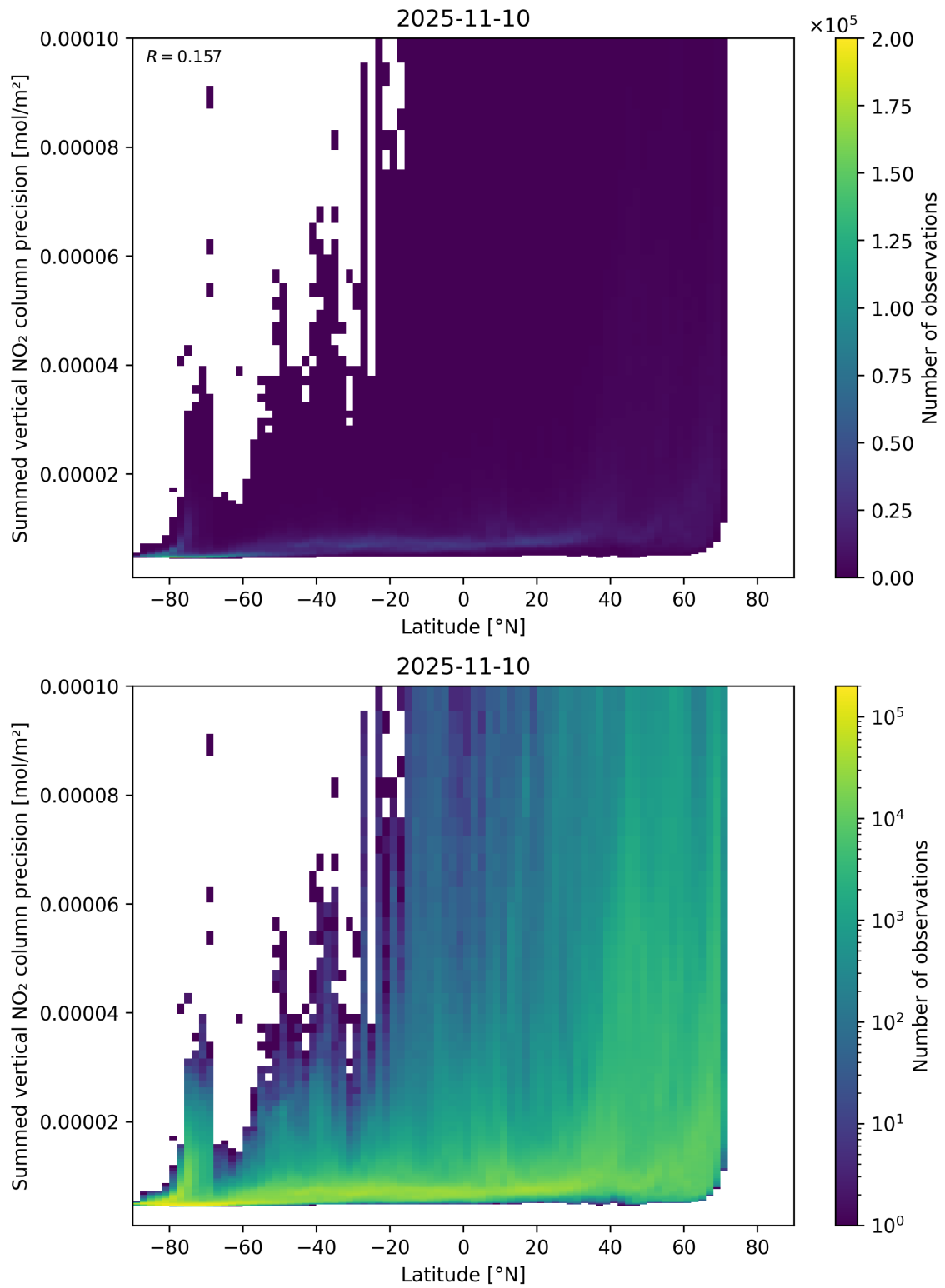
Figure 89: Scatter density plot of “Latitude” against “Summed vertical NO 2 column precision” for 2025-11-09 to 2025-11-11.
