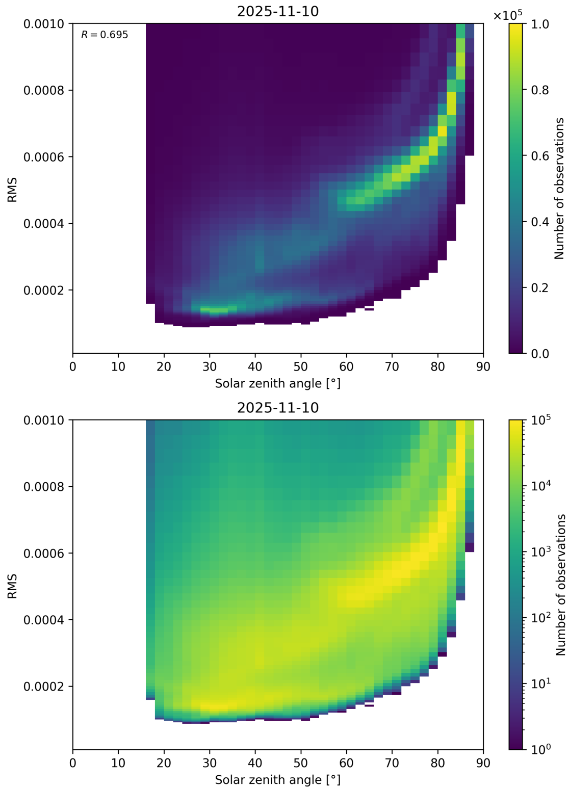
Figure 157: Scatter density plot of “Solar zenith angle” against “RMS” for 2025-11-09 to 2025-11-11.
