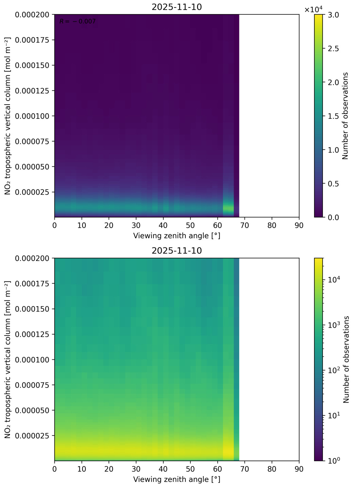
Figure 169: Scatter density plot of “Viewing zenith angle” against “NO 2 tropospheric vertical column” for 2025-11-09 to 2025-11-11.
