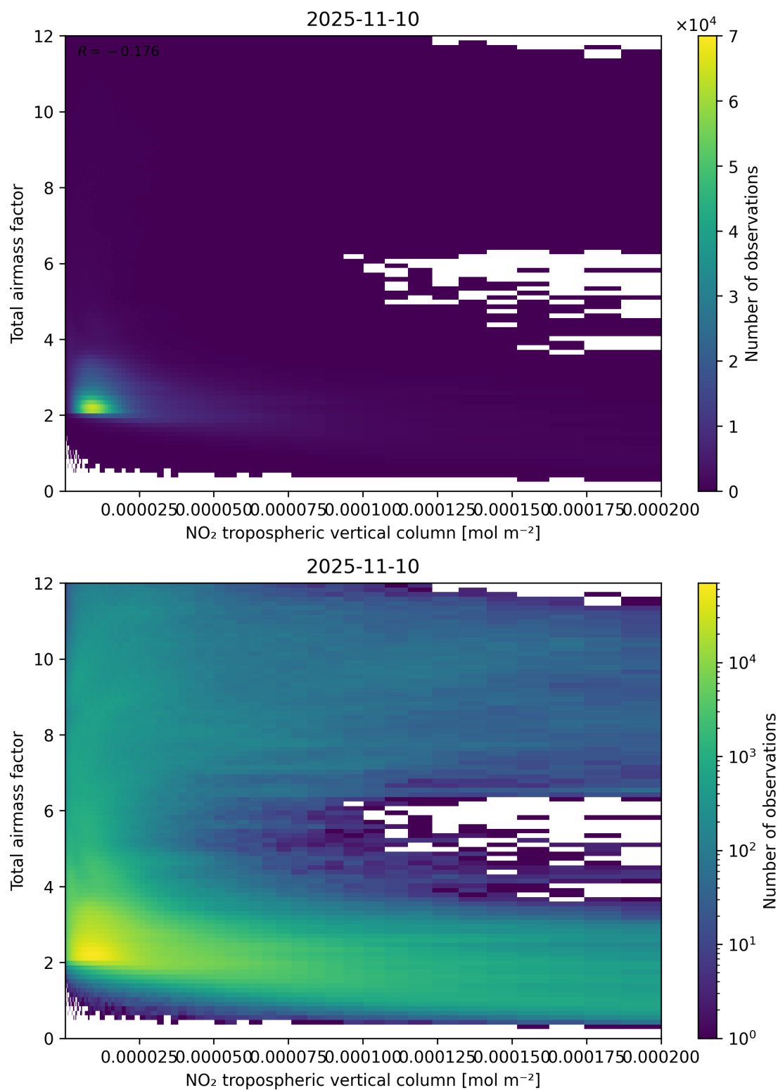
Figure 122: Scatter density plot of “NO 2 tropospheric vertical column” against “Total air mass factor” for 2025-11-09 to 2025-11-11.
