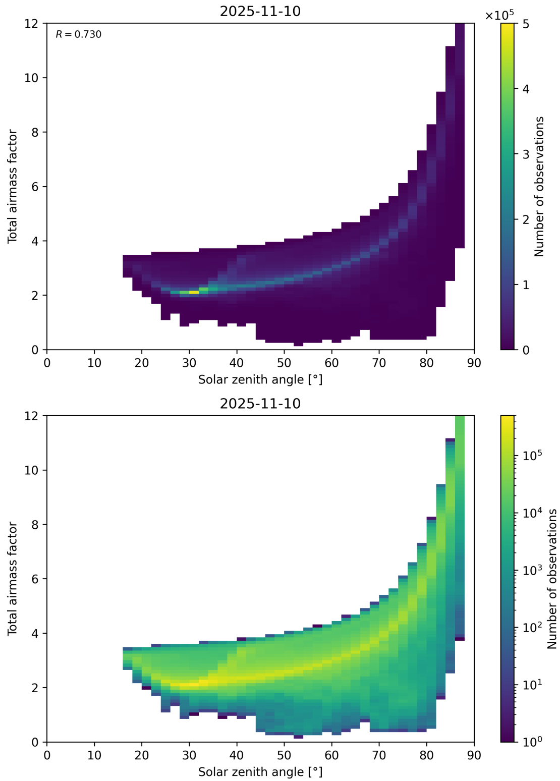
Figure 146: Scatter density plot of “Solar zenith angle” against “Total air mass factor” for 2025-11-09 to 2025-11-11.
