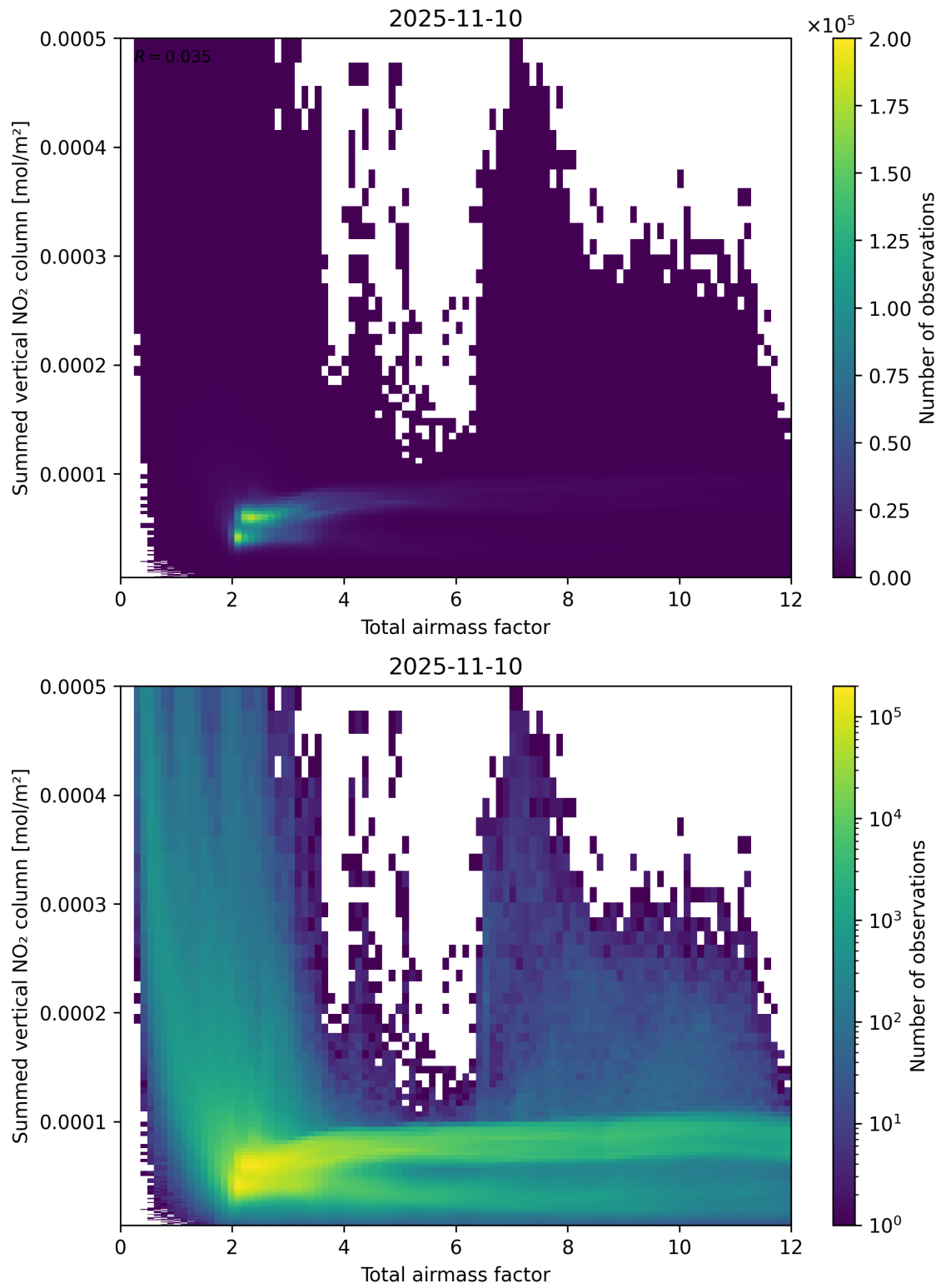
Figure 65: Scatter density plot of “Total airmass factor” against “Summed vertical NO 2 column” for 2025-11-09 to 2025-11-11.
