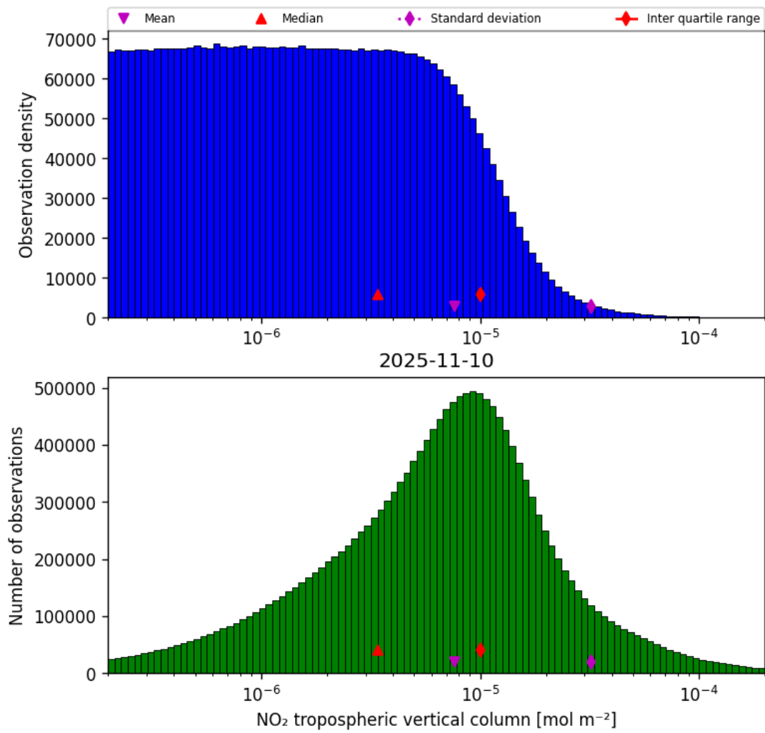
Figure 29: Histogram of “NO 2 tropospheric vertical column” for 2025-11-09 to 2025-11-11
