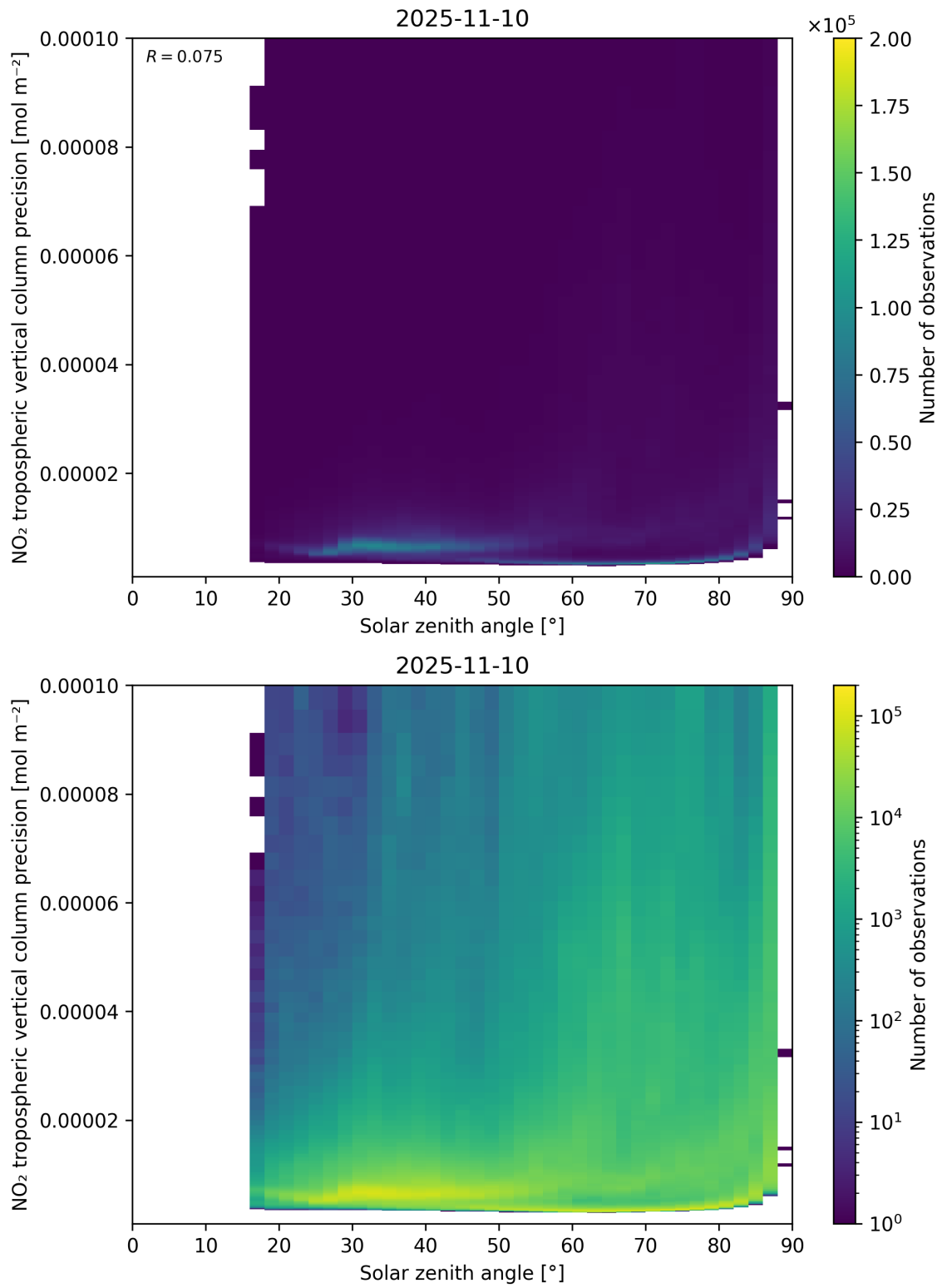
Figure 156: Scatter density plot of “Solar zenith angle” against “NO 2 tropospheric vertical column precision” for 2025-11-09 to 2025-11-11.
