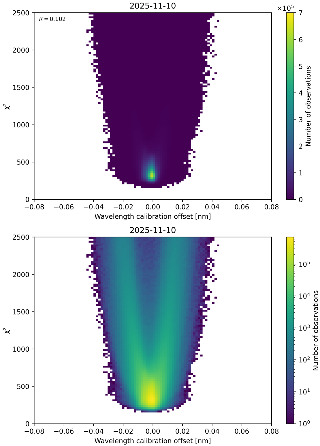
Figure 175: Scatter density plot of “Wavelength calibration offset” against “ \chi^2 ” for 2025-11-09 to 2025-11-11.
