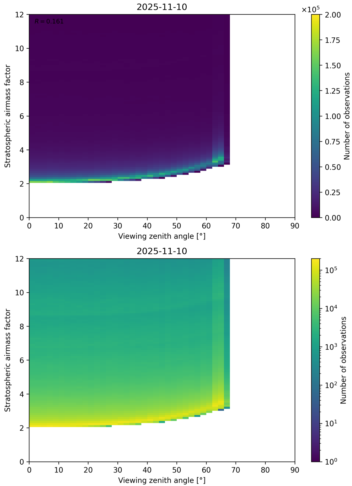
Figure 159: Scatter density plot of “Viewing zenith angle” against “Stratospheric airmass factor” for 2025-11-09 to 2025-11-11.
