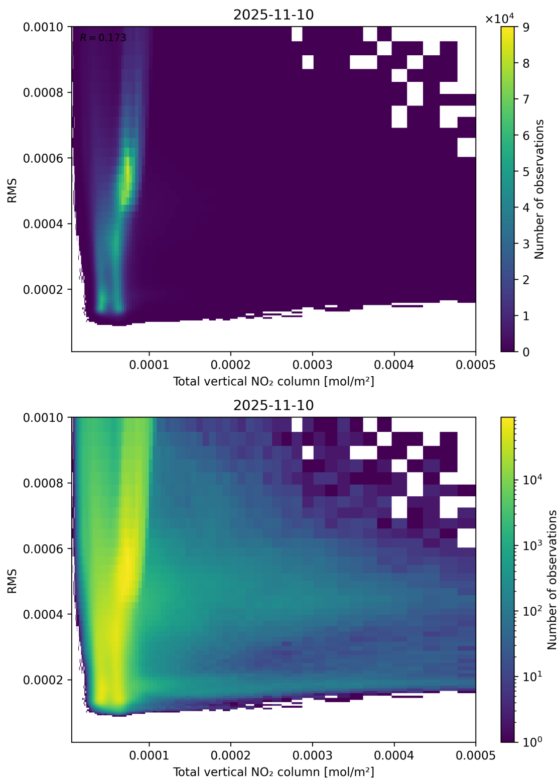
Figure 120: Scatter density plot of “Total vertical NO 2 column” against “RMS” for 2025-11-09 to 2025-11-11.
