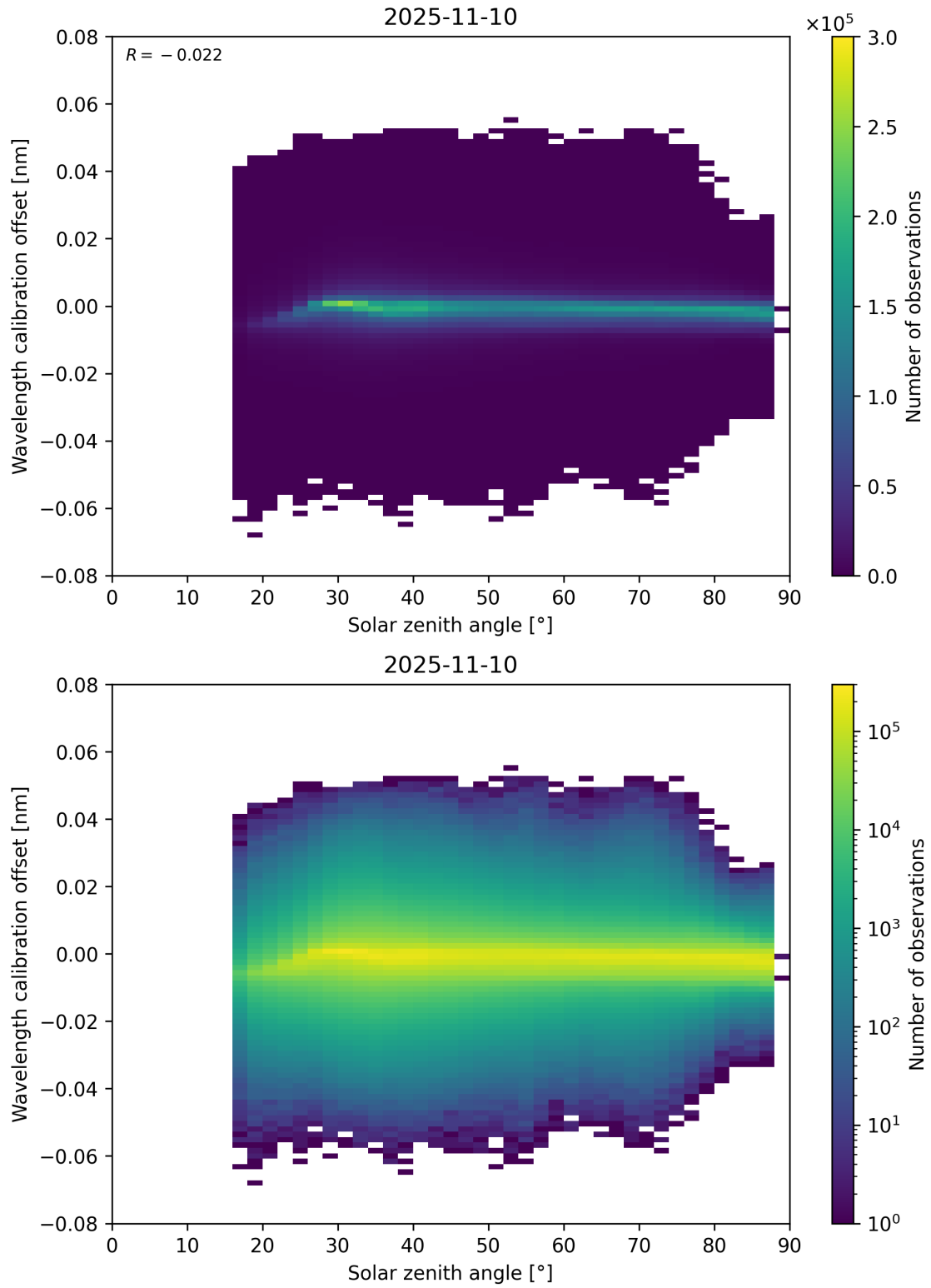
Figure 158: Scatter density plot of “Solar zenith angle” against “Wavelength calibration offset” for 2025-11-09 to 2025-11-11.
