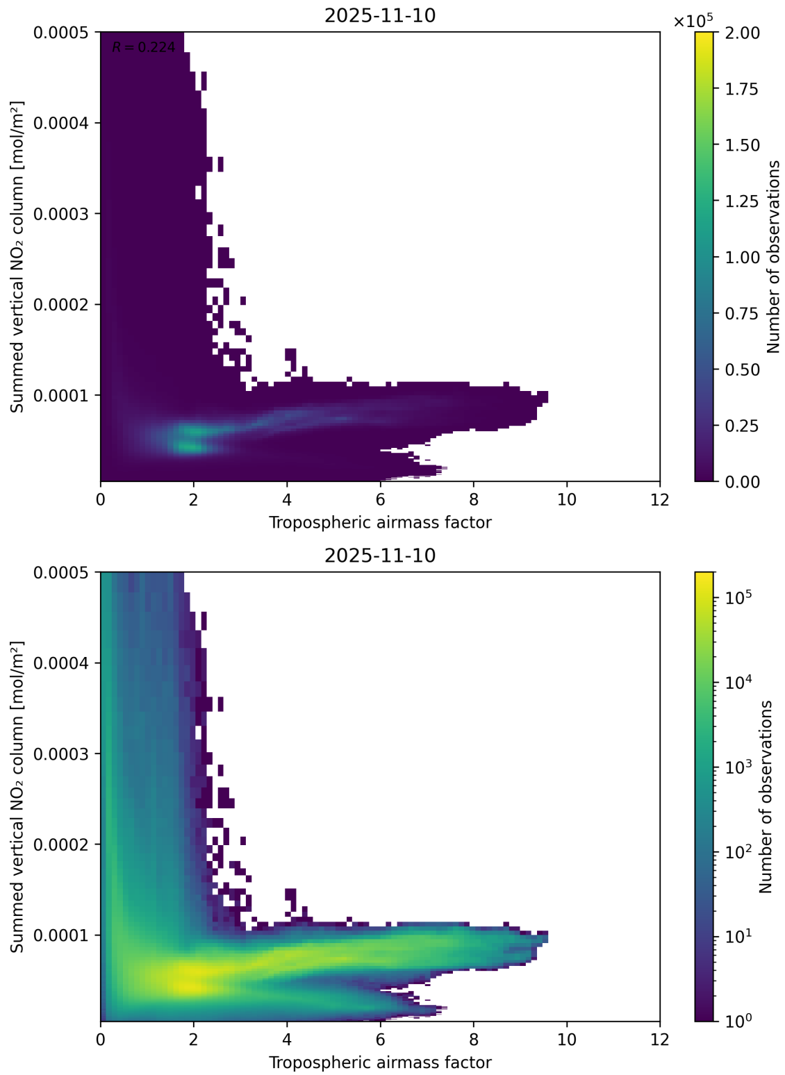
Figure 75: Scatter density plot of “Tropospheric air mass factor” against “Summed vertical NO 2 column” for 2025-11-09 to 2025-11-11.
