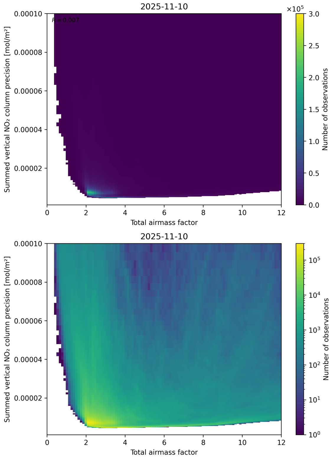
Figure 66: Scatter density plot of “Total airmass factor” against “Summed vertical NO 2 column precision” for 2025-11-09 to 2025-11-11.
