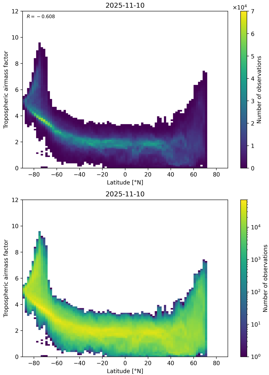
Figure 85: Scatter density plot of “Latitude” against “Tropospheric airmass factor” for 2025-11-09 to 2025-11-11.
