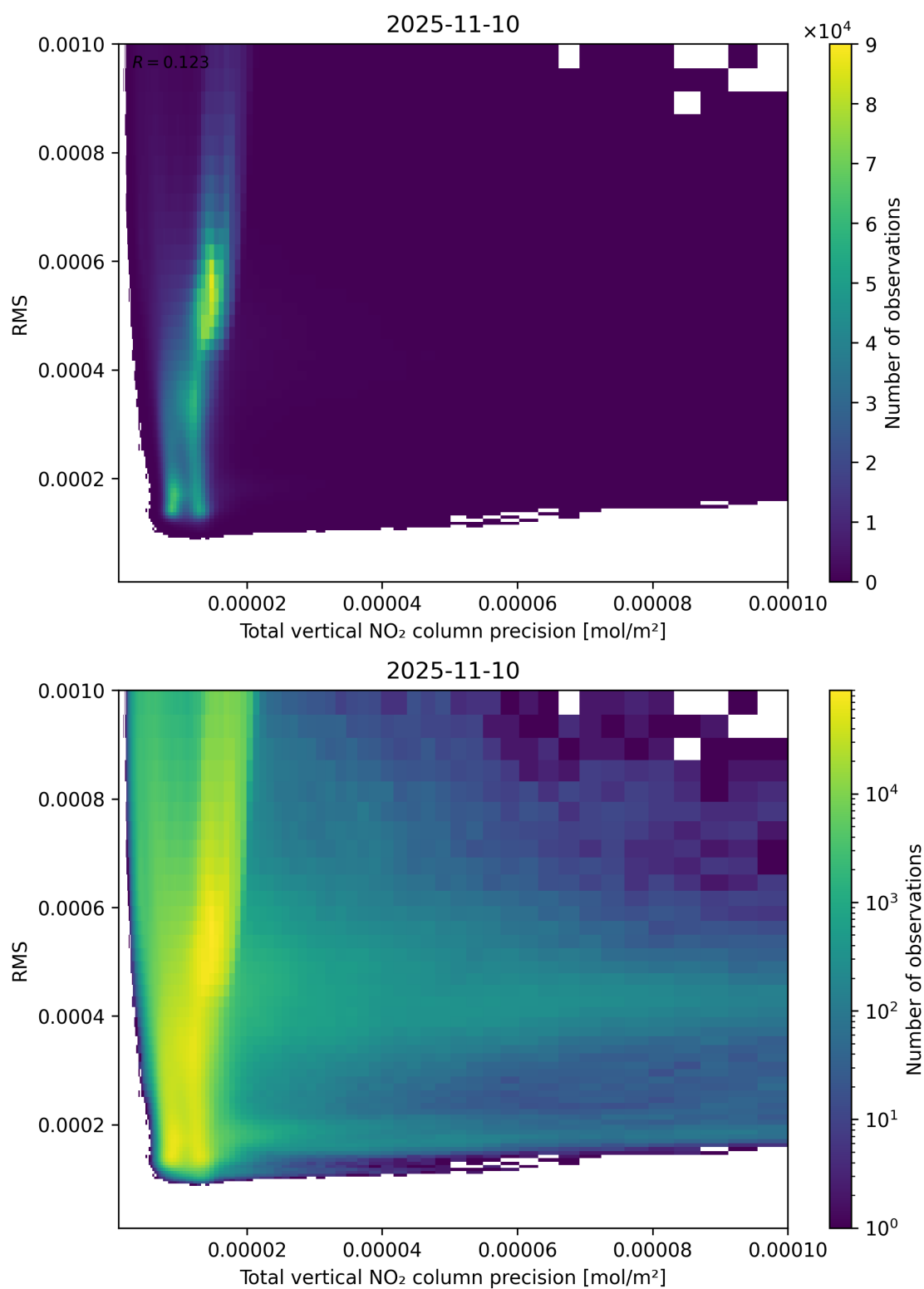
Figure 119: Scatter density plot of “Total vertical NO 2 column precision” against “RMS” for 2025-11-09 to 2025-11-11.
