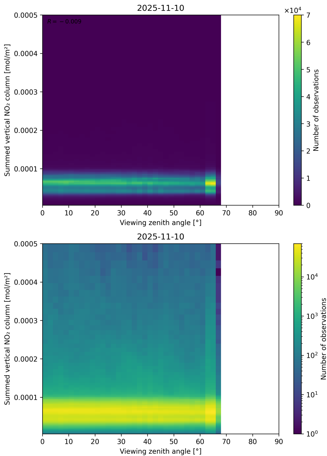
Figure 165: Scatter density plot of “Viewing zenith angle” against “Summed vertical NO 2 column” for 2025-11-09 to 2025-11-11.
