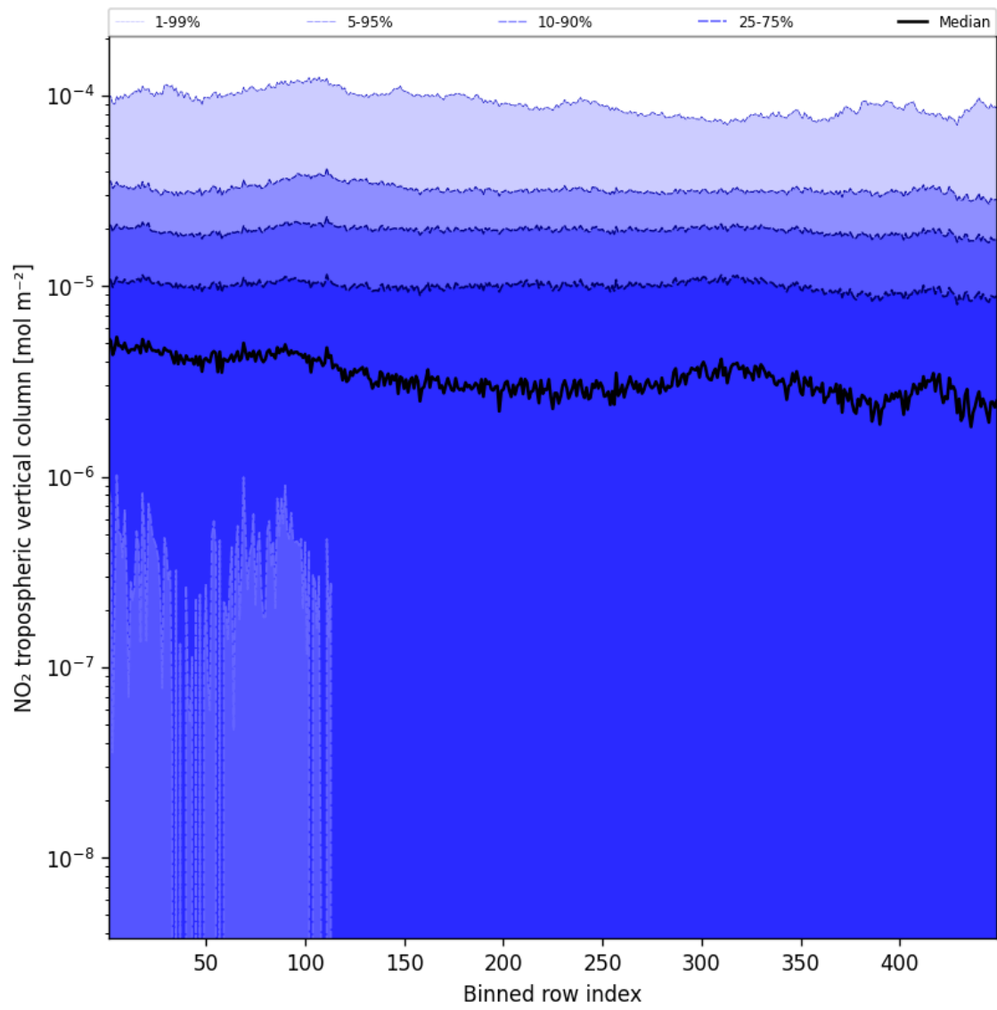
Figure 46: Along track statistics of “NO 2 tropospheric vertical column” for 2025-11-09 to 2025-11-11
