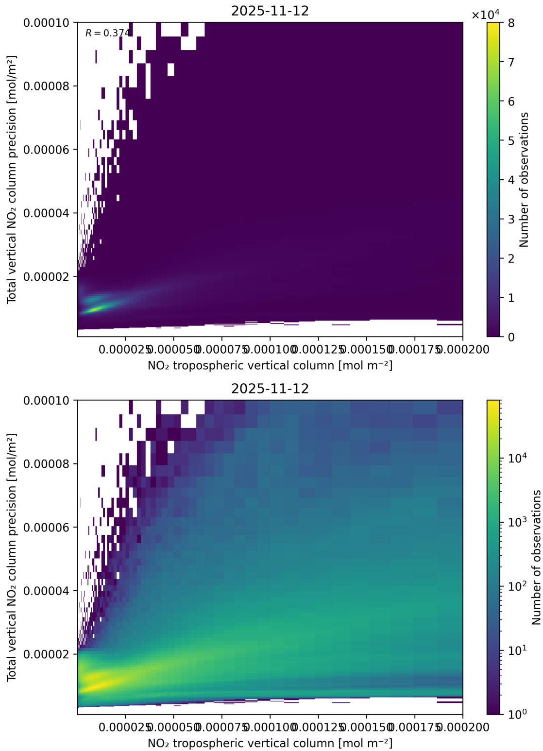
Figure 129: Scatter density plot of “NO 2 tropospheric vertical column” against “Total vertical NO 2 column precision” for 2025-11-12 to 2025-11-13.
