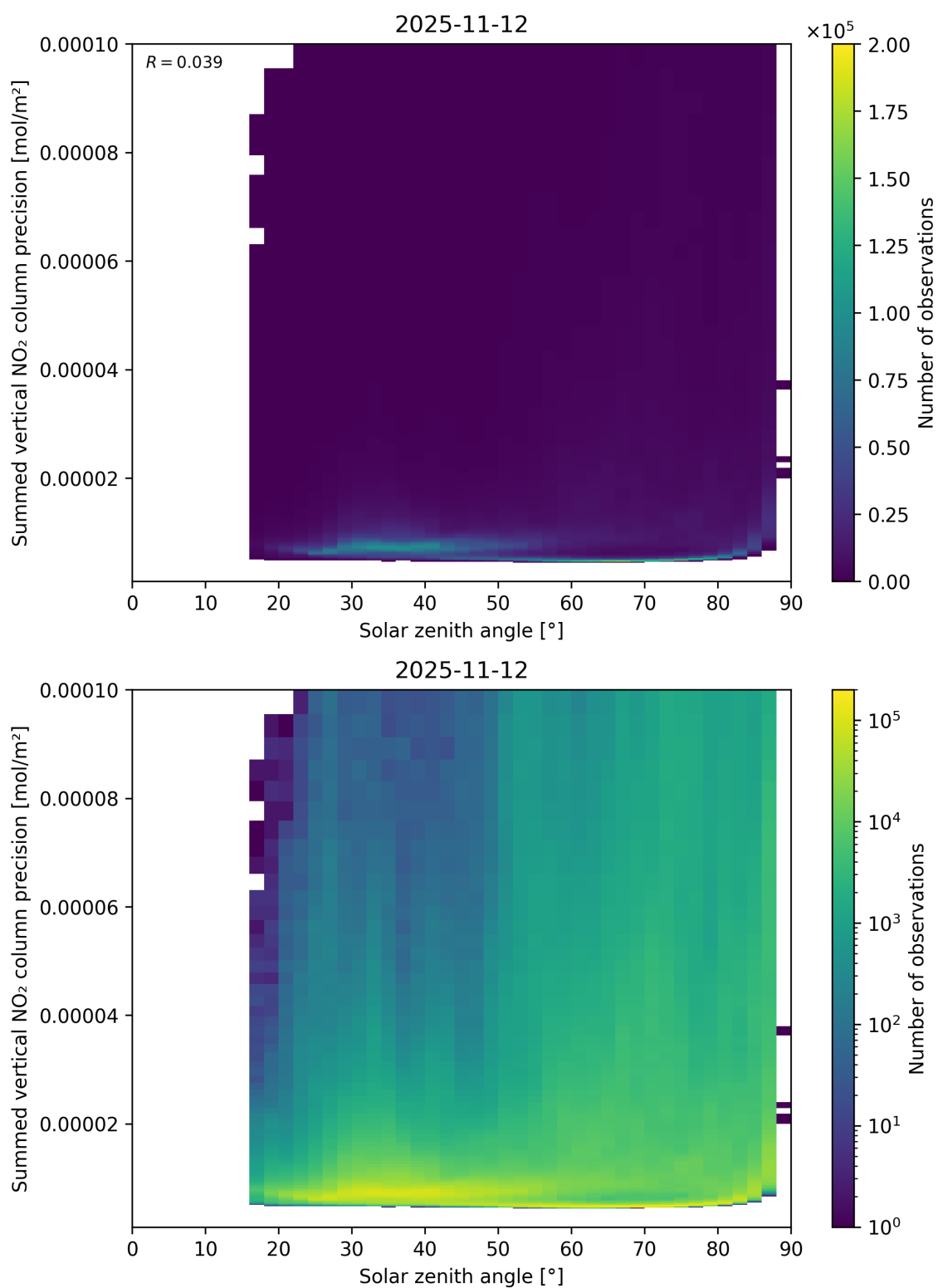
Figure 152: Scatter density plot of “Solar zenith angle” against “Summed vertical NO 2 column precision” for 2025-11-12 to 2025-11-13.
