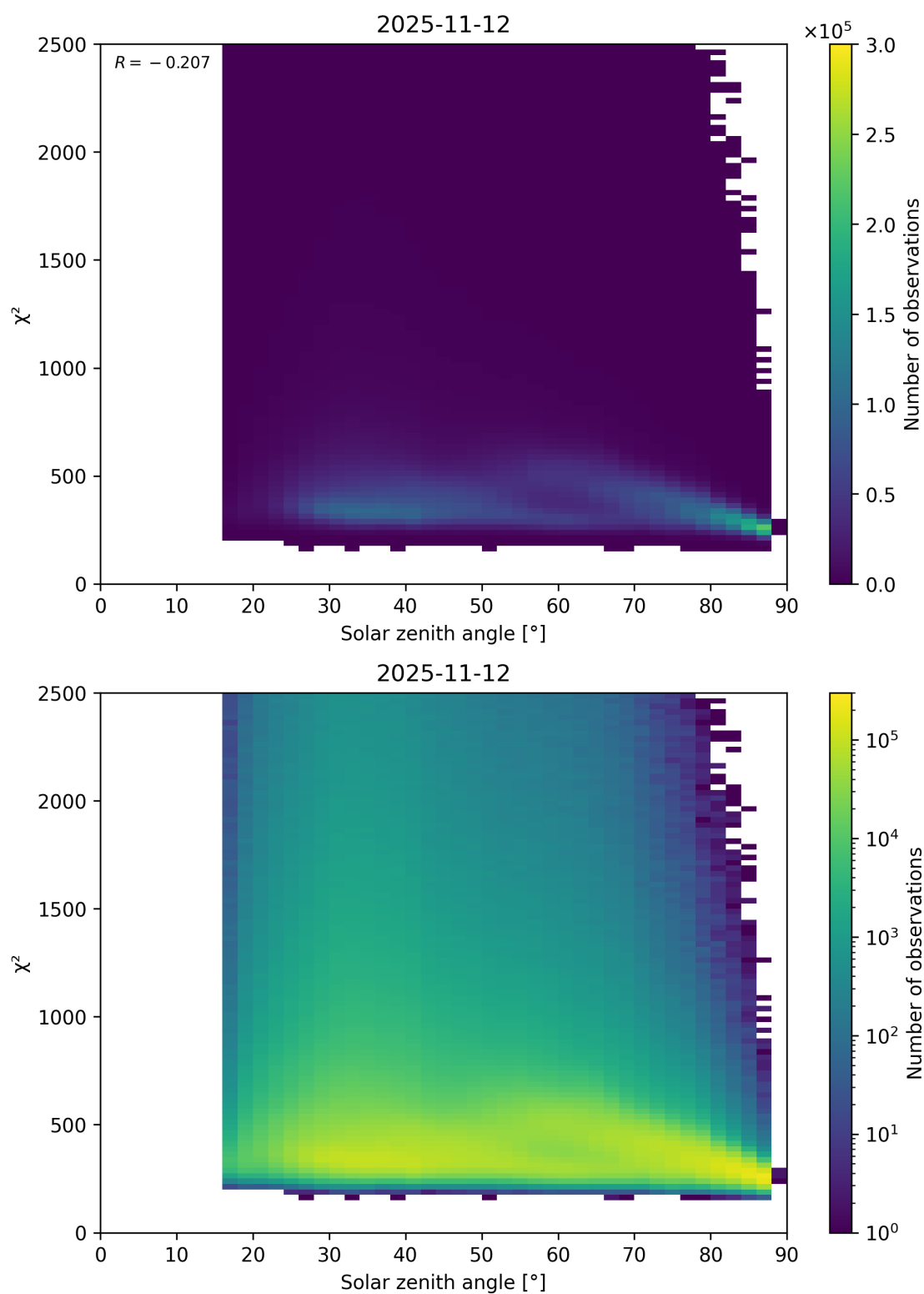
Figure 148: Scatter density plot of “Solar zenith angle” against “ \chi^2 ” for 2025-11-12 to 2025-11-13.
