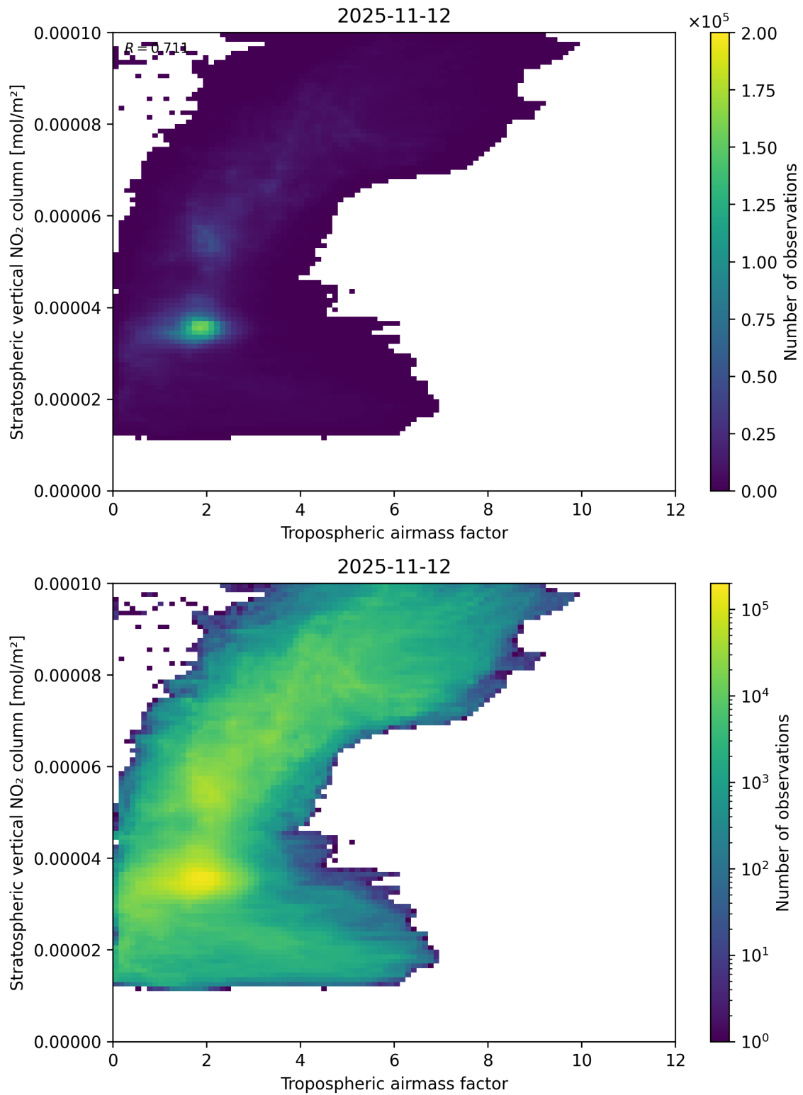
Figure 74: Scatter density plot of “Tropospheric air mass factor” against “Stratospheric vertical NO 2 column” for 2025-11-12 to 2025-11-13.
