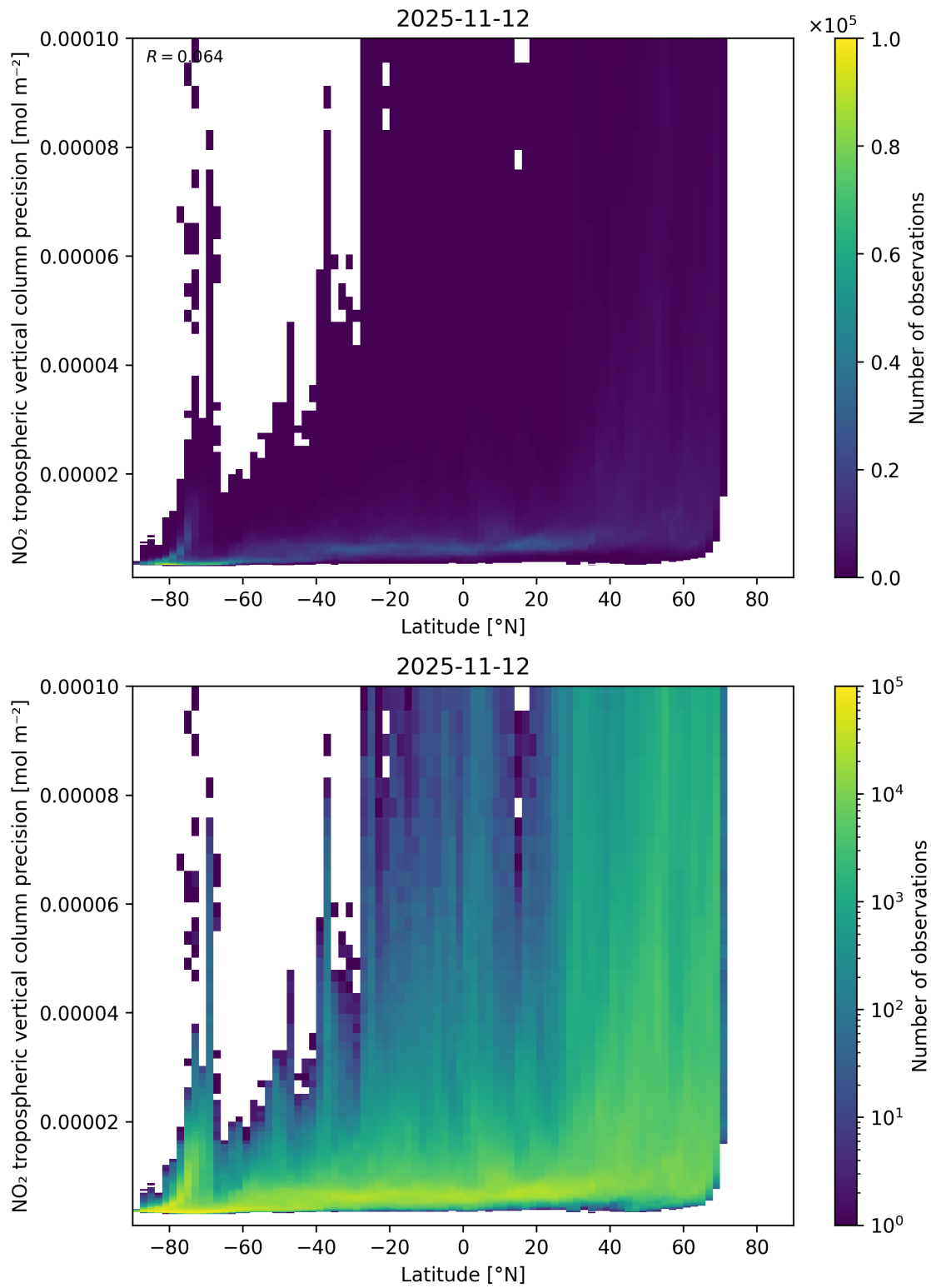
Figure 93: Scatter density plot of “Latitude” against “NO 2 tropospheric vertical column precision” for 2025-11-12 to 2025-11-13.
