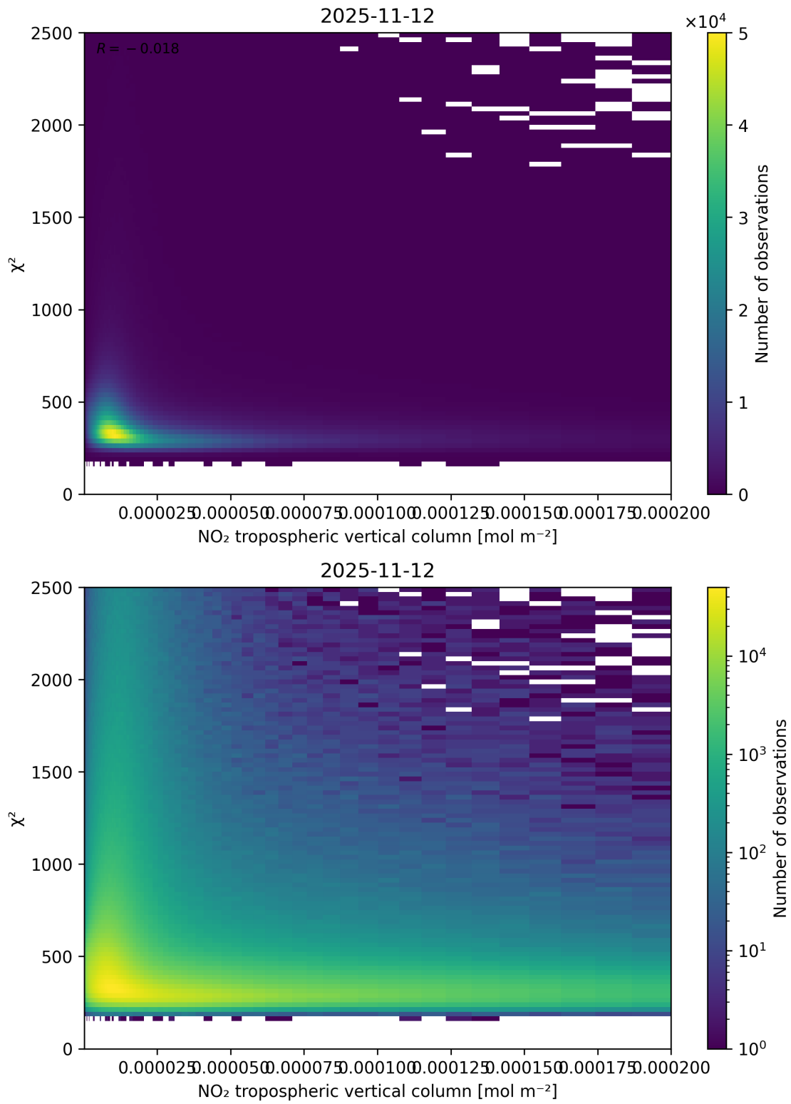
Figure 124: Scatter density plot of “NO 2 tropospheric vertical column” against “ \chi^2 ” for 2025-11-12 to 2025-11-13.
