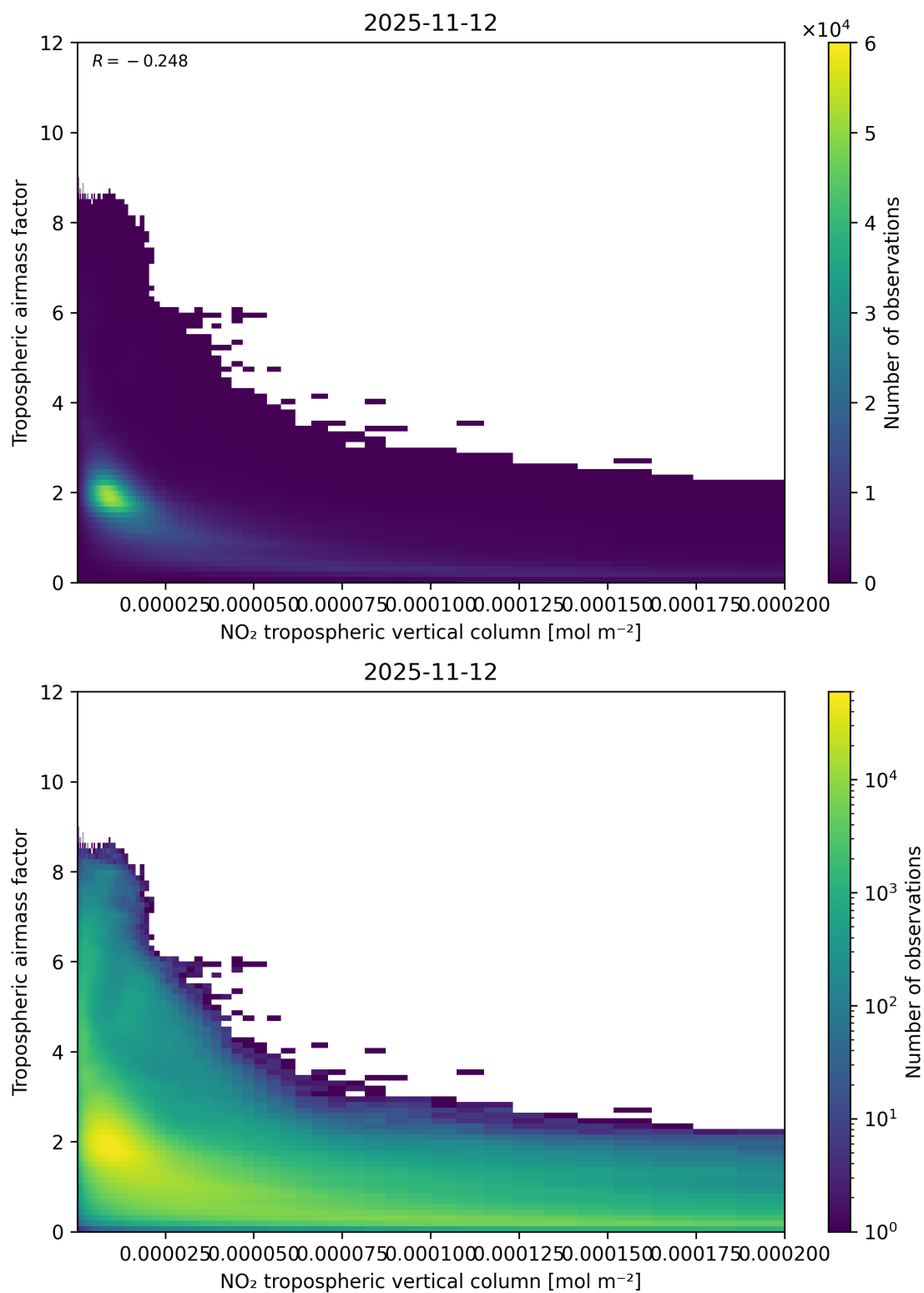
Figure 123: Scatter density plot of “NO 2 tropospheric vertical column” against “Tropospheric air mass factor” for 2025-11-12 to 2025-11-13.
