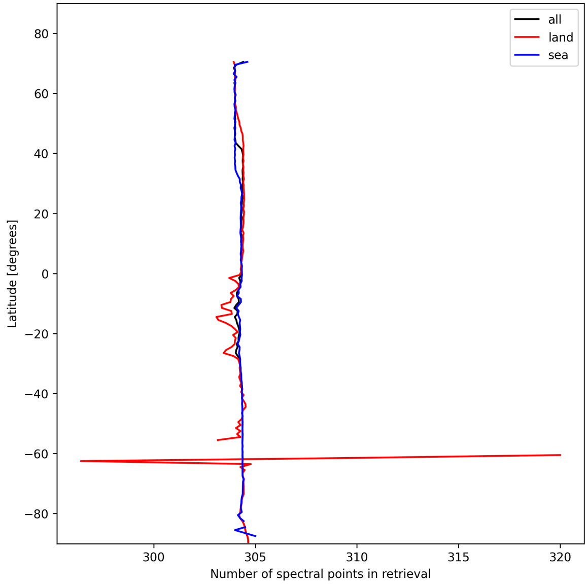
Figure 16: Zonal average of “Number of spectral points in retrieval” for 2025-11-12 to 2025-11-13.
