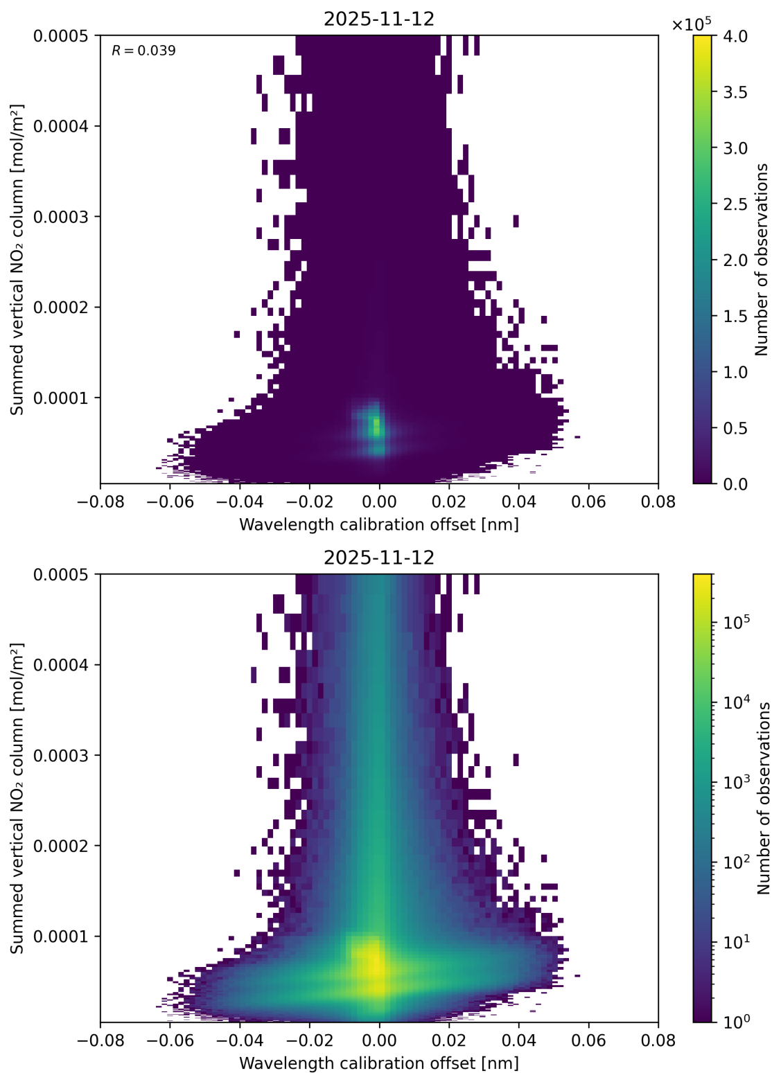
Figure 177: Scatter density plot of “Wavelength calibration offset” against “Summed vertical NO 2 column” for 2025-11-12 to 2025-11-13.
