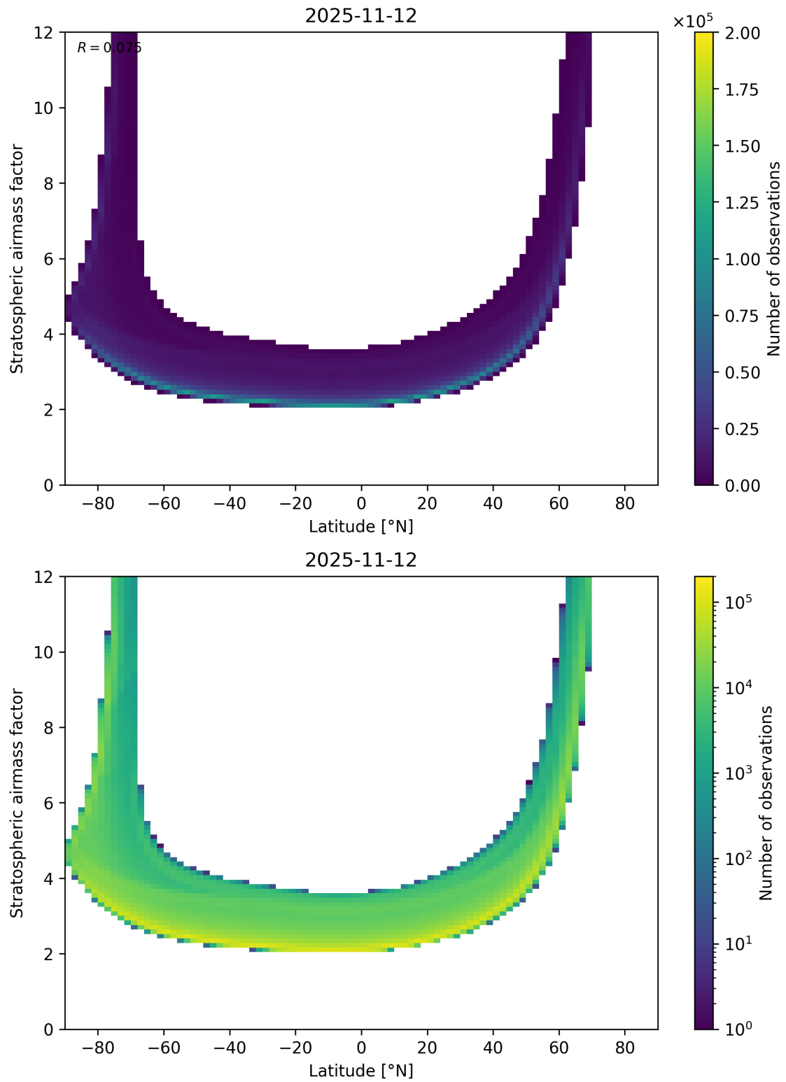
Figure 83: Scatter density plot of “Latitude” against “Stratospheric airmass factor” for 2025-11-12 to 2025-11-13.
