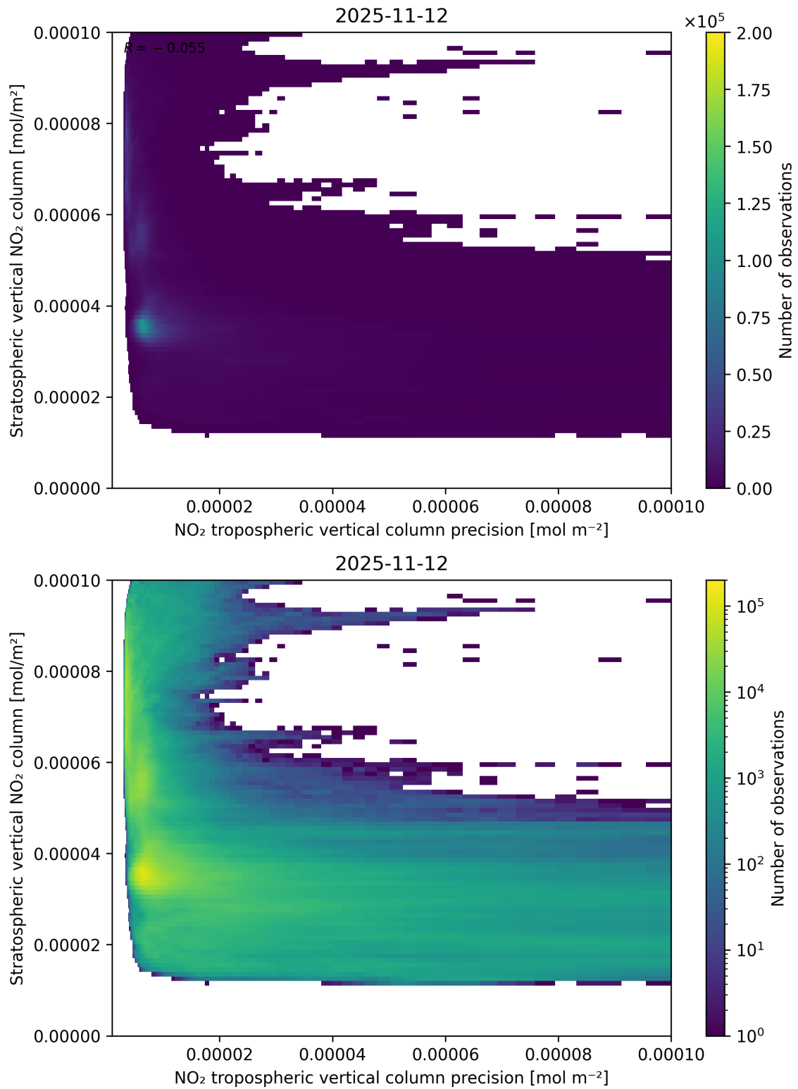
Figure 135: Scatter density plot of “NO 2 tropospheric vertical column precision” against “Stratospheric vertical NO 2 column” for 2025-11-12 to 2025-11-13.
