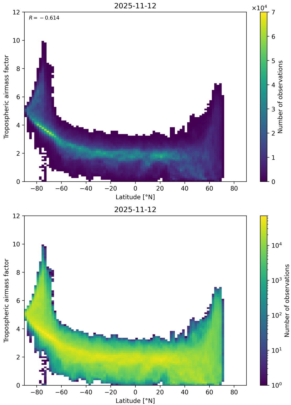
Figure 85: Scatter density plot of “Latitude” against “Tropospheric air mass factor” for 2025-11-12 to 2025-11-13.
