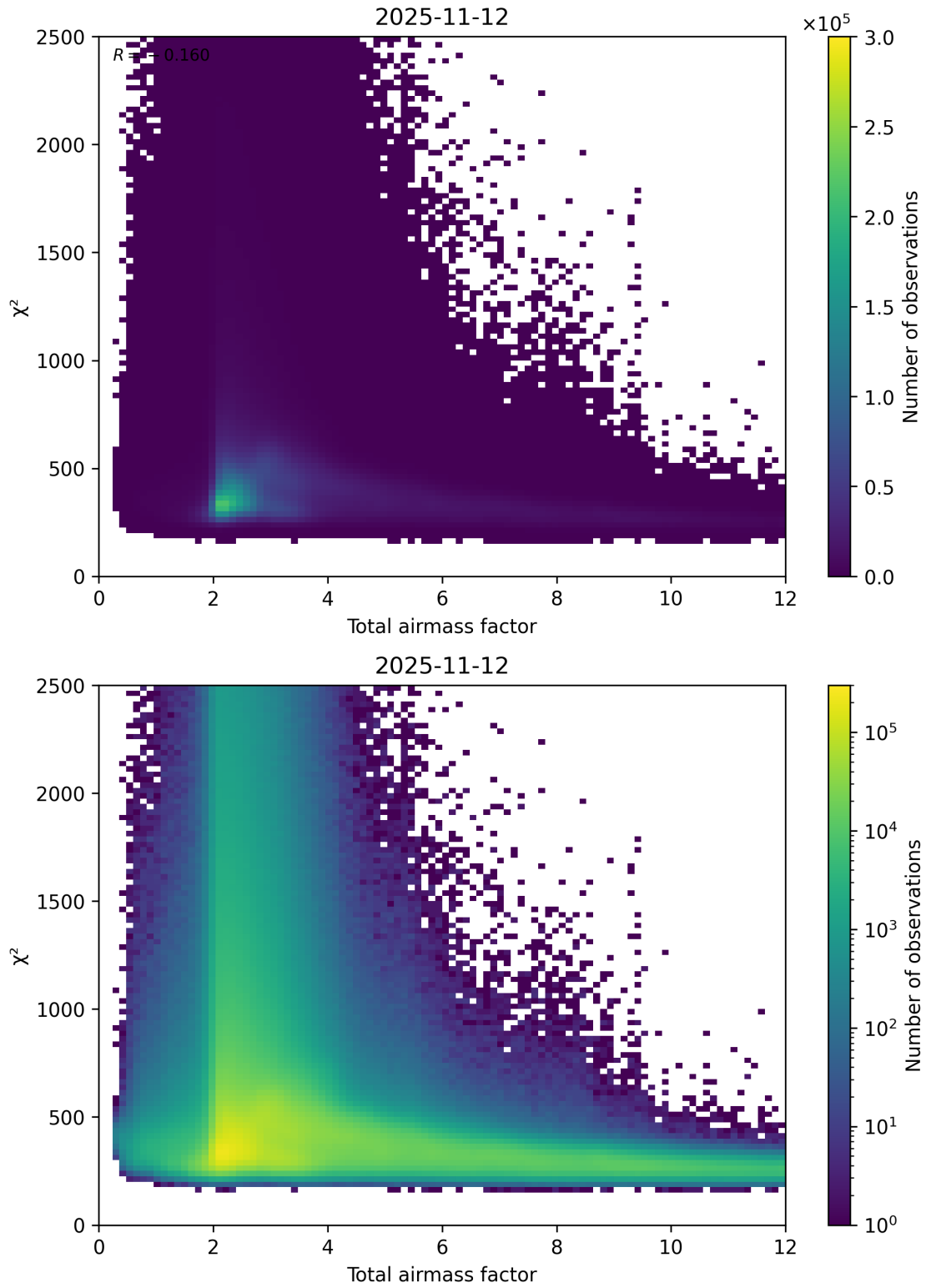
Figure 63: Scatter density plot of “Total airmass factor” against “ \chi^2 ” for 2025-11-12 to 2025-11-13.
