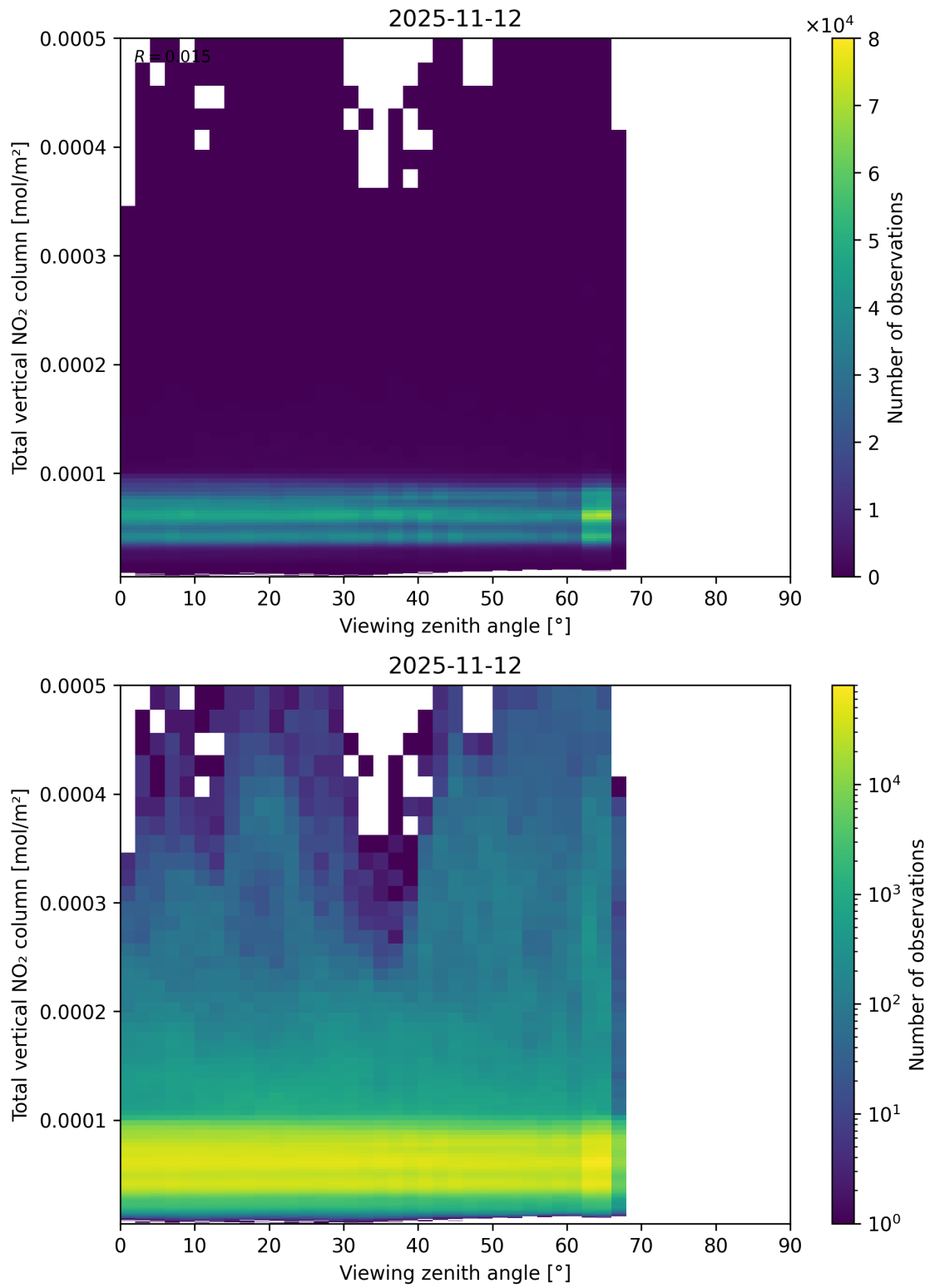
Figure 167: Scatter density plot of “Viewing zenith angle” against “Total vertical NO 2 column” for 2025-11-12 to 2025-11-13.
