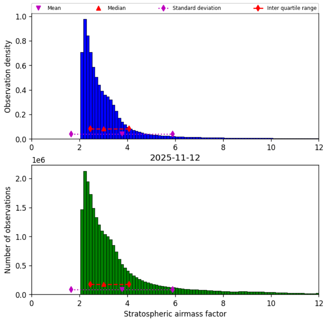
Figure 44: Histogram of “Stratospheric airmass factor” for 2025-11-12 to 2025-11-13
