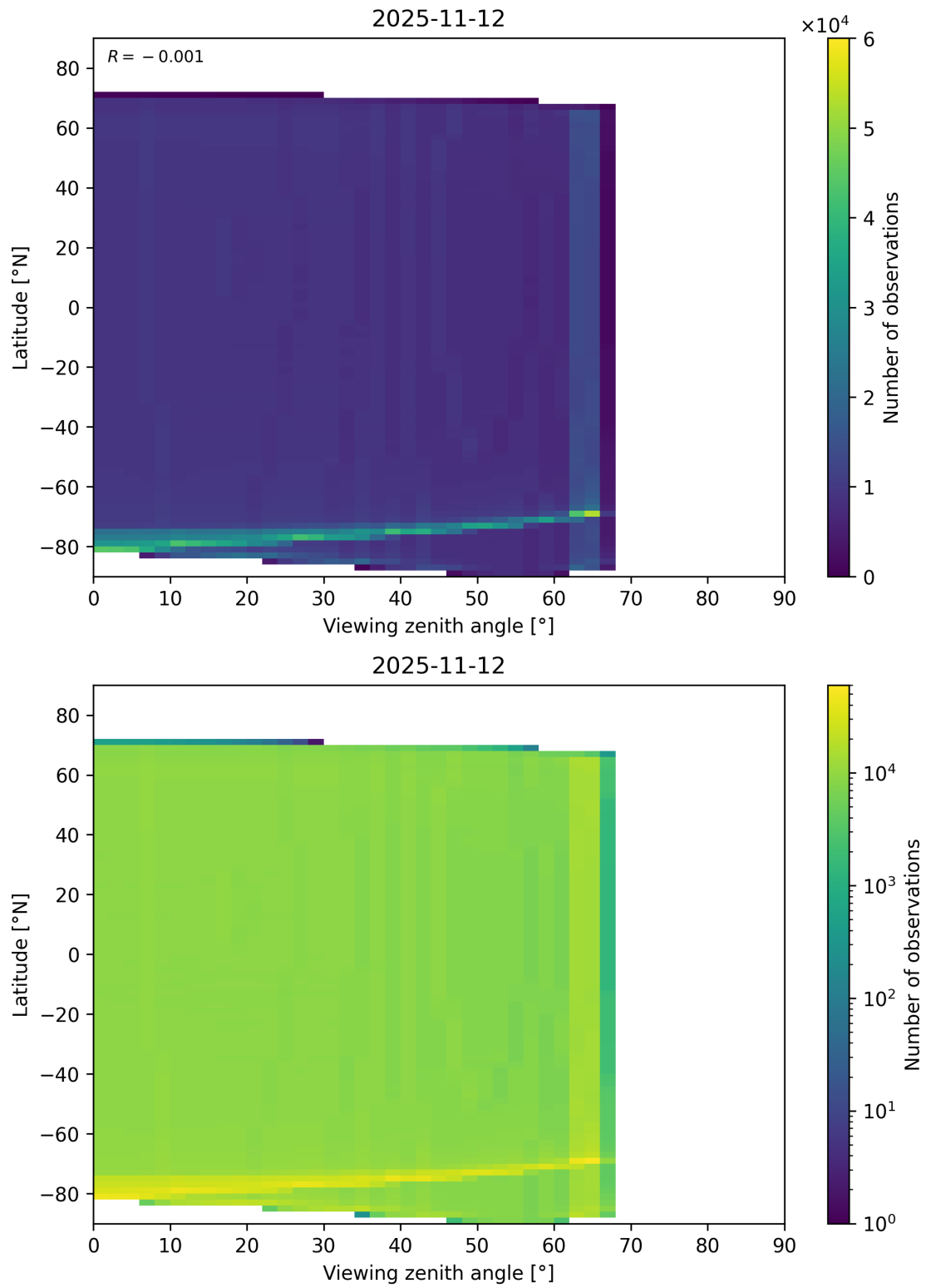
Figure 163: Scatter density plot of “Viewing zenith angle” against “Latitude” for 2025-11-12 to 2025-11-13.
