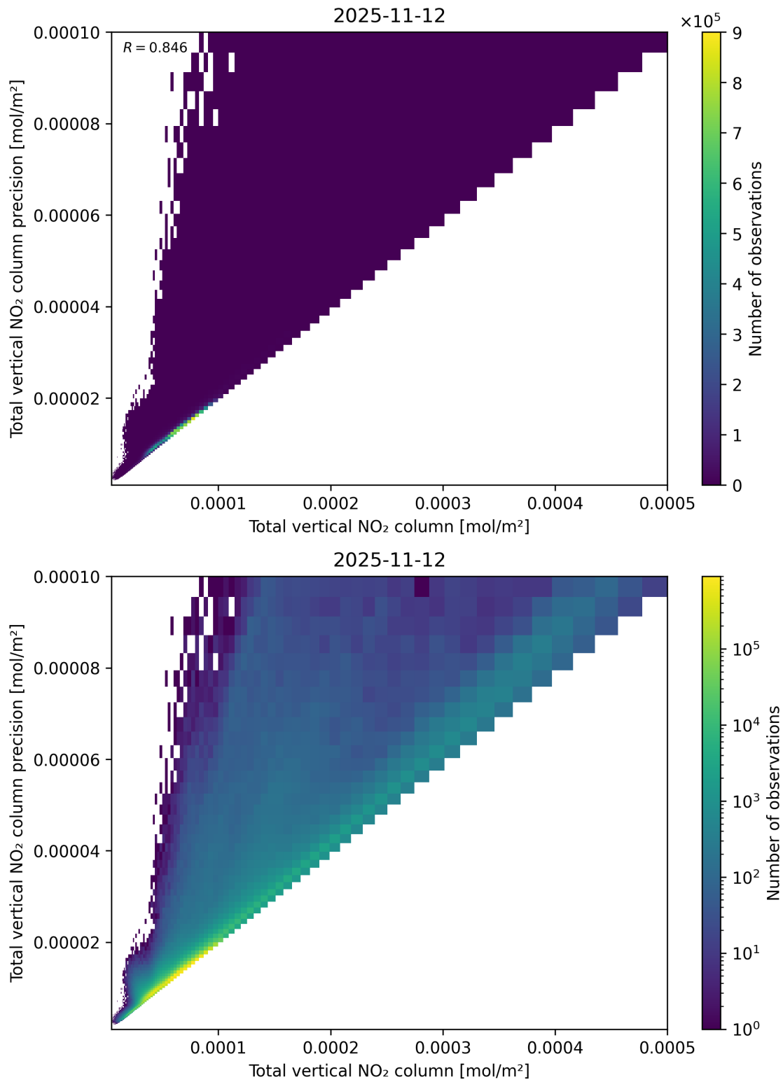
Figure 114: Scatter density plot of “Total vertical NO 2 column” against “Total vertical NO 2 column precision” for 2025-11-12 to 2025-11-13.
