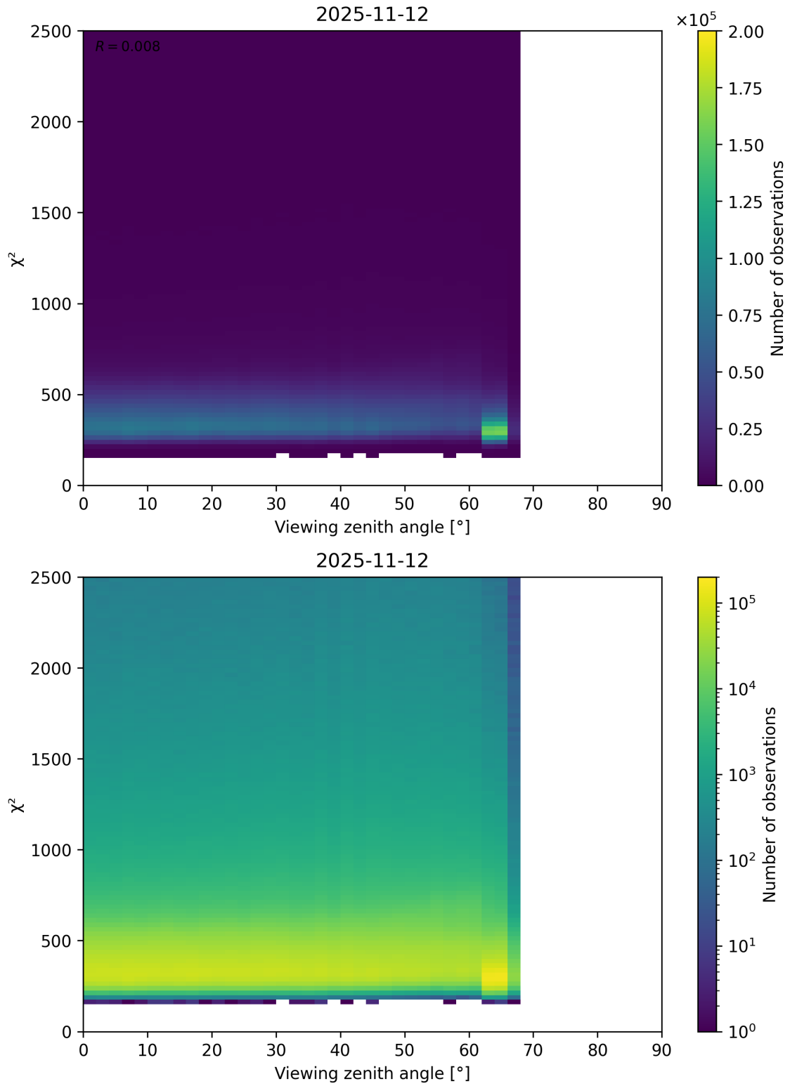
Figure 162: Scatter density plot of “Viewing zenith angle” against “ \chi^2 ” for 2025-11-12 to 2025-11-13.
