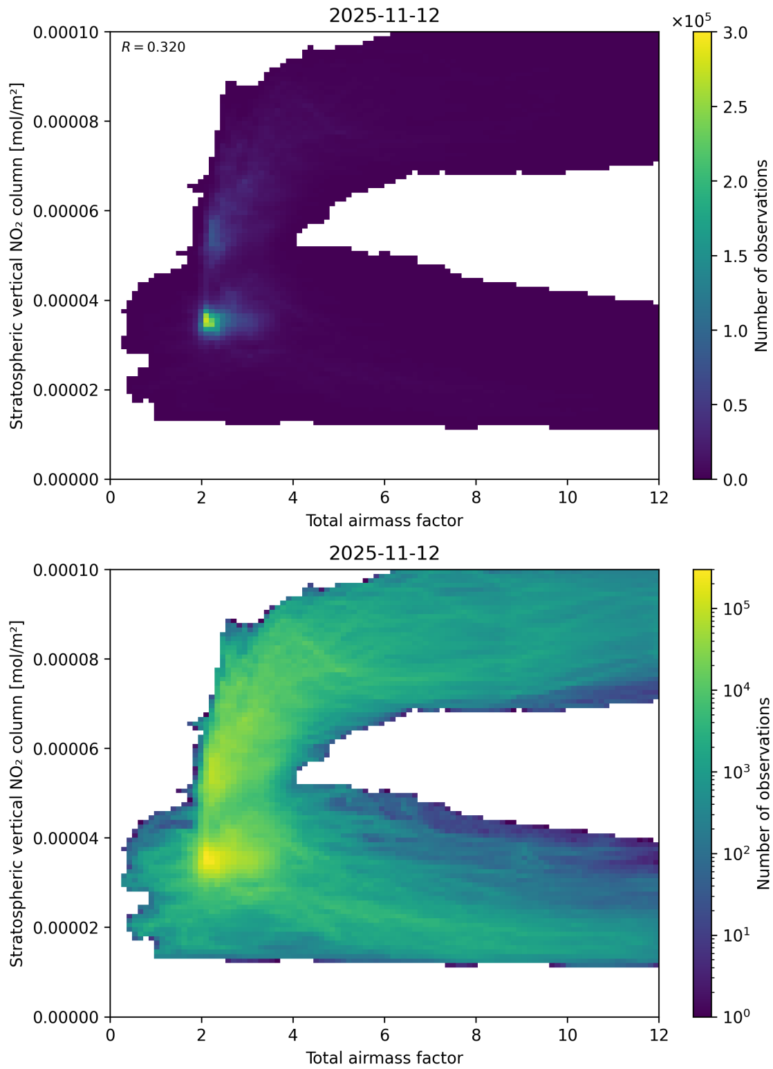
Figure 64: Scatter density plot of “Total airmass factor” against “Stratospheric vertical NO 2 column” for 2025-11-12 to 2025-11-13.
