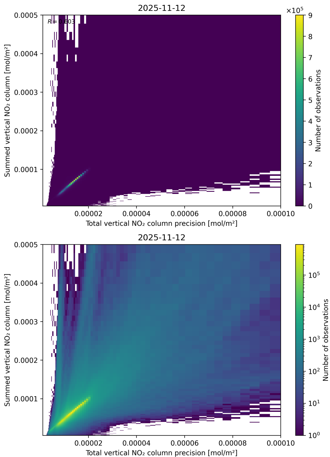
Figure 117: Scatter density plot of “Total vertical NO 2 column precision” against “Summed vertical NO 2 column” for 2025-11-12 to 2025-11-13.
