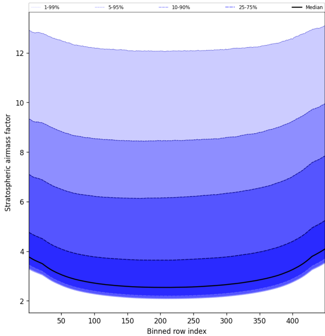
Figure 61: Along track statistics of “Stratospheric airmass factor” for 2025-11-12 to 2025-11-13
