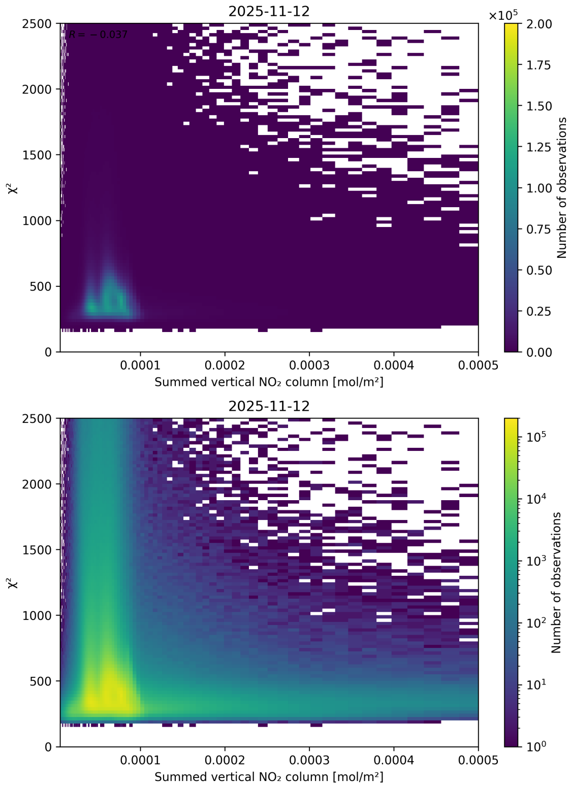
Figure 104: Scatter density plot of “Summed vertical NO 2 column” against “ \chi^2 ” for 2025-11-12 to 2025-11-13.
