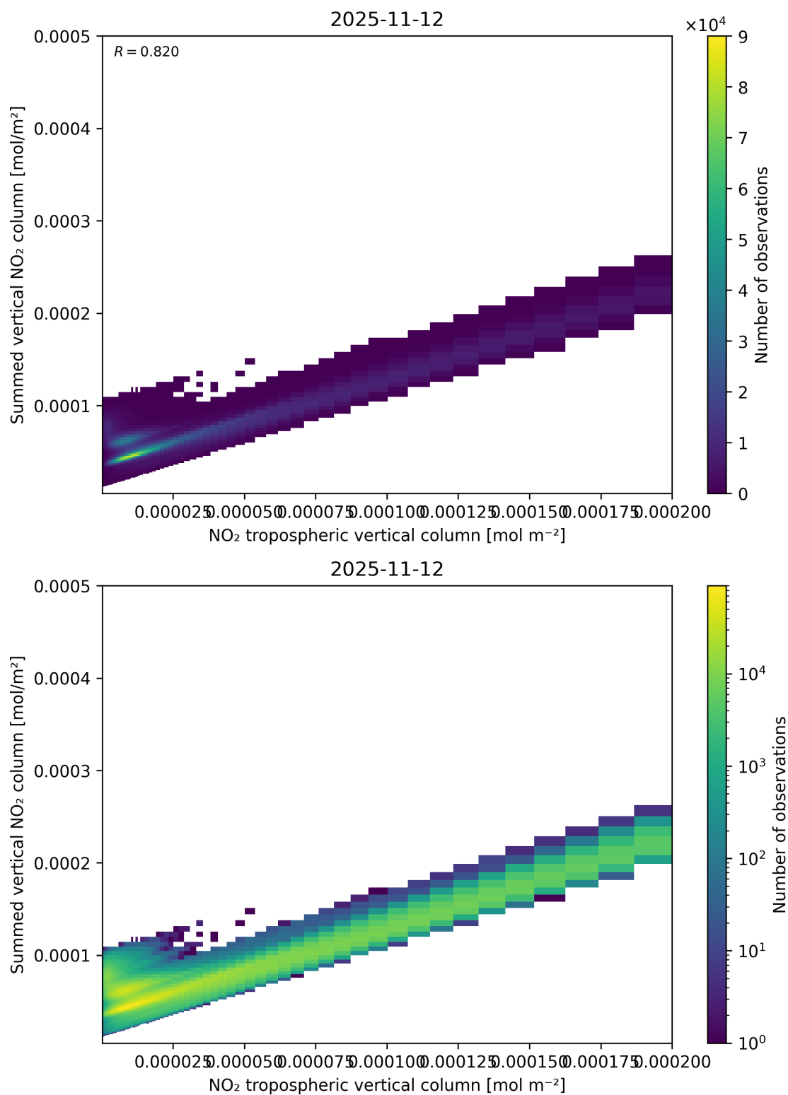
Figure 126: Scatter density plot of “NO 2 tropospheric vertical column” against “Summed vertical NO 2 column” for 2025-11-12 to 2025-11-13.
