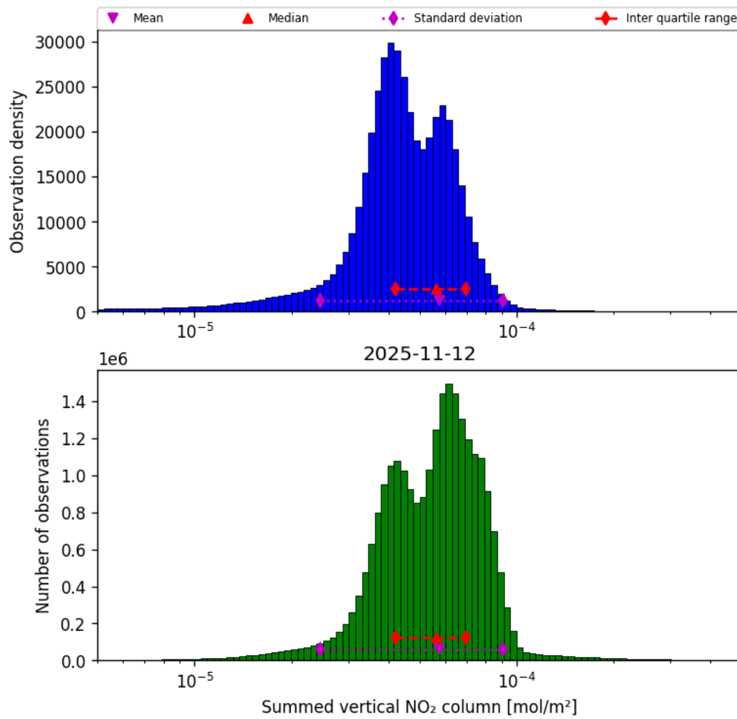
Figure 40: Histogram of “Summed vertical NO 2 column” for 2025-11-12 to 2025-11-13
