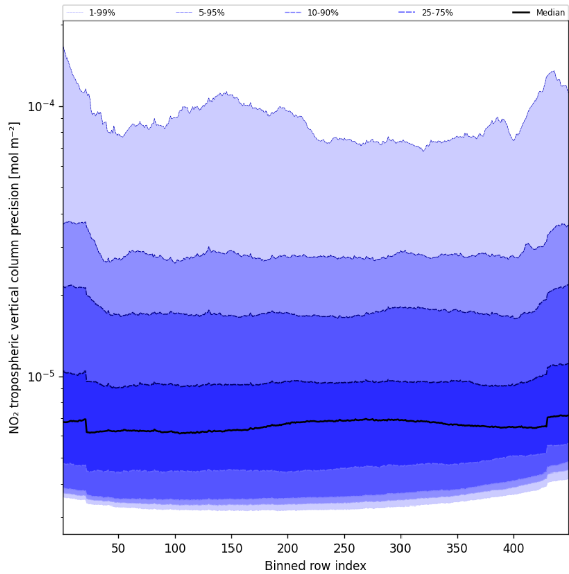
Figure 47: Along track statistics of “NO 2 tropospheric vertical column precision” for 2025-11-12 to 2025-11-13
