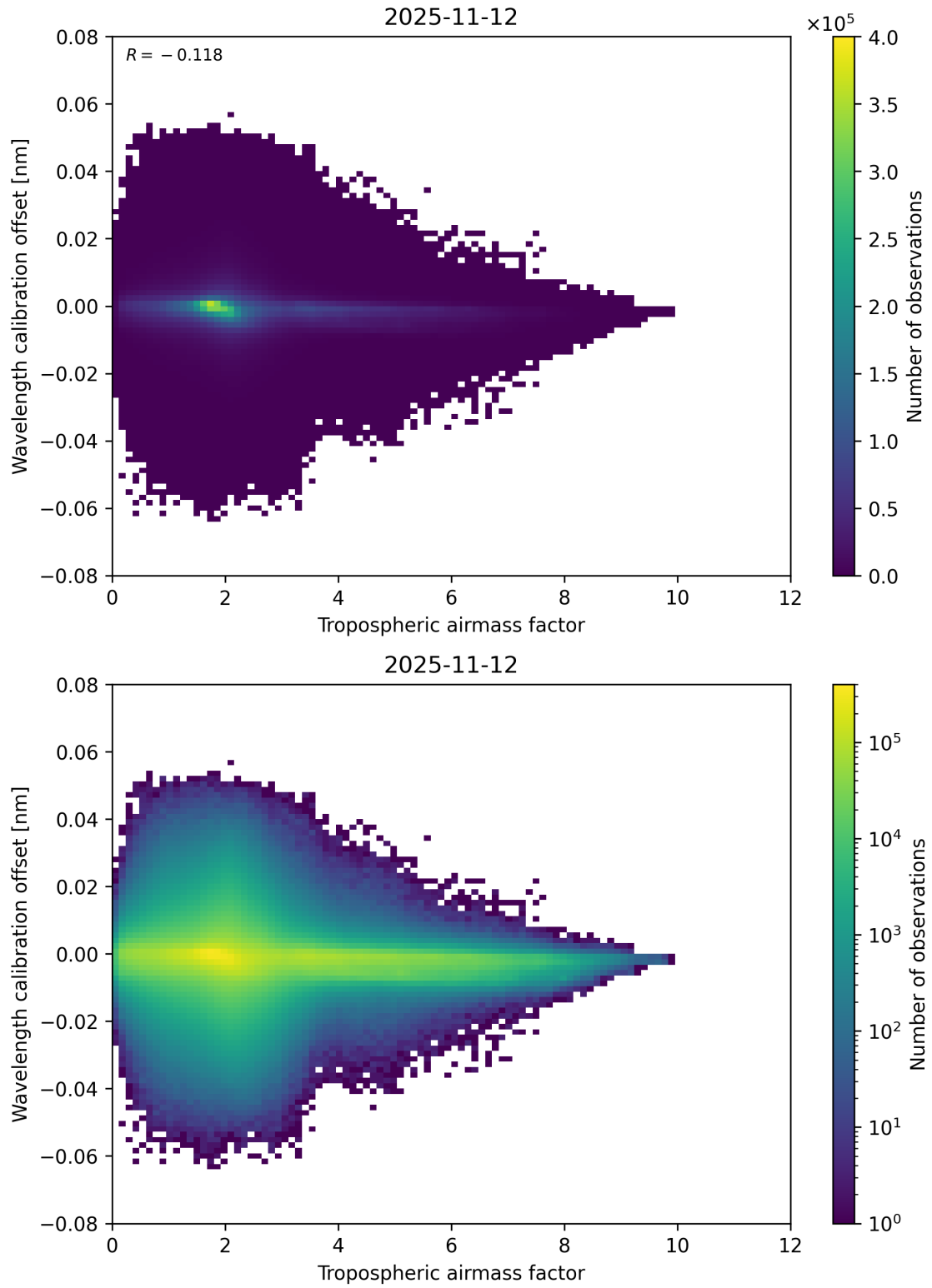
Figure 80: Scatter density plot of “Tropospheric airmass factor” against “Wavelength calibration offset” for 2025-11-12 to 2025-11-13.
