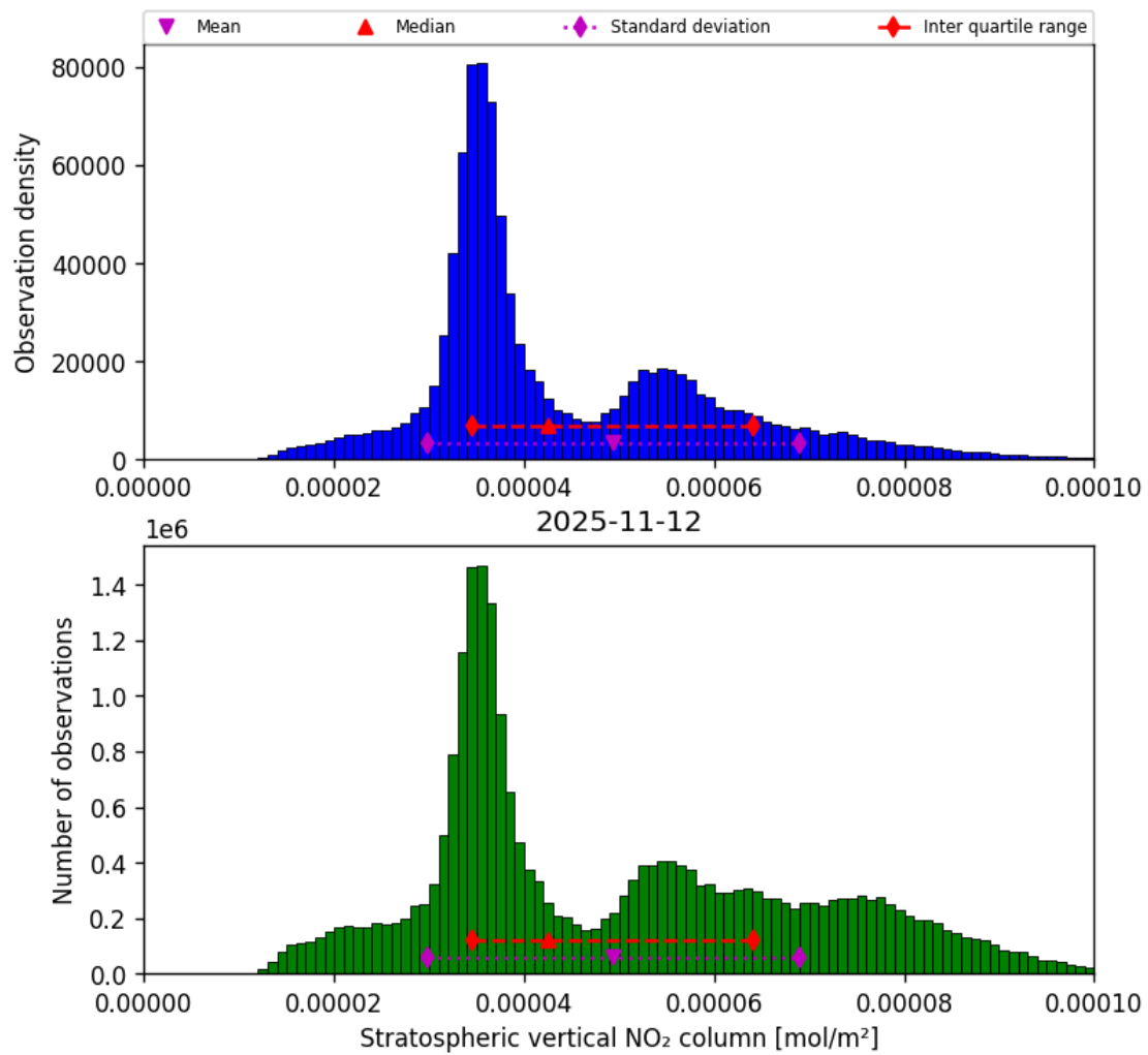
Figure 36: Histogram of “Stratospheric vertical NO 2 column” for 2025-11-12 to 2025-11-13
