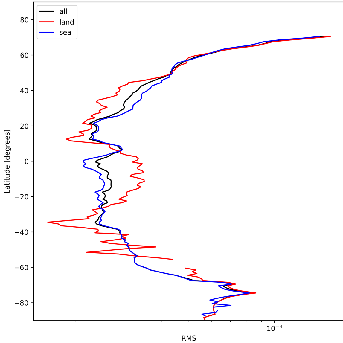
Figure 26: Zonal average of “RMS” for 2025-11-12 to 2025-11-13.
