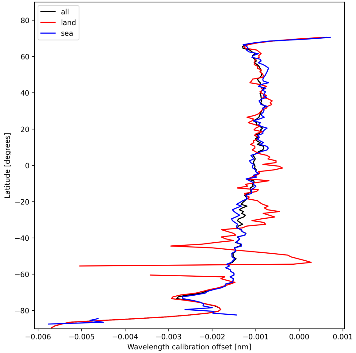
Figure 18: Zonal average of “Wavelength calibration offset” for 2025-11-12 to 2025-11-13.
