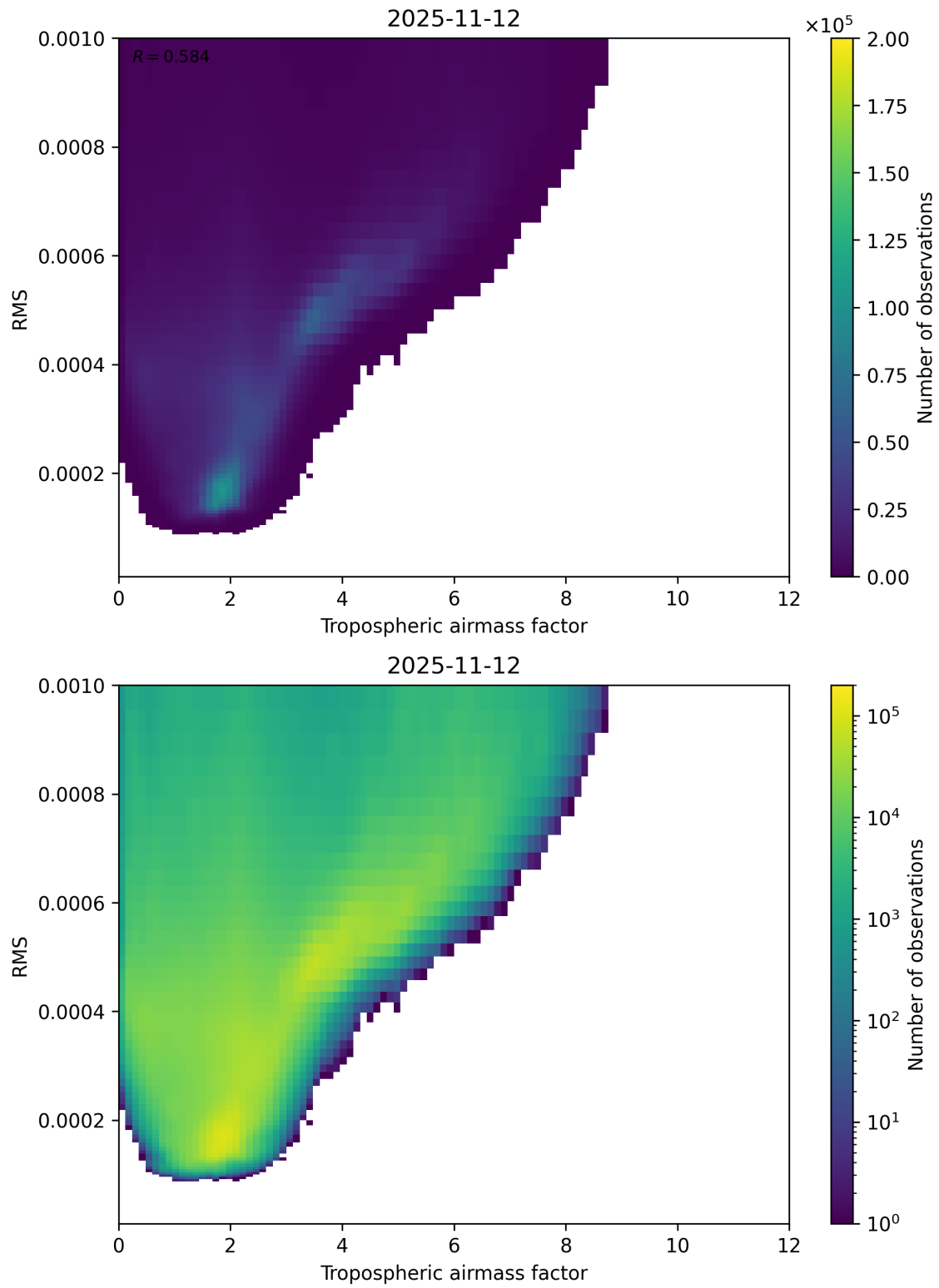
Figure 79: Scatter density plot of “Tropospheric airmass factor” against “RMS” for 2025-11-12 to 2025-11-13.
