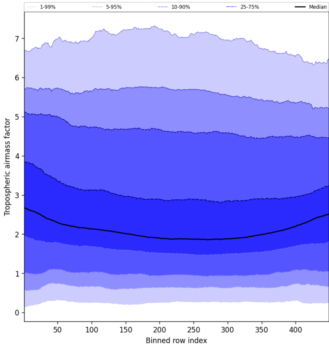
Figure 48: Along track statistics of “Tropospheric air mass factor” for 2025-11-12 to 2025-11-13
