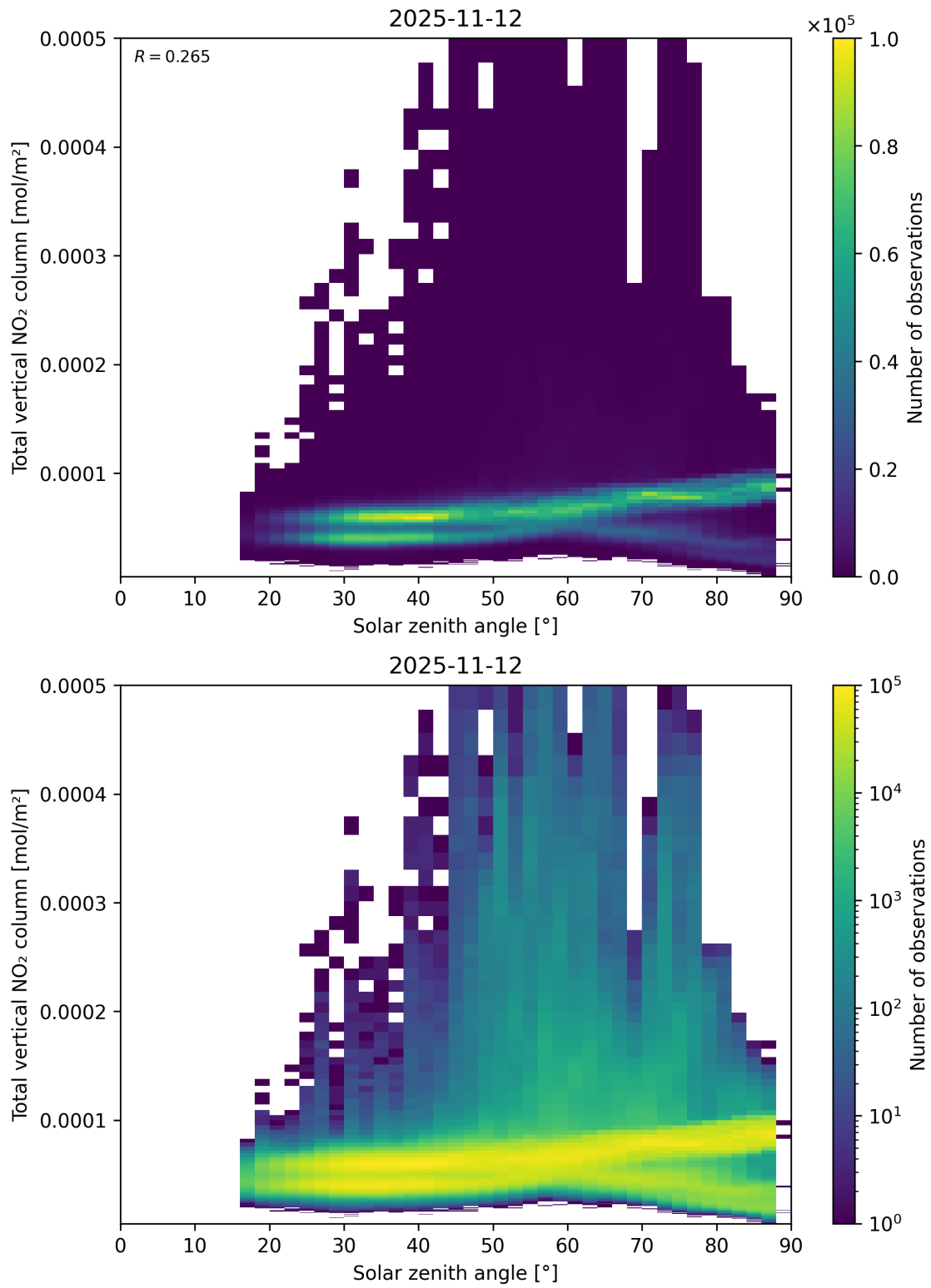
Figure 153: Scatter density plot of “Solar zenith angle” against “Total vertical NO 2 column” for 2025-11-12 to 2025-11-13.
