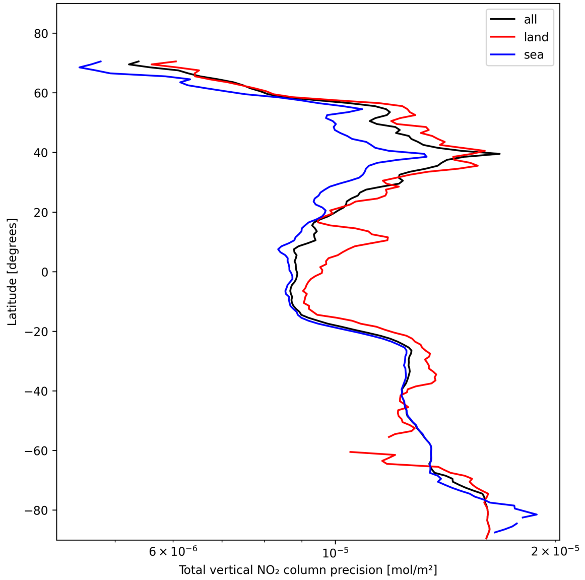
Figure 22: Zonal average of “Total vertical NO 2 column precision” for 2025-11-12 to 2025-11-13.
