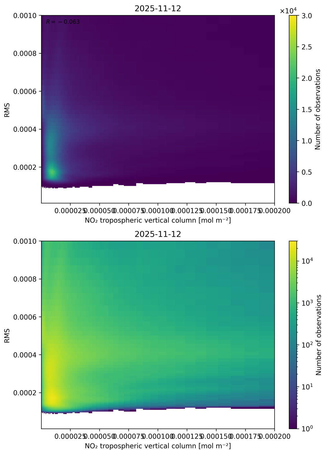
Figure 142: Scatter density plot of “NO 2 tropospheric vertical column” against “RMS” for 2025-11-12 to 2025-11-13.
