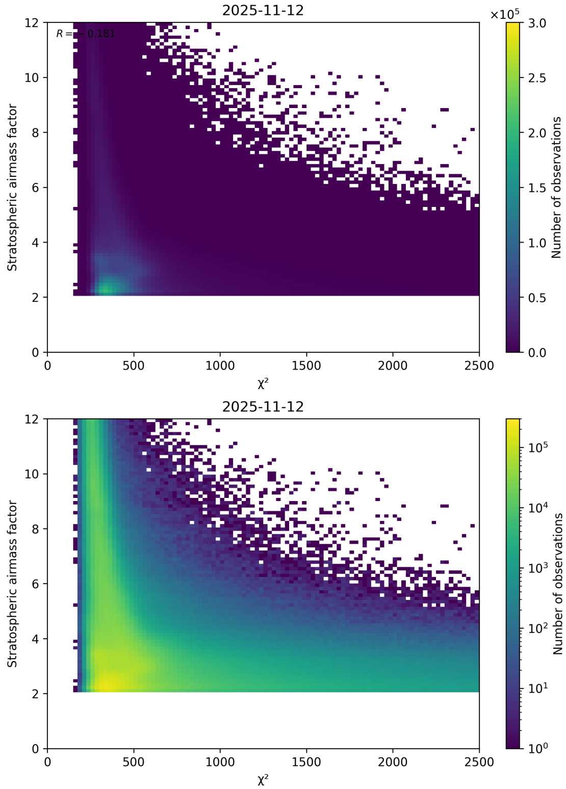
Figure 81: Scatter density plot of “ \chi^2 ” against “Stratospheric airmass factor” for 2025-11-12 to 2025-11-13.
