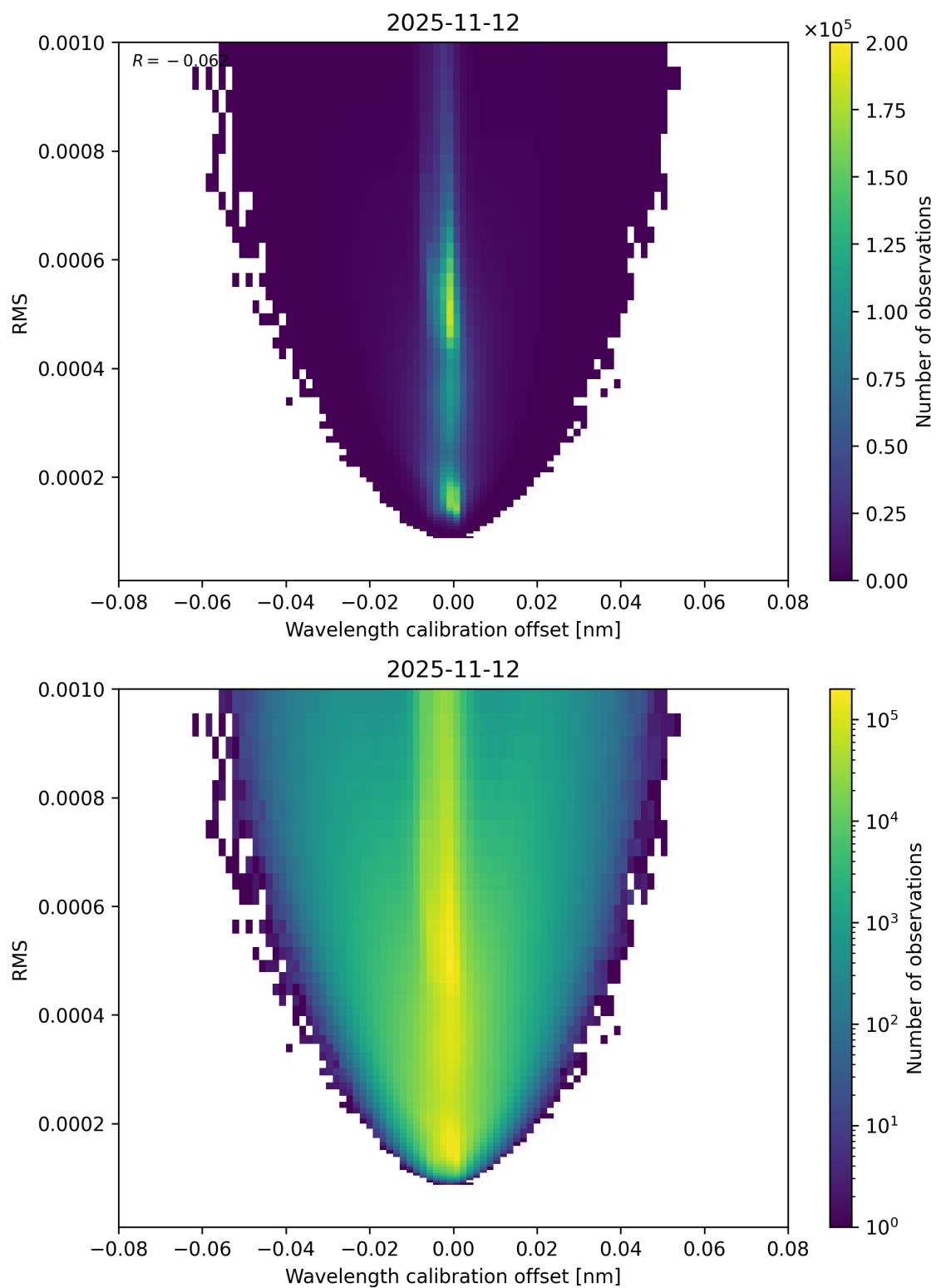
Figure 181: Scatter density plot of “Wavelength calibration offset” against “RMS” for 2025-11-12 to 2025-11-13.
