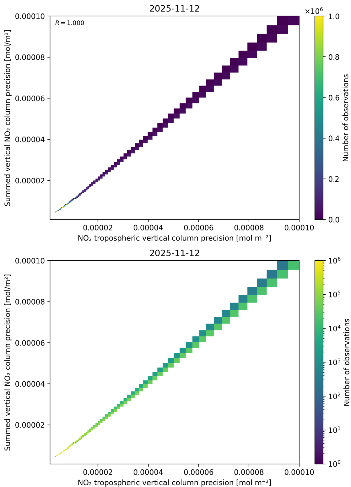
Figure 137: Scatter density plot of “NO 2 tropospheric vertical column precision” against “Summed vertical NO 2 column precision” for 2025-11-12 to 2025-11-13.
