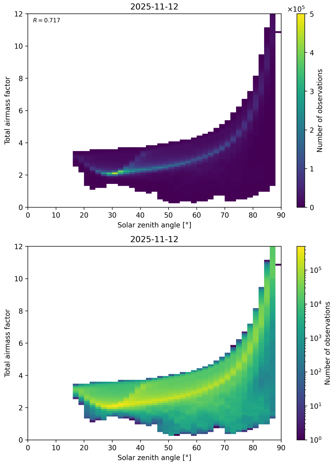
Figure 146: Scatter density plot of “Solar zenith angle” against “Total air mass factor” for 2025-11-12 to 2025-11-13.
