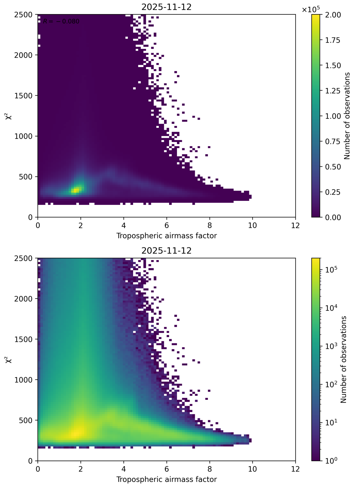
Figure 73: Scatter density plot of “Tropospheric airmass factor” against “ \chi^2 ” for 2025-11-12 to 2025-11-13.
