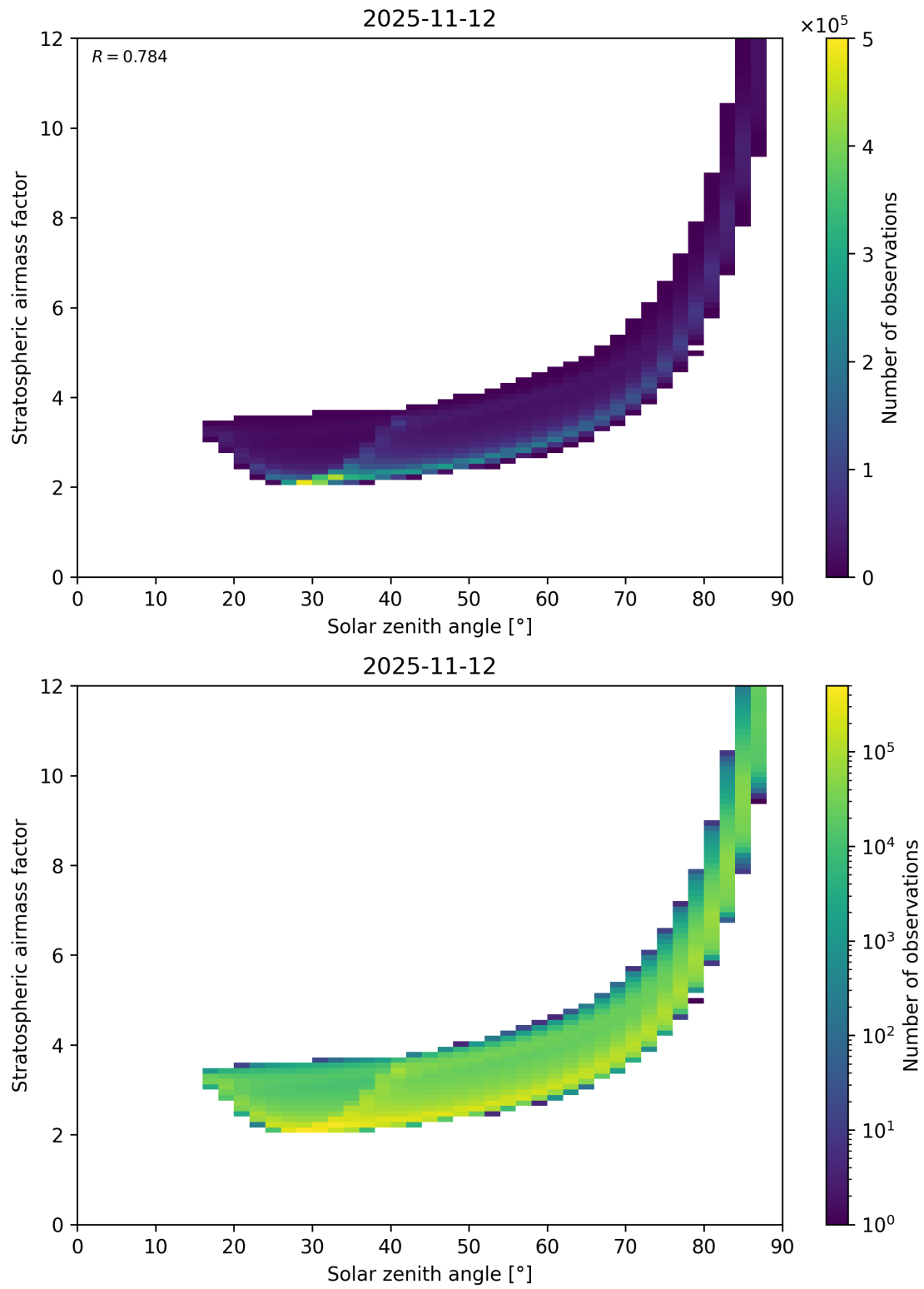
Figure 145: Scatter density plot of “Solar zenith angle” against “Stratospheric airmass factor” for 2025-11-12 to 2025-11-13.
