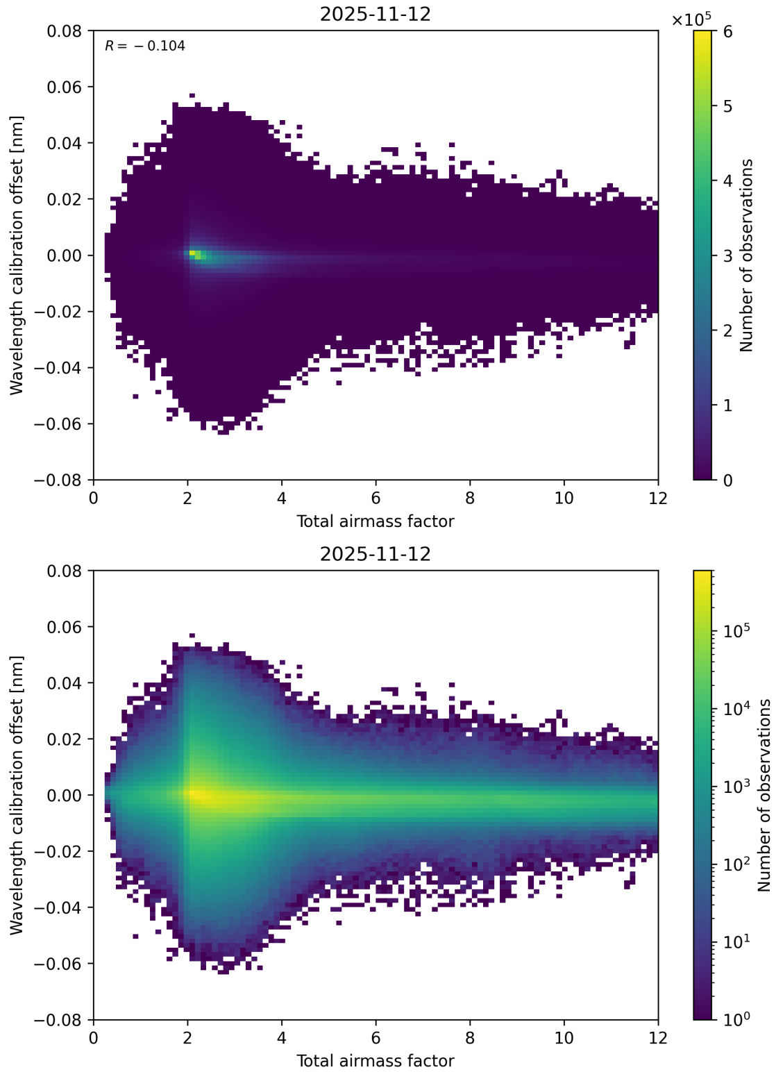
Figure 70: Scatter density plot of “Total airmass factor” against “Wavelength calibration offset” for 2025-11-12 to 2025-11-13.
