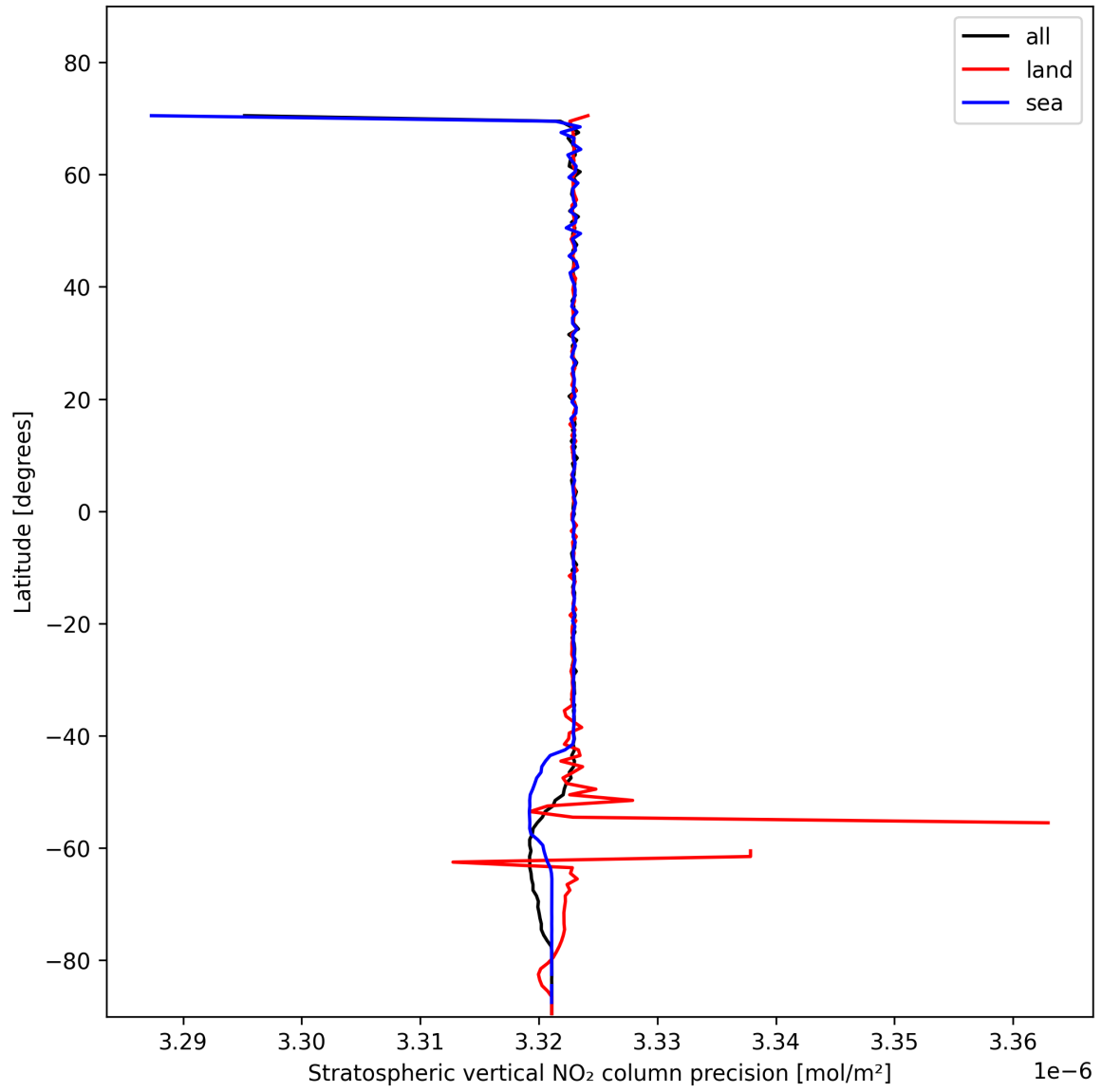
Figure 20: Zonal average of "Stratospheric vertical NO 2 column precision" for 2025-11-12 to 2025-11-13.
