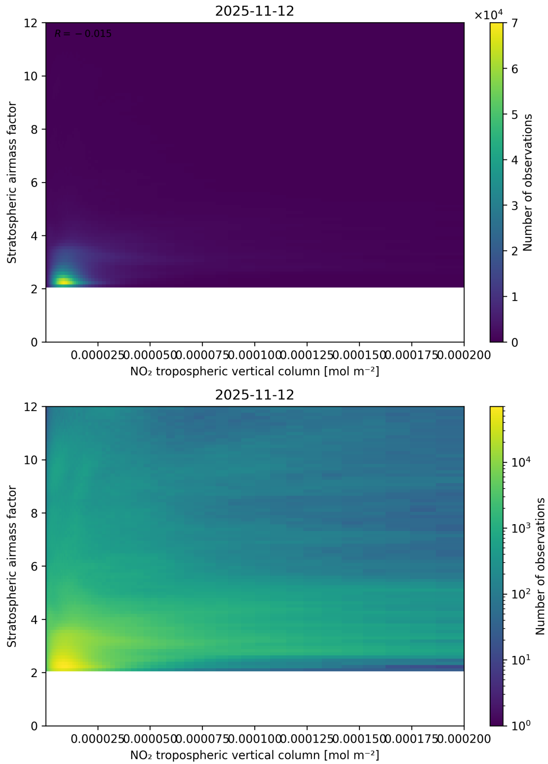
Figure 121: Scatter density plot of “NO 2 tropospheric vertical column” against “Stratospheric airmass factor” for 2025-11-12 to 2025-11-13.
