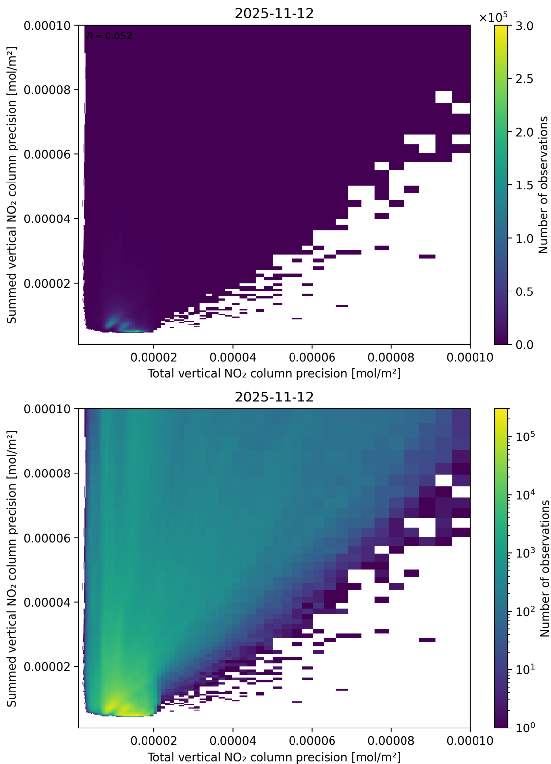
Figure 118: Scatter density plot of “Total vertical NO 2 column precision” against “Summed vertical NO 2 column precision” for 2025-11-12 to 2025-11-13.
