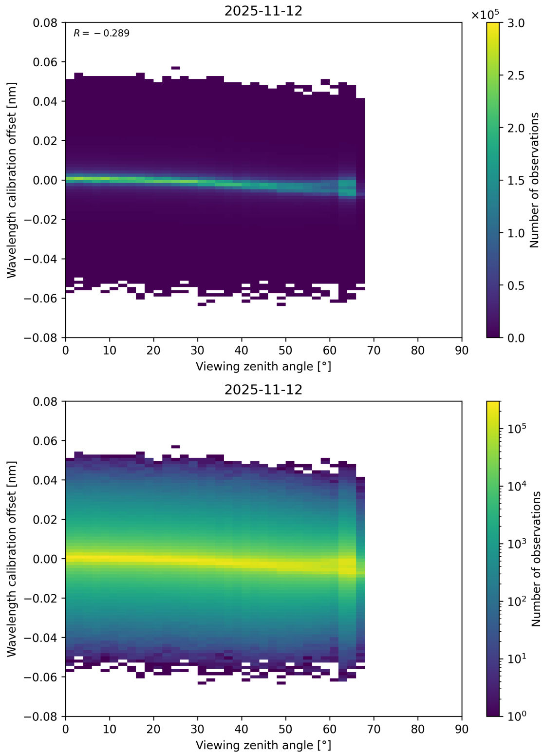
Figure 173: Scatter density plot of “Viewing zenith angle” against “Wavelength calibration offset” for 2025-11-12 to 2025-11-13.
