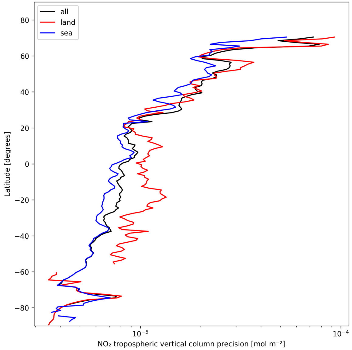
Figure 13: Zonal average of “NO 2 tropospheric vertical column precision” for 2025-11-12 to 2025-11-13.
