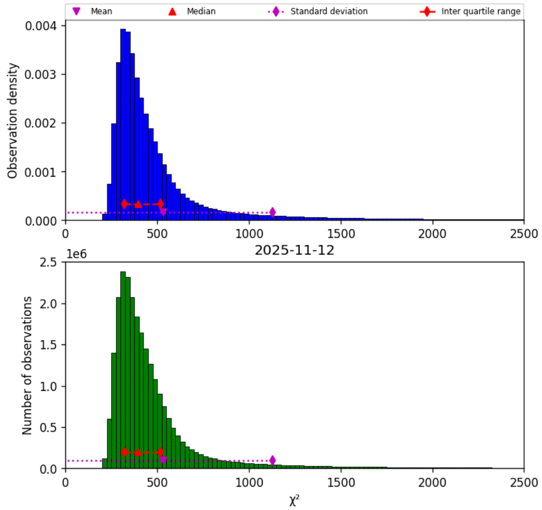
Figure 42: Histogram of “ \chi^2 ” for 2025-11-12 to 2025-11-13
