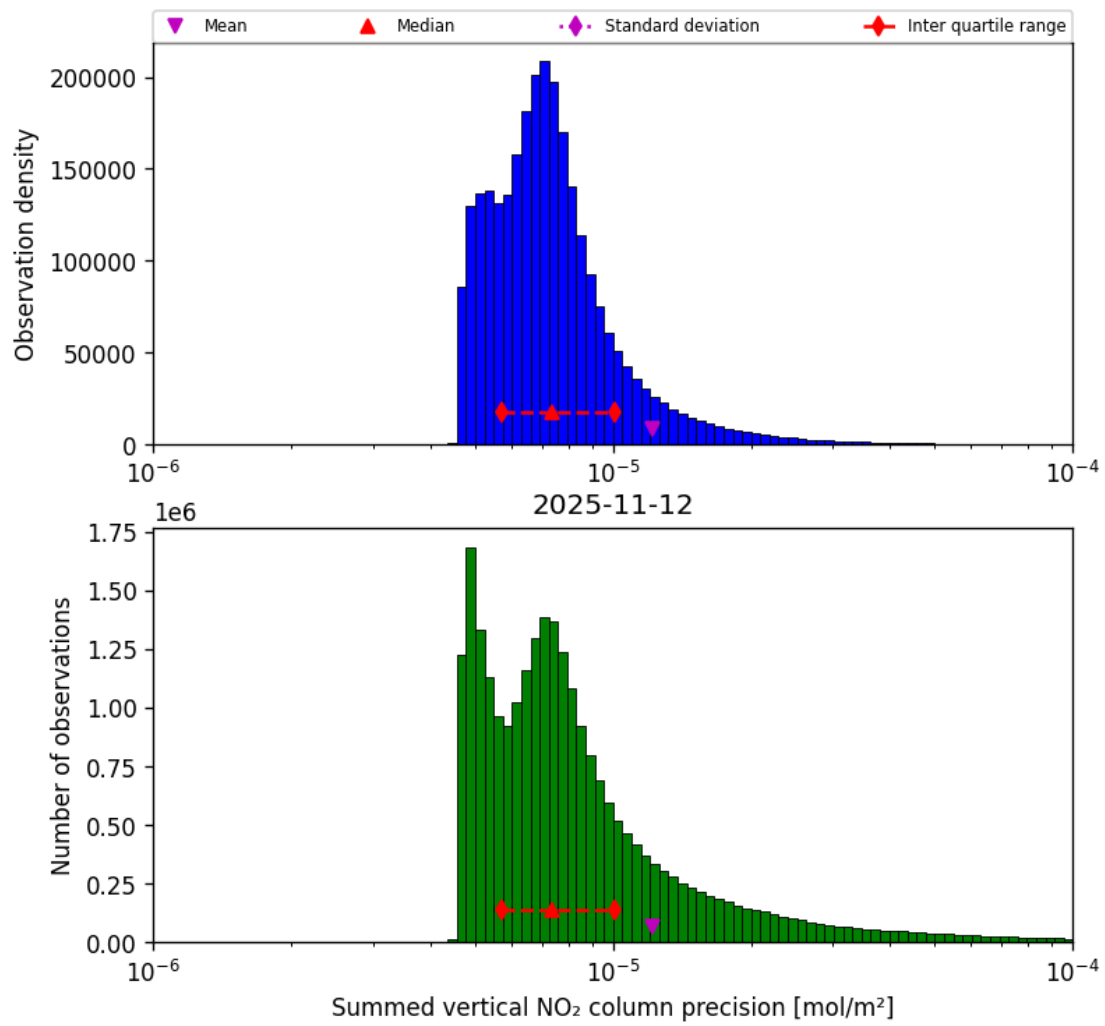
Figure 41: Histogram of “Summed vertical NO 2 column precision” for 2025-11-12 to 2025-11-13
