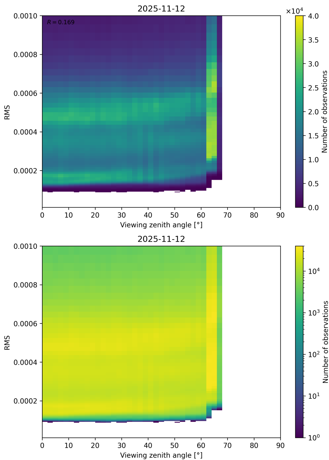
Figure 171: Scatter density plot of “Viewing zenith angle” against “RMS” for 2025-11-12 to 2025-11-13.
