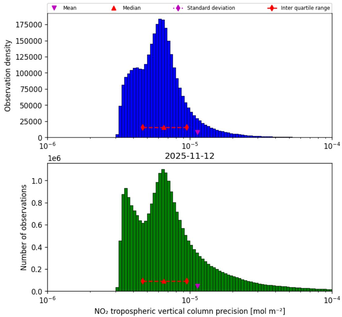
Figure 30: Histogram of “NO 2 tropospheric vertical column precision” for 2025-11-12 to 2025-11-13
