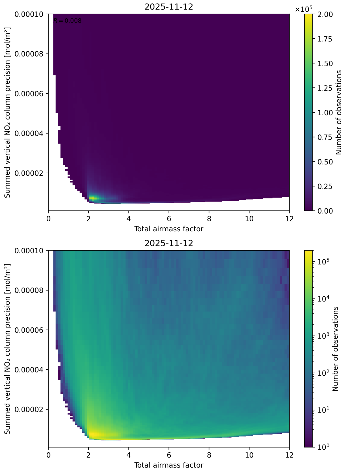
Figure 66: Scatter density plot of “Total airmass factor” against “Summed vertical NO 2 column precision” for 2025-11-12 to 2025-11-13.
