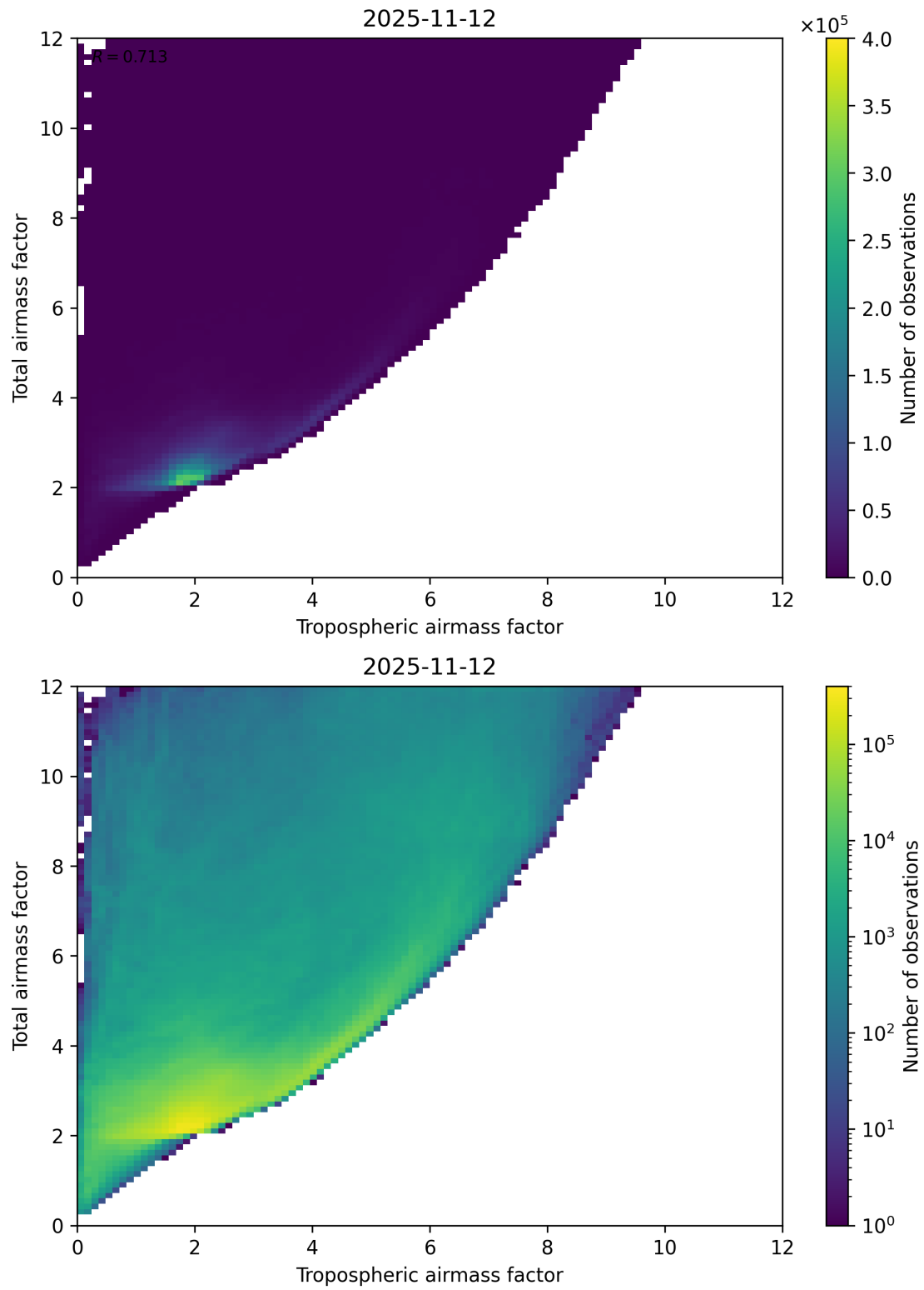
Figure 72: Scatter density plot of “Tropospheric airmass factor” against “Total airmass factor” for 2025-11-12 to 2025-11-13.
