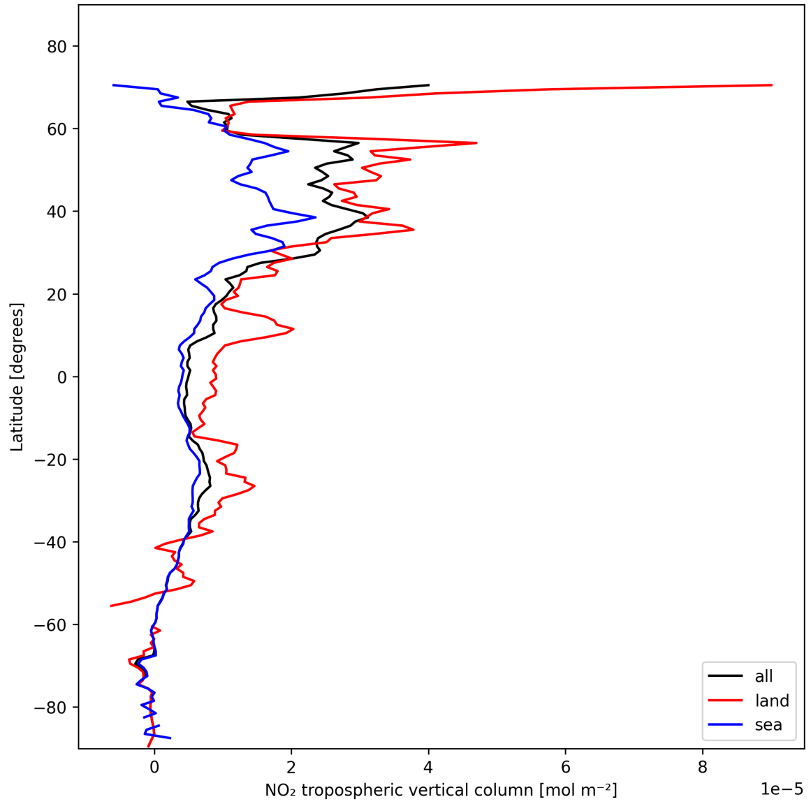
Figure 12: Zonal average of “NO 2 tropospheric vertical column” for 2025-11-12 to 2025-11-13.
