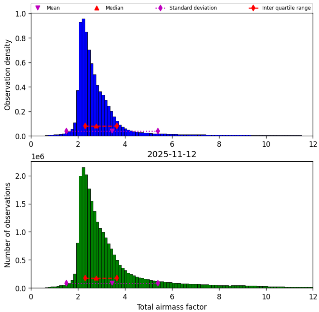
Figure 32: Histogram of “Total airmass factor” for 2025-11-12 to 2025-11-13
