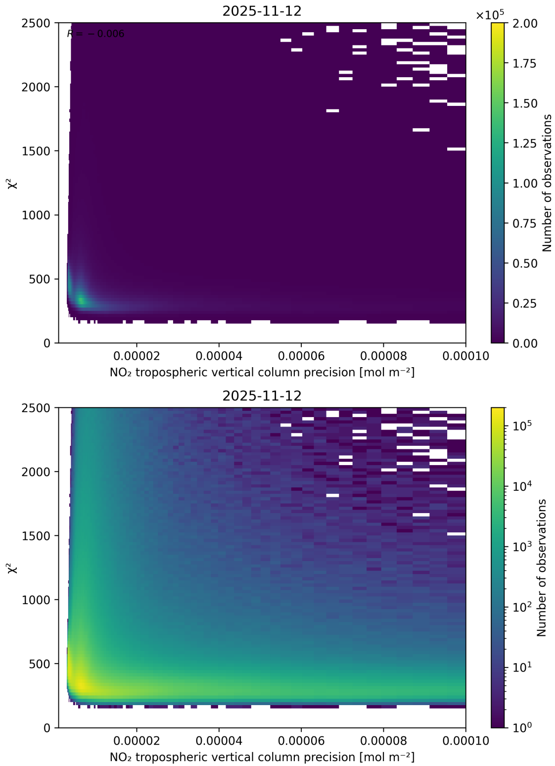
Figure 134: Scatter density plot of “NO 2 tropospheric vertical column precision” against “ \chi^2 ” for 2025-11-12 to 2025-11-13.
