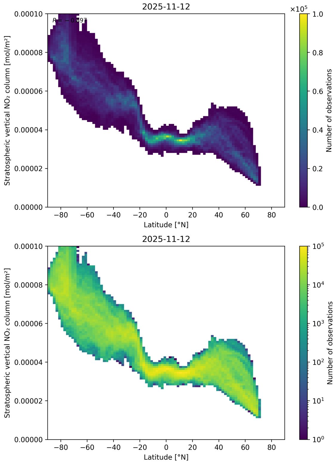
Figure 87: Scatter density plot of “Latitude” against “Stratospheric vertical NO 2 column” for 2025-11-12 to 2025-11-13.
