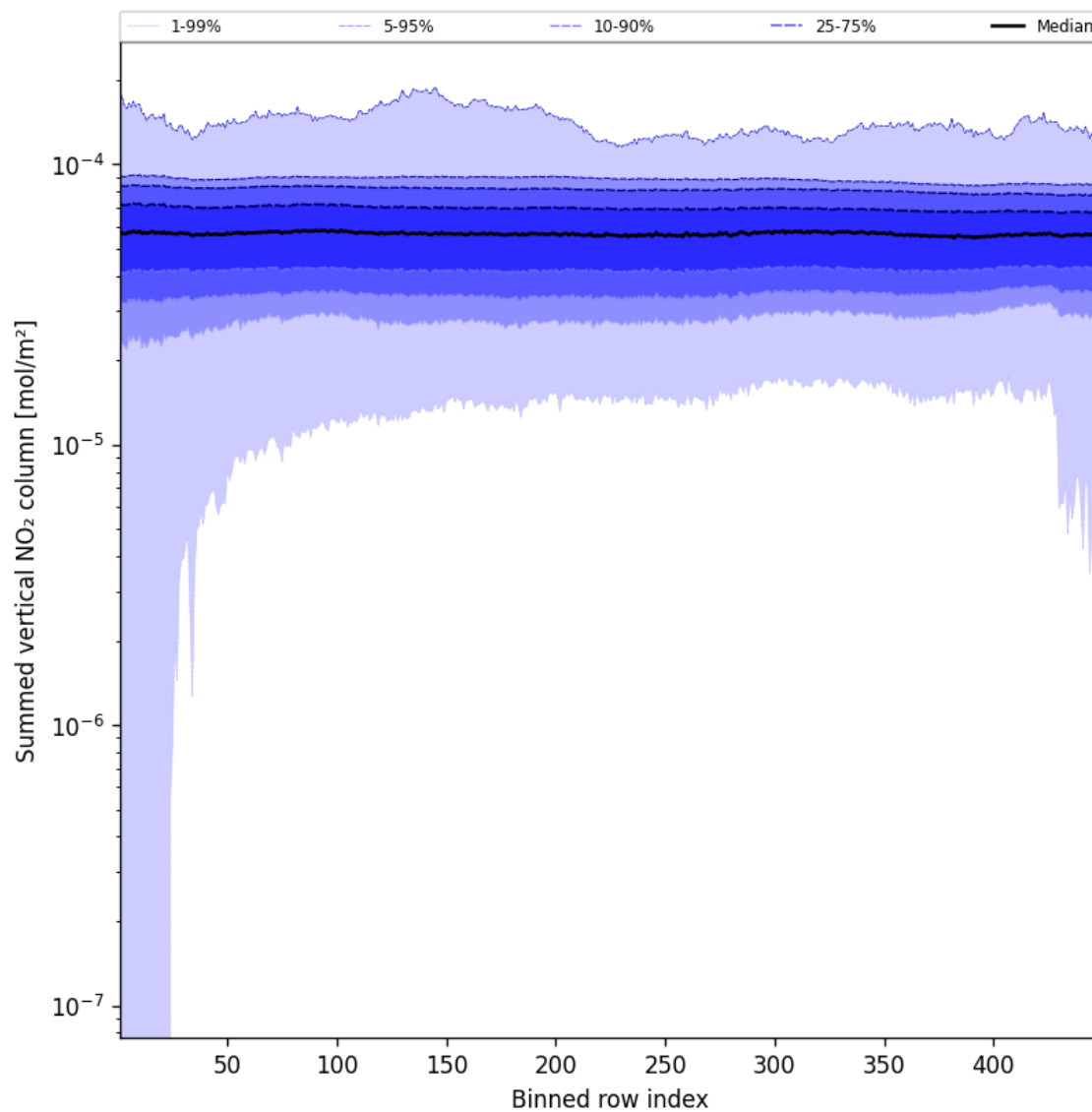
Figure 57: Along track statistics of “Summed vertical NO 2 column” for 2025-11-12 to 2025-11-13
