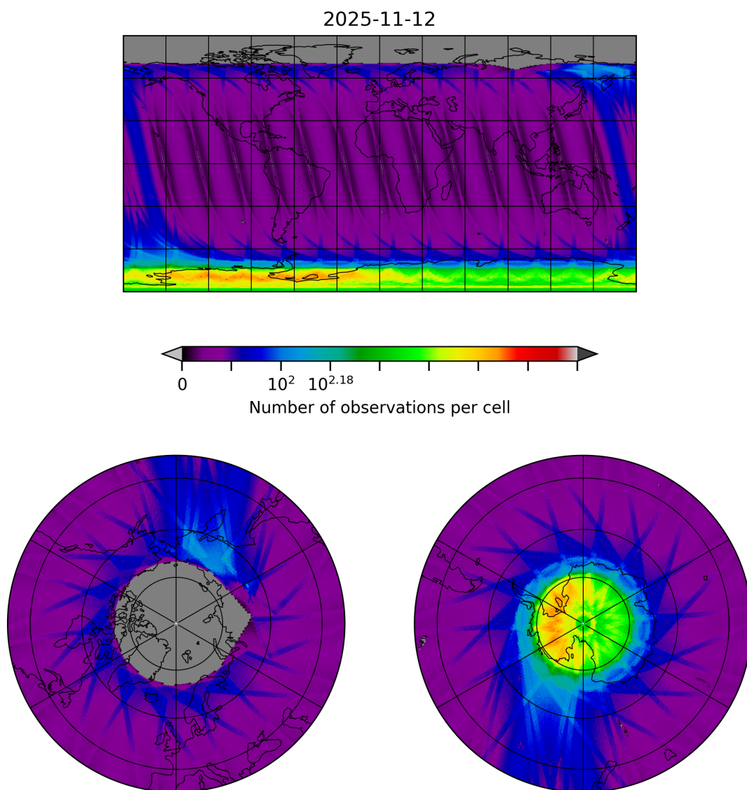
Figure 10: Map of the number of observations for 2025-11-12 to 2025-11-13
