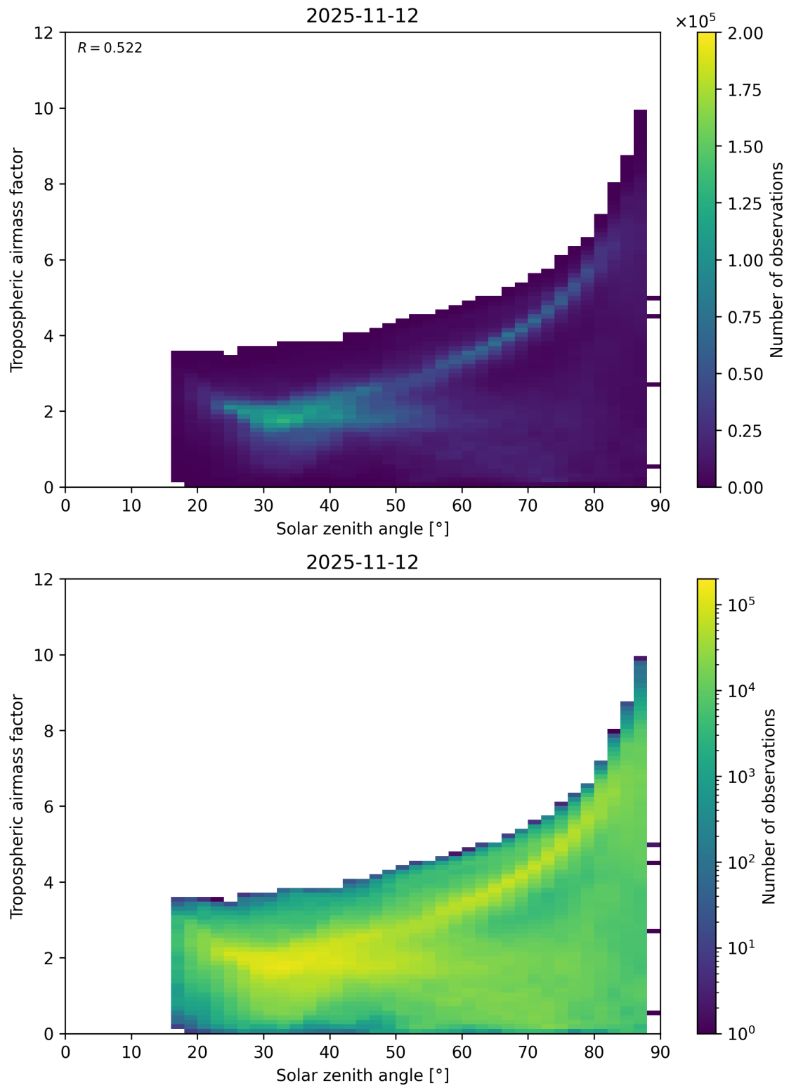
Figure 147: Scatter density plot of “Solar zenith angle” against “Tropospheric airmass factor” for 2025-11-12 to 2025-11-13.
