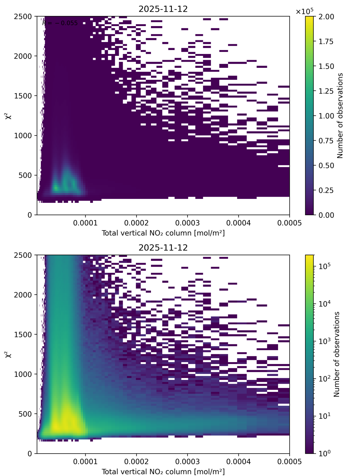
Figure 111: Scatter density plot of “Total vertical NO 2 column” against “ \chi^2 ” for 2025-11-12 to 2025-11-13.
