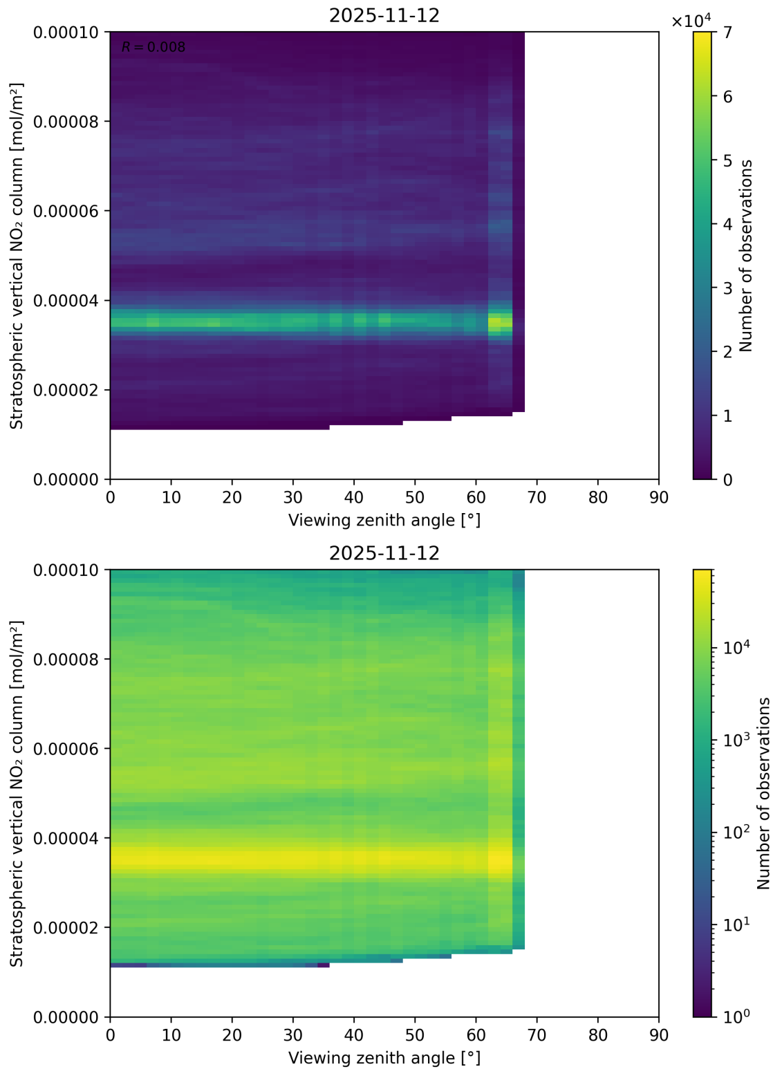
Figure 164: Scatter density plot of “Viewing zenith angle” against “Stratospheric vertical NO 2 column” for 2025-11-12 to 2025-11-13.
