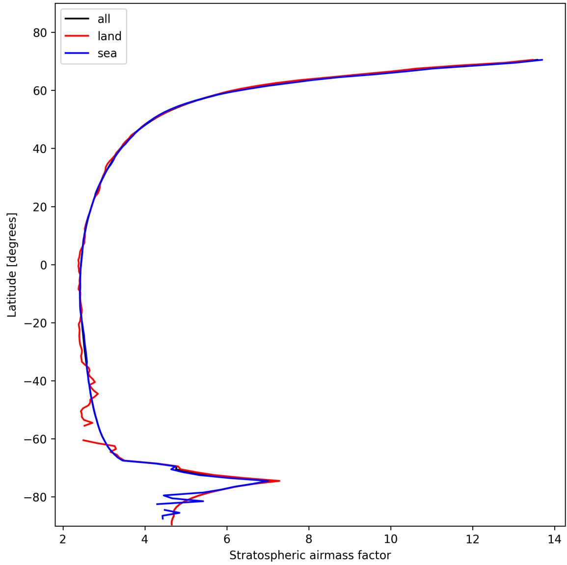
Figure 27: Zonal average of “Stratospheric airmass factor” for 2025-11-12 to 2025-11-13.
