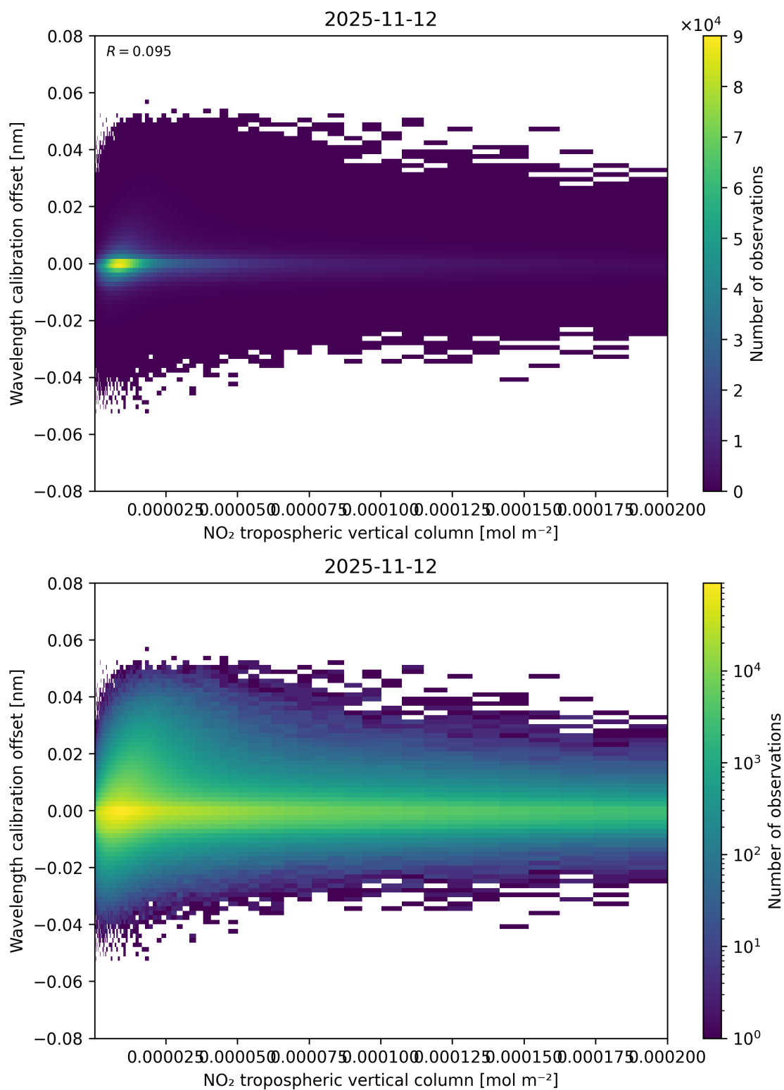
Figure 143: Scatter density plot of “NO 2 tropospheric vertical column” against “Wavelength calibration offset” for 2025-11-12 to 2025-11-13.
