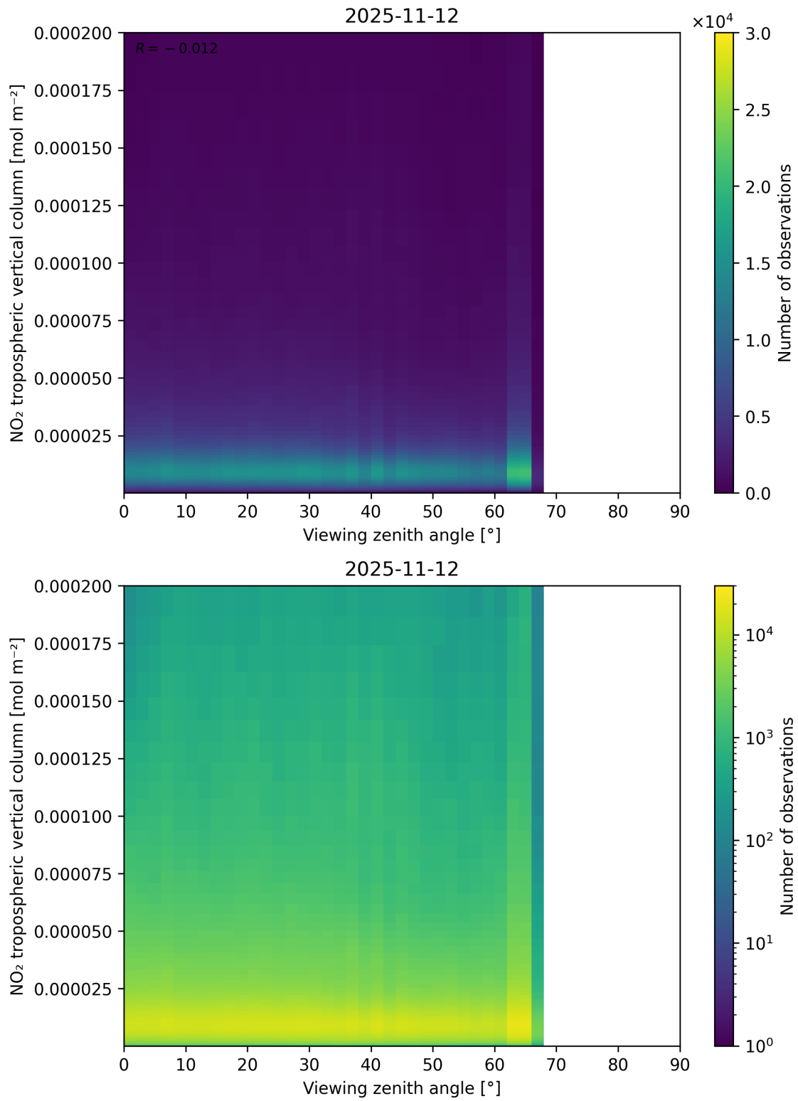
Figure 169: Scatter density plot of “Viewing zenith angle” against “NO 2 tropospheric vertical column” for 2025-11-12 to 2025-11-13.
