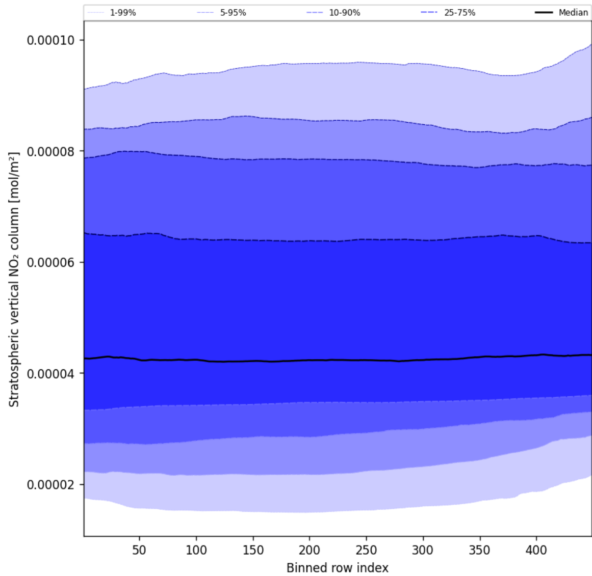
Figure 53: Along track statistics of “Stratospheric vertical NO 2 column” for 2025-11-12 to 2025-11-13
