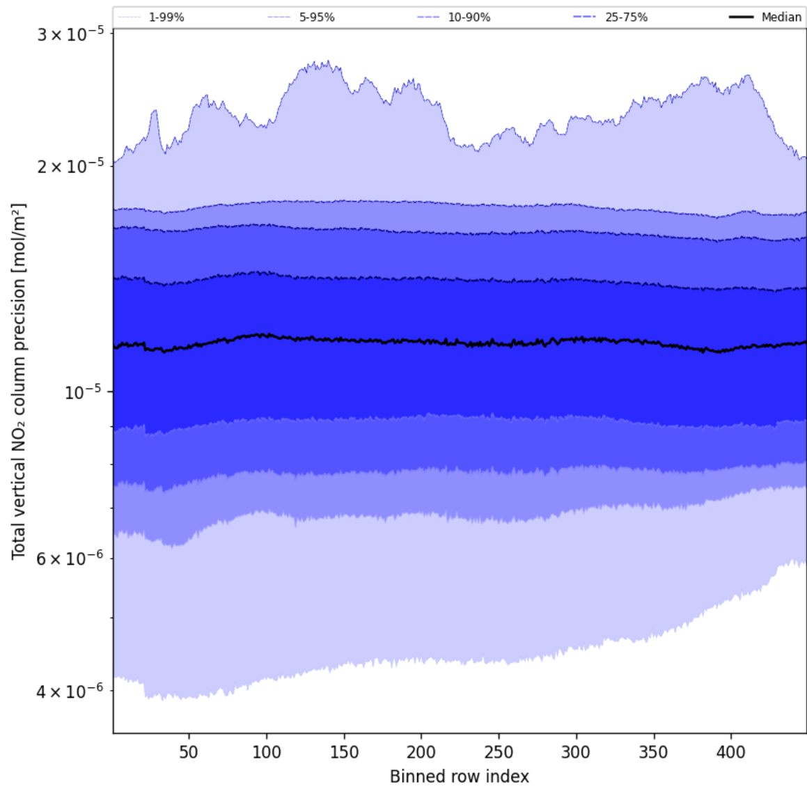
Figure 56: Along track statistics of “Total vertical NO 2 column precision” for 2025-11-12 to 2025-11-13
