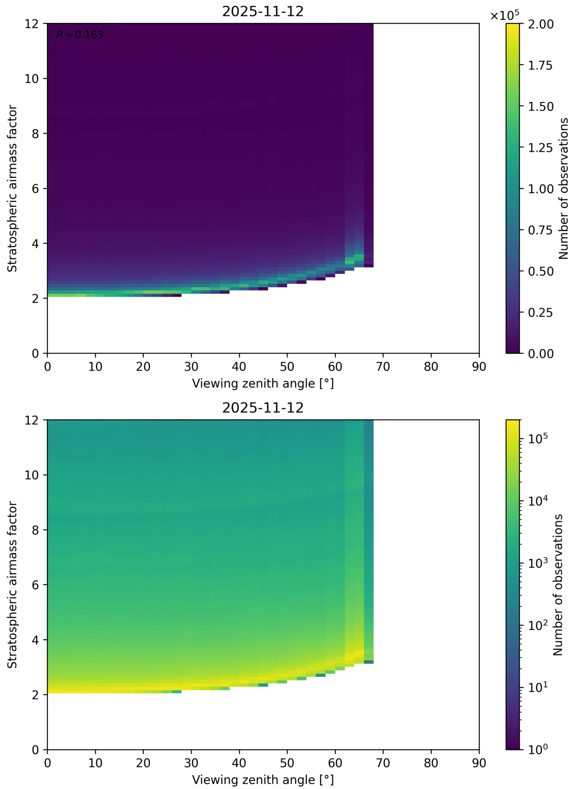
Figure 159: Scatter density plot of “Viewing zenith angle” against “Stratospheric airmass factor” for 2025-11-12 to 2025-11-13.
