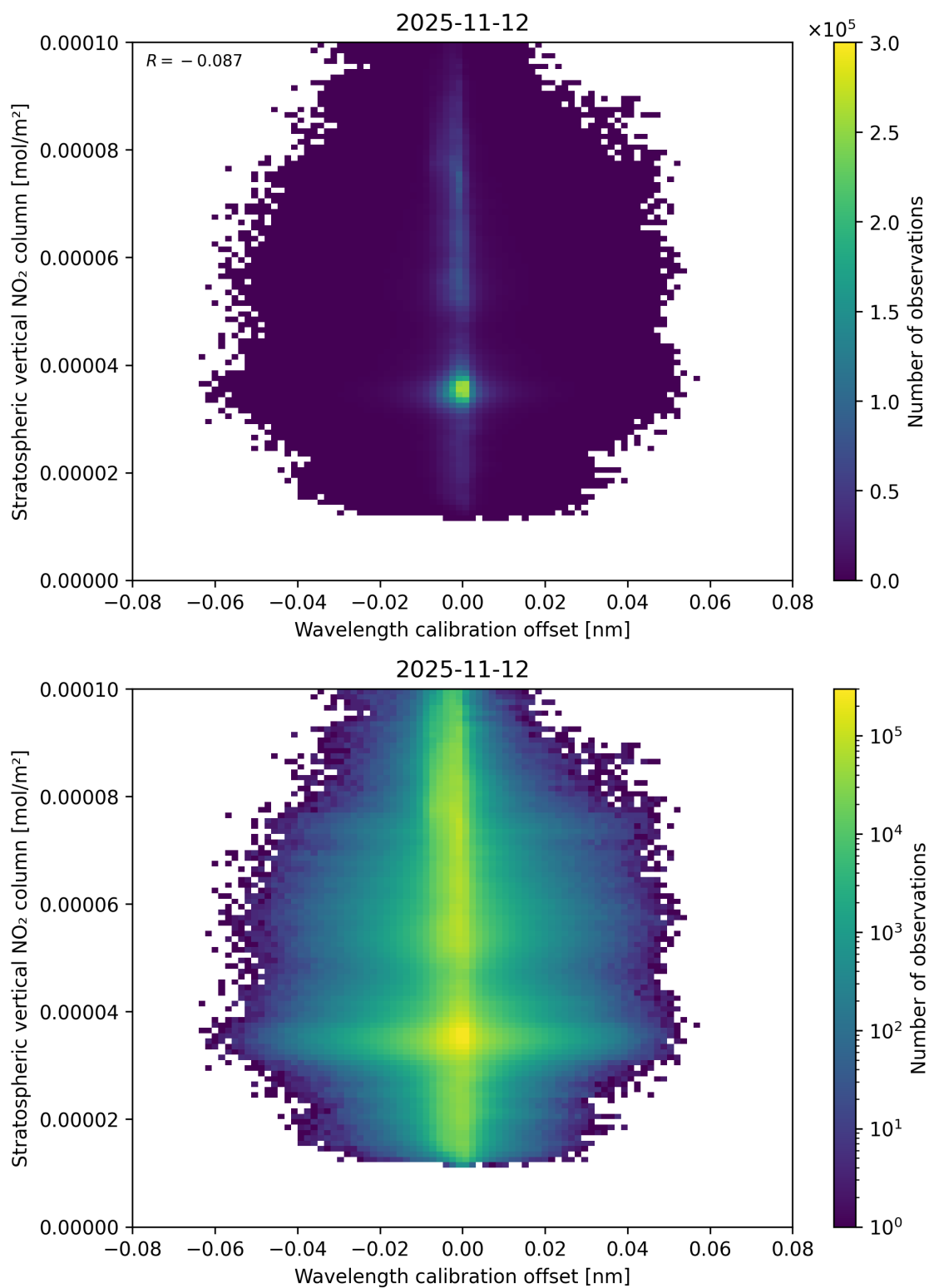
Figure 176: Scatter density plot of “Wavelength calibration offset” against “Stratospheric vertical NO 2 column” for 2025-11-12 to 2025-11-13.
