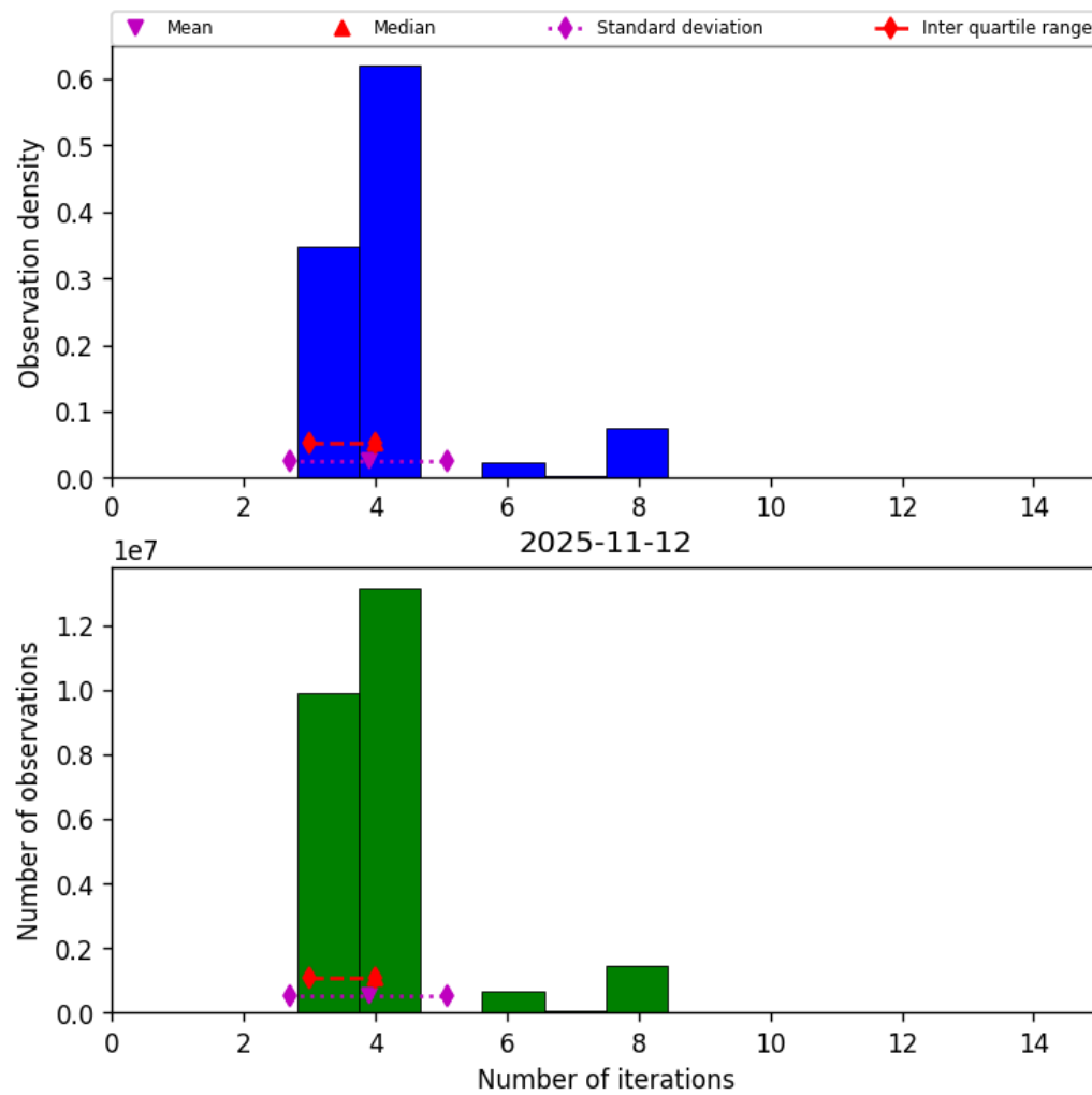
Figure 34: Histogram of “Number of iterations” for 2025-11-12 to 2025-11-13
