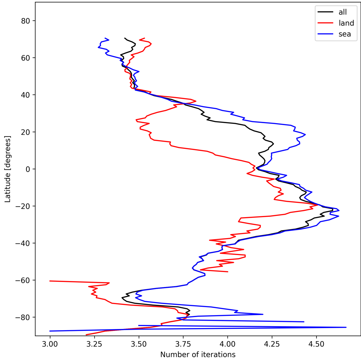
Figure 17: Zonal average of “Number of iterations” for 2025-11-12 to 2025-11-13.
