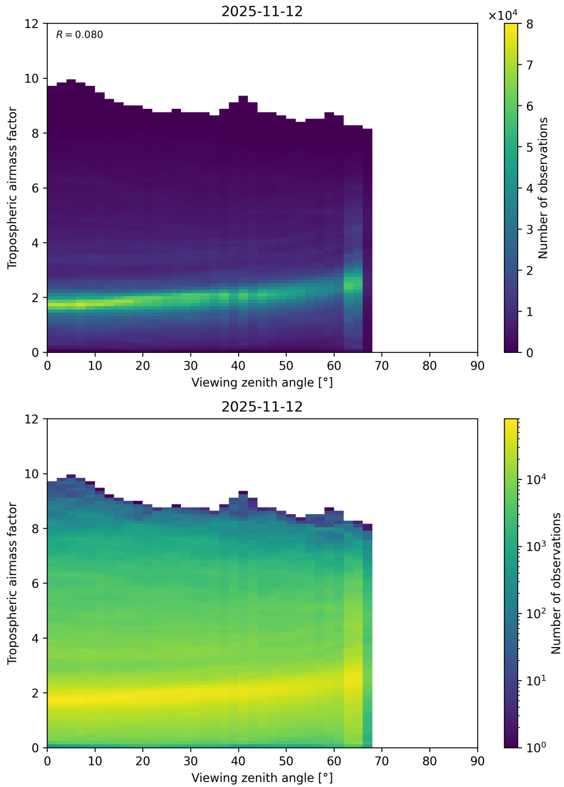
Figure 161: Scatter density plot of “Viewing zenith angle” against “Tropospheric airmass factor” for 2025-11-12 to 2025-11-13.
