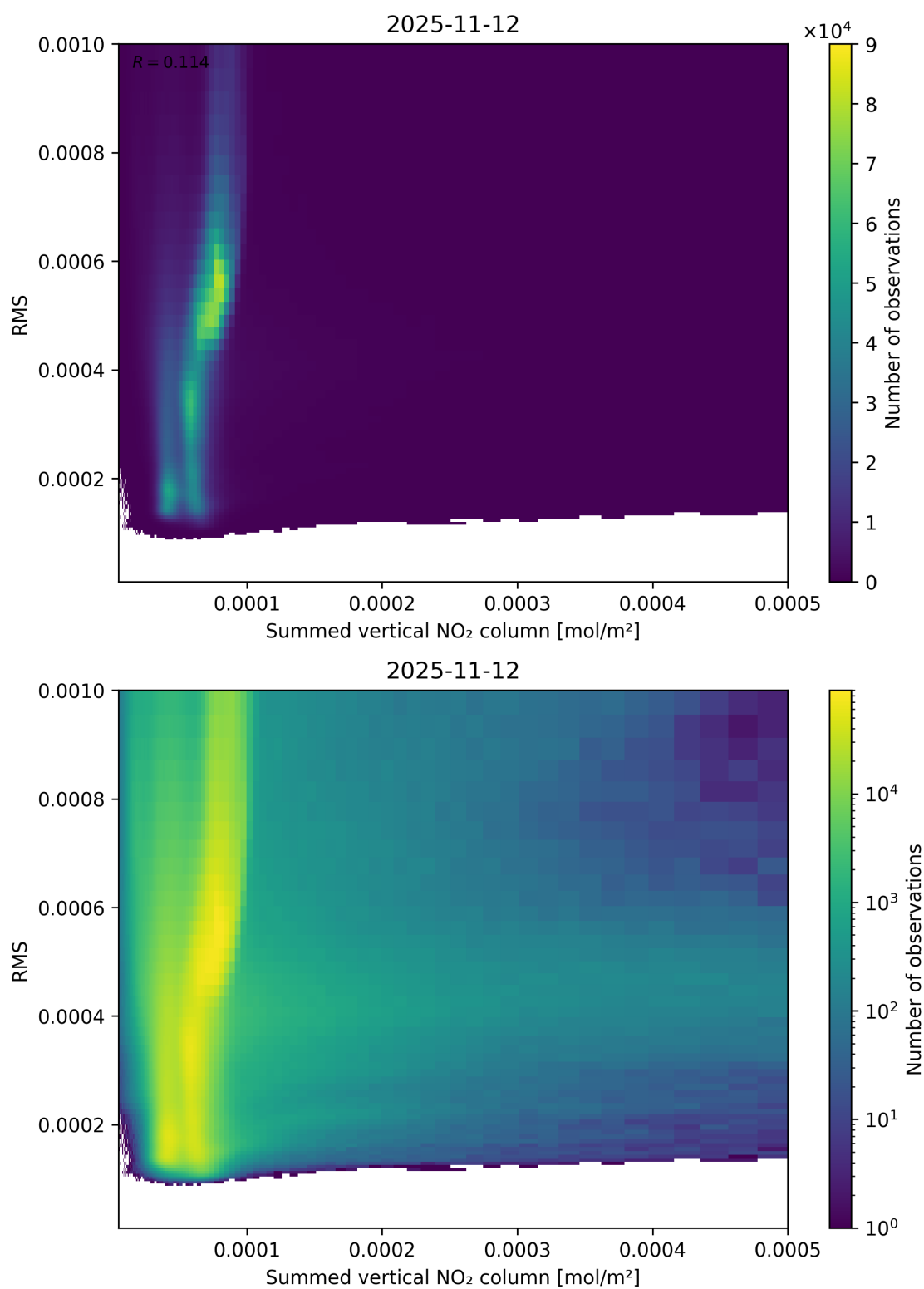
Figure 109: Scatter density plot of “Summed vertical NO 2 column” against “RMS” for 2025-11-12 to 2025-11-13.
