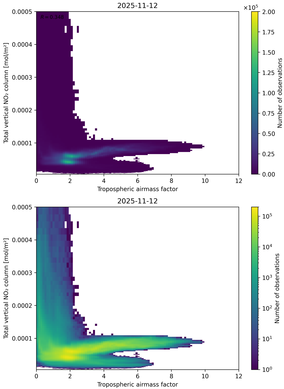
Figure 77: Scatter density plot of “Tropospheric airmass factor” against “Total vertical NO 2 column” for 2025-11-12 to 2025-11-13.
