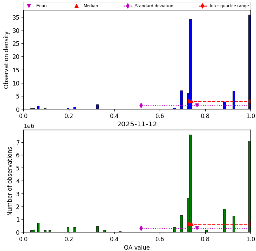
Figure 28: Histogram of “QA value” for 2025-11-12 to 2025-11-13
