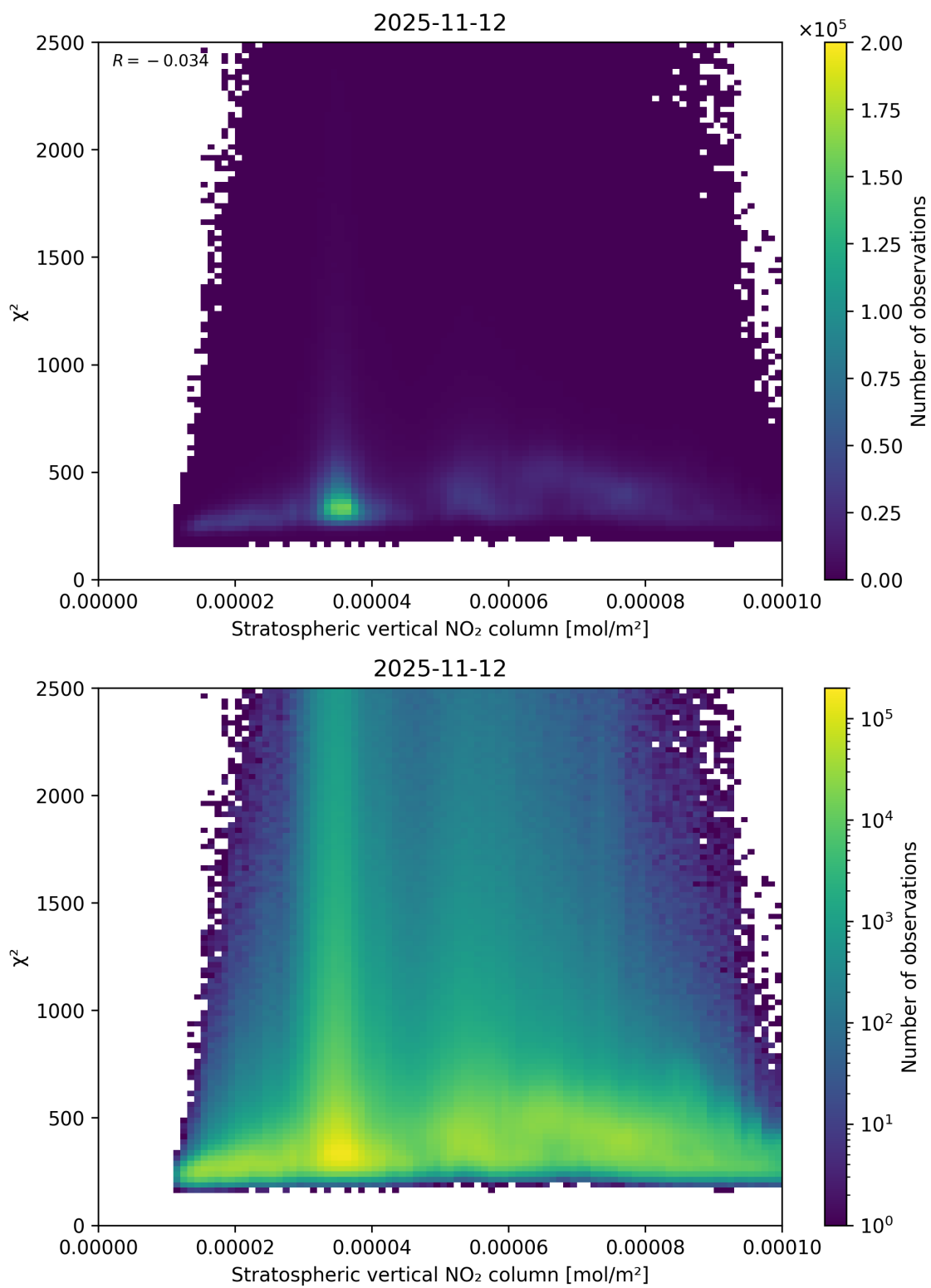
Figure 97: Scatter density plot of “Stratospheric vertical NO 2 column” against “ \chi^2 ” for 2025-11-12 to 2025-11-13.
