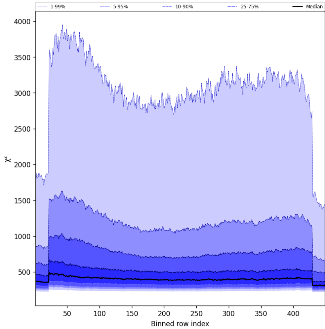
Figure 59: Along track statistics of “ \chi^2 ” for 2025-11-12 to 2025-11-13
