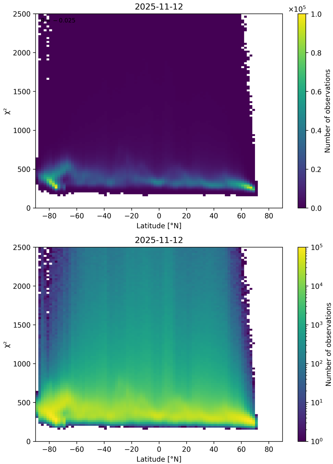
Figure 86: Scatter density plot of “Latitude” against “ \chi^2 ” for 2025-11-12 to 2025-11-13.
