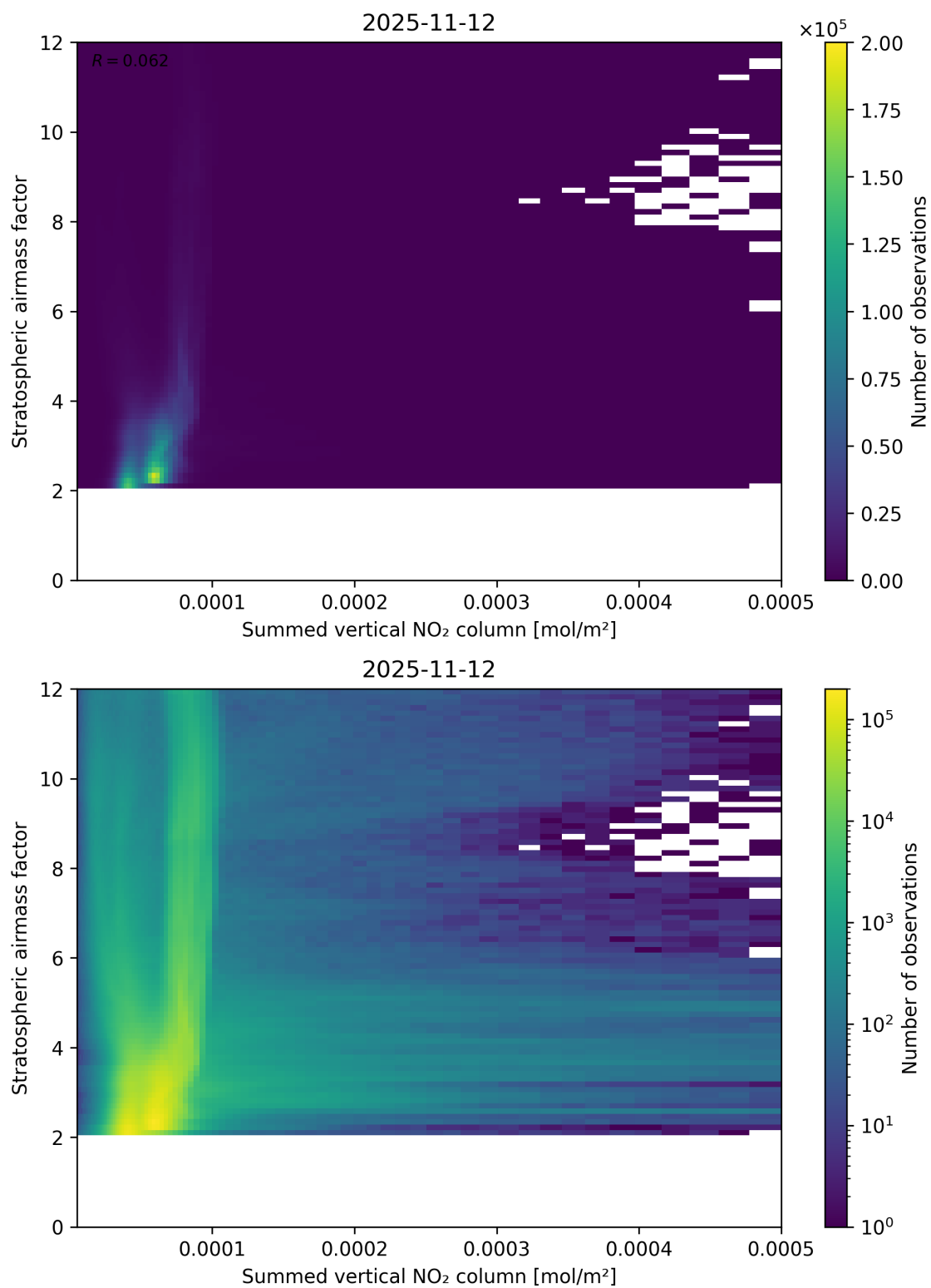
Figure 103: Scatter density plot of “Summed vertical NO 2 column” against “Stratospheric airmass factor” for 2025-11-12 to 2025-11-13.
