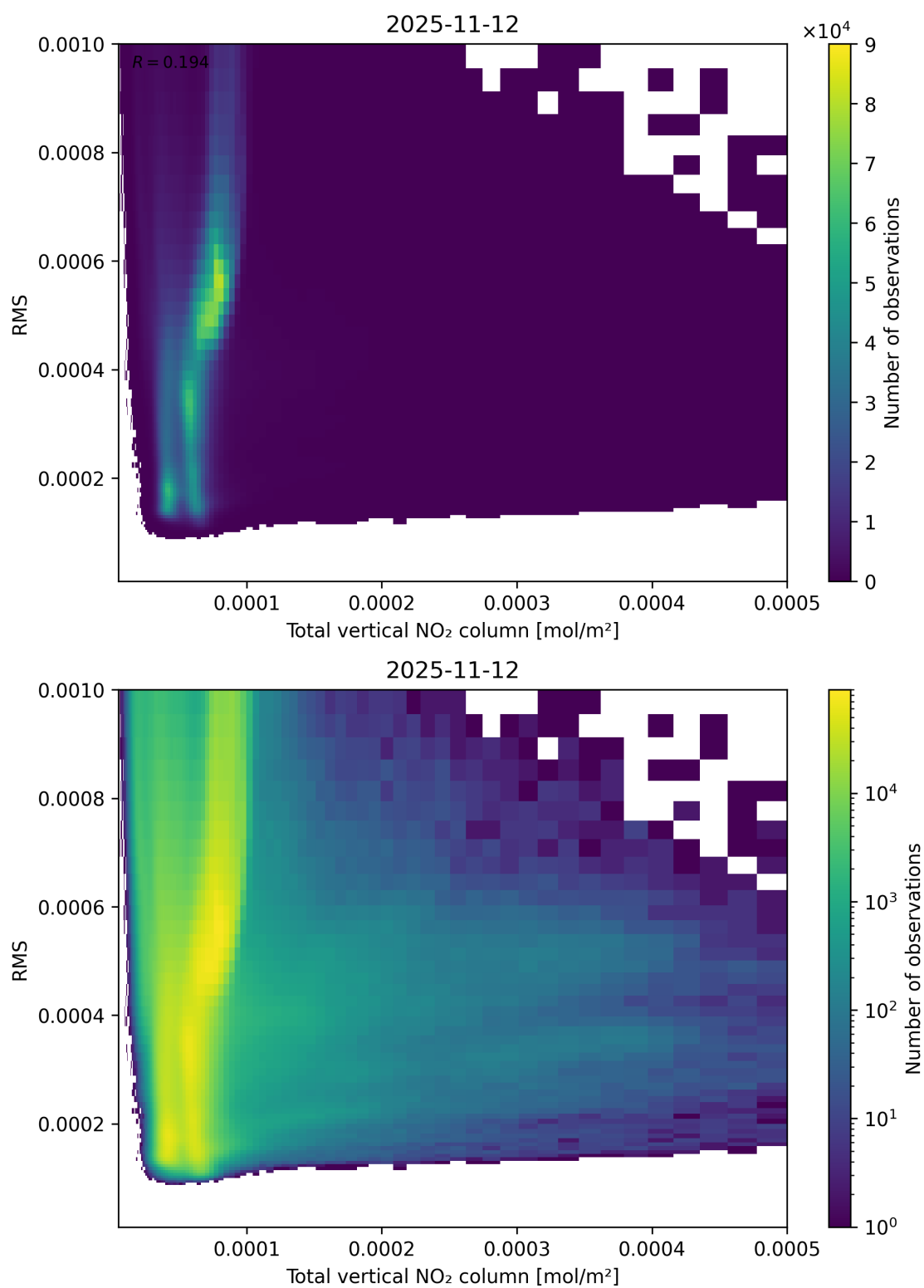
Figure 120: Scatter density plot of “Total vertical NO 2 column” against “RMS” for 2025-11-12 to 2025-11-13.
