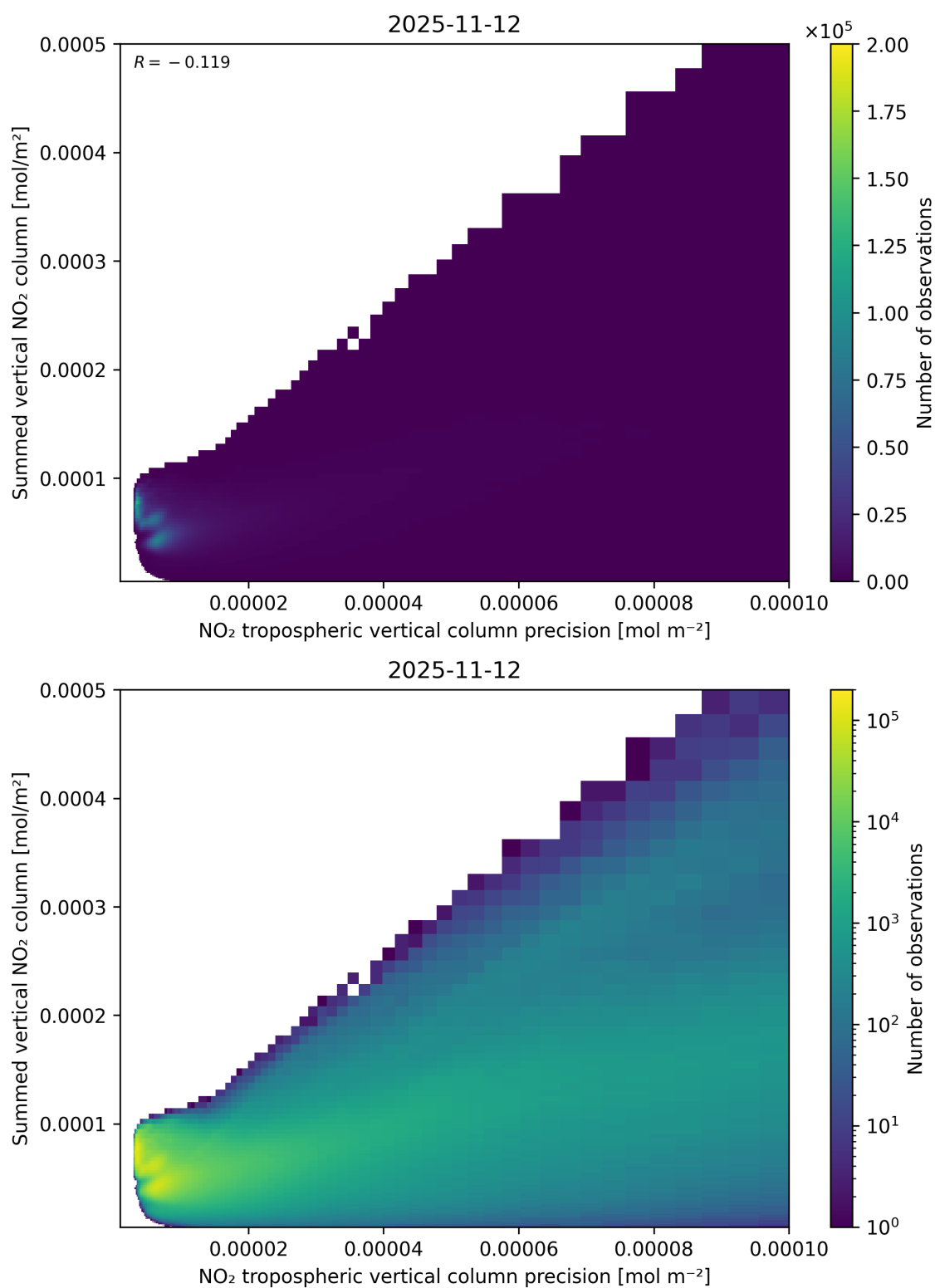
Figure 136: Scatter density plot of “NO 2 tropospheric vertical column precision” against “Summed vertical NO 2 column” for 2025-11-12 to 2025-11-13.
