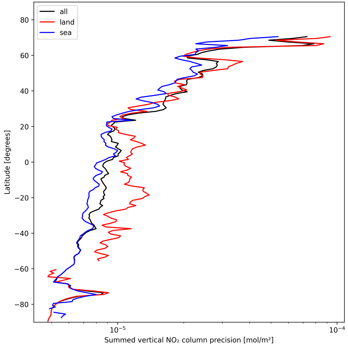
Figure 24: Zonal average of “Summed vertical NO 2 column precision” for 2025-11-12 to 2025-11-13.
