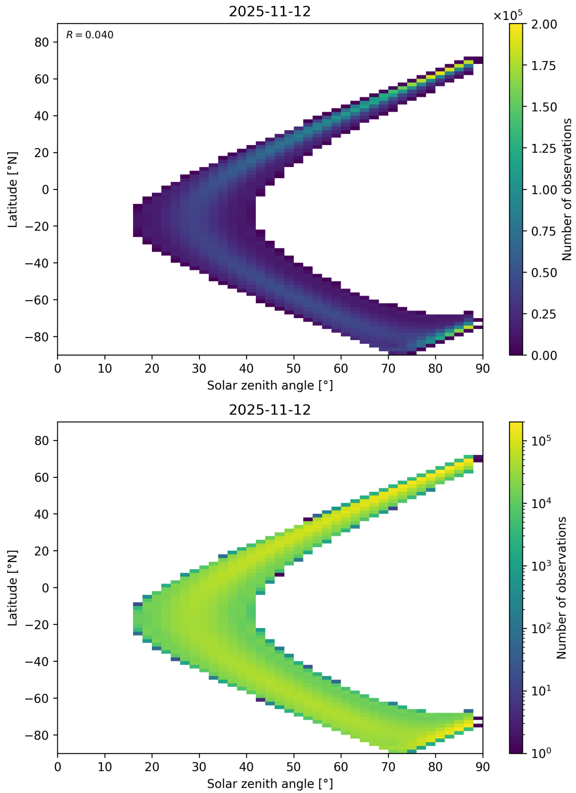
Figure 149: Scatter density plot of “Solar zenith angle” against “Latitude” for 2025-11-12 to 2025-11-13.
