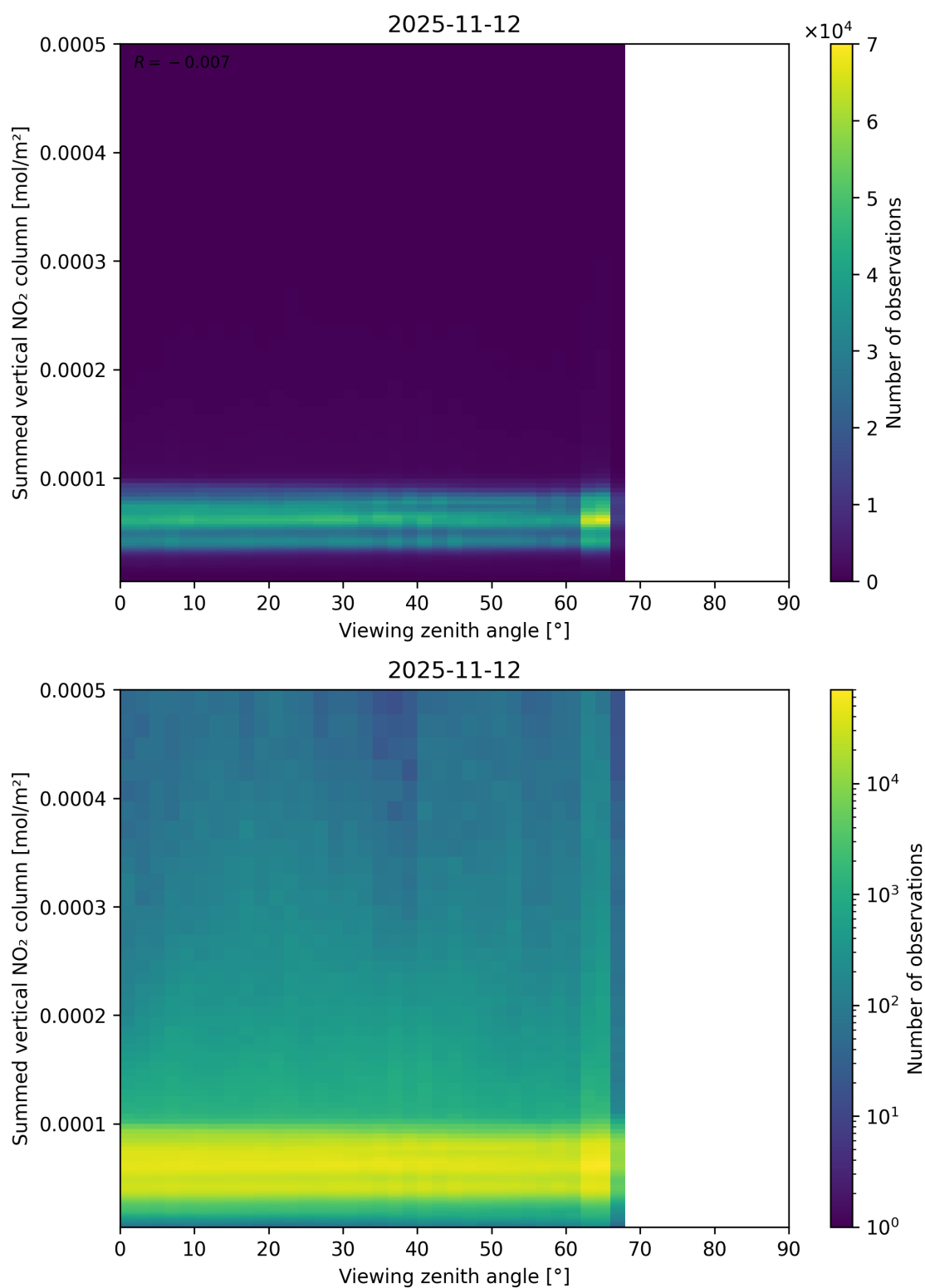
Figure 165: Scatter density plot of “Viewing zenith angle” against “Summed vertical NO 2 column” for 2025-11-12 to 2025-11-13.
