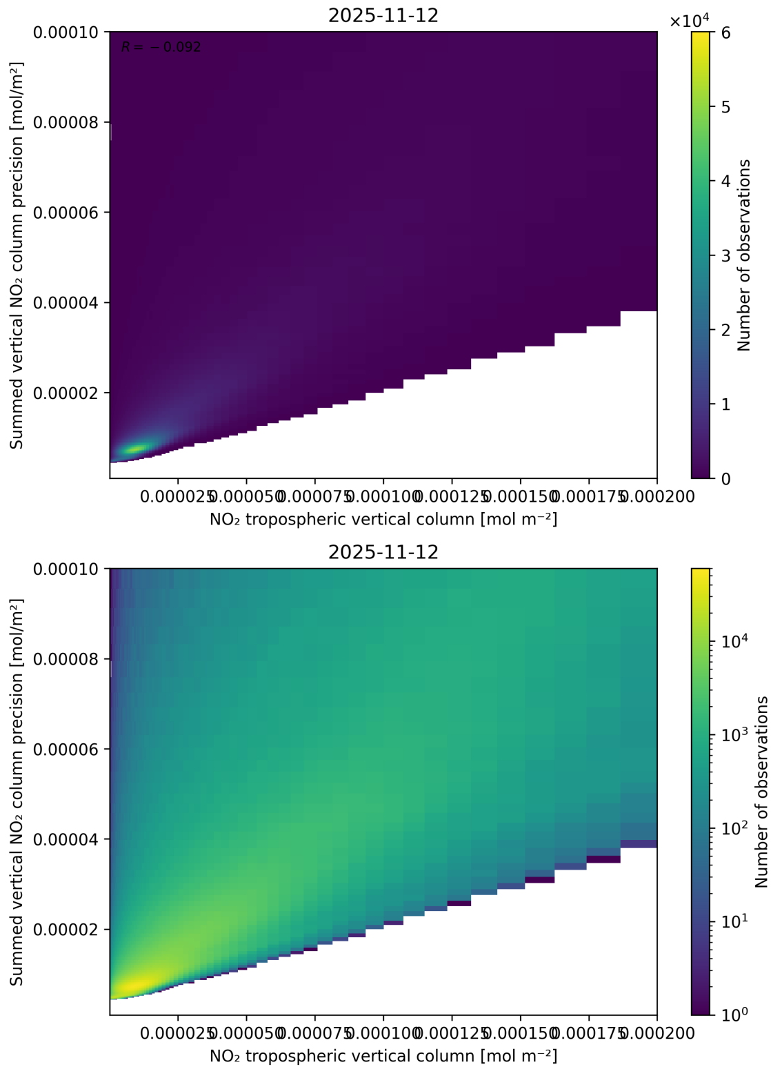
Figure 127: Scatter density plot of “NO 2 tropospheric vertical column” against “Summed vertical NO 2 column precision” for 2025-11-12 to 2025-11-13.
