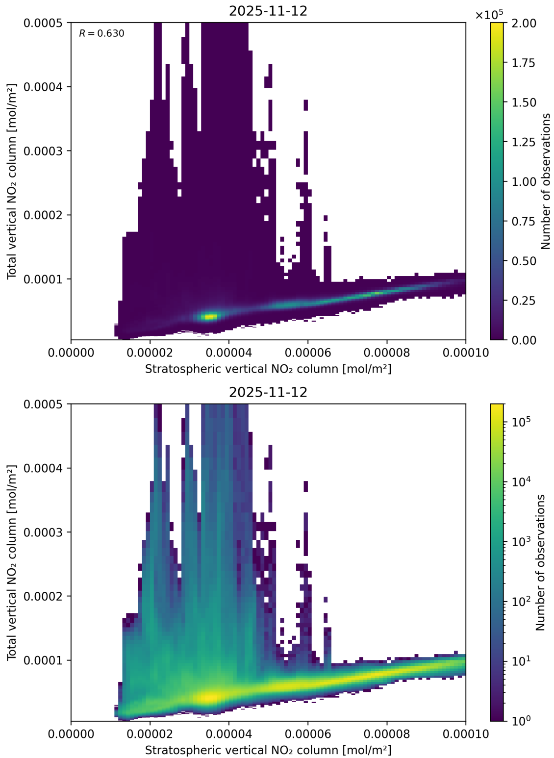
Figure 100: Scatter density plot of “Stratospheric vertical NO 2 column” against “Total vertical NO 2 column” for 2025-11-12 to 2025-11-13.
