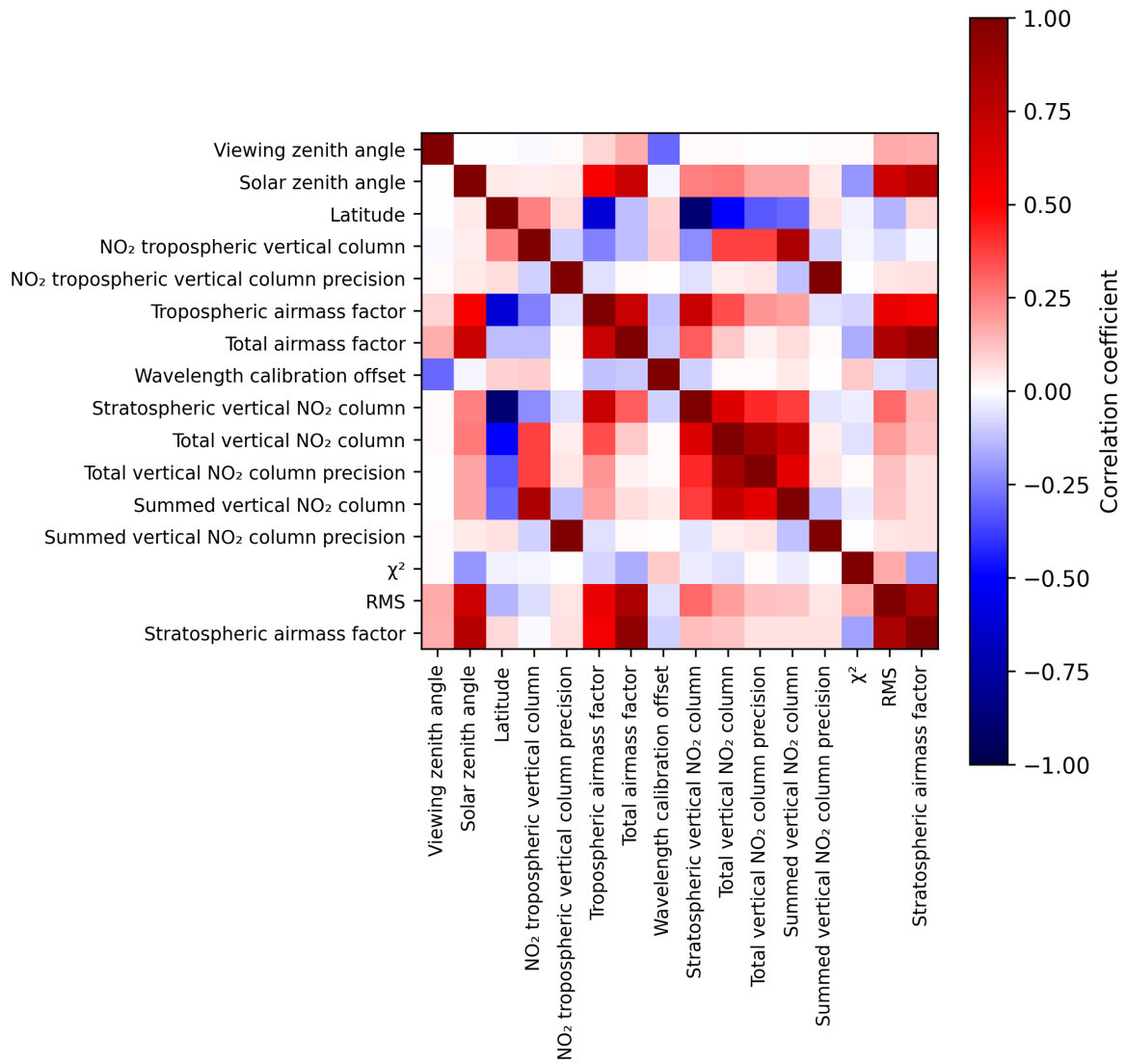
Figure 2: Map of correlation matrix for 2025-11-12 to 2025-11-13.
