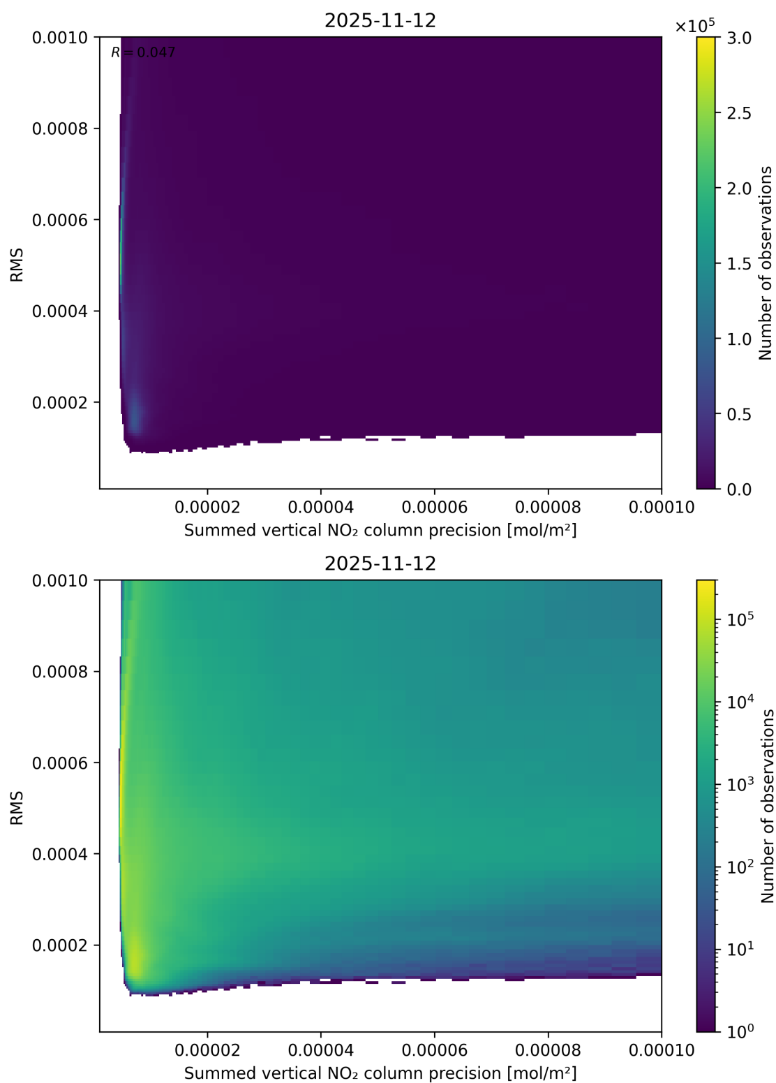
Figure 108: Scatter density plot of “Summed vertical NO 2 column precision” against “RMS” for 2025-11-12 to 2025-11-13.
