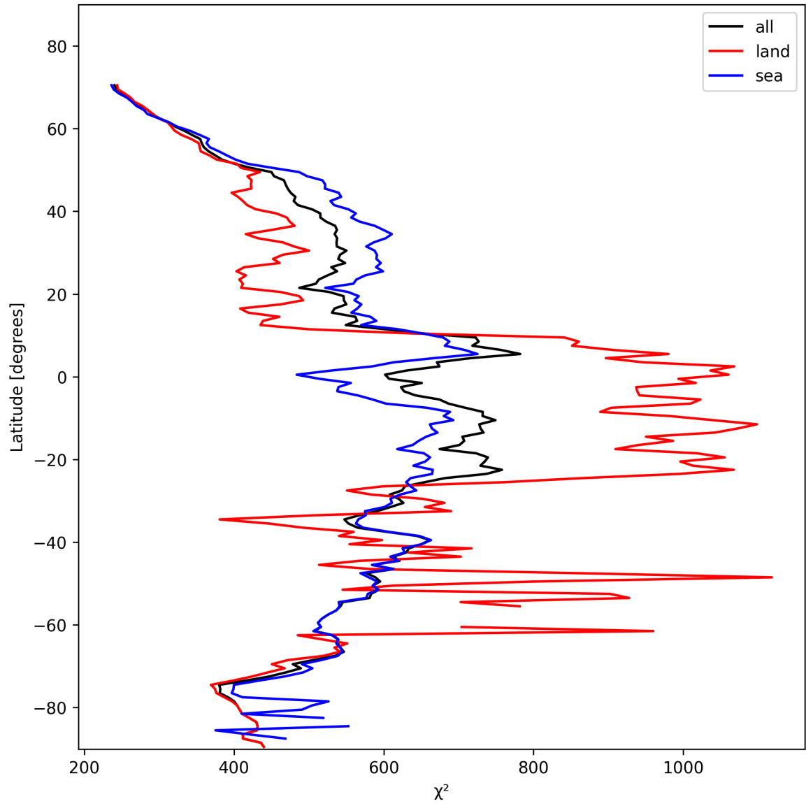
Figure 25: Zonal average of “ \chi^2 ” for 2025-11-12 to 2025-11-13.
