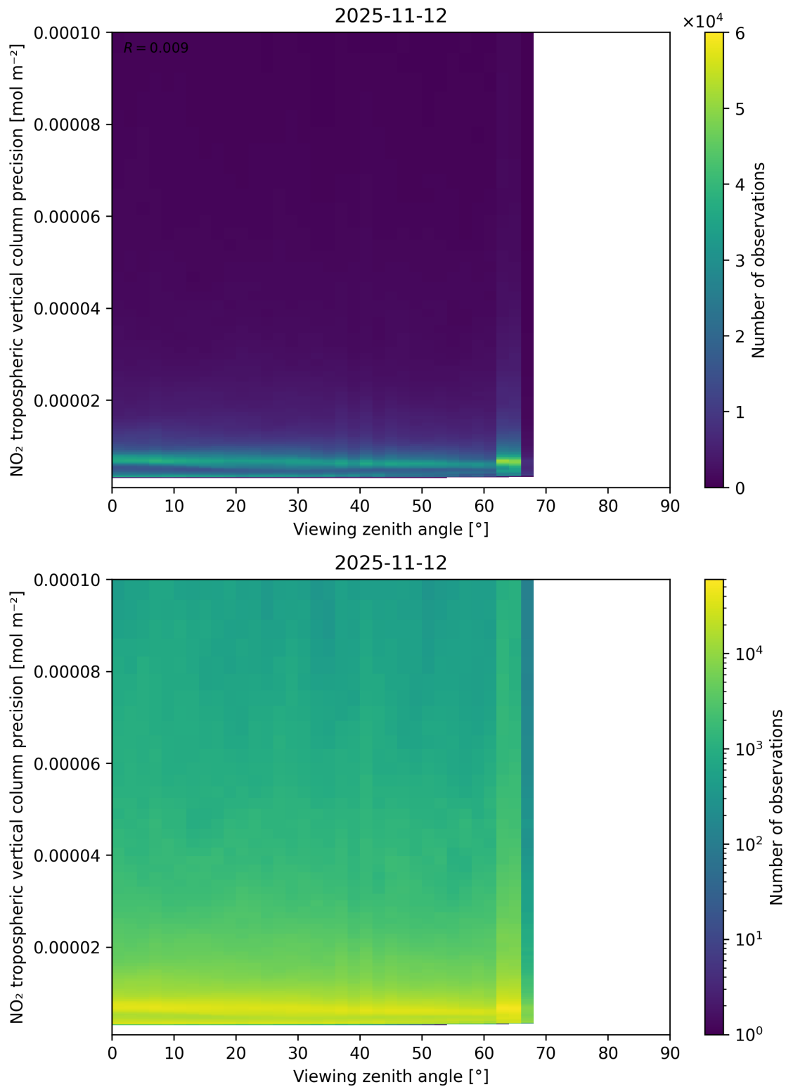
Figure 170: Scatter density plot of “Viewing zenith angle” against “NO 2 tropospheric vertical column precision” for 2025-11-12 to 2025-11-13.
