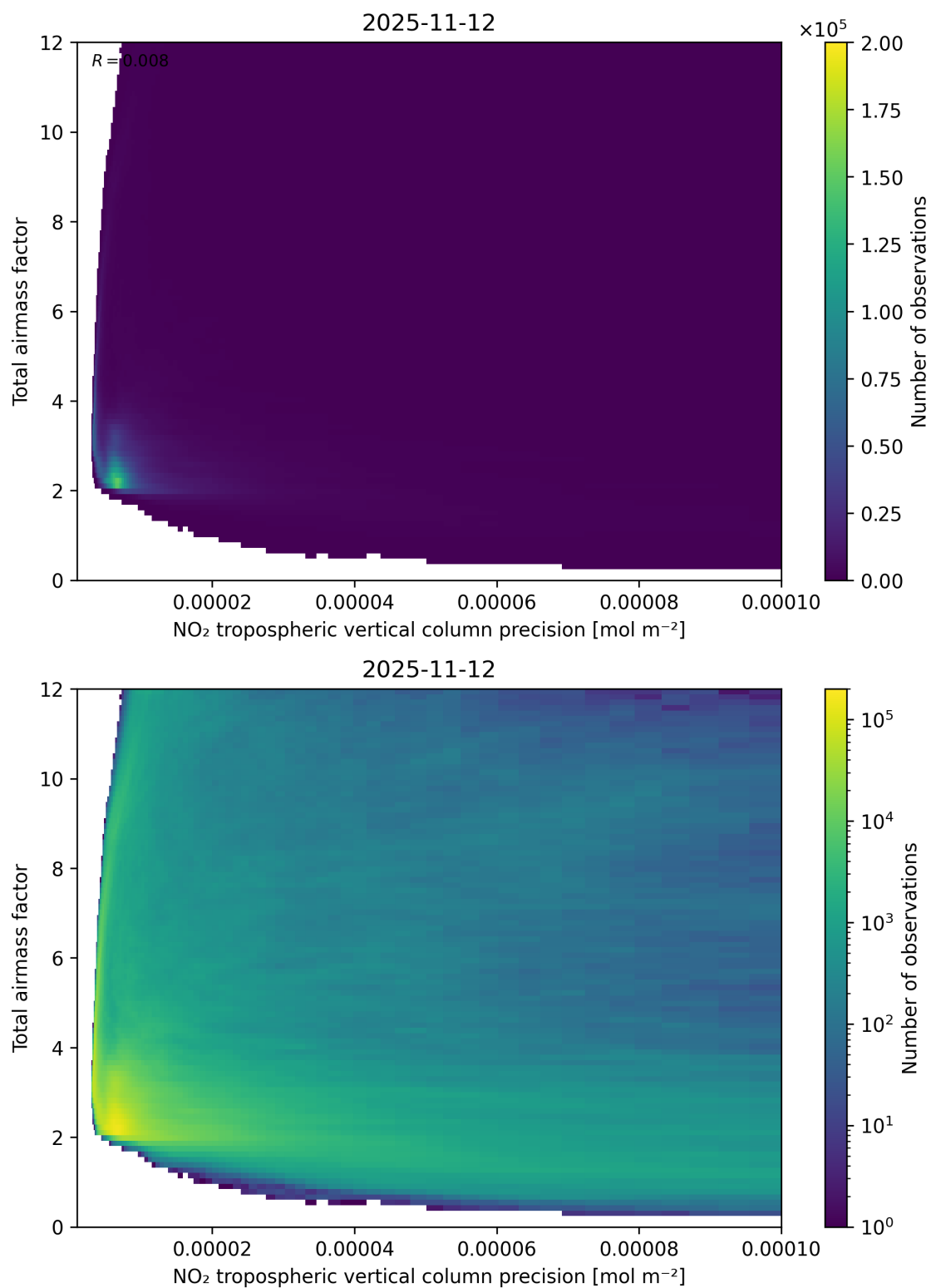
Figure 132: Scatter density plot of “NO 2 tropospheric vertical column precision” against “Total air mass factor” for 2025-11-12 to 2025-11-13.
