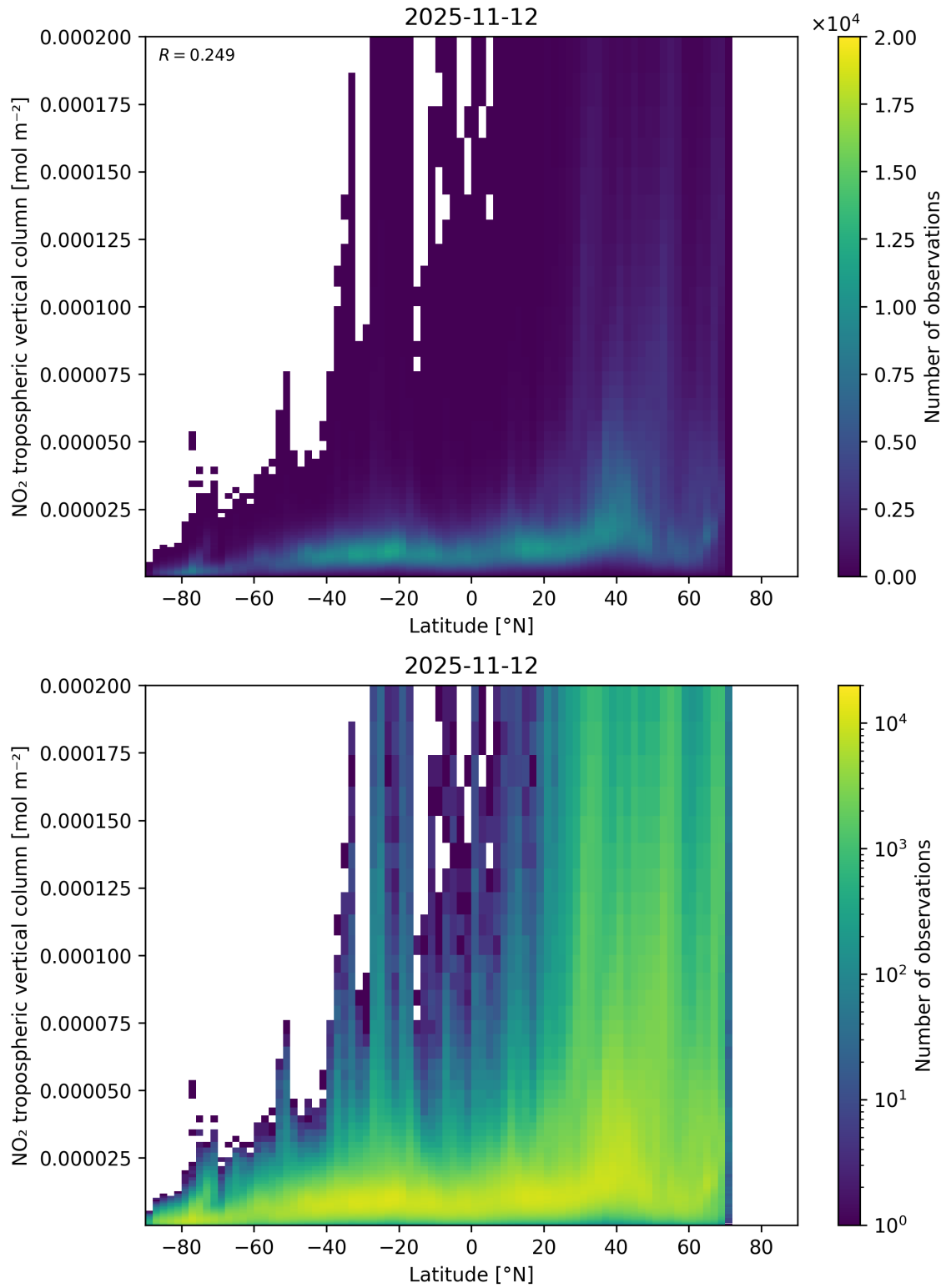
Figure 92: Scatter density plot of “Latitude” against “NO 2 tropospheric vertical column” for 2025-11-12 to 2025-11-13.
