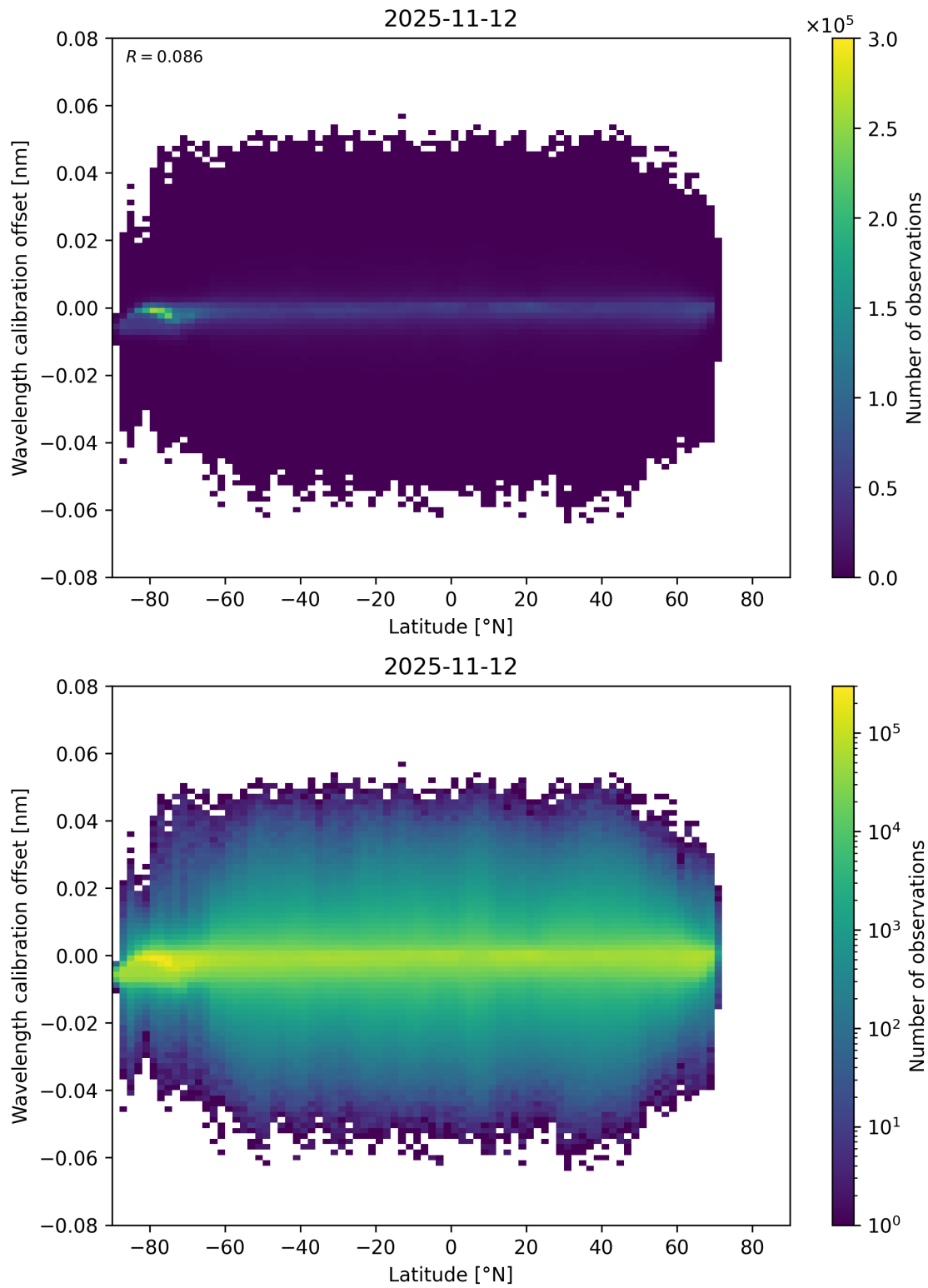
Figure 95: Scatter density plot of “Latitude” against “Wavelength calibration offset” for 2025-11-12 to 2025-11-13.
