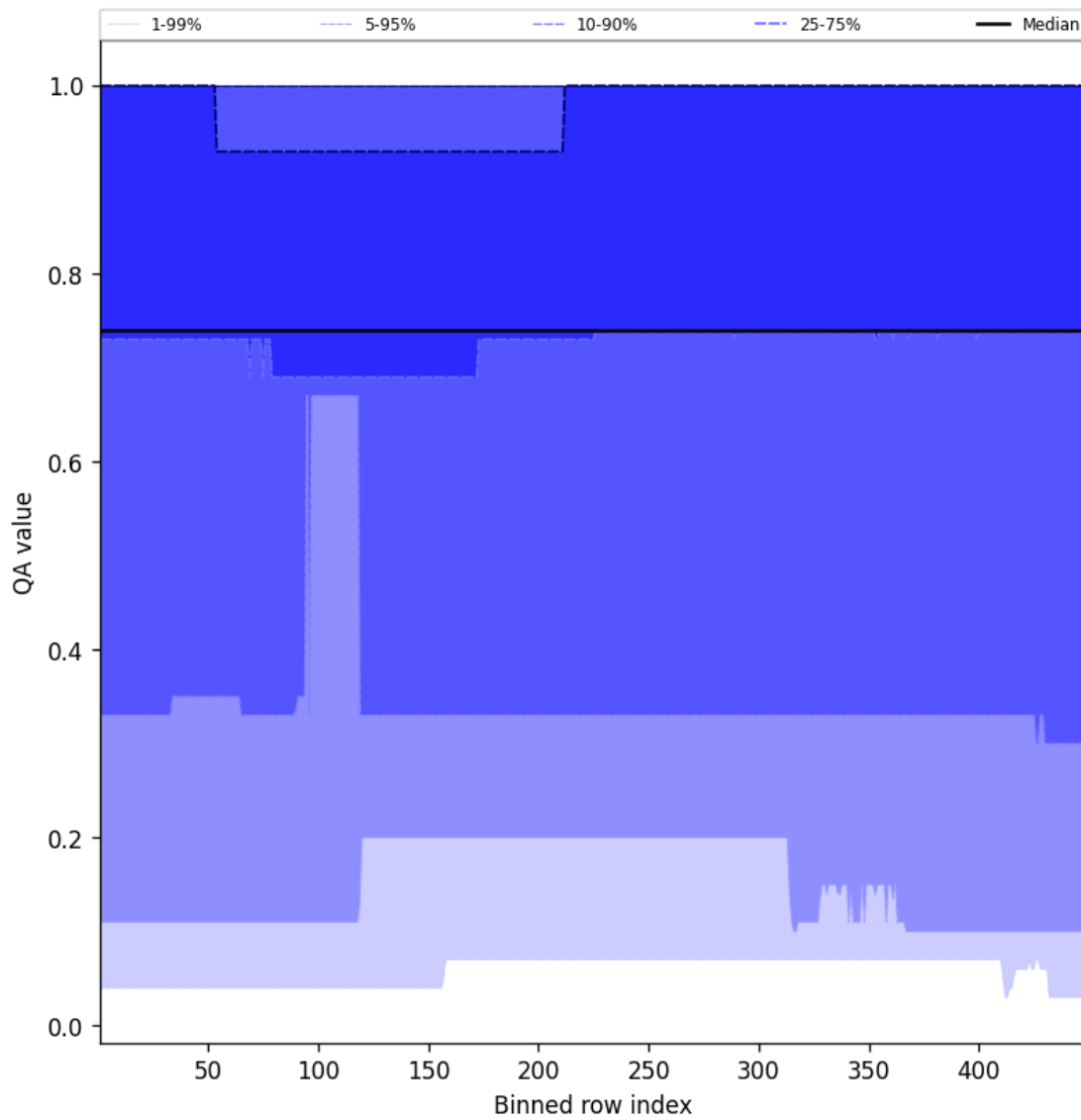
Figure 45: Along track statistics of “QA value” for 2025-11-12 to 2025-11-13
