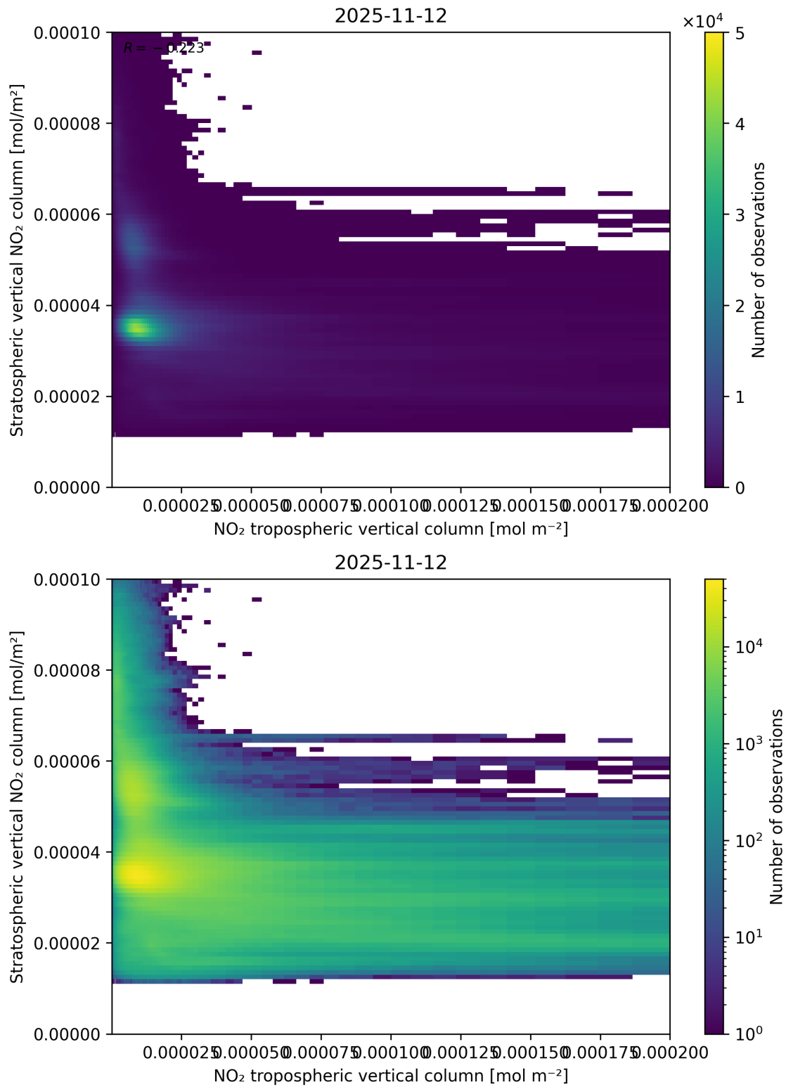
Figure 125: Scatter density plot of “NO 2 tropospheric vertical column” against “Stratospheric vertical NO 2 column” for 2025-11-12 to 2025-11-13.
