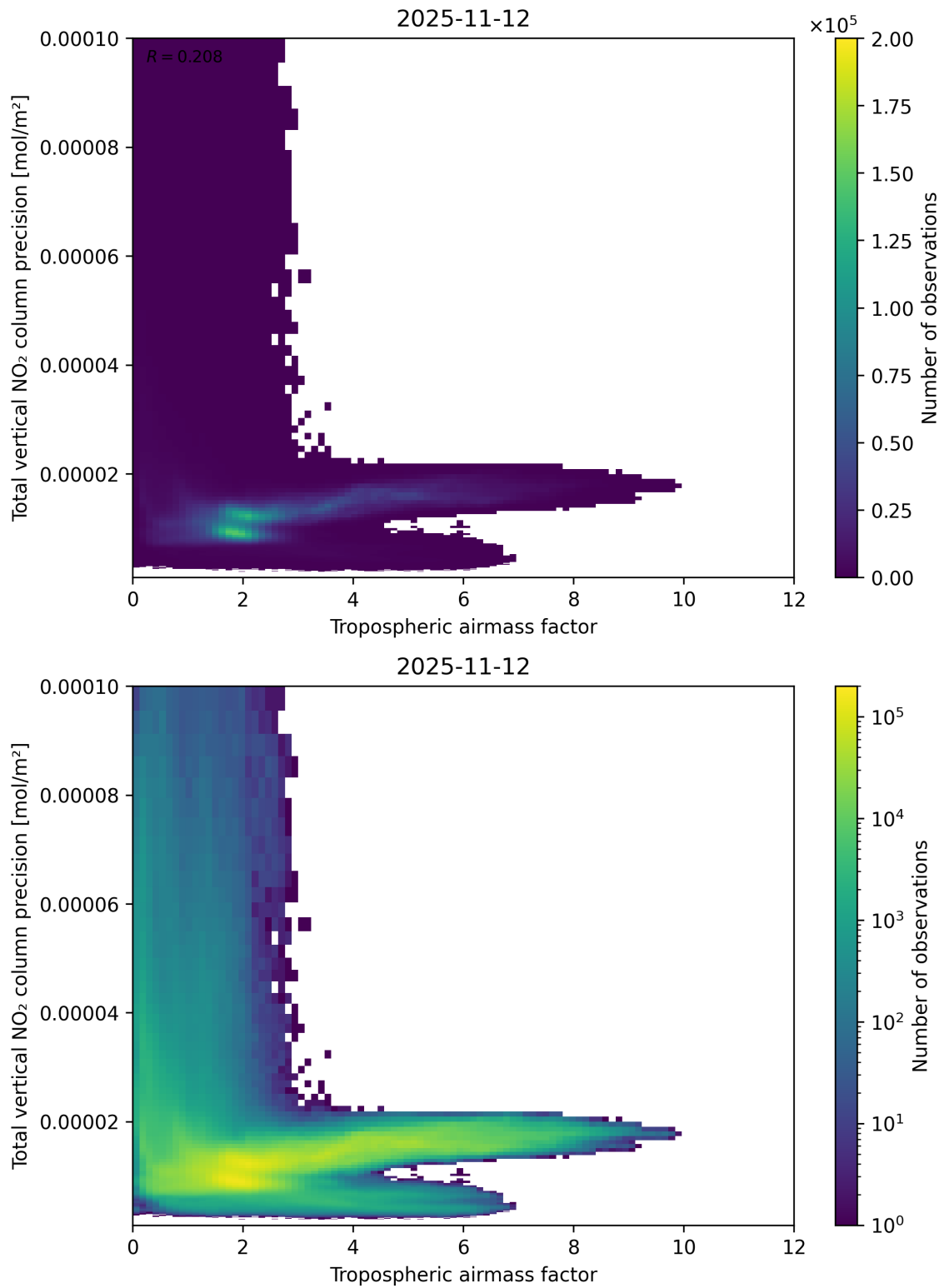
Figure 78: Scatter density plot of “Tropospheric air mass factor” against “Total vertical NO 2 column precision” for 2025-11-12 to 2025-11-13.
