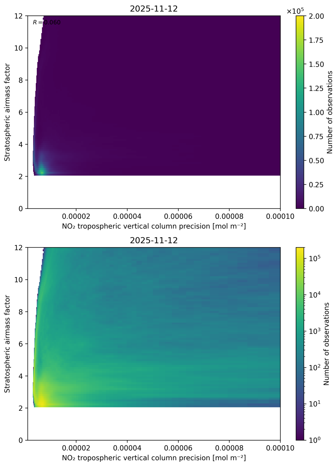
Figure 131: Scatter density plot of “NO 2 tropospheric vertical column precision” against “Stratospheric airmass factor” for 2025-11-12 to 2025-11-13.
