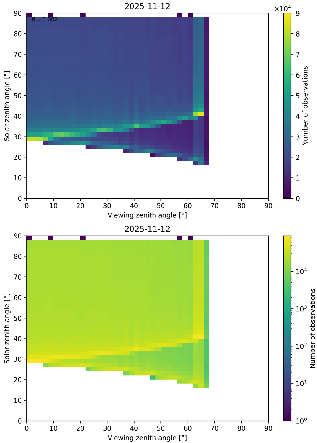
Figure 172: Scatter density plot of “Viewing zenith angle” against “Solar zenith angle” for 2025-11-12 to 2025-11-13.
