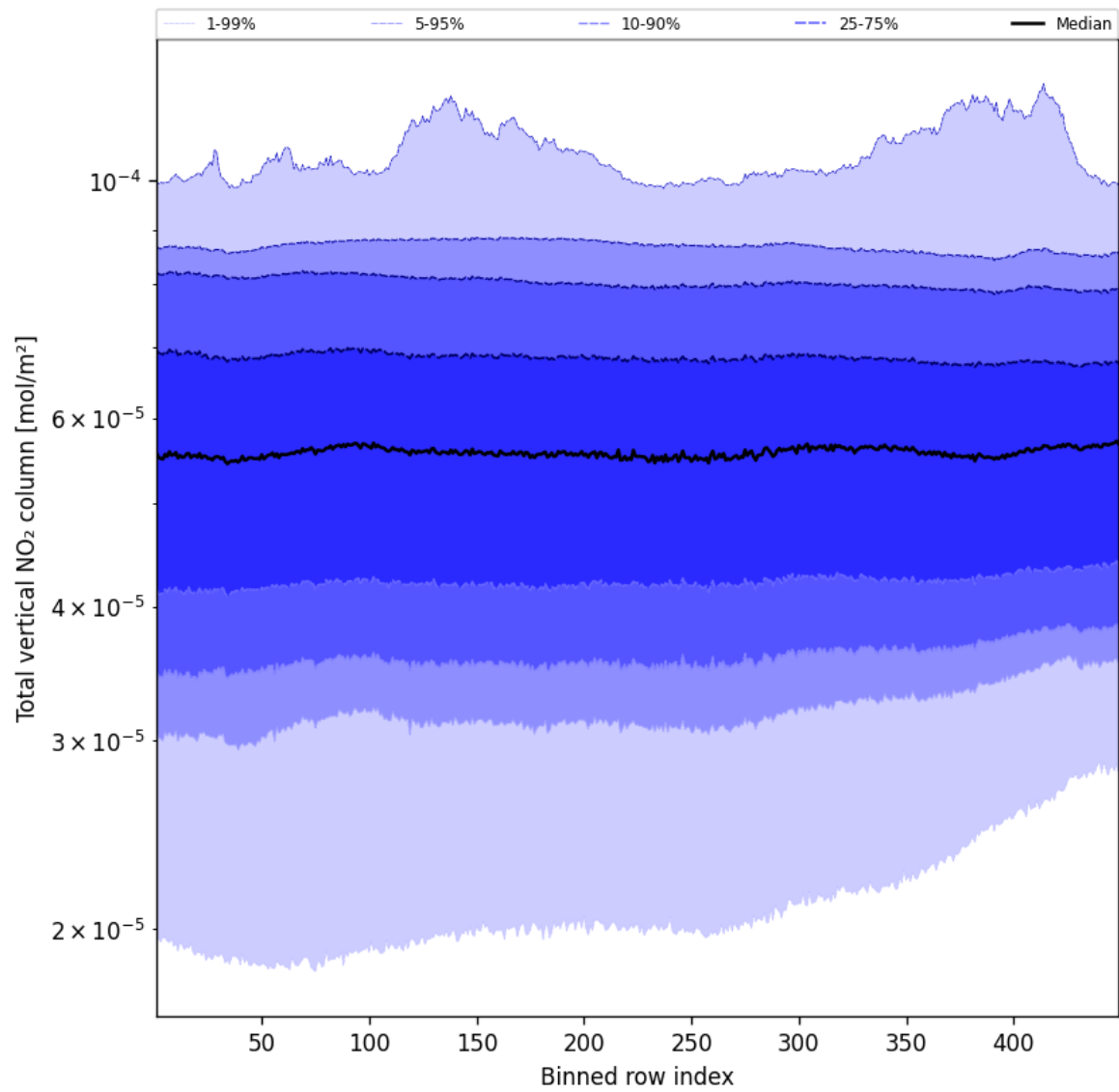
Figure 55: Along track statistics of “Total vertical NO 2 column” for 2025-11-12 to 2025-11-13
