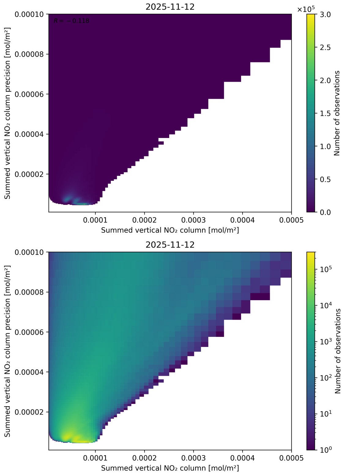
Figure 105: Scatter density plot of “Summed vertical NO 2 column” against “Summed vertical NO 2 column precision” for 2025-11-12 to 2025-11-13.
