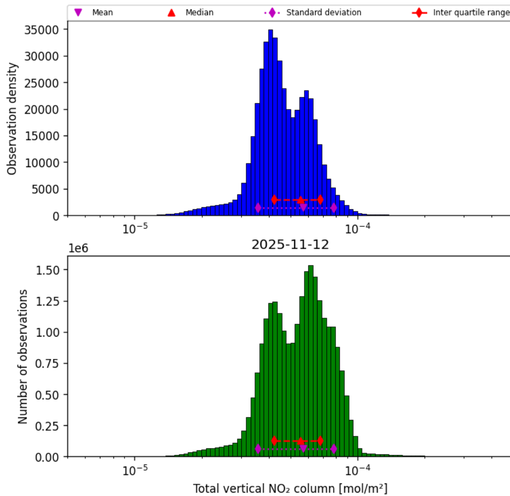
Figure 38: Histogram of “Total vertical NO 2 column” for 2025-11-12 to 2025-11-13
