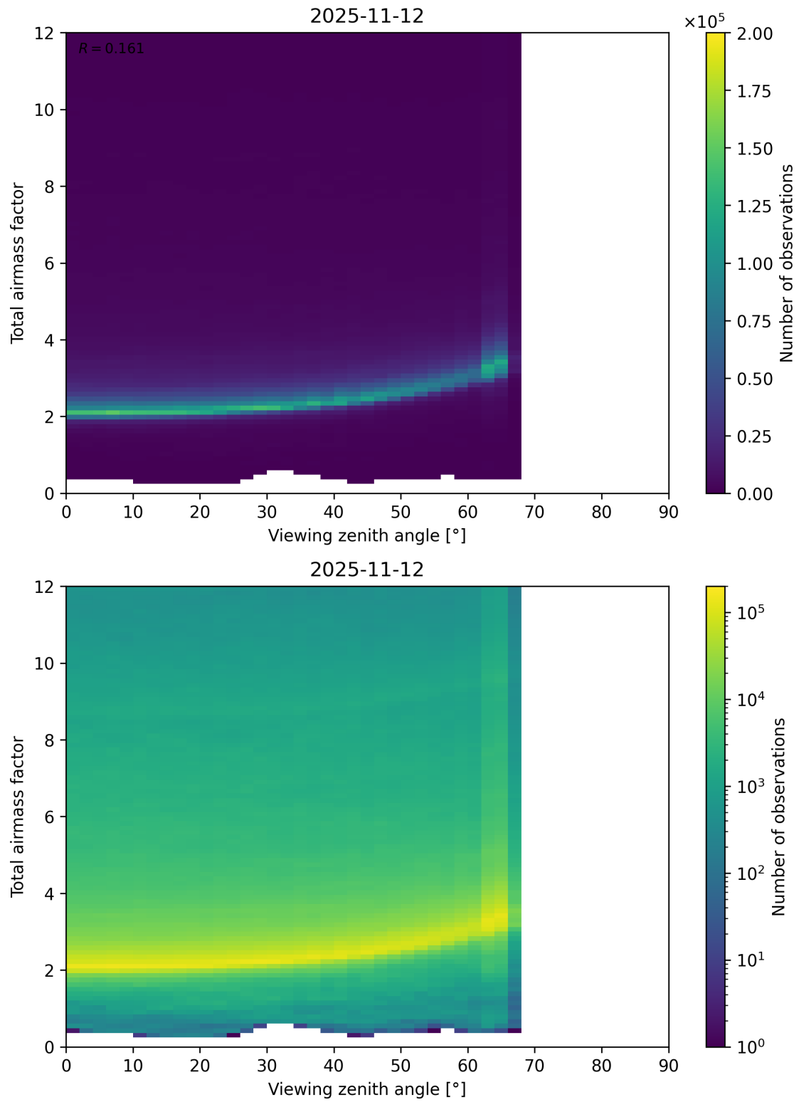
Figure 160: Scatter density plot of “Viewing zenith angle” against “Total airmass factor” for 2025-11-12 to 2025-11-13.
