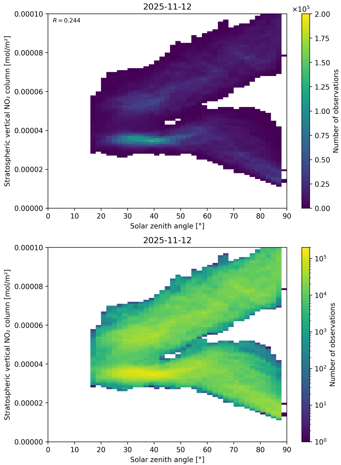
Figure 150: Scatter density plot of “Solar zenith angle” against “Stratospheric vertical NO 2 column” for 2025-11-12 to 2025-11-13.
