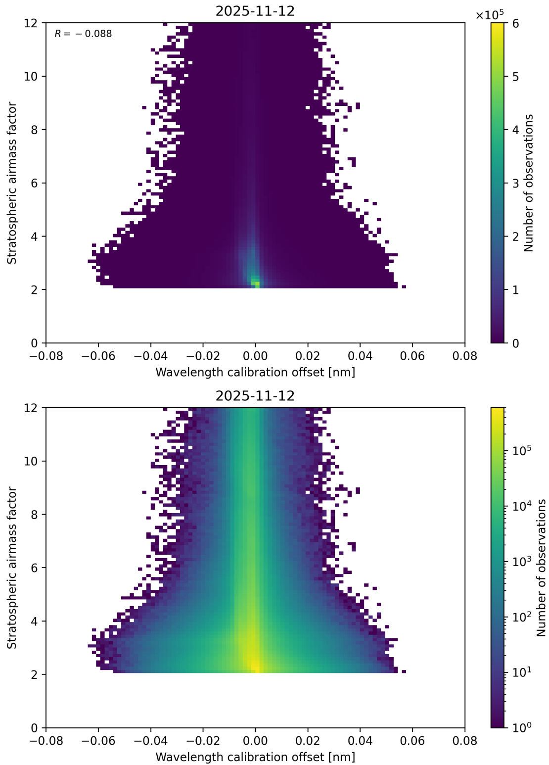
Figure 174: Scatter density plot of “Wavelength calibration offset” against “Stratospheric airmass factor” for 2025-11-12 to 2025-11-13.
