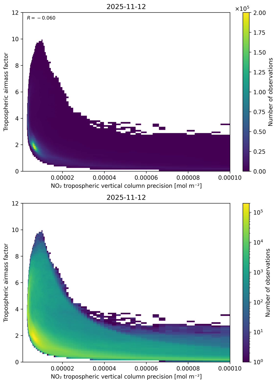
Figure 133: Scatter density plot of “NO 2 tropospheric vertical column precision” against “Tropospheric airmass factor” for 2025-11-12 to 2025-11-13.
