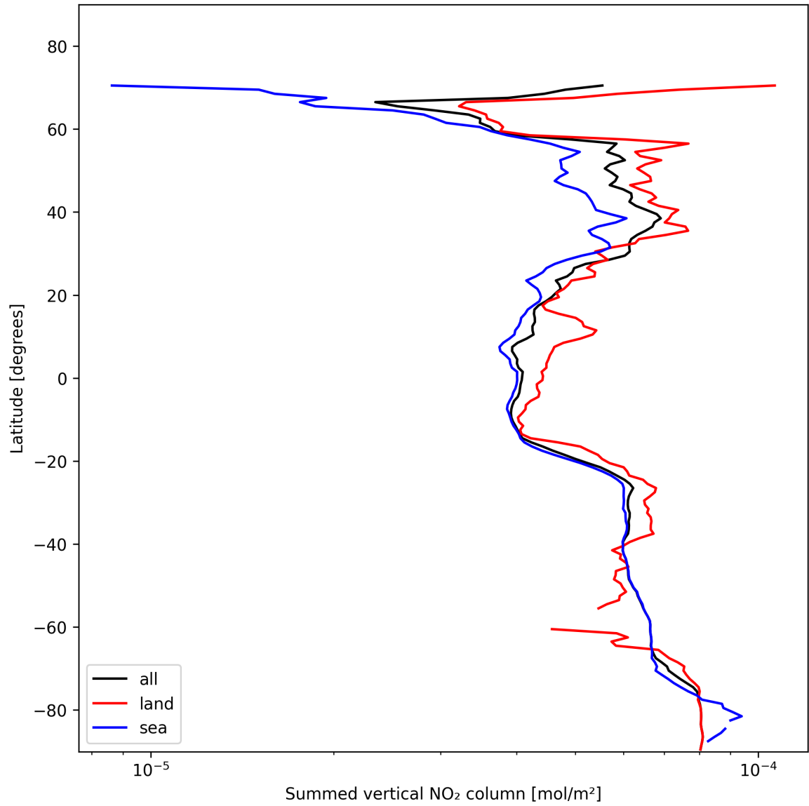
Figure 23: Zonal average of “Summed vertical NO 2 column” for 2025-11-12 to 2025-11-13.
