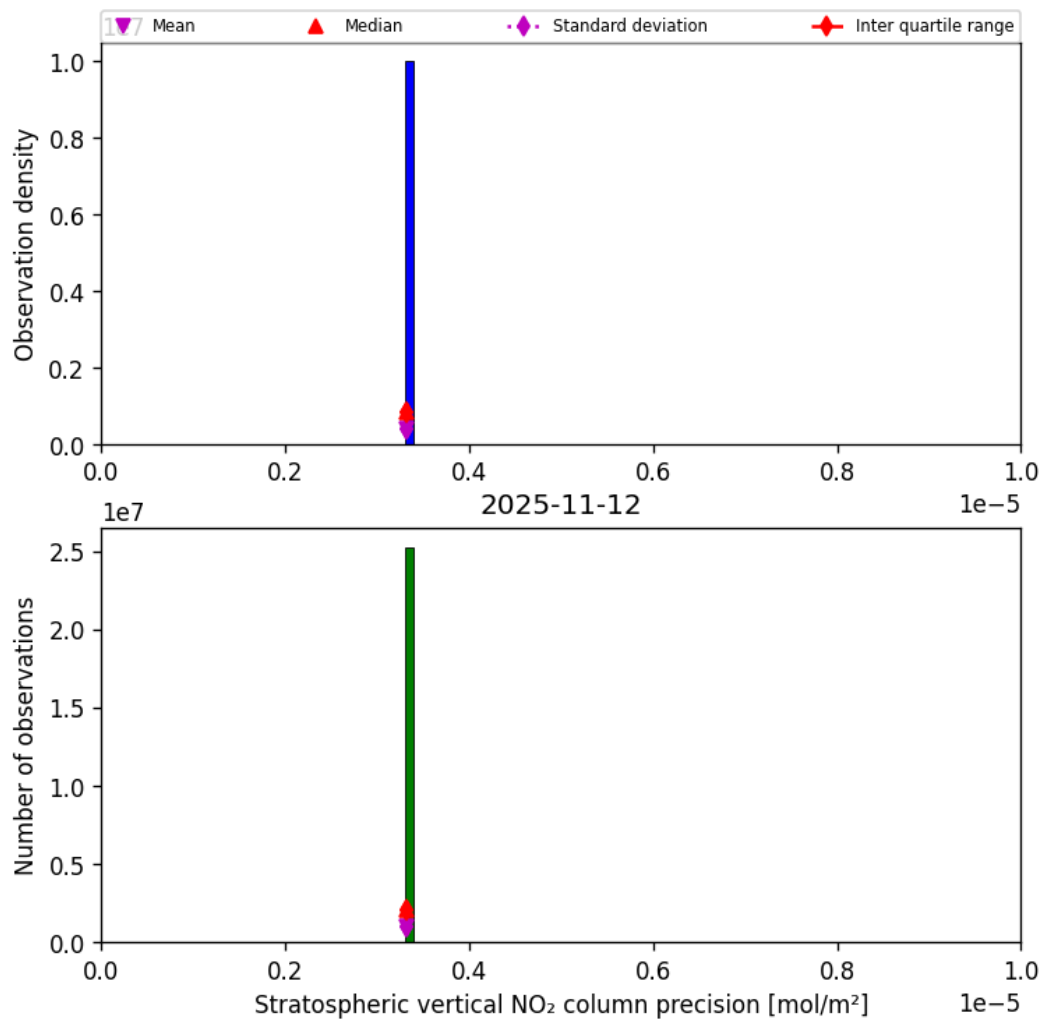
Figure 37: Histogram of “Stratospheric vertical NO 2 column precision” for 2025-11-12 to 2025-11-13
