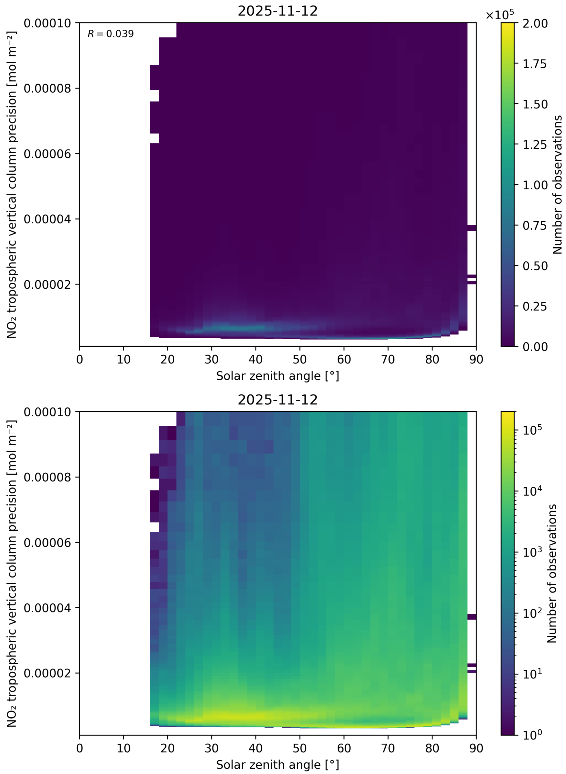
Figure 156: Scatter density plot of “Solar zenith angle” against “NO 2 tropospheric vertical column precision” for 2025-11-12 to 2025-11-13.
