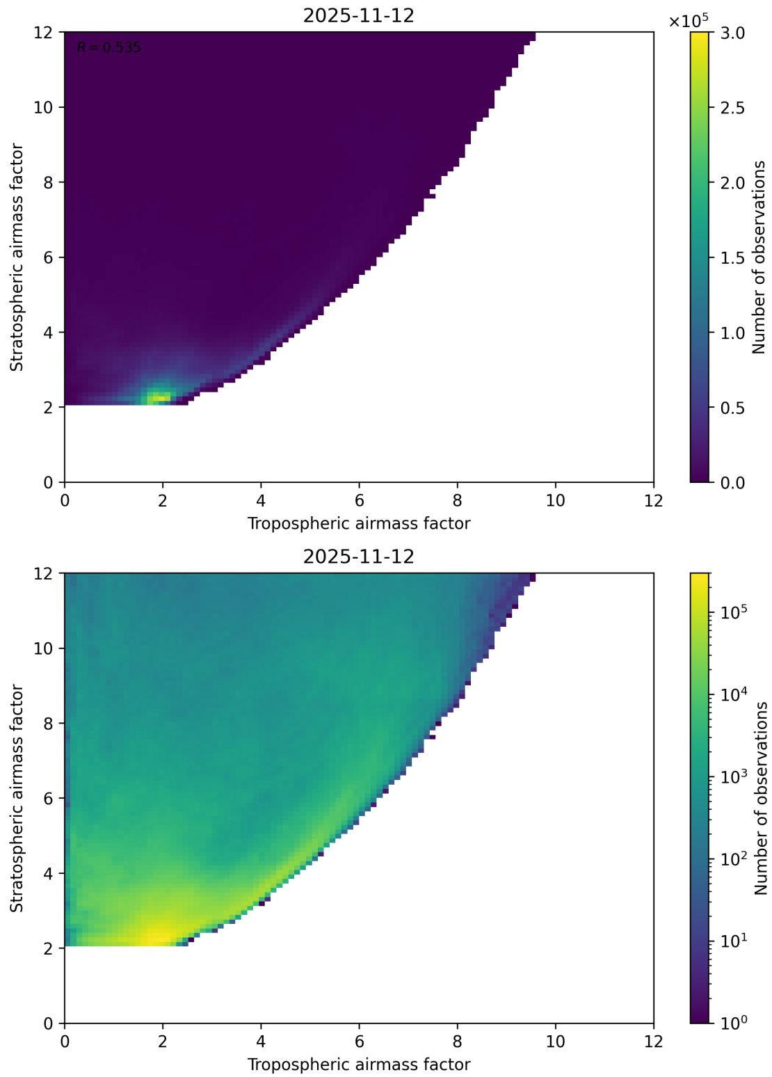
Figure 71: Scatter density plot of “Tropospheric airmass factor” against “Stratospheric airmass factor” for 2025-11-12 to 2025-11-13.
