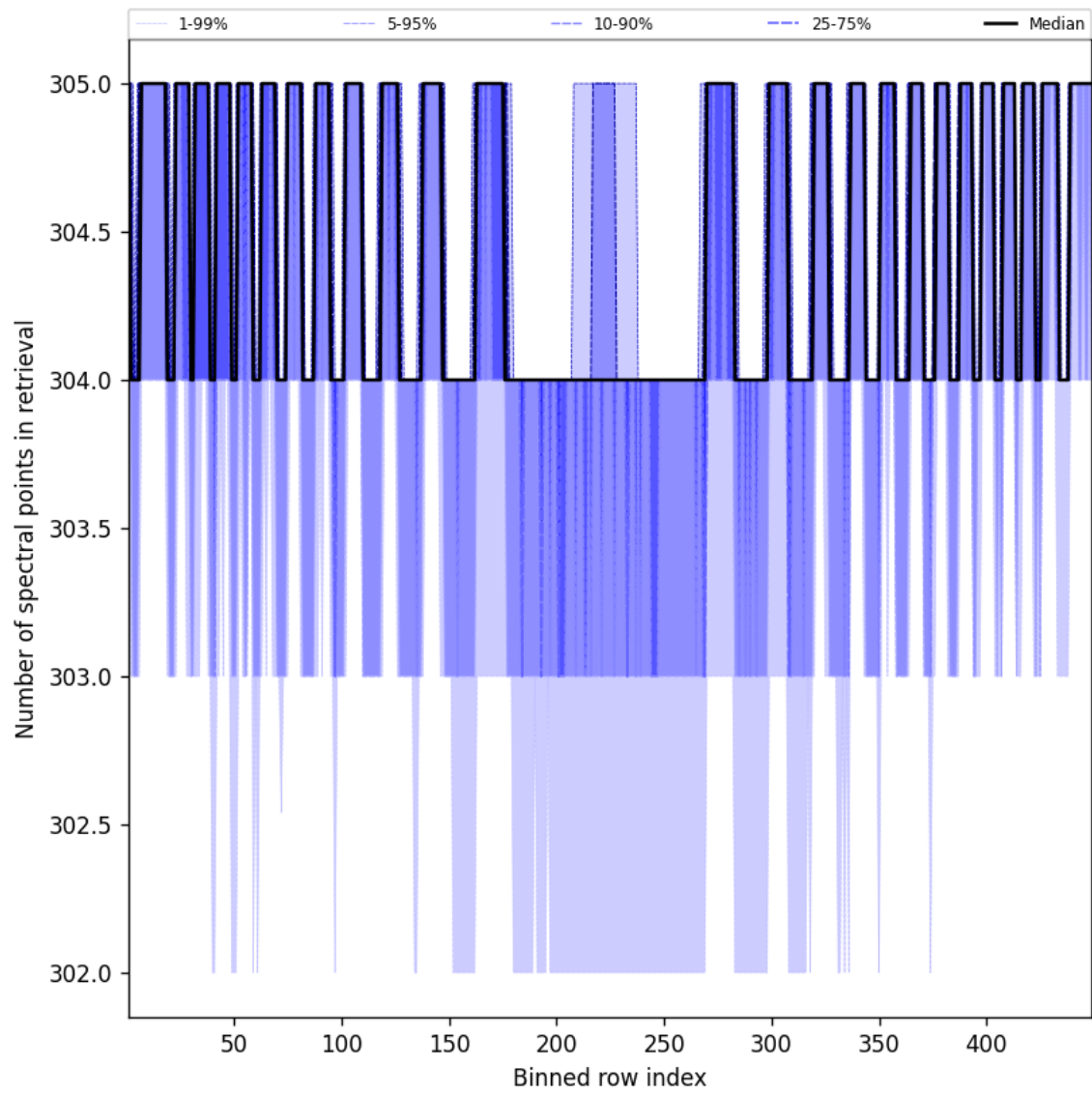
Figure 50: Along track statistics of “Number of spectral points in retrieval” for 2025-11-12 to 2025-11-13
