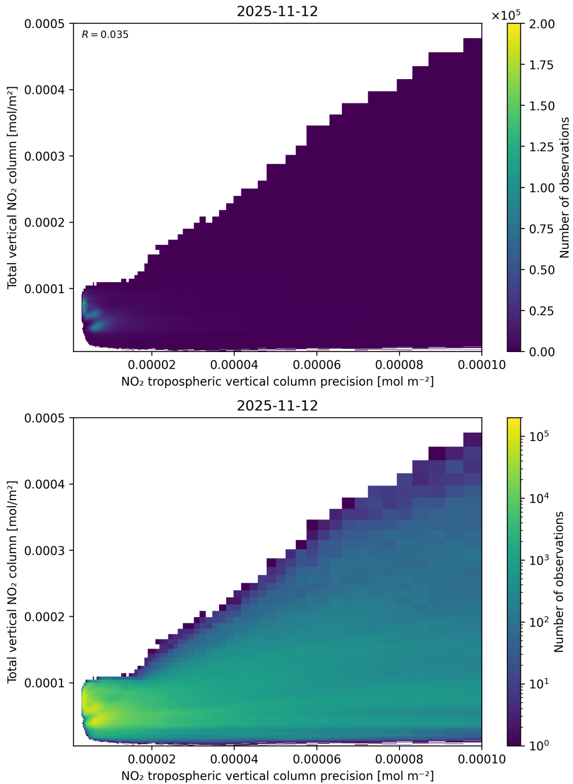
Figure 138: Scatter density plot of “NO 2 tropospheric vertical column precision” against “Total vertical NO 2 column” for 2025-11-12 to 2025-11-13.
