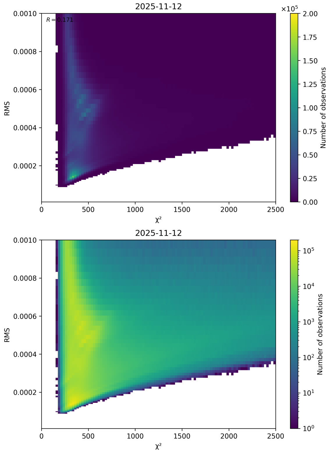
Figure 82: Scatter density plot of “ \chi^2 ” against “RMS” for 2025-11-12 to 2025-11-13.
