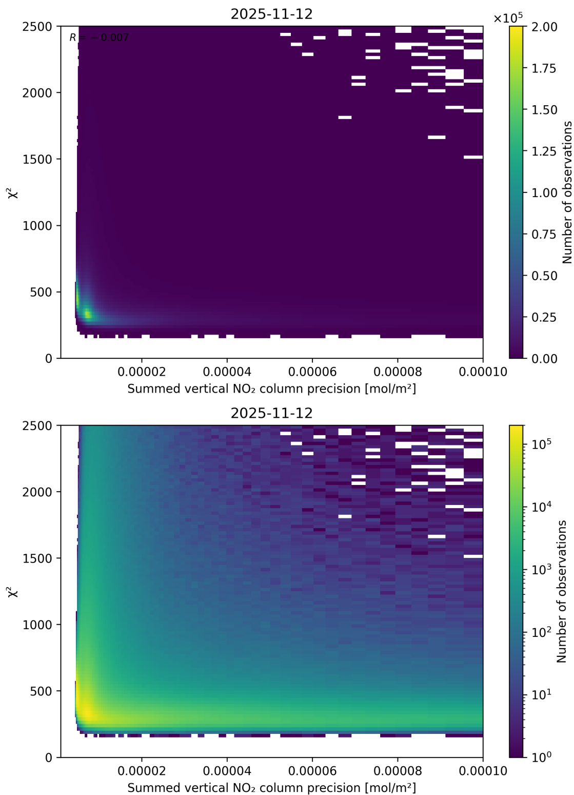
Figure 107: Scatter density plot of “Summed vertical NO 2 column precision” against “ \chi^2 ” for 2025-11-12 to 2025-11-13.
