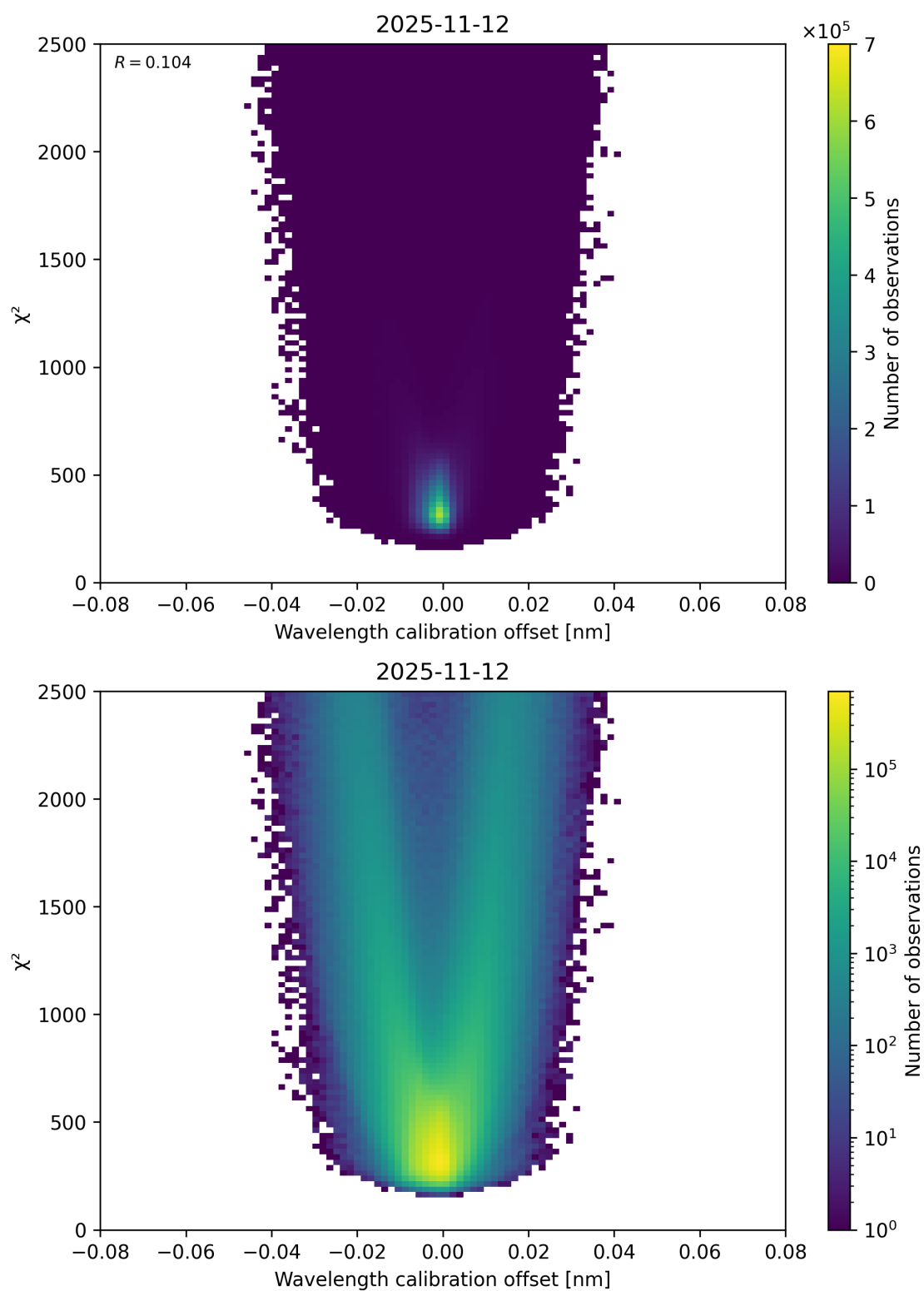
Figure 175: Scatter density plot of “Wavelength calibration offset” against “ \chi^2 ” for 2025-11-12 to 2025-11-13.
