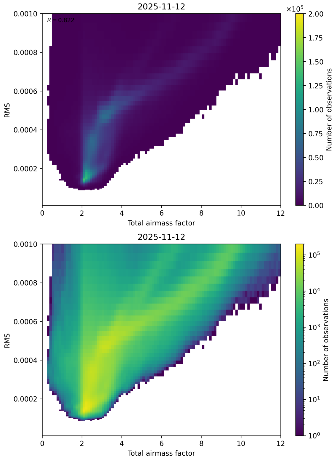
Figure 69: Scatter density plot of “Total airmass factor” against “RMS” for 2025-11-12 to 2025-11-13.
