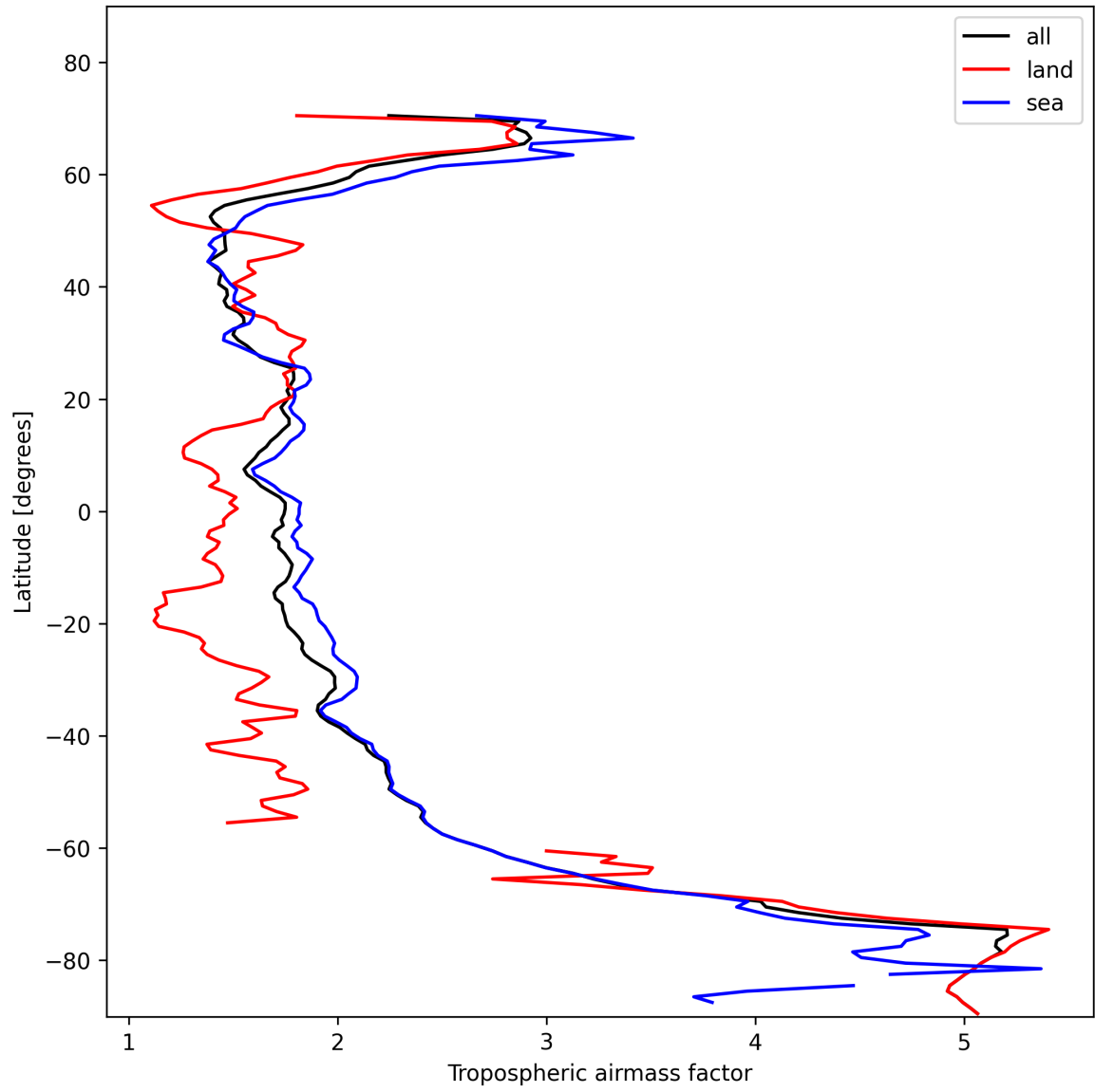
Figure 14: Zonal average of “Tropospheric airmass factor” for 2025-11-12 to 2025-11-13.
