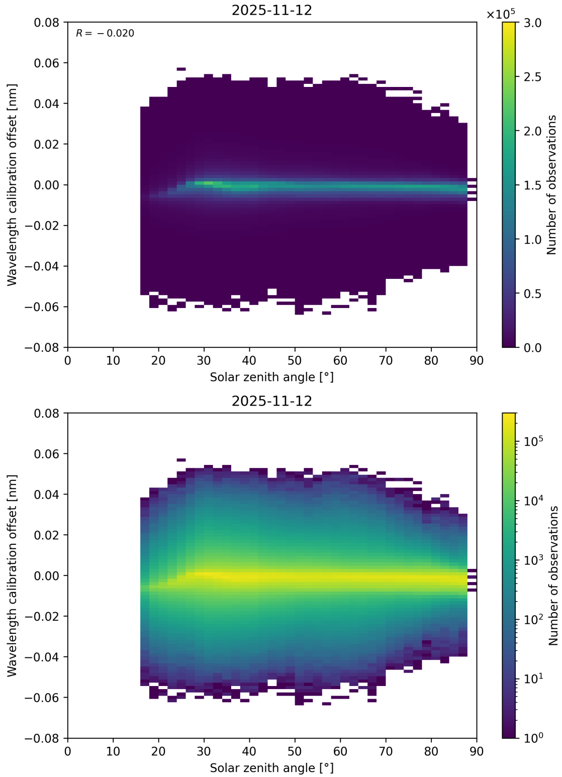
Figure 158: Scatter density plot of “Solar zenith angle” against “Wavelength calibration offset” for 2025-11-12 to 2025-11-13.
