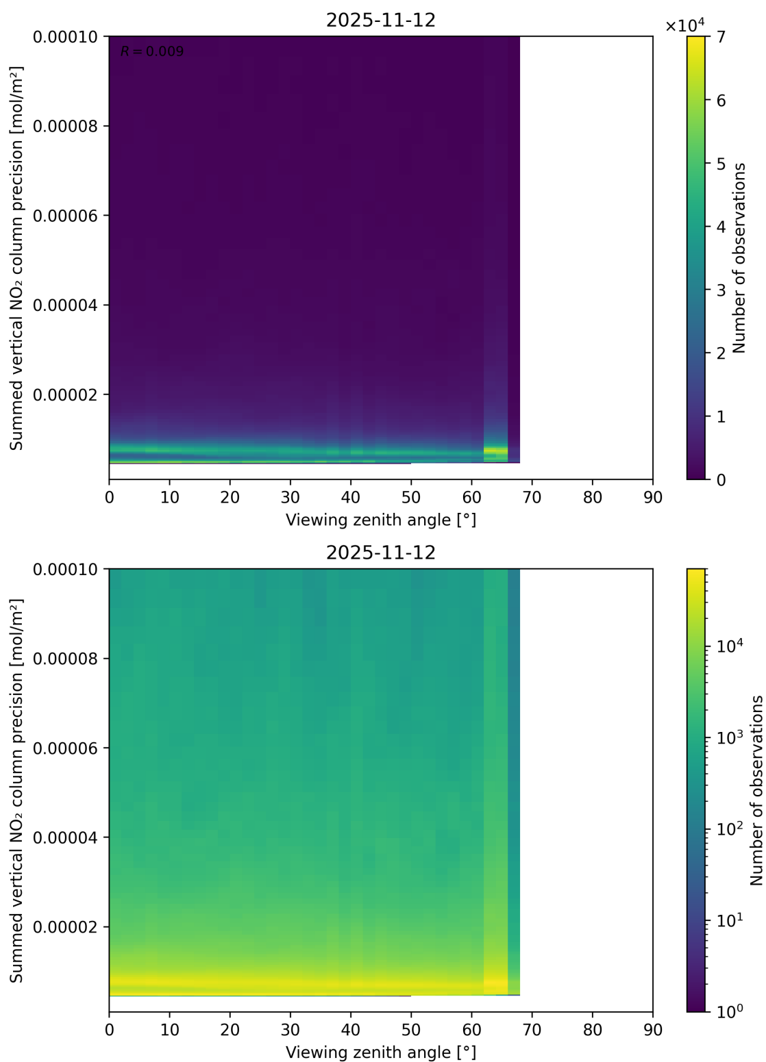
Figure 166: Scatter density plot of “Viewing zenith angle” against “Summed vertical NO 2 column precision” for 2025-11-12 to 2025-11-13.
