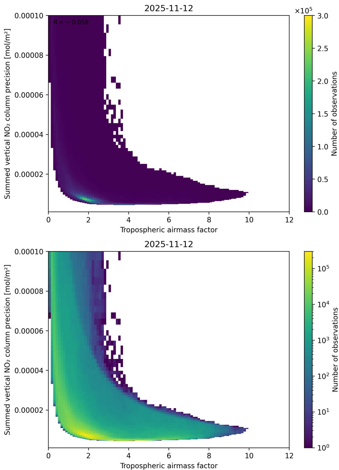
Figure 76: Scatter density plot of “Tropospheric air mass factor” against “Summed vertical NO 2 column precision” for 2025-11-12 to 2025-11-13.
