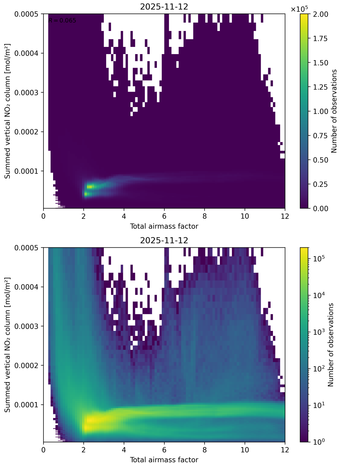
Figure 65: Scatter density plot of “Total airmass factor” against “Summed vertical NO 2 column” for 2025-11-12 to 2025-11-13.
