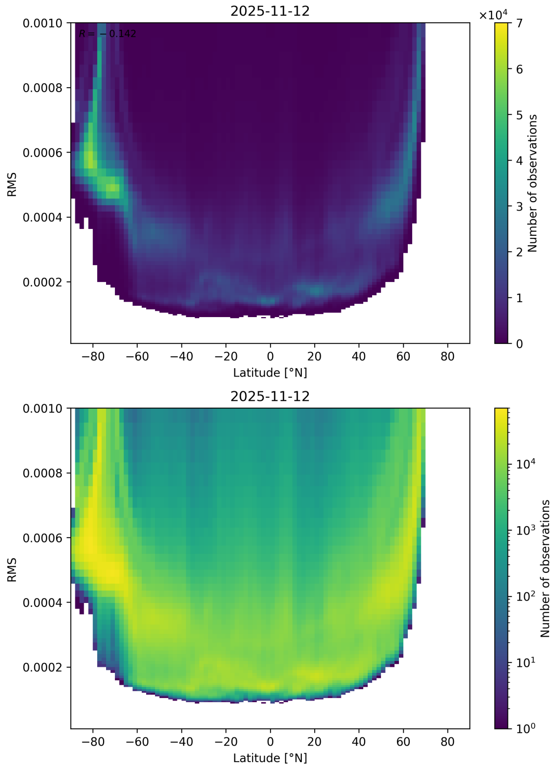
Figure 94: Scatter density plot of “Latitude” against “RMS” for 2025-11-12 to 2025-11-13.
