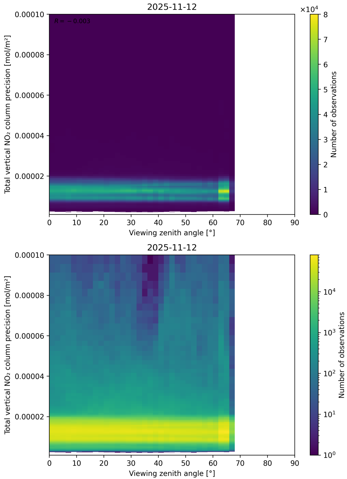
Figure 168: Scatter density plot of “Viewing zenith angle” against “Total vertical NO 2 column precision” for 2025-11-12 to 2025-11-13.
