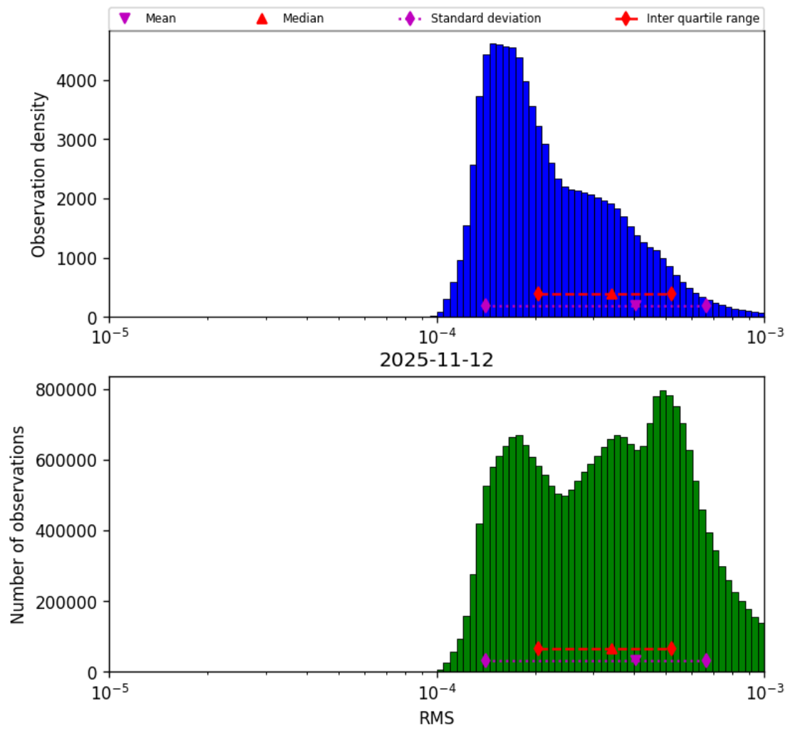
Figure 43: Histogram of “RMS” for 2025-11-12 to 2025-11-13
