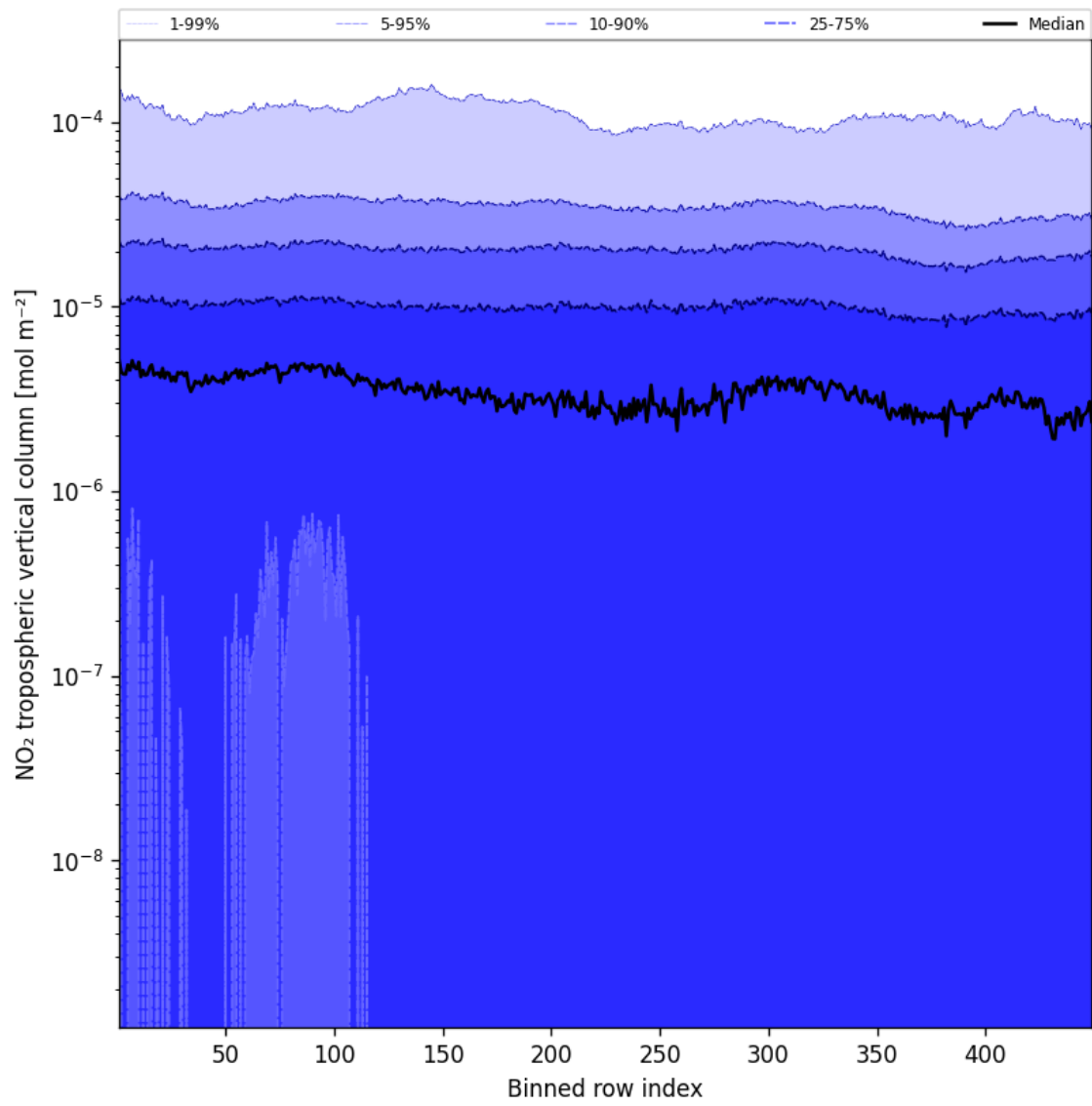
Figure 46: Along track statistics of “NO 2 tropospheric vertical column” for 2025-11-12 to 2025-11-13
