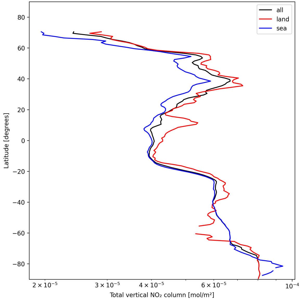
Figure 21: Zonal average of “Total vertical NO 2 column” for 2025-11-12 to 2025-11-13.
