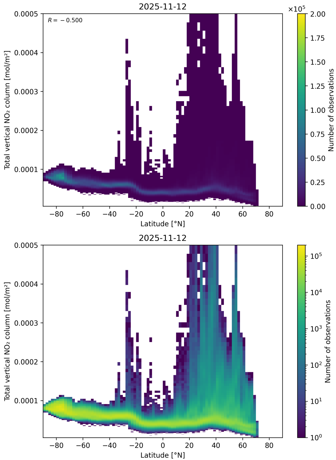
Figure 90: Scatter density plot of “Latitude” against “Total vertical NO 2 column” for 2025-11-12 to 2025-11-13.
