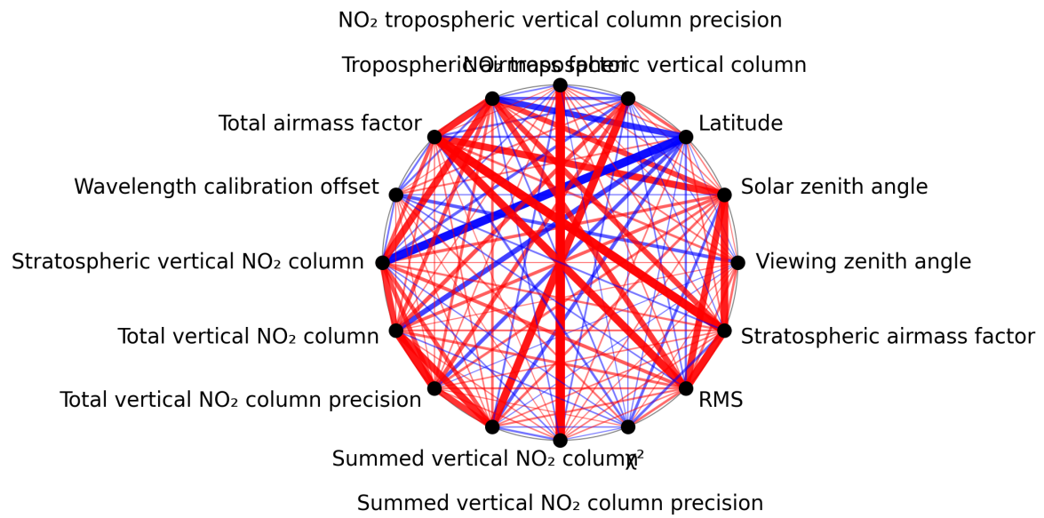
Figure 1: Map of correlation graph for 2025-11-12 to 2025-11-13.
