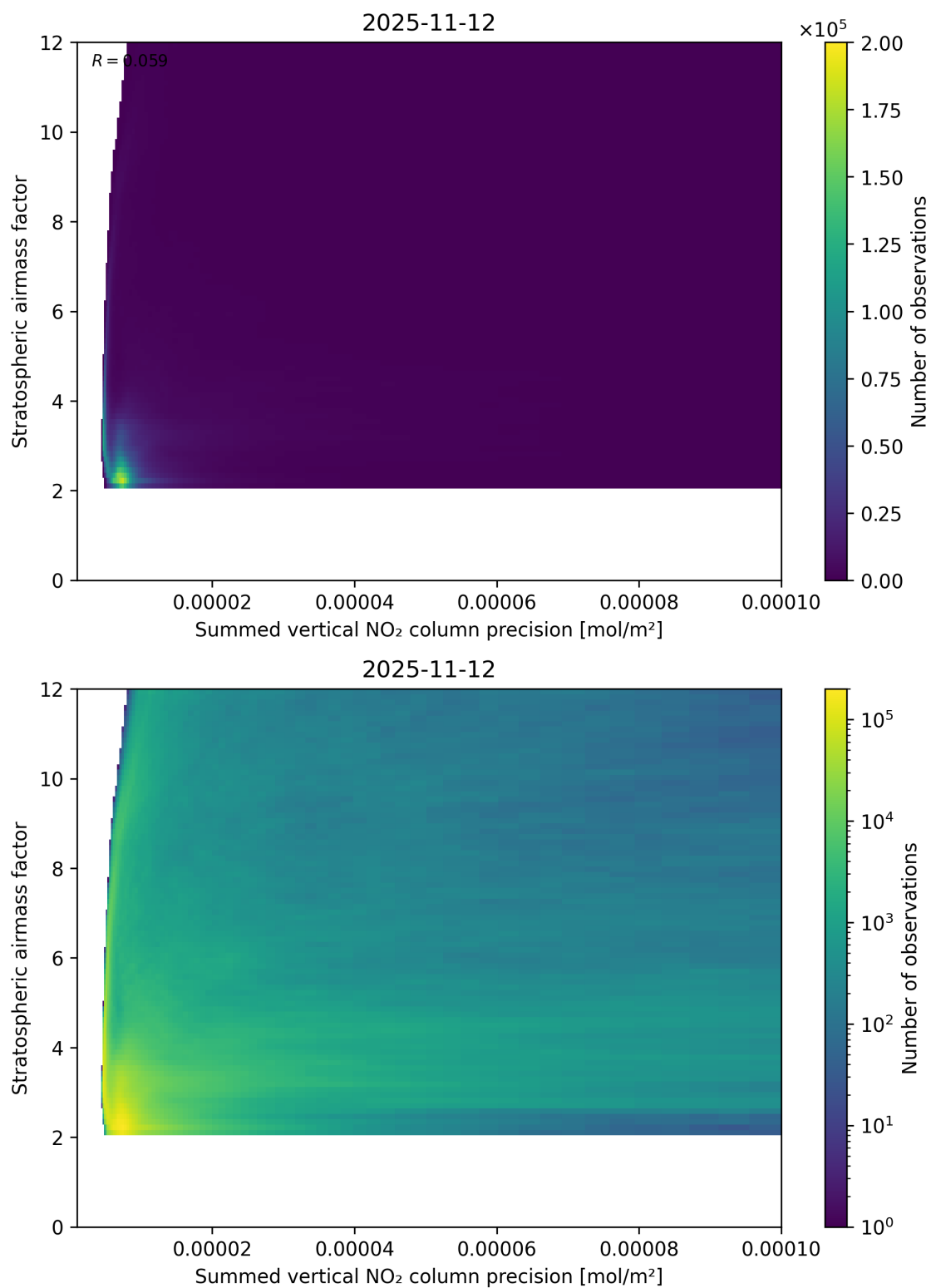
Figure 106: Scatter density plot of “Summed vertical NO 2 column precision” against “Stratospheric airmass factor” for 2025-11-12 to 2025-11-13.
