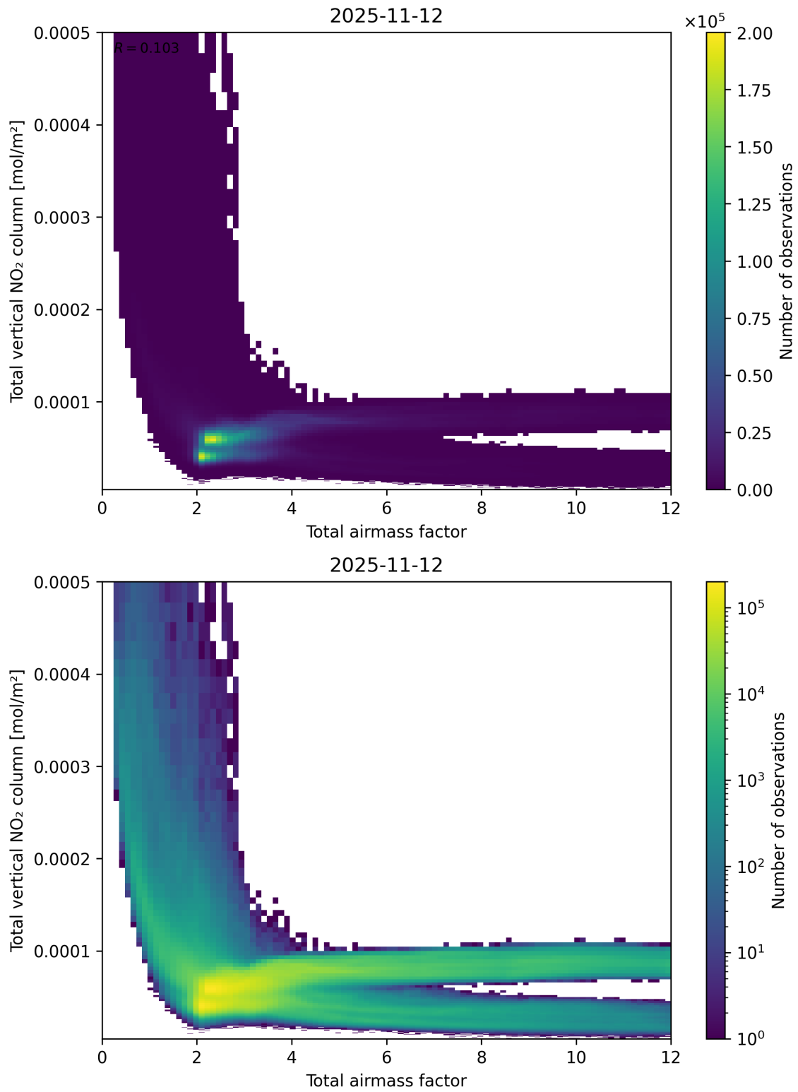
Figure 67: Scatter density plot of “Total air mass factor” against “Total vertical NO 2 column” for 2025-11-12 to 2025-11-13.
