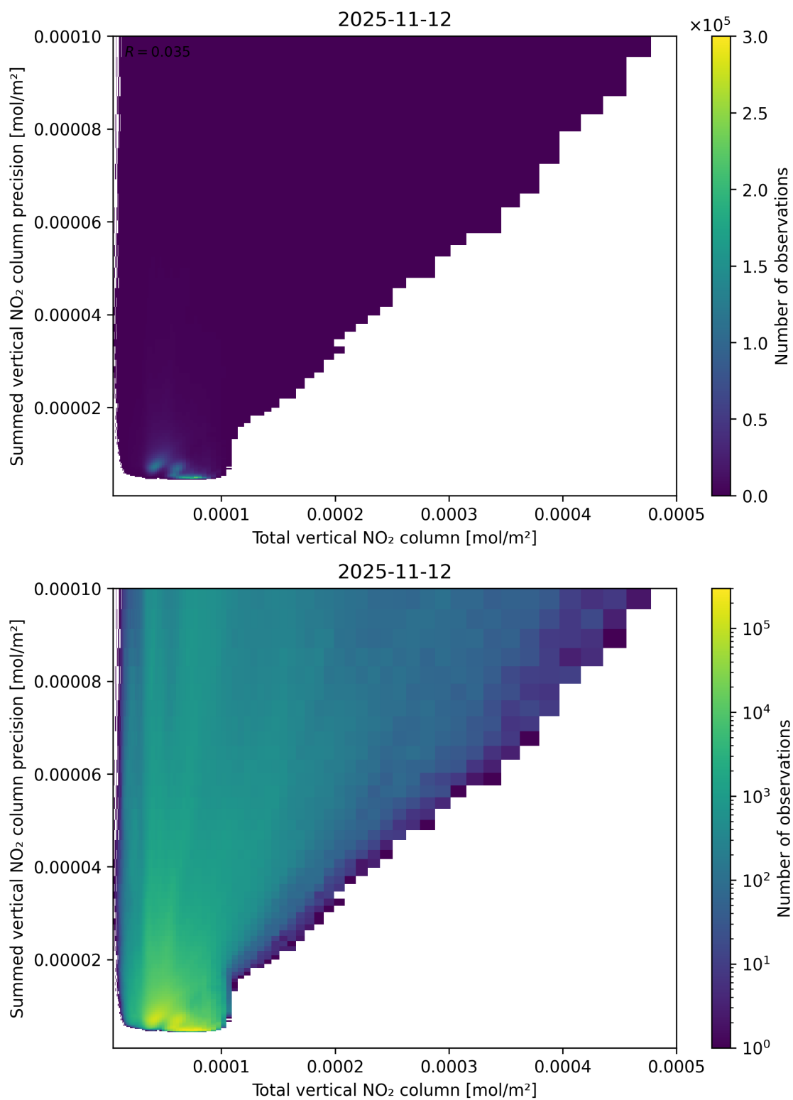
Figure 113: Scatter density plot of “Total vertical NO 2 column” against “Summed vertical NO 2 column precision” for 2025-11-12 to 2025-11-13.
