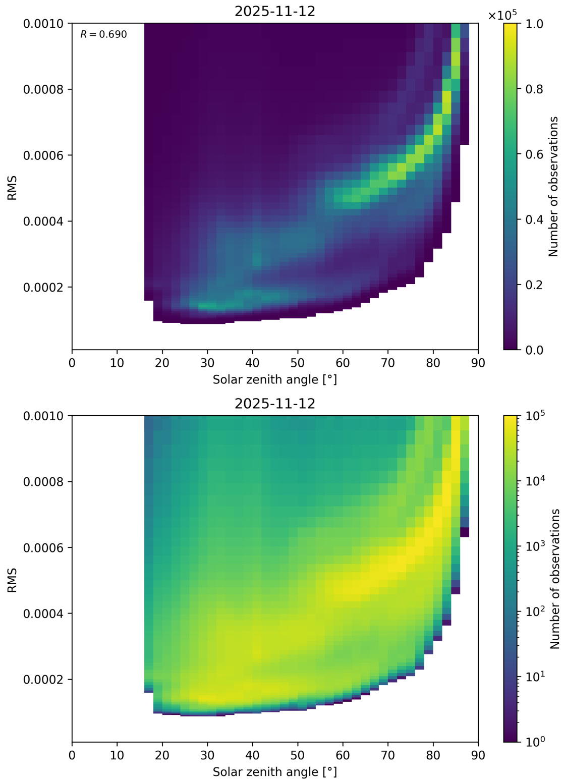
Figure 157: Scatter density plot of “Solar zenith angle” against “RMS” for 2025-11-12 to 2025-11-13.
