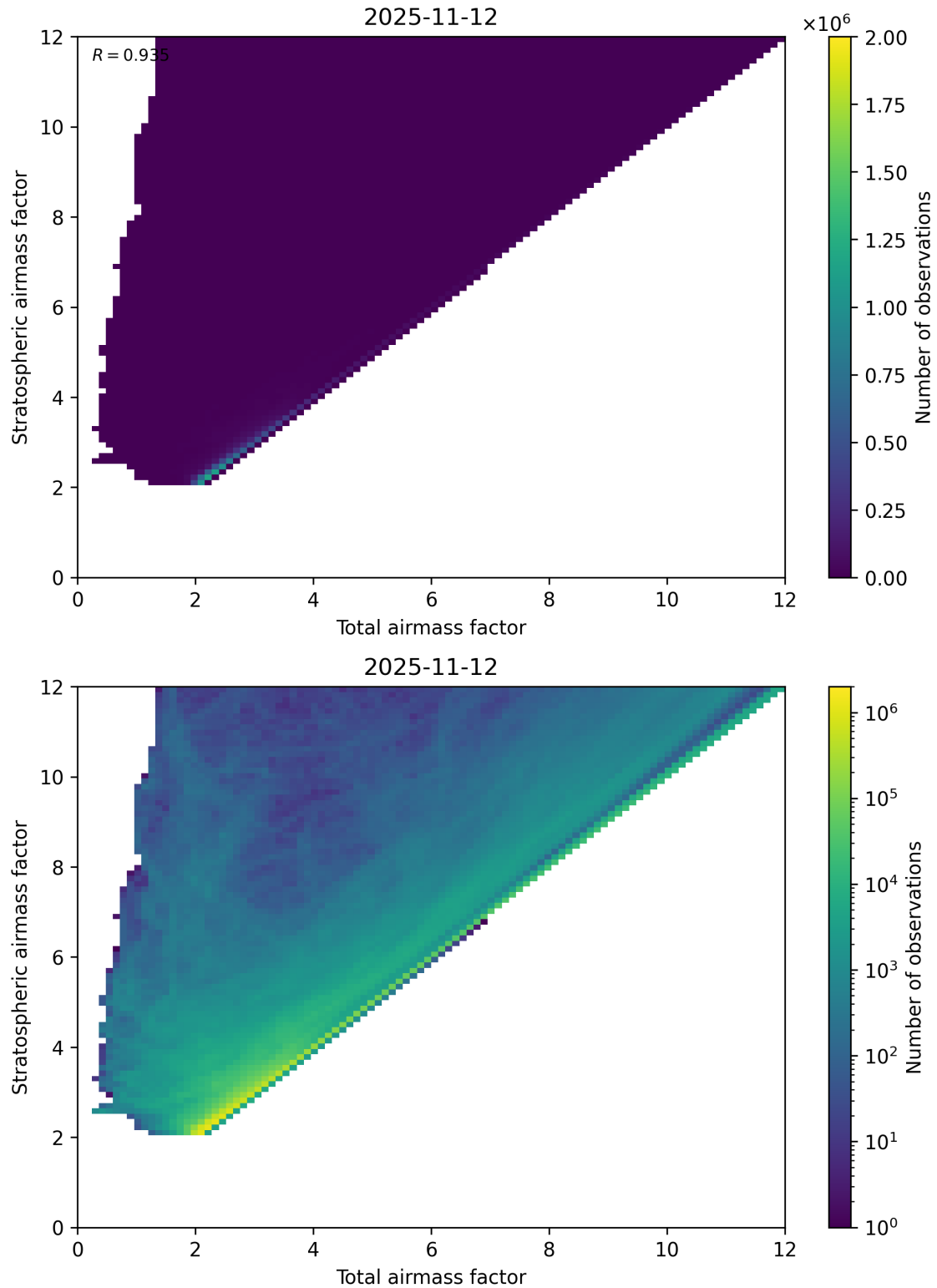
Figure 62: Scatter density plot of “Total airmass factor” against “Stratospheric airmass factor” for 2025-11-12 to 2025-11-13.
