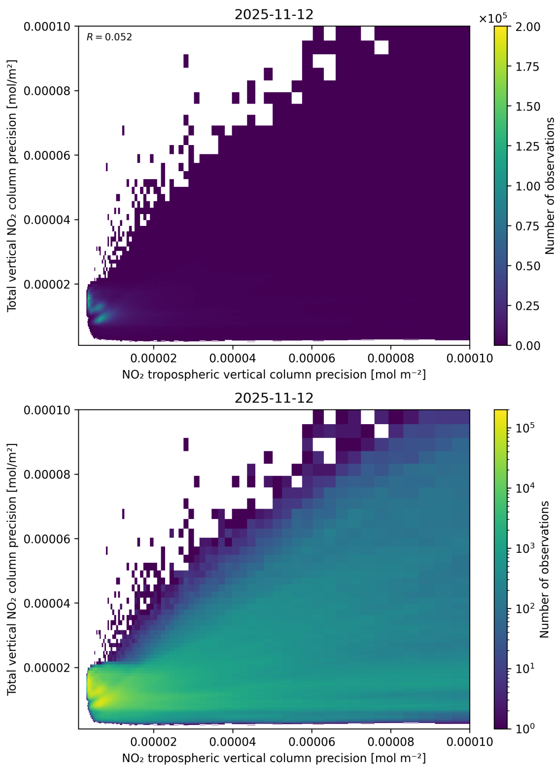
Figure 139: Scatter density plot of “NO 2 tropospheric vertical column precision” against “Total vertical NO 2 column precision” for 2025-11-12 to 2025-11-13.
