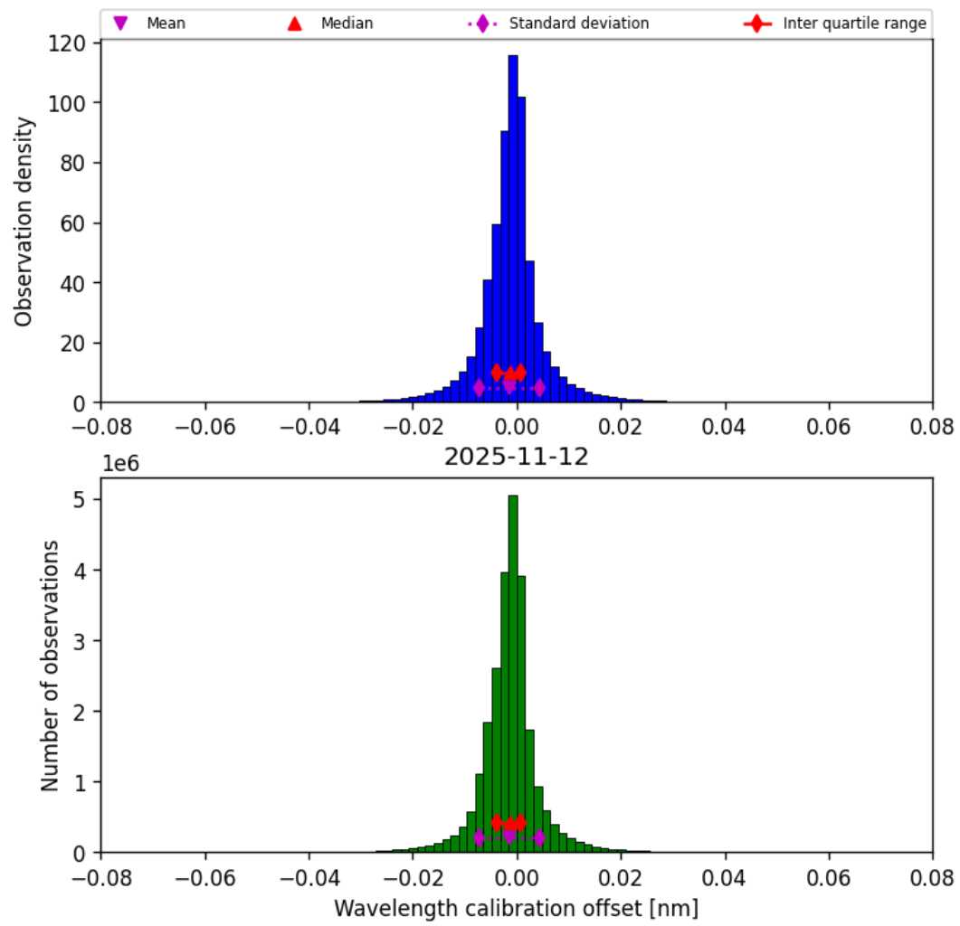
Figure 35: Histogram of “Wavelength calibration offset” for 2025-11-12 to 2025-11-13
