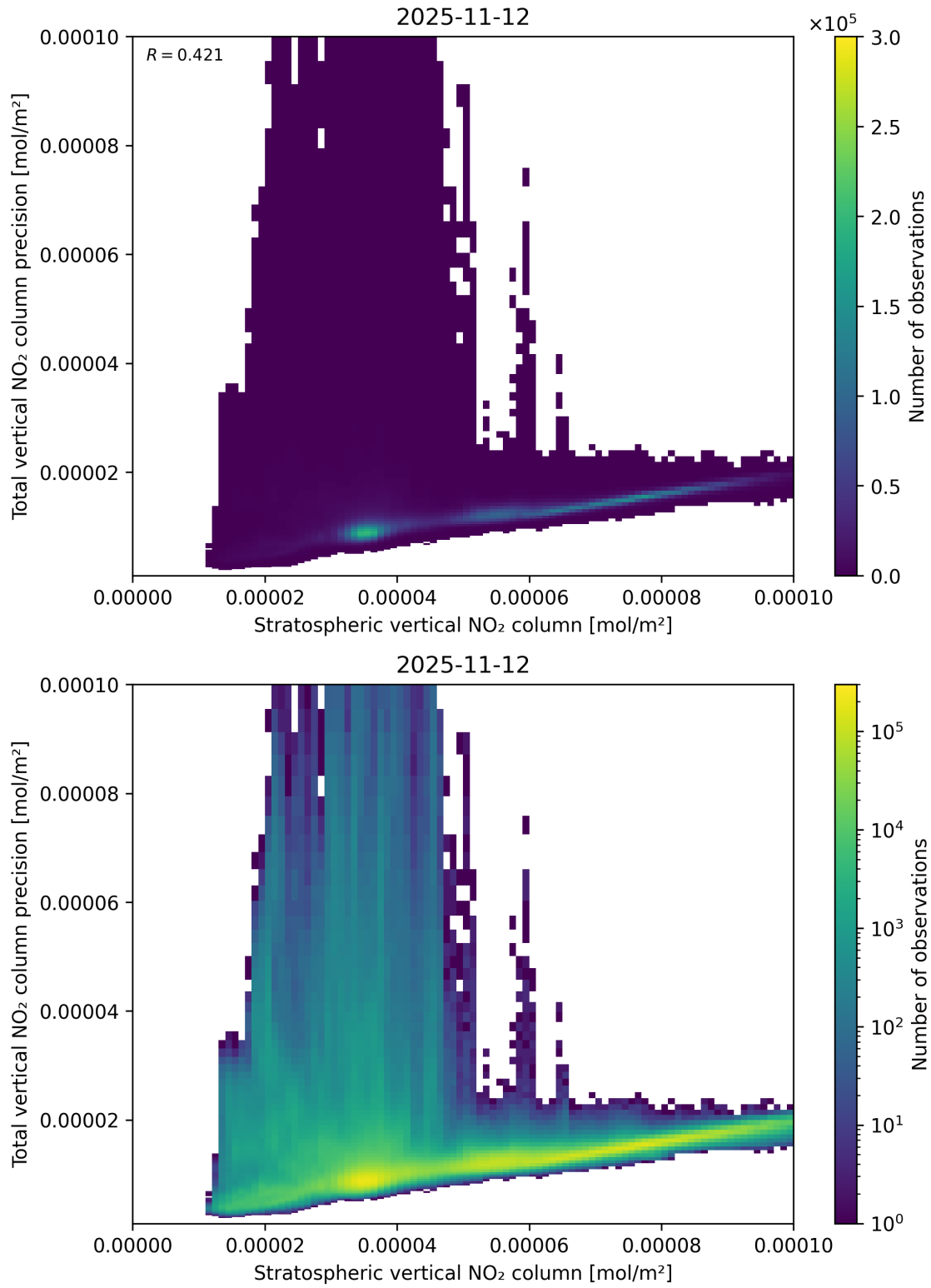
Figure 101: Scatter density plot of “Stratospheric vertical NO 2 column” against “Total vertical NO 2 column precision” for 2025-11-12 to 2025-11-13.
