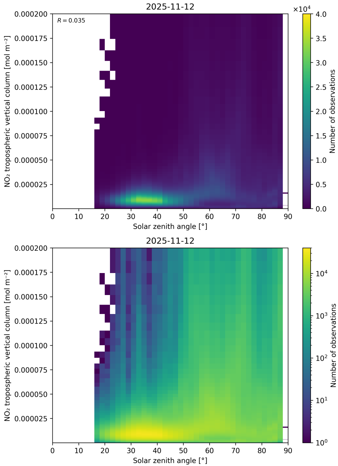
Figure 155: Scatter density plot of “Solar zenith angle” against “NO 2 tropospheric vertical column” for 2025-11-12 to 2025-11-13.
