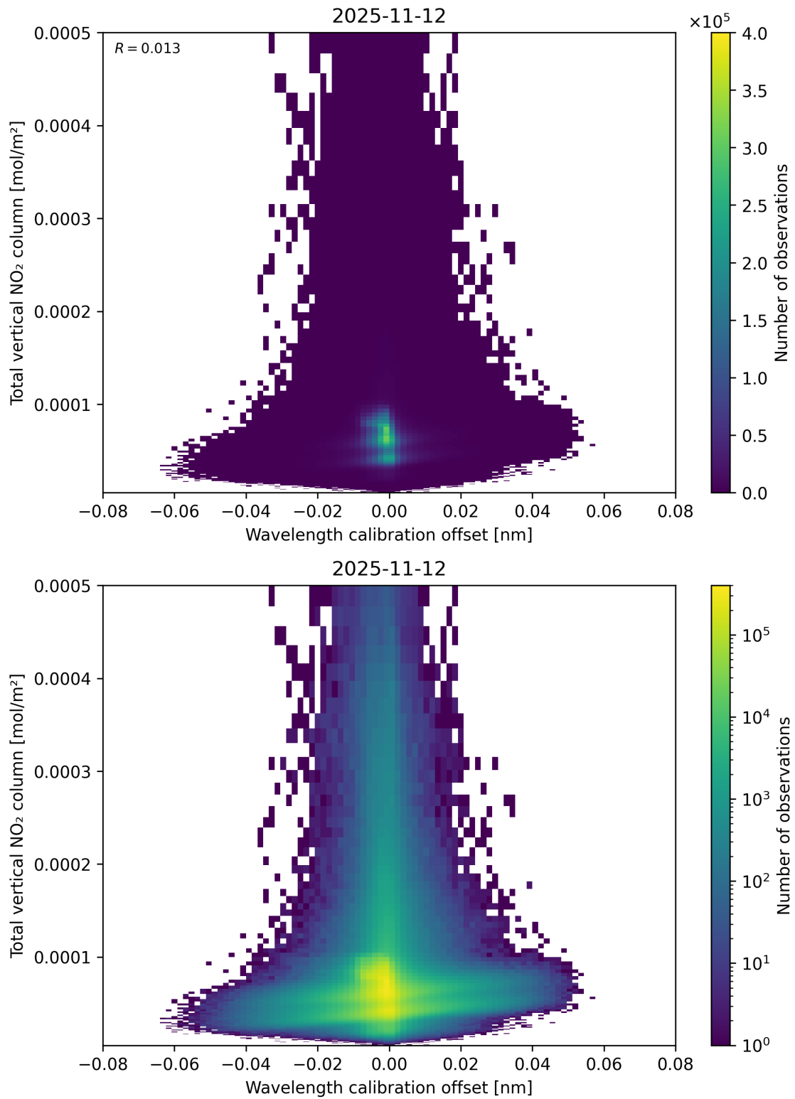
Figure 179: Scatter density plot of “Wavelength calibration offset” against “Total vertical NO 2 column” for 2025-11-12 to 2025-11-13.
