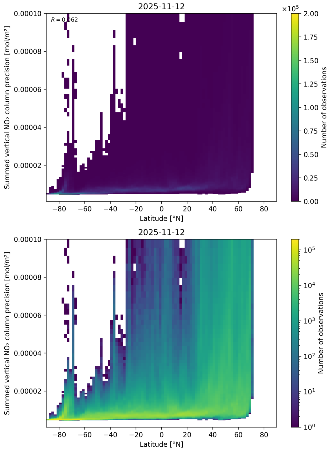
Figure 89: Scatter density plot of “Latitude” against “Summed vertical NO 2 column precision” for 2025-11-12 to 2025-11-13.
