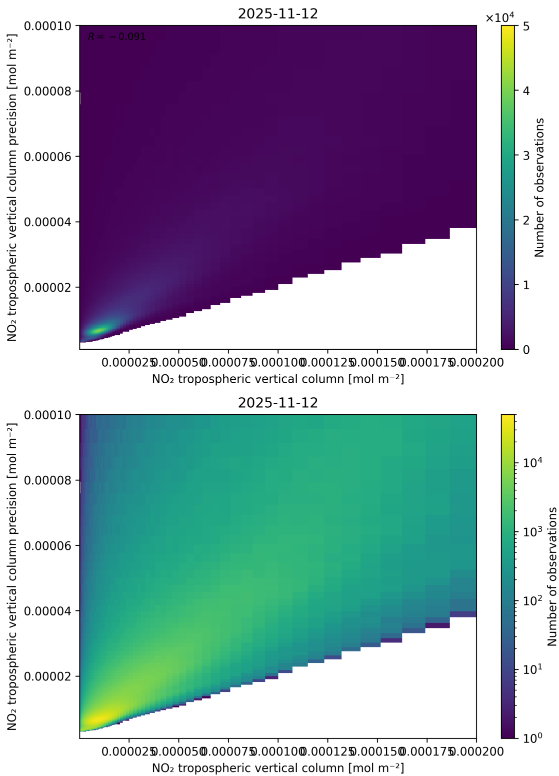
Figure 130: Scatter density plot of “NO 2 tropospheric vertical column” against “NO 2 tropospheric vertical column precision” for 2025-11-12 to 2025-11-13.
