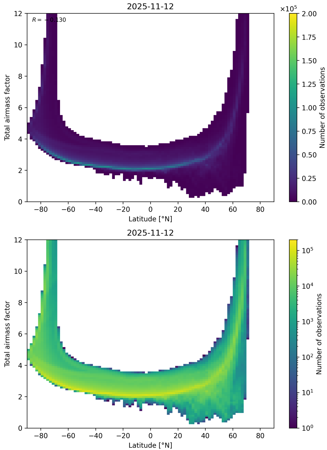
Figure 84: Scatter density plot of “Latitude” against “Total airmass factor” for 2025-11-12 to 2025-11-13.
