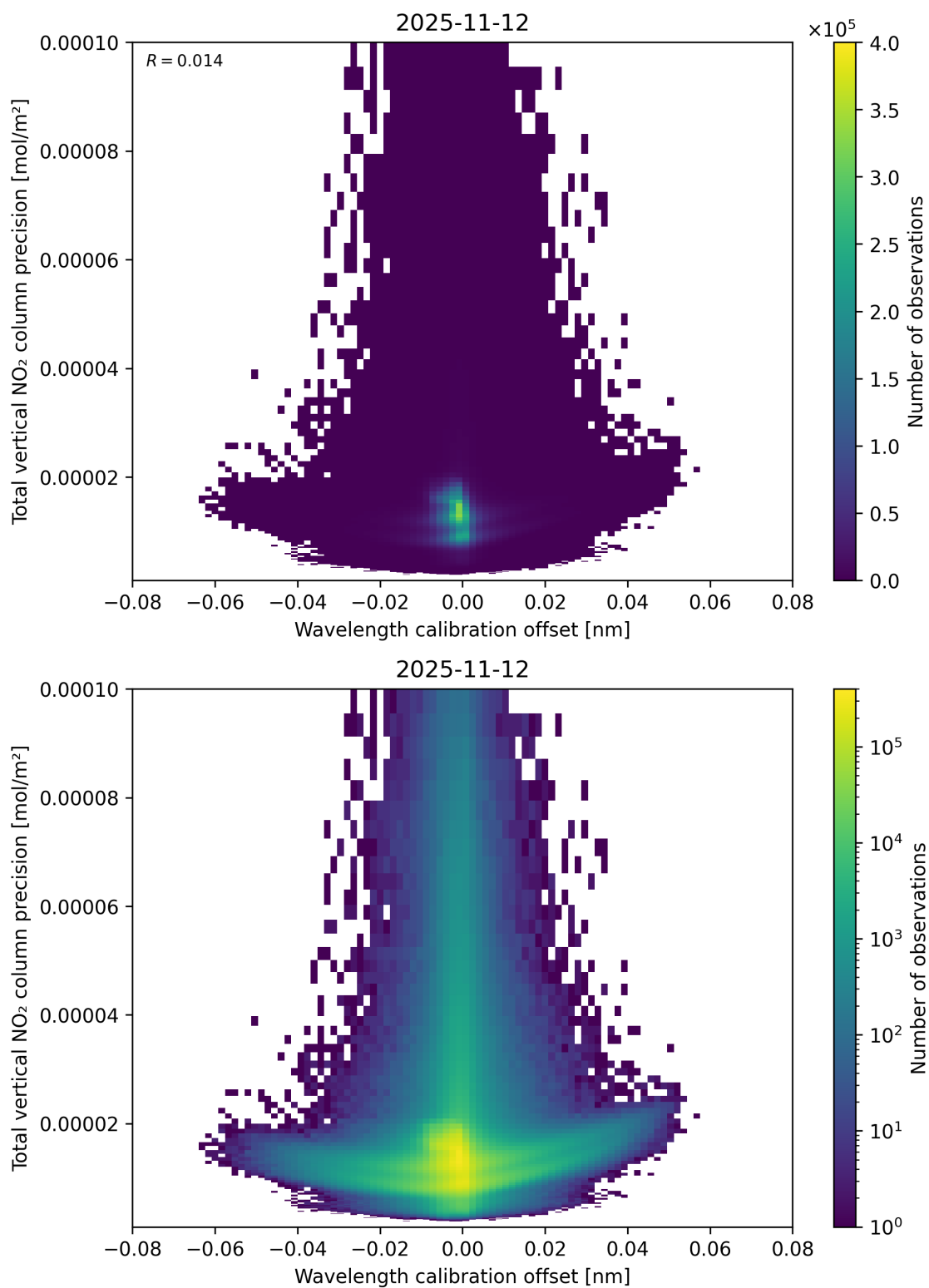
Figure 180: Scatter density plot of “Wavelength calibration offset” against “Total vertical NO 2 column precision” for 2025-11-12 to 2025-11-13.
