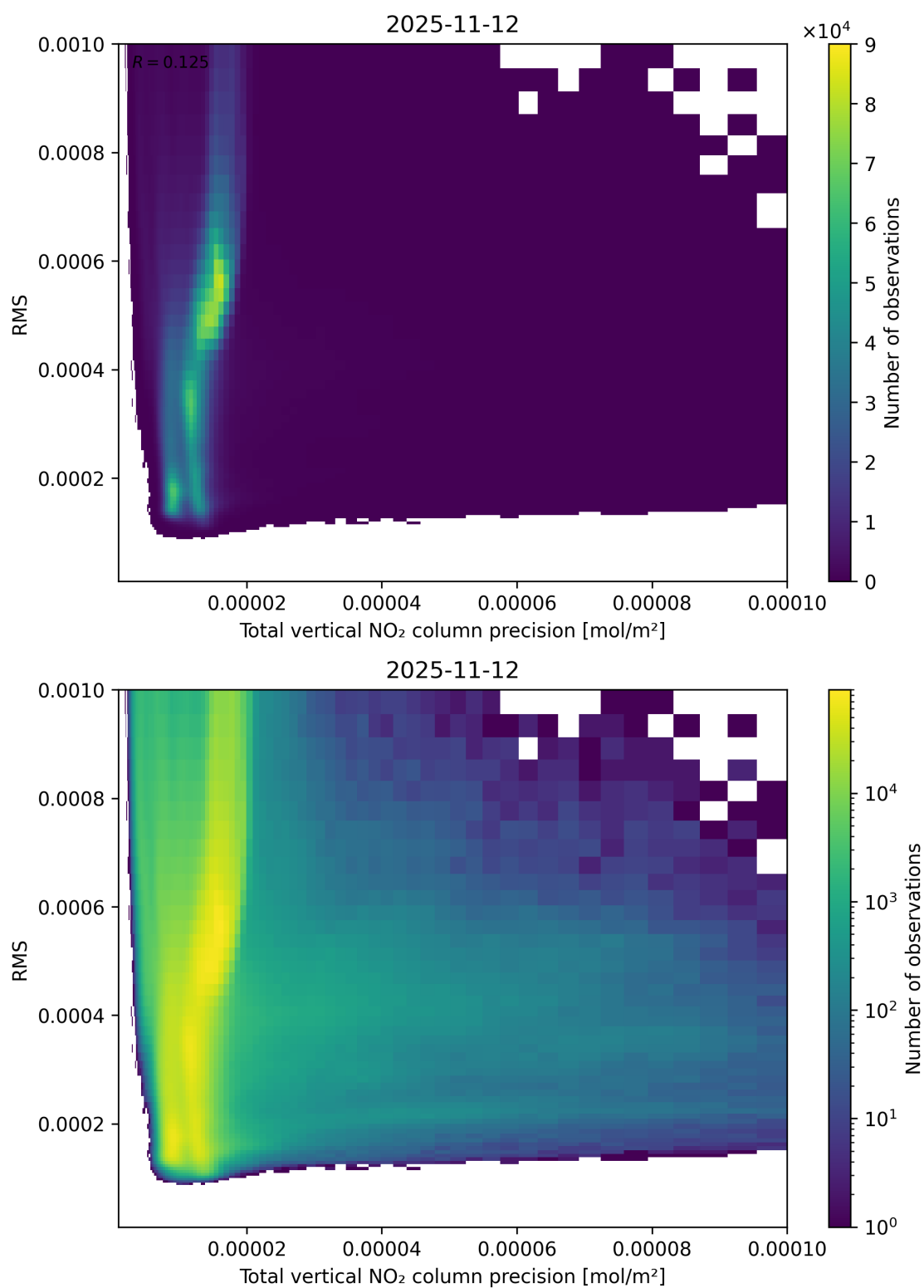
Figure 119: Scatter density plot of “Total vertical NO 2 column precision” against “RMS” for 2025-11-12 to 2025-11-13.
