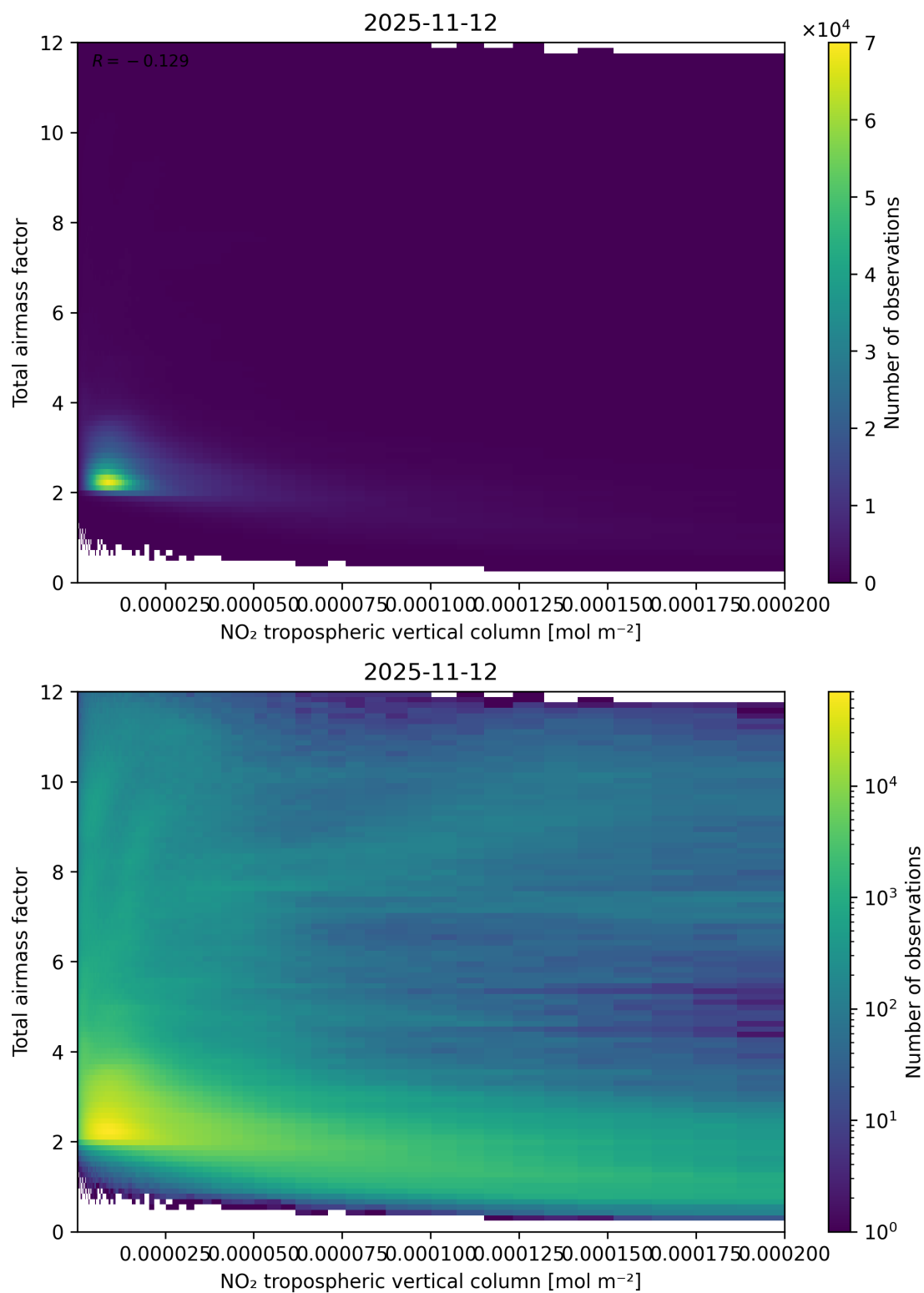
Figure 122: Scatter density plot of “NO 2 tropospheric vertical column” against “Total air mass factor” for 2025-11-12 to 2025-11-13.
