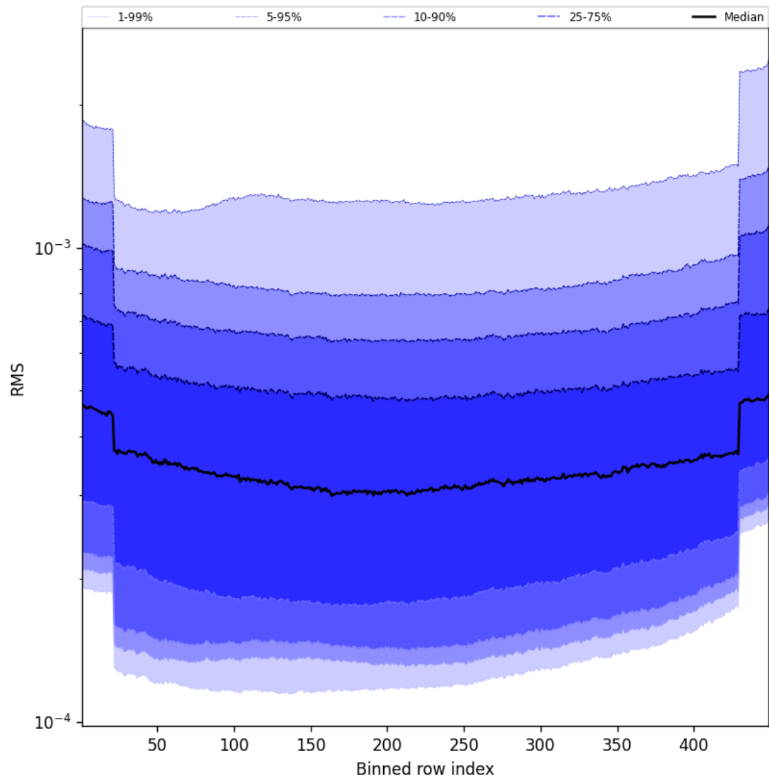
Figure 60: Along track statistics of “RMS” for 2025-11-12 to 2025-11-13
