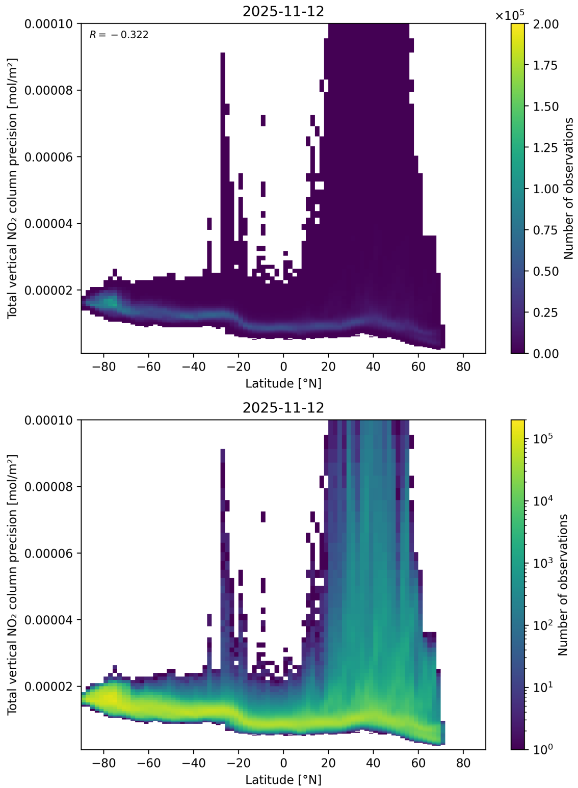
Figure 91: Scatter density plot of “Latitude” against “Total vertical NO 2 column precision” for 2025-11-12 to 2025-11-13.
