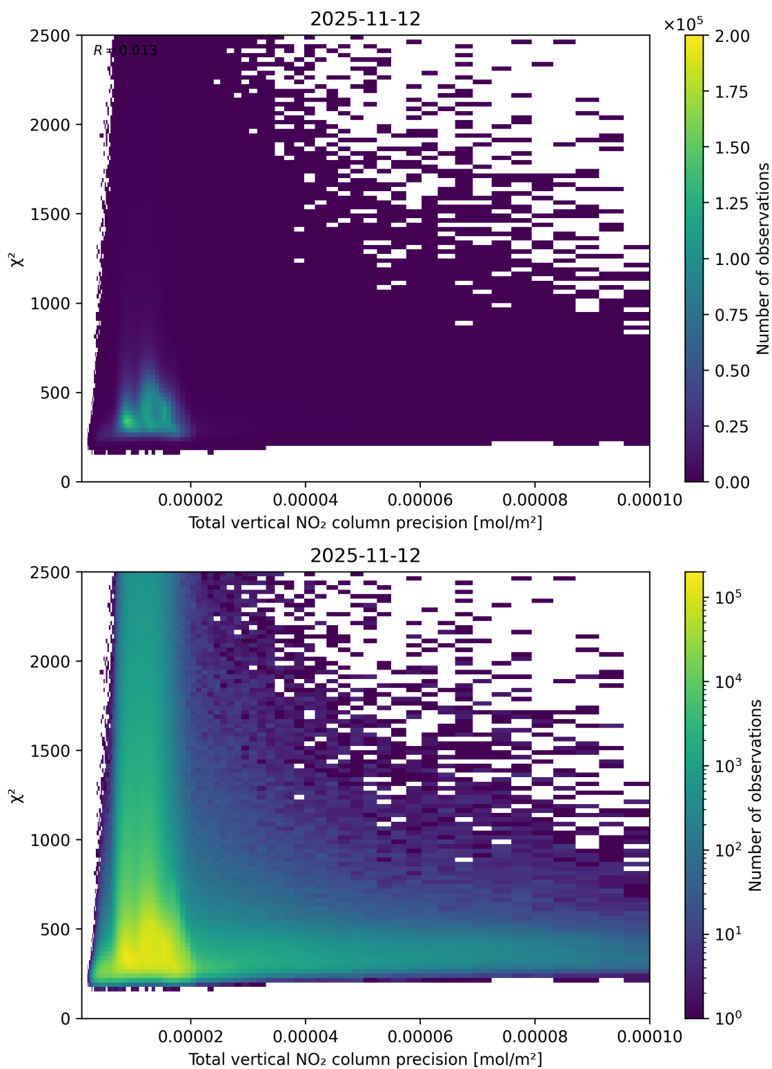
Figure 116: Scatter density plot of “Total vertical NO 2 column precision” against “ \chi^2 ” for 2025-11-12 to 2025-11-13.
