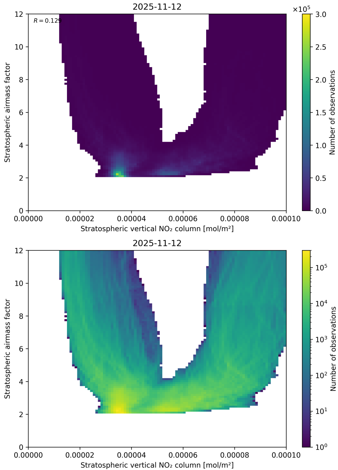
Figure 96: Scatter density plot of “Stratospheric vertical NO 2 column” against “Stratospheric airmass factor” for 2025-11-12 to 2025-11-13.
