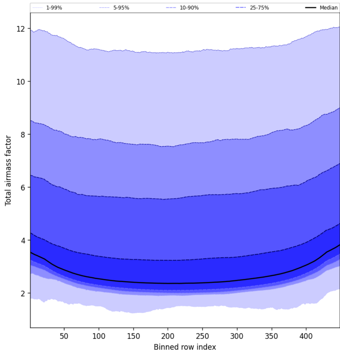
Figure 49: Along track statistics of “Total airmass factor” for 2025-11-12 to 2025-11-13
