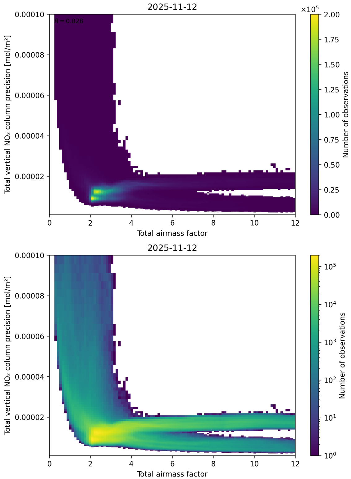
Figure 68: Scatter density plot of “Total airmass factor” against “Total vertical NO 2 column precision” for 2025-11-12 to 2025-11-13.
