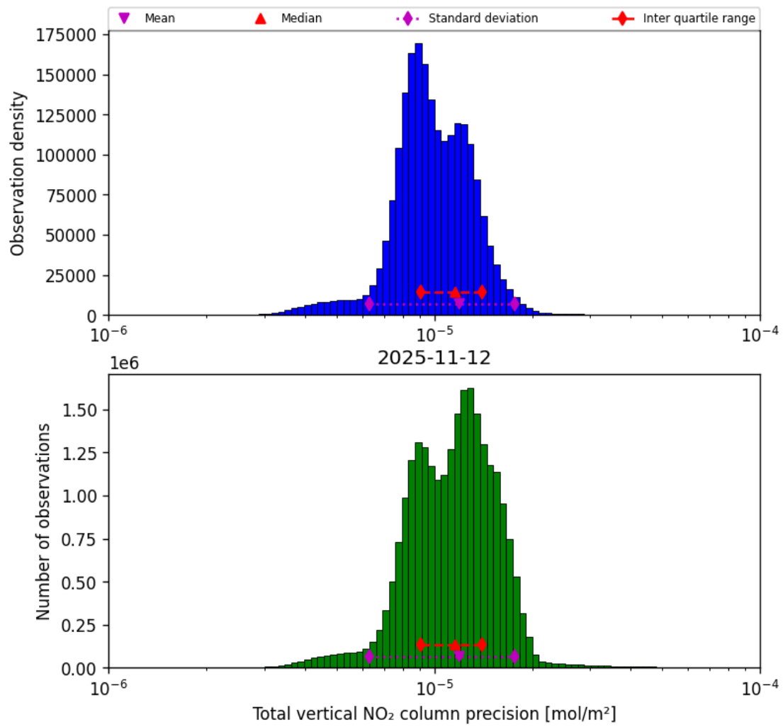
Figure 39: Histogram of “Total vertical NO 2 column precision” for 2025-11-12 to 2025-11-13
