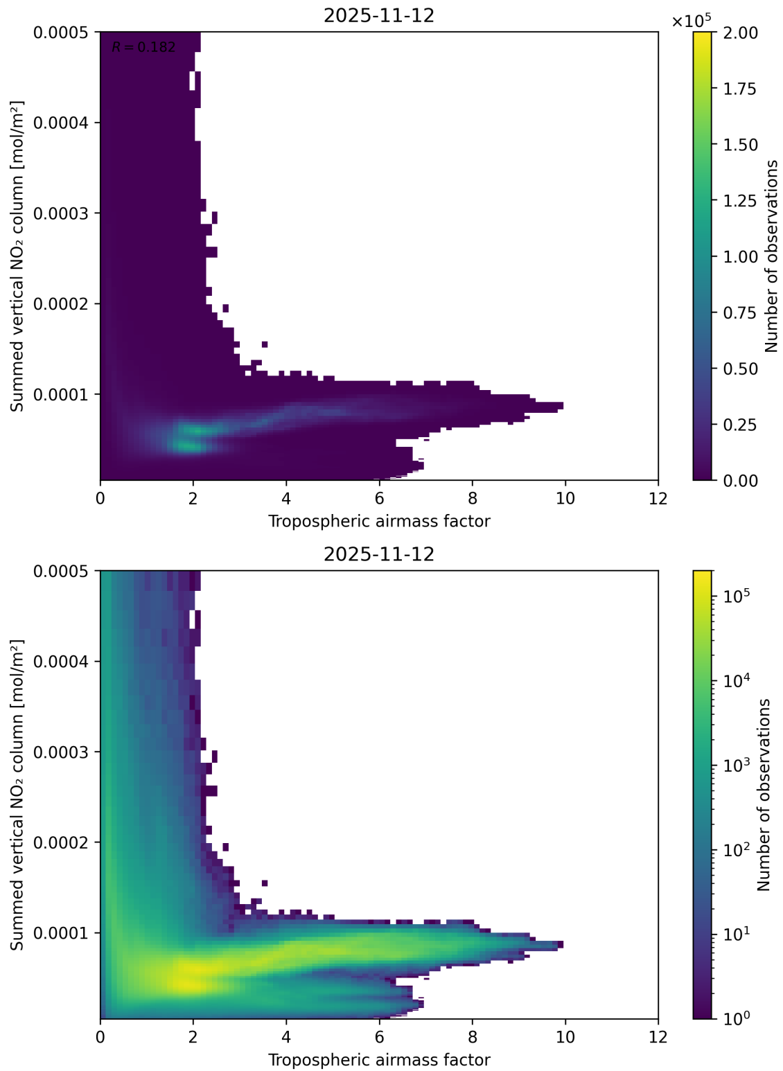
Figure 75: Scatter density plot of “Tropospheric air mass factor” against “Summed vertical NO 2 column” for 2025-11-12 to 2025-11-13.
