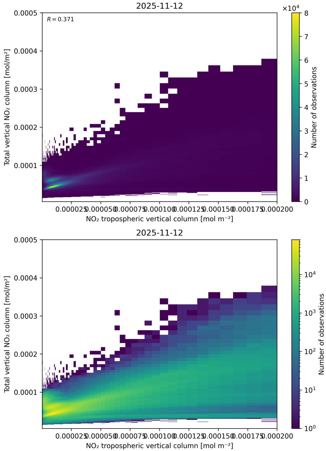
Figure 128: Scatter density plot of “NO 2 tropospheric vertical column” against “Total vertical NO 2 column” for 2025-11-12 to 2025-11-13.
