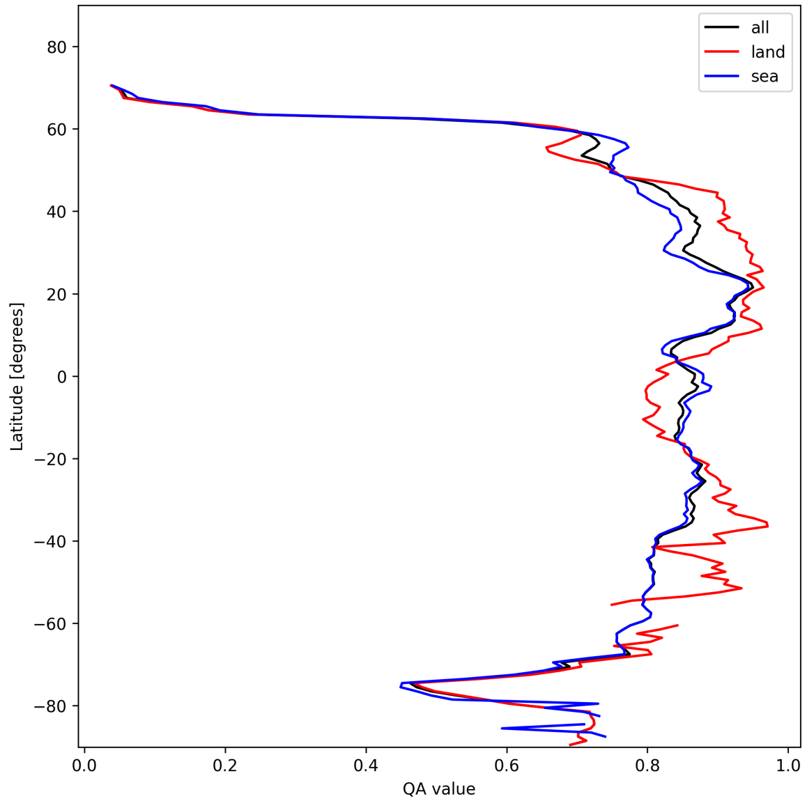
Figure 11: Zonal average of “QA value” for 2025-11-12 to 2025-11-13.
