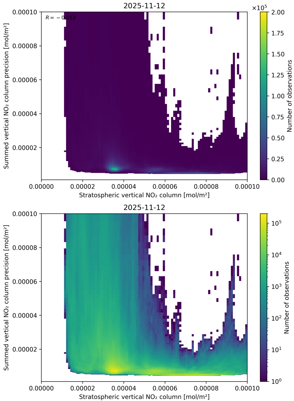
Figure 99: Scatter density plot of “Stratospheric vertical NO 2 column” against “Summed vertical NO 2 column precision” for 2025-11-12 to 2025-11-13.
