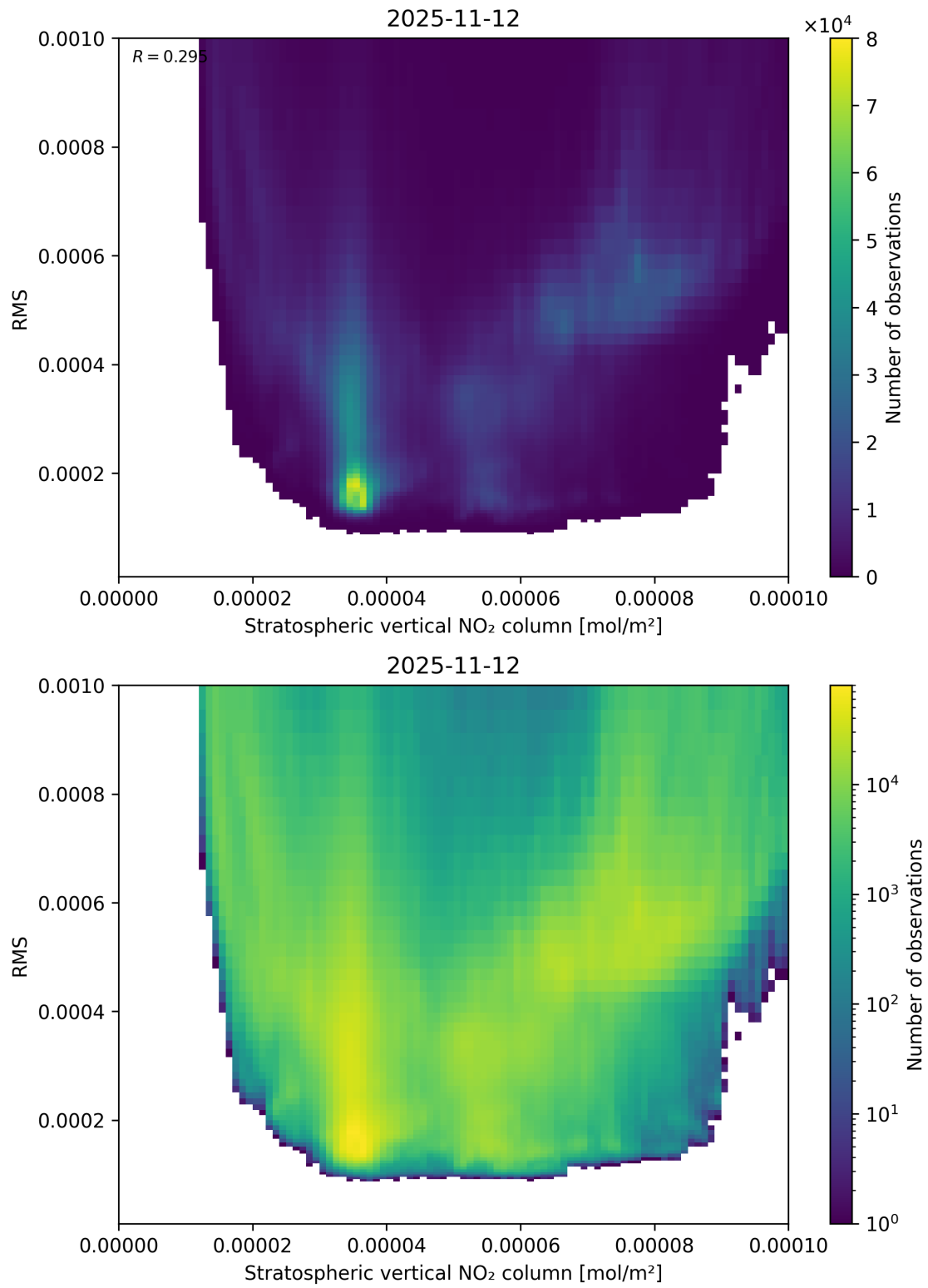
Figure 102: Scatter density plot of “Stratospheric vertical NO 2 column” against “RMS” for 2025-11-12 to 2025-11-13.
