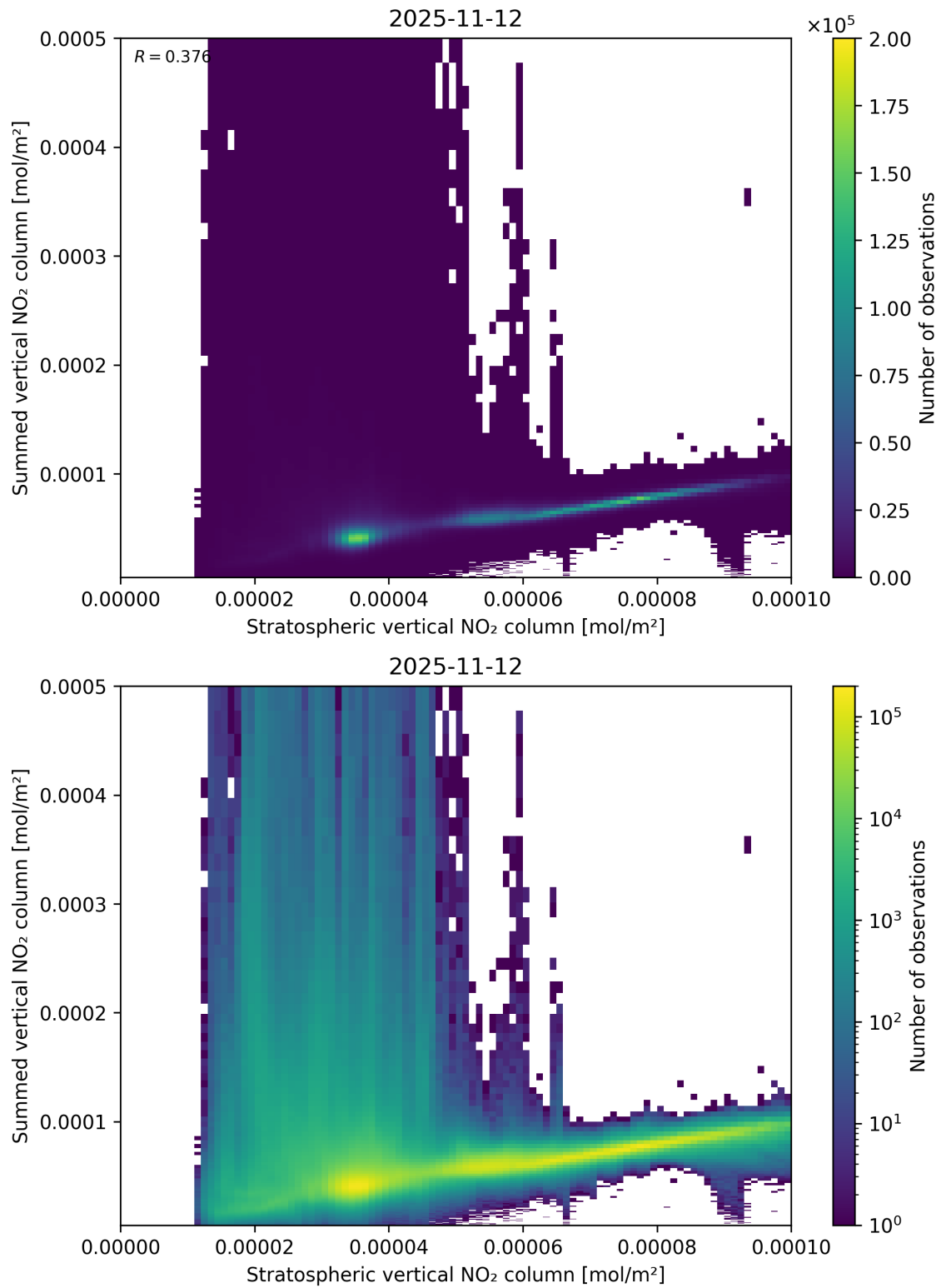
Figure 98: Scatter density plot of “Stratospheric vertical NO 2 column” against “Summed vertical NO 2 column” for 2025-11-12 to 2025-11-13.
