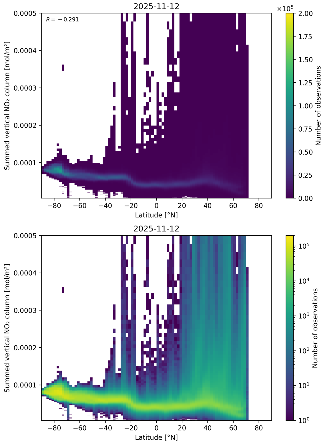
Figure 88: Scatter density plot of “Latitude” against “Summed vertical NO 2 column” for 2025-11-12 to 2025-11-13.
