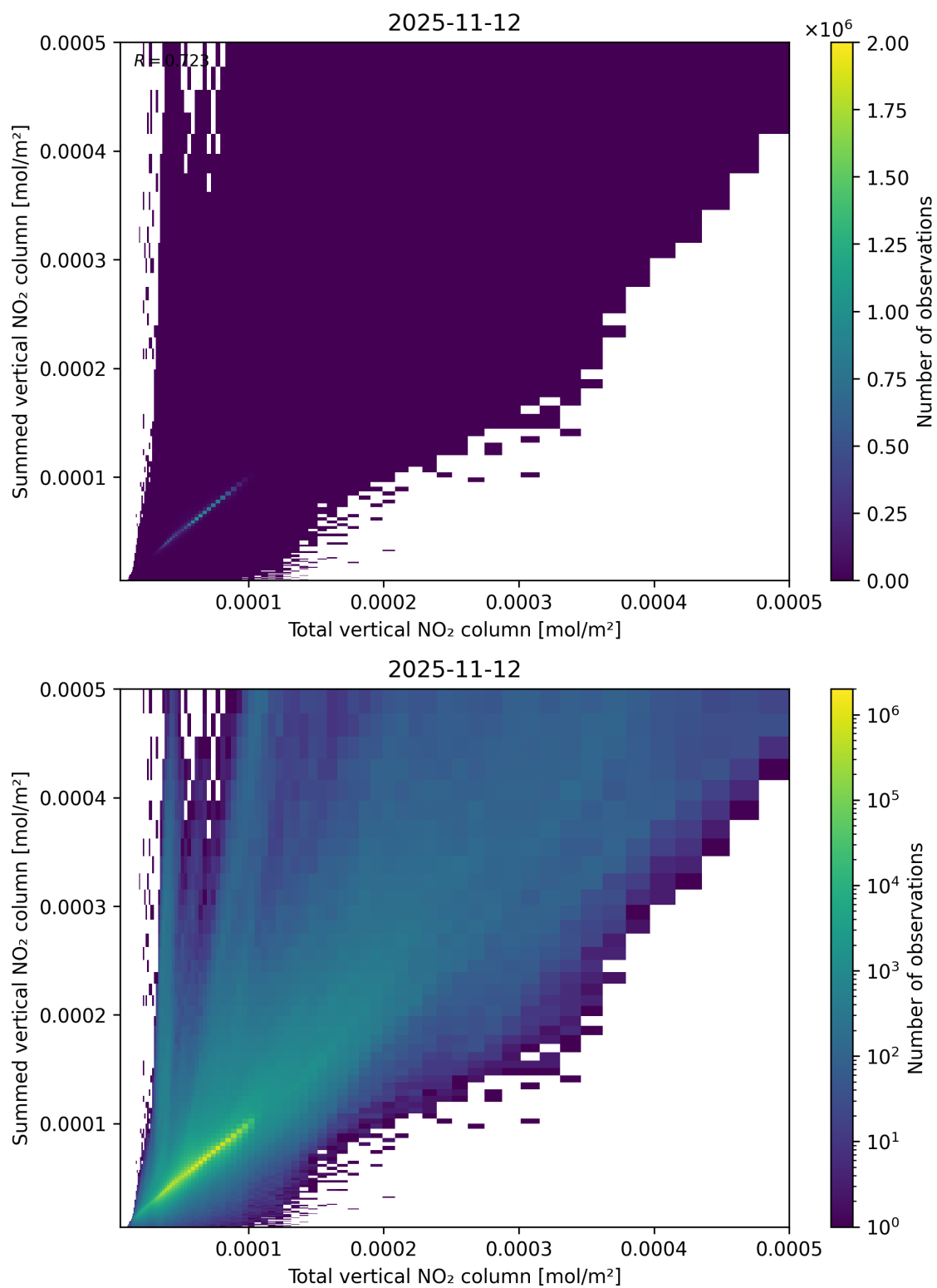
Figure 112: Scatter density plot of “Total vertical NO 2 column” against “Summed vertical NO 2 column” for 2025-11-12 to 2025-11-13.
