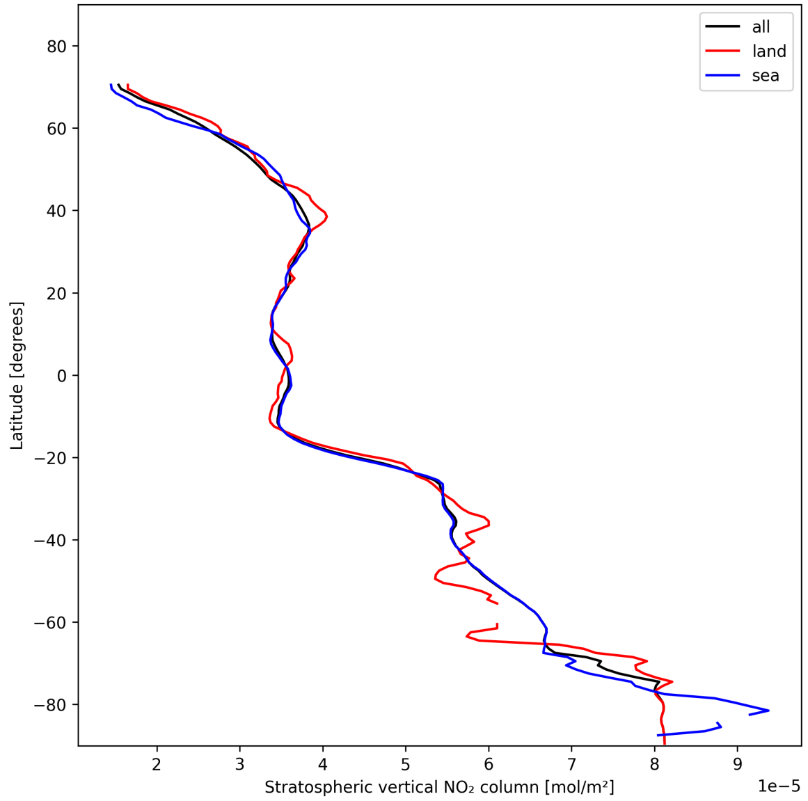
Figure 19: Zonal average of “Stratospheric vertical NO 2 column” for 2025-11-12 to 2025-11-13.
