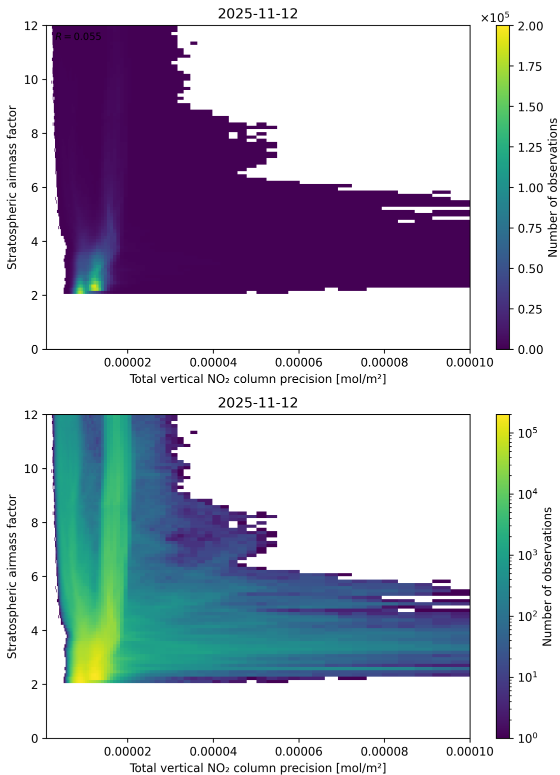
Figure 115: Scatter density plot of “Total vertical NO 2 column precision” against “Stratospheric air mass factor” for 2025-11-12 to 2025-11-13.
