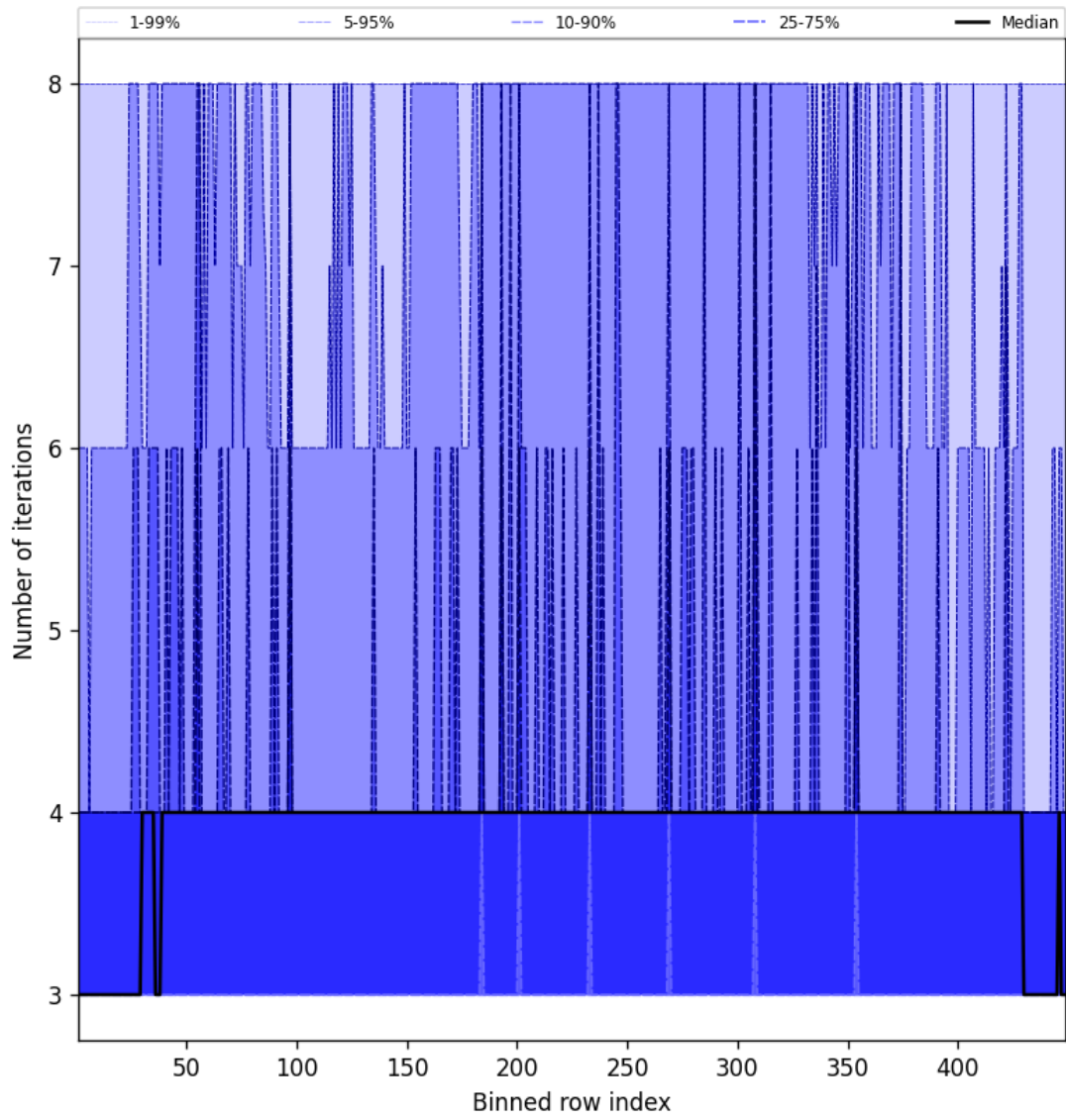
Figure 51: Along track statistics of “Number of iterations” for 2025-11-12 to 2025-11-13
