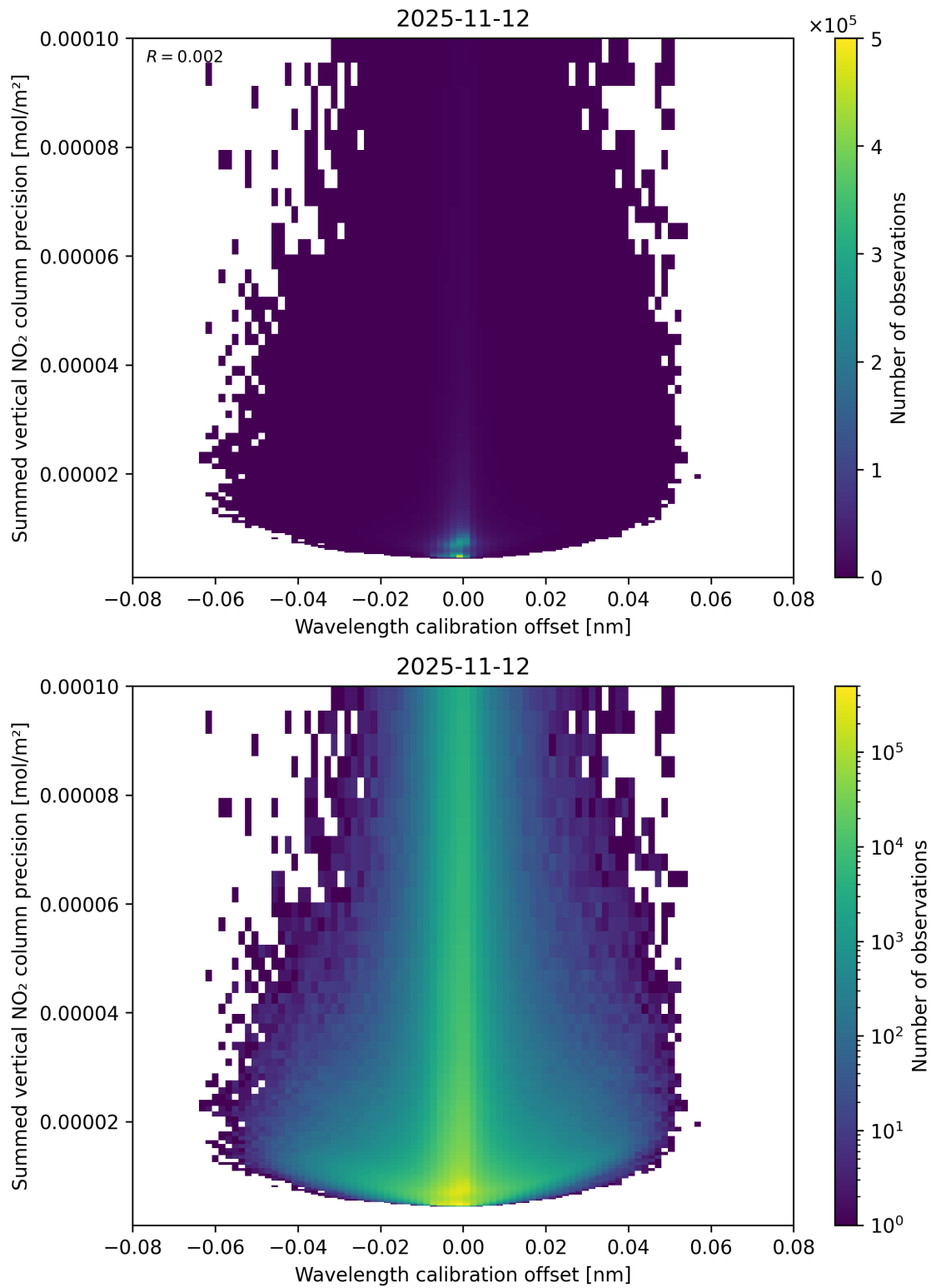
Figure 178: Scatter density plot of “Wavelength calibration offset” against “Summed vertical NO 2 column precision” for 2025-11-12 to 2025-11-13.
