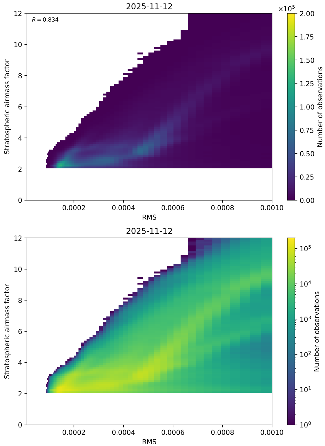
Figure 144: Scatter density plot of “RMS” against “Stratospheric airmass factor” for 2025-11-12 to 2025-11-13.
