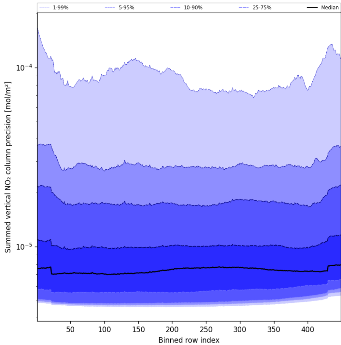
Figure 58: Along track statistics of “Summed vertical NO 2 column precision” for 2025-11-12 to 2025-11-13
