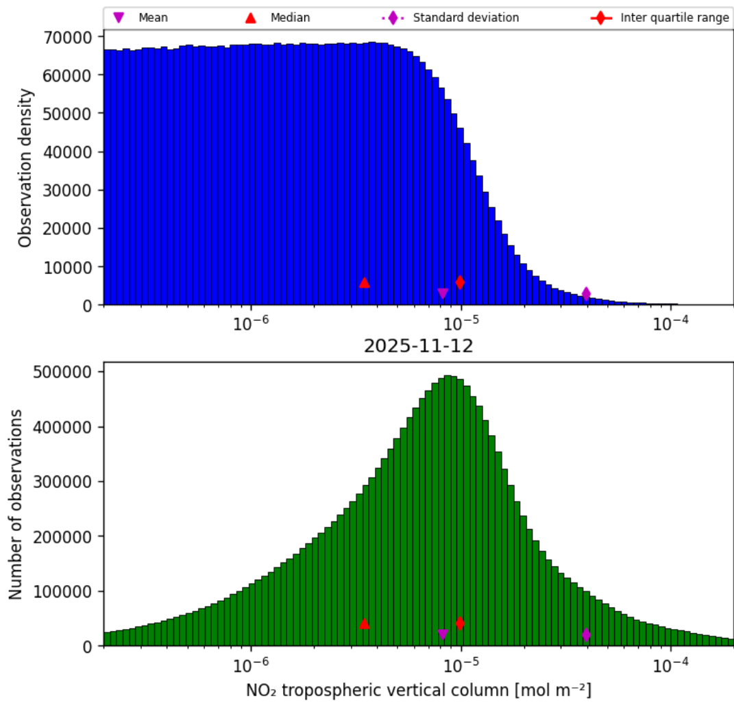
Figure 29: Histogram of “NO 2 tropospheric vertical column” for 2025-11-12 to 2025-11-13
