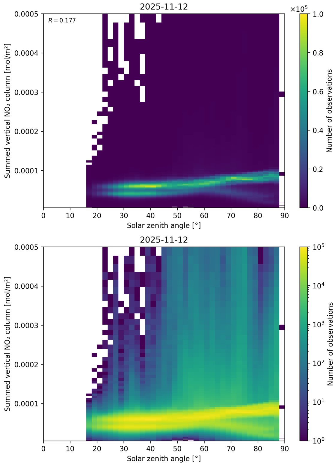
Figure 151: Scatter density plot of “Solar zenith angle” against “Summed vertical NO 2 column” for 2025-11-12 to 2025-11-13.
