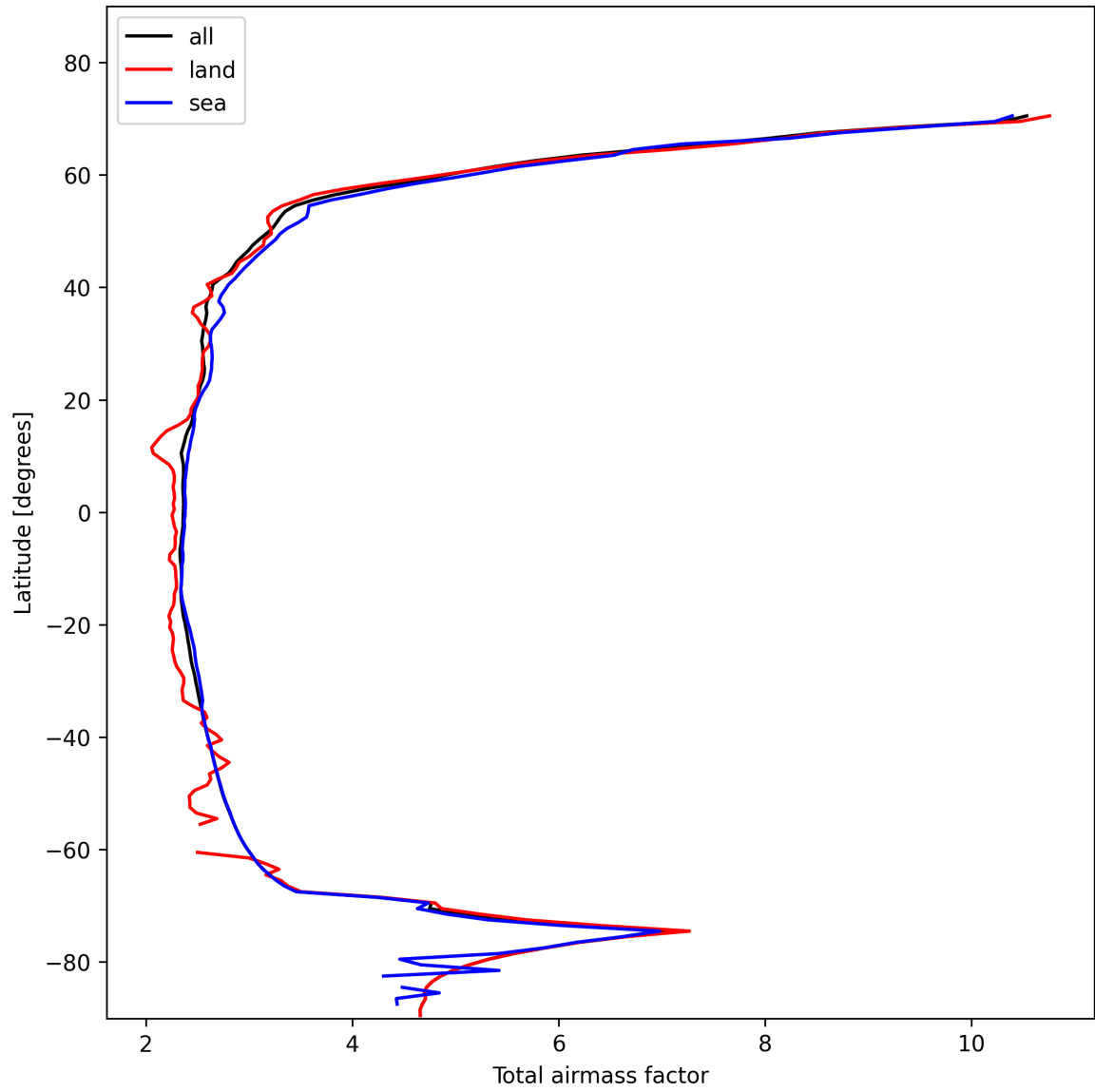
Figure 15: Zonal average of “Total airmass factor” for 2025-11-12 to 2025-11-13.
