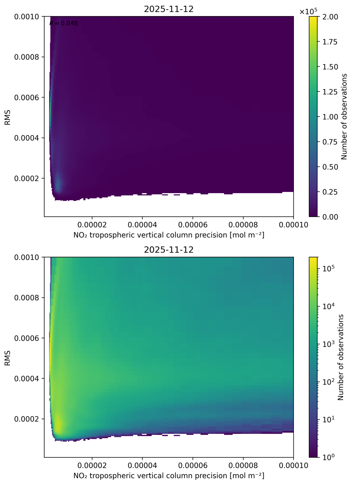
Figure 140: Scatter density plot of “NO 2 tropospheric vertical column precision” against “RMS” for 2025-11-12 to 2025-11-13.
