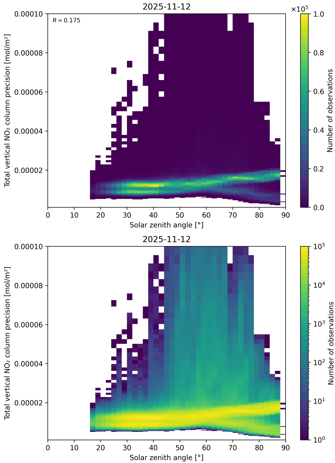
Figure 154: Scatter density plot of “Solar zenith angle” against “Total vertical NO 2 column precision” for 2025-11-12 to 2025-11-13.
