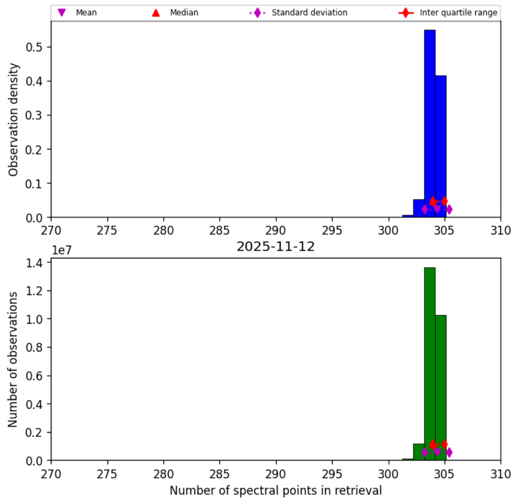
Figure 33: Histogram of “Number of spectral points in retrieval” for 2025-11-12 to 2025-11-13
