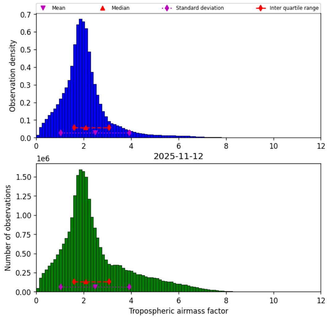
Figure 31: Histogram of “Tropospheric airmass factor” for 2025-11-12 to 2025-11-13
