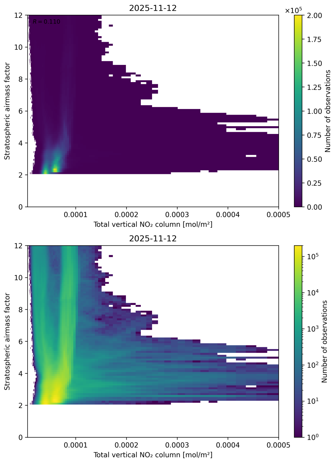
Figure 110: Scatter density plot of “Total vertical NO 2 column” against “Stratospheric airmass factor” for 2025-11-12 to 2025-11-13.
