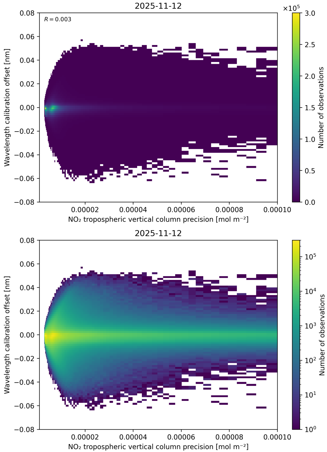
Figure 141: Scatter density plot of “NO 2 tropospheric vertical column precision” against “Wavelength calibration offset” for 2025-11-12 to 2025-11-13.
