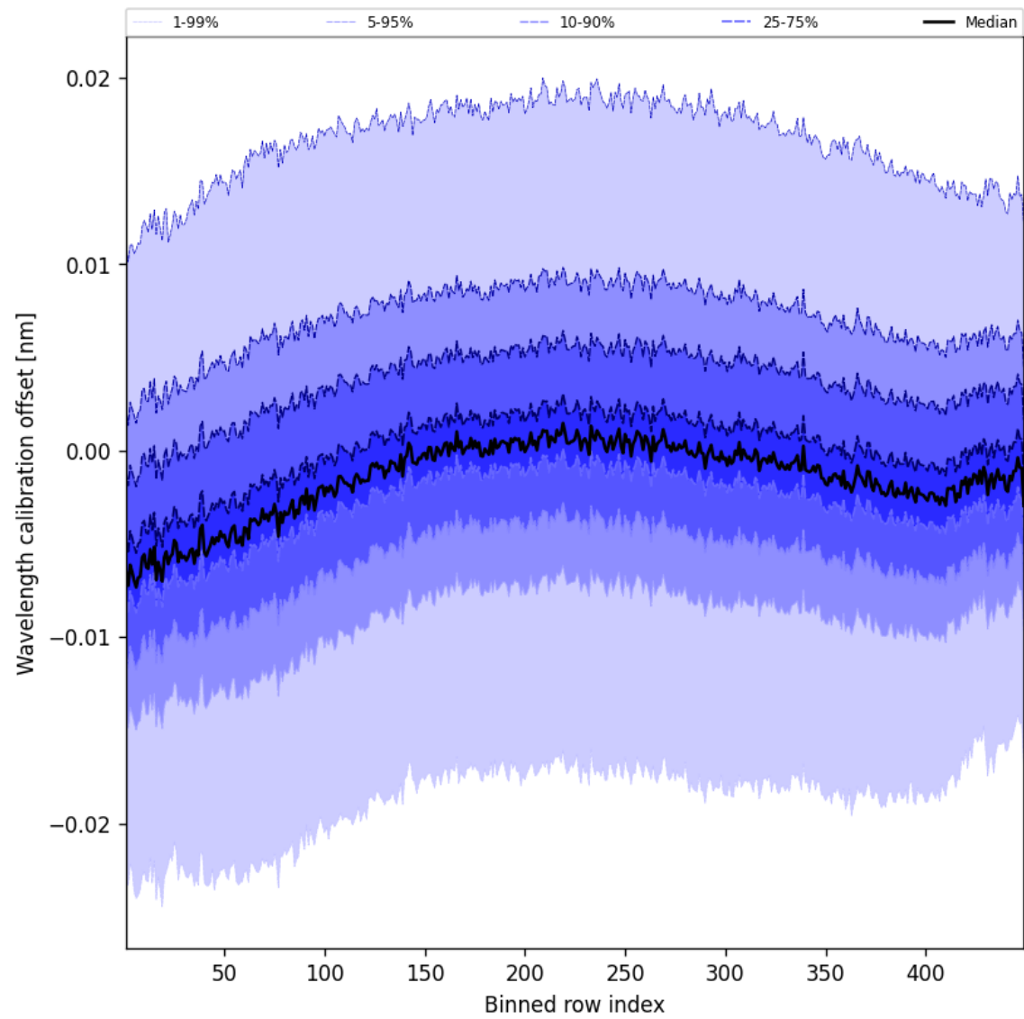
Figure 52: Along track statistics of “Wavelength calibration offset” for 2025-11-12 to 2025-11-13
