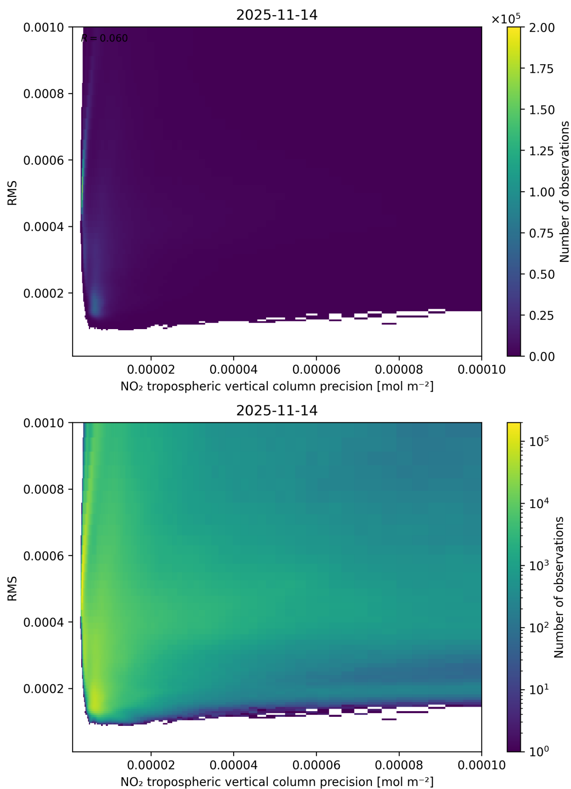
Figure 140: Scatter density plot of “NO 2 tropospheric vertical column precision” against “RMS” for 2025-11-13 to 2025-11-15.
