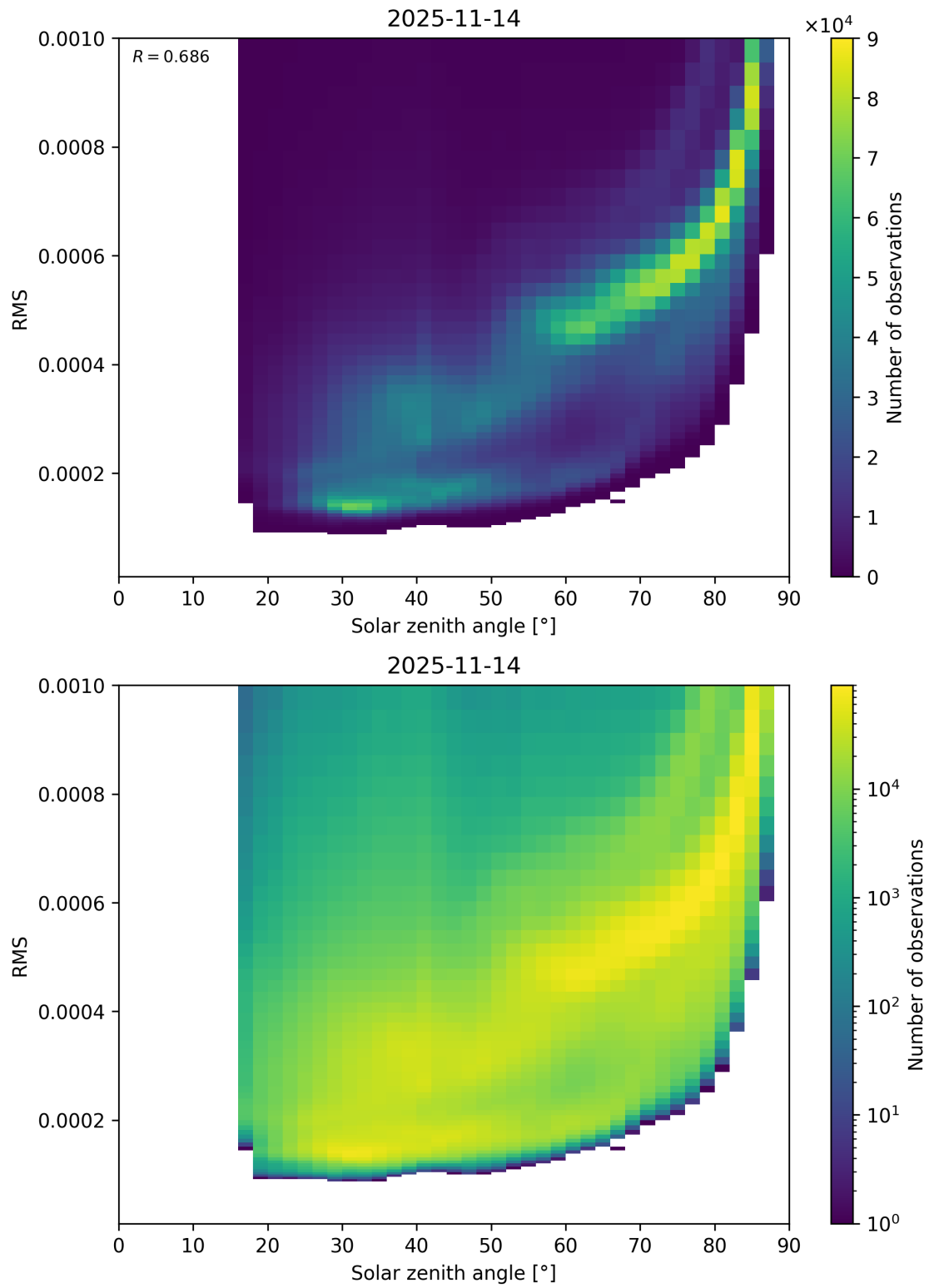
Figure 157: Scatter density plot of “Solar zenith angle” against “RMS” for 2025-11-13 to 2025-11-15.
