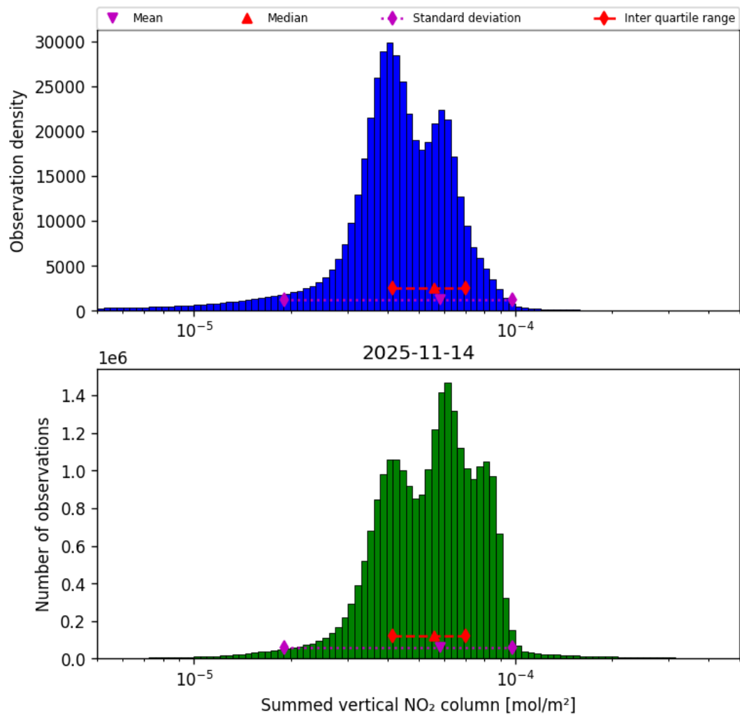
Figure 40: Histogram of “Summed vertical NO 2 column” for 2025-11-13 to 2025-11-15
