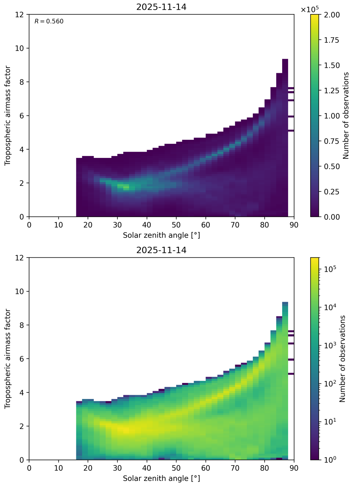
Figure 147: Scatter density plot of “Solar zenith angle” against “Tropospheric airmass factor” for 2025-11-13 to 2025-11-15.
