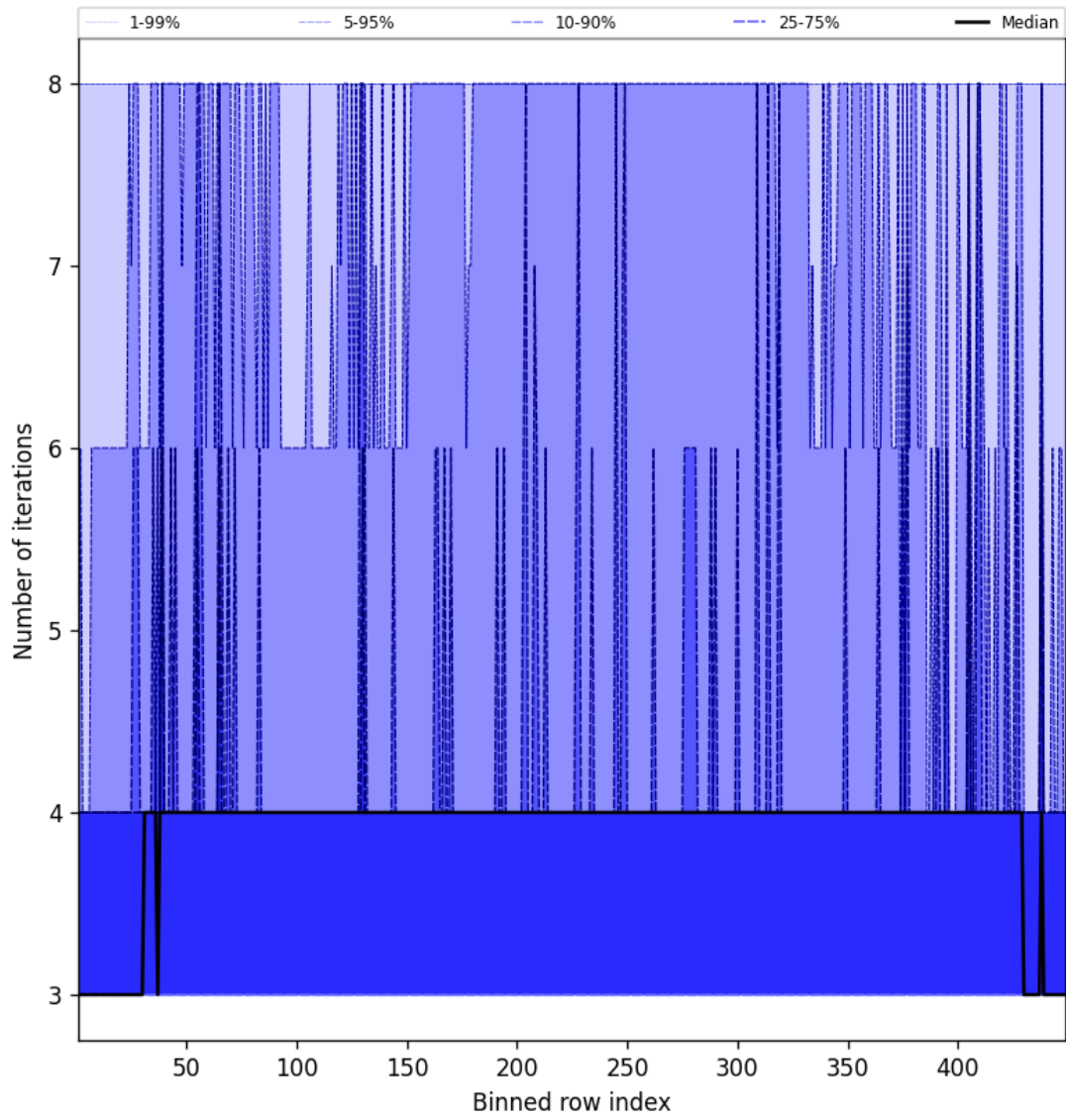
Figure 51: Along track statistics of “Number of iterations” for 2025-11-13 to 2025-11-15
