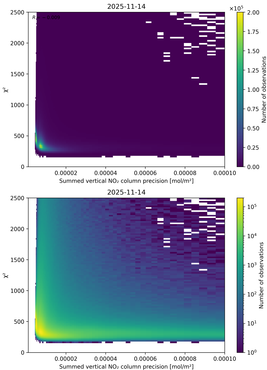
Figure 107: Scatter density plot of “Summed vertical NO 2 column precision” against “ \chi^2 ” for 2025-11-13 to 2025-11-15.
