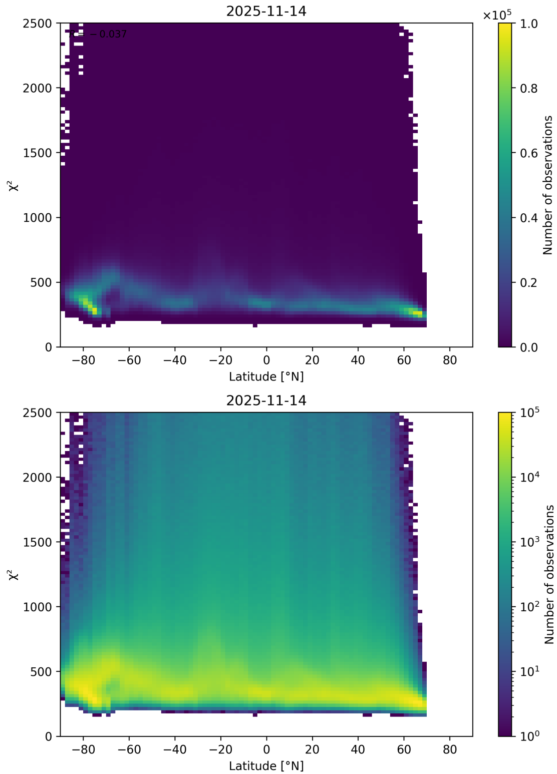
Figure 86: Scatter density plot of “Latitude” against “ \chi^2 ” for 2025-11-13 to 2025-11-15.
