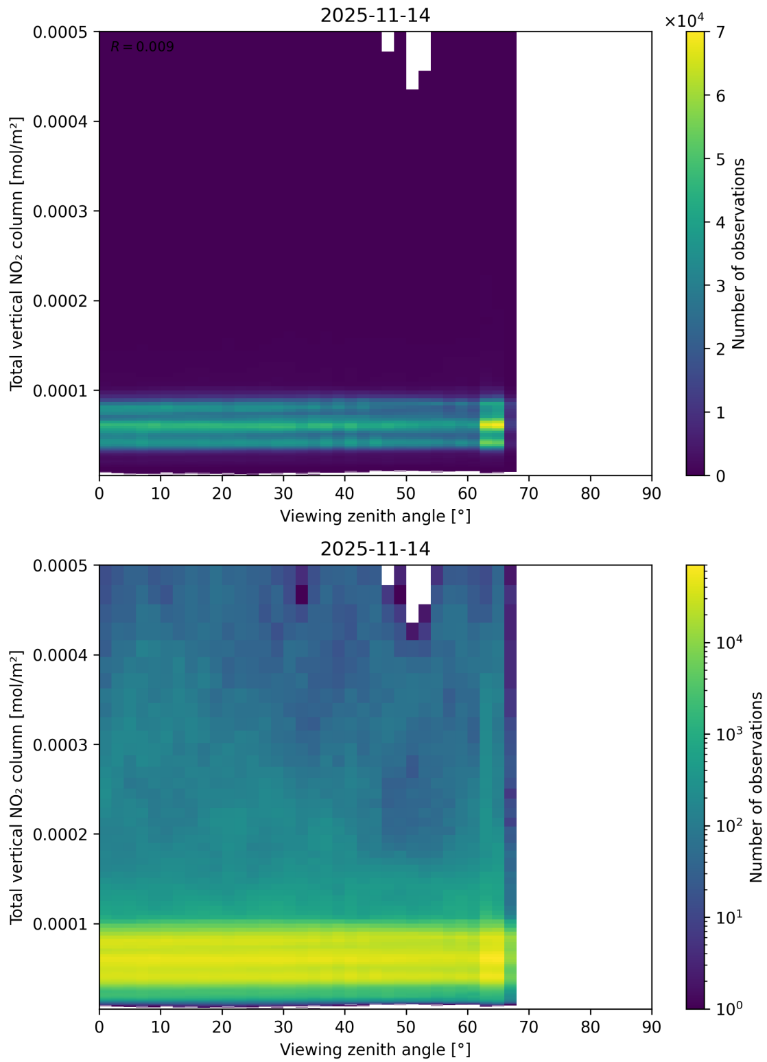
Figure 167: Scatter density plot of “Viewing zenith angle” against “Total vertical NO 2 column” for 2025-11-13 to 2025-11-15.
