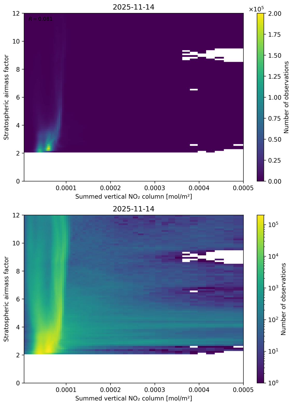
Figure 103: Scatter density plot of “Summed vertical NO 2 column” against “Stratospheric air mass factor” for 2025-11-13 to 2025-11-15.
