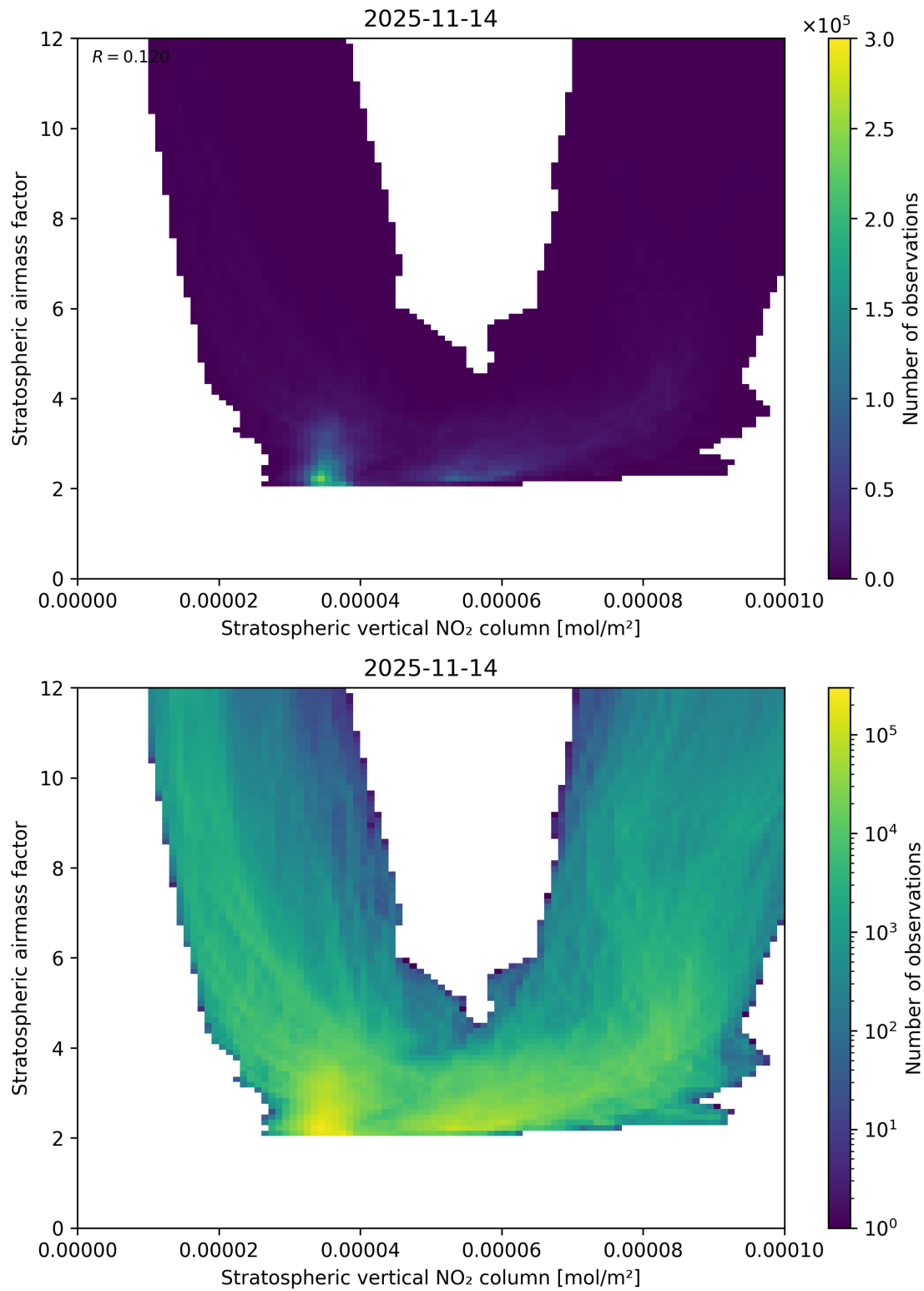
Figure 96: Scatter density plot of “Stratospheric vertical NO 2 column” against “Stratospheric airmass factor” for 2025-11-13 to 2025-11-15.
