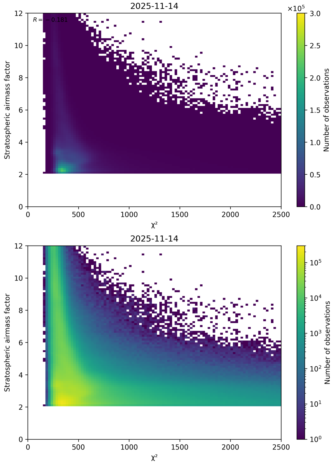
Figure 81: Scatter density plot of “ \chi^2 ” against “Stratospheric airmass factor” for 2025-11-13 to 2025-11-15.
