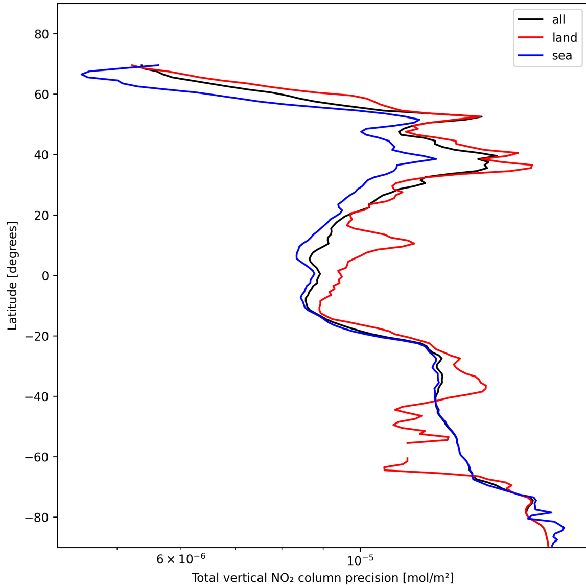
Figure 22: Zonal average of “Total vertical NO 2 column precision” for 2025-11-13 to 2025-11-15.
