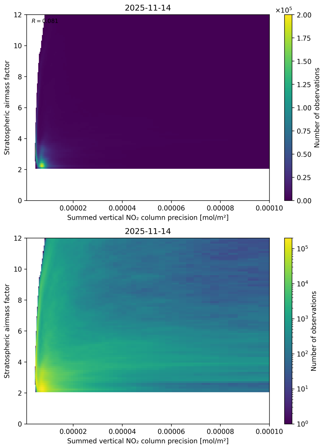
Figure 106: Scatter density plot of “Summed vertical NO 2 column precision” against “Stratospheric airmass factor” for 2025-11-13 to 2025-11-15.
