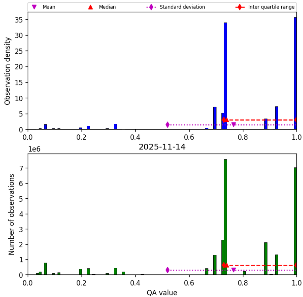
Figure 28: Histogram of “QA value” for 2025-11-13 to 2025-11-15
