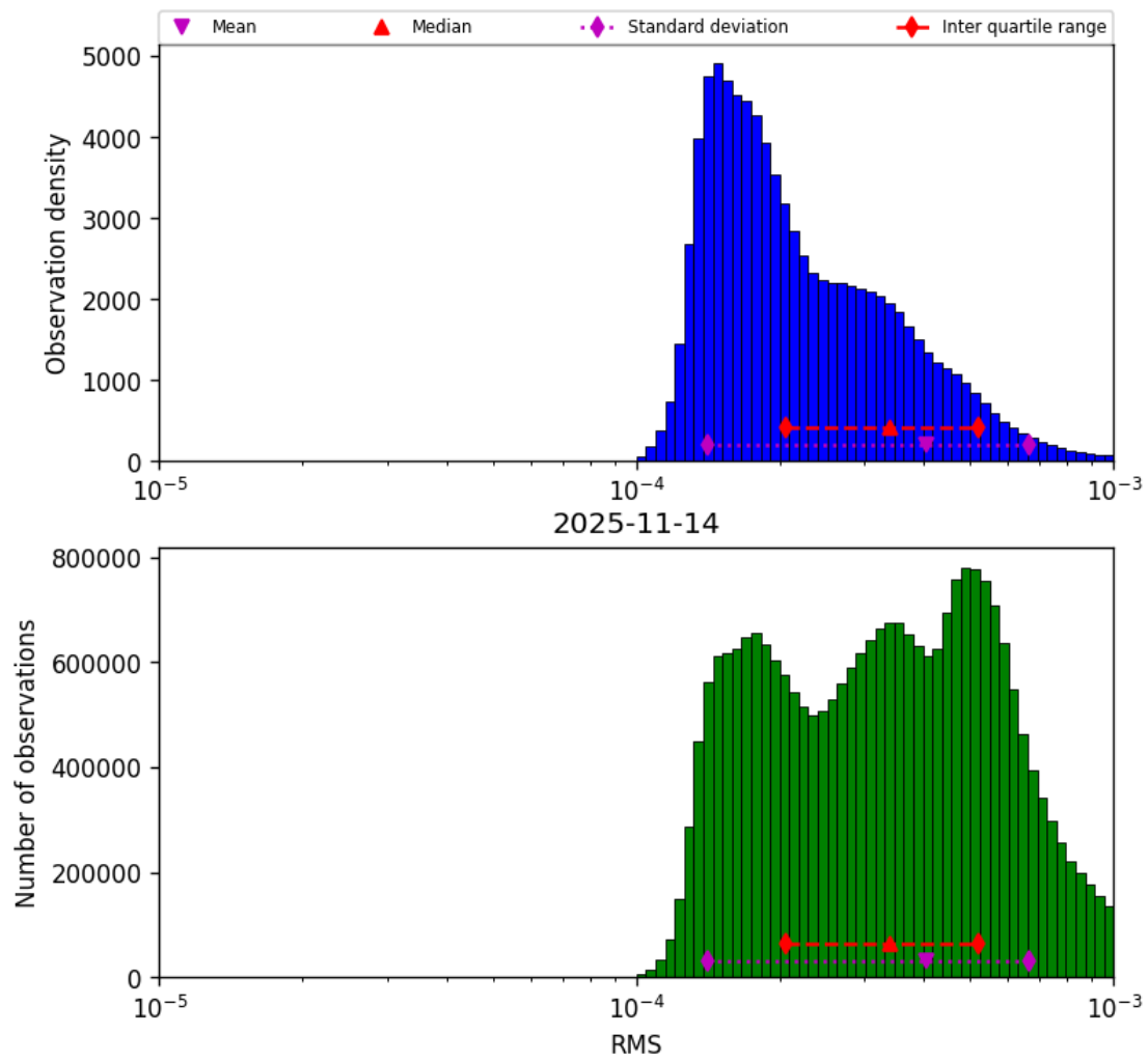
Figure 43: Histogram of “RMS” for 2025-11-13 to 2025-11-15
