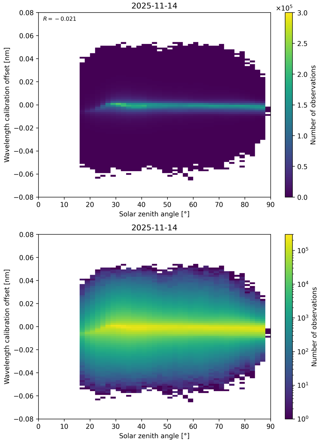
Figure 158: Scatter density plot of “Solar zenith angle” against “Wavelength calibration offset” for 2025-11-13 to 2025-11-15.
