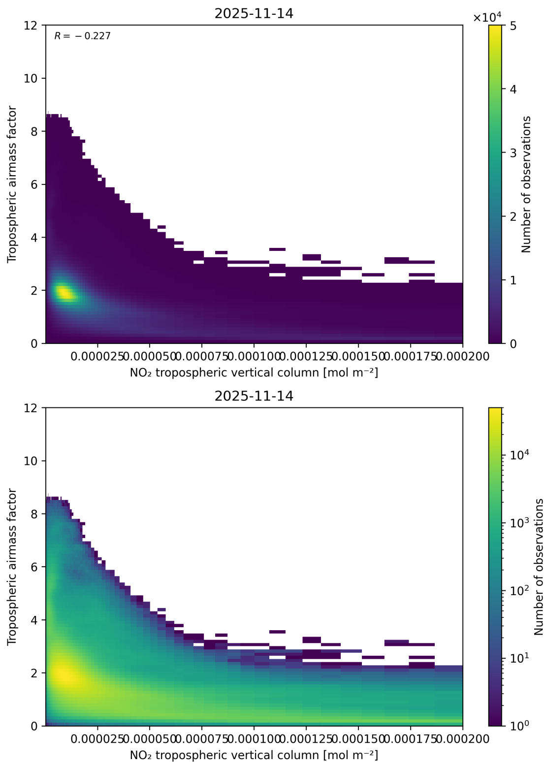
Figure 123: Scatter density plot of “NO 2 tropospheric vertical column” against “Tropospheric air mass factor” for 2025-11-13 to 2025-11-15.
