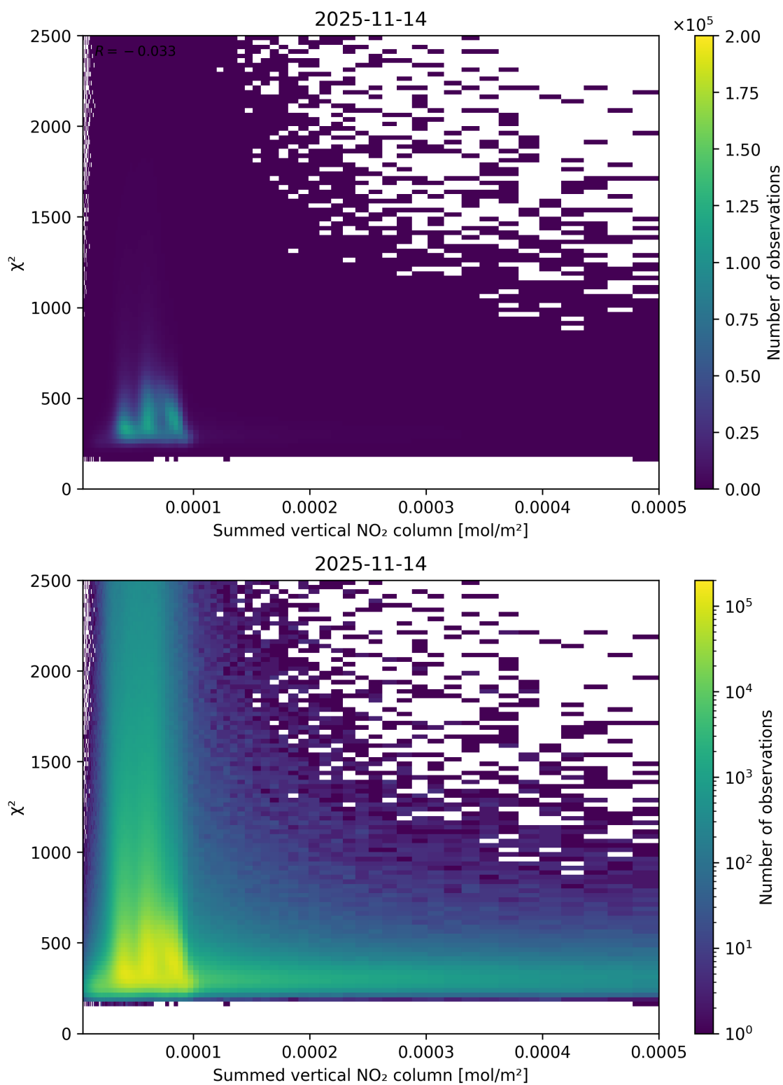
Figure 104: Scatter density plot of “Summed vertical NO 2 column” against “ \chi^2 ” for 2025-11-13 to 2025-11-15.
