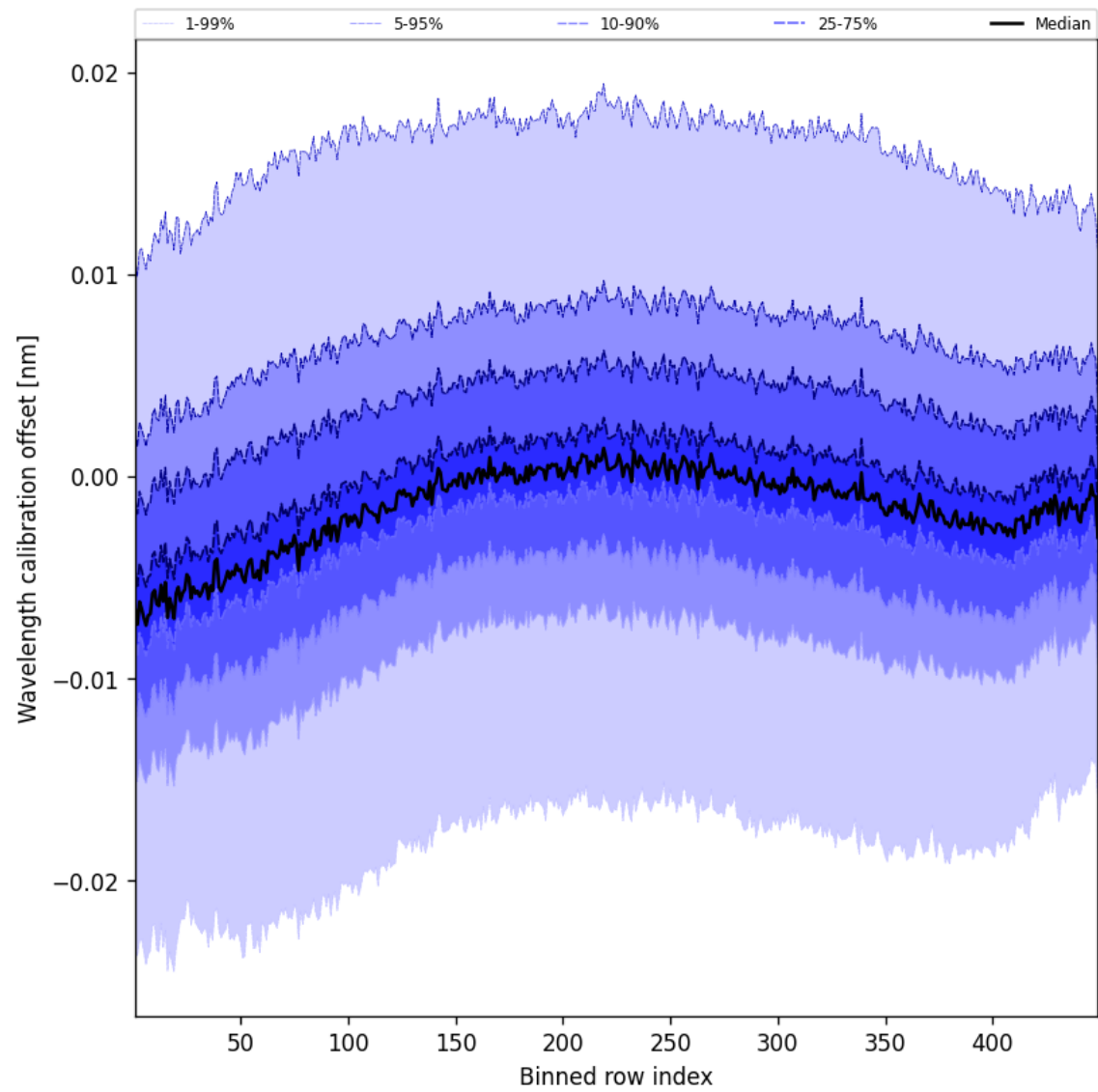
Figure 52: Along track statistics of “Wavelength calibration offset” for 2025-11-13 to 2025-11-15
