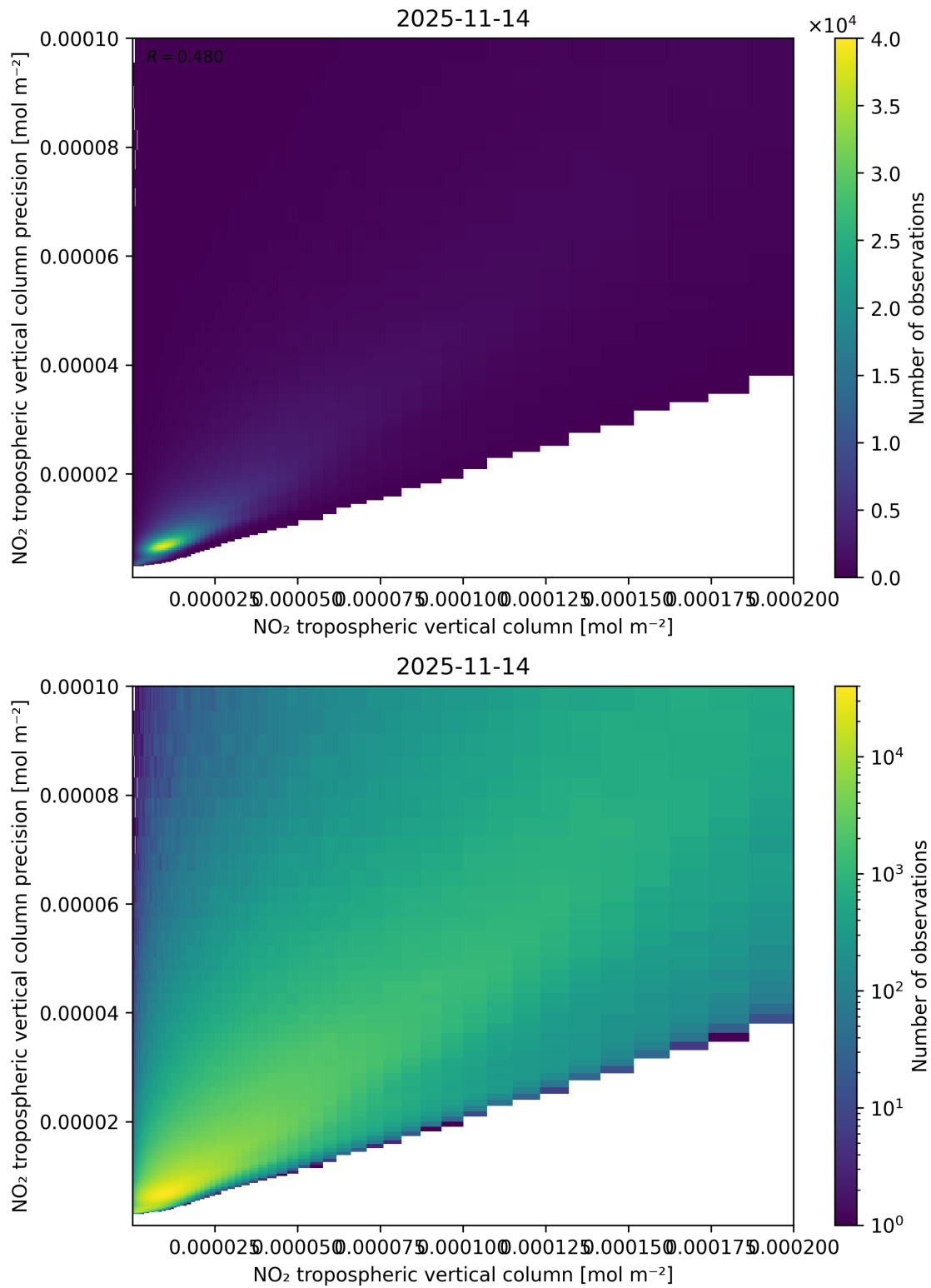
Figure 130: Scatter density plot of “NO 2 tropospheric vertical column” against “NO 2 tropospheric vertical column precision” for 2025-11-13 to 2025-11-15.
