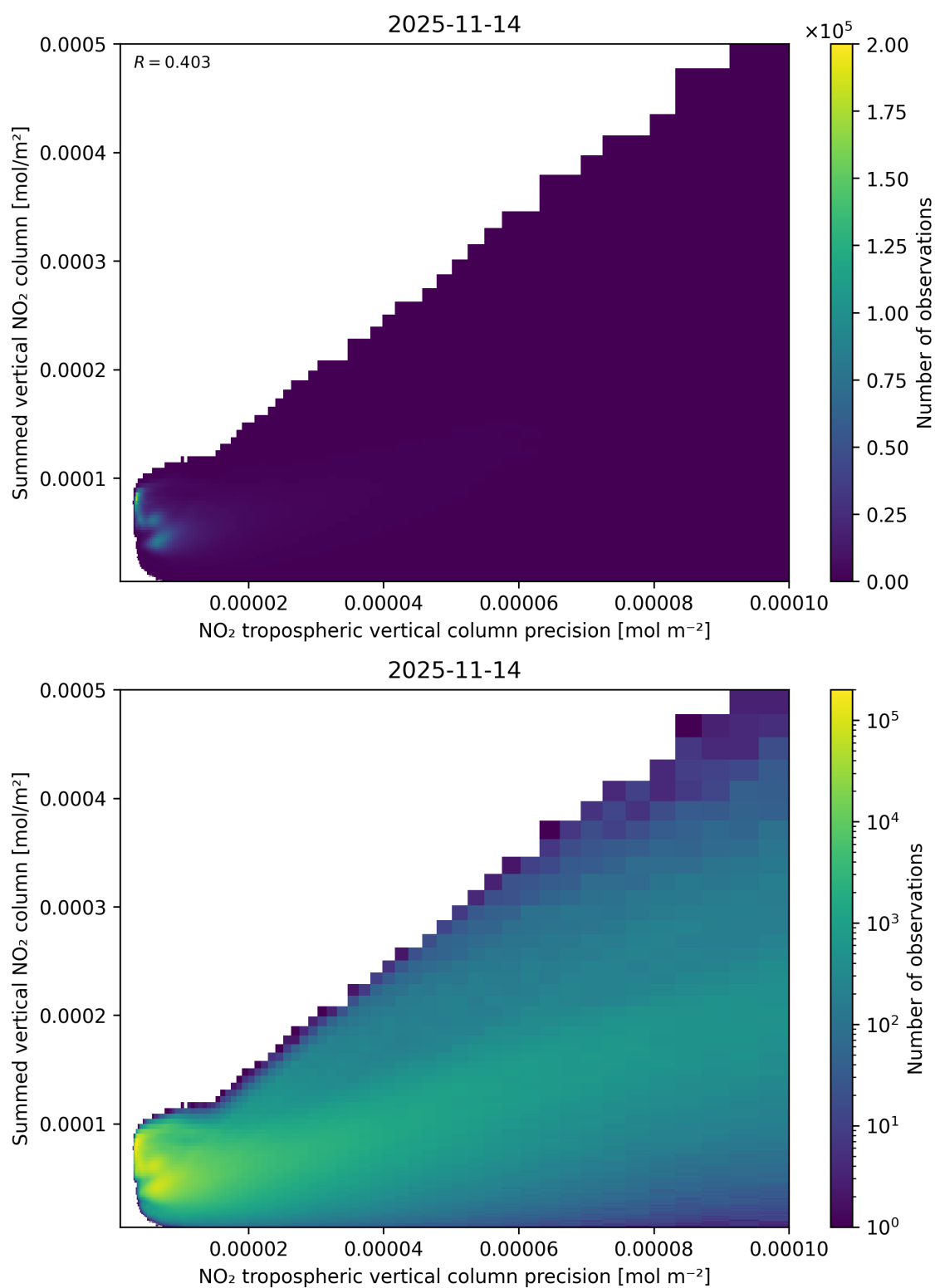
Figure 136: Scatter density plot of “NO 2 tropospheric vertical column precision” against “Summed vertical NO 2 column” for 2025-11-13 to 2025-11-15.
