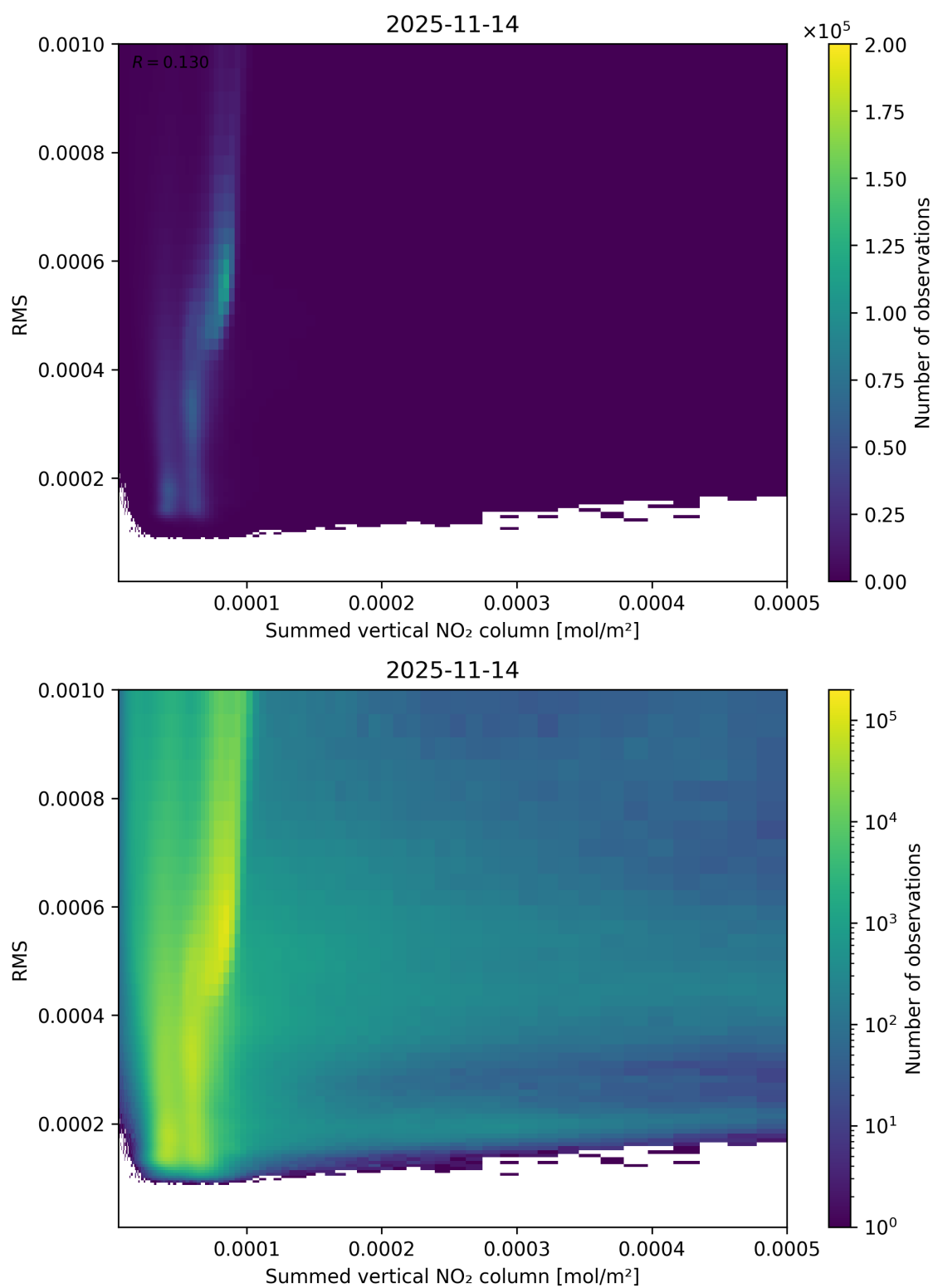
Figure 109: Scatter density plot of “Summed vertical NO 2 column” against “RMS” for 2025-11-13 to 2025-11-15.
