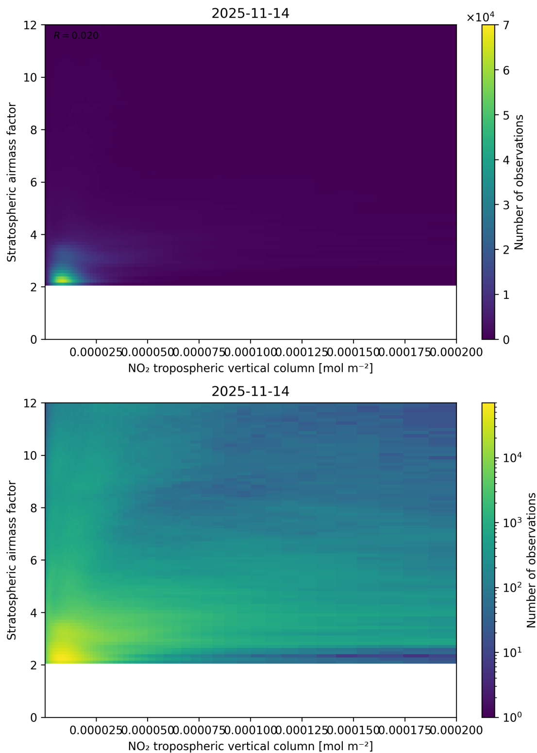
Figure 121: Scatter density plot of “NO 2 tropospheric vertical column” against “Stratospheric airmass factor” for 2025-11-13 to 2025-11-15.
