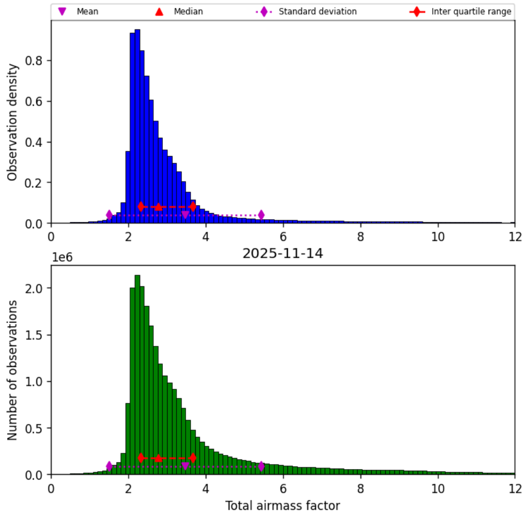
Figure 32: Histogram of “Total airmass factor” for 2025-11-13 to 2025-11-15
