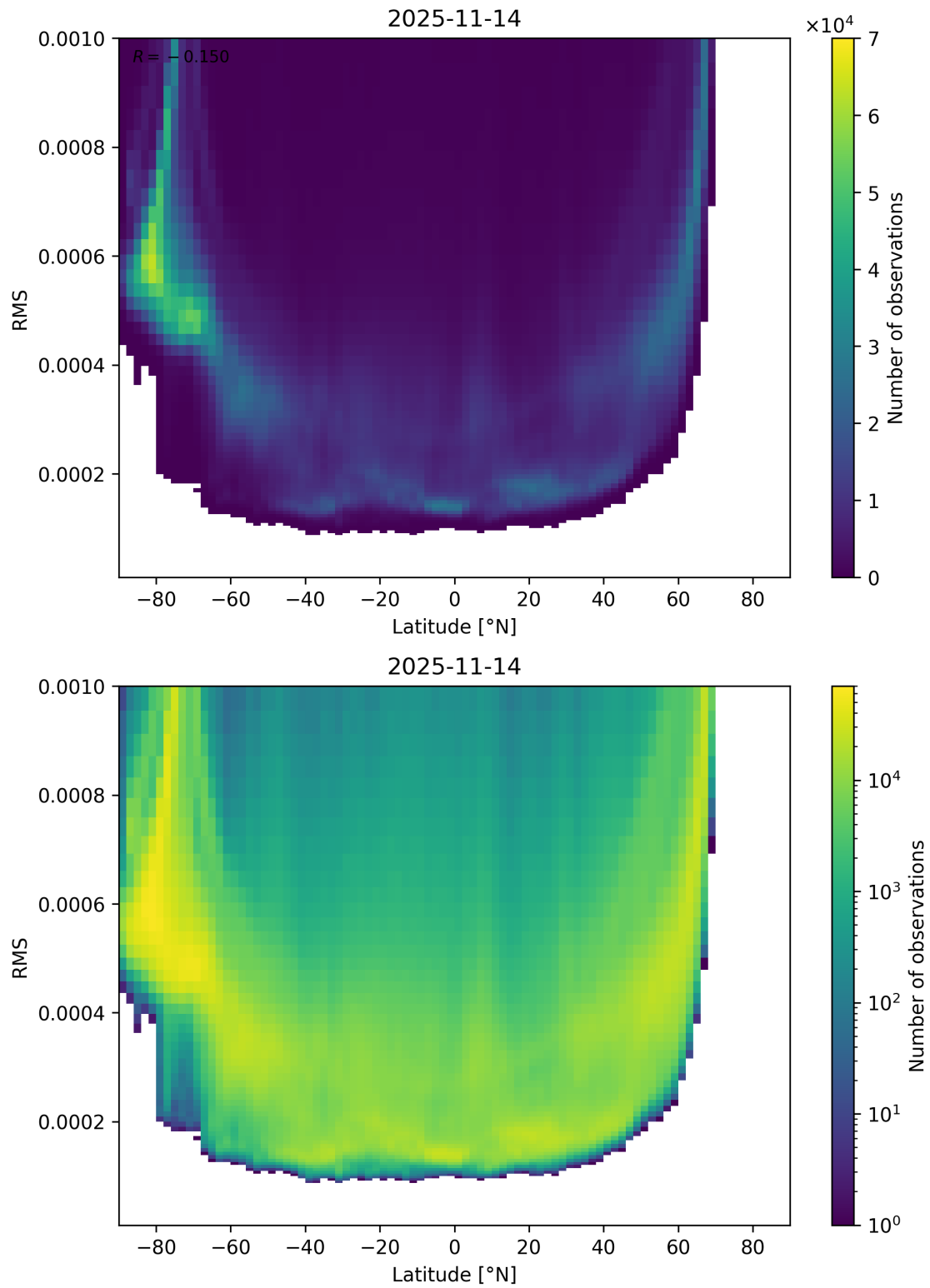
Figure 94: Scatter density plot of “Latitude” against “RMS” for 2025-11-13 to 2025-11-15.
