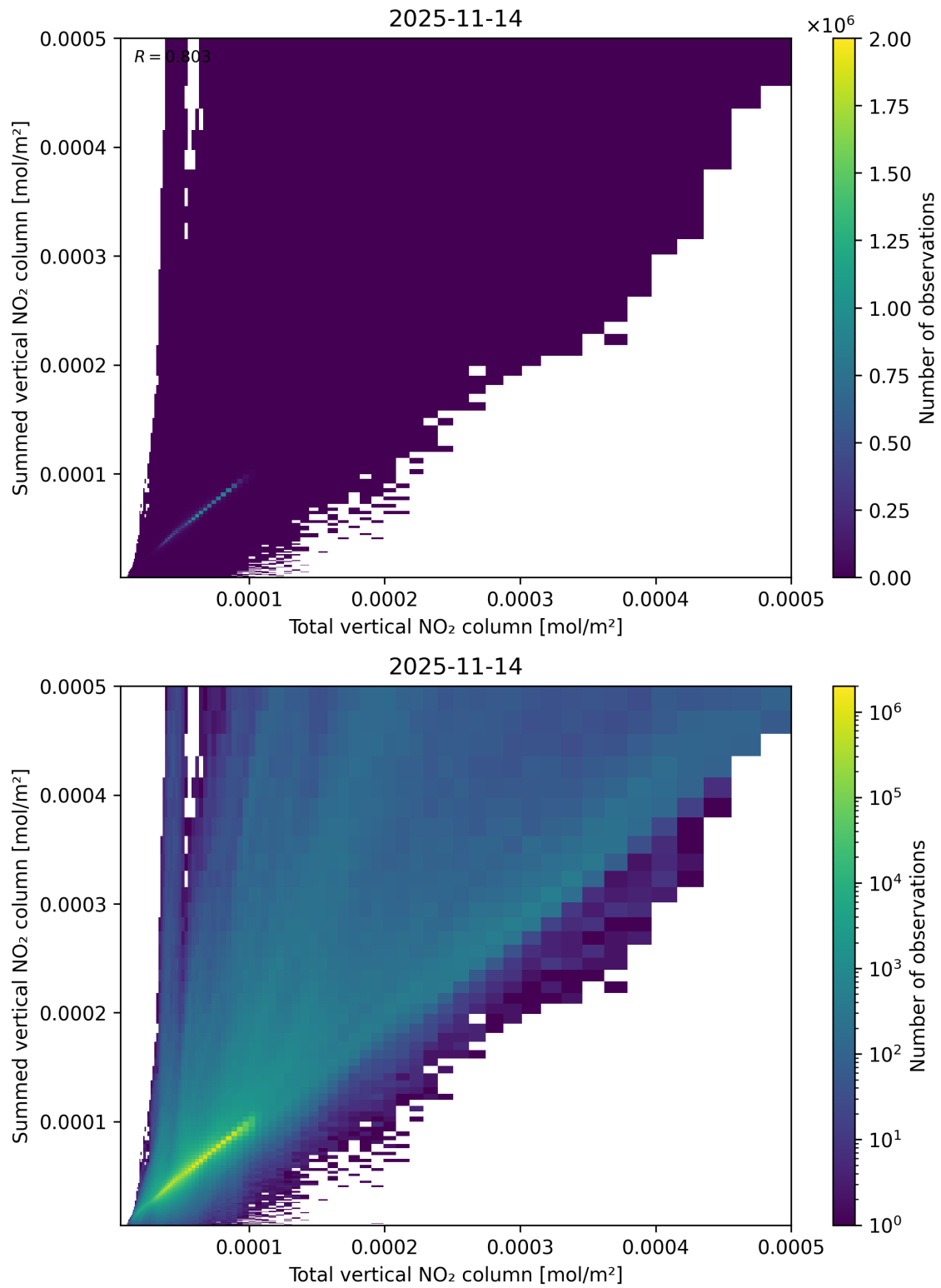
Figure 112: Scatter density plot of “Total vertical NO 2 column” against “Summed vertical NO 2 column” for 2025-11-13 to 2025-11-15.
