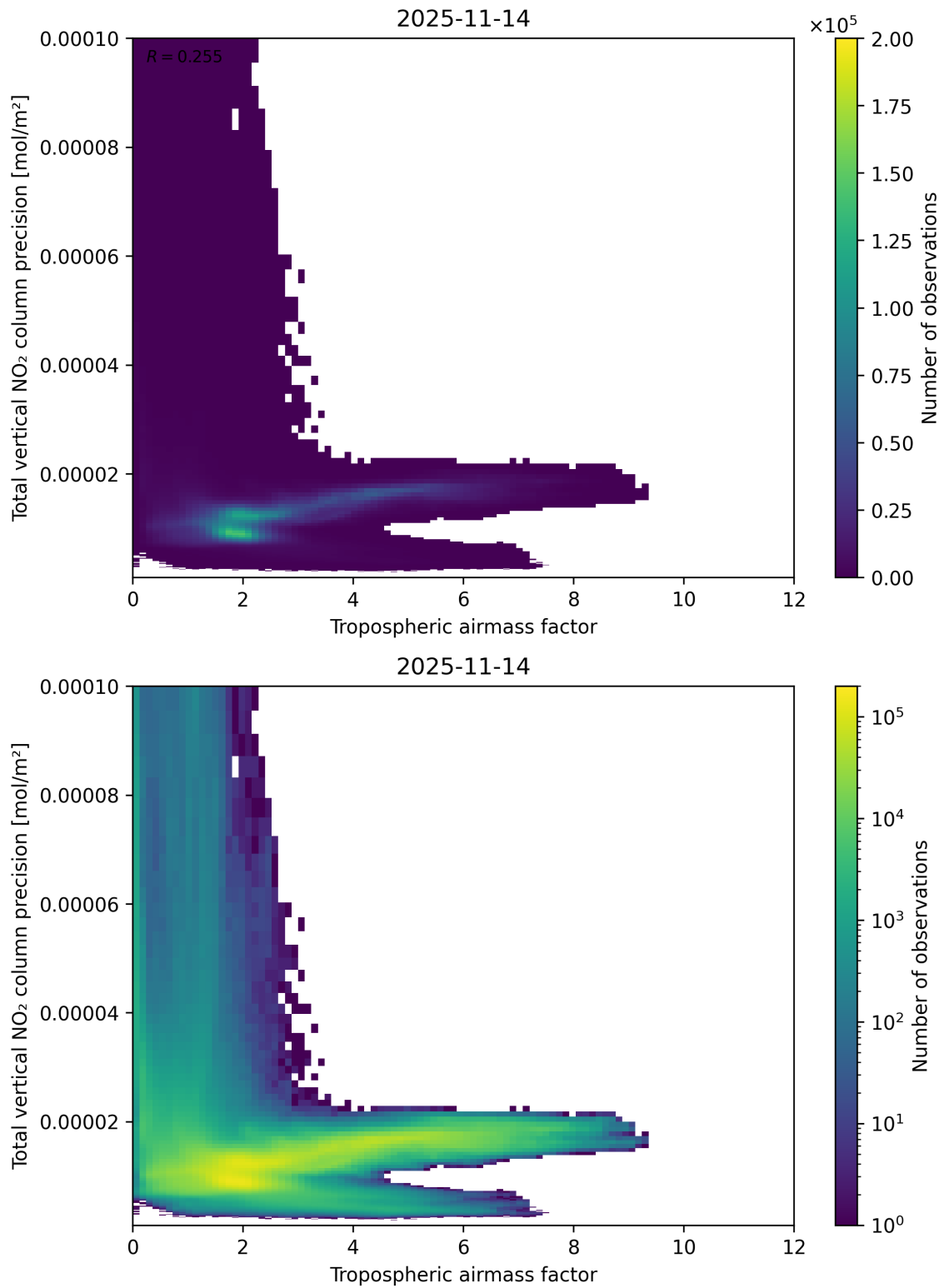
Figure 78: Scatter density plot of “Tropospheric air mass factor” against “Total vertical NO 2 column precision” for 2025-11-13 to 2025-11-15.
