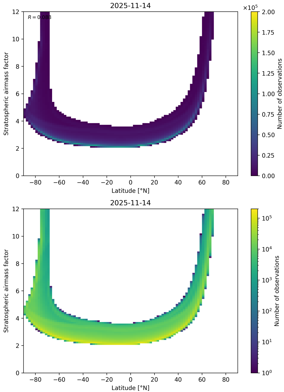
Figure 83: Scatter density plot of “Latitude” against “Stratospheric air mass factor” for 2025-11-13 to 2025-11-15.
