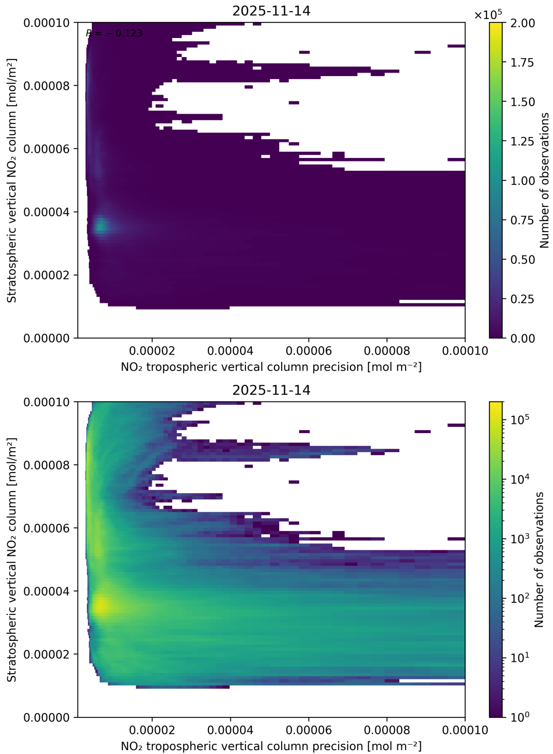
Figure 135: Scatter density plot of “NO 2 tropospheric vertical column precision” against “Stratospheric vertical NO 2 column” for 2025-11-13 to 2025-11-15.
