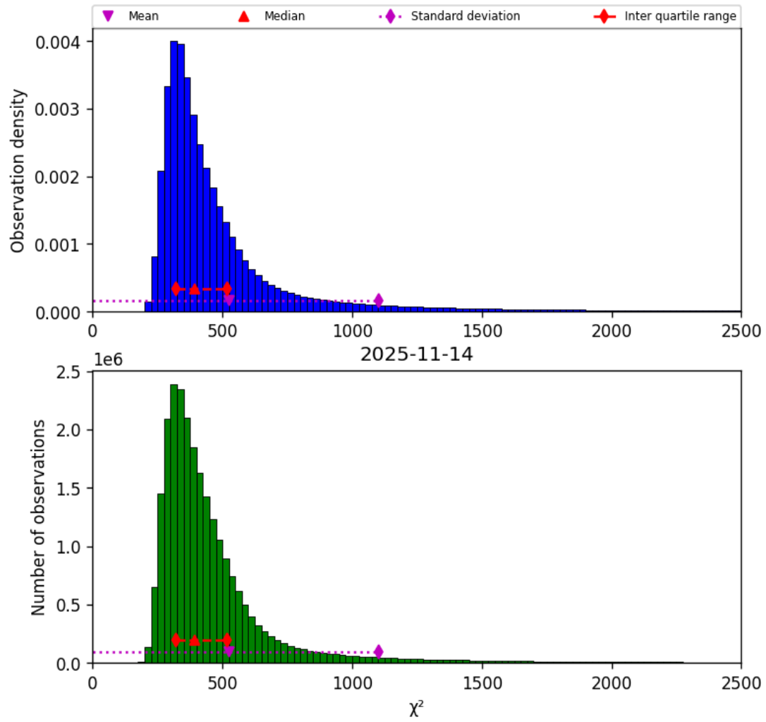
Figure 42: Histogram of “ \chi^2 ” for 2025-11-13 to 2025-11-15
