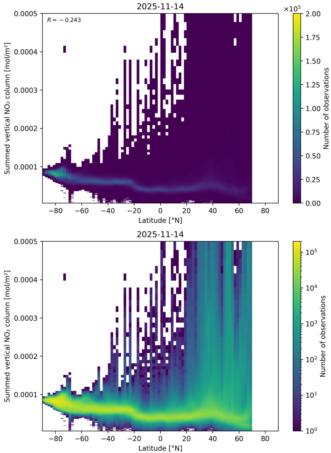
Figure 88: Scatter density plot of “Latitude” against “Summed vertical NO 2 column” for 2025-11-13 to 2025-11-15.
