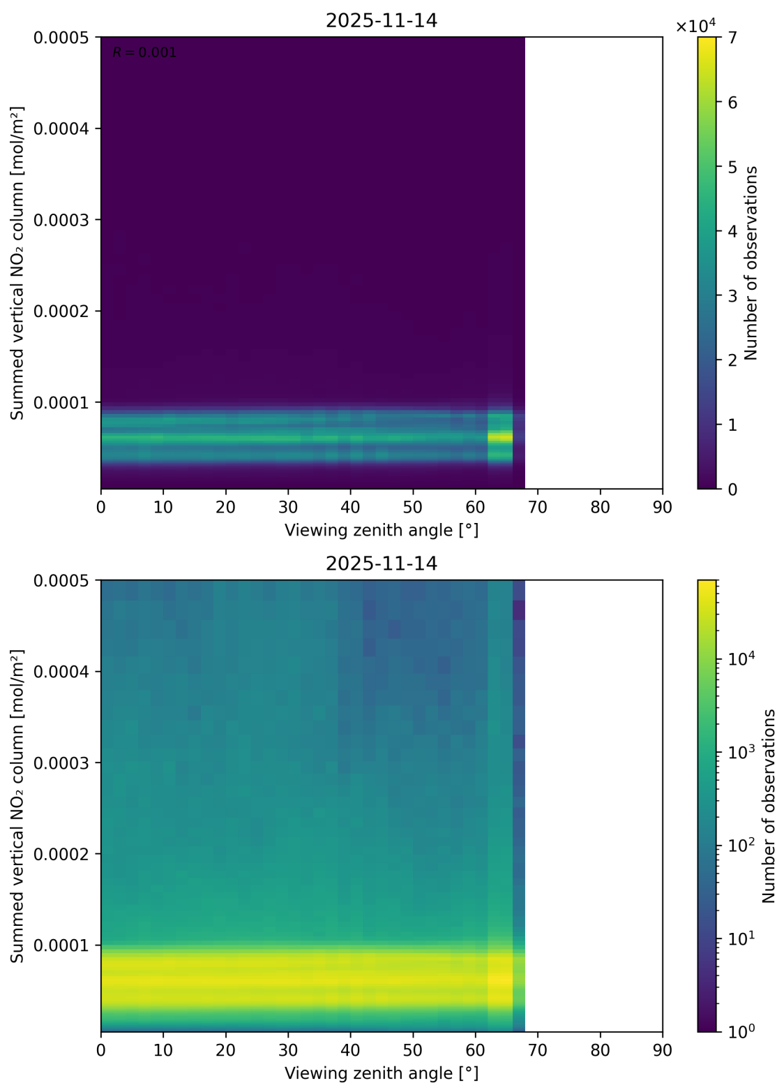
Figure 165: Scatter density plot of “Viewing zenith angle” against “Summed vertical NO 2 column” for 2025-11-13 to 2025-11-15.
