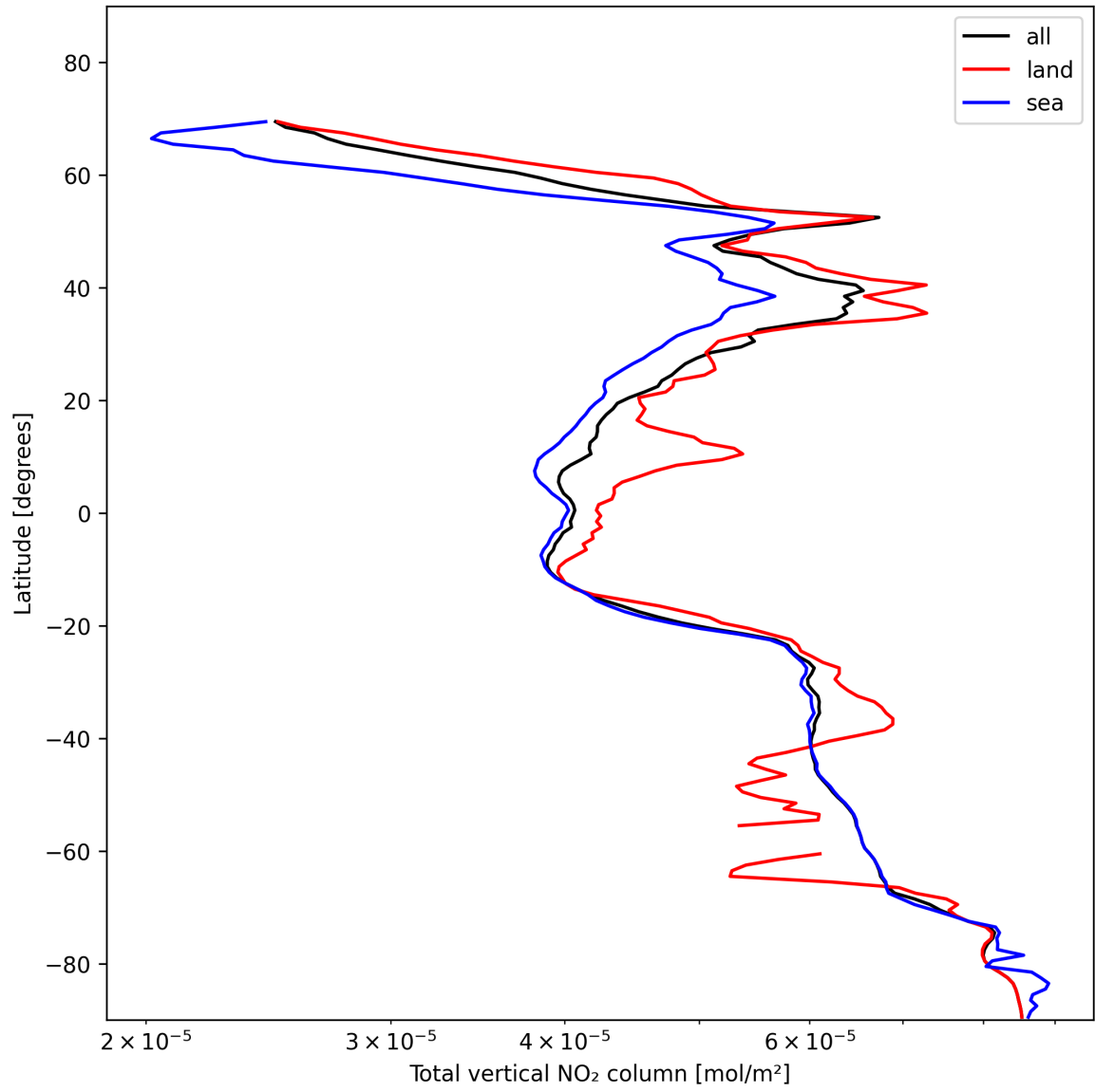
Figure 21: Zonal average of “Total vertical NO 2 column” for 2025-11-13 to 2025-11-15.
