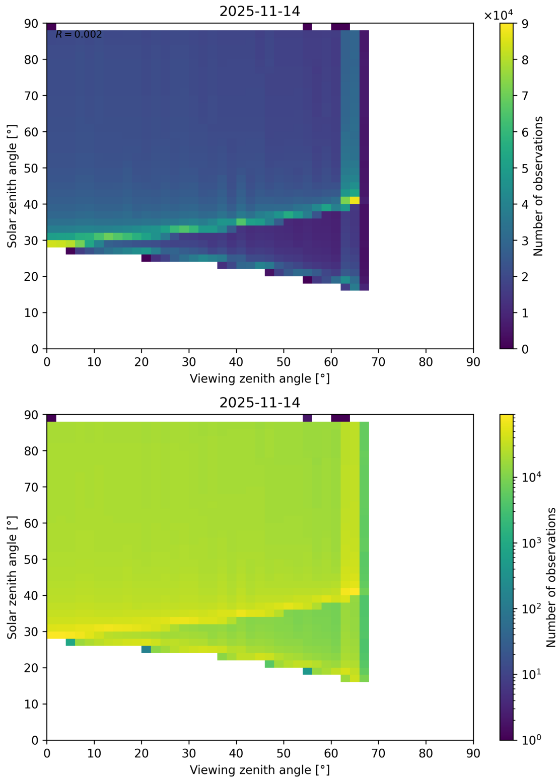
Figure 172: Scatter density plot of “Viewing zenith angle” against “Solar zenith angle” for 2025-11-13 to 2025-11-15.
