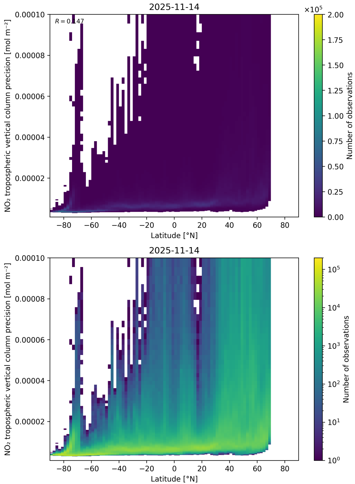
Figure 93: Scatter density plot of “Latitude” against “NO 2 tropospheric vertical column precision” for 2025-11-13 to 2025-11-15.
