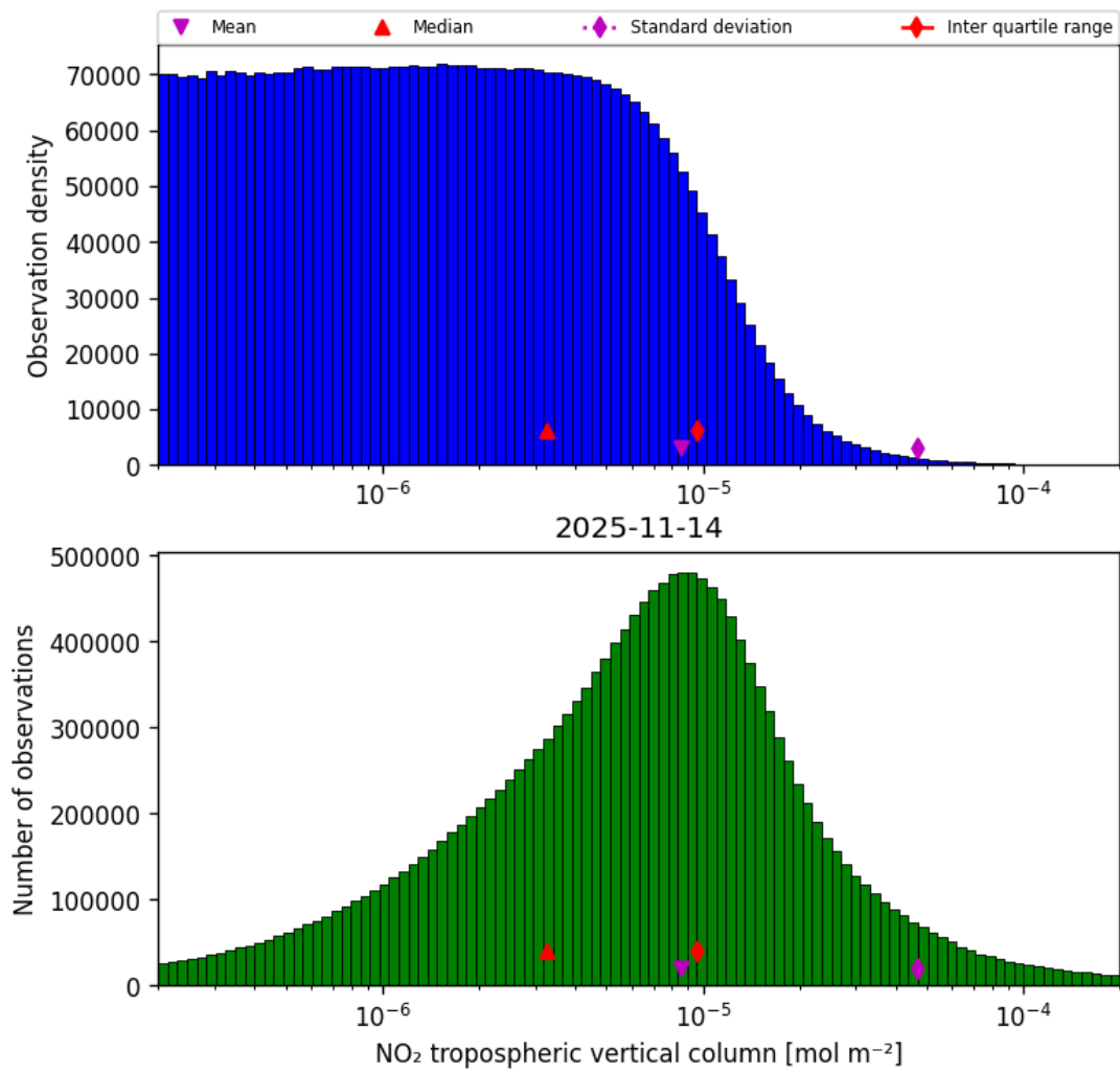
Figure 29: Histogram of “NO 2 tropospheric vertical column” for 2025-11-13 to 2025-11-15
