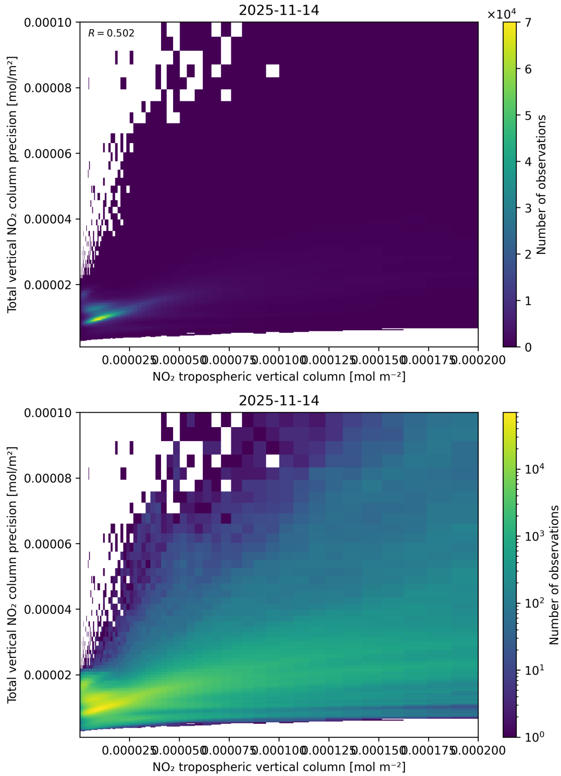
Figure 129: Scatter density plot of “NO 2 tropospheric vertical column” against “Total vertical NO 2 column precision” for 2025-11-13 to 2025-11-15.
