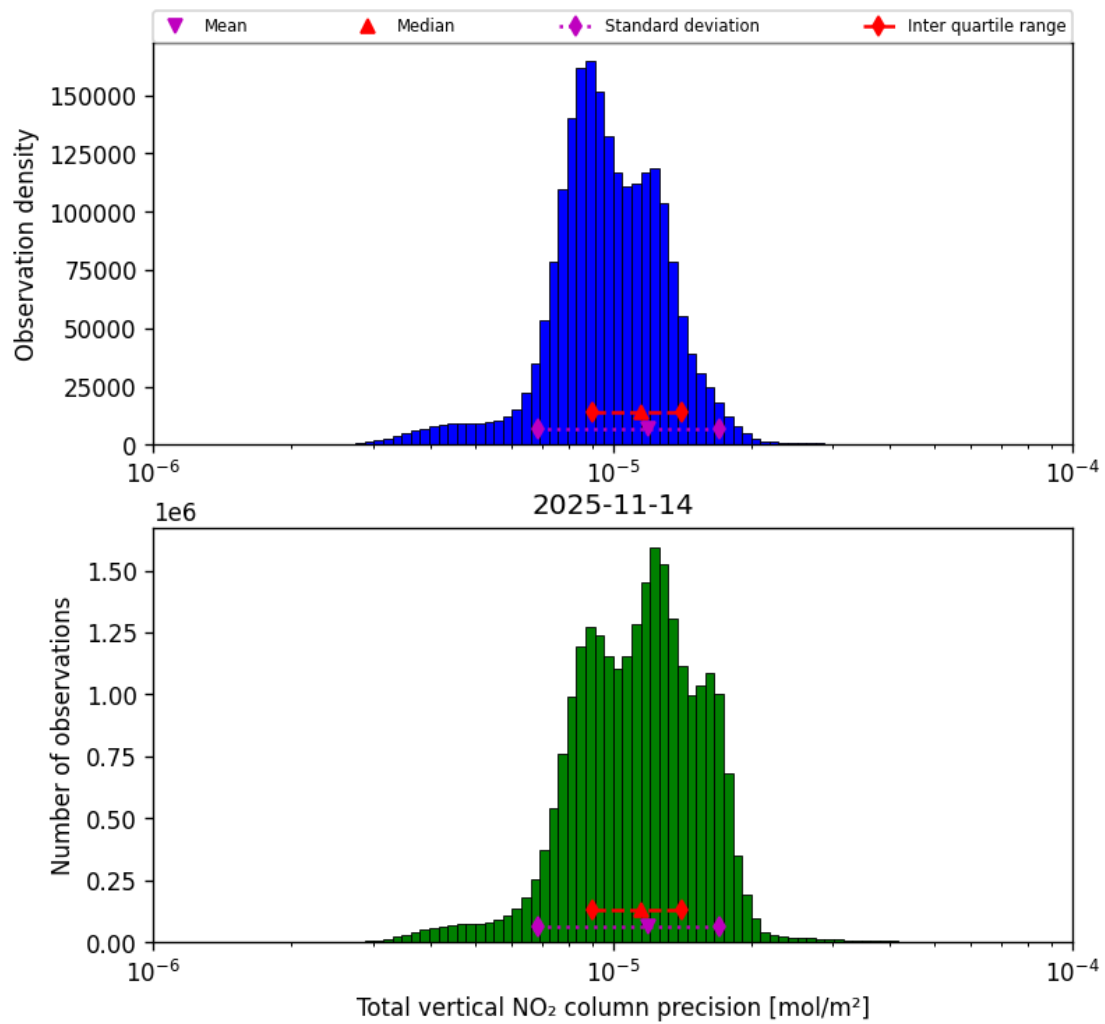
Figure 39: Histogram of “Total vertical NO 2 column precision” for 2025-11-13 to 2025-11-15
