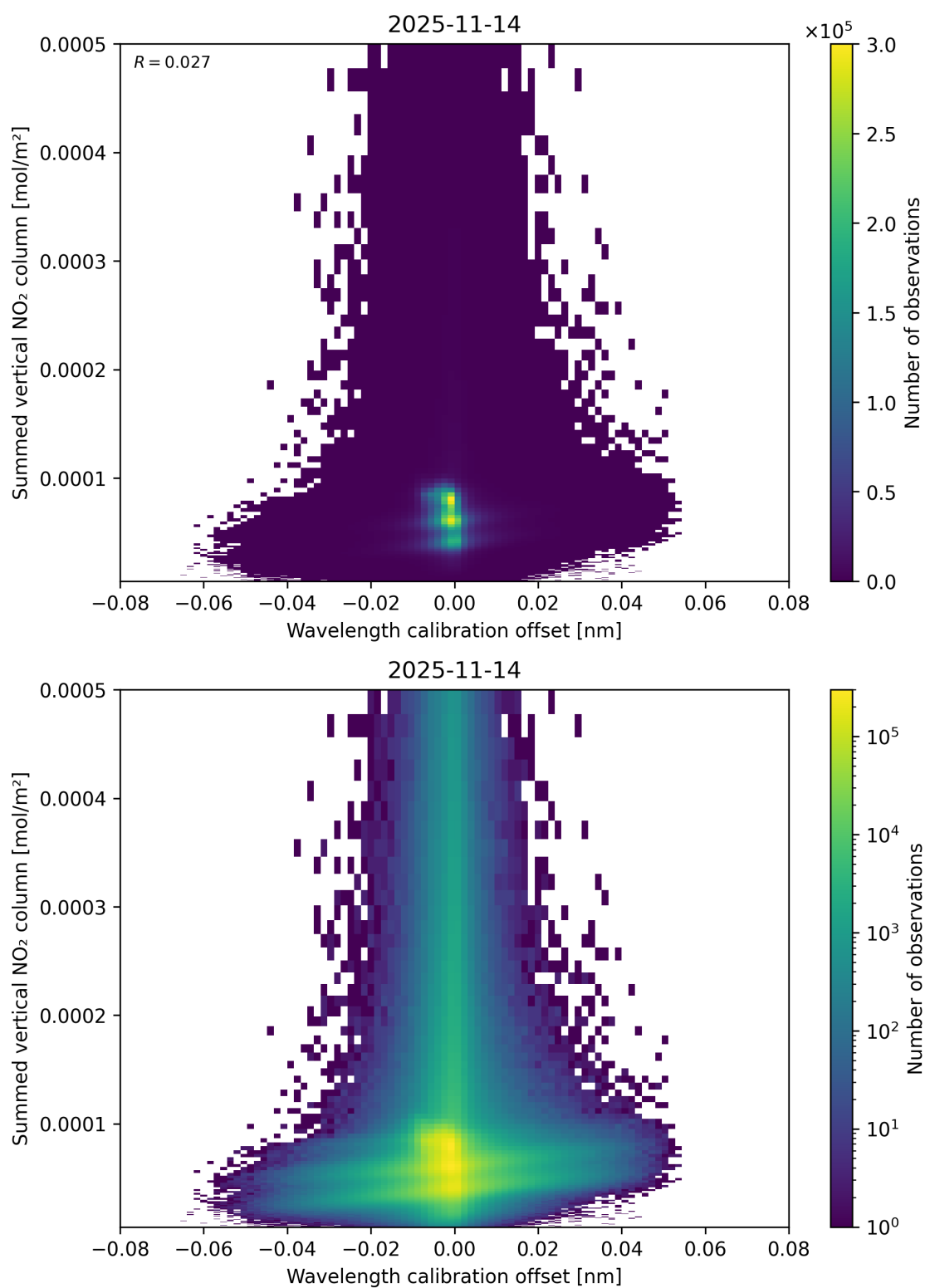
Figure 177: Scatter density plot of “Wavelength calibration offset” against “Summed vertical NO 2 column” for 2025-11-13 to 2025-11-15.
