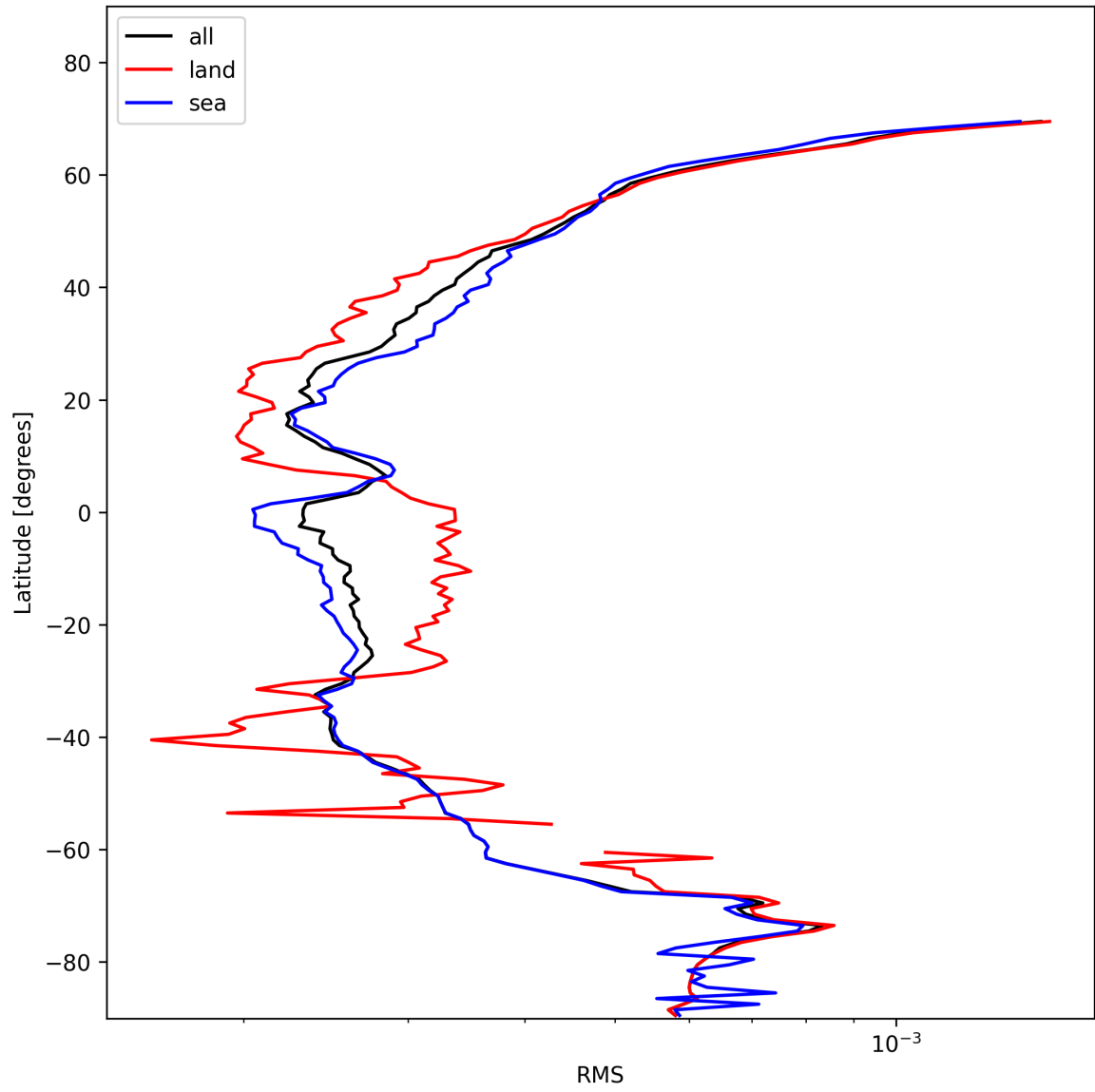
Figure 26: Zonal average of “RMS” for 2025-11-13 to 2025-11-15.
