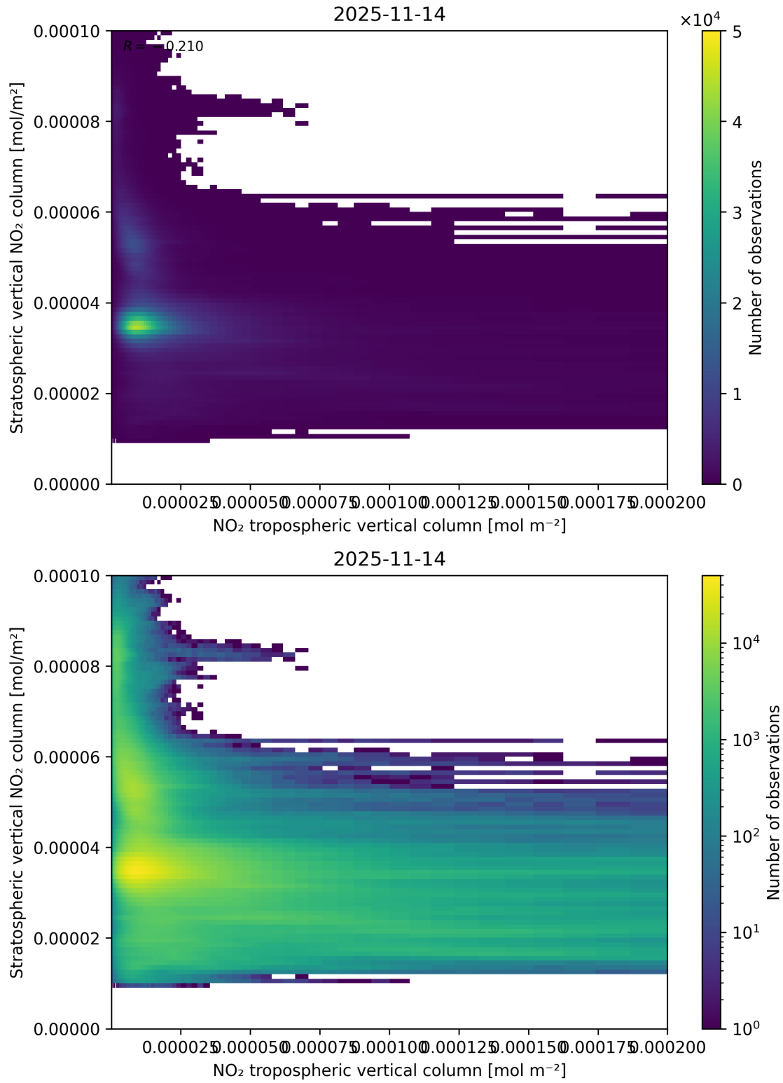
Figure 125: Scatter density plot of “NO 2 tropospheric vertical column” against “Stratospheric vertical NO 2 column” for 2025-11-13 to 2025-11-15.
