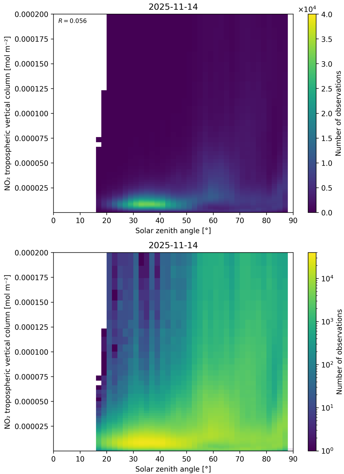
Figure 155: Scatter density plot of “Solar zenith angle” against “NO 2 tropospheric vertical column” for 2025-11-13 to 2025-11-15.
