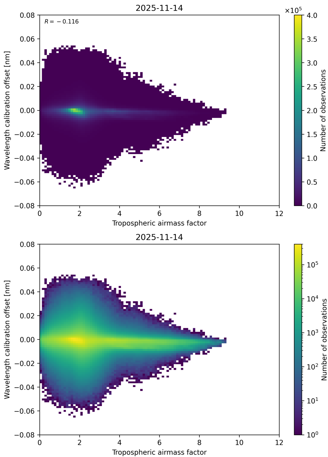
Figure 80: Scatter density plot of “Tropospheric airmass factor” against “Wavelength calibration offset” for 2025-11-13 to 2025-11-15.
