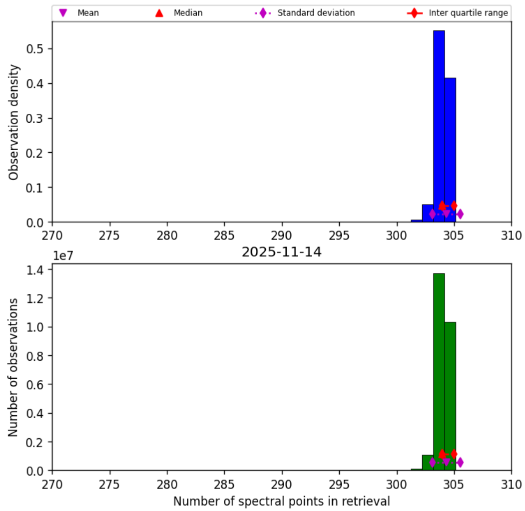
Figure 33: Histogram of “Number of spectral points in retrieval” for 2025-11-13 to 2025-11-15
