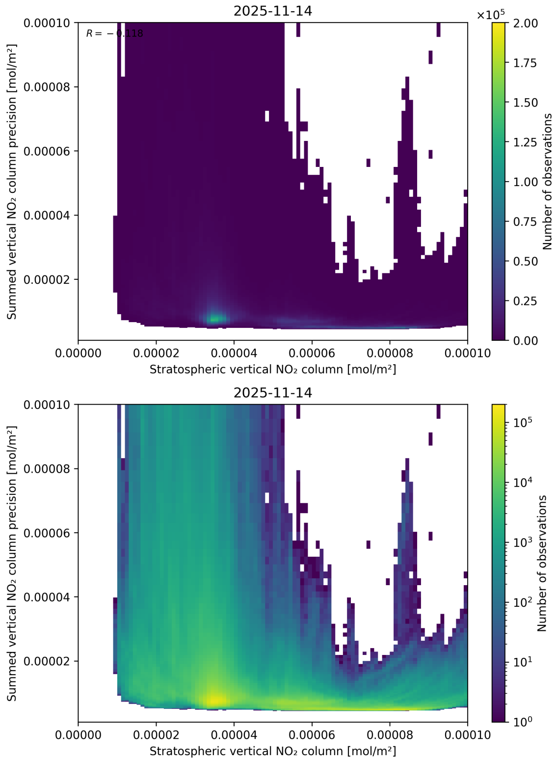
Figure 99: Scatter density plot of “Stratospheric vertical NO 2 column” against “Summed vertical NO 2 column precision” for 2025-11-13 to 2025-11-15.
