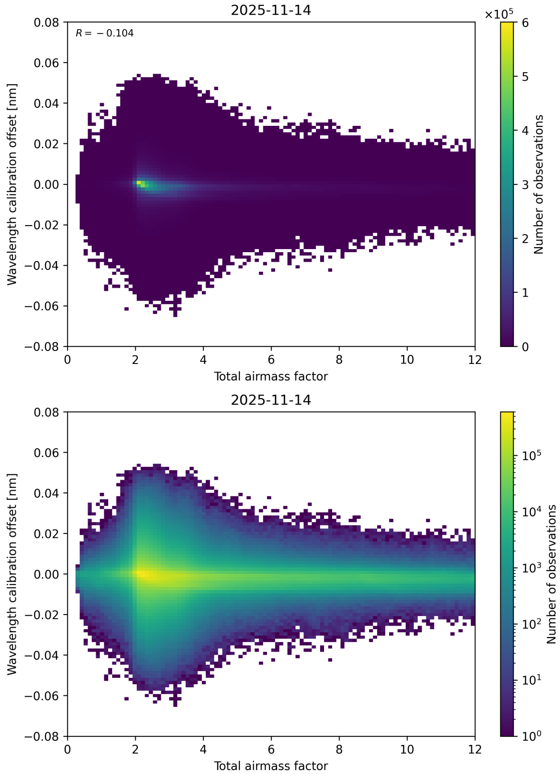
Figure 70: Scatter density plot of “Total airmass factor” against “Wavelength calibration offset” for 2025-11-13 to 2025-11-15.
