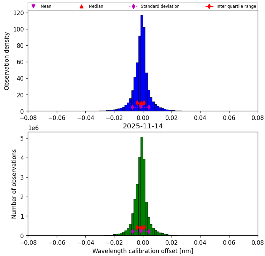
Figure 35: Histogram of “Wavelength calibration offset” for 2025-11-13 to 2025-11-15
