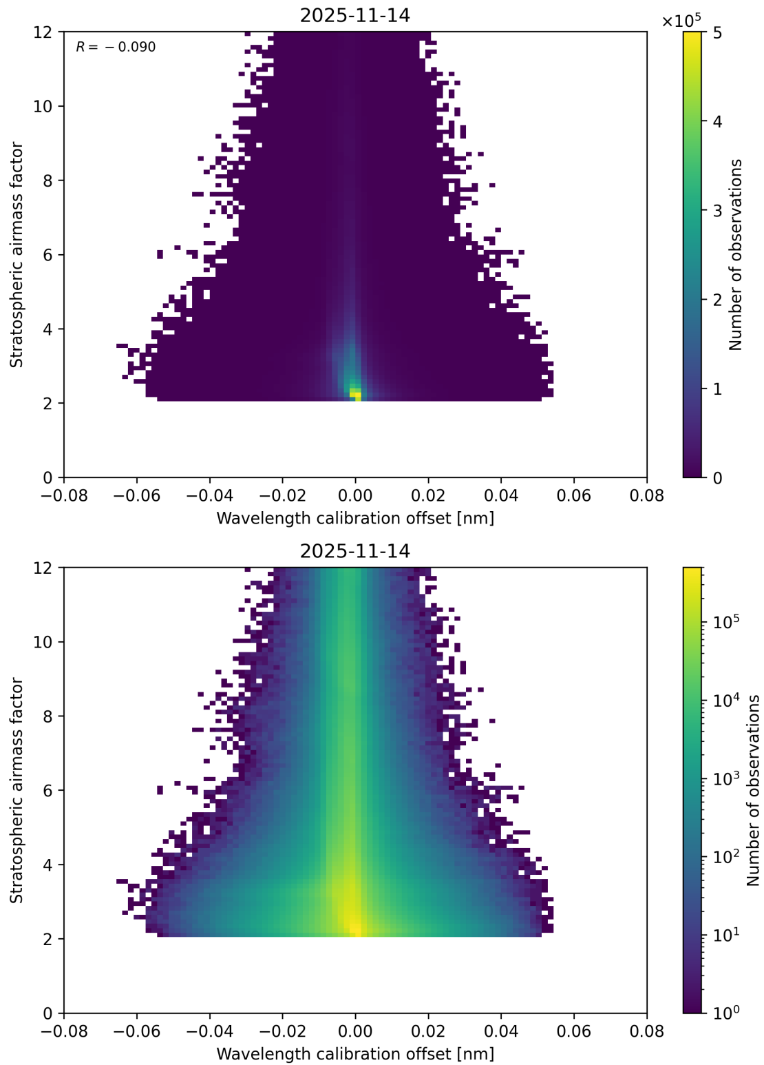
Figure 174: Scatter density plot of “Wavelength calibration offset” against “Stratospheric airmass factor” for 2025-11-13 to 2025-11-15.
