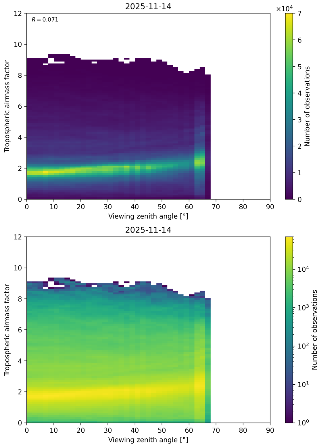
Figure 161: Scatter density plot of “Viewing zenith angle” against “Tropospheric airmass factor” for 2025-11-13 to 2025-11-15.
