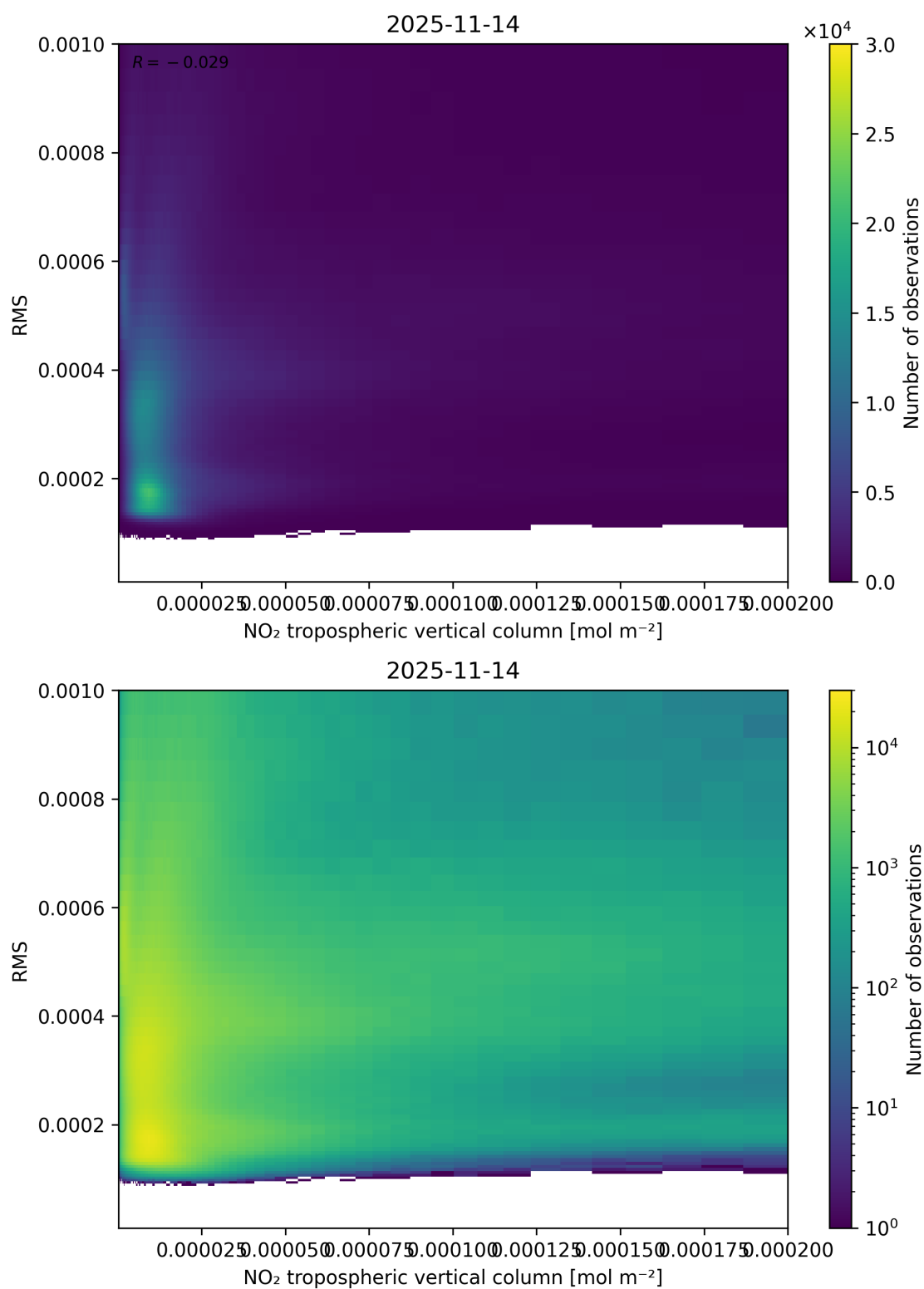
Figure 142: Scatter density plot of “NO 2 tropospheric vertical column” against “RMS” for 2025-11-13 to 2025-11-15.
