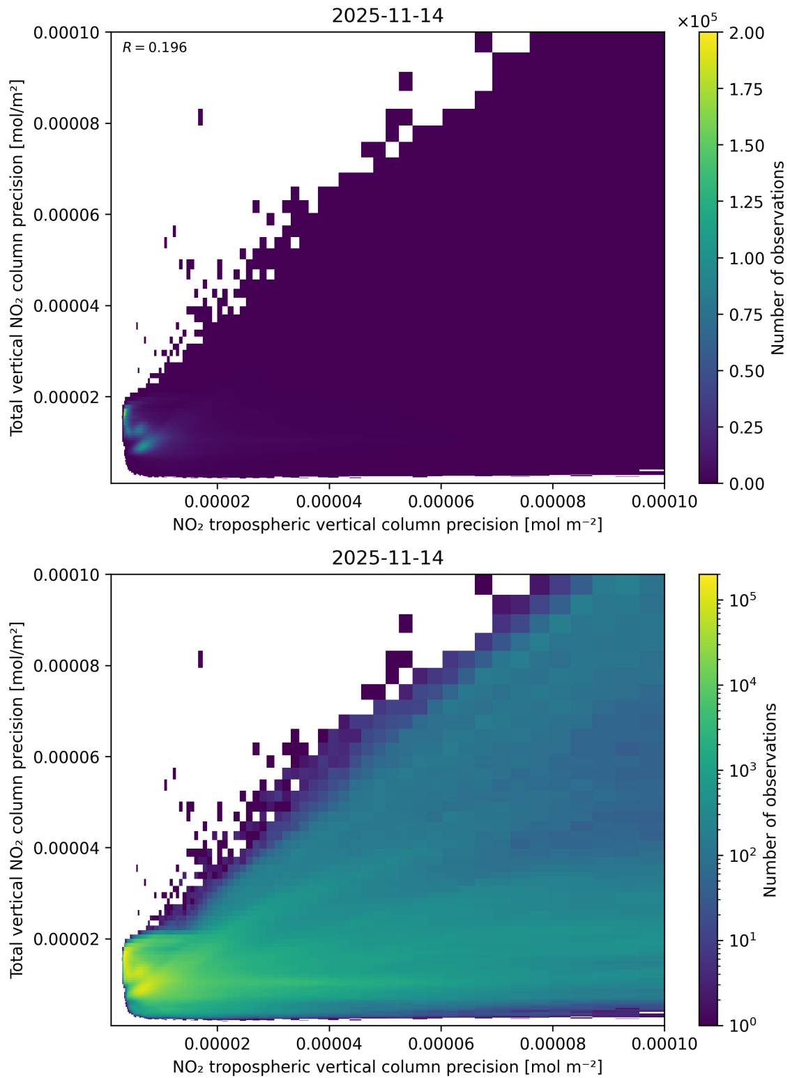
Figure 139: Scatter density plot of “NO 2 tropospheric vertical column precision” against “Total vertical NO 2 column precision” for 2025-11-13 to 2025-11-15.
