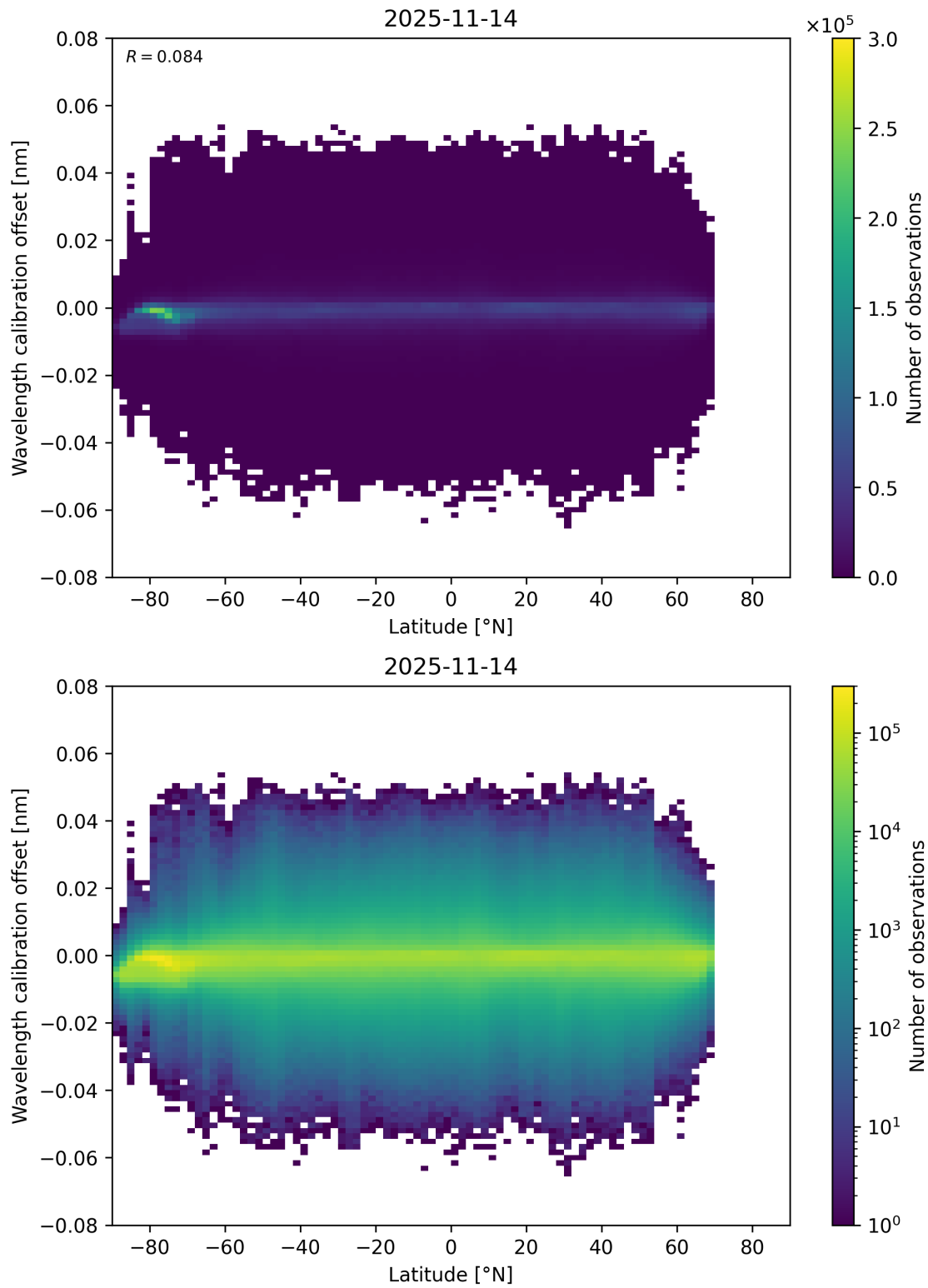
Figure 95: Scatter density plot of “Latitude” against “Wavelength calibration offset” for 2025-11-13 to 2025-11-15.
