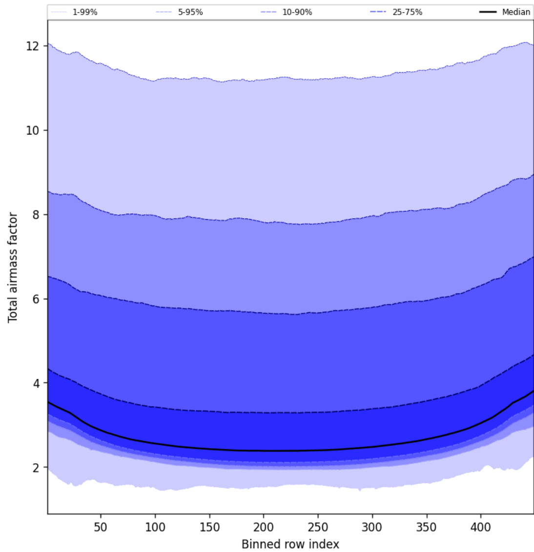
Figure 49: Along track statistics of “Total airmass factor” for 2025-11-13 to 2025-11-15
