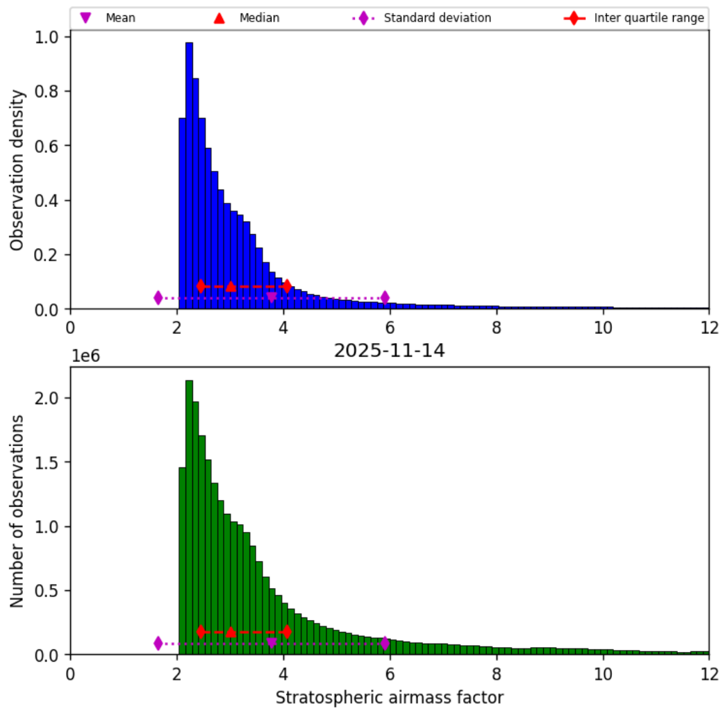
Figure 44: Histogram of “Stratospheric airmass factor” for 2025-11-13 to 2025-11-15
