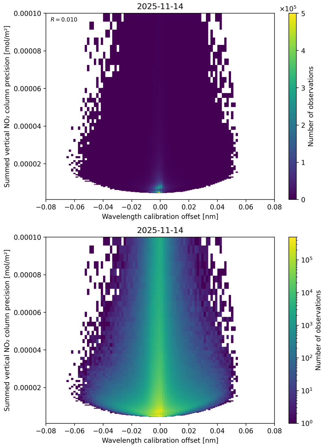
Figure 178: Scatter density plot of “Wavelength calibration offset” against “Summed vertical NO 2 column precision” for 2025-11-13 to 2025-11-15.
