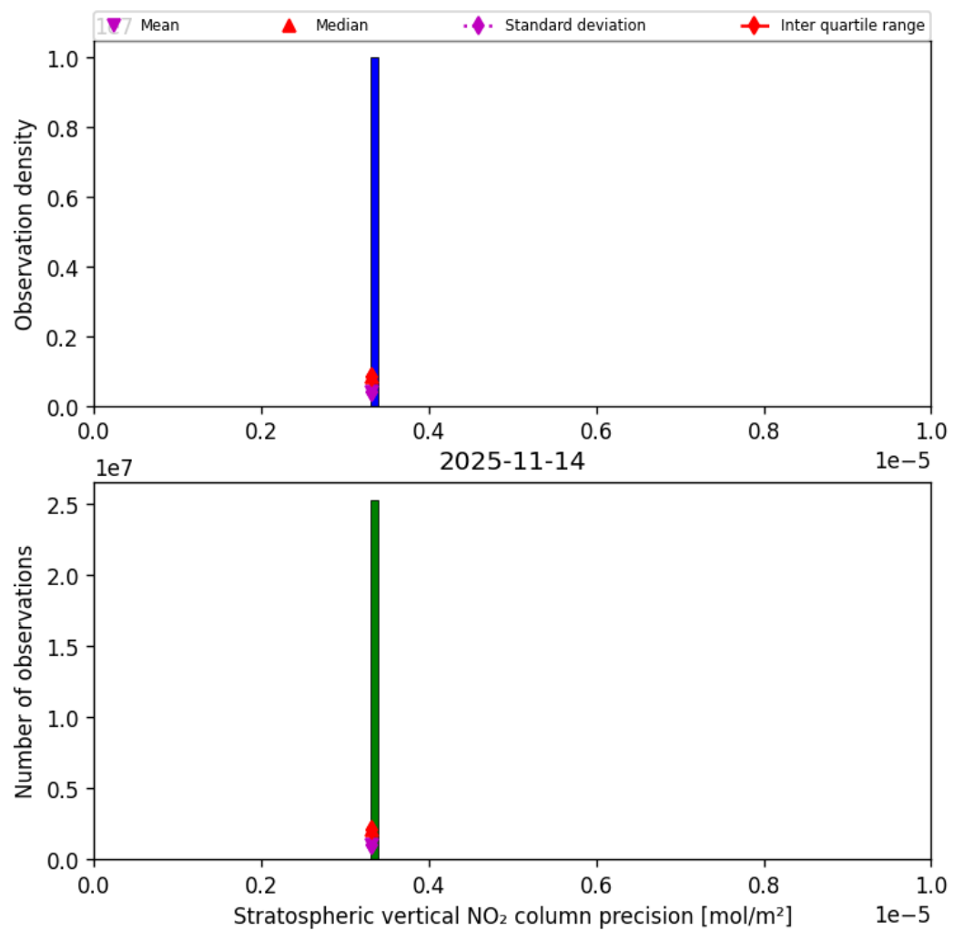
Figure 37: Histogram of “Stratospheric vertical NO 2 column precision” for 2025-11-13 to 2025-11-15
