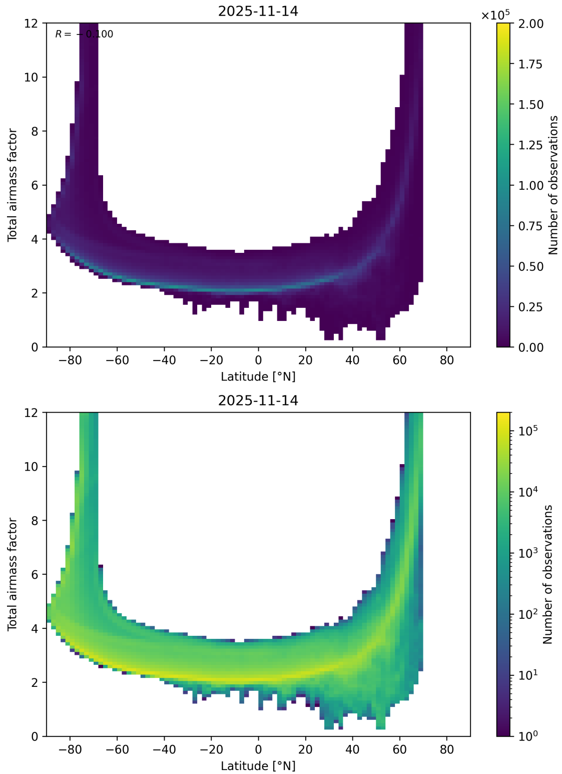
Figure 84: Scatter density plot of “Latitude” against “Total airmass factor” for 2025-11-13 to 2025-11-15.
