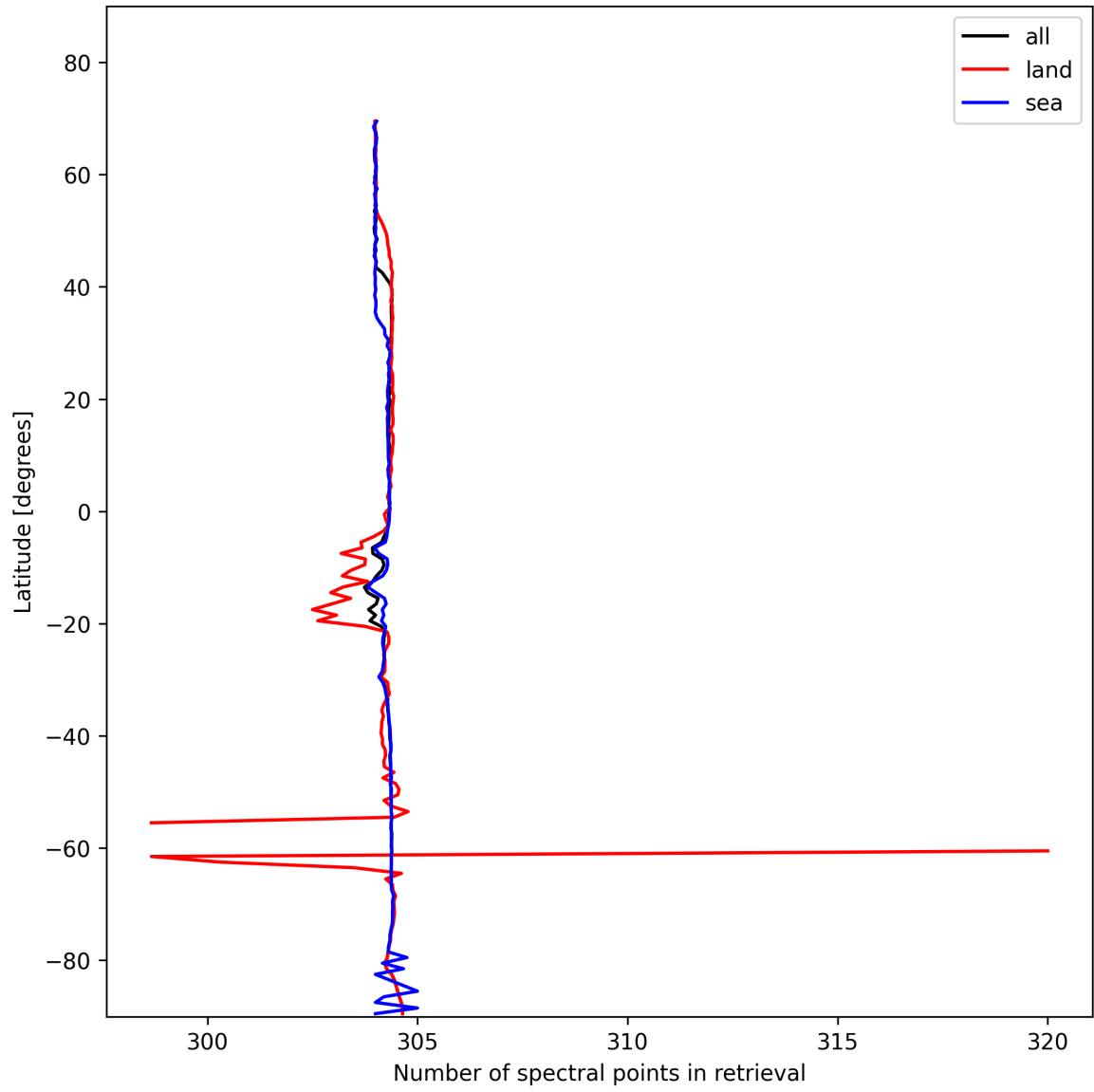
Figure 16: Zonal average of “Number of spectral points in retrieval” for 2025-11-13 to 2025-11-15.
