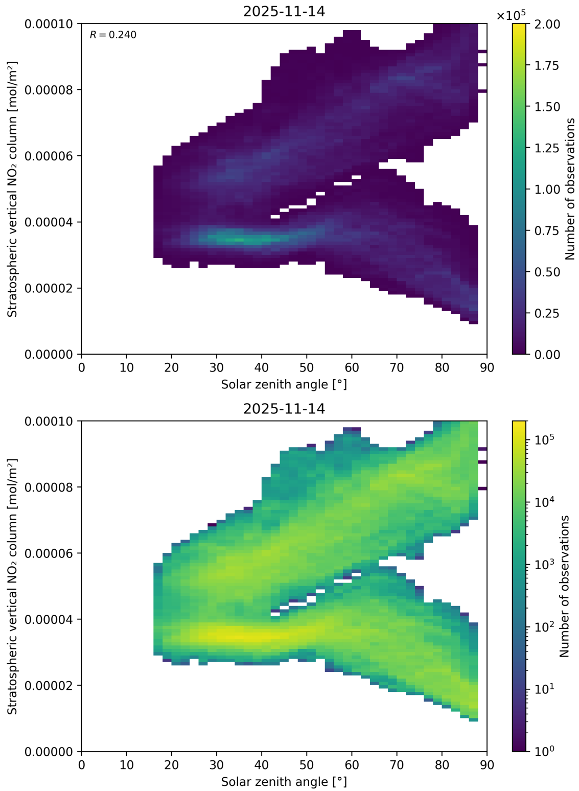
Figure 150: Scatter density plot of “Solar zenith angle” against “Stratospheric vertical NO 2 column” for 2025-11-13 to 2025-11-15.
