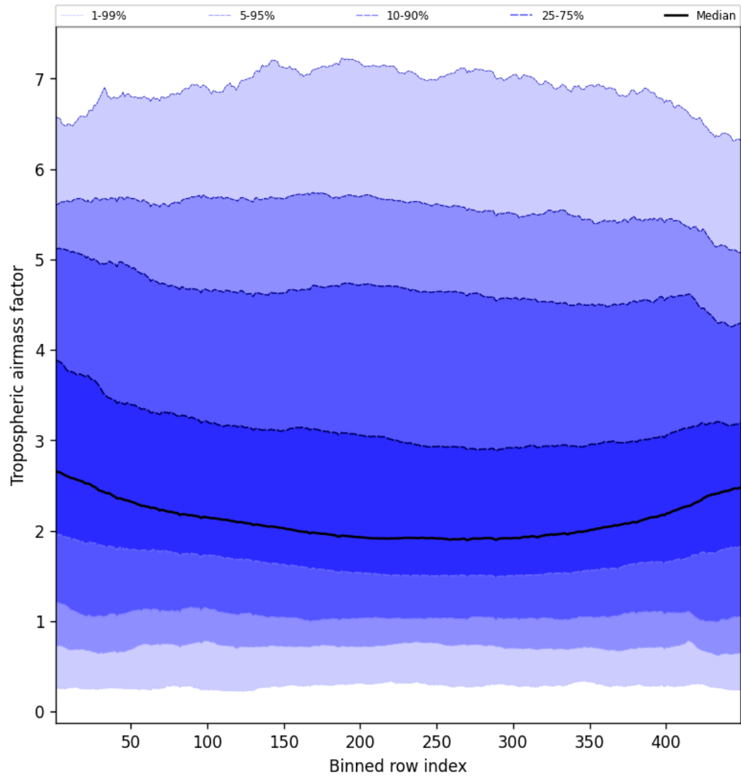
Figure 48: Along track statistics of “Tropospheric airmass factor” for 2025-11-13 to 2025-11-15
