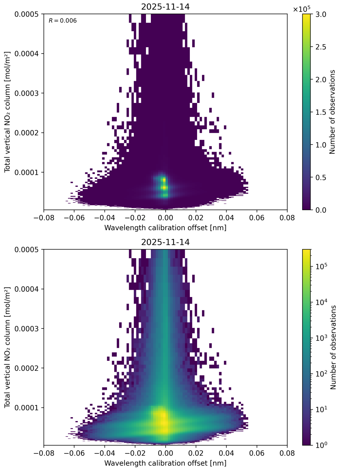
Figure 179: Scatter density plot of “Wavelength calibration offset” against “Total vertical NO 2 column” for 2025-11-13 to 2025-11-15.
