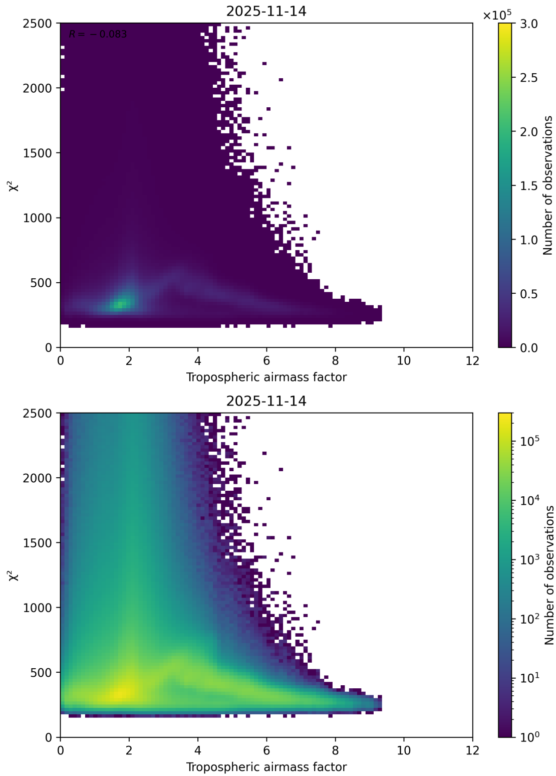
Figure 73: Scatter density plot of “Tropospheric airmass factor” against “ \chi^2 ” for 2025-11-13 to 2025-11-15.
