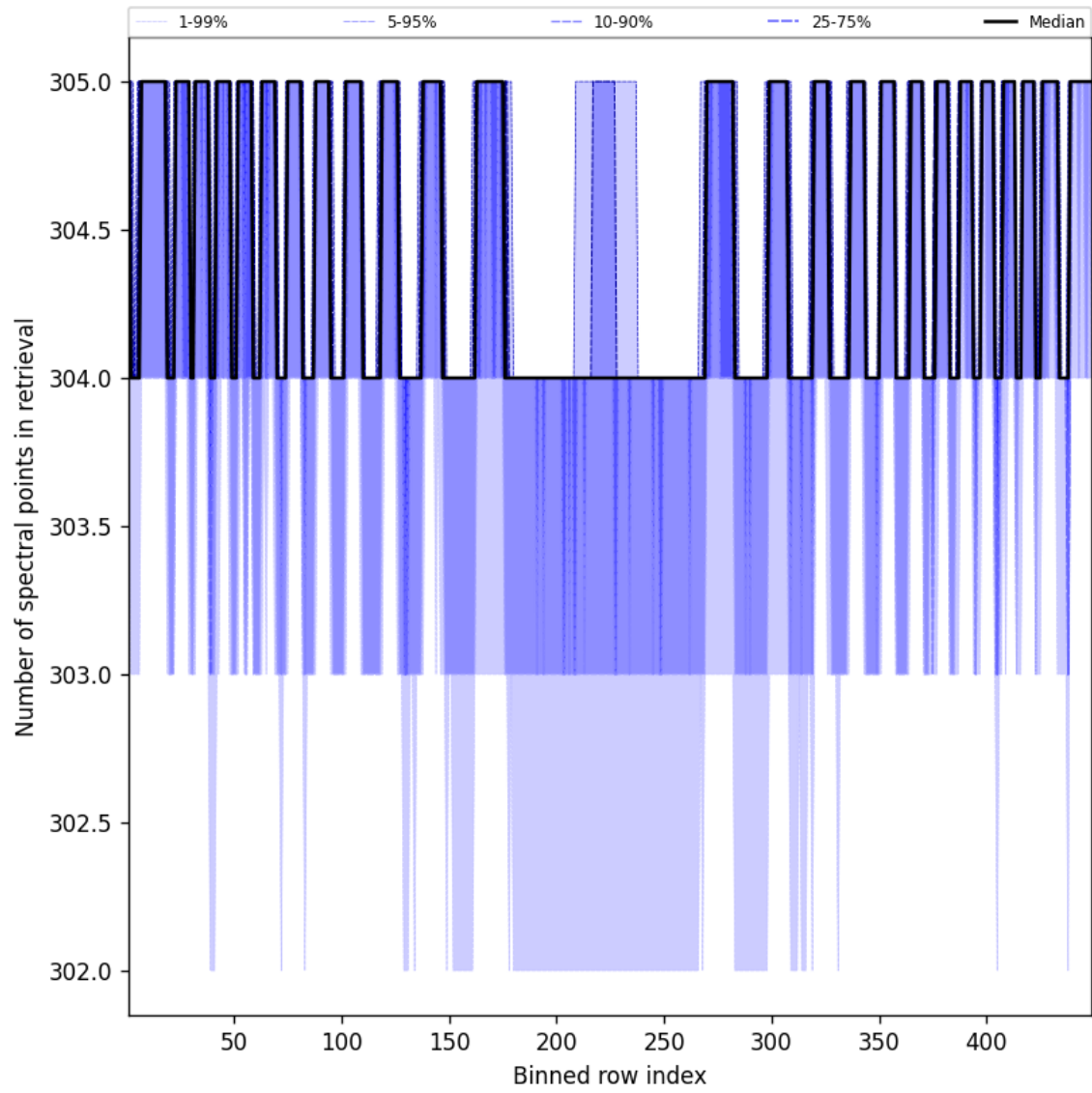
Figure 50: Along track statistics of “Number of spectral points in retrieval” for 2025-11-13 to 2025-11-15
