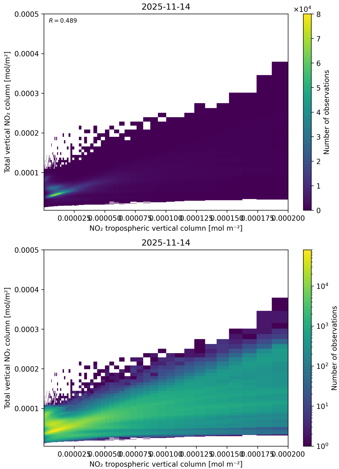
Figure 128: Scatter density plot of “NO 2 tropospheric vertical column” against “Total vertical NO 2 column” for 2025-11-13 to 2025-11-15.
