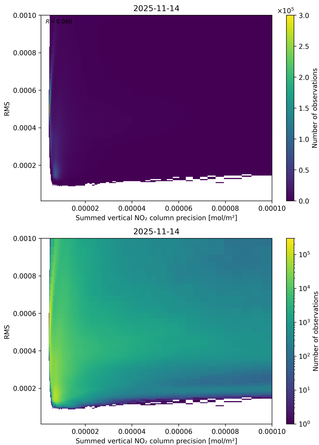
Figure 108: Scatter density plot of “Summed vertical NO 2 column precision” against “RMS” for 2025-11-13 to 2025-11-15.
