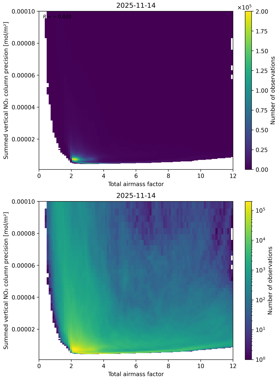
Figure 66: Scatter density plot of “Total airmass factor” against “Summed vertical NO 2 column precision” for 2025-11-13 to 2025-11-15.
