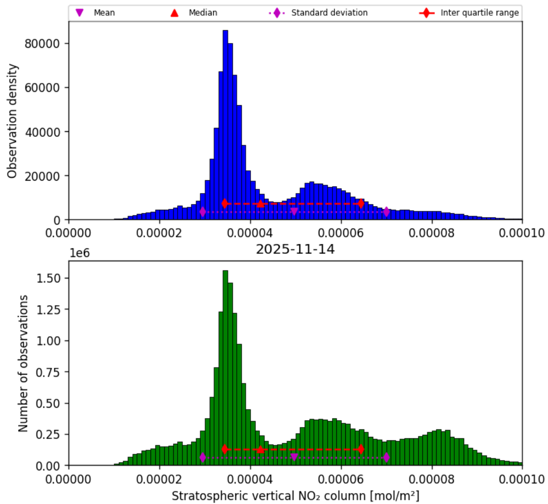
Figure 36: Histogram of “Stratospheric vertical NO 2 column” for 2025-11-13 to 2025-11-15
