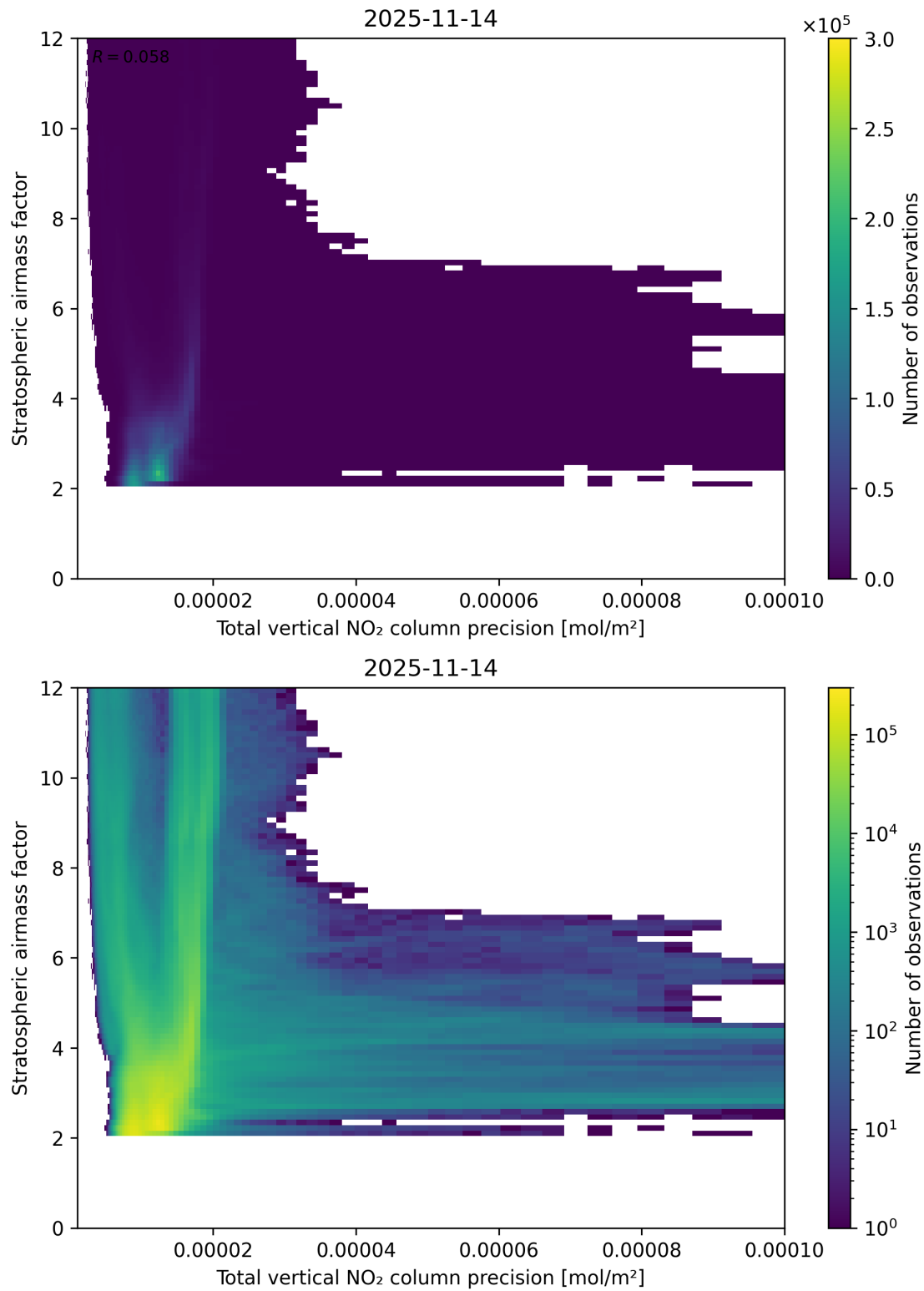
Figure 115: Scatter density plot of “Total vertical NO 2 column precision” against “Stratospheric air mass factor” for 2025-11-13 to 2025-11-15.
