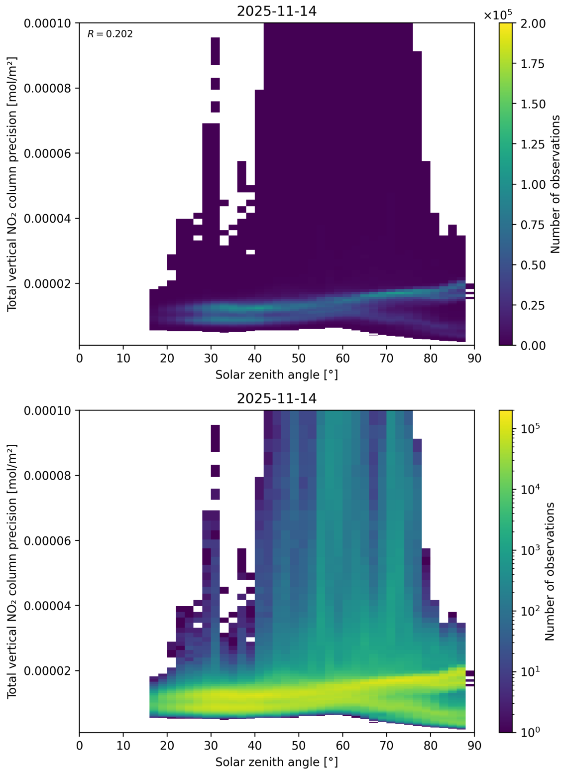
Figure 154: Scatter density plot of “Solar zenith angle” against “Total vertical NO 2 column precision” for 2025-11-13 to 2025-11-15.
