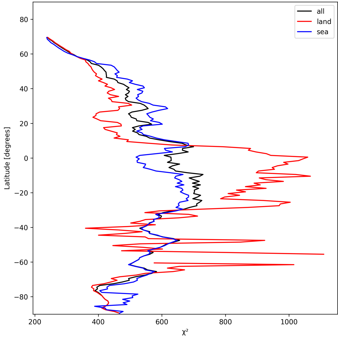
Figure 25: Zonal average of “ \chi^2 ” for 2025-11-13 to 2025-11-15.
