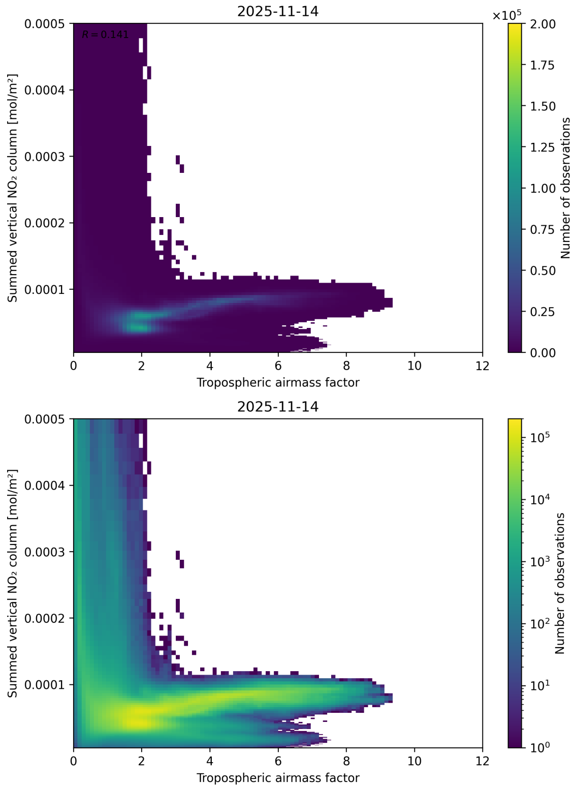
Figure 75: Scatter density plot of “Tropospheric airmass factor” against “Summed vertical NO 2 column” for 2025-11-13 to 2025-11-15.
