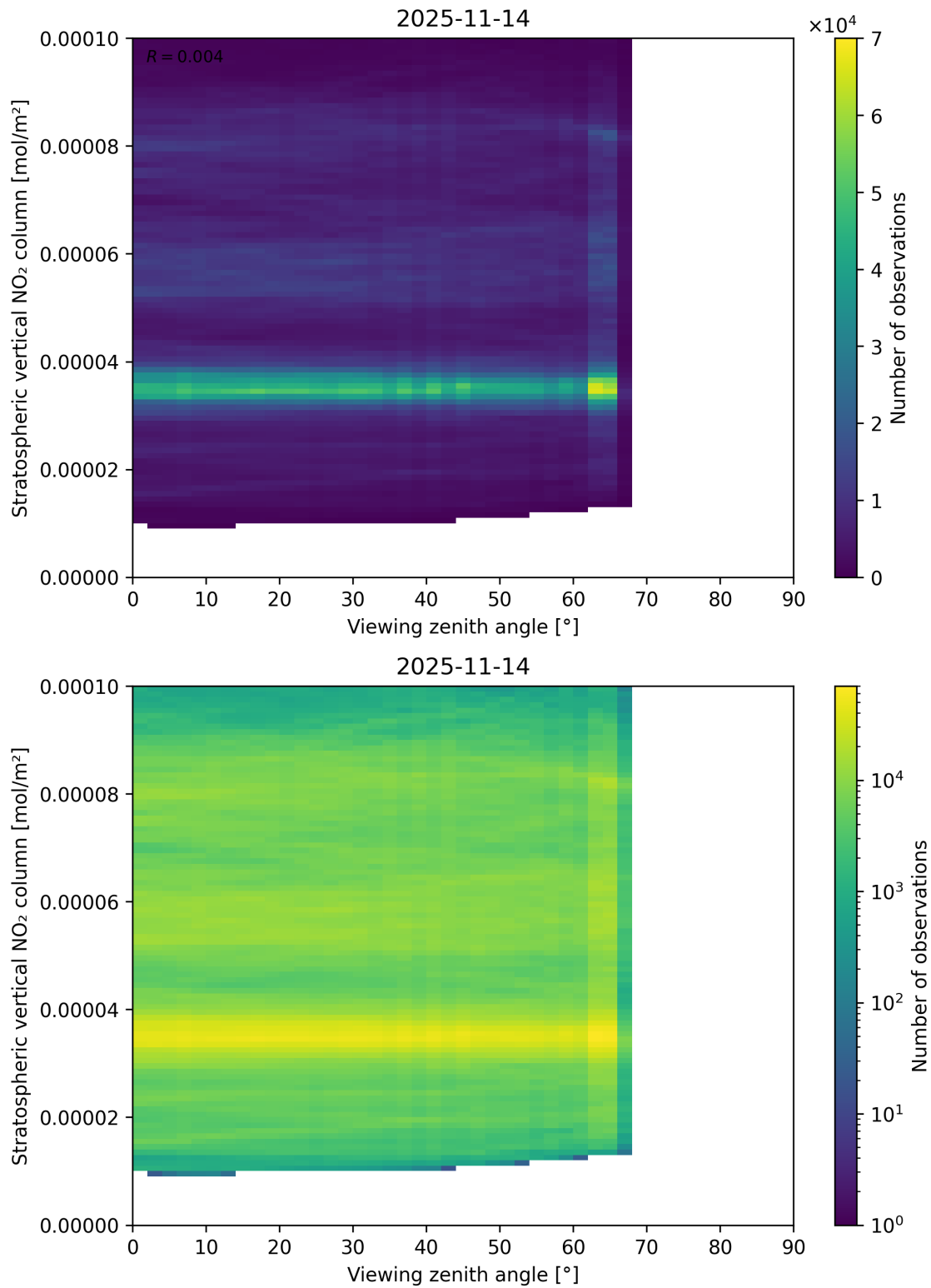
Figure 164: Scatter density plot of “Viewing zenith angle” against “Stratospheric vertical NO 2 column” for 2025-11-13 to 2025-11-15.
