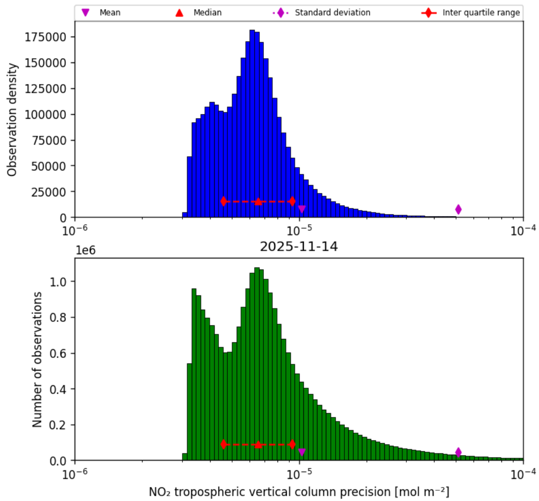
Figure 30: Histogram of “NO 2 tropospheric vertical column precision” for 2025-11-13 to 2025-11-15
