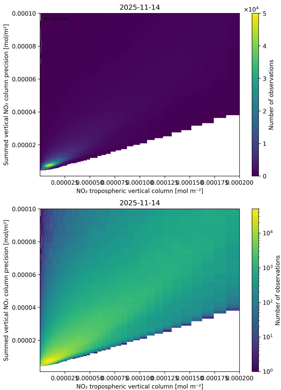
Figure 127: Scatter density plot of “NO 2 tropospheric vertical column” against “Summed vertical NO 2 column precision” for 2025-11-13 to 2025-11-15.
