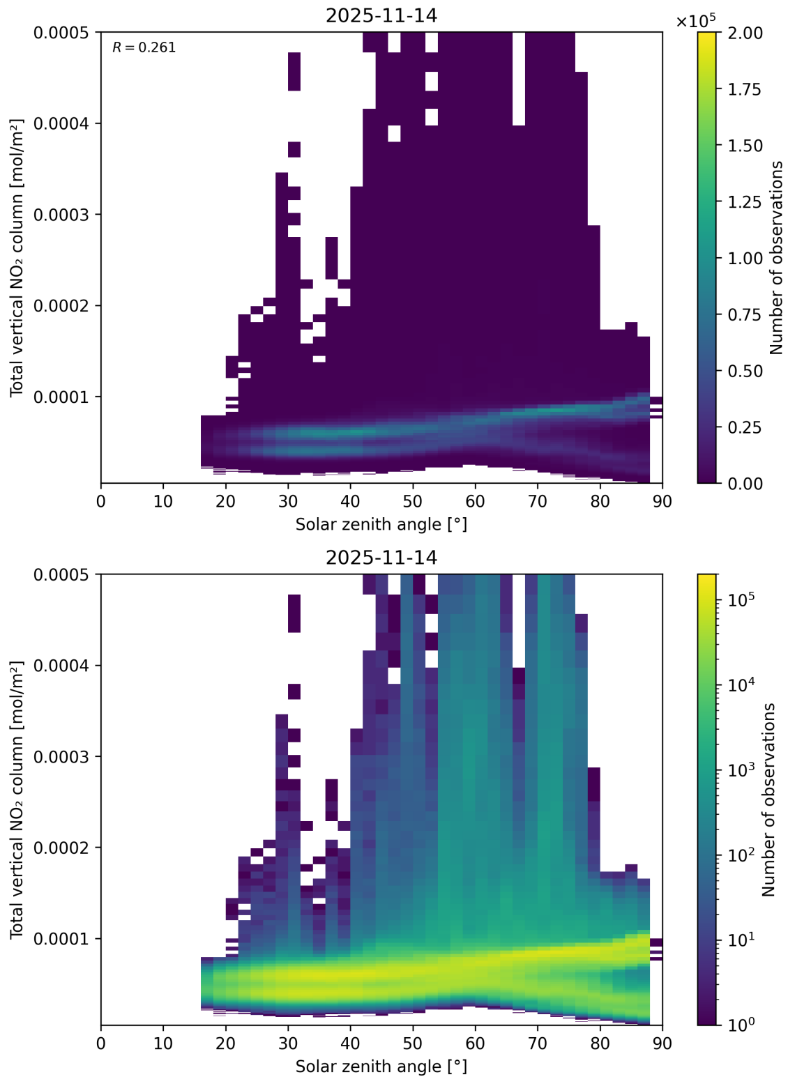
Figure 153: Scatter density plot of “Solar zenith angle” against “Total vertical NO 2 column” for 2025-11-13 to 2025-11-15.
