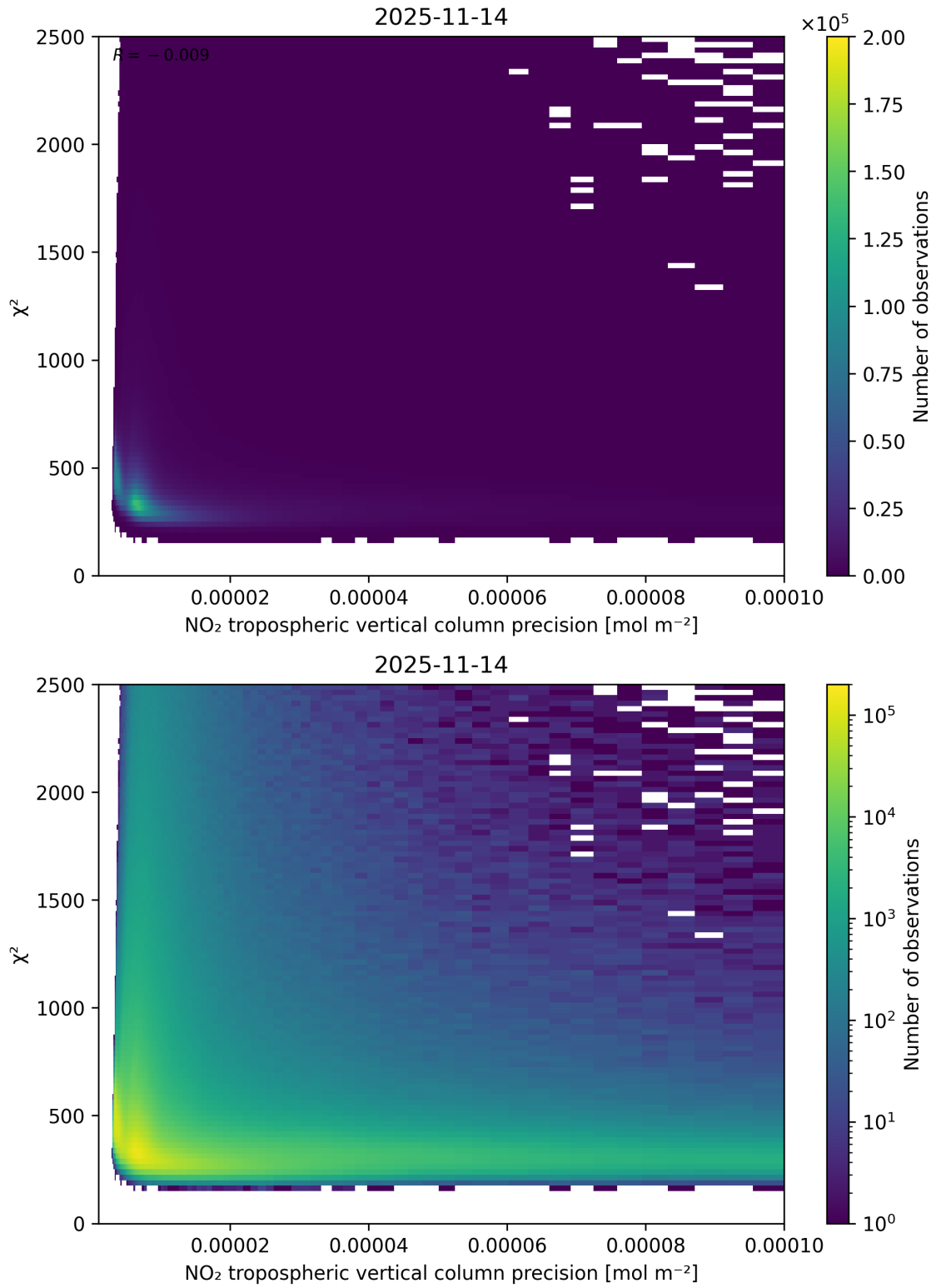
Figure 134: Scatter density plot of “NO 2 tropospheric vertical column precision” against “ \chi^2 ” for 2025-11-13 to 2025-11-15.
