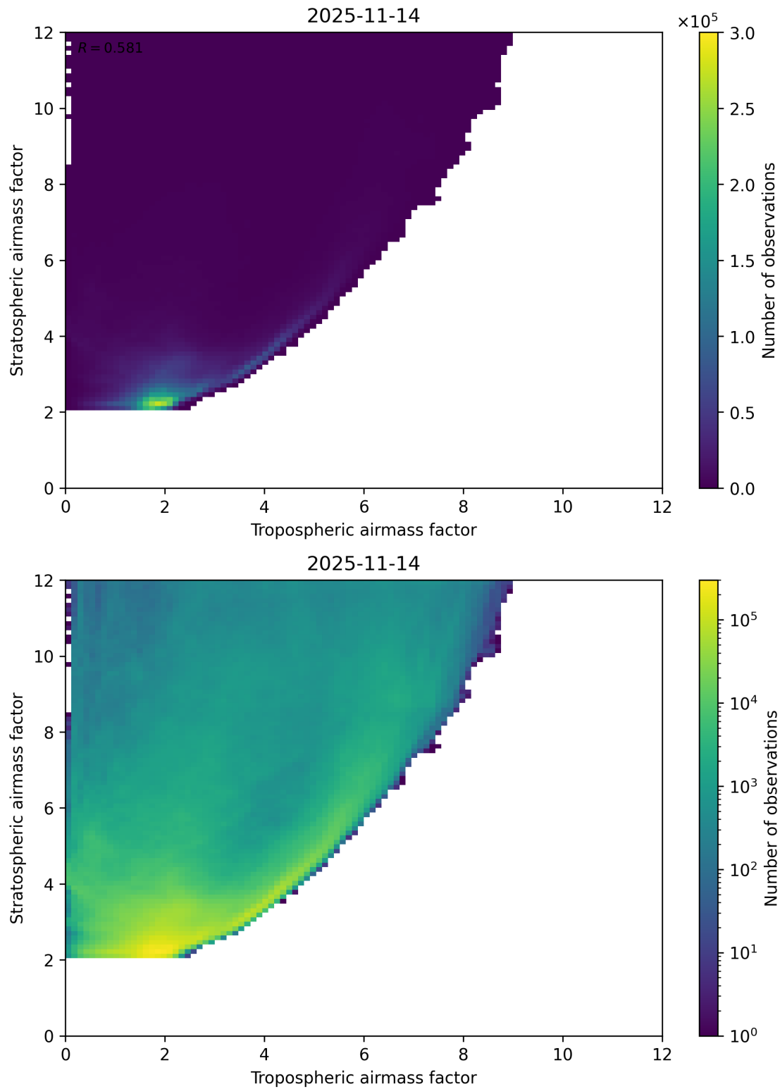
Figure 71: Scatter density plot of “Tropospheric airmass factor” against “Stratospheric airmass factor” for 2025-11-13 to 2025-11-15.
