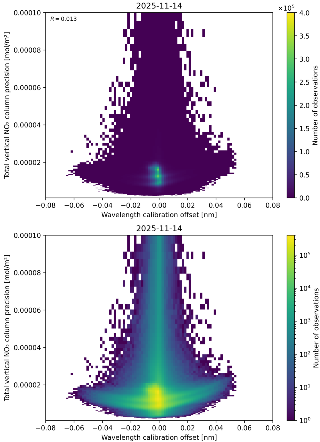
Figure 180: Scatter density plot of “Wavelength calibration offset” against “Total vertical NO 2 column precision” for 2025-11-13 to 2025-11-15.
