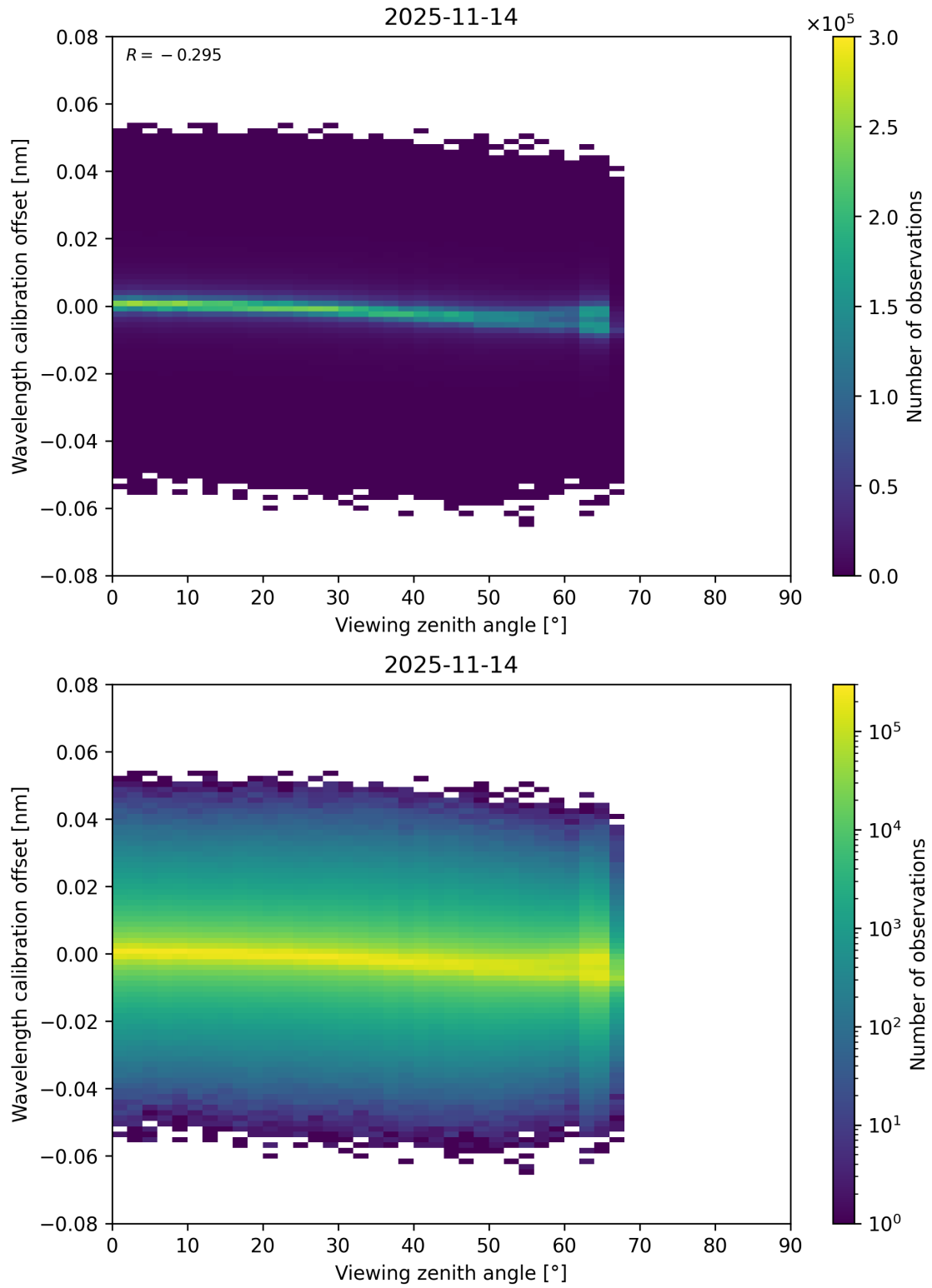
Figure 173: Scatter density plot of “Viewing zenith angle” against “Wavelength calibration offset” for 2025-11-13 to 2025-11-15.
