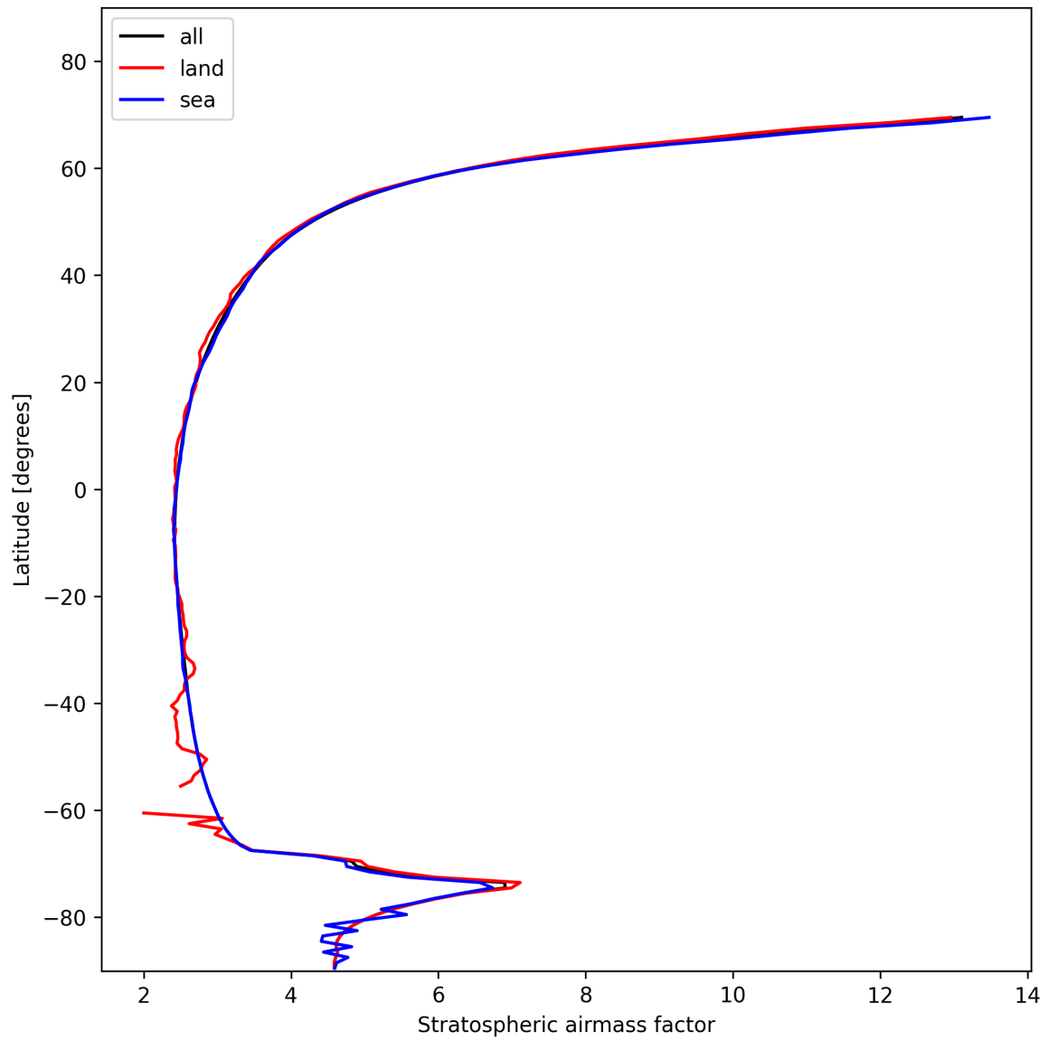
Figure 27: Zonal average of “Stratospheric airmass factor” for 2025-11-13 to 2025-11-15.
