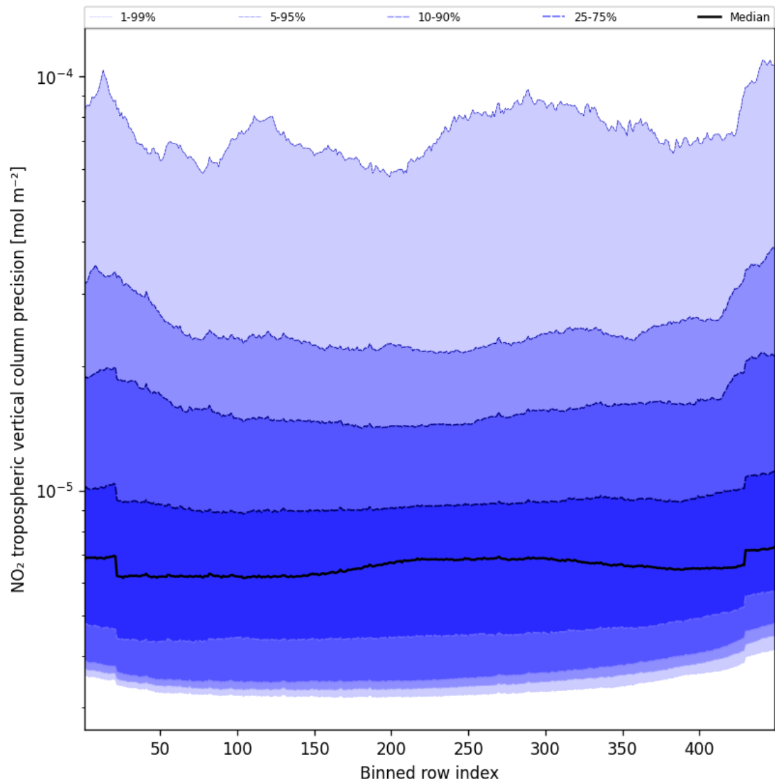
Figure 47: Along track statistics of “NO 2 tropospheric vertical column precision” for 2025-11-13 to 2025-11-15
