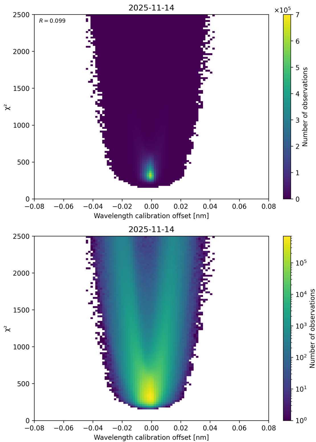
Figure 175: Scatter density plot of “Wavelength calibration offset” against “ \chi^2 ” for 2025-11-13 to 2025-11-15.
