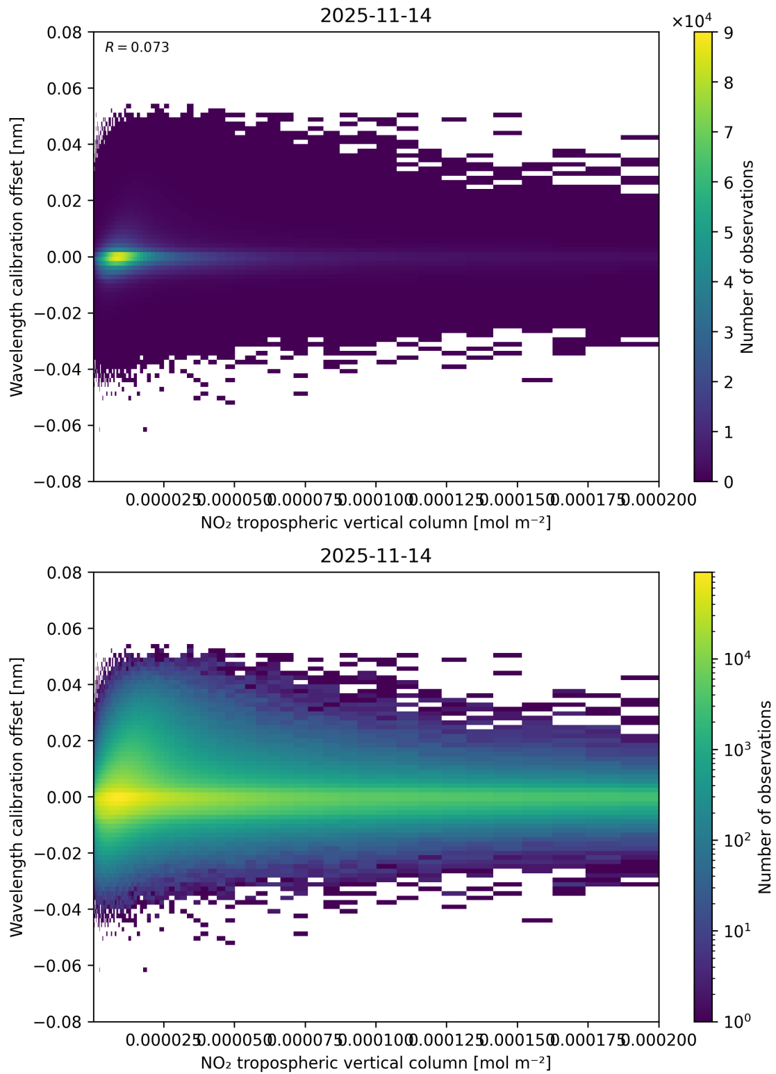
Figure 143: Scatter density plot of “NO 2 tropospheric vertical column” against “Wavelength calibration offset” for 2025-11-13 to 2025-11-15.
