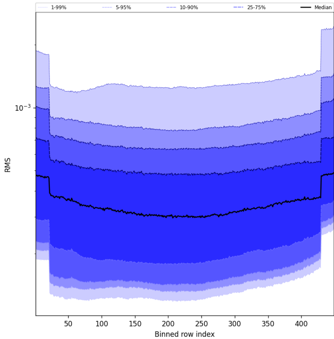
Figure 60: Along track statistics of “RMS” for 2025-11-13 to 2025-11-15
