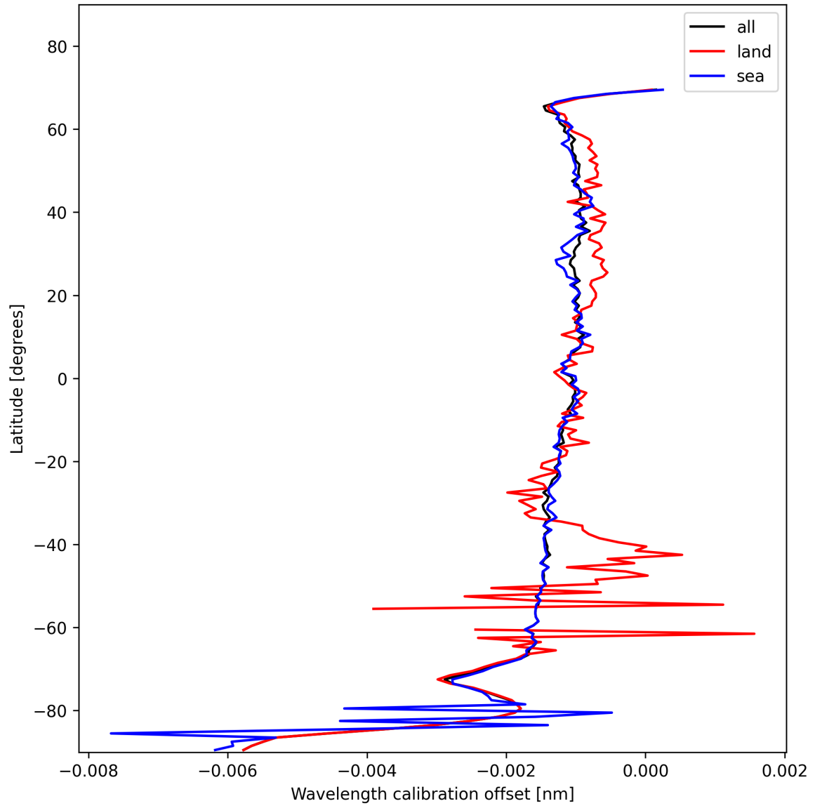
Figure 18: Zonal average of “Wavelength calibration offset” for 2025-11-13 to 2025-11-15.
