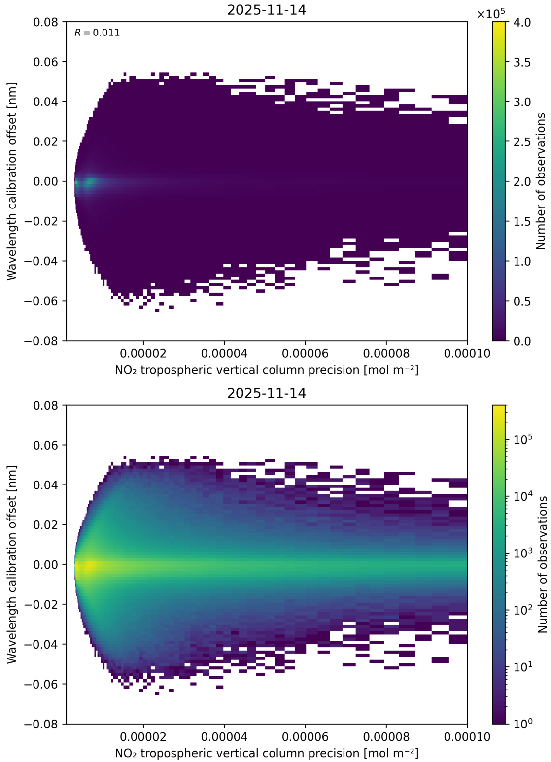
Figure 141: Scatter density plot of “NO 2 tropospheric vertical column precision” against “Wavelength calibration offset” for 2025-11-13 to 2025-11-15.
