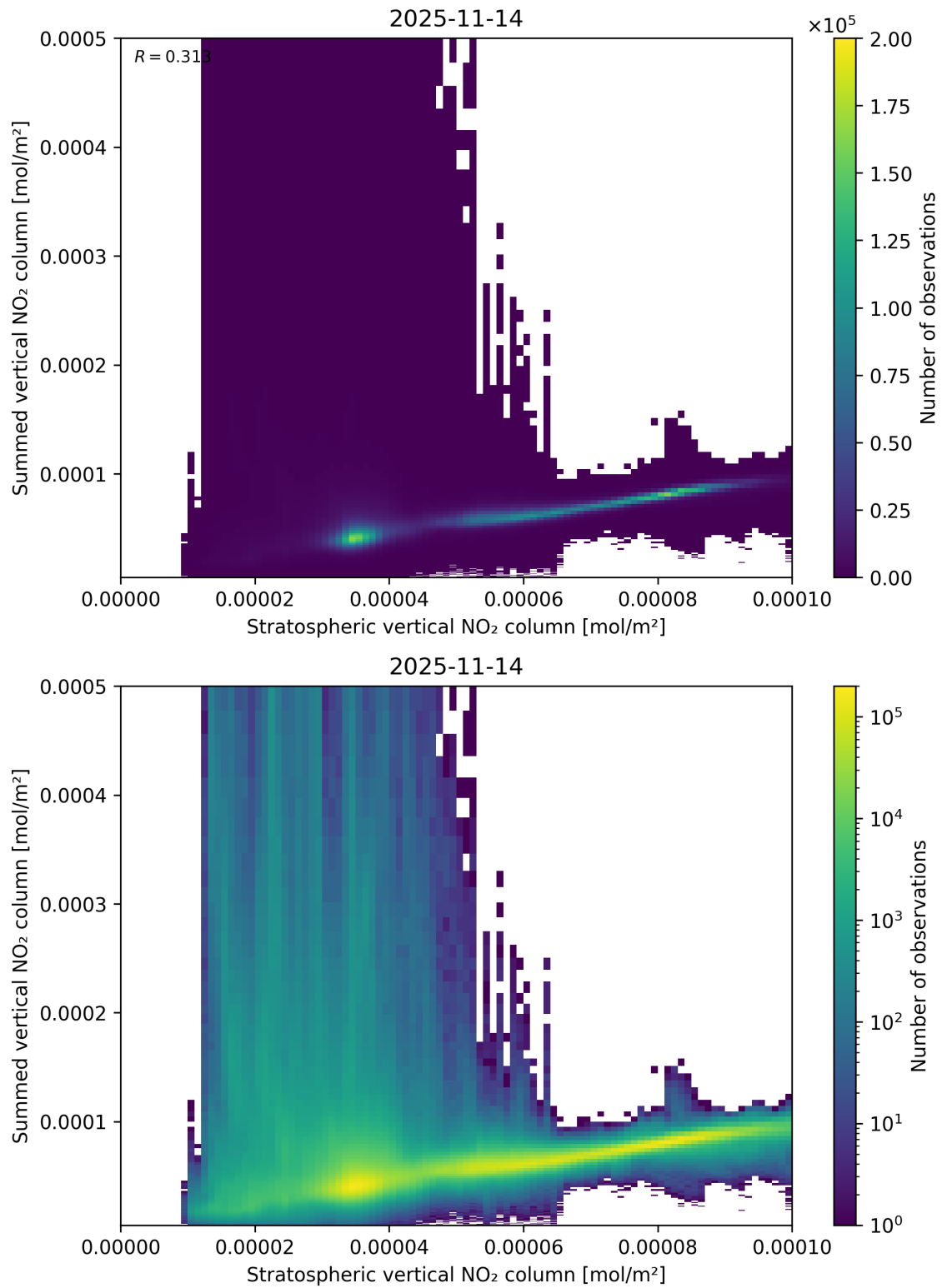
Figure 98: Scatter density plot of “Stratospheric vertical NO 2 column” against “Summed vertical NO 2 column” for 2025-11-13 to 2025-11-15.
