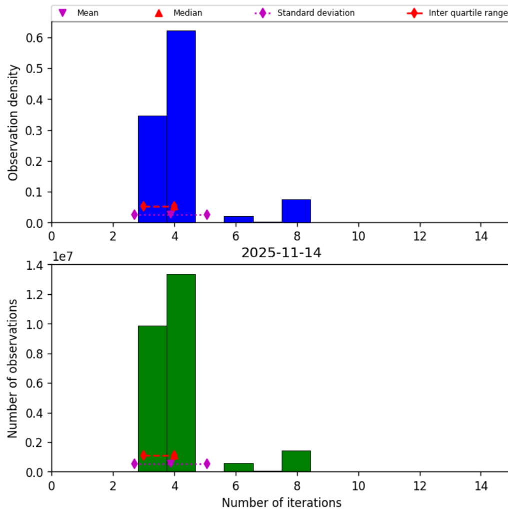
Figure 34: Histogram of “Number of iterations” for 2025-11-13 to 2025-11-15
