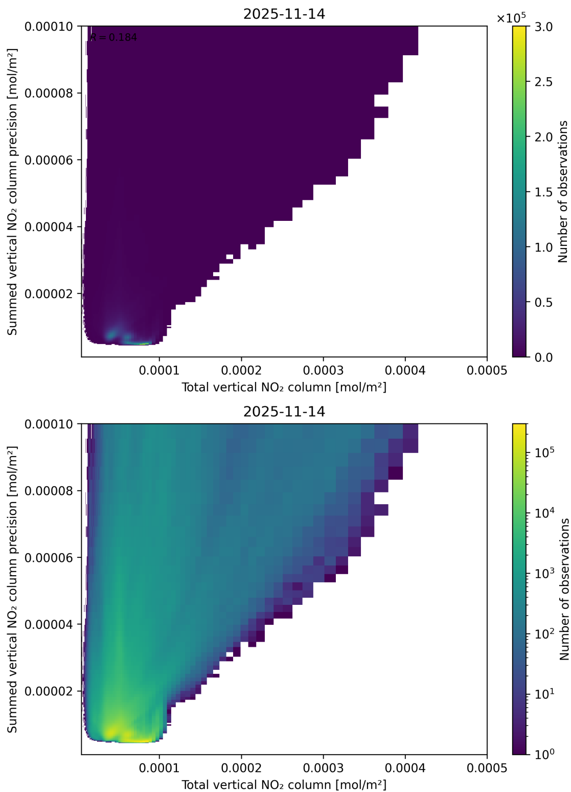
Figure 113: Scatter density plot of “Total vertical NO 2 column” against “Summed vertical NO 2 column precision” for 2025-11-13 to 2025-11-15.
