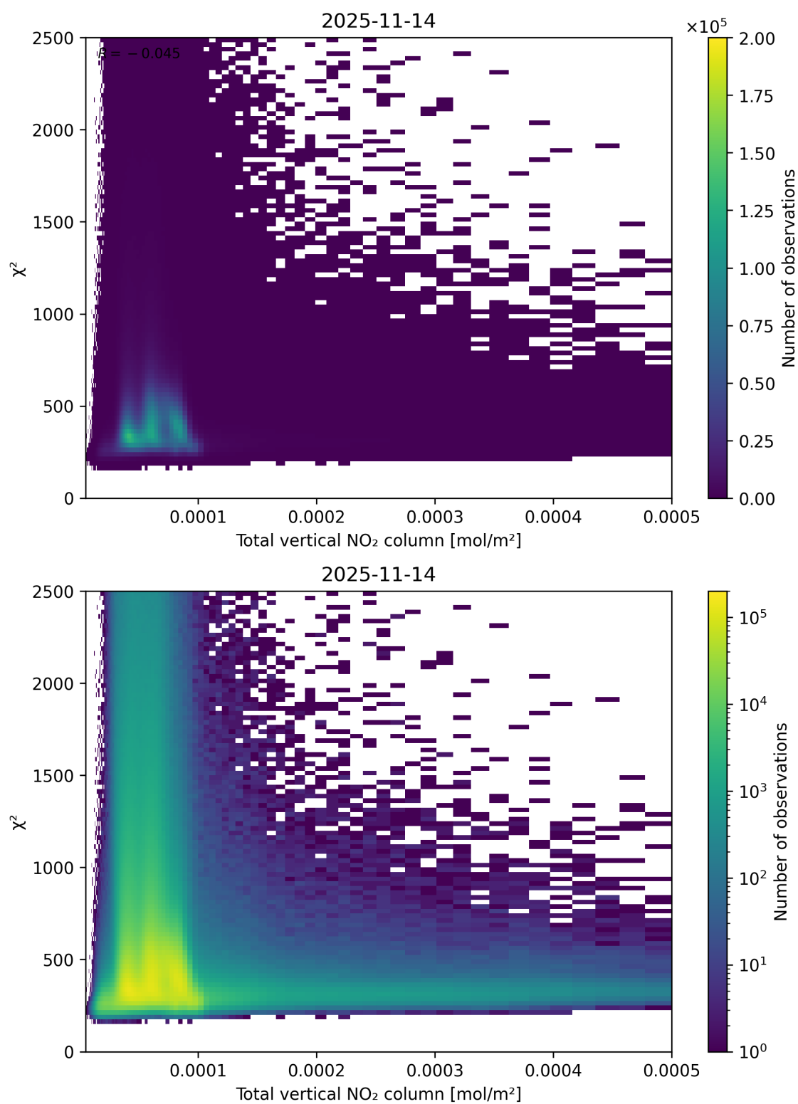
Figure 111: Scatter density plot of “Total vertical NO 2 column” against “ \chi^2 ” for 2025-11-13 to 2025-11-15.
