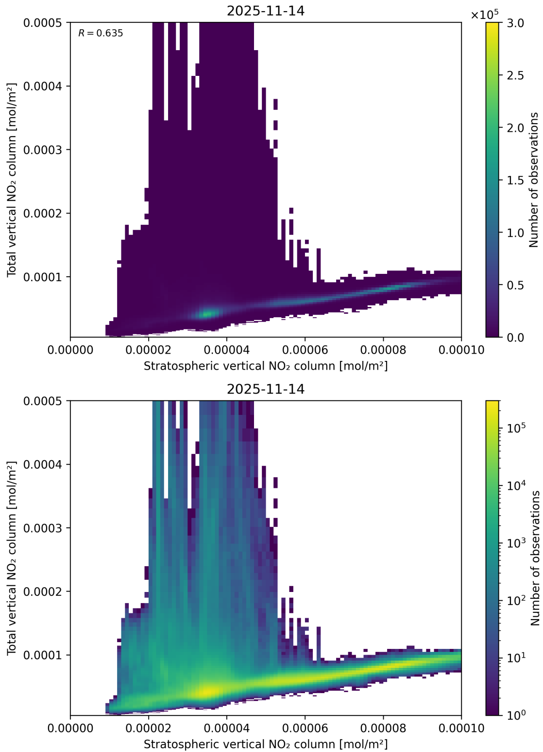
Figure 100: Scatter density plot of “Stratospheric vertical NO 2 column” against “Total vertical NO 2 column” for 2025-11-13 to 2025-11-15.
