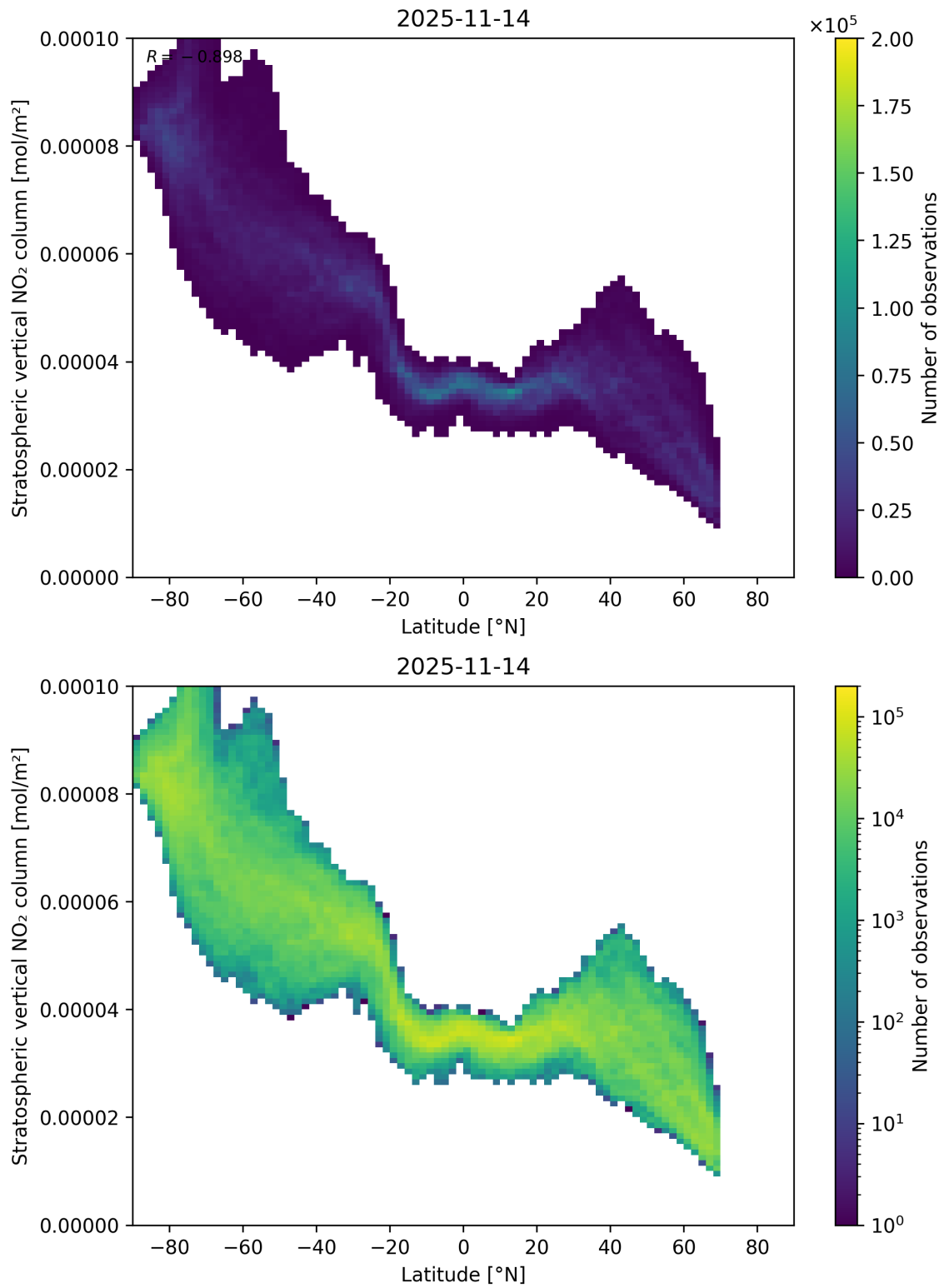
Figure 87: Scatter density plot of “Latitude” against “Stratospheric vertical NO 2 column” for 2025-11-13 to 2025-11-15.
