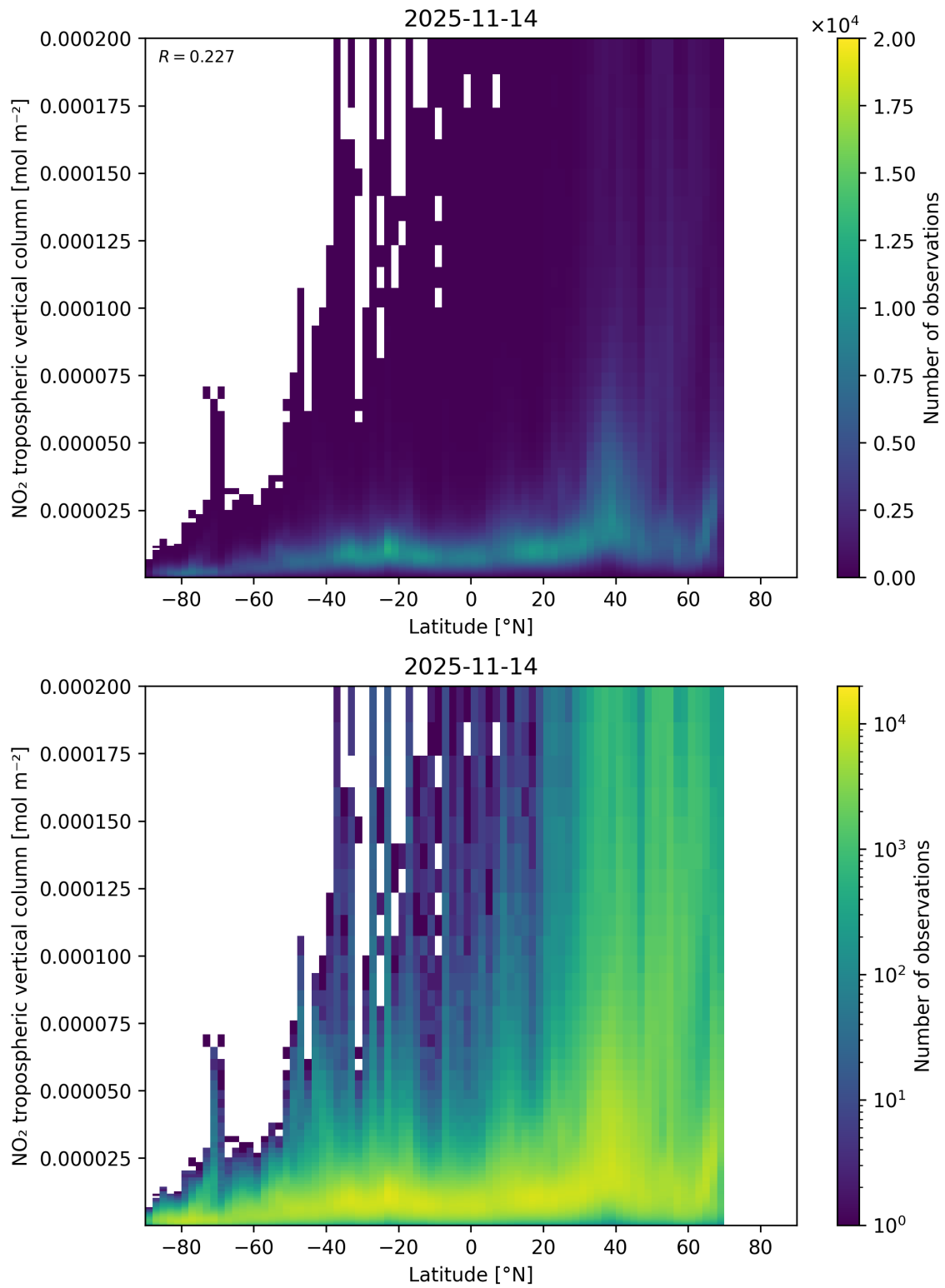
Figure 92: Scatter density plot of “Latitude” against “NO 2 tropospheric vertical column” for 2025-11-13 to 2025-11-15.
