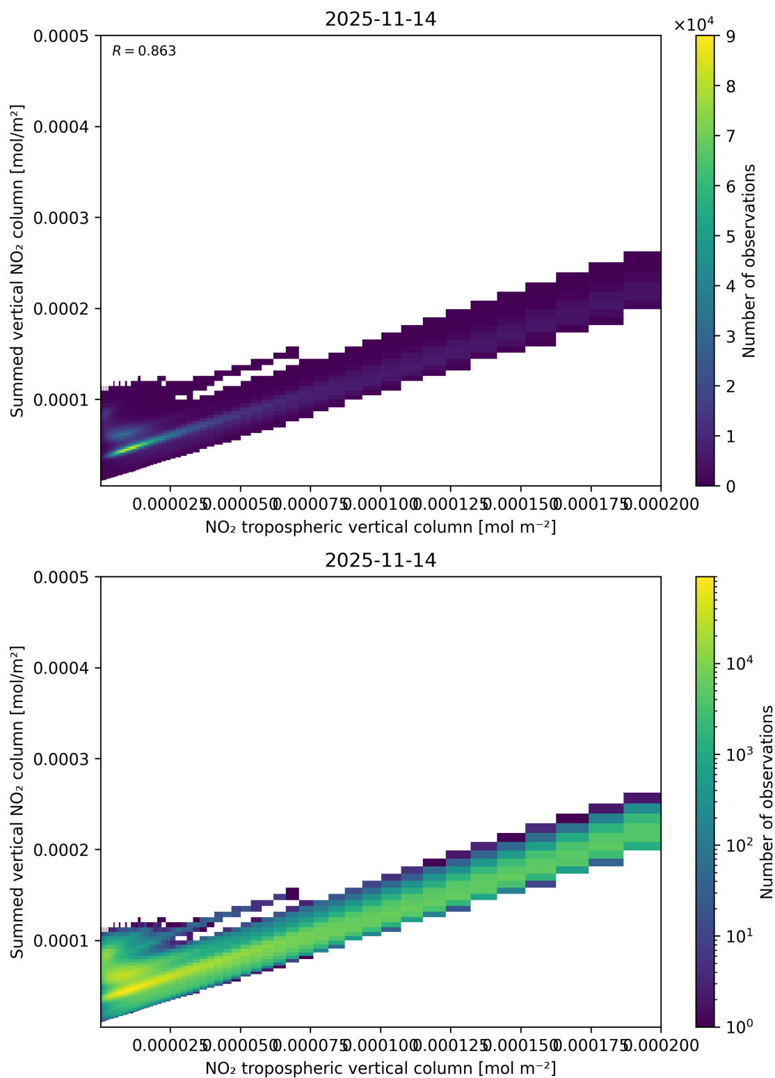
Figure 126: Scatter density plot of “NO 2 tropospheric vertical column” against “Summed vertical NO 2 column” for 2025-11-13 to 2025-11-15.
