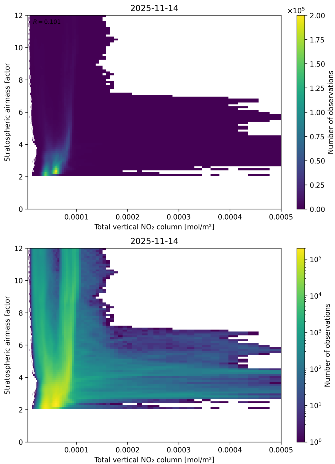
Figure 110: Scatter density plot of “Total vertical NO 2 column” against “Stratospheric airmass factor” for 2025-11-13 to 2025-11-15.
