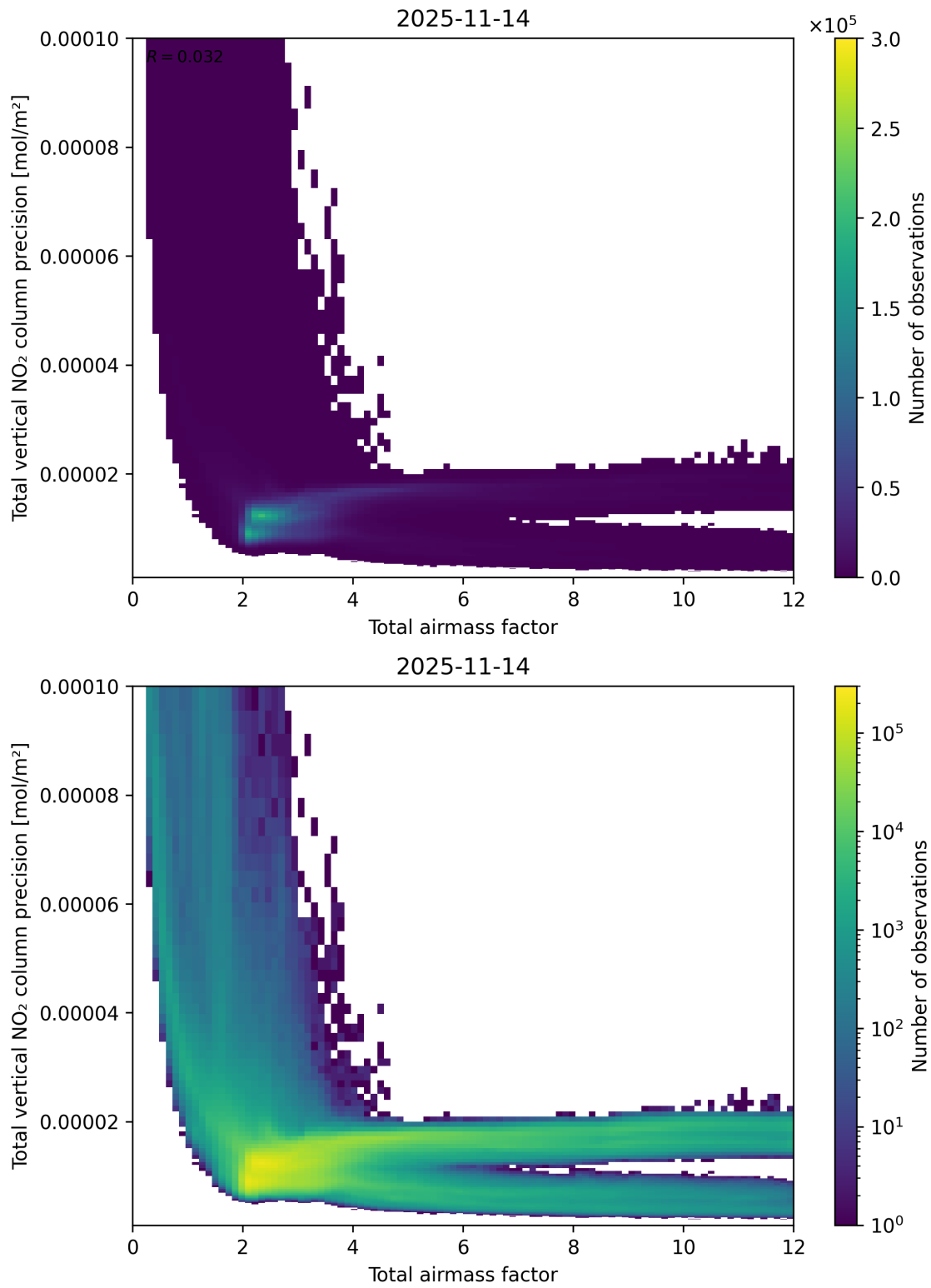
Figure 68: Scatter density plot of “Total airmass factor” against “Total vertical NO 2 column precision” for 2025-11-13 to 2025-11-15.
