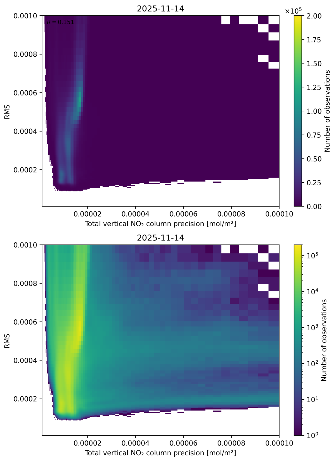
Figure 119: Scatter density plot of “Total vertical NO 2 column precision” against “RMS” for 2025-11-13 to 2025-11-15.
