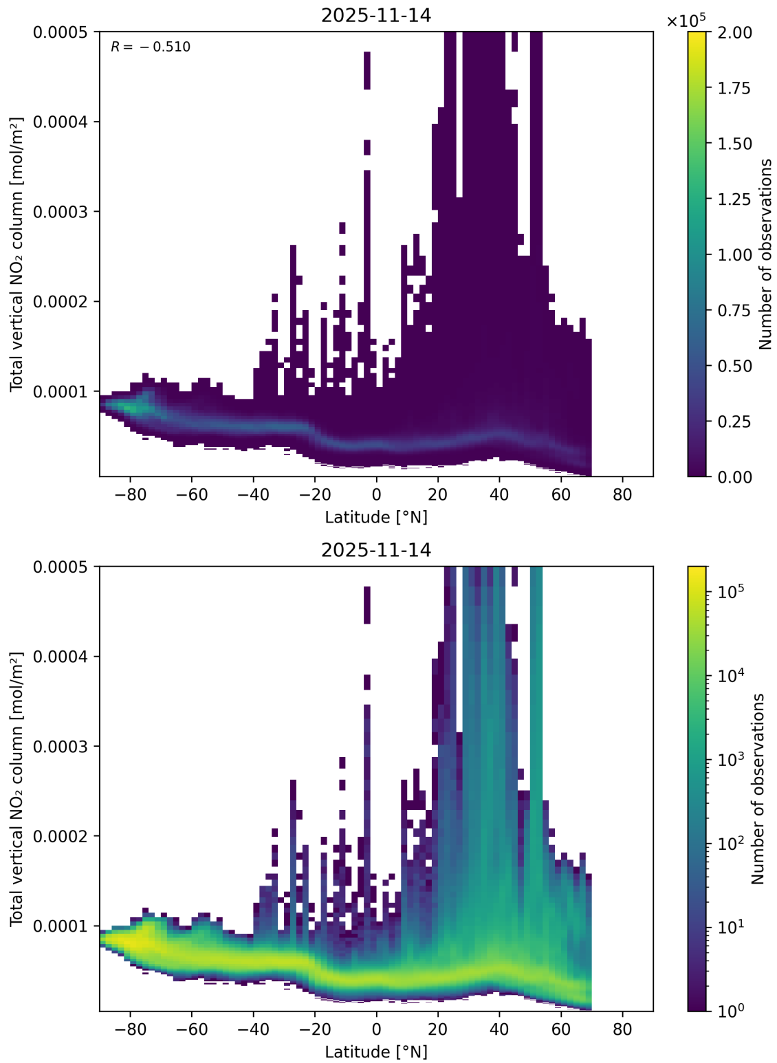
Figure 90: Scatter density plot of “Latitude” against “Total vertical NO 2 column” for 2025-11-13 to 2025-11-15.
