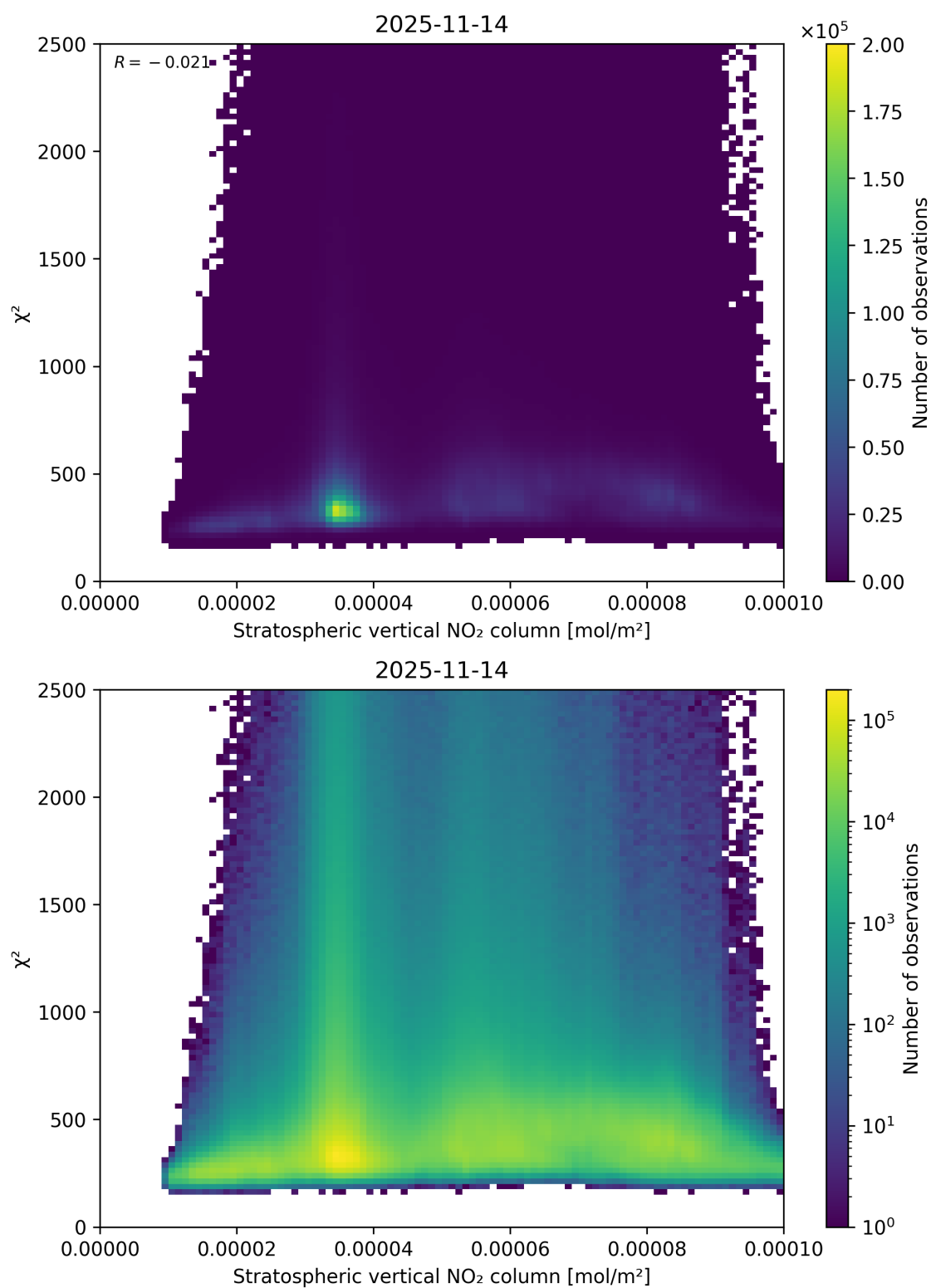
Figure 97: Scatter density plot of “Stratospheric vertical NO 2 column” against “ \chi^2 ” for 2025-11-13 to 2025-11-15.
