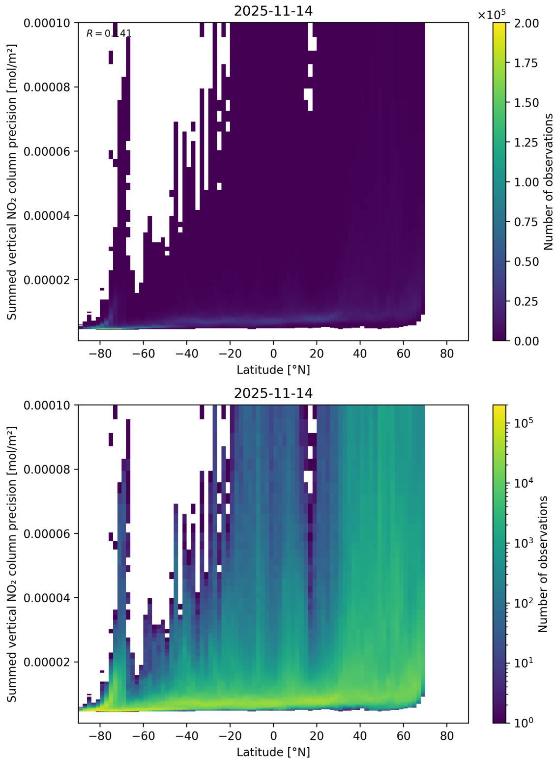
Figure 89: Scatter density plot of “Latitude” against “Summed vertical NO 2 column precision” for 2025-11-13 to 2025-11-15.
