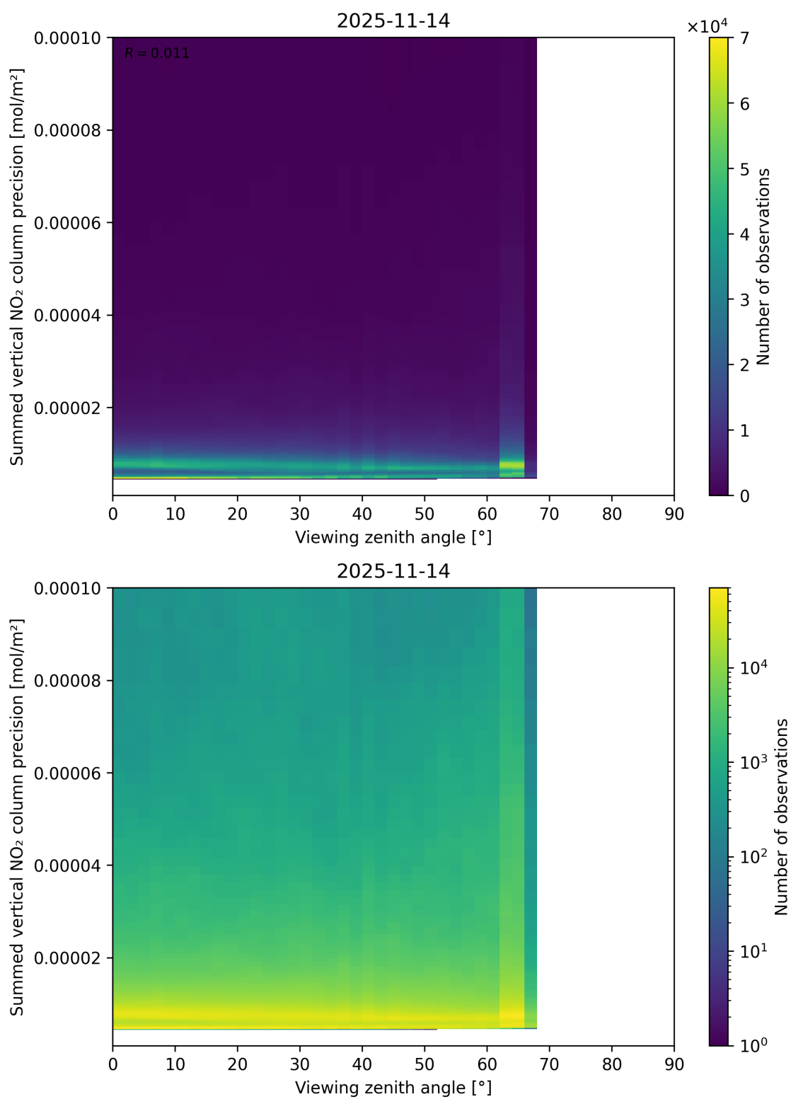
Figure 166: Scatter density plot of “Viewing zenith angle” against “Summed vertical NO 2 column precision” for 2025-11-13 to 2025-11-15.
