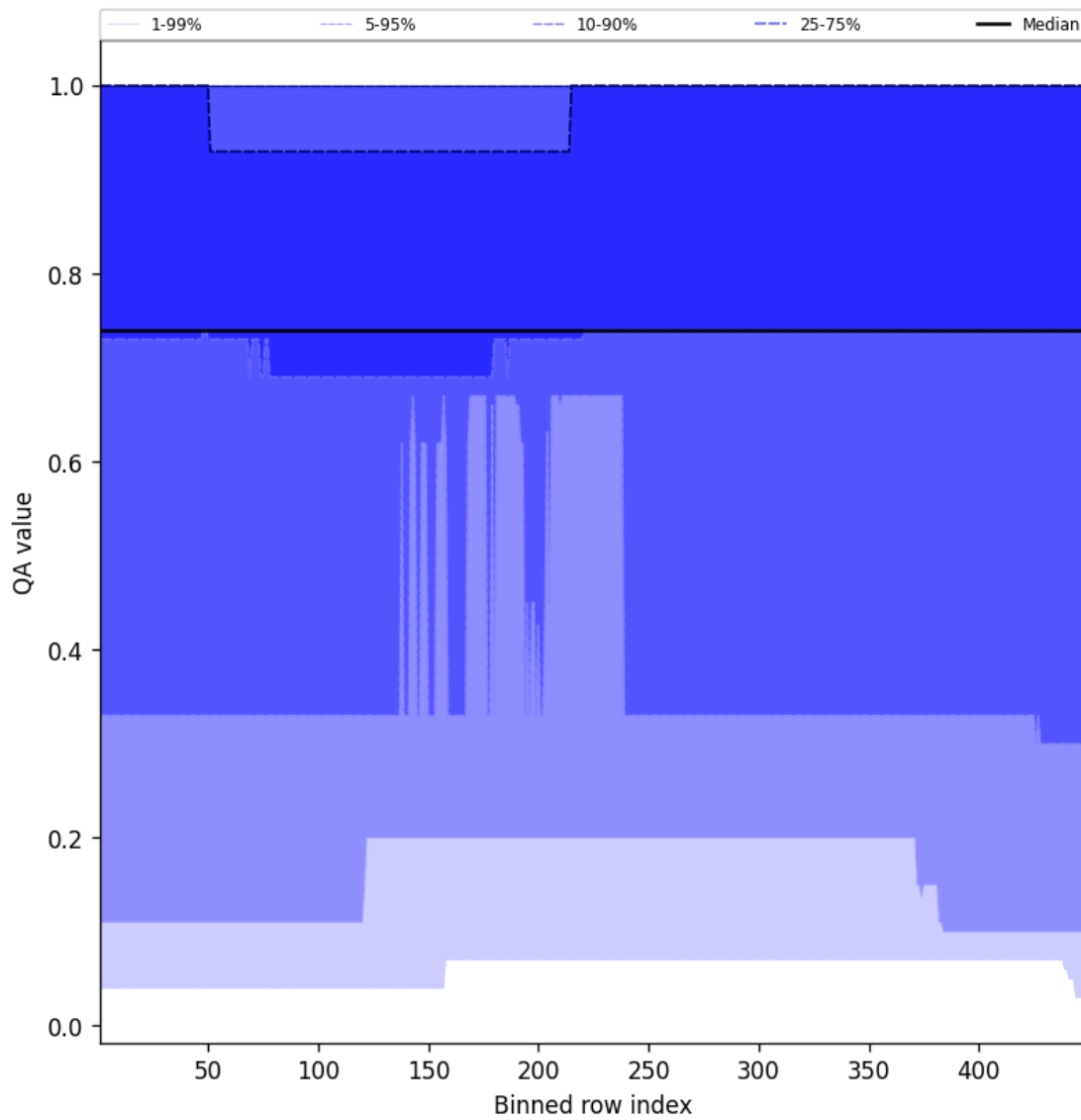
Figure 45: Along track statistics of “QA value” for 2025-11-13 to 2025-11-15
