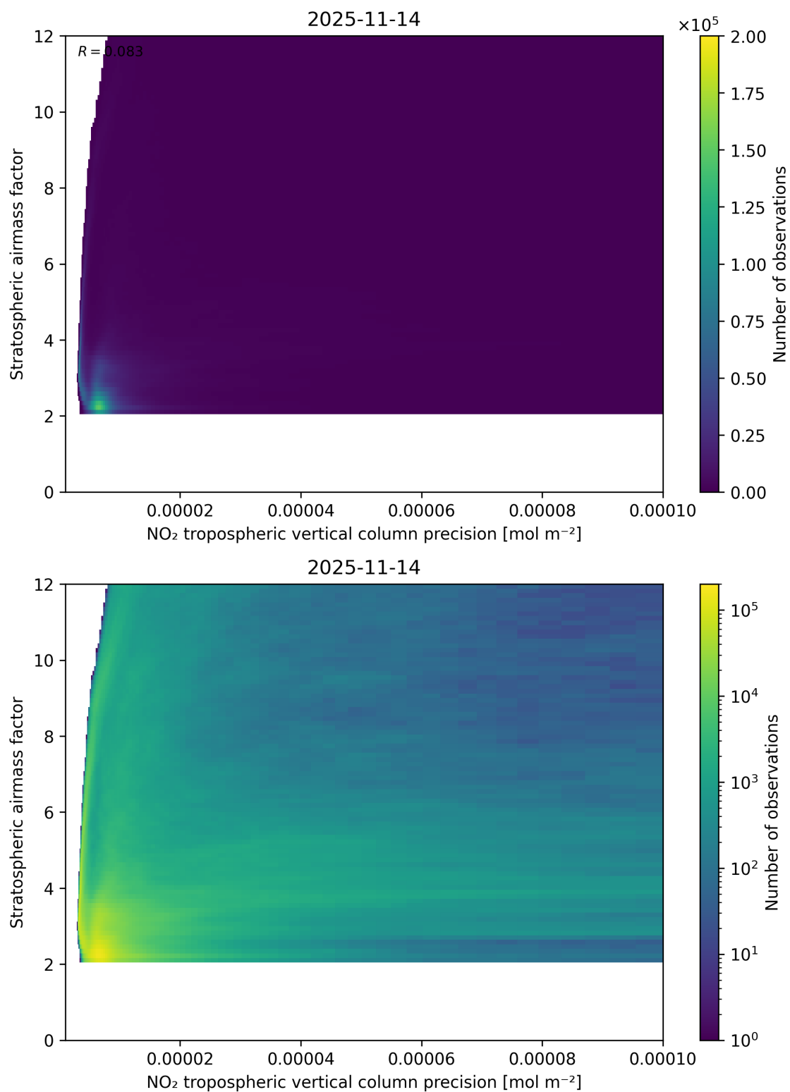
Figure 131: Scatter density plot of “NO 2 tropospheric vertical column precision” against “Stratospheric airmass factor” for 2025-11-13 to 2025-11-15.
