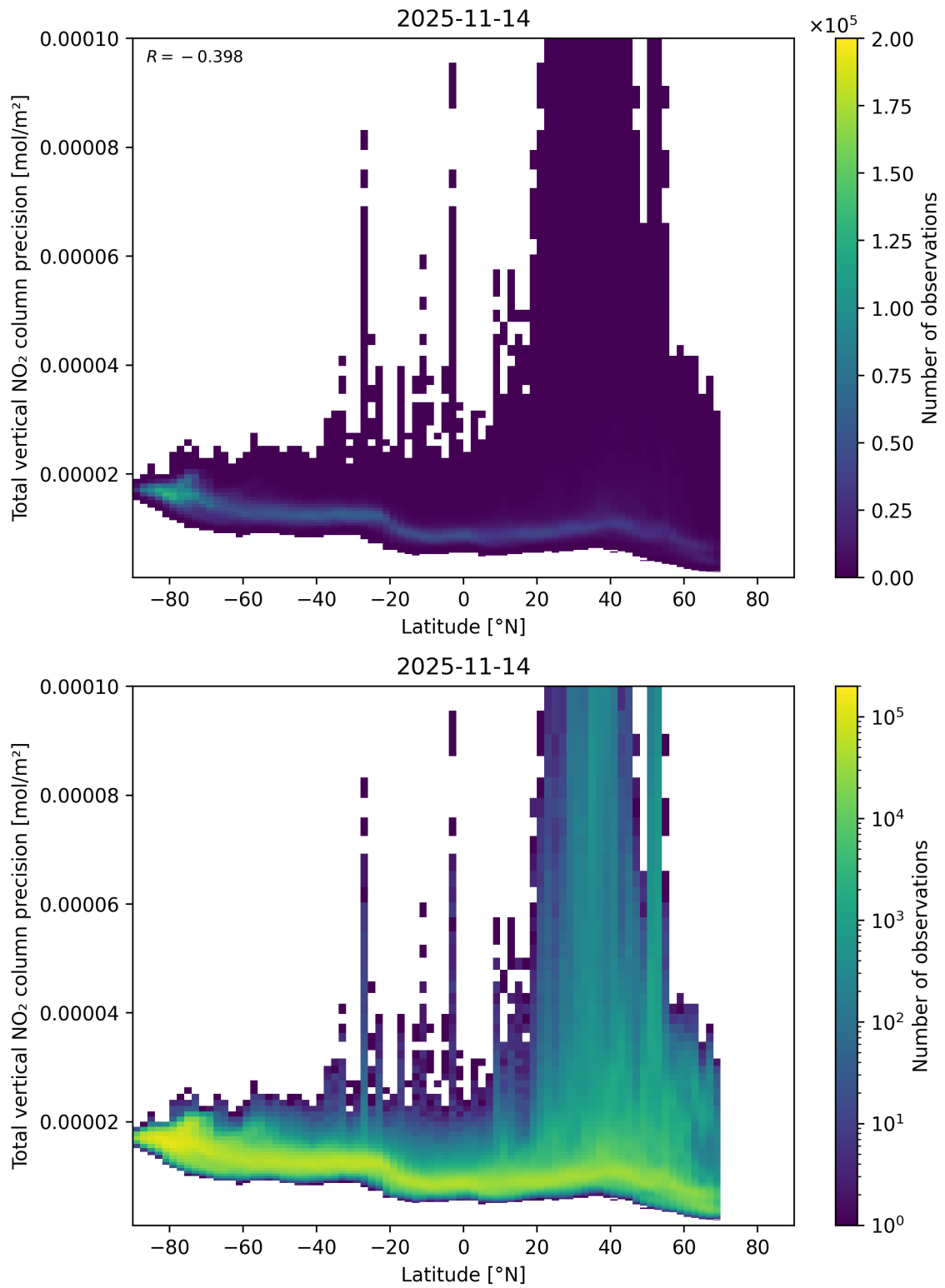
Figure 91: Scatter density plot of “Latitude” against “Total vertical NO 2 column precision” for 2025-11-13 to 2025-11-15.
