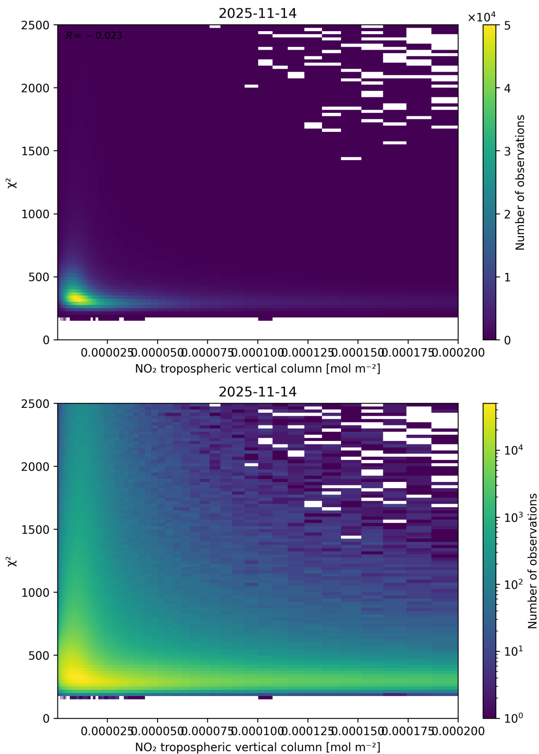
Figure 124: Scatter density plot of “NO 2 tropospheric vertical column” against “ \chi^2 ” for 2025-11-13 to 2025-11-15.
