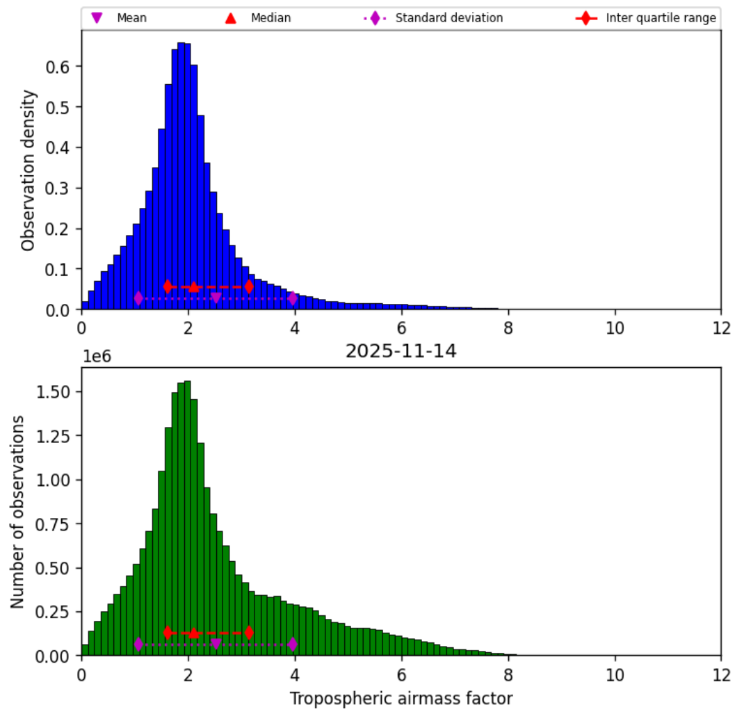
Figure 31: Histogram of “Tropospheric airmass factor” for 2025-11-13 to 2025-11-15
