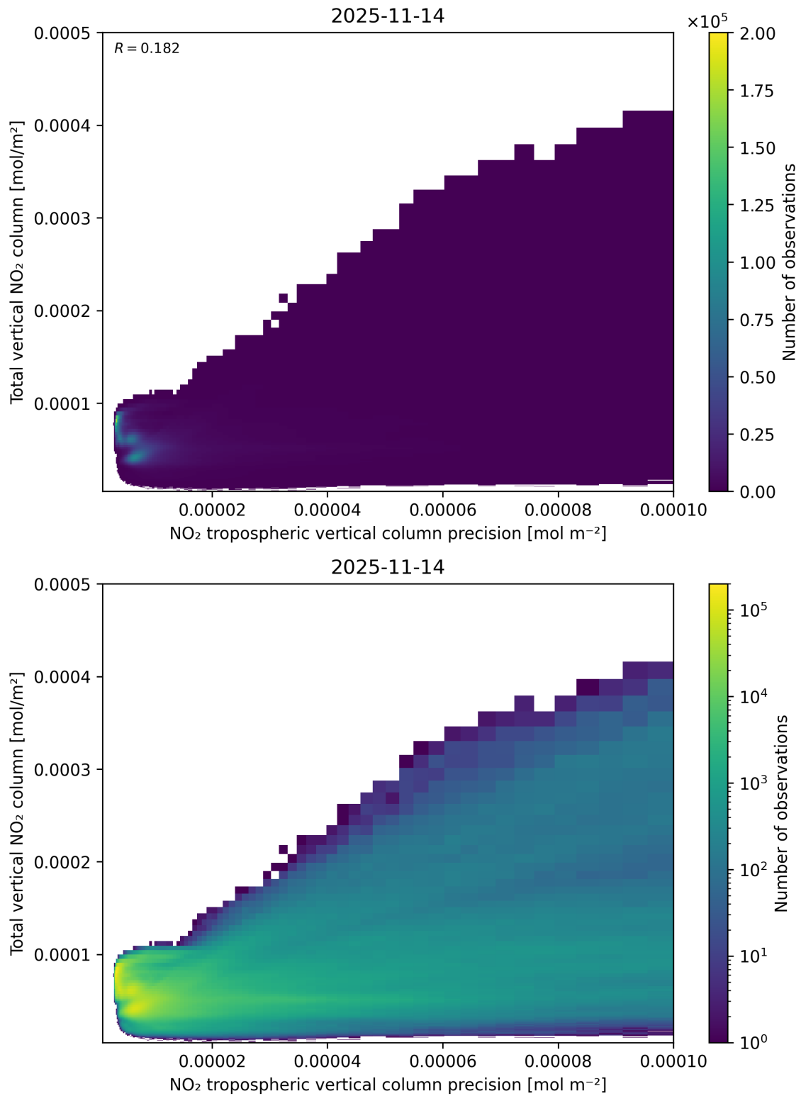
Figure 138: Scatter density plot of “NO 2 tropospheric vertical column precision” against “Total vertical NO 2 column” for 2025-11-13 to 2025-11-15.
