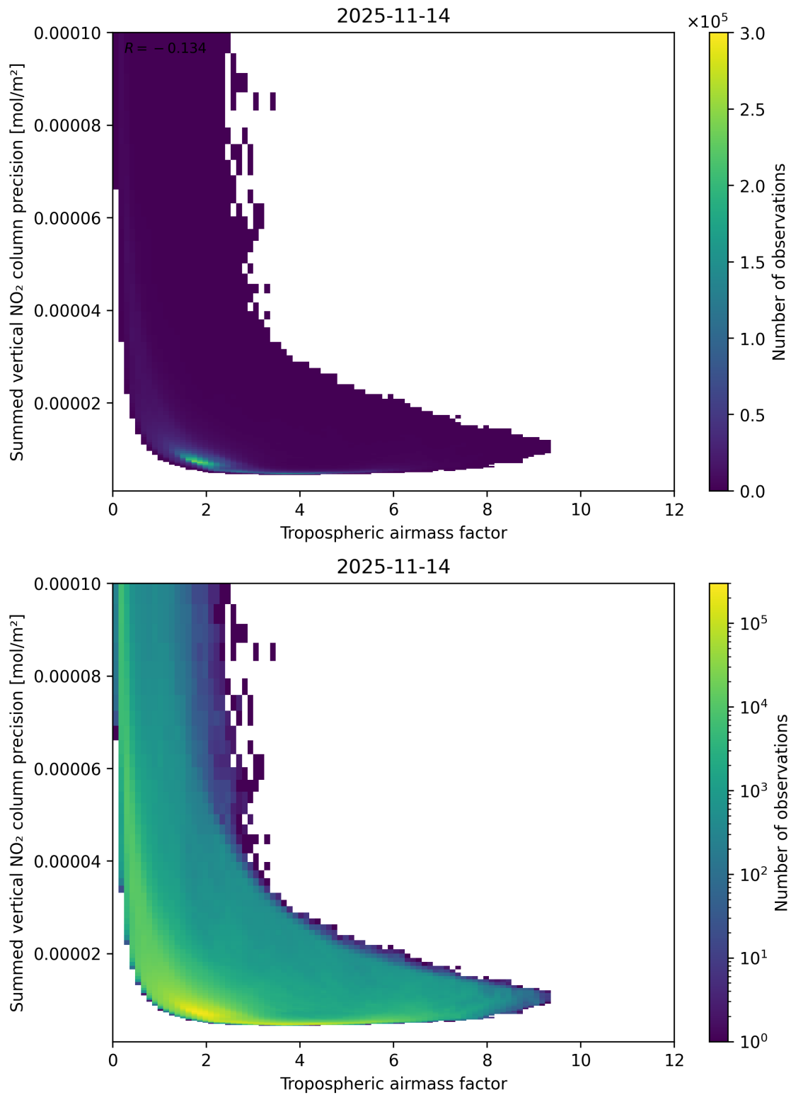
Figure 76: Scatter density plot of “Tropospheric airmass factor” against “Summed vertical NO 2 column precision” for 2025-11-13 to 2025-11-15.
