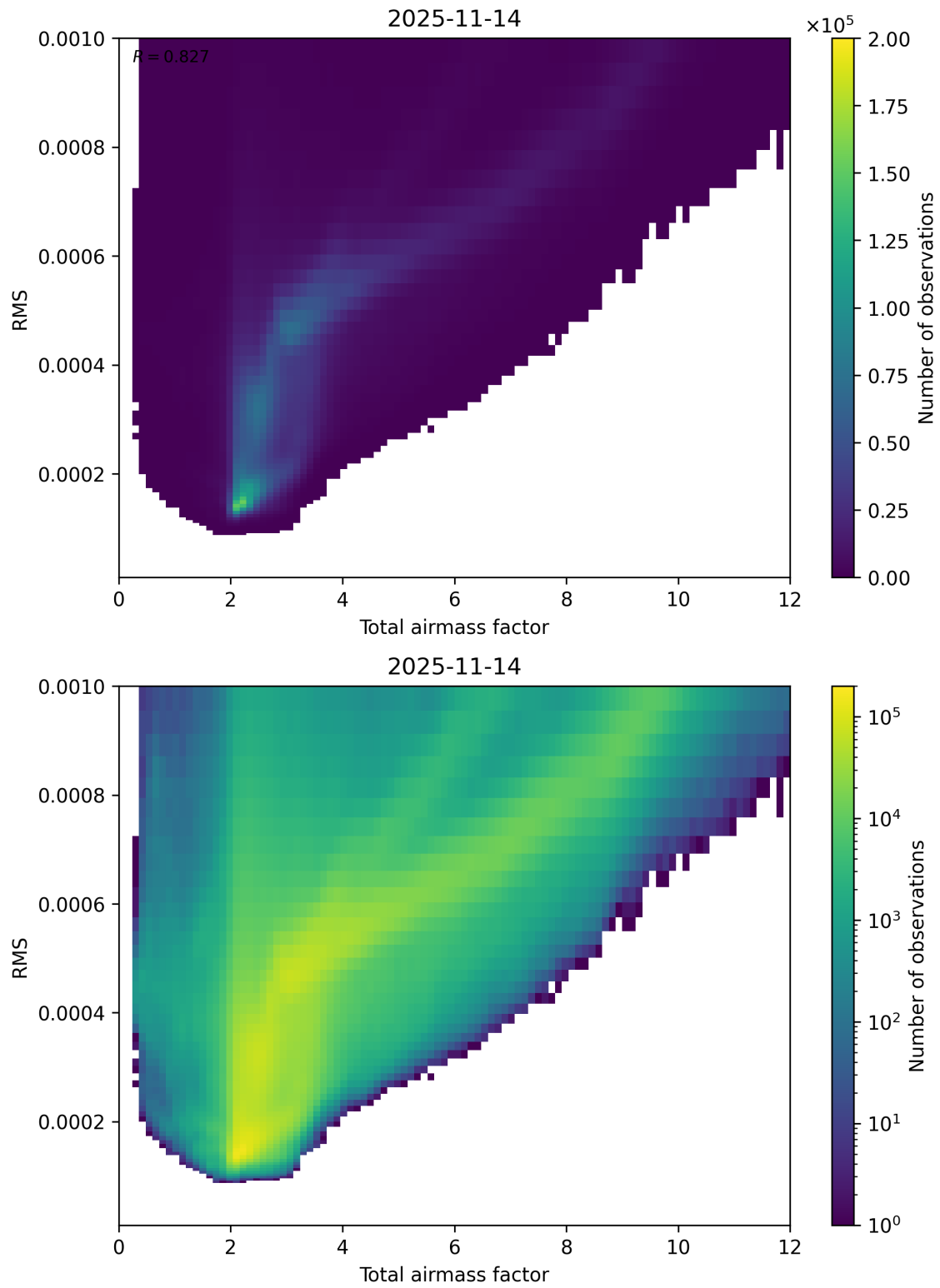
Figure 69: Scatter density plot of “Total airmass factor” against “RMS” for 2025-11-13 to 2025-11-15.
