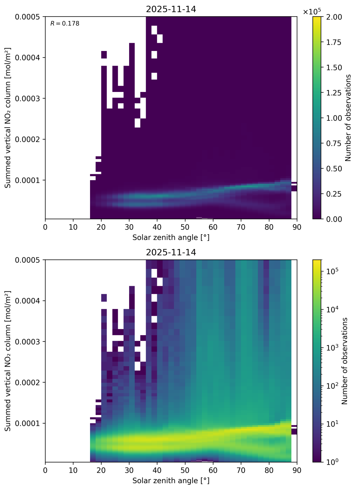
Figure 151: Scatter density plot of “Solar zenith angle” against “Summed vertical NO 2 column” for 2025-11-13 to 2025-11-15.
