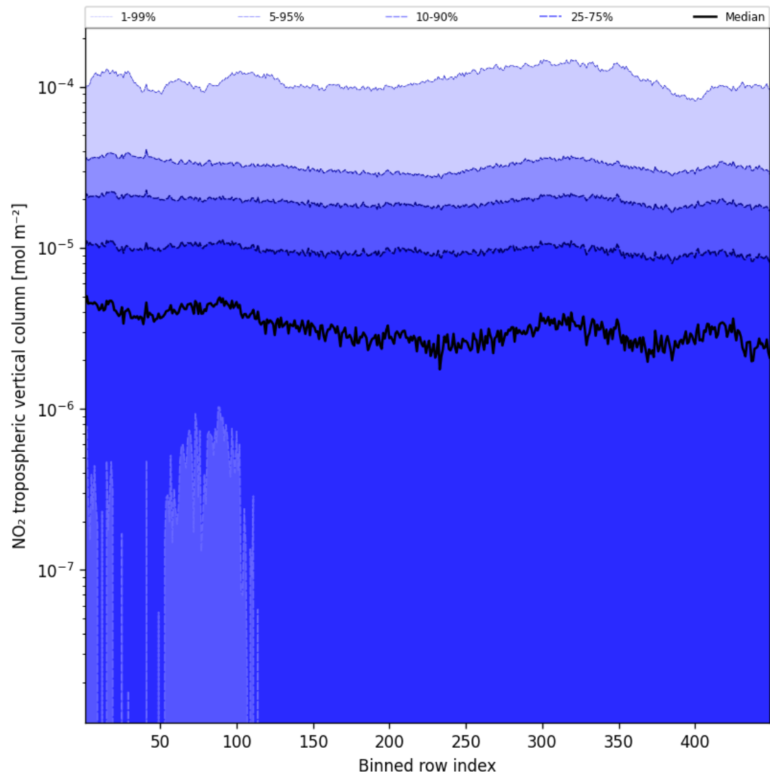
Figure 46: Along track statistics of “NO 2 tropospheric vertical column” for 2025-11-13 to 2025-11-15
