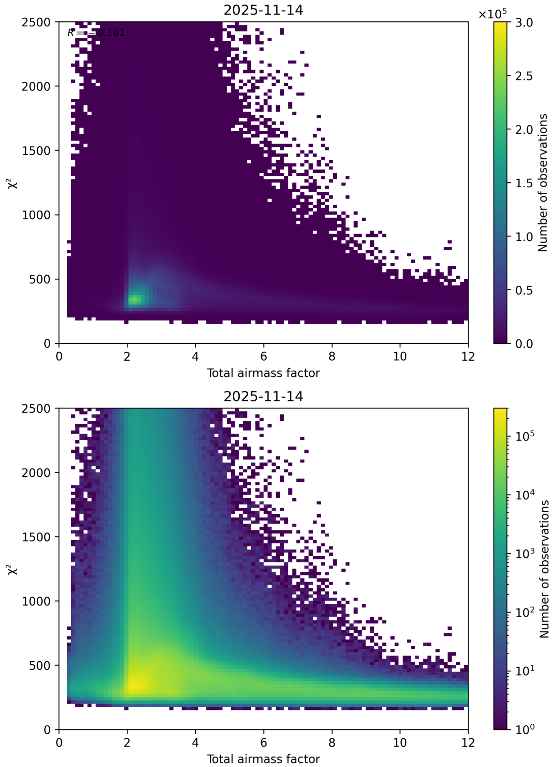
Figure 63: Scatter density plot of “Total airmass factor” against “ \chi^2 ” for 2025-11-13 to 2025-11-15.
