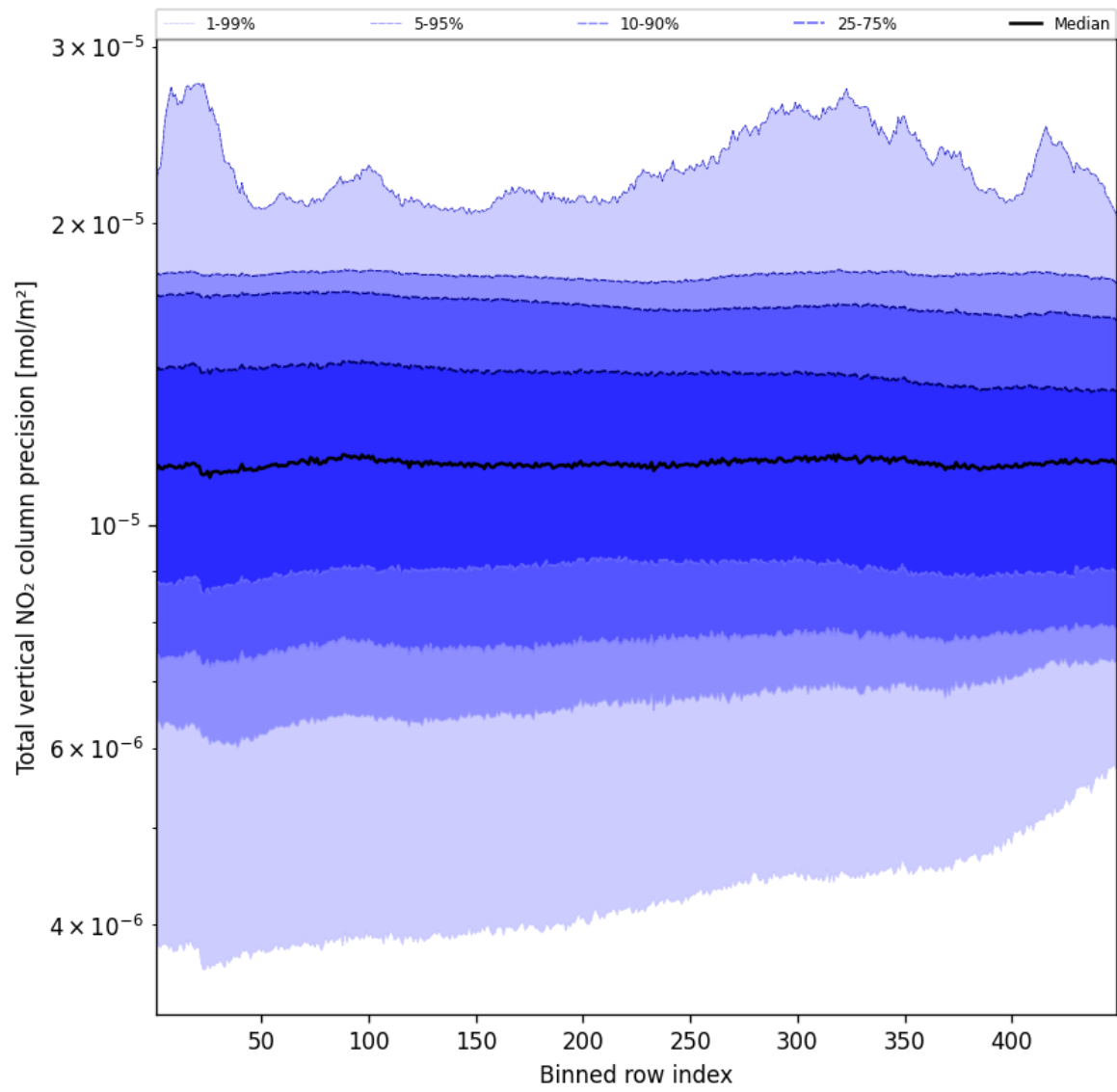
Figure 56: Along track statistics of “Total vertical NO 2 column precision” for 2025-11-13 to 2025-11-15
