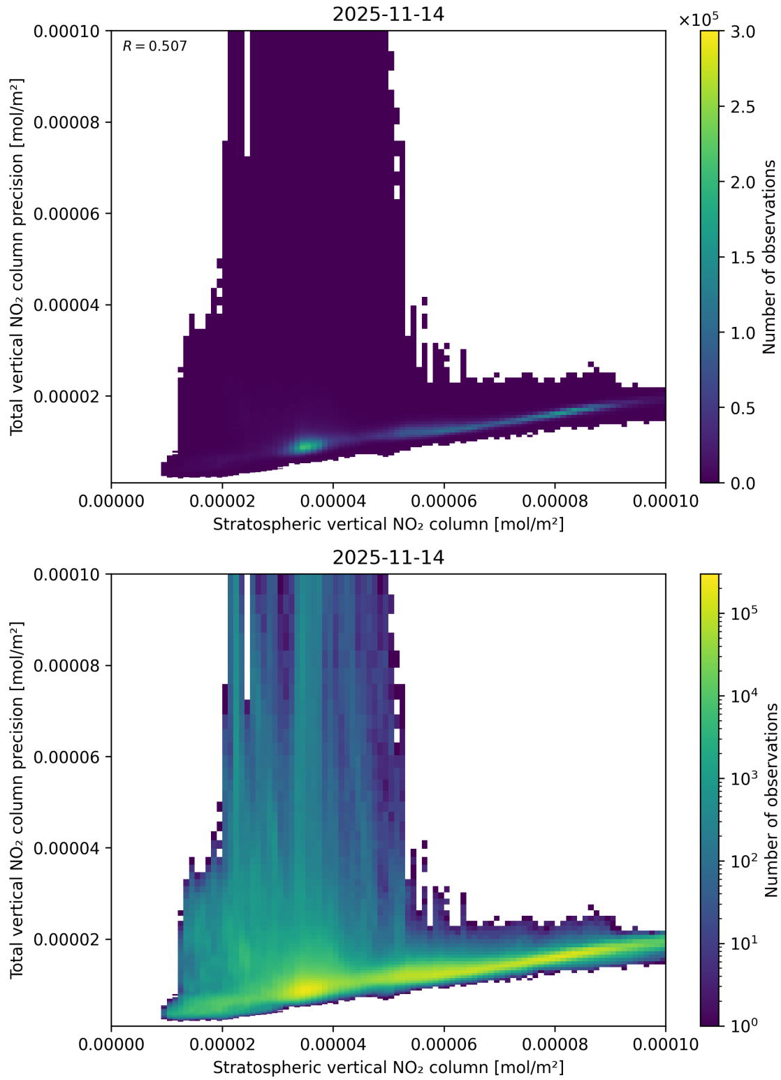
Figure 101: Scatter density plot of “Stratospheric vertical NO 2 column” against “Total vertical NO 2 column precision” for 2025-11-13 to 2025-11-15.
