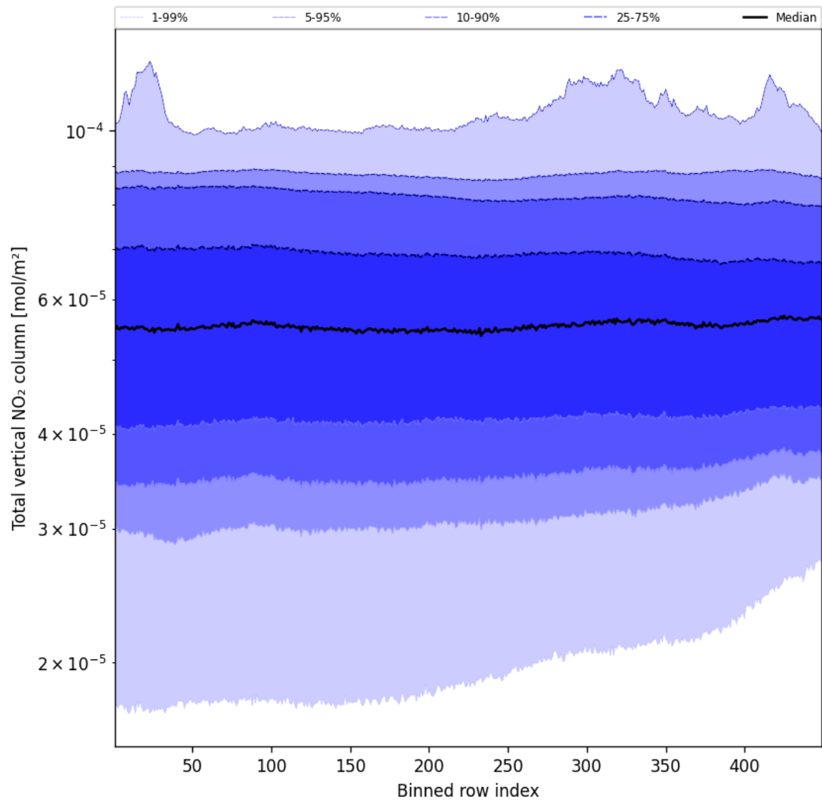
Figure 55: Along track statistics of “Total vertical NO 2 column” for 2025-11-13 to 2025-11-15
