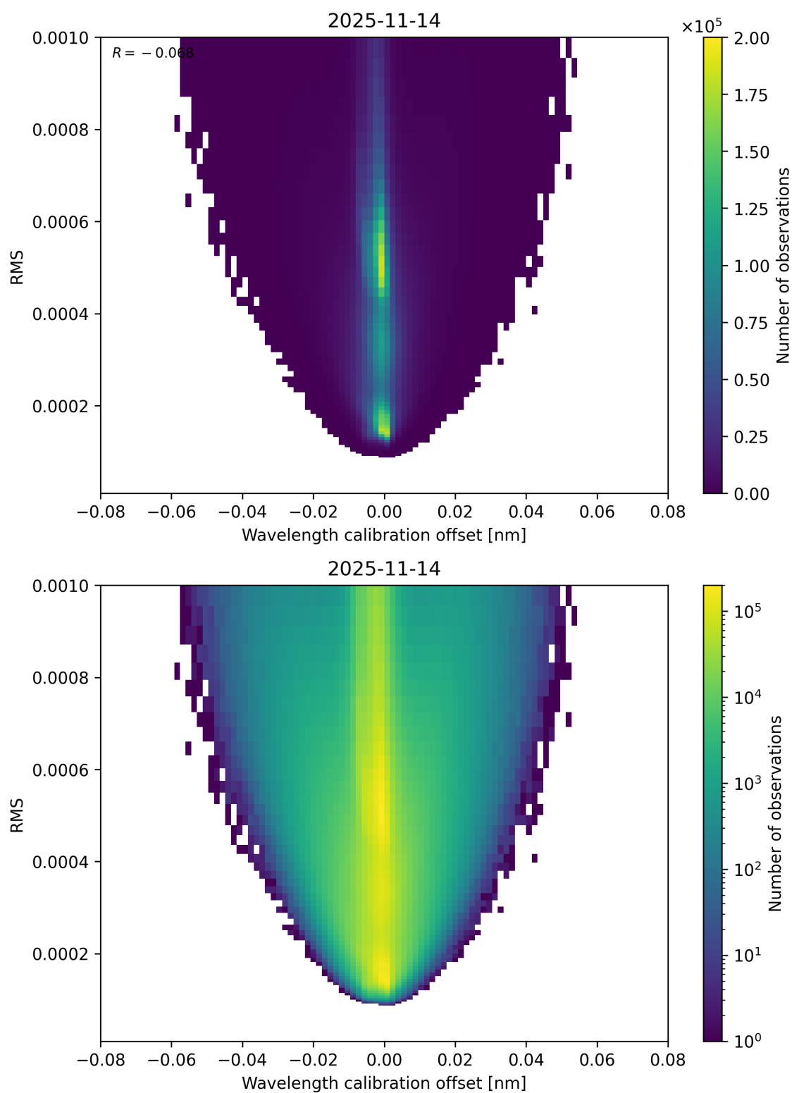
Figure 181: Scatter density plot of “Wavelength calibration offset” against “RMS” for 2025-11-13 to 2025-11-15.
