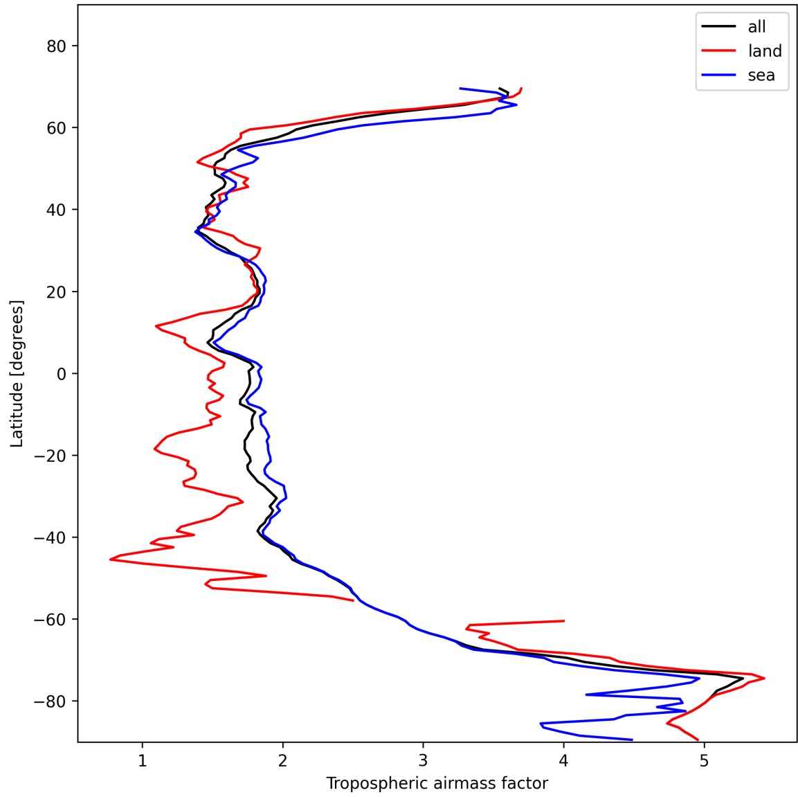
Figure 14: Zonal average of “Tropospheric airmass factor” for 2025-11-13 to 2025-11-15.
