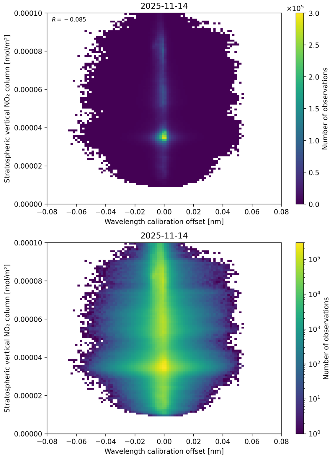
Figure 176: Scatter density plot of “Wavelength calibration offset” against “Stratospheric vertical NO 2 column” for 2025-11-13 to 2025-11-15.
