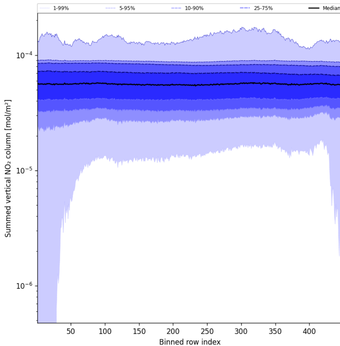
Figure 57: Along track statistics of “Summed vertical NO 2 column” for 2025-11-13 to 2025-11-15
