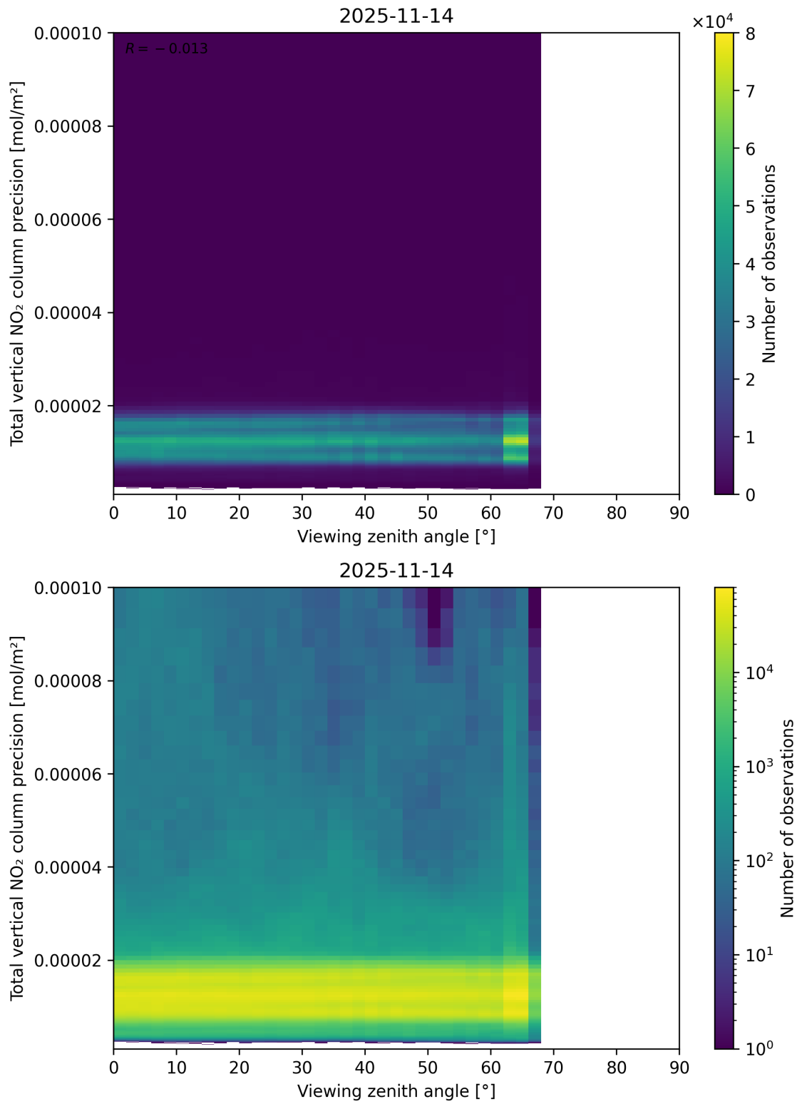
Figure 168: Scatter density plot of “Viewing zenith angle” against “Total vertical NO 2 column precision” for 2025-11-13 to 2025-11-15.
