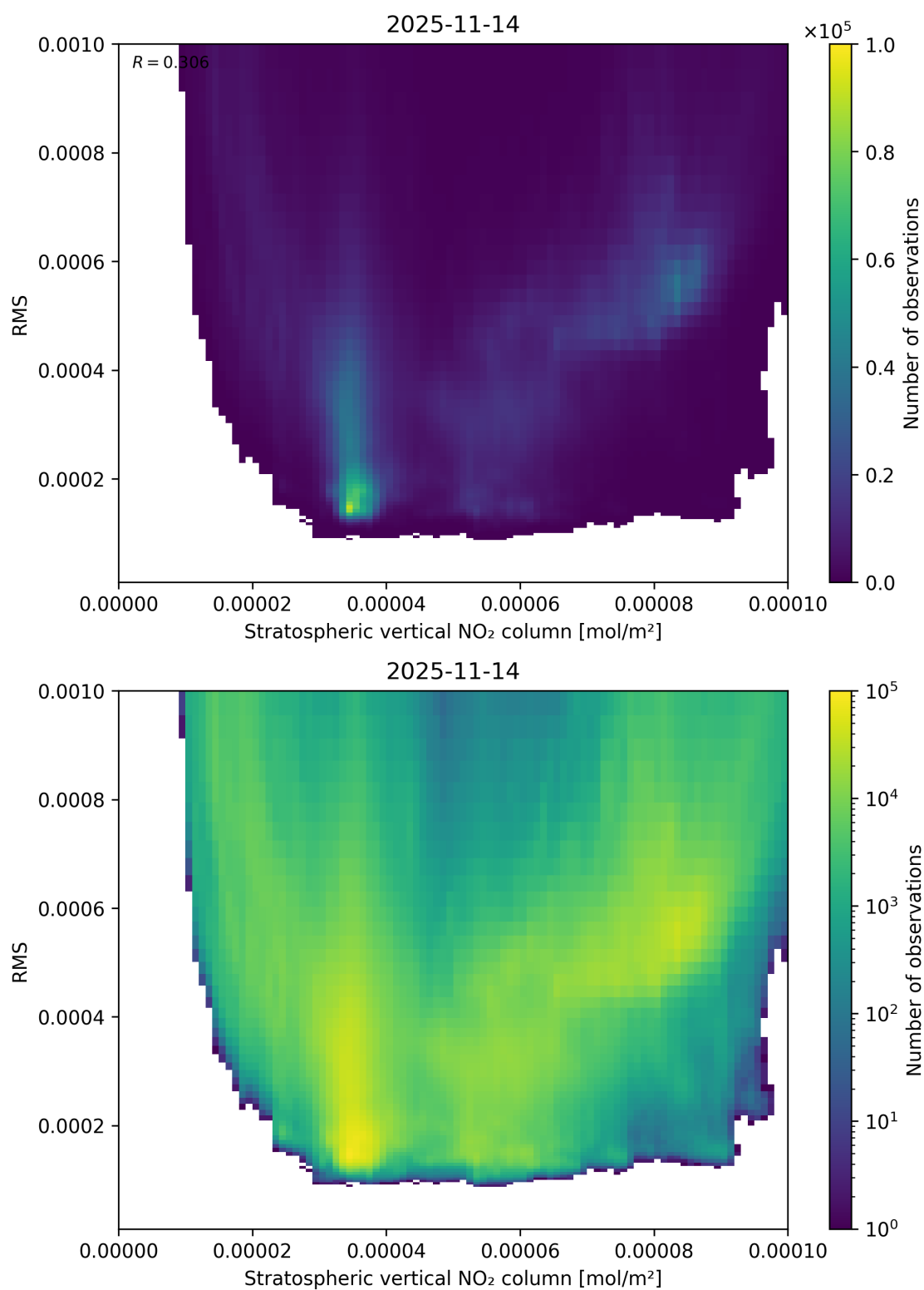
Figure 102: Scatter density plot of “Stratospheric vertical NO 2 column” against “RMS” for 2025-11-13 to 2025-11-15.
