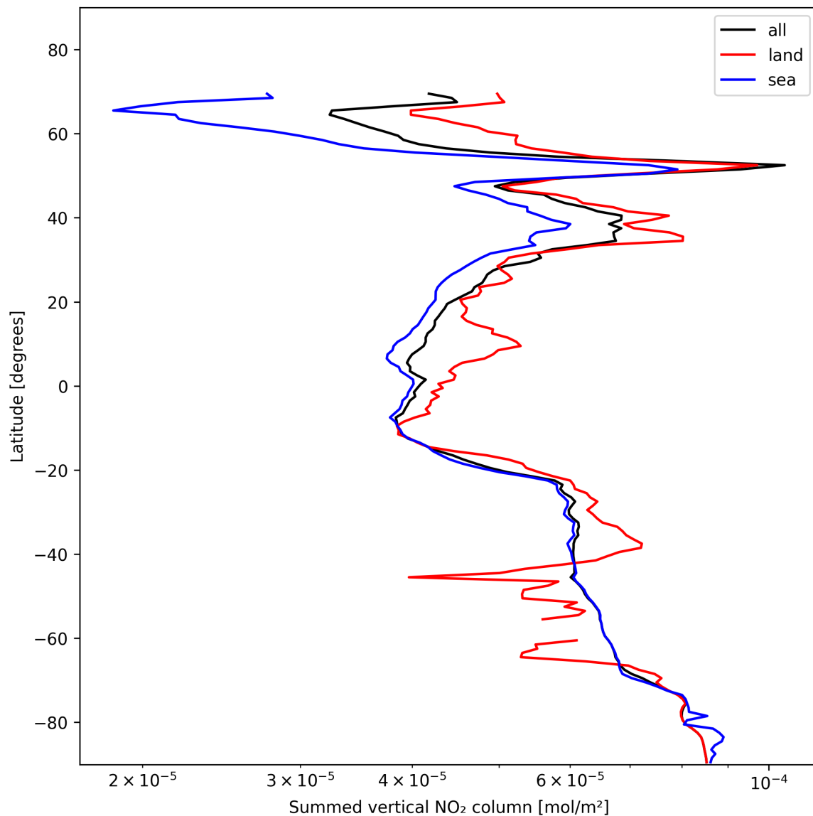
Figure 23: Zonal average of “Summed vertical NO 2 column” for 2025-11-13 to 2025-11-15.
