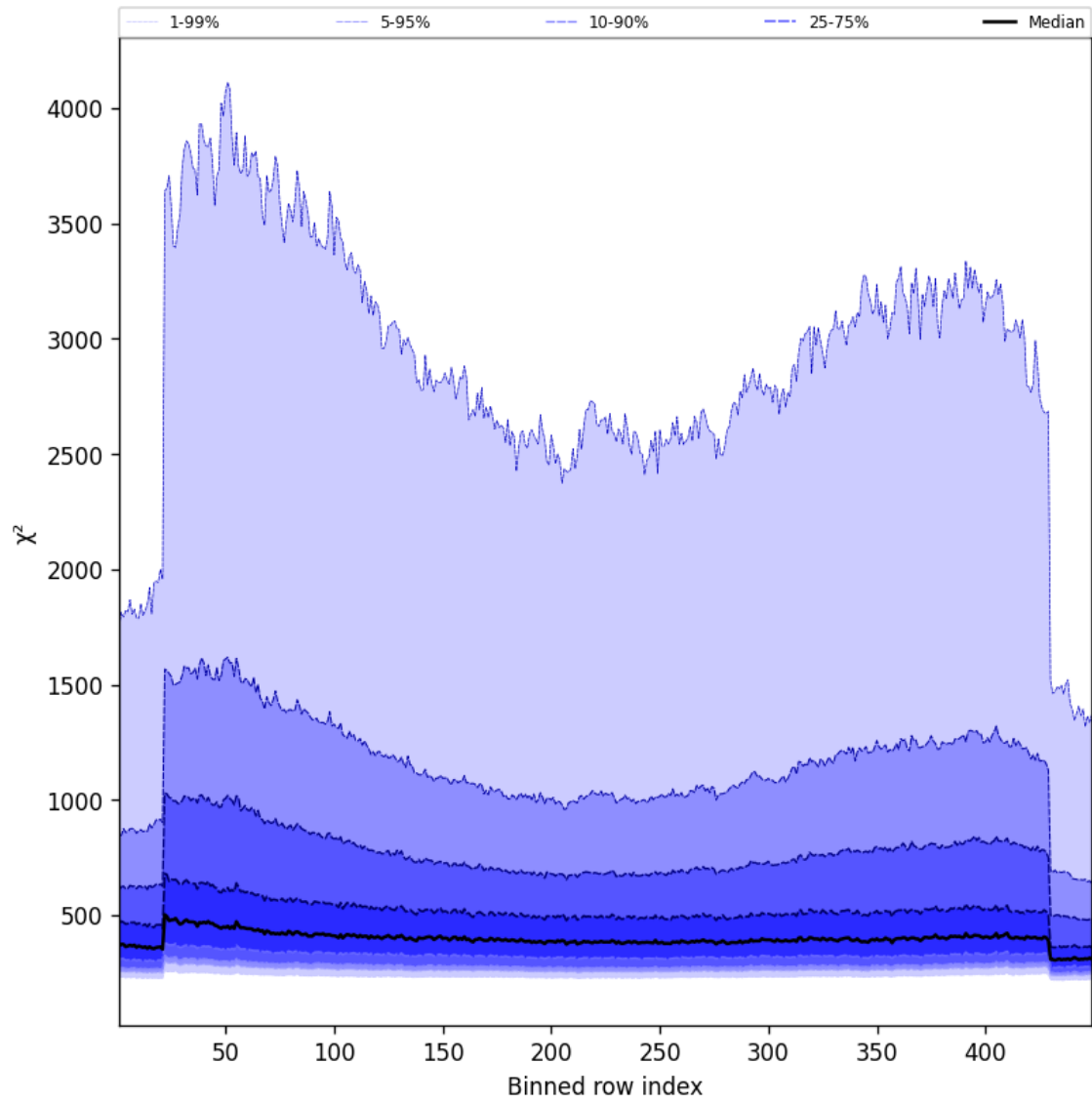
Figure 59: Along track statistics of “ \chi^2 ” for 2025-11-13 to 2025-11-15
