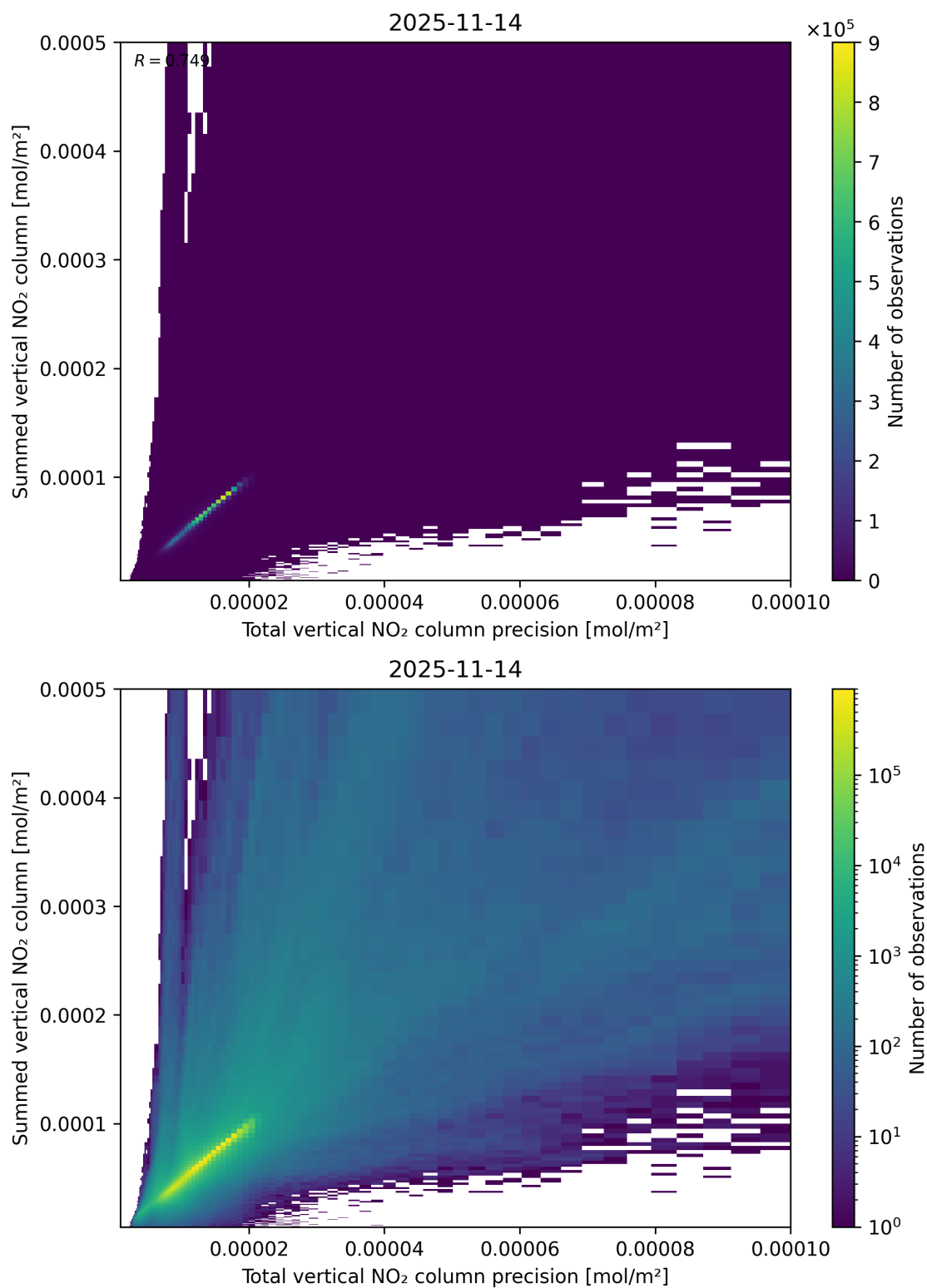
Figure 117: Scatter density plot of “Total vertical NO 2 column precision” against “Summed vertical NO 2 column” for 2025-11-13 to 2025-11-15.
