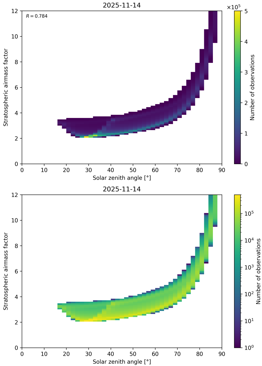
Figure 145: Scatter density plot of “Solar zenith angle” against “Stratospheric airmass factor” for 2025-11-13 to 2025-11-15.
