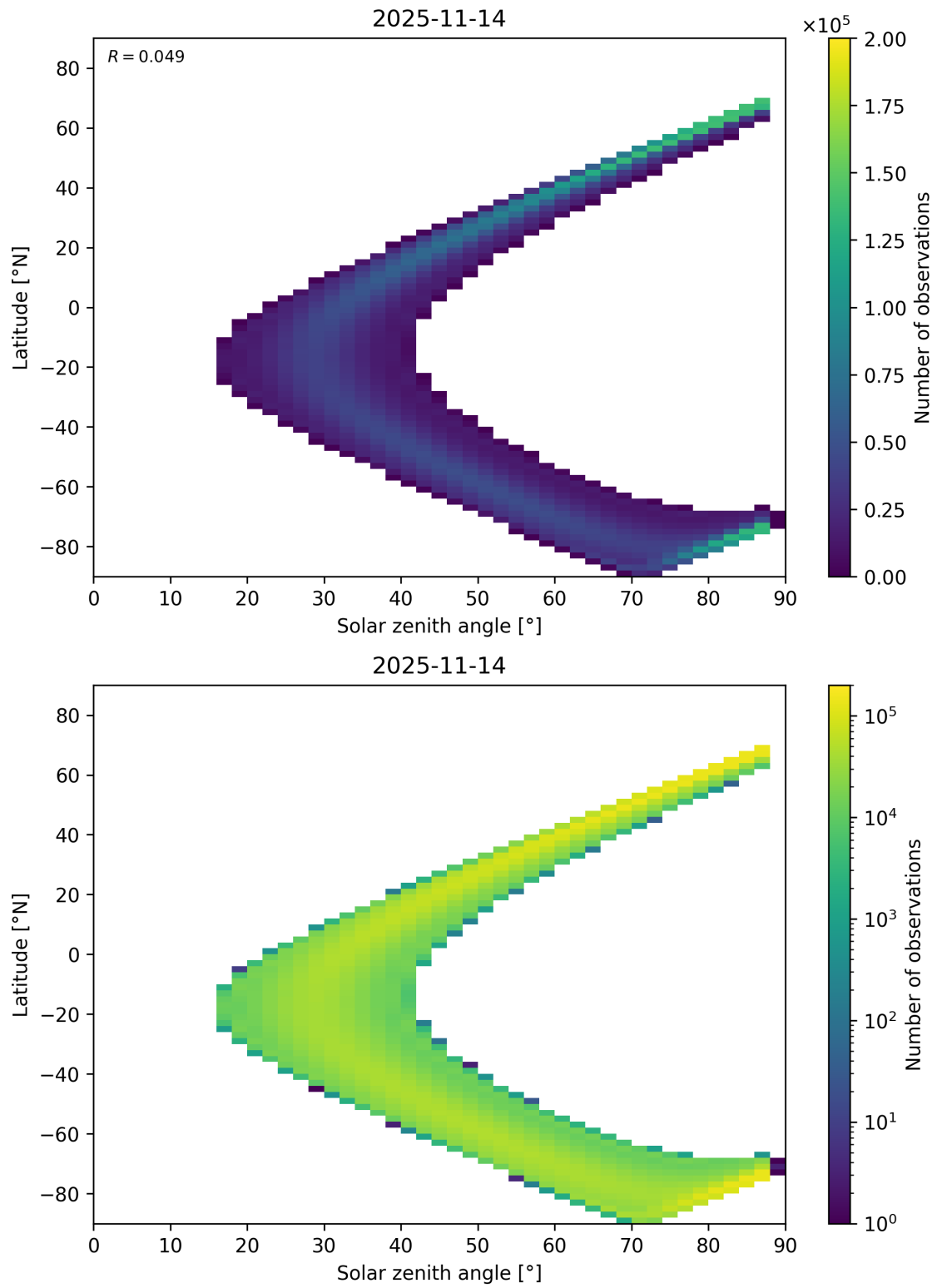
Figure 149: Scatter density plot of “Solar zenith angle” against “Latitude” for 2025-11-13 to 2025-11-15.
