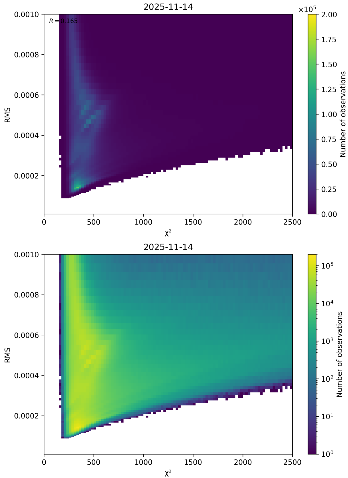
Figure 82: Scatter density plot of “ \chi^2 ” against “RMS” for 2025-11-13 to 2025-11-15.
