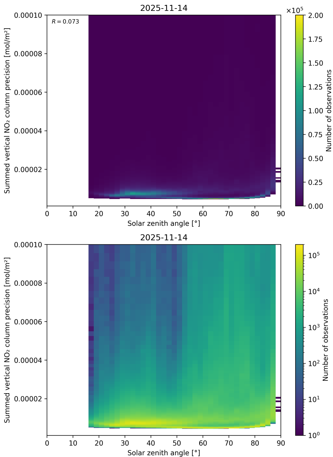
Figure 152: Scatter density plot of “Solar zenith angle” against “Summed vertical NO 2 column precision” for 2025-11-13 to 2025-11-15.
