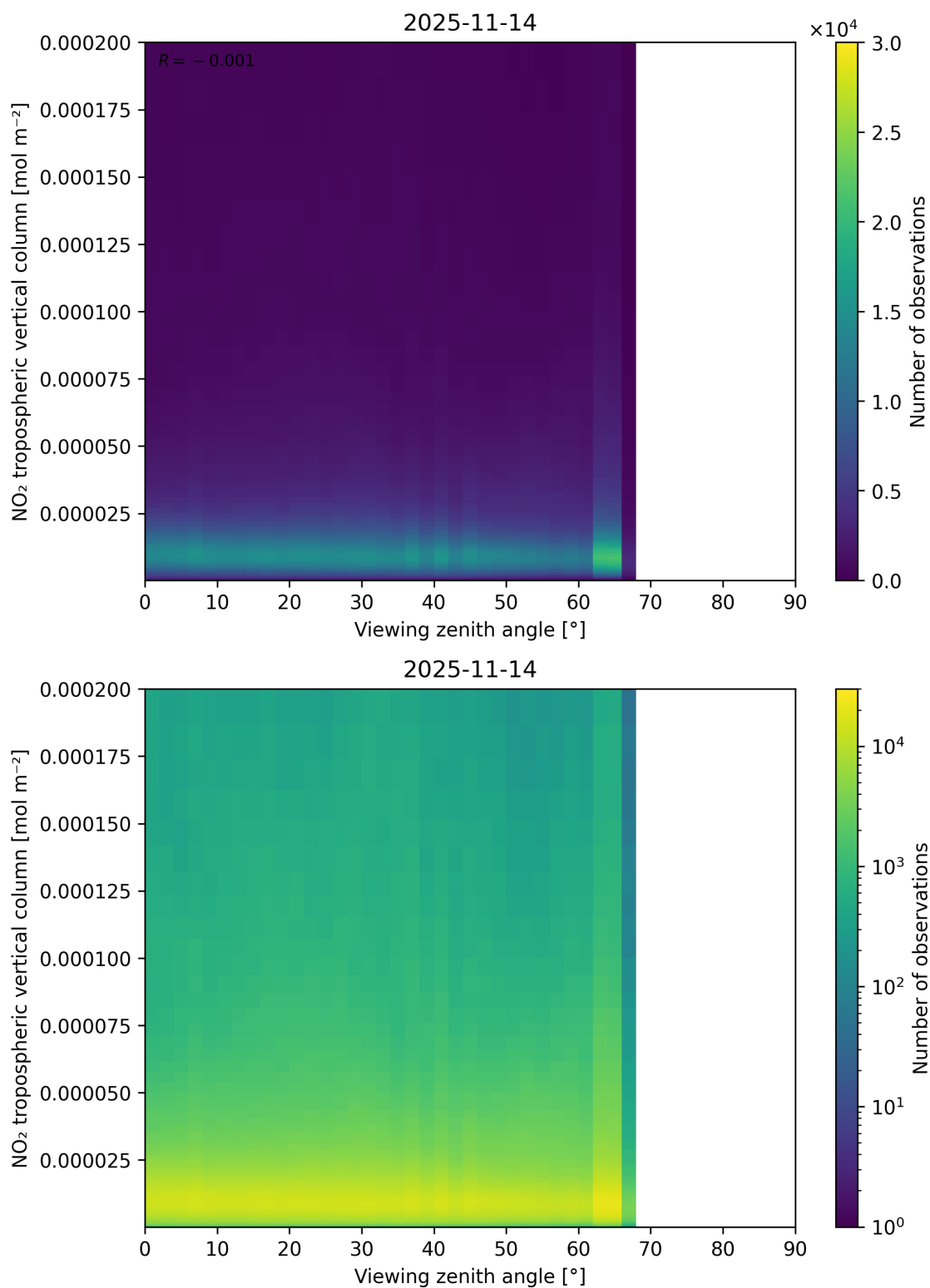
Figure 169: Scatter density plot of “Viewing zenith angle” against “NO 2 tropospheric vertical column” for 2025-11-13 to 2025-11-15.
