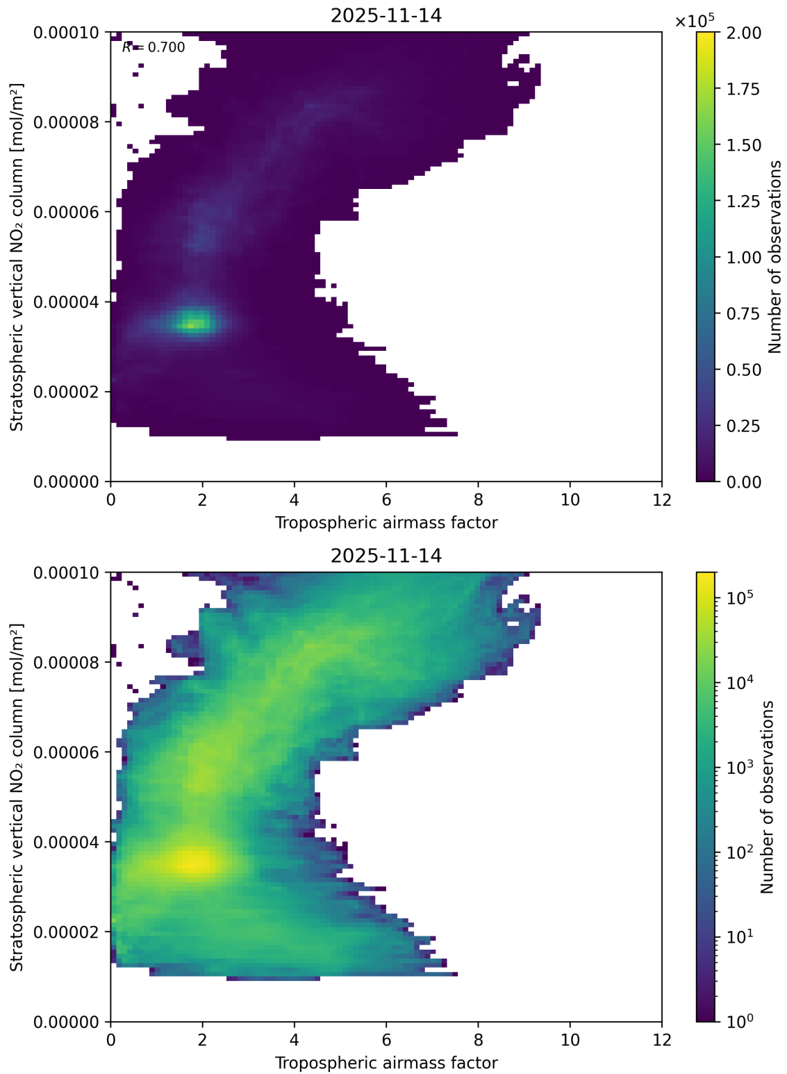
Figure 74: Scatter density plot of “Tropospheric air mass factor” against “Stratospheric vertical NO 2 column” for 2025-11-13 to 2025-11-15.
