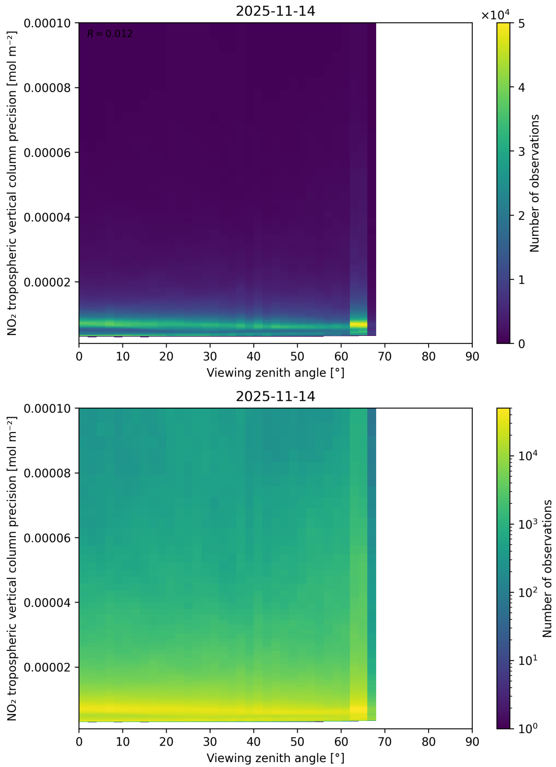
Figure 170: Scatter density plot of “Viewing zenith angle” against “NO 2 tropospheric vertical column precision” for 2025-11-13 to 2025-11-15.
