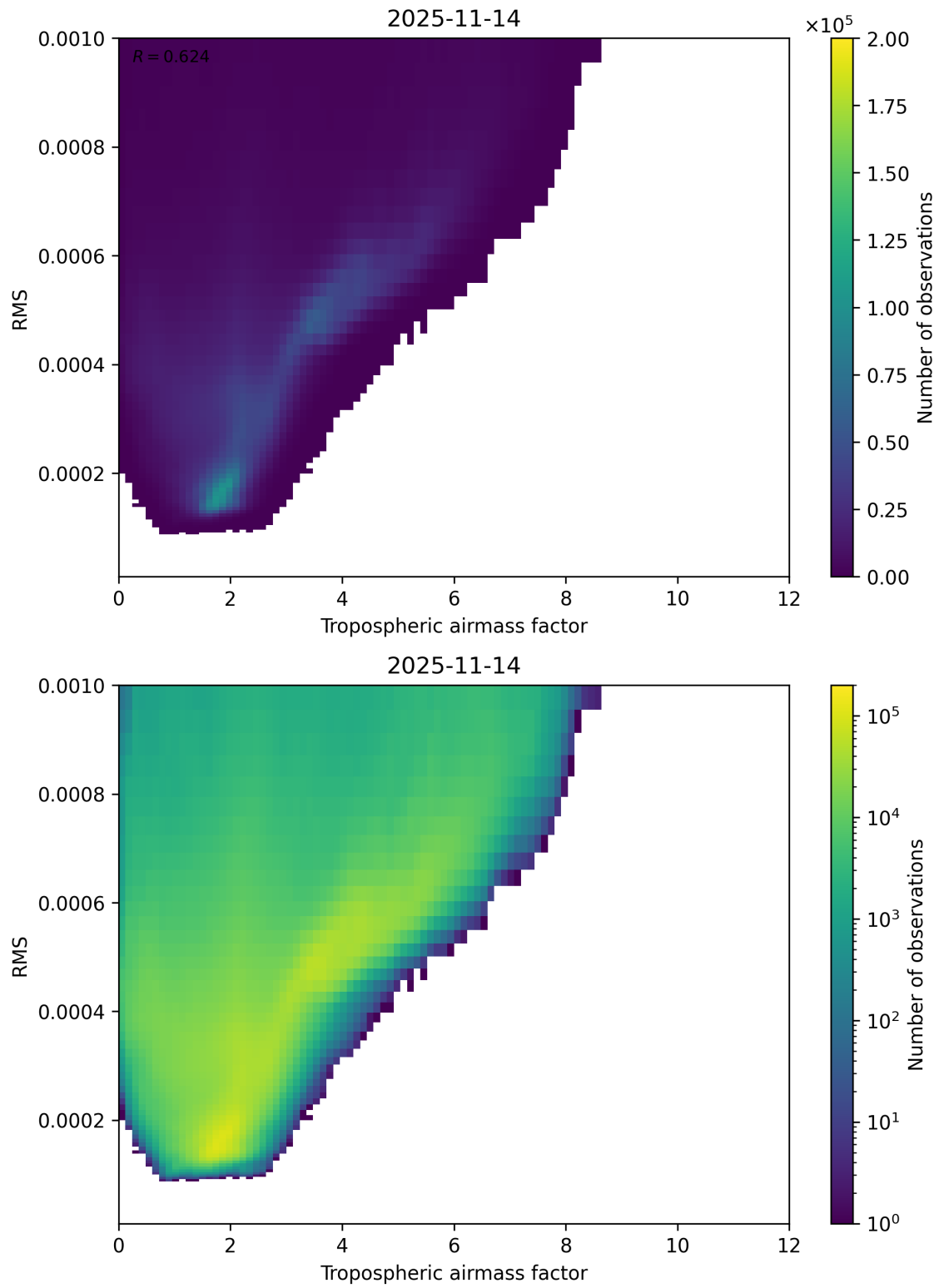
Figure 79: Scatter density plot of “Tropospheric airmass factor” against “RMS” for 2025-11-13 to 2025-11-15.
