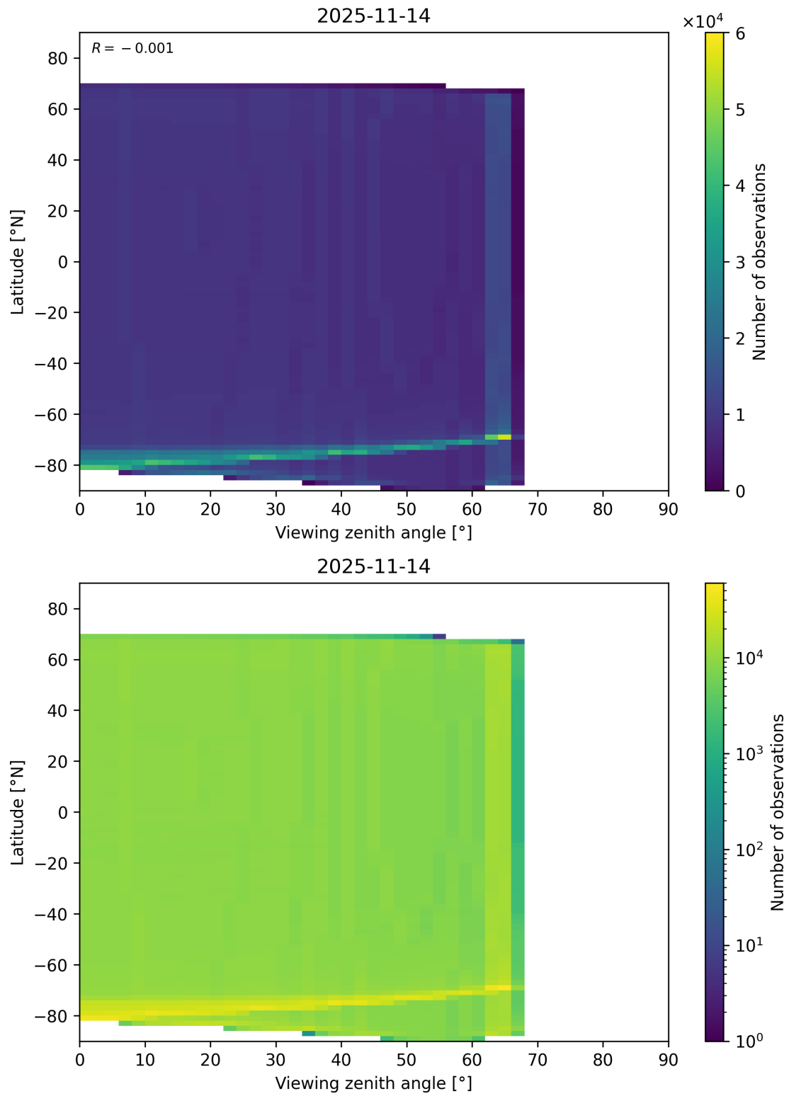
Figure 163: Scatter density plot of “Viewing zenith angle” against “Latitude” for 2025-11-13 to 2025-11-15.
