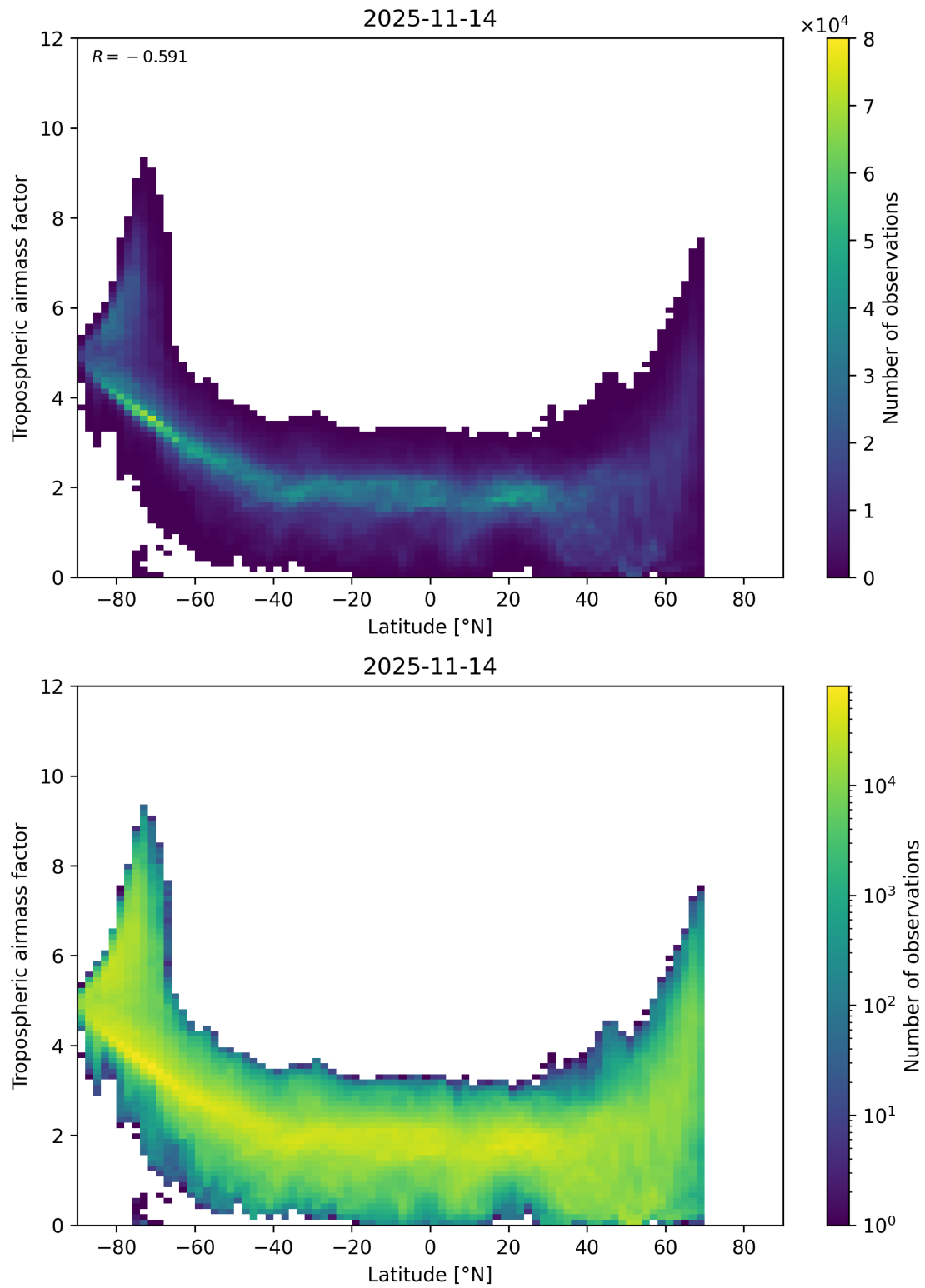
Figure 85: Scatter density plot of “Latitude” against “Tropospheric air mass factor” for 2025-11-13 to 2025-11-15.
