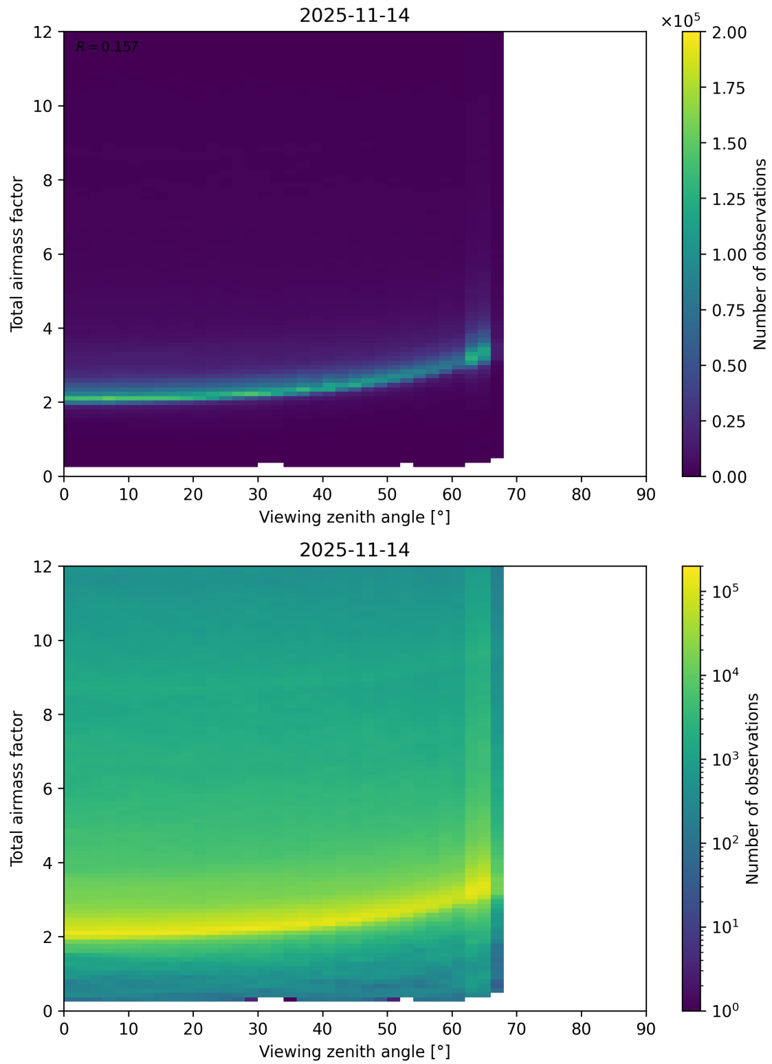
Figure 160: Scatter density plot of “Viewing zenith angle” against “Total airmass factor” for 2025-11-13 to 2025-11-15.
