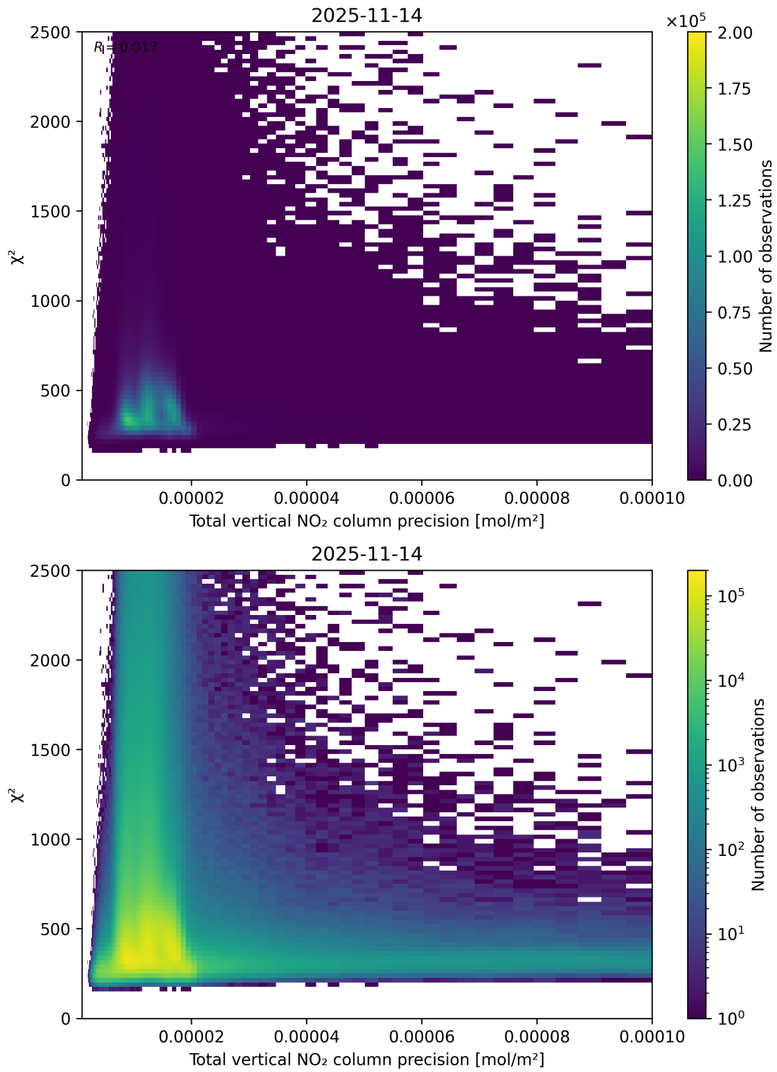
Figure 116: Scatter density plot of “Total vertical NO 2 column precision” against “ \chi^2 ” for 2025-11-13 to 2025-11-15.
