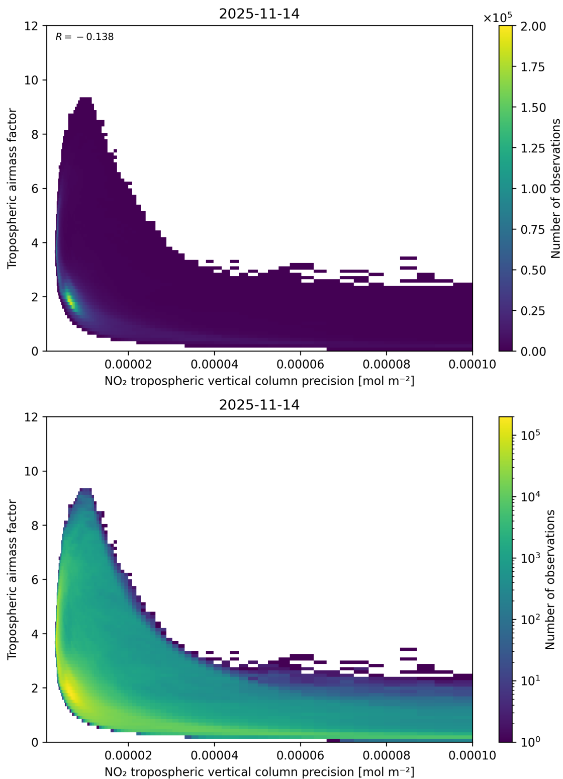
Figure 133: Scatter density plot of “NO 2 tropospheric vertical column precision” against “Tropospheric air mass factor” for 2025-11-13 to 2025-11-15.
