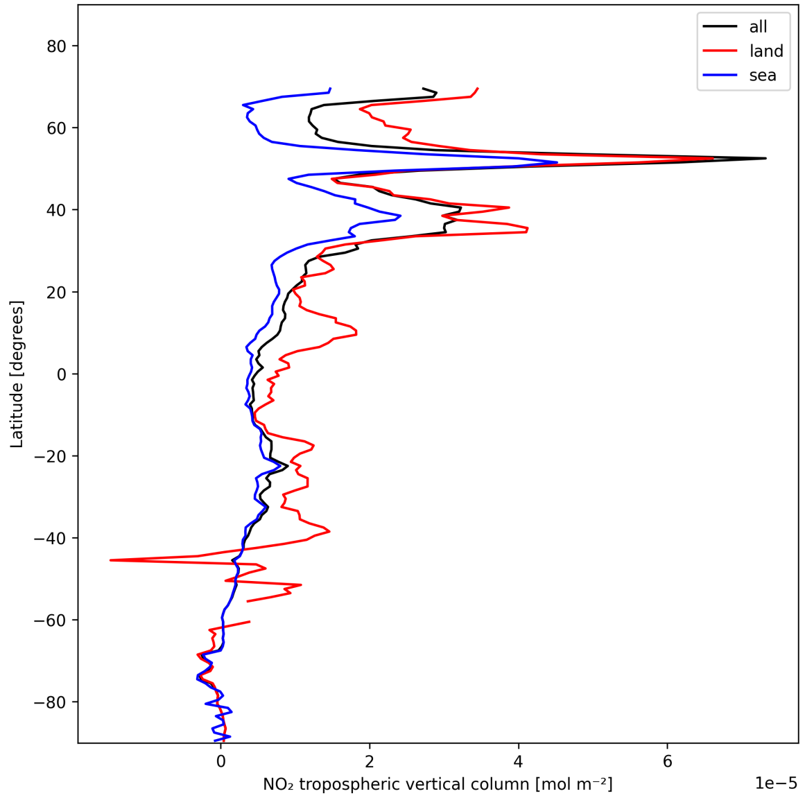
Figure 12: Zonal average of “NO 2 tropospheric vertical column” for 2025-11-13 to 2025-11-15.
