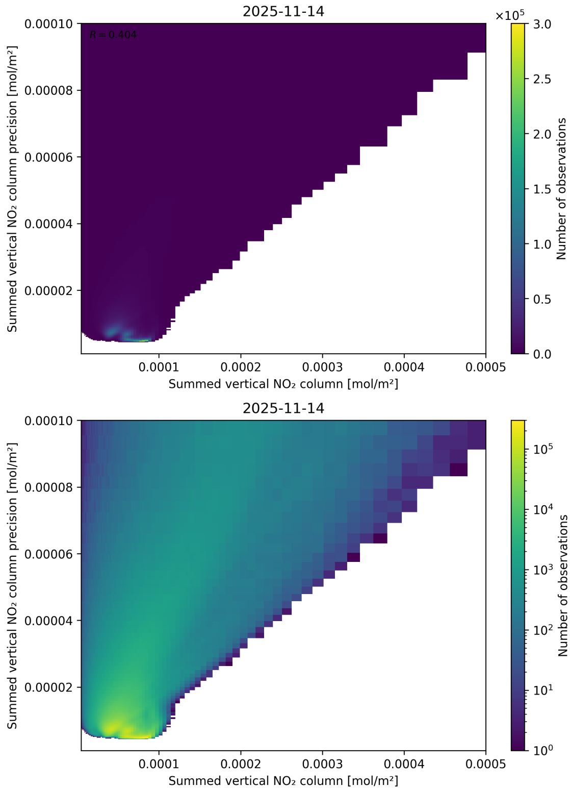
Figure 105: Scatter density plot of “Summed vertical NO 2 column” against “Summed vertical NO 2 column precision” for 2025-11-13 to 2025-11-15.
