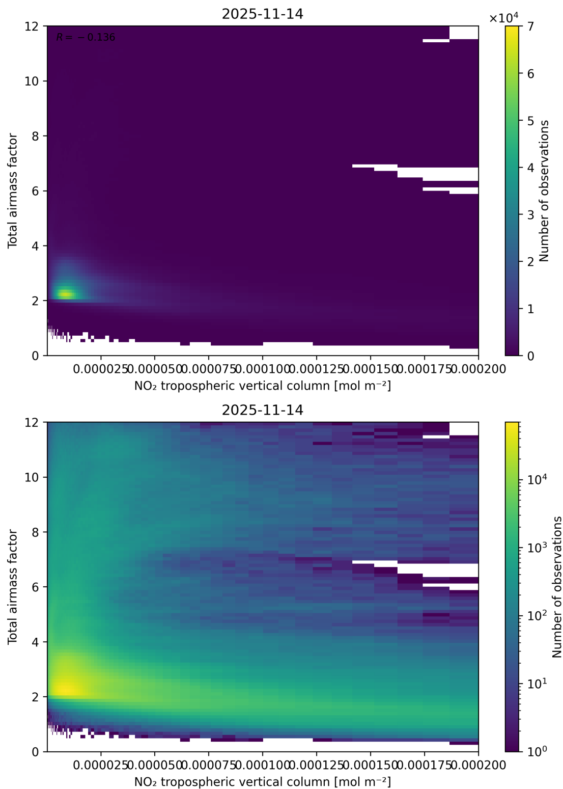
Figure 122: Scatter density plot of “NO 2 tropospheric vertical column” against “Total air mass factor” for 2025-11-13 to 2025-11-15.
