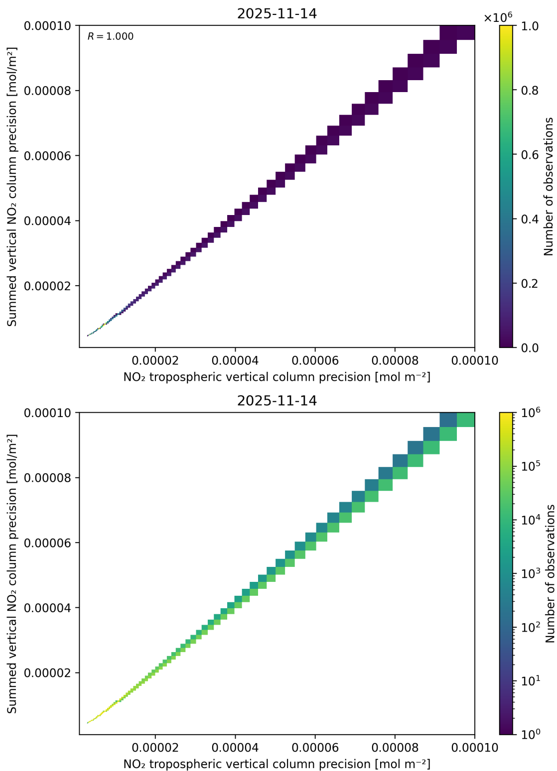
Figure 137: Scatter density plot of “NO 2 tropospheric vertical column precision” against “Summed vertical NO 2 column precision” for 2025-11-13 to 2025-11-15.
