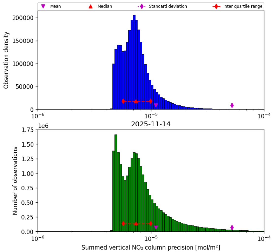
Figure 41: Histogram of "Summed vertical NO 2 column precision" for 2025-11-13 to 2025-11-15
