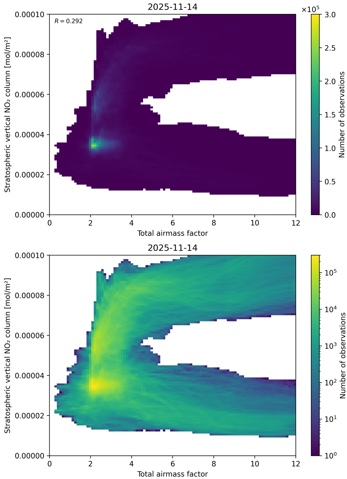
Figure 64: Scatter density plot of “Total airmass factor” against “Stratospheric vertical NO 2 column” for 2025-11-13 to 2025-11-15.
