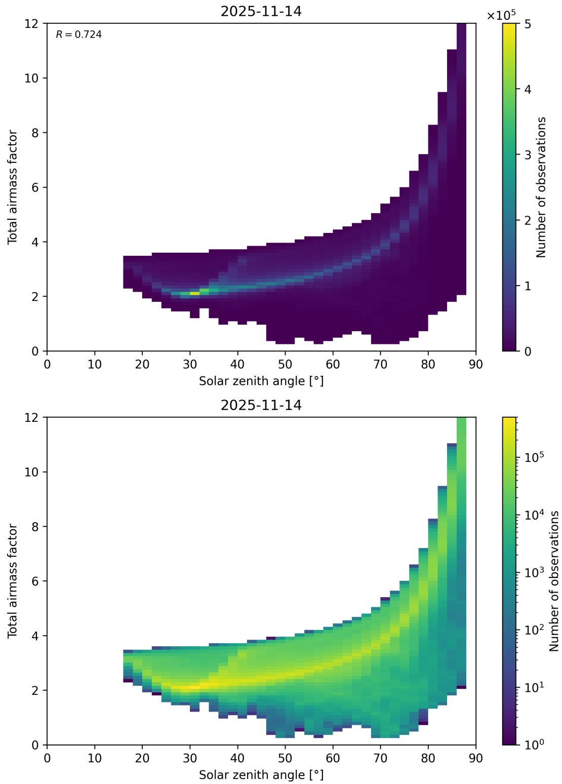
Figure 146: Scatter density plot of “Solar zenith angle” against “Total air mass factor” for 2025-11-13 to 2025-11-15.
