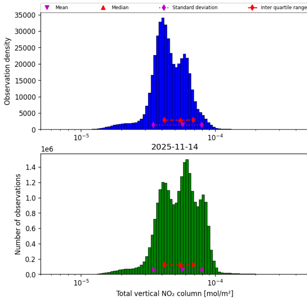
Figure 38: Histogram of “Total vertical NO 2 column” for 2025-11-13 to 2025-11-15
