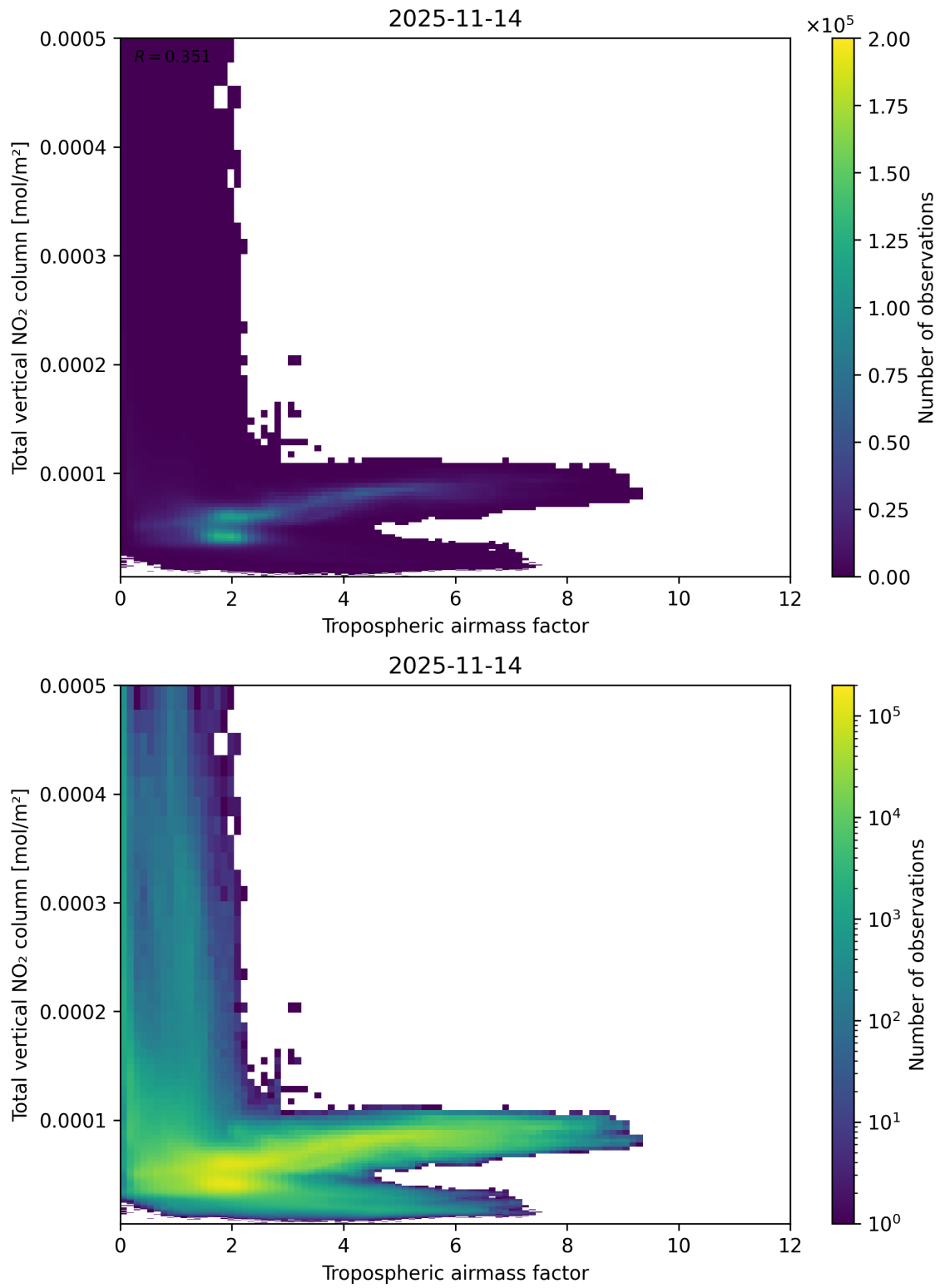
Figure 77: Scatter density plot of “Tropospheric airmass factor” against “Total vertical NO 2 column” for 2025-11-13 to 2025-11-15.
