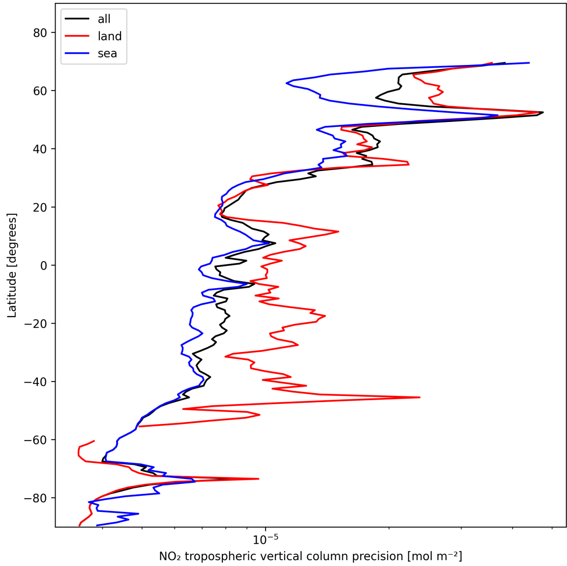
Figure 13: Zonal average of “NO 2 tropospheric vertical column precision” for 2025-11-13 to 2025-11-15.
