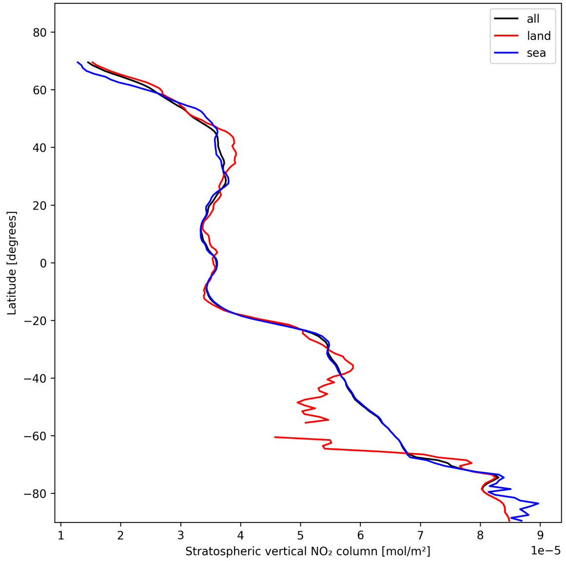
Figure 19: Zonal average of “Stratospheric vertical NO 2 column” for 2025-11-13 to 2025-11-15.
