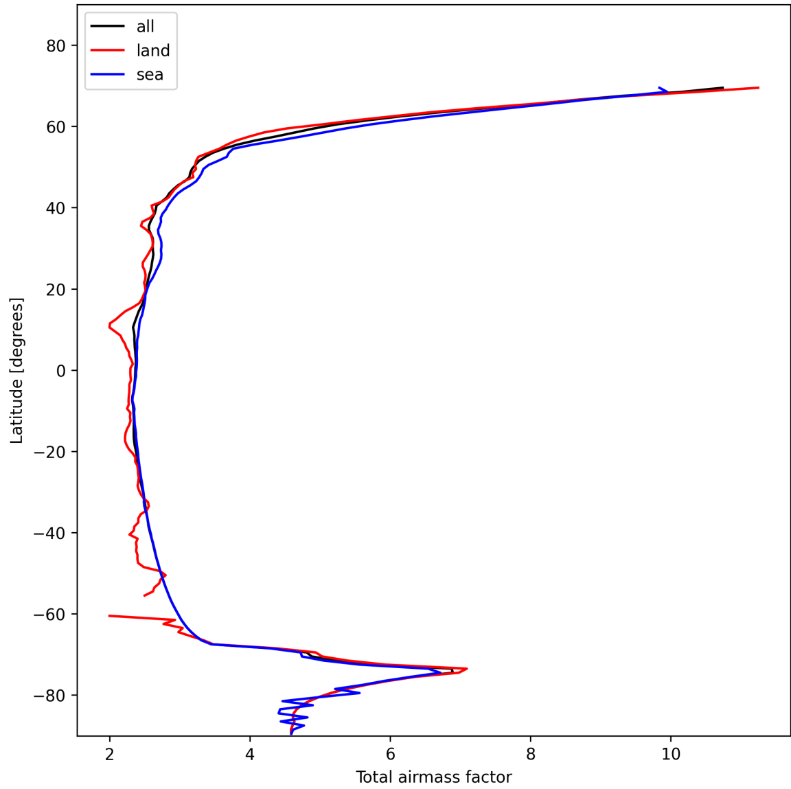
Figure 15: Zonal average of “Total airmass factor” for 2025-11-13 to 2025-11-15.
