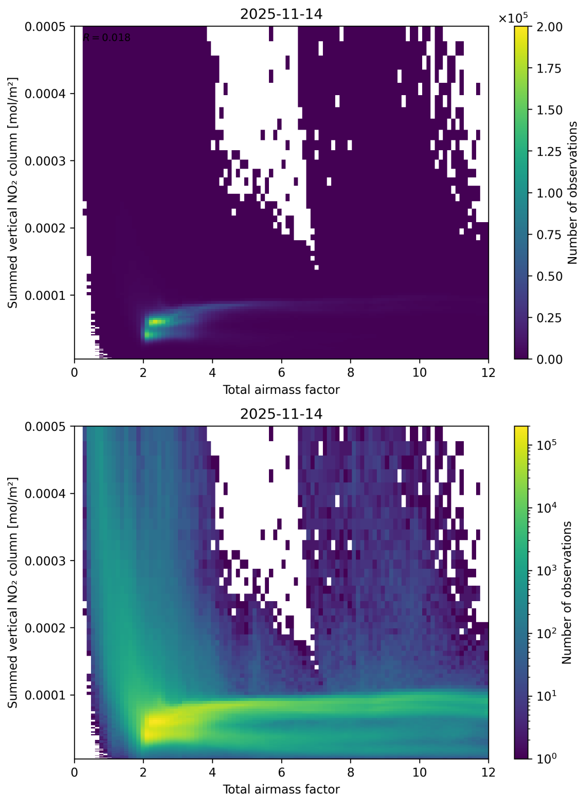
Figure 65: Scatter density plot of “Total airmass factor” against “Summed vertical NO 2 column” for 2025-11-13 to 2025-11-15.
