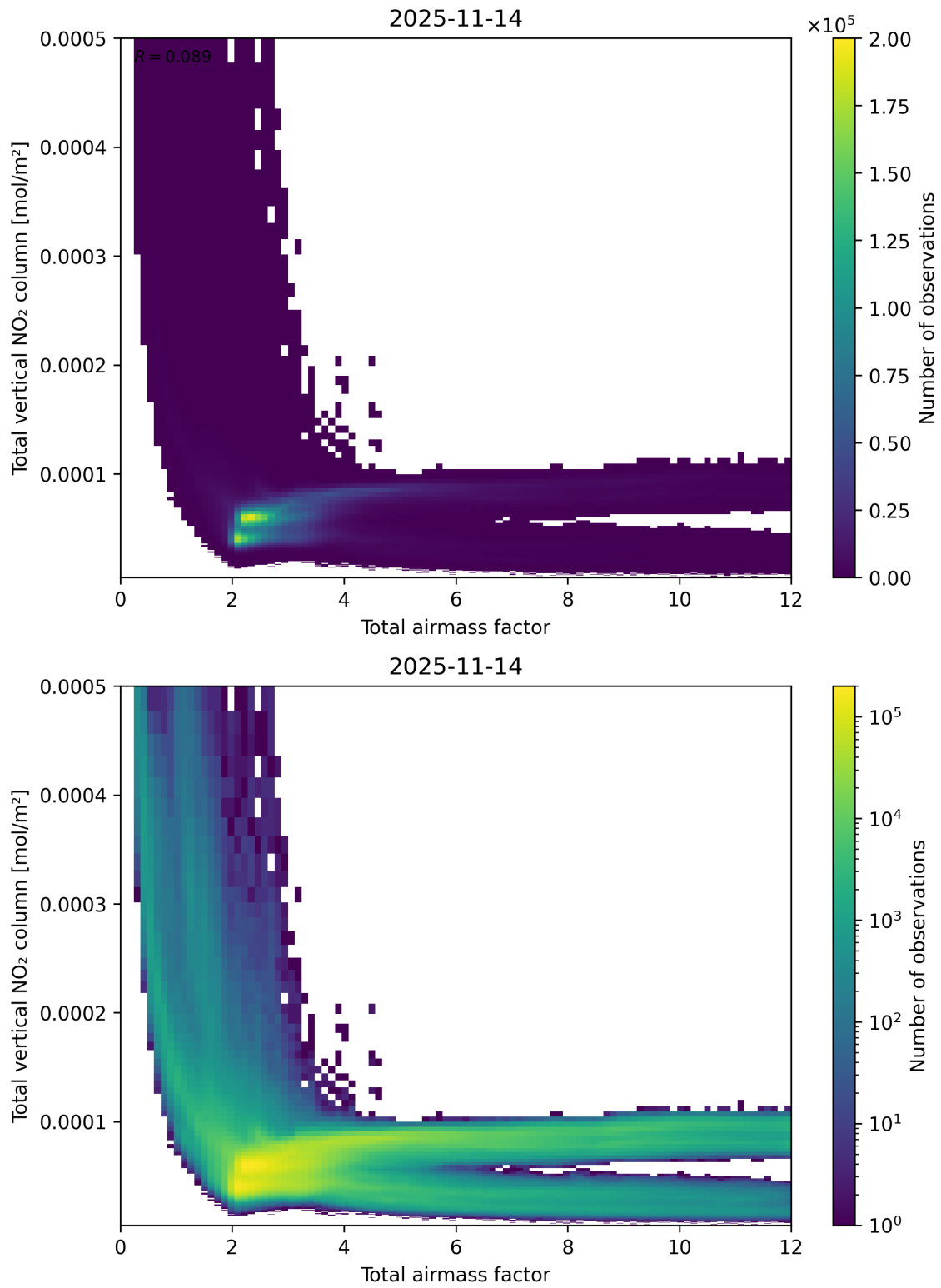
Figure 67: Scatter density plot of “Total airmass factor” against “Total vertical NO 2 column” for 2025-11-13 to 2025-11-15.
