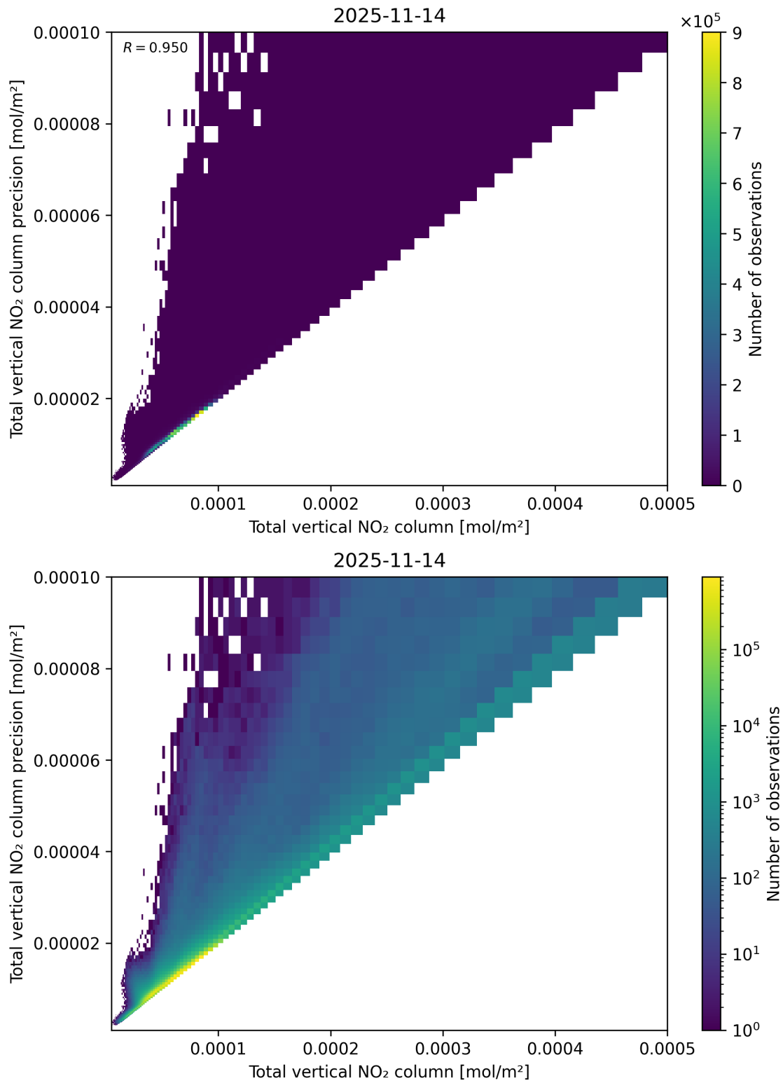
Figure 114: Scatter density plot of “Total vertical NO 2 column” against “Total vertical NO 2 column precision” for 2025-11-13 to 2025-11-15.
