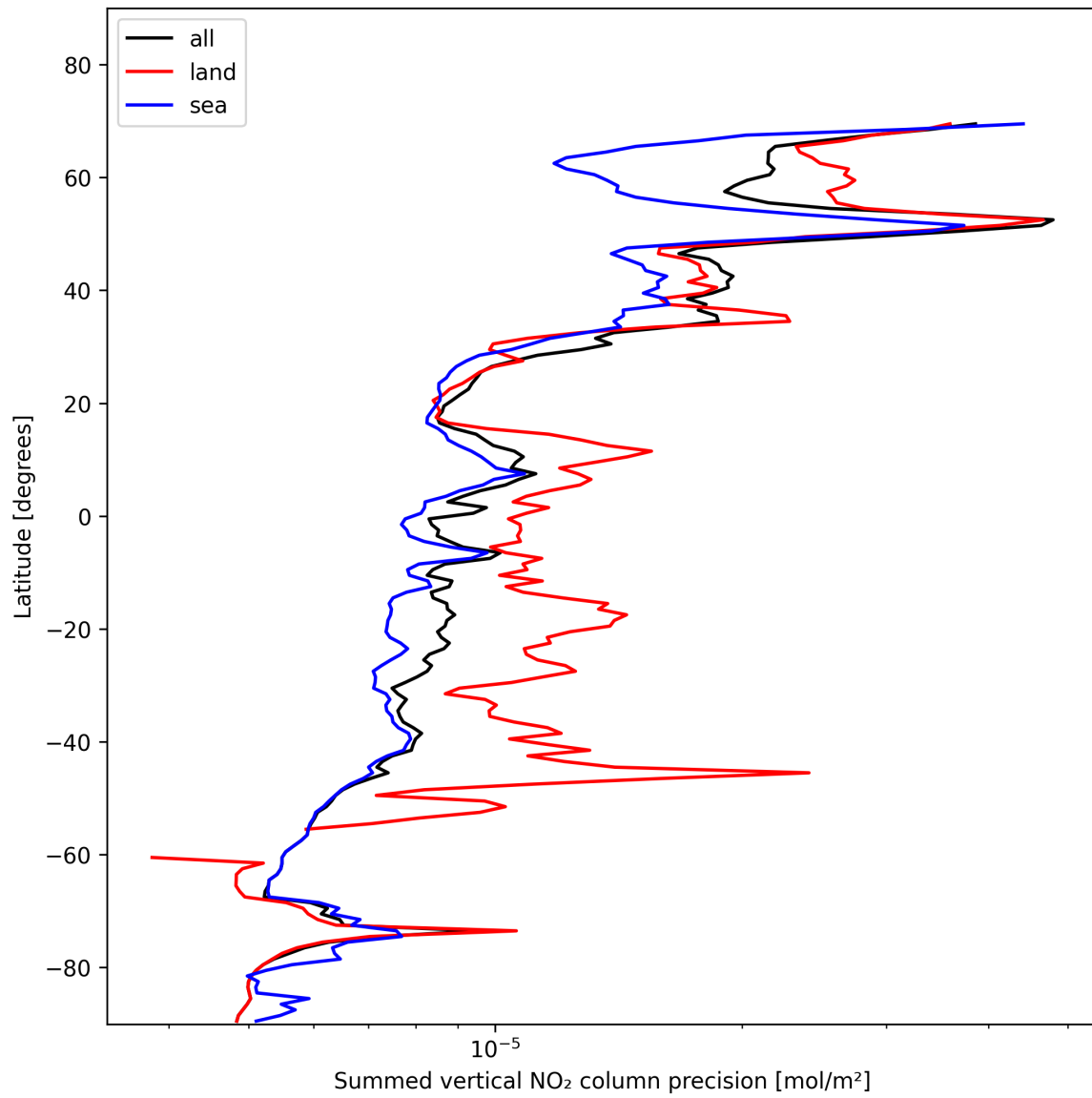
Figure 24: Zonal average of “Summed vertical NO 2 column precision” for 2025-11-13 to 2025-11-15.
