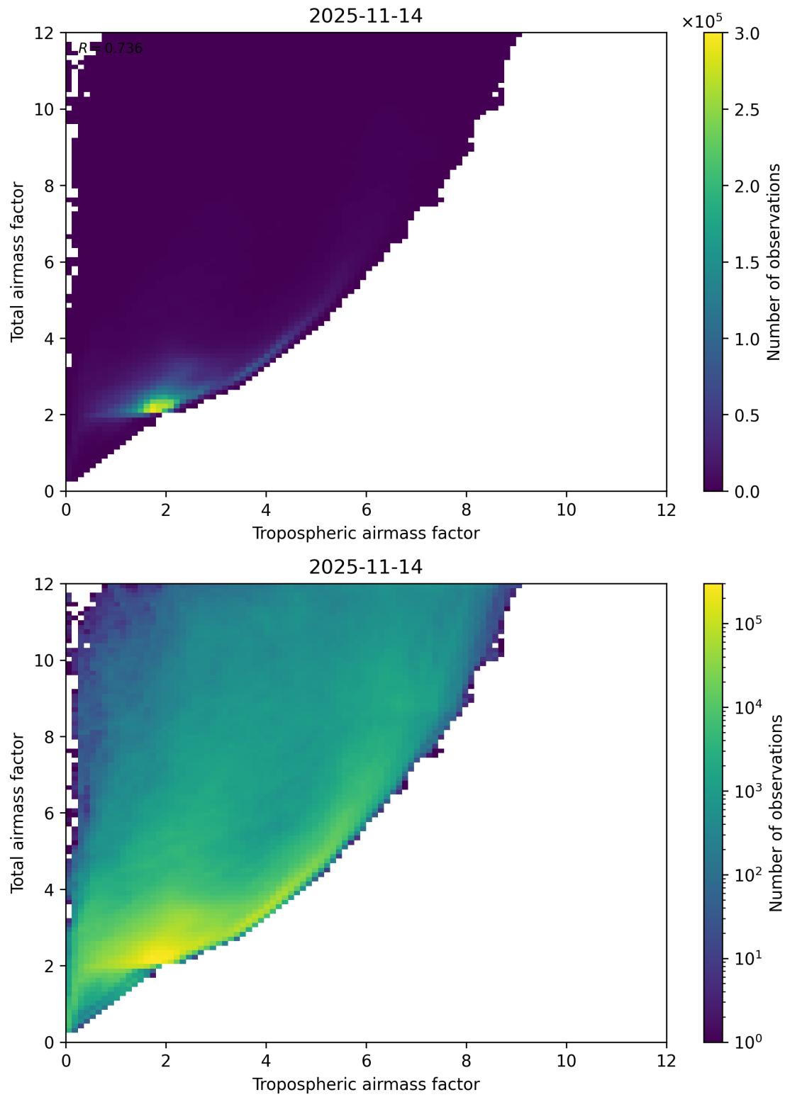
Figure 72: Scatter density plot of “Tropospheric airmass factor” against “Total airmass factor” for 2025-11-13 to 2025-11-15.
