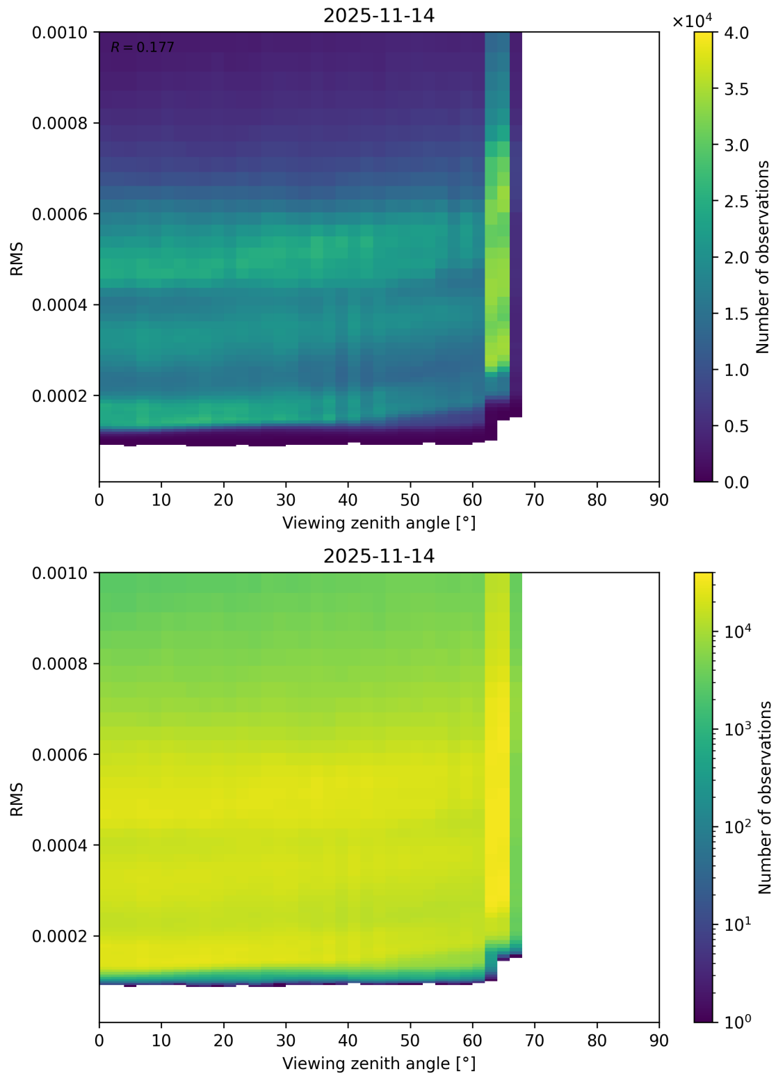
Figure 171: Scatter density plot of “Viewing zenith angle” against “RMS” for 2025-11-13 to 2025-11-15.
