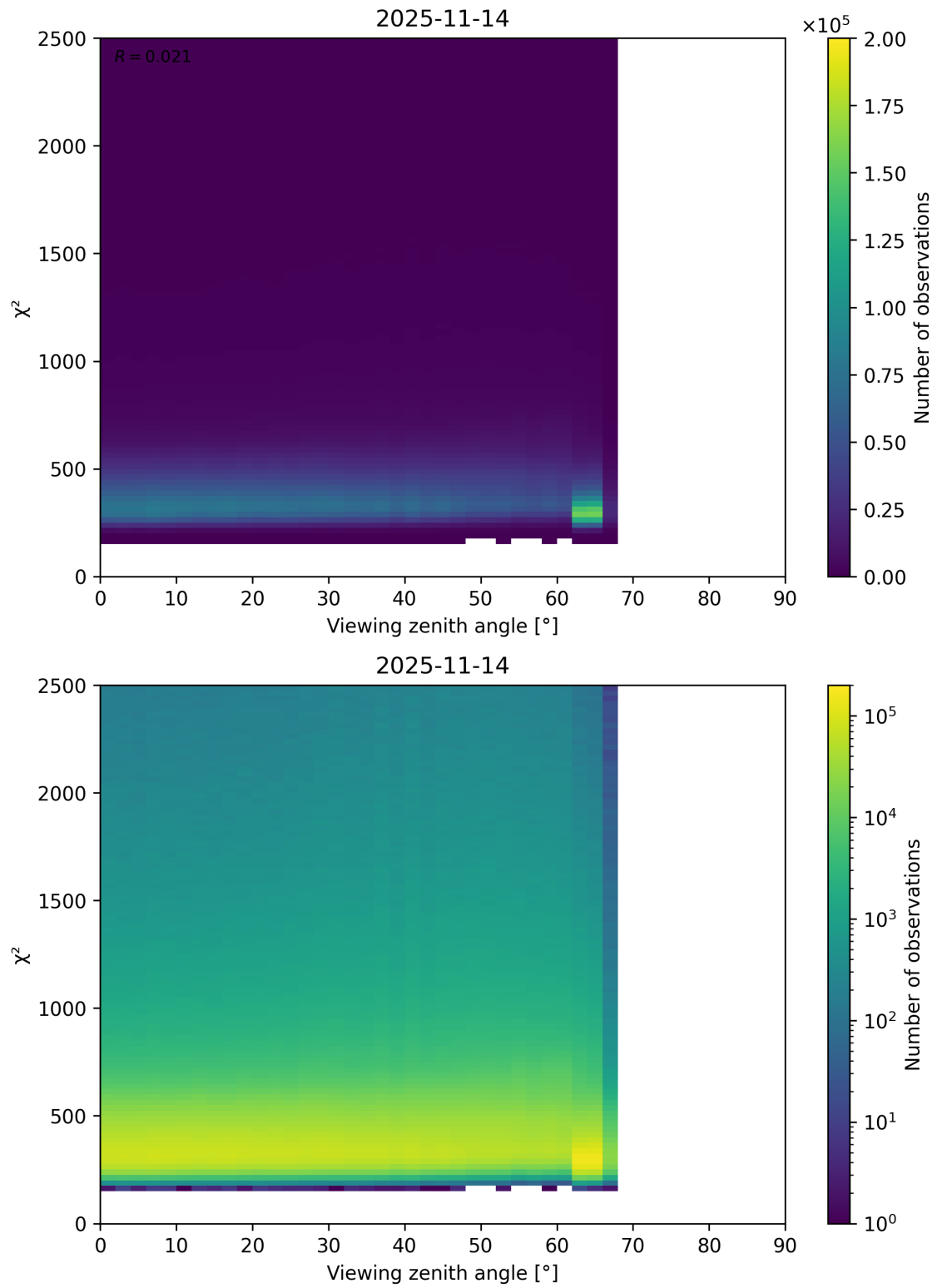
Figure 162: Scatter density plot of “Viewing zenith angle” against “ \chi^2 ” for 2025-11-13 to 2025-11-15.
