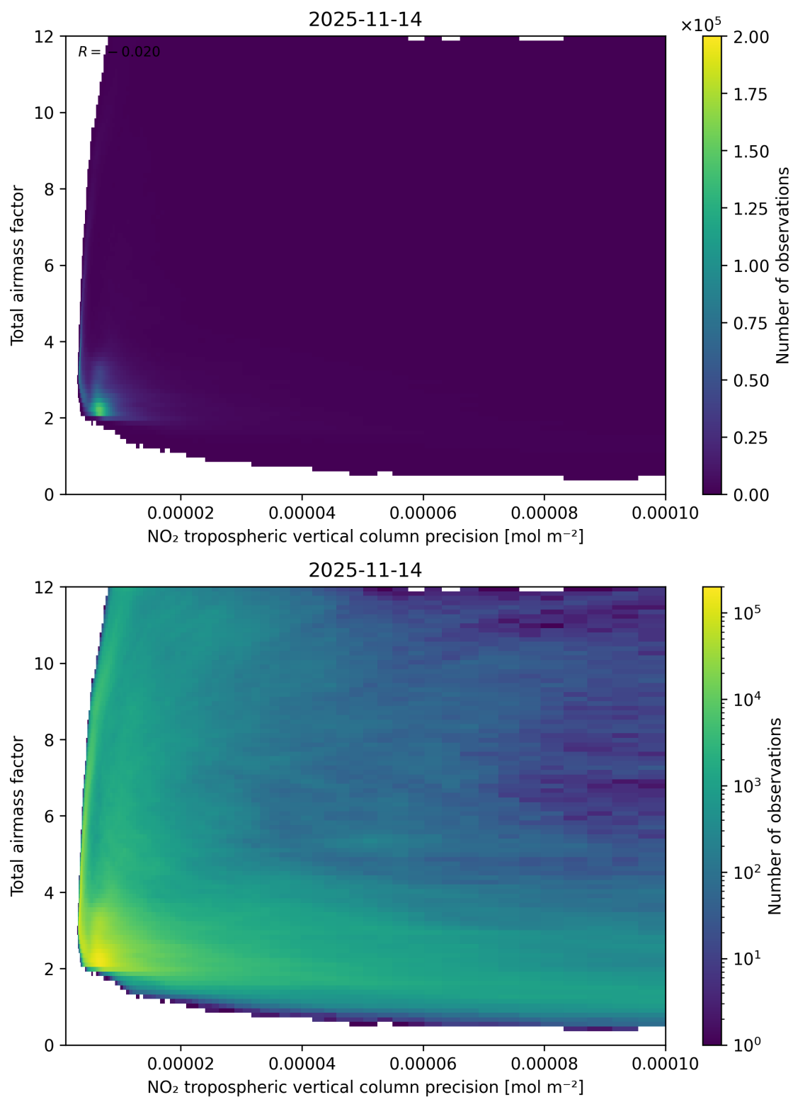
Figure 132: Scatter density plot of “NO 2 tropospheric vertical column precision” against “Total air mass factor” for 2025-11-13 to 2025-11-15.
