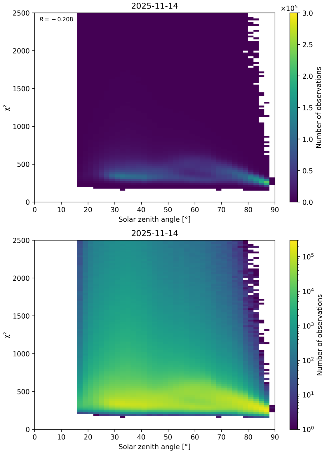
Figure 148: Scatter density plot of “Solar zenith angle” against “ \chi^2 ” for 2025-11-13 to 2025-11-15.
