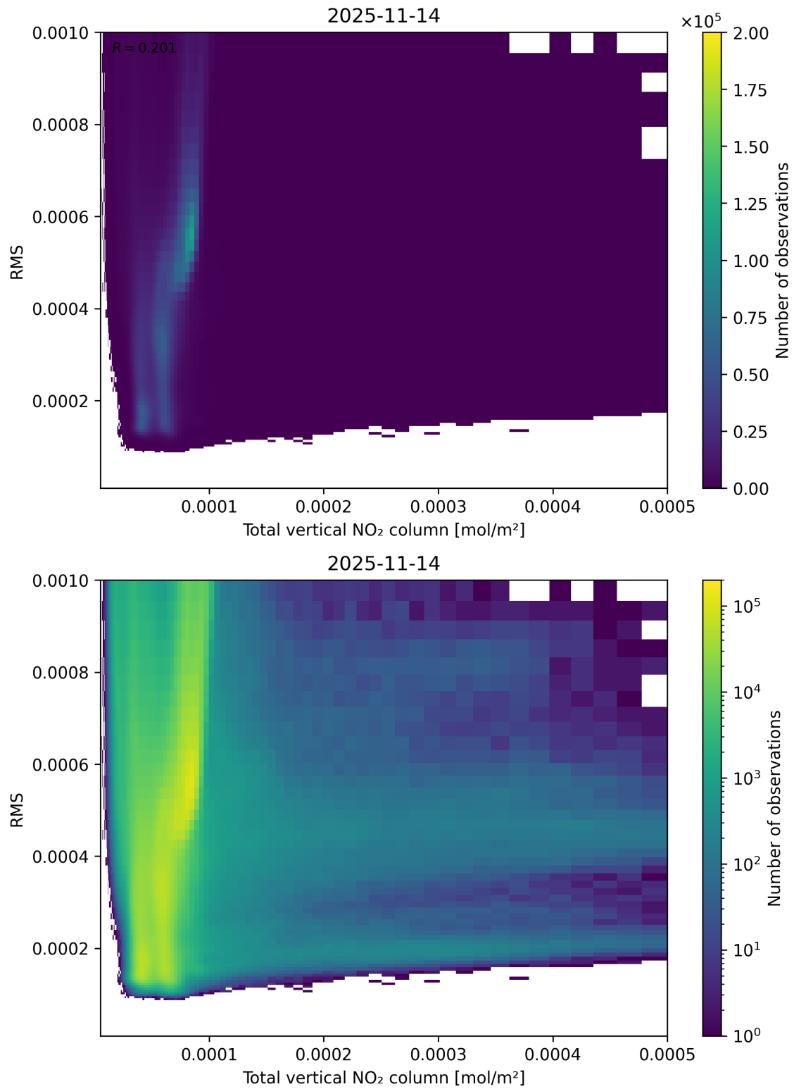
Figure 120: Scatter density plot of “Total vertical NO 2 column” against “RMS” for 2025-11-13 to 2025-11-15.
