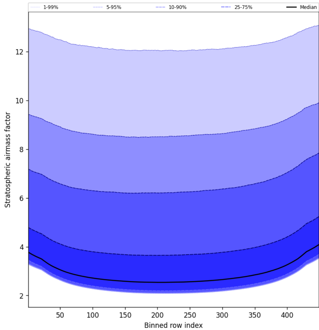
Figure 61: Along track statistics of “Stratospheric air mass factor” for 2025-11-13 to 2025-11-15
