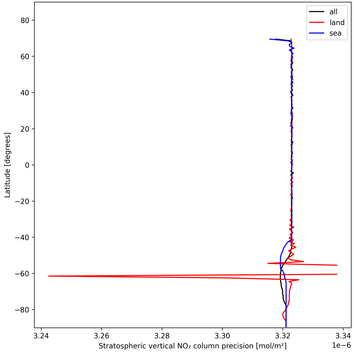
Figure 20: Zonal average of "Stratospheric vertical NO 2 column precision" for 2025-11-13 to 2025-11-15.
