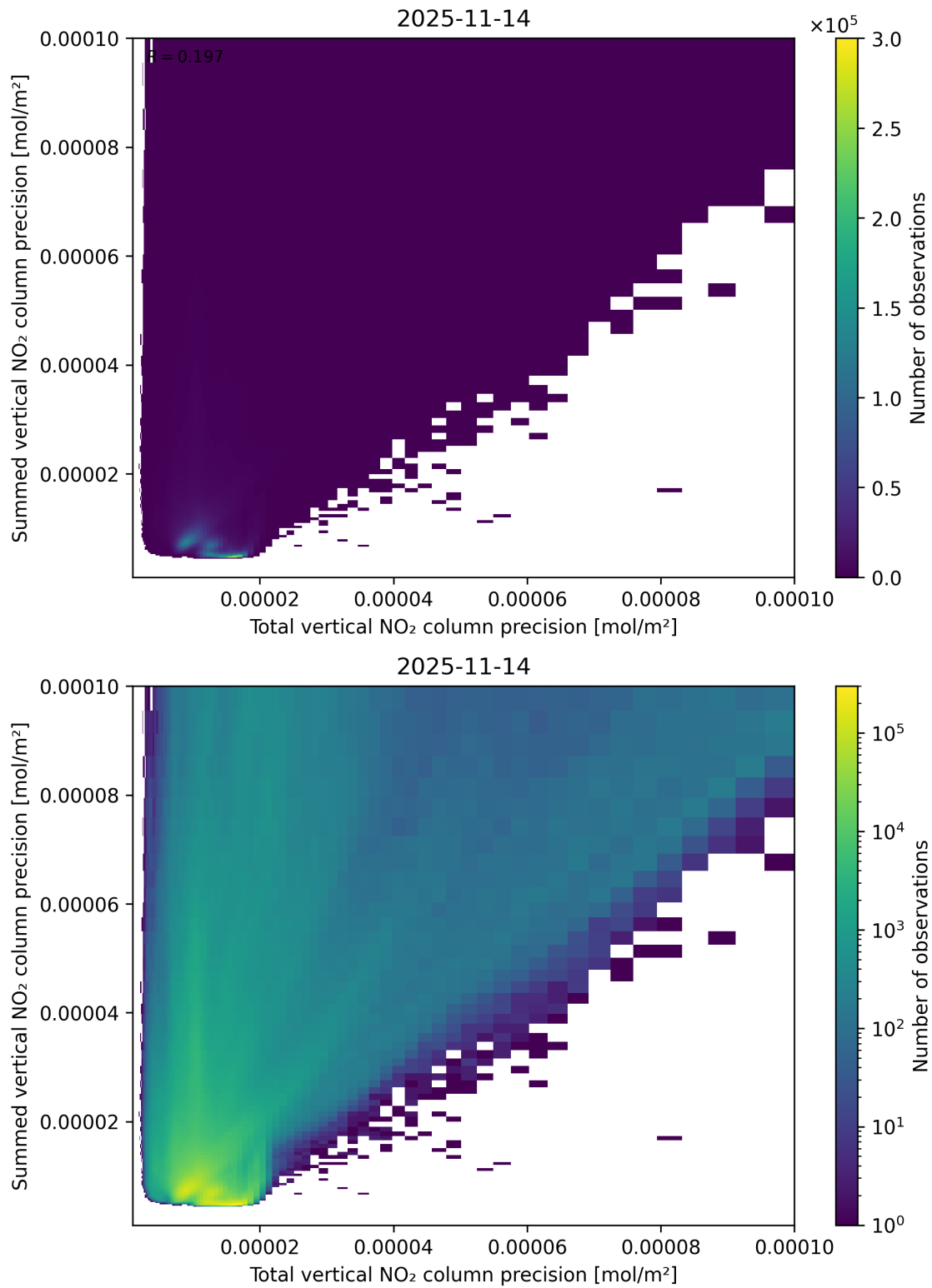
Figure 118: Scatter density plot of “Total vertical NO 2 column precision” against “Summed vertical NO 2 column precision” for 2025-11-13 to 2025-11-15.
