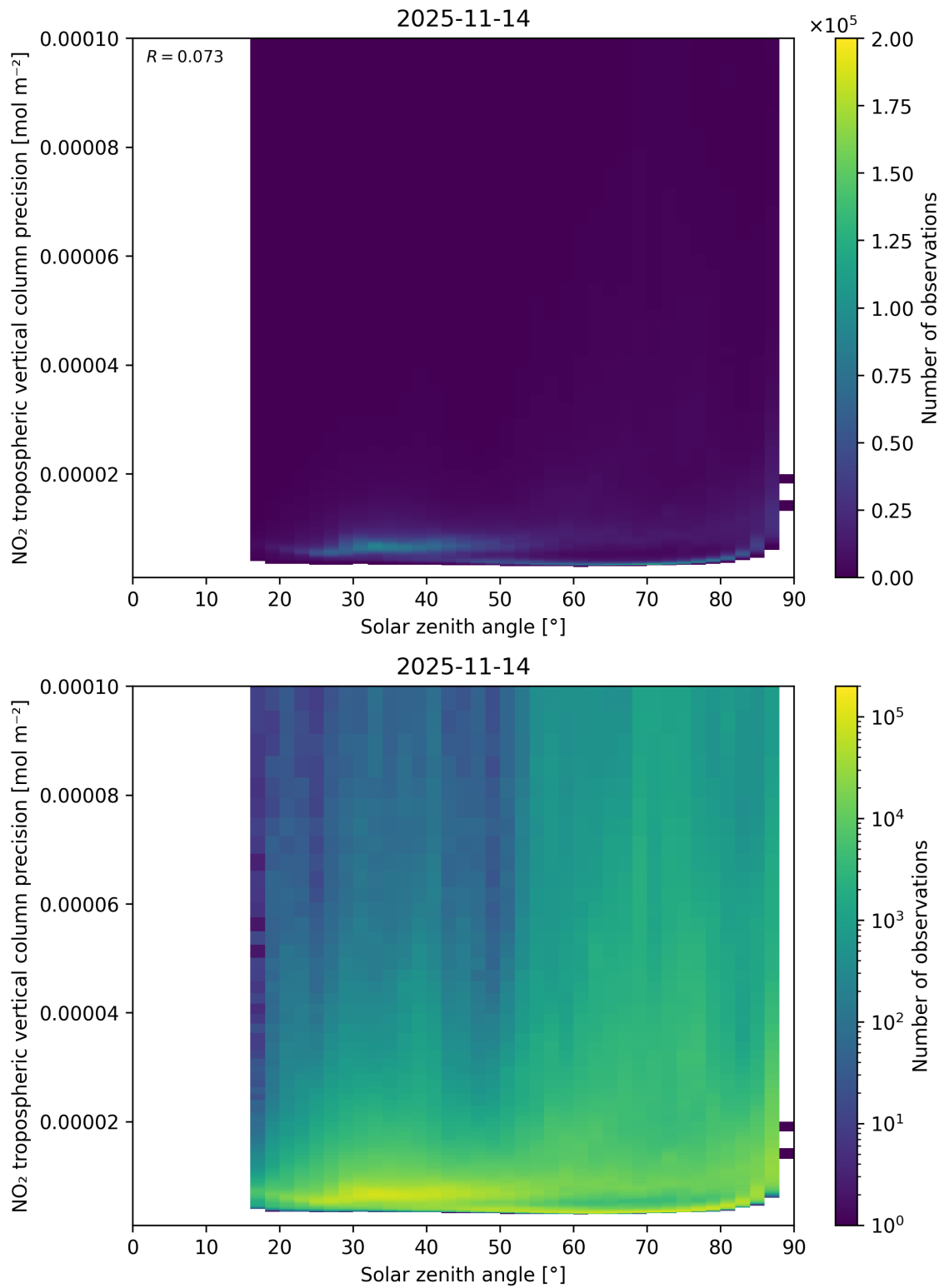
Figure 156: Scatter density plot of “Solar zenith angle” against “NO 2 tropospheric vertical column precision” for 2025-11-13 to 2025-11-15.
