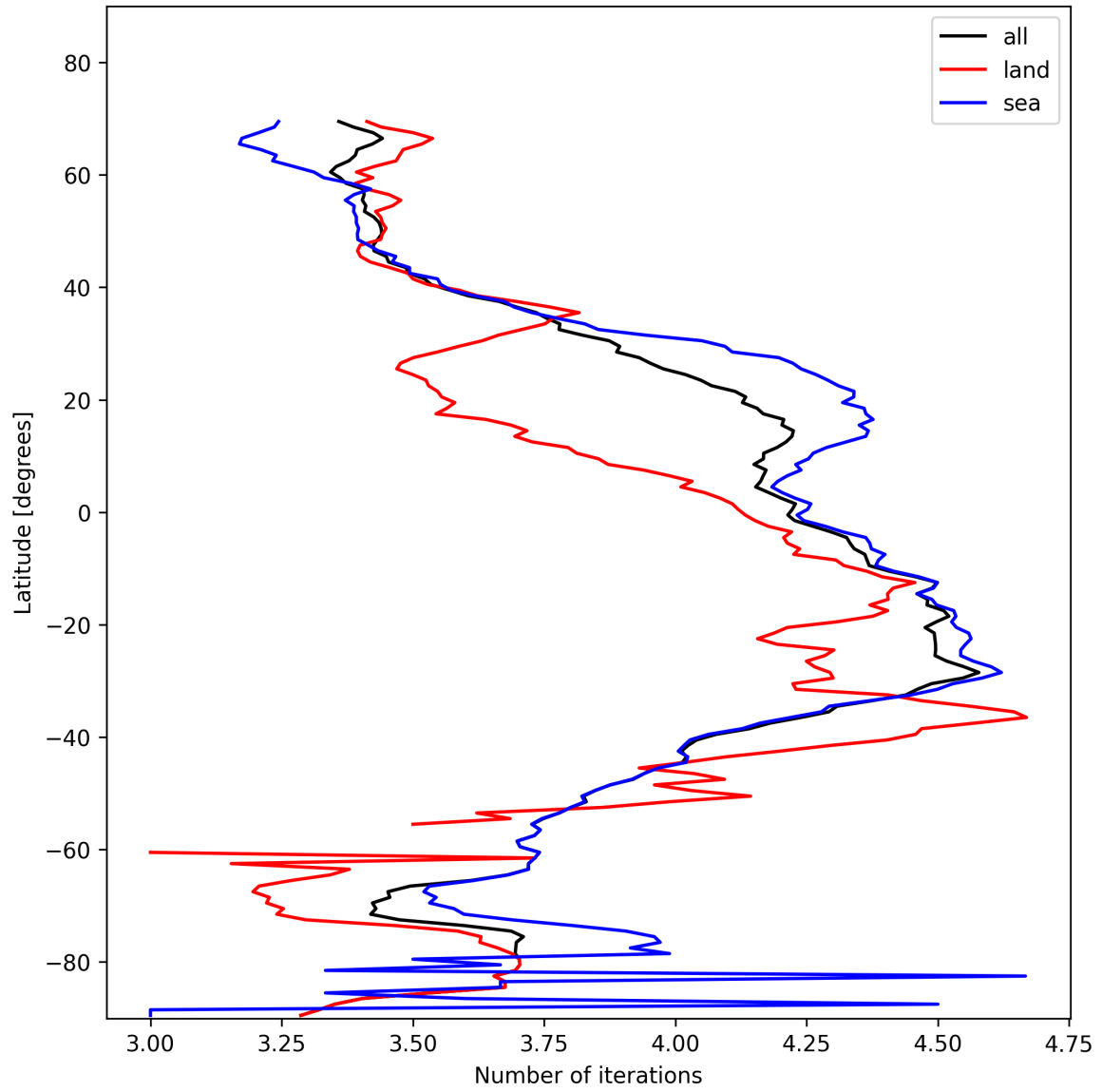
Figure 17: Zonal average of “Number of iterations” for 2025-11-13 to 2025-11-15.
