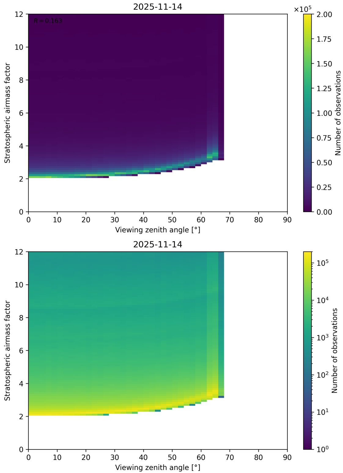
Figure 159: Scatter density plot of “Viewing zenith angle” against “Stratospheric airmass factor” for 2025-11-13 to 2025-11-15.
