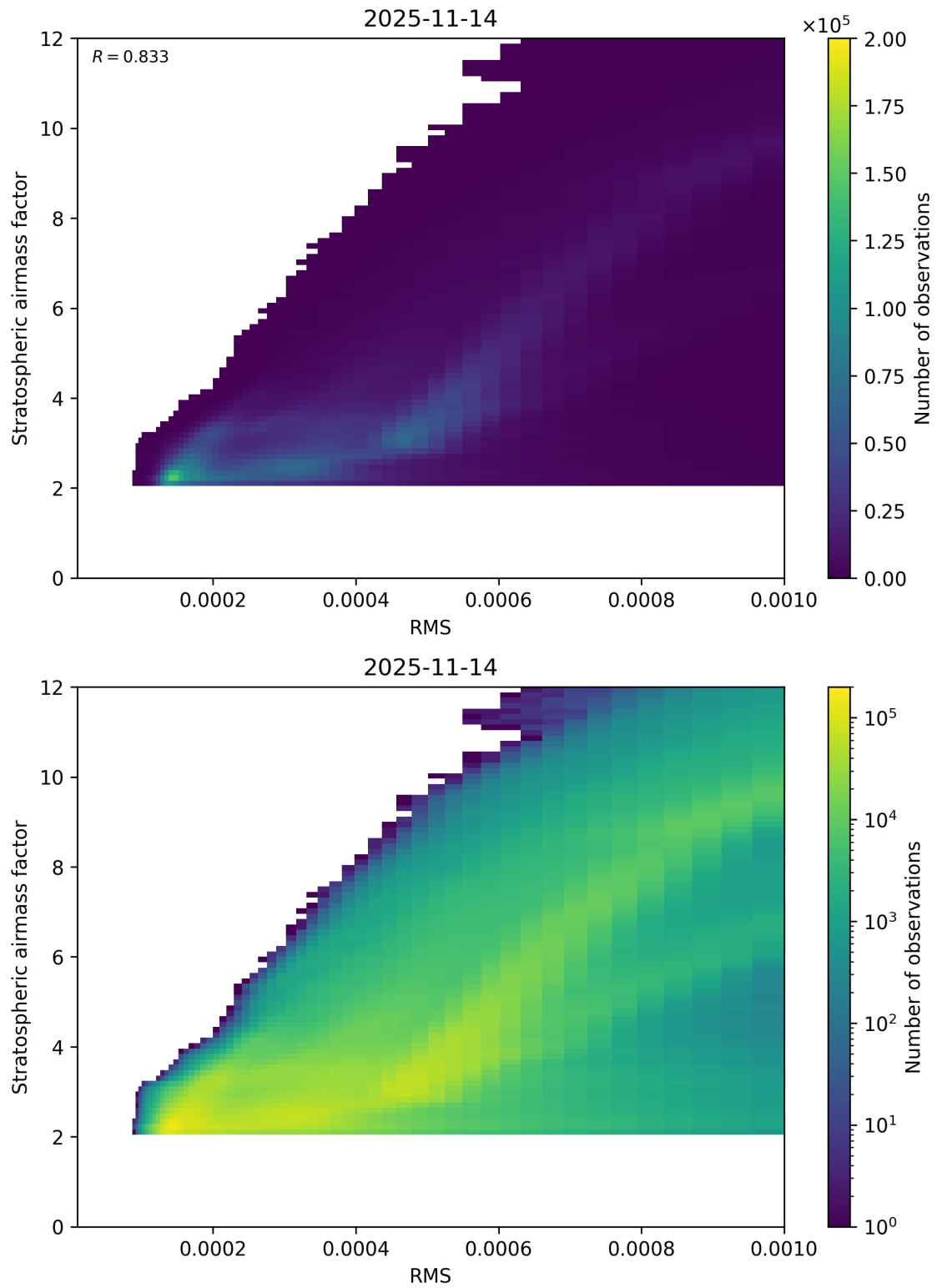
Figure 144: Scatter density plot of “RMS” against “Stratospheric airmass factor” for 2025-11-13 to 2025-11-15.
