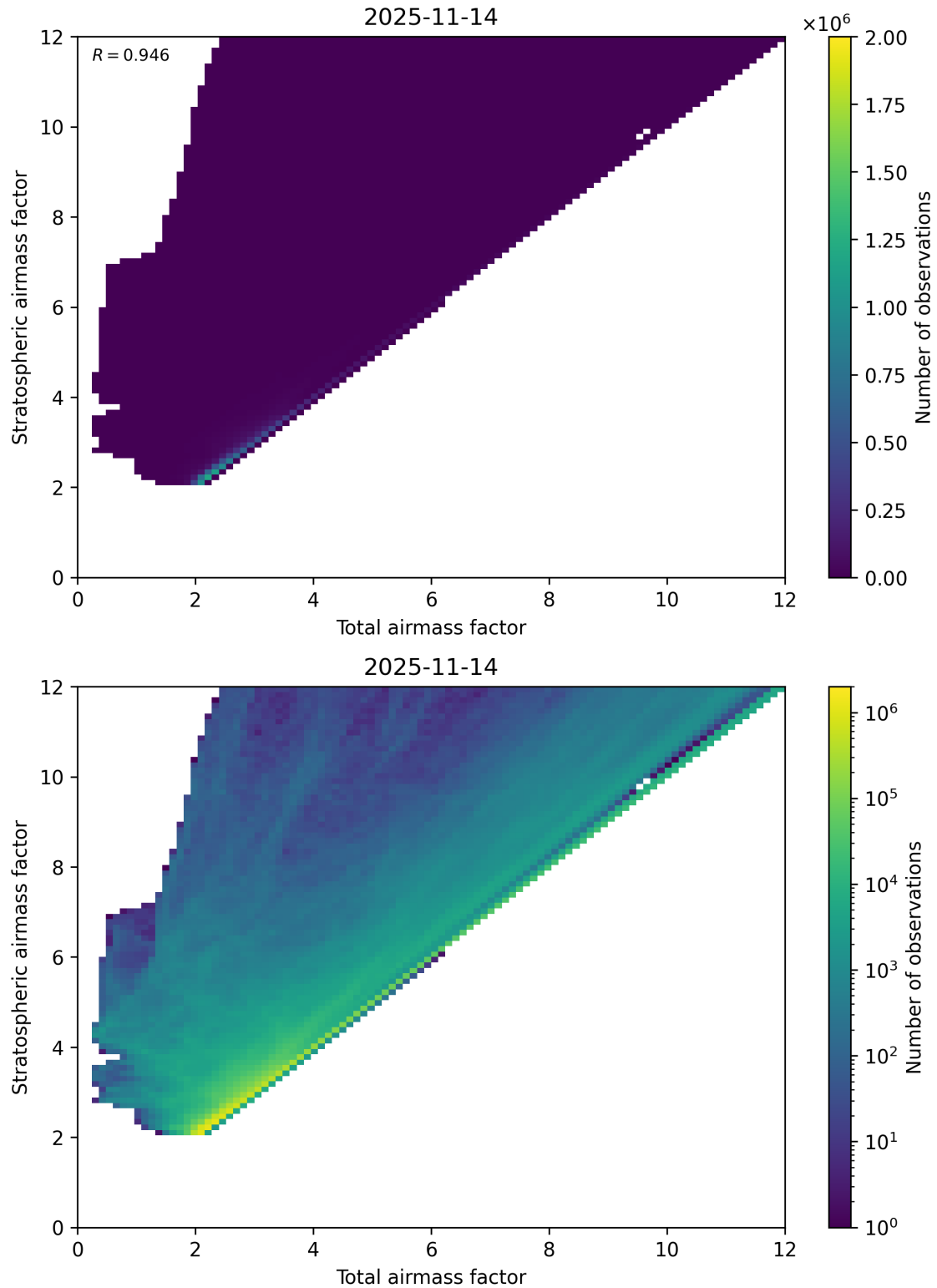
Figure 62: Scatter density plot of “Total airmass factor” against “Stratospheric airmass factor” for 2025-11-13 to 2025-11-15.
