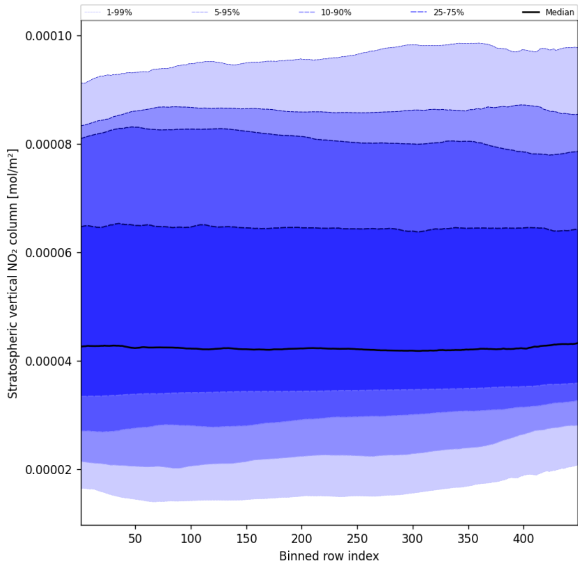
Figure 53: Along track statistics of “Stratospheric vertical NO 2 column” for 2025-11-13 to 2025-11-15
