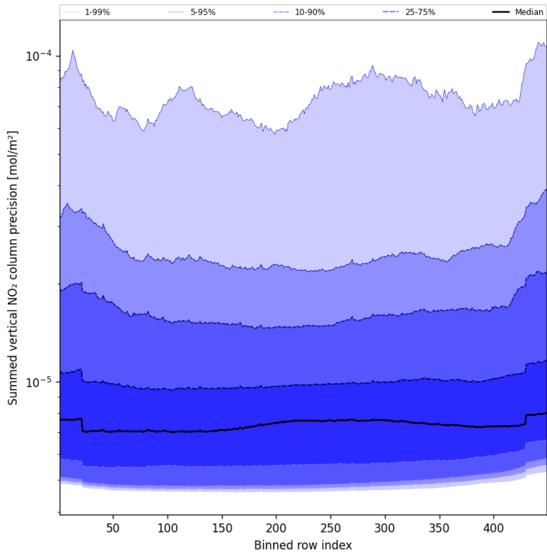
Figure 58: Along track statistics of “Summed vertical NO 2 column precision” for 2025-11-13 to 2025-11-15
