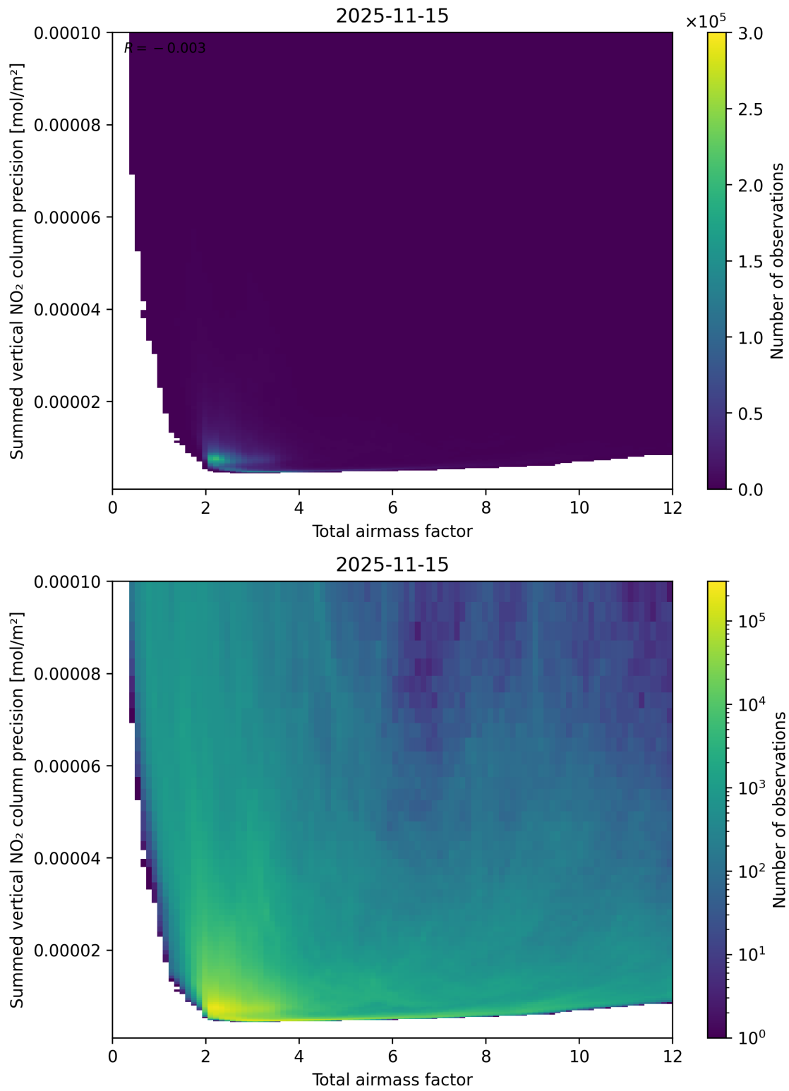
Figure 66: Scatter density plot of “Total airmass factor” against “Summed vertical NO 2 column precision” for 2025-11-14 to 2025-11-16.
