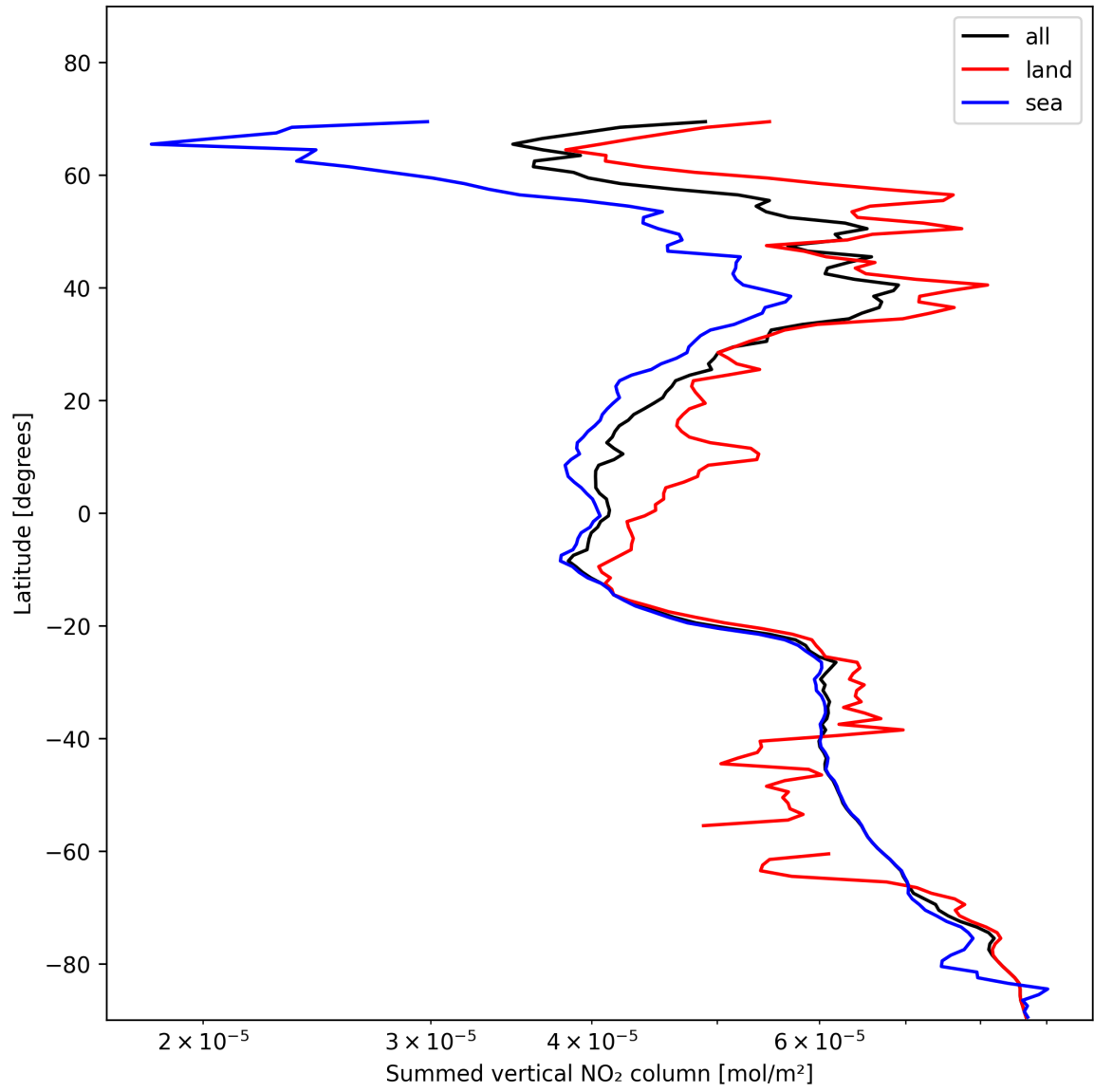
Figure 23: Zonal average of “Summed vertical NO 2 column” for 2025-11-14 to 2025-11-16.
