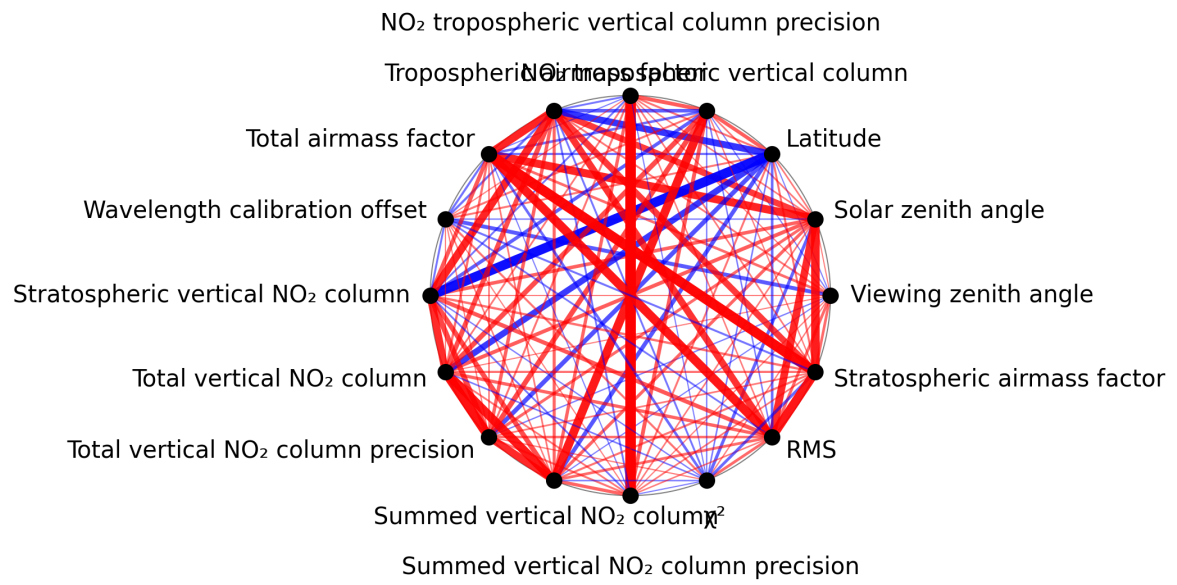
Figure 1: Map of correlation graph for 2025-11-14 to 2025-11-16.
