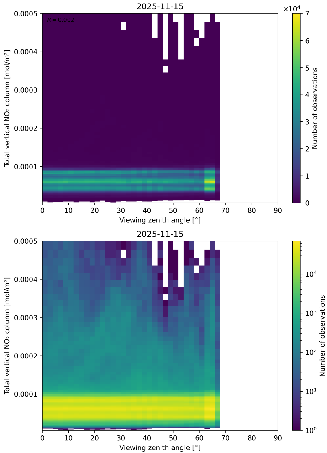
Figure 167: Scatter density plot of “Viewing zenith angle” against “Total vertical NO 2 column” for 2025-11-14 to 2025-11-16.
