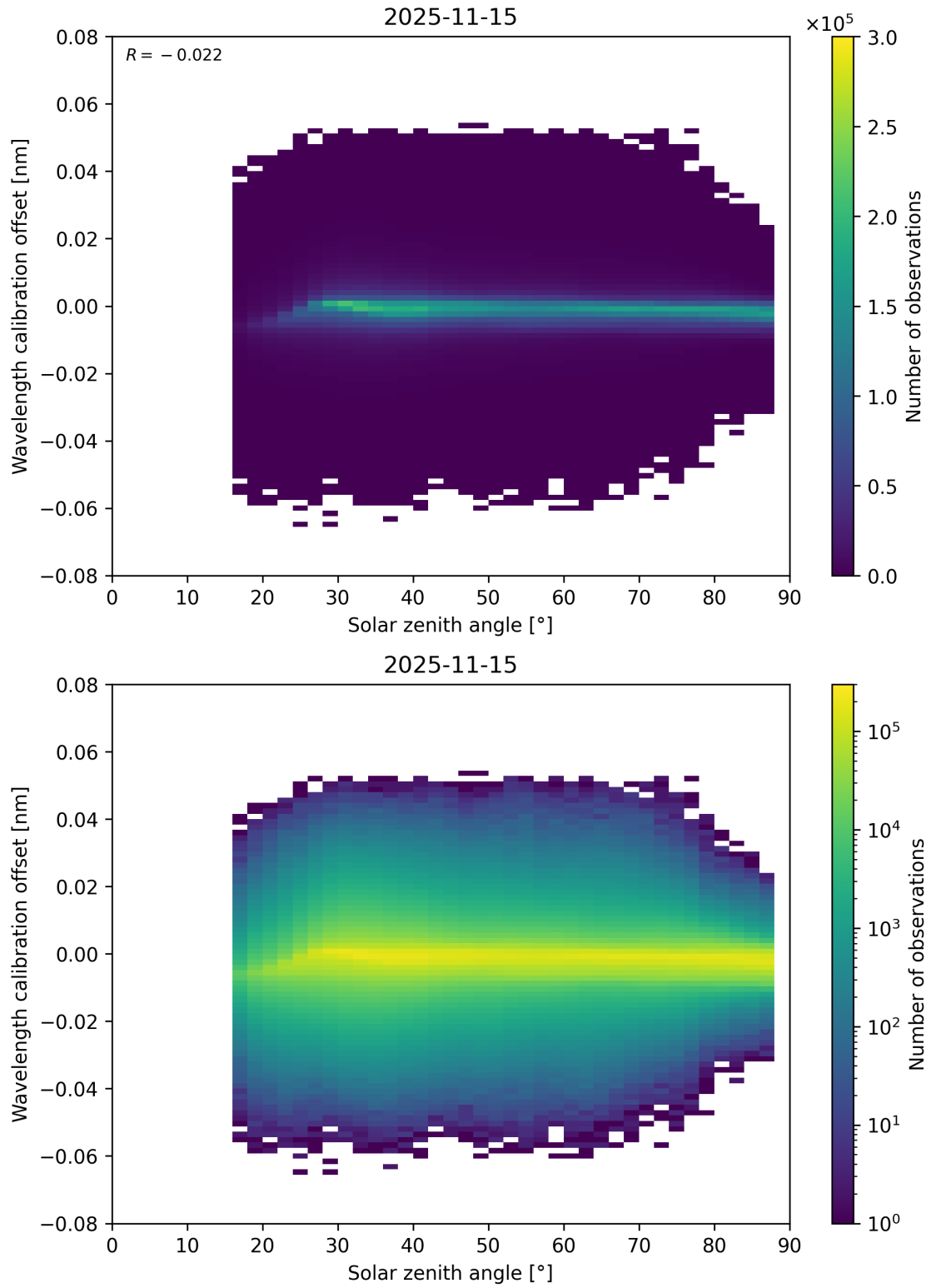
Figure 158: Scatter density plot of “Solar zenith angle” against “Wavelength calibration offset” for 2025-11-14 to 2025-11-16.
