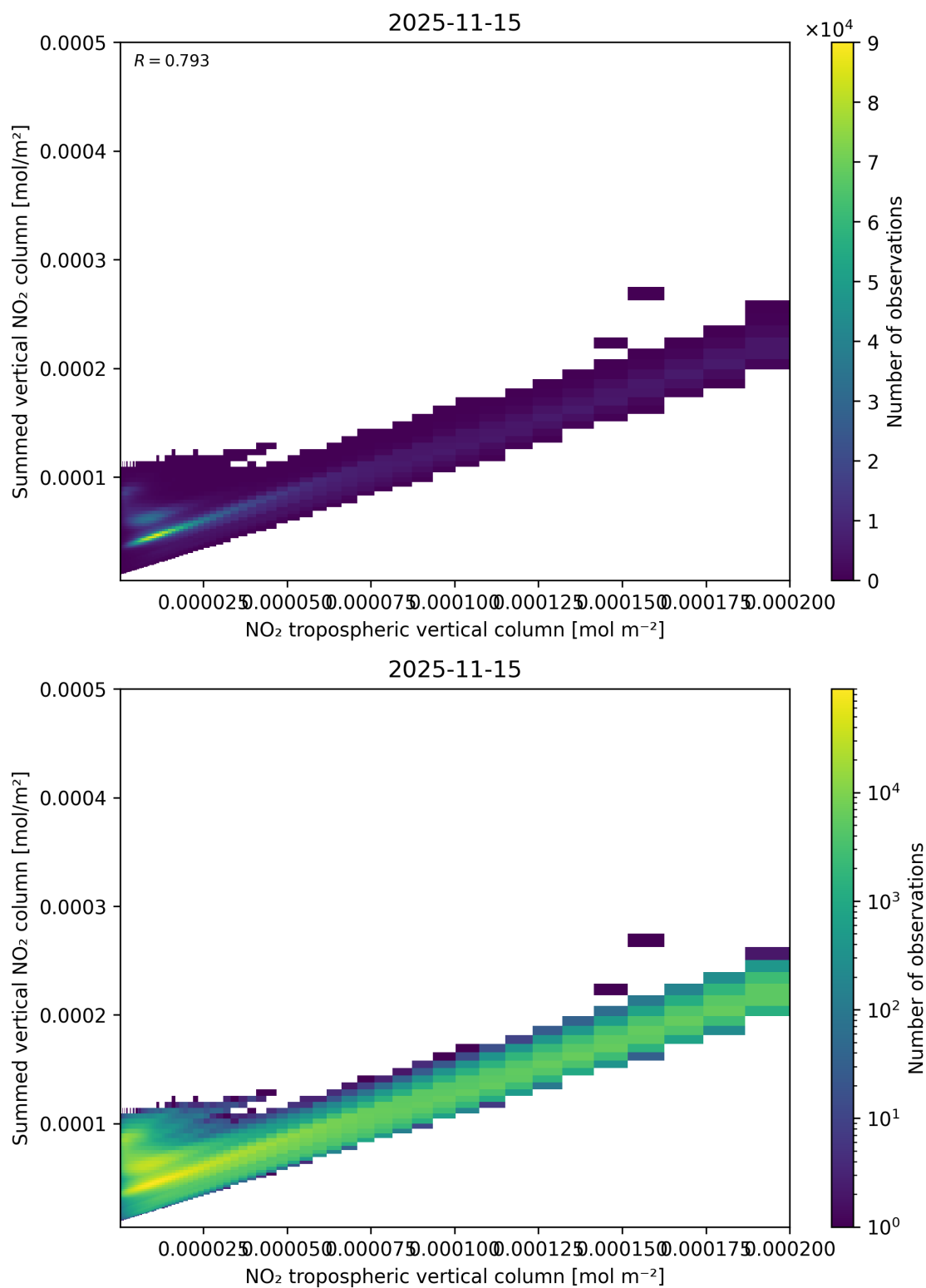
Figure 126: Scatter density plot of “NO 2 tropospheric vertical column” against “Summed vertical NO 2 column” for 2025-11-14 to 2025-11-16.
