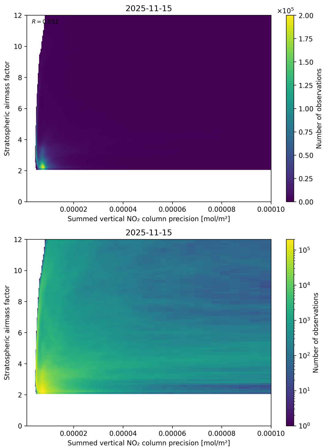
Figure 106: Scatter density plot of “Summed vertical NO 2 column precision” against “Stratospheric airmass factor” for 2025-11-14 to 2025-11-16.
