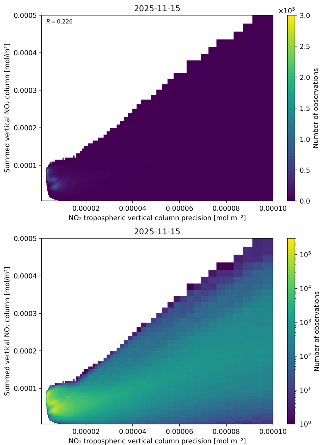
Figure 136: Scatter density plot of “NO 2 tropospheric vertical column precision” against “Summed vertical NO 2 column” for 2025-11-14 to 2025-11-16.
