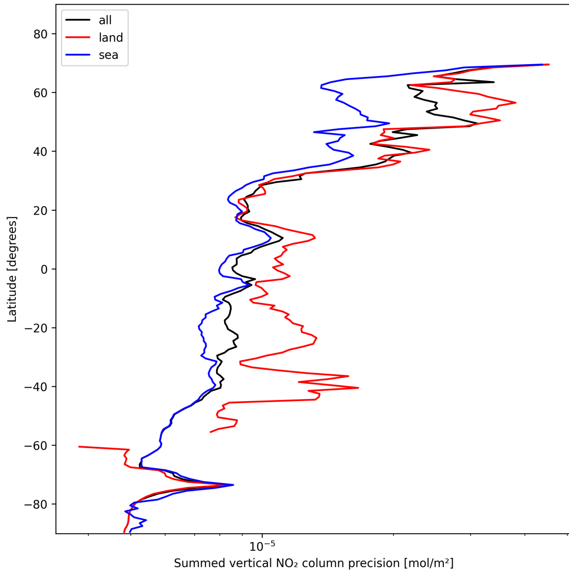
Figure 24: Zonal average of “Summed vertical NO 2 column precision” for 2025-11-14 to 2025-11-16.
