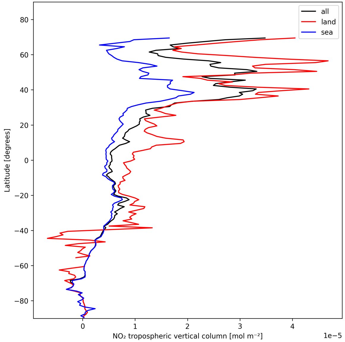
Figure 12: Zonal average of “NO 2 tropospheric vertical column” for 2025-11-14 to 2025-11-16.
