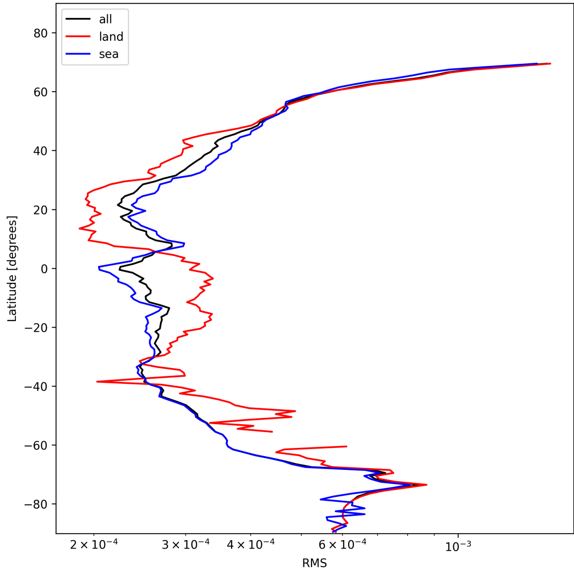
Figure 26: Zonal average of “RMS” for 2025-11-14 to 2025-11-16.
