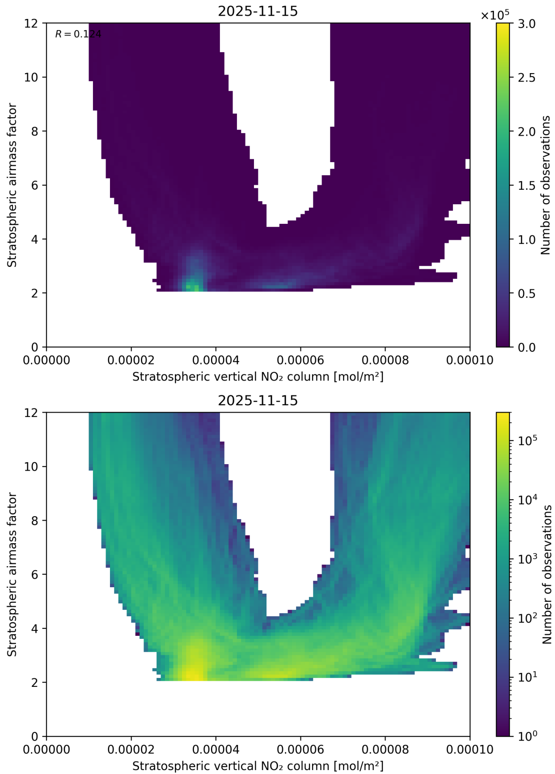
Figure 96: Scatter density plot of “Stratospheric vertical NO 2 column” against “Stratospheric airmass factor” for 2025-11-14 to 2025-11-16.
