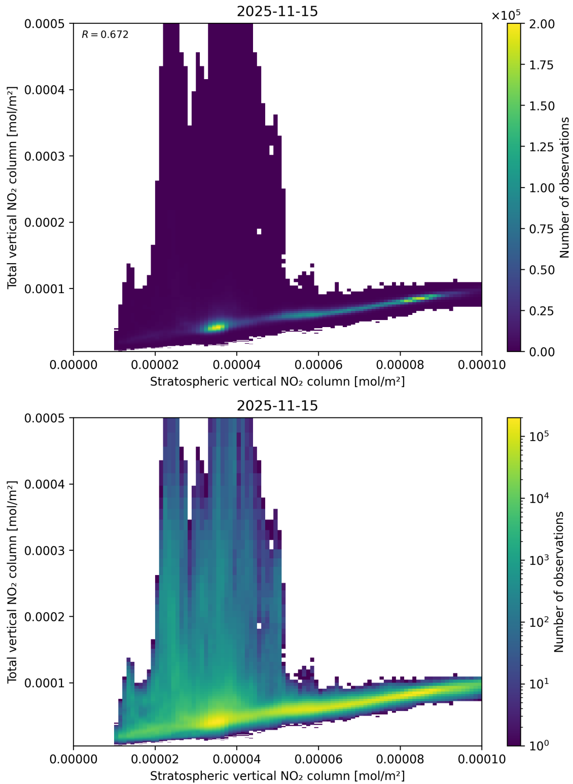
Figure 100: Scatter density plot of “Stratospheric vertical NO 2 column” against “Total vertical NO 2 column” for 2025-11-14 to 2025-11-16.
