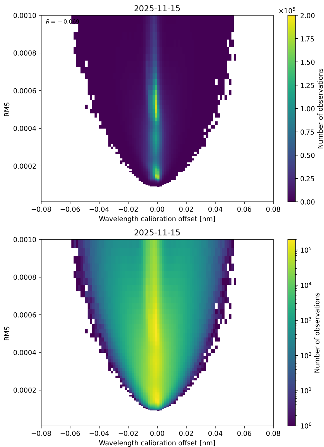
Figure 181: Scatter density plot of “Wavelength calibration offset” against “RMS” for 2025-11-14 to 2025-11-16.
