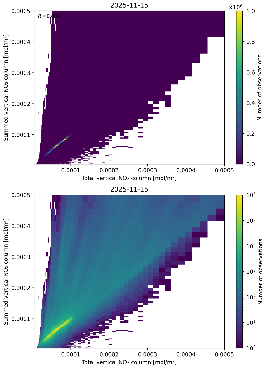
Figure 112: Scatter density plot of “Total vertical NO 2 column” against “Summed vertical NO 2 column” for 2025-11-14 to 2025-11-16.
