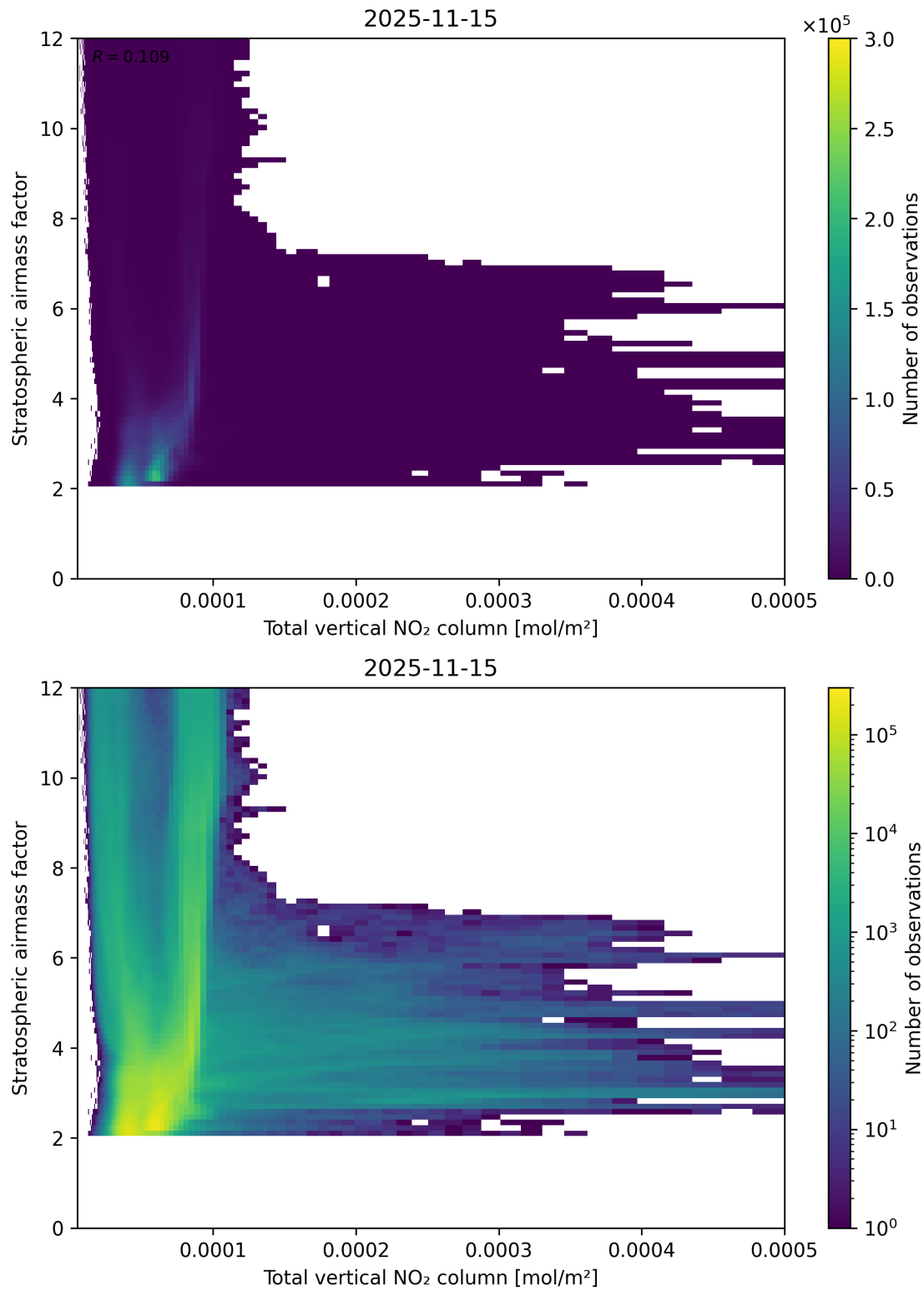
Figure 110: Scatter density plot of “Total vertical NO 2 column” against “Stratospheric airmass factor” for 2025-11-14 to 2025-11-16.
