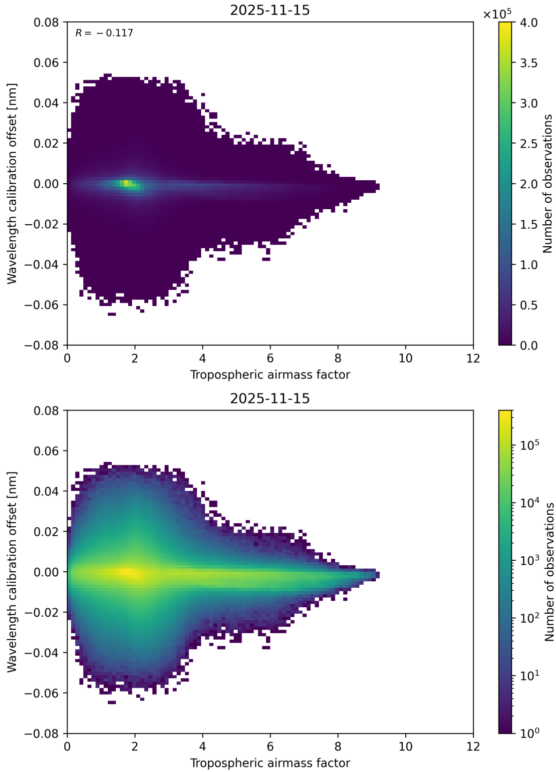
Figure 80: Scatter density plot of “Tropospheric airmass factor” against “Wavelength calibration offset” for 2025-11-14 to 2025-11-16.
