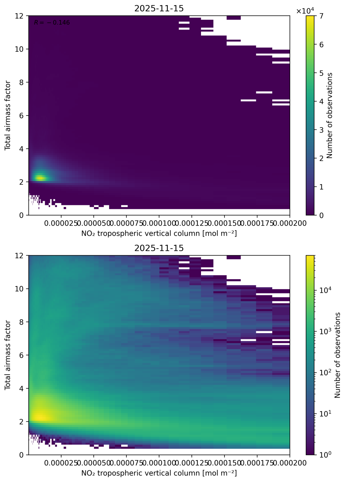
Figure 122: Scatter density plot of “NO 2 tropospheric vertical column” against “Total air mass factor” for 2025-11-14 to 2025-11-16.
