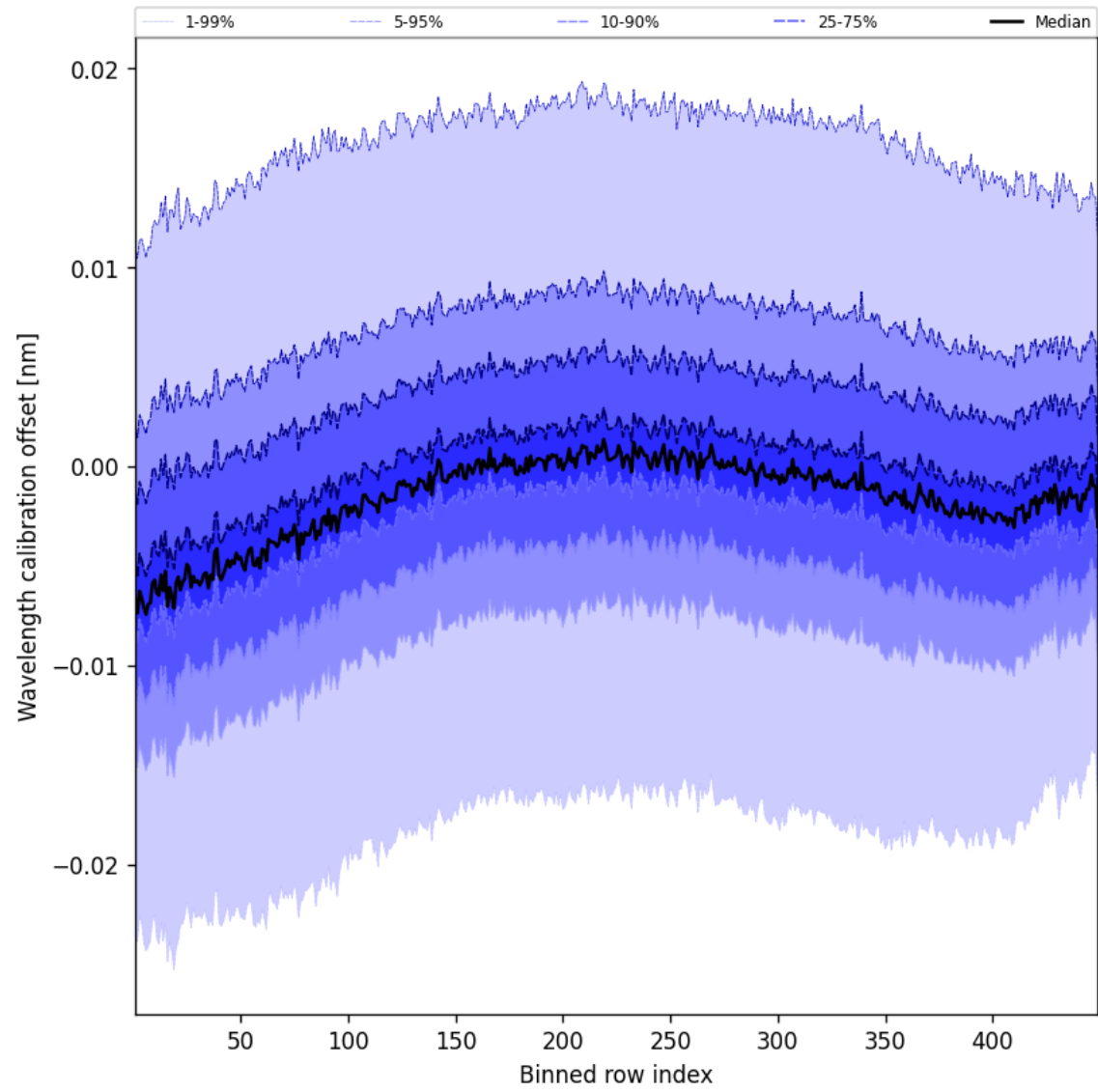
Figure 52: Along track statistics of “Wavelength calibration offset” for 2025-11-14 to 2025-11-16
