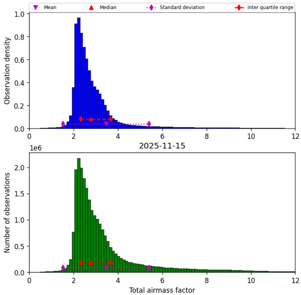
Figure 32: Histogram of “Total airmass factor” for 2025-11-14 to 2025-11-16
