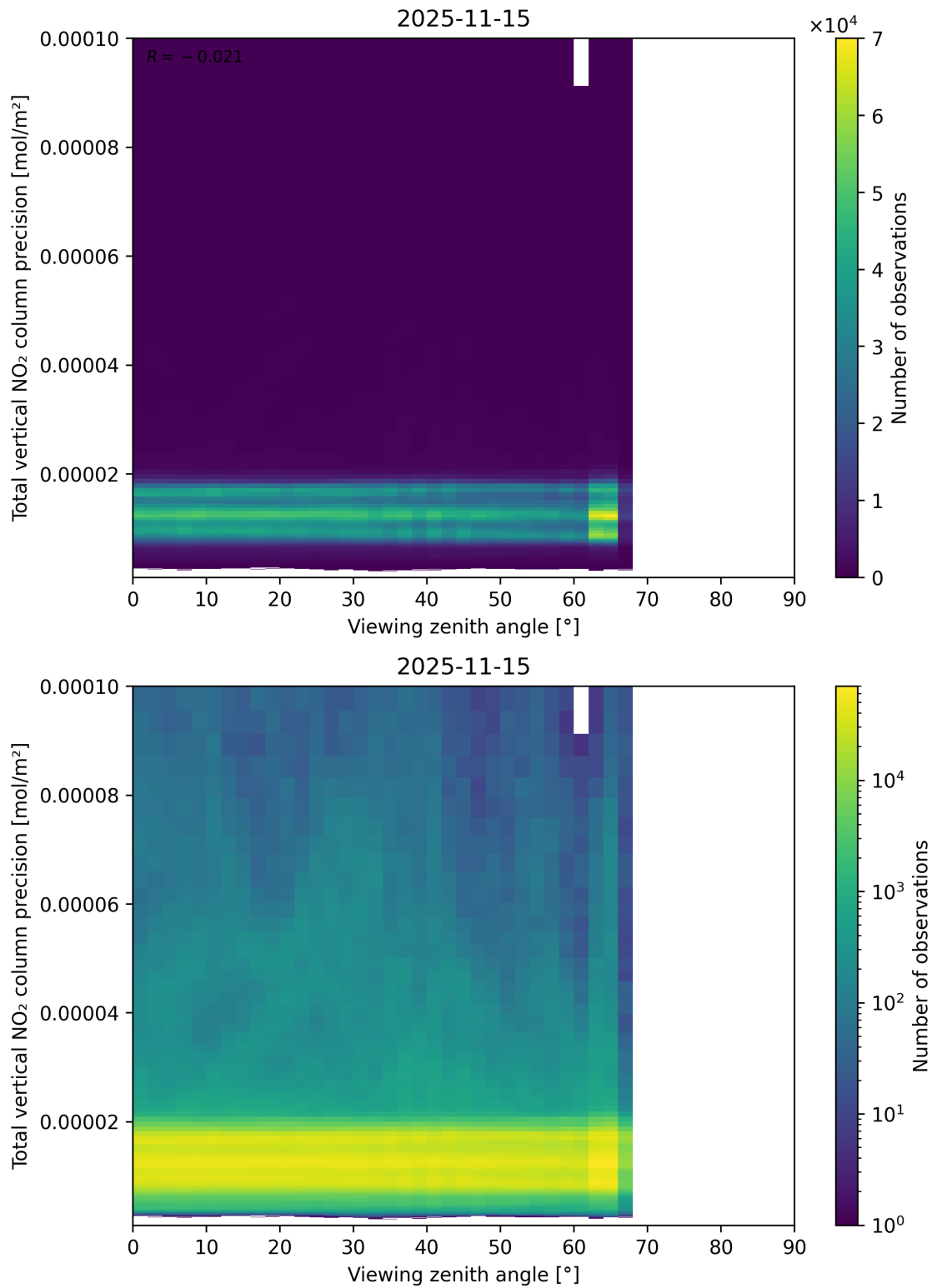
Figure 168: Scatter density plot of “Viewing zenith angle” against “Total vertical NO 2 column precision” for 2025-11-14 to 2025-11-16.
