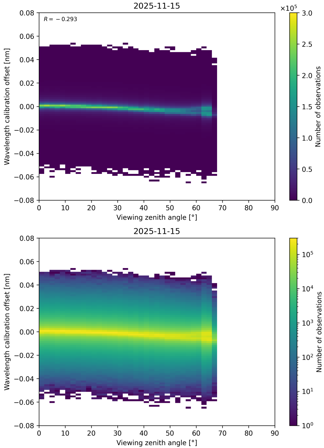
Figure 173: Scatter density plot of “Viewing zenith angle” against “Wavelength calibration offset” for 2025-11-14 to 2025-11-16.
