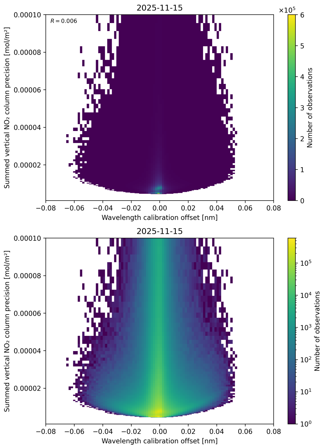
Figure 178: Scatter density plot of “Wavelength calibration offset” against “Summed vertical NO 2 column precision” for 2025-11-14 to 2025-11-16.
