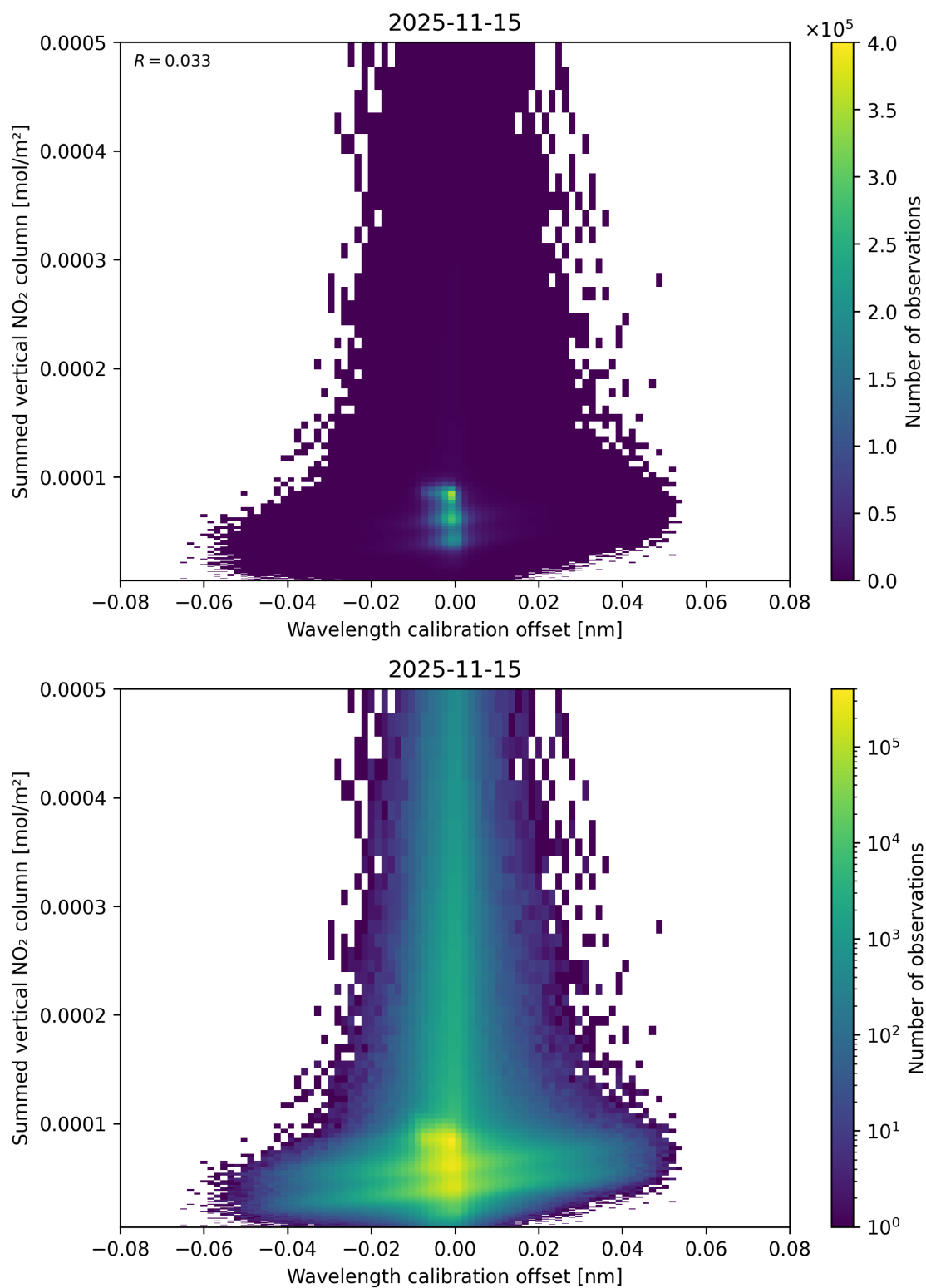
Figure 177: Scatter density plot of “Wavelength calibration offset” against “Summed vertical NO 2 column” for 2025-11-14 to 2025-11-16.
