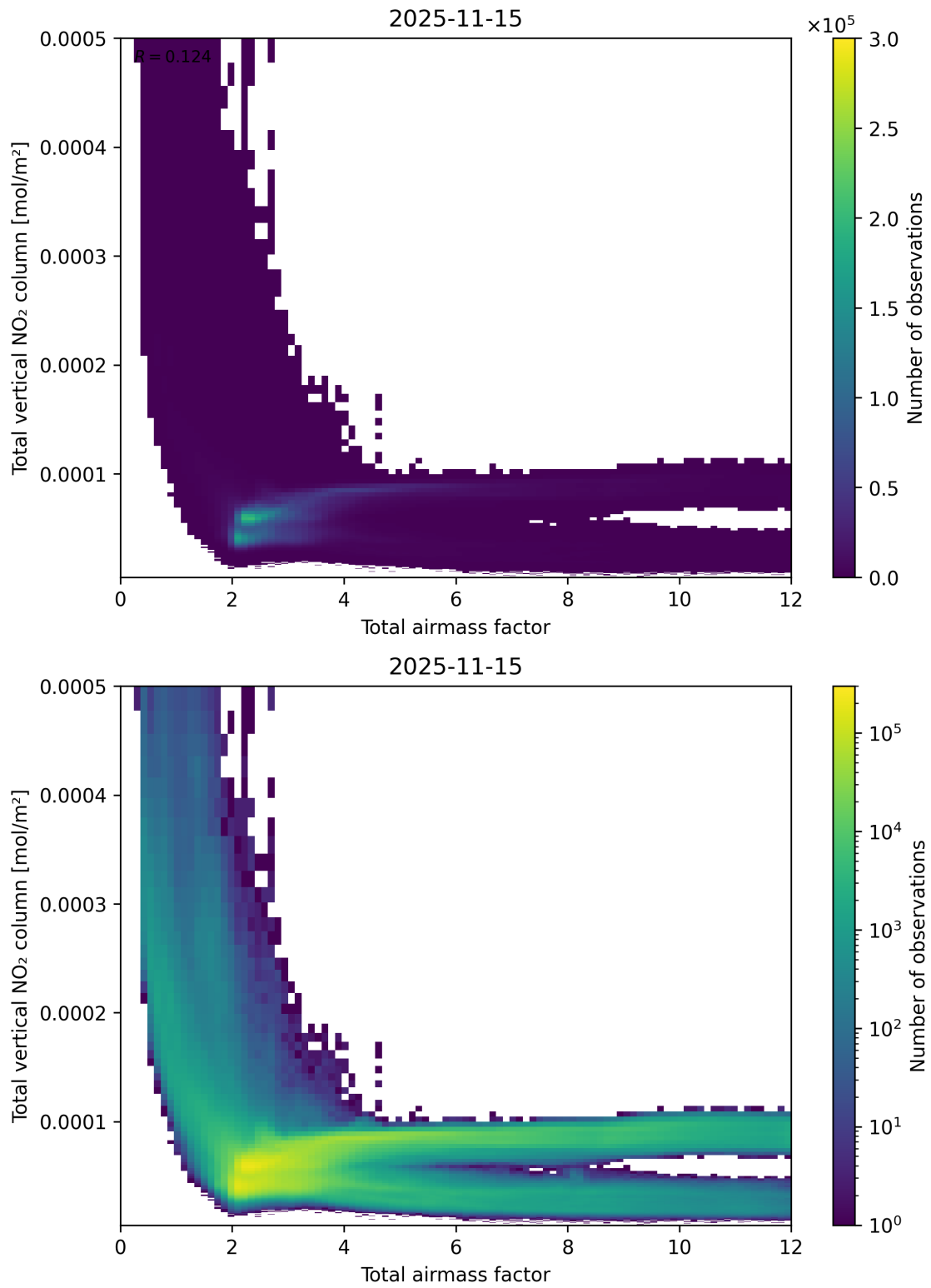
Figure 67: Scatter density plot of “Total airmass factor” against “Total vertical NO 2 column” for 2025-11-14 to 2025-11-16.
