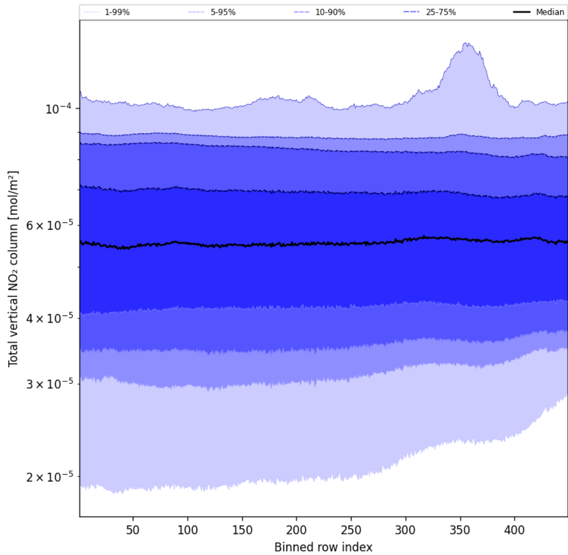
Figure 55: Along track statistics of “Total vertical NO 2 column” for 2025-11-14 to 2025-11-16
