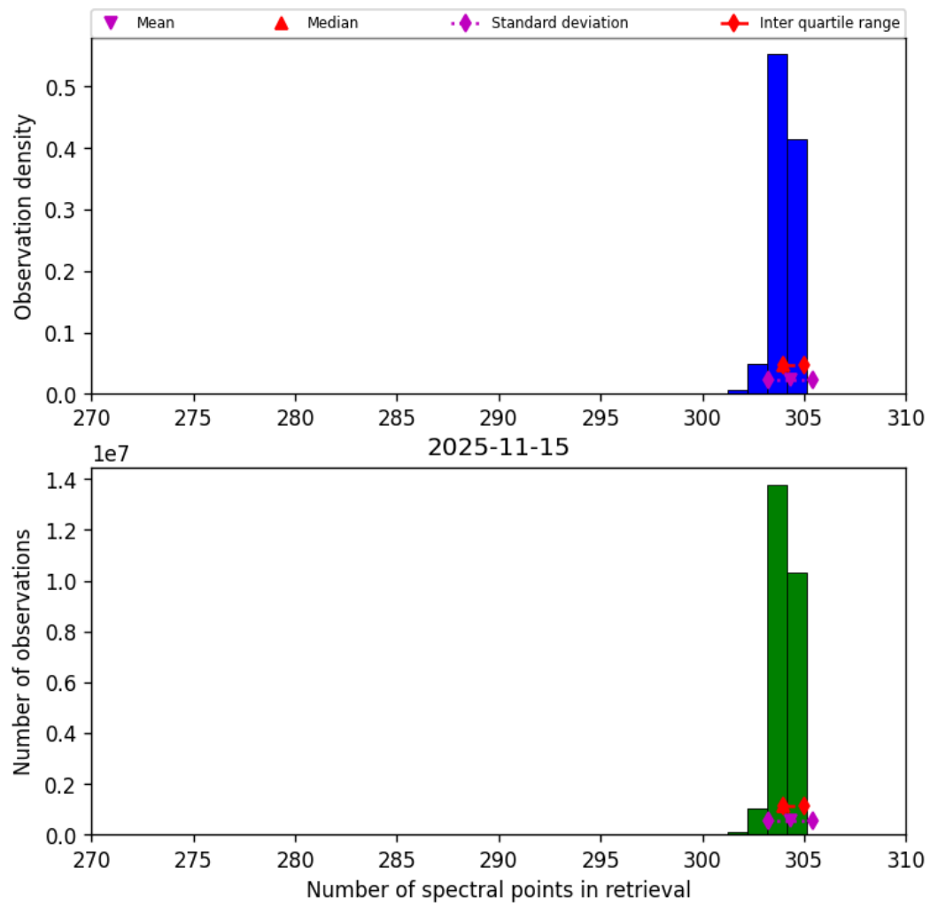
Figure 33: Histogram of “Number of spectral points in retrieval” for 2025-11-14 to 2025-11-16
