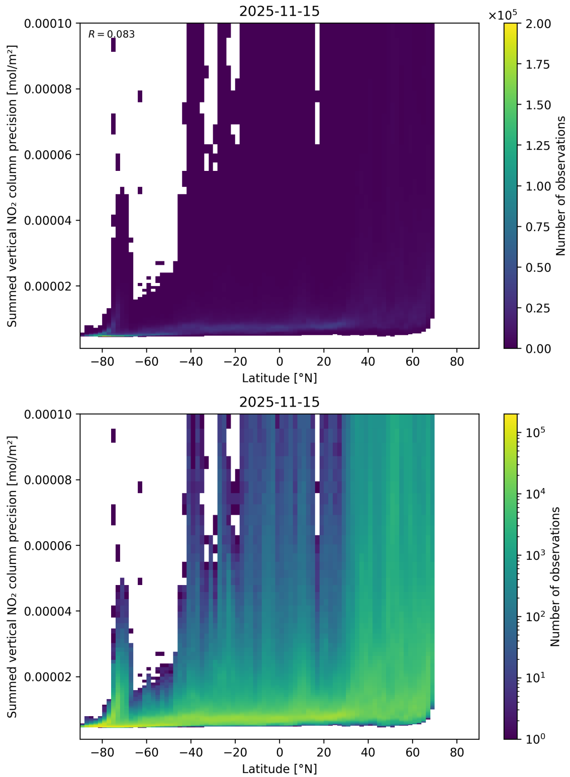
Figure 89: Scatter density plot of “Latitude” against “Summed vertical NO 2 column precision” for 2025-11-14 to 2025-11-16.
