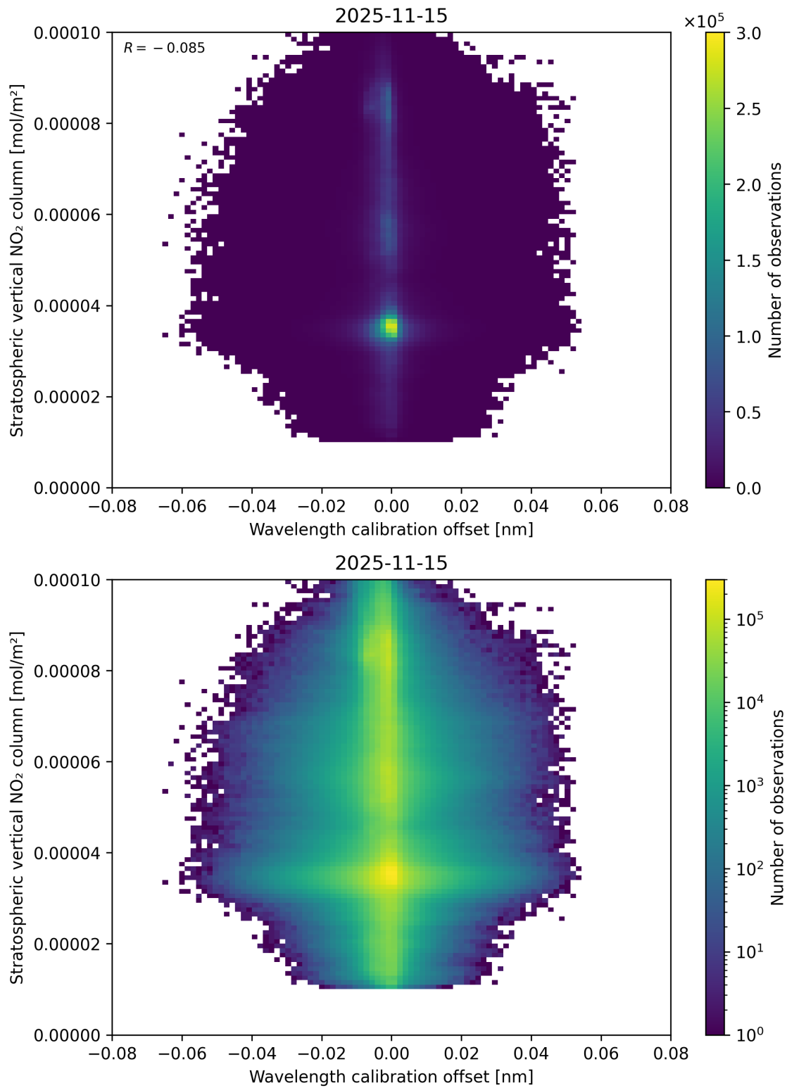
Figure 176: Scatter density plot of “Wavelength calibration offset” against “Stratospheric vertical NO 2 column” for 2025-11-14 to 2025-11-16.
