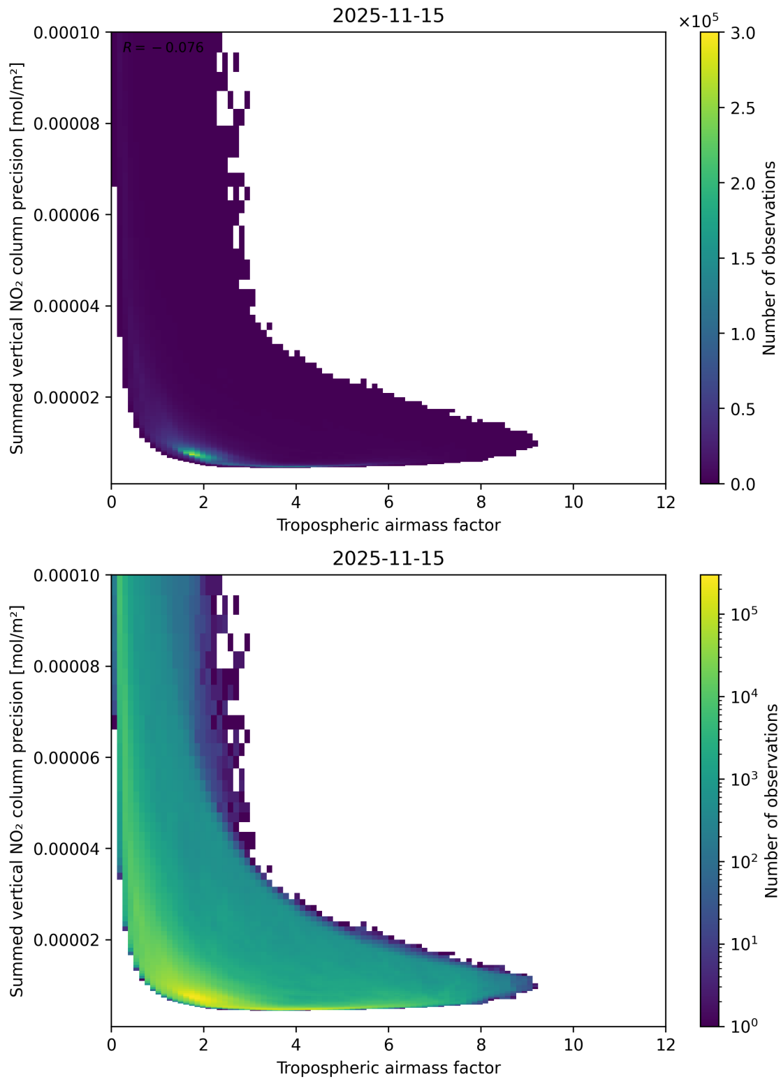
Figure 76: Scatter density plot of “Tropospheric airmass factor” against “Summed vertical NO 2 column precision” for 2025-11-14 to 2025-11-16.
