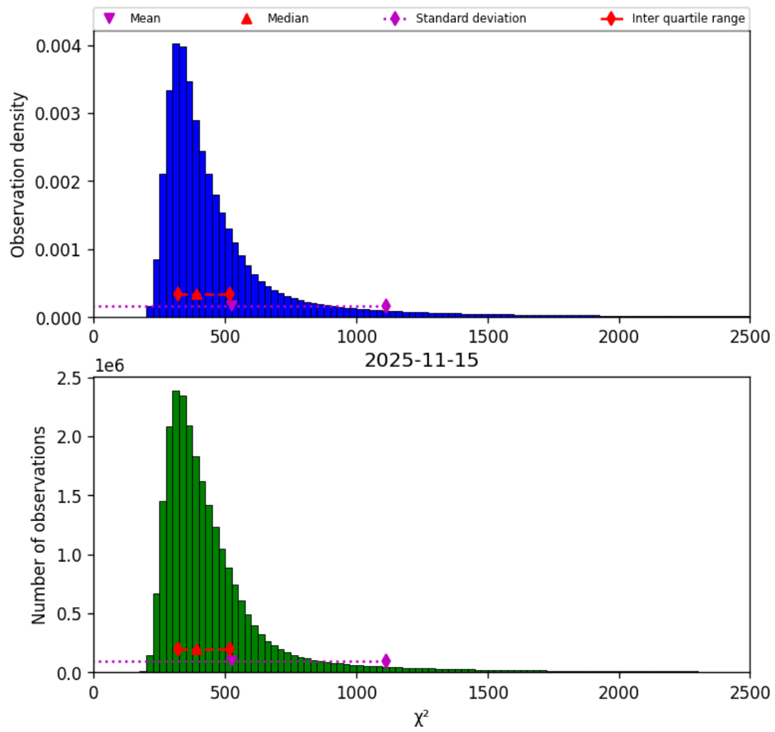
Figure 42: Histogram of “ \chi^2 ” for 2025-11-14 to 2025-11-16
