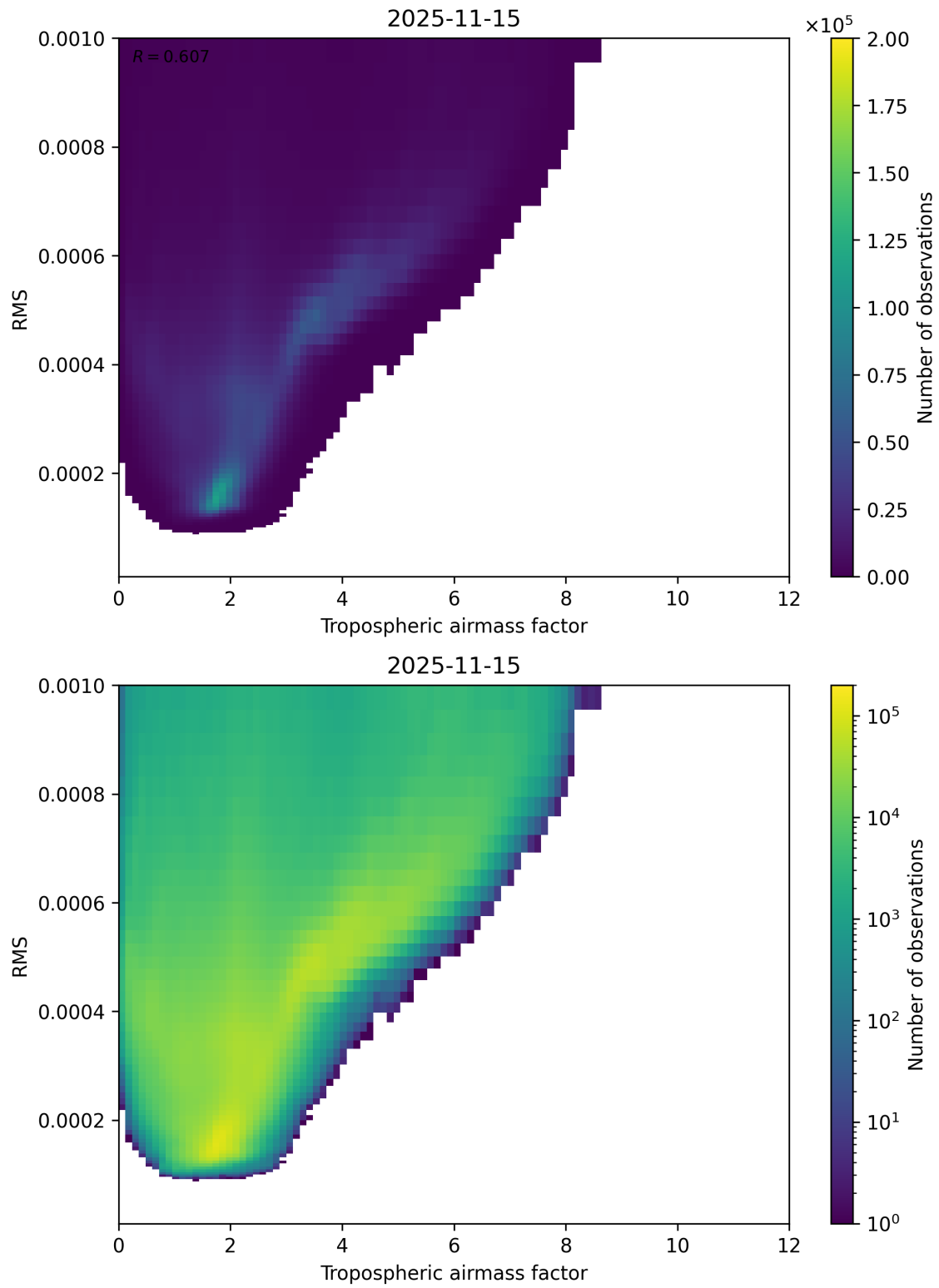
Figure 79: Scatter density plot of “Tropospheric airmass factor” against “RMS” for 2025-11-14 to 2025-11-16.
