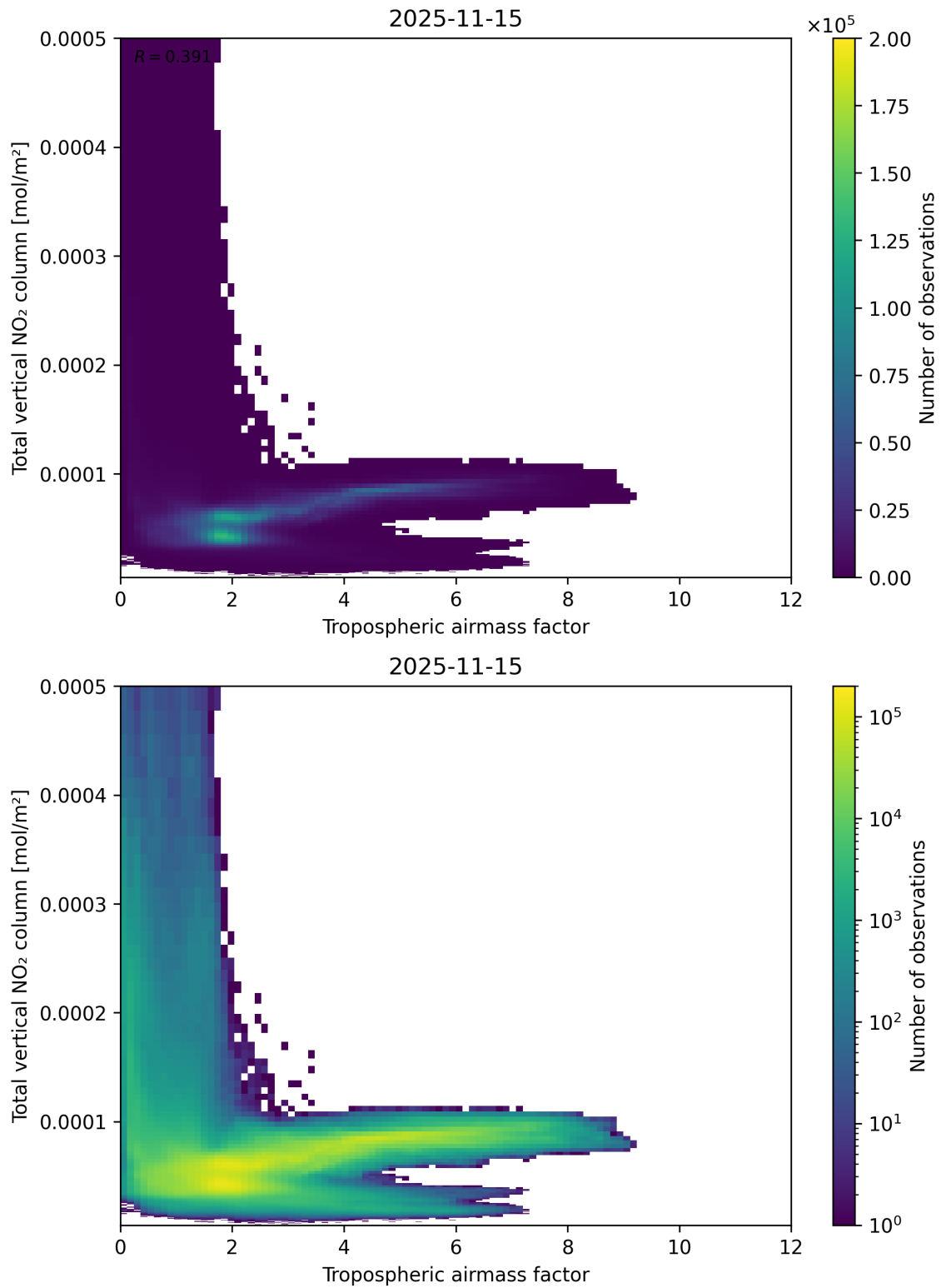
Figure 77: Scatter density plot of “Tropospheric airmass factor” against “Total vertical NO 2 column” for 2025-11-14 to 2025-11-16.
