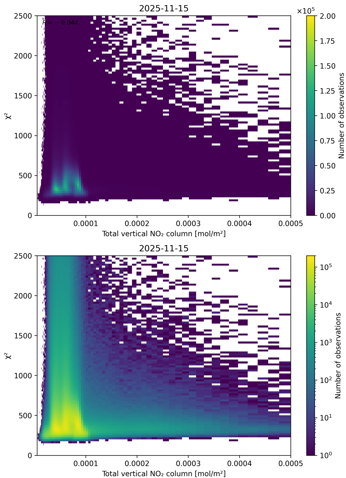
Figure 111: Scatter density plot of “Total vertical NO 2 column” against “ \chi^2 ” for 2025-11-14 to 2025-11-16.
