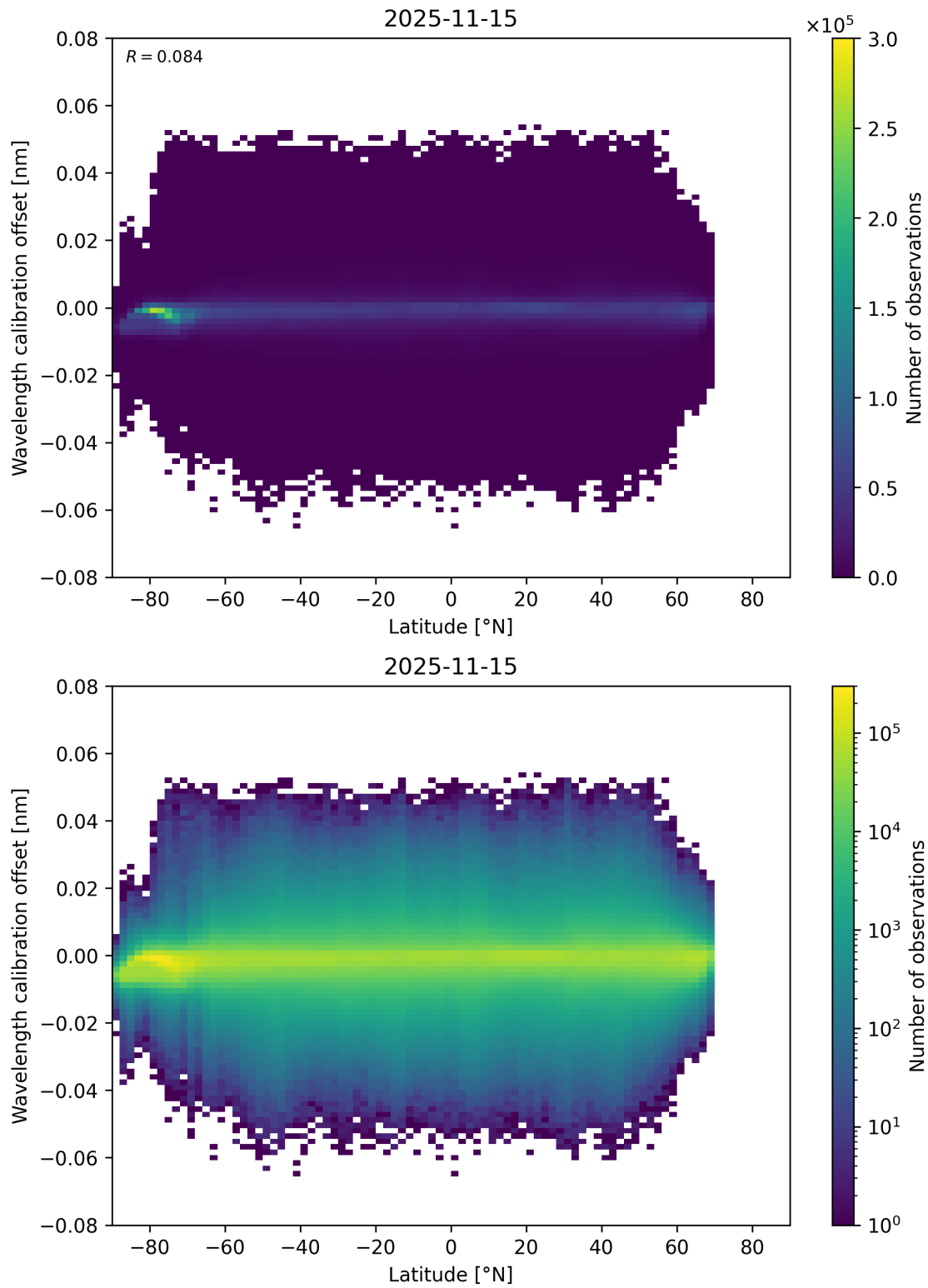
Figure 95: Scatter density plot of “Latitude” against “Wavelength calibration offset” for 2025-11-14 to 2025-11-16.
