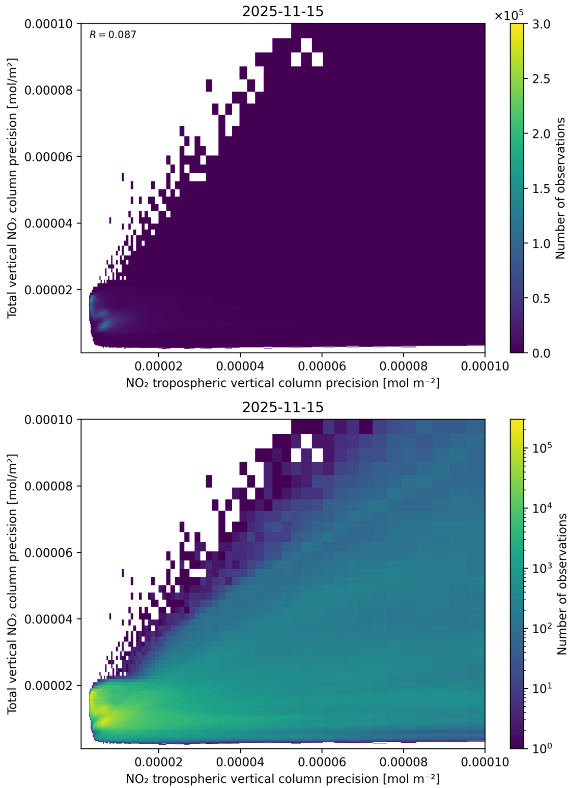
Figure 139: Scatter density plot of “NO 2 tropospheric vertical column precision” against “Total vertical NO 2 column precision” for 2025-11-14 to 2025-11-16.
