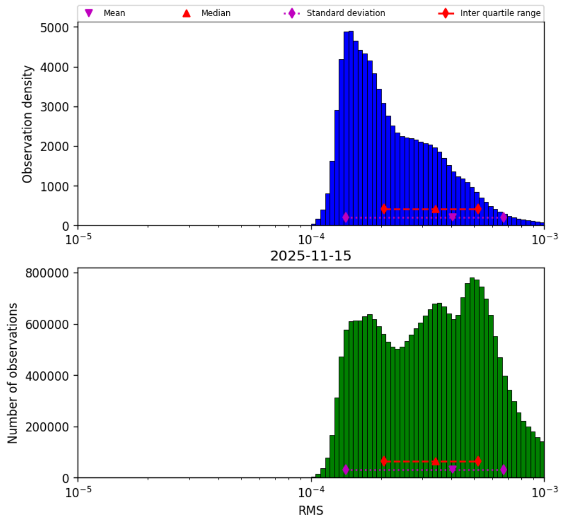
Figure 43: Histogram of “RMS” for 2025-11-14 to 2025-11-16
