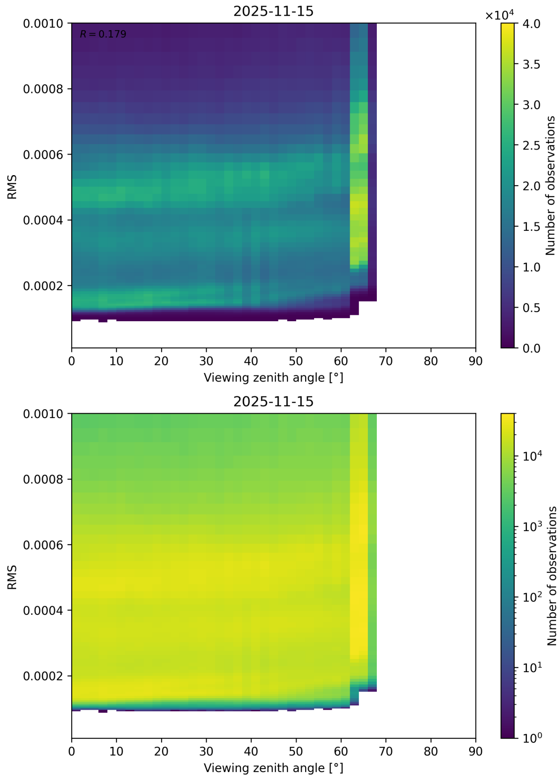
Figure 171: Scatter density plot of “Viewing zenith angle” against “RMS” for 2025-11-14 to 2025-11-16.
