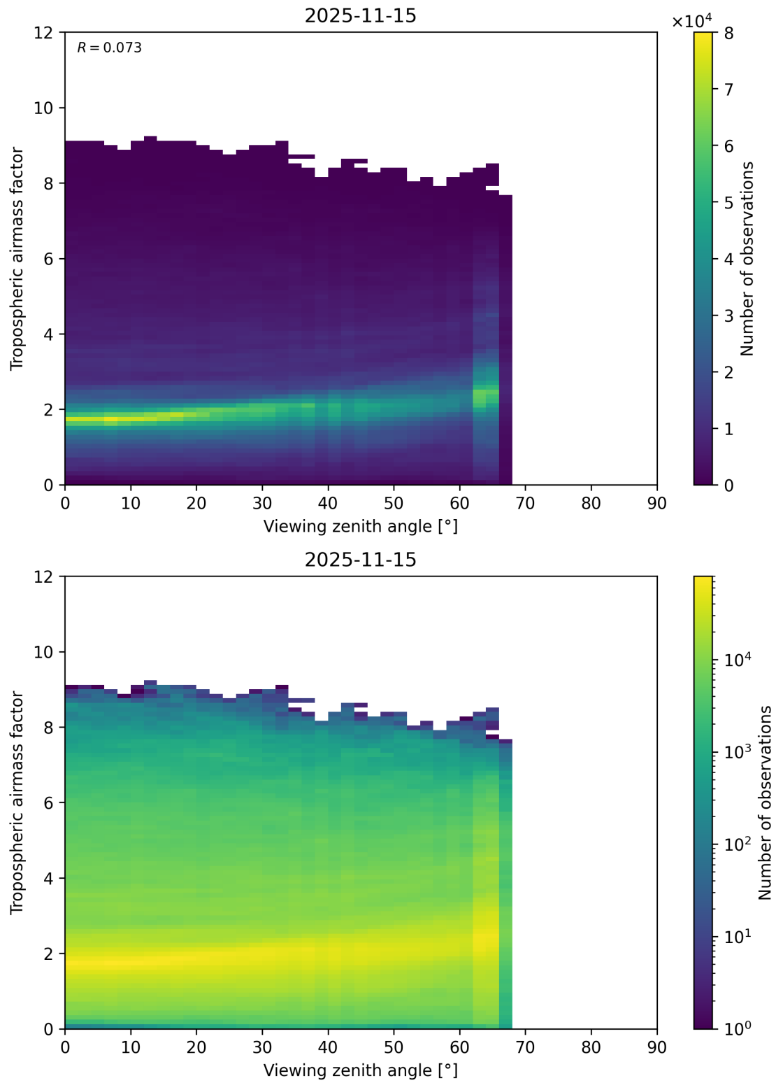
Figure 161: Scatter density plot of “Viewing zenith angle” against “Tropospheric airmass factor” for 2025-11-14 to 2025-11-16.
