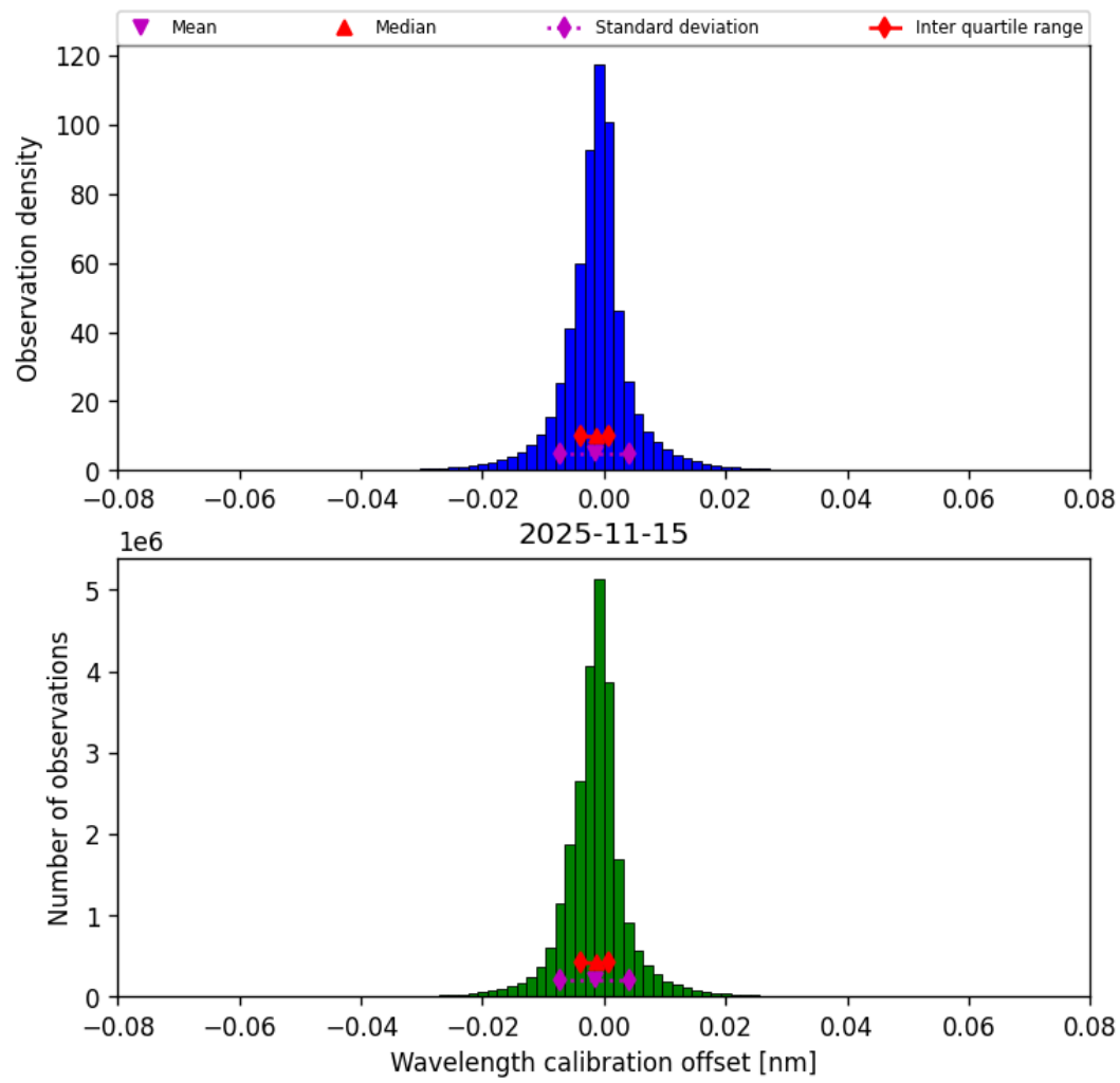
Figure 35: Histogram of “Wavelength calibration offset” for 2025-11-14 to 2025-11-16
