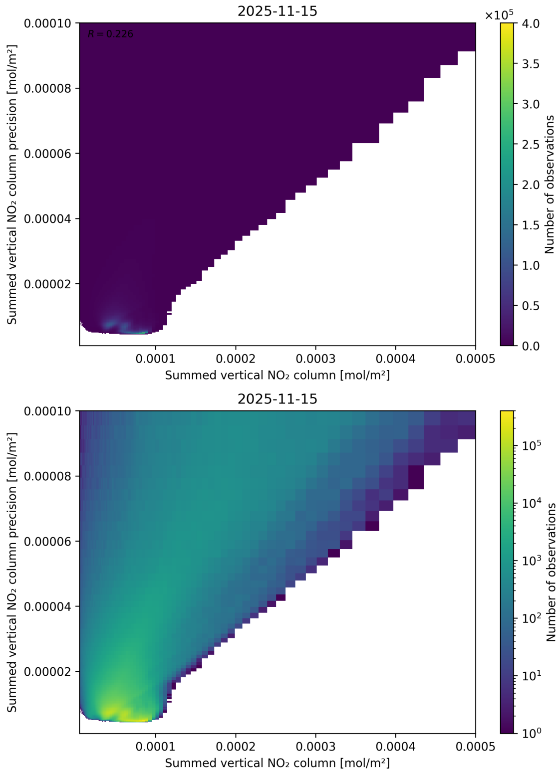
Figure 105: Scatter density plot of “Summed vertical NO 2 column” against “Summed vertical NO 2 column precision” for 2025-11-14 to 2025-11-16.
