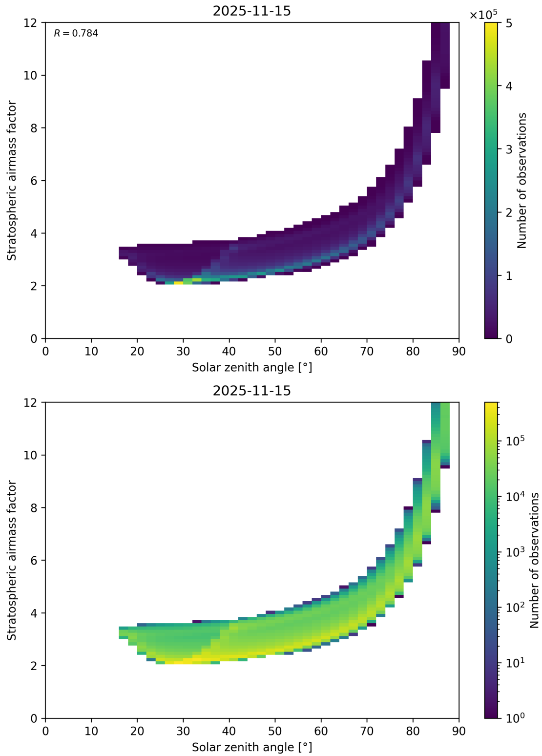
Figure 145: Scatter density plot of “Solar zenith angle” against “Stratospheric airmass factor” for 2025-11-14 to 2025-11-16.
