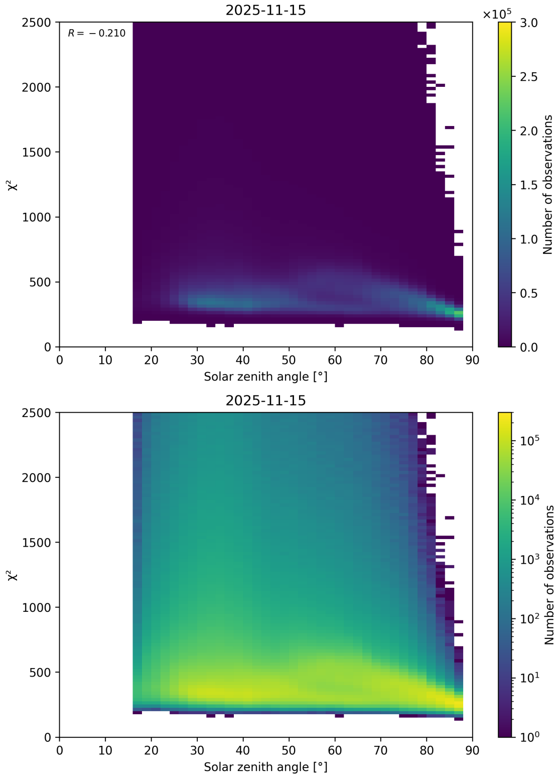
Figure 148: Scatter density plot of “Solar zenith angle” against “ \chi^2 ” for 2025-11-14 to 2025-11-16.
