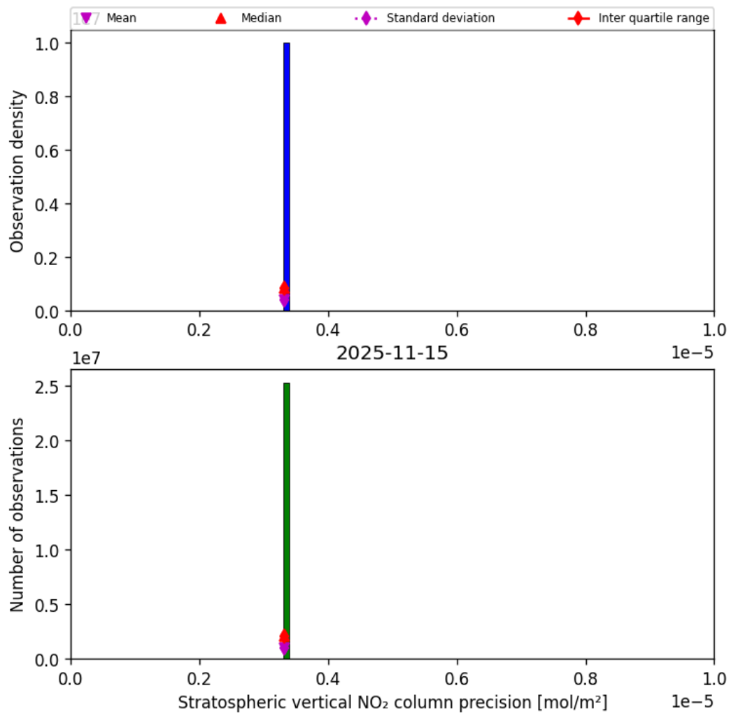
Figure 37: Histogram of “Stratospheric vertical NO 2 column precision” for 2025-11-14 to 2025-11-16
