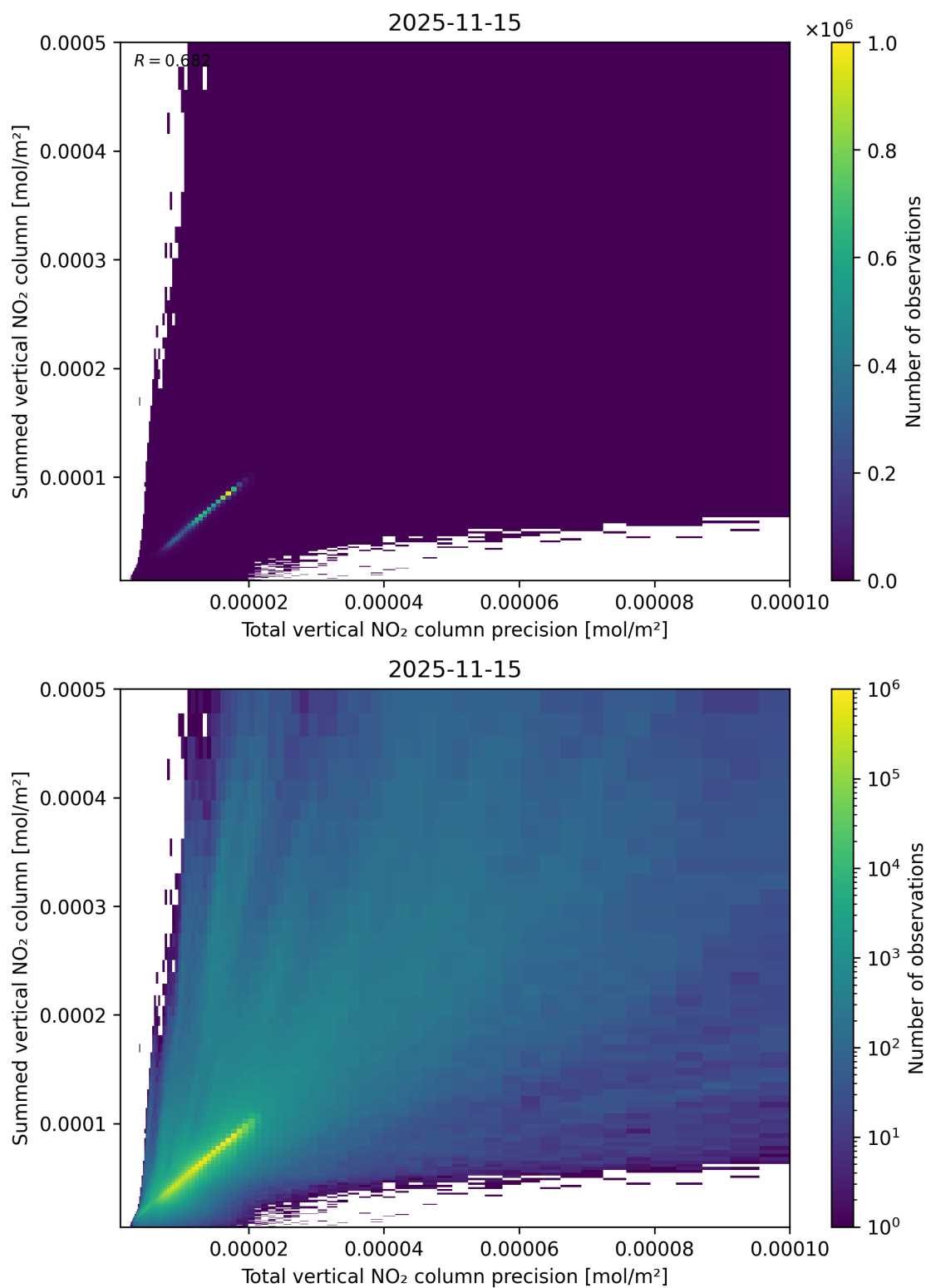
Figure 117: Scatter density plot of “Total vertical NO 2 column precision” against “Summed vertical NO 2 column” for 2025-11-14 to 2025-11-16.
