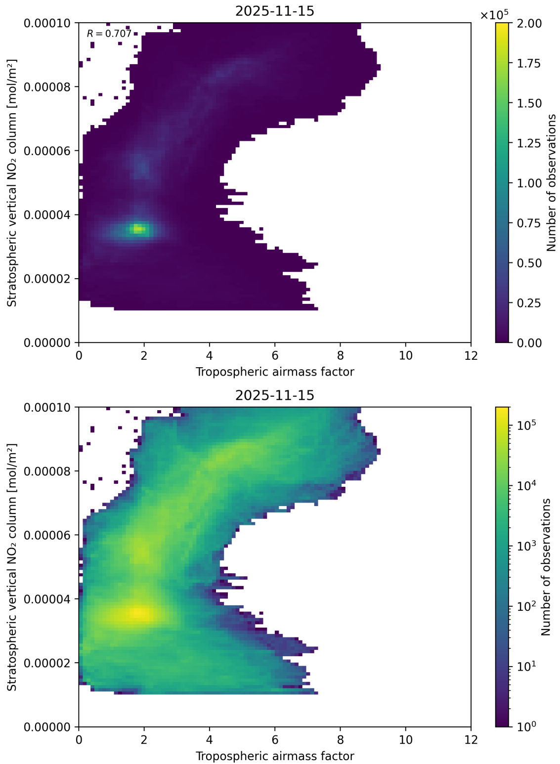
Figure 74: Scatter density plot of “Tropospheric air mass factor” against “Stratospheric vertical NO 2 column” for 2025-11-14 to 2025-11-16.
