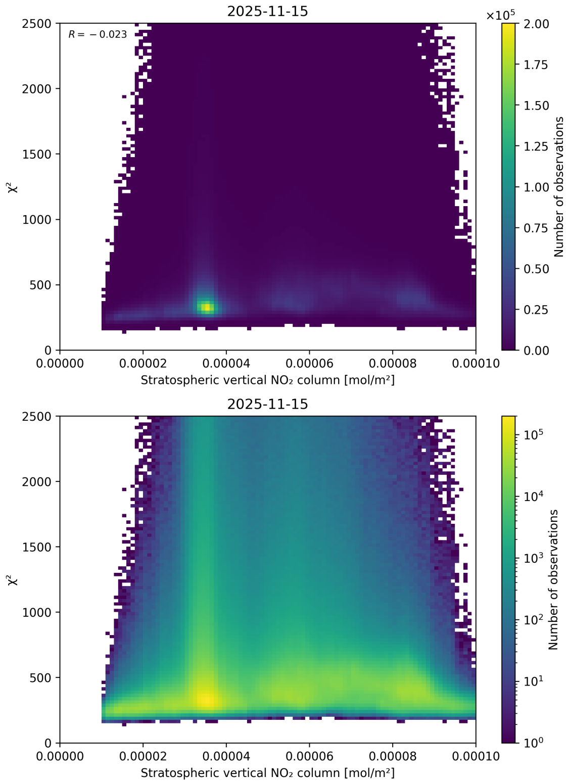
Figure 97: Scatter density plot of “Stratospheric vertical NO 2 column” against “ \chi^2 ” for 2025-11-14 to 2025-11-16.
