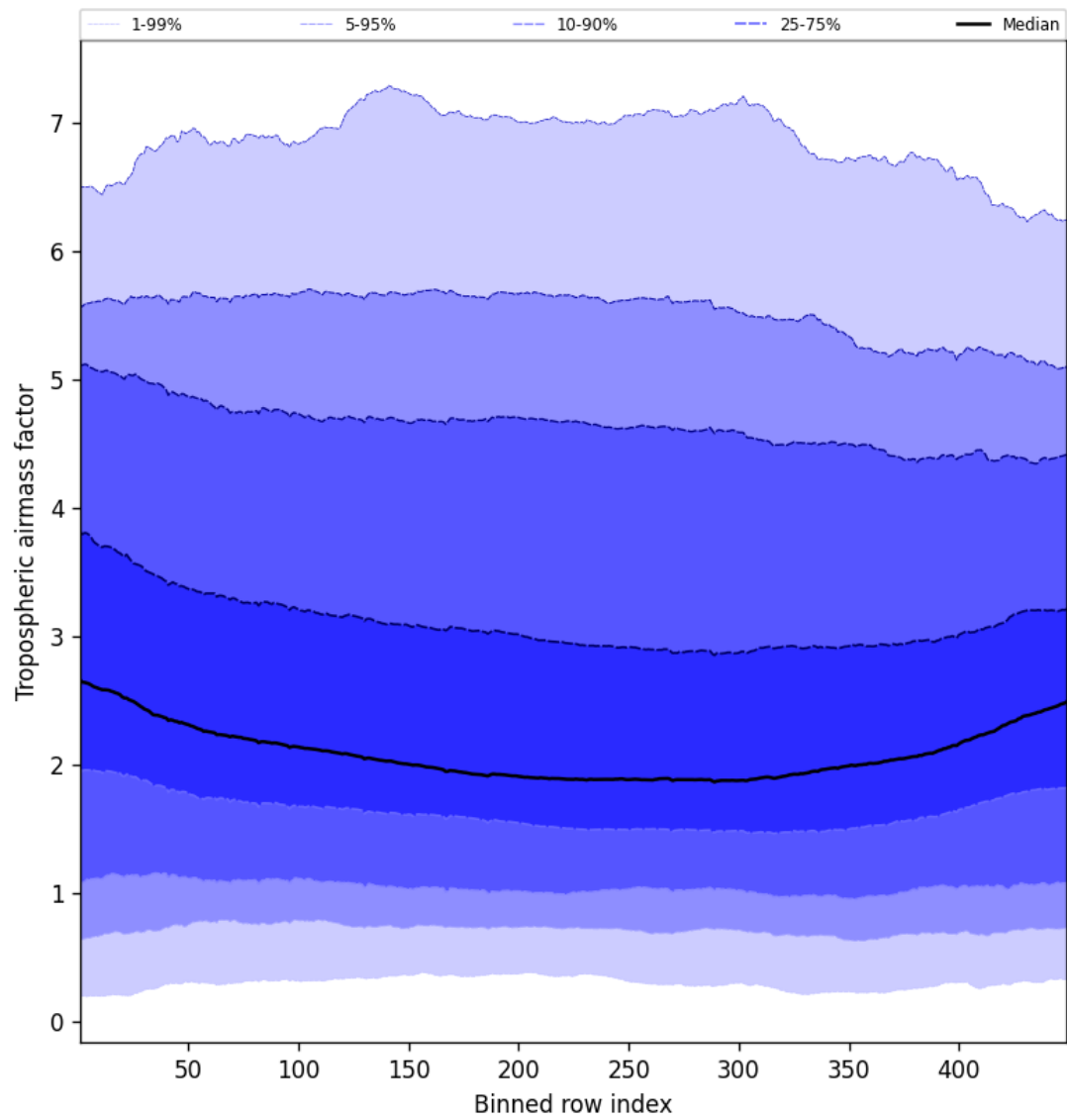
Figure 48: Along track statistics of “Tropospheric air mass factor” for 2025-11-14 to 2025-11-16
