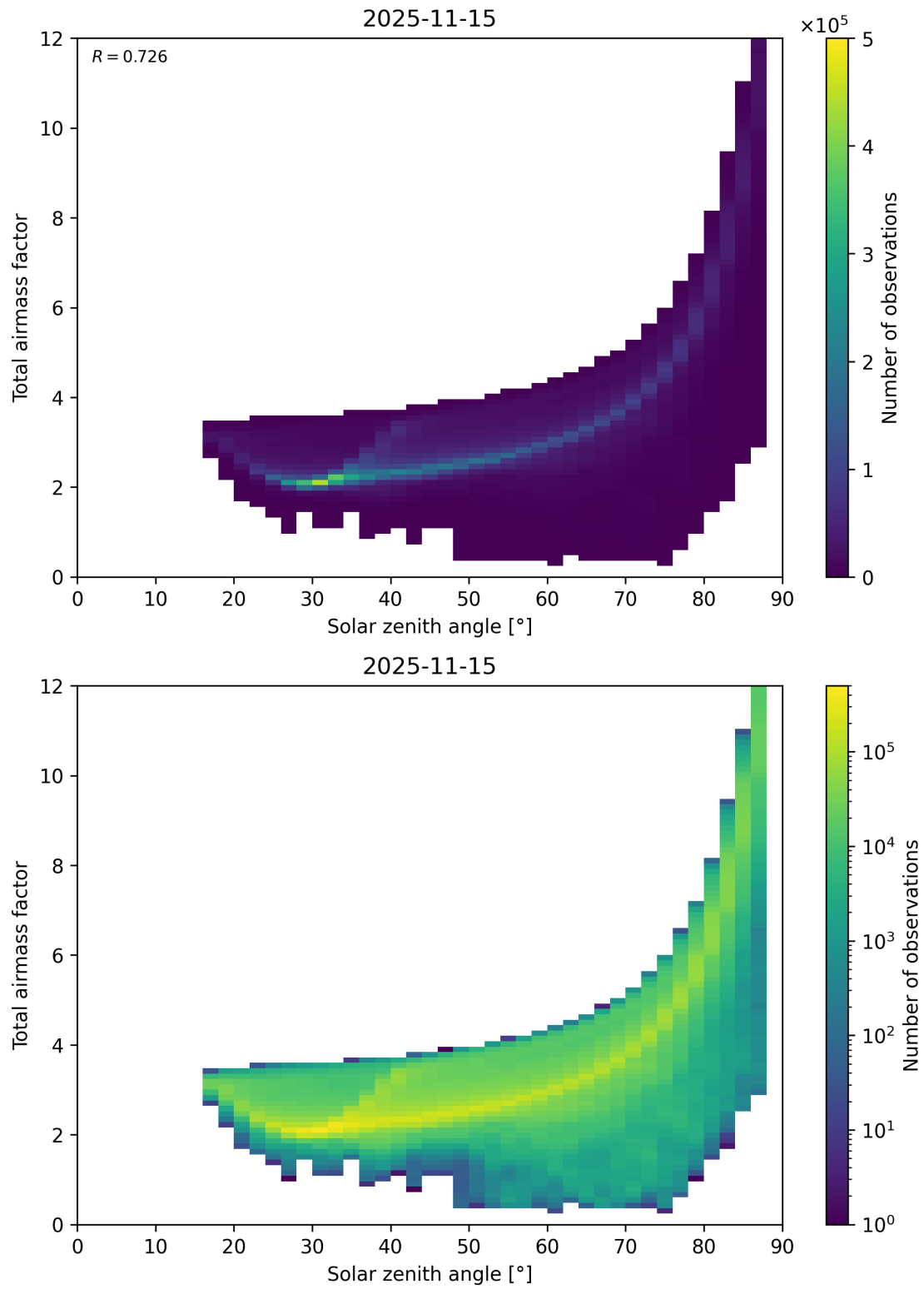
Figure 146: Scatter density plot of “Solar zenith angle” against “Total air mass factor” for 2025-11-14 to 2025-11-16.
