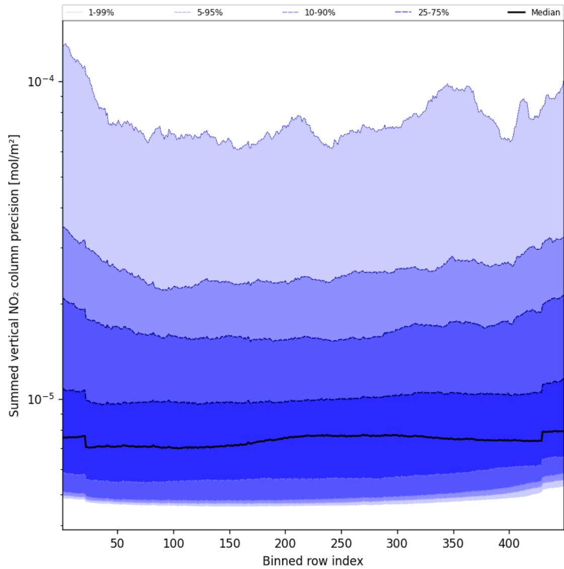
Figure 58: Along track statistics of “Summed vertical NO 2 column precision” for 2025-11-14 to 2025-11-16
