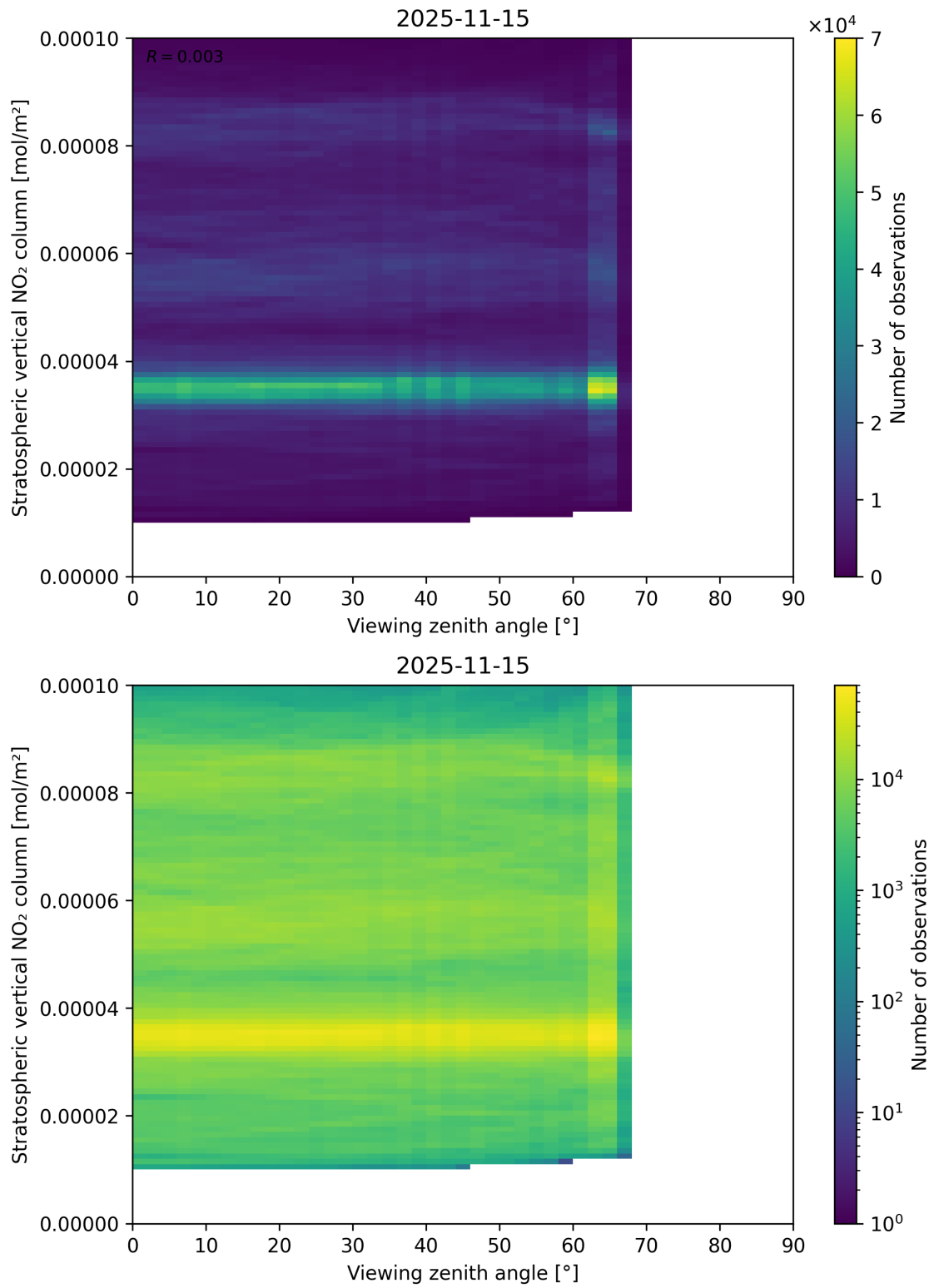
Figure 164: Scatter density plot of “Viewing zenith angle” against “Stratospheric vertical NO 2 column” for 2025-11-14 to 2025-11-16.
