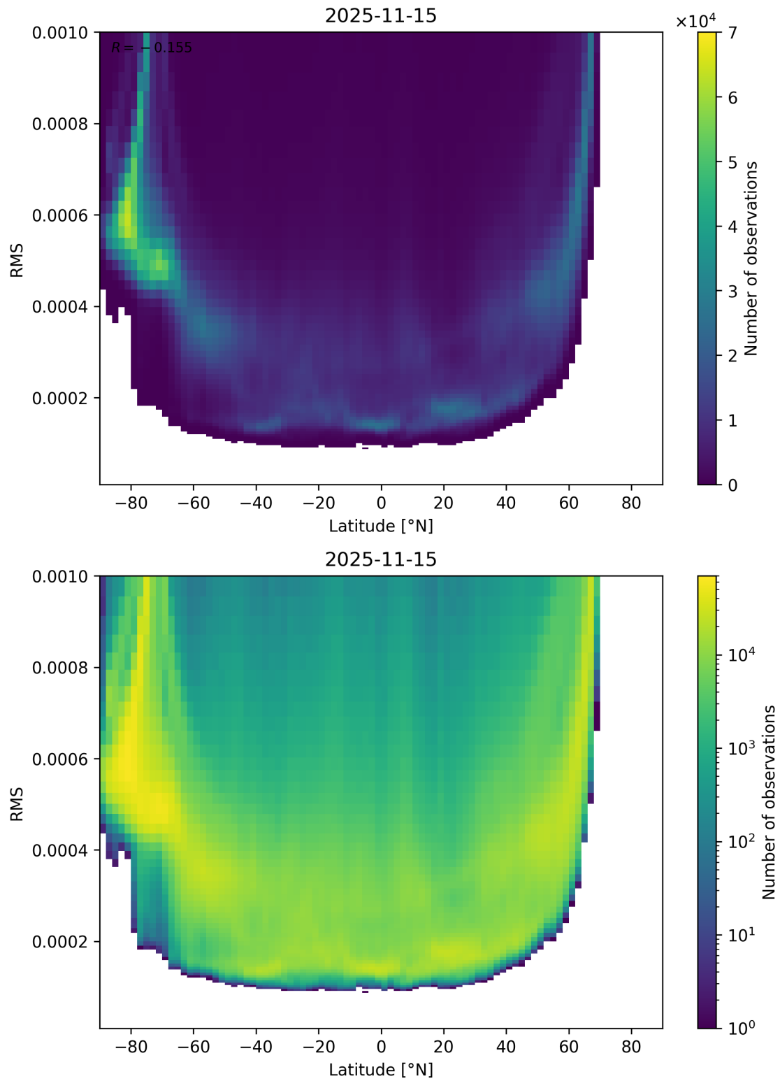
Figure 94: Scatter density plot of “Latitude” against “RMS” for 2025-11-14 to 2025-11-16.
