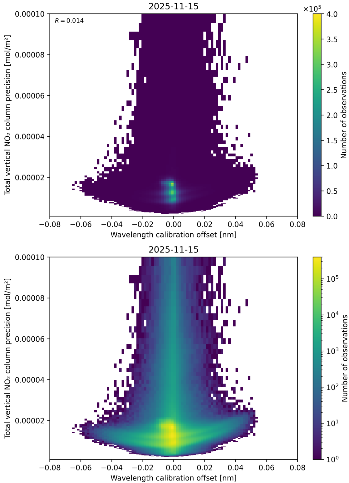
Figure 180: Scatter density plot of “Wavelength calibration offset” against “Total vertical NO 2 column precision” for 2025-11-14 to 2025-11-16.
