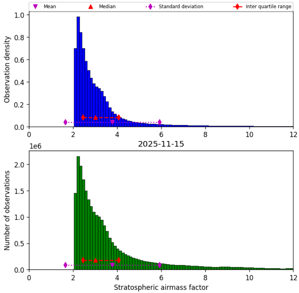
Figure 44: Histogram of “Stratospheric airmass factor” for 2025-11-14 to 2025-11-16
