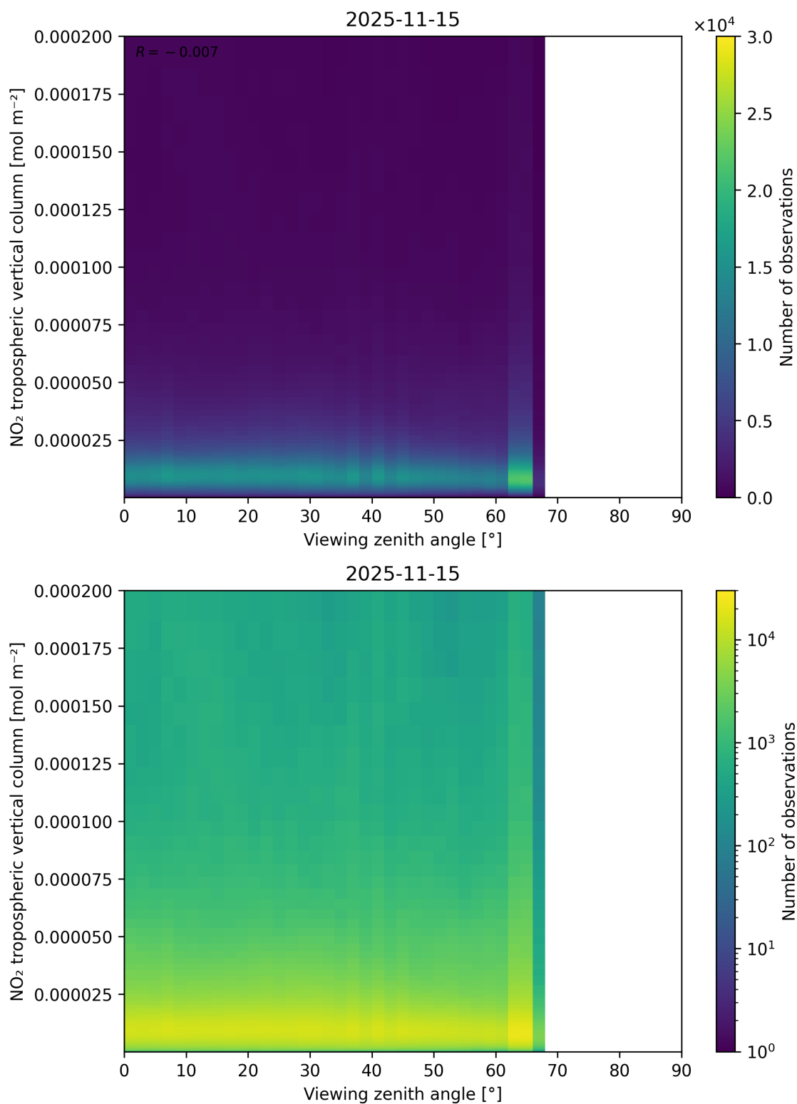
Figure 169: Scatter density plot of “Viewing zenith angle” against “NO 2 tropospheric vertical column” for 2025-11-14 to 2025-11-16.
