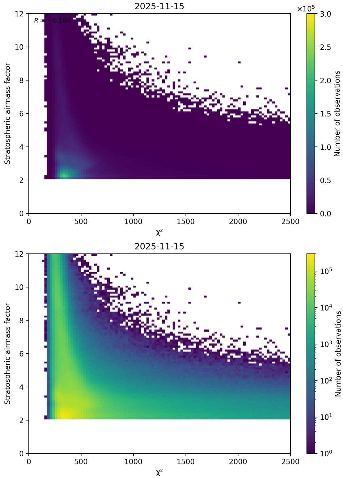
Figure 81: Scatter density plot of “ \chi^2 ” against “Stratospheric airmass factor” for 2025-11-14 to 2025-11-16.
