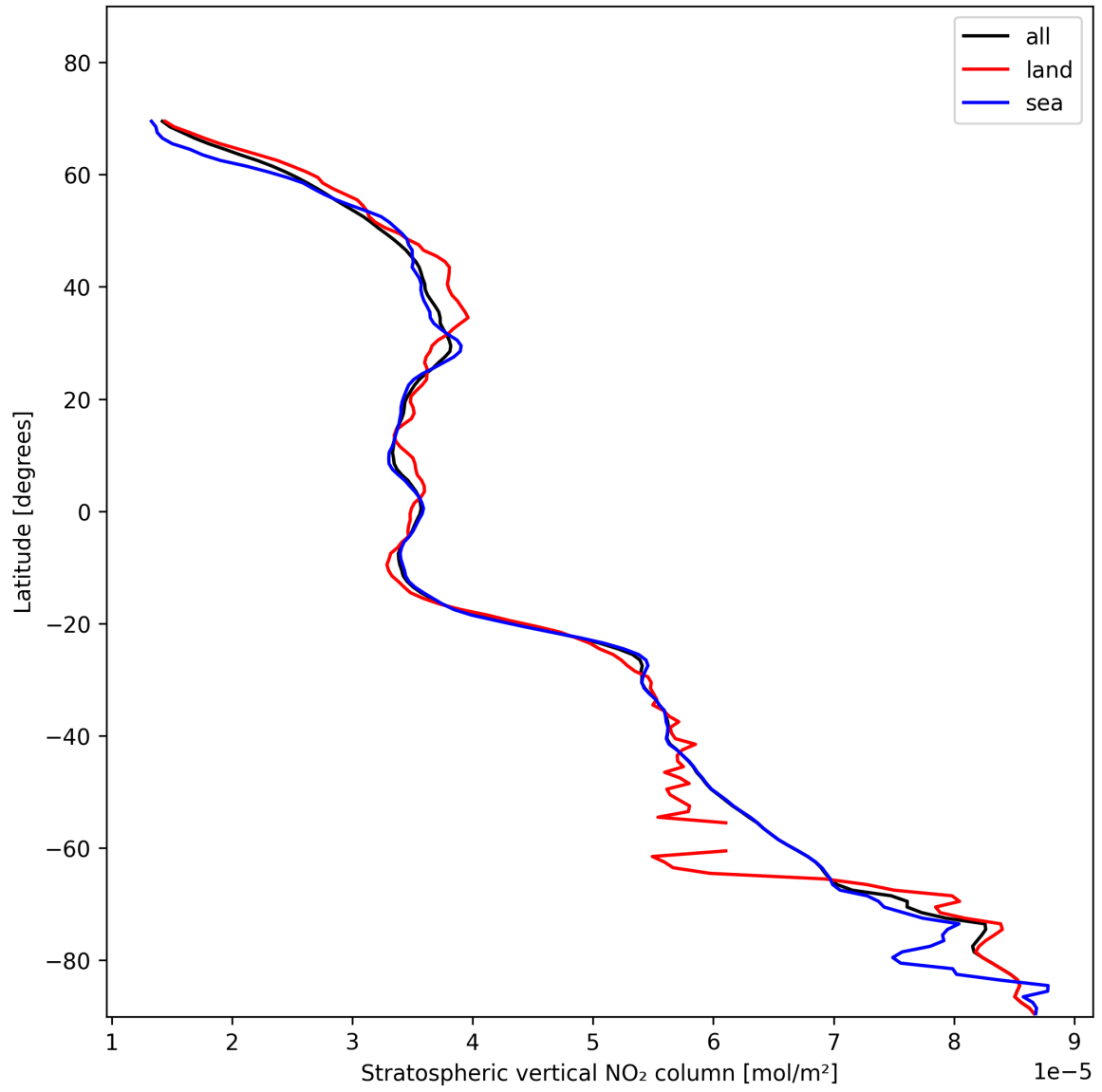
Figure 19: Zonal average of “Stratospheric vertical NO 2 column” for 2025-11-14 to 2025-11-16.
