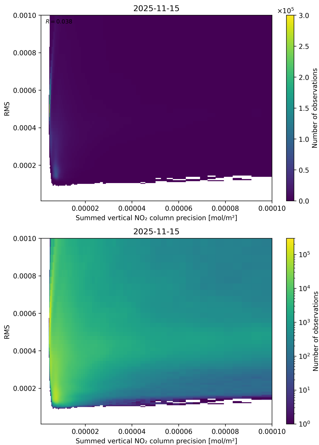
Figure 108: Scatter density plot of “Summed vertical NO 2 column precision” against “RMS” for 2025-11-14 to 2025-11-16.
