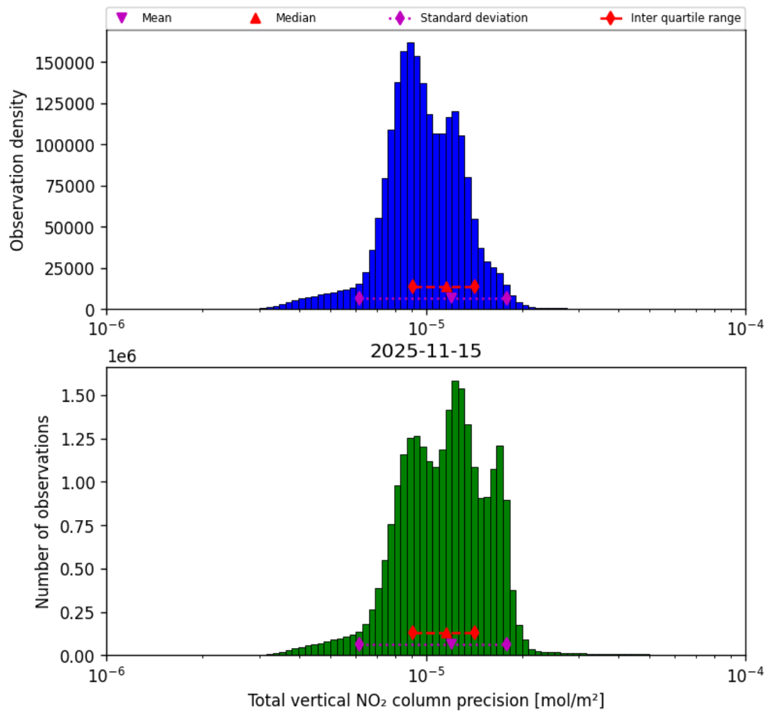
Figure 39: Histogram of “Total vertical NO 2 column precision” for 2025-11-14 to 2025-11-16
