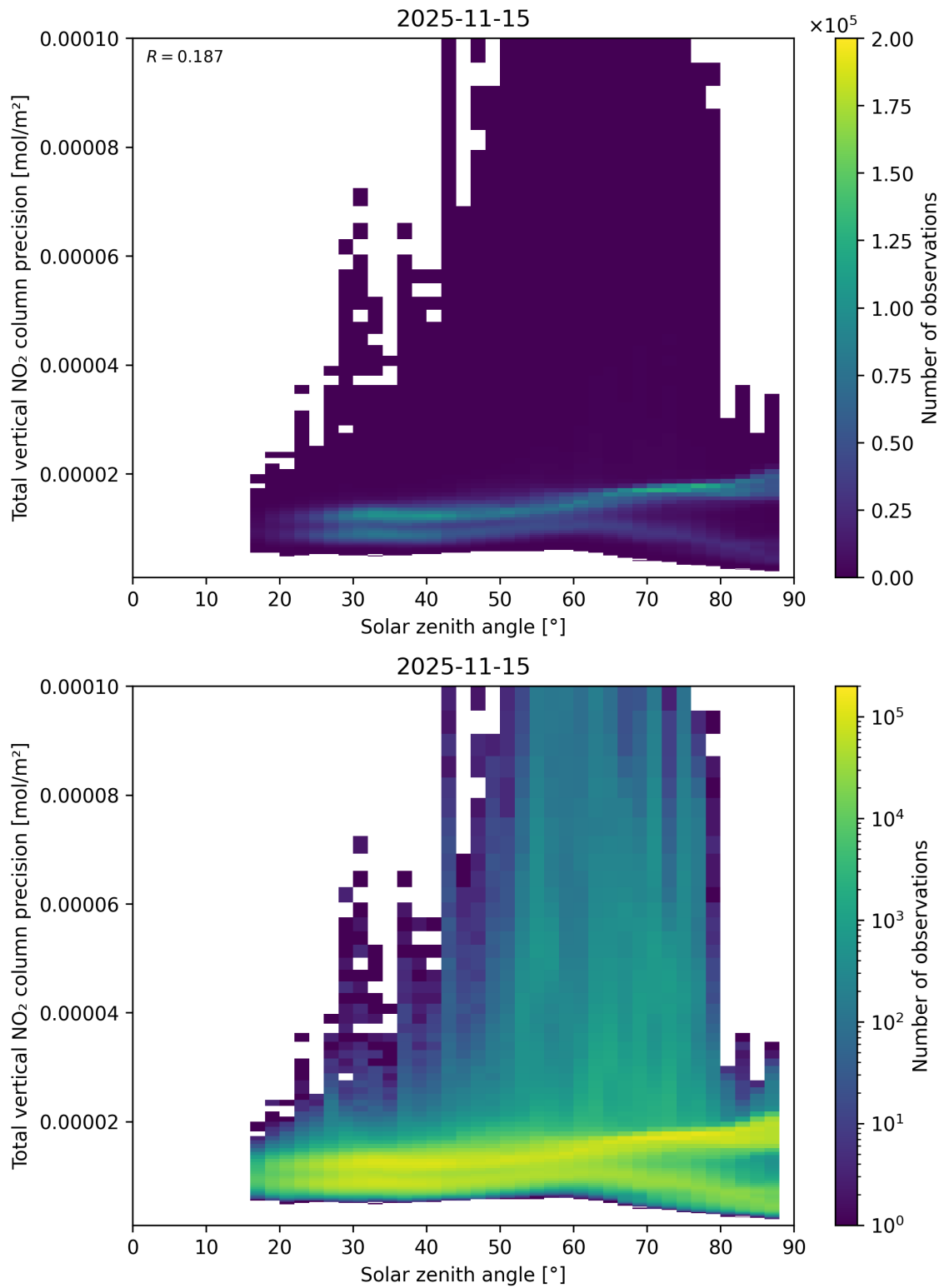
Figure 154: Scatter density plot of “Solar zenith angle” against “Total vertical NO 2 column precision” for 2025-11-14 to 2025-11-16.
