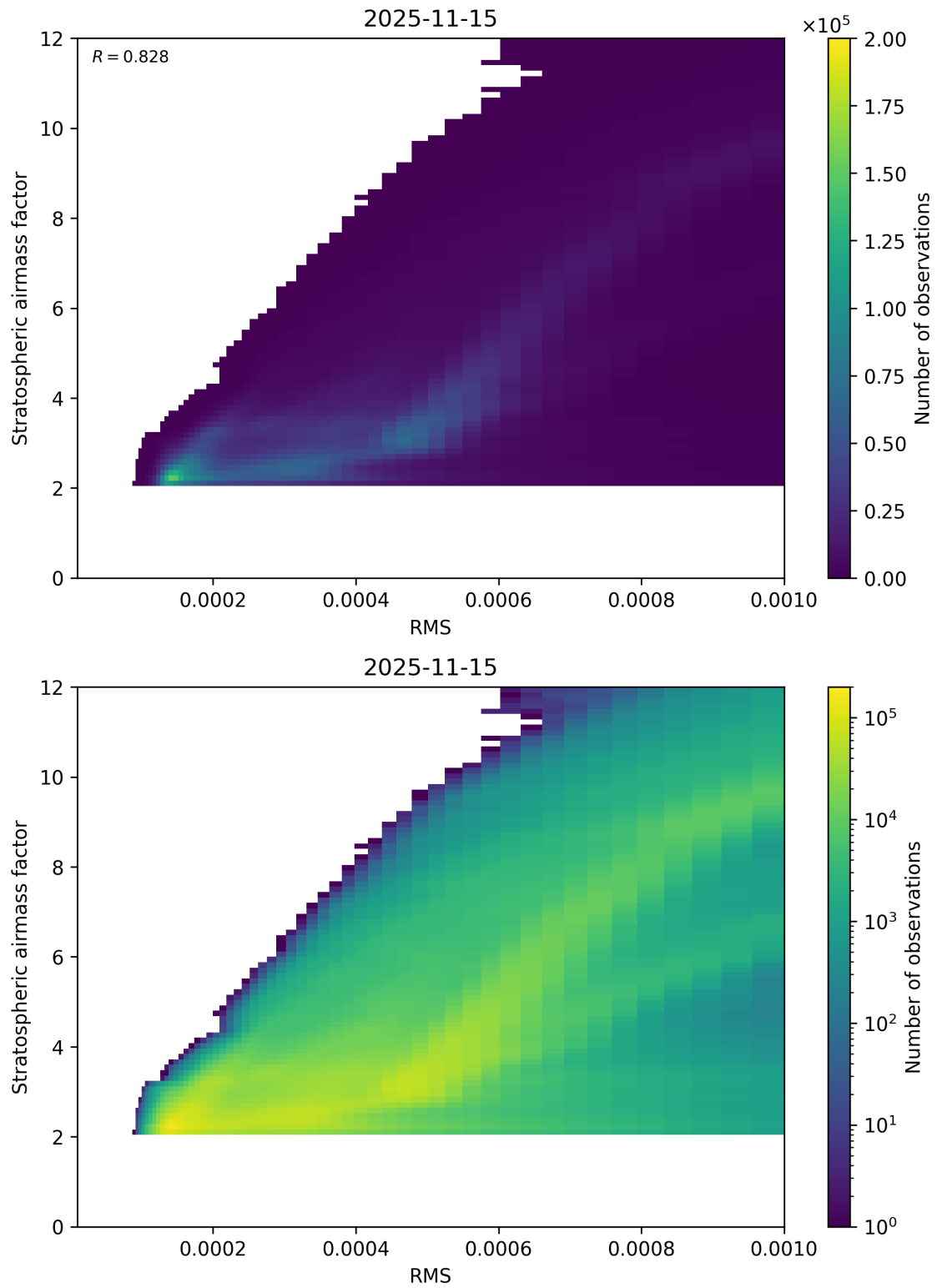
Figure 144: Scatter density plot of “RMS” against “Stratospheric airmass factor” for 2025-11-14 to 2025-11-16.
