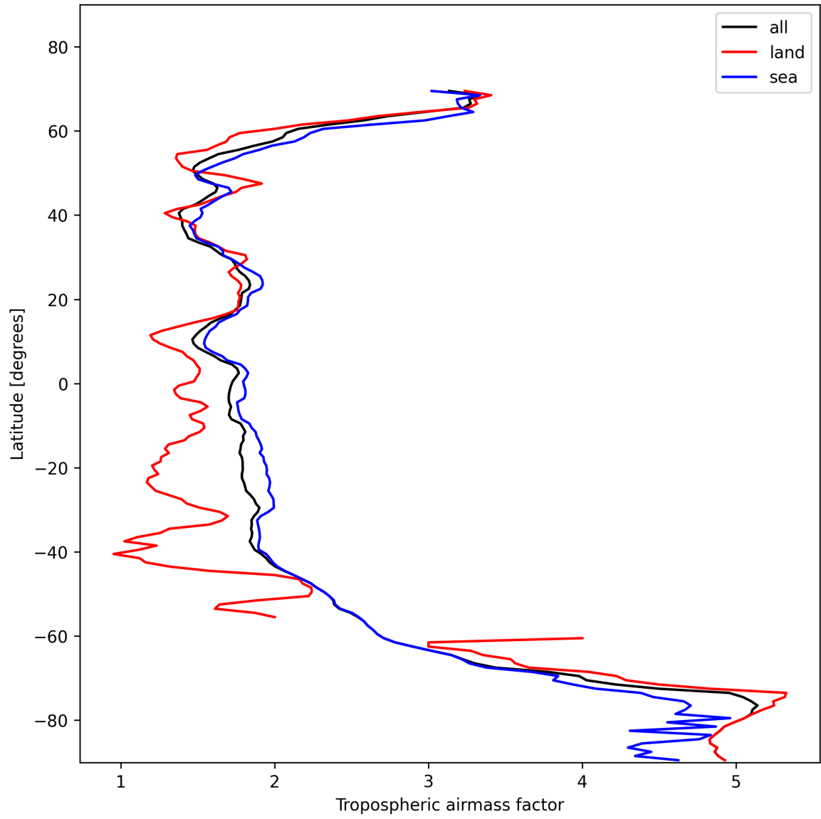
Figure 14: Zonal average of “Tropospheric airmass factor” for 2025-11-14 to 2025-11-16.
