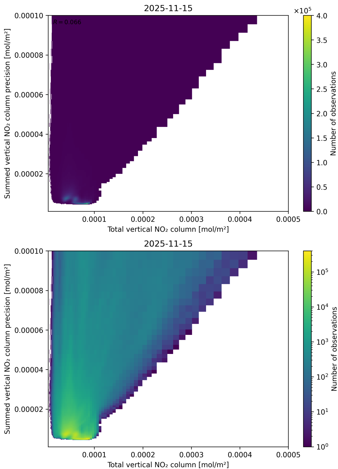
Figure 113: Scatter density plot of “Total vertical NO 2 column” against “Summed vertical NO 2 column precision” for 2025-11-14 to 2025-11-16.
