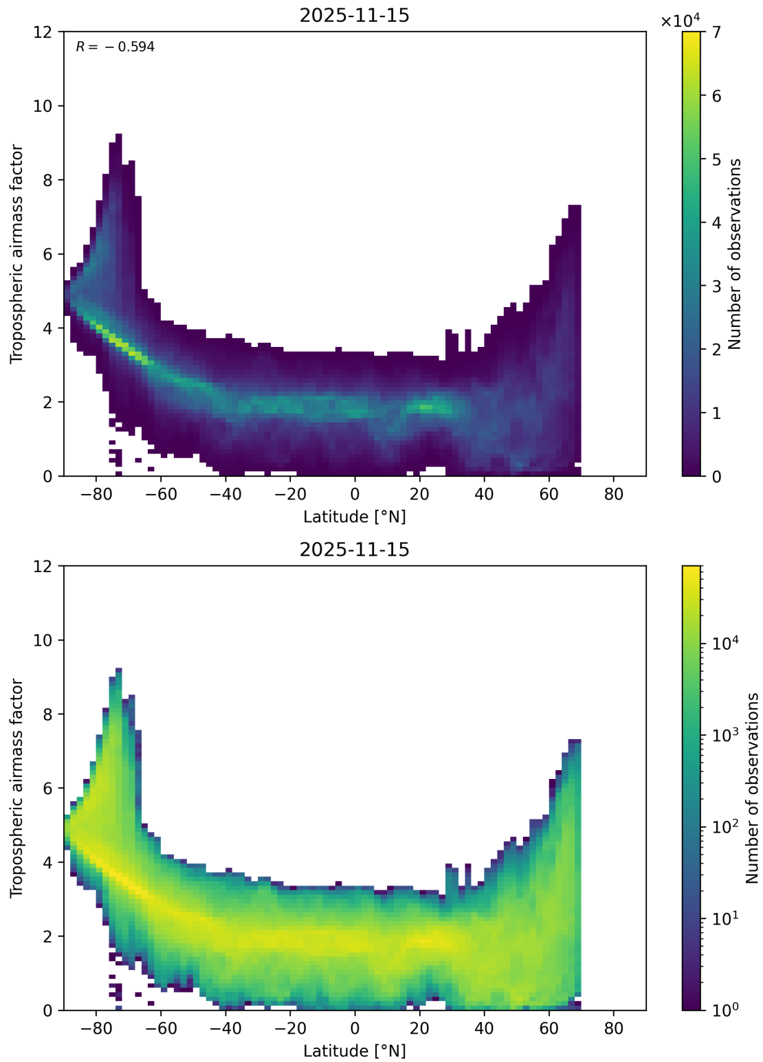
Figure 85: Scatter density plot of “Latitude” against “Tropospheric air mass factor” for 2025-11-14 to 2025-11-16.
