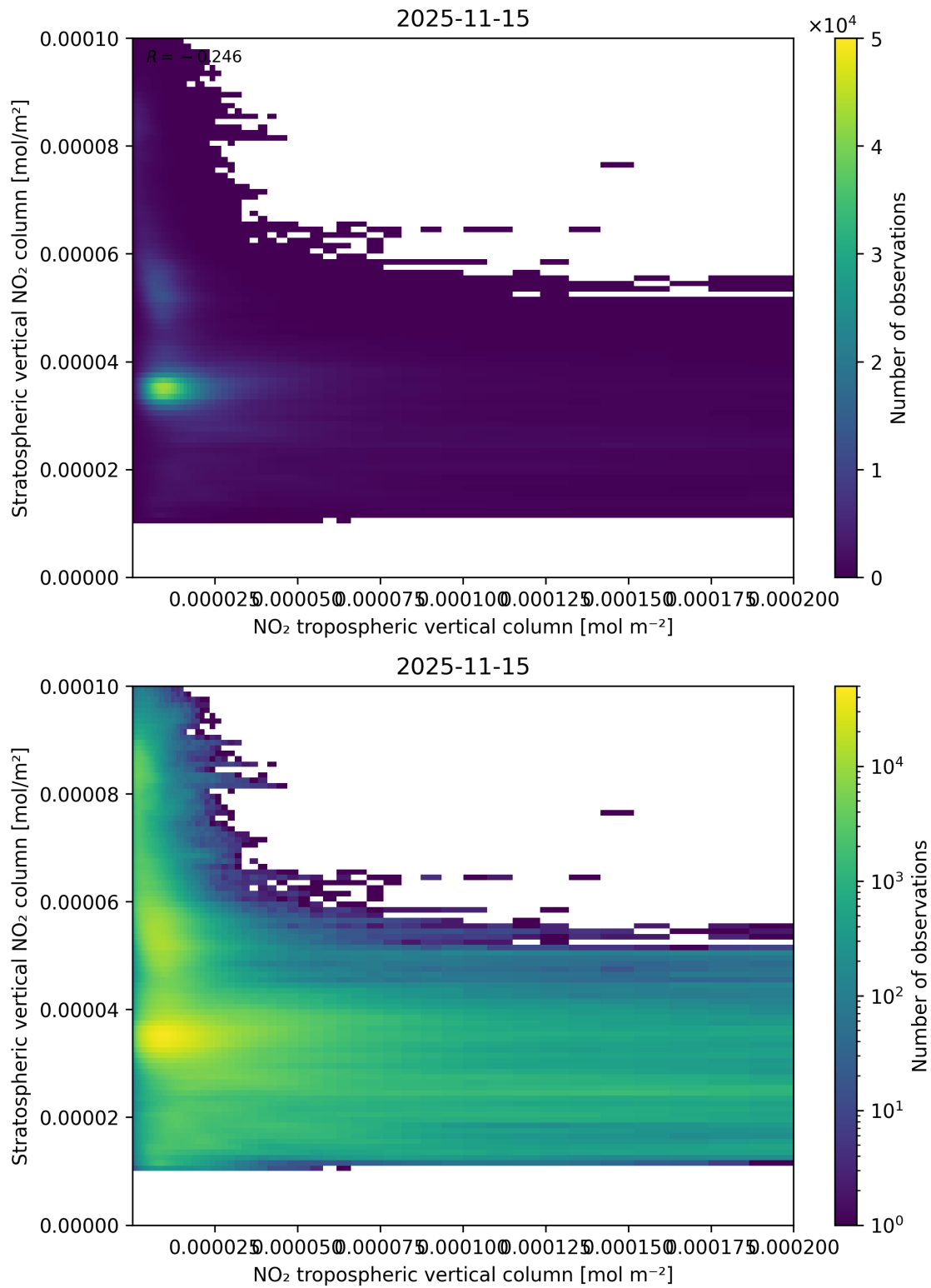
Figure 125: Scatter density plot of “NO 2 tropospheric vertical column” against “Stratospheric vertical NO 2 column” for 2025-11-14 to 2025-11-16.
