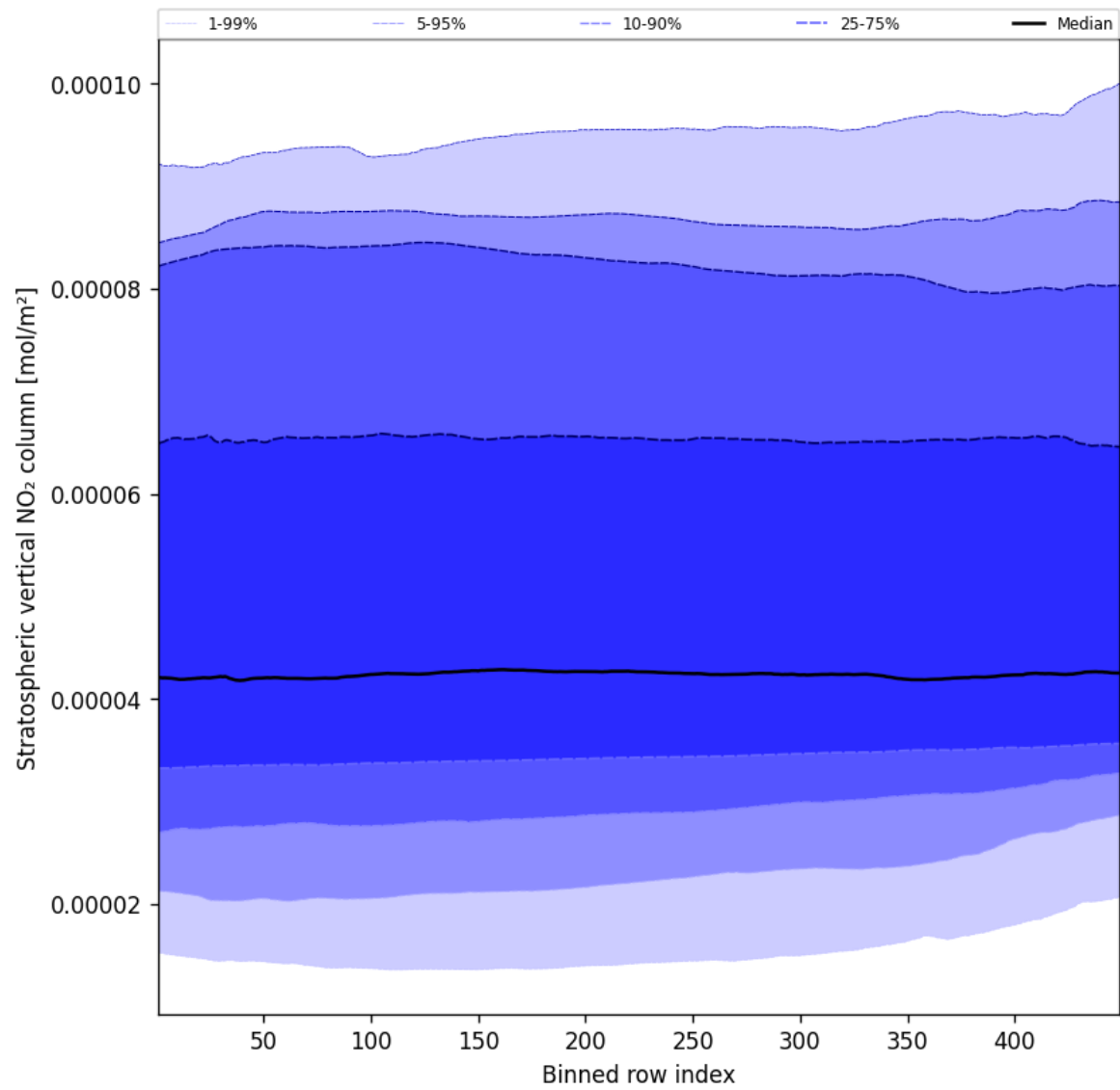
Figure 53: Along track statistics of “Stratospheric vertical NO 2 column” for 2025-11-14 to 2025-11-16
