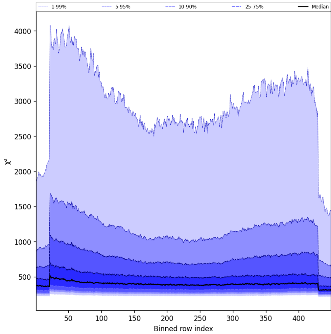
Figure 59: Along track statistics of “ \chi^2 ” for 2025-11-14 to 2025-11-16
