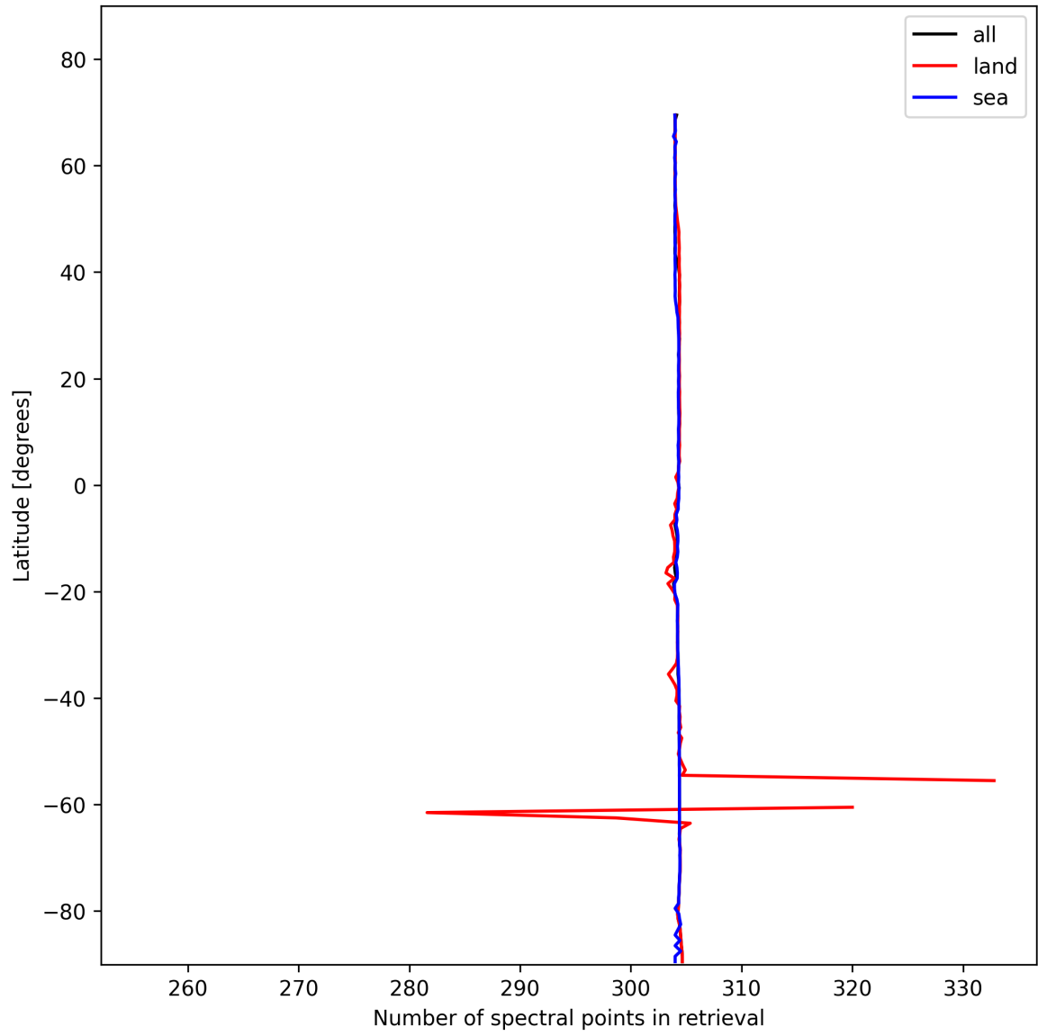
Figure 16: Zonal average of “Number of spectral points in retrieval” for 2025-11-14 to 2025-11-16.
