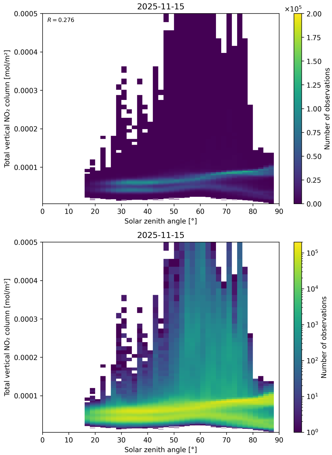
Figure 153: Scatter density plot of “Solar zenith angle” against “Total vertical NO 2 column” for 2025-11-14 to 2025-11-16.
