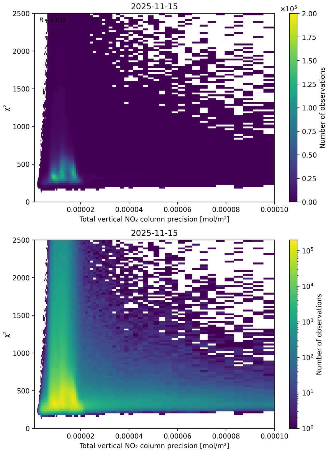
Figure 116: Scatter density plot of “Total vertical NO 2 column precision” against “ \chi^2 ” for 2025-11-14 to 2025-11-16.
