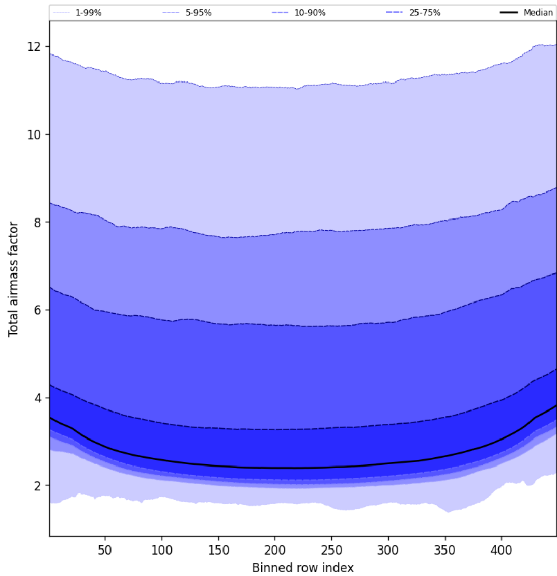
Figure 49: Along track statistics of “Total airmass factor” for 2025-11-14 to 2025-11-16
