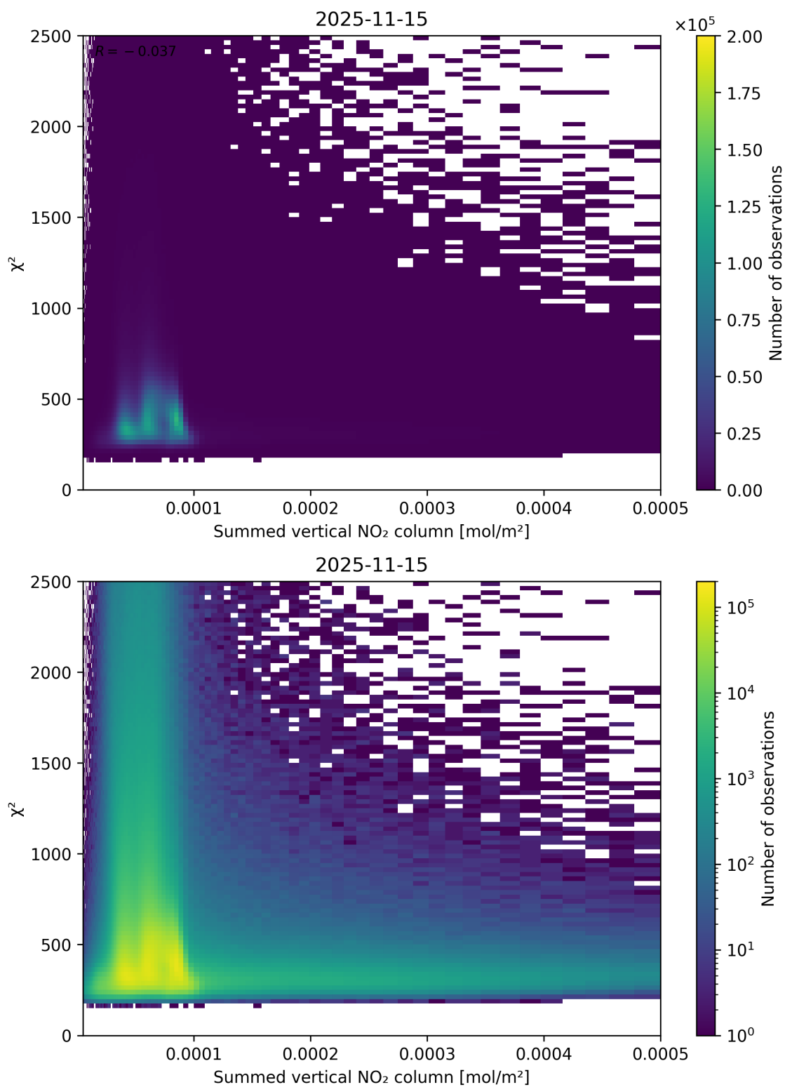
Figure 104: Scatter density plot of “Summed vertical NO 2 column” against “ \chi^2 ” for 2025-11-14 to 2025-11-16.
