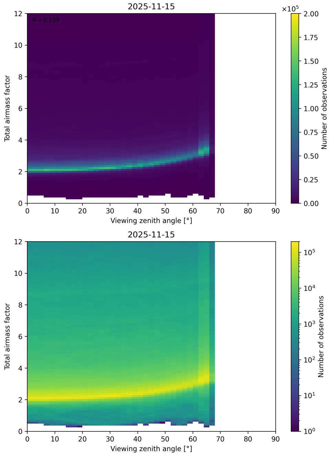
Figure 160: Scatter density plot of “Viewing zenith angle” against “Total airmass factor” for 2025-11-14 to 2025-11-16.
