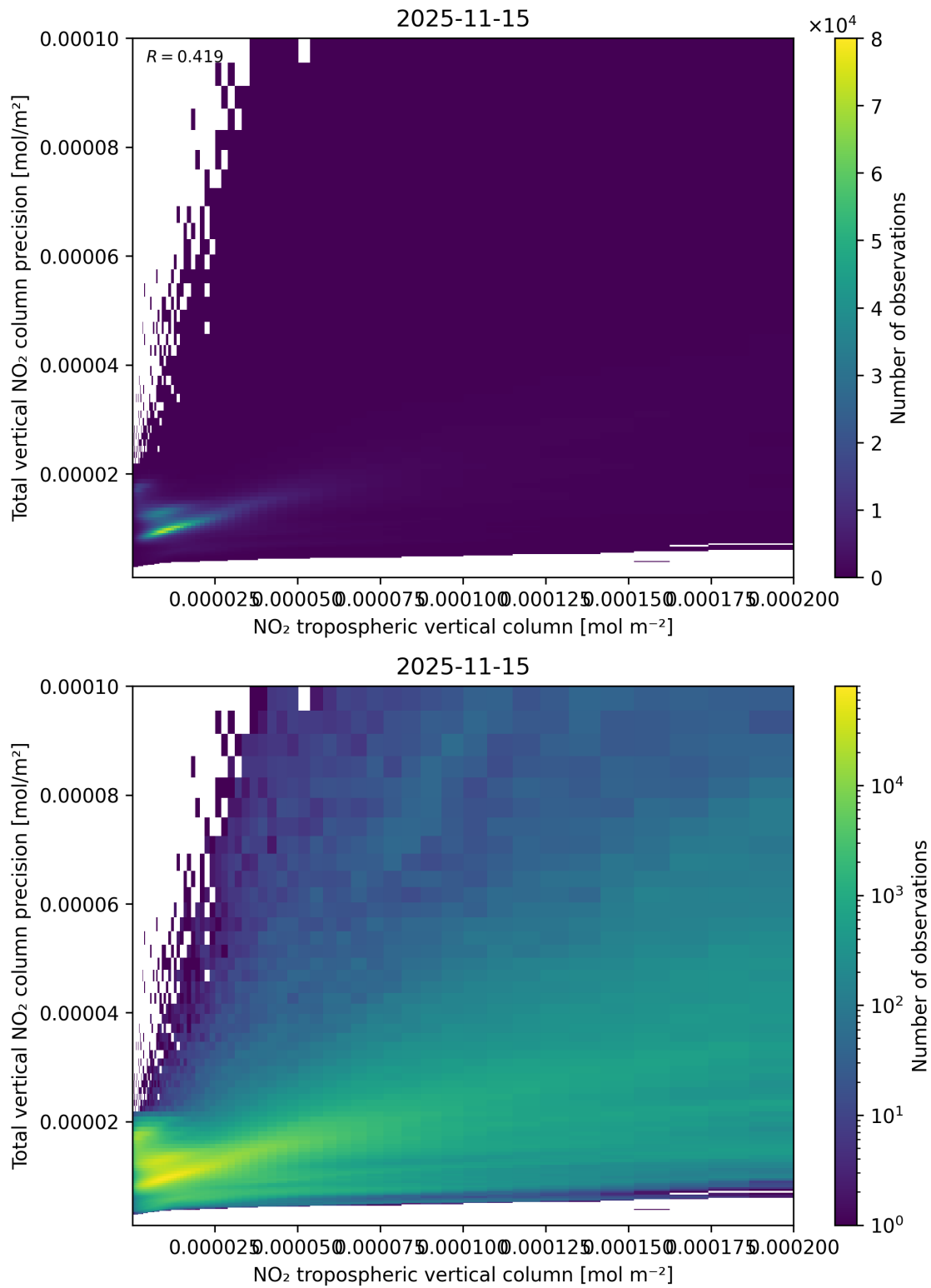
Figure 129: Scatter density plot of “NO 2 tropospheric vertical column” against “Total vertical NO 2 column precision” for 2025-11-14 to 2025-11-16.
