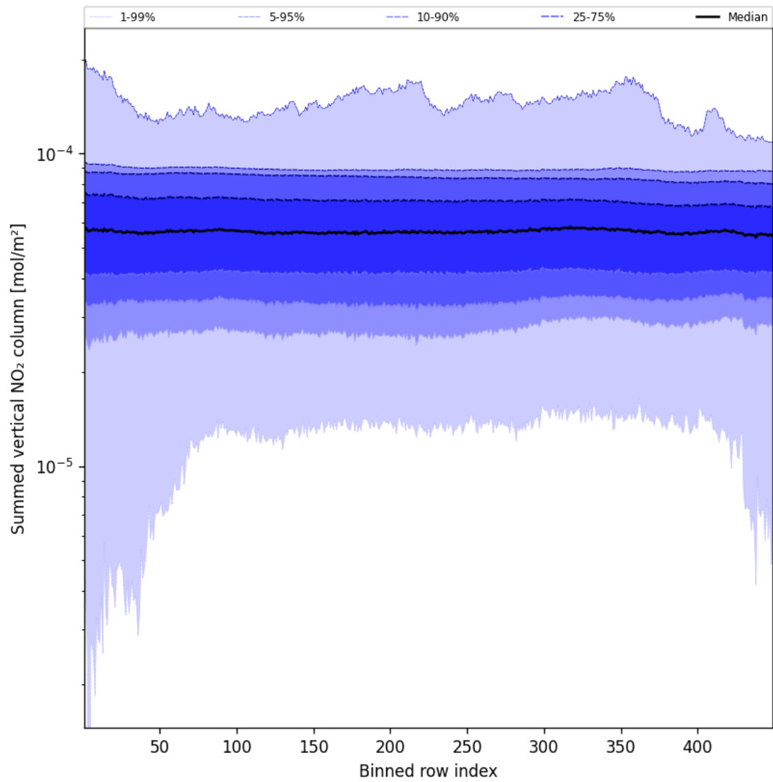
Figure 57: Along track statistics of “Summed vertical NO 2 column” for 2025-11-14 to 2025-11-16
