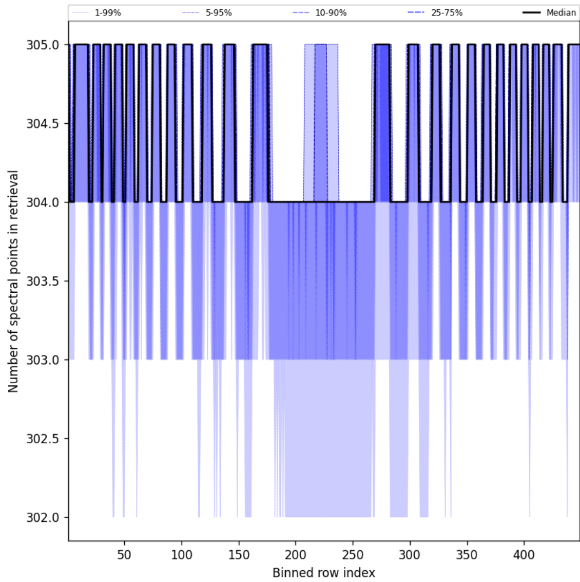
Figure 50: Along track statistics of “Number of spectral points in retrieval” for 2025-11-14 to 2025-11-16
