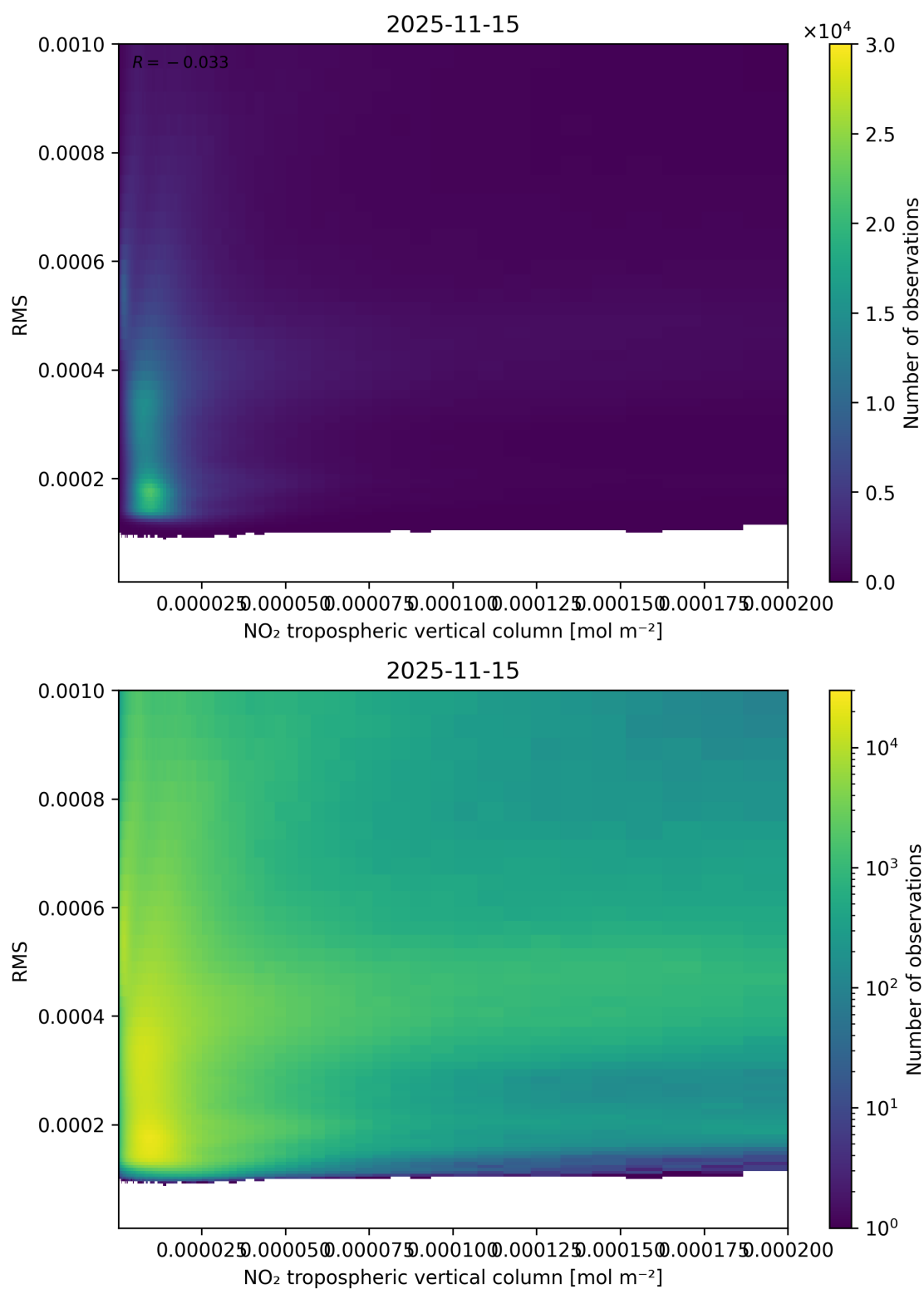
Figure 142: Scatter density plot of “NO 2 tropospheric vertical column” against “RMS” for 2025-11-14 to 2025-11-16.
