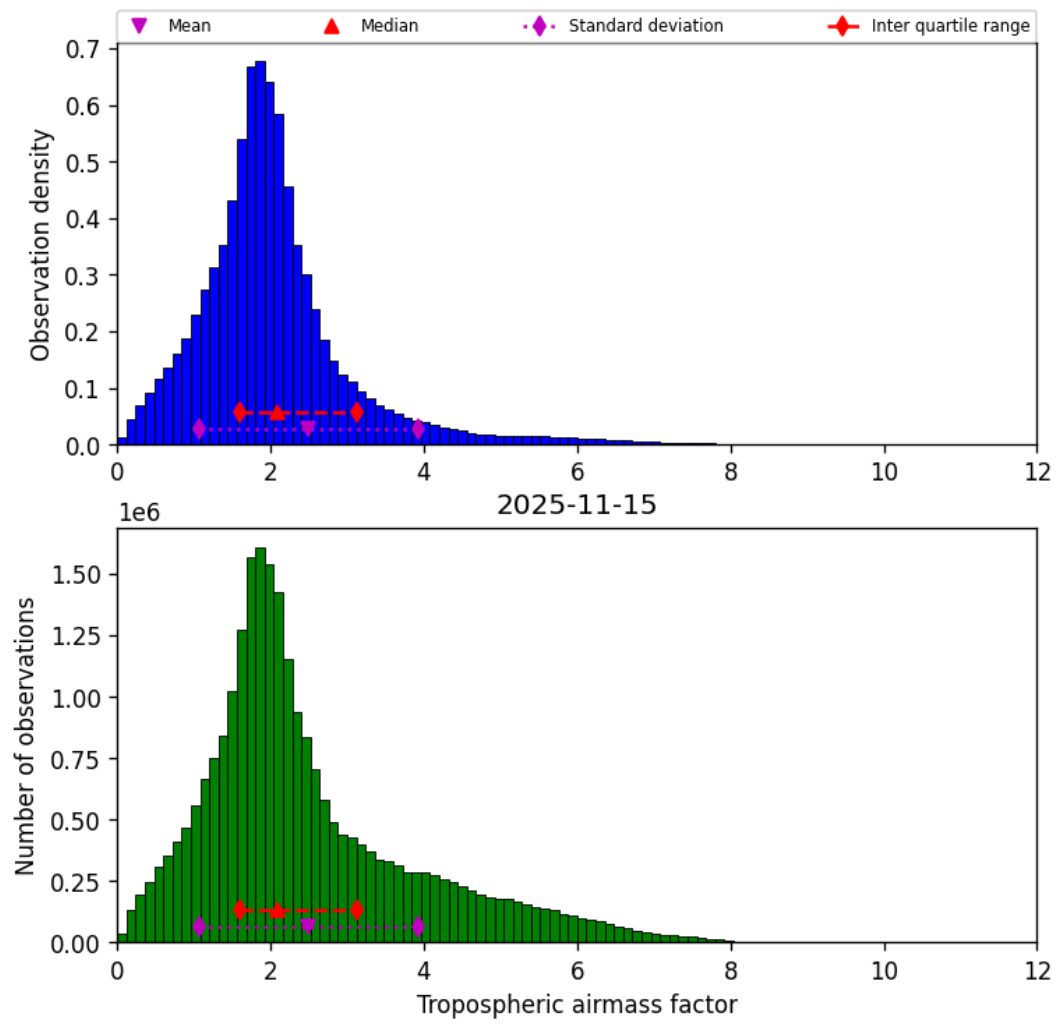
Figure 31: Histogram of “Tropospheric airmass factor” for 2025-11-14 to 2025-11-16
