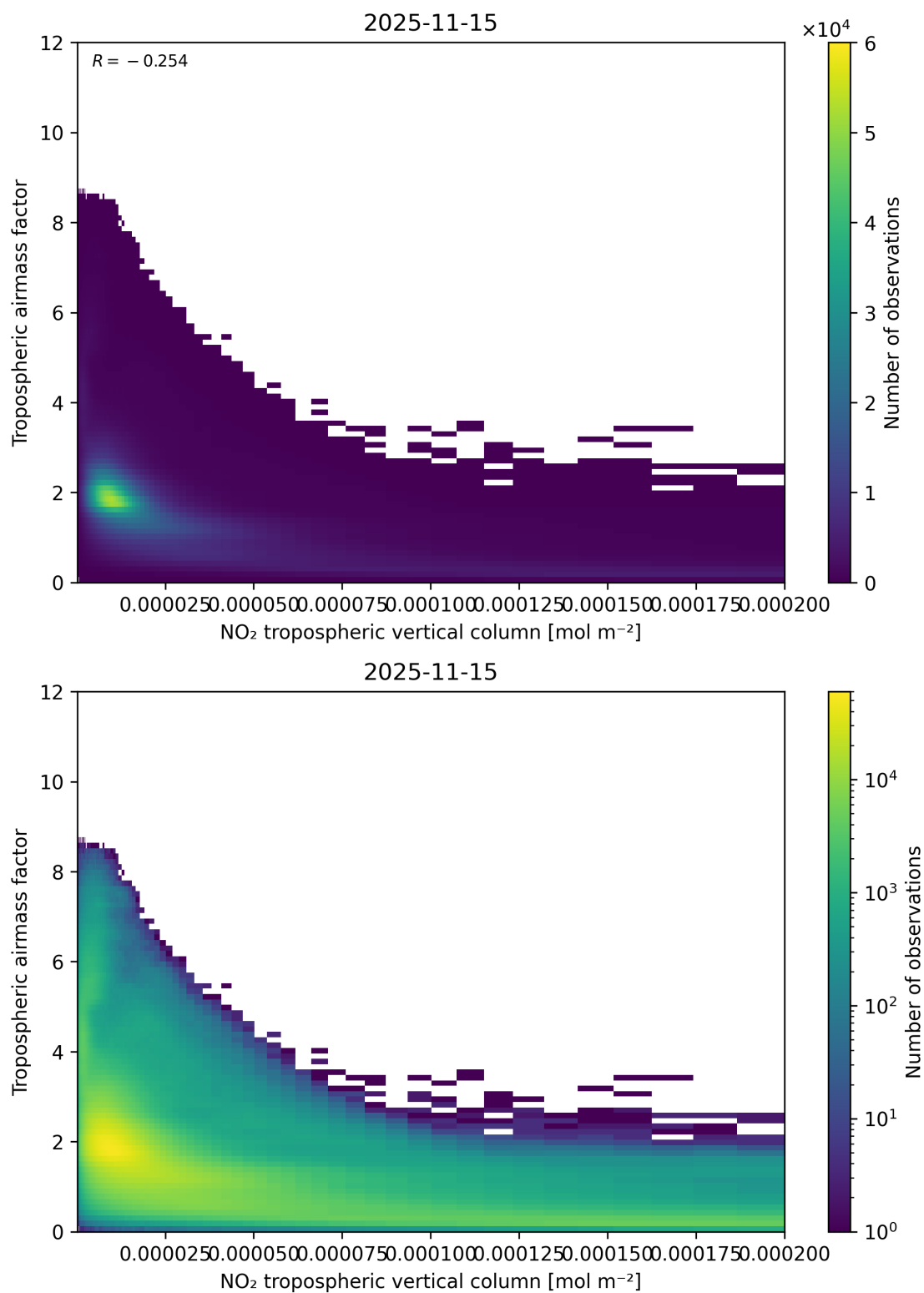
Figure 123: Scatter density plot of “NO 2 tropospheric vertical column” against “Tropospheric air mass factor” for 2025-11-14 to 2025-11-16.
