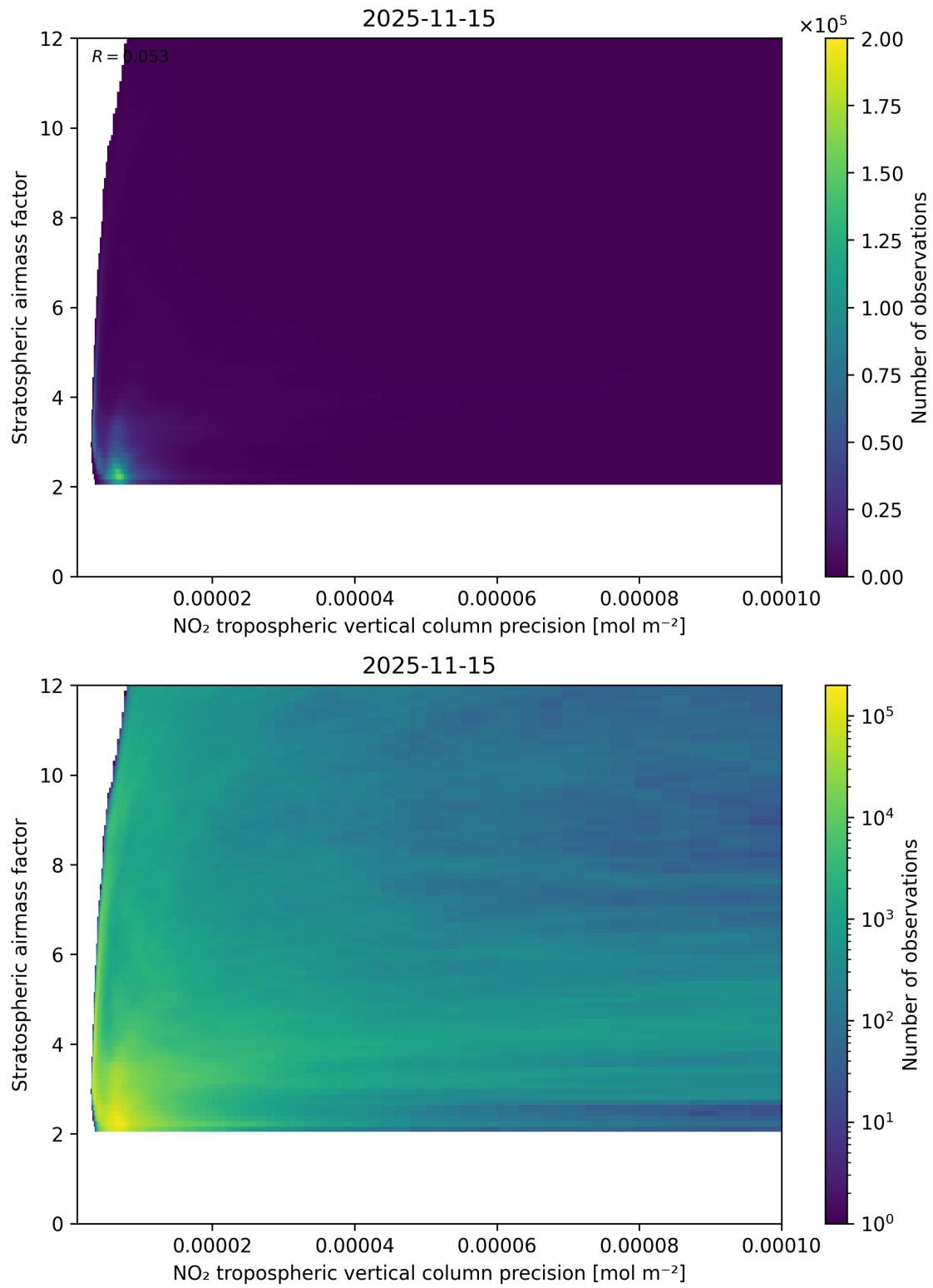
Figure 131: Scatter density plot of “NO 2 tropospheric vertical column precision” against “Stratospheric airmass factor” for 2025-11-14 to 2025-11-16.
