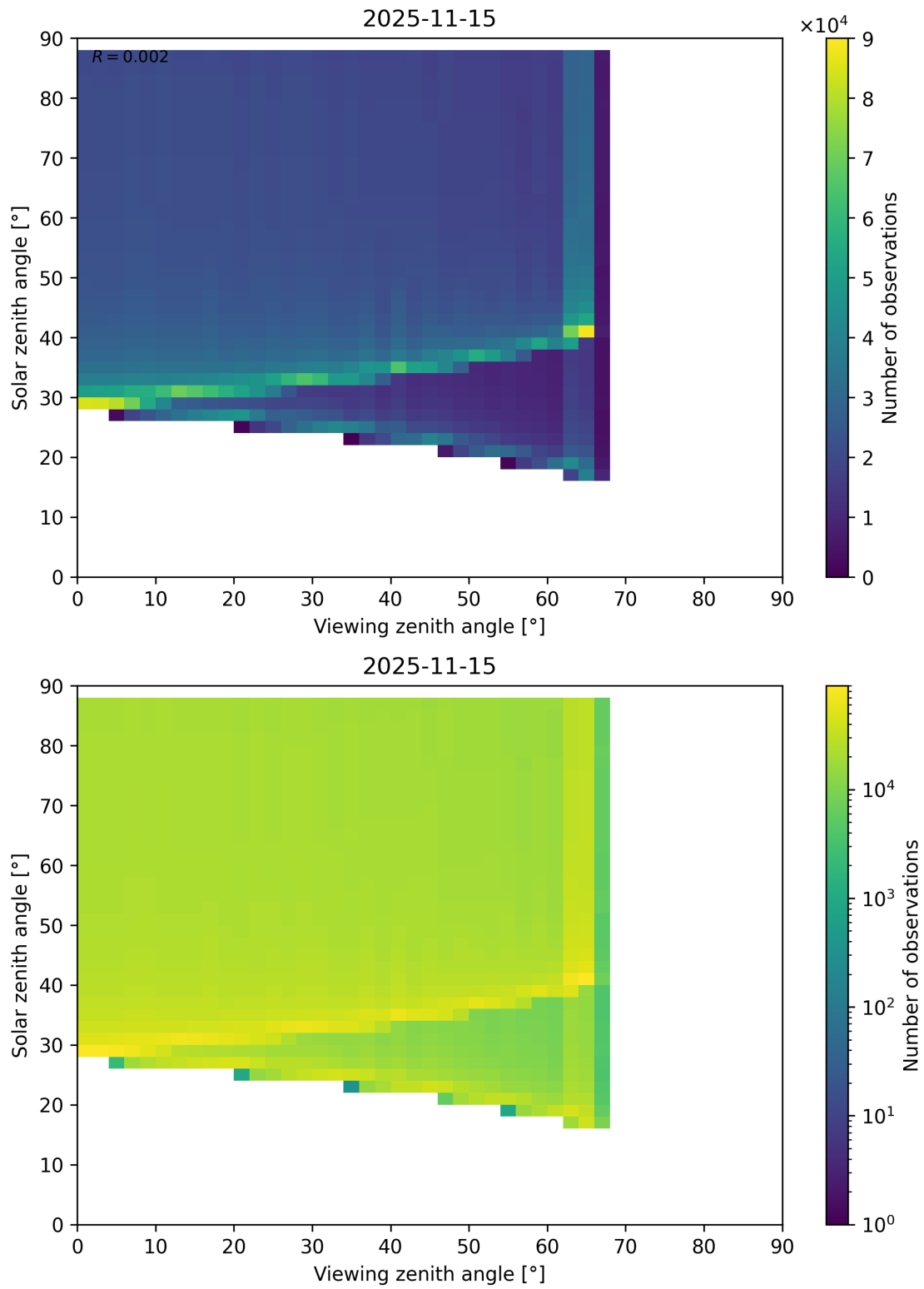
Figure 172: Scatter density plot of “Viewing zenith angle” against “Solar zenith angle” for 2025-11-14 to 2025-11-16.
