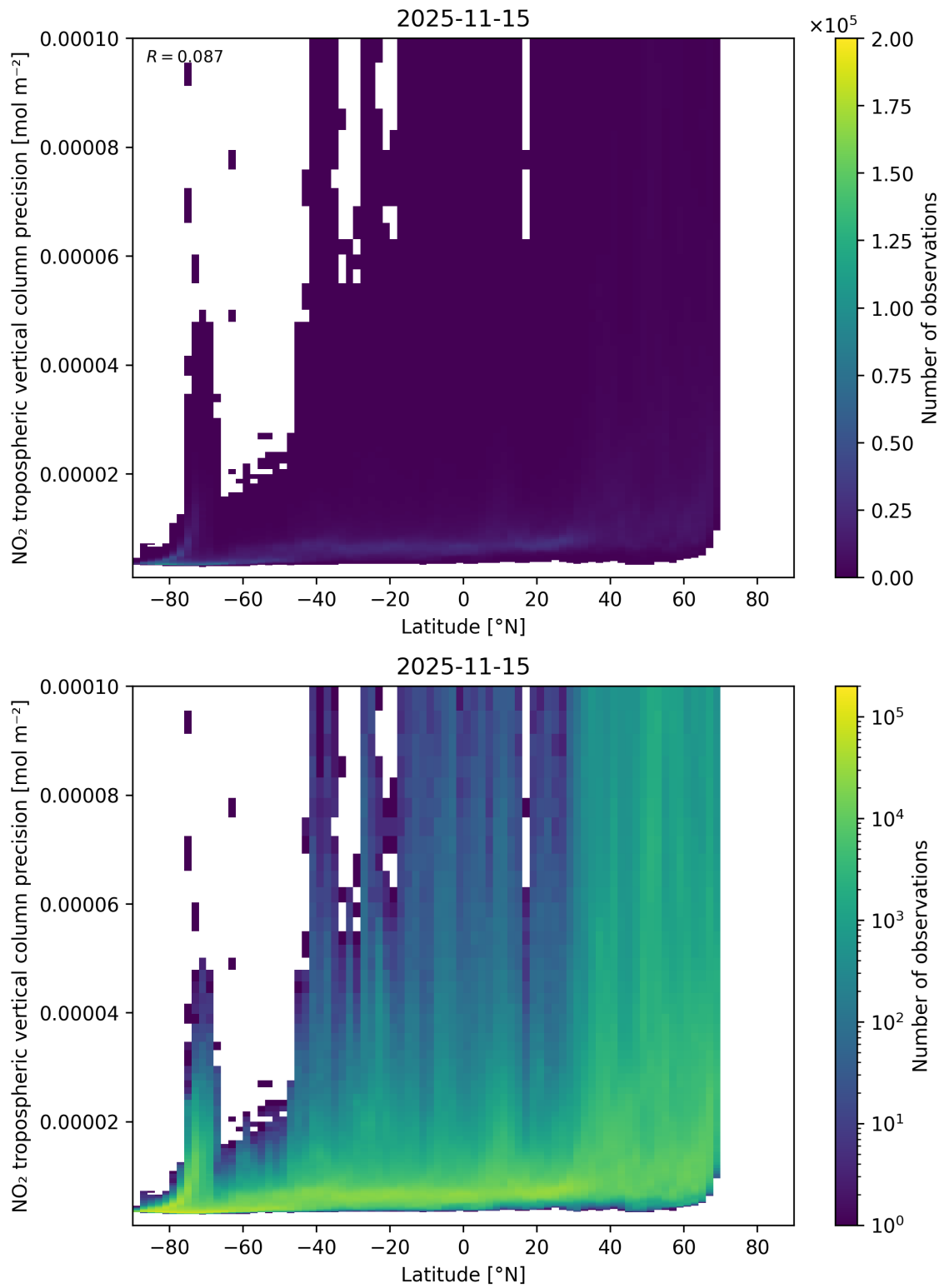
Figure 93: Scatter density plot of “Latitude” against “NO 2 tropospheric vertical column precision” for 2025-11-14 to 2025-11-16.
