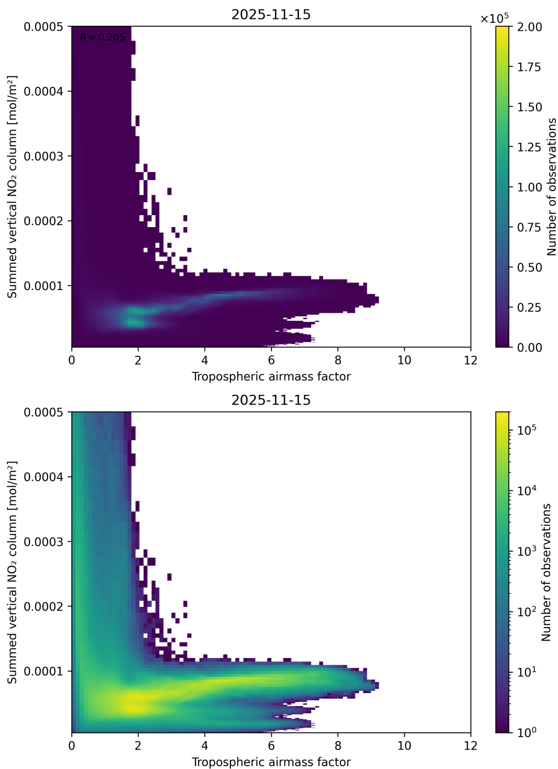
Figure 75: Scatter density plot of “Tropospheric air mass factor” against “Summed vertical NO 2 column” for 2025-11-14 to 2025-11-16.
