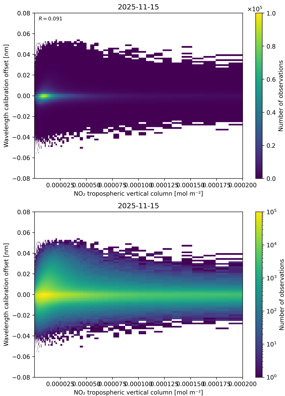
Figure 143: Scatter density plot of “NO 2 tropospheric vertical column” against “Wavelength calibration offset” for 2025-11-14 to 2025-11-16.
