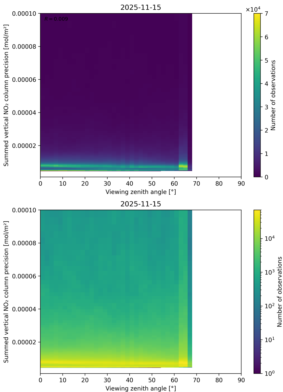
Figure 166: Scatter density plot of “Viewing zenith angle” against “Summed vertical NO 2 column precision” for 2025-11-14 to 2025-11-16.
