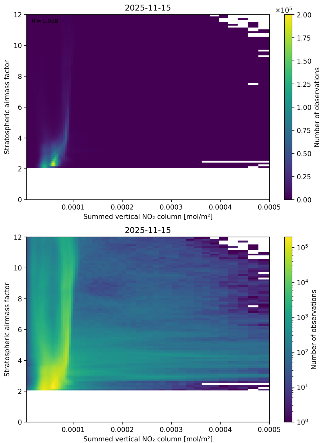
Figure 103: Scatter density plot of “Summed vertical NO 2 column” against “Stratospheric airmass factor” for 2025-11-14 to 2025-11-16.
