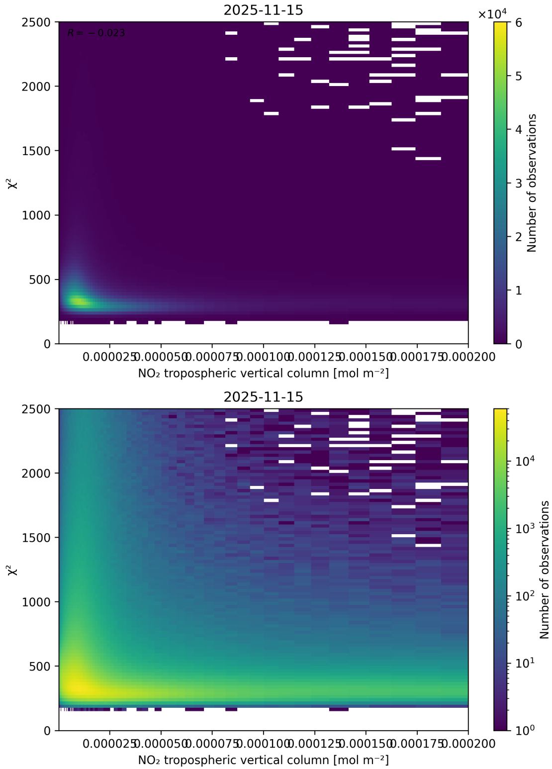
Figure 124: Scatter density plot of “NO 2 tropospheric vertical column” against “ \chi^2 ” for 2025-11-14 to 2025-11-16.
