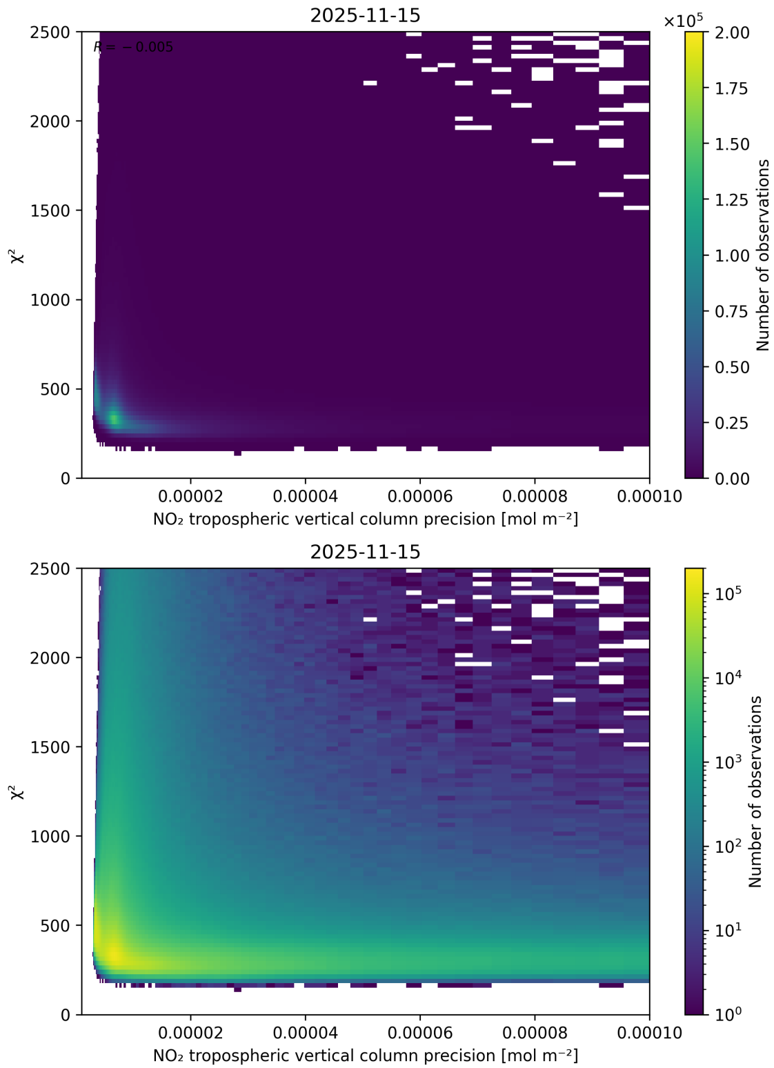
Figure 134: Scatter density plot of “NO 2 tropospheric vertical column precision” against “ \chi^2 ” for 2025-11-14 to 2025-11-16.
