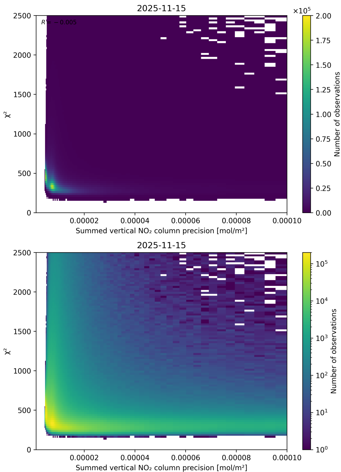
Figure 107: Scatter density plot of “Summed vertical NO 2 column precision” against “ \chi^2 ” for 2025-11-14 to 2025-11-16.
