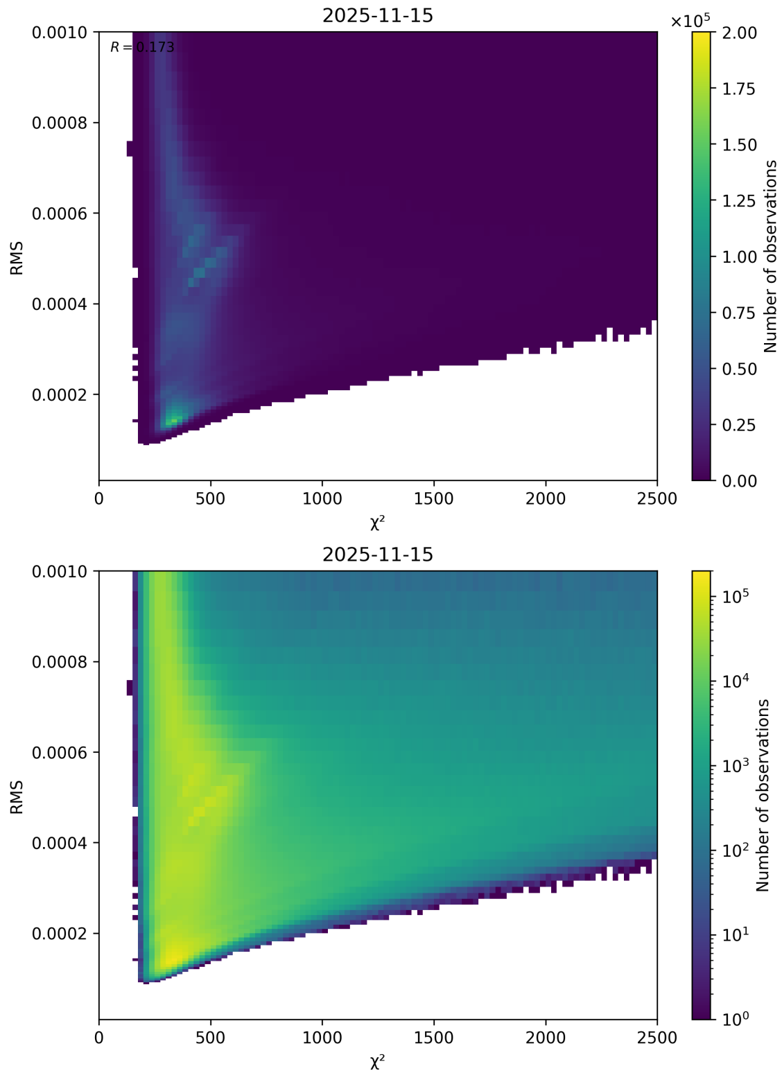
Figure 82: Scatter density plot of “ \chi^2 ” against “RMS” for 2025-11-14 to 2025-11-16.
