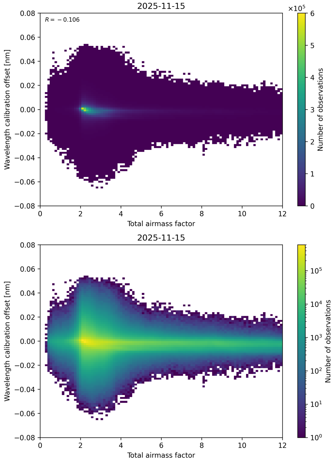
Figure 70: Scatter density plot of “Total airmass factor” against “Wavelength calibration offset” for 2025-11-14 to 2025-11-16.
