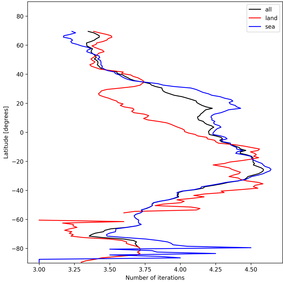
Figure 17: Zonal average of “Number of iterations” for 2025-11-14 to 2025-11-16.
