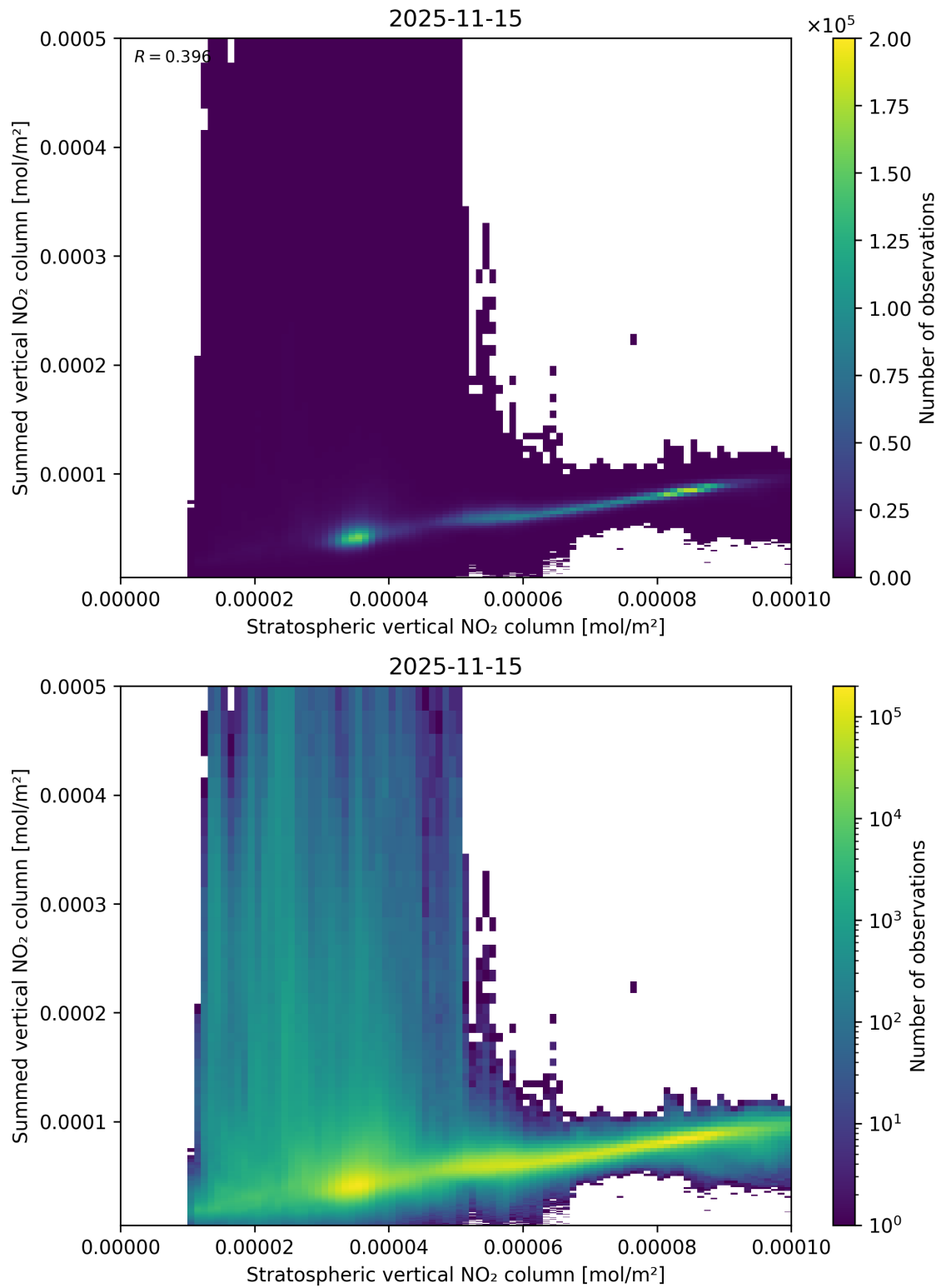
Figure 98: Scatter density plot of “Stratospheric vertical NO 2 column” against “Summed vertical NO 2 column” for 2025-11-14 to 2025-11-16.
