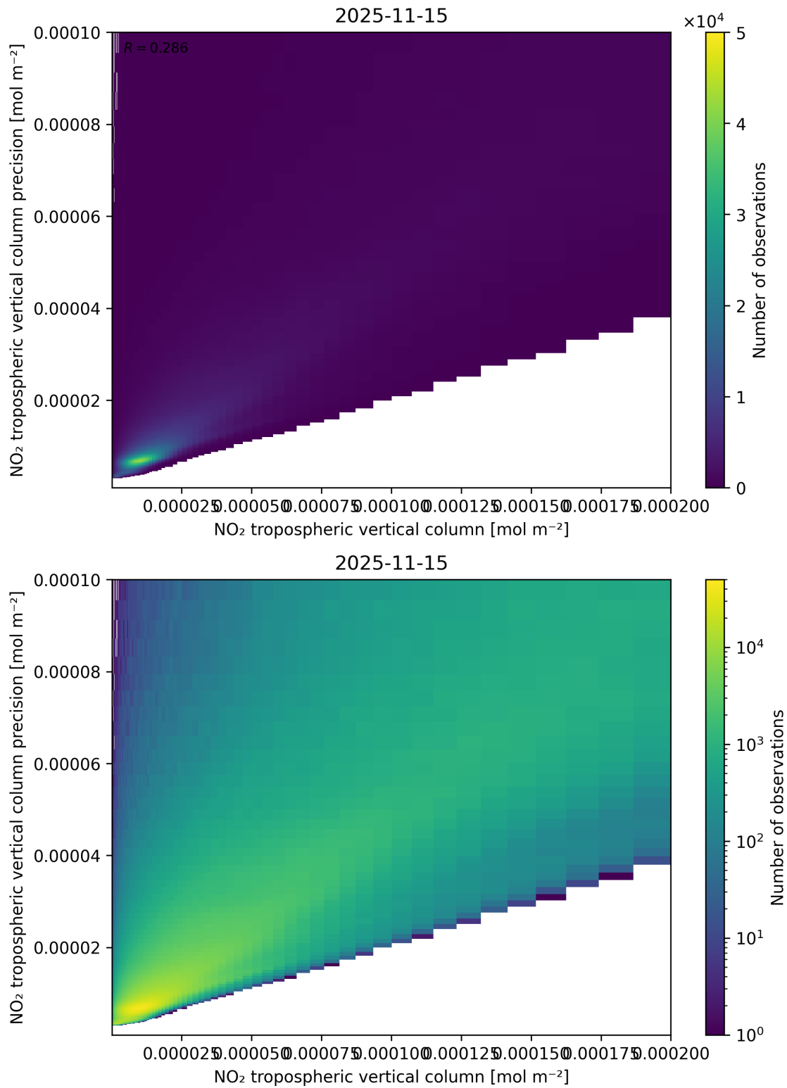
Figure 130: Scatter density plot of “NO 2 tropospheric vertical column” against “NO 2 tropospheric vertical column precision” for 2025-11-14 to 2025-11-16.
