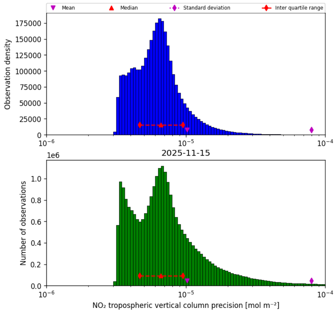
Figure 30: Histogram of “NO 2 tropospheric vertical column precision” for 2025-11-14 to 2025-11-16
