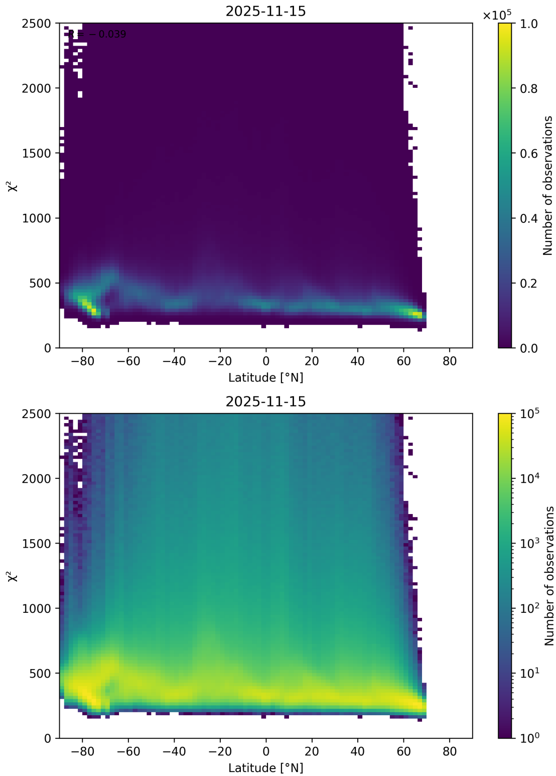
Figure 86: Scatter density plot of “Latitude” against “ \chi^2 ” for 2025-11-14 to 2025-11-16.
