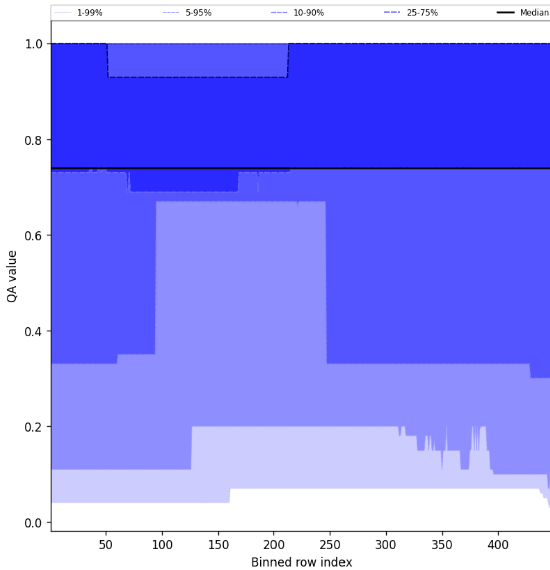
Figure 45: Along track statistics of “QA value” for 2025-11-14 to 2025-11-16
