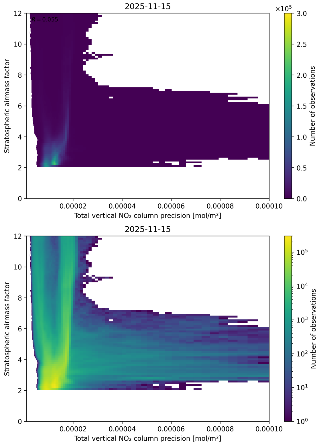
Figure 115: Scatter density plot of “Total vertical NO 2 column precision” against “Stratospheric air mass factor” for 2025-11-14 to 2025-11-16.
