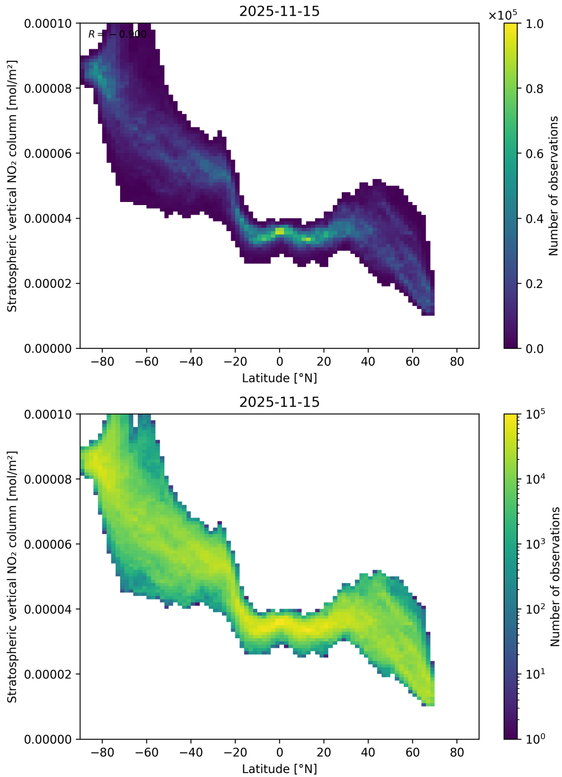
Figure 87: Scatter density plot of “Latitude” against “Stratospheric vertical NO 2 column” for 2025-11-14 to 2025-11-16.
