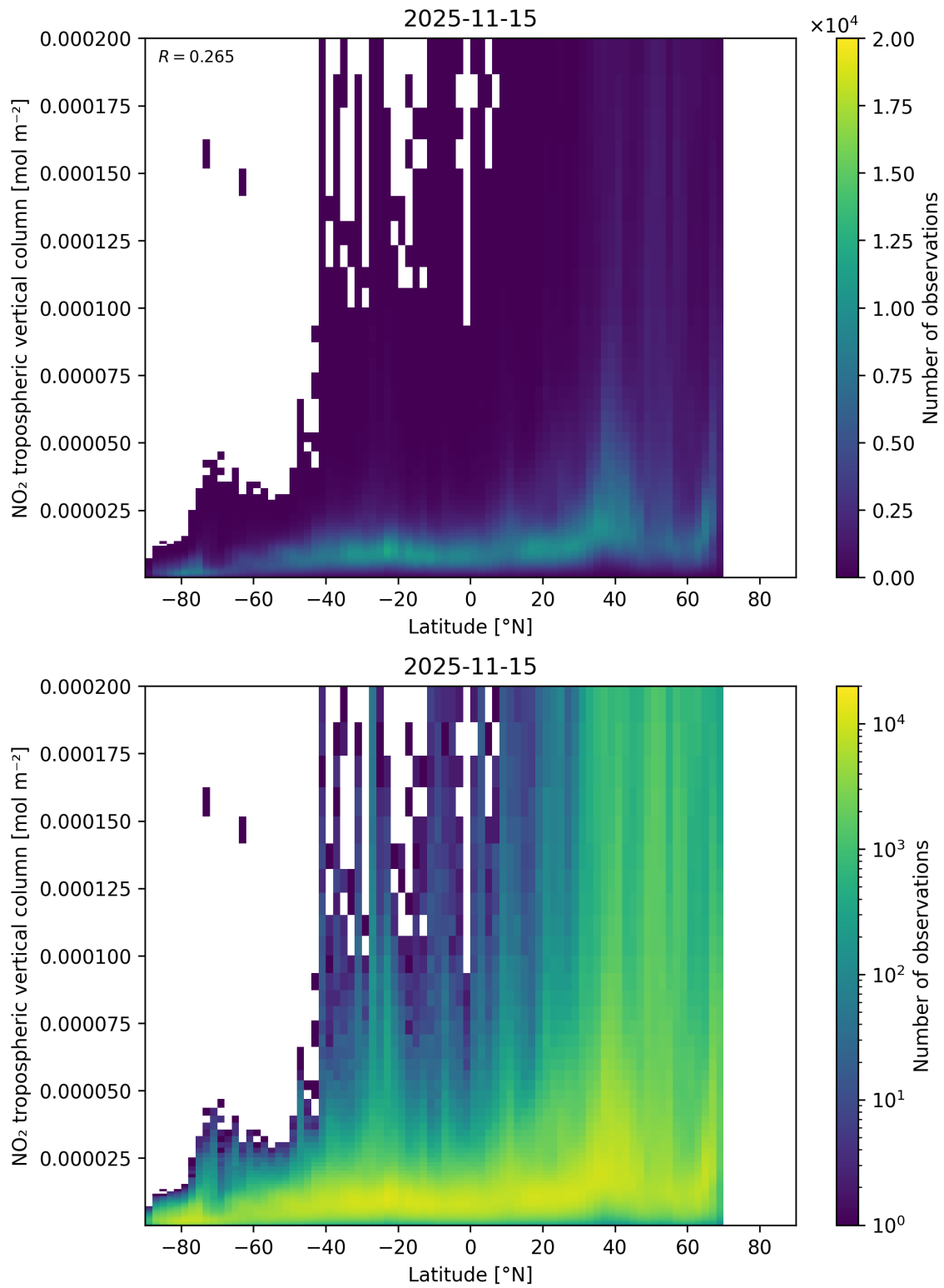
Figure 92: Scatter density plot of “Latitude” against “NO 2 tropospheric vertical column” for 2025-11-14 to 2025-11-16.
