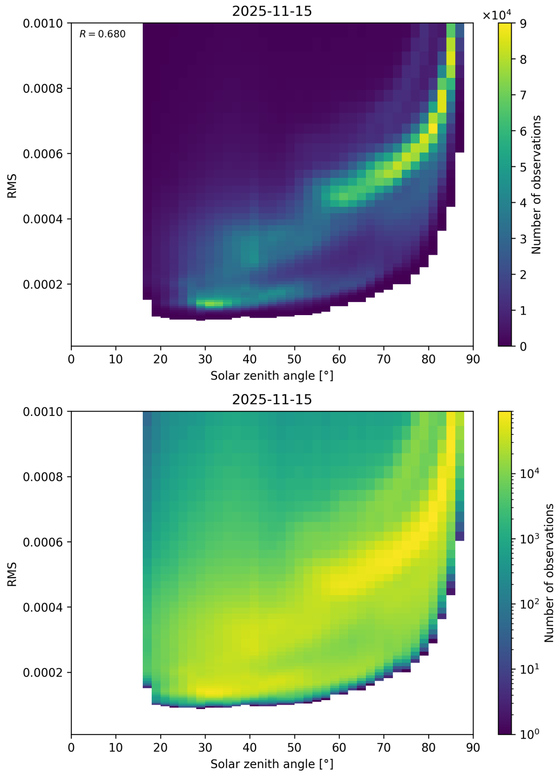
Figure 157: Scatter density plot of “Solar zenith angle” against “RMS” for 2025-11-14 to 2025-11-16.
