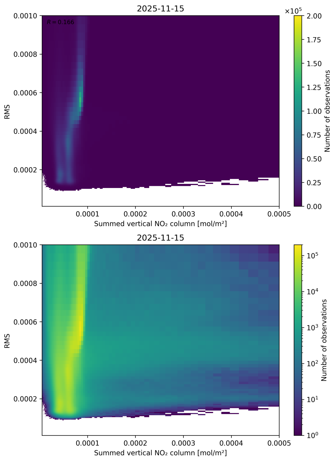
Figure 109: Scatter density plot of “Summed vertical NO 2 column” against “RMS” for 2025-11-14 to 2025-11-16.
