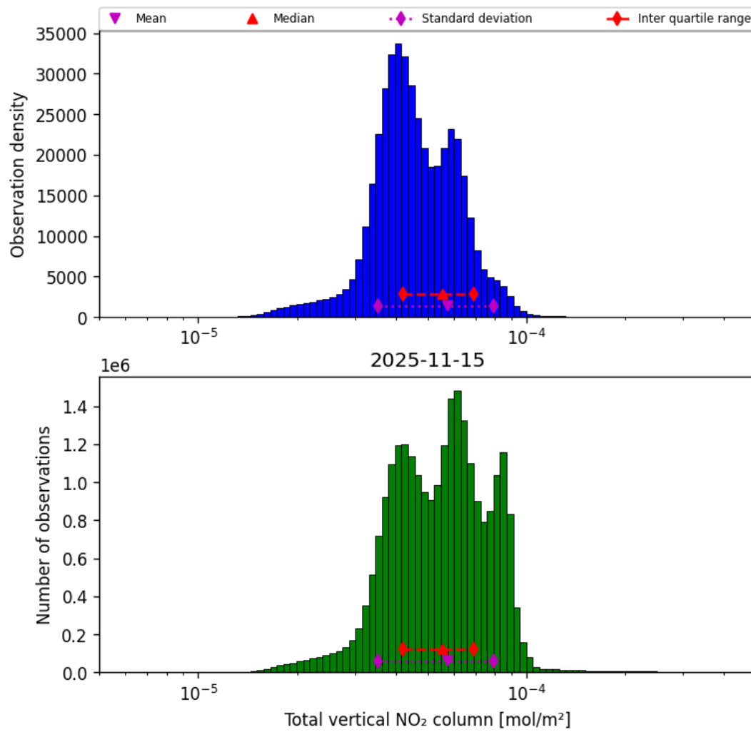
Figure 38: Histogram of “Total vertical NO 2 column” for 2025-11-14 to 2025-11-16
