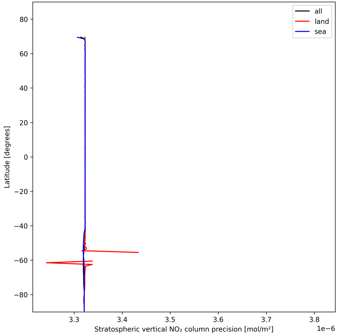
Figure 20: Zonal average of “Stratospheric vertical NO 2 column precision” for 2025-11-14 to 2025-11-16.
