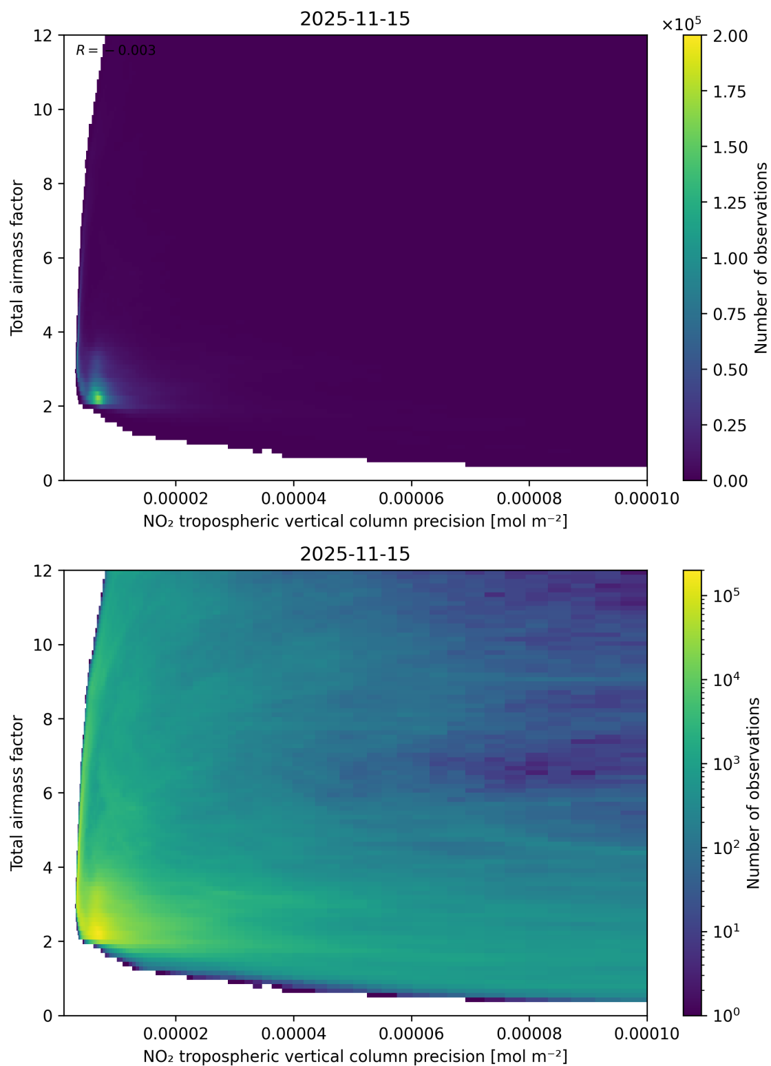
Figure 132: Scatter density plot of “NO 2 tropospheric vertical column precision” against “Total air mass factor” for 2025-11-14 to 2025-11-16.
