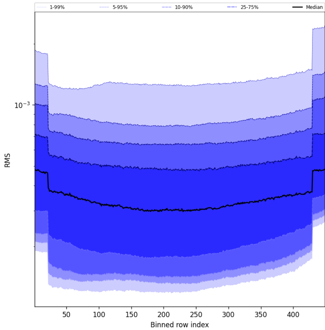
Figure 60: Along track statistics of “RMS” for 2025-11-14 to 2025-11-16
