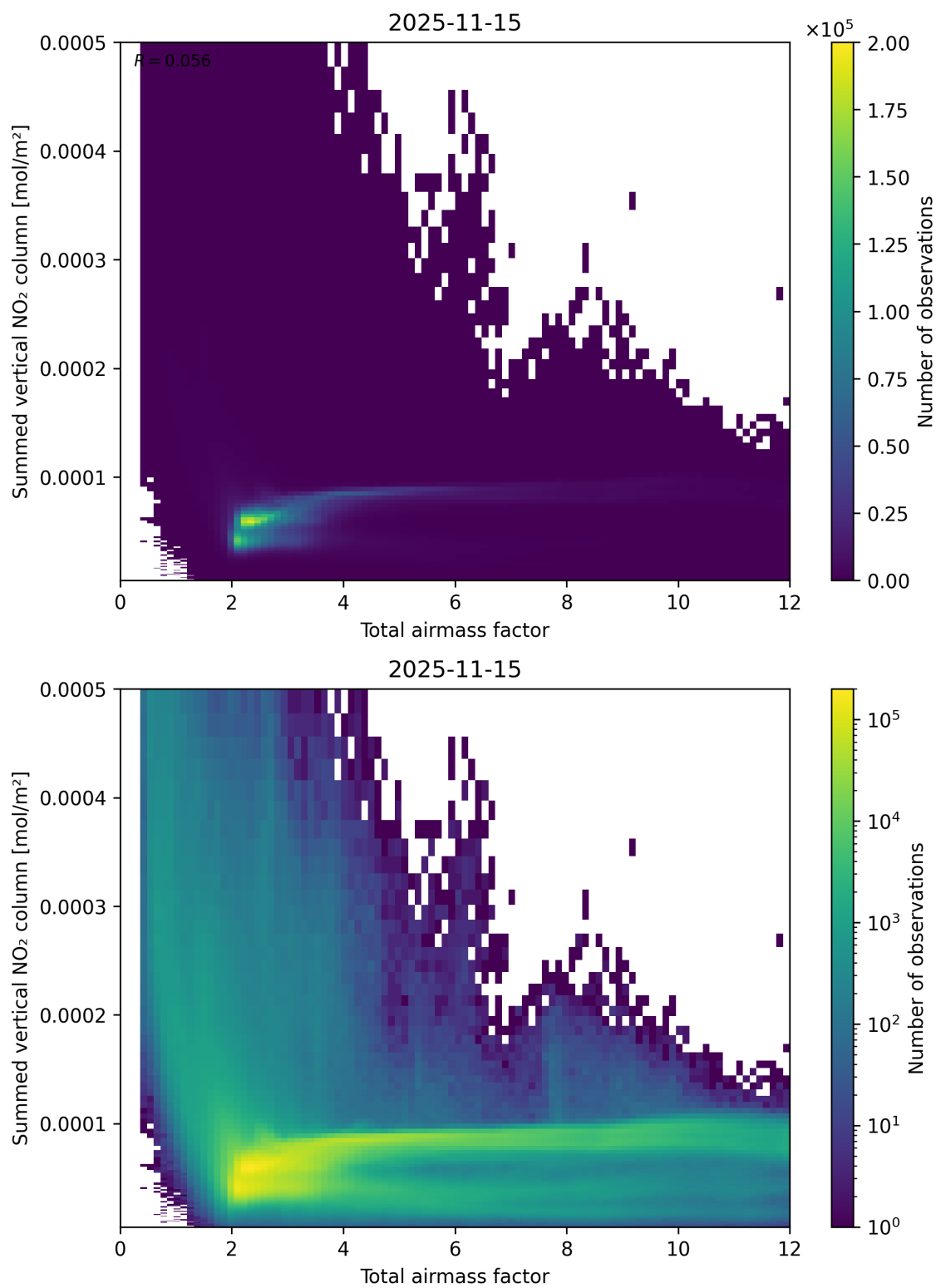
Figure 65: Scatter density plot of “Total airmass factor” against “Summed vertical NO 2 column” for 2025-11-14 to 2025-11-16.
