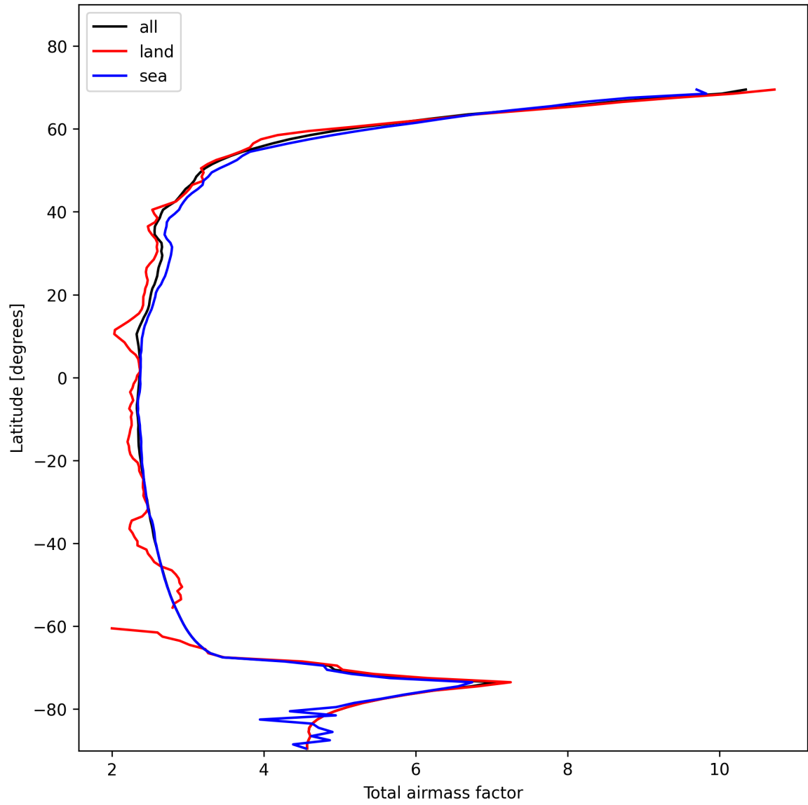
Figure 15: Zonal average of “Total airmass factor” for 2025-11-14 to 2025-11-16.
