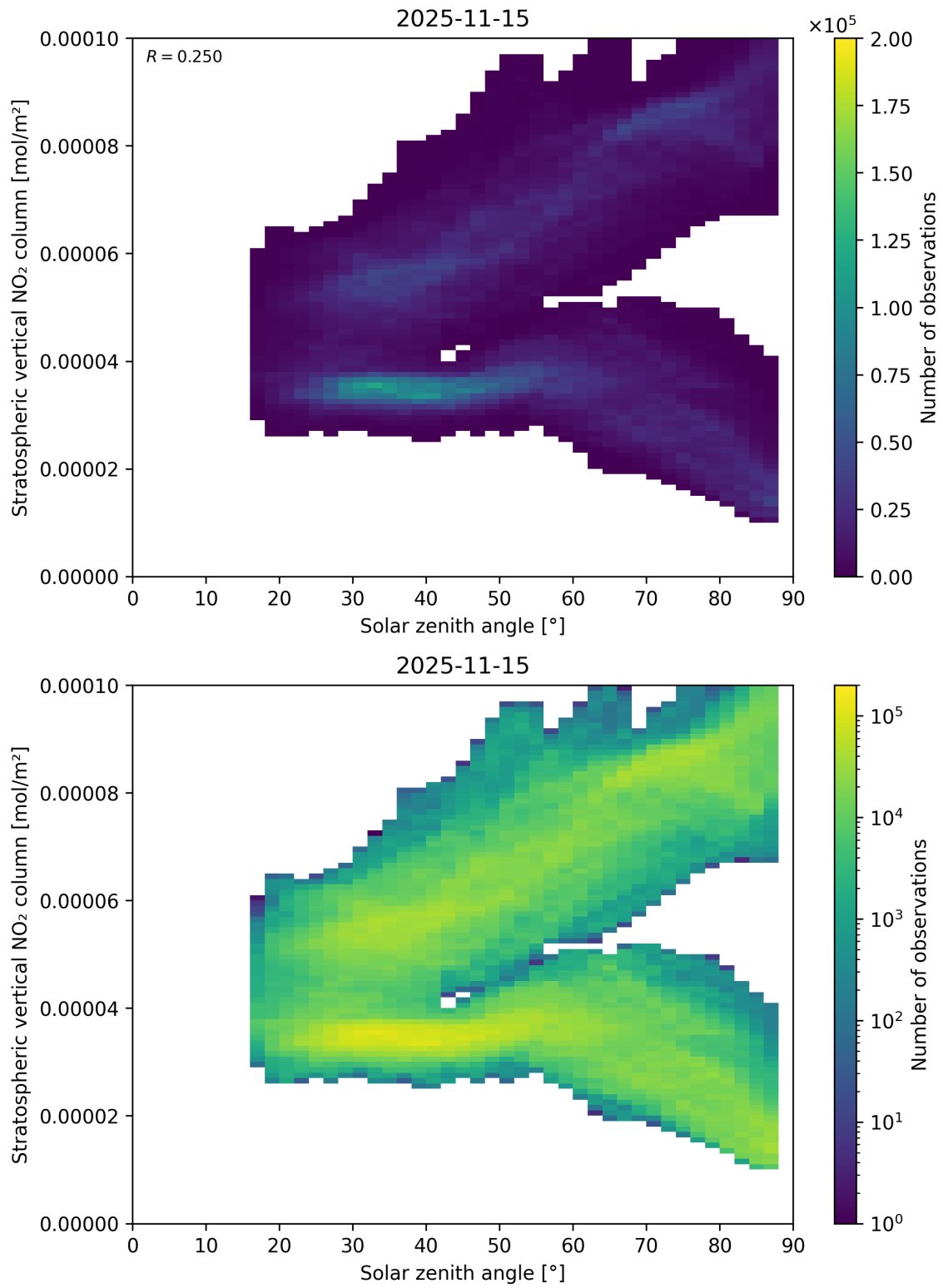
Figure 150: Scatter density plot of “Solar zenith angle” against “Stratospheric vertical NO 2 column” for 2025-11-14 to 2025-11-16.
