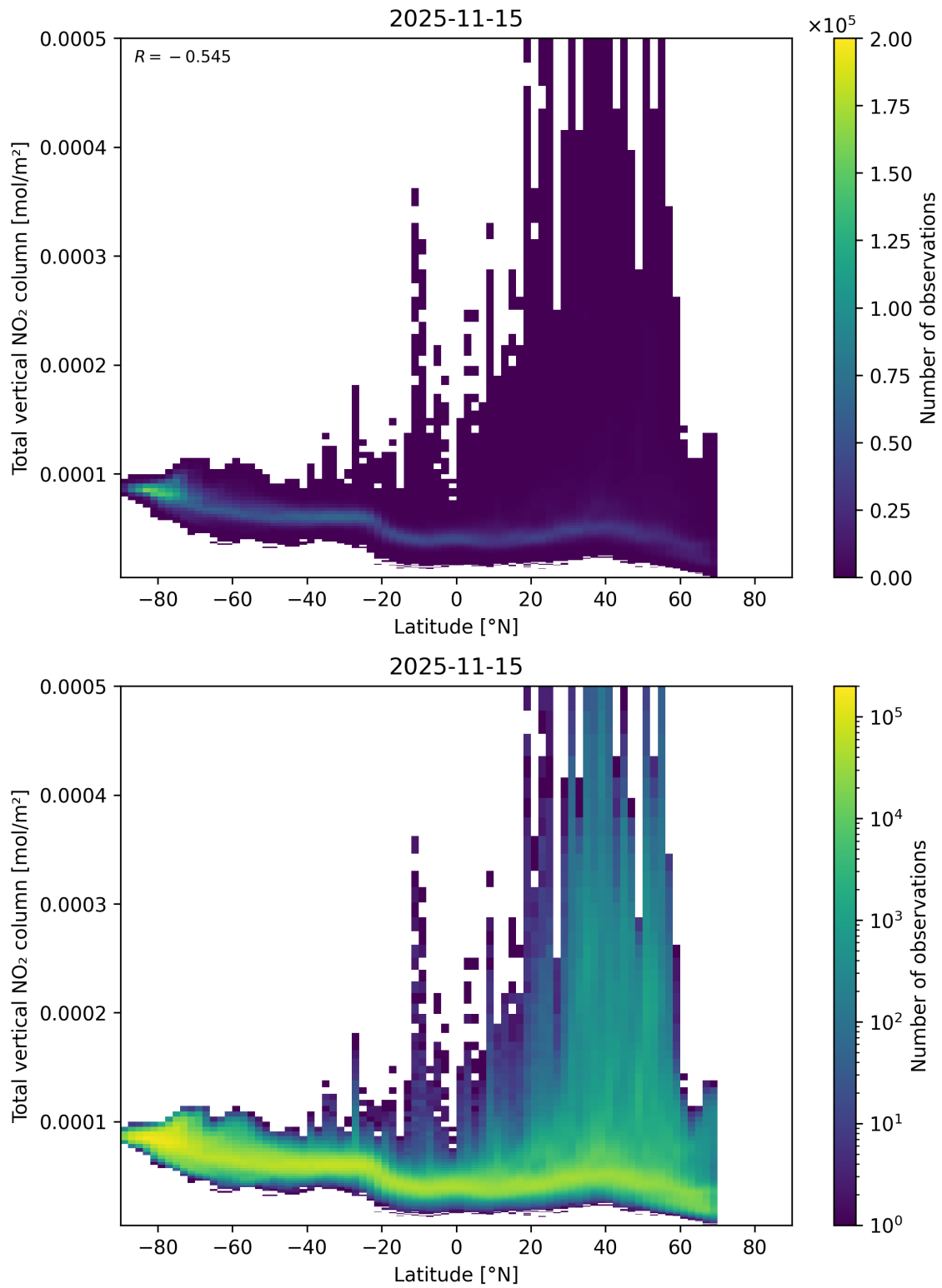
Figure 90: Scatter density plot of “Latitude” against “Total vertical NO 2 column” for 2025-11-14 to 2025-11-16.
