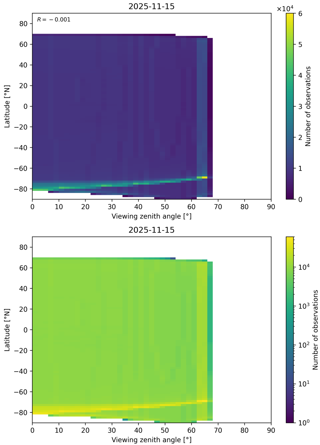
Figure 163: Scatter density plot of “Viewing zenith angle” against “Latitude” for 2025-11-14 to 2025-11-16.
