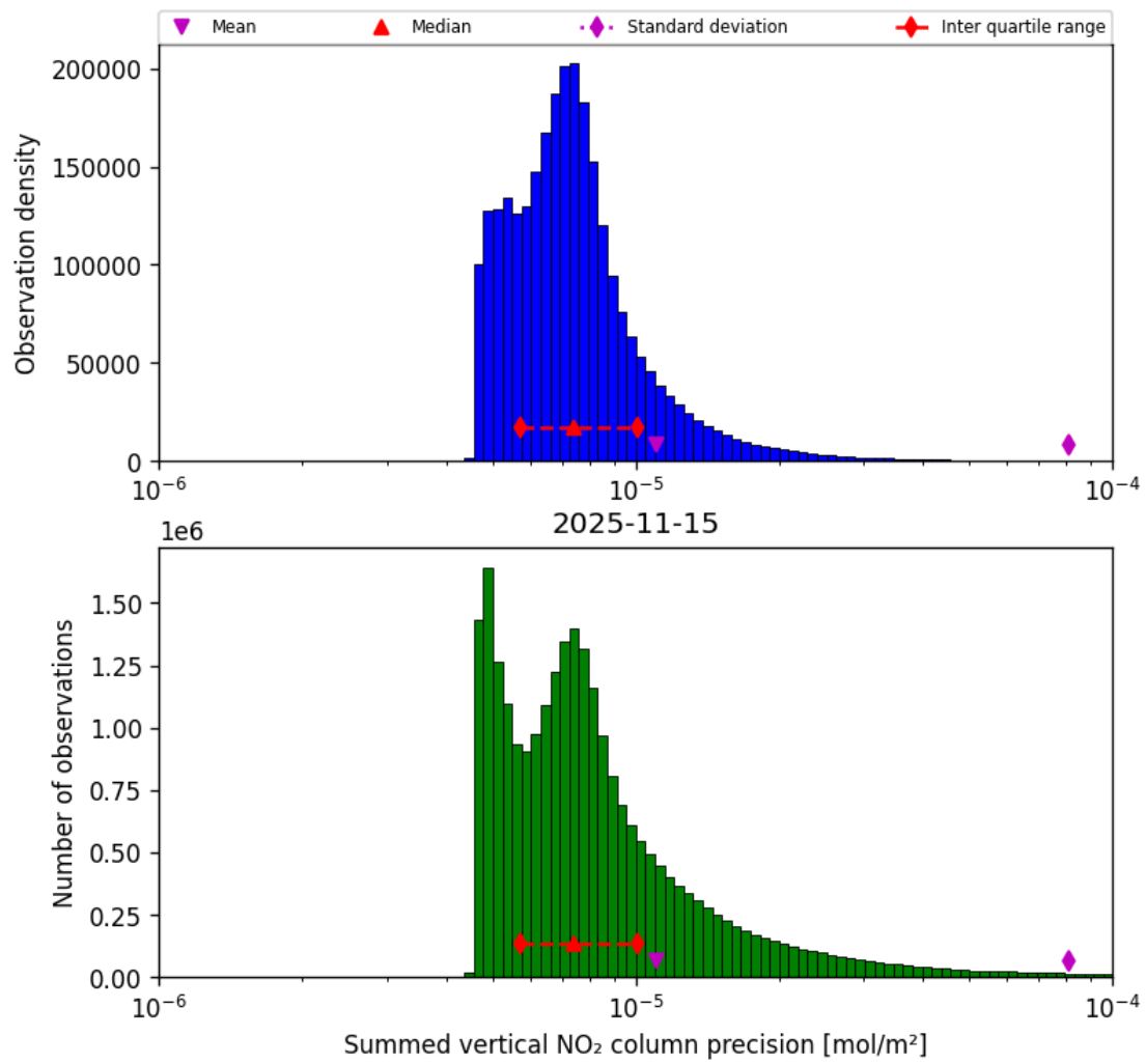
Figure 41: Histogram of "Summed vertical NO 2 column precision" for 2025-11-14 to 2025-11-16
