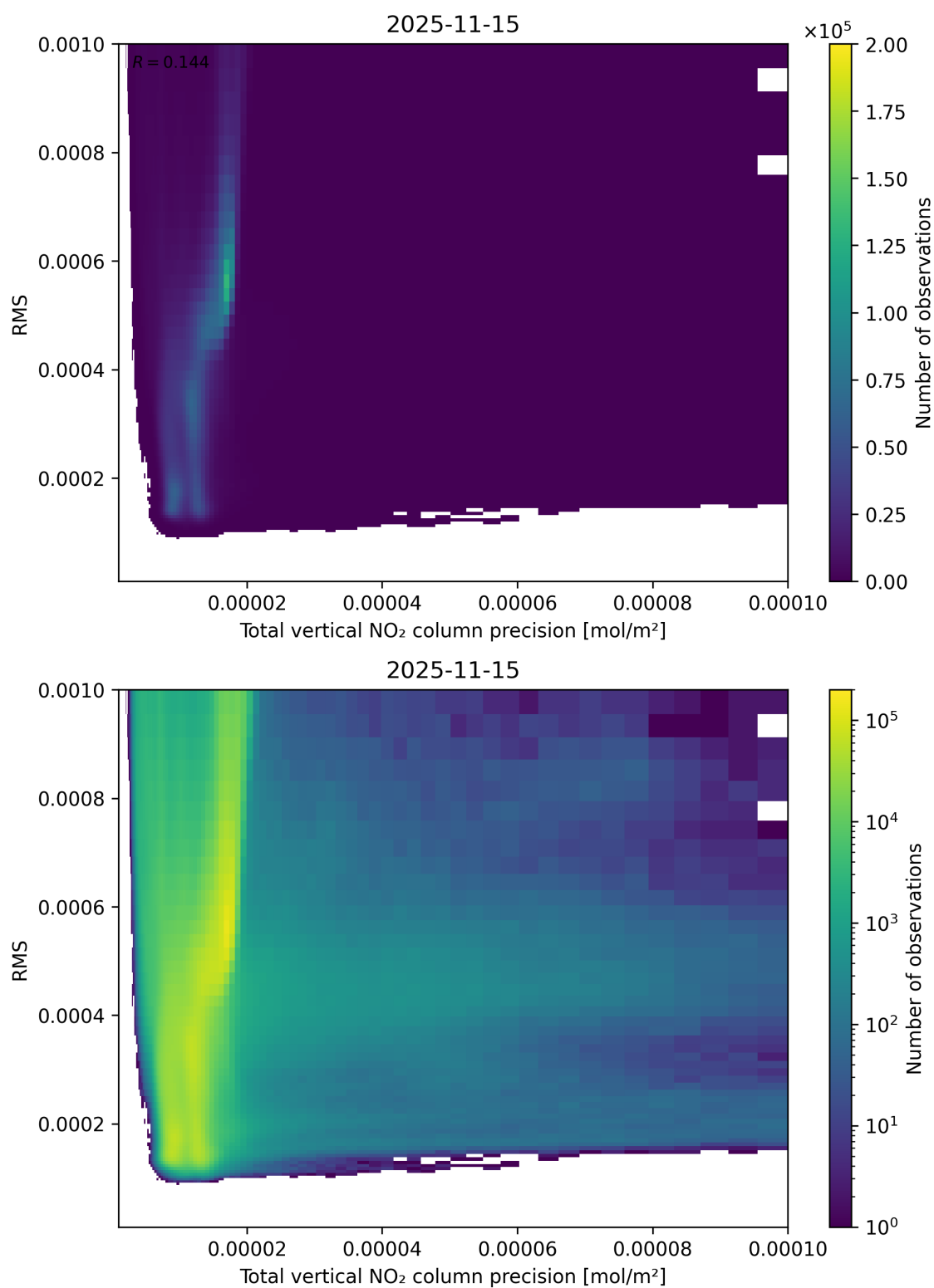
Figure 119: Scatter density plot of “Total vertical NO 2 column precision” against “RMS” for 2025-11-14 to 2025-11-16.
