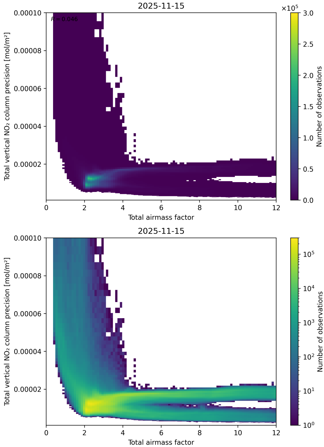
Figure 68: Scatter density plot of “Total airmass factor” against “Total vertical NO 2 column precision” for 2025-11-14 to 2025-11-16.
