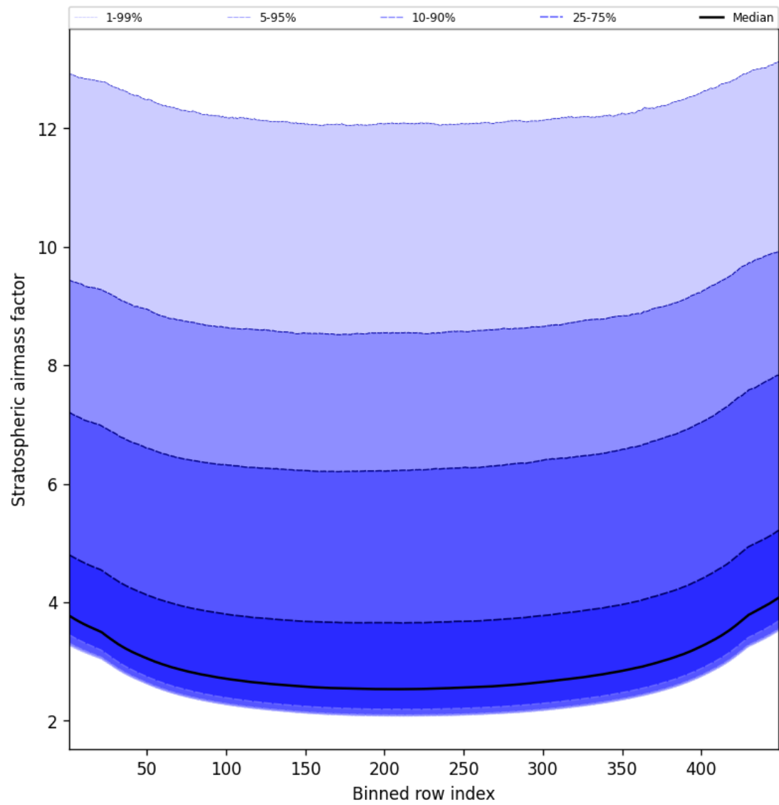
Figure 61: Along track statistics of “Stratospheric air mass factor” for 2025-11-14 to 2025-11-16
