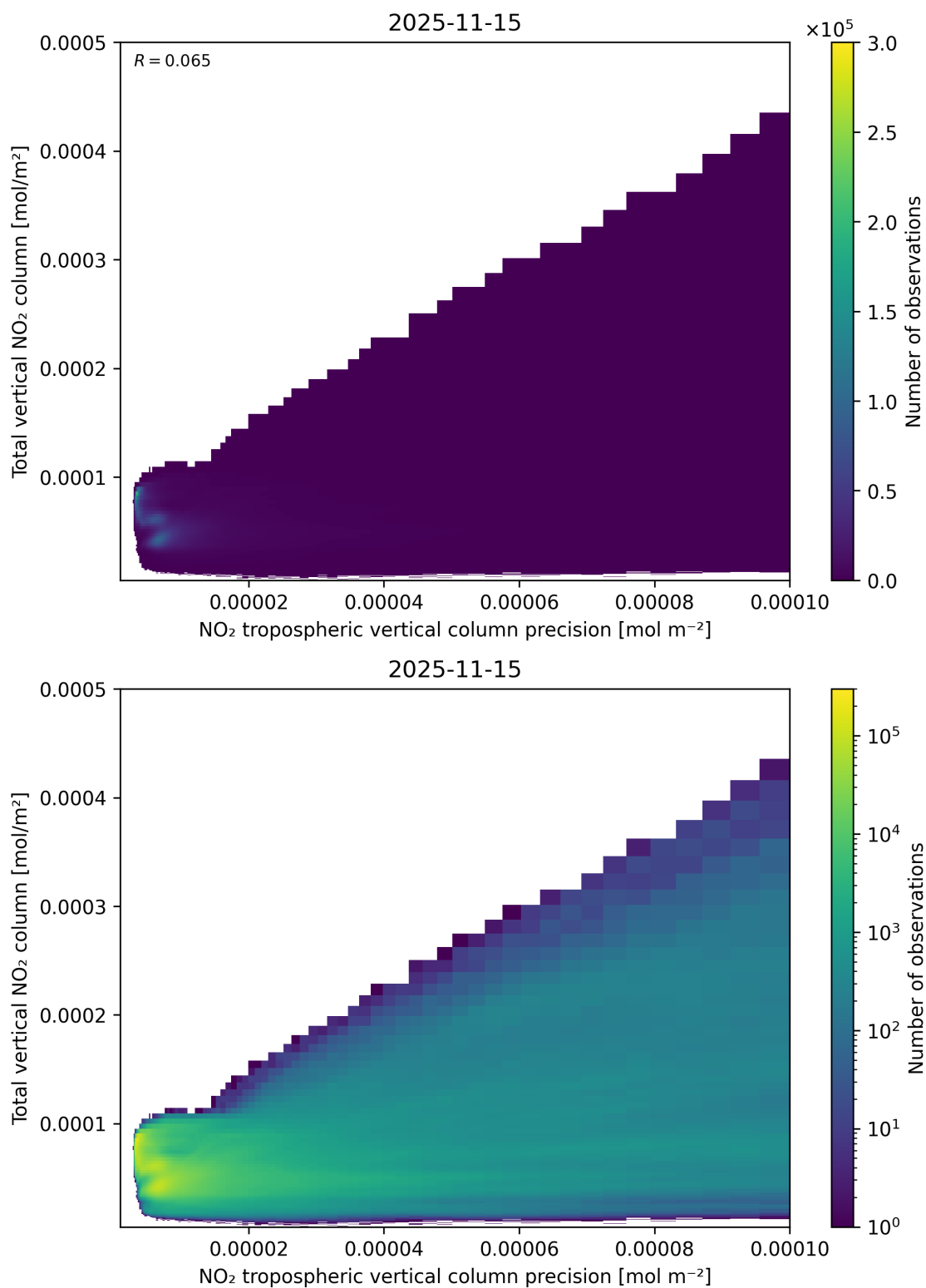
Figure 138: Scatter density plot of “NO 2 tropospheric vertical column precision” against “Total vertical NO 2 column” for 2025-11-14 to 2025-11-16.
