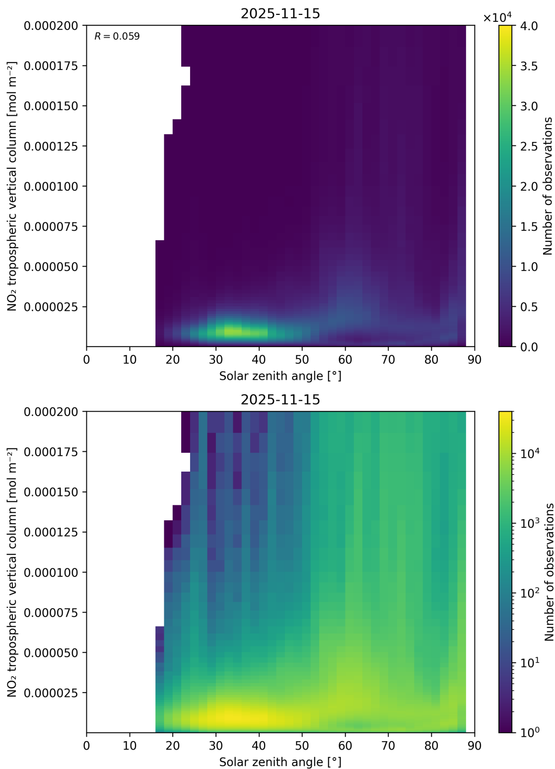
Figure 155: Scatter density plot of “Solar zenith angle” against “NO 2 tropospheric vertical column” for 2025-11-14 to 2025-11-16.
