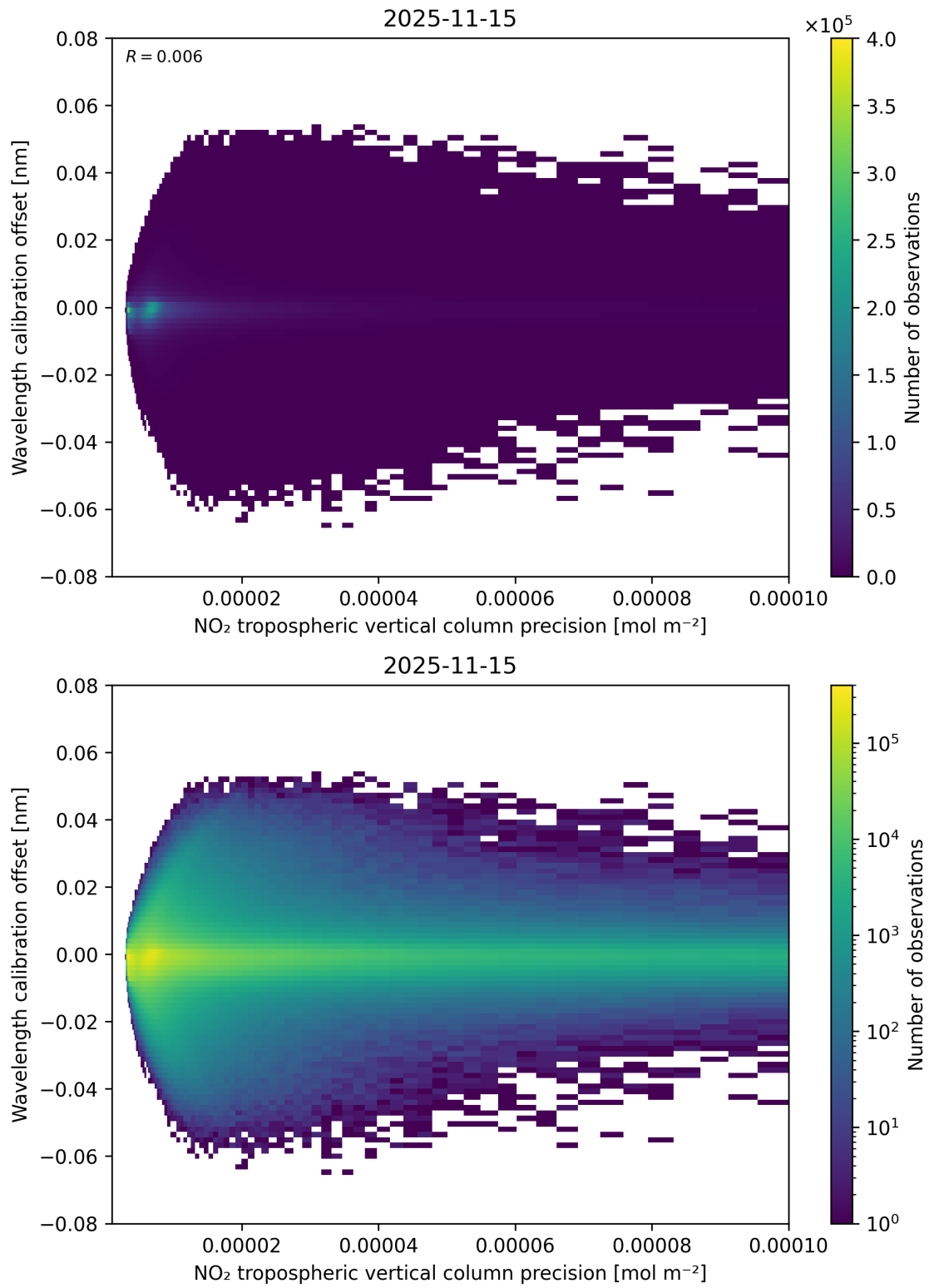
Figure 141: Scatter density plot of “NO 2 tropospheric vertical column precision” against “Wavelength calibration offset” for 2025-11-14 to 2025-11-16.
