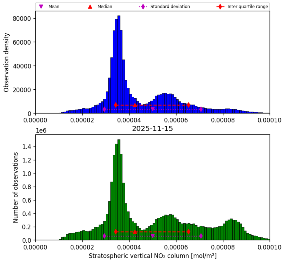
Figure 36: Histogram of “Stratospheric vertical NO 2 column” for 2025-11-14 to 2025-11-16
