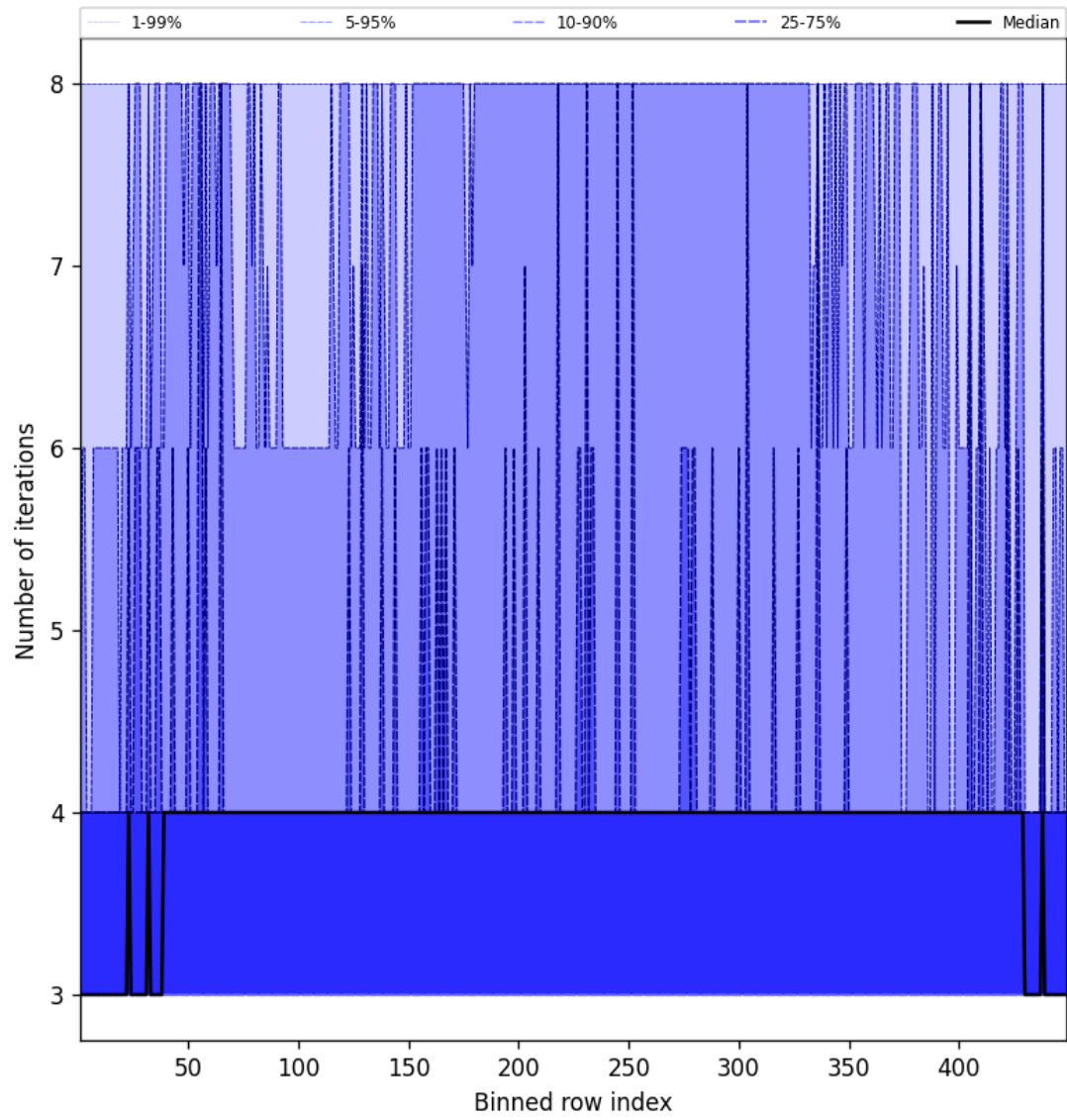
Figure 51: Along track statistics of “Number of iterations” for 2025-11-14 to 2025-11-16
