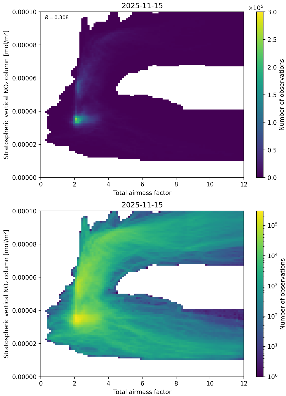
Figure 64: Scatter density plot of “Total airmass factor” against “Stratospheric vertical \text{NO}_2 column” for 2025-11-14 to 2025-11-16.
