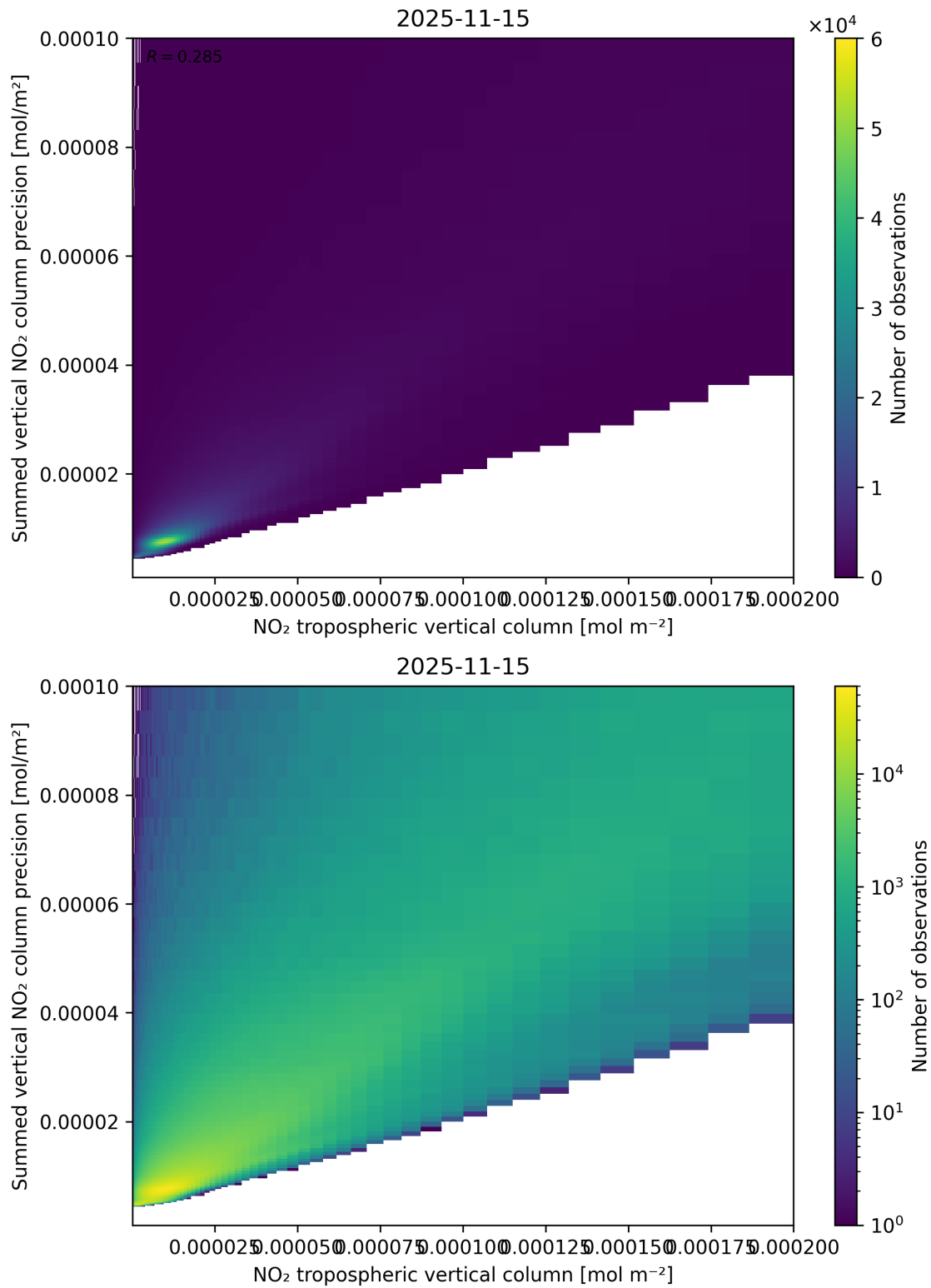
Figure 127: Scatter density plot of “NO 2 tropospheric vertical column” against “Summed vertical NO 2 column precision” for 2025-11-14 to 2025-11-16.
