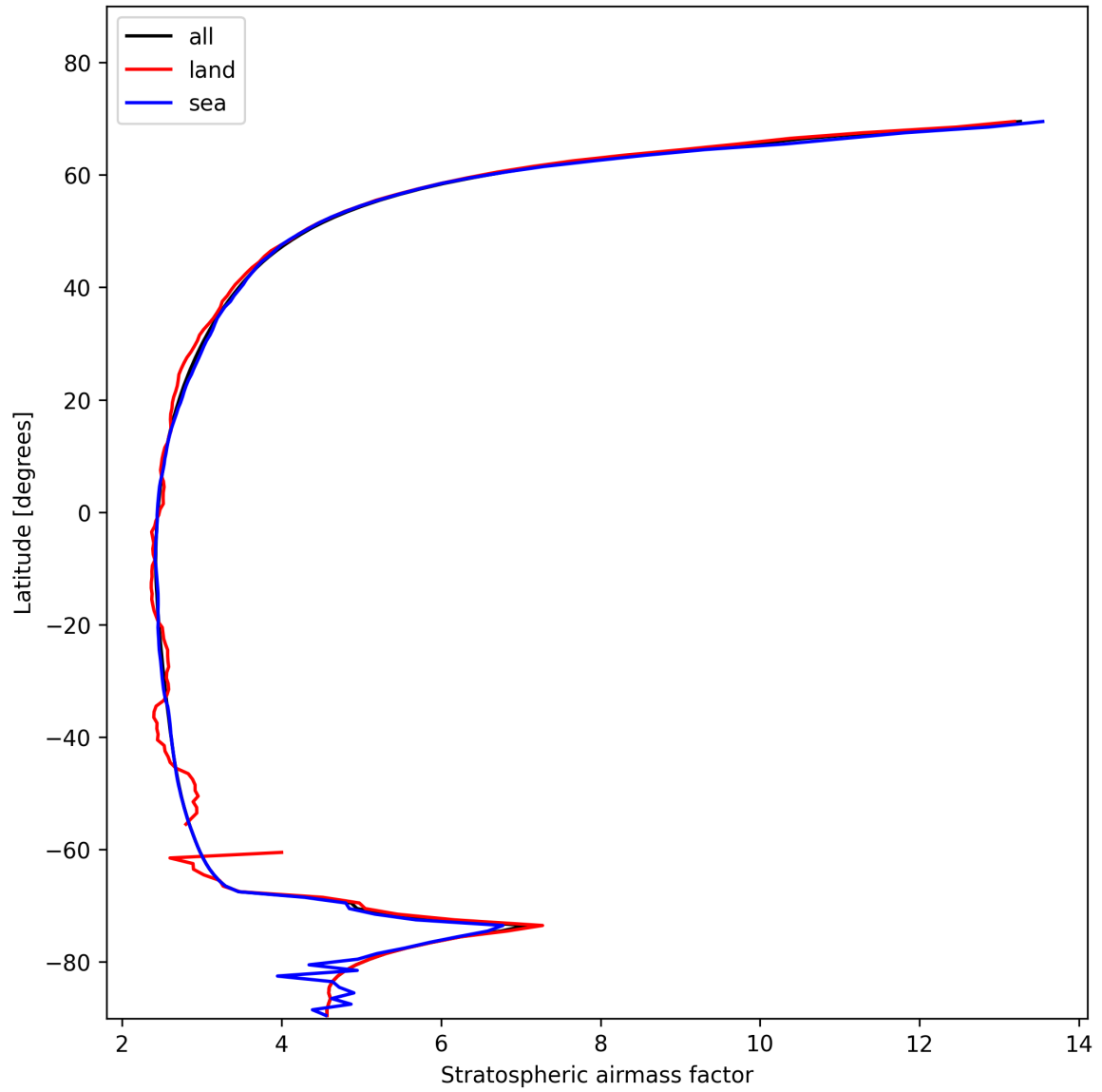
Figure 27: Zonal average of “Stratospheric air mass factor” for 2025-11-14 to 2025-11-16.
