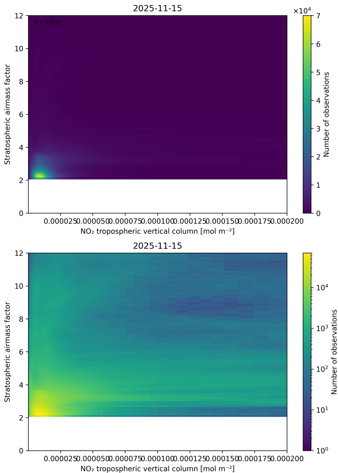
Figure 121: Scatter density plot of “NO 2 tropospheric vertical column” against “Stratospheric airmass factor” for 2025-11-14 to 2025-11-16.
