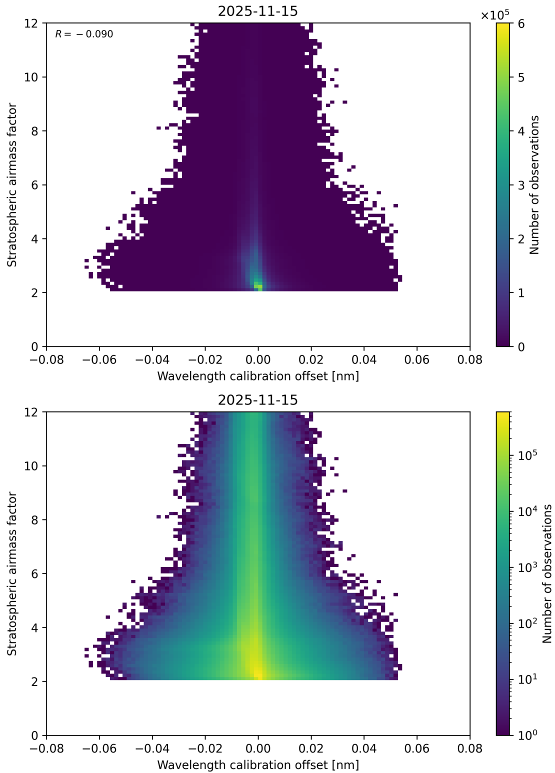
Figure 174: Scatter density plot of “Wavelength calibration offset” against “Stratospheric airmass factor” for 2025-11-14 to 2025-11-16.
