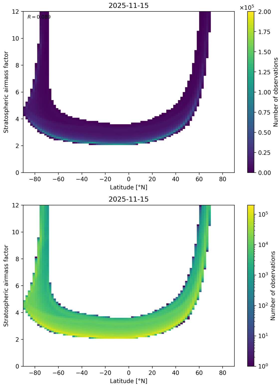
Figure 83: Scatter density plot of “Latitude” against “Stratospheric air mass factor” for 2025-11-14 to 2025-11-16.
