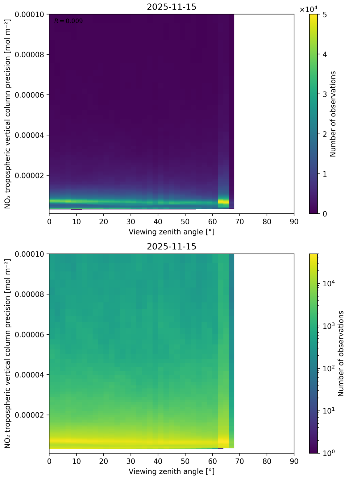
Figure 170: Scatter density plot of “Viewing zenith angle” against “NO 2 tropospheric vertical column precision” for 2025-11-14 to 2025-11-16.
