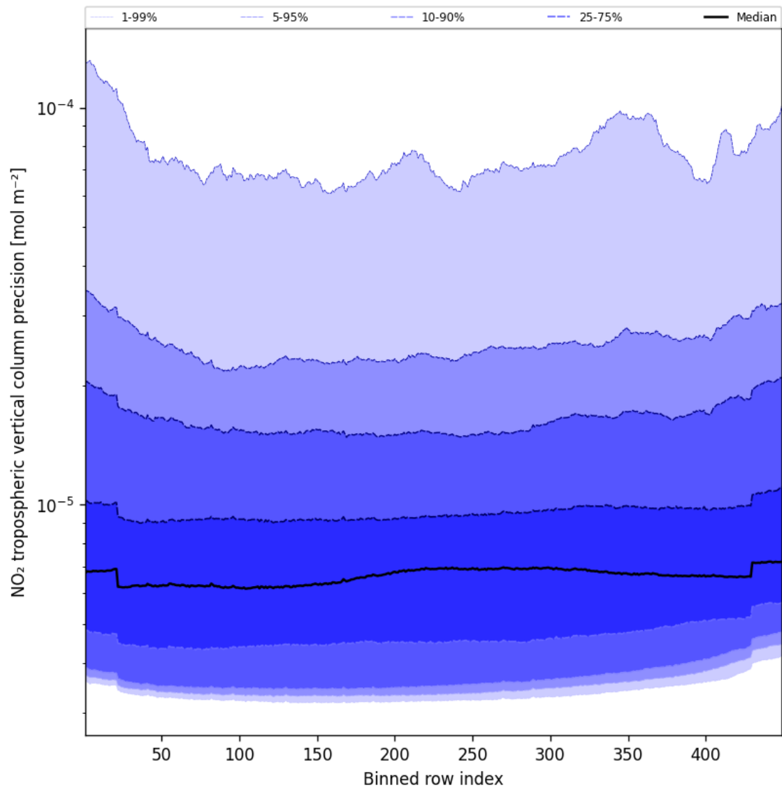
Figure 47: Along track statistics of “NO 2 tropospheric vertical column precision” for 2025-11-14 to 2025-11-16
