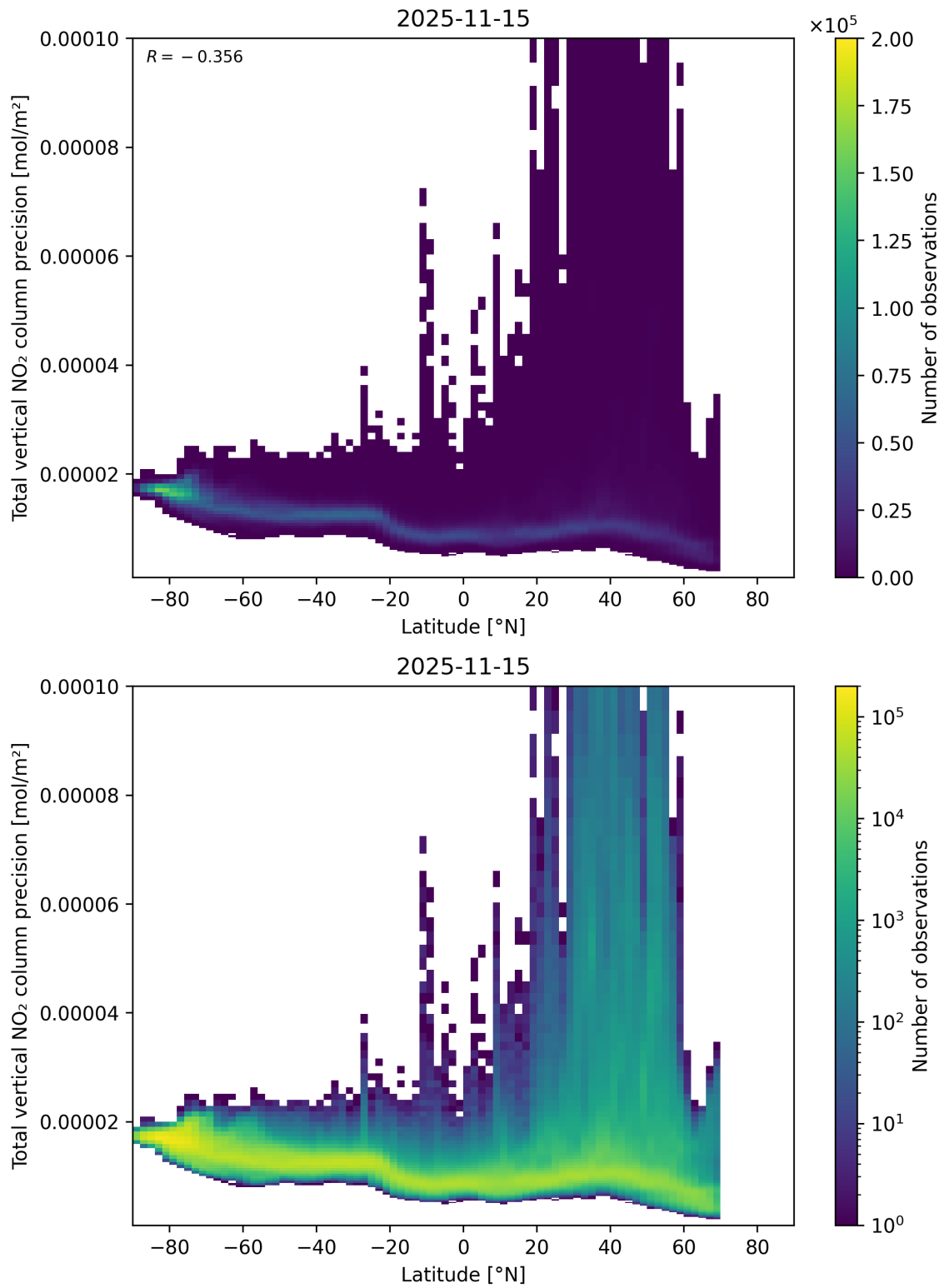
Figure 91: Scatter density plot of “Latitude” against “Total vertical NO 2 column precision” for 2025-11-14 to 2025-11-16.
