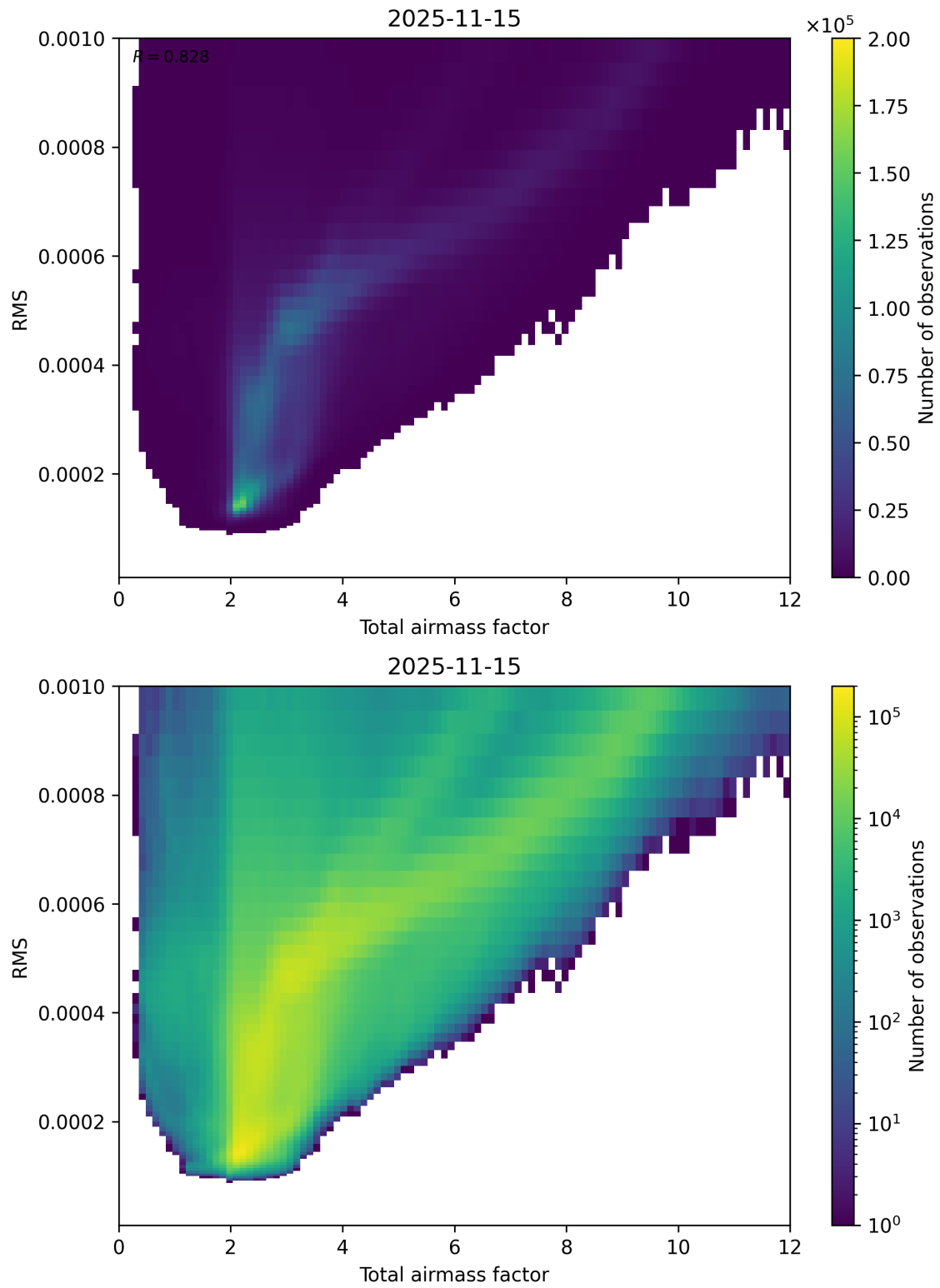
Figure 69: Scatter density plot of “Total airmass factor” against “RMS” for 2025-11-14 to 2025-11-16.
