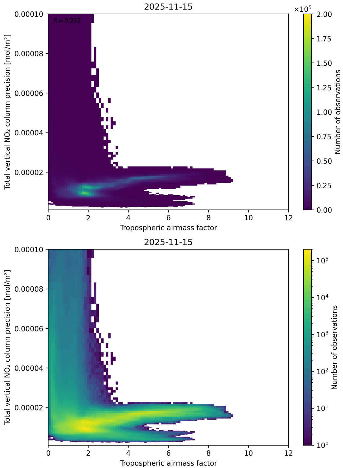
Figure 78: Scatter density plot of “Tropospheric air mass factor” against “Total vertical NO 2 column precision” for 2025-11-14 to 2025-11-16.
