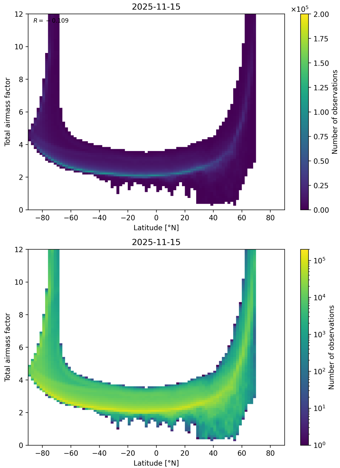
Figure 84: Scatter density plot of “Latitude” against “Total airmass factor” for 2025-11-14 to 2025-11-16.
