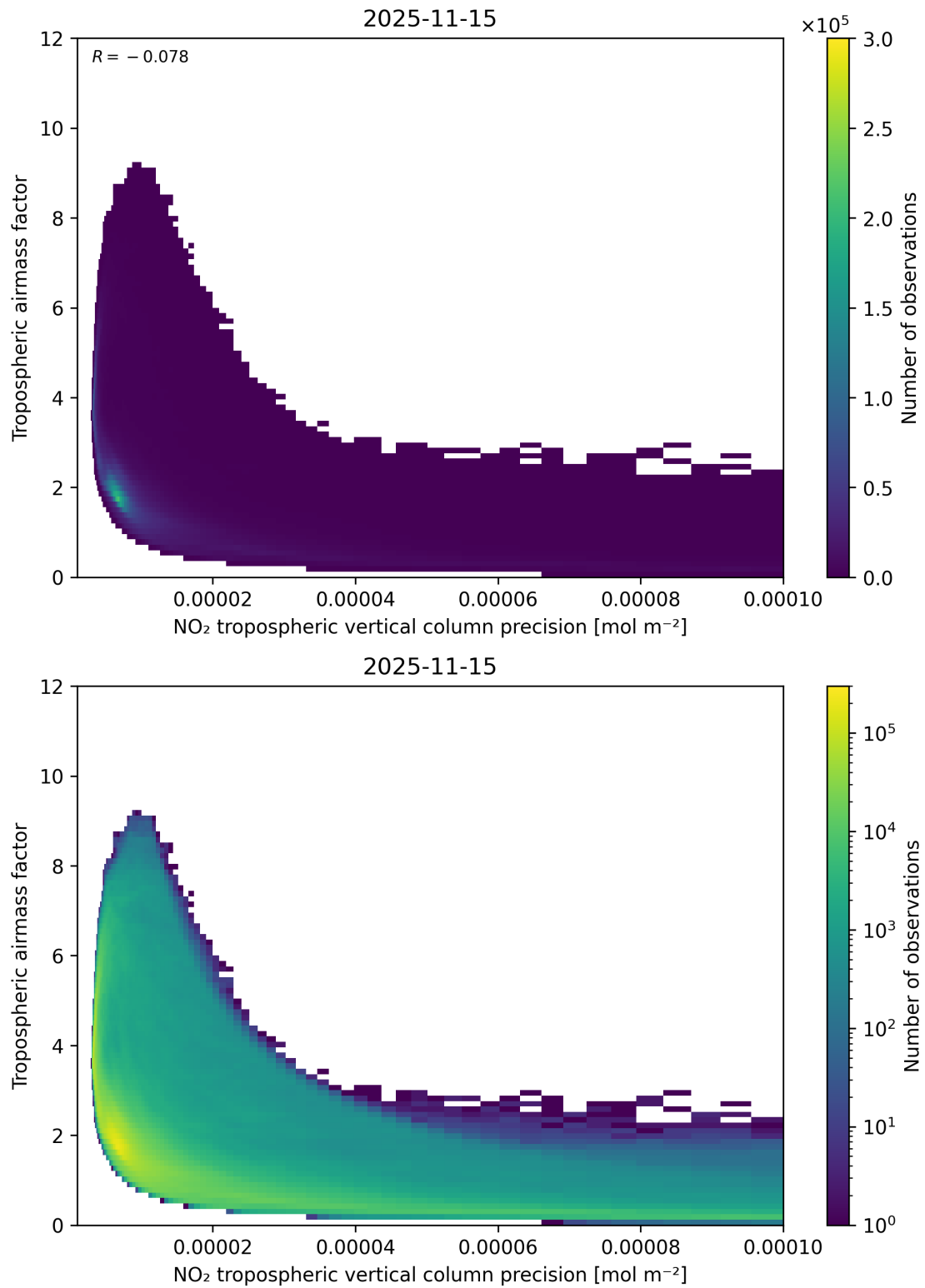
Figure 133: Scatter density plot of “NO 2 tropospheric vertical column precision” against “Tropospheric air mass factor” for 2025-11-14 to 2025-11-16.
