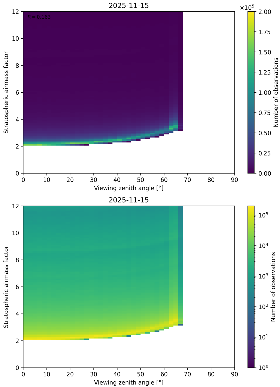
Figure 159: Scatter density plot of “Viewing zenith angle” against “Stratospheric airmass factor” for 2025-11-14 to 2025-11-16.
