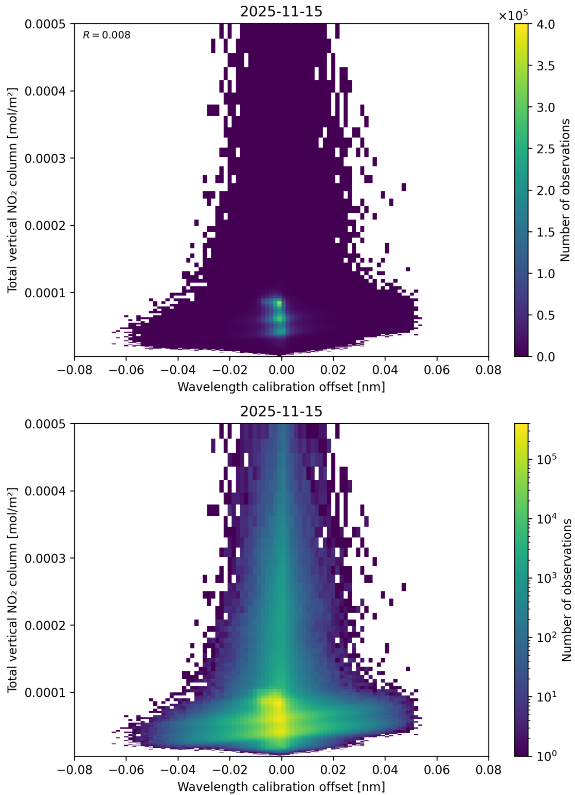
Figure 179: Scatter density plot of “Wavelength calibration offset” against “Total vertical NO 2 column” for 2025-11-14 to 2025-11-16.
