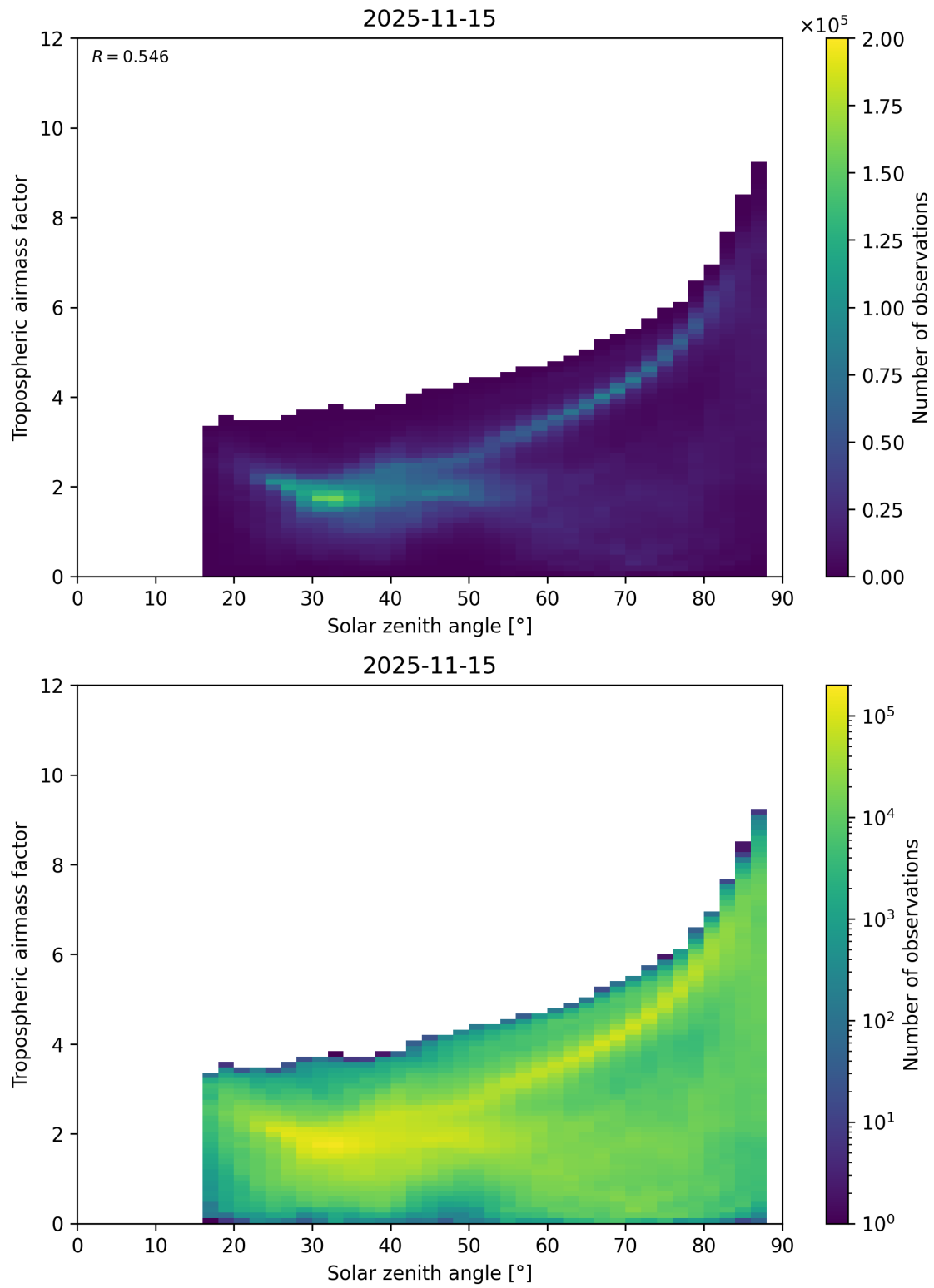
Figure 147: Scatter density plot of “Solar zenith angle” against “Tropospheric airmass factor” for 2025-11-14 to 2025-11-16.
