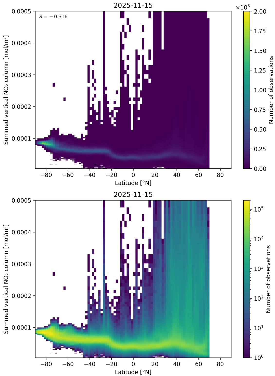
Figure 88: Scatter density plot of “Latitude” against “Summed vertical NO 2 column” for 2025-11-14 to 2025-11-16.
