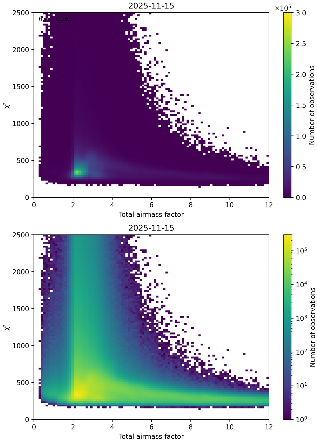
Figure 63: Scatter density plot of “Total airmass factor” against “ \chi^2 ” for 2025-11-14 to 2025-11-16.
