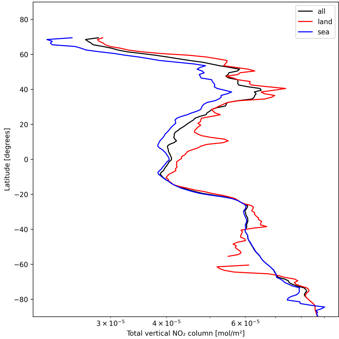
Figure 21: Zonal average of “Total vertical NO 2 column” for 2025-11-14 to 2025-11-16.
