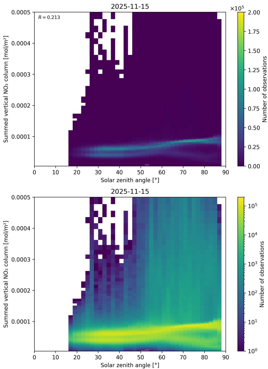
Figure 151: Scatter density plot of “Solar zenith angle” against “Summed vertical NO 2 column” for 2025-11-14 to 2025-11-16.
