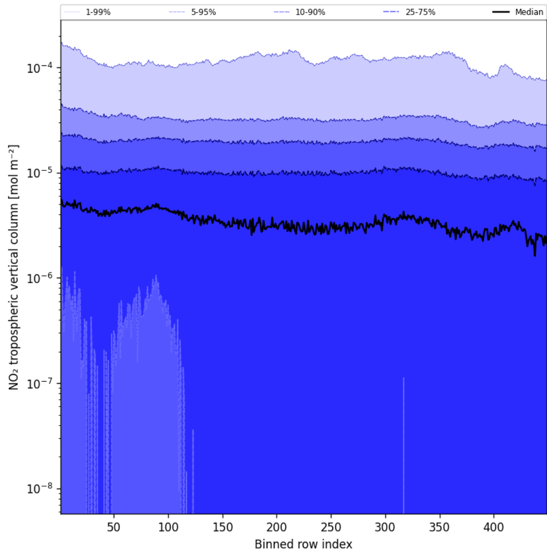
Figure 46: Along track statistics of “NO 2 tropospheric vertical column” for 2025-11-14 to 2025-11-16
