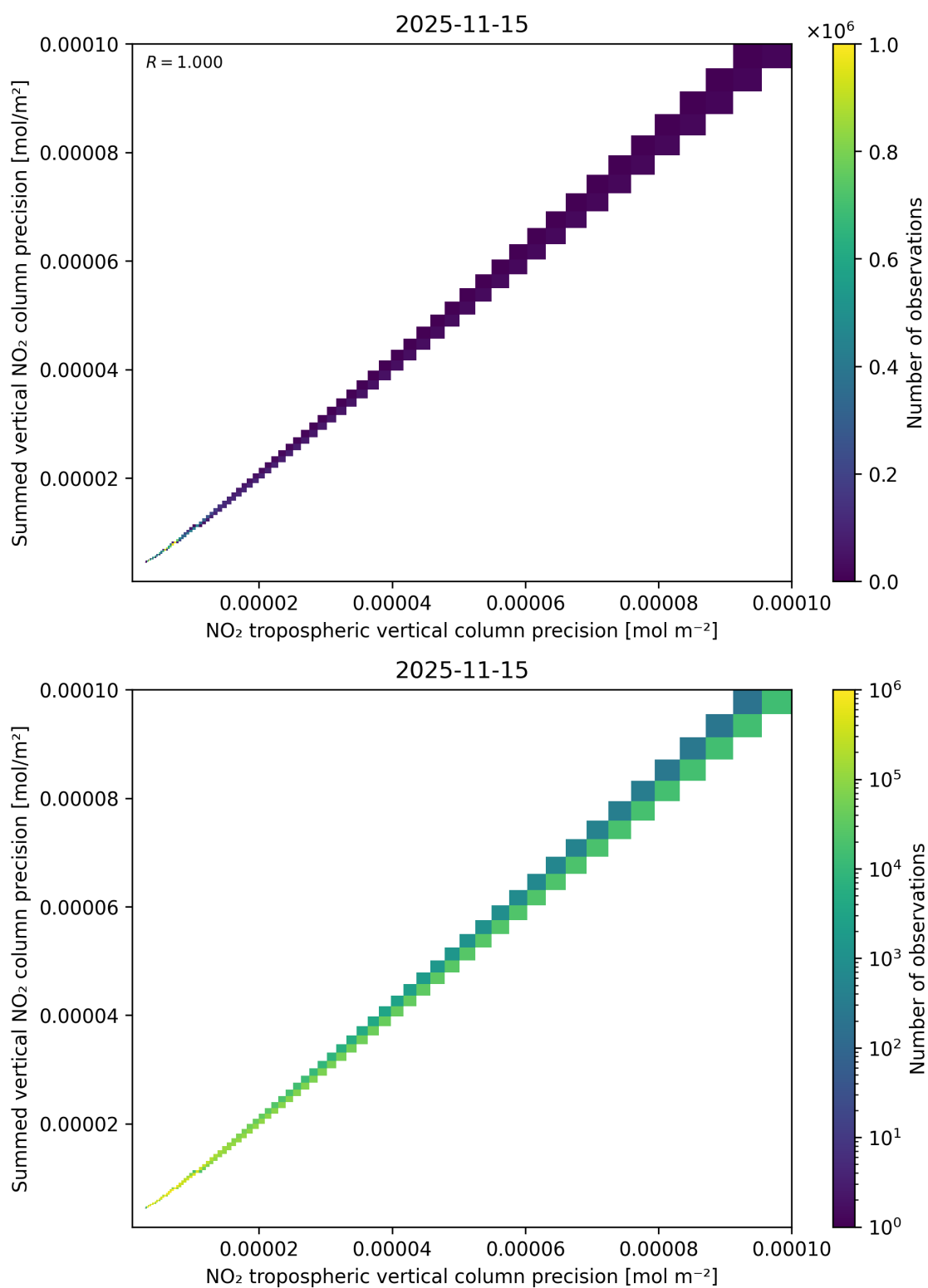
Figure 137: Scatter density plot of “NO 2 tropospheric vertical column precision” against “Summed vertical NO 2 column precision” for 2025-11-14 to 2025-11-16.
