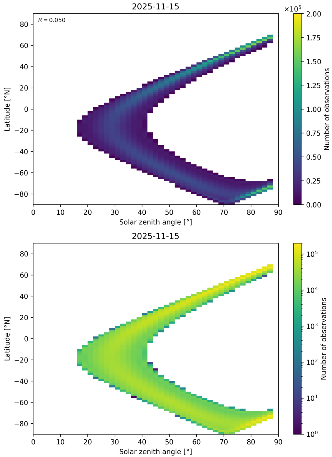
Figure 149: Scatter density plot of “Solar zenith angle” against “Latitude” for 2025-11-14 to 2025-11-16.
