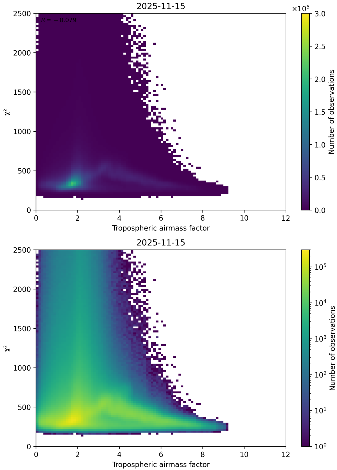
Figure 73: Scatter density plot of “Tropospheric airmass factor” against “ \chi^2 ” for 2025-11-14 to 2025-11-16.
