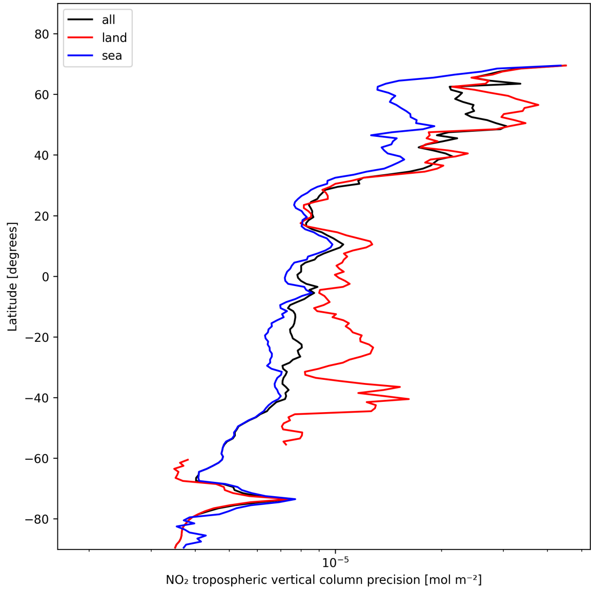
Figure 13: Zonal average of “NO 2 tropospheric vertical column precision” for 2025-11-14 to 2025-11-16.
