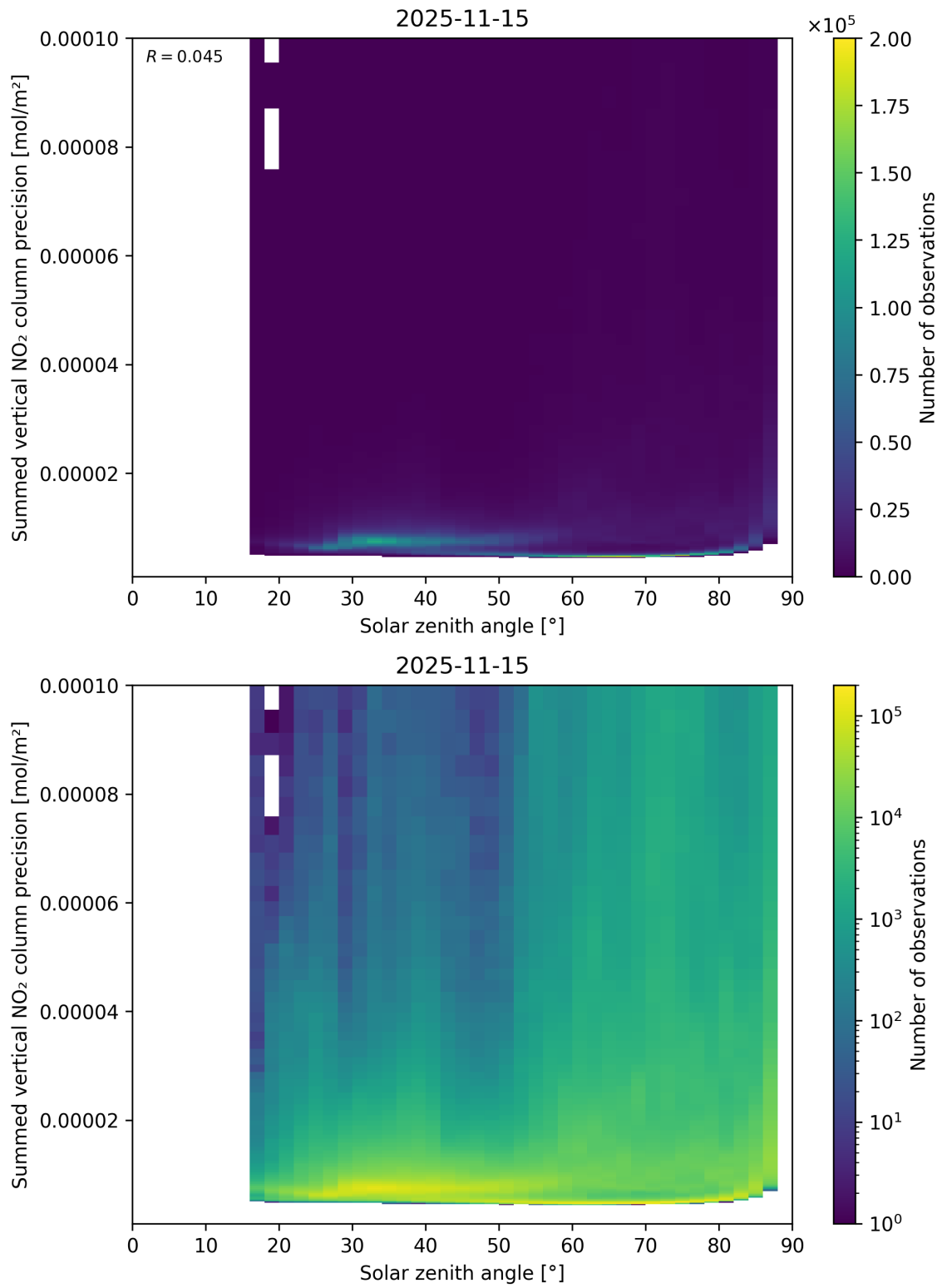
Figure 152: Scatter density plot of “Solar zenith angle” against “Summed vertical NO 2 column precision” for 2025-11-14 to 2025-11-16.
