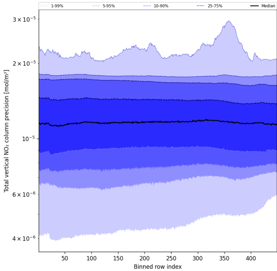
Figure 56: Along track statistics of “Total vertical NO 2 column precision” for 2025-11-14 to 2025-11-16
