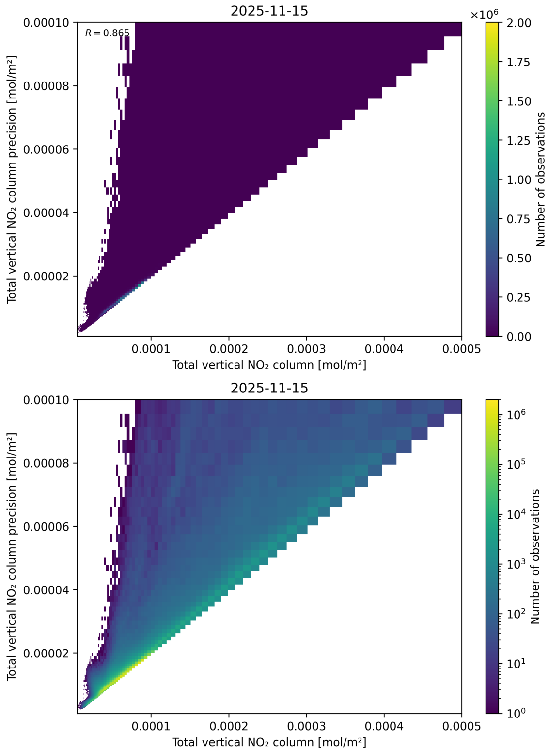
Figure 114: Scatter density plot of “Total vertical NO 2 column” against “Total vertical NO 2 column precision” for 2025-11-14 to 2025-11-16.
