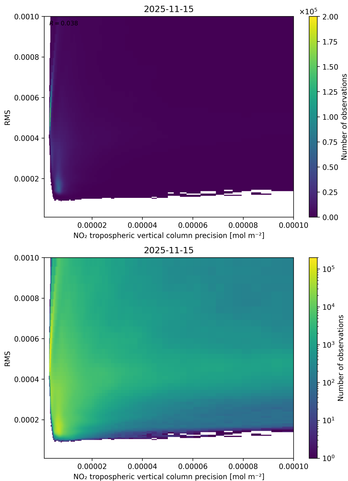
Figure 140: Scatter density plot of “NO 2 tropospheric vertical column precision” against “RMS” for 2025-11-14 to 2025-11-16.
