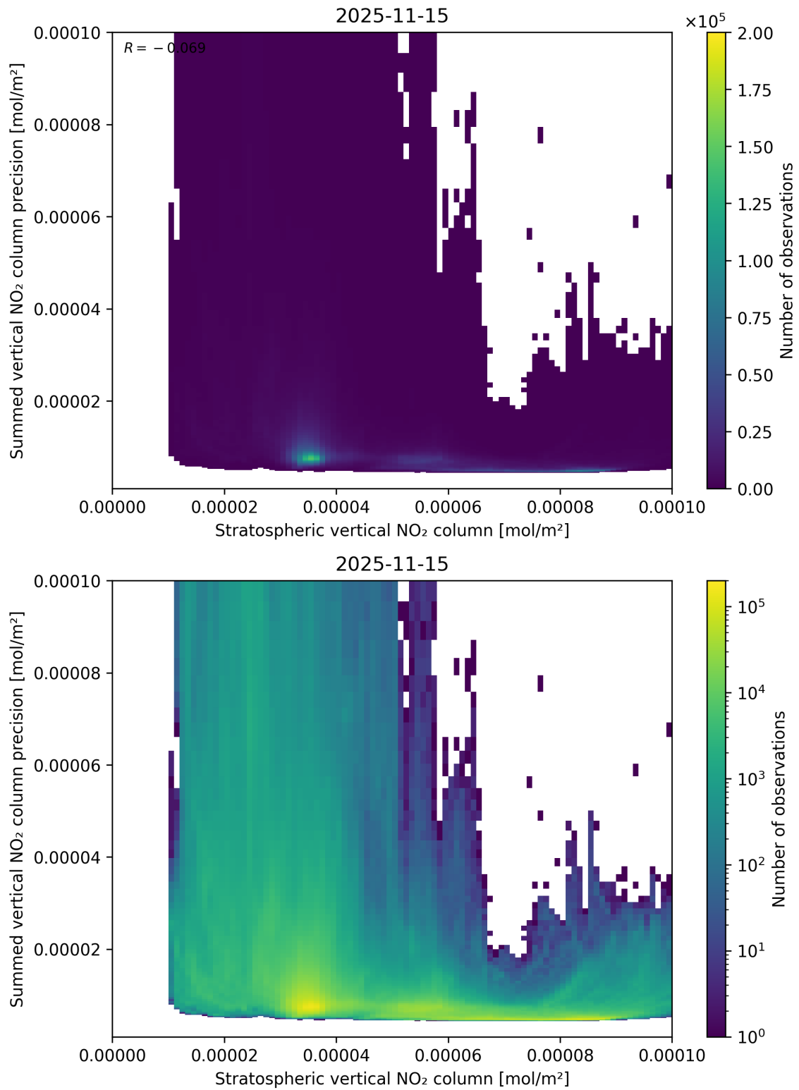
Figure 99: Scatter density plot of “Stratospheric vertical NO 2 column” against “Summed vertical NO 2 column precision” for 2025-11-14 to 2025-11-16.
