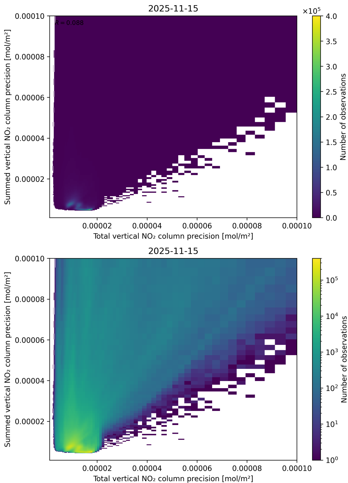
Figure 118: Scatter density plot of “Total vertical NO 2 column precision” against “Summed vertical NO 2 column precision” for 2025-11-14 to 2025-11-16.
