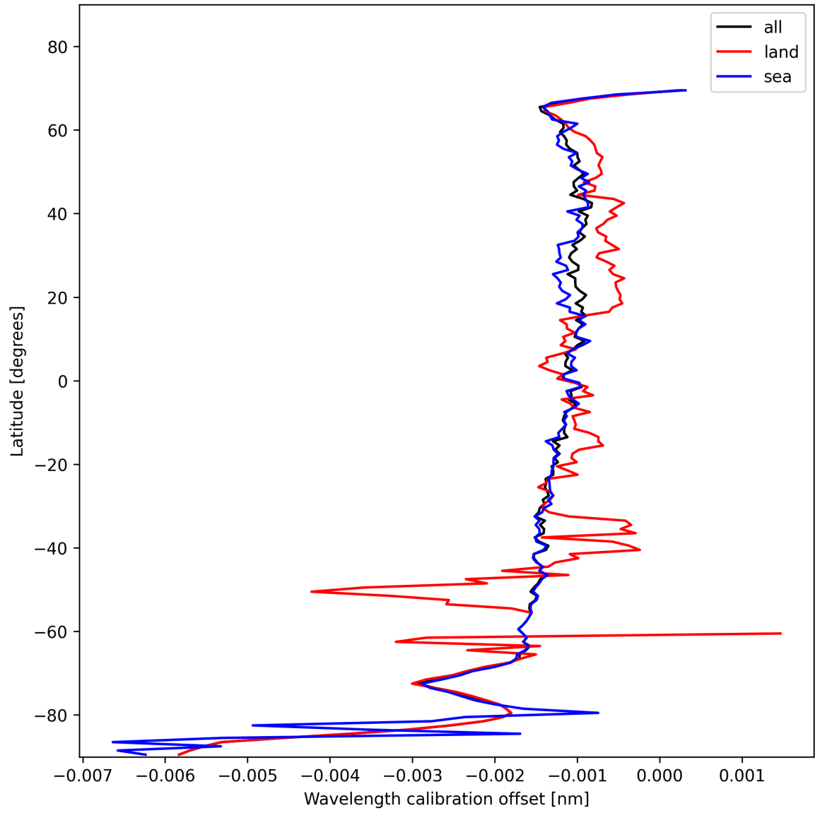
Figure 18: Zonal average of “Wavelength calibration offset” for 2025-11-14 to 2025-11-16.
