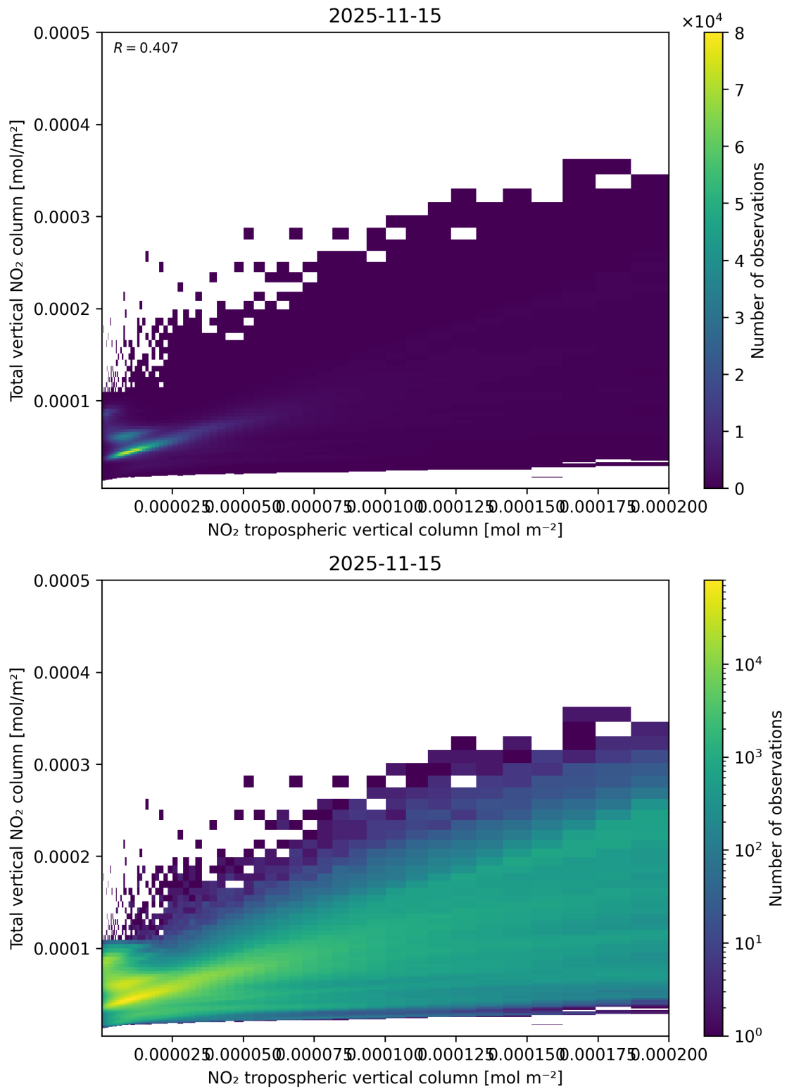
Figure 128: Scatter density plot of “NO 2 tropospheric vertical column” against “Total vertical NO 2 column” for 2025-11-14 to 2025-11-16.
