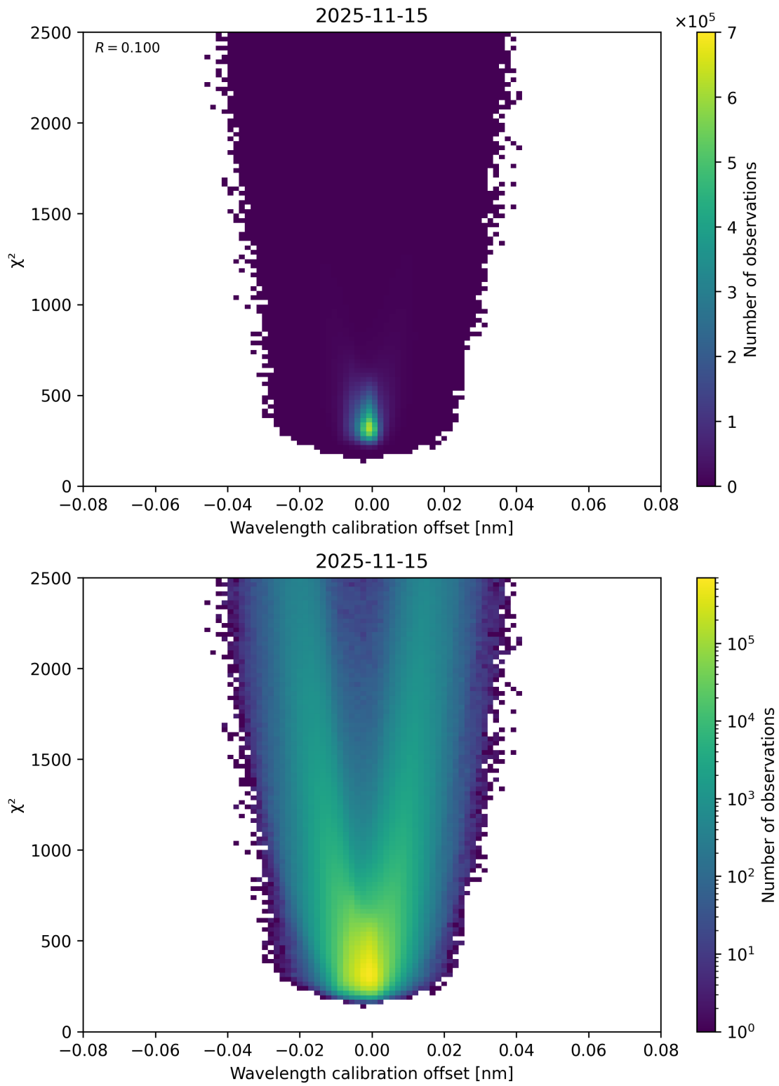
Figure 175: Scatter density plot of “Wavelength calibration offset” against “ \chi^2 ” for 2025-11-14 to 2025-11-16.
