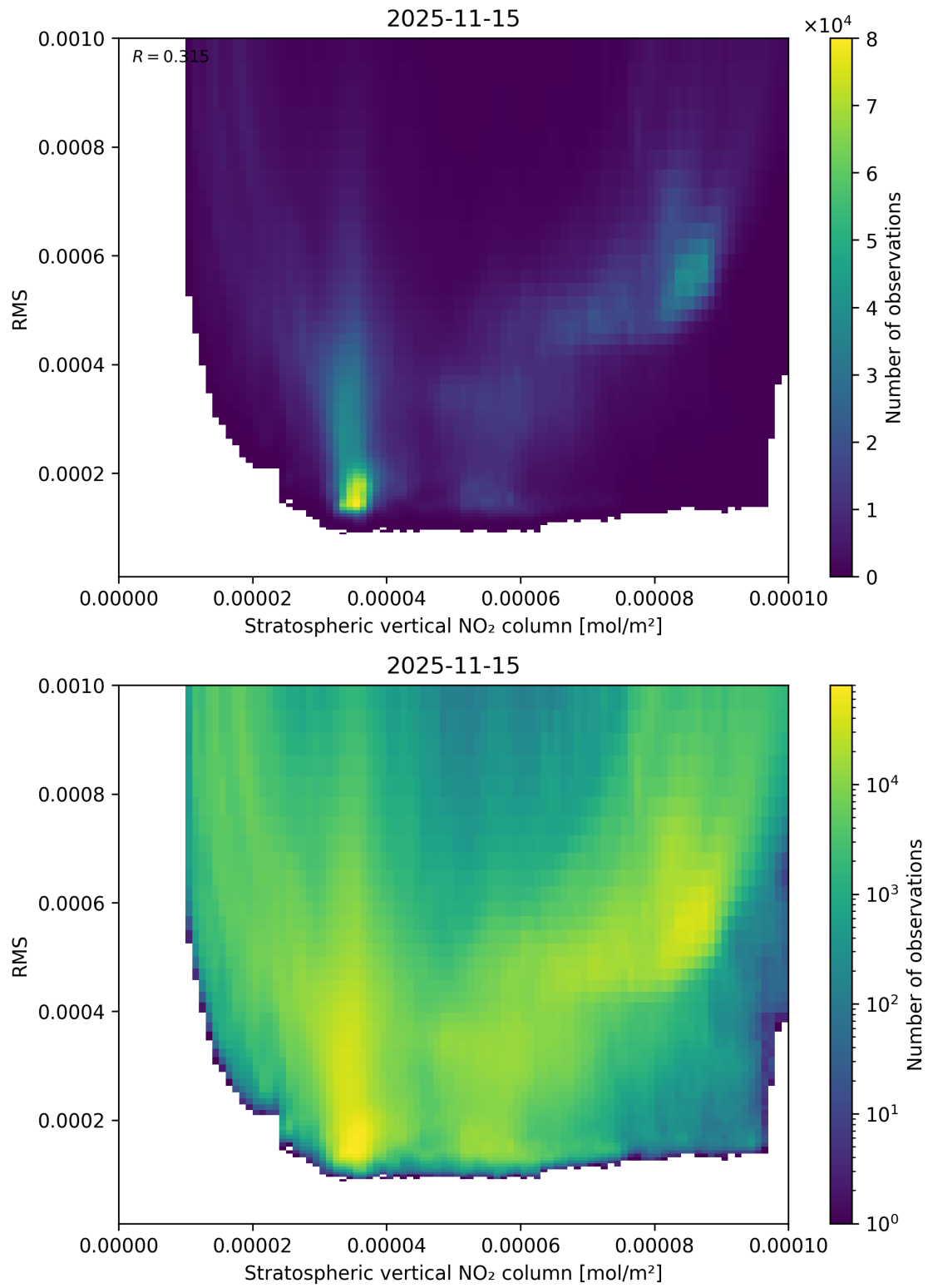
Figure 102: Scatter density plot of “Stratospheric vertical NO 2 column” against “RMS” for 2025-11-14 to 2025-11-16.
