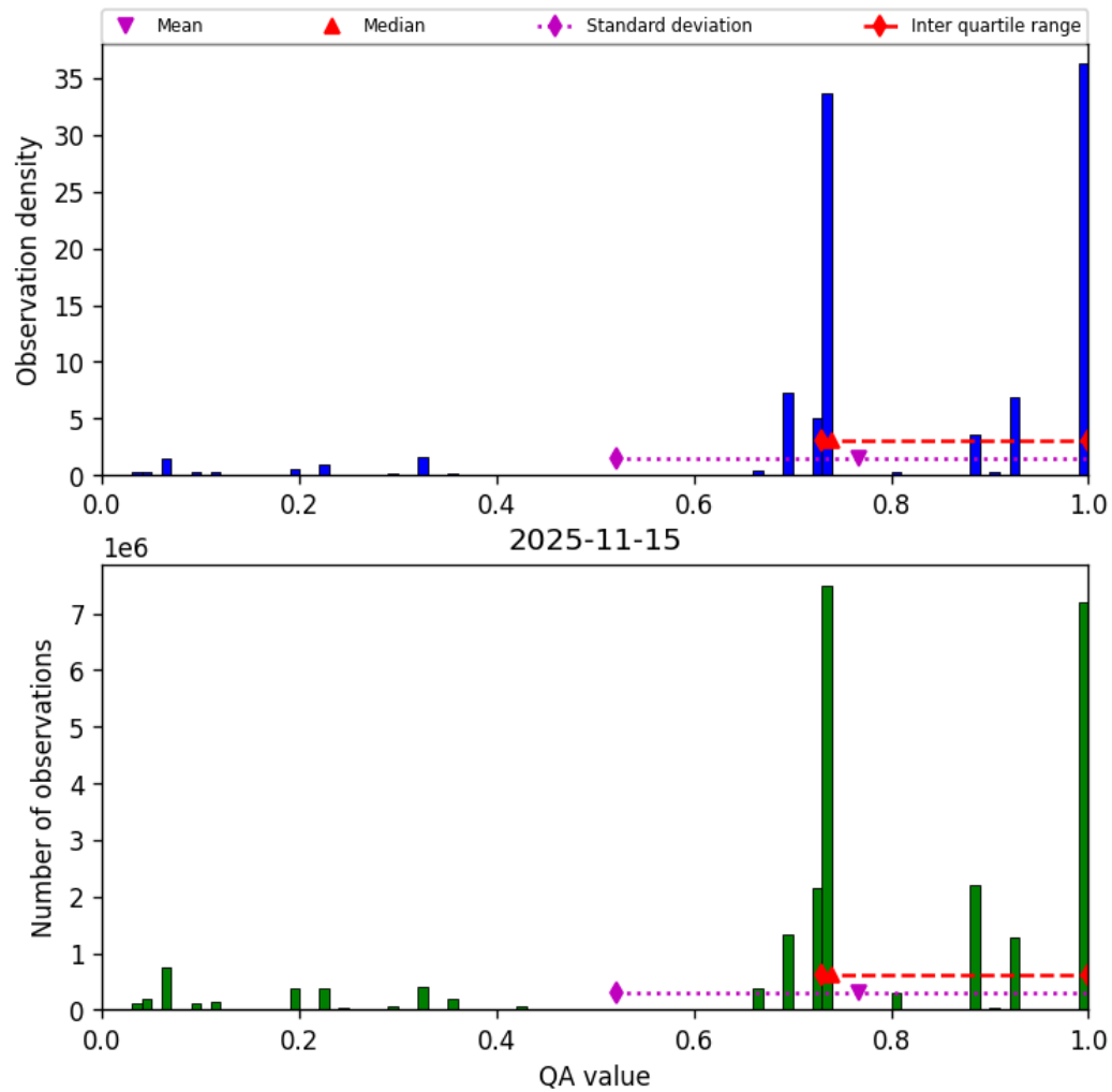
Figure 28: Histogram of “QA value” for 2025-11-14 to 2025-11-16
