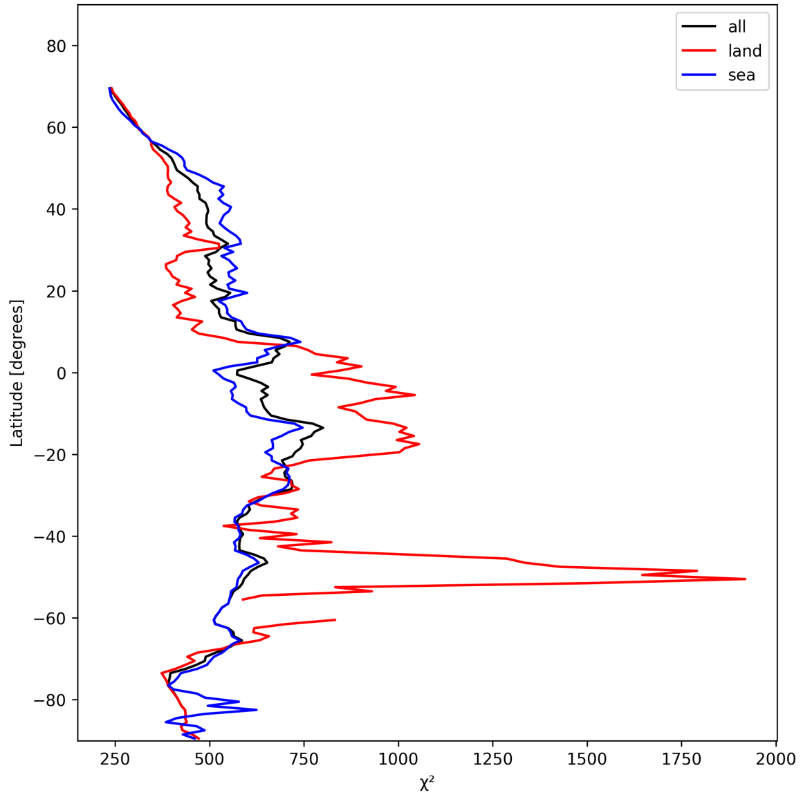
Figure 25: Zonal average of “ \chi^2 ” for 2025-11-14 to 2025-11-16.
