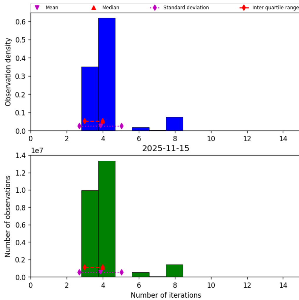
Figure 34: Histogram of “Number of iterations” for 2025-11-14 to 2025-11-16
