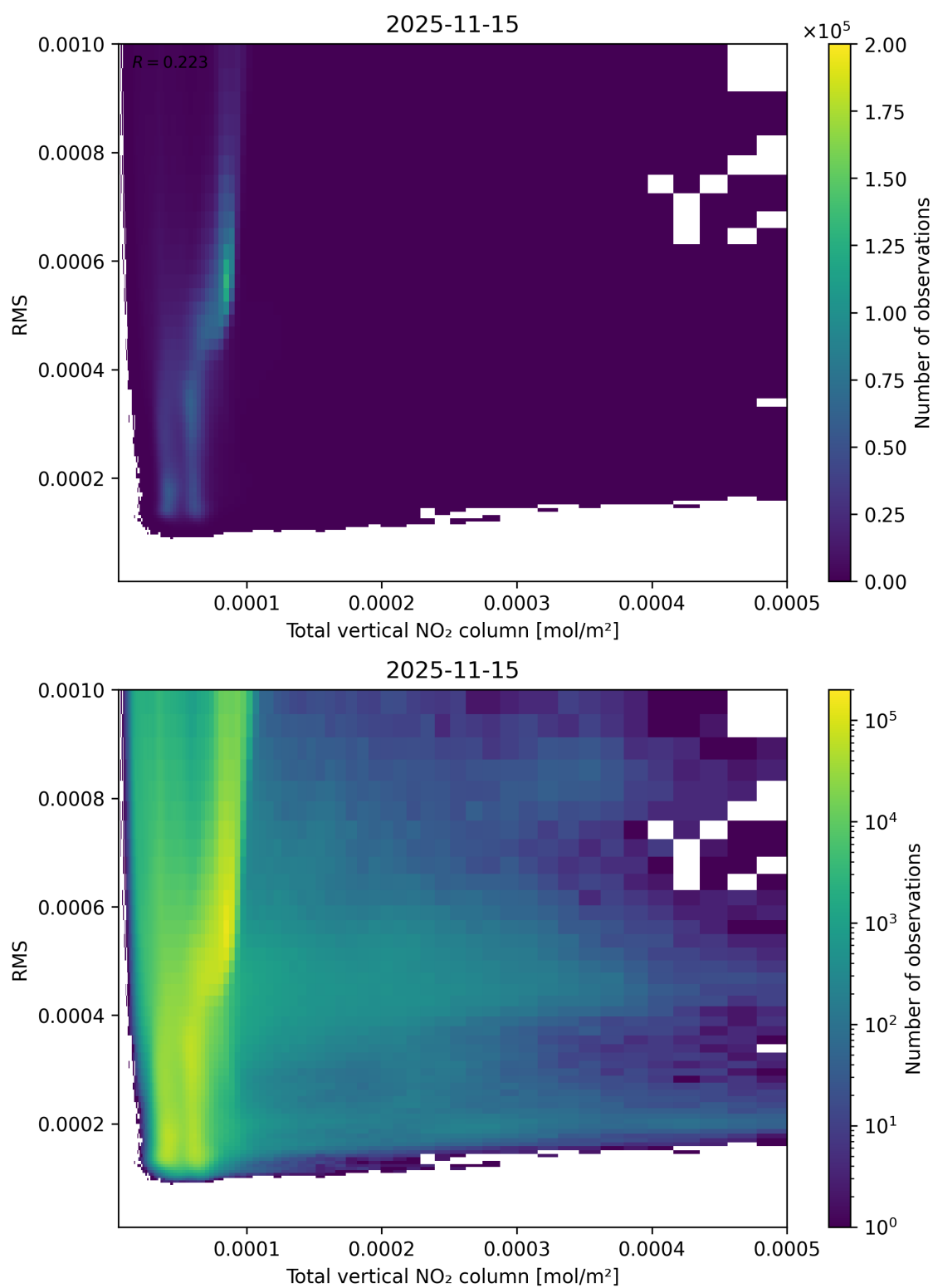
Figure 120: Scatter density plot of “Total vertical NO 2 column” against “RMS” for 2025-11-14 to 2025-11-16.
