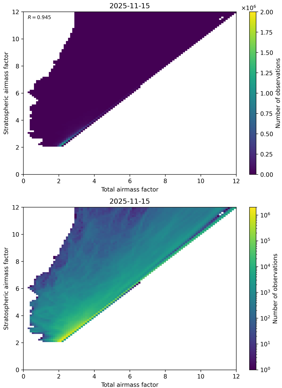
Figure 62: Scatter density plot of “Total airmass factor” against “Stratospheric airmass factor” for 2025-11-14 to 2025-11-16.
