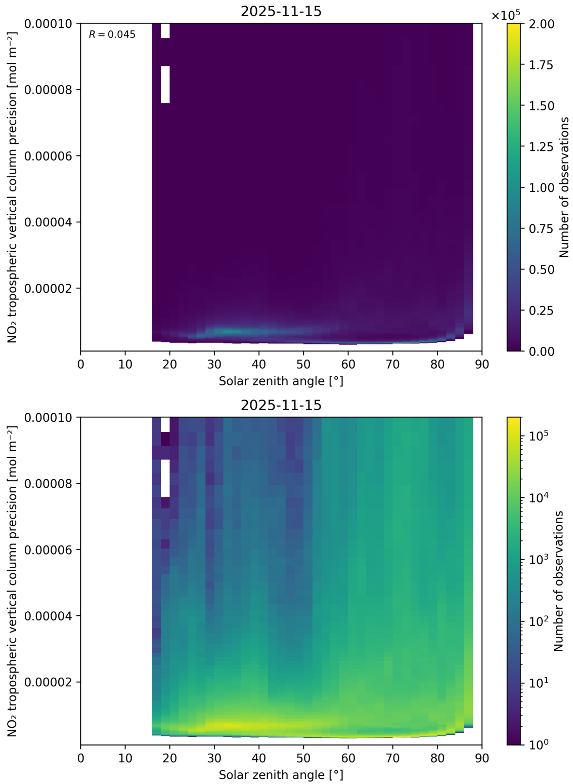
Figure 156: Scatter density plot of “Solar zenith angle” against “NO 2 tropospheric vertical column precision” for 2025-11-14 to 2025-11-16.
