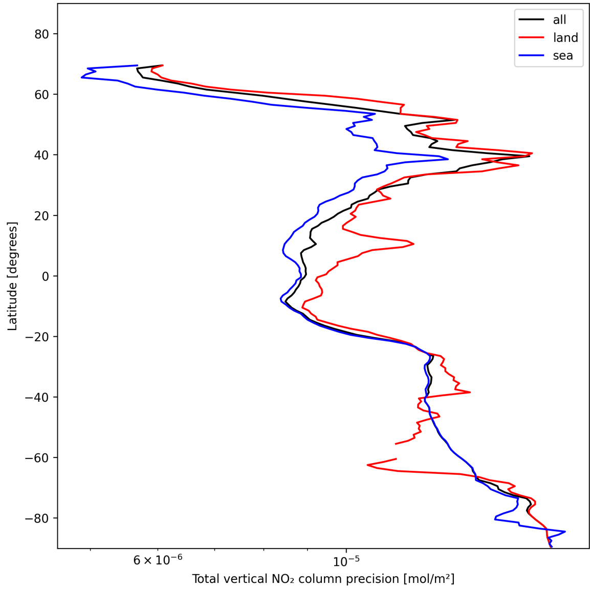
Figure 22: Zonal average of “Total vertical NO 2 column precision” for 2025-11-14 to 2025-11-16.
