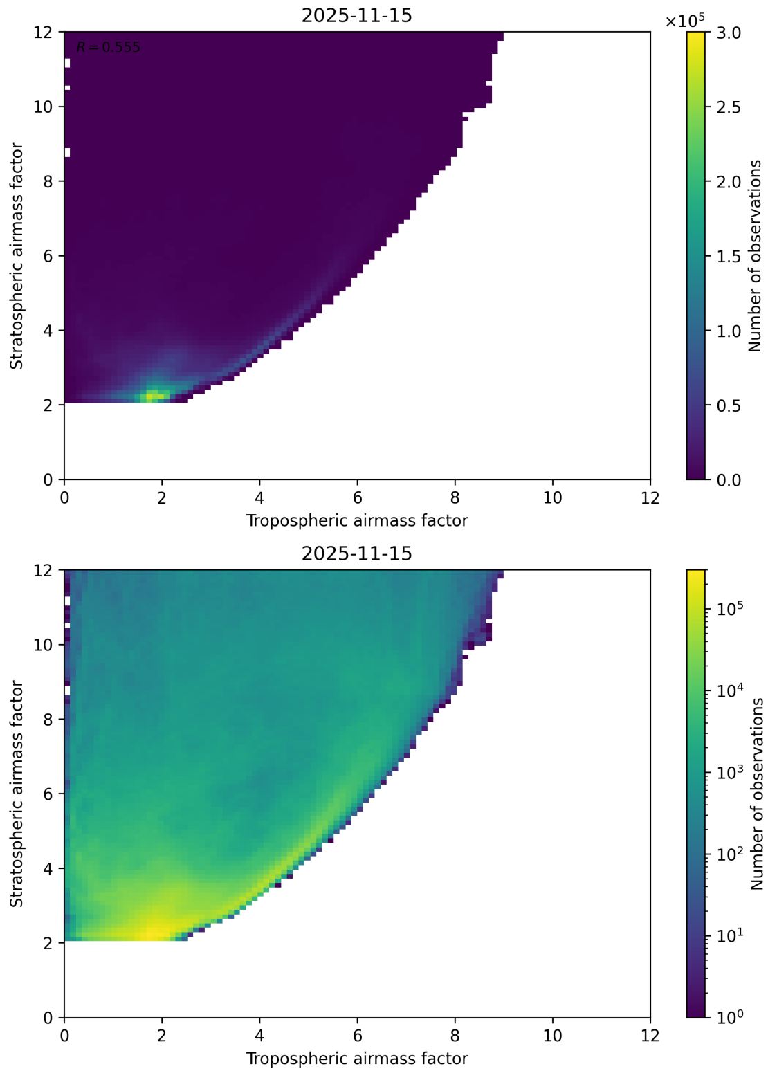
Figure 71: Scatter density plot of “Tropospheric airmass factor” against “Stratospheric airmass factor” for 2025-11-14 to 2025-11-16.
