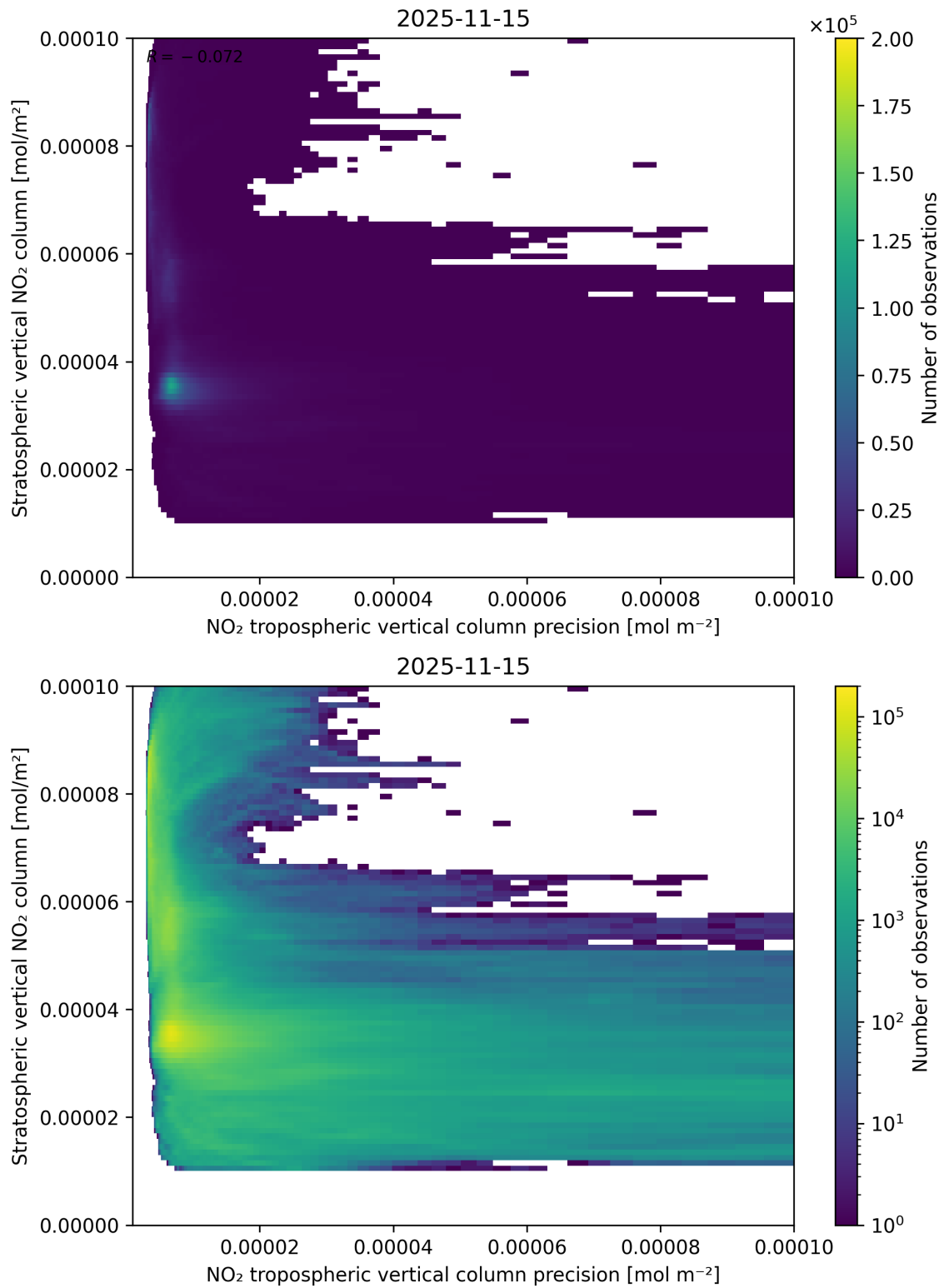
Figure 135: Scatter density plot of “NO 2 tropospheric vertical column precision” against “Stratospheric vertical NO 2 column” for 2025-11-14 to 2025-11-16.
