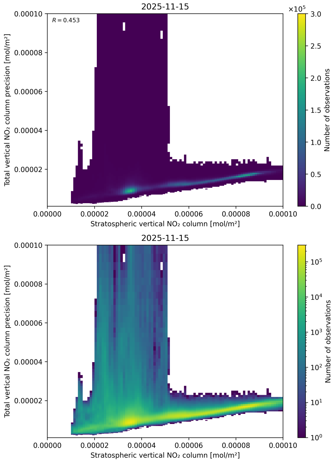
Figure 101: Scatter density plot of “Stratospheric vertical NO 2 column” against “Total vertical NO 2 column precision” for 2025-11-14 to 2025-11-16.
