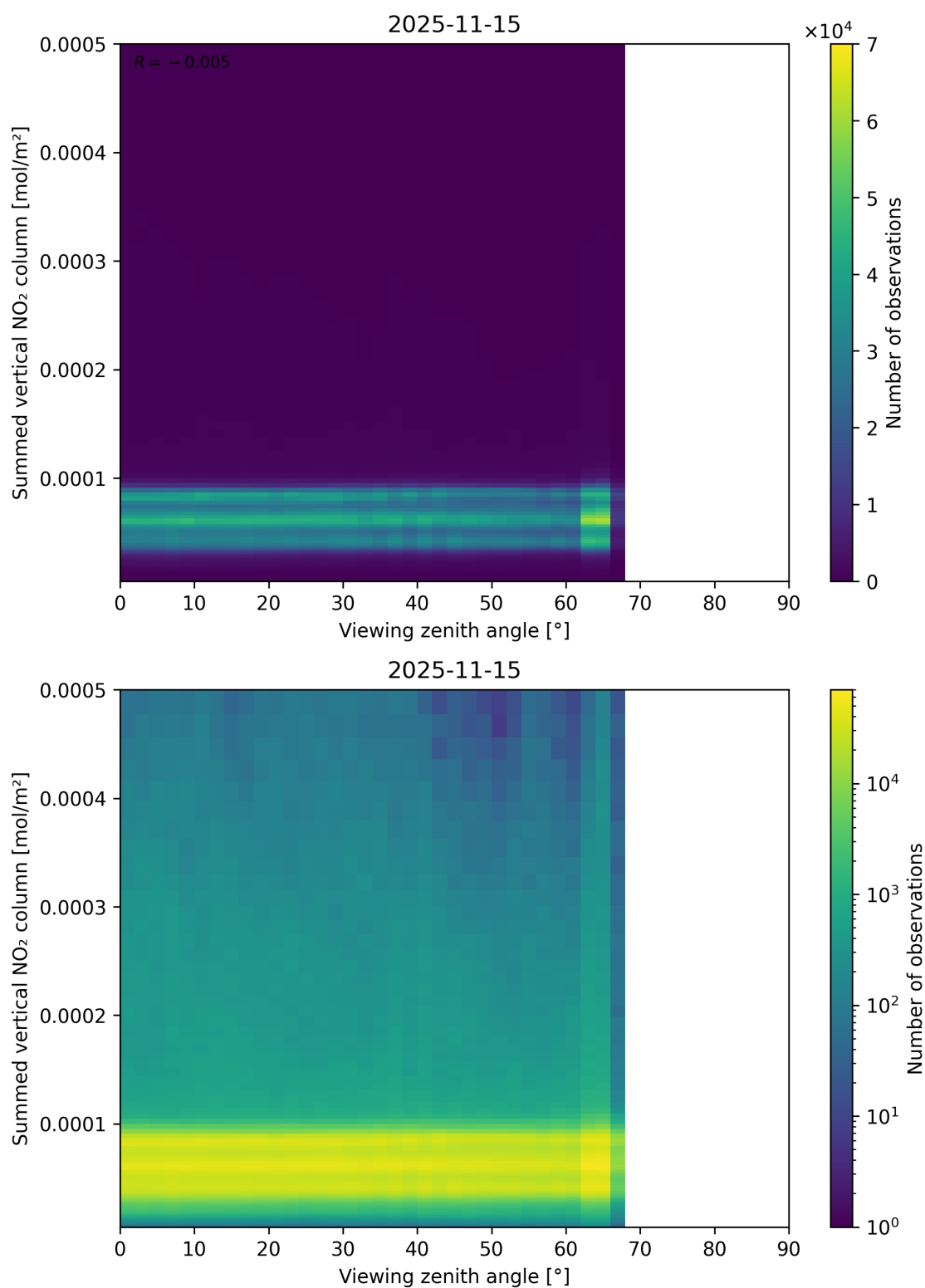
Figure 165: Scatter density plot of “Viewing zenith angle” against “Summed vertical NO 2 column” for 2025-11-14 to 2025-11-16.
