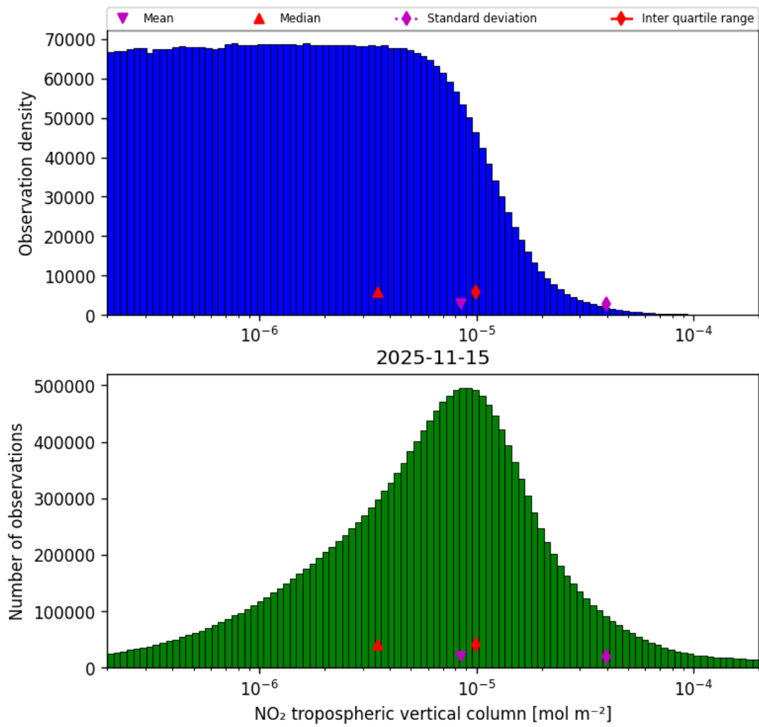
Figure 29: Histogram of “NO 2 tropospheric vertical column” for 2025-11-14 to 2025-11-16
