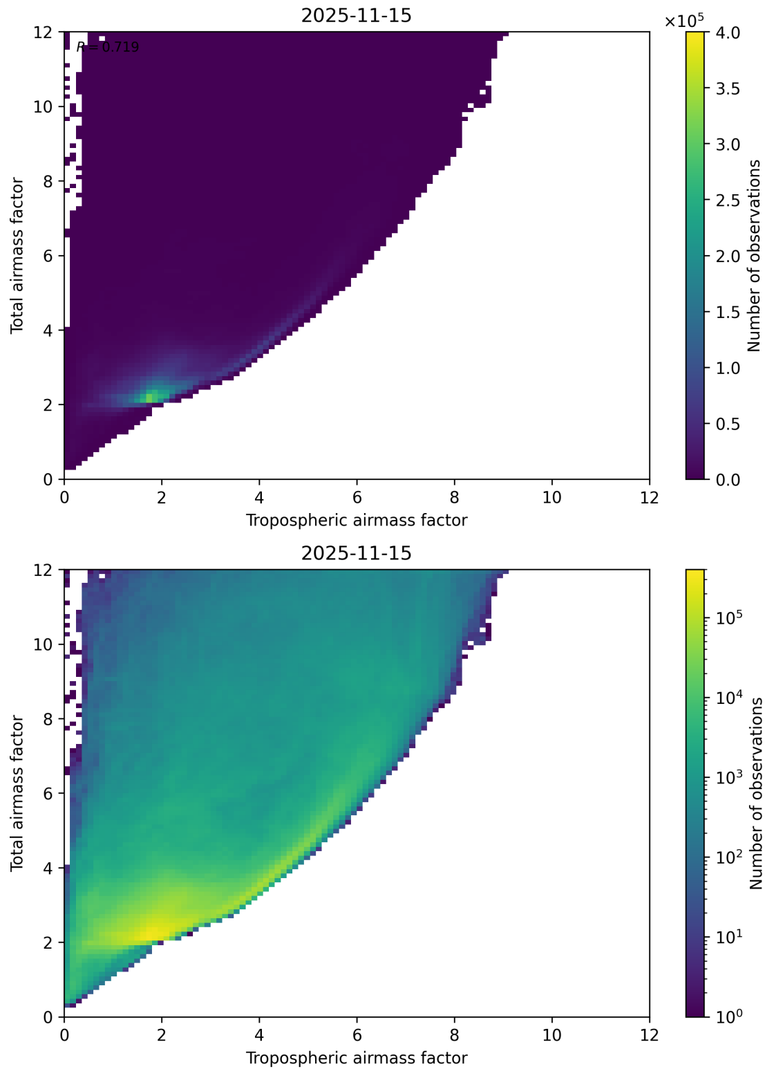
Figure 72: Scatter density plot of “Tropospheric airmass factor” against “Total airmass factor” for 2025-11-14 to 2025-11-16.
