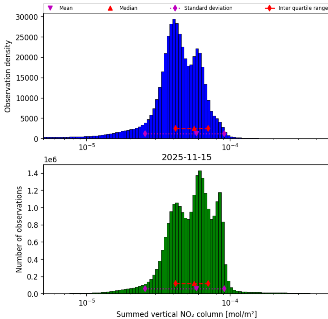
Figure 40: Histogram of “Summed vertical NO 2 column” for 2025-11-14 to 2025-11-16
