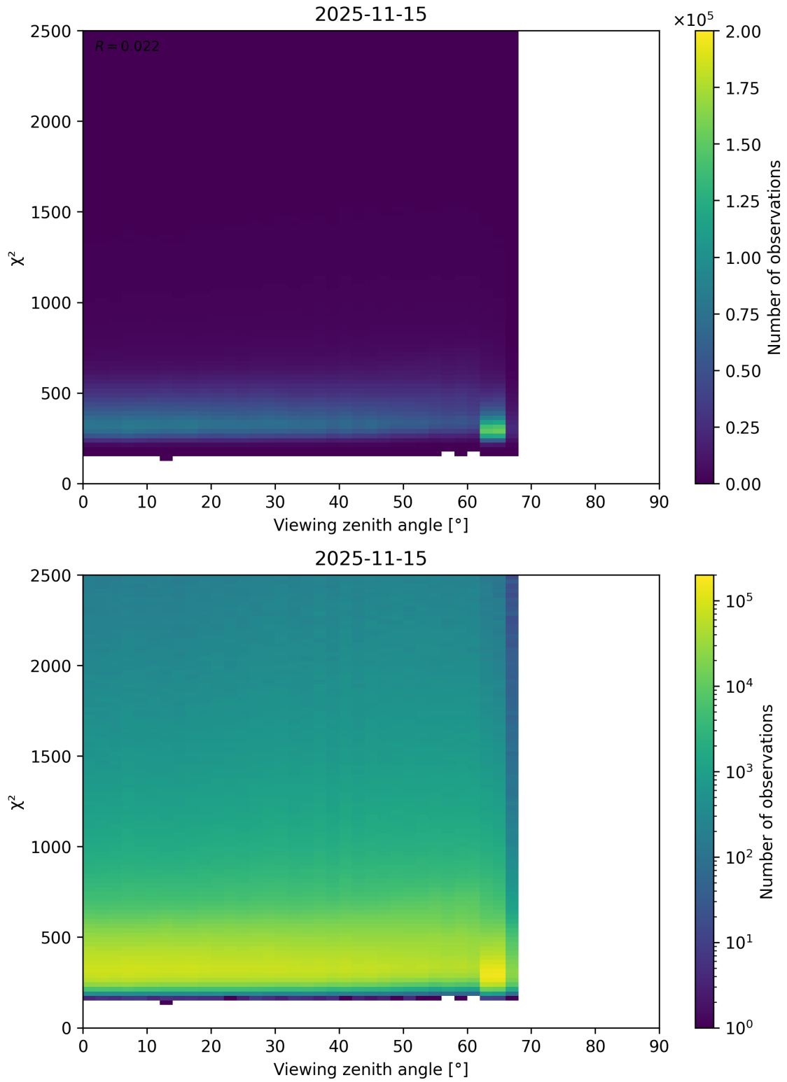
Figure 162: Scatter density plot of “Viewing zenith angle” against “ \chi^2 ” for 2025-11-14 to 2025-11-16.
