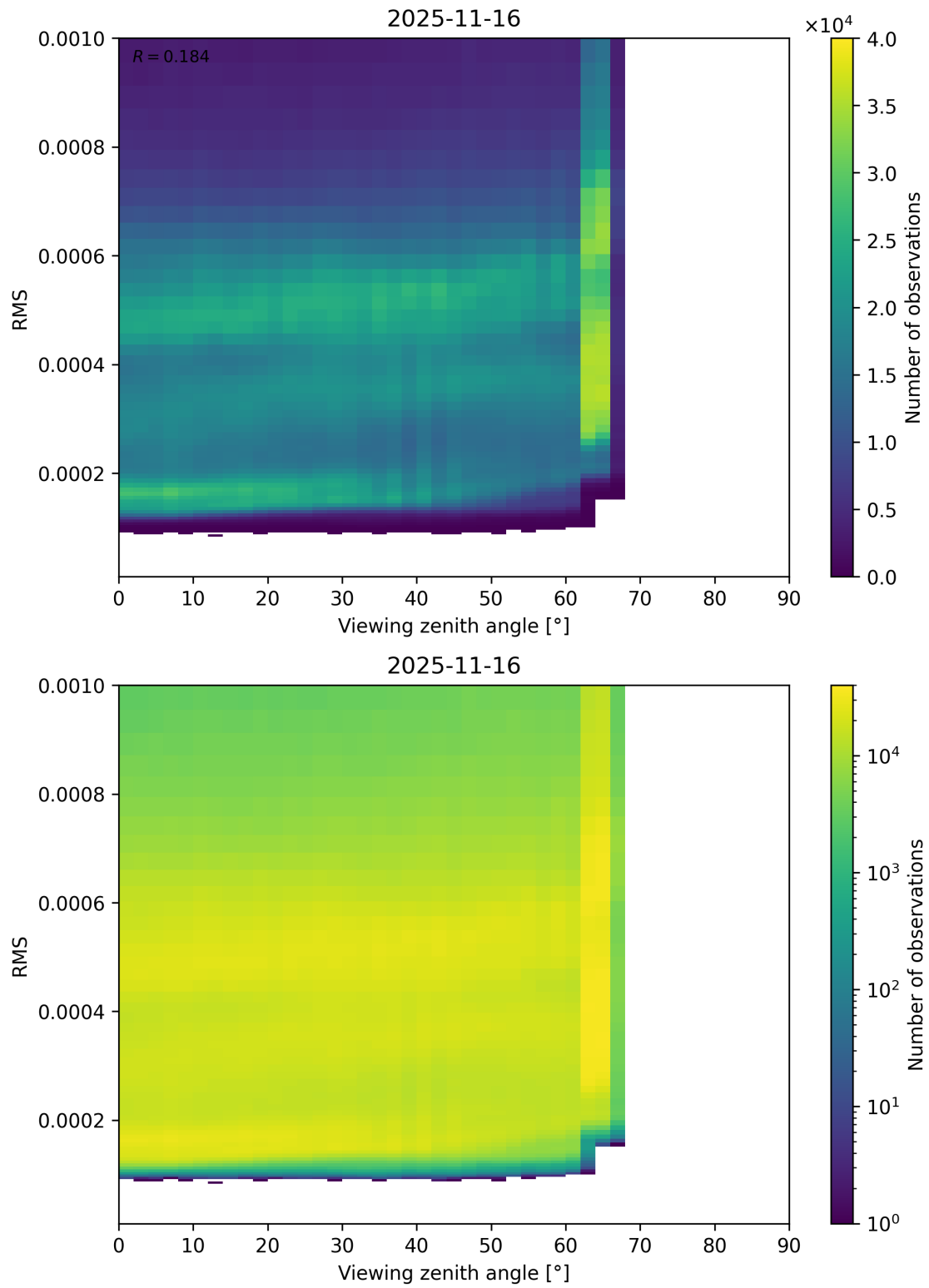
Figure 171: Scatter density plot of “Viewing zenith angle” against “RMS” for 2025-11-15 to 2025-11-17.
