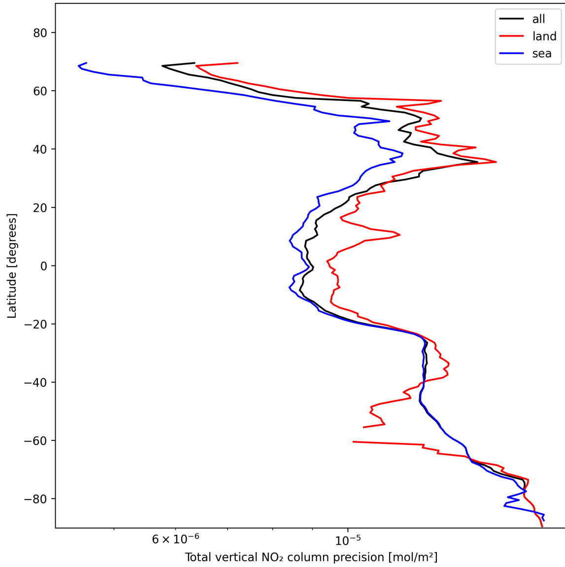
Figure 22: Zonal average of “Total vertical NO 2 column precision” for 2025-11-15 to 2025-11-17.
