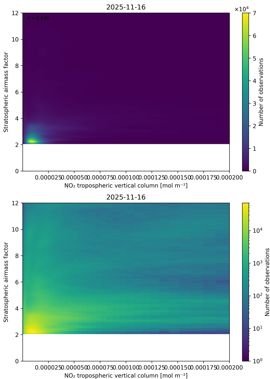
Figure 121: Scatter density plot of “NO 2 tropospheric vertical column” against “Stratospheric airmass factor” for 2025-11-15 to 2025-11-17.
