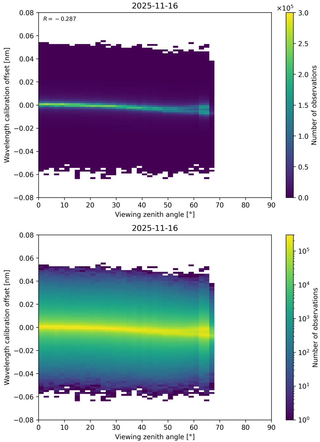
Figure 173: Scatter density plot of “Viewing zenith angle” against “Wavelength calibration offset” for 2025-11-15 to 2025-11-17.
