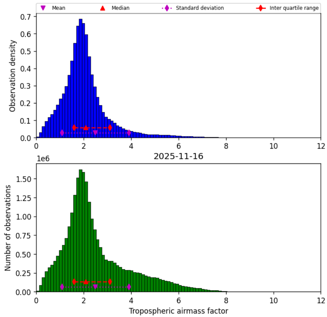
Figure 31: Histogram of “Tropospheric airmass factor” for 2025-11-15 to 2025-11-17
