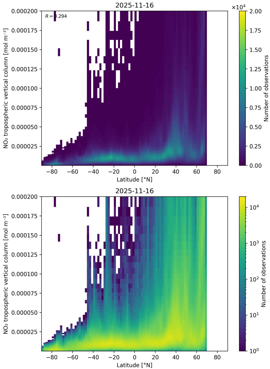
Figure 92: Scatter density plot of “Latitude” against “NO 2 tropospheric vertical column” for 2025-11-15 to 2025-11-17.
