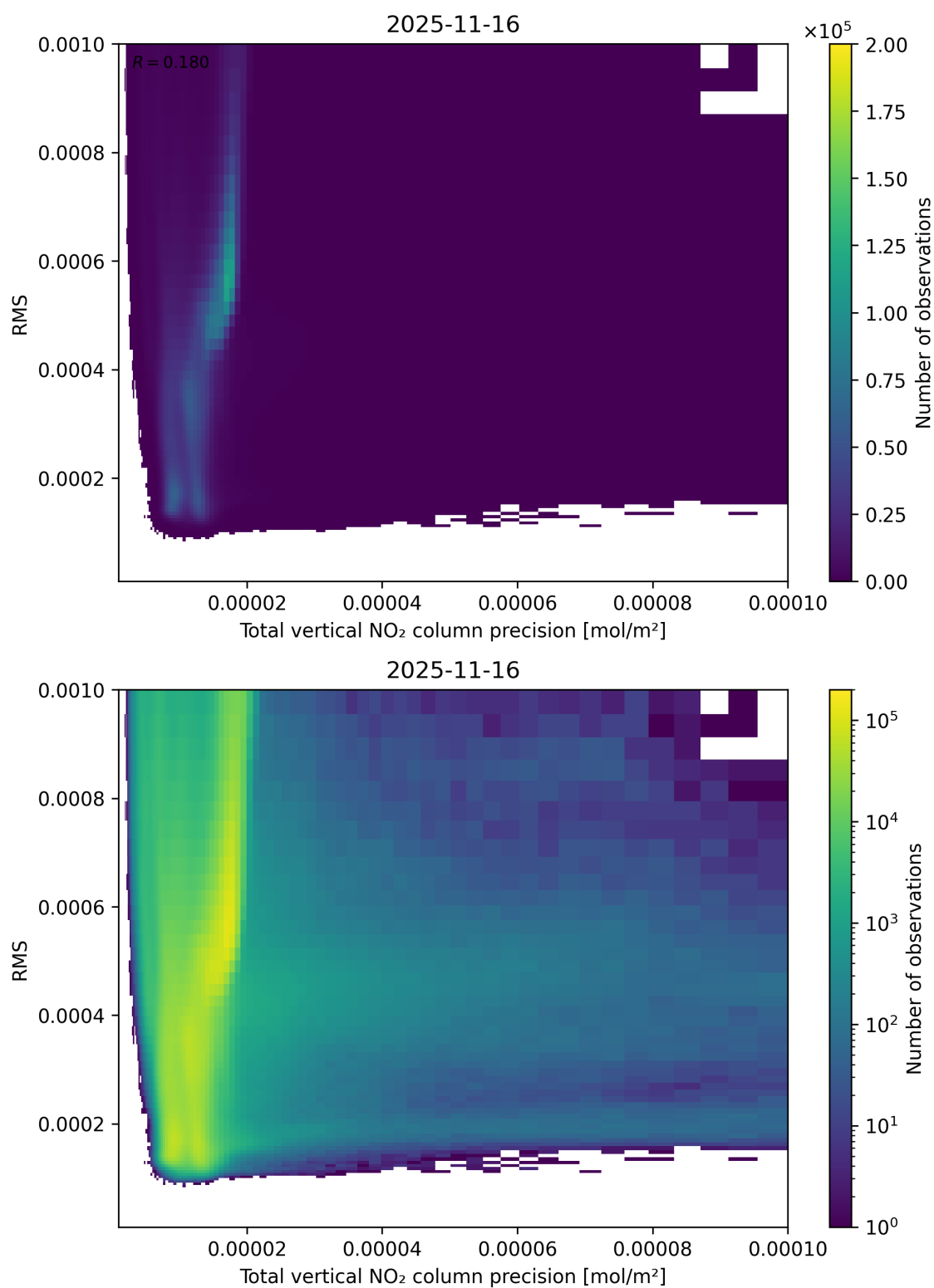
Figure 119: Scatter density plot of “Total vertical NO 2 column precision” against “RMS” for 2025-11-15 to 2025-11-17.
