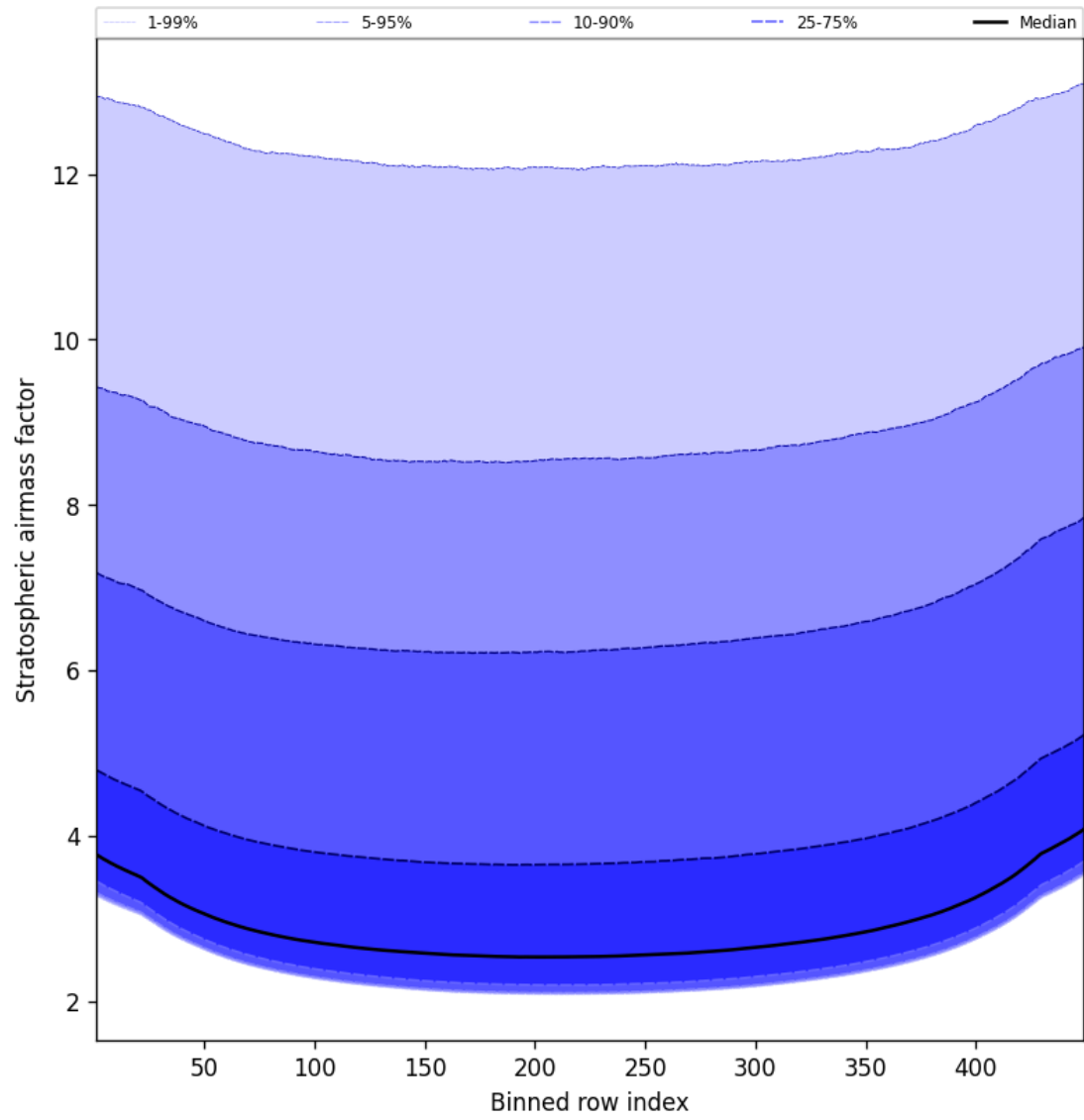
Figure 61: Along track statistics of “Stratospheric airmass factor” for 2025-11-15 to 2025-11-17
