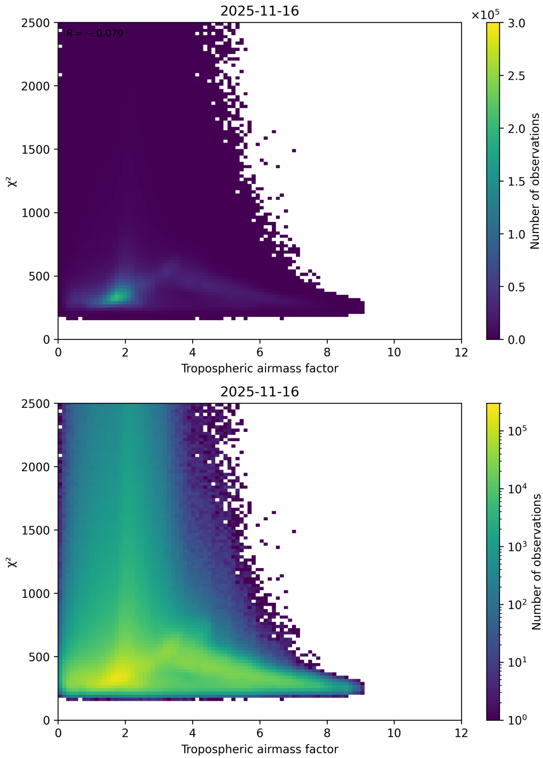
Figure 73: Scatter density plot of “Tropospheric airmass factor” against “ \chi^2 ” for 2025-11-15 to 2025-11-17.
