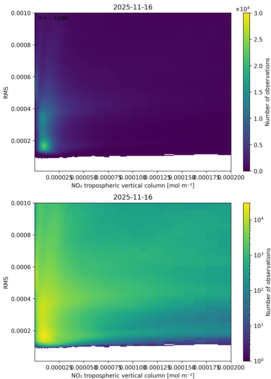
Figure 142: Scatter density plot of “NO 2 tropospheric vertical column” against “RMS” for 2025-11-15 to 2025-11-17.
