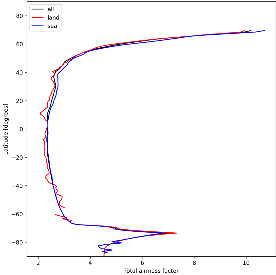
Figure 15: Zonal average of “Total airmass factor” for 2025-11-15 to 2025-11-17.
