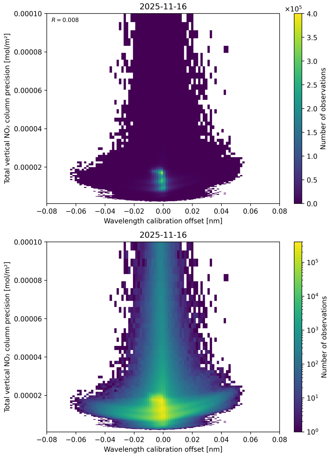
Figure 180: Scatter density plot of “Wavelength calibration offset” against “Total vertical NO 2 column precision” for 2025-11-15 to 2025-11-17.
