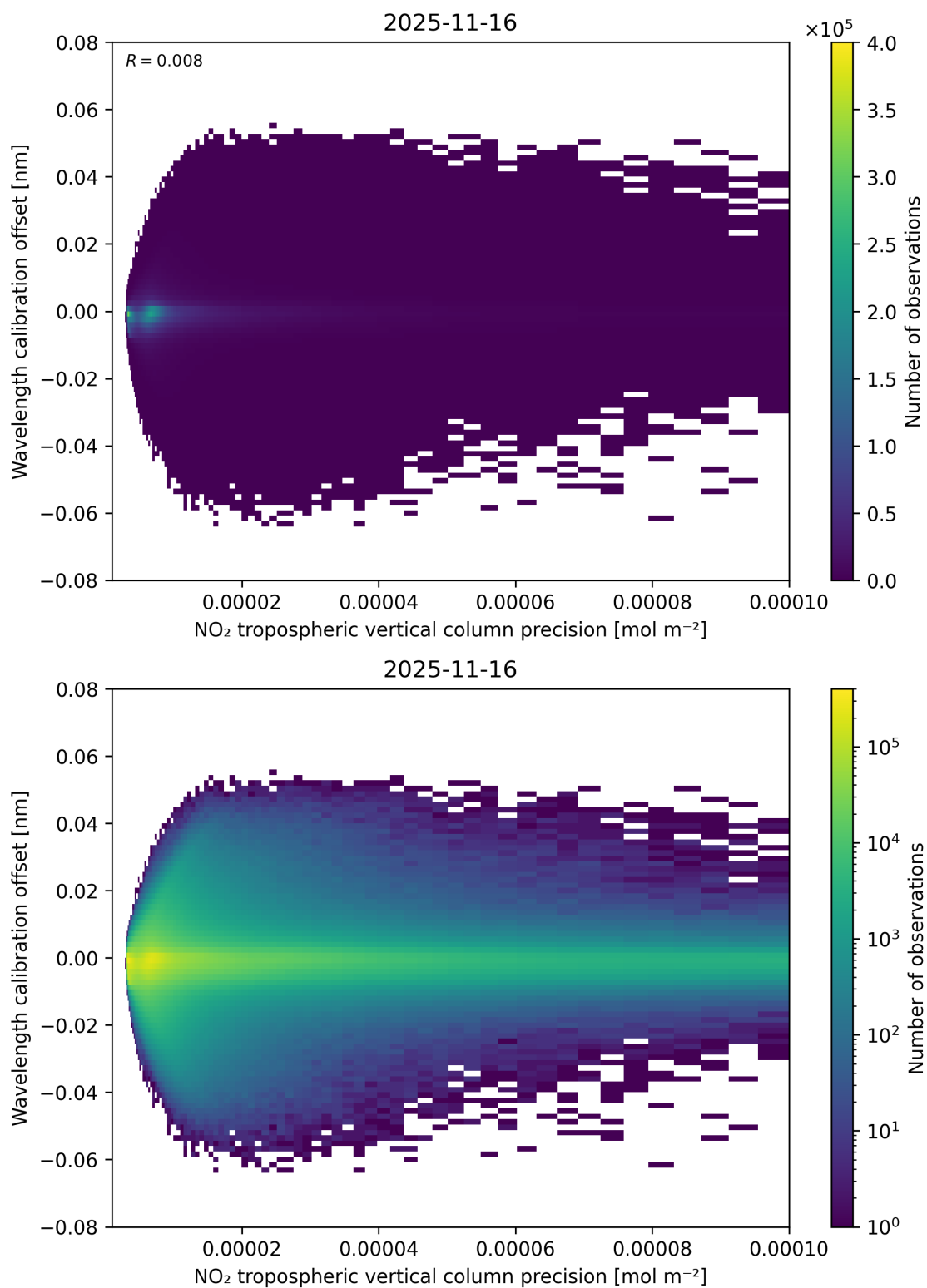
Figure 141: Scatter density plot of “NO 2 tropospheric vertical column precision” against “Wavelength calibration offset” for 2025-11-15 to 2025-11-17.
