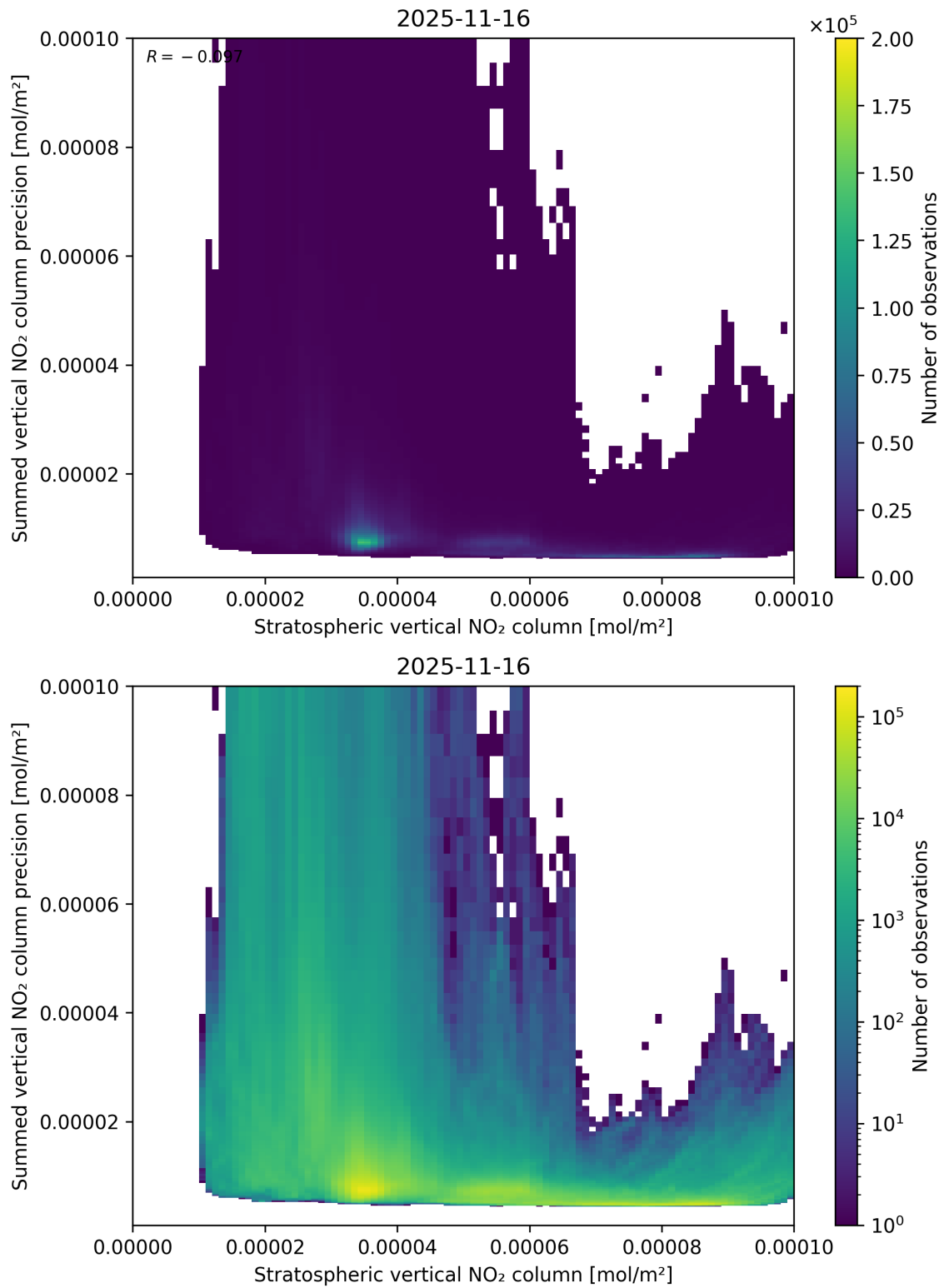
Figure 99: Scatter density plot of “Stratospheric vertical NO 2 column” against “Summed vertical NO 2 column precision” for 2025-11-15 to 2025-11-17.
