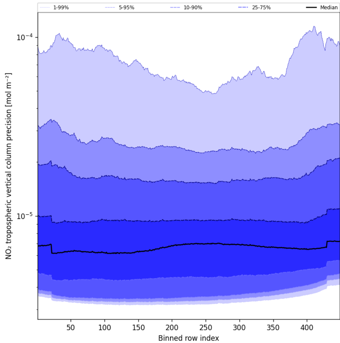
Figure 47: Along track statistics of “NO 2 tropospheric vertical column precision” for 2025-11-15 to 2025-11-17
