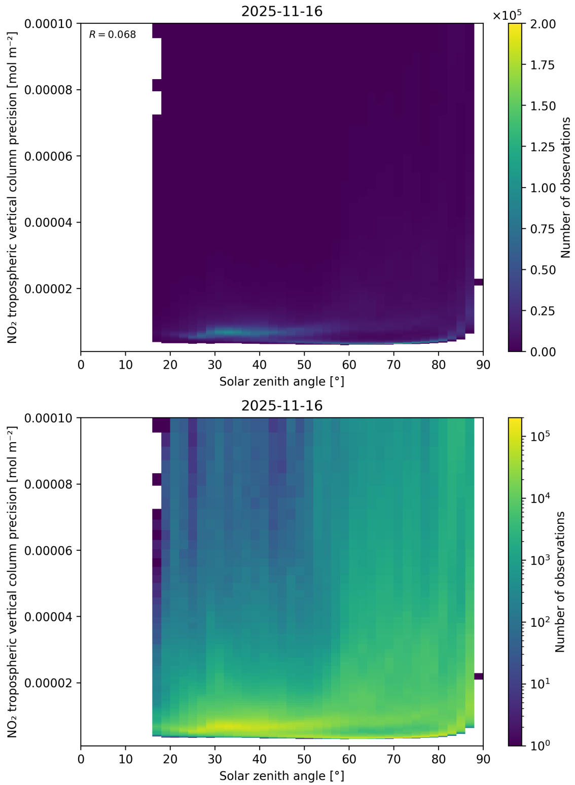
Figure 156: Scatter density plot of “Solar zenith angle” against “NO 2 tropospheric vertical column precision” for 2025-11-15 to 2025-11-17.
