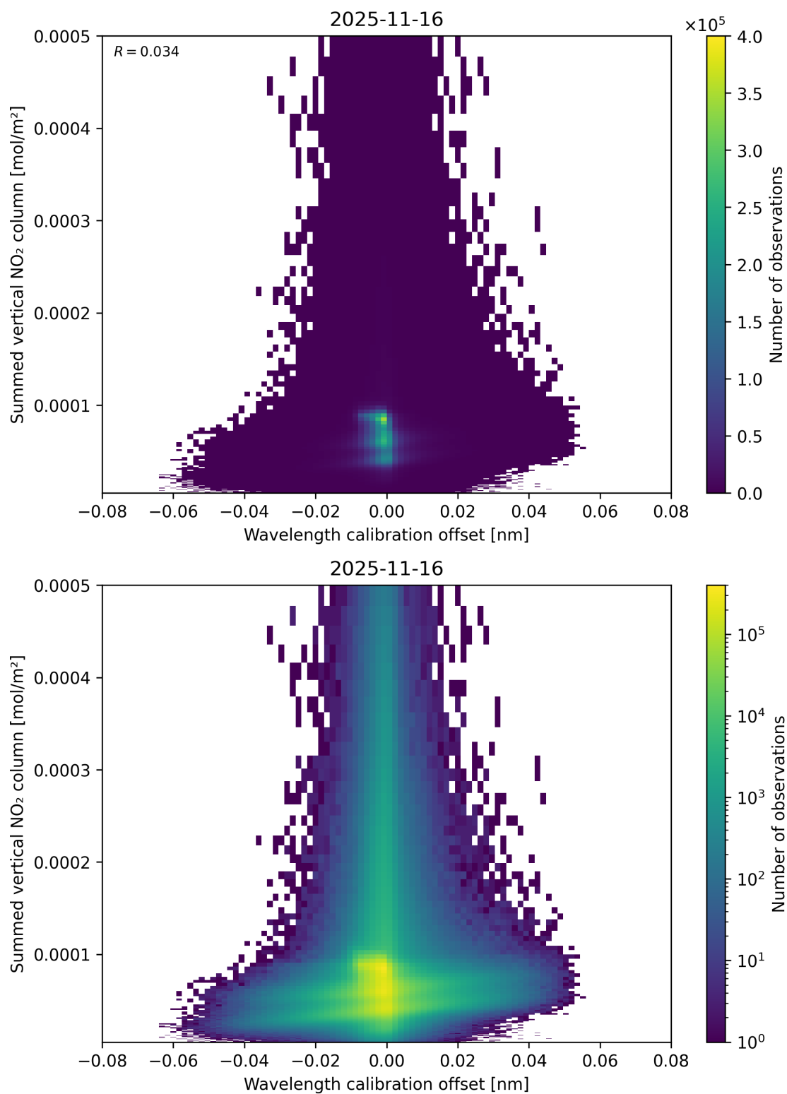
Figure 177: Scatter density plot of “Wavelength calibration offset” against “Summed vertical NO 2 column” for 2025-11-15 to 2025-11-17.
