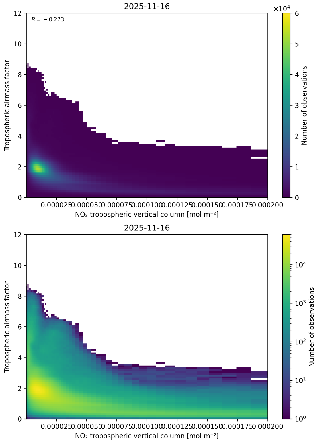
Figure 123: Scatter density plot of “NO 2 tropospheric vertical column” against “Tropospheric air mass factor” for 2025-11-15 to 2025-11-17.
