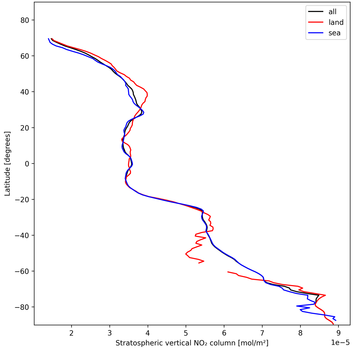
Figure 19: Zonal average of “Stratospheric vertical NO 2 column” for 2025-11-15 to 2025-11-17.
