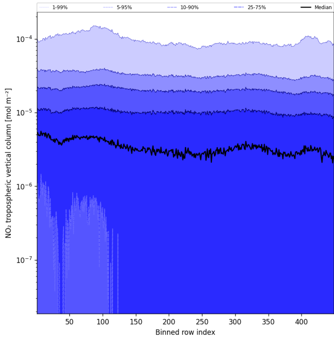
Figure 46: Along track statistics of “NO 2 tropospheric vertical column” for 2025-11-15 to 2025-11-17
