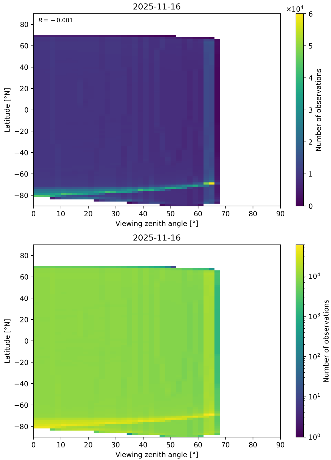
Figure 163: Scatter density plot of “Viewing zenith angle” against “Latitude” for 2025-11-15 to 2025-11-17.
