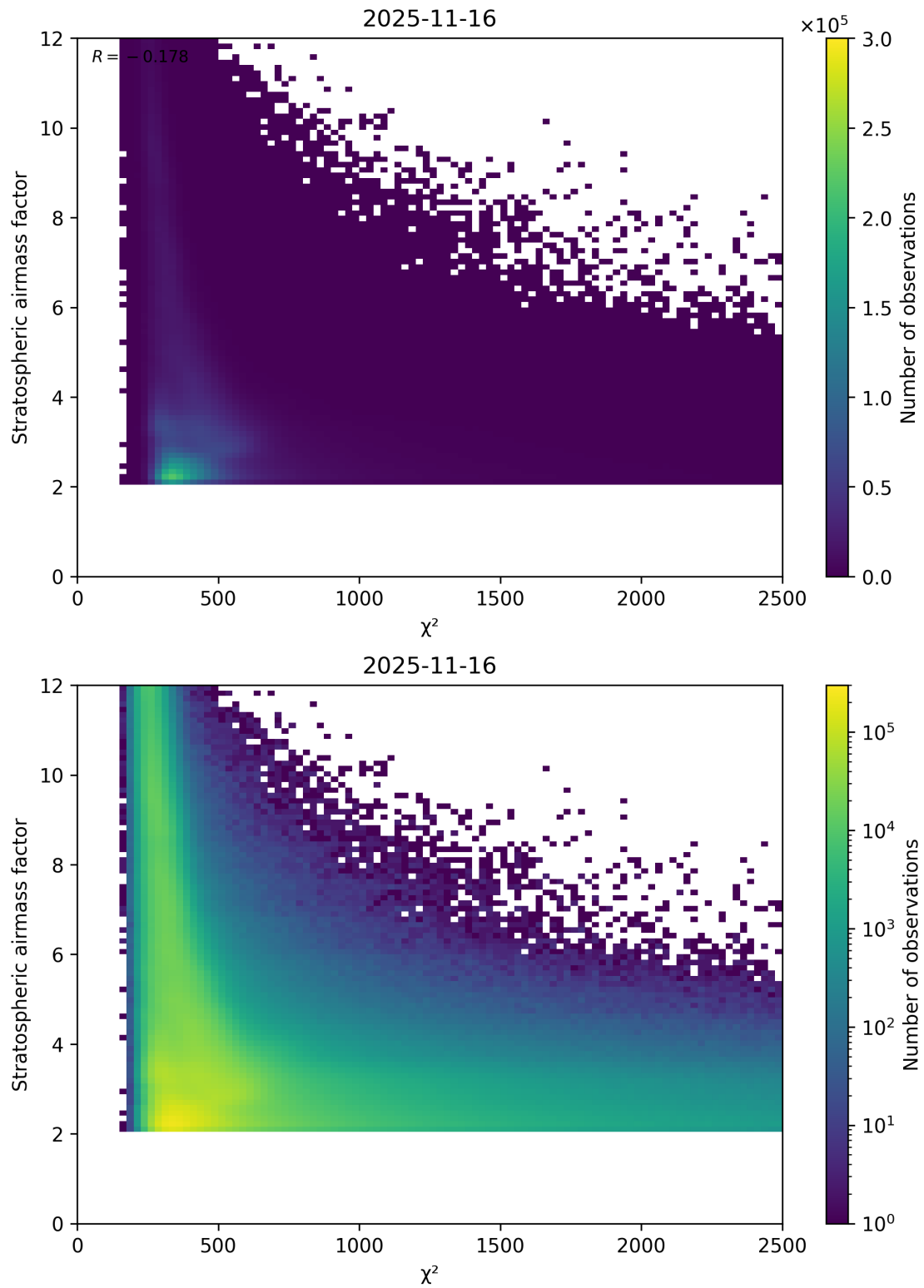
Figure 81: Scatter density plot of “ \chi^2 ” against “Stratospheric air mass factor” for 2025-11-15 to 2025-11-17.
