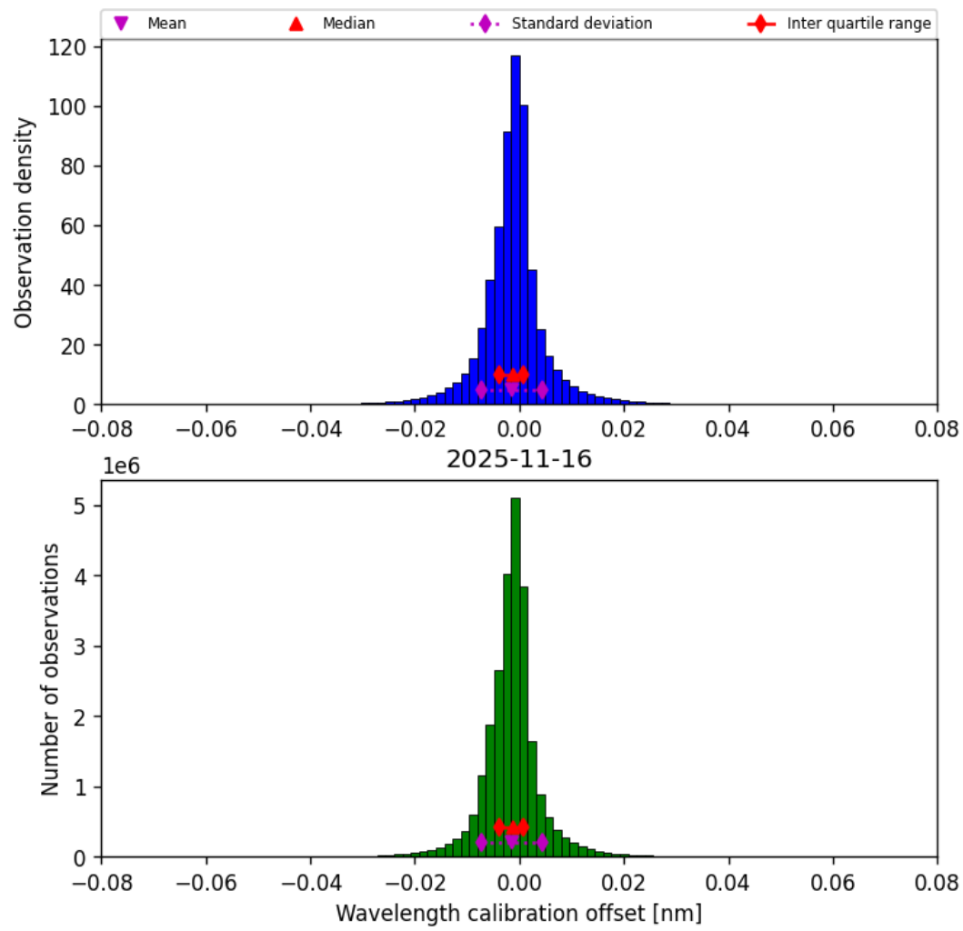
Figure 35: Histogram of “Wavelength calibration offset” for 2025-11-15 to 2025-11-17
