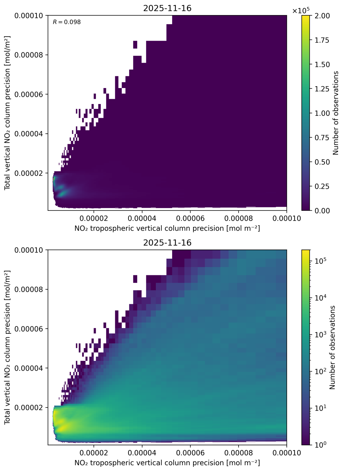
Figure 139: Scatter density plot of “NO 2 tropospheric vertical column precision” against “Total vertical NO 2 column precision” for 2025-11-15 to 2025-11-17.
