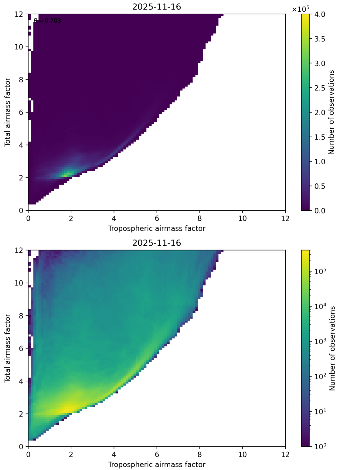
Figure 72: Scatter density plot of “Tropospheric airmass factor” against “Total airmass factor” for 2025-11-15 to 2025-11-17.
