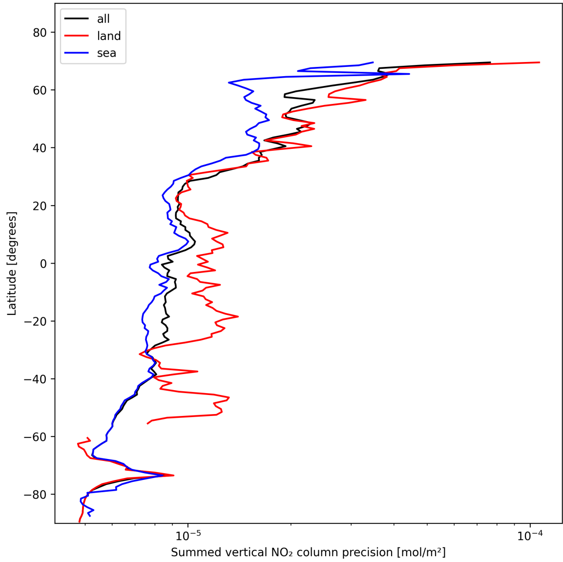
Figure 24: Zonal average of "Summed vertical NO 2 column precision" for 2025-11-15 to 2025-11-17.
