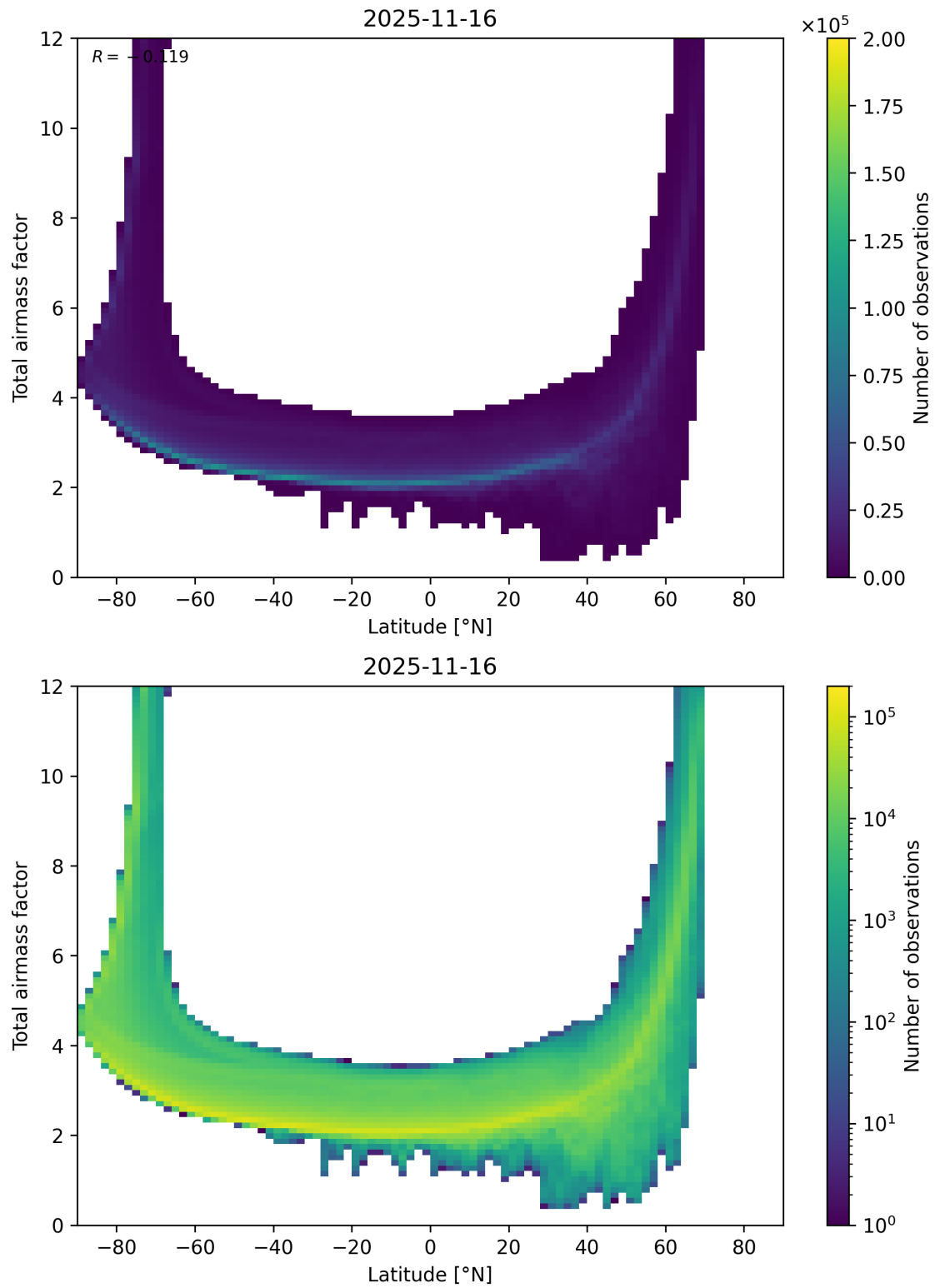
Figure 84: Scatter density plot of “Latitude” against “Total airmass factor” for 2025-11-15 to 2025-11-17.
