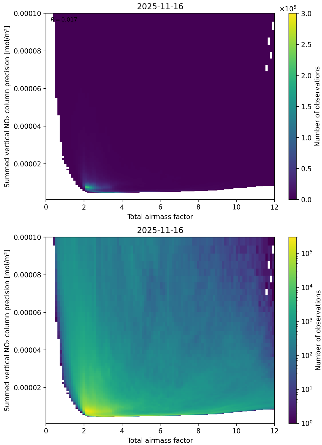
Figure 66: Scatter density plot of “Total airmass factor” against “Summed vertical NO 2 column precision” for 2025-11-15 to 2025-11-17.
