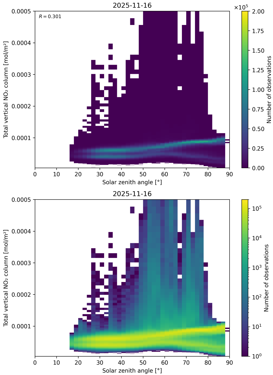
Figure 153: Scatter density plot of “Solar zenith angle” against “Total vertical NO 2 column” for 2025-11-15 to 2025-11-17.
