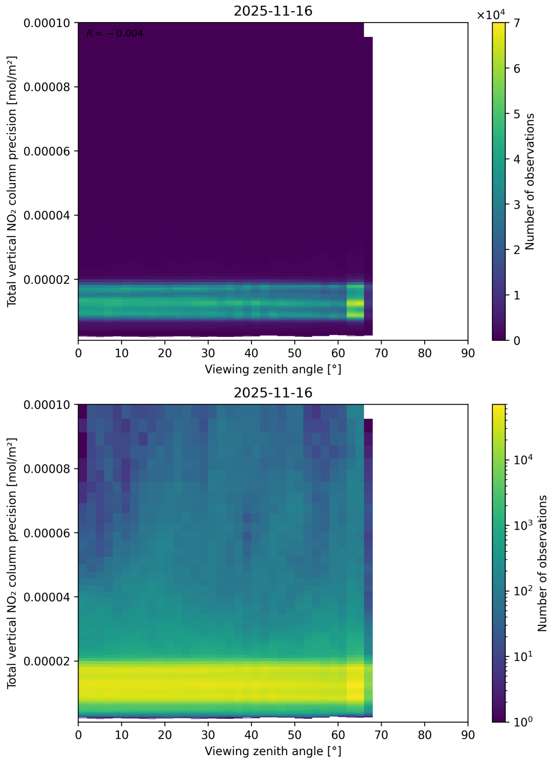
Figure 168: Scatter density plot of “Viewing zenith angle” against “Total vertical NO 2 column precision” for 2025-11-15 to 2025-11-17.
