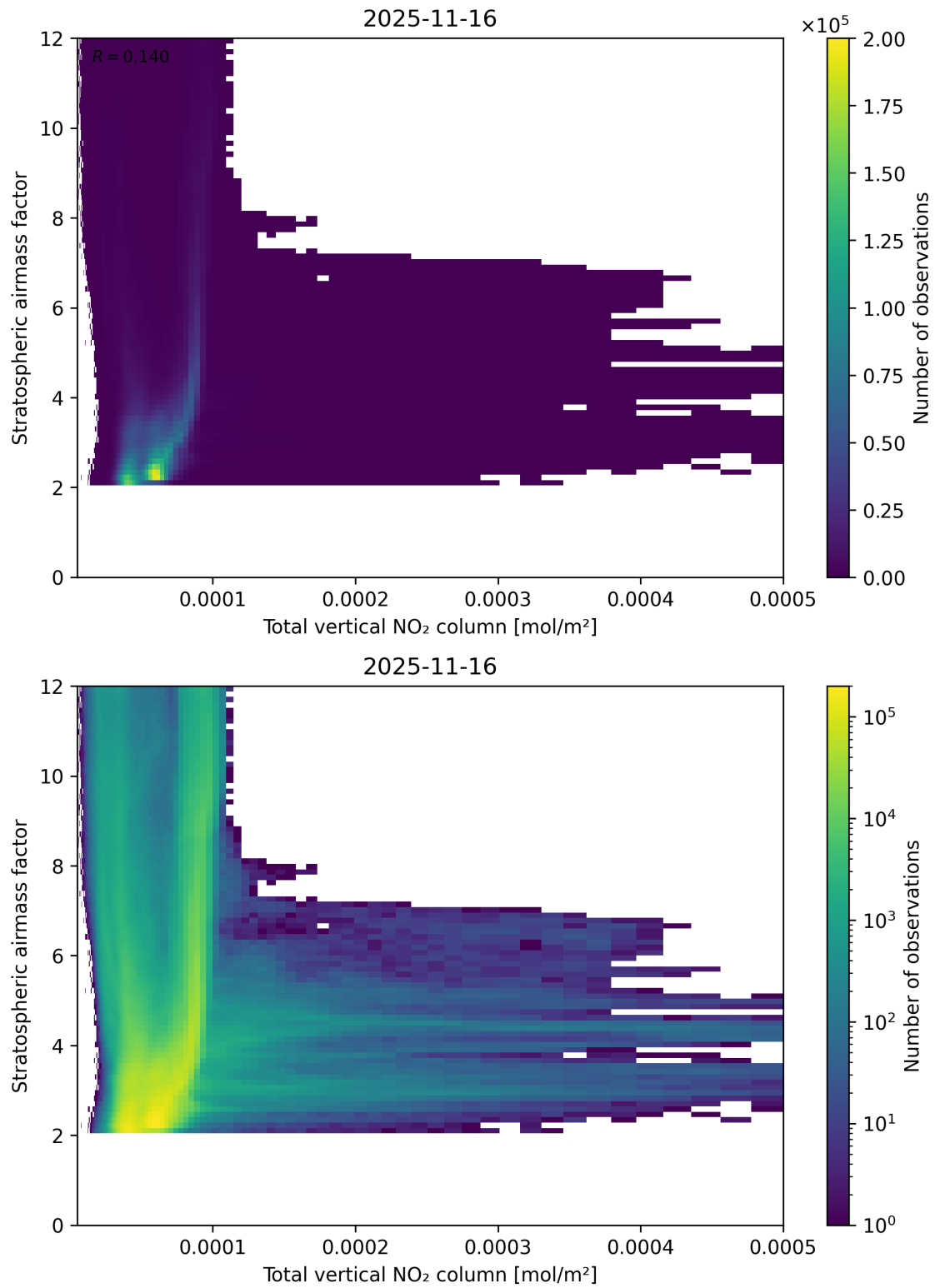
Figure 110: Scatter density plot of “Total vertical NO 2 column” against “Stratospheric airmass factor” for 2025-11-15 to 2025-11-17.
