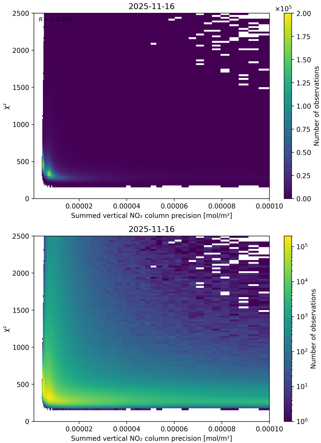
Figure 107: Scatter density plot of “Summed vertical NO 2 column precision” against “ \chi^2 ” for 2025-11-15 to 2025-11-17.
