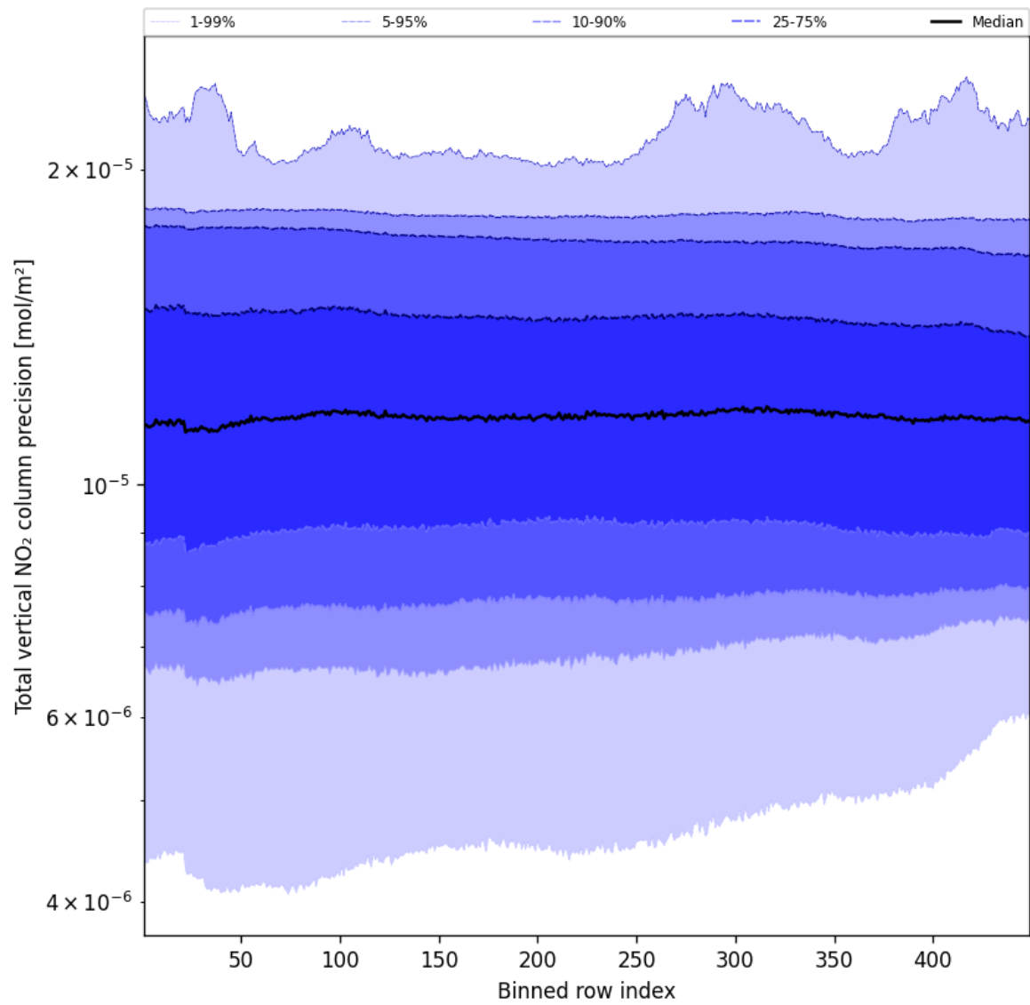
Figure 56: Along track statistics of “Total vertical NO 2 column precision” for 2025-11-15 to 2025-11-17
