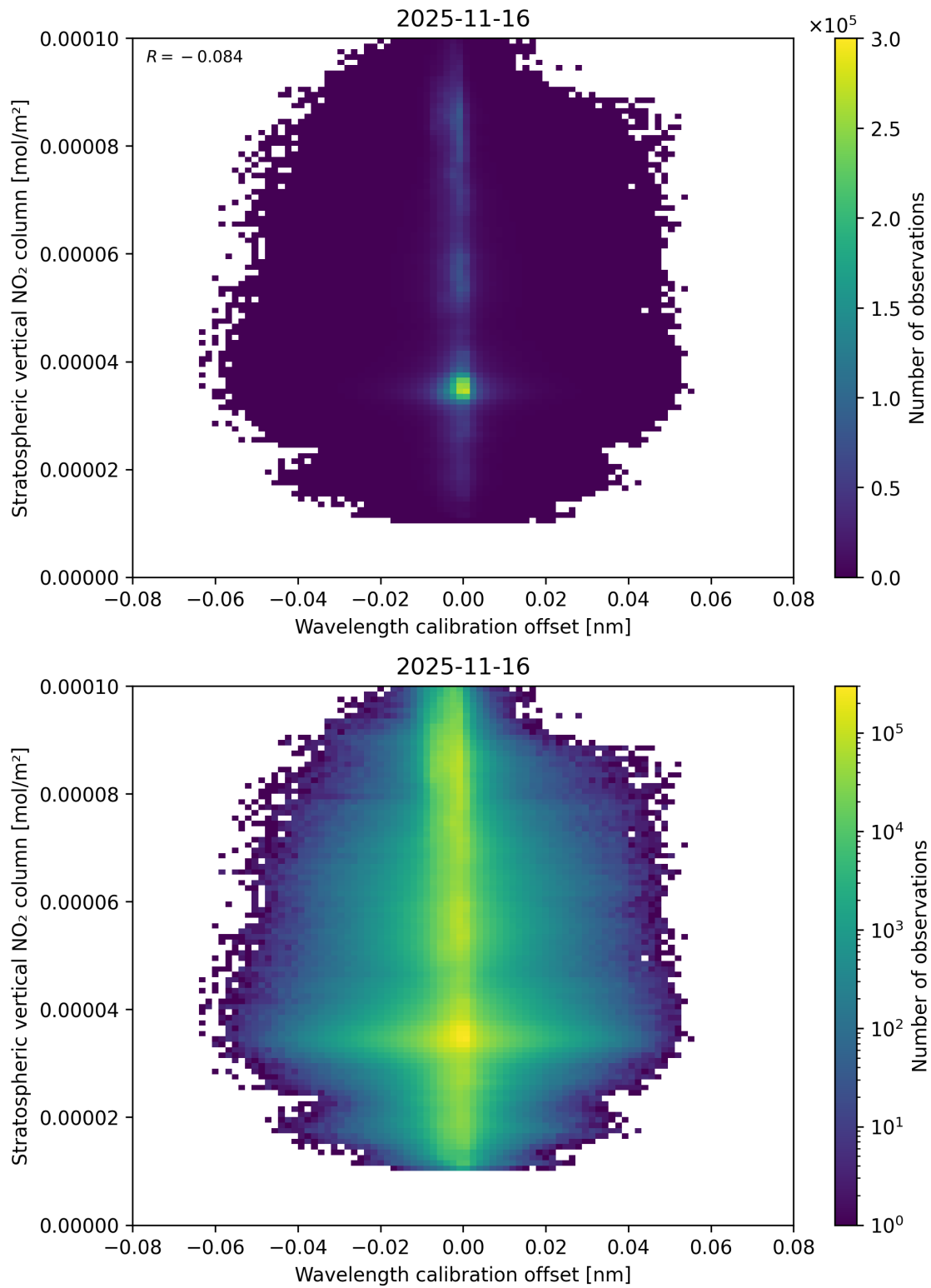
Figure 176: Scatter density plot of “Wavelength calibration offset” against “Stratospheric vertical NO 2 column” for 2025-11-15 to 2025-11-17.
