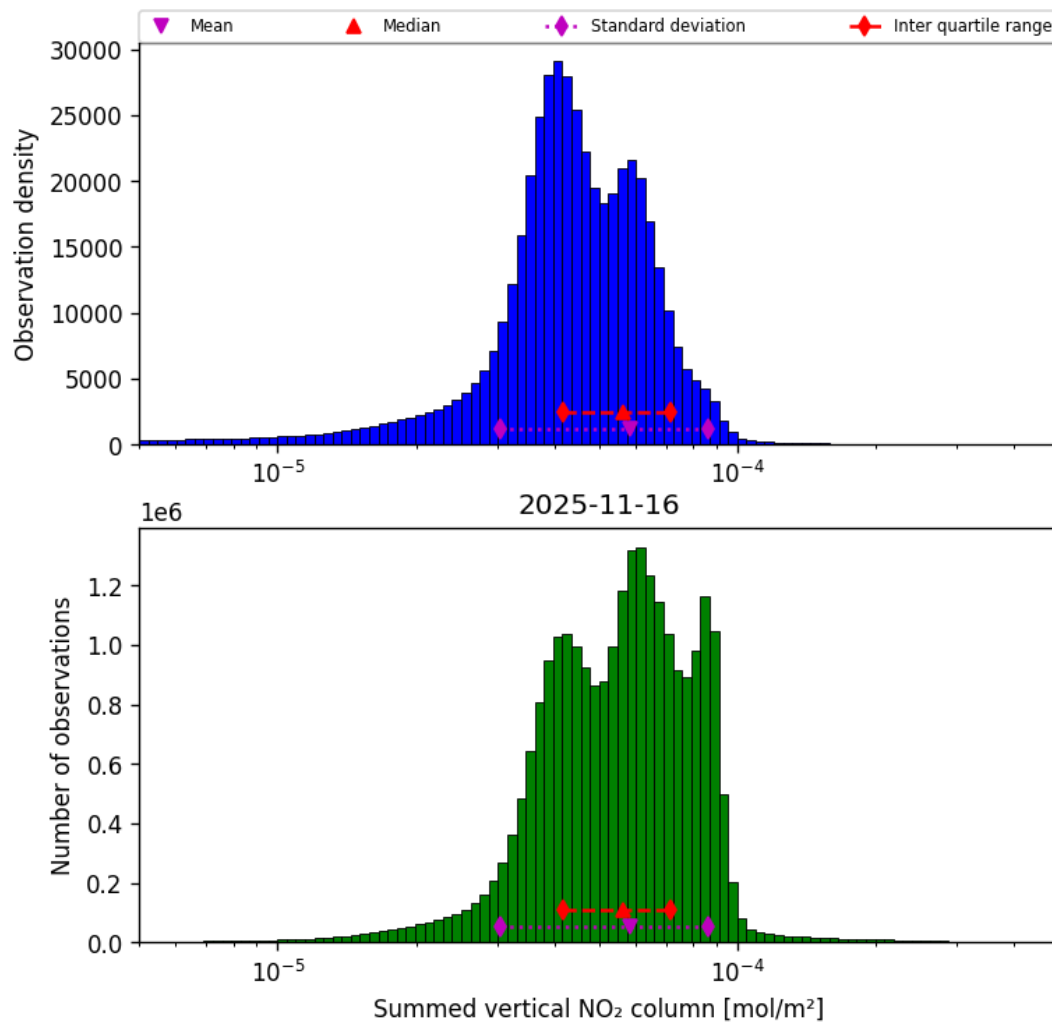
Figure 40: Histogram of “Summed vertical NO 2 column” for 2025-11-15 to 2025-11-17
