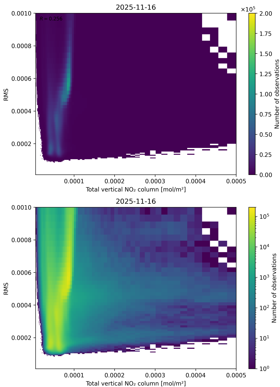
Figure 120: Scatter density plot of “Total vertical NO 2 column” against “RMS” for 2025-11-15 to 2025-11-17.
