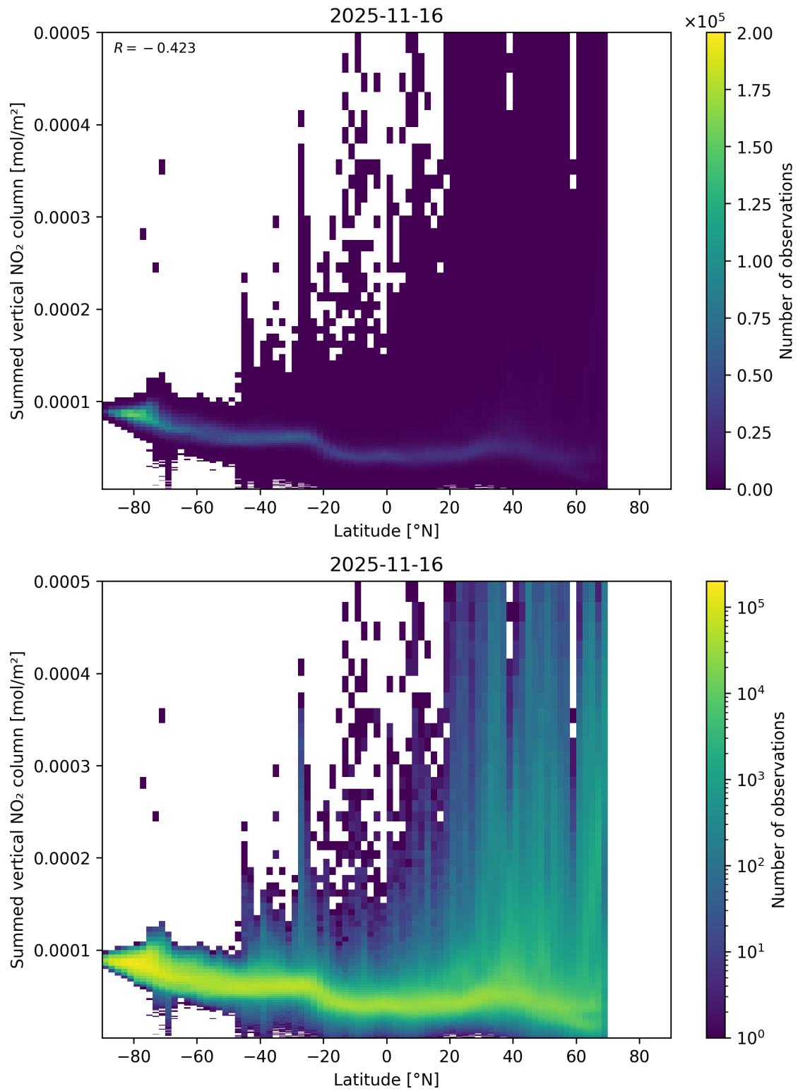
Figure 88: Scatter density plot of “Latitude” against “Summed vertical NO 2 column” for 2025-11-15 to 2025-11-17.
