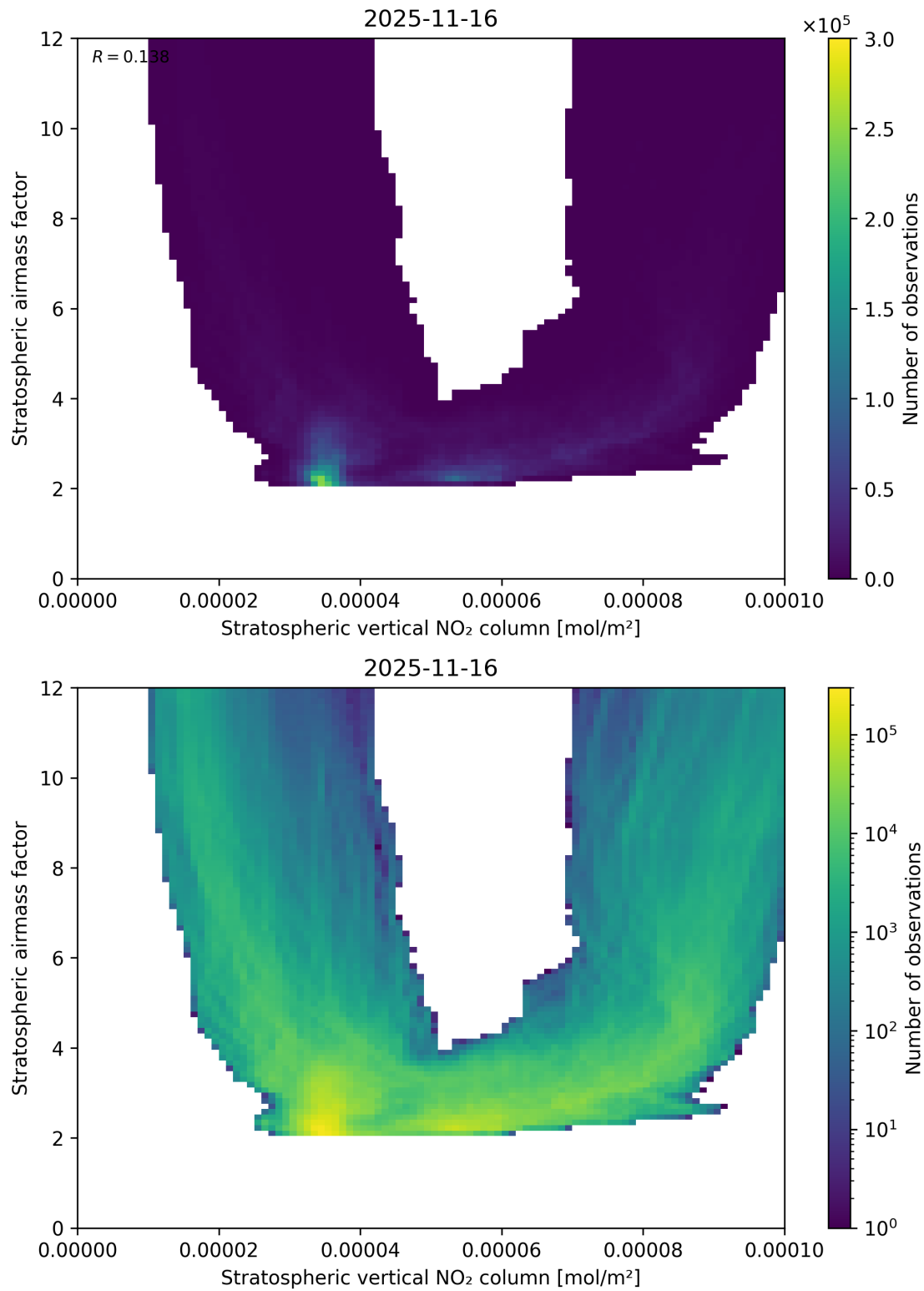
Figure 96: Scatter density plot of “Stratospheric vertical NO 2 column” against “Stratospheric airmass factor” for 2025-11-15 to 2025-11-17.
