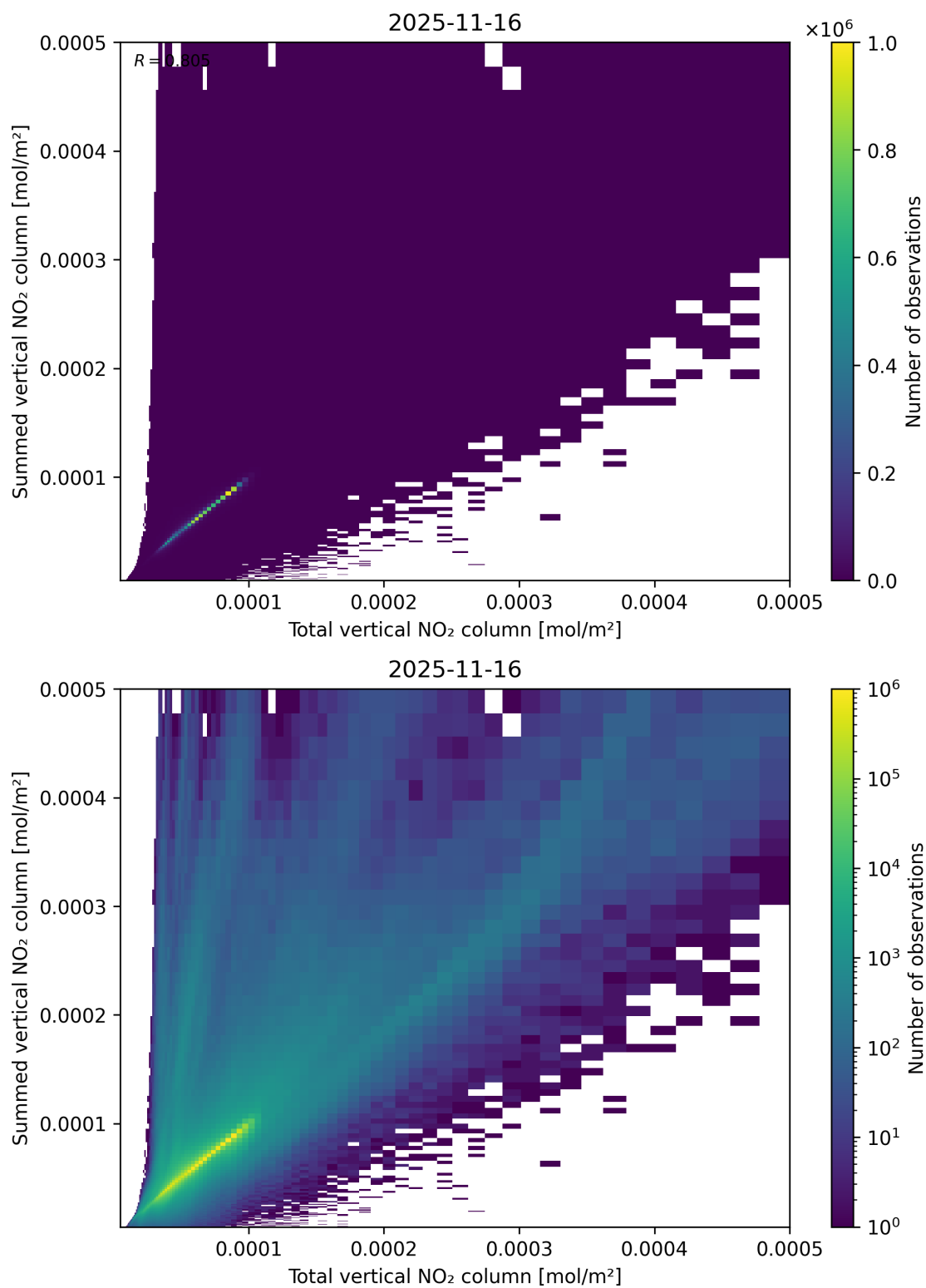
Figure 112: Scatter density plot of “Total vertical NO 2 column” against “Summed vertical NO 2 column” for 2025-11-15 to 2025-11-17.
