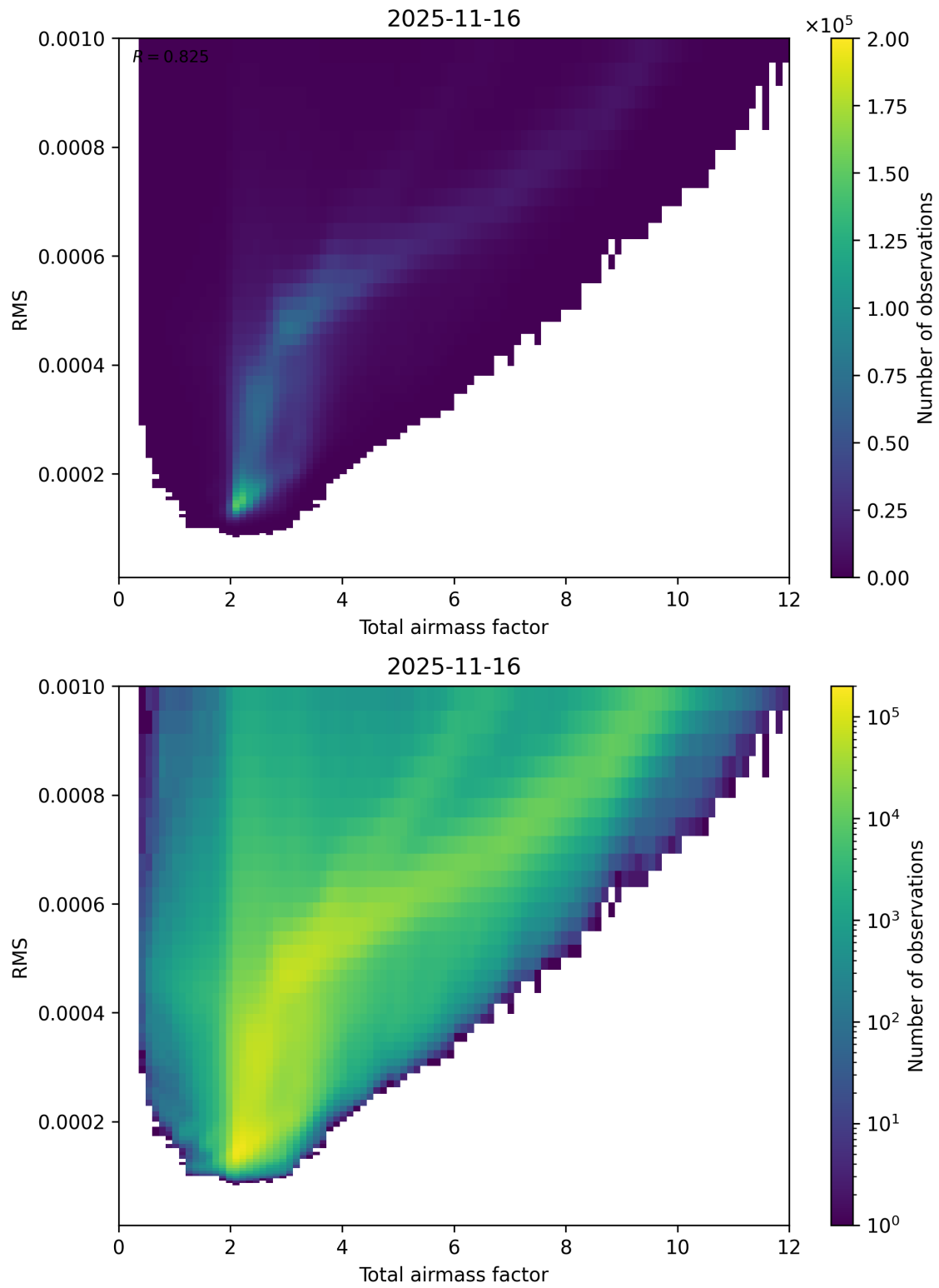
Figure 69: Scatter density plot of “Total airmass factor” against “RMS” for 2025-11-15 to 2025-11-17.
