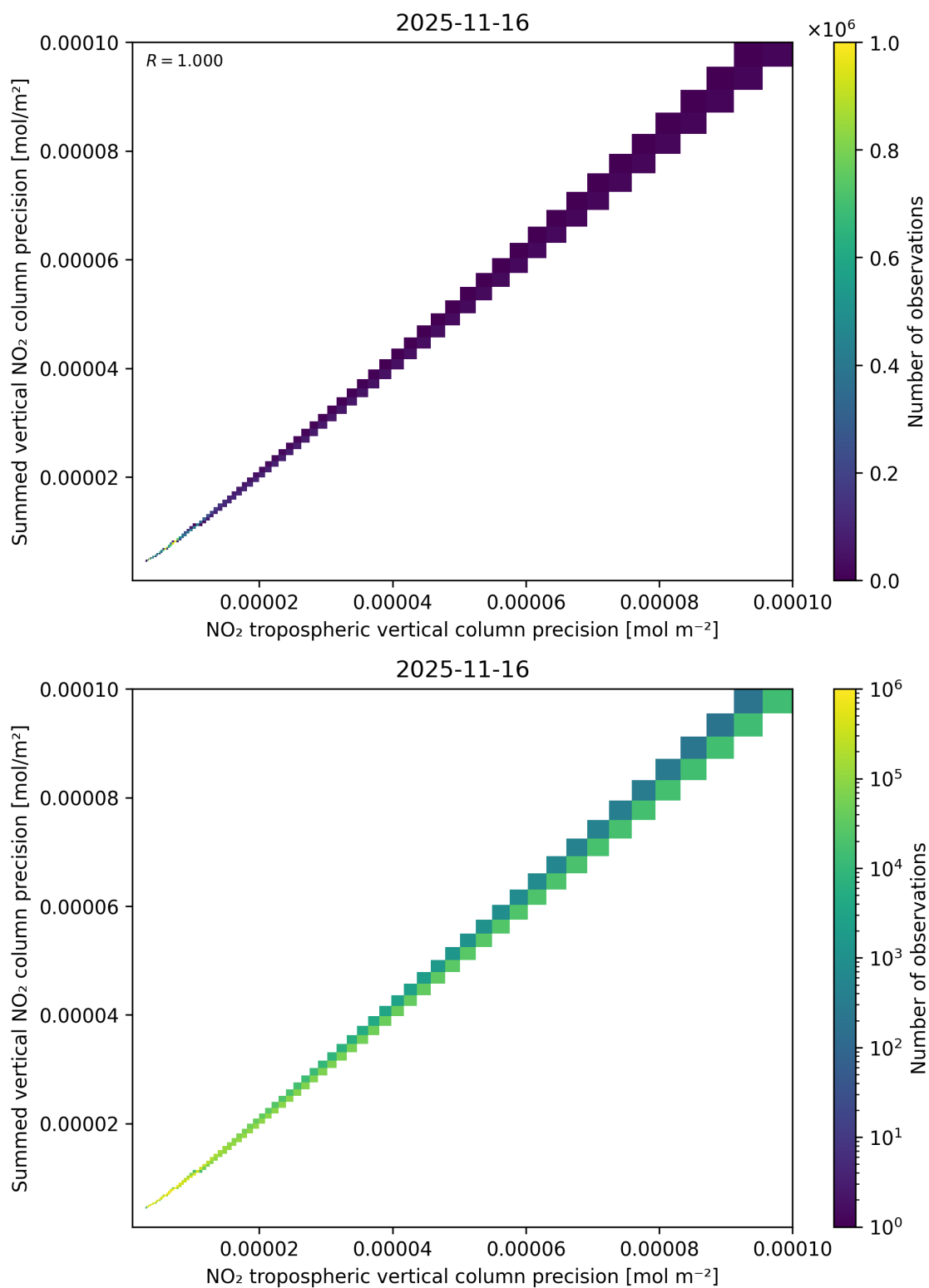
Figure 137: Scatter density plot of “NO 2 tropospheric vertical column precision” against “Summed vertical NO 2 column precision” for 2025-11-15 to 2025-11-17.
