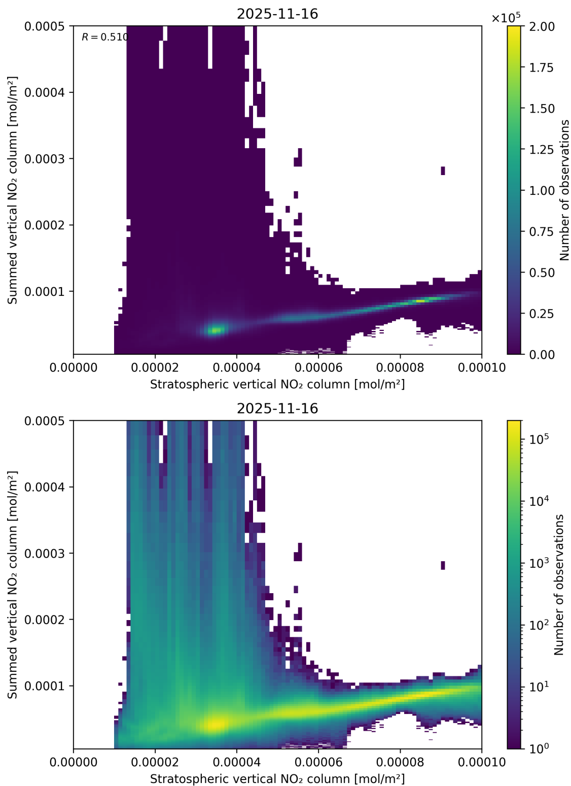
Figure 98: Scatter density plot of “Stratospheric vertical NO 2 column” against “Summed vertical NO 2 column” for 2025-11-15 to 2025-11-17.
