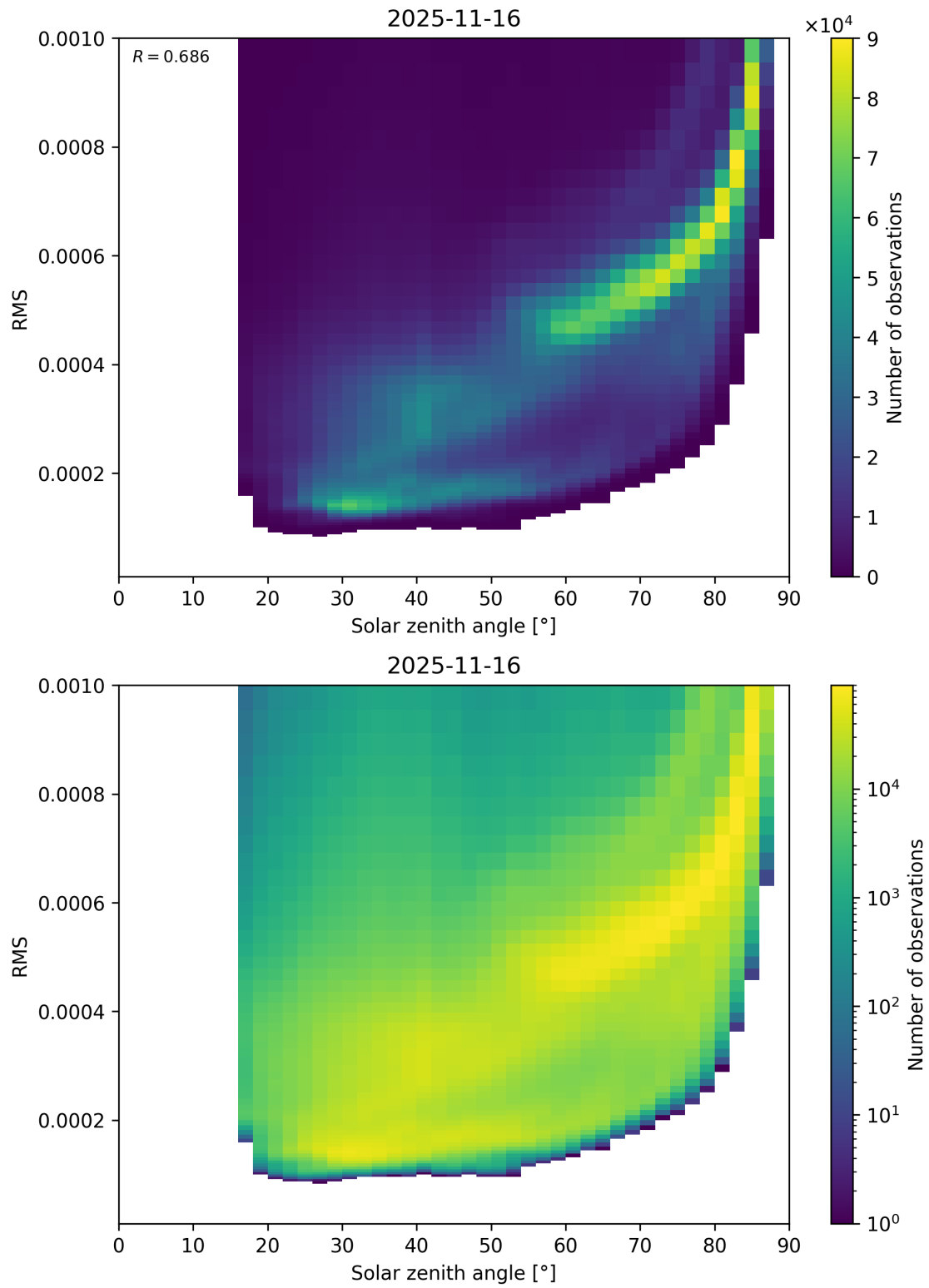
Figure 157: Scatter density plot of “Solar zenith angle” against “RMS” for 2025-11-15 to 2025-11-17.
