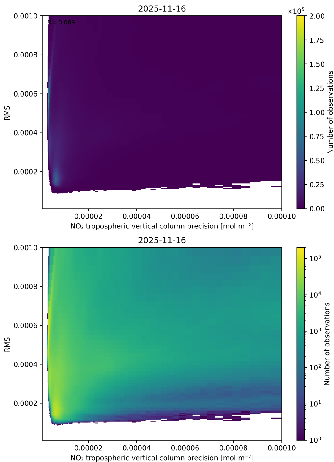
Figure 140: Scatter density plot of “NO 2 tropospheric vertical column precision” against “RMS” for 2025-11-15 to 2025-11-17.
