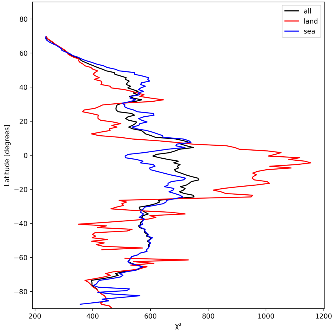
Figure 25: Zonal average of “ \chi^2 ” for 2025-11-15 to 2025-11-17.
