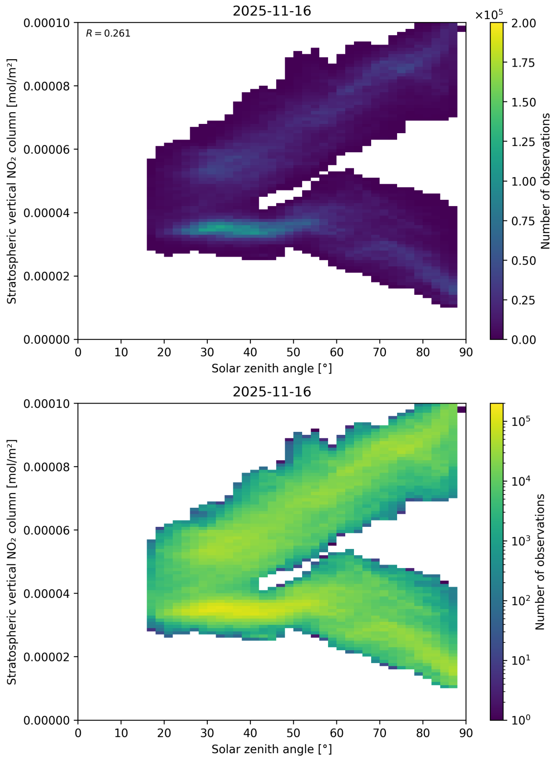
Figure 150: Scatter density plot of “Solar zenith angle” against “Stratospheric vertical NO 2 column” for 2025-11-15 to 2025-11-17.
