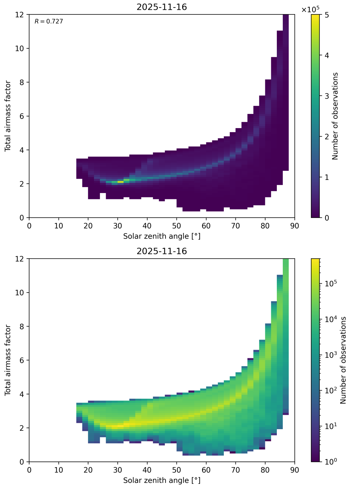
Figure 146: Scatter density plot of “Solar zenith angle” against “Total airmass factor” for 2025-11-15 to 2025-11-17.
