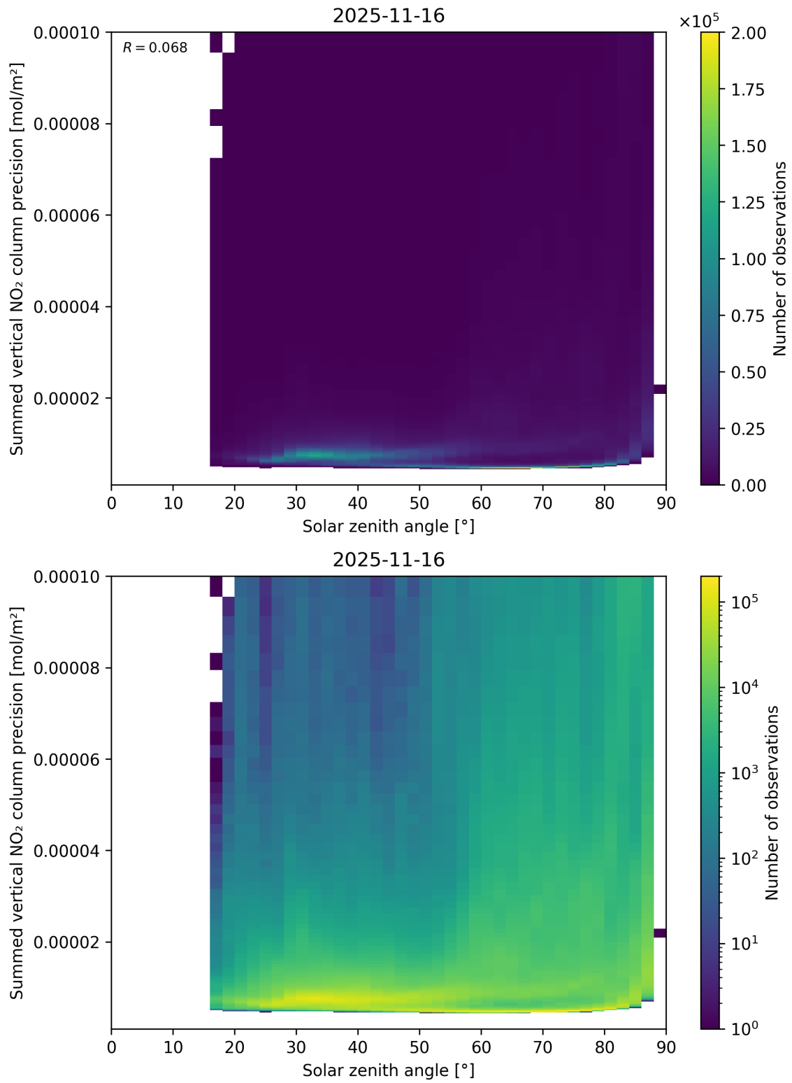
Figure 152: Scatter density plot of “Solar zenith angle” against “Summed vertical NO 2 column precision” for 2025-11-15 to 2025-11-17.
