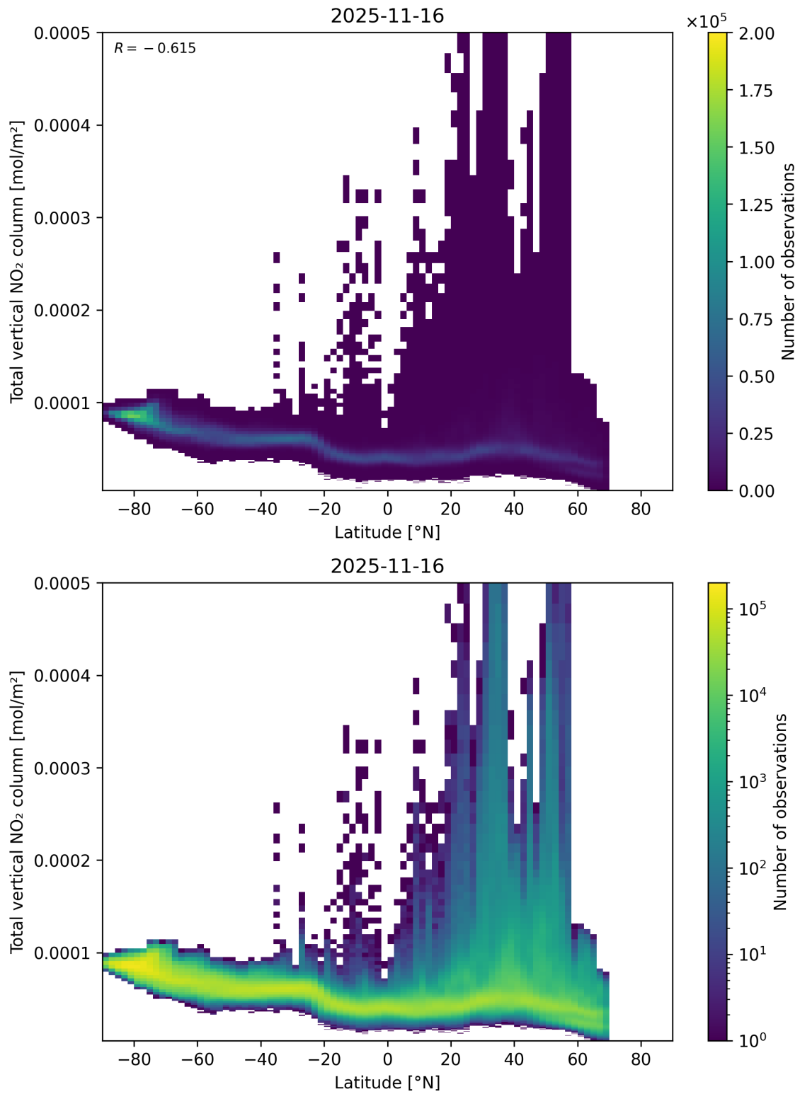
Figure 90: Scatter density plot of “Latitude” against “Total vertical NO 2 column” for 2025-11-15 to 2025-11-17.
