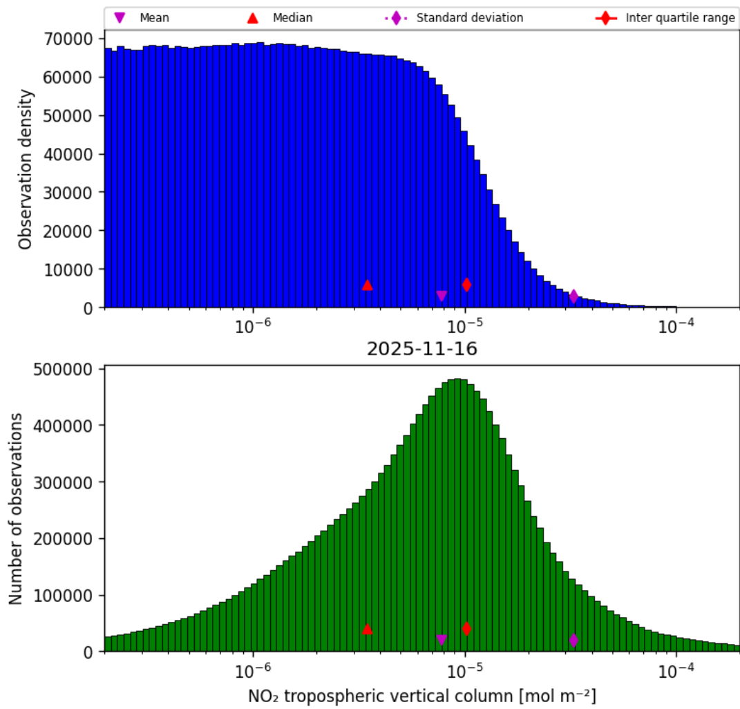
Figure 29: Histogram of “NO 2 tropospheric vertical column” for 2025-11-15 to 2025-11-17
