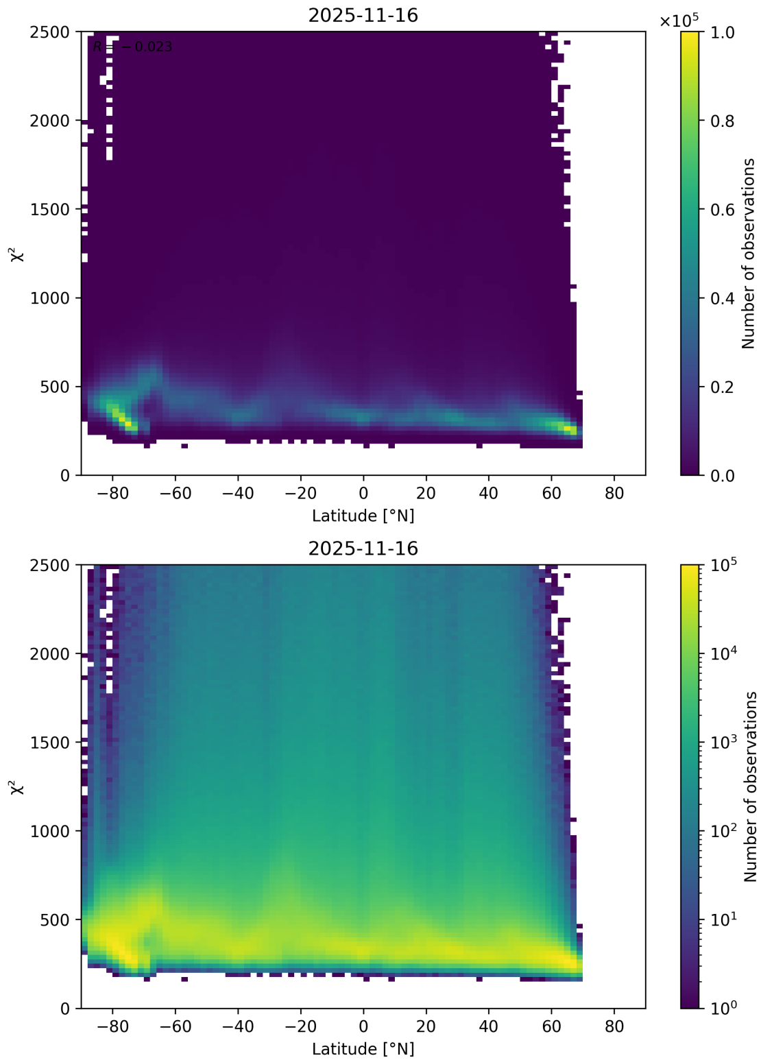
Figure 86: Scatter density plot of “Latitude” against “ \chi^2 ” for 2025-11-15 to 2025-11-17.
