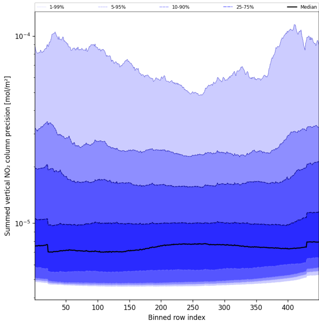
Figure 58: Along track statistics of “Summed vertical NO 2 column precision” for 2025-11-15 to 2025-11-17
