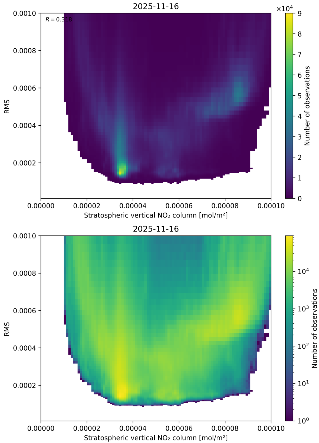
Figure 102: Scatter density plot of “Stratospheric vertical NO 2 column” against “RMS” for 2025-11-15 to 2025-11-17.
