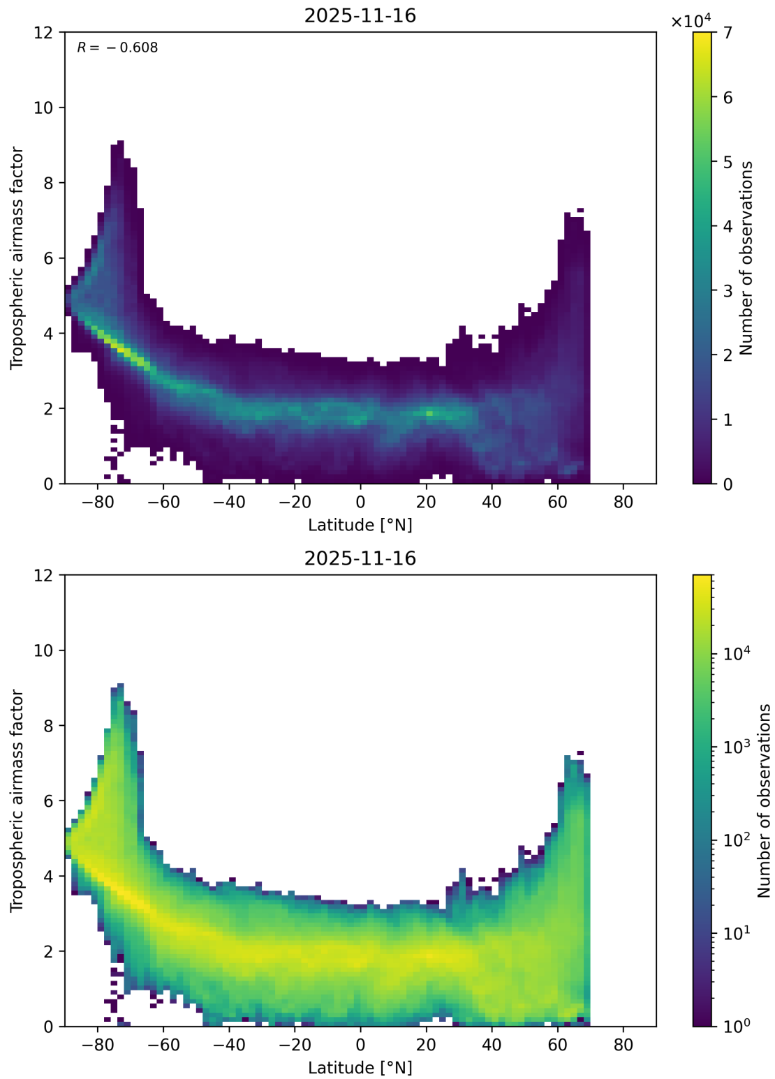
Figure 85: Scatter density plot of “Latitude” against “Tropospheric airmass factor” for 2025-11-15 to 2025-11-17.
