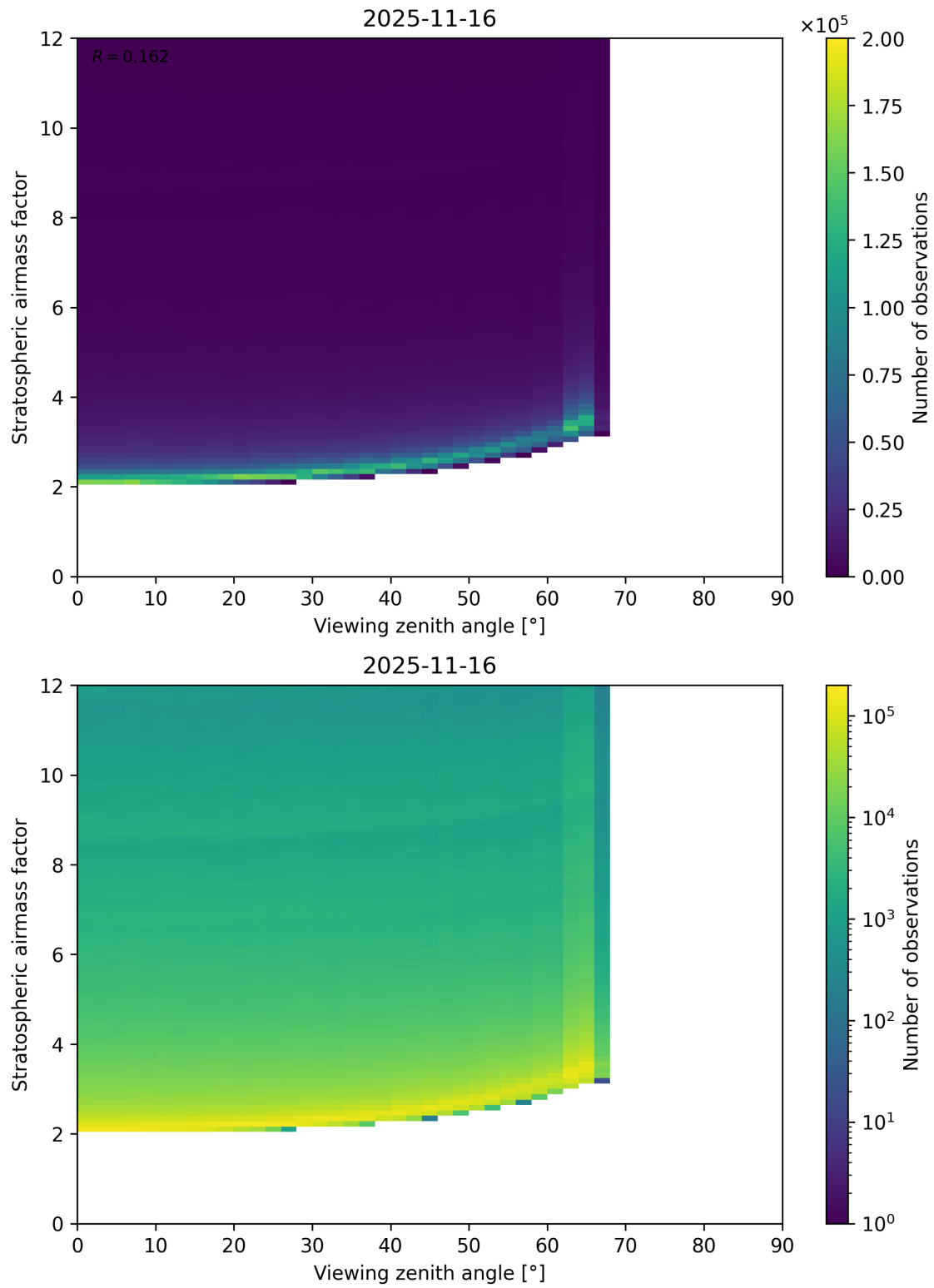
Figure 159: Scatter density plot of “Viewing zenith angle” against “Stratospheric airmass factor” for 2025-11-15 to 2025-11-17.
