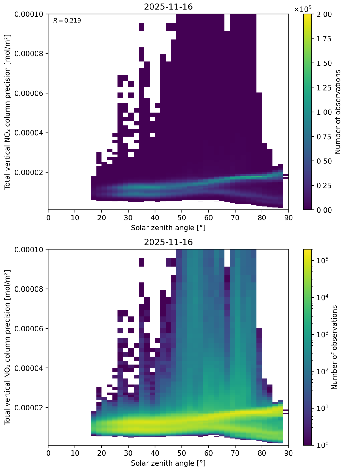
Figure 154: Scatter density plot of “Solar zenith angle” against “Total vertical NO 2 column precision” for 2025-11-15 to 2025-11-17.
