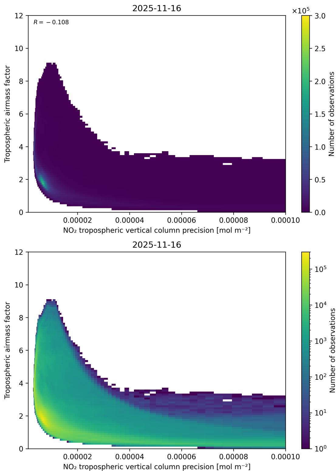
Figure 133: Scatter density plot of “NO 2 tropospheric vertical column precision” against “Tropospheric air mass factor” for 2025-11-15 to 2025-11-17.
