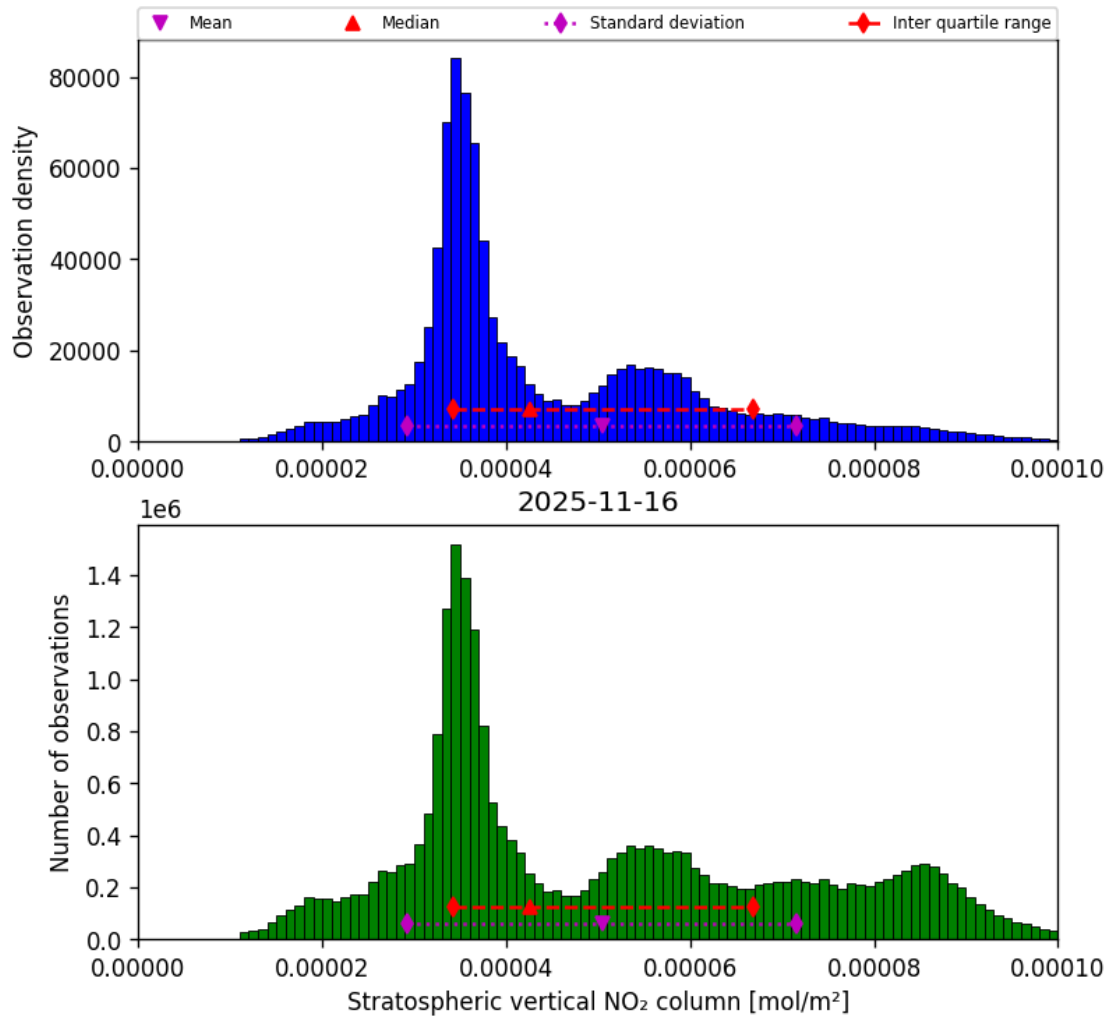
Figure 36: Histogram of “Stratospheric vertical NO 2 column” for 2025-11-15 to 2025-11-17
