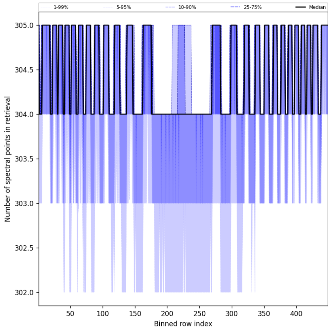
Figure 50: Along track statistics of “Number of spectral points in retrieval” for 2025-11-15 to 2025-11-17
