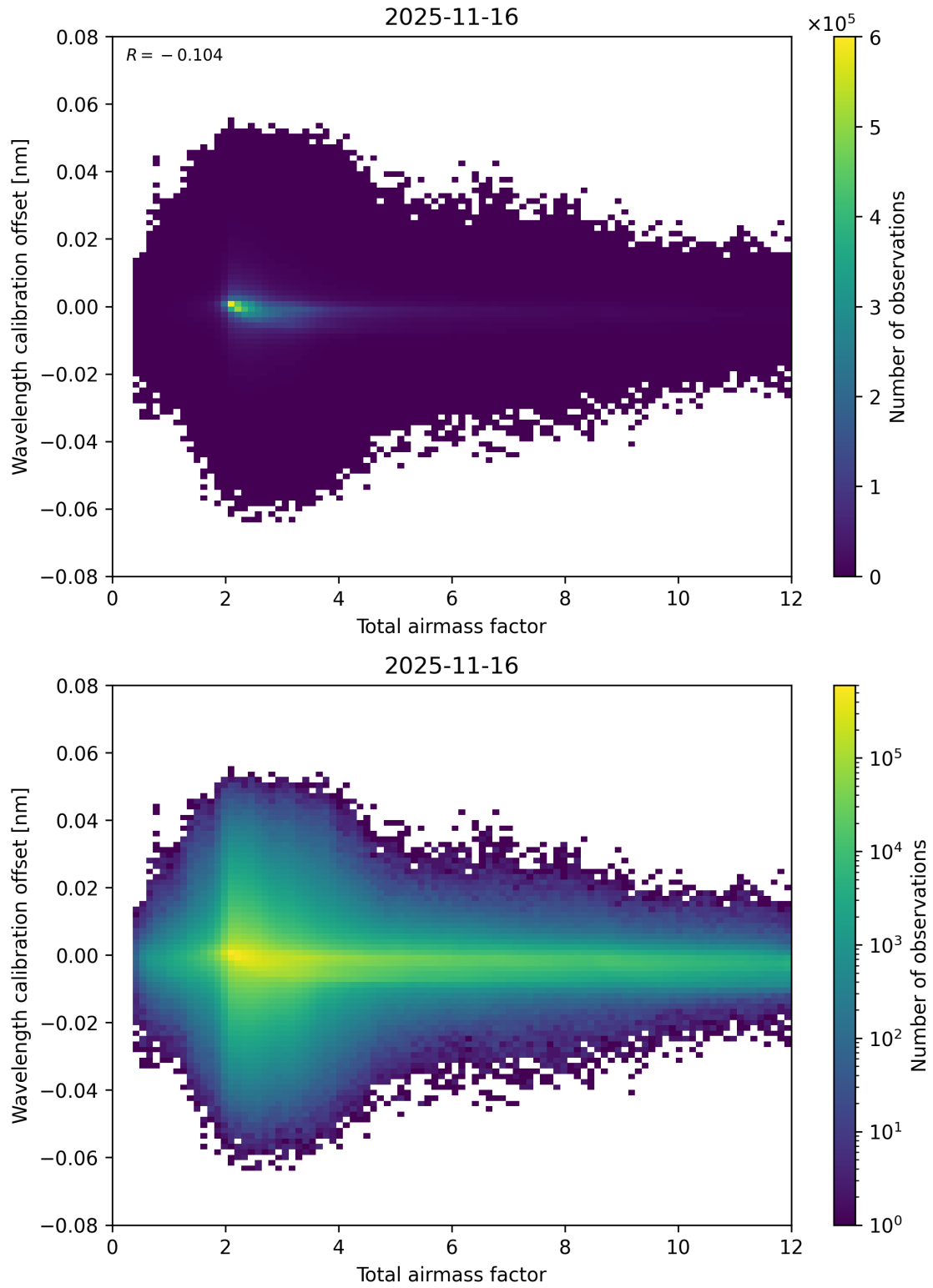
Figure 70: Scatter density plot of “Total airmass factor” against “Wavelength calibration offset” for 2025-11-15 to 2025-11-17.
