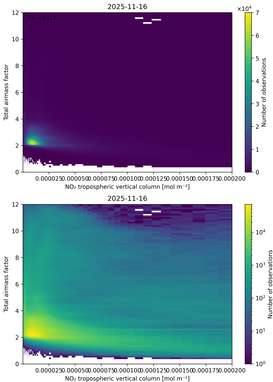
Figure 122: Scatter density plot of “NO 2 tropospheric vertical column” against “Total airmass factor” for 2025-11-15 to 2025-11-17.
