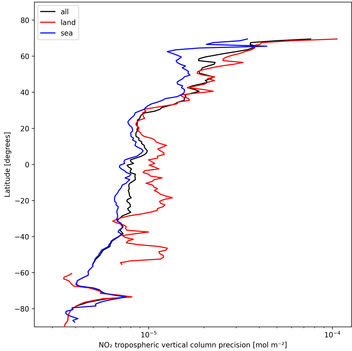
Figure 13: Zonal average of “NO 2 tropospheric vertical column precision” for 2025-11-15 to 2025-11-17.
