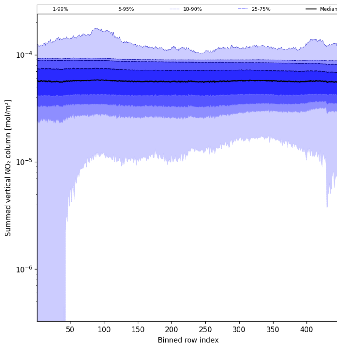
Figure 57: Along track statistics of “Summed vertical NO 2 column” for 2025-11-15 to 2025-11-17
