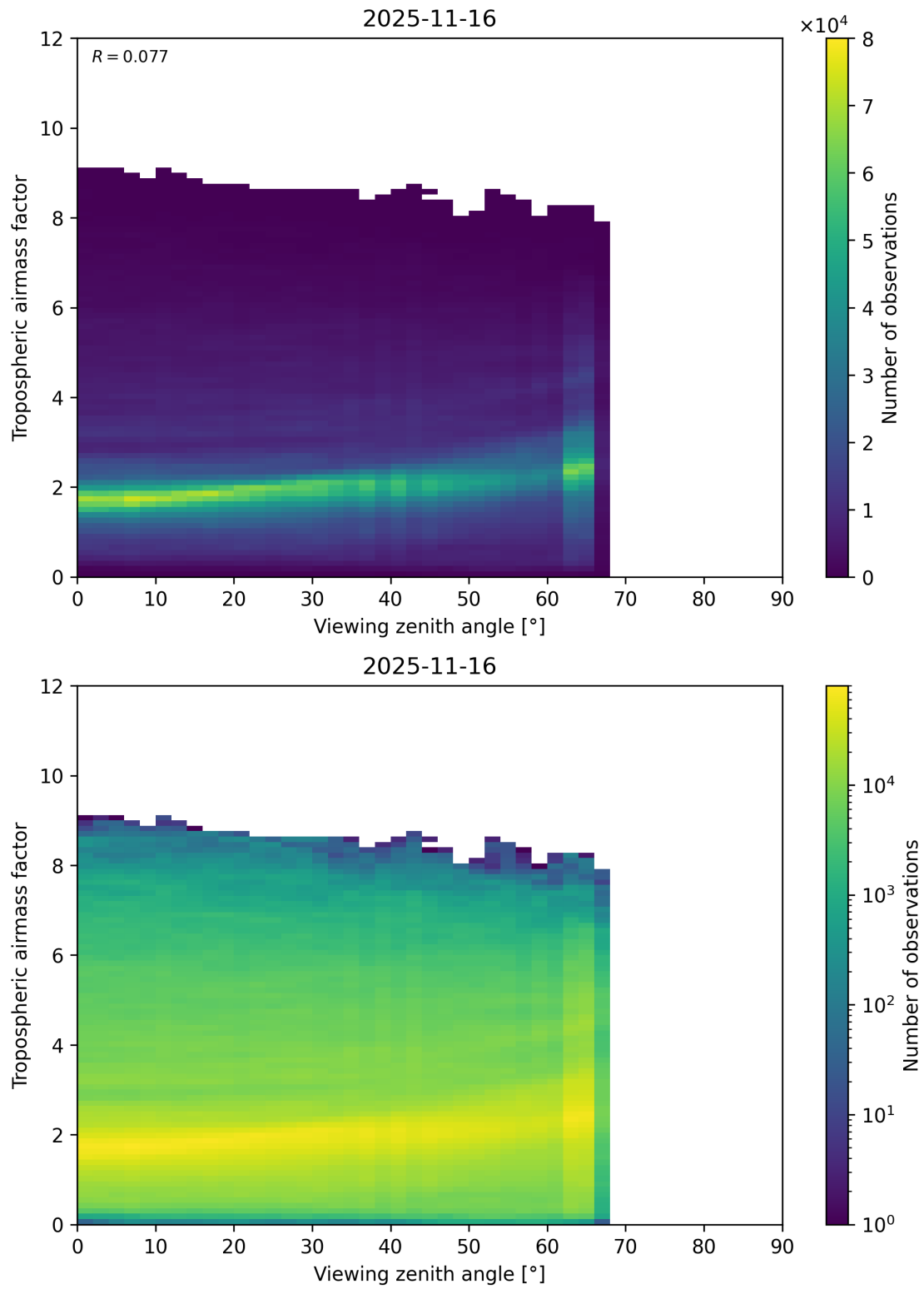
Figure 161: Scatter density plot of “Viewing zenith angle” against “Tropospheric airmass factor” for 2025-11-15 to 2025-11-17.
