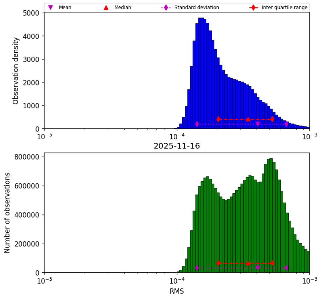
Figure 43: Histogram of “RMS” for 2025-11-15 to 2025-11-17
