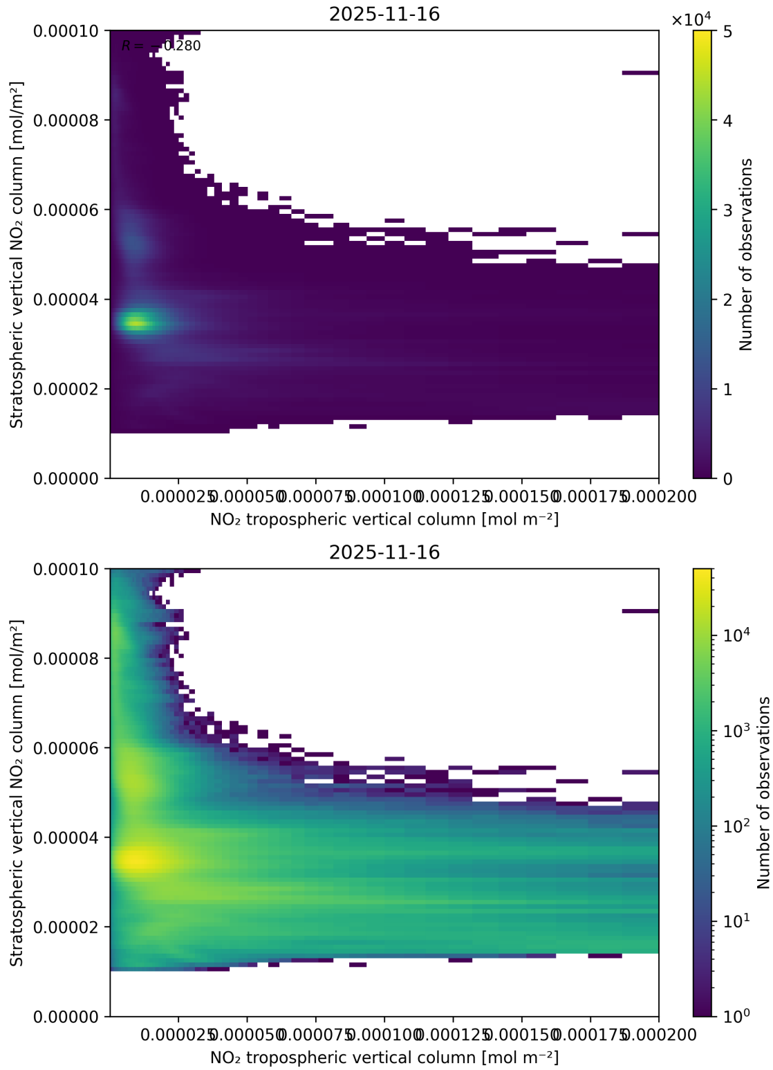
Figure 125: Scatter density plot of “NO 2 tropospheric vertical column” against “Stratospheric vertical NO 2 column” for 2025-11-15 to 2025-11-17.
