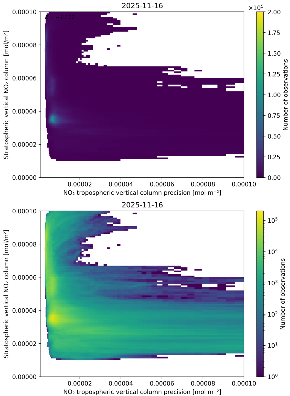
Figure 135: Scatter density plot of “NO 2 tropospheric vertical column precision” against “Stratospheric vertical NO 2 column” for 2025-11-15 to 2025-11-17.
