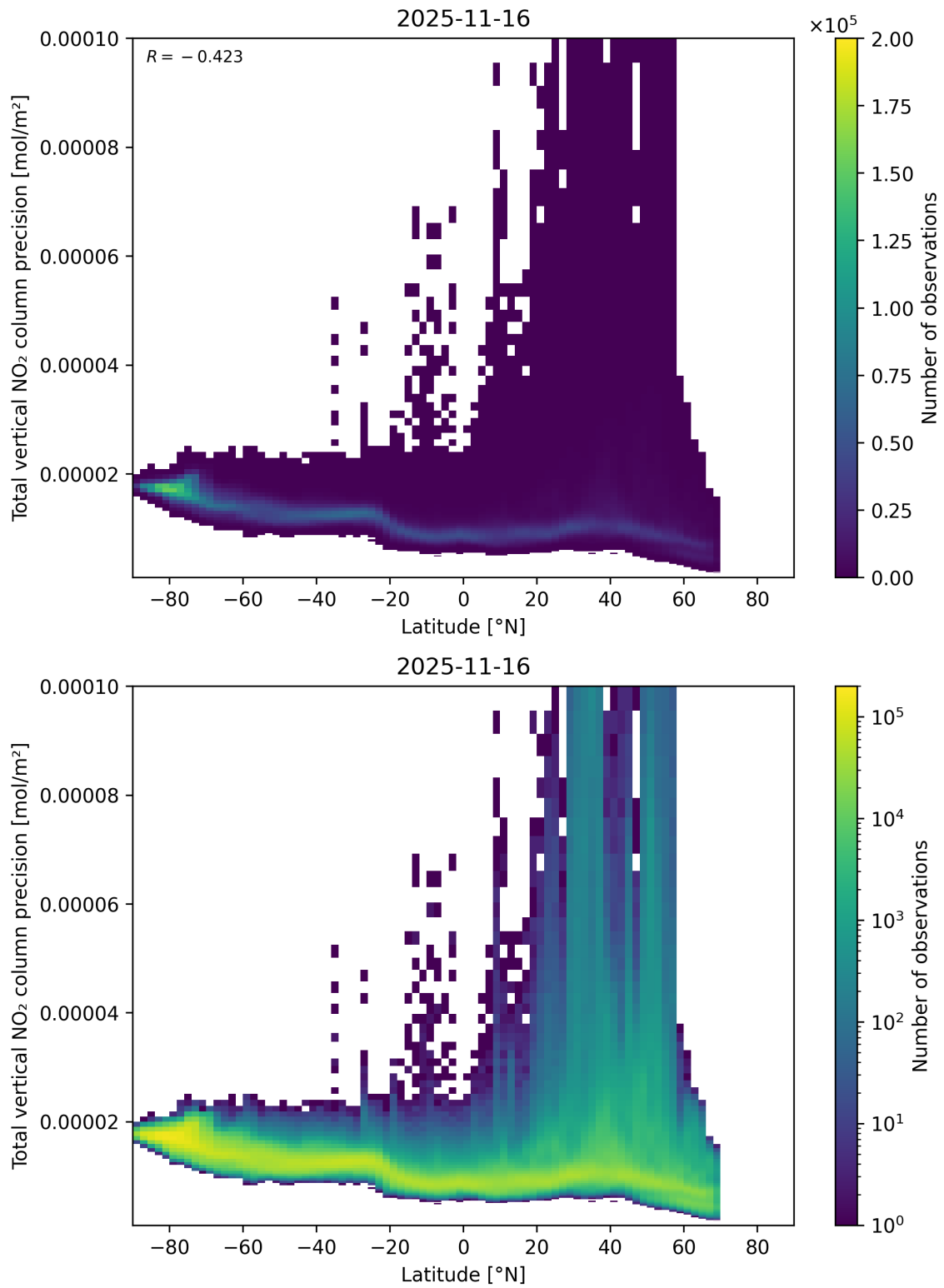
Figure 91: Scatter density plot of “Latitude” against “Total vertical NO 2 column precision” for 2025-11-15 to 2025-11-17.
