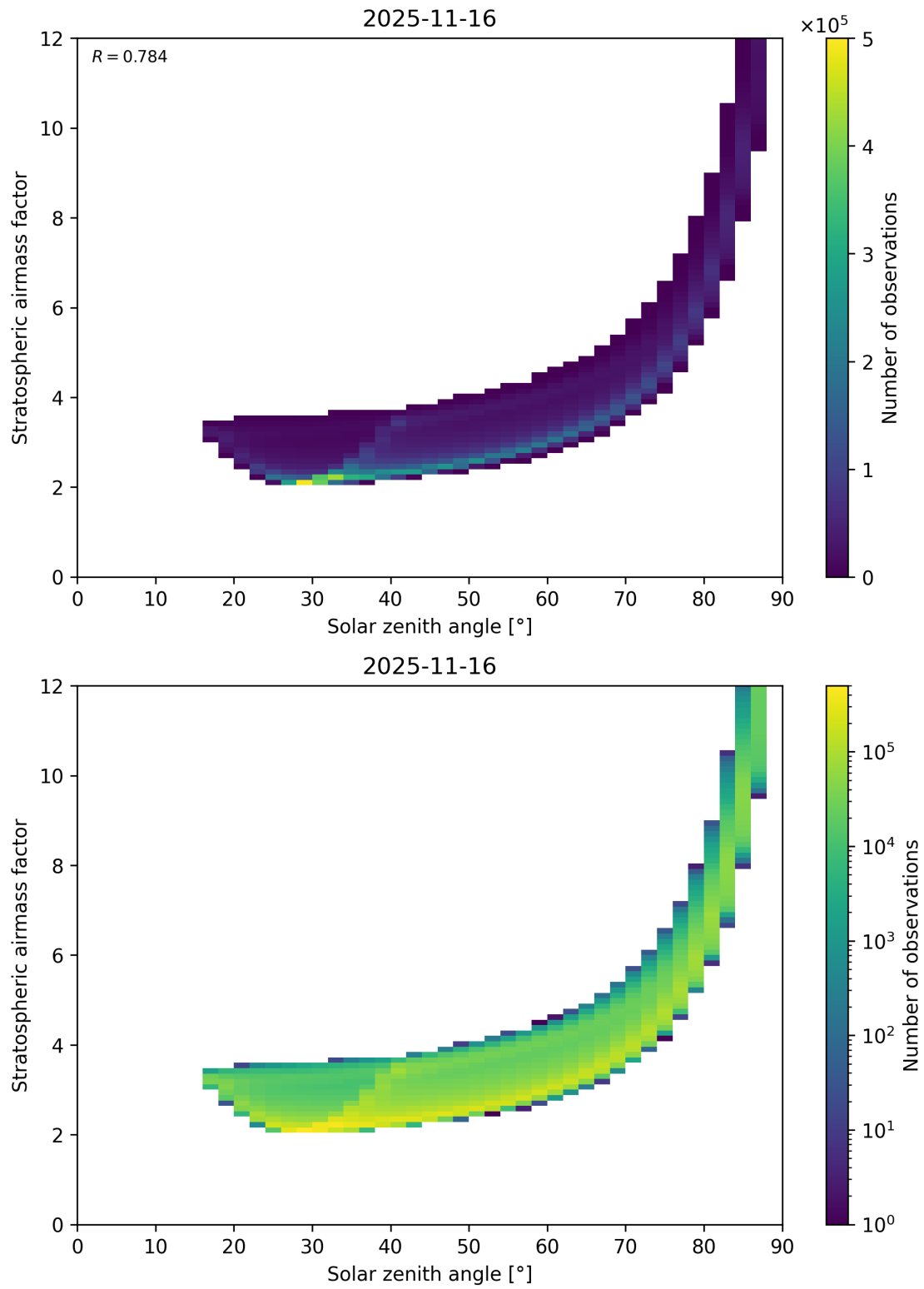
Figure 145: Scatter density plot of “Solar zenith angle” against “Stratospheric airmass factor” for 2025-11-15 to 2025-11-17.
