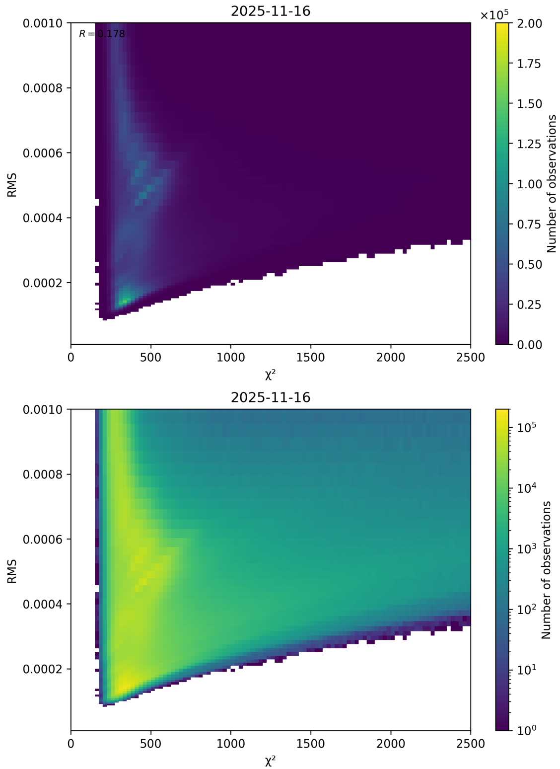
Figure 82: Scatter density plot of “ \chi^2 ” against “RMS” for 2025-11-15 to 2025-11-17.
