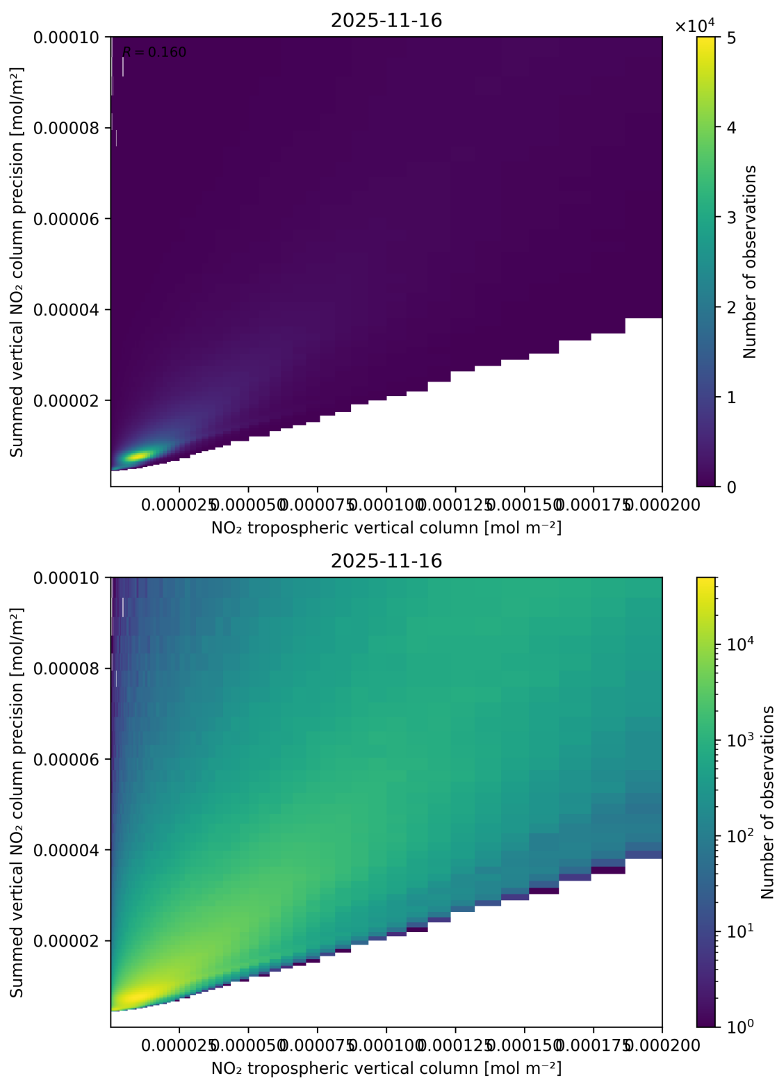
Figure 127: Scatter density plot of “NO 2 tropospheric vertical column” against “Summed vertical NO 2 column precision” for 2025-11-15 to 2025-11-17.
