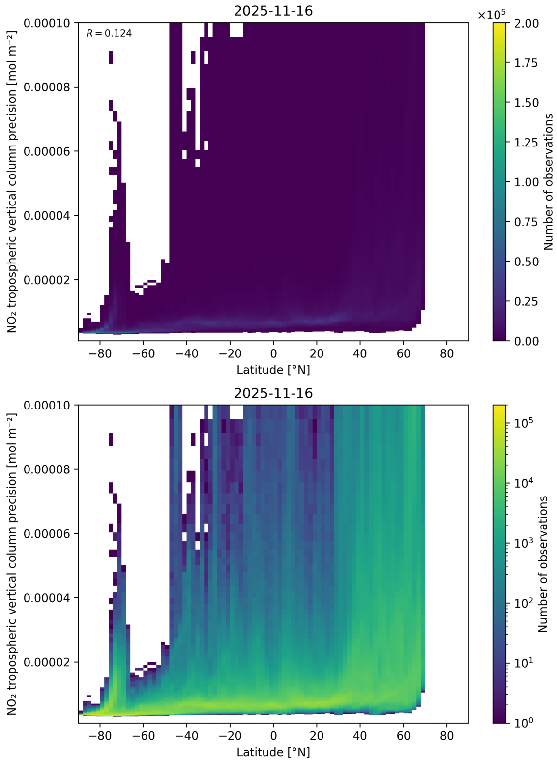
Figure 93: Scatter density plot of “Latitude” against “NO 2 tropospheric vertical column precision” for 2025-11-15 to 2025-11-17.
