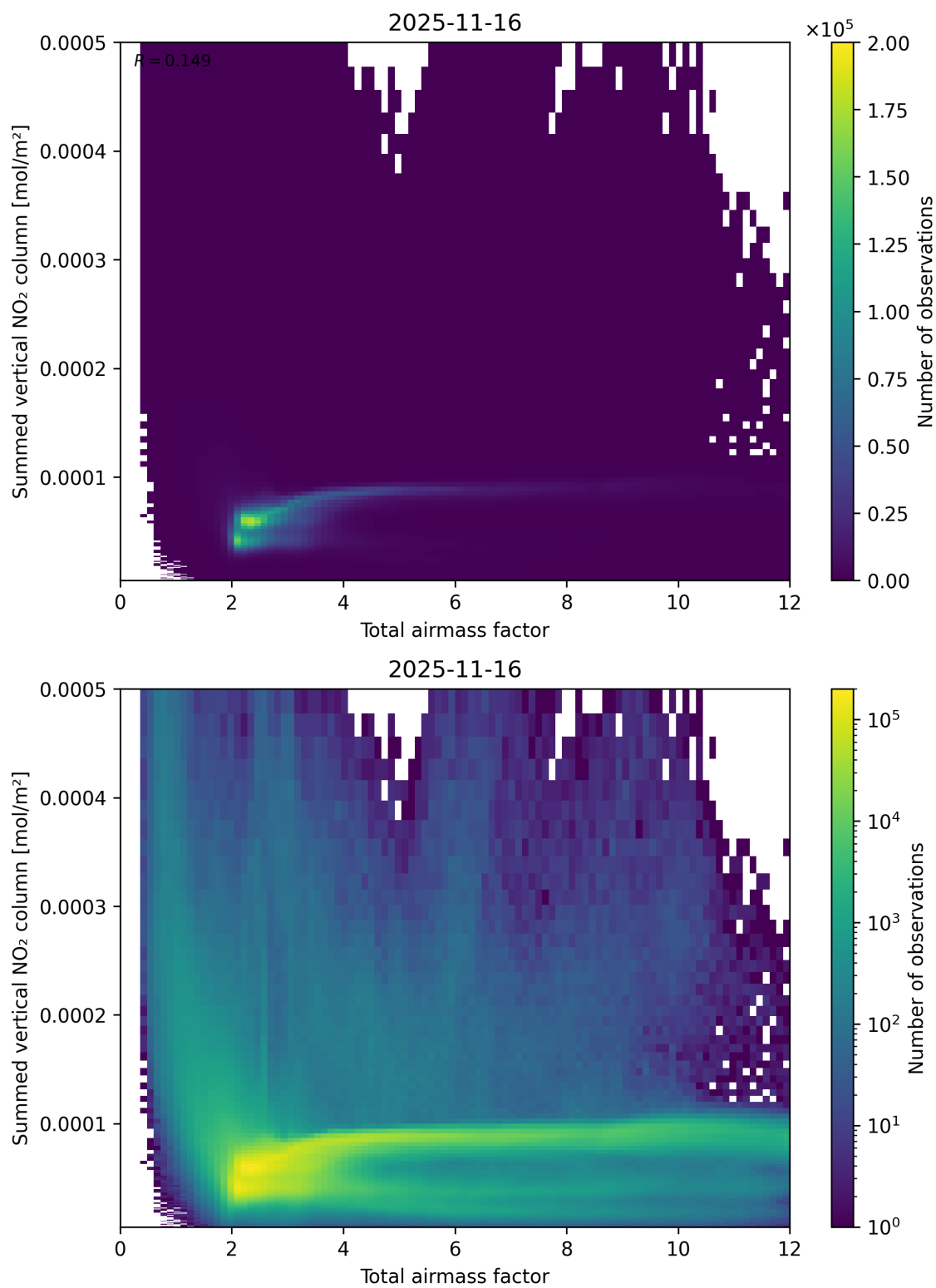
Figure 65: Scatter density plot of “Total airmass factor” against “Summed vertical NO 2 column” for 2025-11-15 to 2025-11-17.
