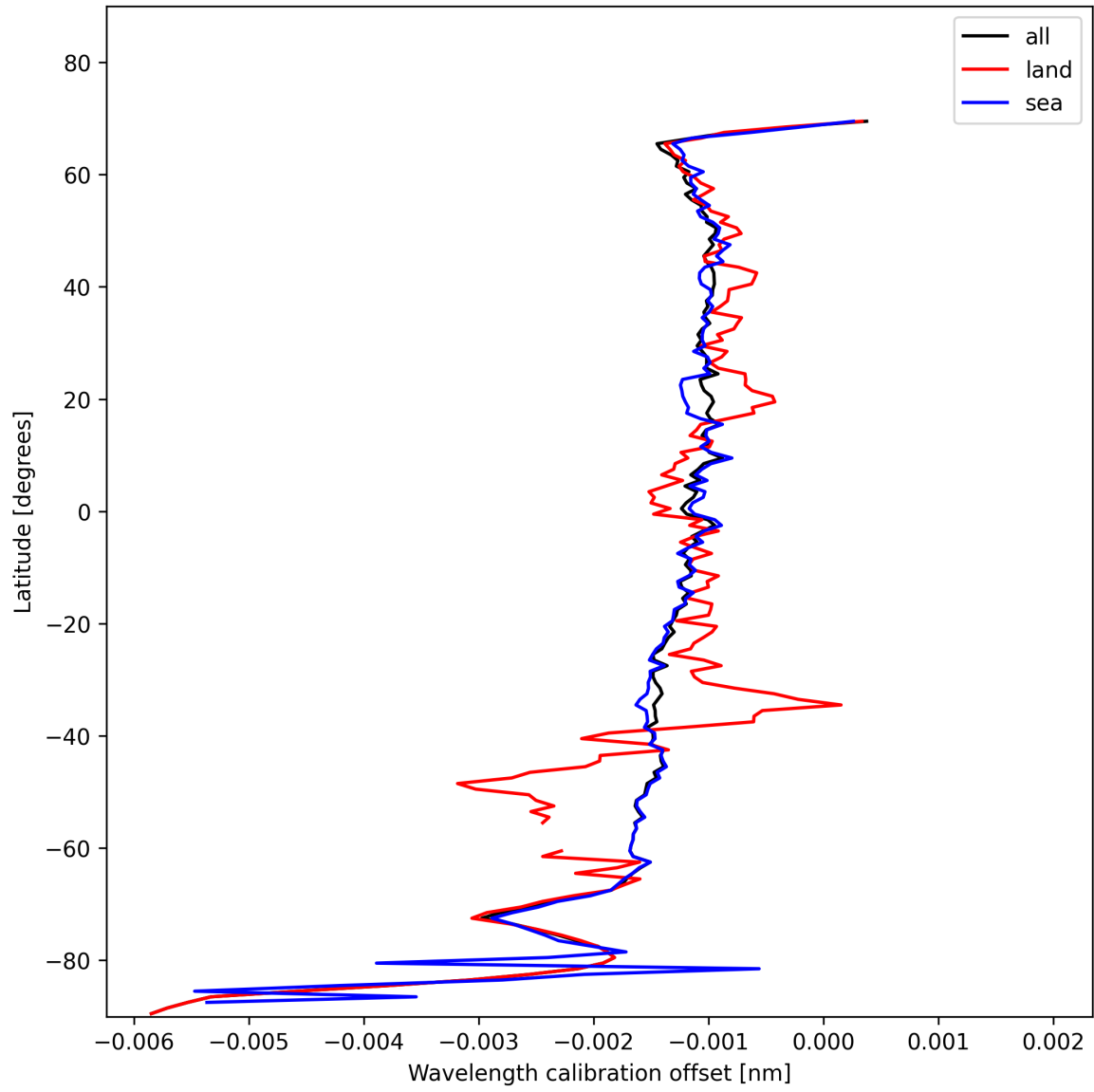
Figure 18: Zonal average of “Wavelength calibration offset” for 2025-11-15 to 2025-11-17.
