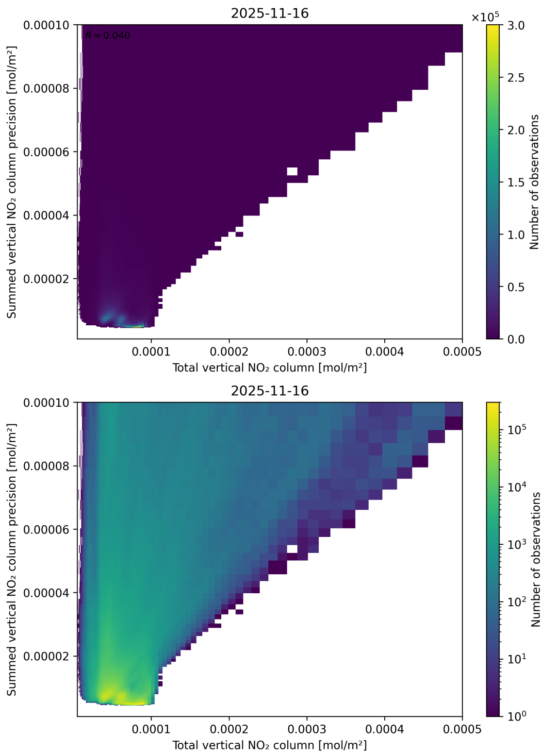
Figure 113: Scatter density plot of “Total vertical NO 2 column” against “Summed vertical NO 2 column precision” for 2025-11-15 to 2025-11-17.
