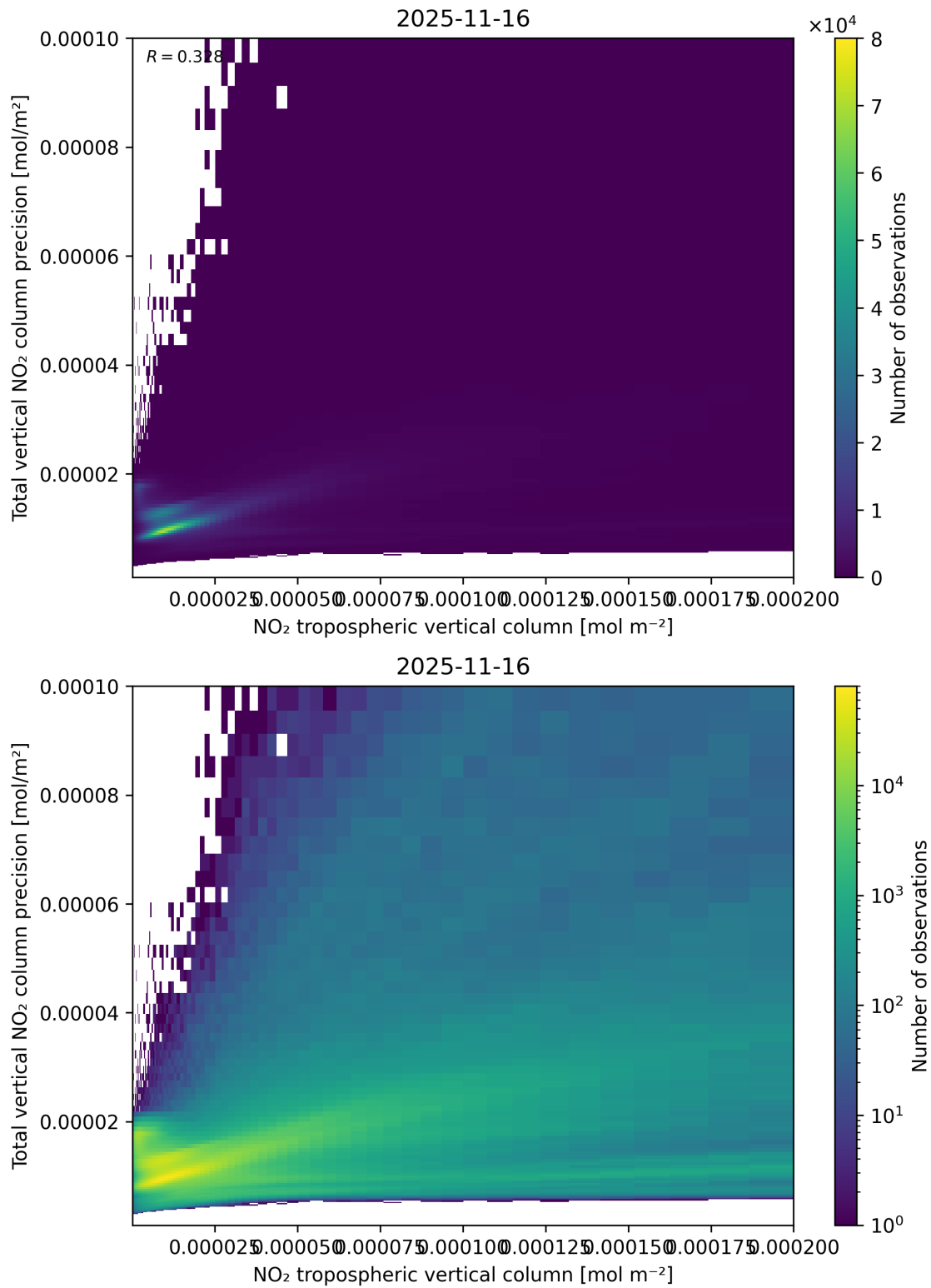
Figure 129: Scatter density plot of “NO 2 tropospheric vertical column” against “Total vertical NO 2 column precision” for 2025-11-15 to 2025-11-17.
