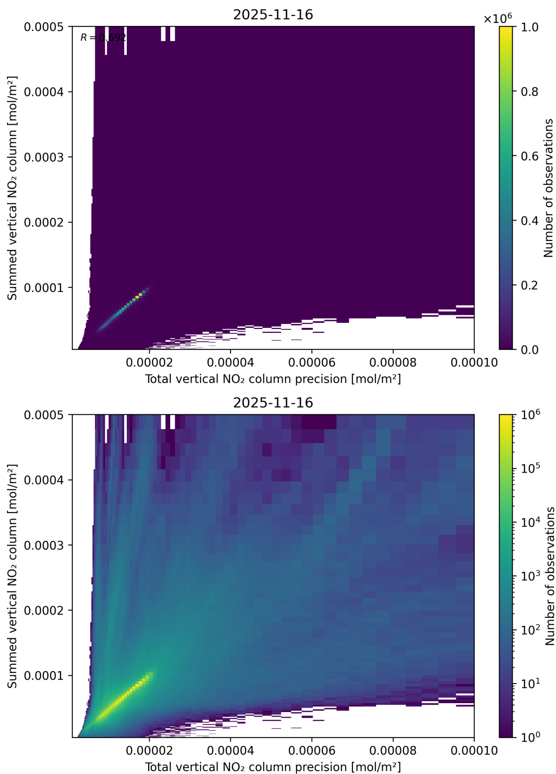
Figure 117: Scatter density plot of “Total vertical NO 2 column precision” against “Summed vertical NO 2 column” for 2025-11-15 to 2025-11-17.
