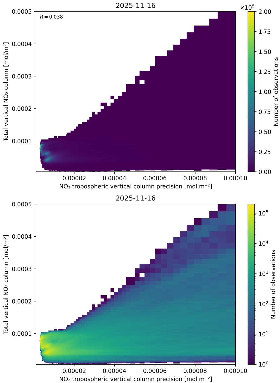
Figure 138: Scatter density plot of “NO 2 tropospheric vertical column precision” against “Total vertical NO 2 column” for 2025-11-15 to 2025-11-17.
