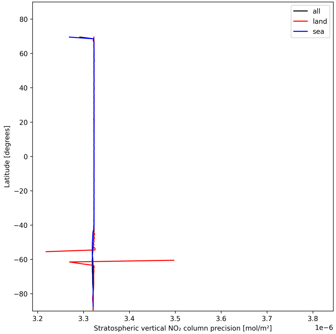
Figure 20: Zonal average of “Stratospheric vertical NO 2 column precision” for 2025-11-15 to 2025-11-17.
