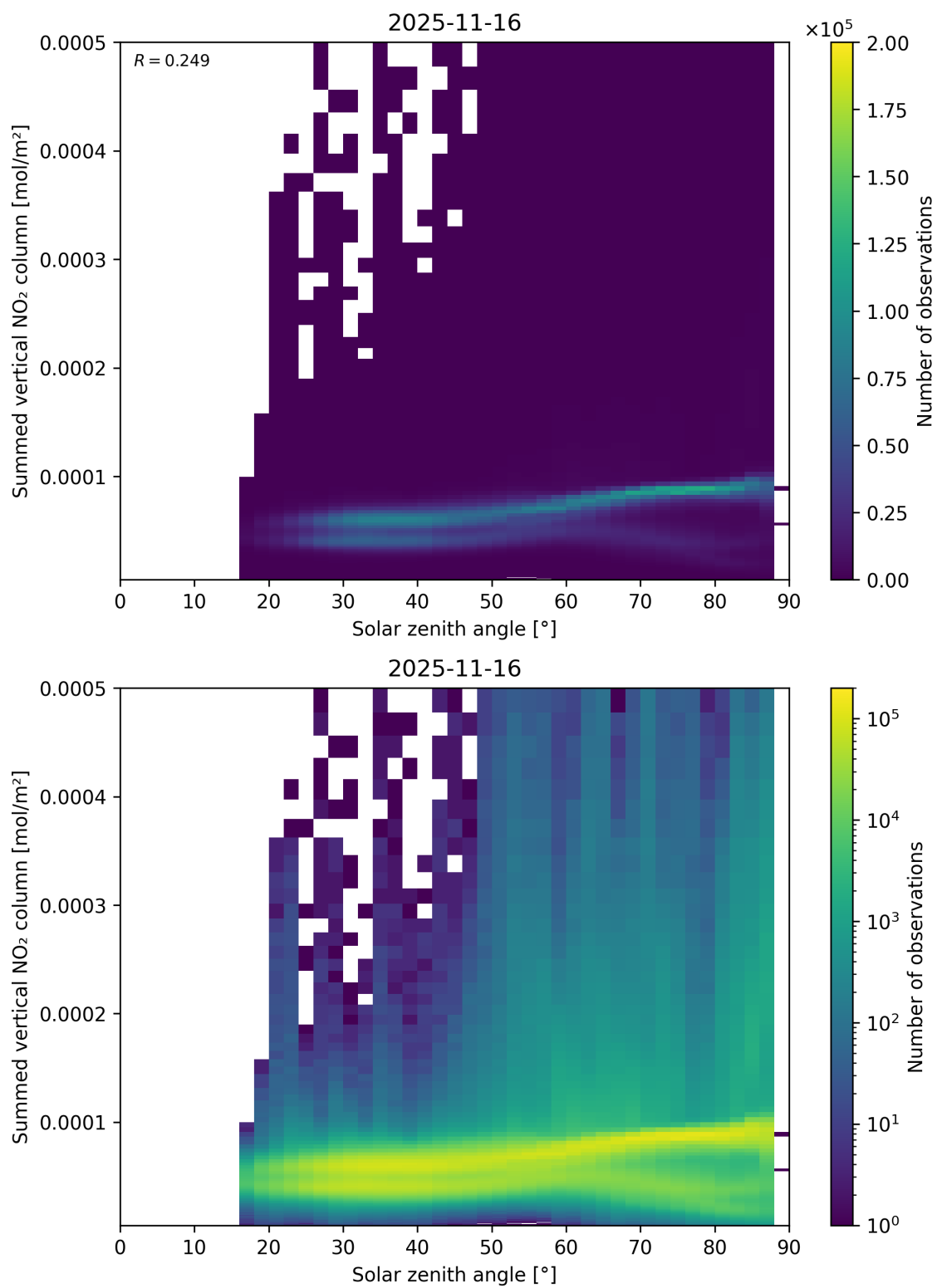
Figure 151: Scatter density plot of “Solar zenith angle” against “Summed vertical NO 2 column” for 2025-11-15 to 2025-11-17.
