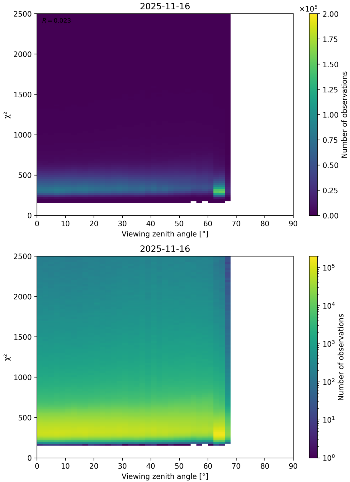
Figure 162: Scatter density plot of “Viewing zenith angle” against “ \chi^2 ” for 2025-11-15 to 2025-11-17.
