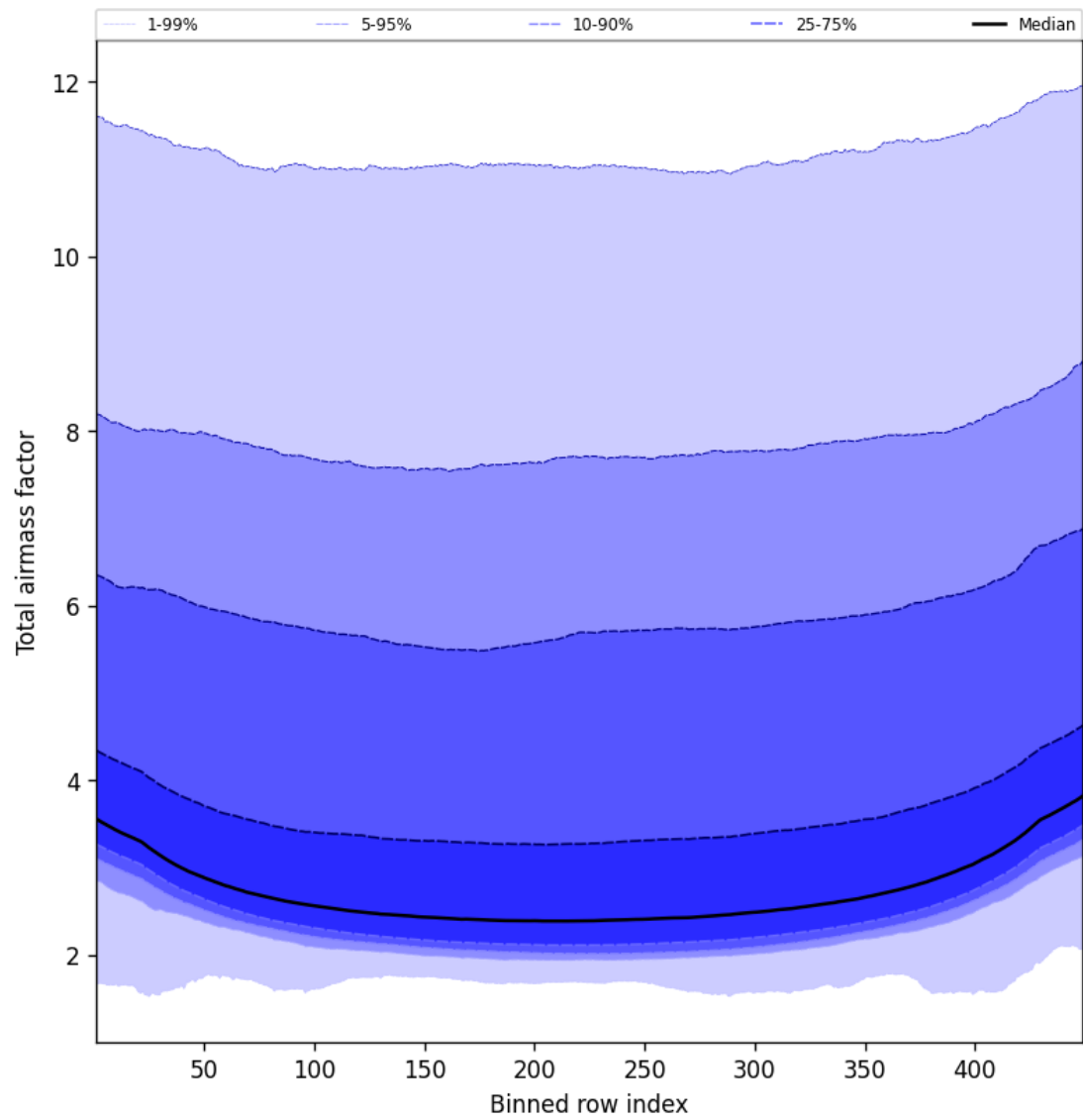
Figure 49: Along track statistics of “Total airmass factor” for 2025-11-15 to 2025-11-17
