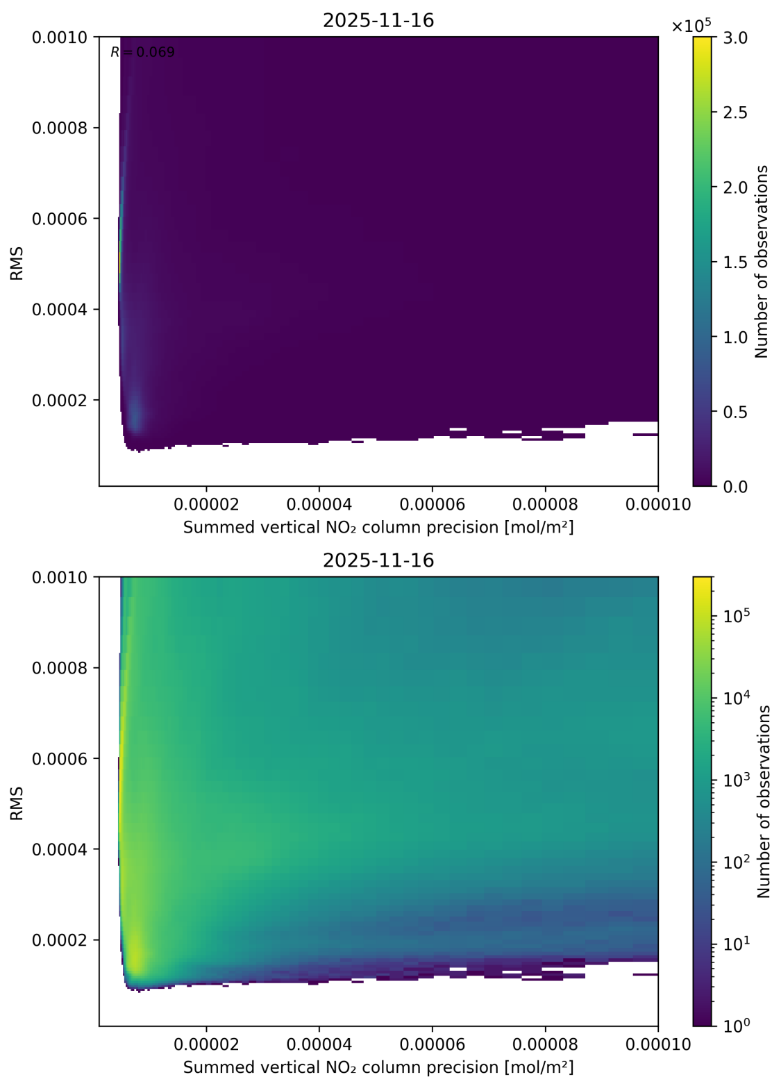
Figure 108: Scatter density plot of “Summed vertical NO 2 column precision” against “RMS” for 2025-11-15 to 2025-11-17.
