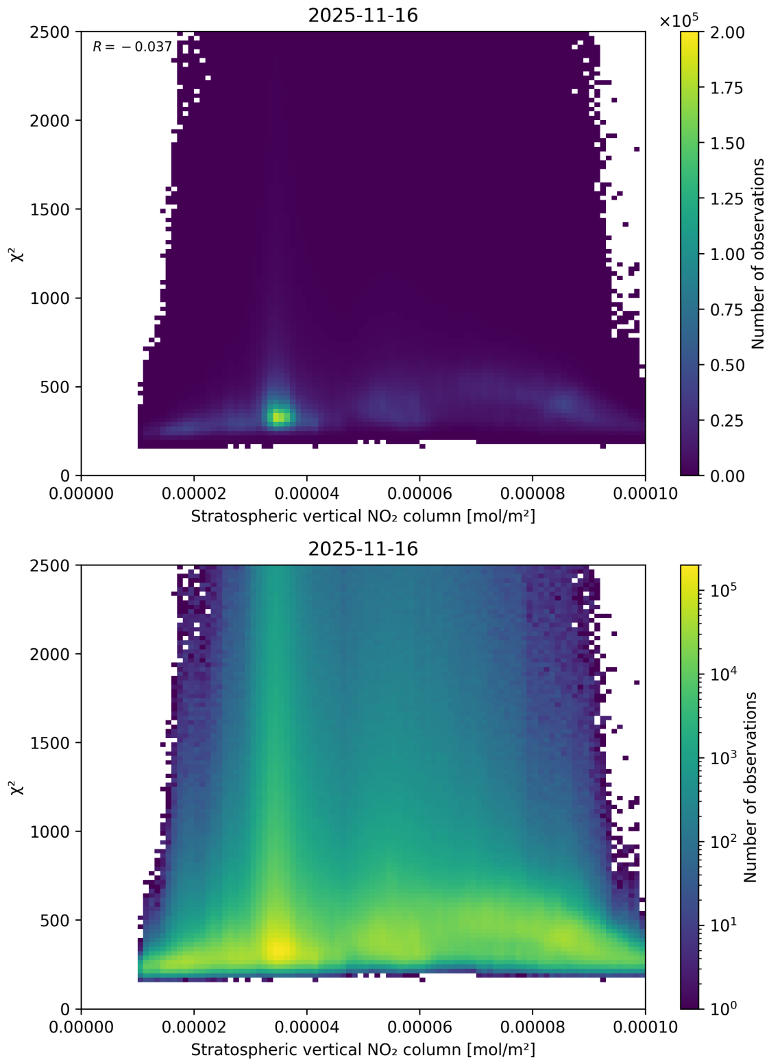
Figure 97: Scatter density plot of “Stratospheric vertical NO 2 column” against “ \chi^2 ” for 2025-11-15 to 2025-11-17.
