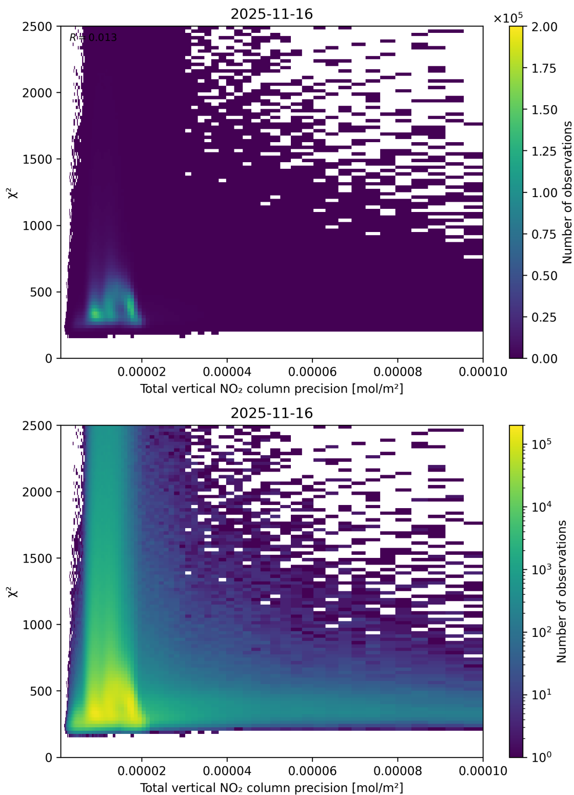
Figure 116: Scatter density plot of “Total vertical NO 2 column precision” against “ \chi^2 ” for 2025-11-15 to 2025-11-17.
