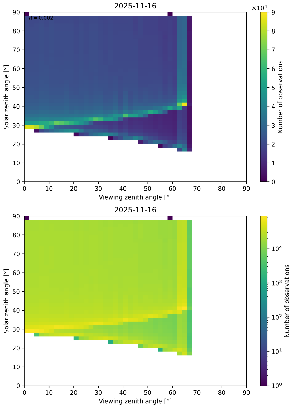
Figure 172: Scatter density plot of “Viewing zenith angle” against “Solar zenith angle” for 2025-11-15 to 2025-11-17.
