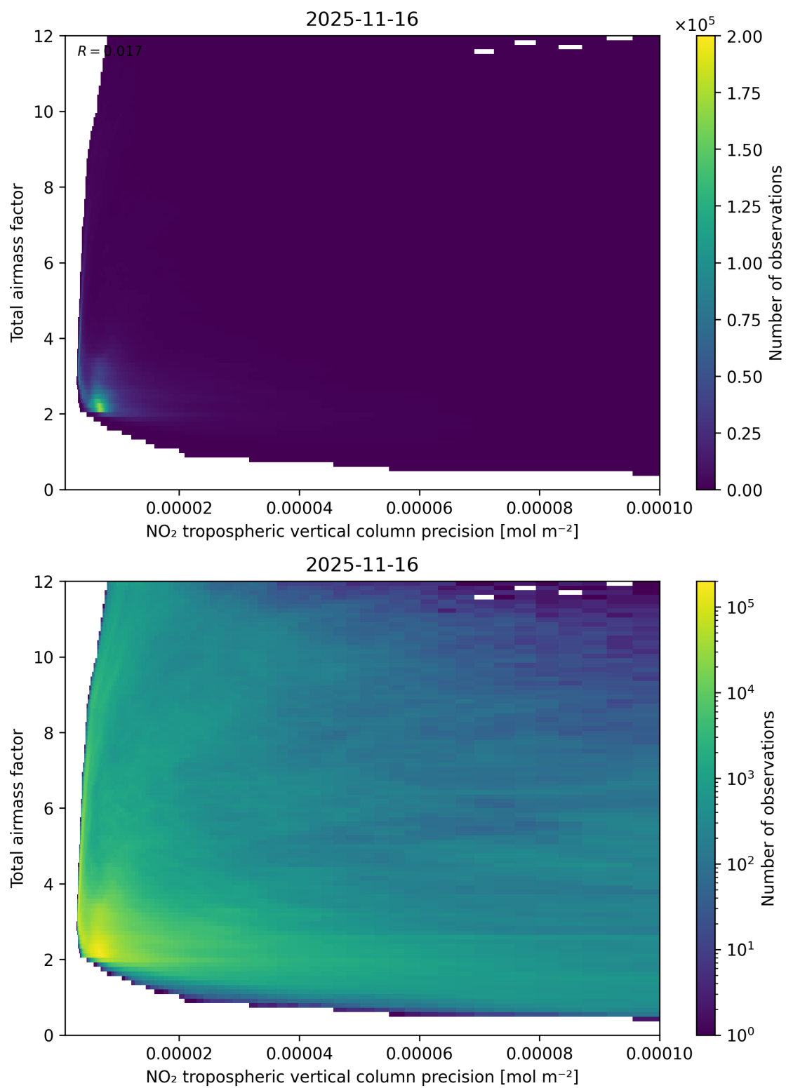
Figure 132: Scatter density plot of “NO 2 tropospheric vertical column precision” against “Total airmass factor” for 2025-11-15 to 2025-11-17.
