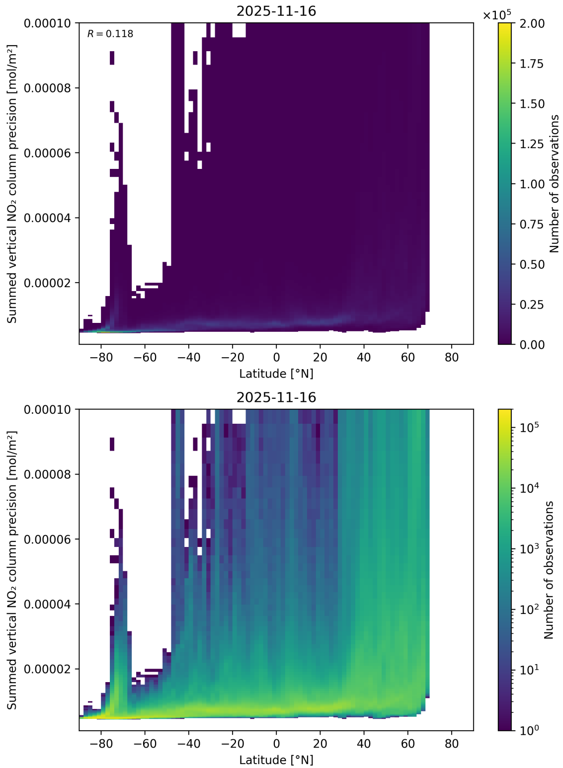
Figure 89: Scatter density plot of “Latitude” against “Summed vertical NO 2 column precision” for 2025-11-15 to 2025-11-17.
