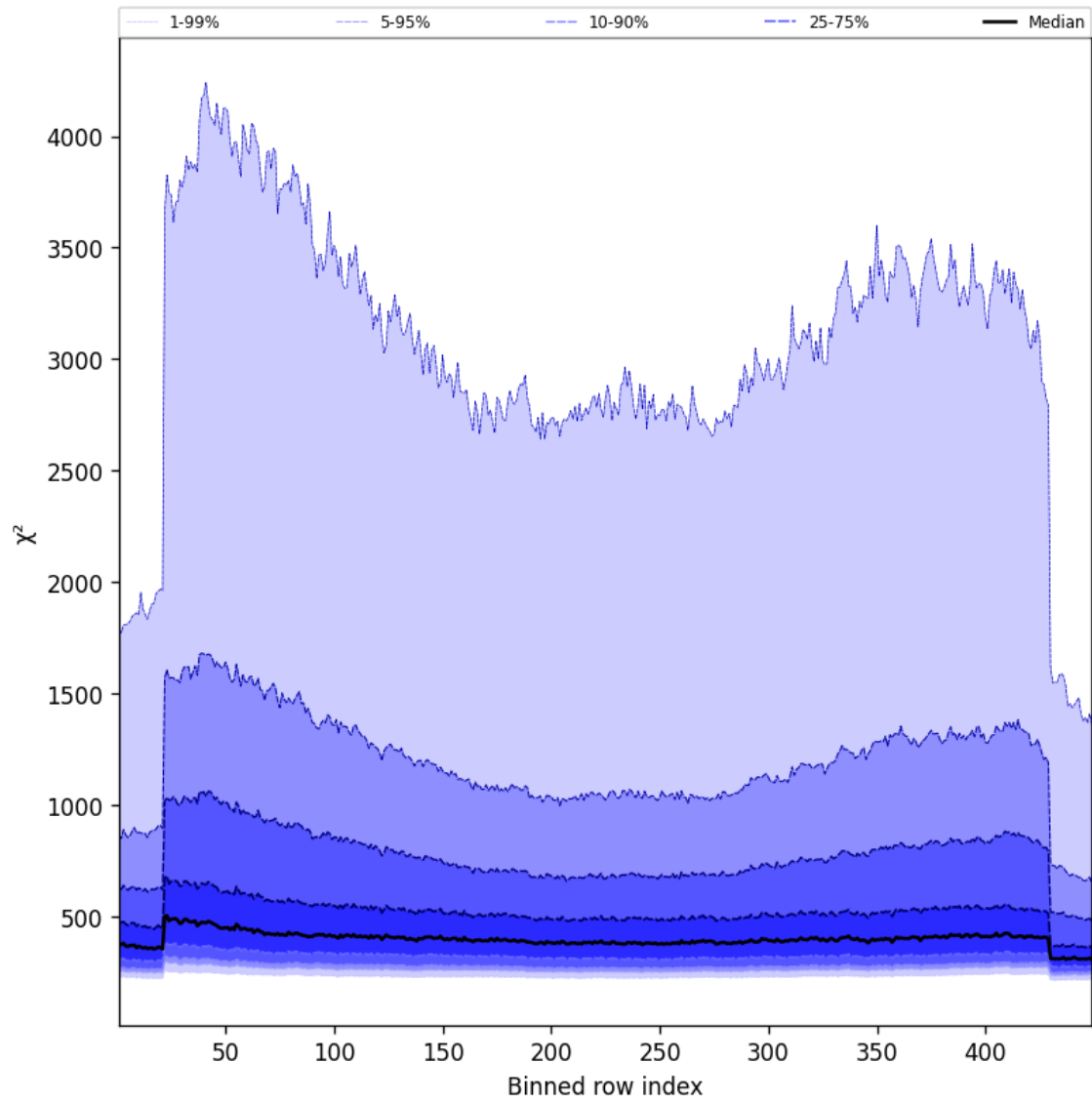
Figure 59: Along track statistics of “ \chi^2 ” for 2025-11-15 to 2025-11-17
