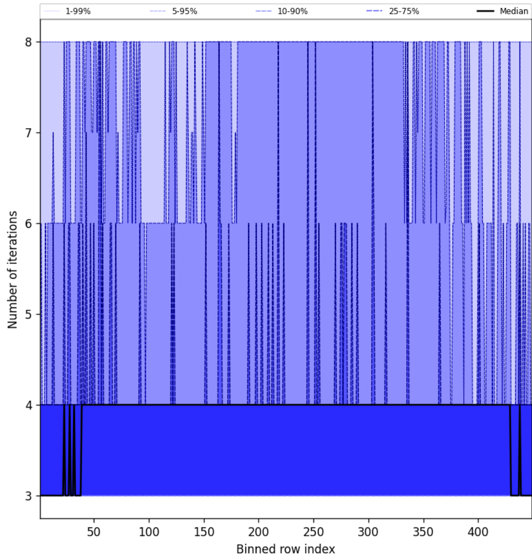
Figure 51: Along track statistics of “Number of iterations” for 2025-11-15 to 2025-11-17
