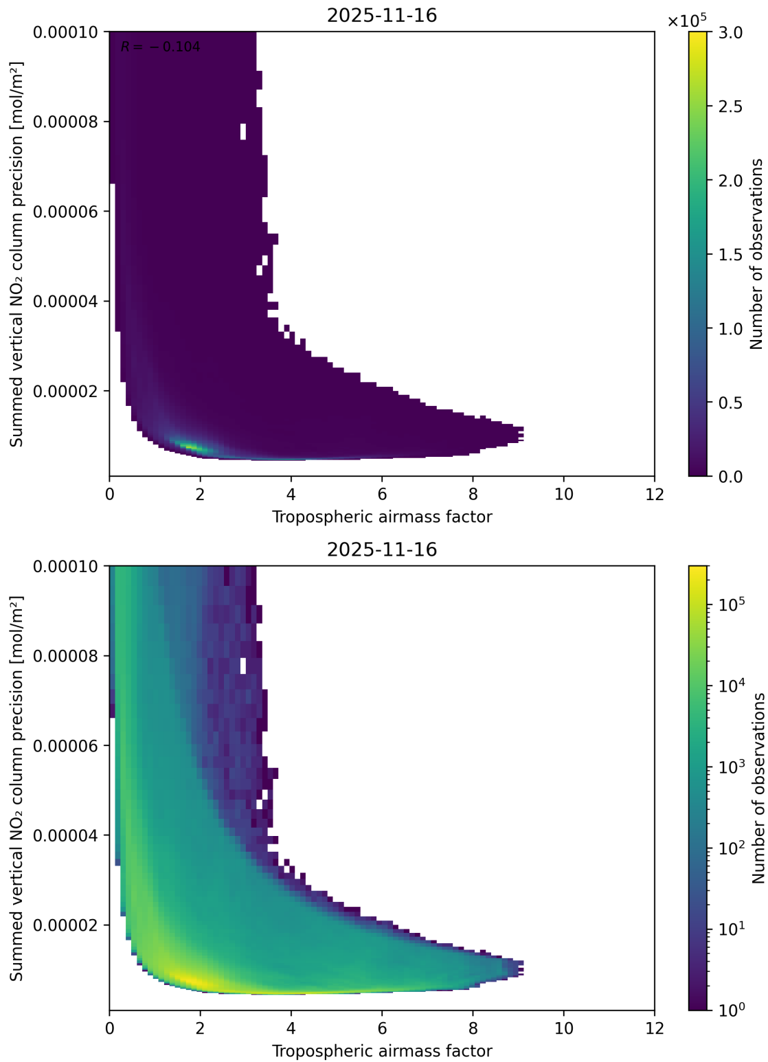
Figure 76: Scatter density plot of “Tropospheric airmass factor” against “Summed vertical NO 2 column precision” for 2025-11-15 to 2025-11-17.
