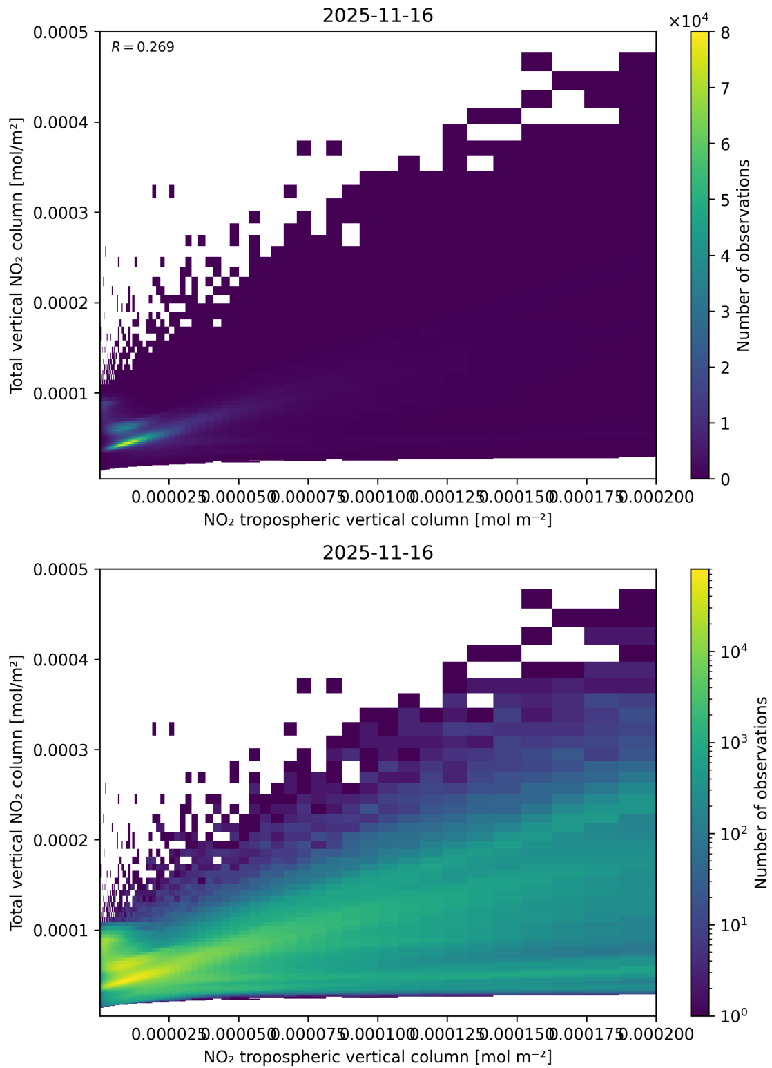
Figure 128: Scatter density plot of “NO 2 tropospheric vertical column” against “Total vertical NO 2 column” for 2025-11-15 to 2025-11-17.
