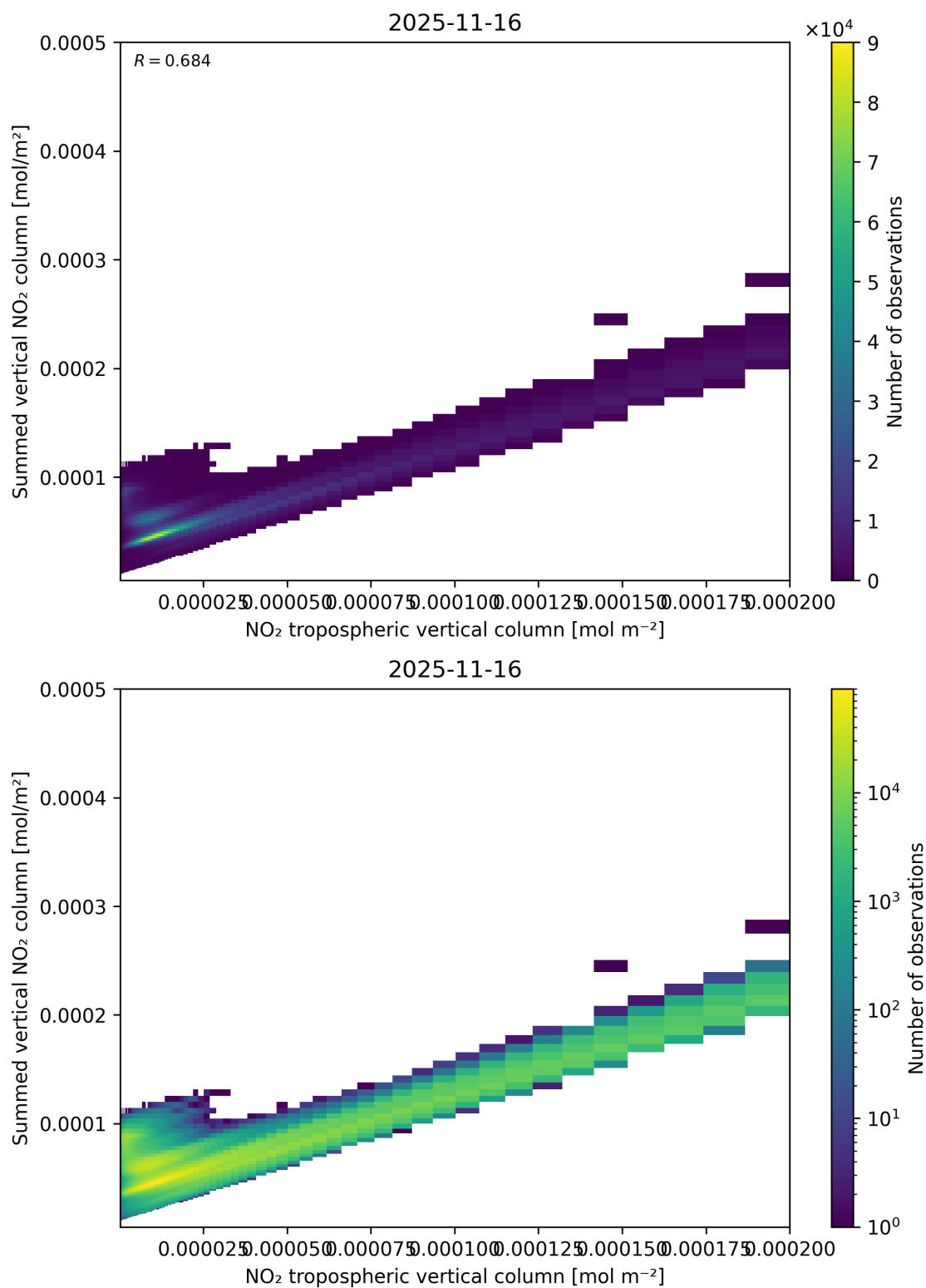
Figure 126: Scatter density plot of “NO 2 tropospheric vertical column” against “Summed vertical NO 2 column” for 2025-11-15 to 2025-11-17.
