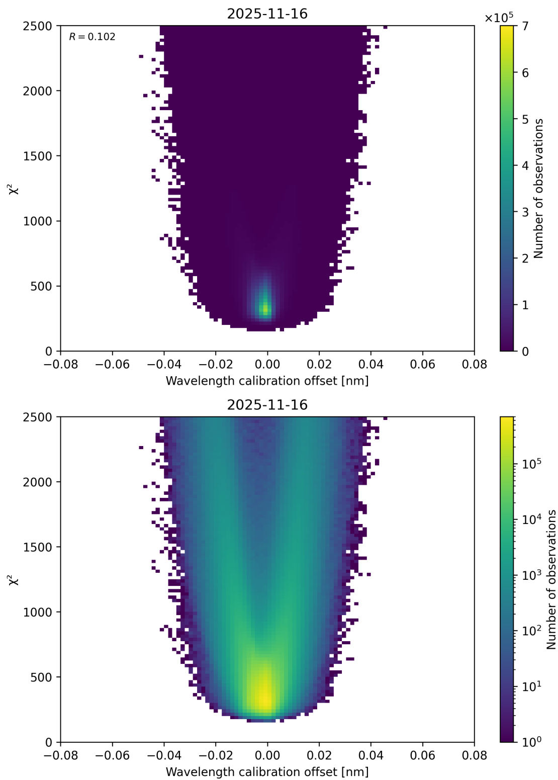
Figure 175: Scatter density plot of “Wavelength calibration offset” against “ \chi^2 ” for 2025-11-15 to 2025-11-17.
