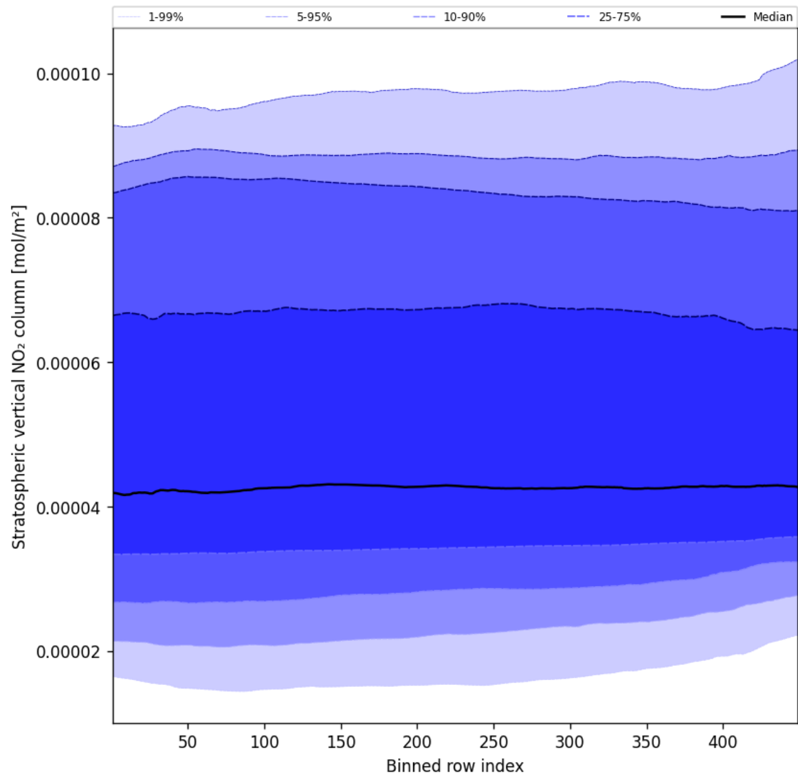
Figure 53: Along track statistics of “Stratospheric vertical NO 2 column” for 2025-11-15 to 2025-11-17
