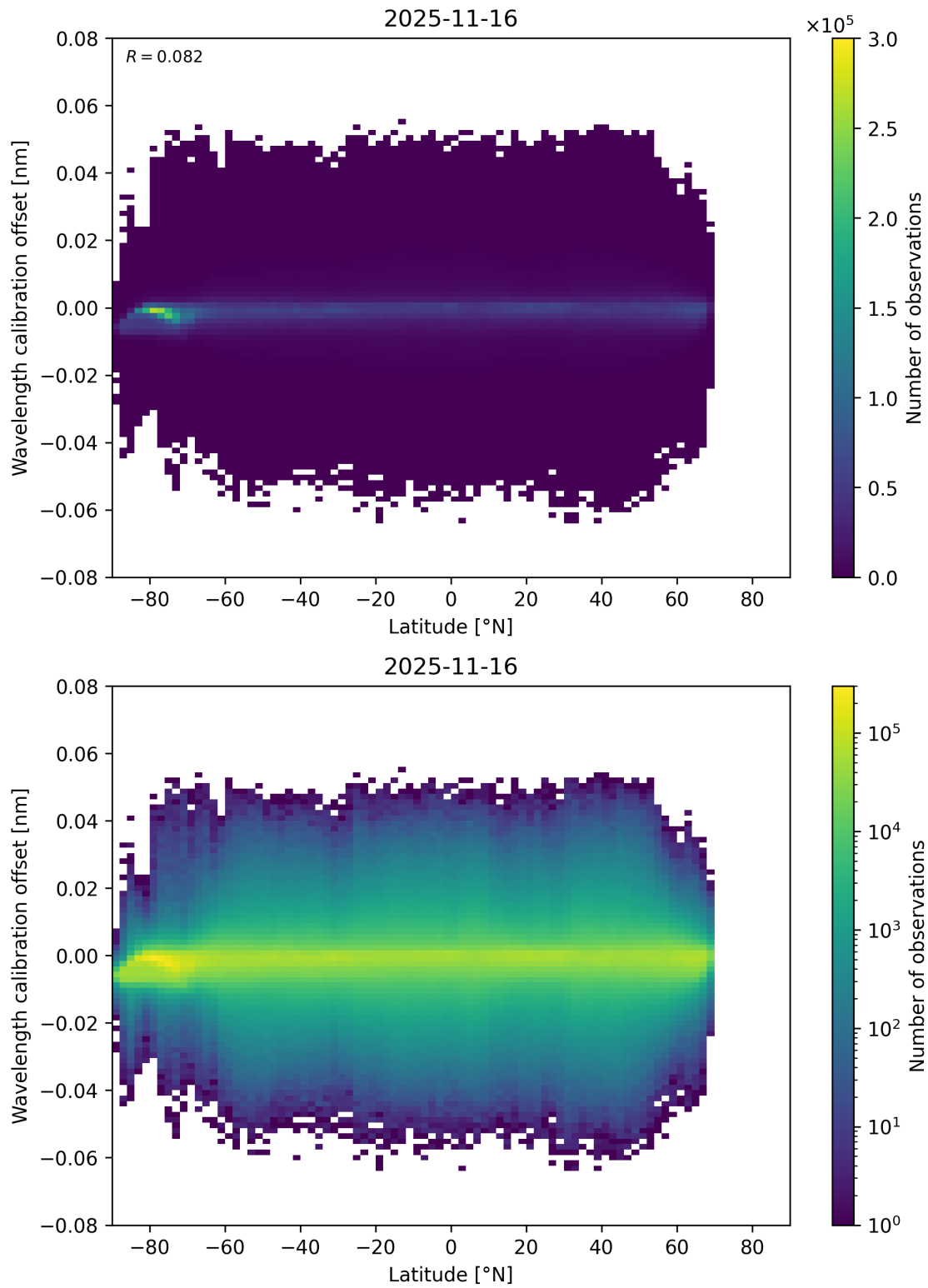
Figure 95: Scatter density plot of “Latitude” against “Wavelength calibration offset” for 2025-11-15 to 2025-11-17.
