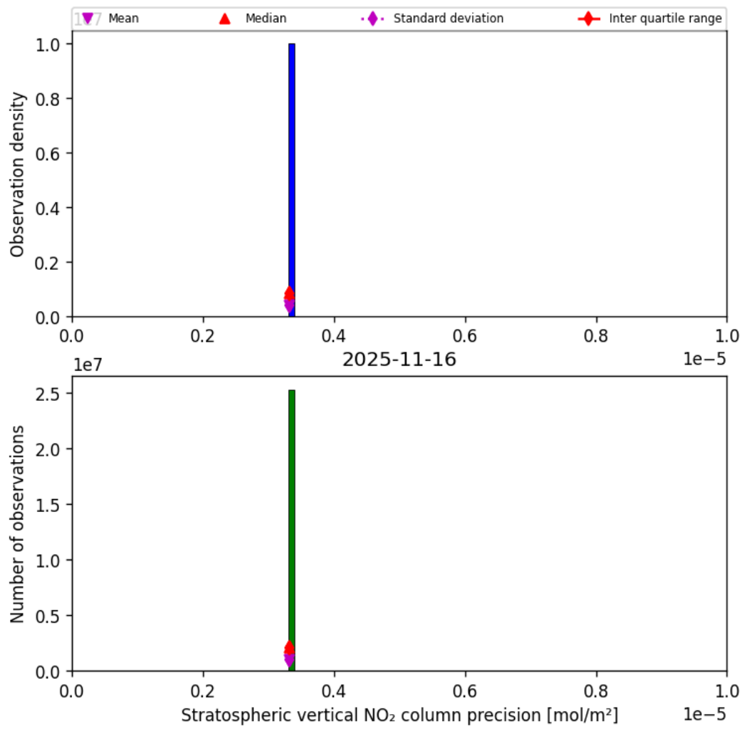
Figure 37: Histogram of “Stratospheric vertical NO 2 column precision” for 2025-11-15 to 2025-11-17
