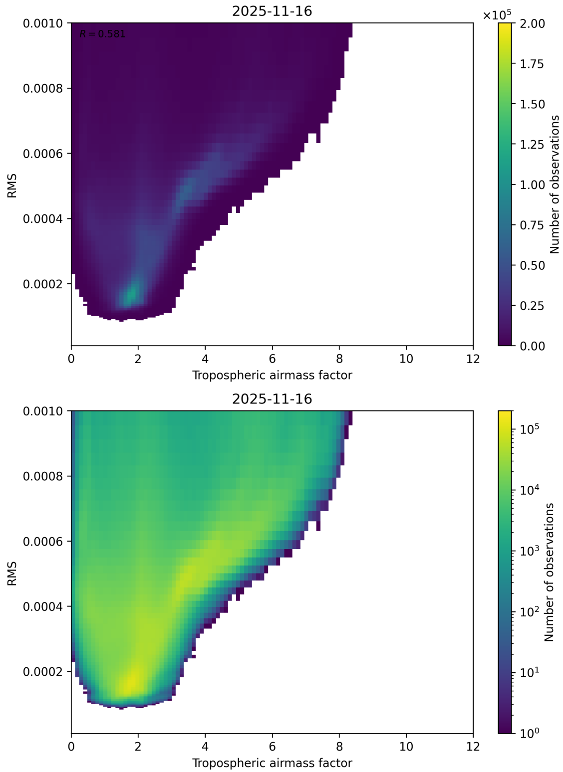
Figure 79: Scatter density plot of “Tropospheric airmass factor” against “RMS” for 2025-11-15 to 2025-11-17.
