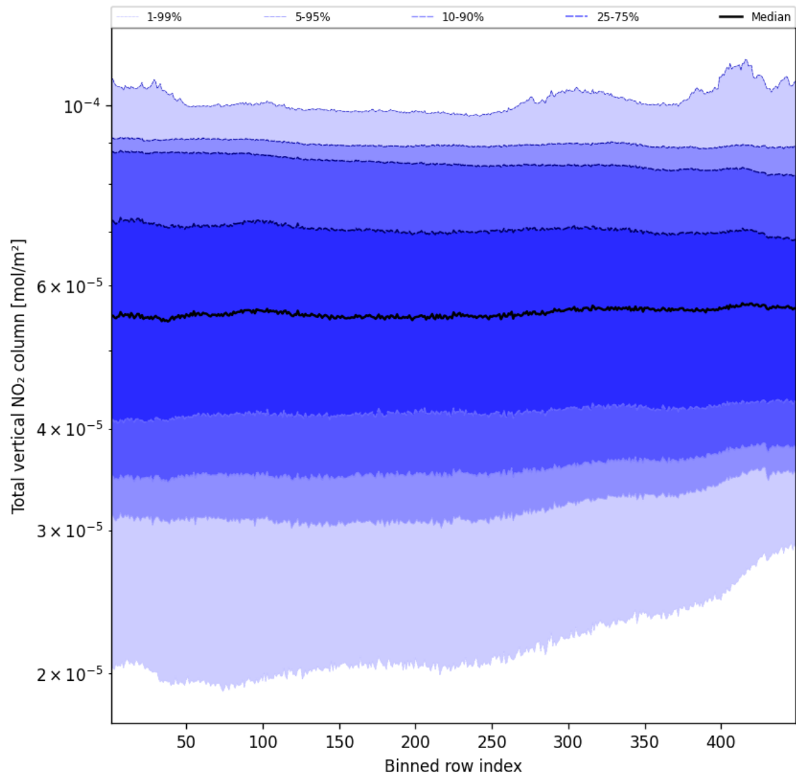
Figure 55: Along track statistics of “Total vertical NO 2 column” for 2025-11-15 to 2025-11-17
