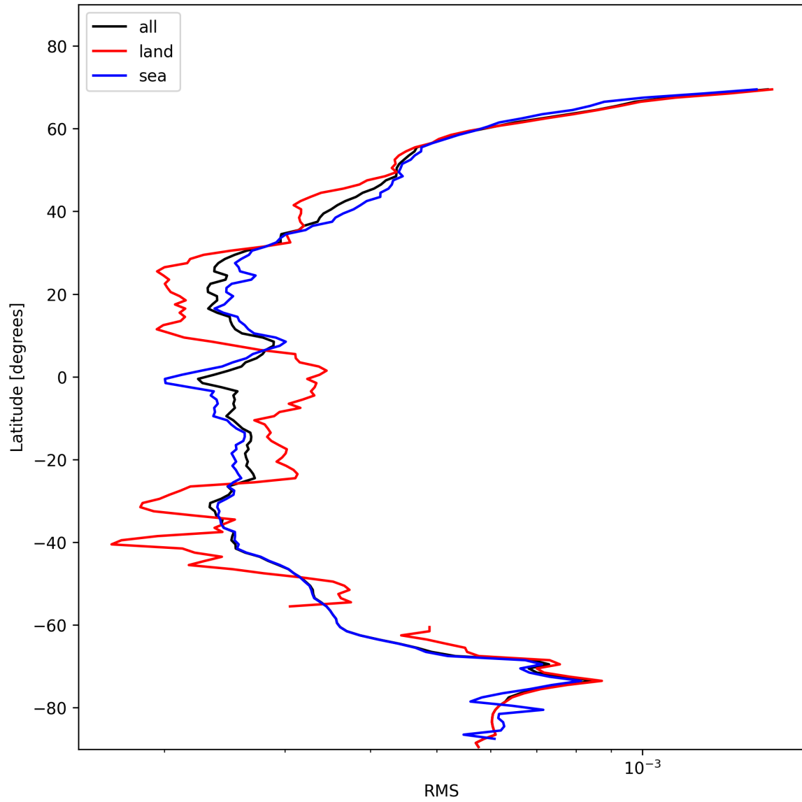
Figure 26: Zonal average of “RMS” for 2025-11-15 to 2025-11-17.
