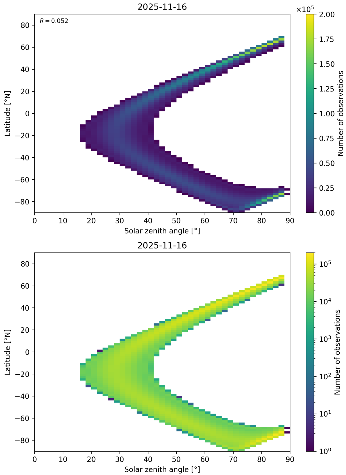
Figure 149: Scatter density plot of “Solar zenith angle” against “Latitude” for 2025-11-15 to 2025-11-17.
