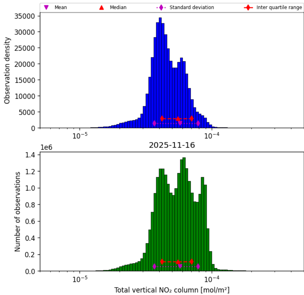
Figure 38: Histogram of “Total vertical NO 2 column” for 2025-11-15 to 2025-11-17
