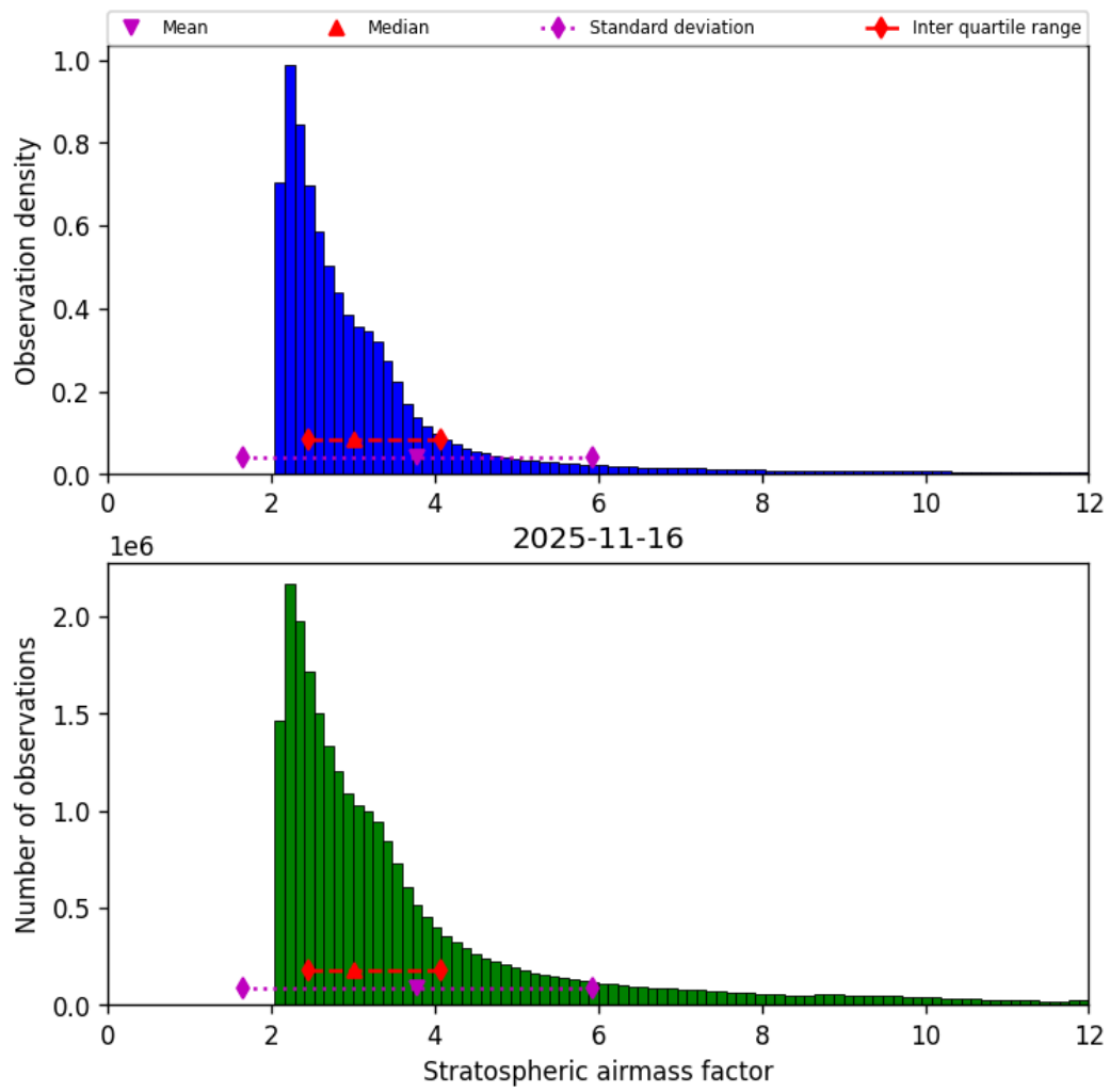
Figure 44: Histogram of “Stratospheric airmass factor” for 2025-11-15 to 2025-11-17
