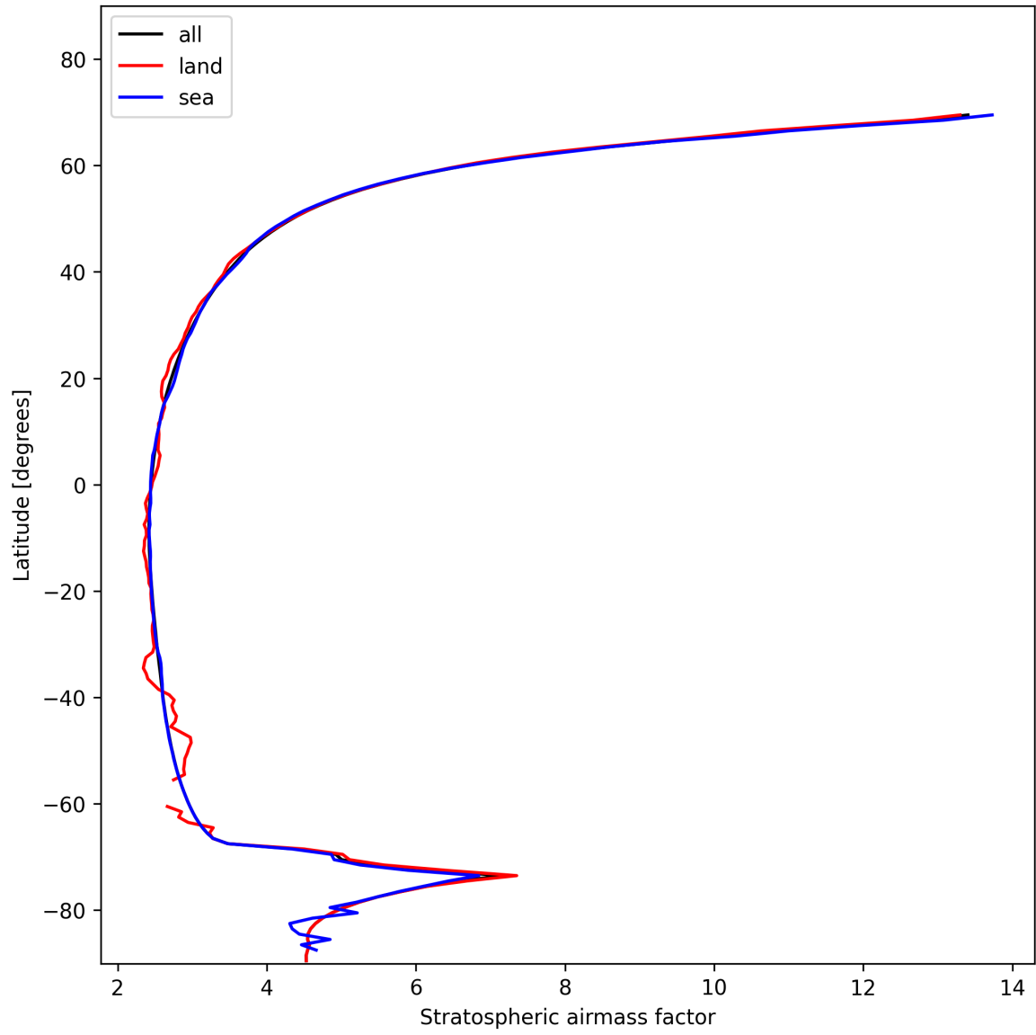
Figure 27: Zonal average of “Stratospheric airmass factor” for 2025-11-15 to 2025-11-17.
