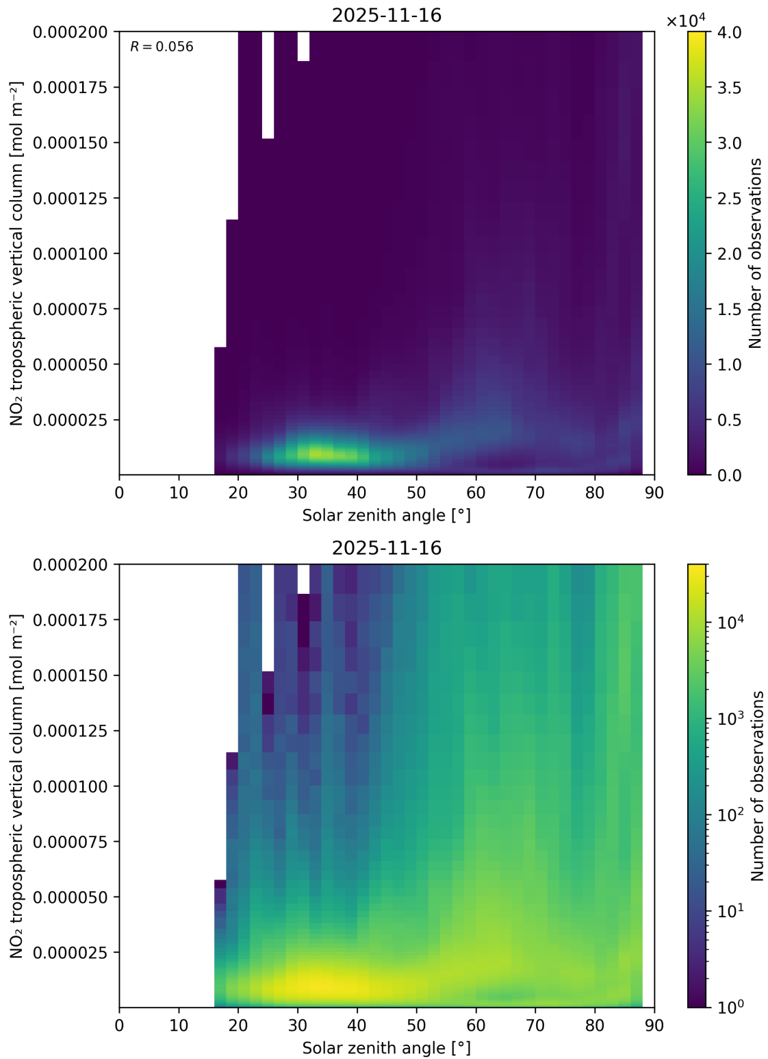
Figure 155: Scatter density plot of “Solar zenith angle” against “NO 2 tropospheric vertical column” for 2025-11-15 to 2025-11-17.
