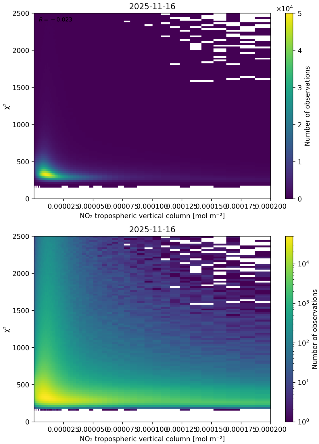
Figure 124: Scatter density plot of “NO 2 tropospheric vertical column” against “ \chi^2 ” for 2025-11-15 to 2025-11-17.
