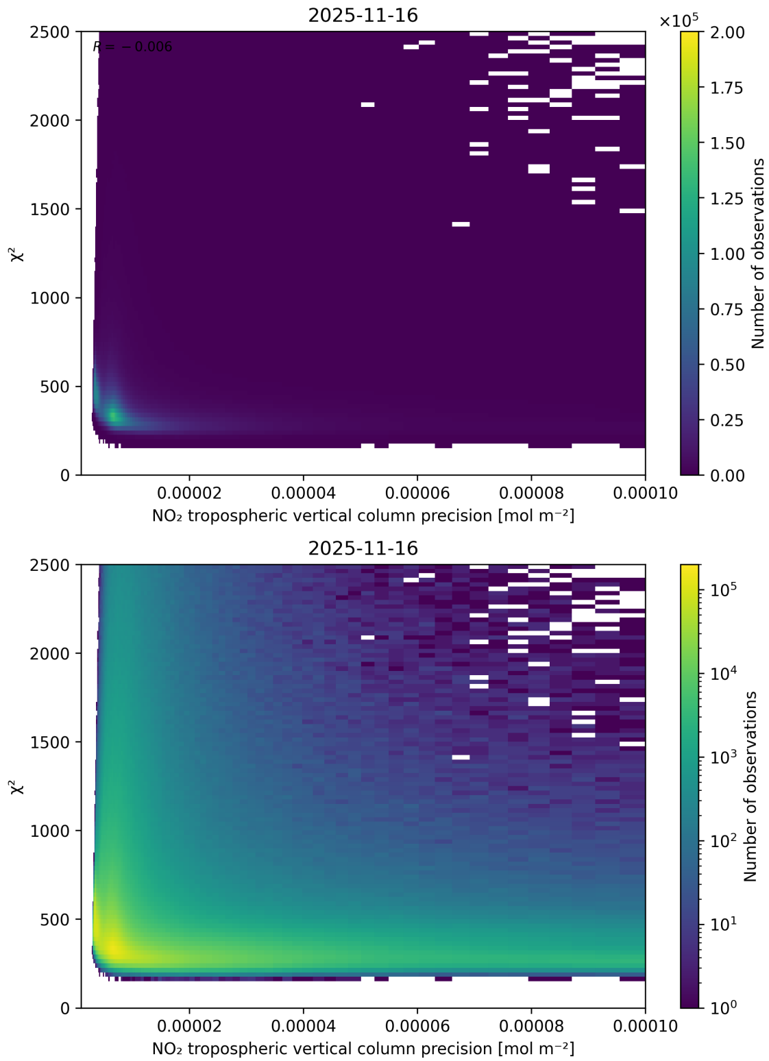
Figure 134: Scatter density plot of “NO 2 tropospheric vertical column precision” against “ \chi^2 ” for 2025-11-15 to 2025-11-17.
