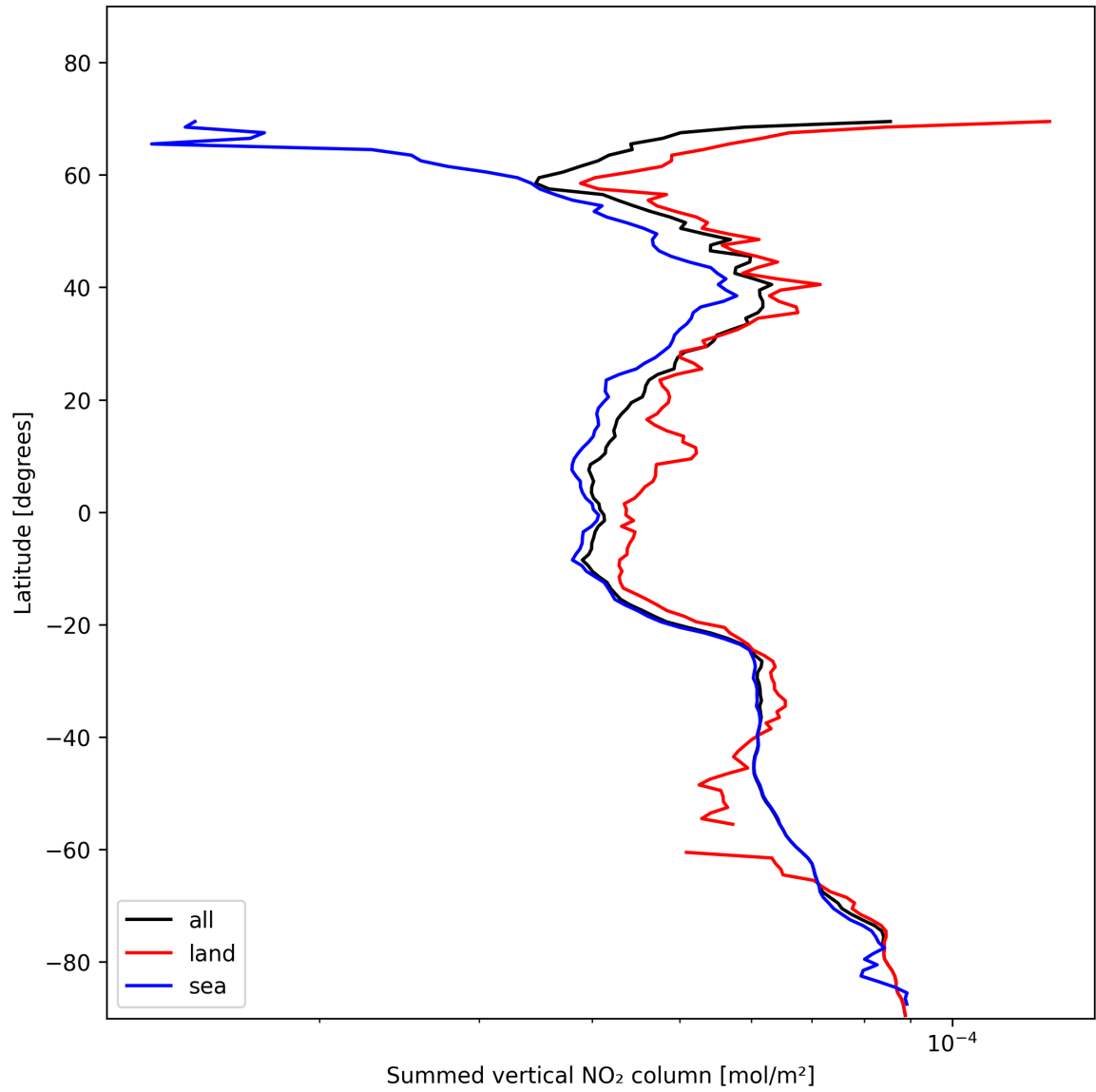
Figure 23: Zonal average of “Summed vertical NO 2 column” for 2025-11-15 to 2025-11-17.
