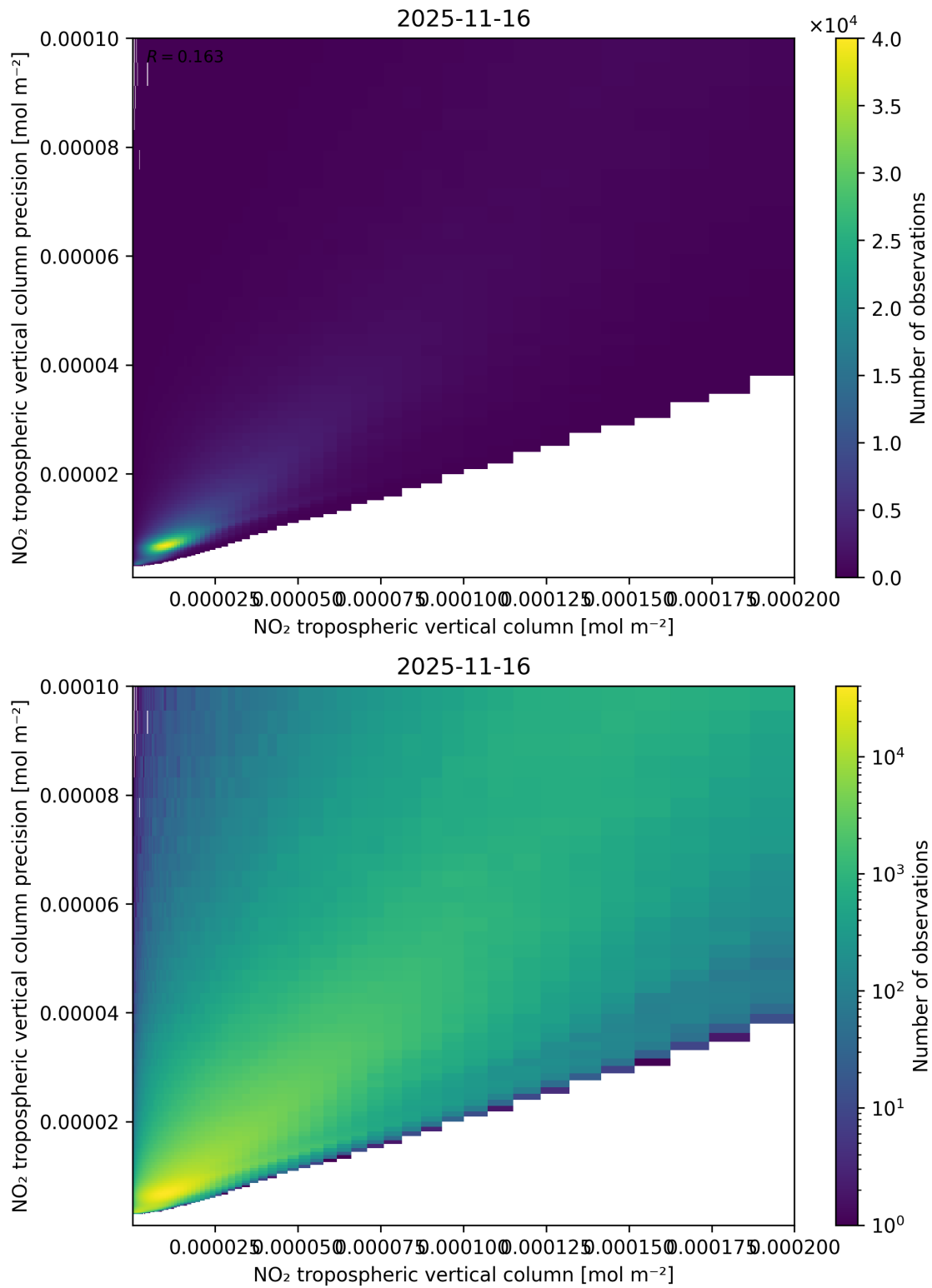
Figure 130: Scatter density plot of “NO 2 tropospheric vertical column” against “NO 2 tropospheric vertical column precision” for 2025-11-15 to 2025-11-17.
