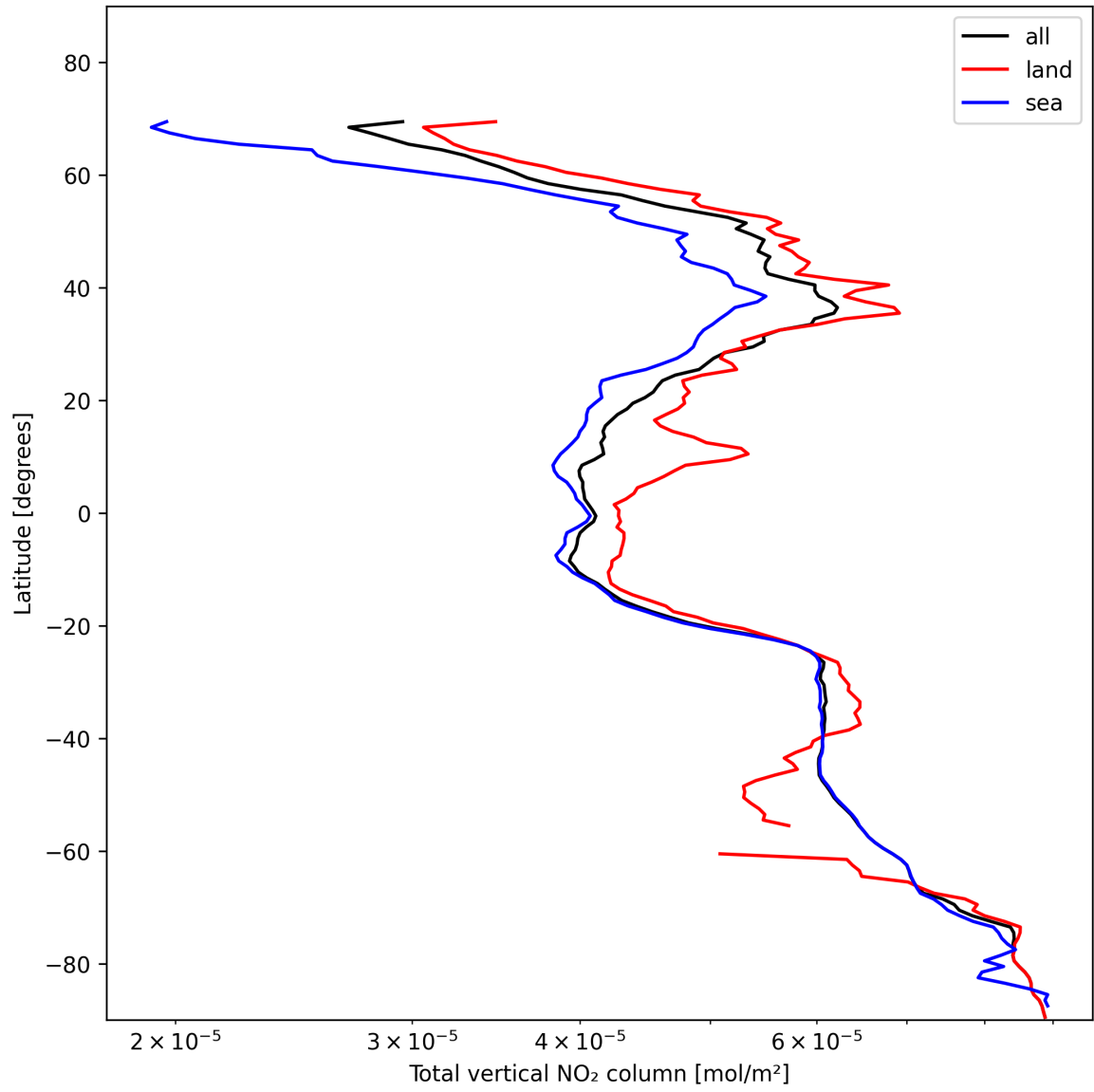
Figure 21: Zonal average of “Total vertical NO 2 column” for 2025-11-15 to 2025-11-17.
