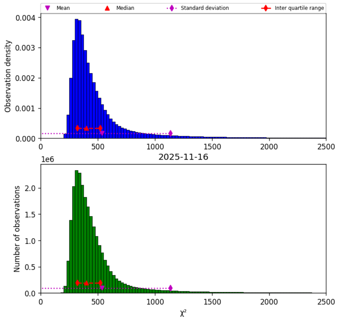
Figure 42: Histogram of “ \chi^2 ” for 2025-11-15 to 2025-11-17
