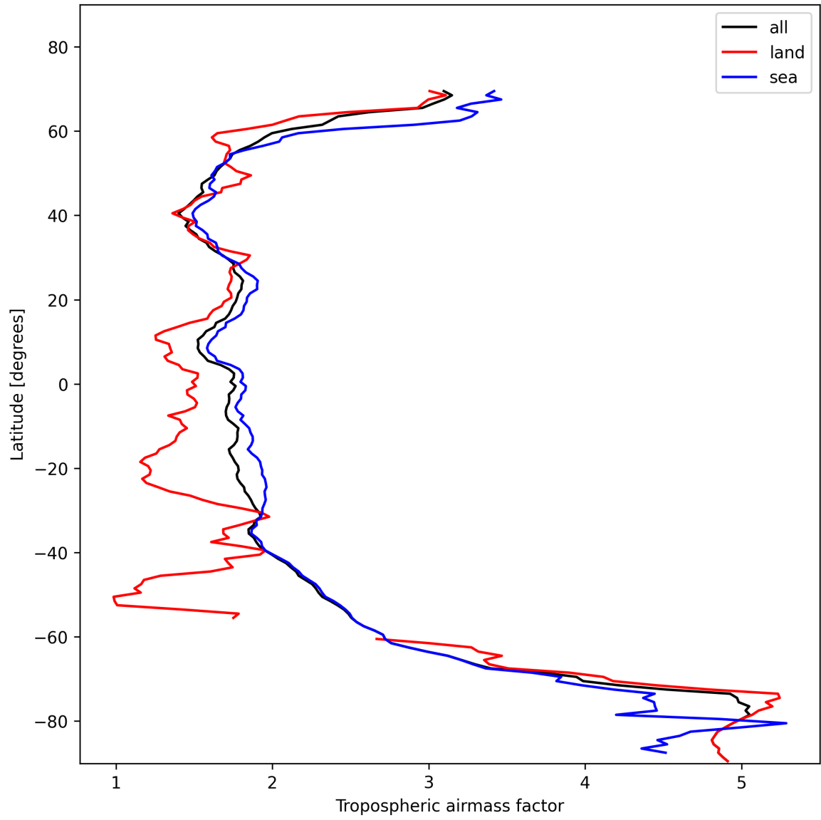
Figure 14: Zonal average of “Tropospheric airmass factor” for 2025-11-15 to 2025-11-17.
