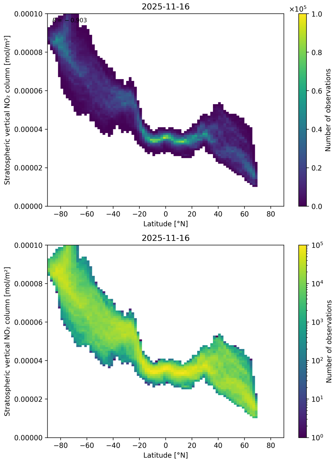
Figure 87: Scatter density plot of “Latitude” against “Stratospheric vertical NO 2 column” for 2025-11-15 to 2025-11-17.
