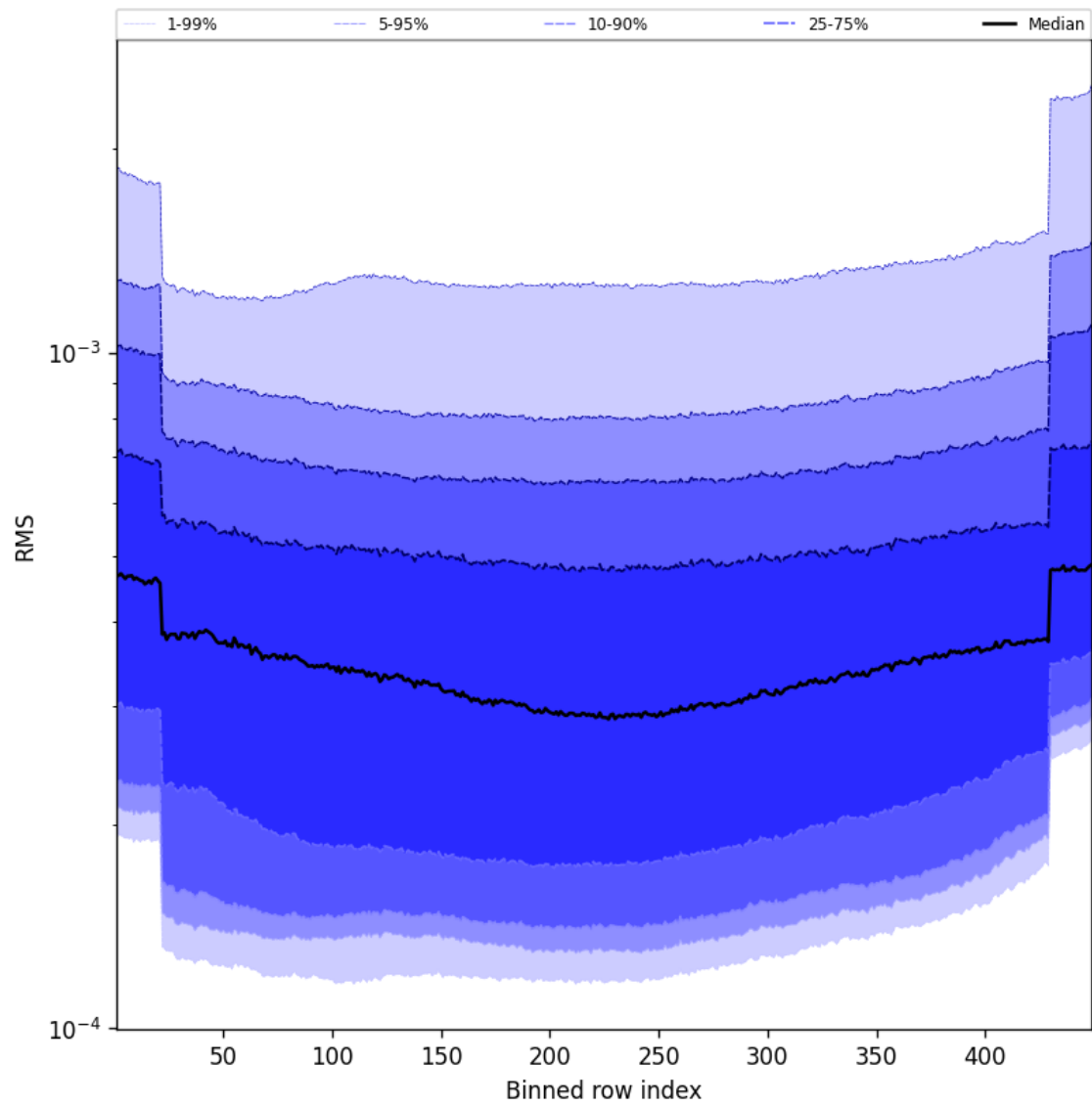
Figure 60: Along track statistics of “RMS” for 2025-11-15 to 2025-11-17
