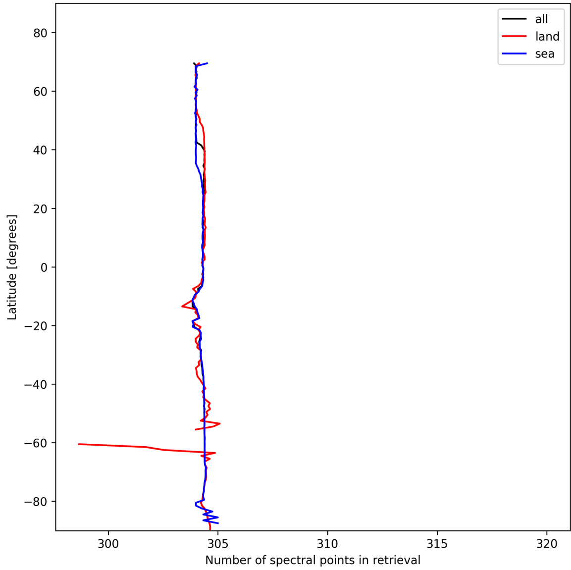
Figure 16: Zonal average of “Number of spectral points in retrieval” for 2025-11-15 to 2025-11-17.
