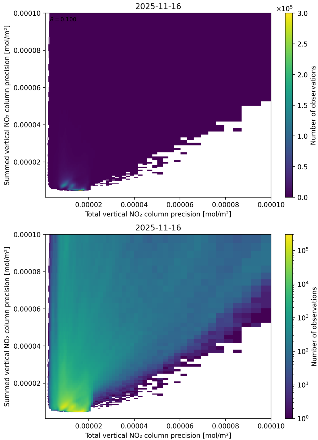
Figure 118: Scatter density plot of “Total vertical NO 2 column precision” against “Summed vertical NO 2 column precision” for 2025-11-15 to 2025-11-17.
