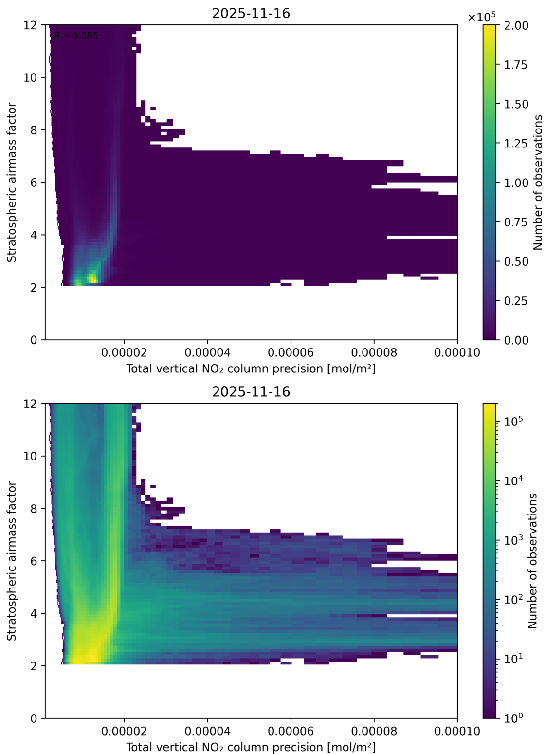
Figure 115: Scatter density plot of “Total vertical NO 2 column precision” against “Stratospheric airmass factor” for 2025-11-15 to 2025-11-17.
