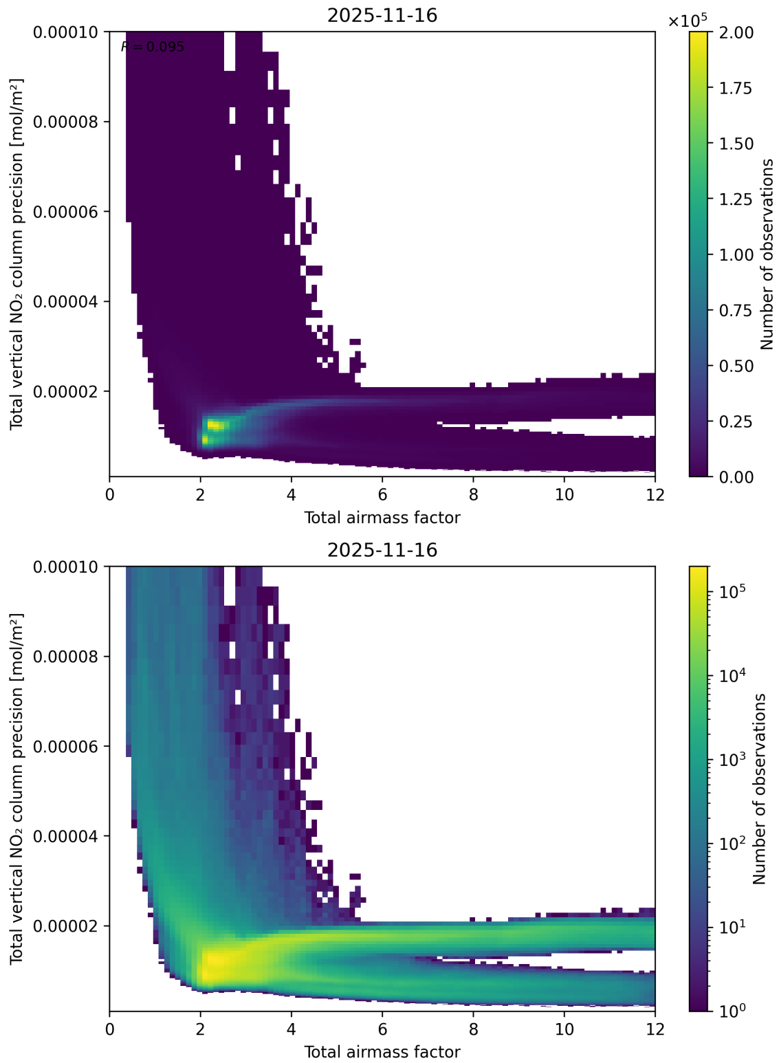
Figure 68: Scatter density plot of “Total airmass factor” against “Total vertical NO 2 column precision” for 2025-11-15 to 2025-11-17.
