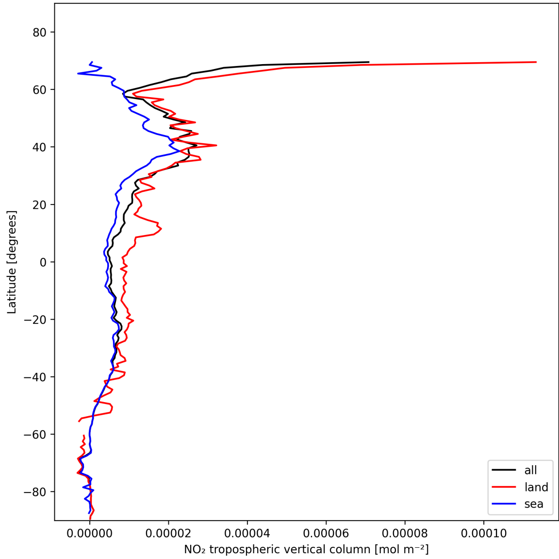
Figure 12: Zonal average of “NO 2 tropospheric vertical column” for 2025-11-15 to 2025-11-17.
