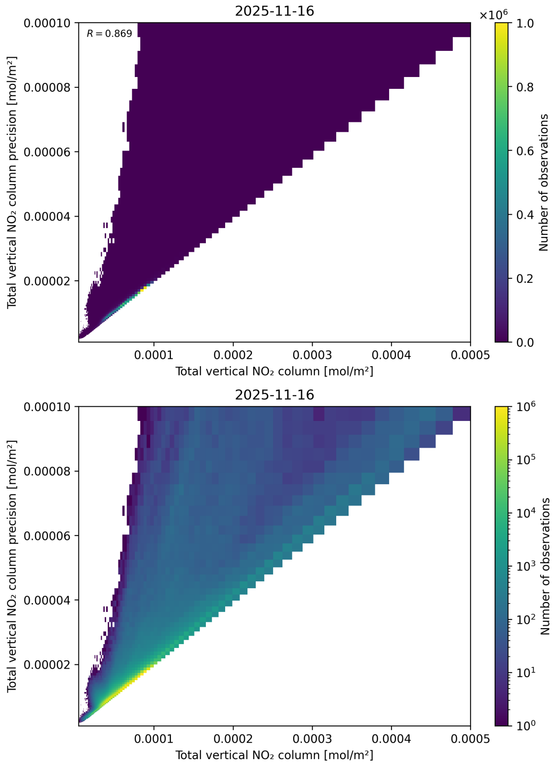
Figure 114: Scatter density plot of “Total vertical NO 2 column” against “Total vertical NO 2 column precision” for 2025-11-15 to 2025-11-17.
