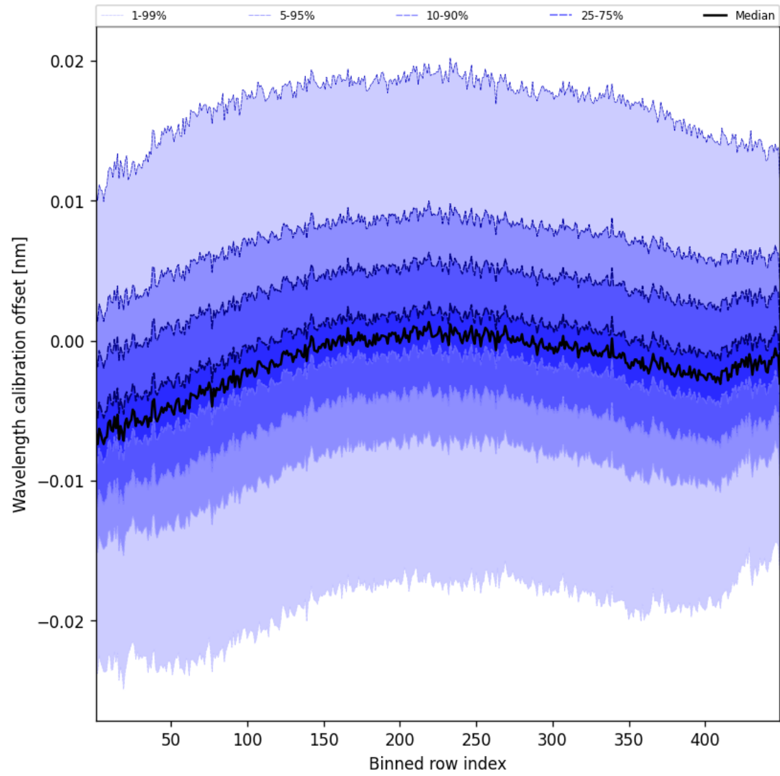
Figure 52: Along track statistics of “Wavelength calibration offset” for 2025-11-15 to 2025-11-17
