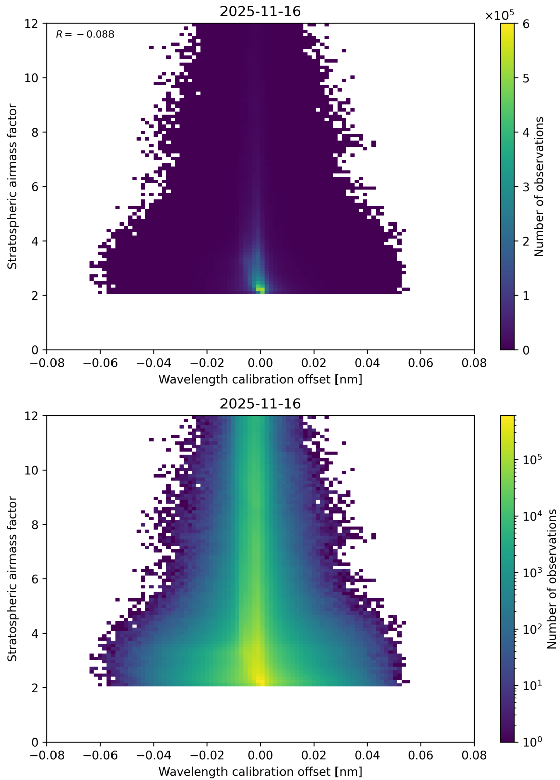
Figure 174: Scatter density plot of “Wavelength calibration offset” against “Stratospheric airmass factor” for 2025-11-15 to 2025-11-17.
