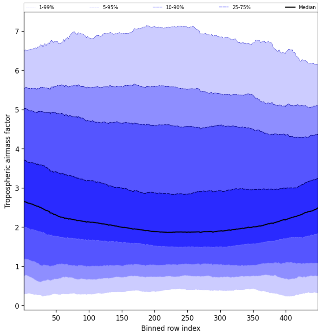
Figure 48: Along track statistics of “Tropospheric air mass factor” for 2025-11-15 to 2025-11-17
