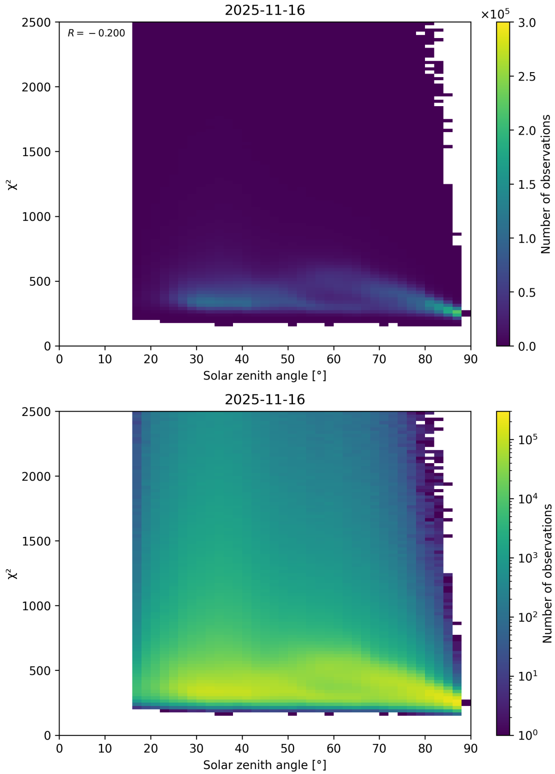
Figure 148: Scatter density plot of “Solar zenith angle” against “ \chi^2 ” for 2025-11-15 to 2025-11-17.
