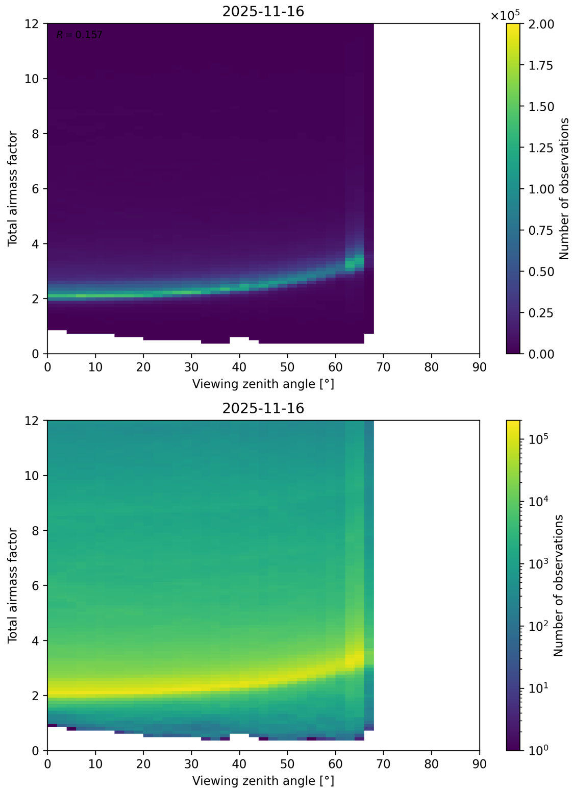
Figure 160: Scatter density plot of “Viewing zenith angle” against “Total airmass factor” for 2025-11-15 to 2025-11-17.
