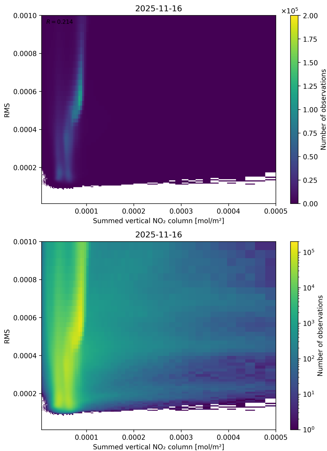
Figure 109: Scatter density plot of “Summed vertical NO 2 column” against “RMS” for 2025-11-15 to 2025-11-17.
