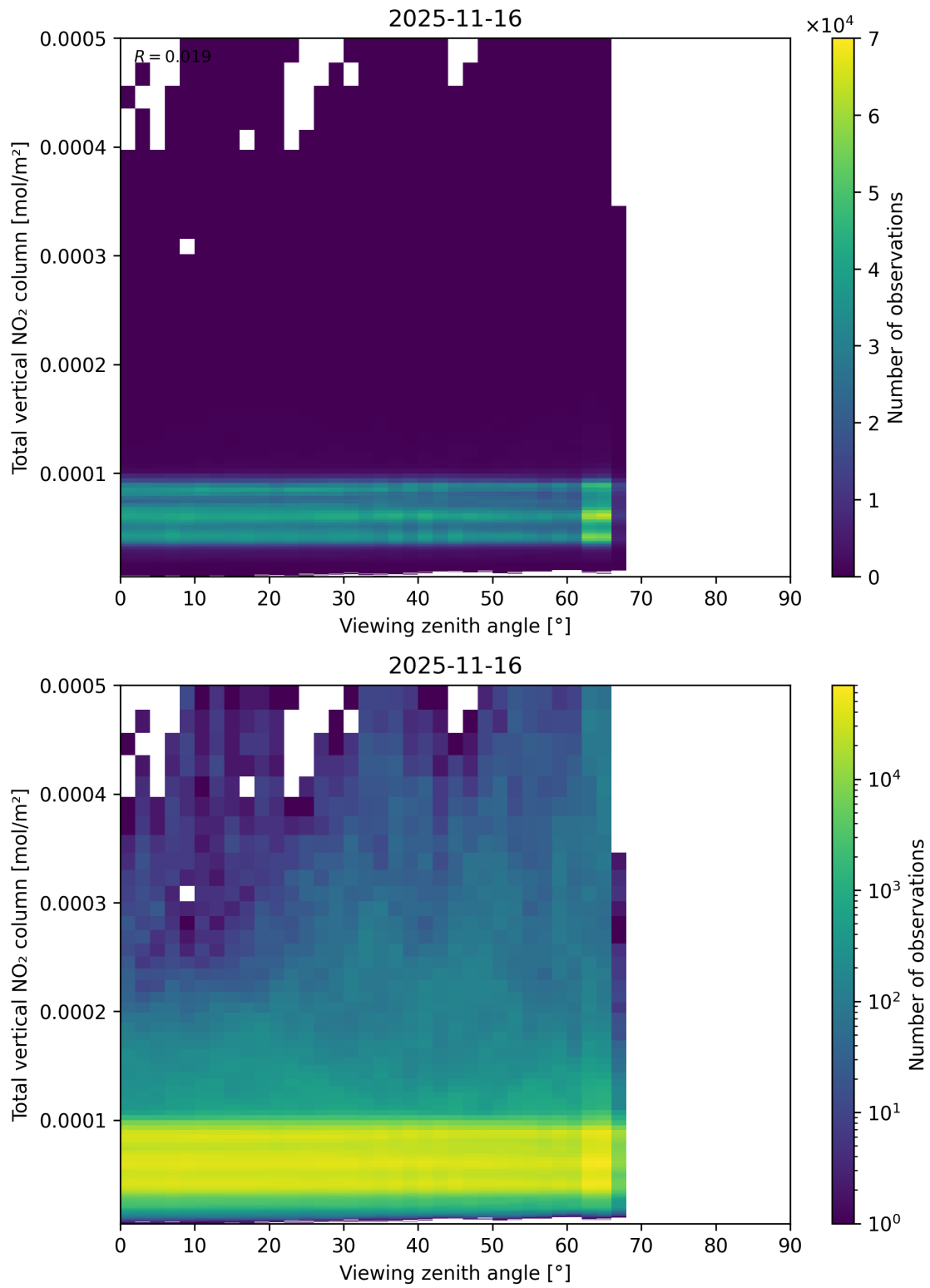
Figure 167: Scatter density plot of “Viewing zenith angle” against “Total vertical NO 2 column” for 2025-11-15 to 2025-11-17.
