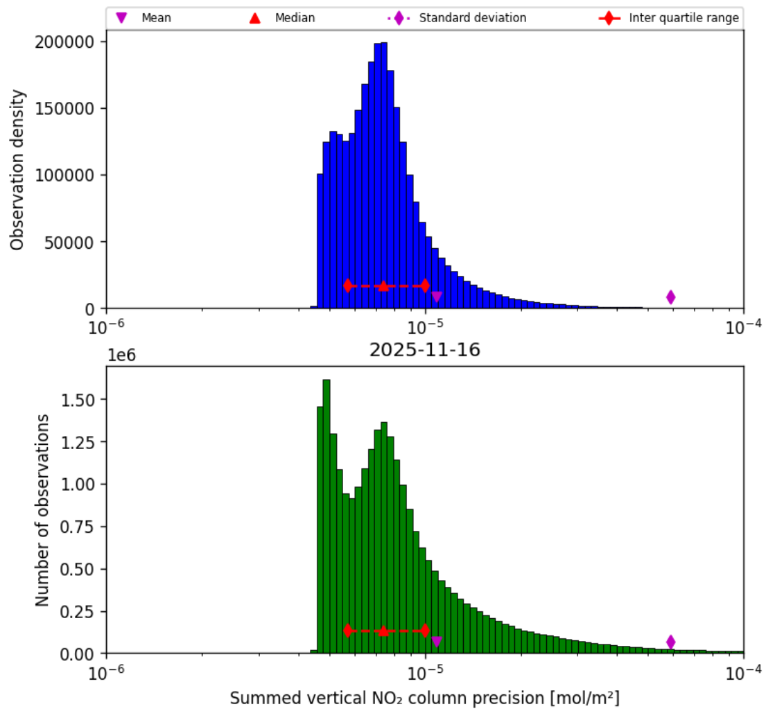
Figure 41: Histogram of “Summed vertical NO 2 column precision” for 2025-11-15 to 2025-11-17
