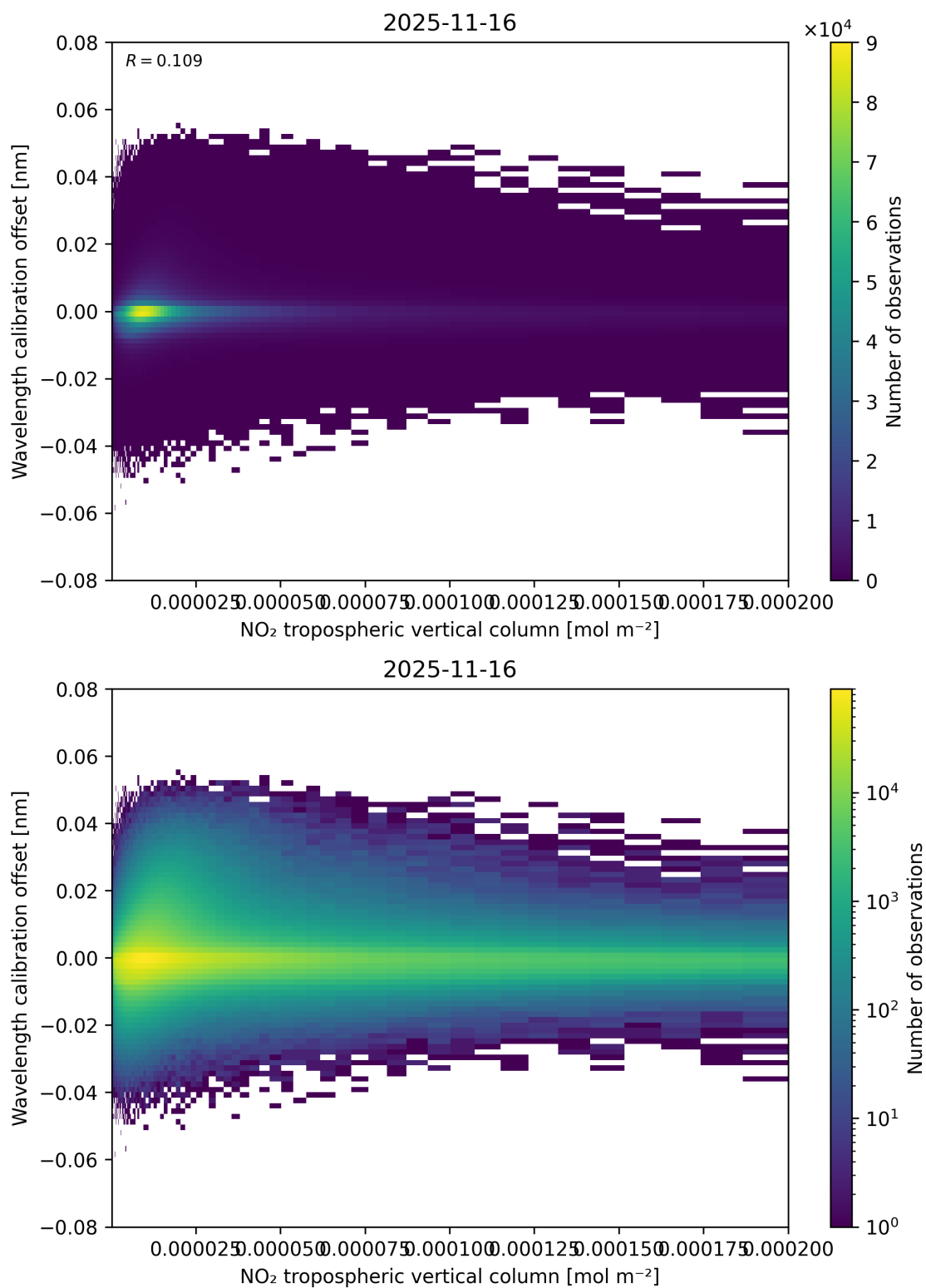
Figure 143: Scatter density plot of “NO 2 tropospheric vertical column” against “Wavelength calibration offset” for 2025-11-15 to 2025-11-17.
