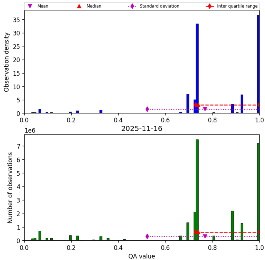
Figure 28: Histogram of “QA value” for 2025-11-15 to 2025-11-17
