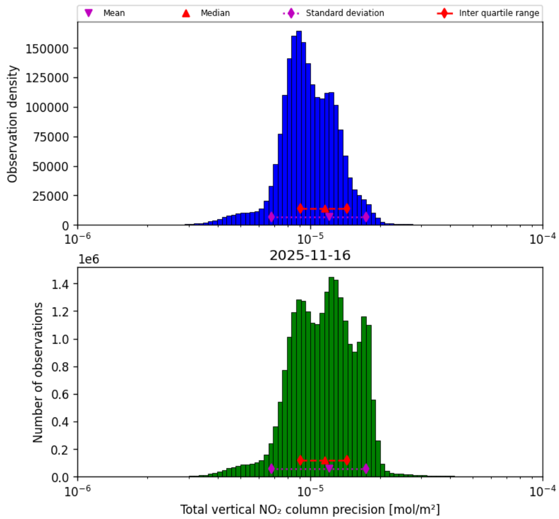
Figure 39: Histogram of “Total vertical NO 2 column precision” for 2025-11-15 to 2025-11-17
