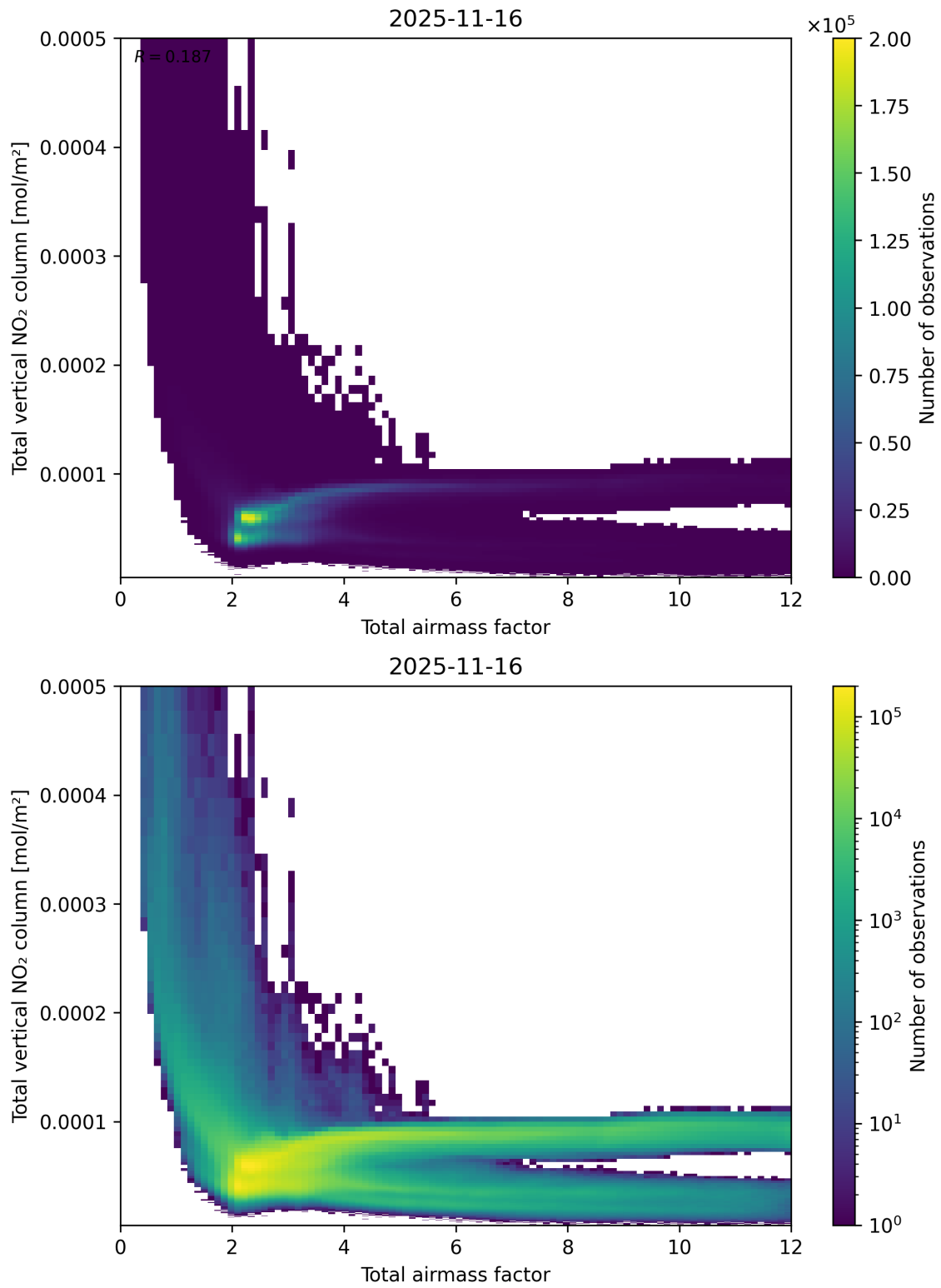
Figure 67: Scatter density plot of “Total airmass factor” against “Total vertical NO 2 column” for 2025-11-15 to 2025-11-17.
