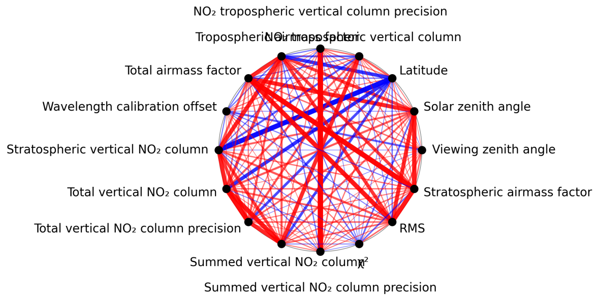
Figure 1: Map of correlation graph for 2025-11-15 to 2025-11-17.
