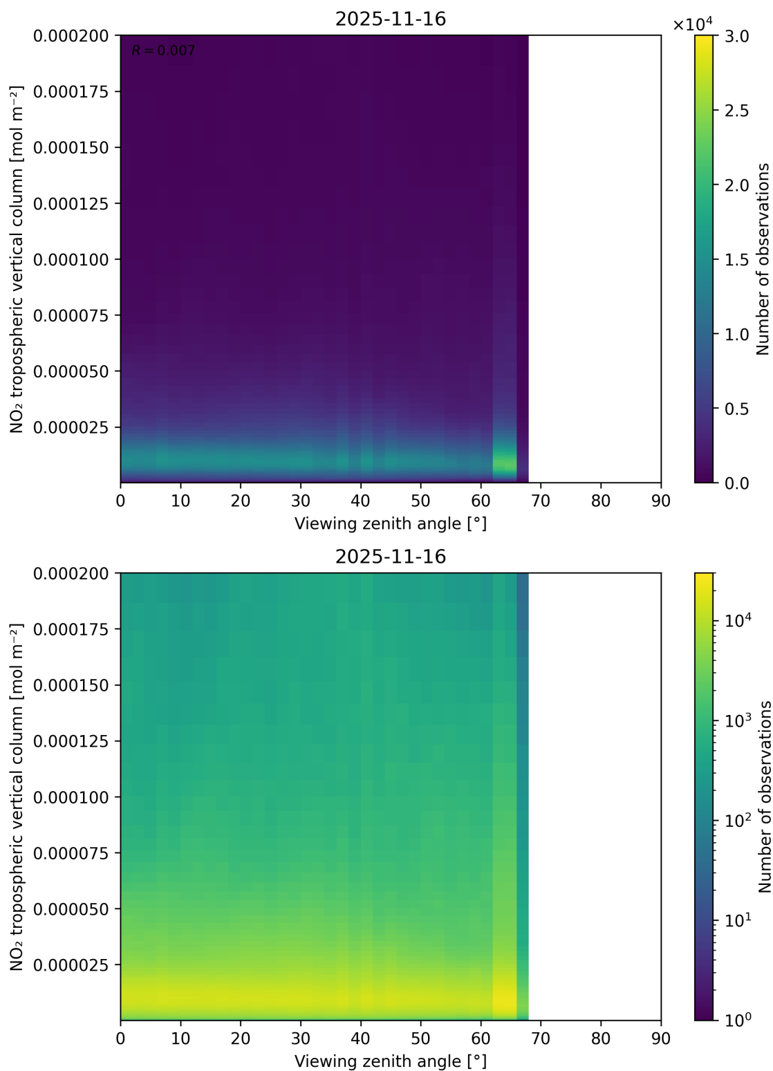
Figure 169: Scatter density plot of “Viewing zenith angle” against “NO 2 tropospheric vertical column” for 2025-11-15 to 2025-11-17.
