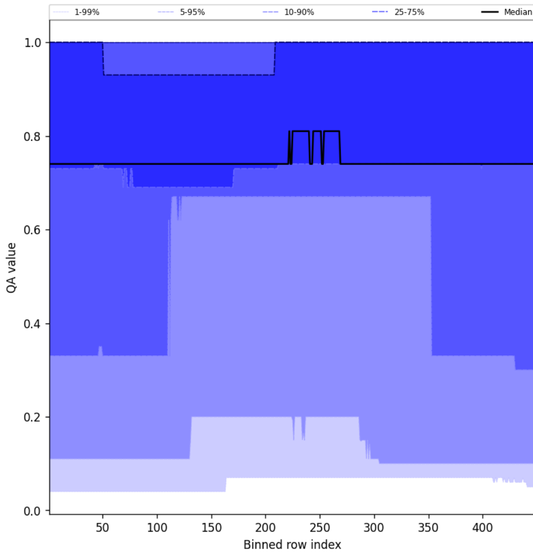
Figure 45: Along track statistics of “QA value” for 2025-11-15 to 2025-11-17
