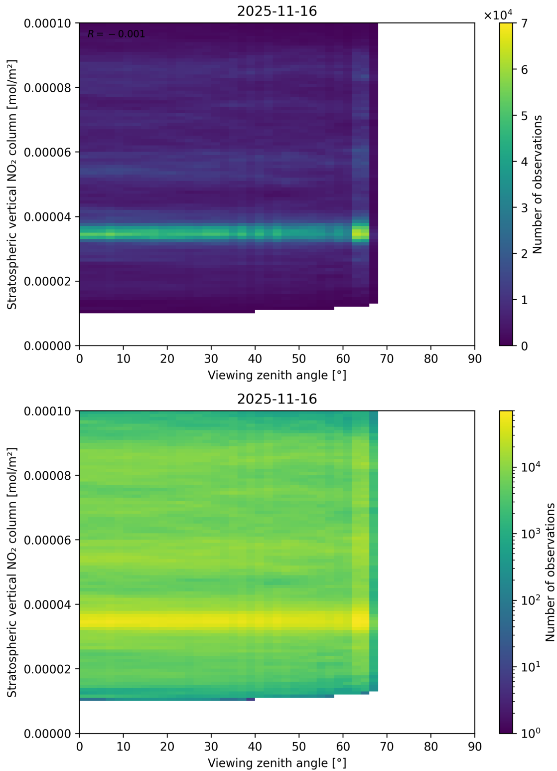
Figure 164: Scatter density plot of “Viewing zenith angle” against “Stratospheric vertical NO 2 column” for 2025-11-15 to 2025-11-17.
