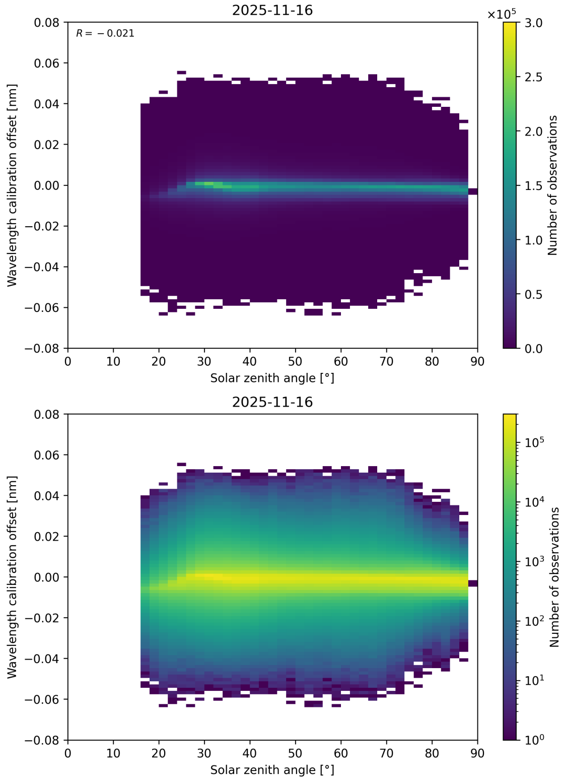
Figure 158: Scatter density plot of “Solar zenith angle” against “Wavelength calibration offset” for 2025-11-15 to 2025-11-17.
