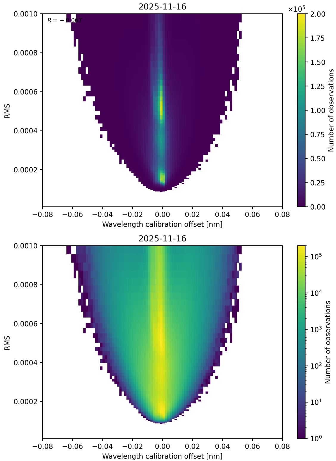
Figure 181: Scatter density plot of “Wavelength calibration offset” against “RMS” for 2025-11-15 to 2025-11-17.
