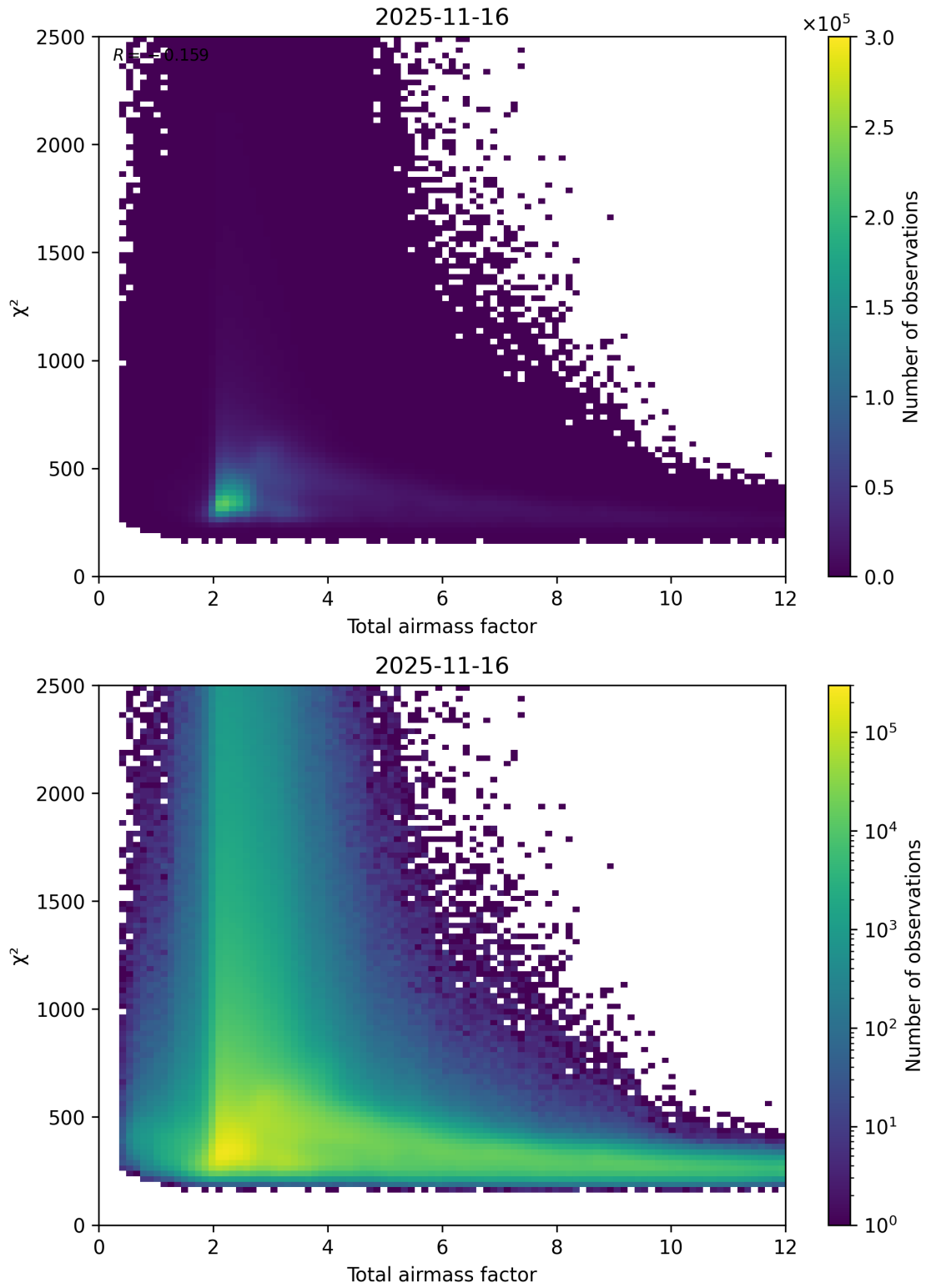
Figure 63: Scatter density plot of “Total airmass factor” against “ \chi^2 ” for 2025-11-15 to 2025-11-17.
