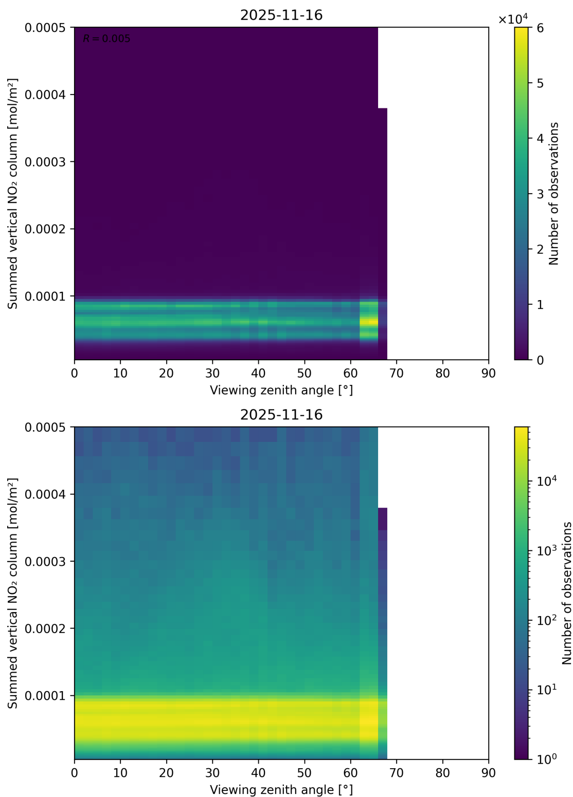
Figure 165: Scatter density plot of “Viewing zenith angle” against “Summed vertical NO 2 column” for 2025-11-15 to 2025-11-17.
