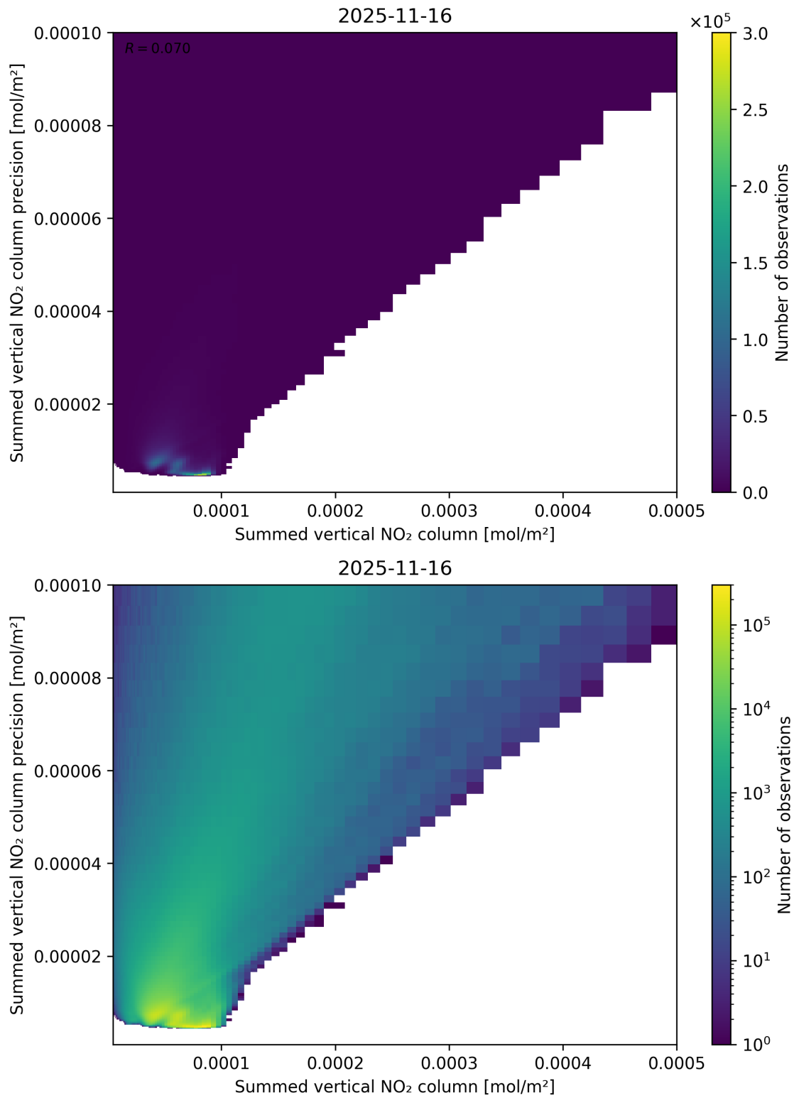
Figure 105: Scatter density plot of “Summed vertical NO 2 column” against “Summed vertical NO 2 column precision” for 2025-11-15 to 2025-11-17.
