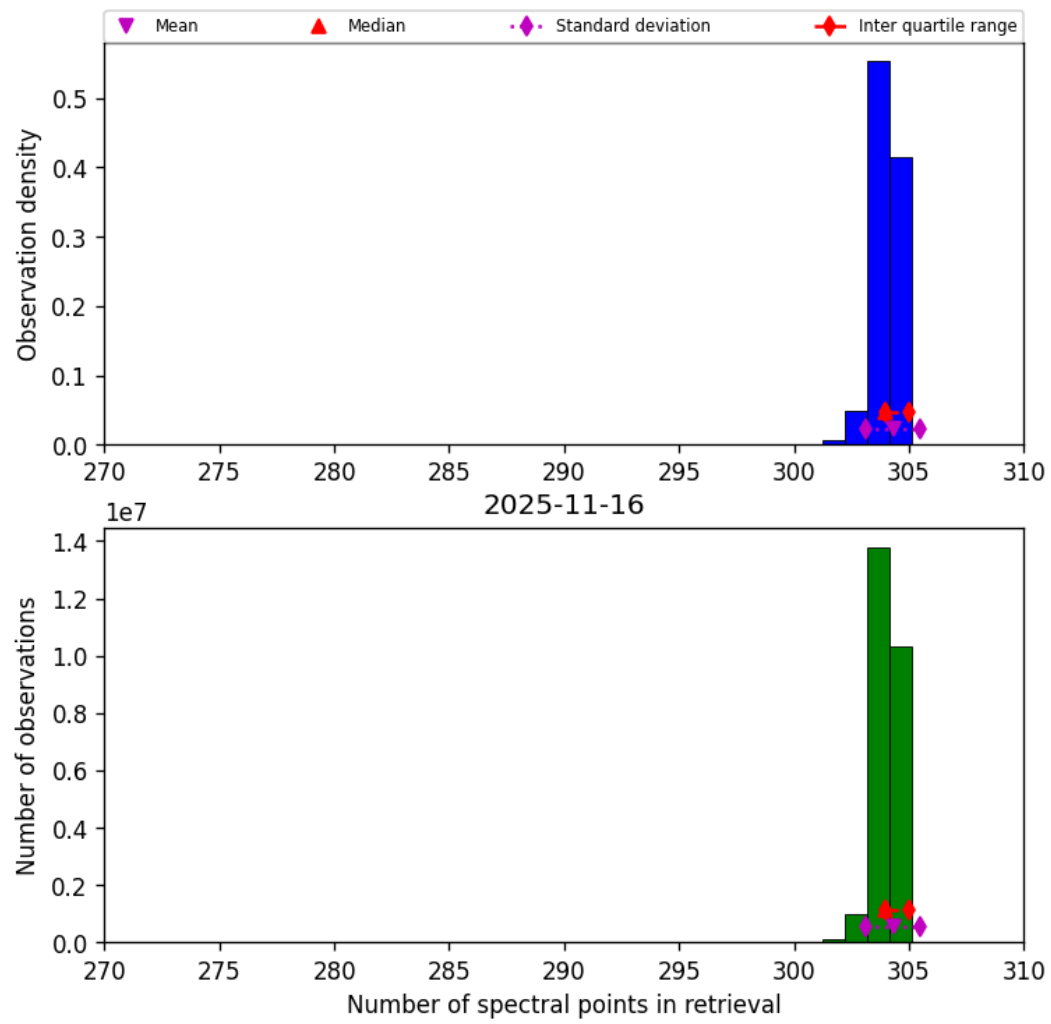
Figure 33: Histogram of “Number of spectral points in retrieval” for 2025-11-15 to 2025-11-17
