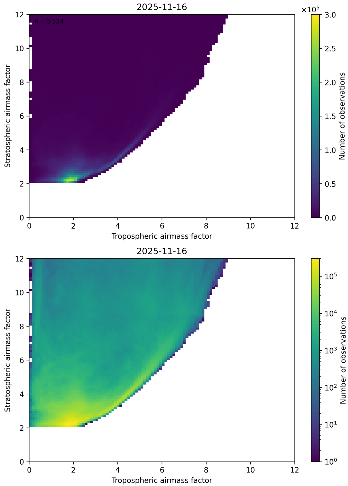
Figure 71: Scatter density plot of “Tropospheric airmass factor” against “Stratospheric airmass factor” for 2025-11-15 to 2025-11-17.
