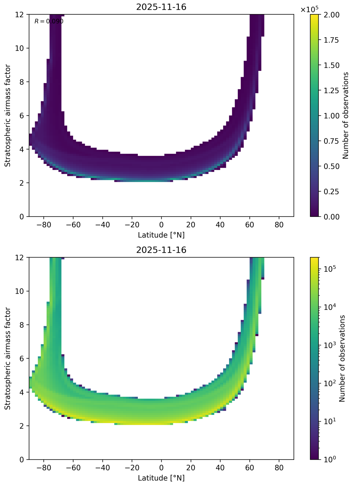
Figure 83: Scatter density plot of “Latitude” against “Stratospheric airmass factor” for 2025-11-15 to 2025-11-17.
