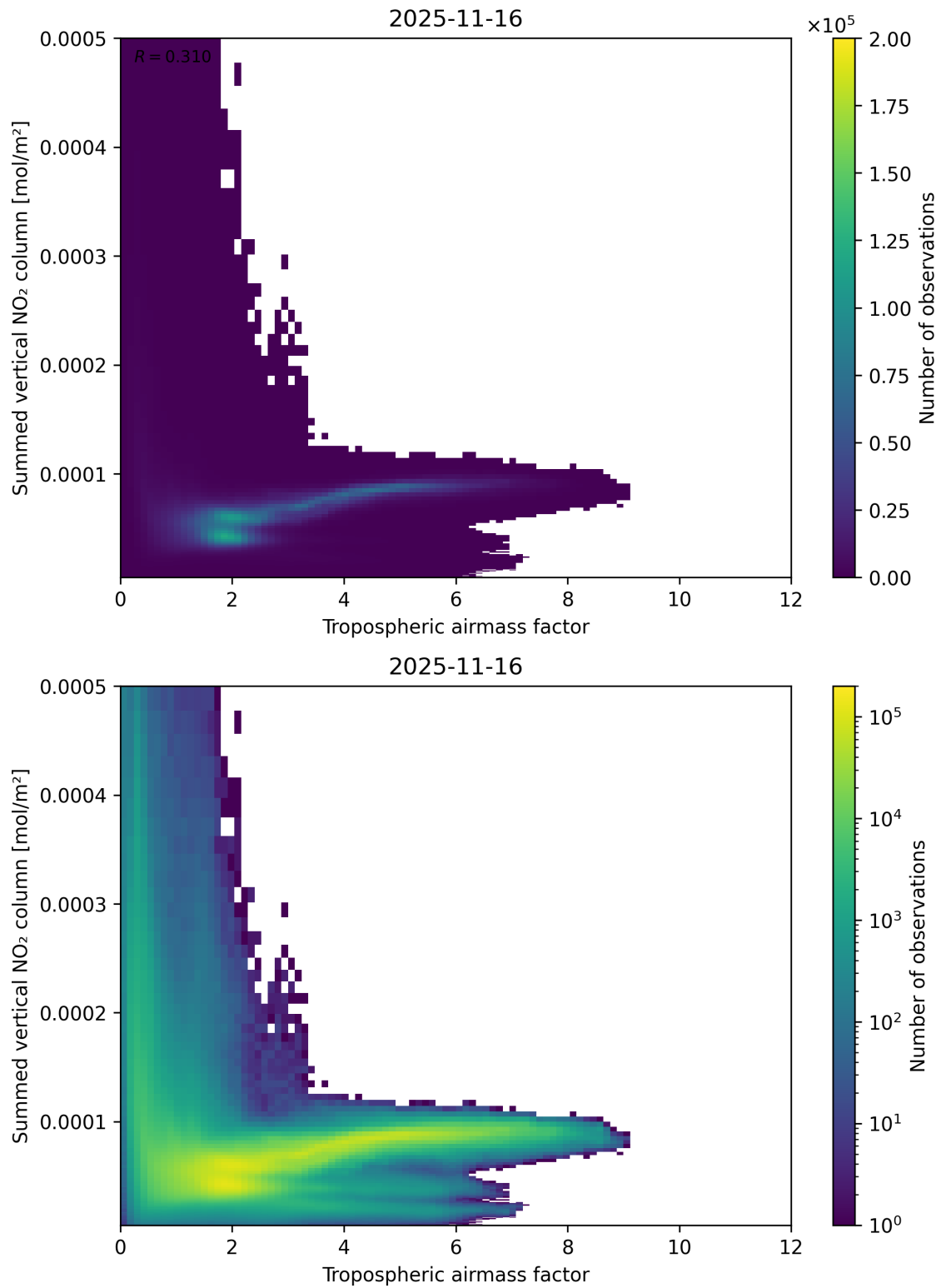
Figure 75: Scatter density plot of “Tropospheric airmass factor” against “Summed vertical NO 2 column” for 2025-11-15 to 2025-11-17.
