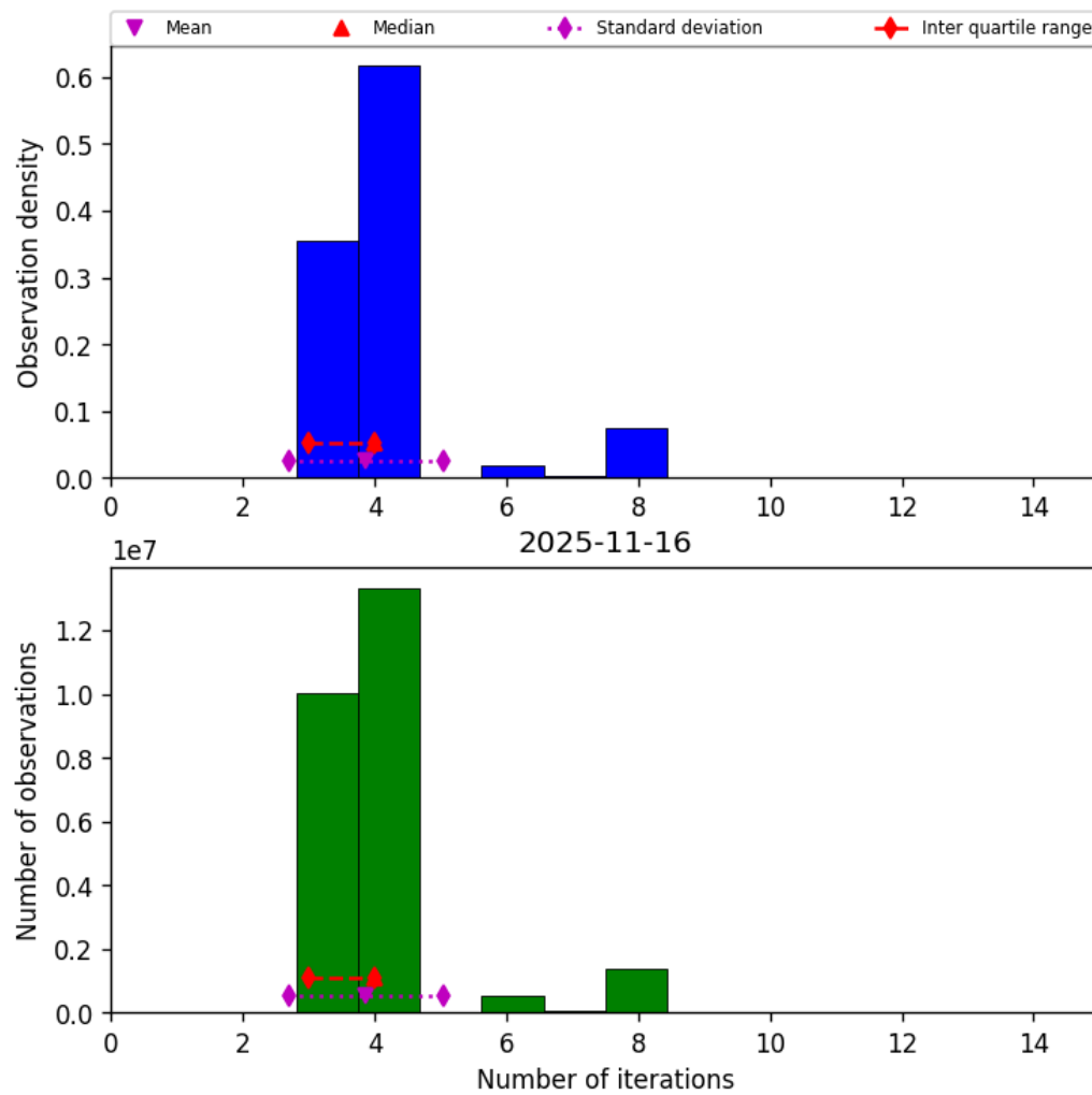
Figure 34: Histogram of “Number of iterations” for 2025-11-15 to 2025-11-17
