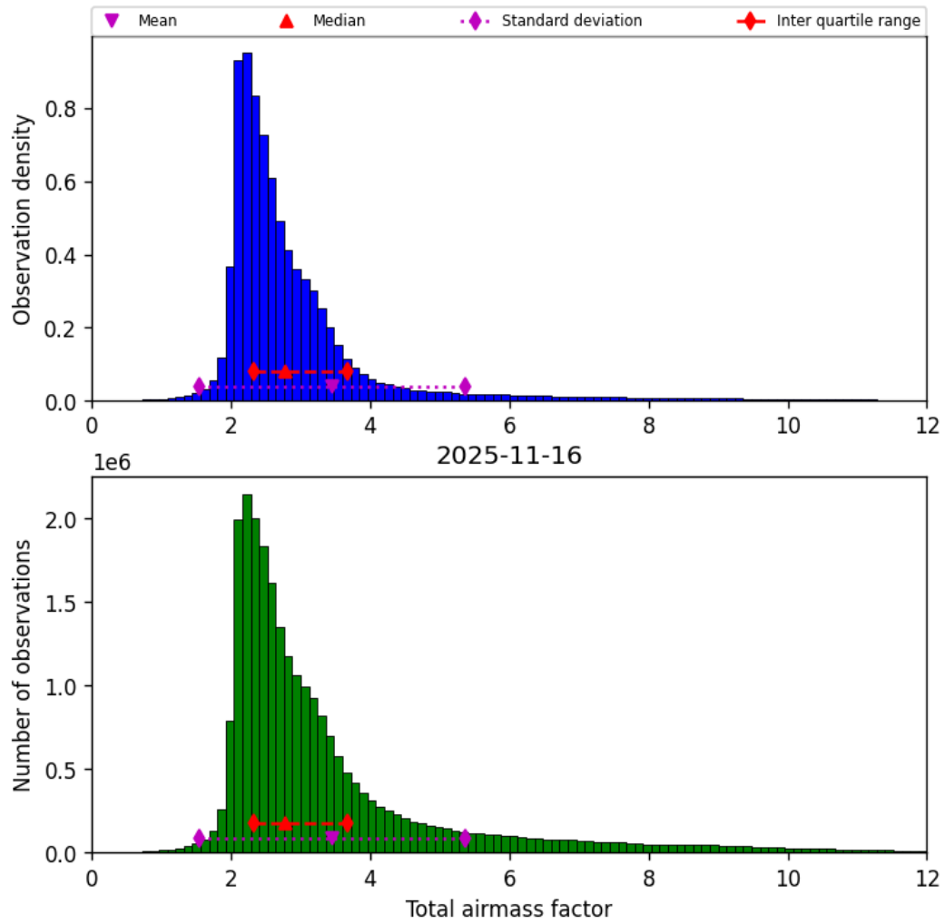
Figure 32: Histogram of “Total airmass factor” for 2025-11-15 to 2025-11-17
