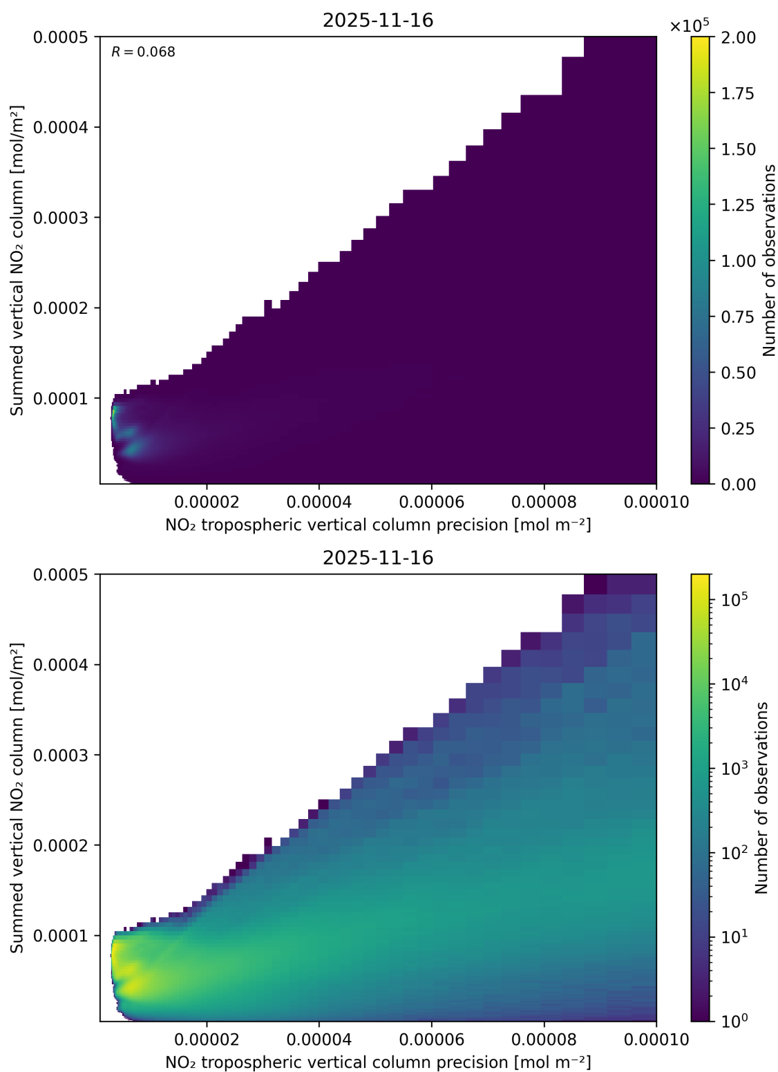
Figure 136: Scatter density plot of “NO 2 tropospheric vertical column precision” against “Summed vertical NO 2 column” for 2025-11-15 to 2025-11-17.
