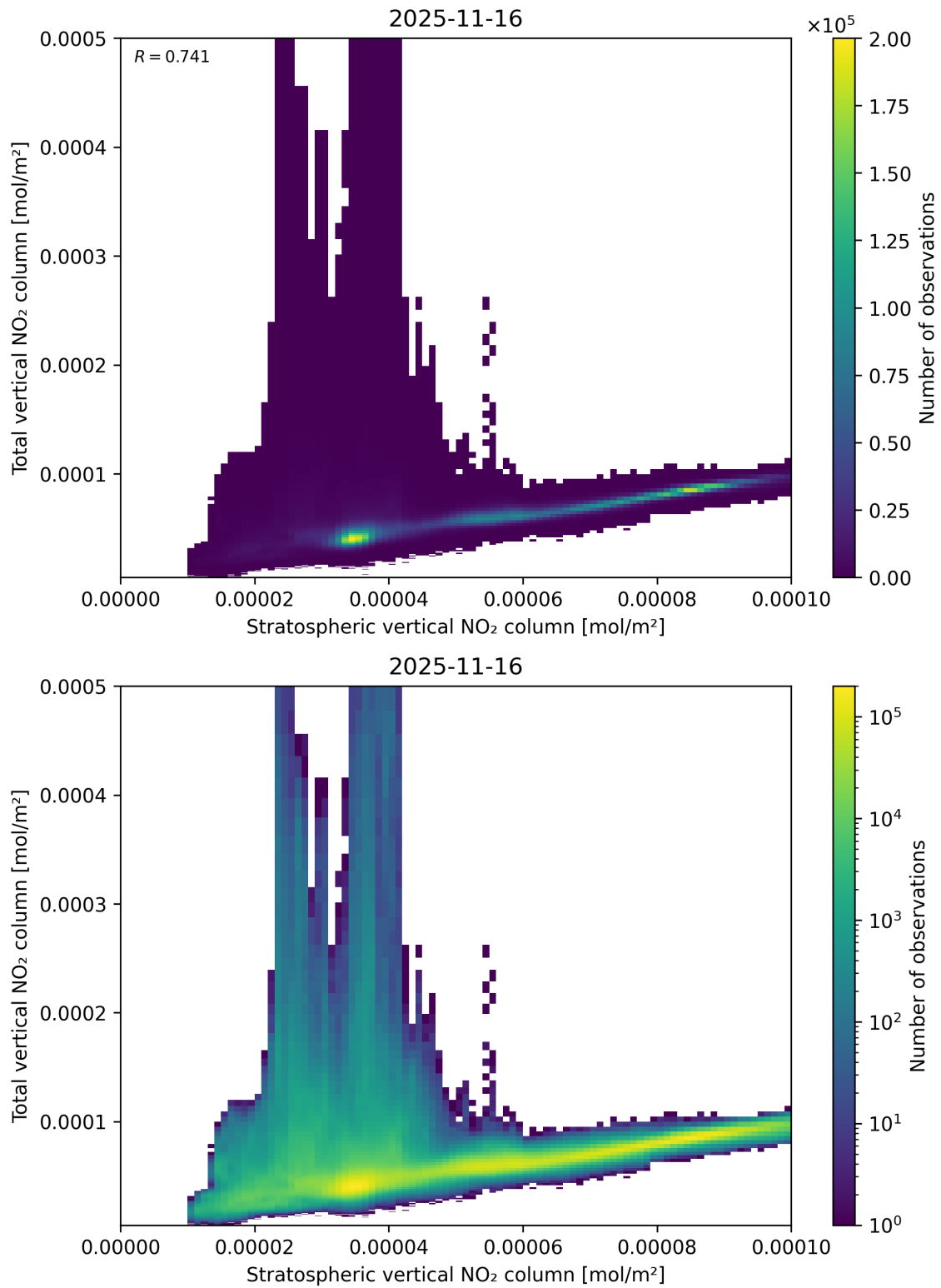
Figure 100: Scatter density plot of “Stratospheric vertical NO 2 column” against “Total vertical NO 2 column” for 2025-11-15 to 2025-11-17.
