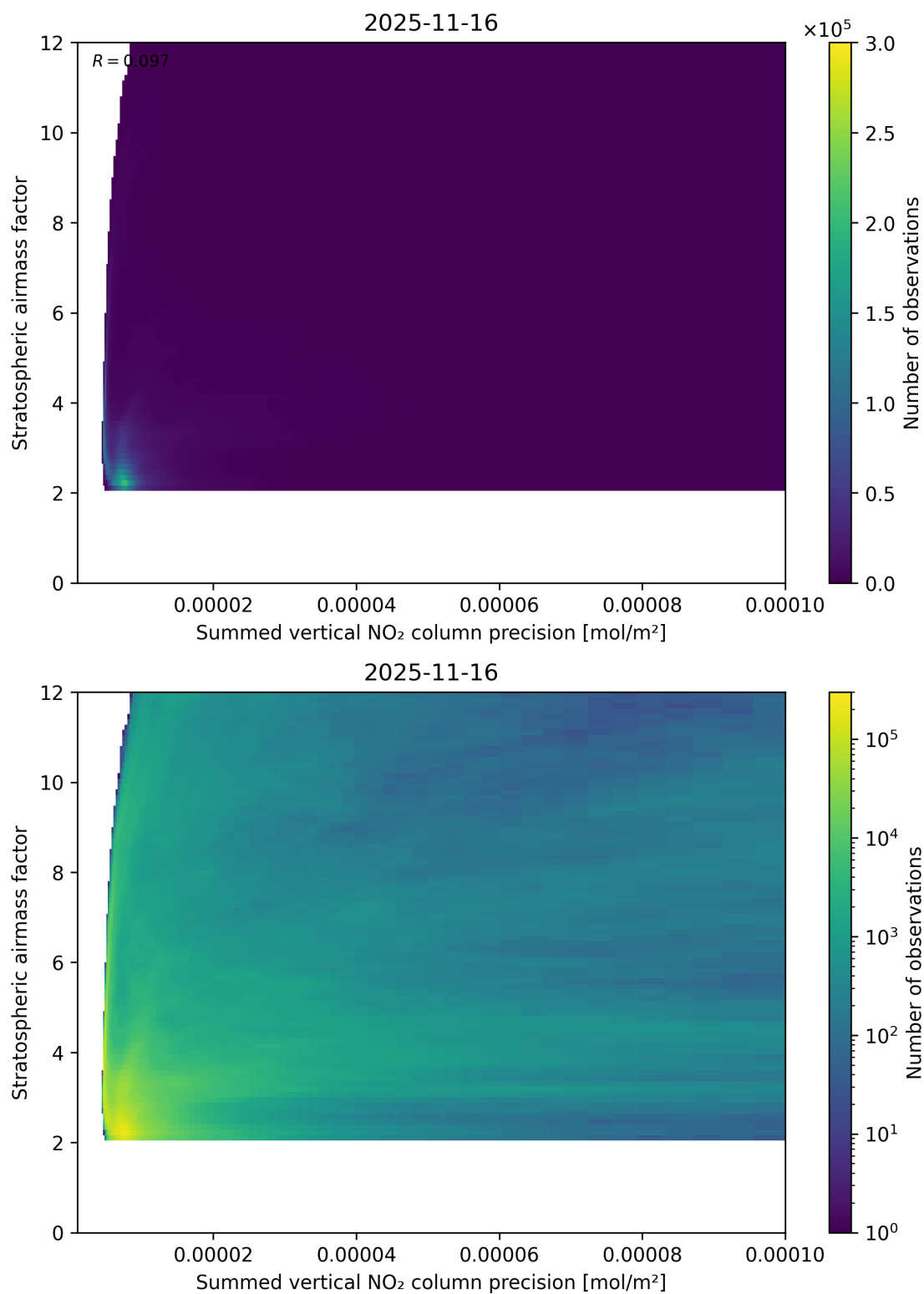
Figure 106: Scatter density plot of “Summed vertical NO 2 column precision” against “Stratospheric airmass factor” for 2025-11-15 to 2025-11-17.
