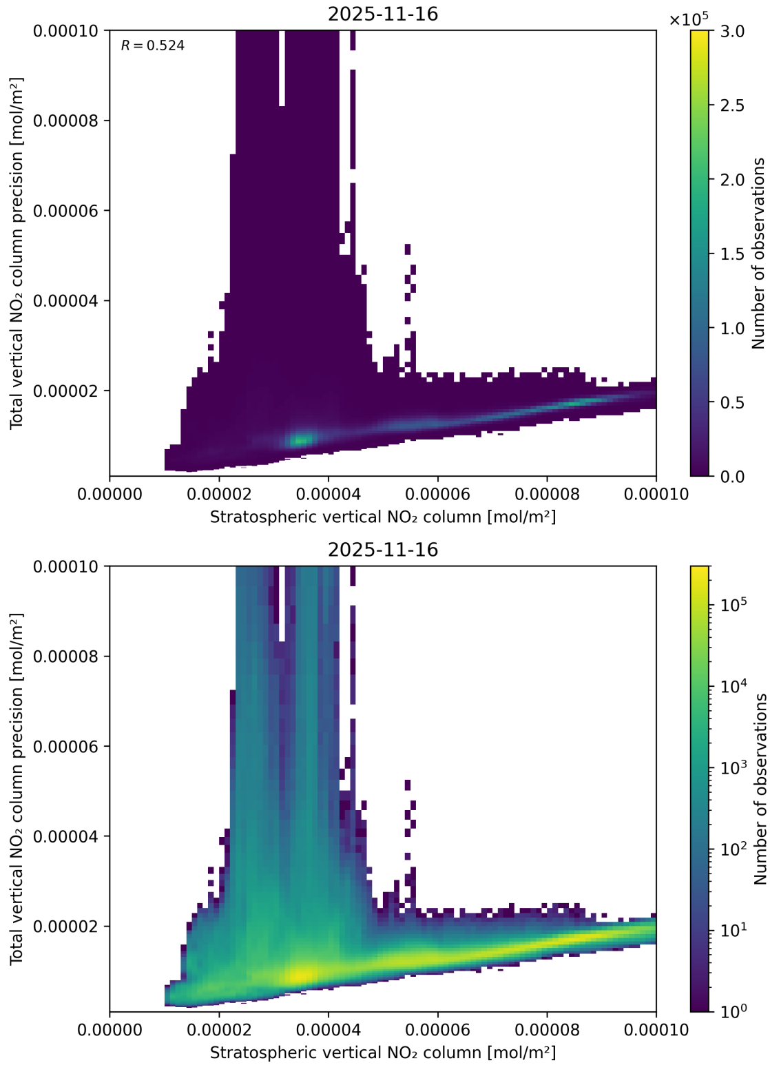
Figure 101: Scatter density plot of “Stratospheric vertical NO 2 column” against “Total vertical NO 2 column precision” for 2025-11-15 to 2025-11-17.
