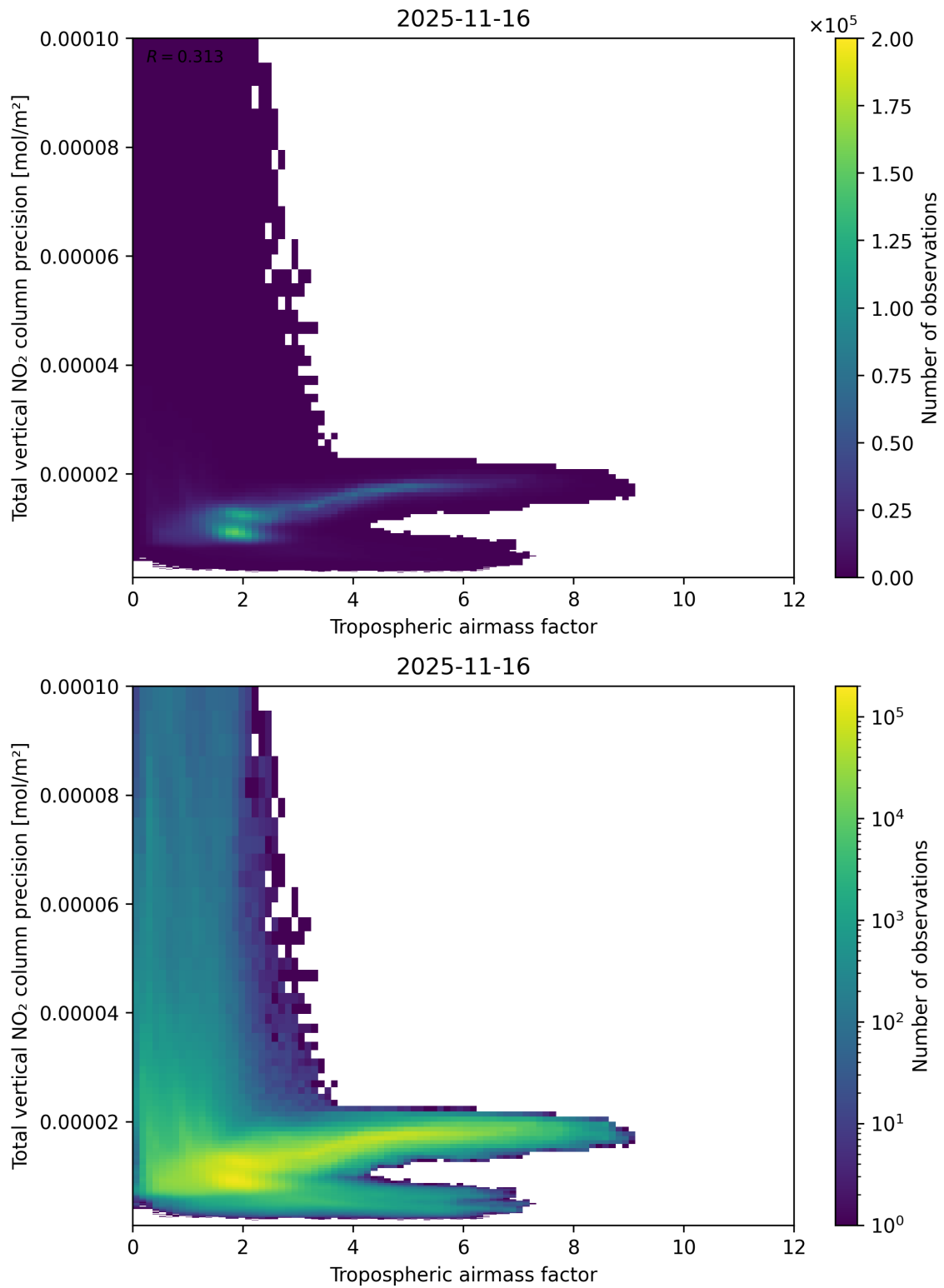
Figure 78: Scatter density plot of “Tropospheric air mass factor” against “Total vertical NO 2 column precision” for 2025-11-15 to 2025-11-17.
