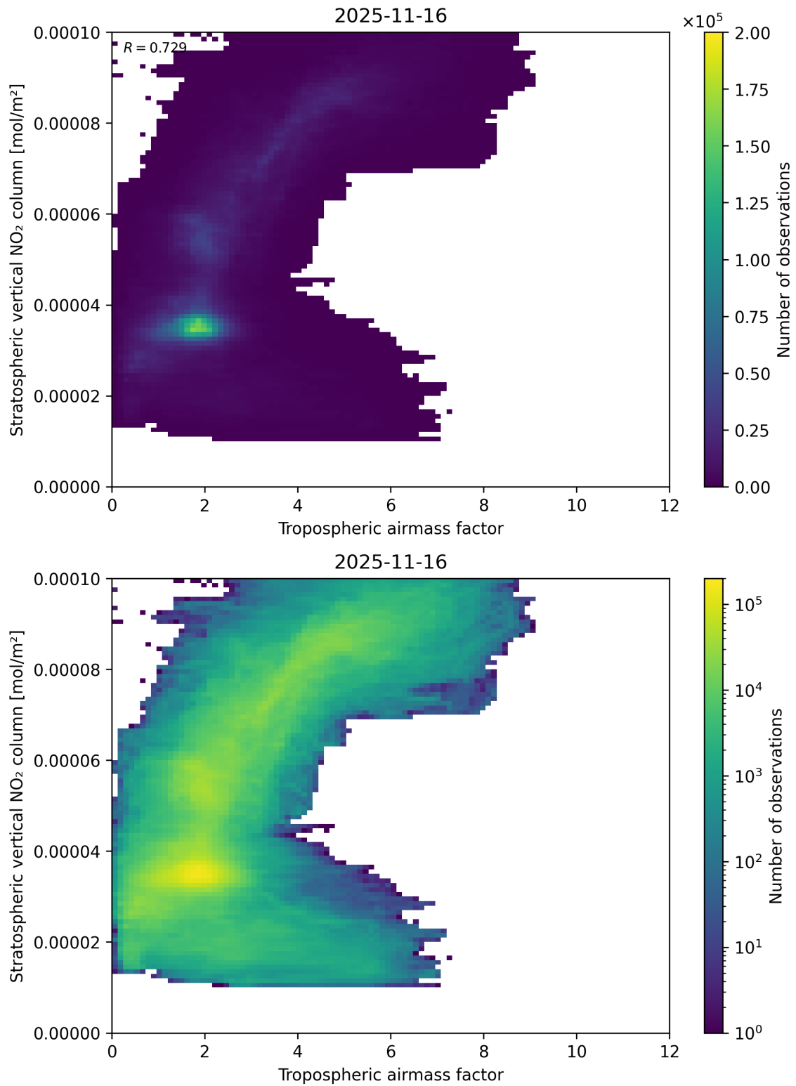
Figure 74: Scatter density plot of “Tropospheric airmass factor” against “Stratospheric vertical NO 2 column” for 2025-11-15 to 2025-11-17.
