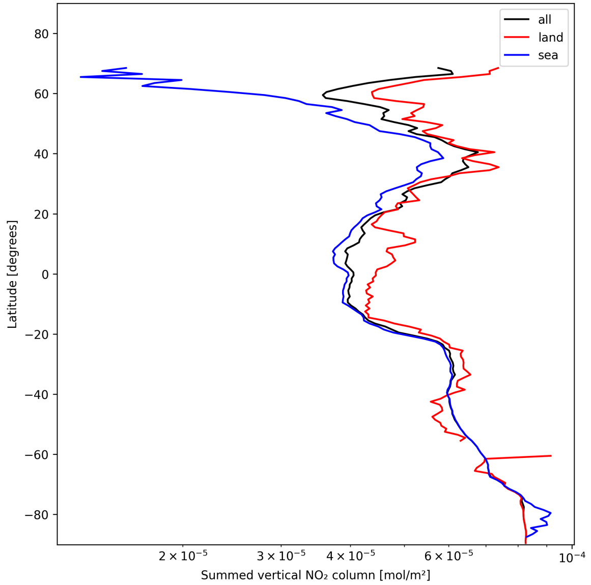
Figure 23: Zonal average of “Summed vertical NO 2 column” for 2025-11-18 to 2025-11-20.
