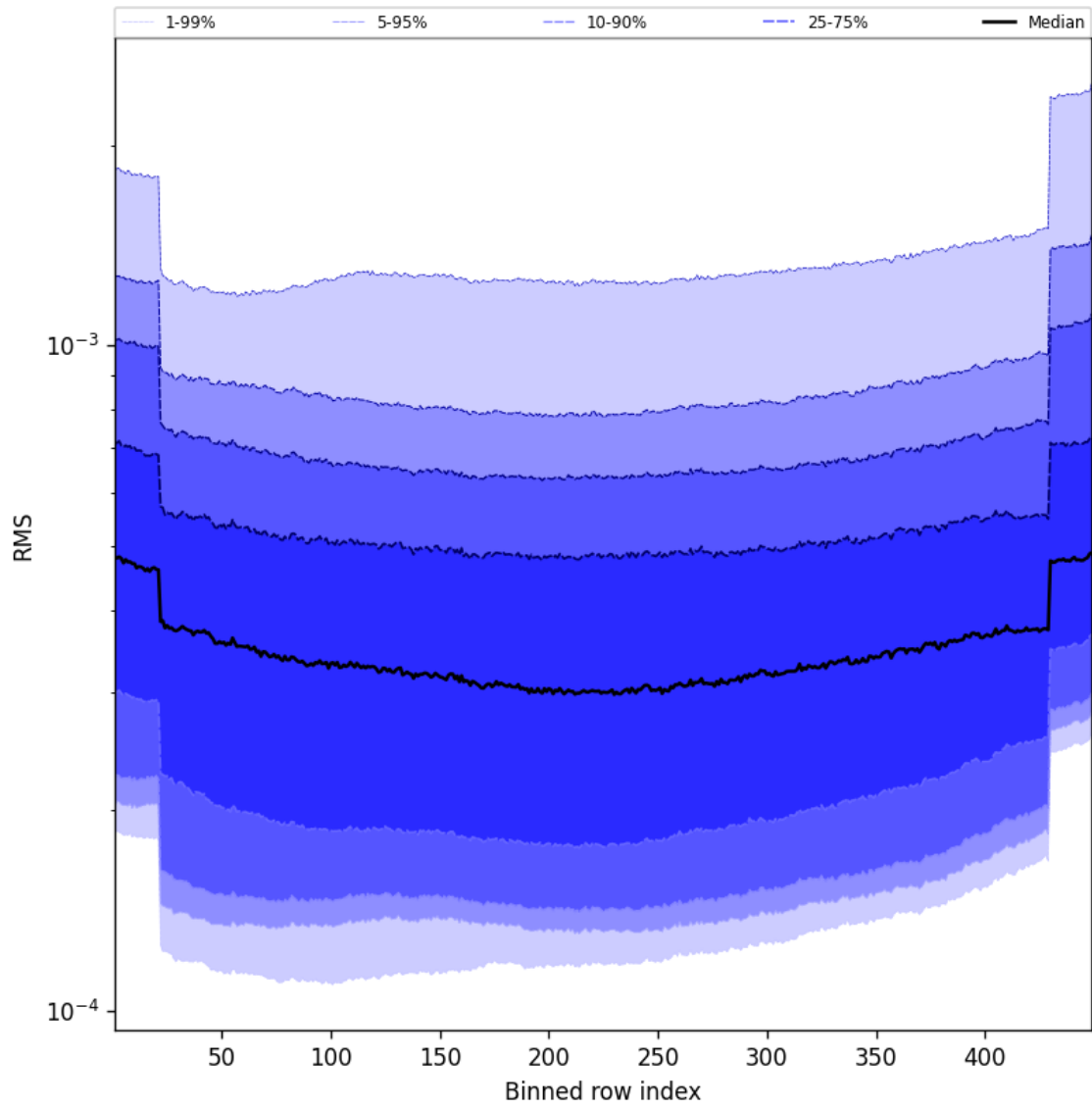
Figure 60: Along track statistics of “RMS” for 2025-11-18 to 2025-11-20
