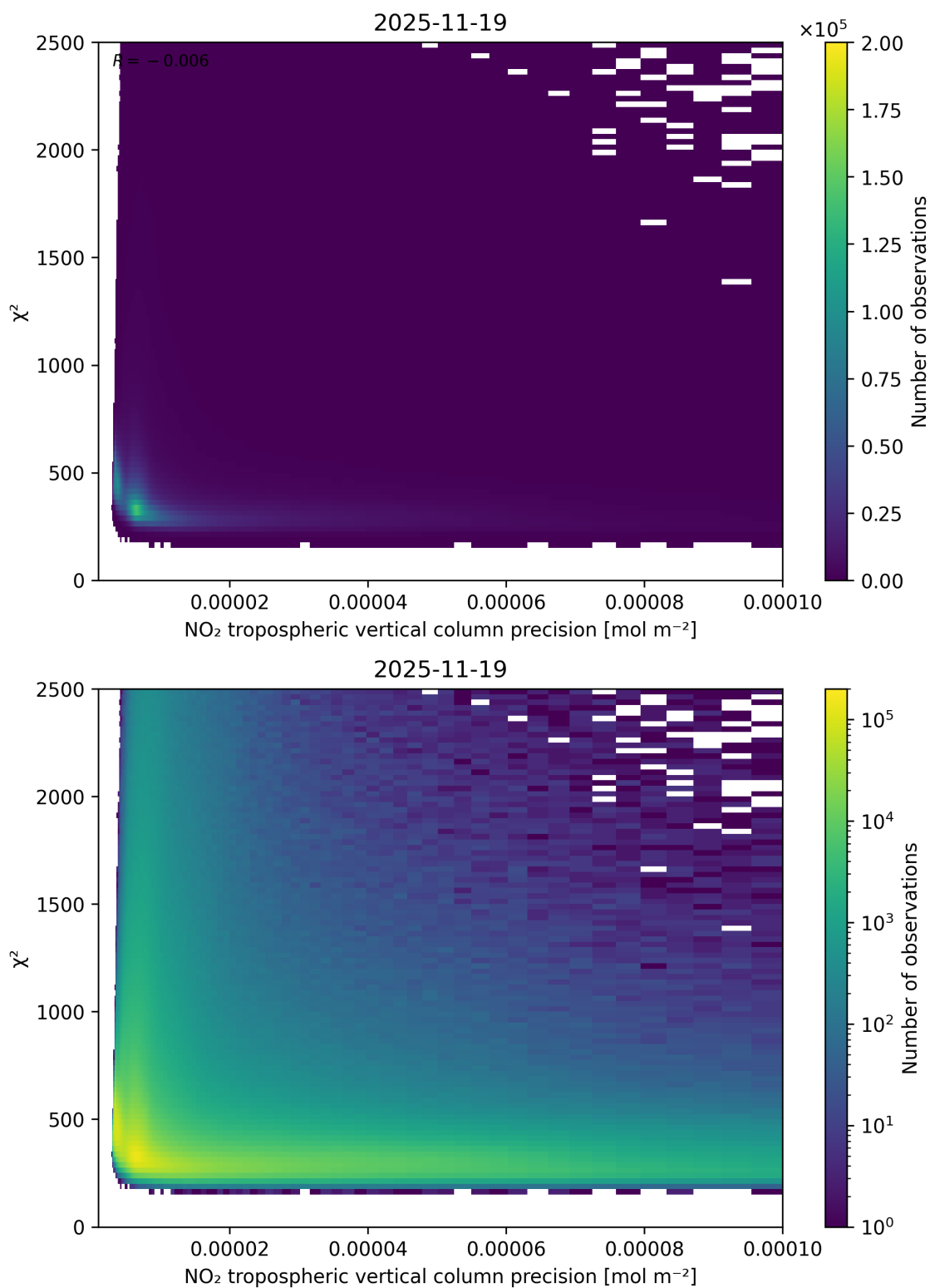
Figure 134: Scatter density plot of “NO 2 tropospheric vertical column precision” against “ \chi^2 ” for 2025-11-18 to 2025-11-20.
