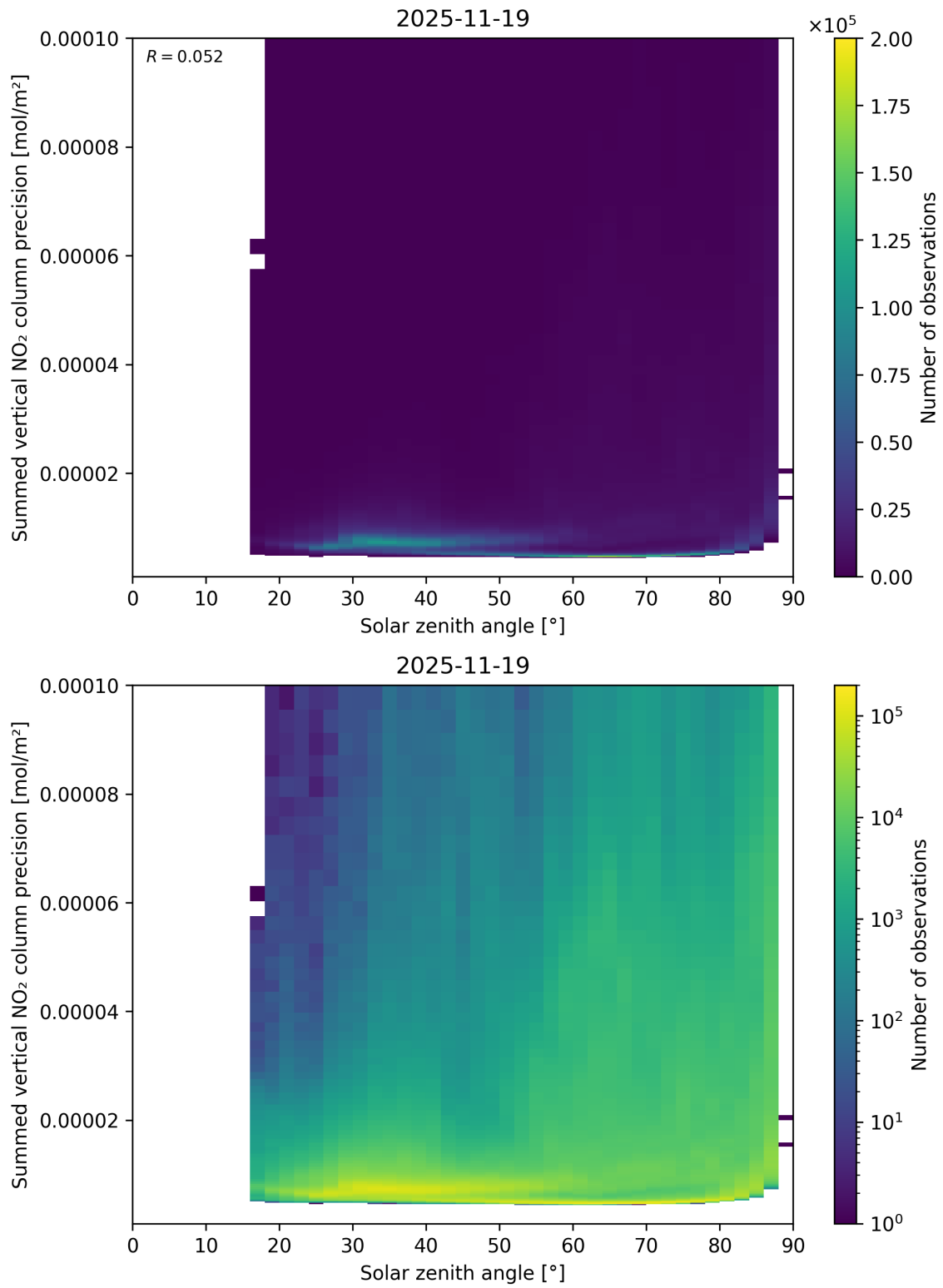
Figure 152: Scatter density plot of “Solar zenith angle” against “Summed vertical NO 2 column precision” for 2025-11-18 to 2025-11-20.
