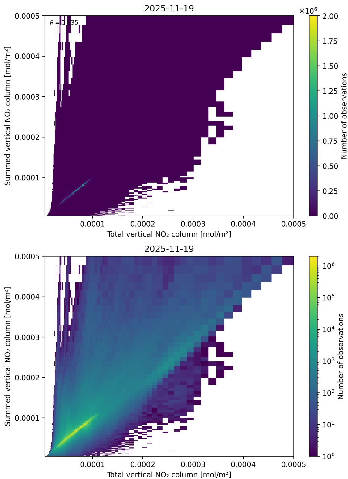
Figure 112: Scatter density plot of “Total vertical NO 2 column” against “Summed vertical NO 2 column” for 2025-11-18 to 2025-11-20.
