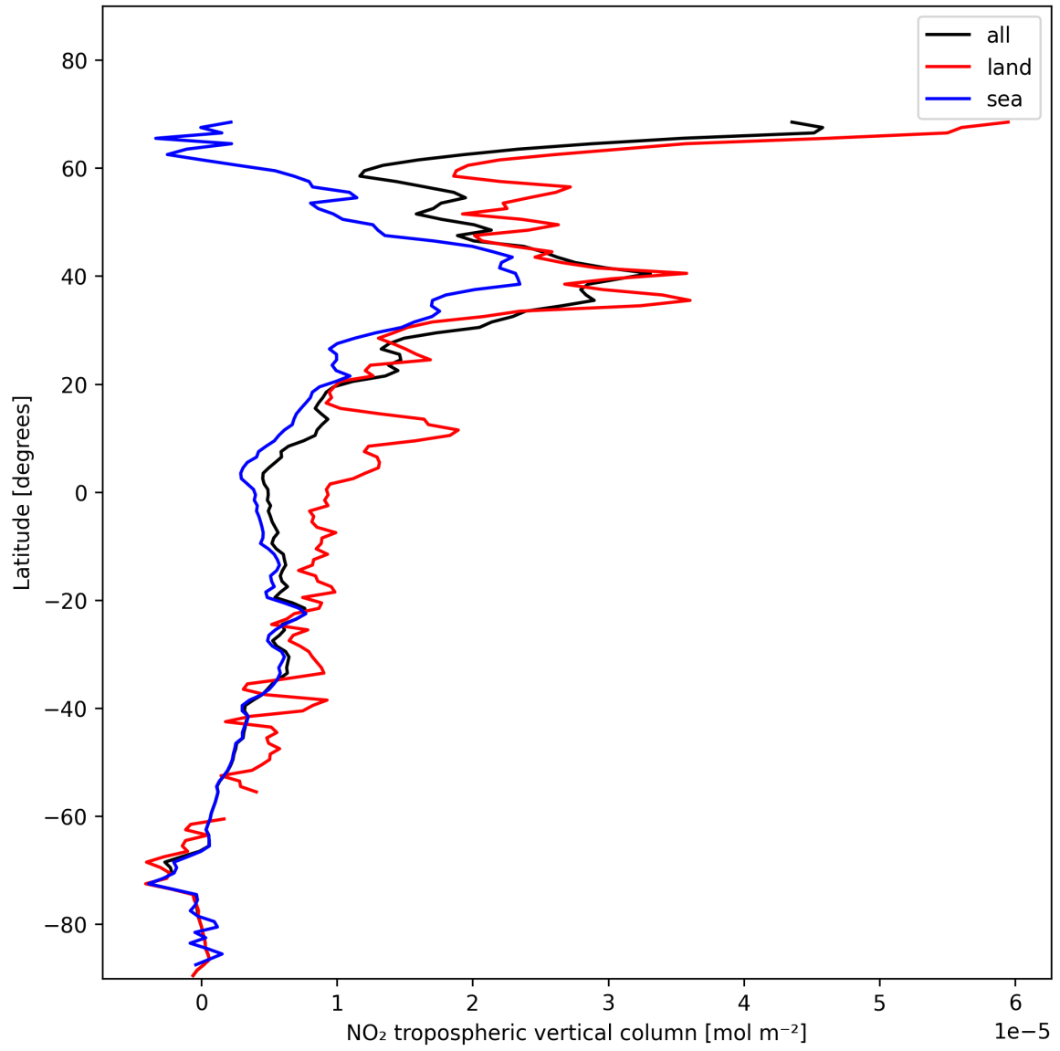
Figure 12: Zonal average of “NO 2 tropospheric vertical column” for 2025-11-18 to 2025-11-20.
