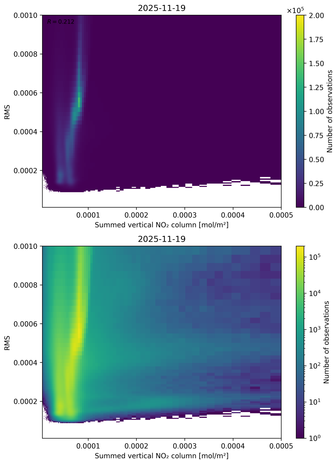
Figure 109: Scatter density plot of “Summed vertical NO 2 column” against “RMS” for 2025-11-18 to 2025-11-20.
