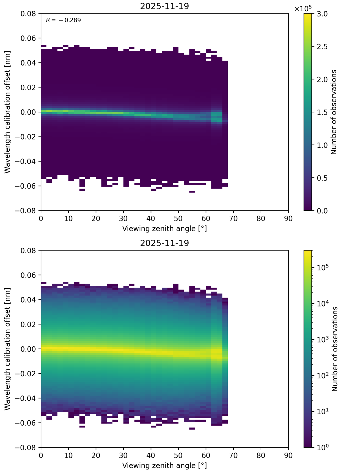
Figure 173: Scatter density plot of “Viewing zenith angle” against “Wavelength calibration offset” for 2025-11-18 to 2025-11-20.
