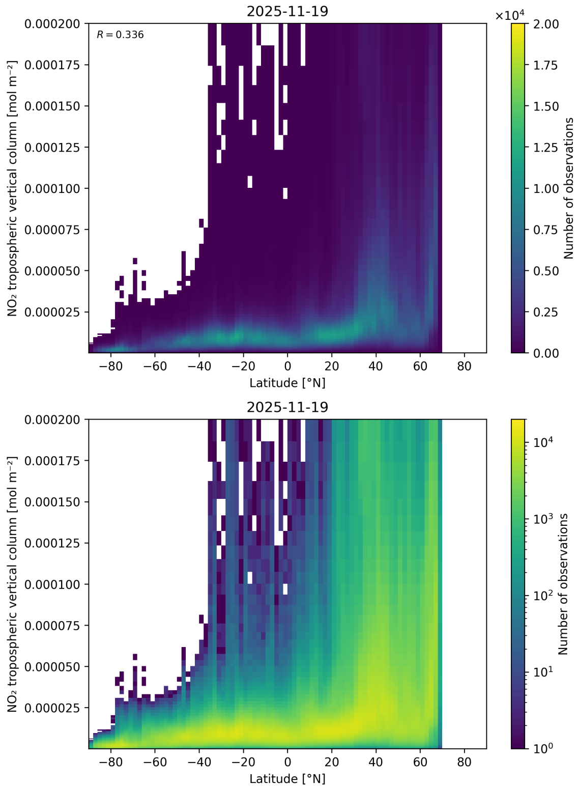
Figure 92: Scatter density plot of “Latitude” against “NO 2 tropospheric vertical column” for 2025-11-18 to 2025-11-20.
