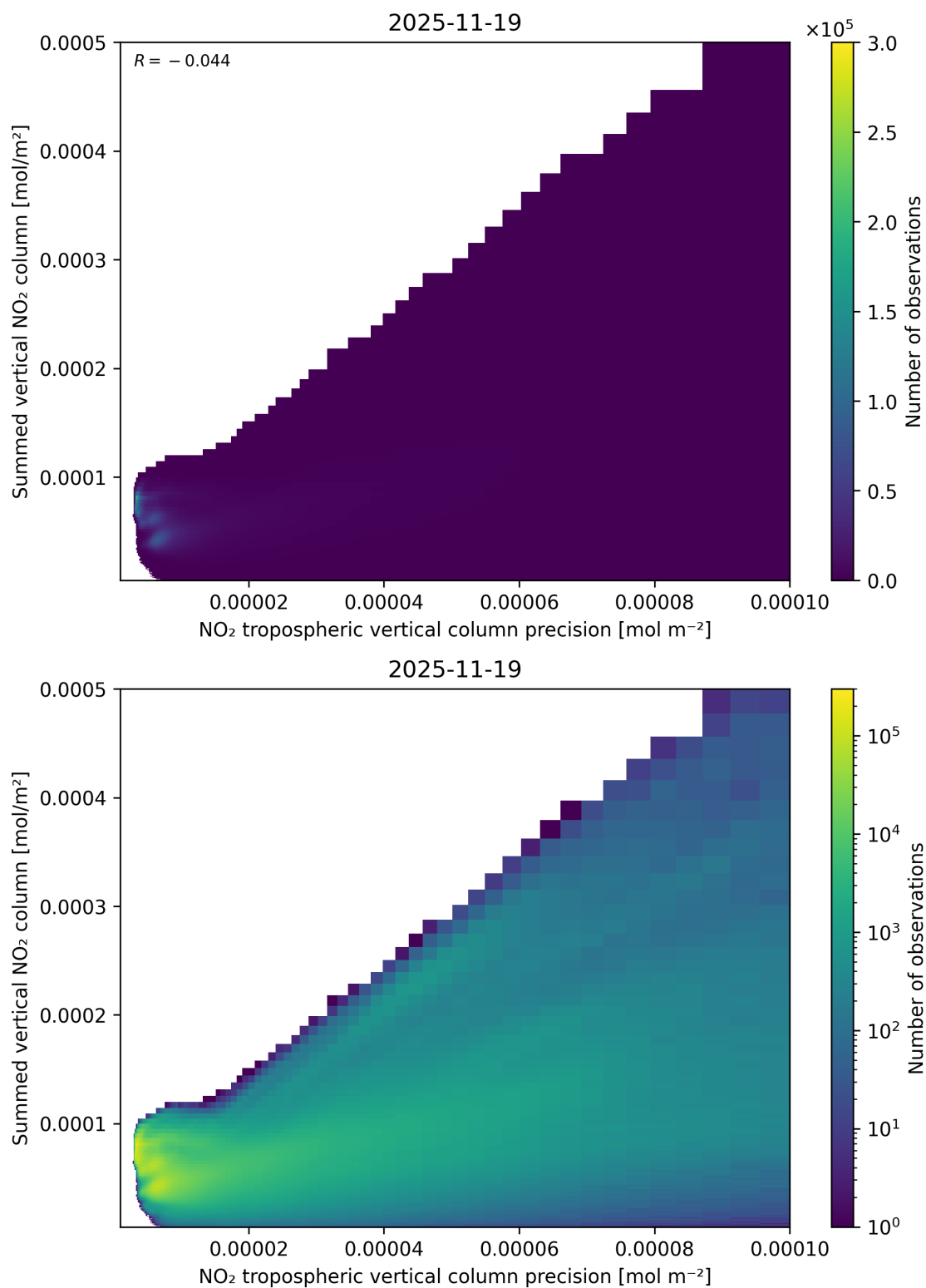
Figure 136: Scatter density plot of “NO 2 tropospheric vertical column precision” against “Summed vertical NO 2 column” for 2025-11-18 to 2025-11-20.
