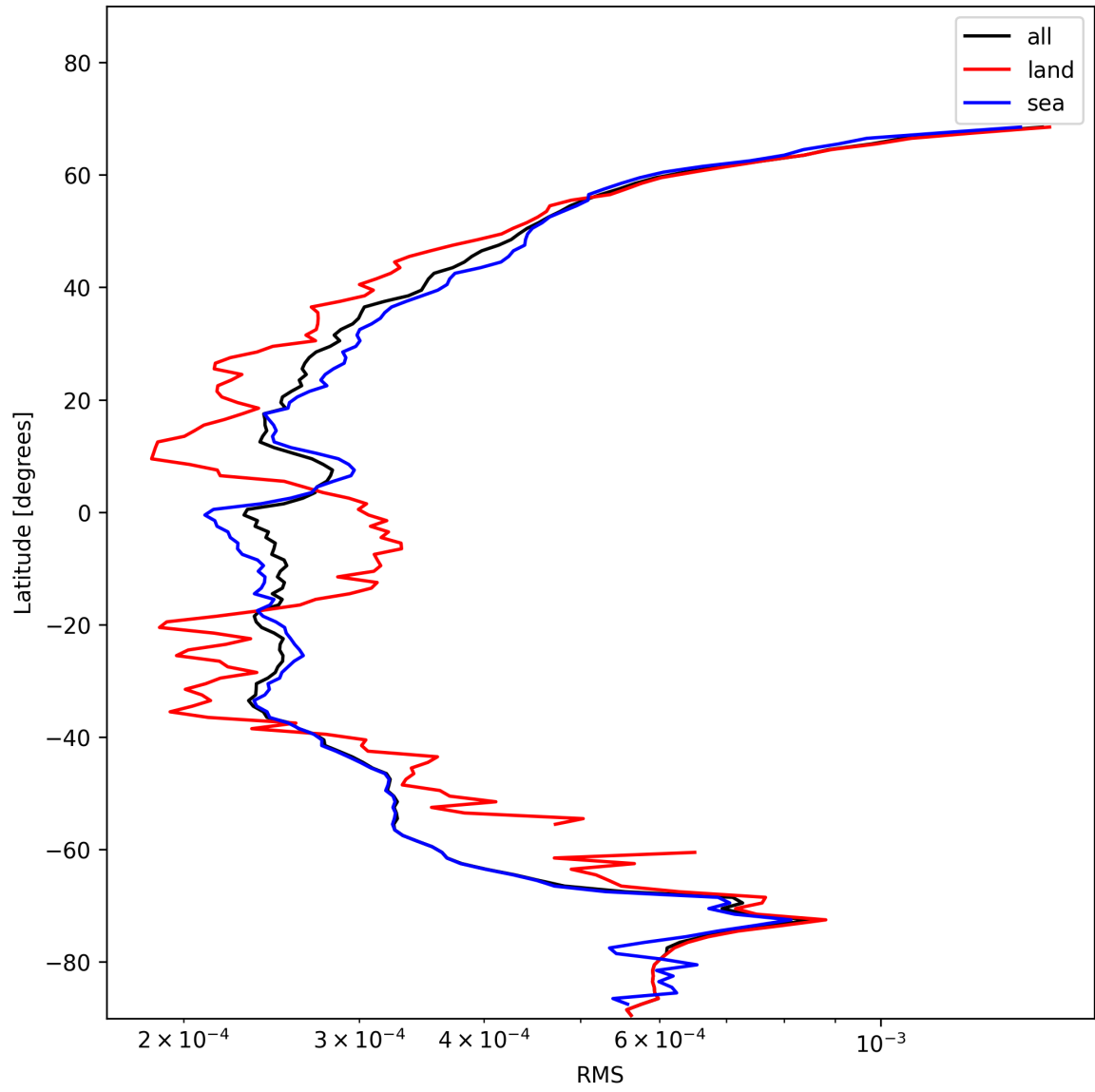
Figure 26: Zonal average of “RMS” for 2025-11-18 to 2025-11-20.
