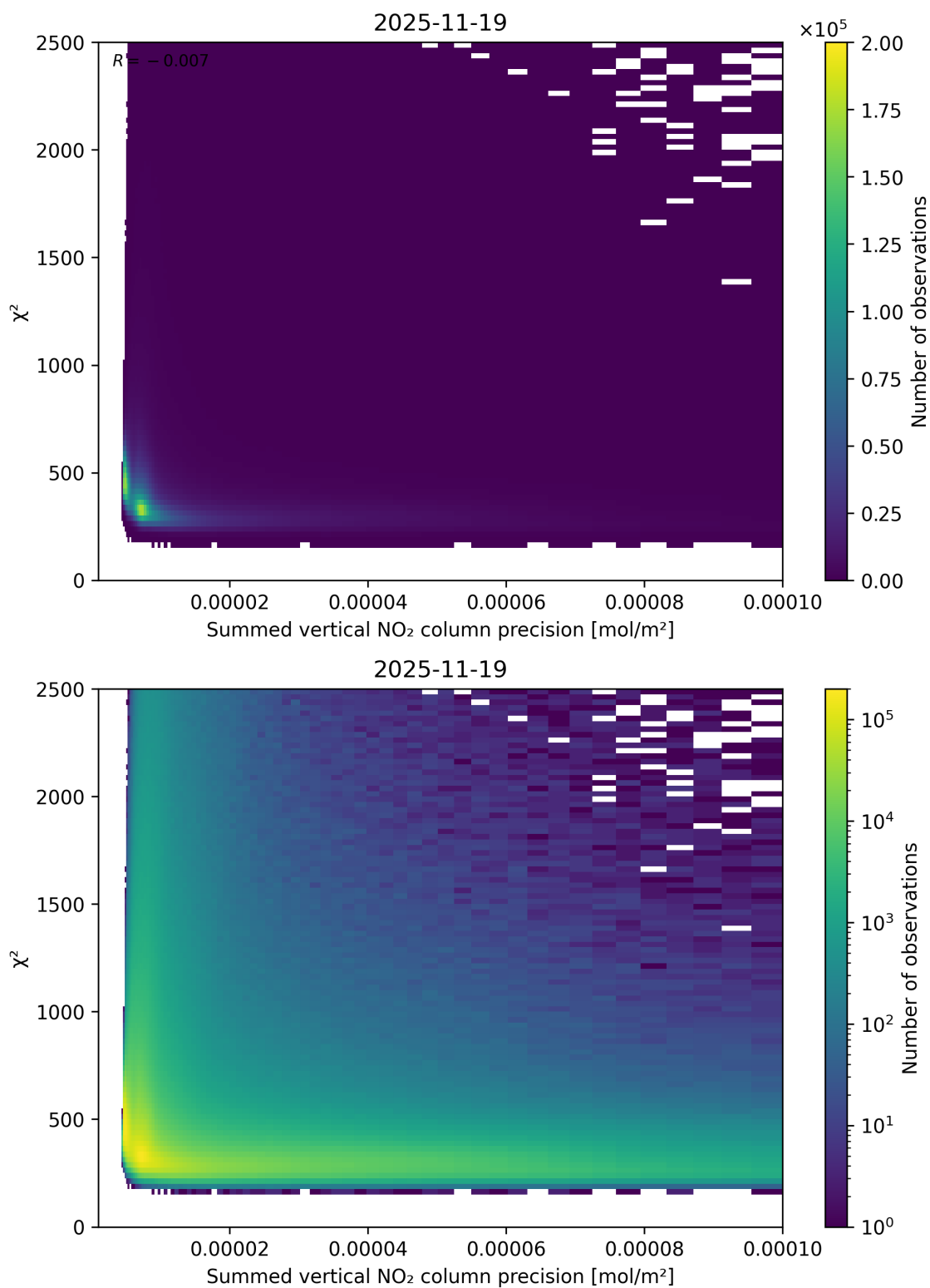
Figure 107: Scatter density plot of “Summed vertical NO 2 column precision” against “ \chi^2 ” for 2025-11-18 to 2025-11-20.
