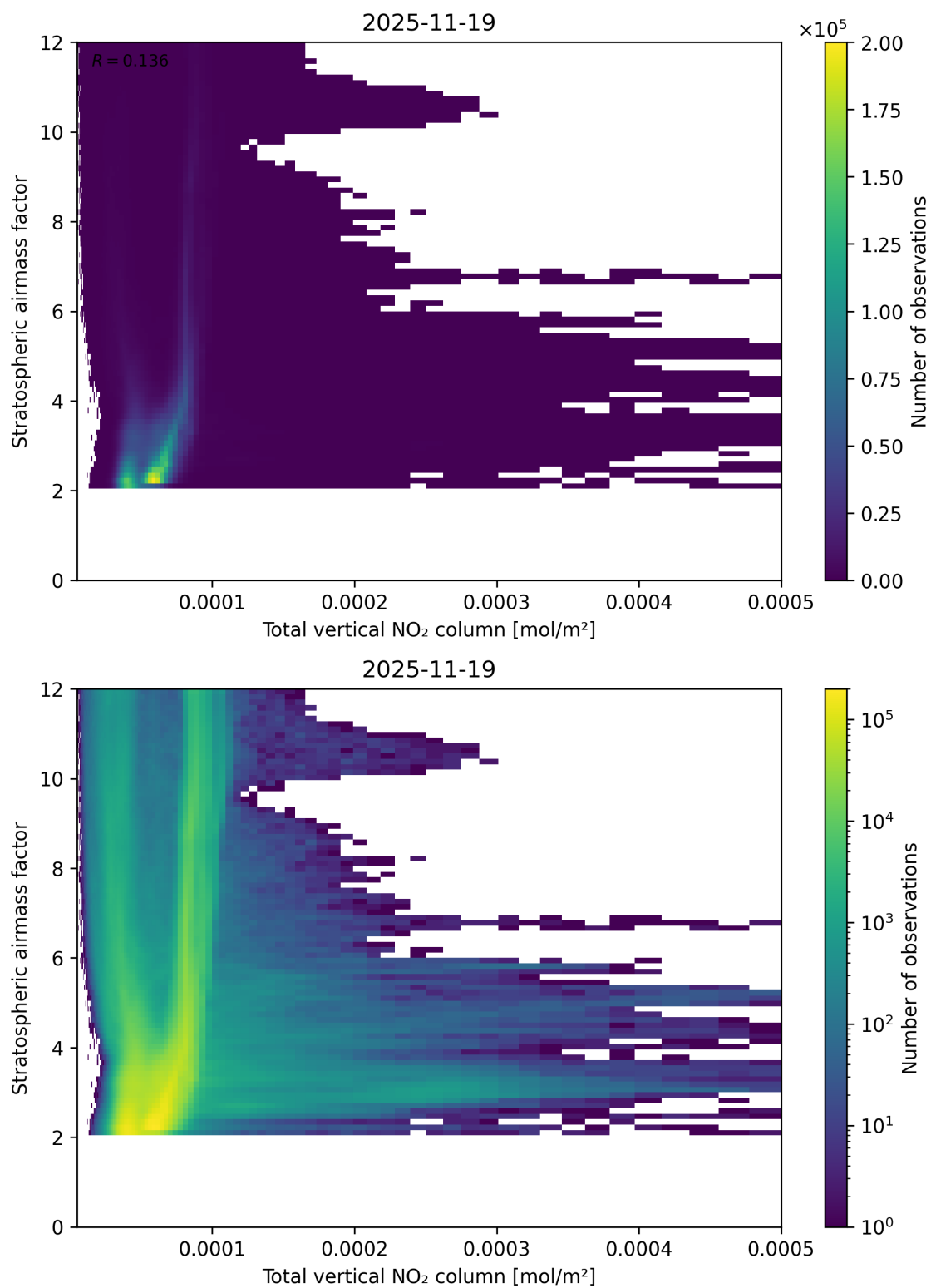
Figure 110: Scatter density plot of “Total vertical NO 2 column” against “Stratospheric airmass factor” for 2025-11-18 to 2025-11-20.
