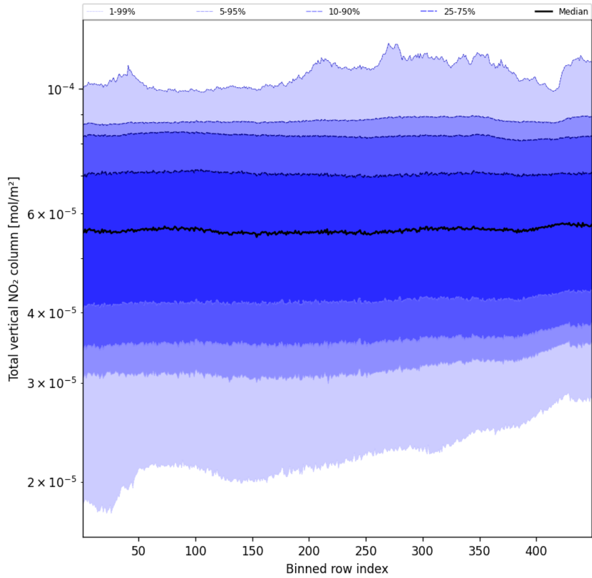
Figure 55: Along track statistics of “Total vertical NO 2 column” for 2025-11-18 to 2025-11-20
