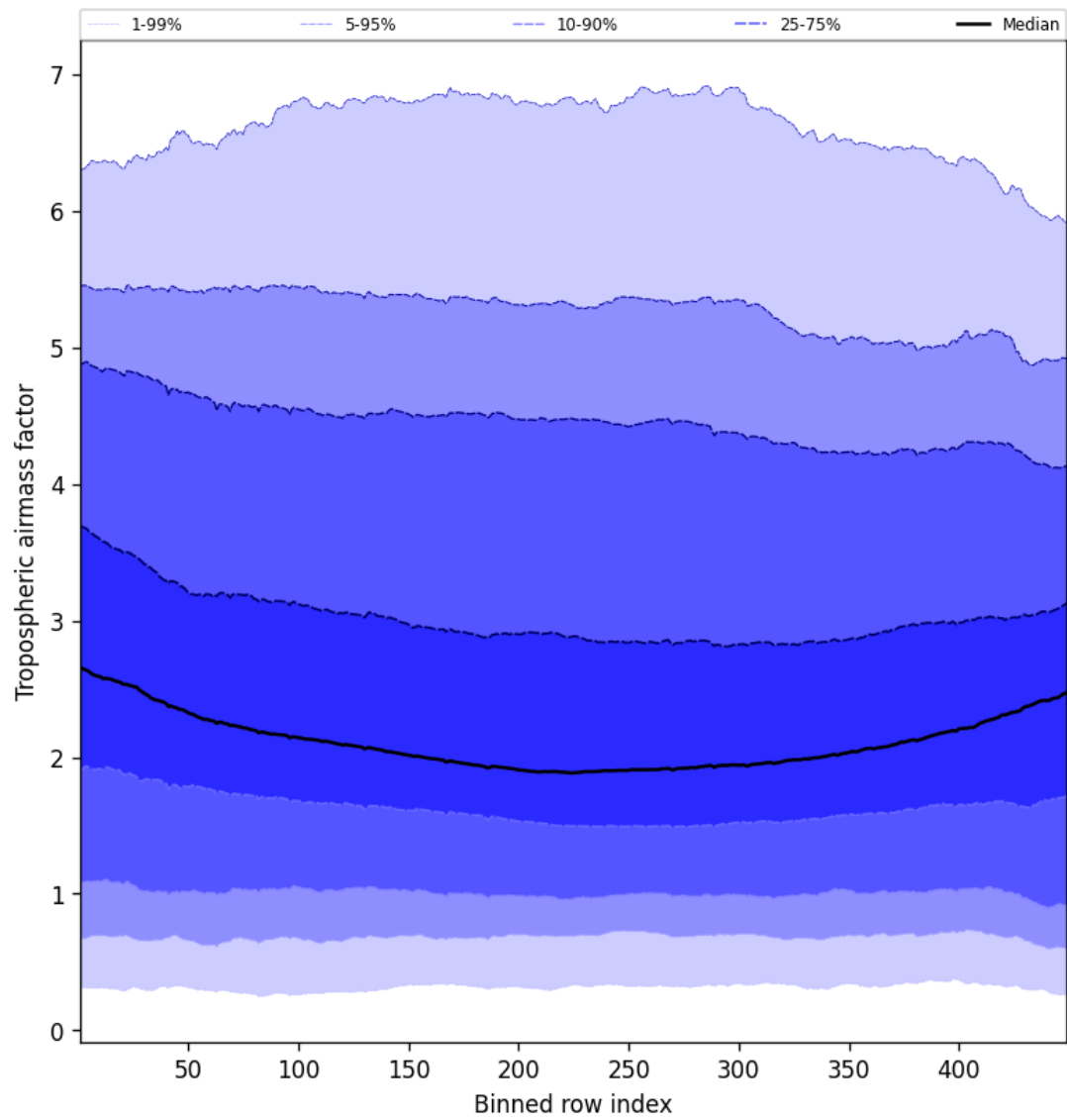
Figure 48: Along track statistics of “Tropospheric airmass factor” for 2025-11-18 to 2025-11-20
