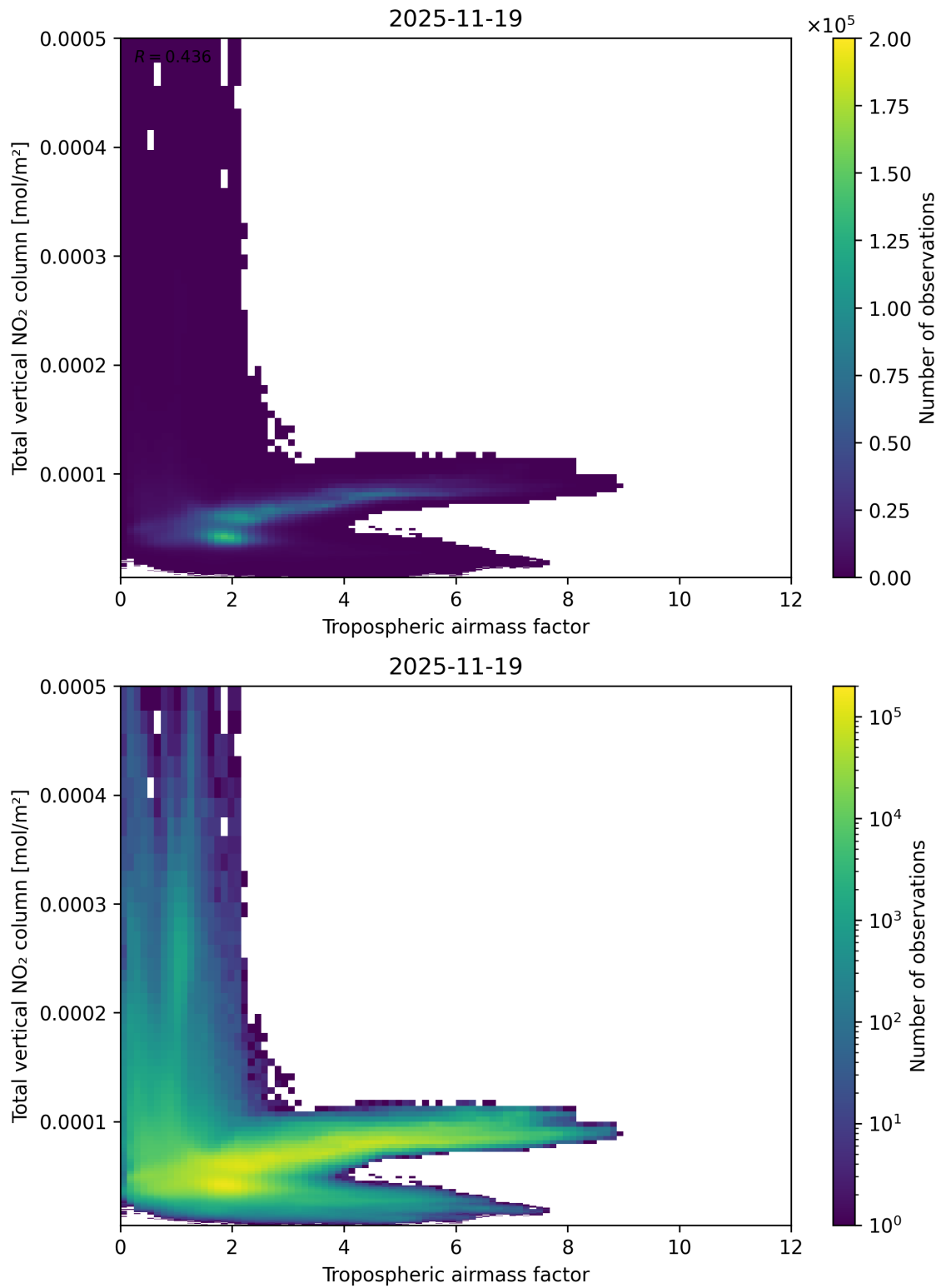
Figure 77: Scatter density plot of “Tropospheric airmass factor” against “Total vertical \text{NO}_2 column” for 2025-11-18 to 2025-11-20.
