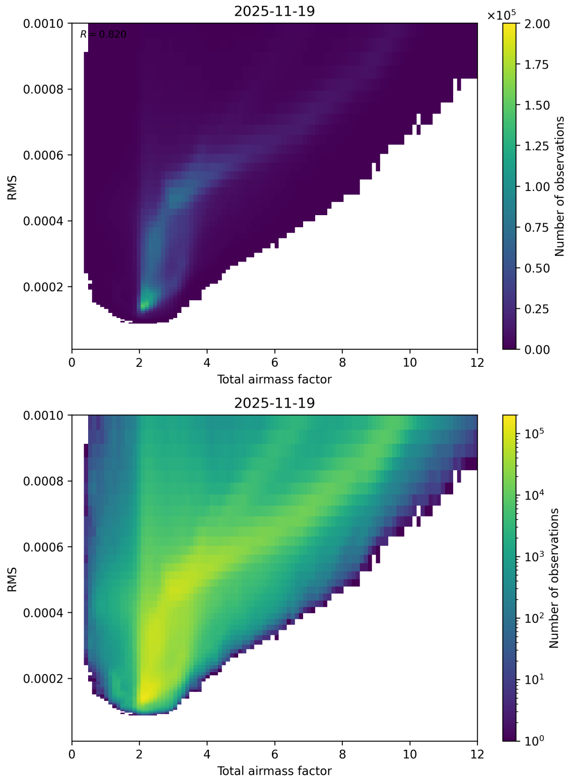
Figure 69: Scatter density plot of “Total airmass factor” against “RMS” for 2025-11-18 to 2025-11-20.
