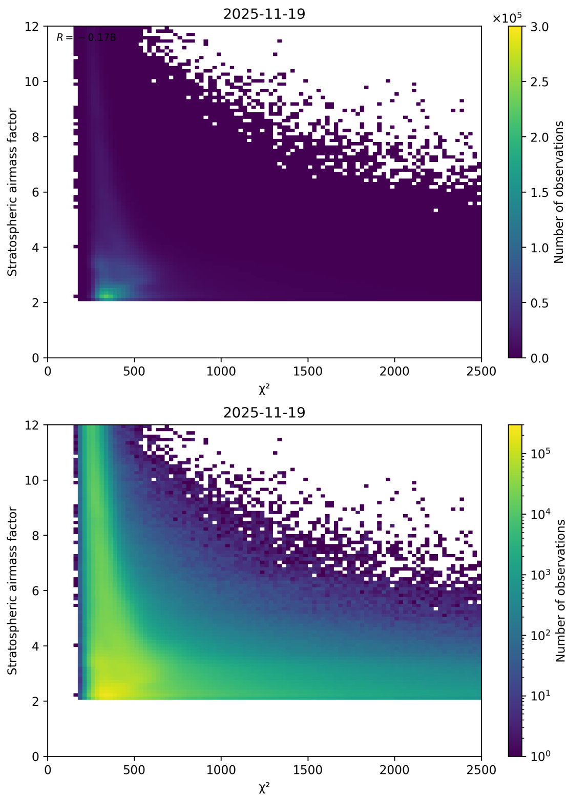
Figure 81: Scatter density plot of “ \chi^2 ” against “Stratospheric airmass factor” for 2025-11-18 to 2025-11-20.
