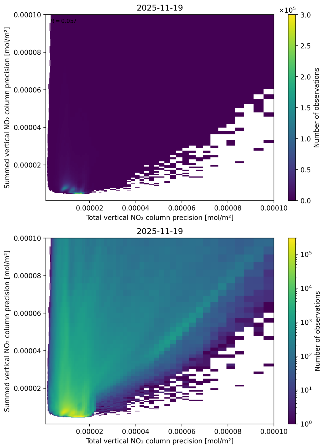
Figure 118: Scatter density plot of “Total vertical NO 2 column precision” against “Summed vertical NO 2 column precision” for 2025-11-18 to 2025-11-20.
