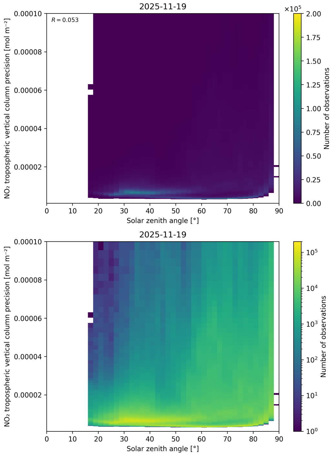
Figure 156: Scatter density plot of “Solar zenith angle” against “NO 2 tropospheric vertical column precision” for 2025-11-18 to 2025-11-20.
