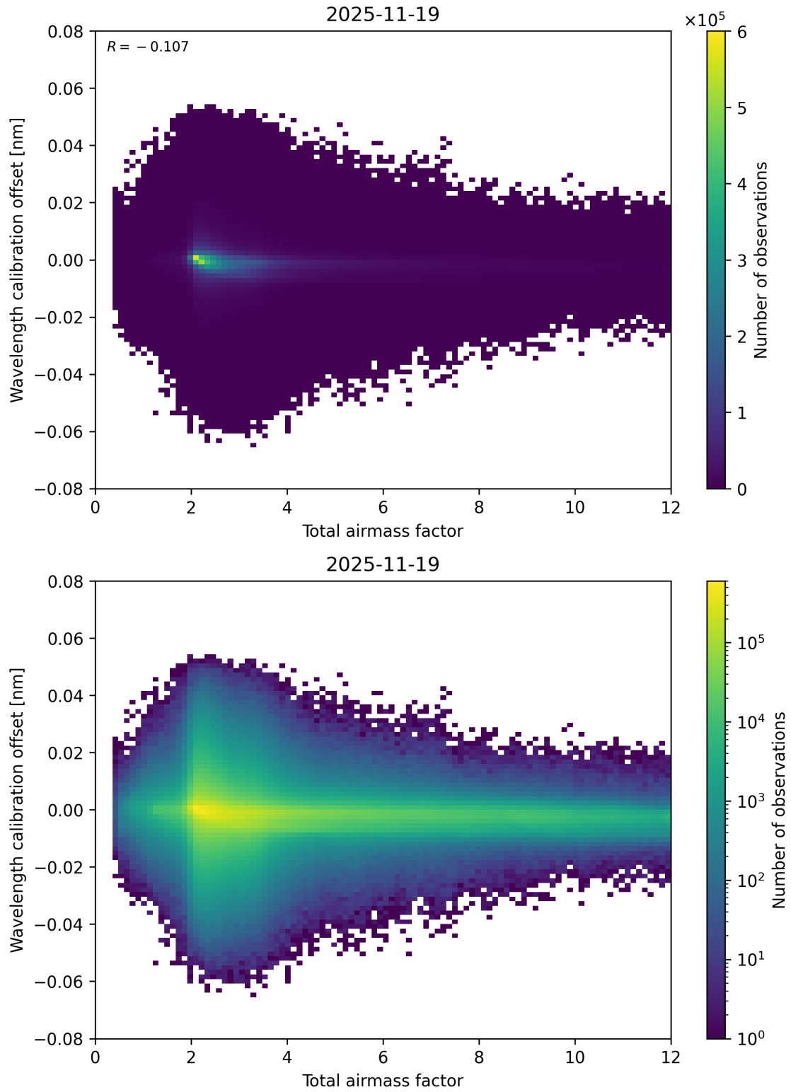
Figure 70: Scatter density plot of “Total airmass factor” against “Wavelength calibration offset” for 2025-11-18 to 2025-11-20.
