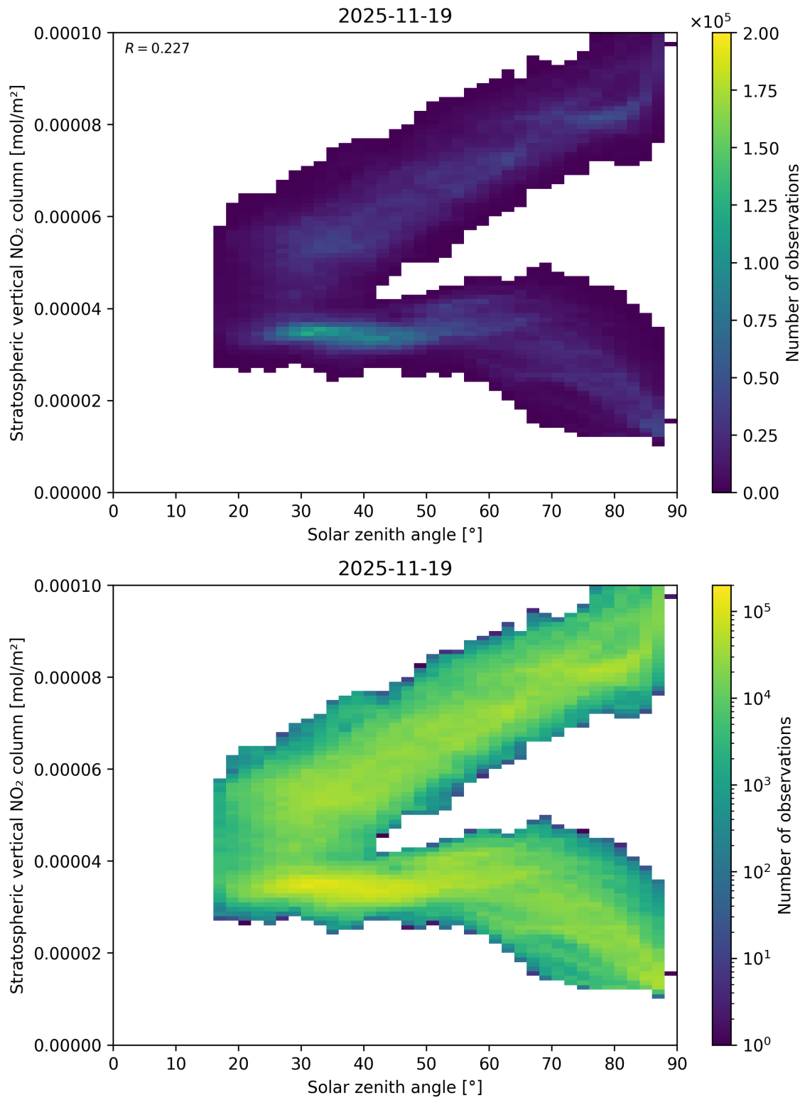
Figure 150: Scatter density plot of “Solar zenith angle” against “Stratospheric vertical NO 2 column” for 2025-11-18 to 2025-11-20.
