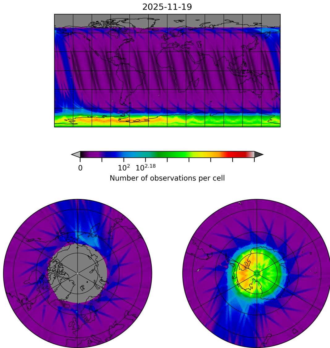
Figure 10: Map of the number of observations for 2025-11-18 to 2025-11-20
