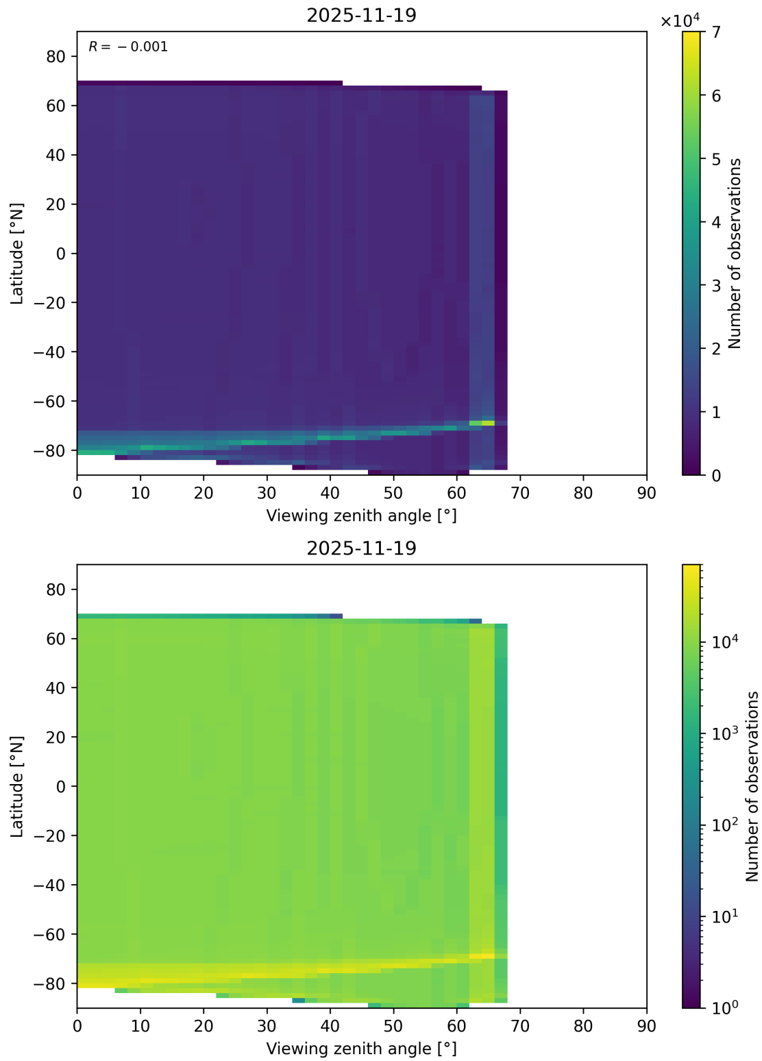
Figure 163: Scatter density plot of “Viewing zenith angle” against “Latitude” for 2025-11-18 to 2025-11-20.
