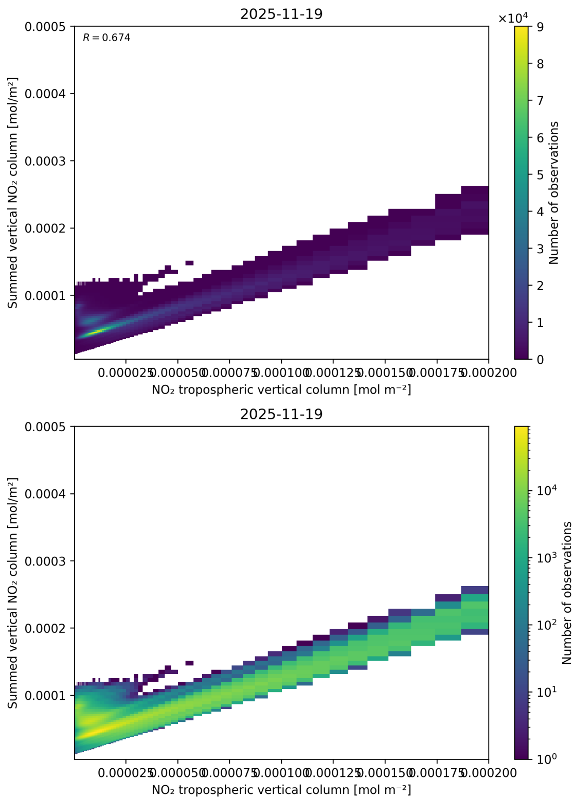
Figure 126: Scatter density plot of “NO 2 tropospheric vertical column” against “Summed vertical NO 2 column” for 2025-11-18 to 2025-11-20.
