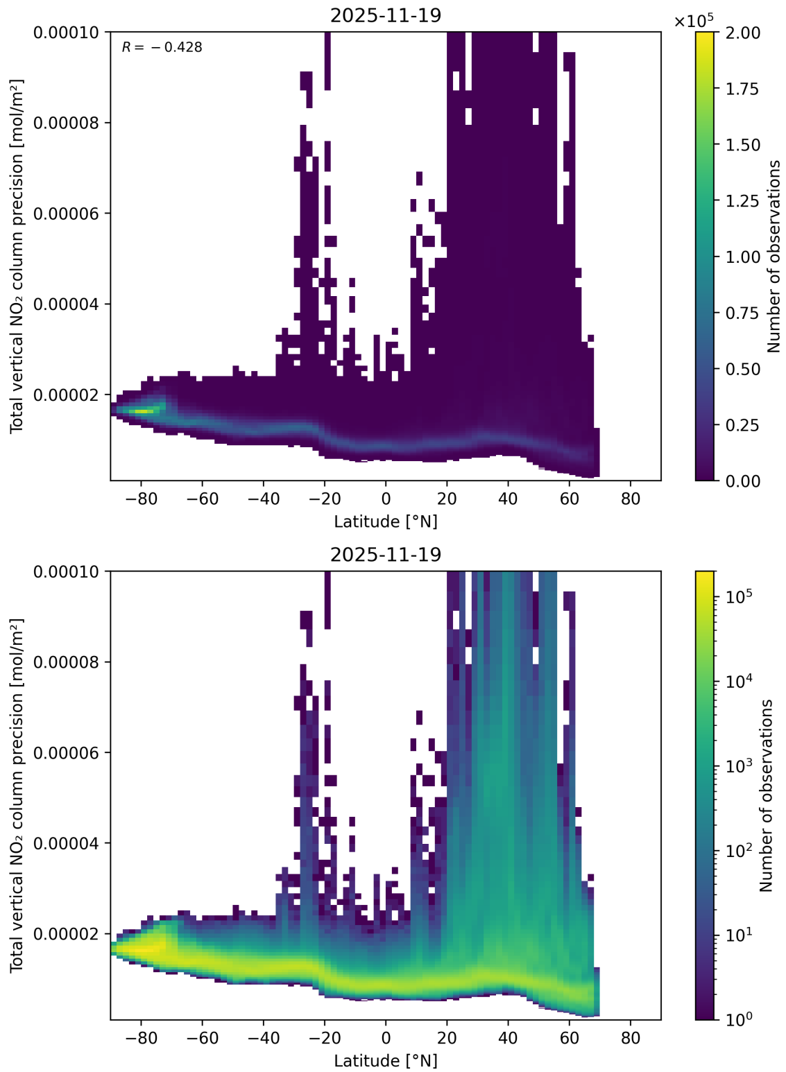
Figure 91: Scatter density plot of “Latitude” against “Total vertical NO 2 column precision” for 2025-11-18 to 2025-11-20.
