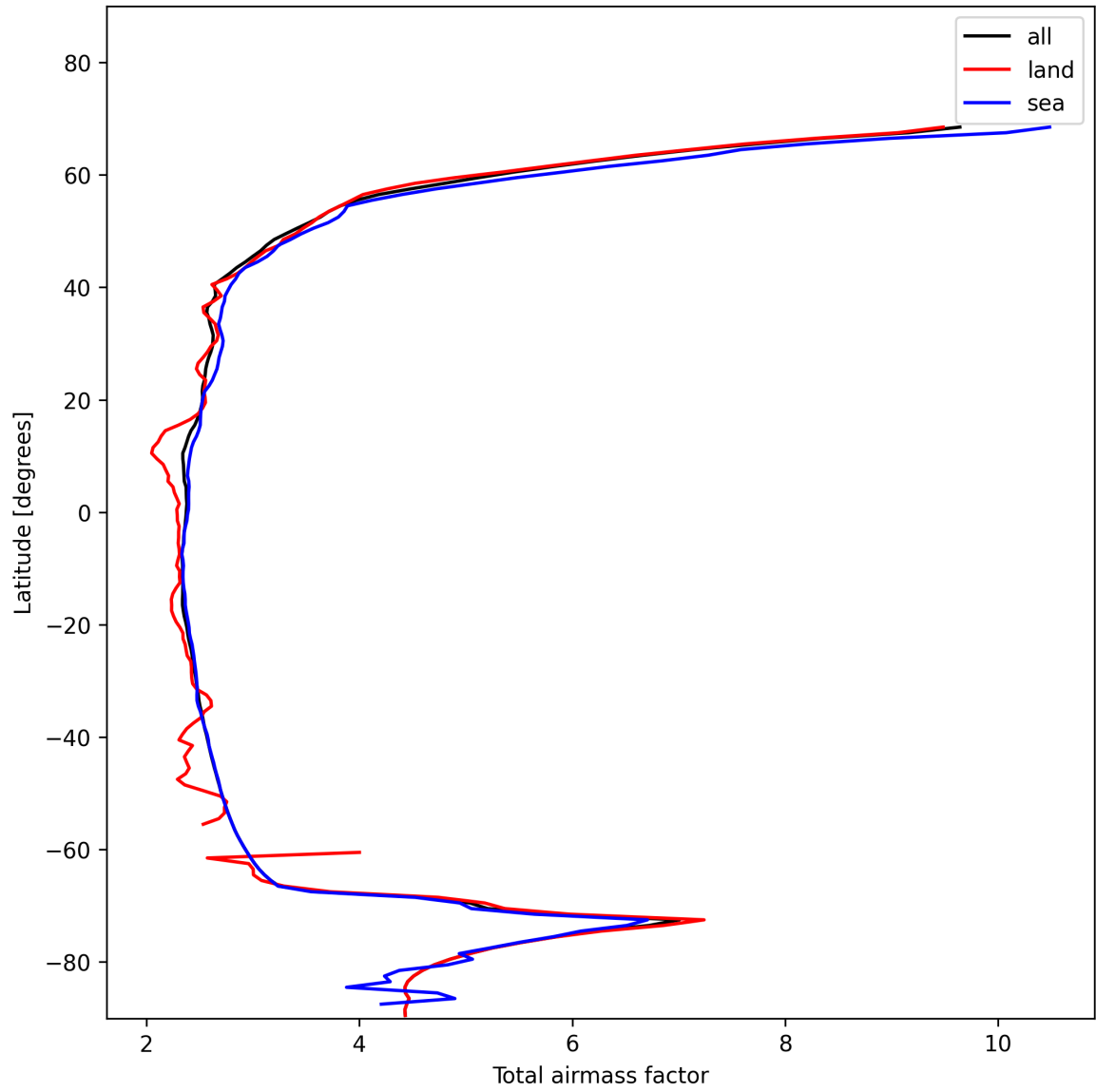
Figure 15: Zonal average of “Total airmass factor” for 2025-11-18 to 2025-11-20.
