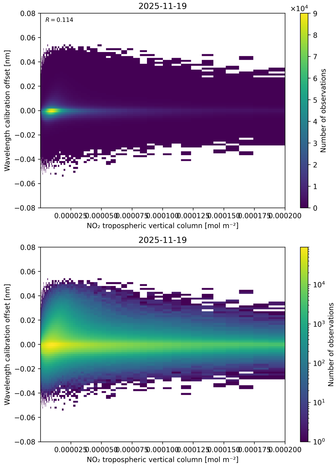
Figure 143: Scatter density plot of “NO 2 tropospheric vertical column” against “Wavelength calibration offset” for 2025-11-18 to 2025-11-20.
