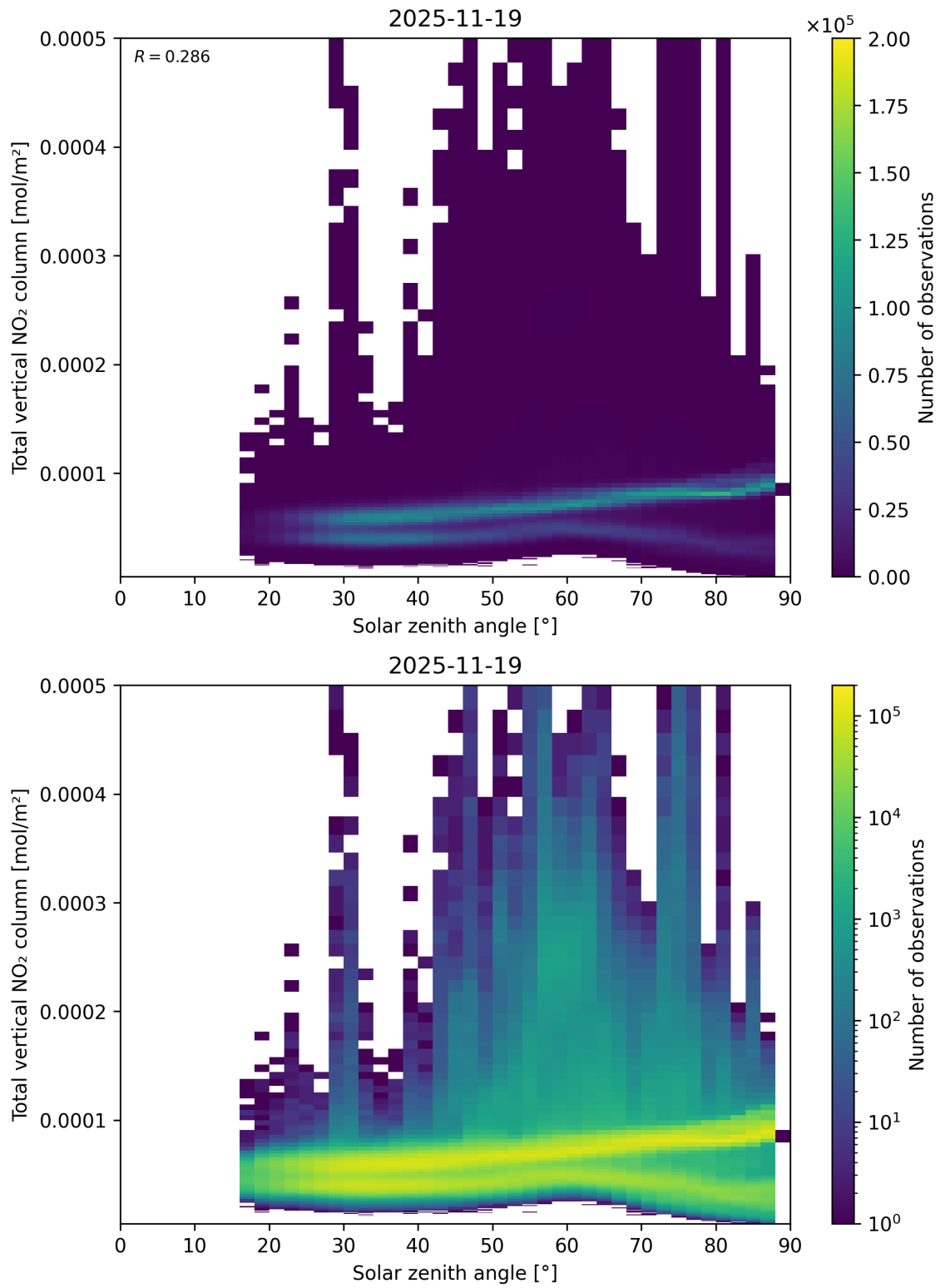
Figure 153: Scatter density plot of “Solar zenith angle” against “Total vertical NO 2 column” for 2025-11-18 to 2025-11-20.
