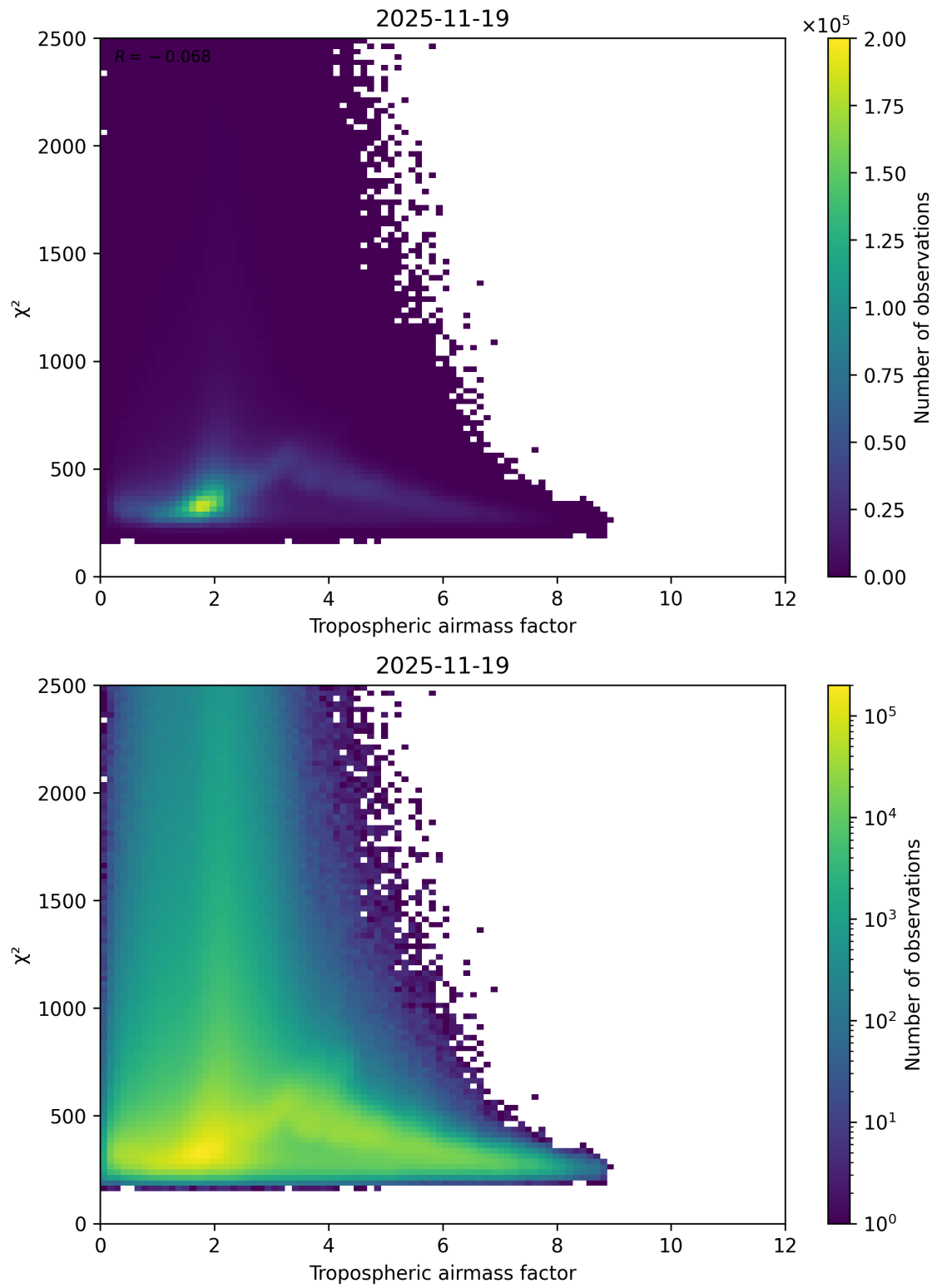
Figure 73: Scatter density plot of “Tropospheric airmass factor” against “ \chi^2 ” for 2025-11-18 to 2025-11-20.
