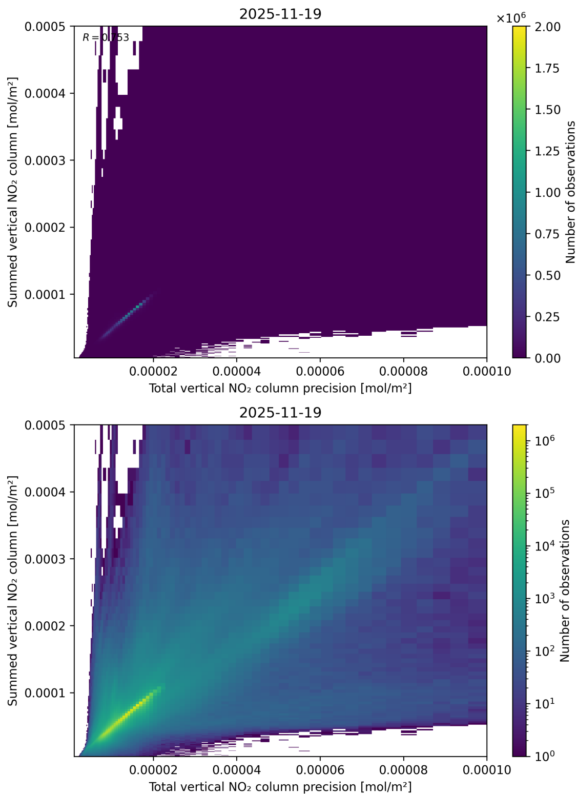
Figure 117: Scatter density plot of “Total vertical NO 2 column precision” against “Summed vertical NO 2 column” for 2025-11-18 to 2025-11-20.
