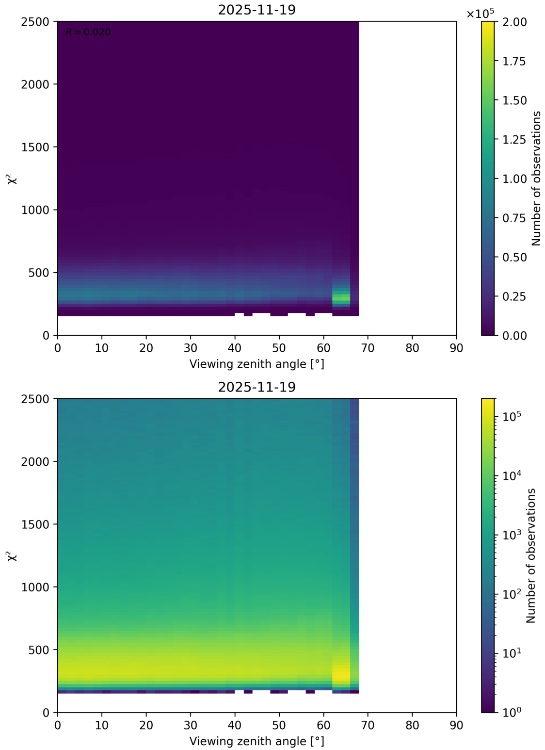
Figure 162: Scatter density plot of “Viewing zenith angle” against “ \chi^2 ” for 2025-11-18 to 2025-11-20.
