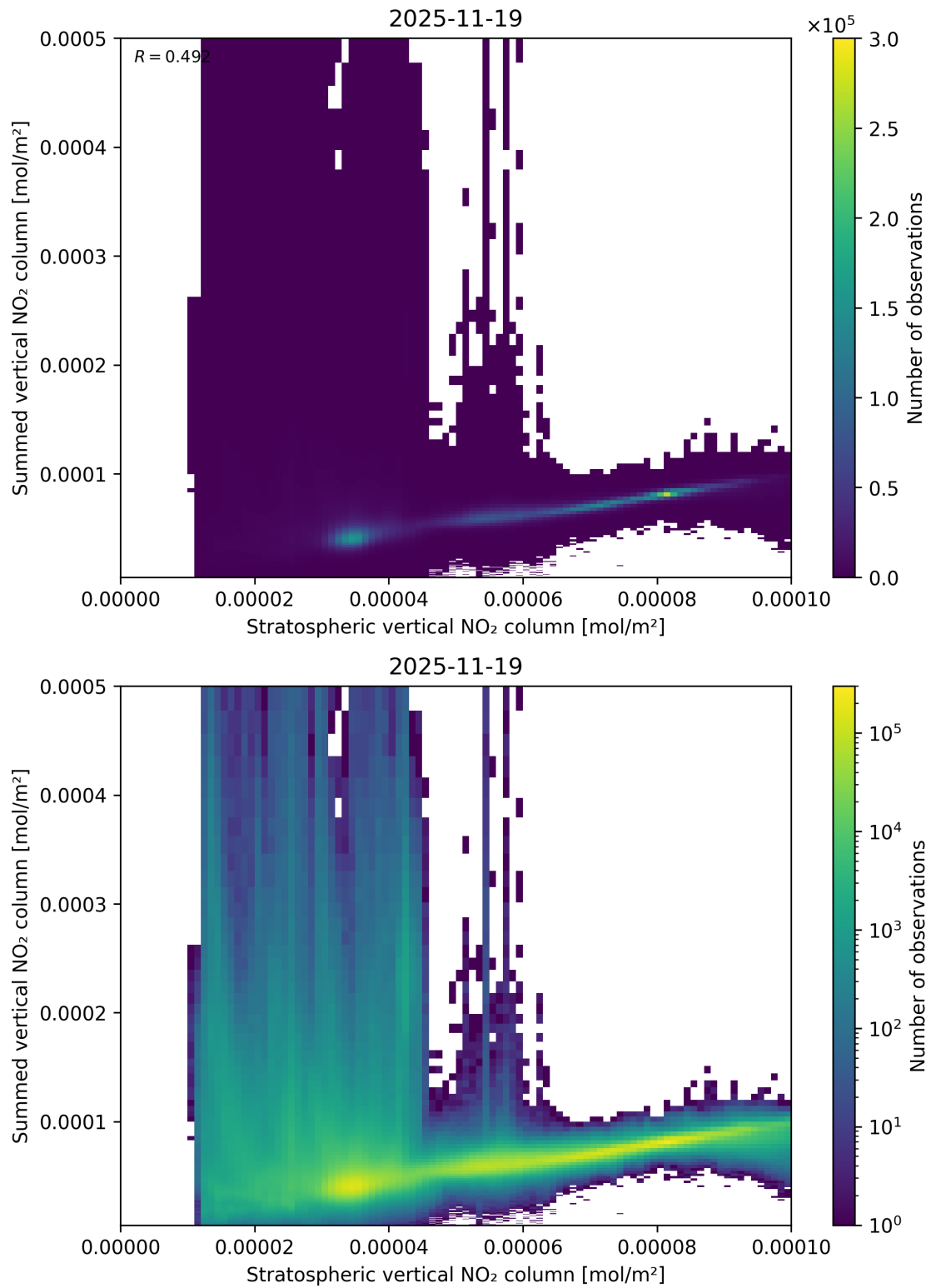
Figure 98: Scatter density plot of “Stratospheric vertical NO 2 column” against “Summed vertical NO 2 column” for 2025-11-18 to 2025-11-20.
