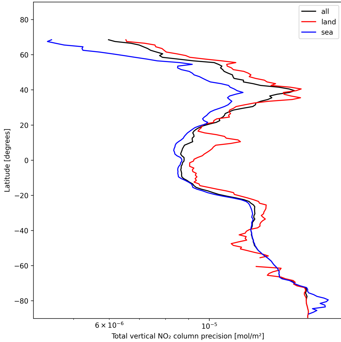
Figure 22: Zonal average of “Total vertical NO 2 column precision” for 2025-11-18 to 2025-11-20.
