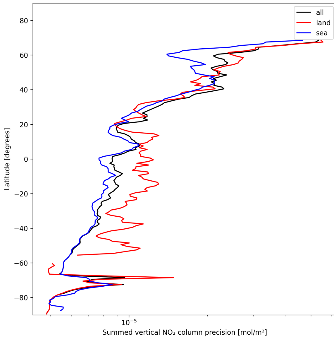
Figure 24: Zonal average of “Summed vertical NO 2 column precision” for 2025-11-18 to 2025-11-20.
