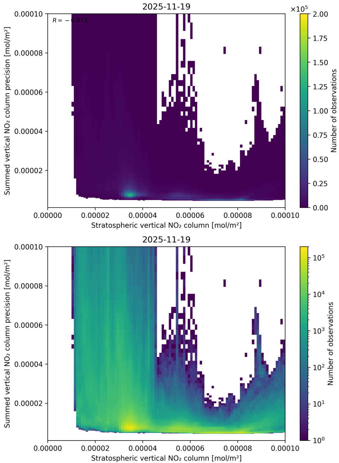
Figure 99: Scatter density plot of “Stratospheric vertical NO 2 column” against “Summed vertical NO 2 column precision” for 2025-11-18 to 2025-11-20.
