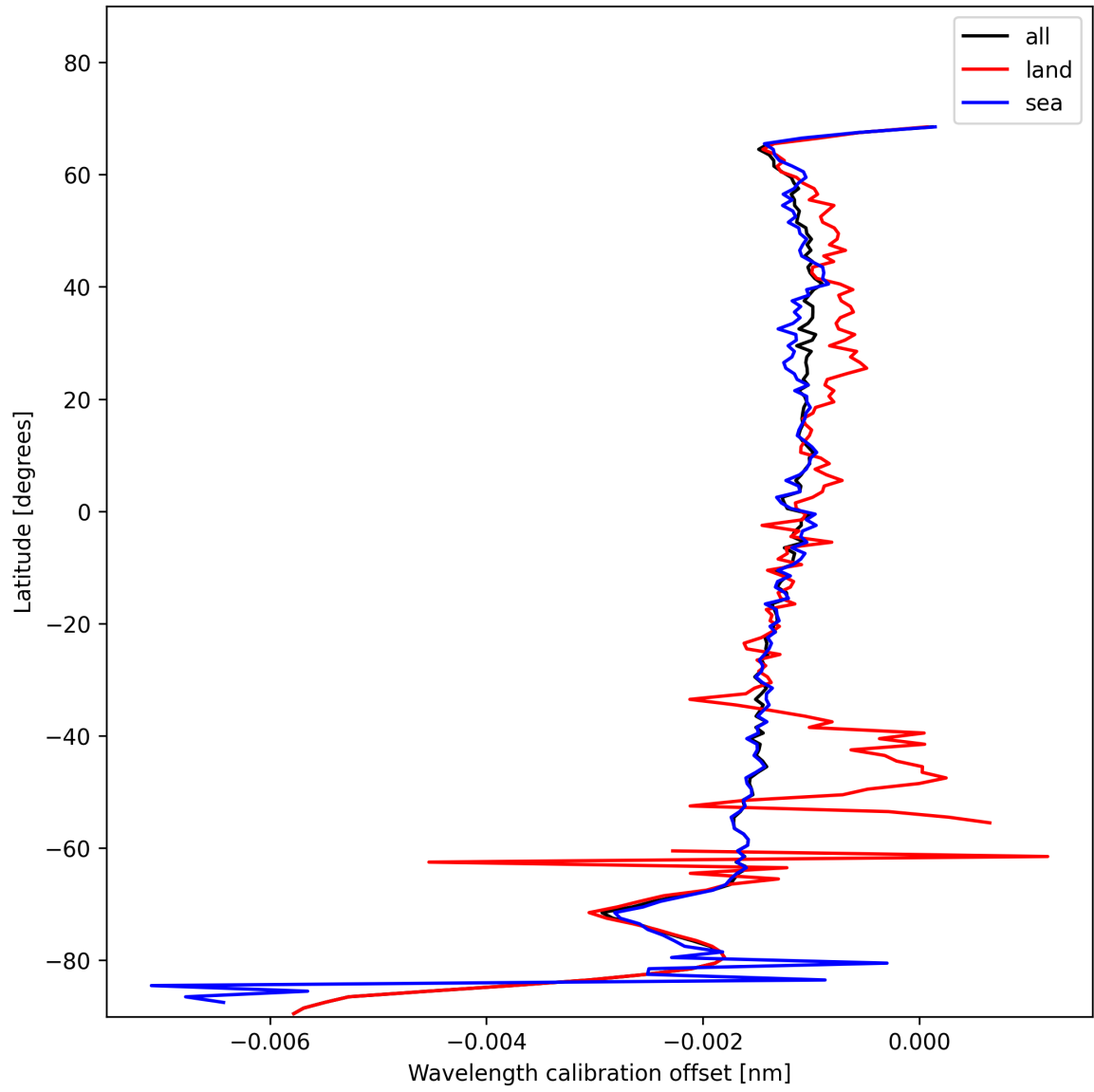
Figure 18: Zonal average of “Wavelength calibration offset” for 2025-11-18 to 2025-11-20.
