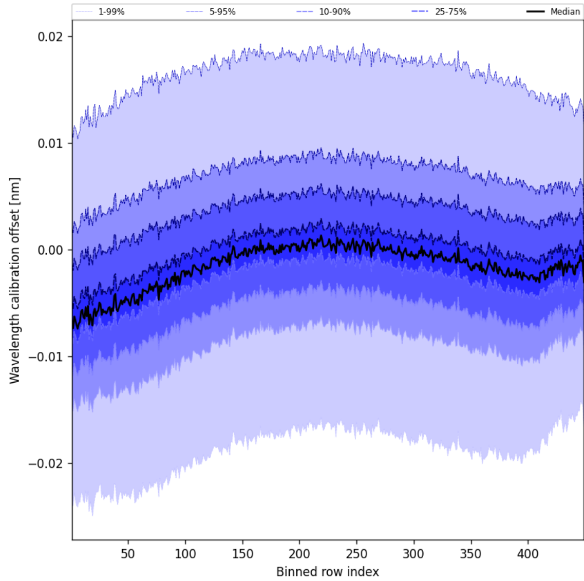
Figure 52: Along track statistics of “Wavelength calibration offset” for 2025-11-18 to 2025-11-20
