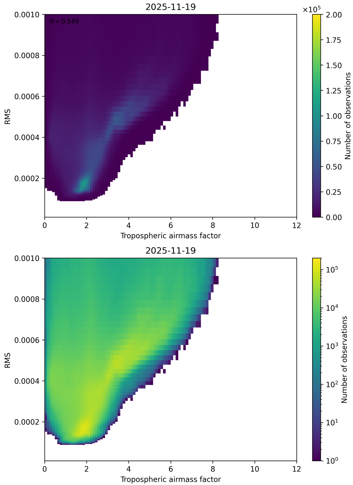
Figure 79: Scatter density plot of “Tropospheric airmass factor” against “RMS” for 2025-11-18 to 2025-11-20.
