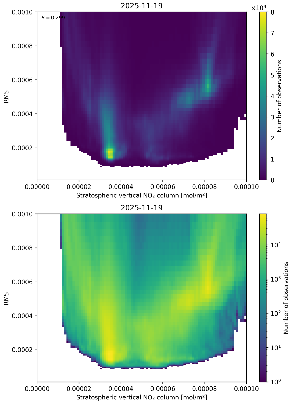
Figure 102: Scatter density plot of “Stratospheric vertical NO 2 column” against “RMS” for 2025-11-18 to 2025-11-20.
