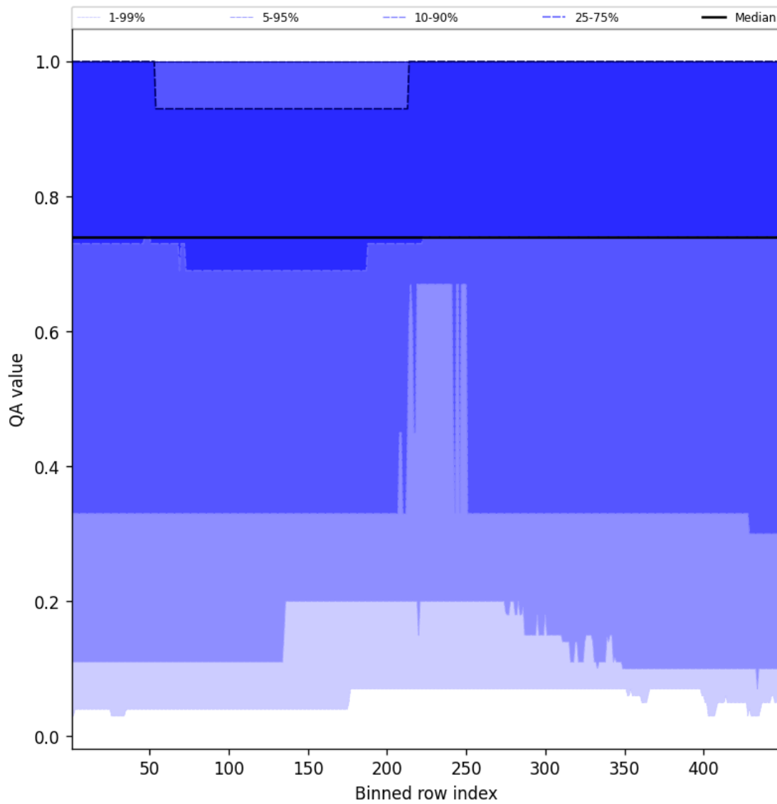
Figure 45: Along track statistics of “QA value” for 2025-11-18 to 2025-11-20
