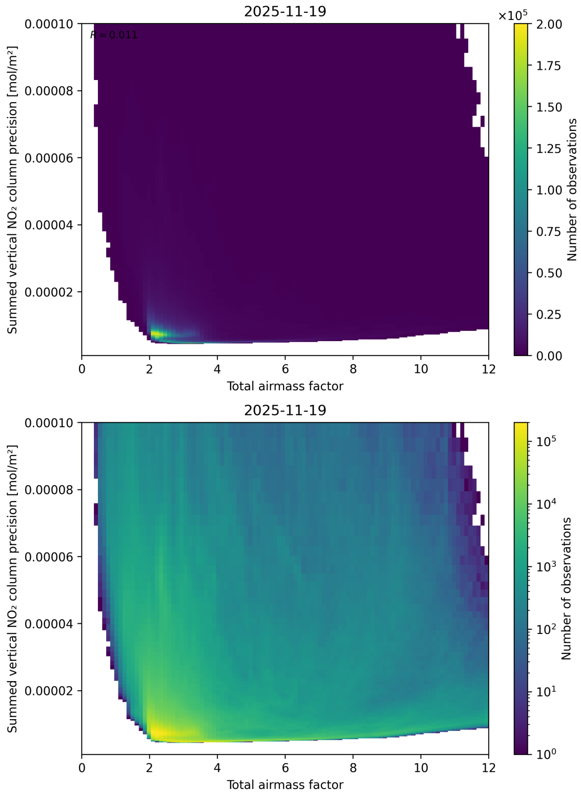
Figure 66: Scatter density plot of “Total airmass factor” against “Summed vertical NO 2 column precision” for 2025-11-18 to 2025-11-20.
