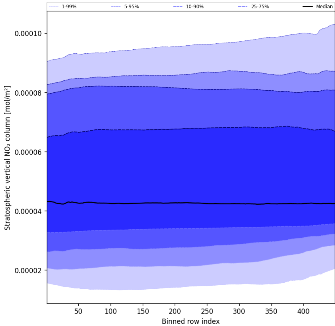
Figure 53: Along track statistics of “Stratospheric vertical NO 2 column” for 2025-11-18 to 2025-11-20
