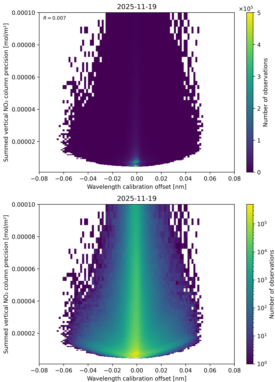
Figure 178: Scatter density plot of “Wavelength calibration offset” against “Summed vertical NO 2 column precision” for 2025-11-18 to 2025-11-20.
