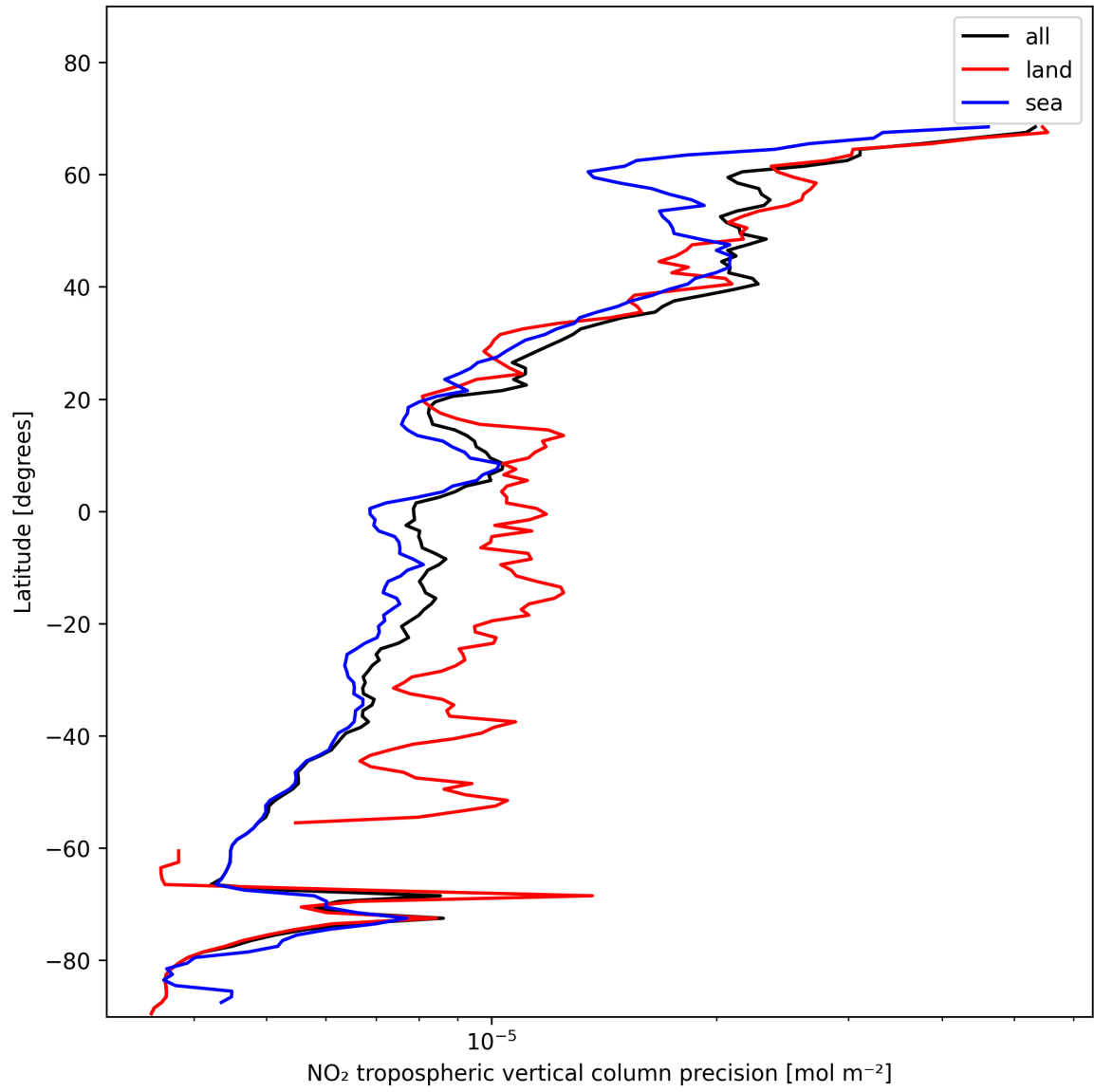
Figure 13: Zonal average of “NO 2 tropospheric vertical column precision” for 2025-11-18 to 2025-11-20.
