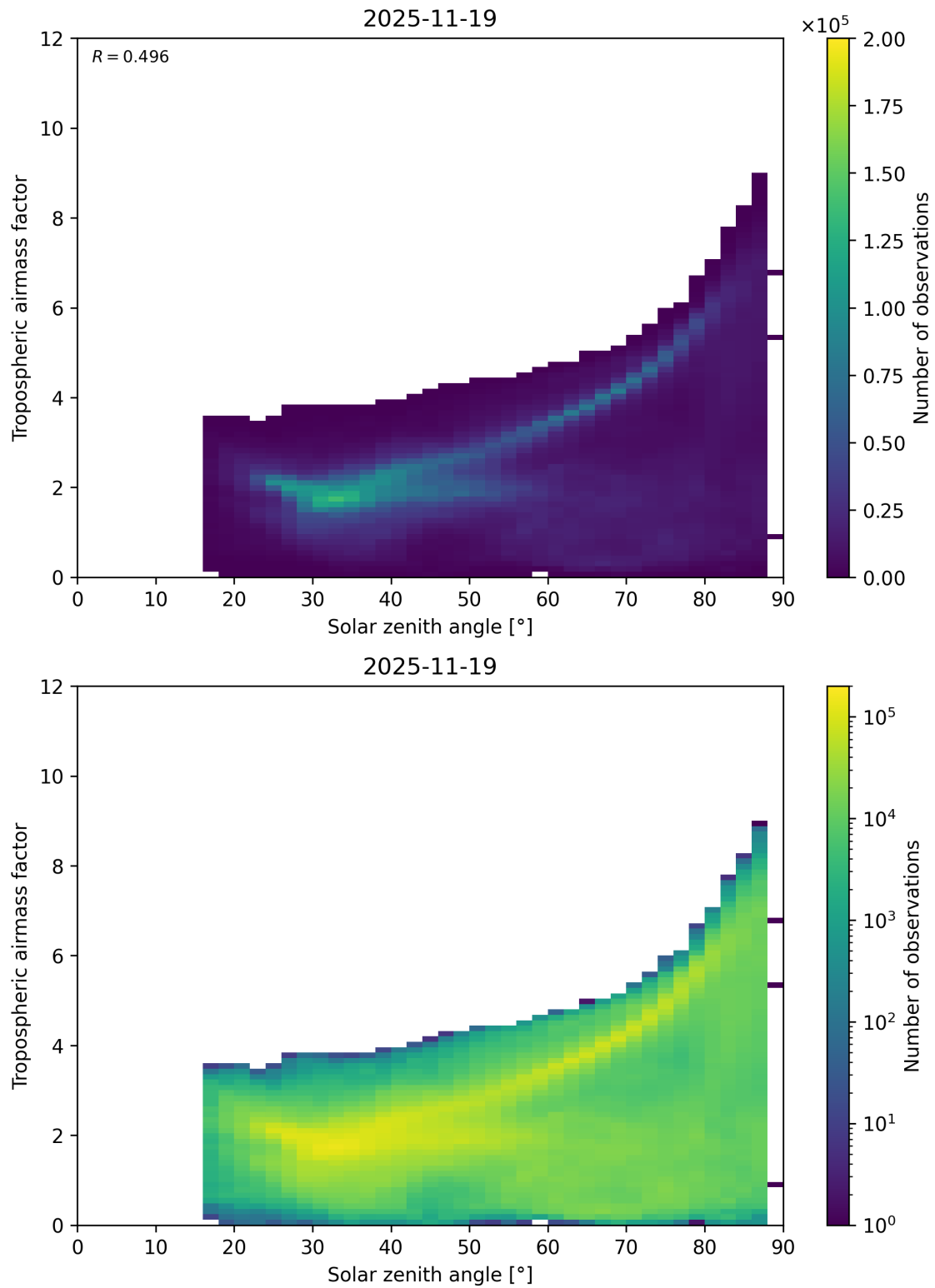
Figure 147: Scatter density plot of “Solar zenith angle” against “Tropospheric airmass factor” for 2025-11-18 to 2025-11-20.
