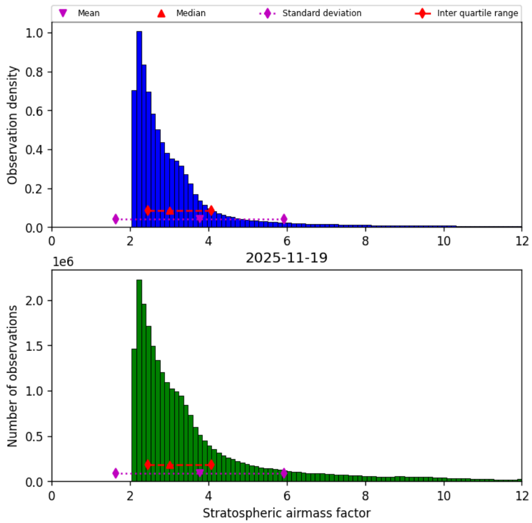
Figure 44: Histogram of “Stratospheric airmass factor” for 2025-11-18 to 2025-11-20
