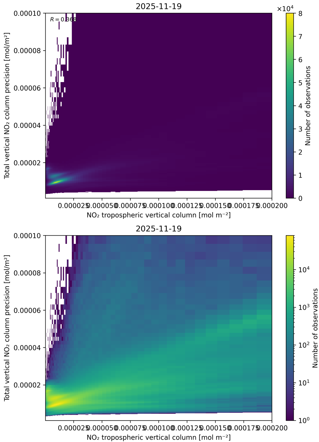
Figure 129: Scatter density plot of “NO 2 tropospheric vertical column” against “Total vertical NO 2 column precision” for 2025-11-18 to 2025-11-20.
