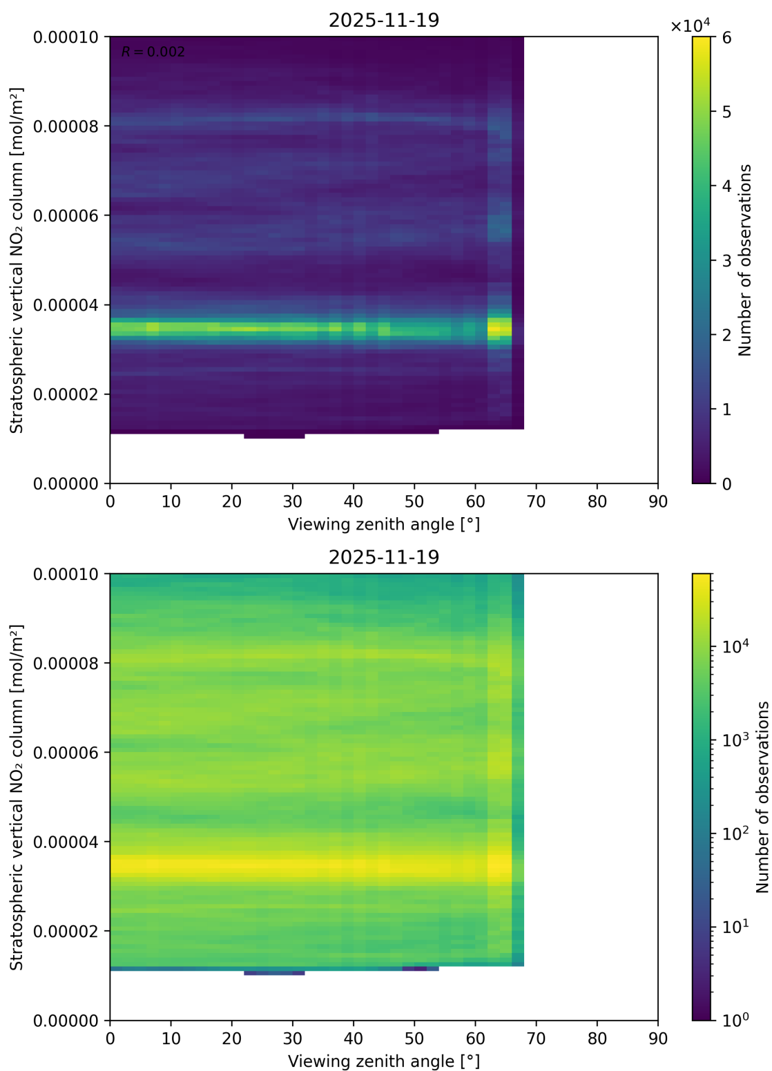
Figure 164: Scatter density plot of “Viewing zenith angle” against “Stratospheric vertical NO 2 column” for 2025-11-18 to 2025-11-20.
