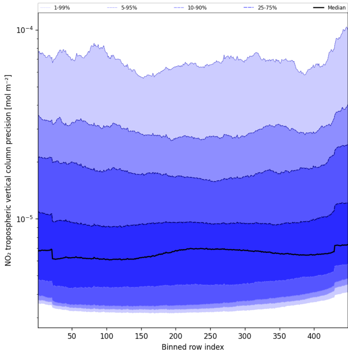
Figure 47: Along track statistics of “NO 2 tropospheric vertical column precision” for 2025-11-18 to 2025-11-20
