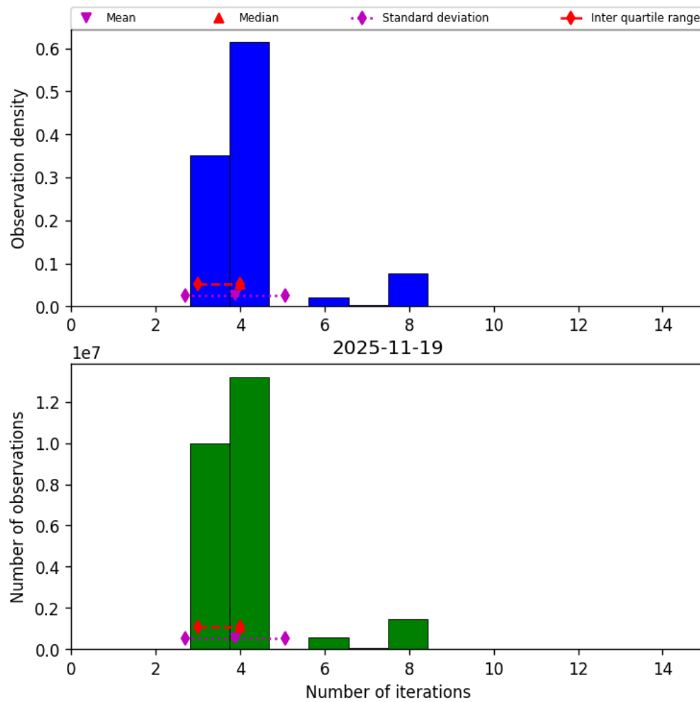
Figure 34: Histogram of “Number of iterations” for 2025-11-18 to 2025-11-20
