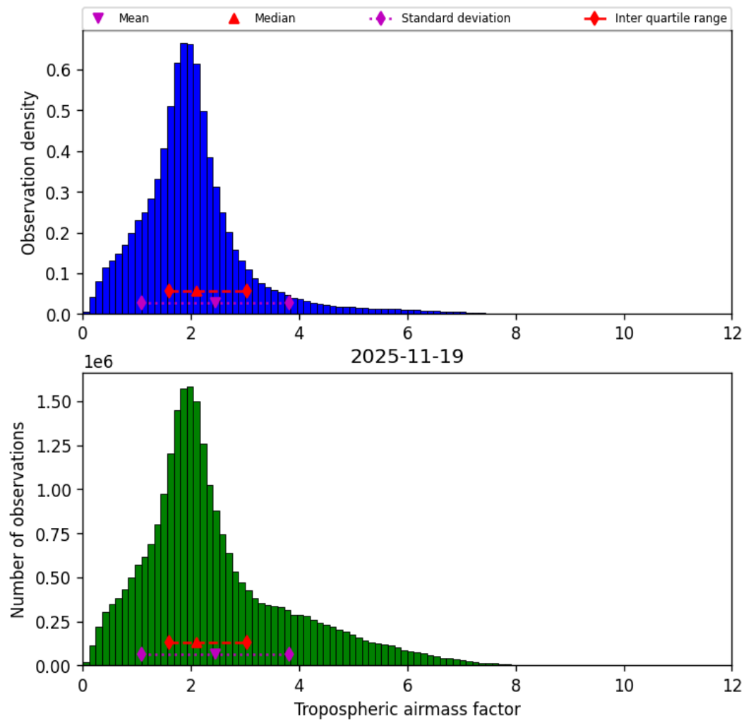
Figure 31: Histogram of “Tropospheric airmass factor” for 2025-11-18 to 2025-11-20
