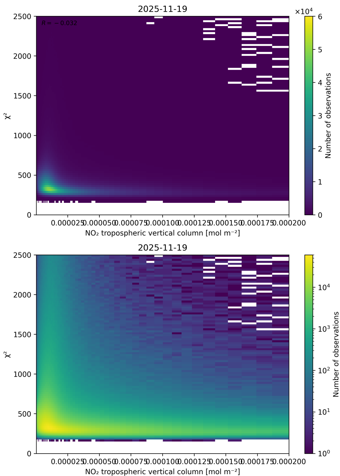
Figure 124: Scatter density plot of “NO 2 tropospheric vertical column” against “ \chi^2 ” for 2025-11-18 to 2025-11-20.
