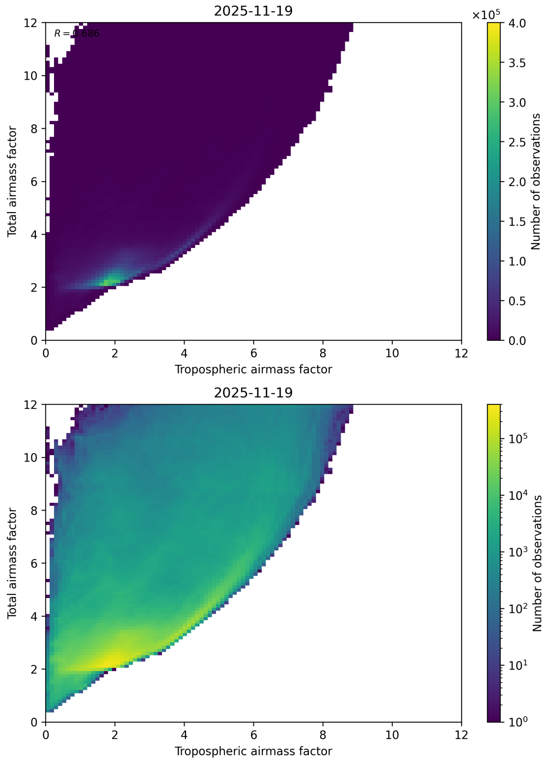
Figure 72: Scatter density plot of “Tropospheric airmass factor” against “Total airmass factor” for 2025-11-18 to 2025-11-20.
