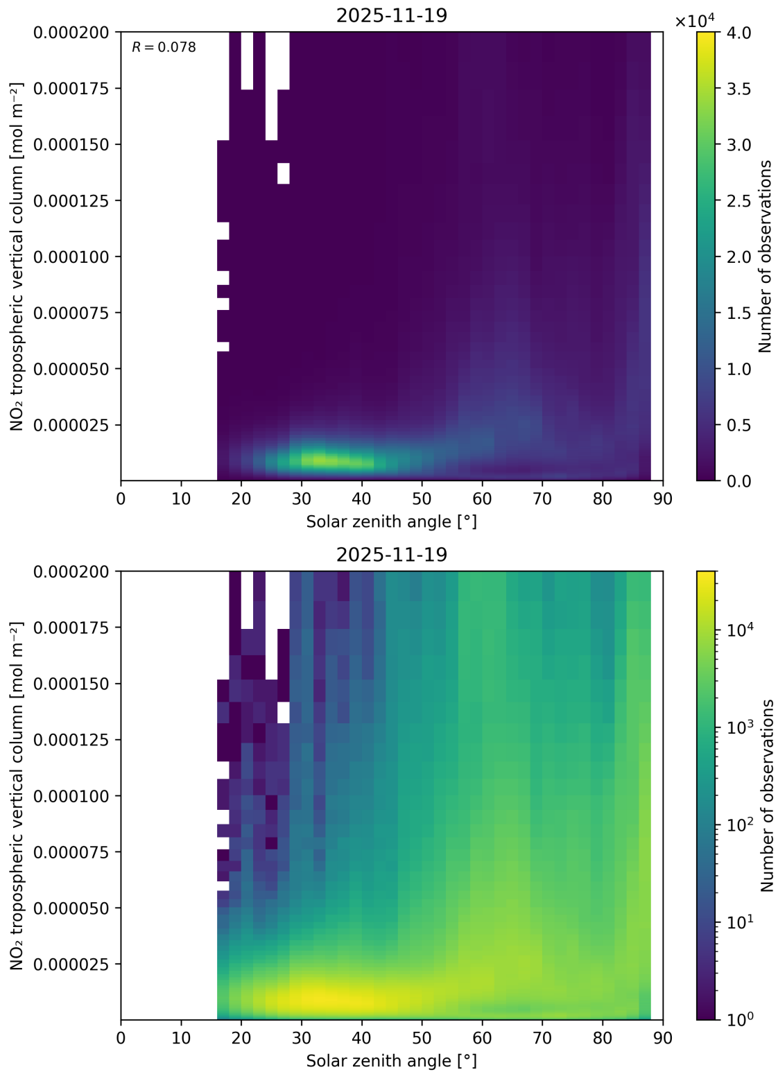
Figure 155: Scatter density plot of “Solar zenith angle” against “NO 2 tropospheric vertical column” for 2025-11-18 to 2025-11-20.
