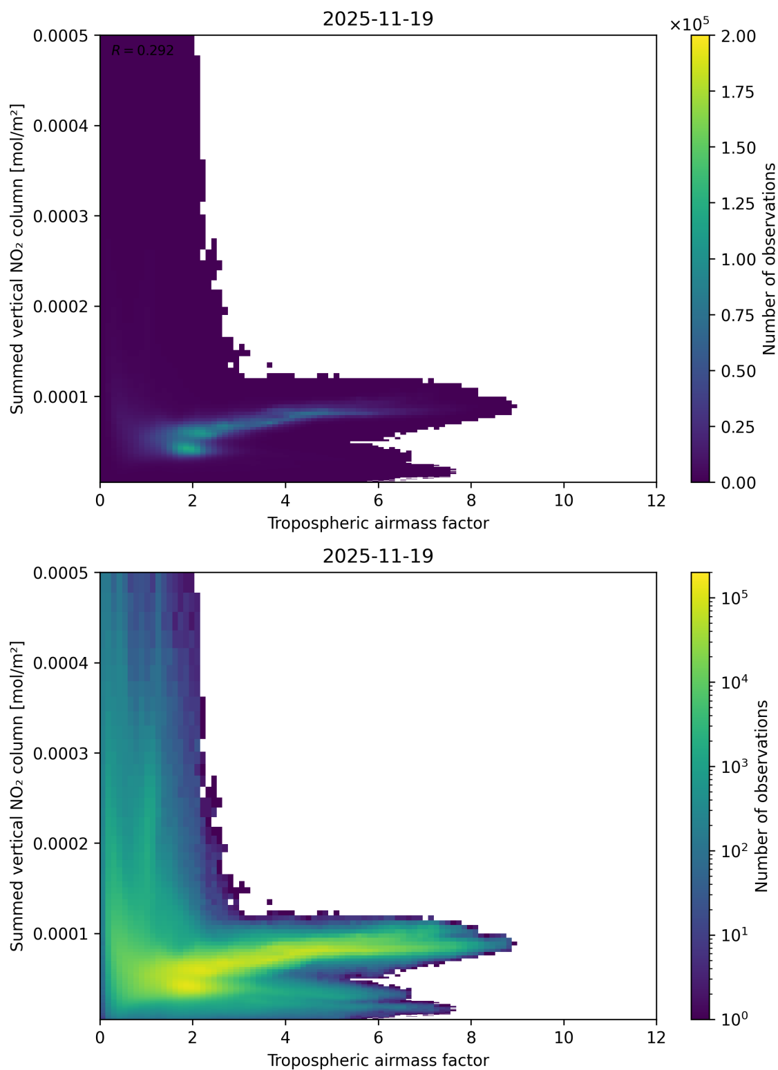
Figure 75: Scatter density plot of “Tropospheric airmass factor” against “Summed vertical NO 2 column” for 2025-11-18 to 2025-11-20.
