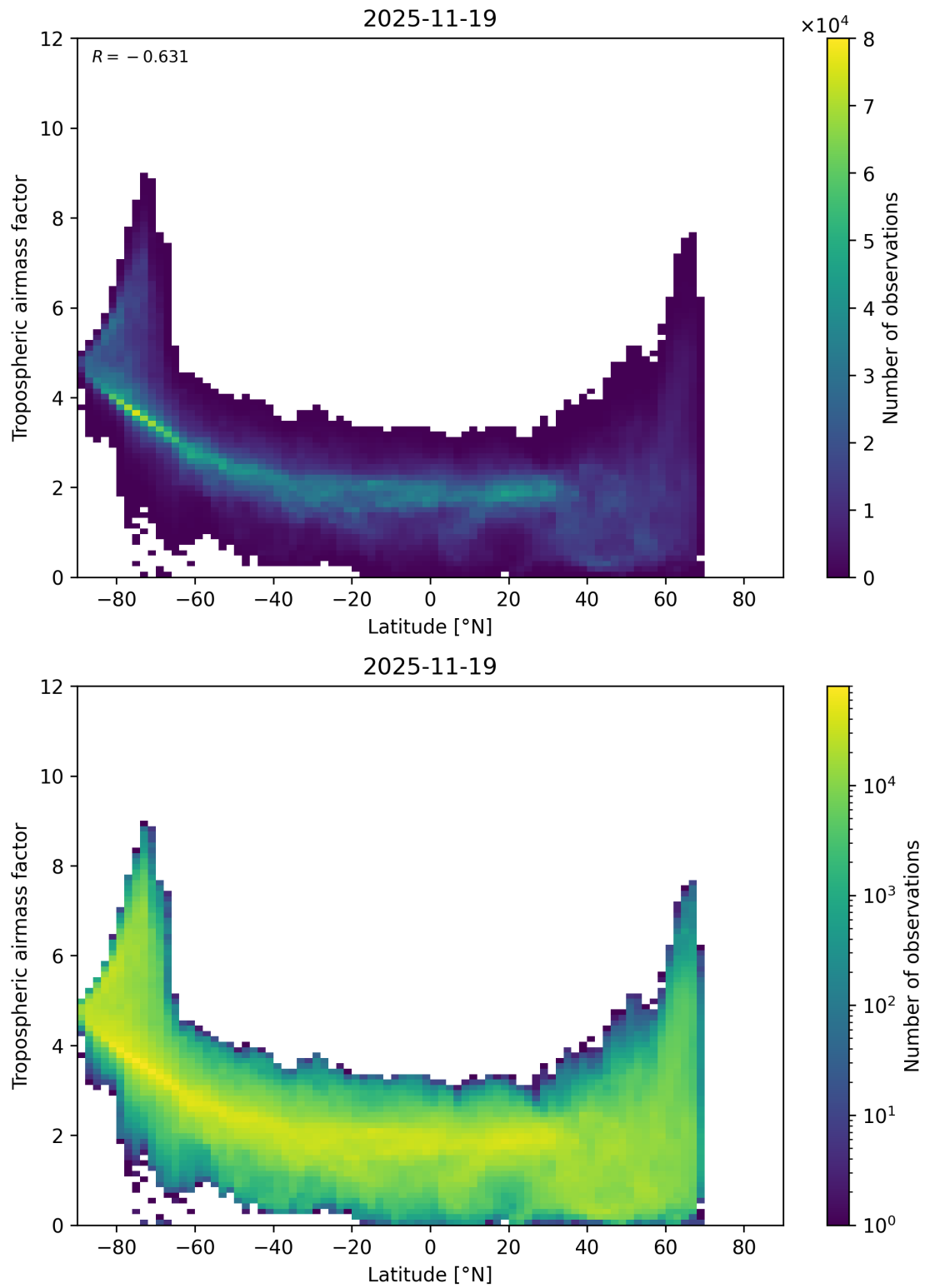
Figure 85: Scatter density plot of “Latitude” against “Tropospheric airmass factor” for 2025-11-18 to 2025-11-20.
