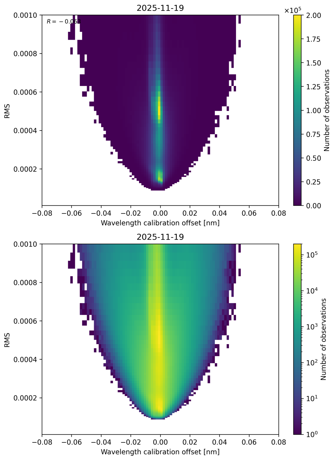
Figure 181: Scatter density plot of “Wavelength calibration offset” against “RMS” for 2025-11-18 to 2025-11-20.
