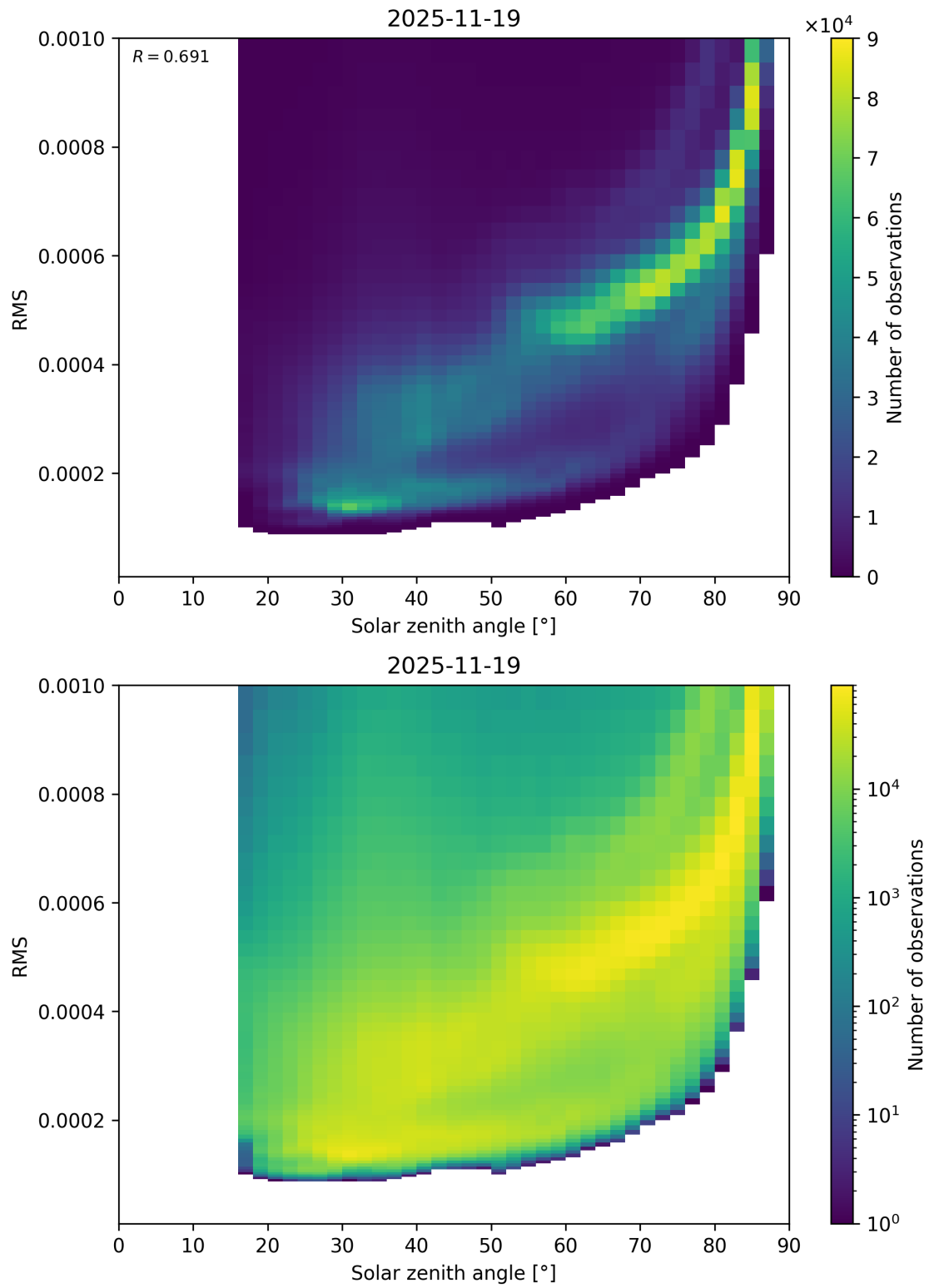
Figure 157: Scatter density plot of “Solar zenith angle” against “RMS” for 2025-11-18 to 2025-11-20.
