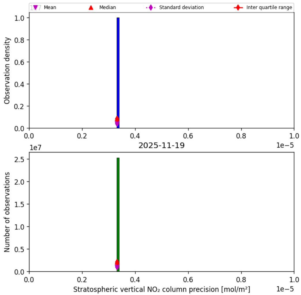
Figure 37: Histogram of “Stratospheric vertical NO 2 column precision” for 2025-11-18 to 2025-11-20
