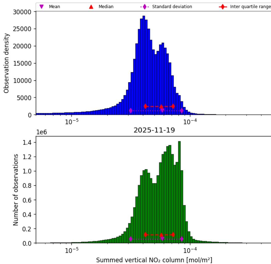
Figure 40: Histogram of “Summed vertical NO 2 column” for 2025-11-18 to 2025-11-20
