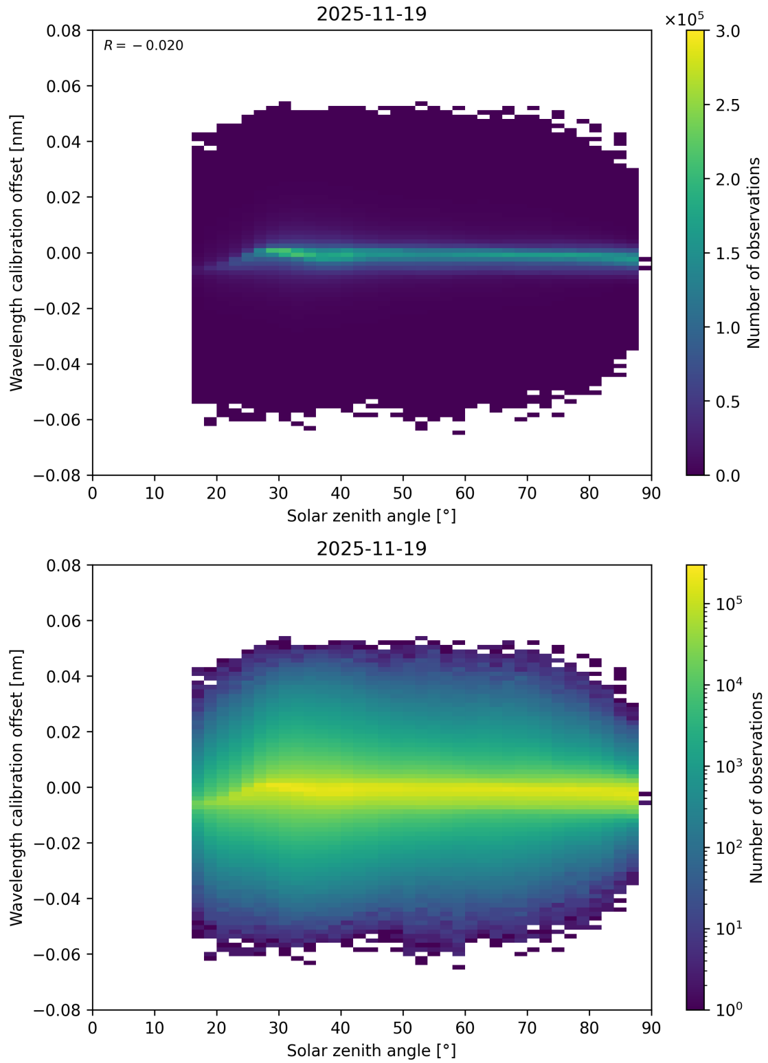
Figure 158: Scatter density plot of “Solar zenith angle” against “Wavelength calibration offset” for 2025-11-18 to 2025-11-20.
