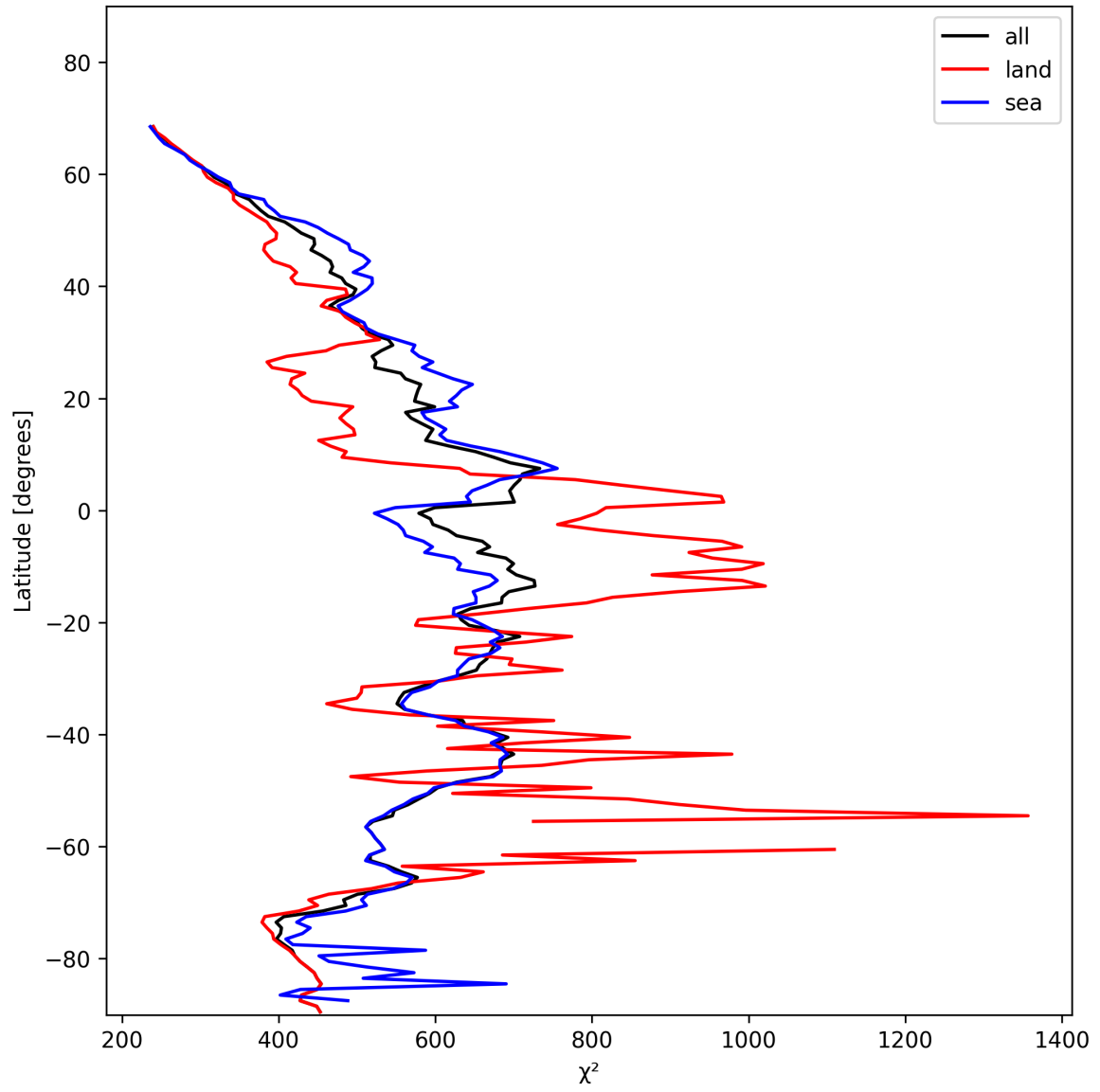
Figure 25: Zonal average of “ \chi^2 ” for 2025-11-18 to 2025-11-20.
