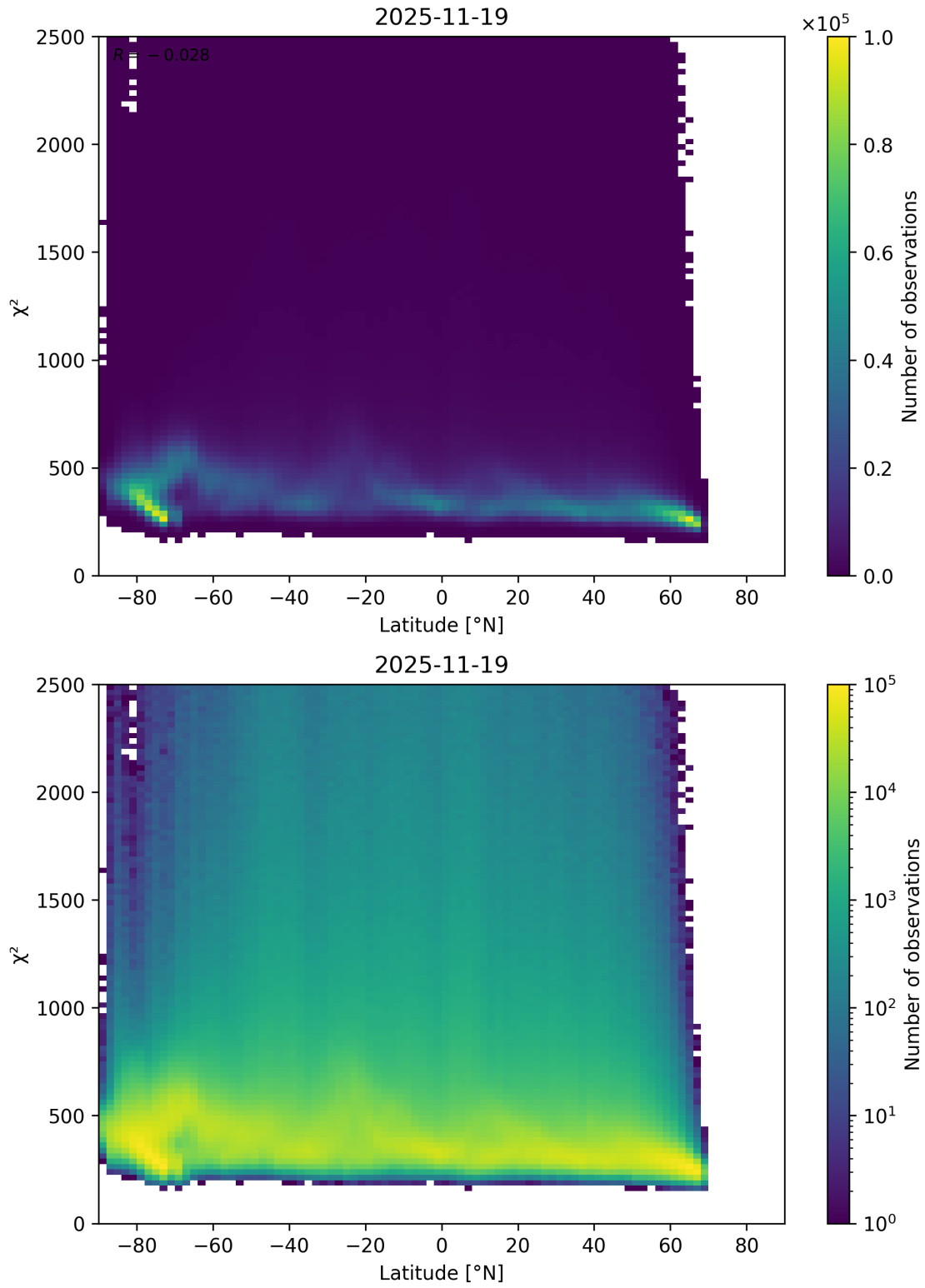
Figure 86: Scatter density plot of “Latitude” against “ \chi^2 ” for 2025-11-18 to 2025-11-20.
