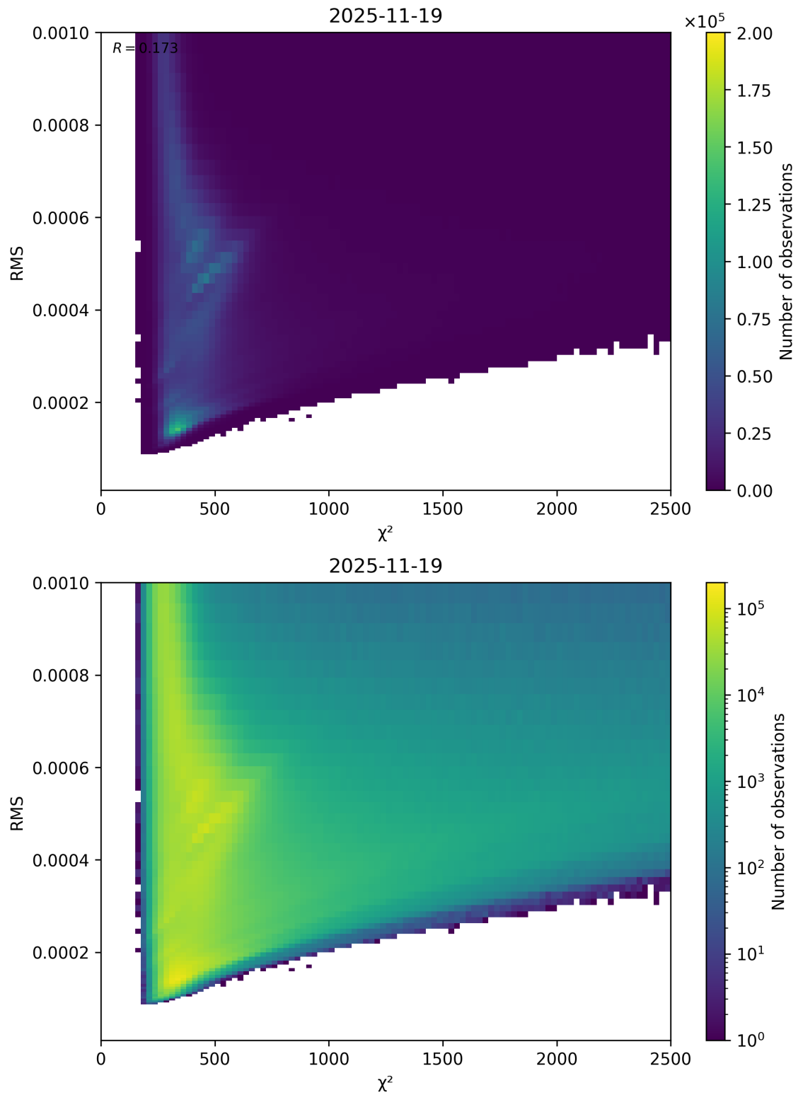
Figure 82: Scatter density plot of “ \chi^2 ” against “RMS” for 2025-11-18 to 2025-11-20.
