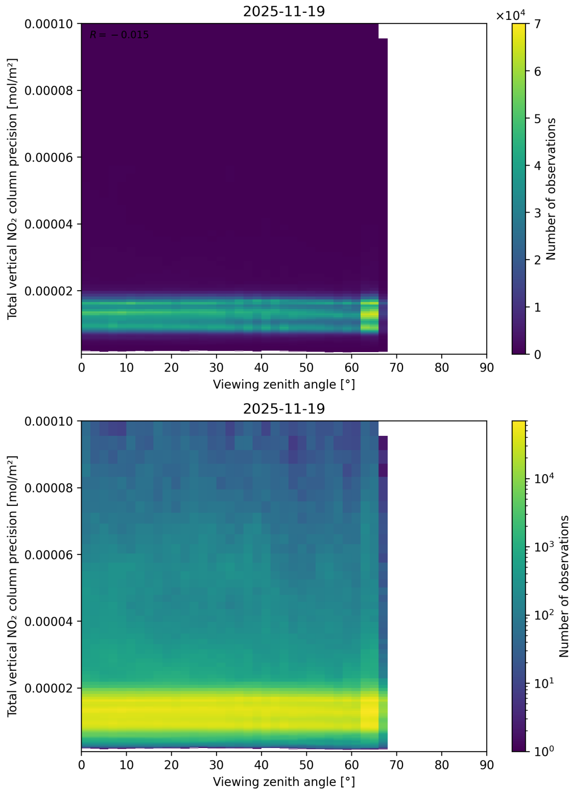
Figure 168: Scatter density plot of “Viewing zenith angle” against “Total vertical NO 2 column precision” for 2025-11-18 to 2025-11-20.
