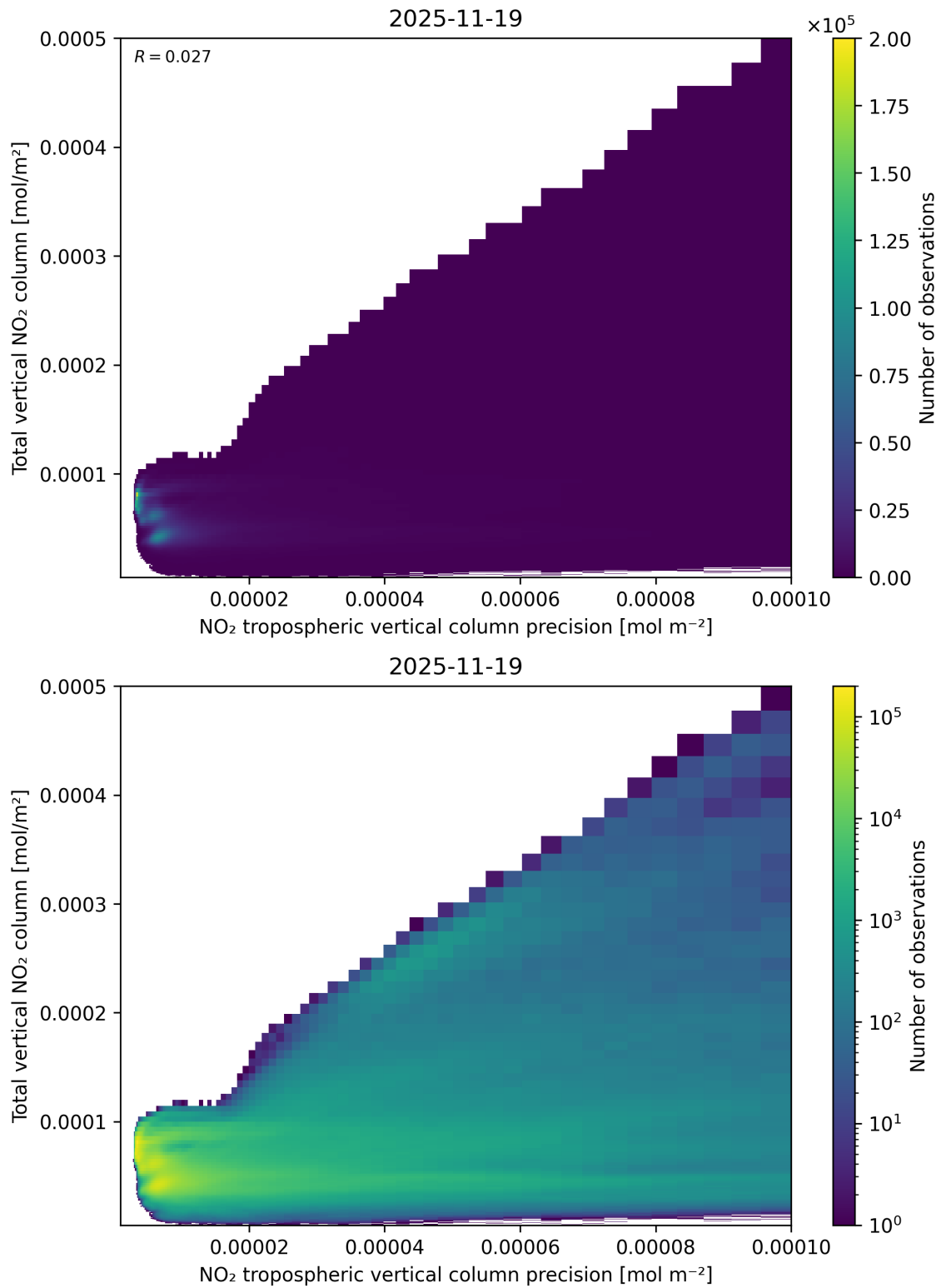
Figure 138: Scatter density plot of “NO 2 tropospheric vertical column precision” against “Total vertical NO 2 column” for 2025-11-18 to 2025-11-20.
