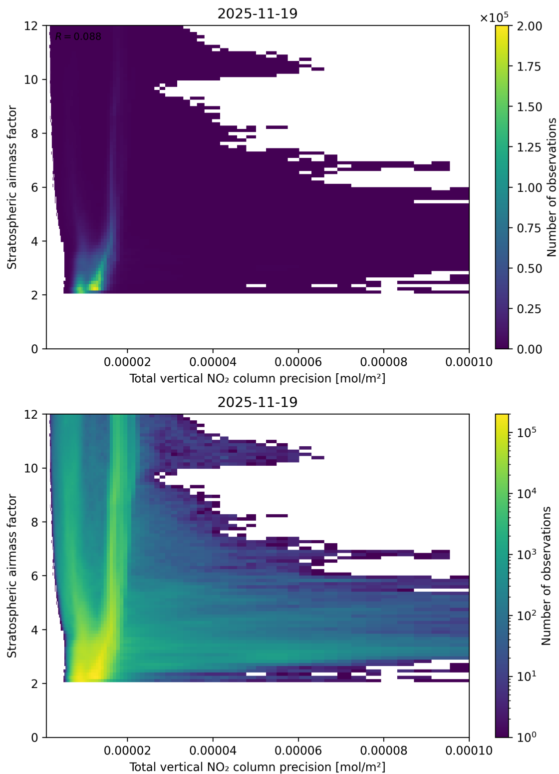
Figure 115: Scatter density plot of “Total vertical NO 2 column precision” against “Stratospheric air mass factor” for 2025-11-18 to 2025-11-20.
