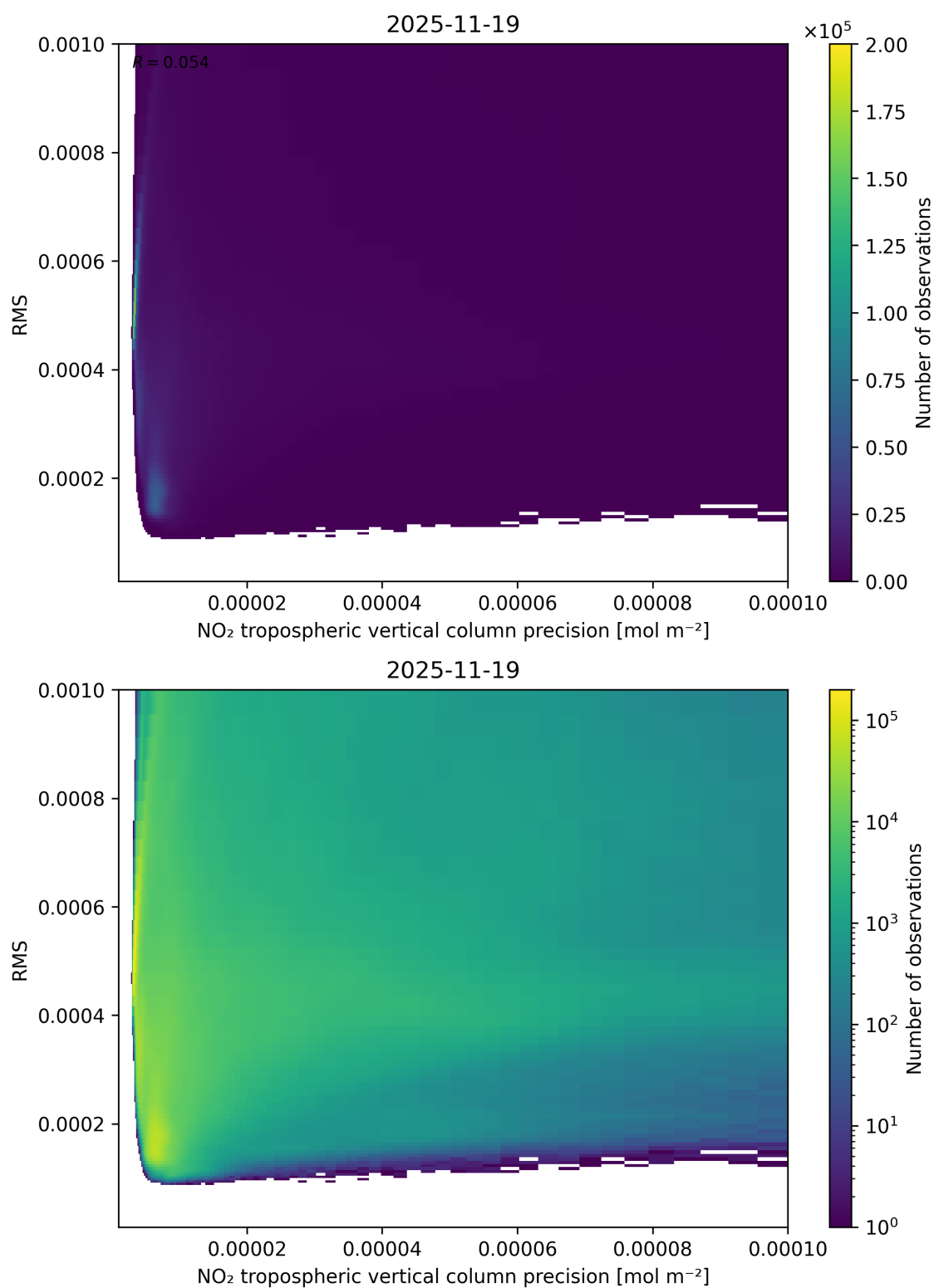
Figure 140: Scatter density plot of “NO 2 tropospheric vertical column precision” against “RMS” for 2025-11-18 to 2025-11-20.
