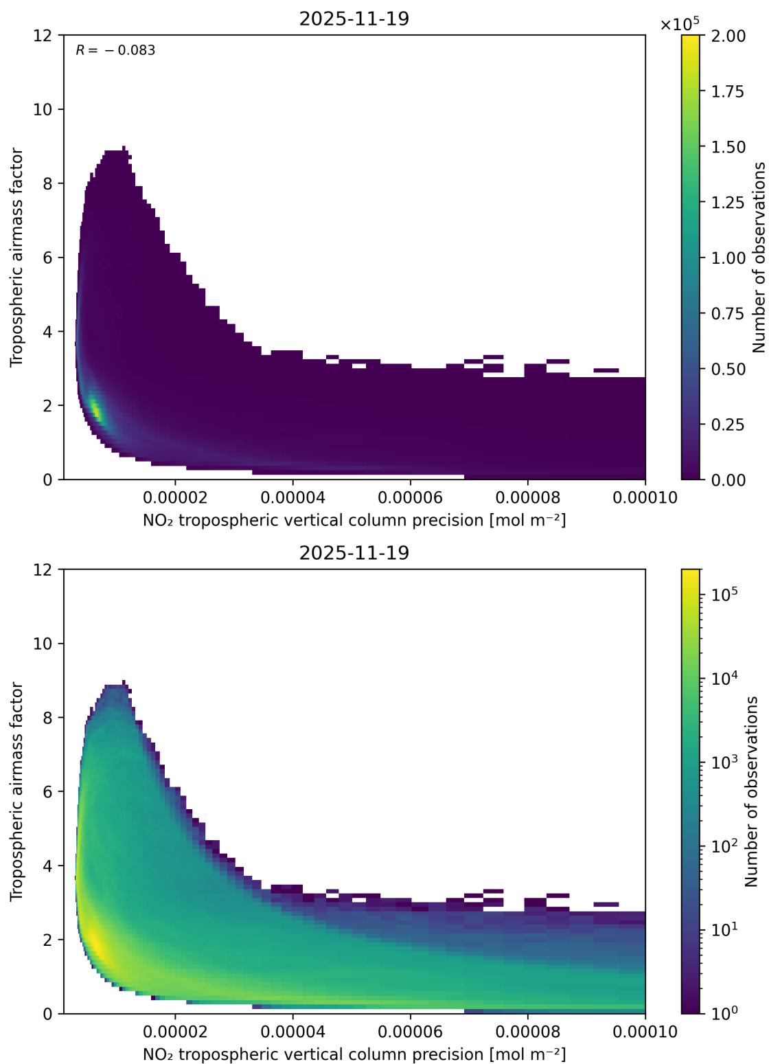
Figure 133: Scatter density plot of “NO 2 tropospheric vertical column precision” against “Tropospheric air mass factor” for 2025-11-18 to 2025-11-20.
