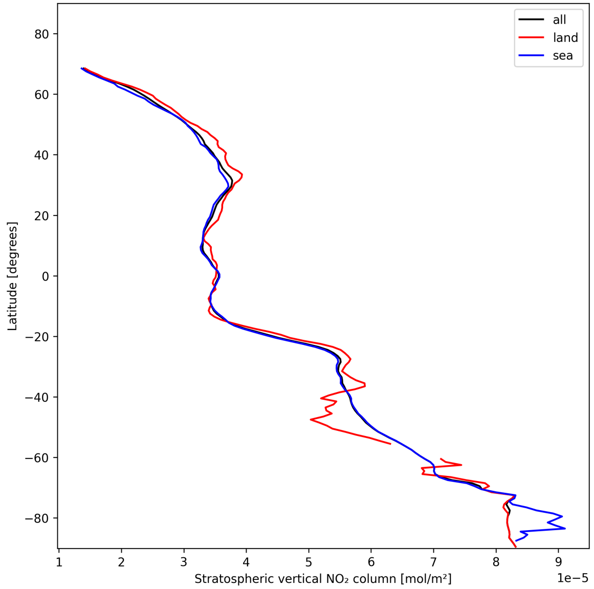
Figure 19: Zonal average of “Stratospheric vertical NO 2 column” for 2025-11-18 to 2025-11-20.
