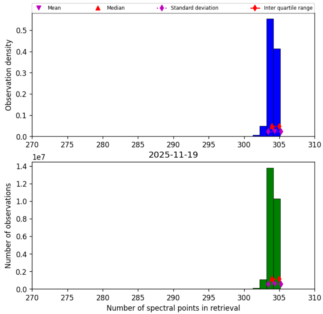
Figure 33: Histogram of “Number of spectral points in retrieval” for 2025-11-18 to 2025-11-20
