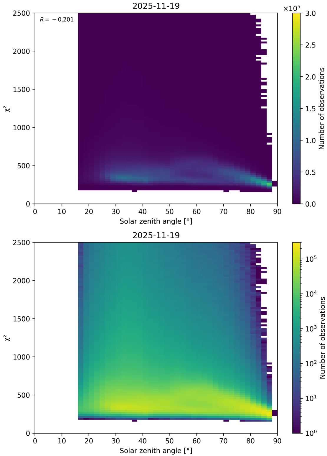
Figure 148: Scatter density plot of “Solar zenith angle” against “ \chi^2 ” for 2025-11-18 to 2025-11-20.
