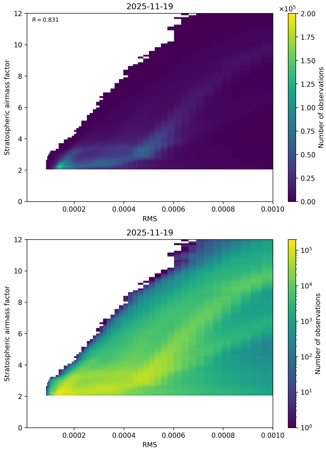
Figure 144: Scatter density plot of “RMS” against “Stratospheric airmass factor” for 2025-11-18 to 2025-11-20.
