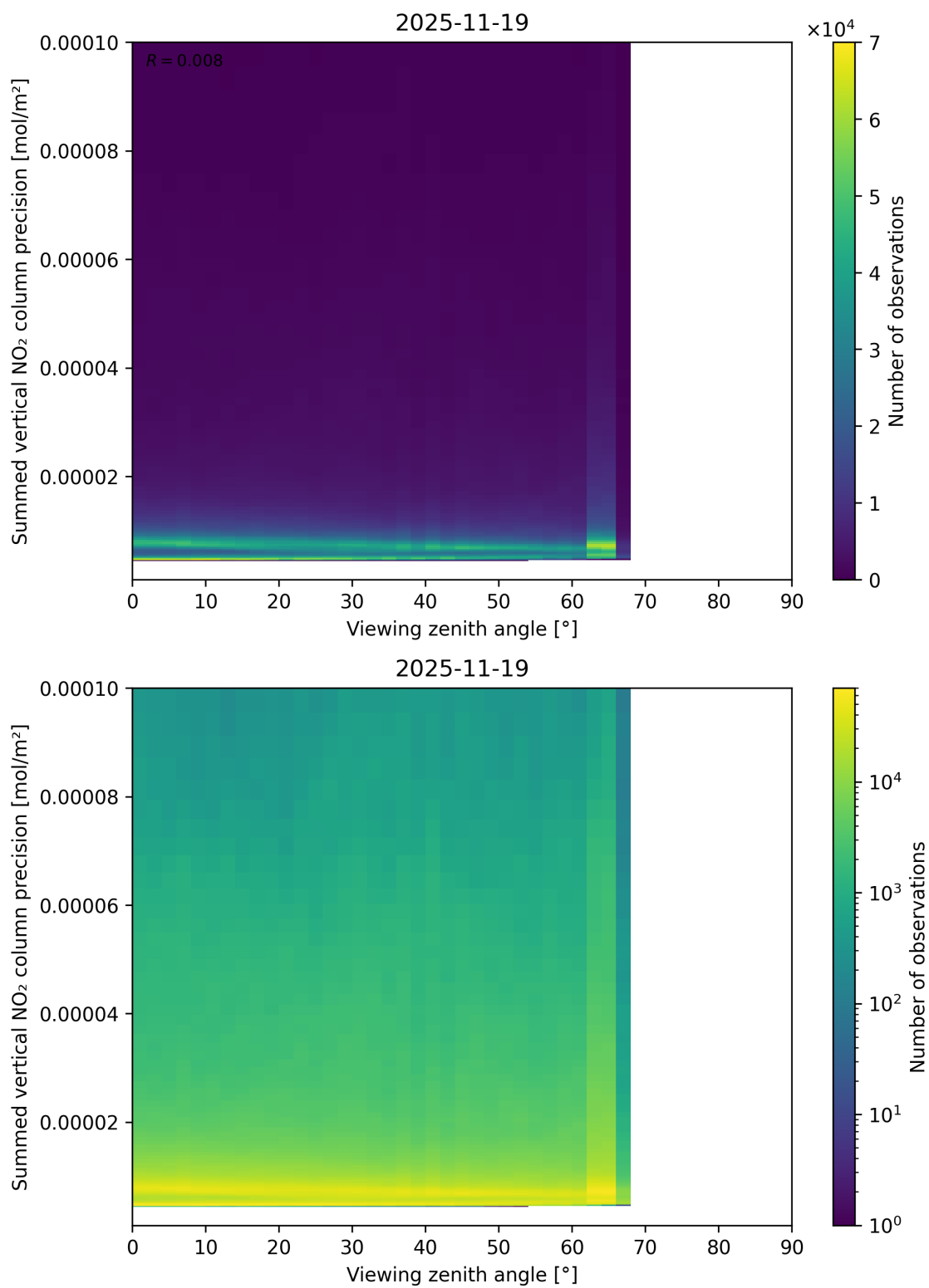
Figure 166: Scatter density plot of “Viewing zenith angle” against “Summed vertical NO 2 column precision” for 2025-11-18 to 2025-11-20.
