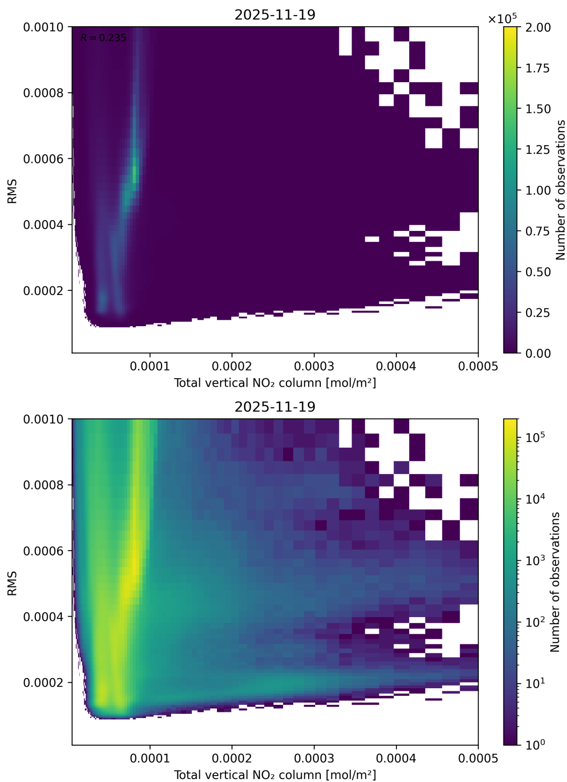
Figure 120: Scatter density plot of “Total vertical NO 2 column” against “RMS” for 2025-11-18 to 2025-11-20.
