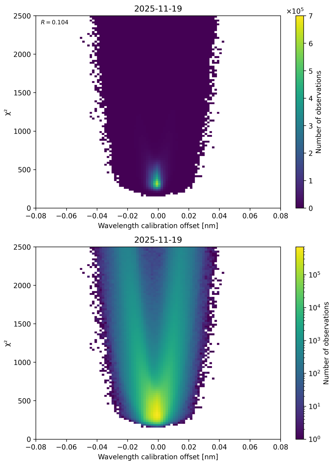
Figure 175: Scatter density plot of “Wavelength calibration offset” against “ \chi^2 ” for 2025-11-18 to 2025-11-20.
