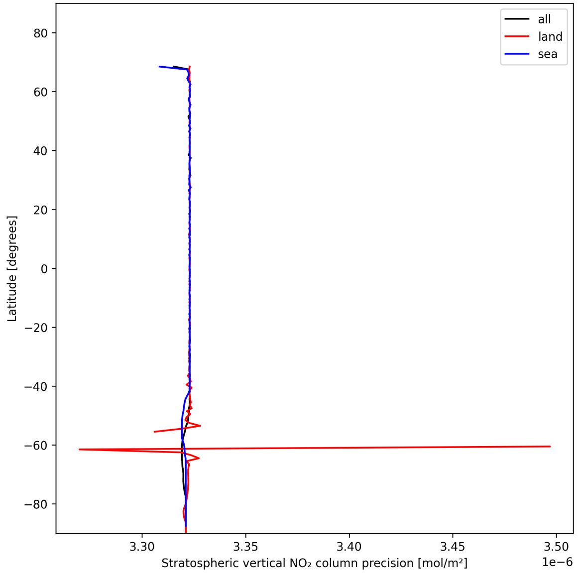
Figure 20: Zonal average of “Stratospheric vertical NO 2 column precision” for 2025-11-18 to 2025-11-20.
