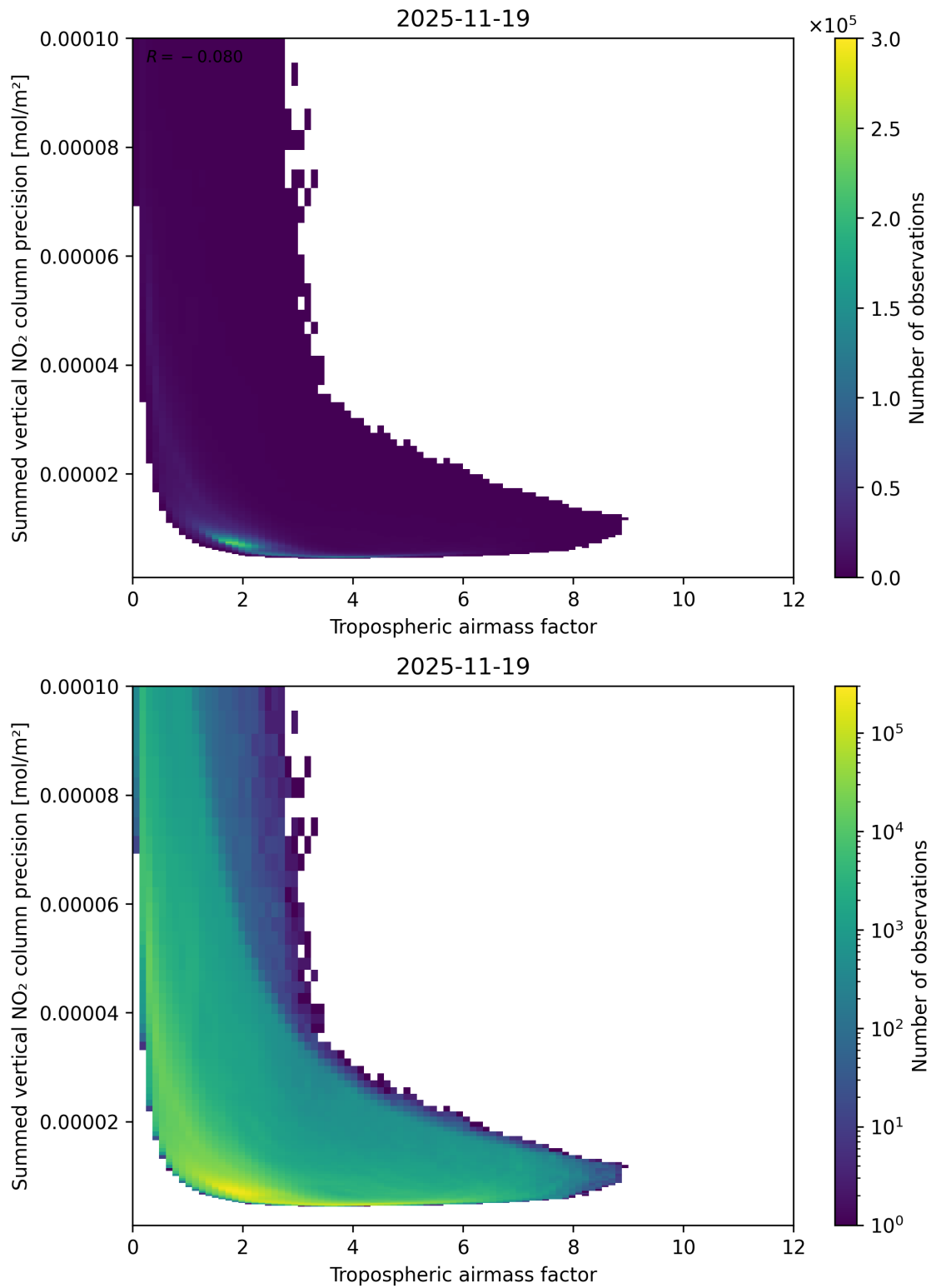
Figure 76: Scatter density plot of “Tropospheric air mass factor” against “Summed vertical NO 2 column precision” for 2025-11-18 to 2025-11-20.
