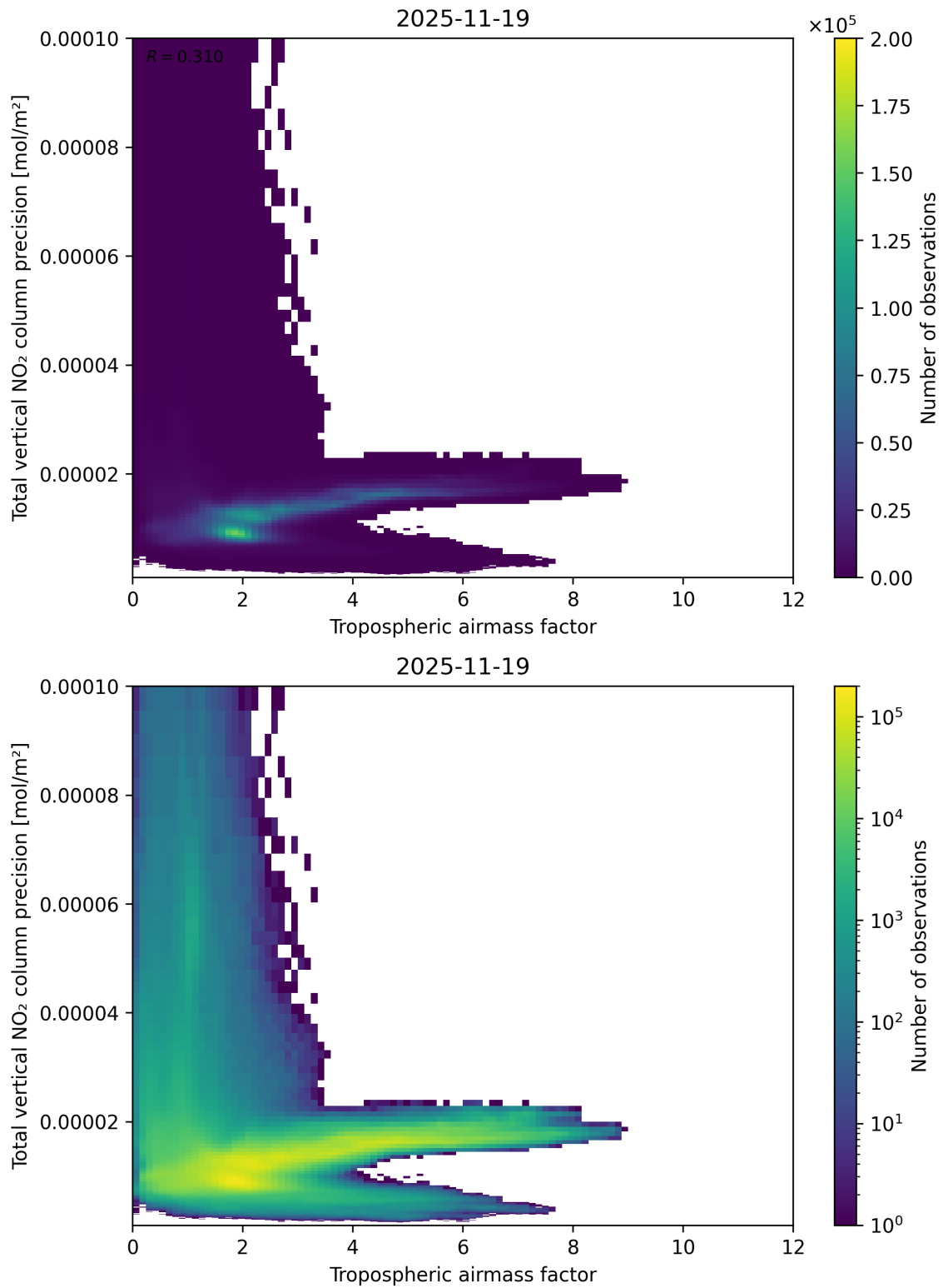
Figure 78: Scatter density plot of “Tropospheric air mass factor” against “Total vertical NO 2 column precision” for 2025-11-18 to 2025-11-20.
