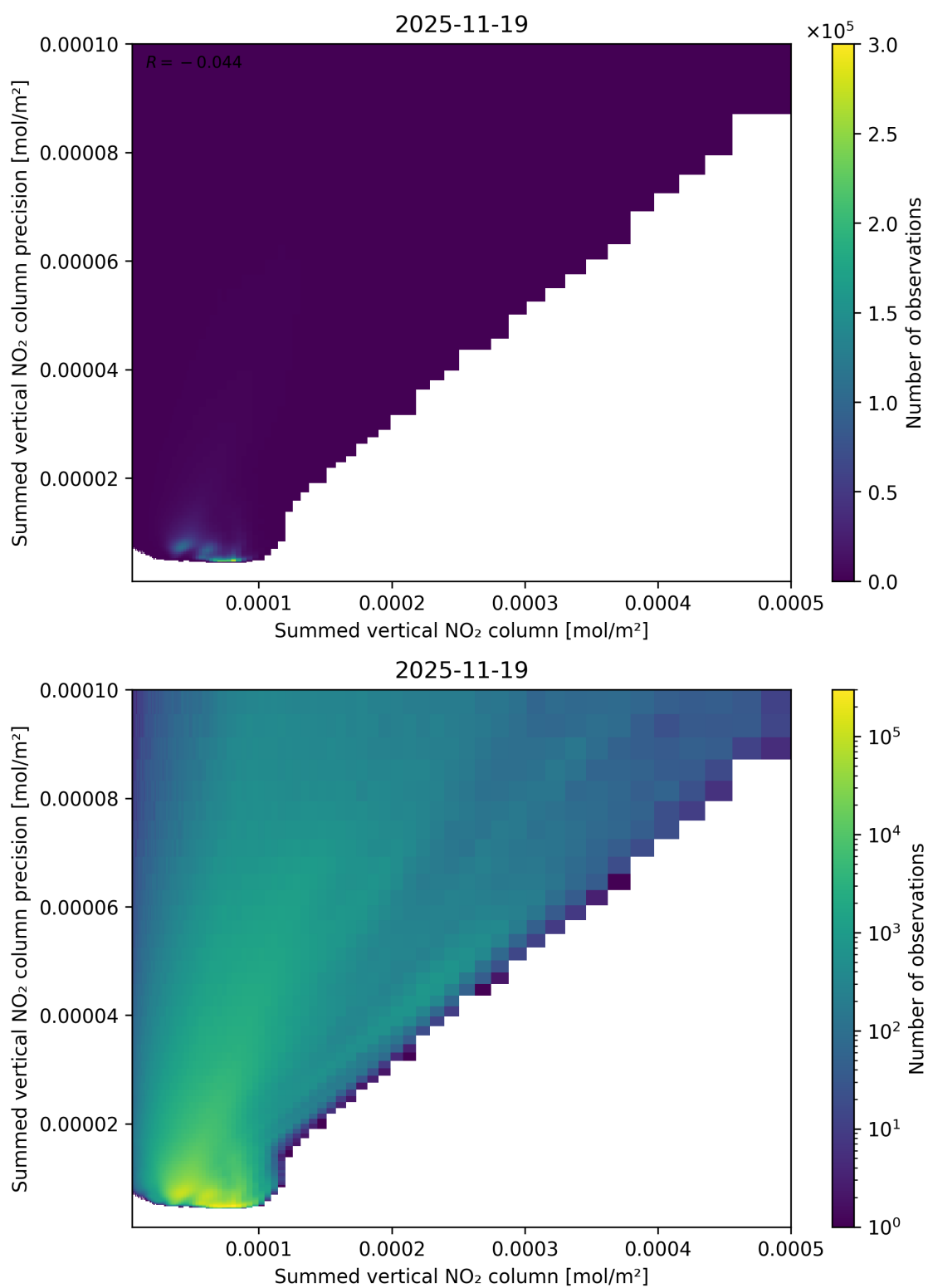
Figure 105: Scatter density plot of “Summed vertical NO 2 column” against “Summed vertical NO 2 column precision” for 2025-11-18 to 2025-11-20.
