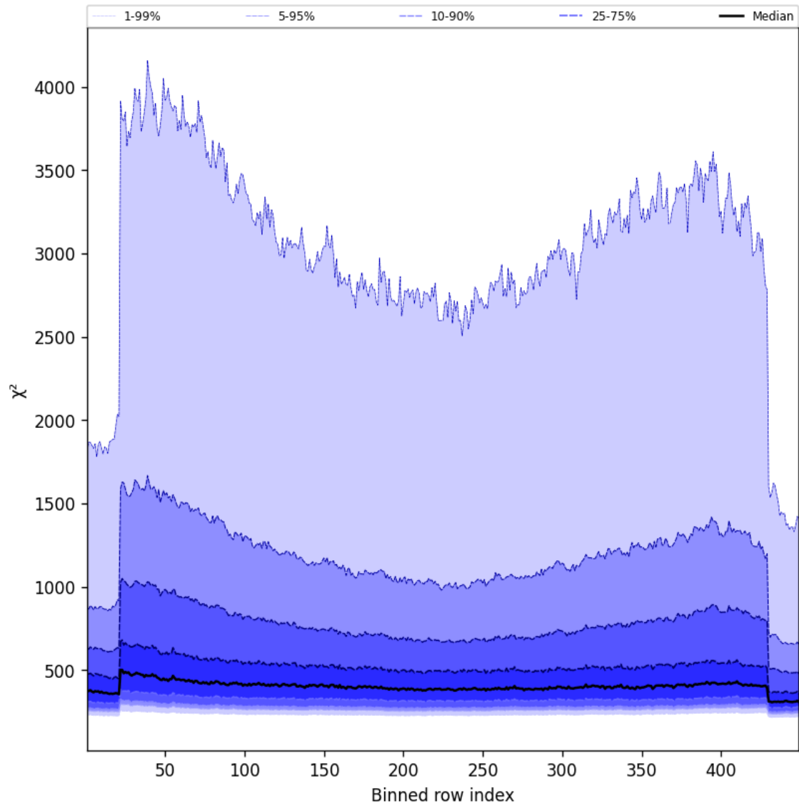
Figure 59: Along track statistics of “ \chi^2 ” for 2025-11-18 to 2025-11-20
