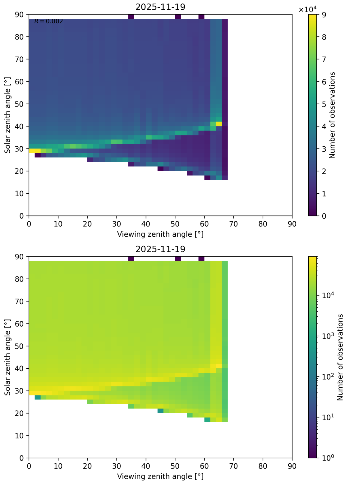
Figure 172: Scatter density plot of “Viewing zenith angle” against “Solar zenith angle” for 2025-11-18 to 2025-11-20.
