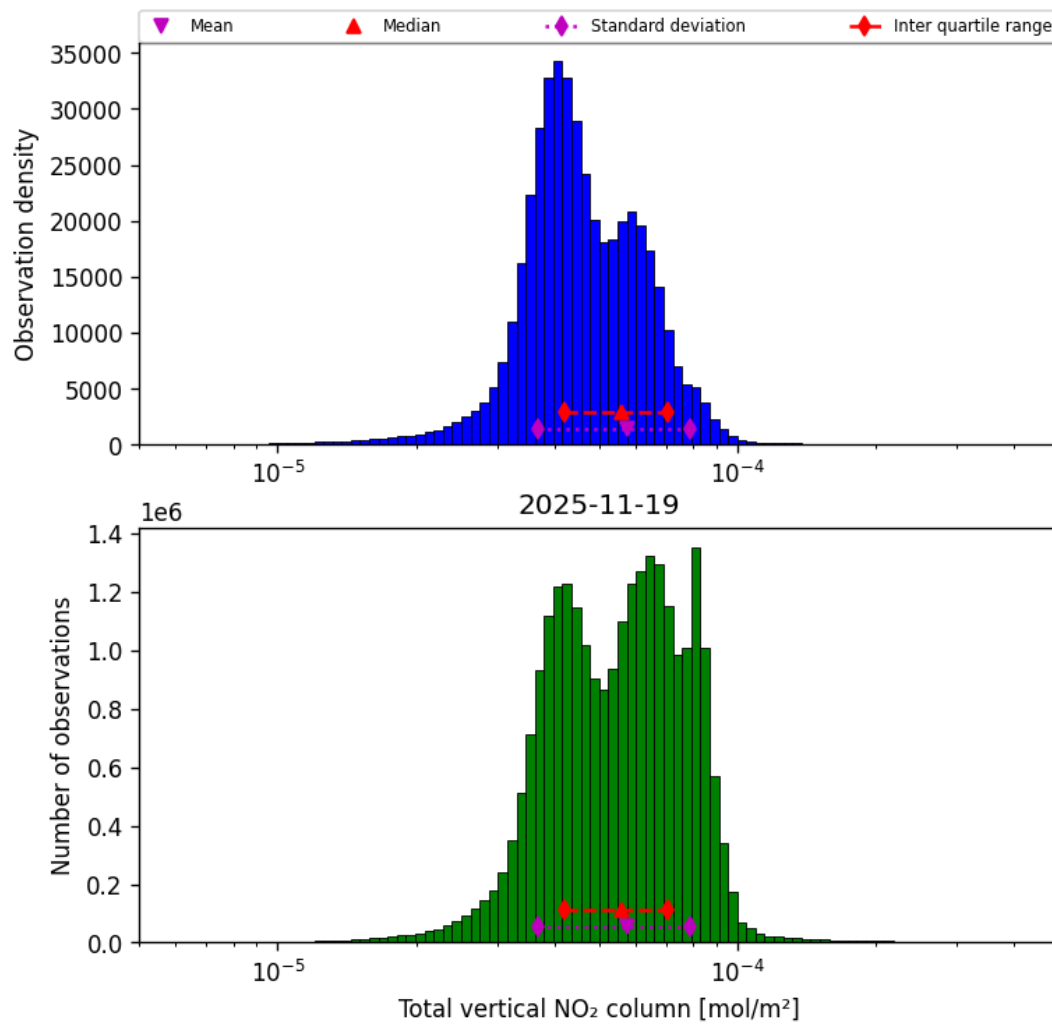
Figure 38: Histogram of “Total vertical NO 2 column” for 2025-11-18 to 2025-11-20
