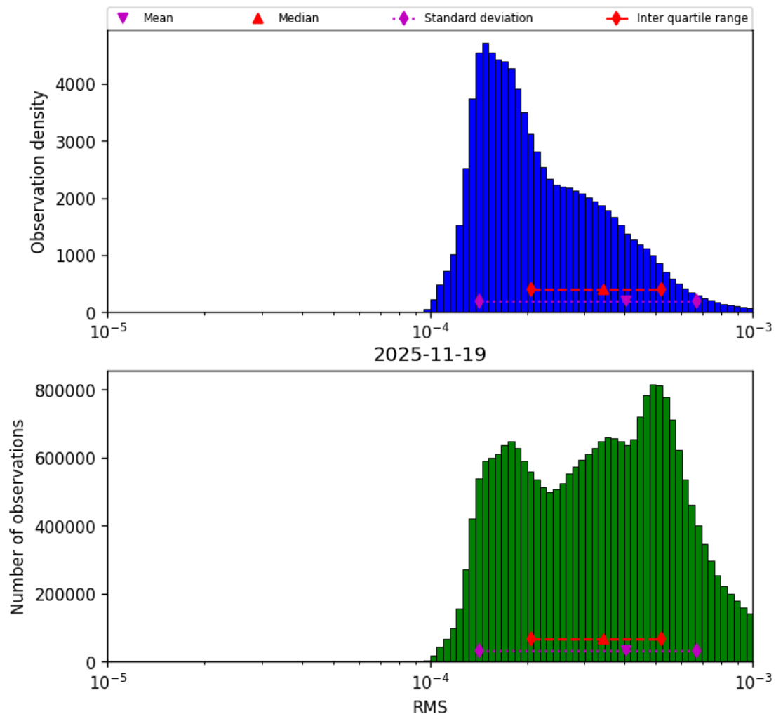
Figure 43: Histogram of “RMS” for 2025-11-18 to 2025-11-20
