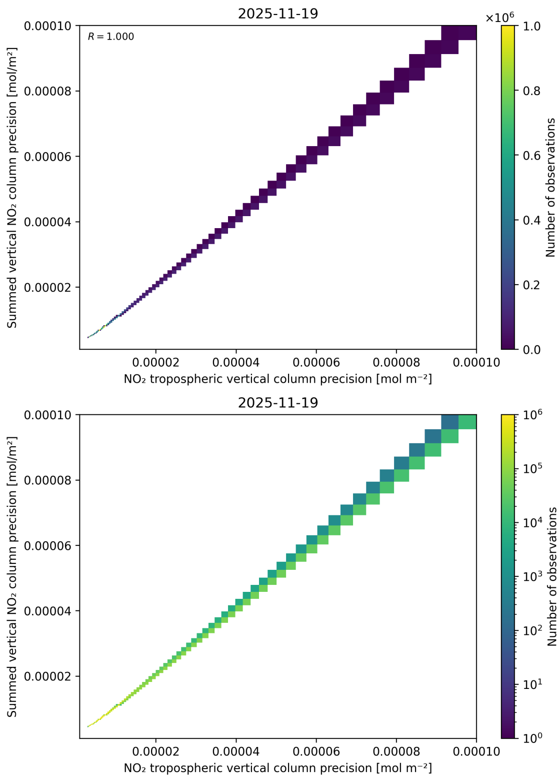
Figure 137: Scatter density plot of “NO 2 tropospheric vertical column precision” against “Summed vertical NO 2 column precision” for 2025-11-18 to 2025-11-20.
