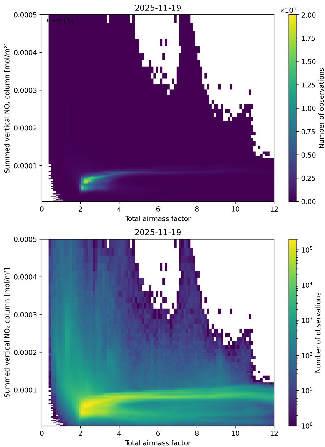
Figure 65: Scatter density plot of “Total airmass factor” against “Summed vertical NO 2 column” for 2025-11-18 to 2025-11-20.
