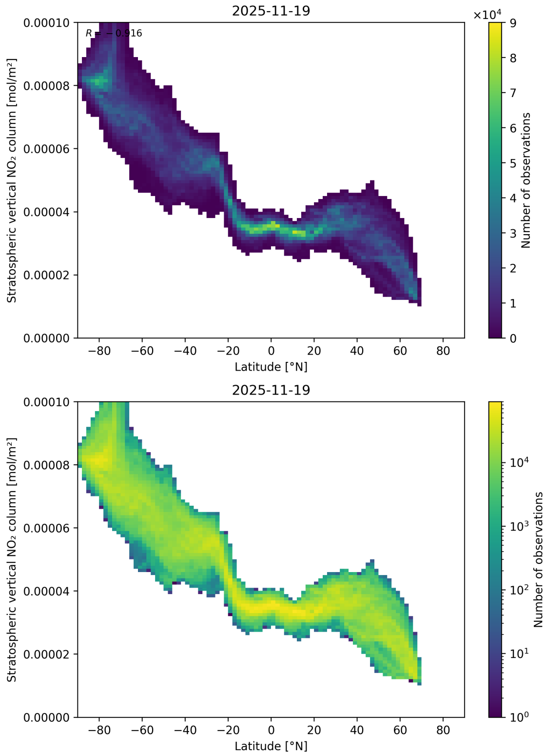
Figure 87: Scatter density plot of “Latitude” against “Stratospheric vertical NO 2 column” for 2025-11-18 to 2025-11-20.
