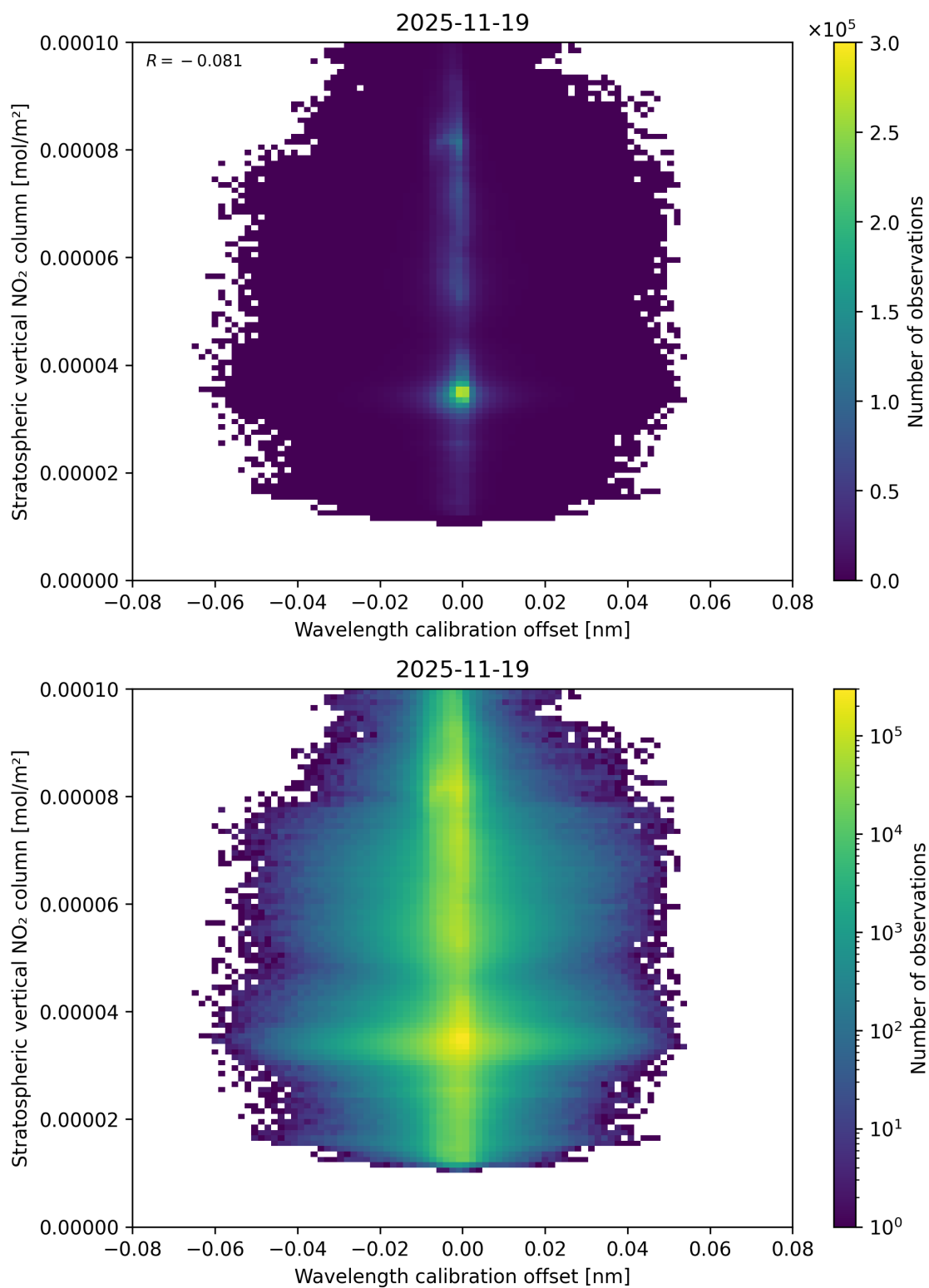
Figure 176: Scatter density plot of “Wavelength calibration offset” against “Stratospheric vertical NO 2 column” for 2025-11-18 to 2025-11-20.
