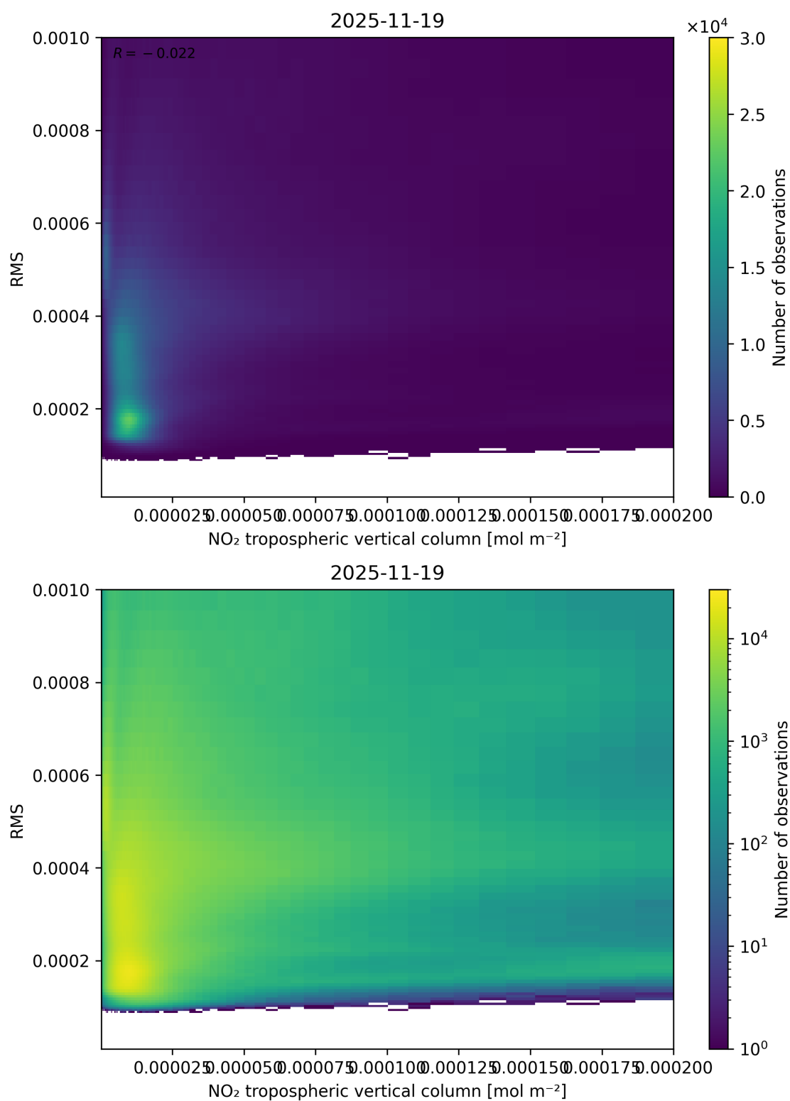
Figure 142: Scatter density plot of “NO 2 tropospheric vertical column” against “RMS” for 2025-11-18 to 2025-11-20.
