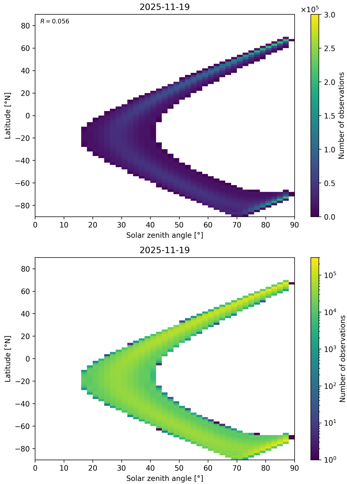
Figure 149: Scatter density plot of “Solar zenith angle” against “Latitude” for 2025-11-18 to 2025-11-20.
