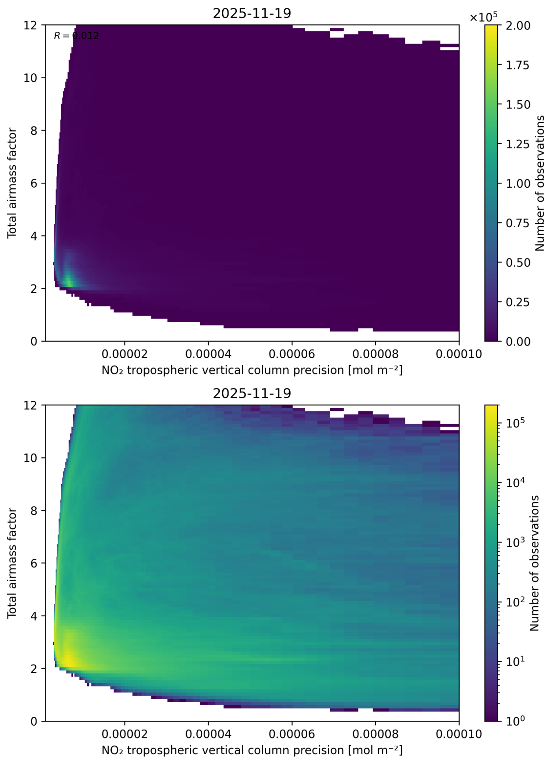
Figure 132: Scatter density plot of “NO 2 tropospheric vertical column precision” against “Total air mass factor” for 2025-11-18 to 2025-11-20.
