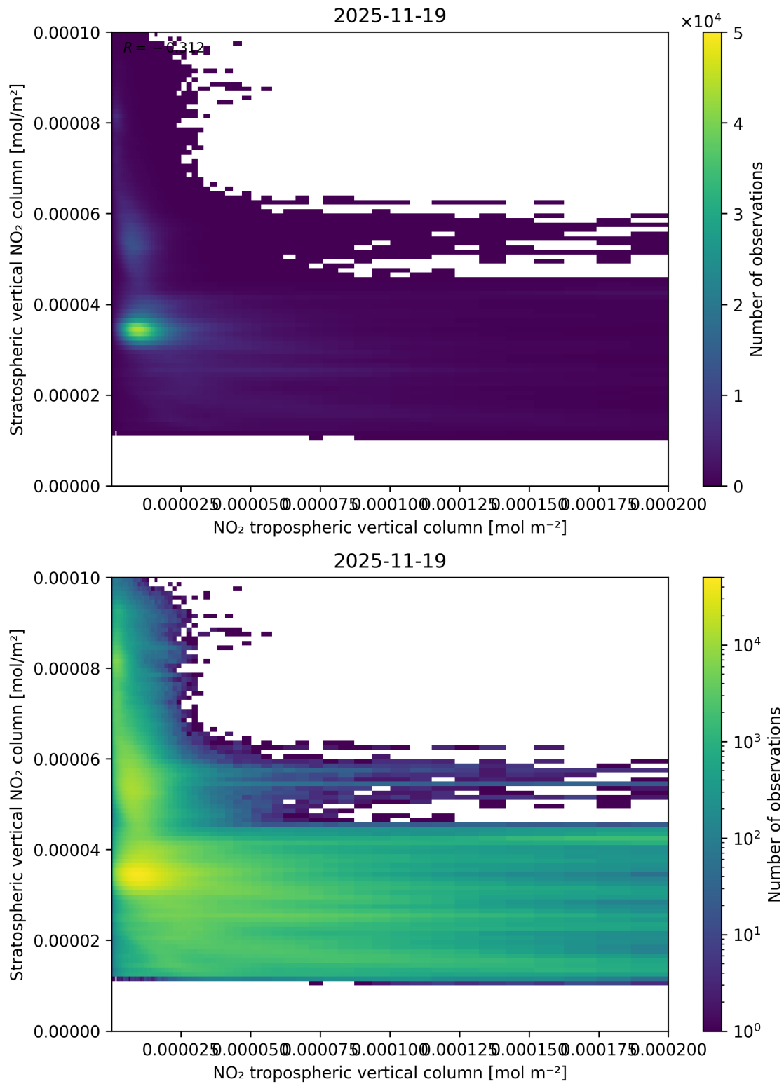
Figure 125: Scatter density plot of “NO 2 tropospheric vertical column” against “Stratospheric vertical NO 2 column” for 2025-11-18 to 2025-11-20.
