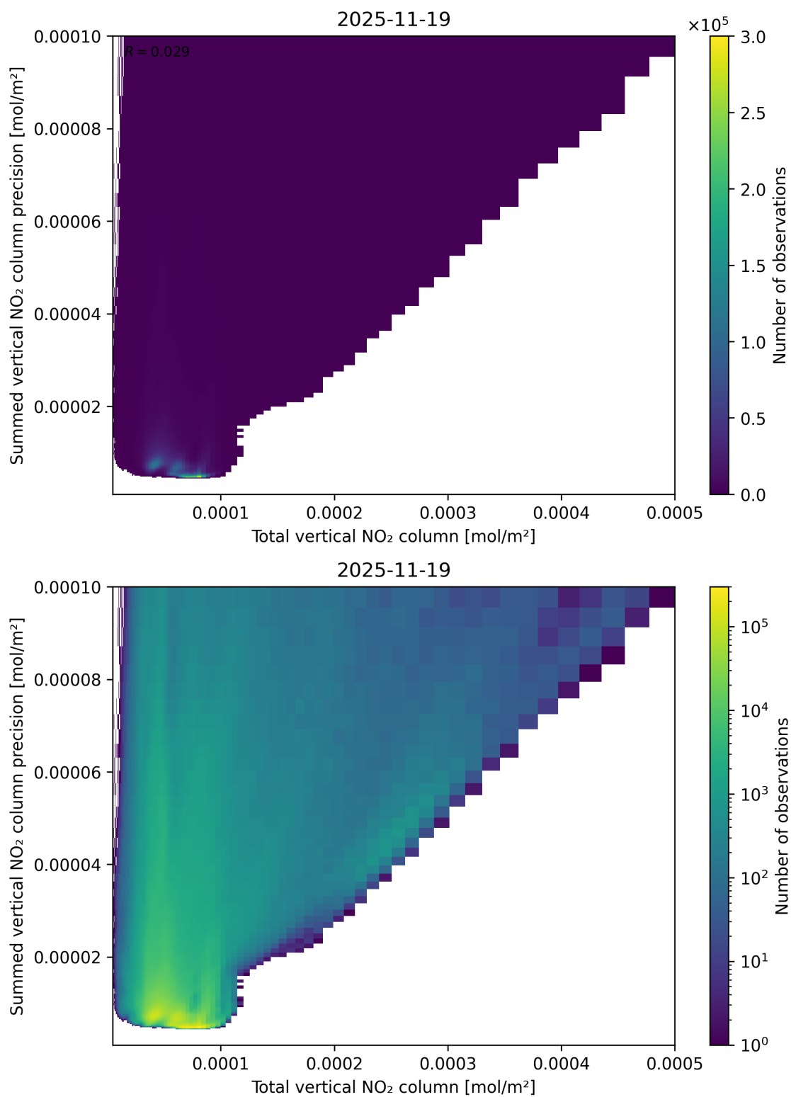
Figure 113: Scatter density plot of “Total vertical NO 2 column” against “Summed vertical NO 2 column precision” for 2025-11-18 to 2025-11-20.
