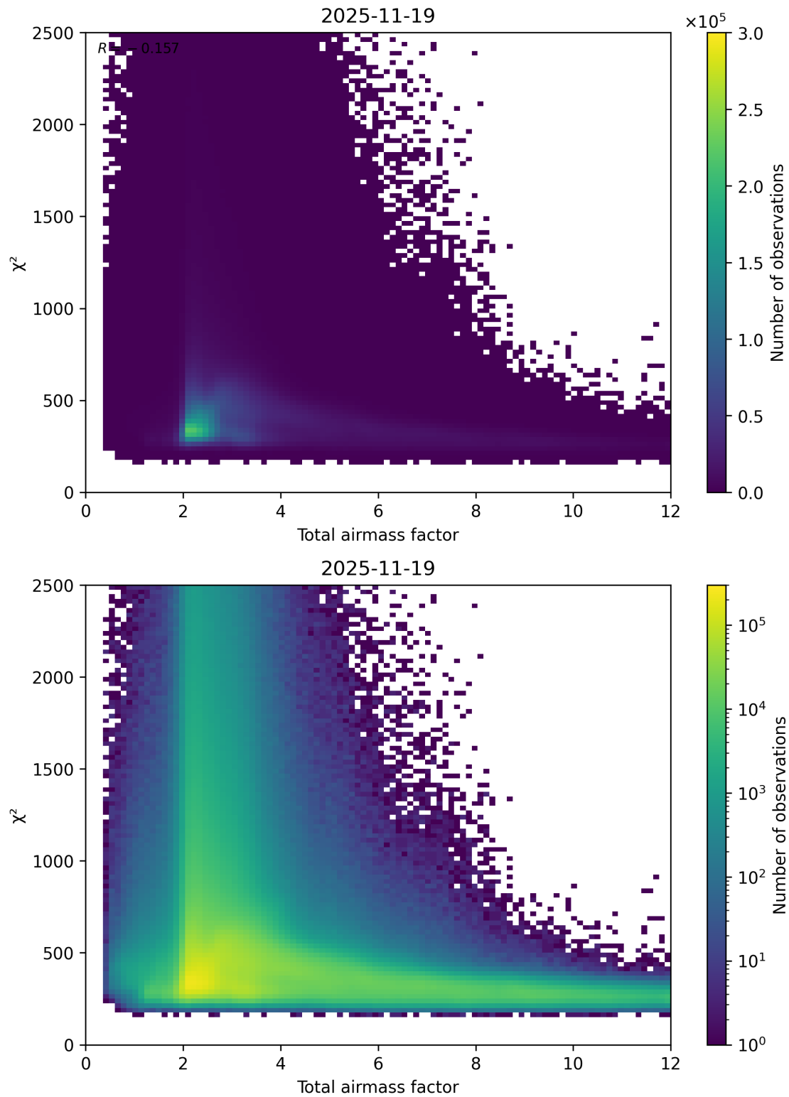
Figure 63: Scatter density plot of “Total airmass factor” against “ \chi^2 ” for 2025-11-18 to 2025-11-20.
