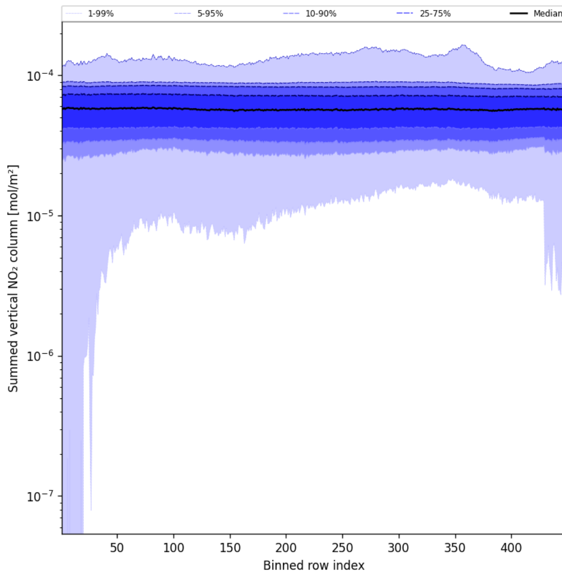
Figure 57: Along track statistics of “Summed vertical NO 2 column” for 2025-11-18 to 2025-11-20
