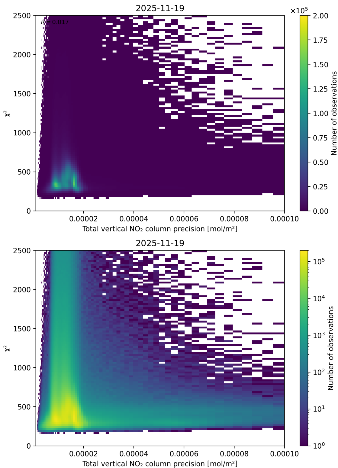
Figure 116: Scatter density plot of “Total vertical NO 2 column precision” against “ \chi^2 ” for 2025-11-18 to 2025-11-20.
