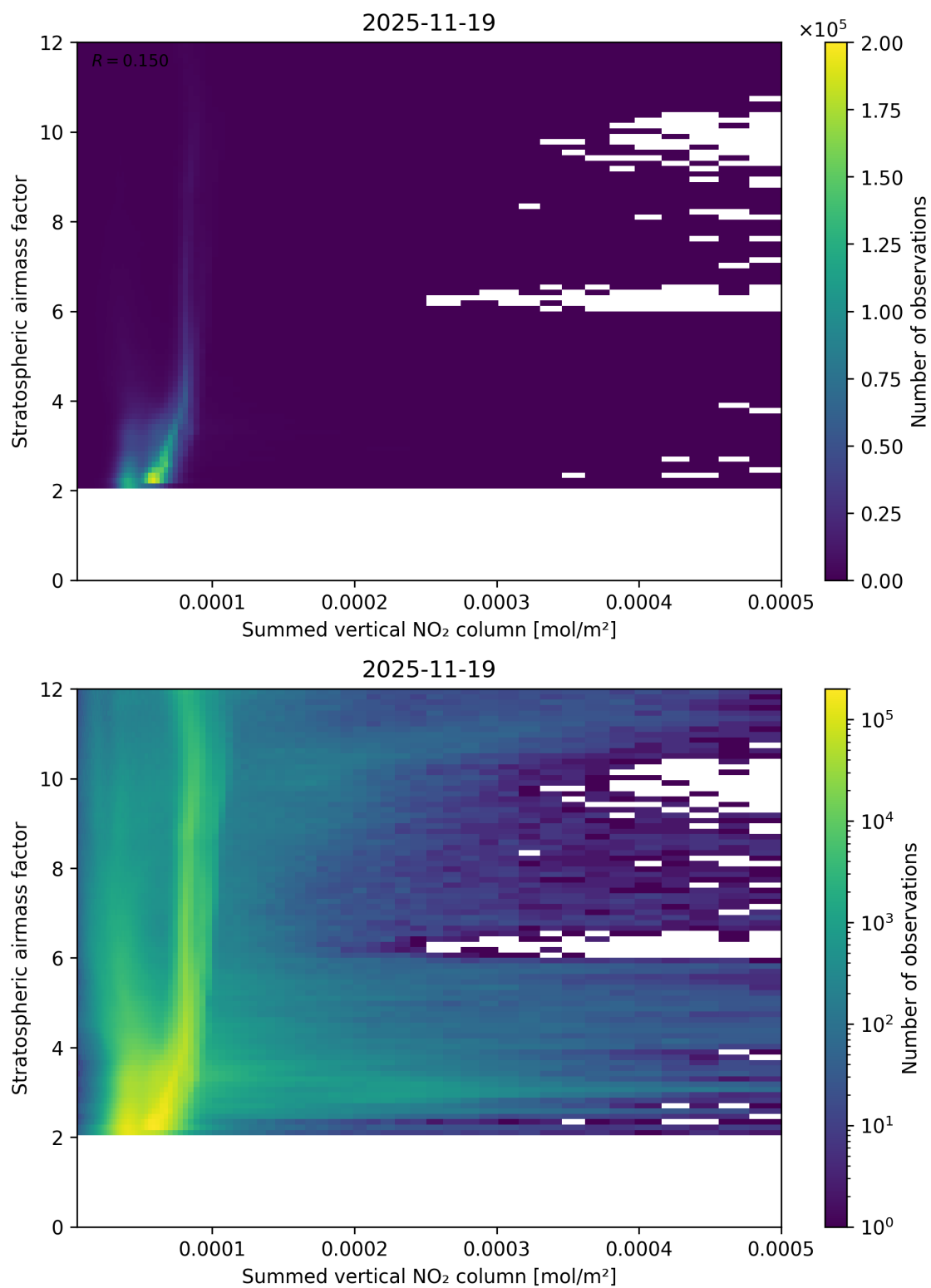
Figure 103: Scatter density plot of “Summed vertical NO 2 column” against “Stratospheric air mass factor” for 2025-11-18 to 2025-11-20.
