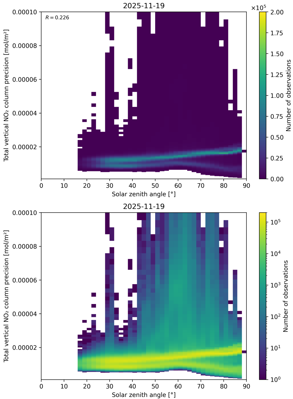
Figure 154: Scatter density plot of “Solar zenith angle” against “Total vertical NO 2 column precision” for 2025-11-18 to 2025-11-20.
