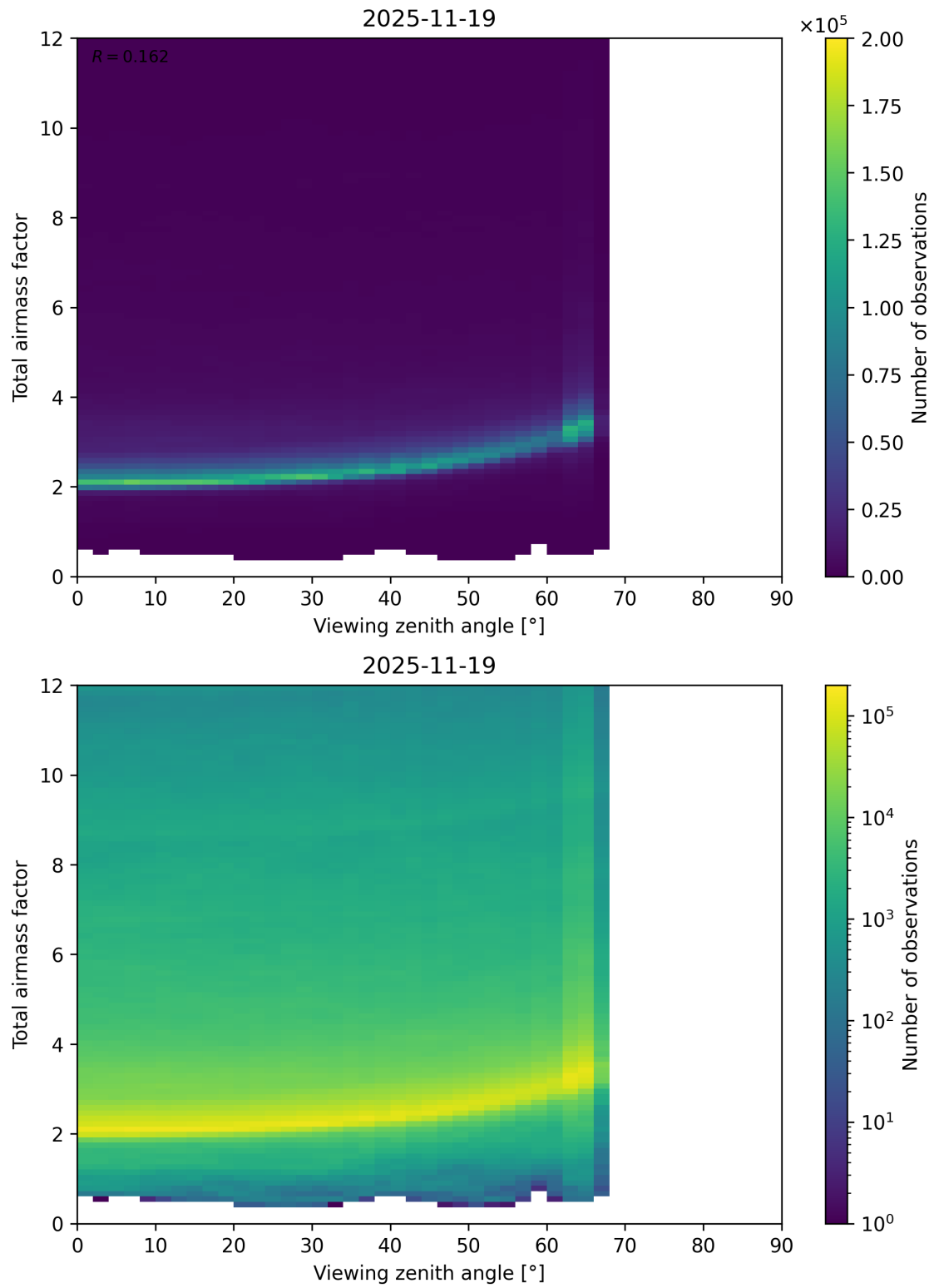
Figure 160: Scatter density plot of “Viewing zenith angle” against “Total airmass factor” for 2025-11-18 to 2025-11-20.
