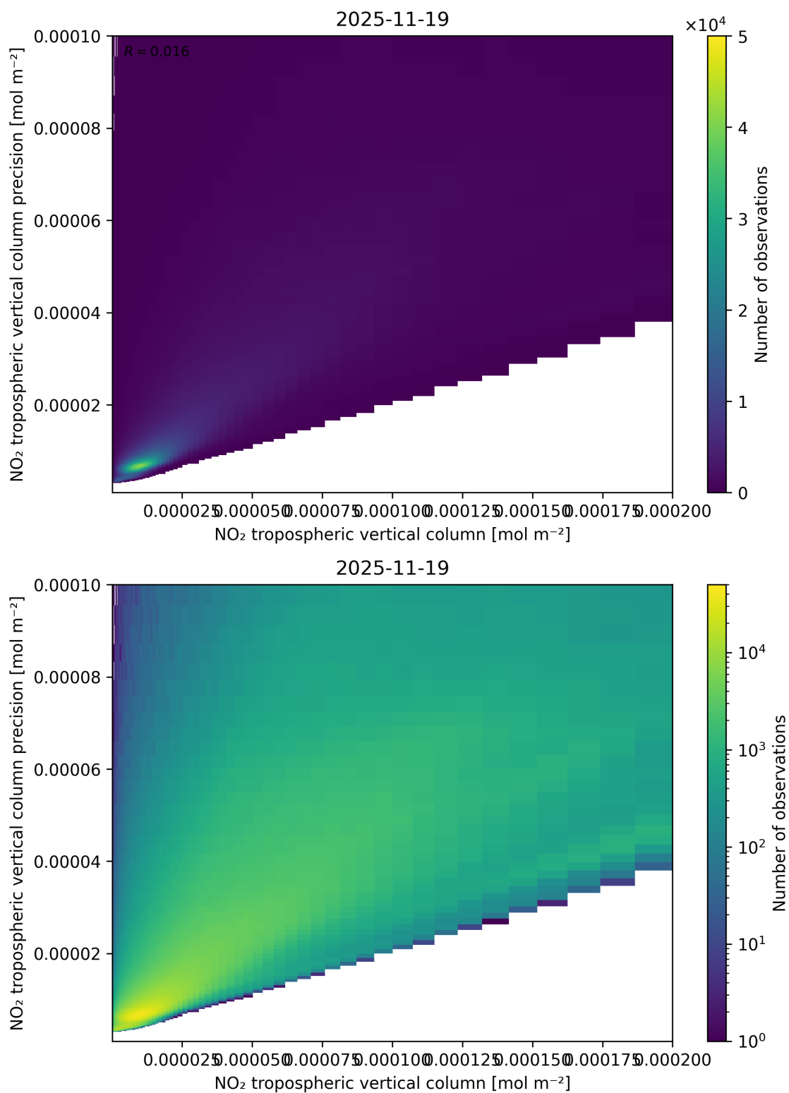
Figure 130: Scatter density plot of “NO 2 tropospheric vertical column” against “NO 2 tropospheric vertical column precision” for 2025-11-18 to 2025-11-20.
