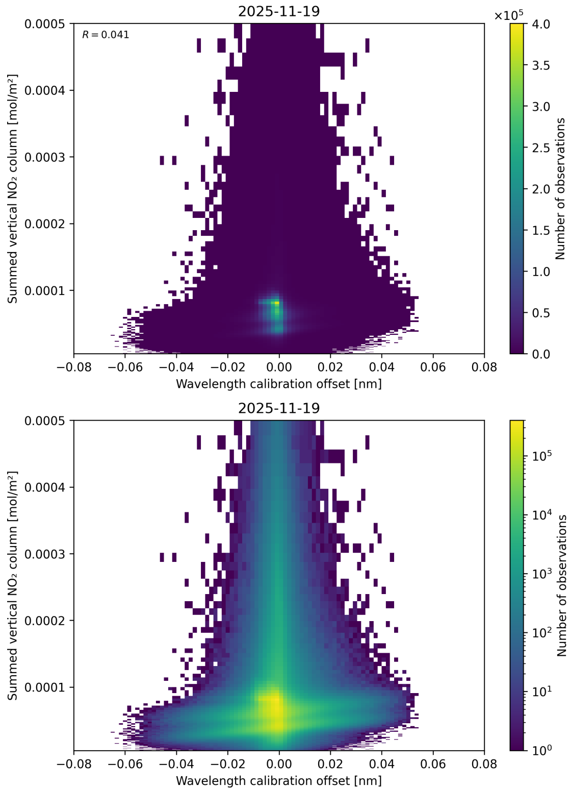
Figure 177: Scatter density plot of “Wavelength calibration offset” against “Summed vertical NO 2 column” for 2025-11-18 to 2025-11-20.
