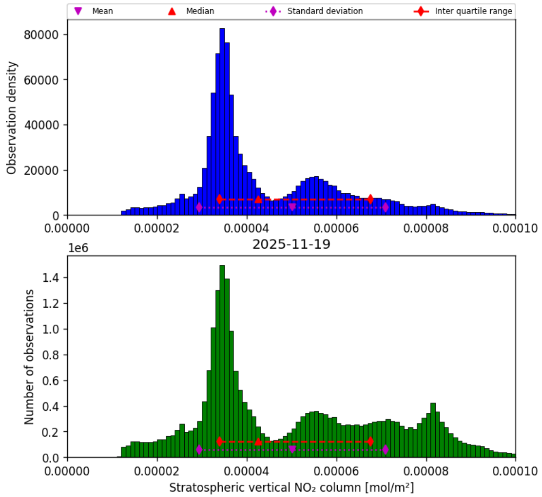
Figure 36: Histogram of “Stratospheric vertical NO 2 column” for 2025-11-18 to 2025-11-20
