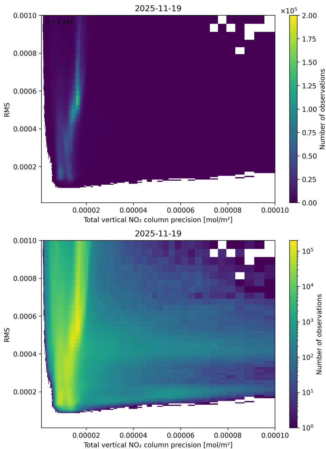
Figure 119: Scatter density plot of “Total vertical NO 2 column precision” against “RMS” for 2025-11-18 to 2025-11-20.
