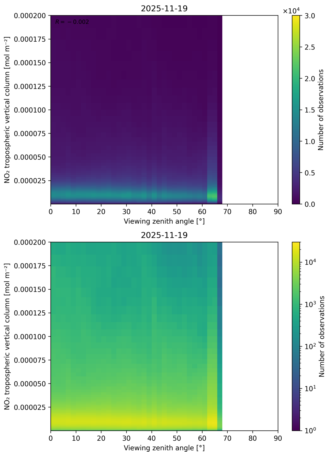
Figure 169: Scatter density plot of “Viewing zenith angle” against “NO 2 tropospheric vertical column” for 2025-11-18 to 2025-11-20.
