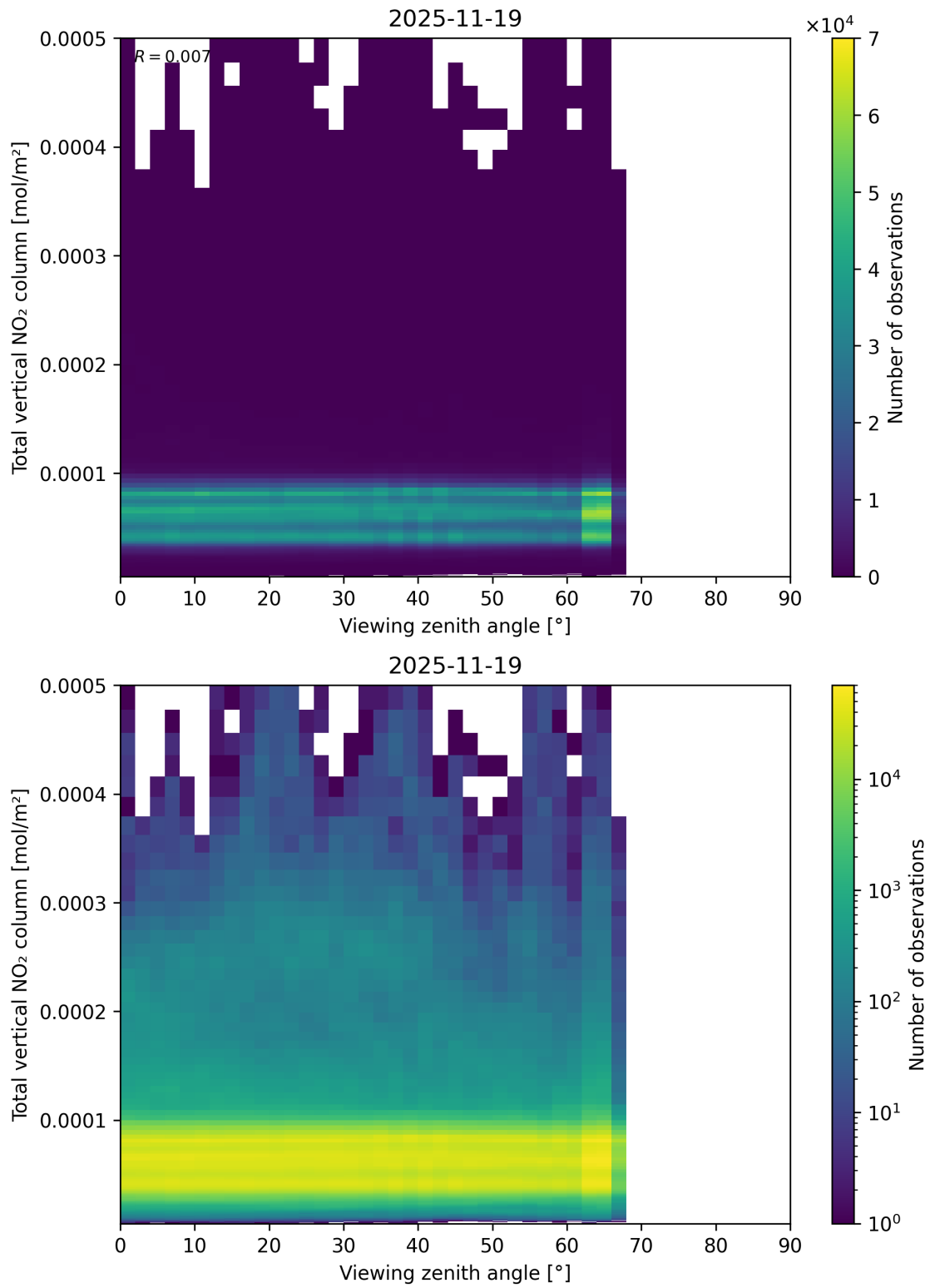
Figure 167: Scatter density plot of “Viewing zenith angle” against “Total vertical NO 2 column” for 2025-11-18 to 2025-11-20.
