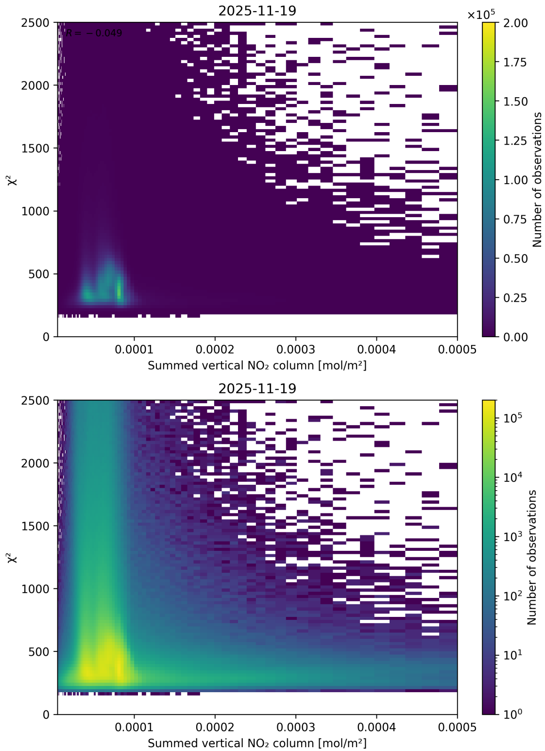
Figure 104: Scatter density plot of “Summed vertical NO 2 column” against “ \chi^2 ” for 2025-11-18 to 2025-11-20.
