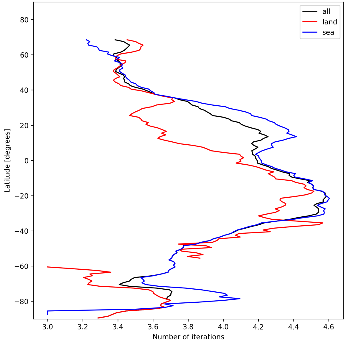
Figure 17: Zonal average of “Number of iterations” for 2025-11-18 to 2025-11-20.
