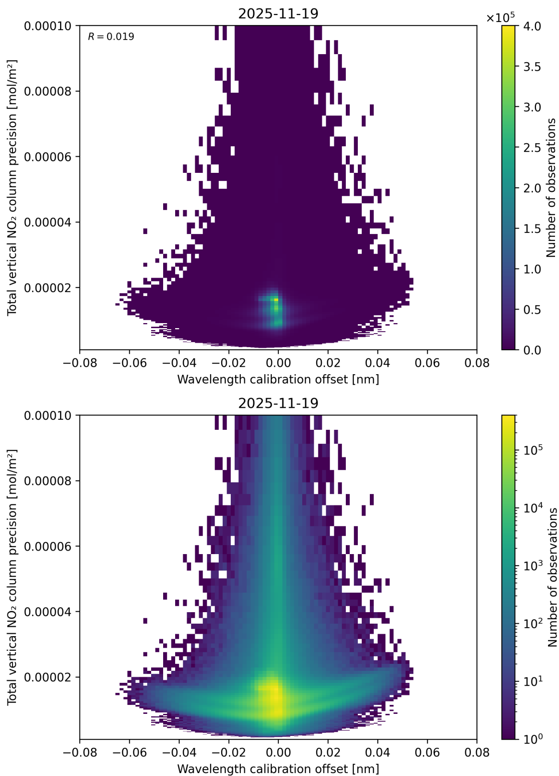
Figure 180: Scatter density plot of “Wavelength calibration offset” against “Total vertical NO 2 column precision” for 2025-11-18 to 2025-11-20.
