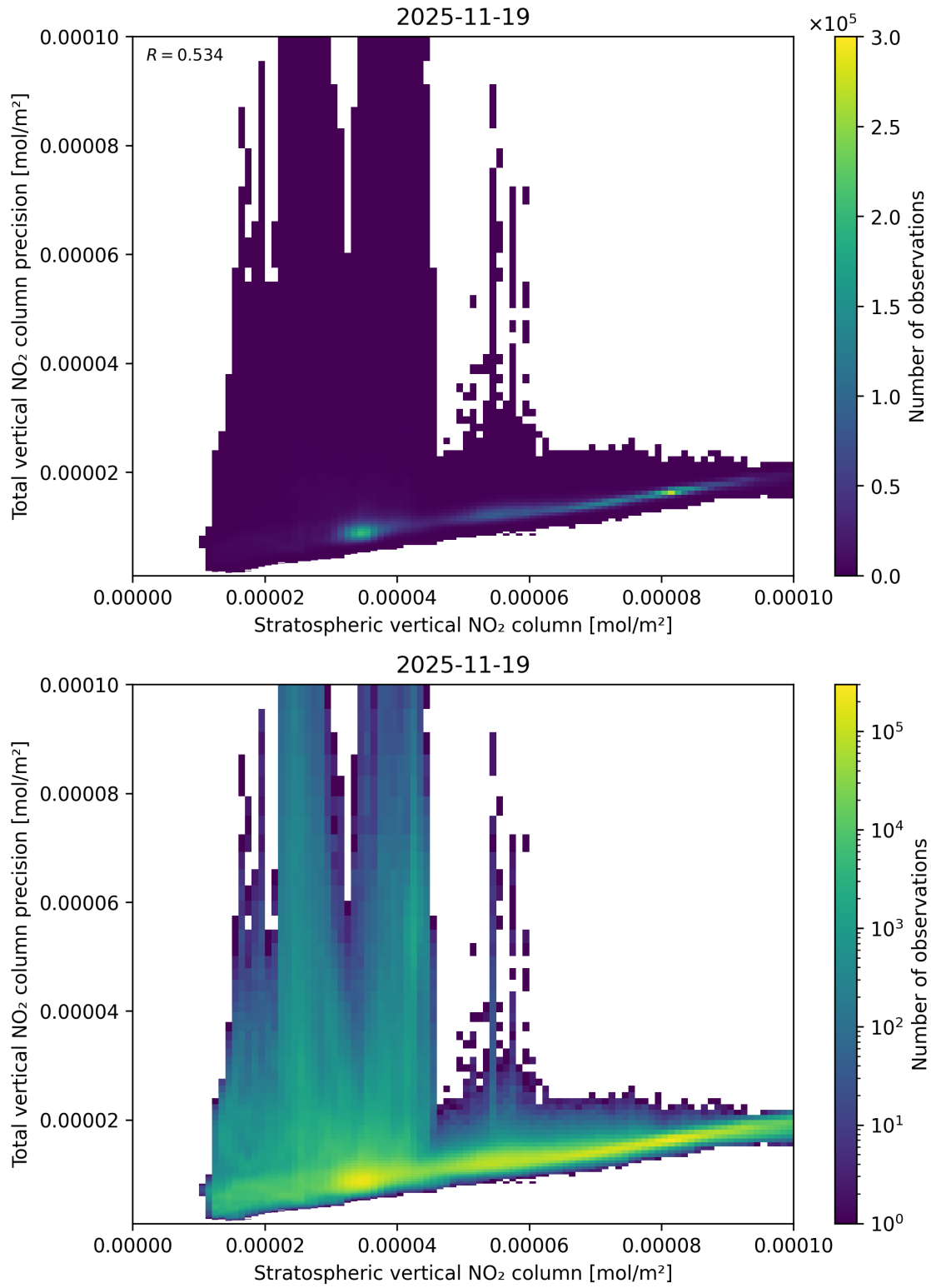
Figure 101: Scatter density plot of “Stratospheric vertical NO 2 column” against “Total vertical NO 2 column precision” for 2025-11-18 to 2025-11-20.
