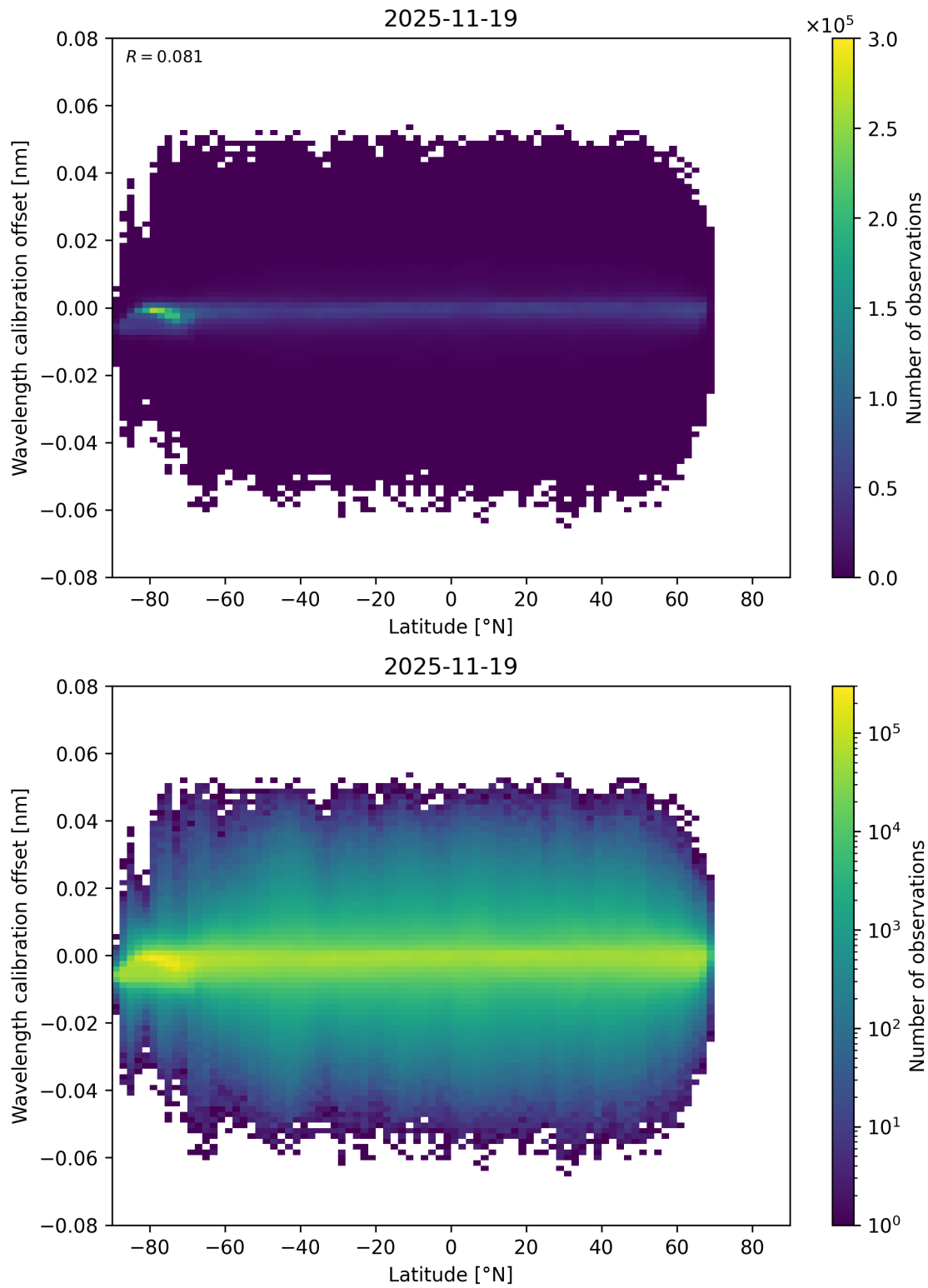
Figure 95: Scatter density plot of “Latitude” against “Wavelength calibration offset” for 2025-11-18 to 2025-11-20.
