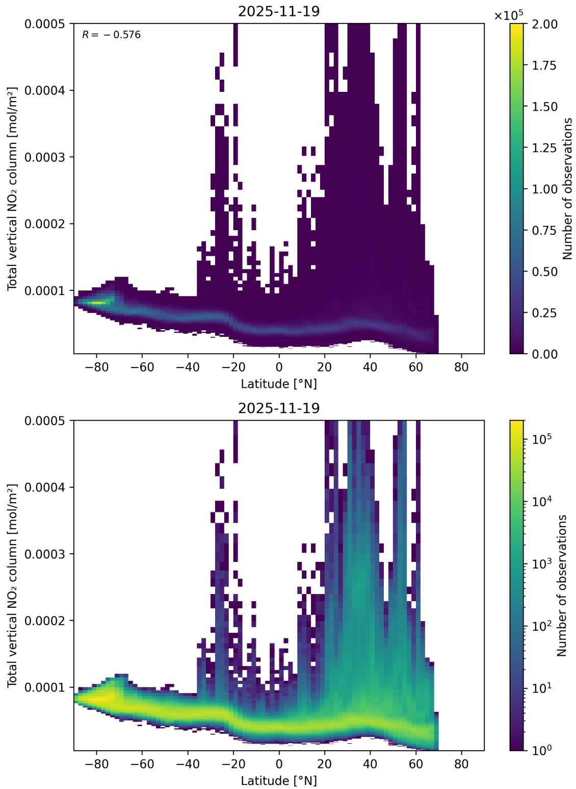
Figure 90: Scatter density plot of “Latitude” against “Total vertical NO 2 column” for 2025-11-18 to 2025-11-20.
