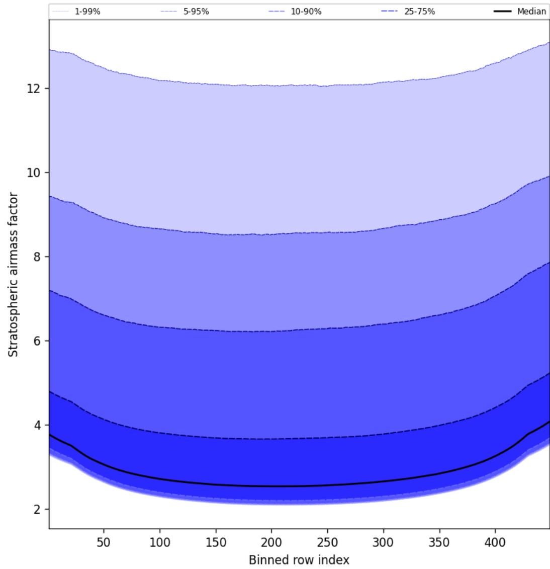
Figure 61: Along track statistics of “Stratospheric airmass factor” for 2025-11-18 to 2025-11-20
