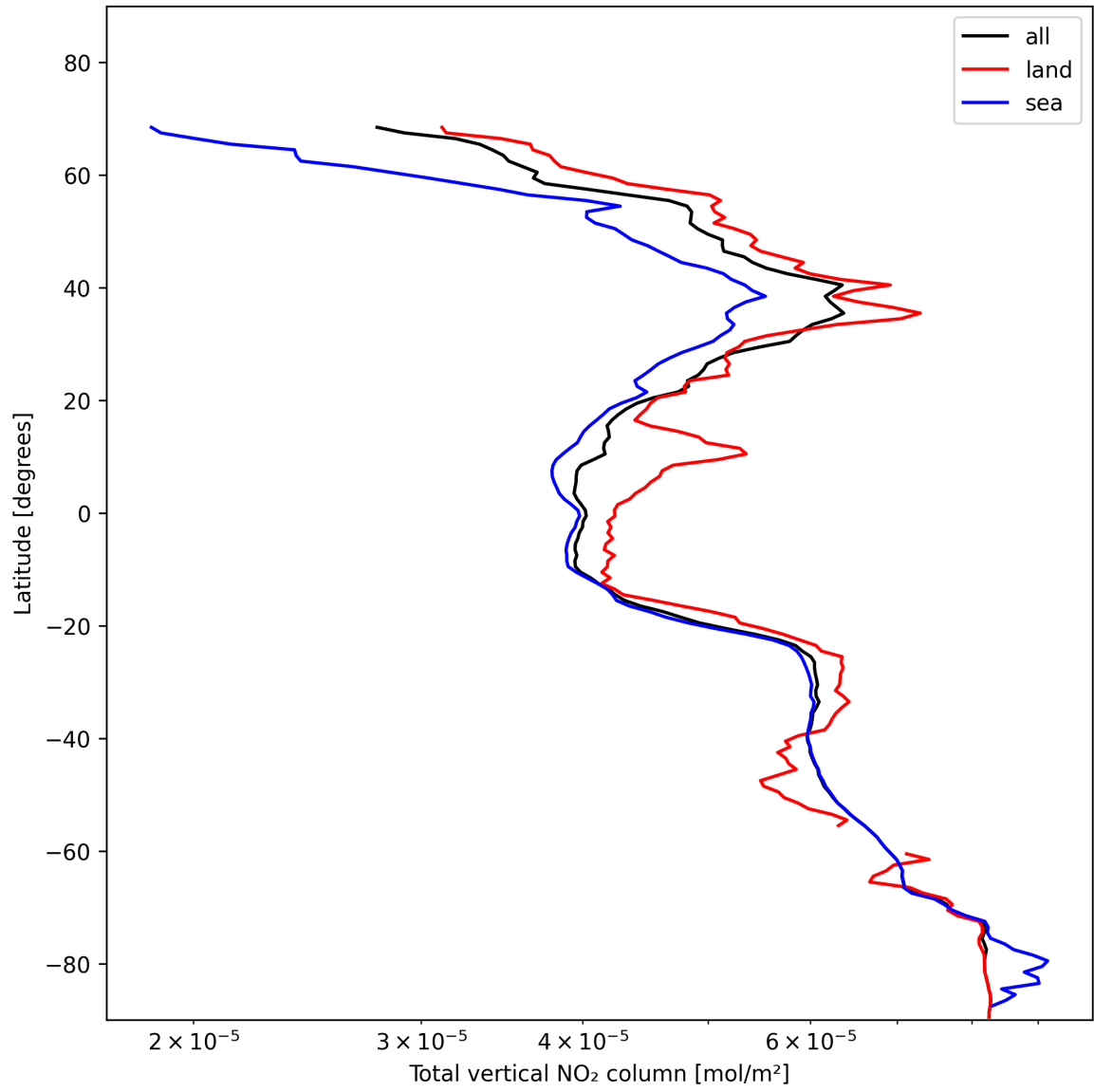
Figure 21: Zonal average of “Total vertical NO 2 column” for 2025-11-18 to 2025-11-20.
