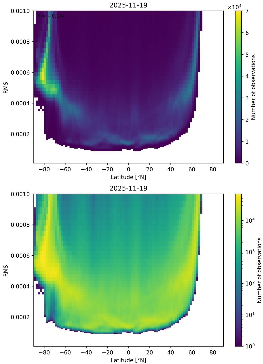
Figure 94: Scatter density plot of “Latitude” against “RMS” for 2025-11-18 to 2025-11-20.
