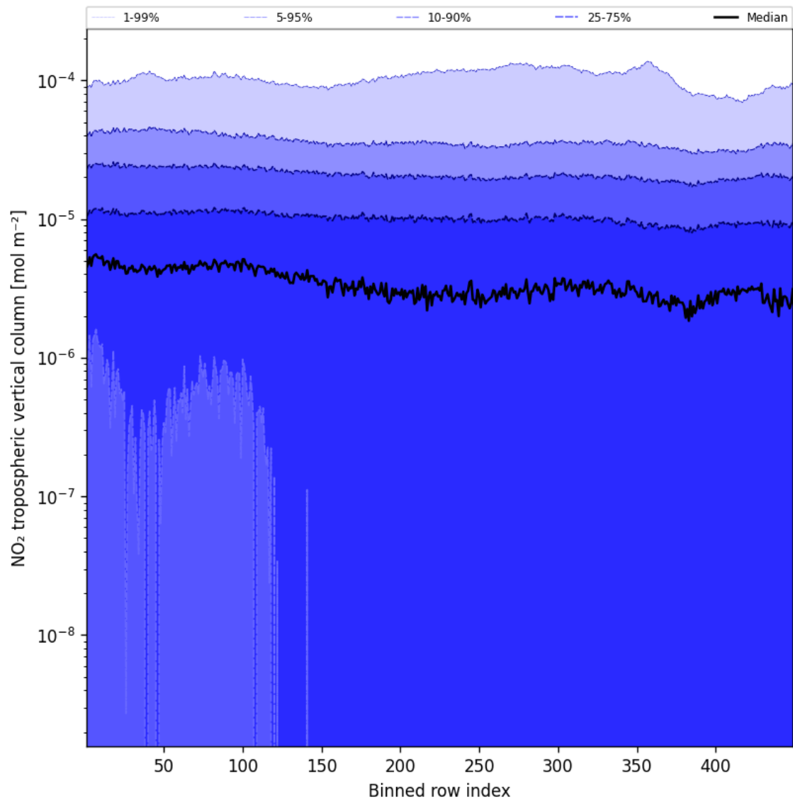
Figure 46: Along track statistics of “NO 2 tropospheric vertical column” for 2025-11-18 to 2025-11-20
