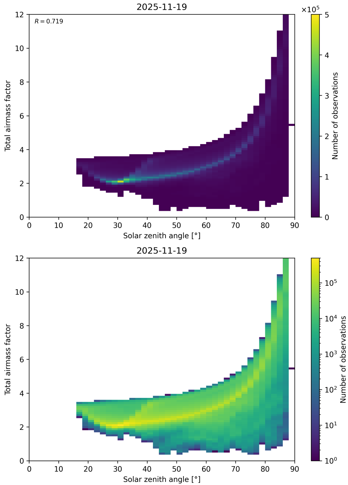
Figure 146: Scatter density plot of “Solar zenith angle” against “Total airmass factor” for 2025-11-18 to 2025-11-20.
