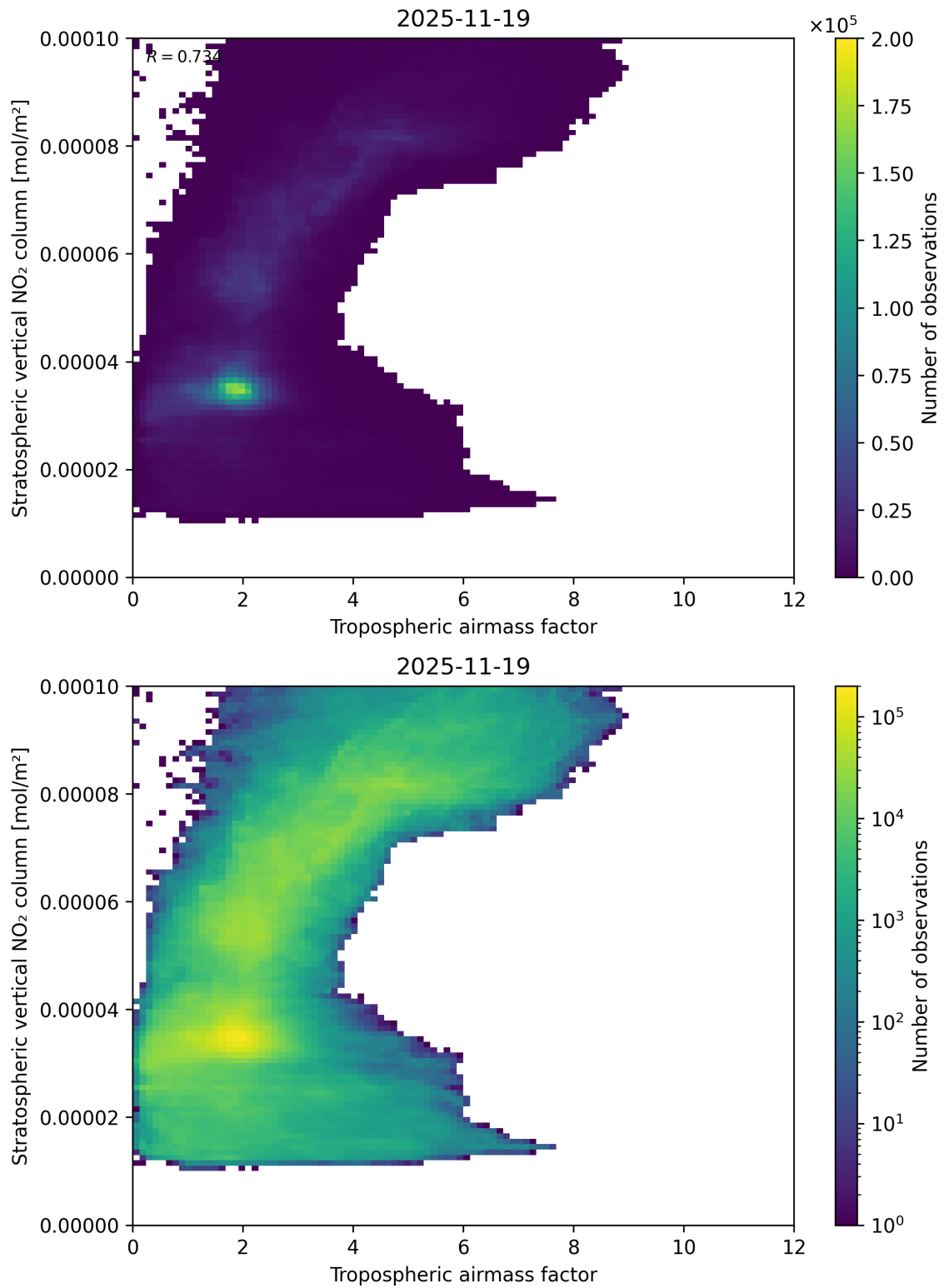
Figure 74: Scatter density plot of “Tropospheric airmass factor” against “Stratospheric vertical NO 2 column” for 2025-11-18 to 2025-11-20.
