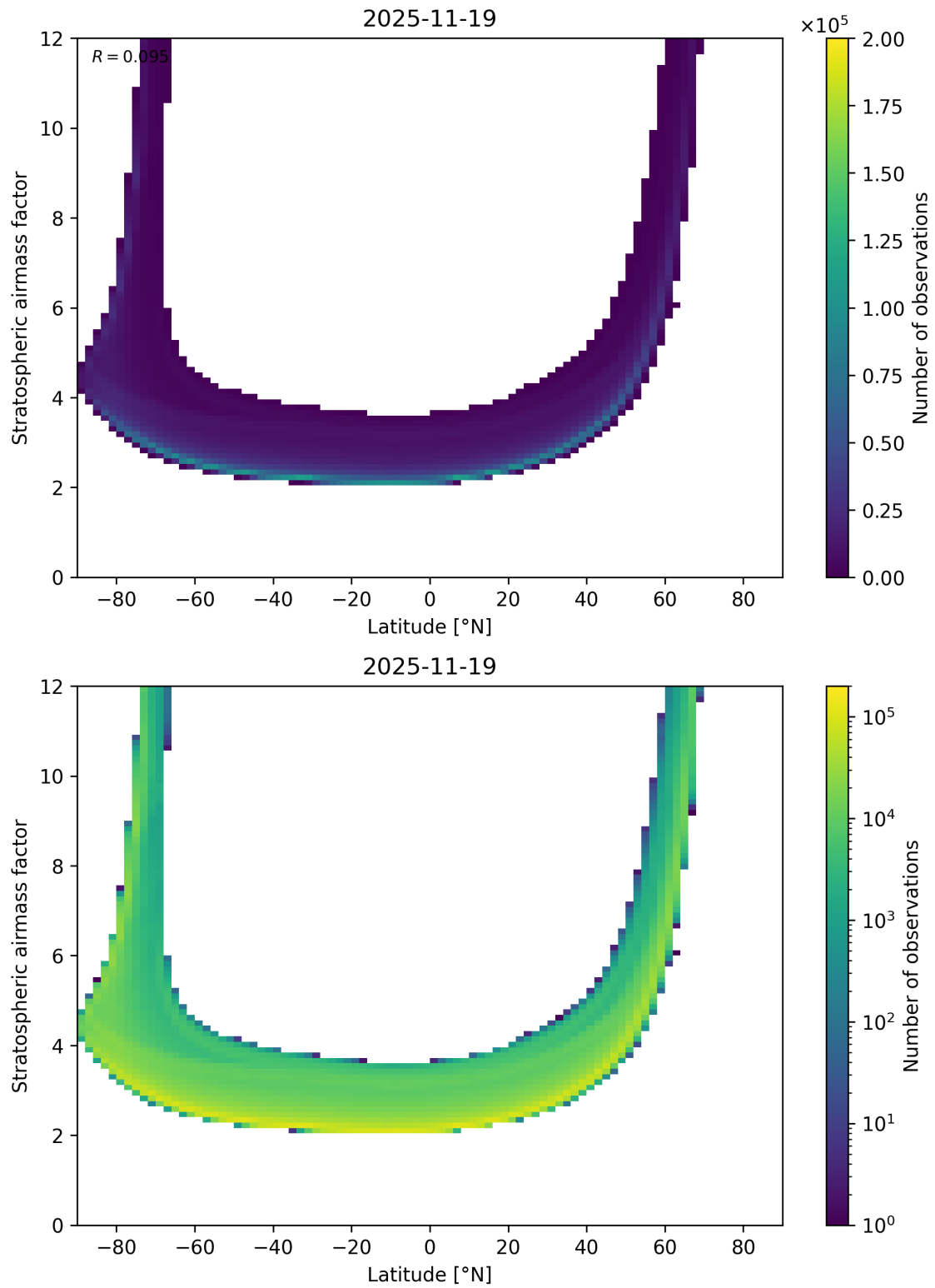
Figure 83: Scatter density plot of “Latitude” against “Stratospheric air mass factor” for 2025-11-18 to 2025-11-20.
