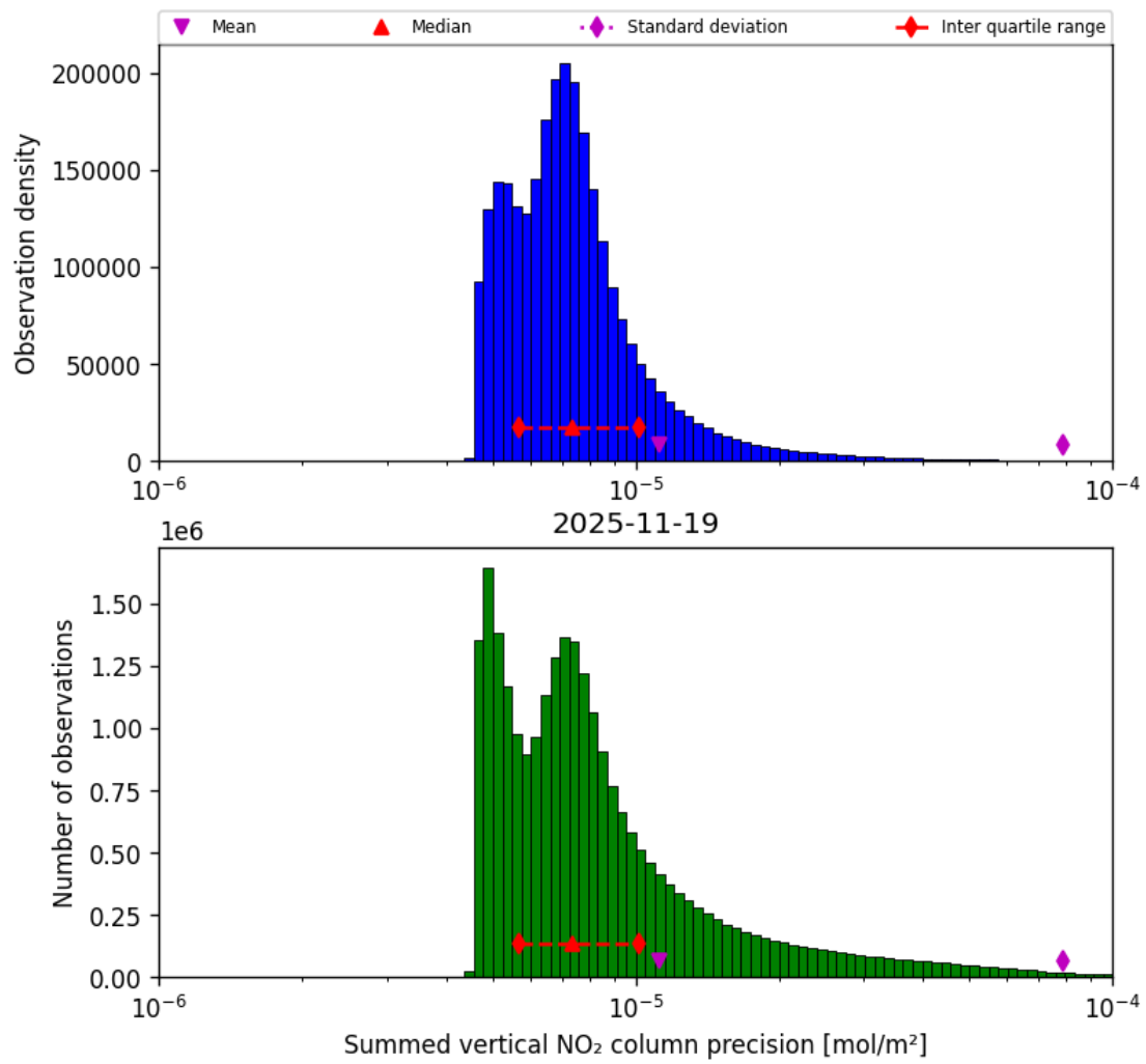
Figure 41: Histogram of "Summed vertical NO 2 column precision" for 2025-11-18 to 2025-11-20
