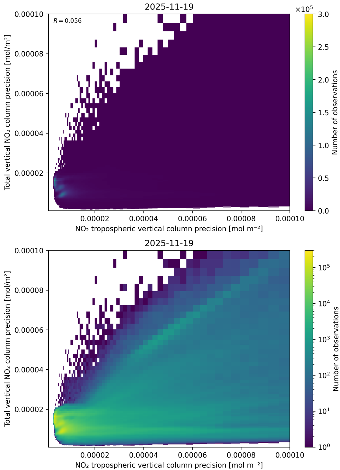
Figure 139: Scatter density plot of “NO 2 tropospheric vertical column precision” against “Total vertical NO 2 column precision” for 2025-11-18 to 2025-11-20.
