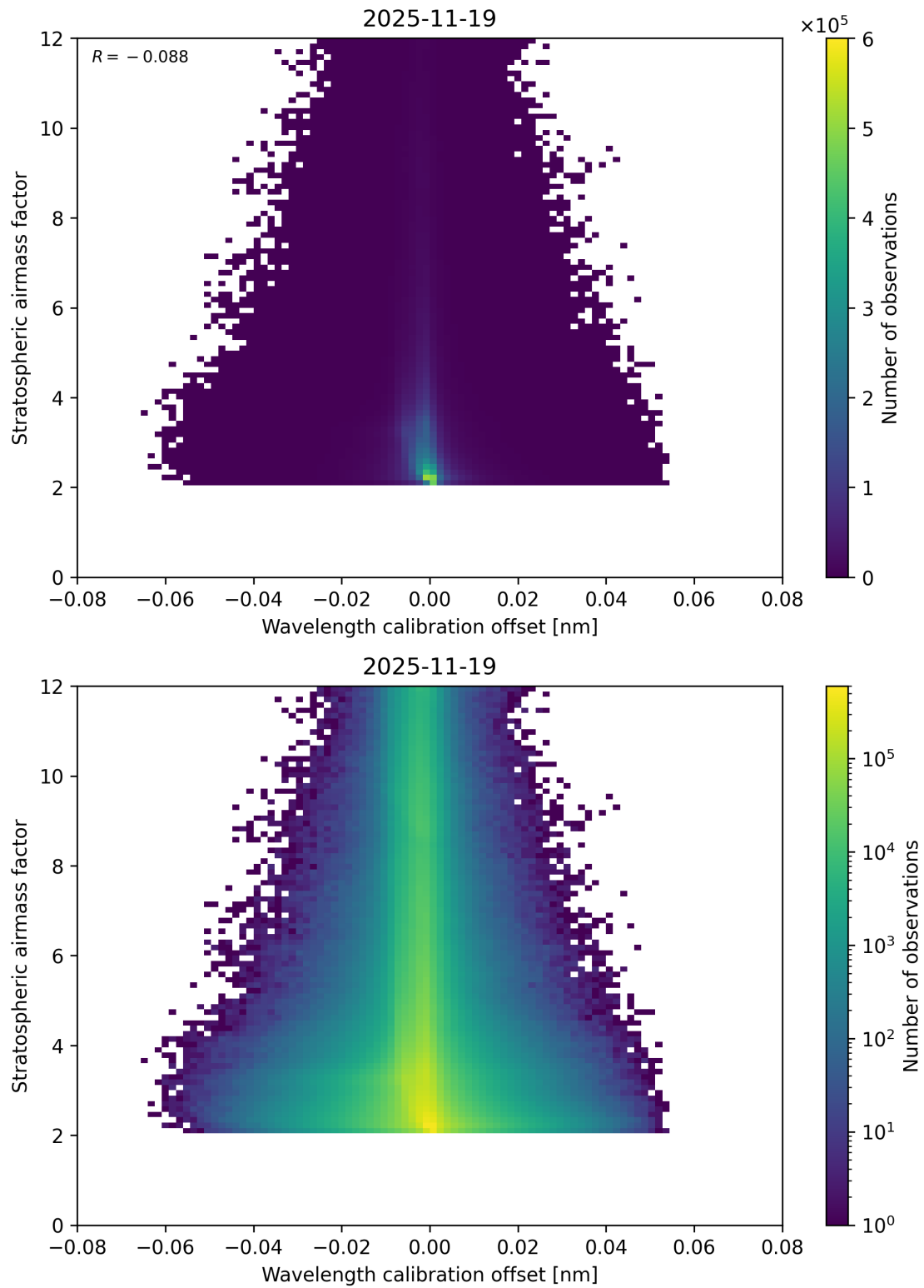
Figure 174: Scatter density plot of “Wavelength calibration offset” against “Stratospheric air mass factor” for 2025-11-18 to 2025-11-20.
