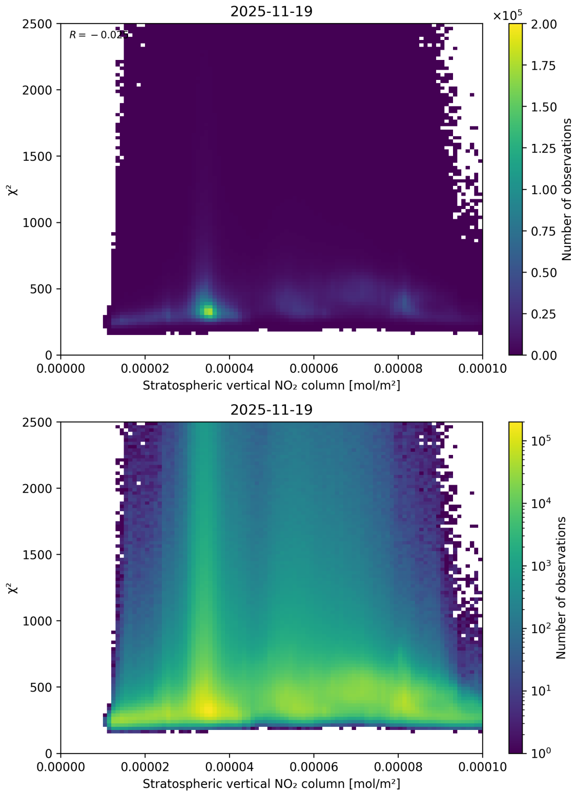
Figure 97: Scatter density plot of “Stratospheric vertical NO 2 column” against “ \chi^2 ” for 2025-11-18 to 2025-11-20.
