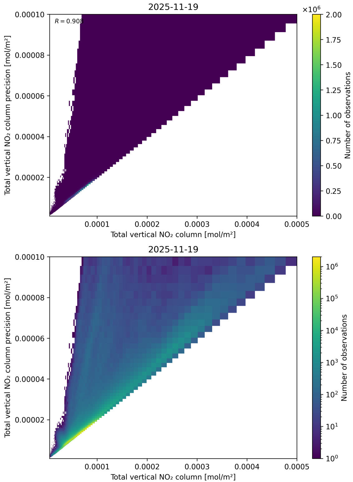
Figure 114: Scatter density plot of “Total vertical NO 2 column” against “Total vertical NO 2 column precision” for 2025-11-18 to 2025-11-20.
