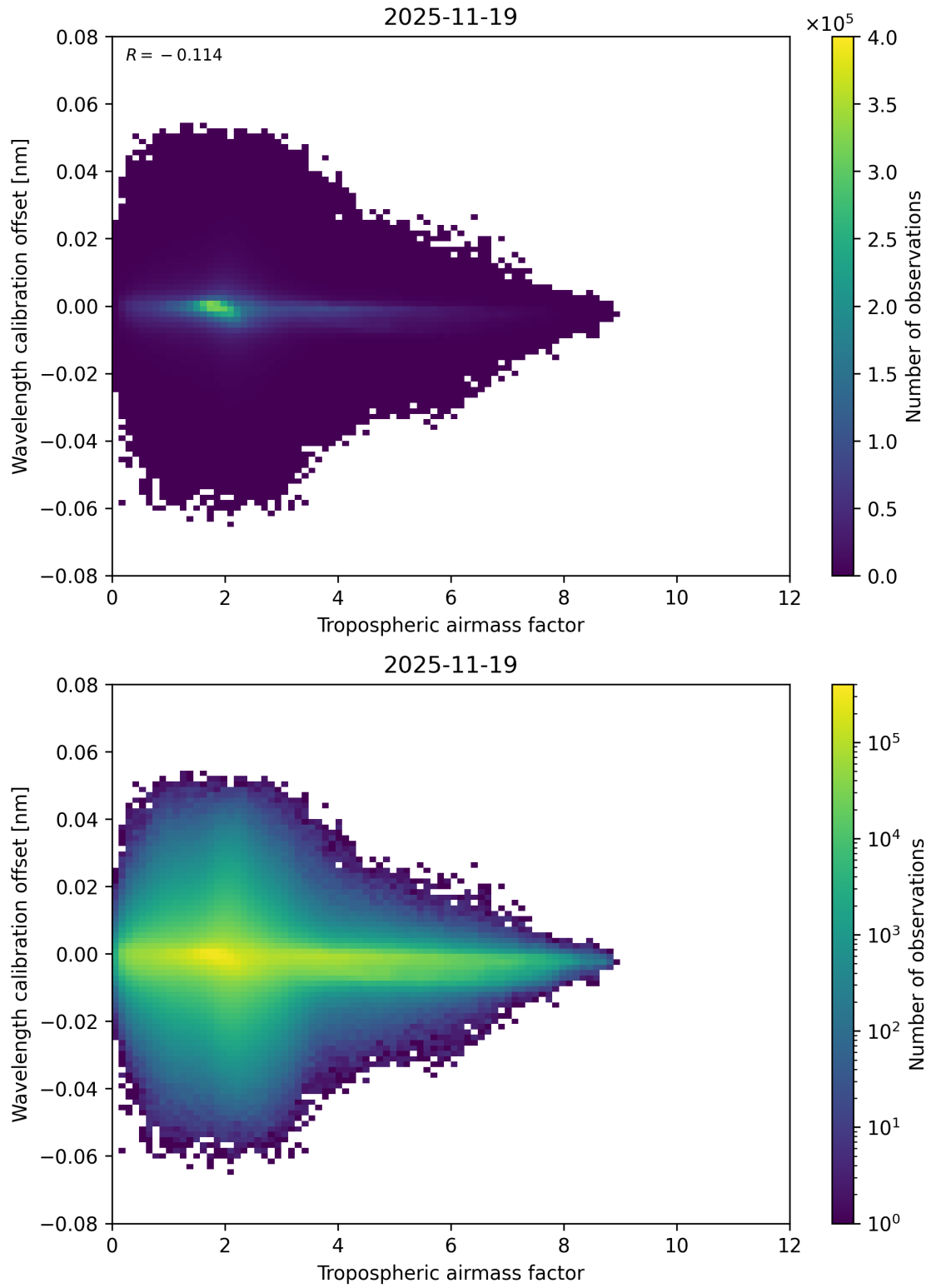
Figure 80: Scatter density plot of “Tropospheric airmass factor” against “Wavelength calibration offset” for 2025-11-18 to 2025-11-20.
