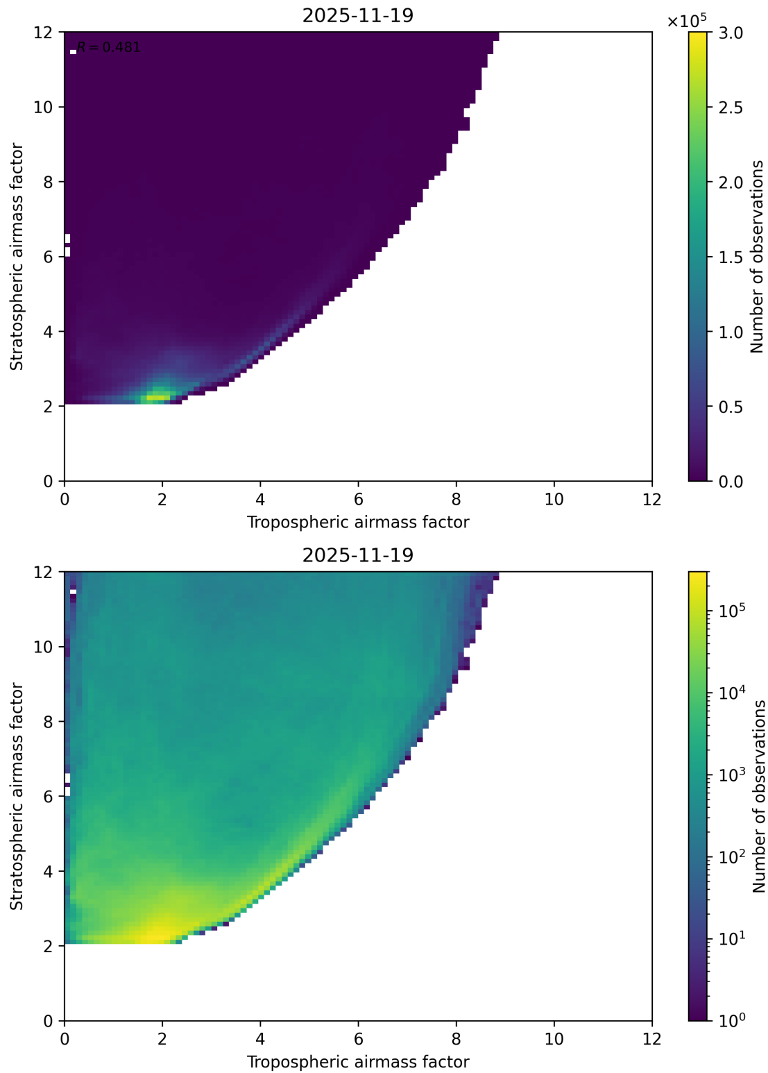
Figure 71: Scatter density plot of “Tropospheric airmass factor” against “Stratospheric airmass factor” for 2025-11-18 to 2025-11-20.
