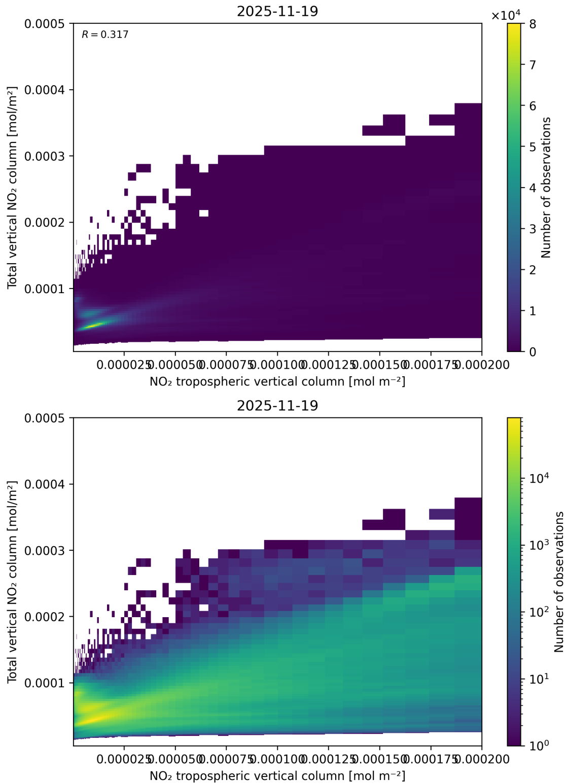
Figure 128: Scatter density plot of “NO 2 tropospheric vertical column” against “Total vertical NO 2 column” for 2025-11-18 to 2025-11-20.
