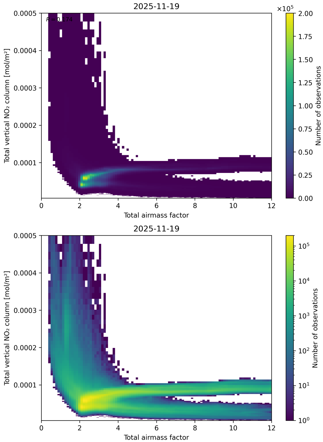
Figure 67: Scatter density plot of “Total airmass factor” against “Total vertical NO 2 column” for 2025-11-18 to 2025-11-20.
