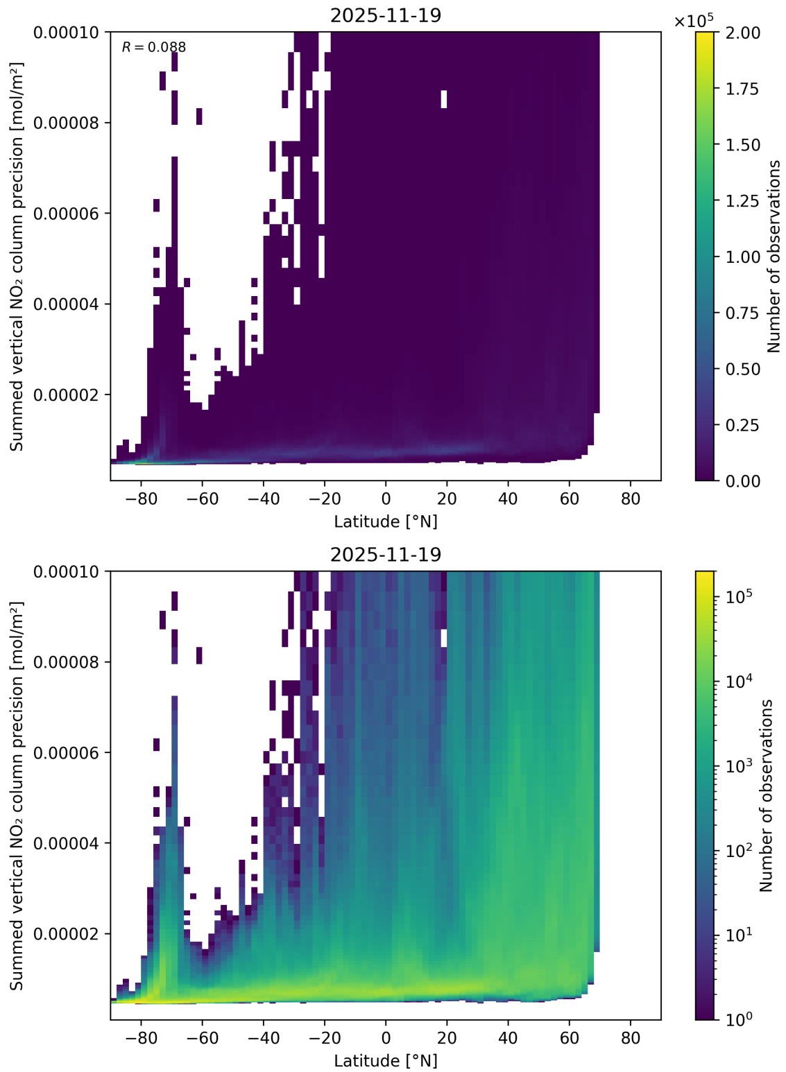
Figure 89: Scatter density plot of “Latitude” against “Summed vertical NO 2 column precision” for 2025-11-18 to 2025-11-20.
