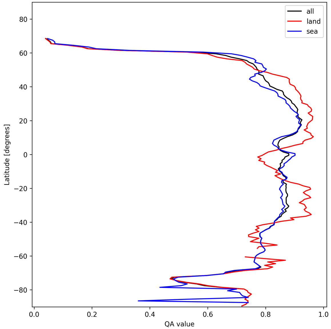
Figure 11: Zonal average of “QA value” for 2025-11-18 to 2025-11-20.
