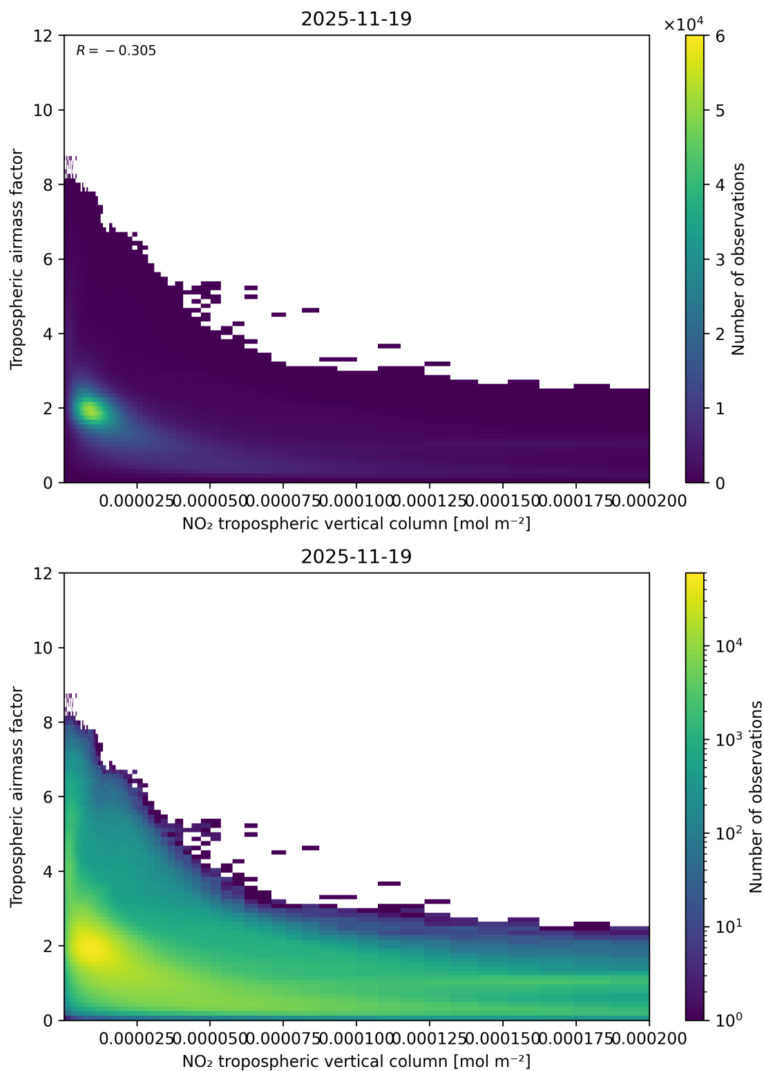
Figure 123: Scatter density plot of “NO 2 tropospheric vertical column” against “Tropospheric air mass factor” for 2025-11-18 to 2025-11-20.
