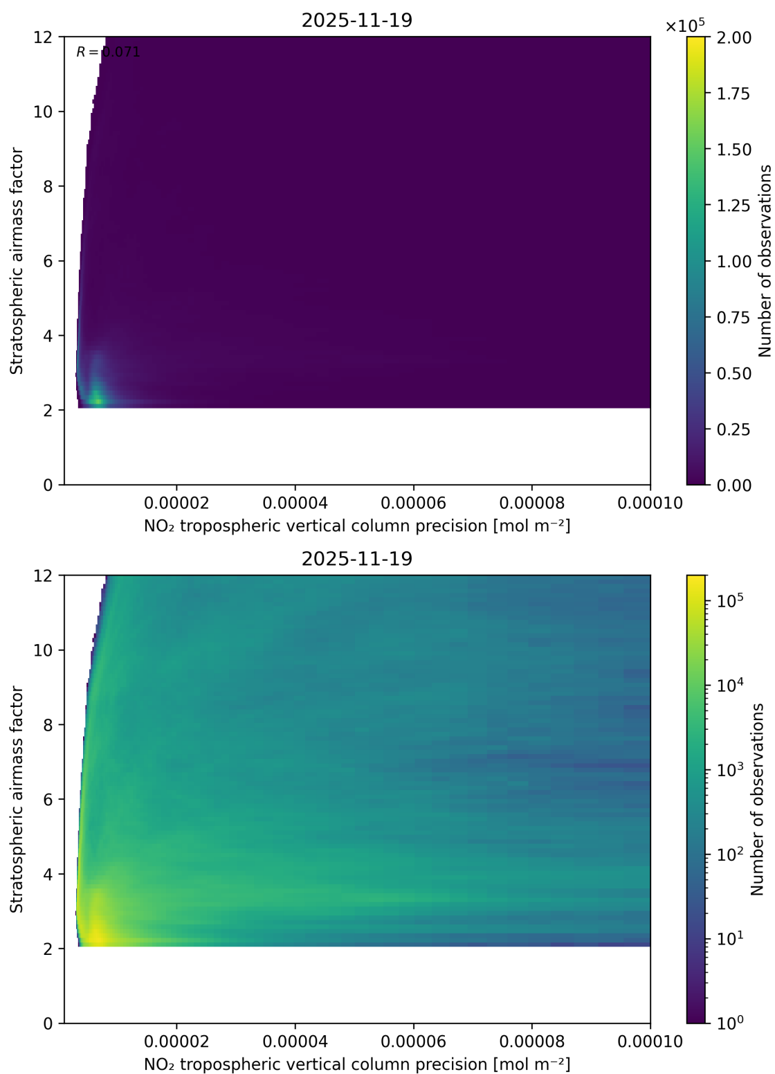
Figure 131: Scatter density plot of “NO 2 tropospheric vertical column precision” against “Stratospheric airmass factor” for 2025-11-18 to 2025-11-20.
