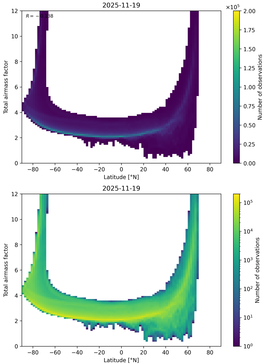
Figure 84: Scatter density plot of “Latitude” against “Total airmass factor” for 2025-11-18 to 2025-11-20.
