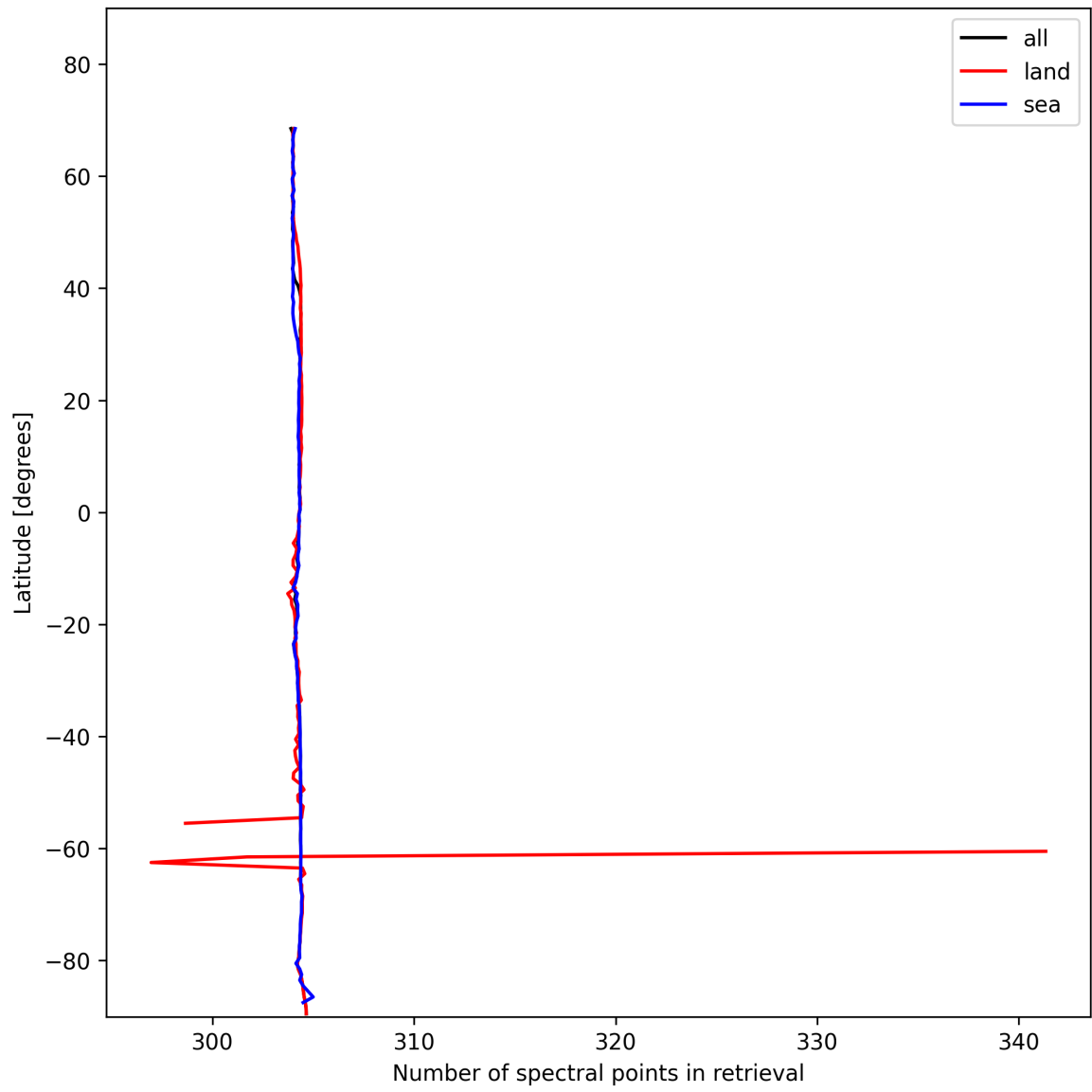
Figure 16: Zonal average of “Number of spectral points in retrieval” for 2025-11-18 to 2025-11-20.
