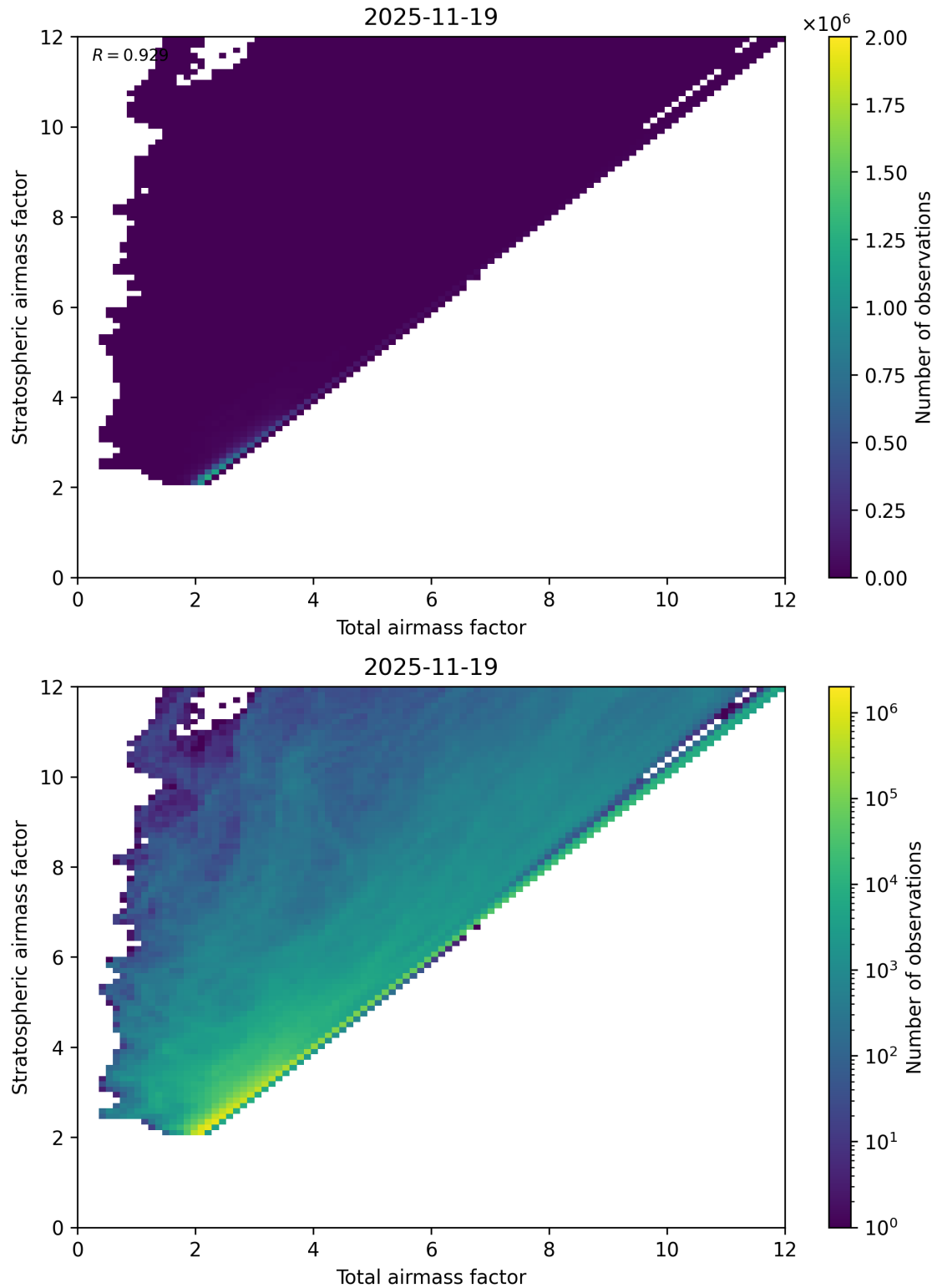
Figure 62: Scatter density plot of “Total airmass factor” against “Stratospheric airmass factor” for 2025-11-18 to 2025-11-20.
