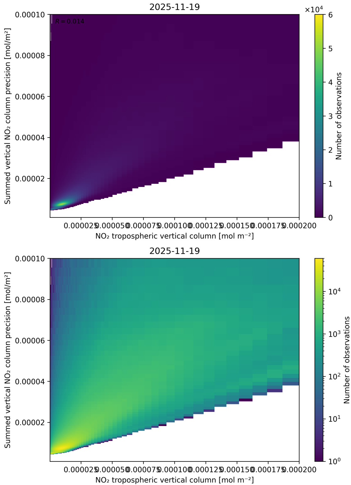
Figure 127: Scatter density plot of “NO 2 tropospheric vertical column” against “Summed vertical NO 2 column precision” for 2025-11-18 to 2025-11-20.
