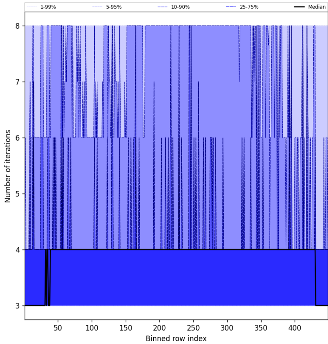
Figure 51: Along track statistics of “Number of iterations” for 2025-11-18 to 2025-11-20
