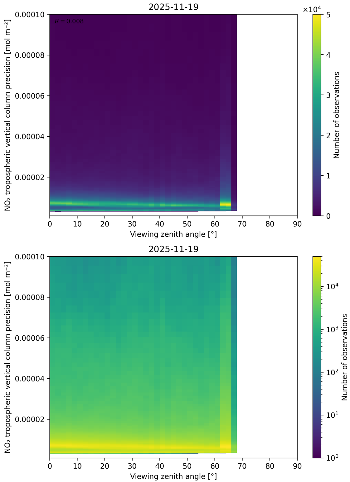
Figure 170: Scatter density plot of “Viewing zenith angle” against “NO 2 tropospheric vertical column precision” for 2025-11-18 to 2025-11-20.
