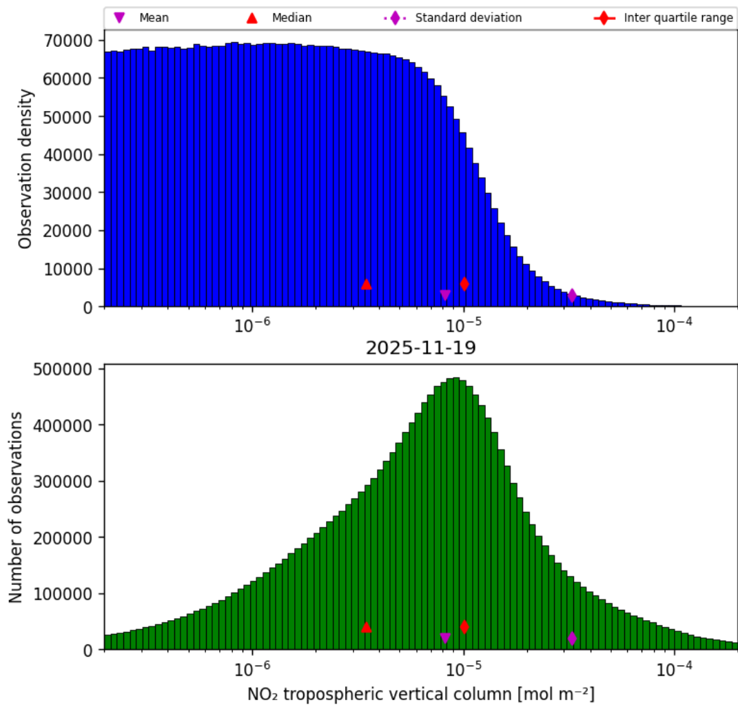
Figure 29: Histogram of “NO 2 tropospheric vertical column” for 2025-11-18 to 2025-11-20
