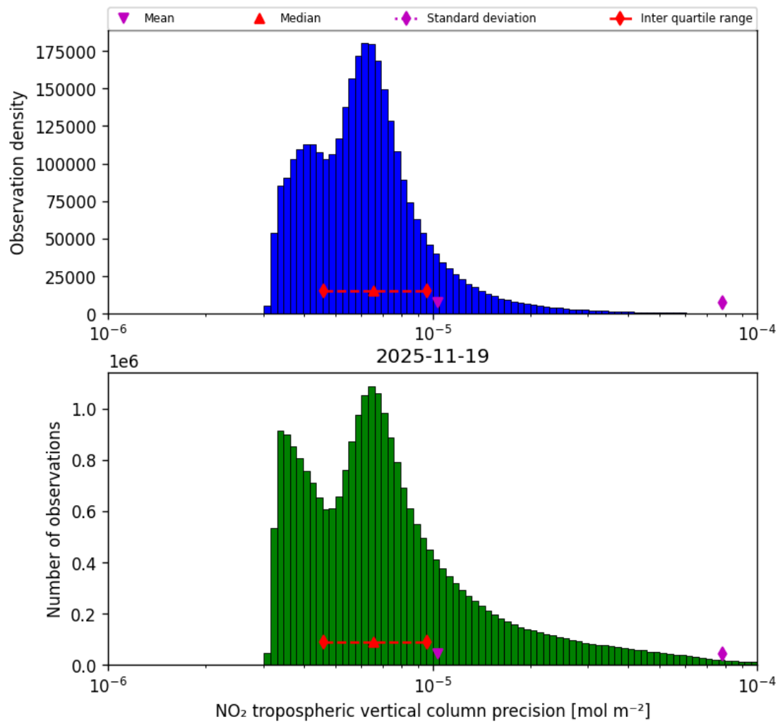
Figure 30: Histogram of “NO 2 tropospheric vertical column precision” for 2025-11-18 to 2025-11-20
