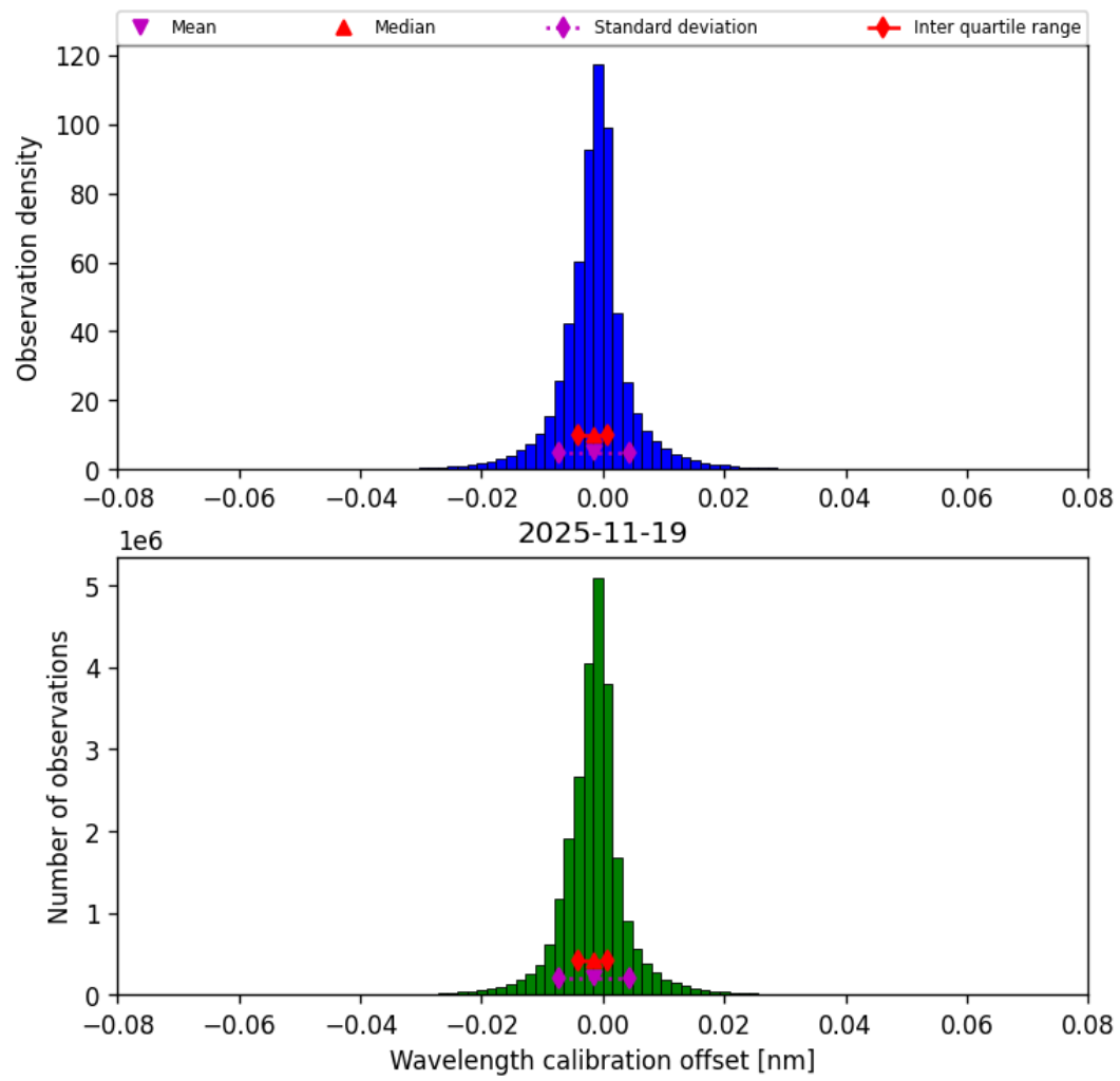
Figure 35: Histogram of “Wavelength calibration offset” for 2025-11-18 to 2025-11-20
