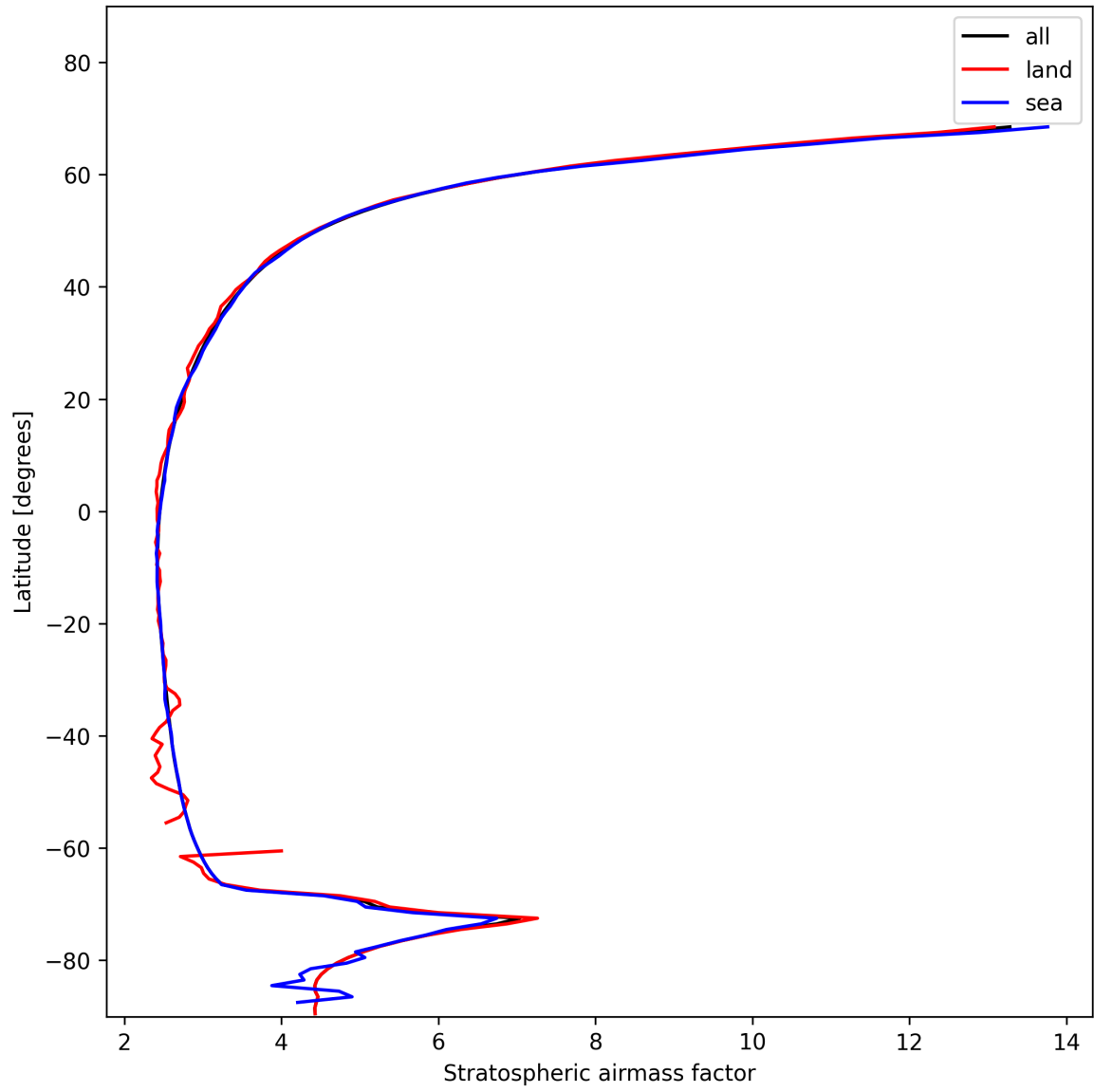
Figure 27: Zonal average of “Stratospheric airmass factor” for 2025-11-18 to 2025-11-20.
