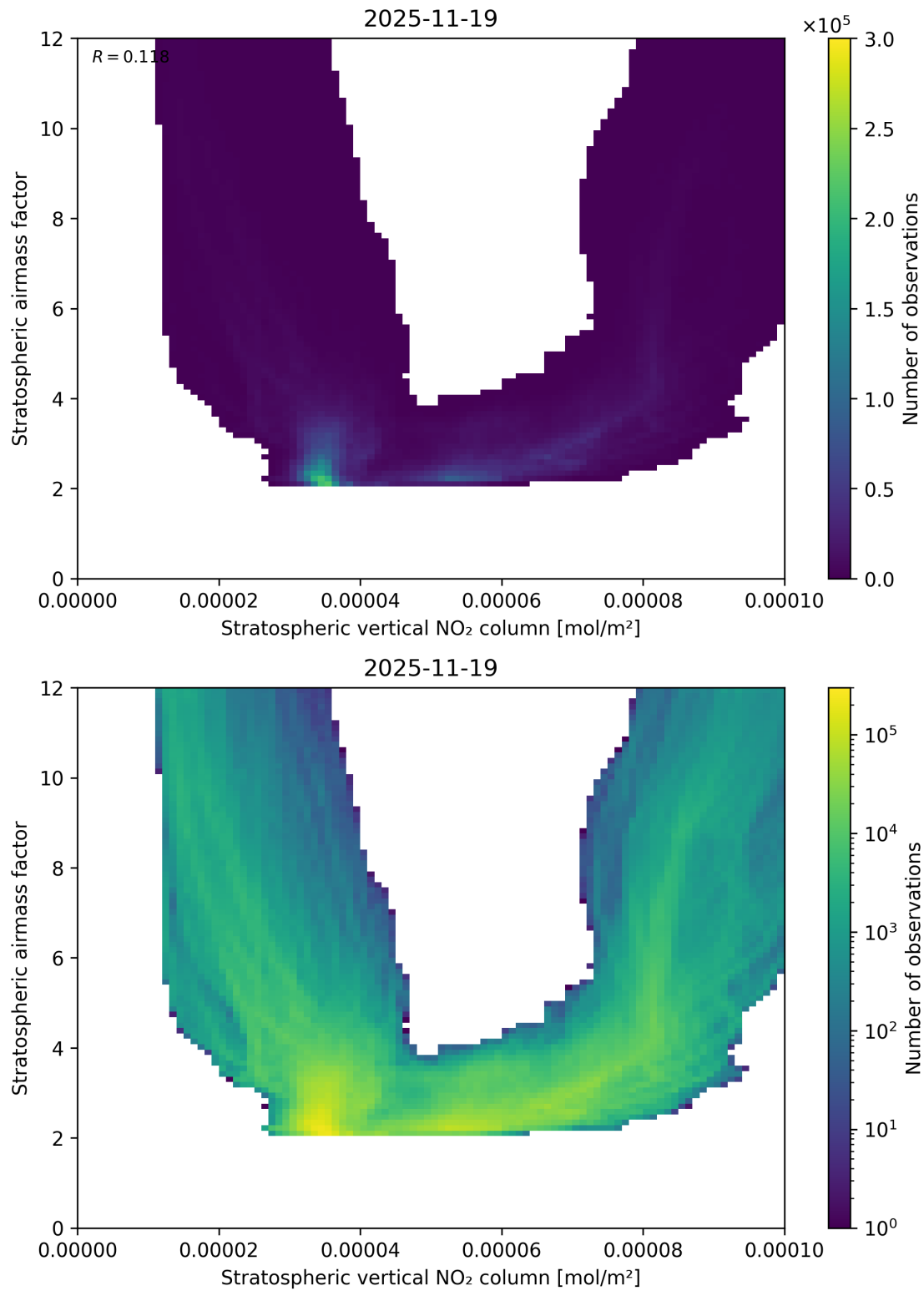
Figure 96: Scatter density plot of “Stratospheric vertical NO 2 column” against “Stratospheric airmass factor” for 2025-11-18 to 2025-11-20.
