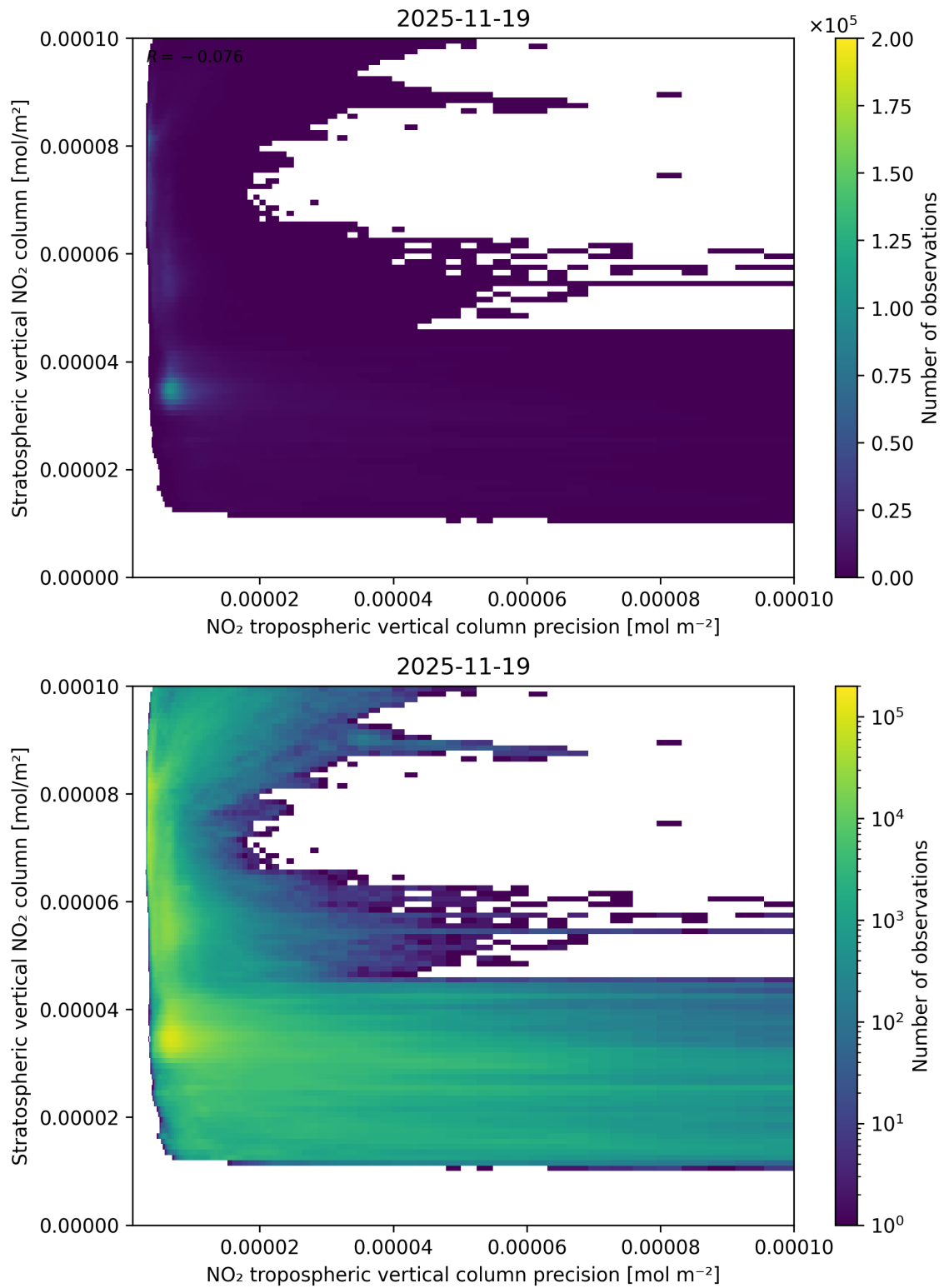
Figure 135: Scatter density plot of “NO 2 tropospheric vertical column precision” against “Stratospheric vertical NO 2 column” for 2025-11-18 to 2025-11-20.
