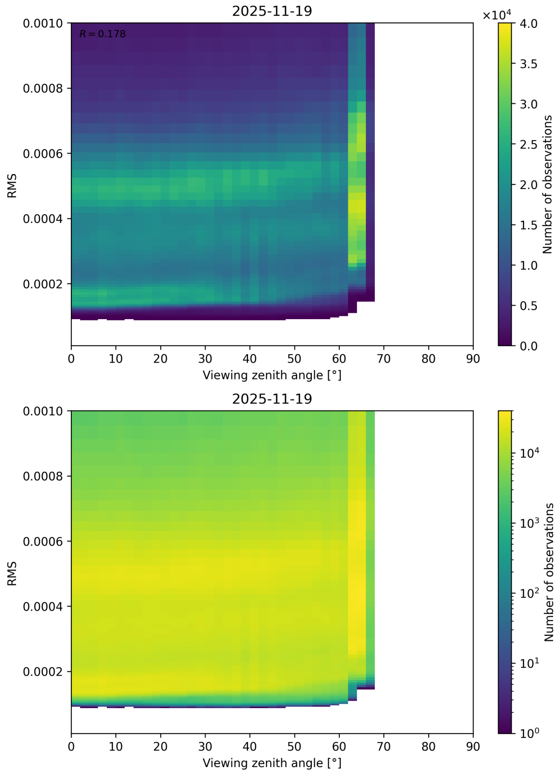
Figure 171: Scatter density plot of “Viewing zenith angle” against “RMS” for 2025-11-18 to 2025-11-20.
