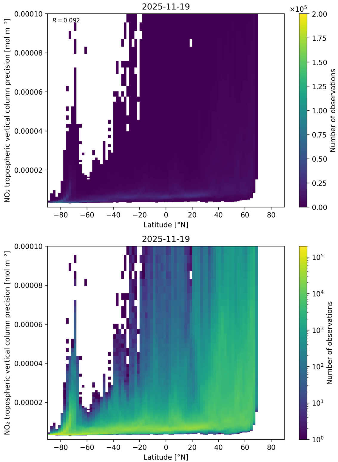
Figure 93: Scatter density plot of “Latitude” against “NO 2 tropospheric vertical column precision” for 2025-11-18 to 2025-11-20.
