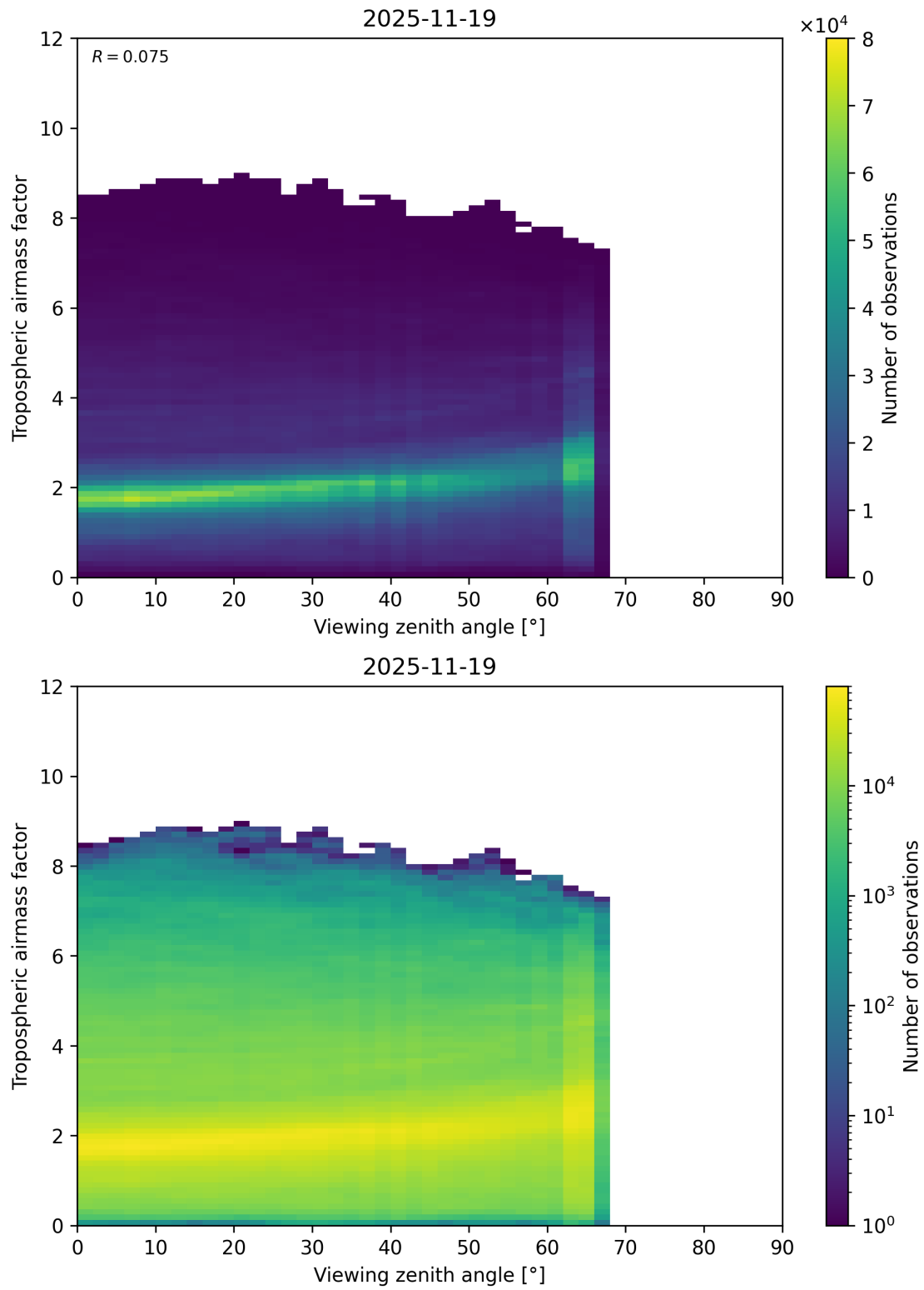
Figure 161: Scatter density plot of “Viewing zenith angle” against “Tropospheric airmass factor” for 2025-11-18 to 2025-11-20.
