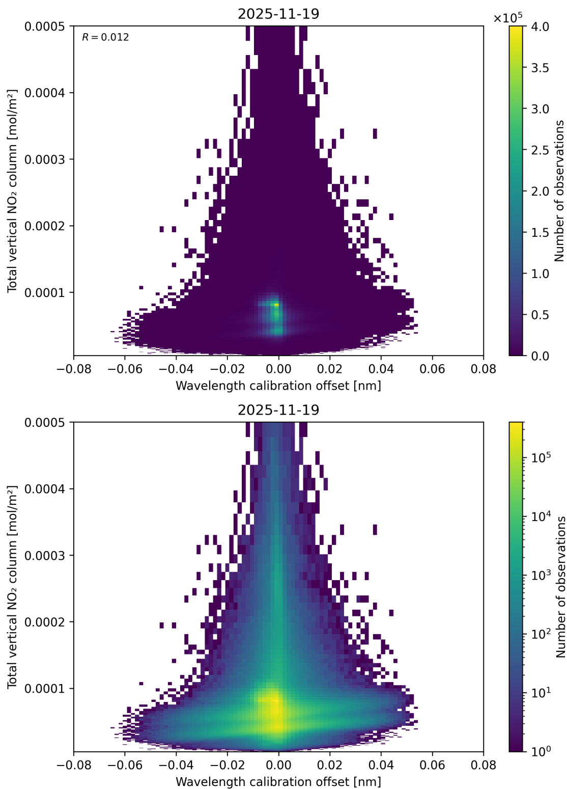
Figure 179: Scatter density plot of “Wavelength calibration offset” against “Total vertical NO 2 column” for 2025-11-18 to 2025-11-20.
