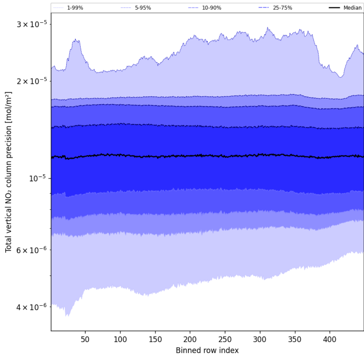
Figure 56: Along track statistics of “Total vertical NO 2 column precision” for 2025-11-18 to 2025-11-20
