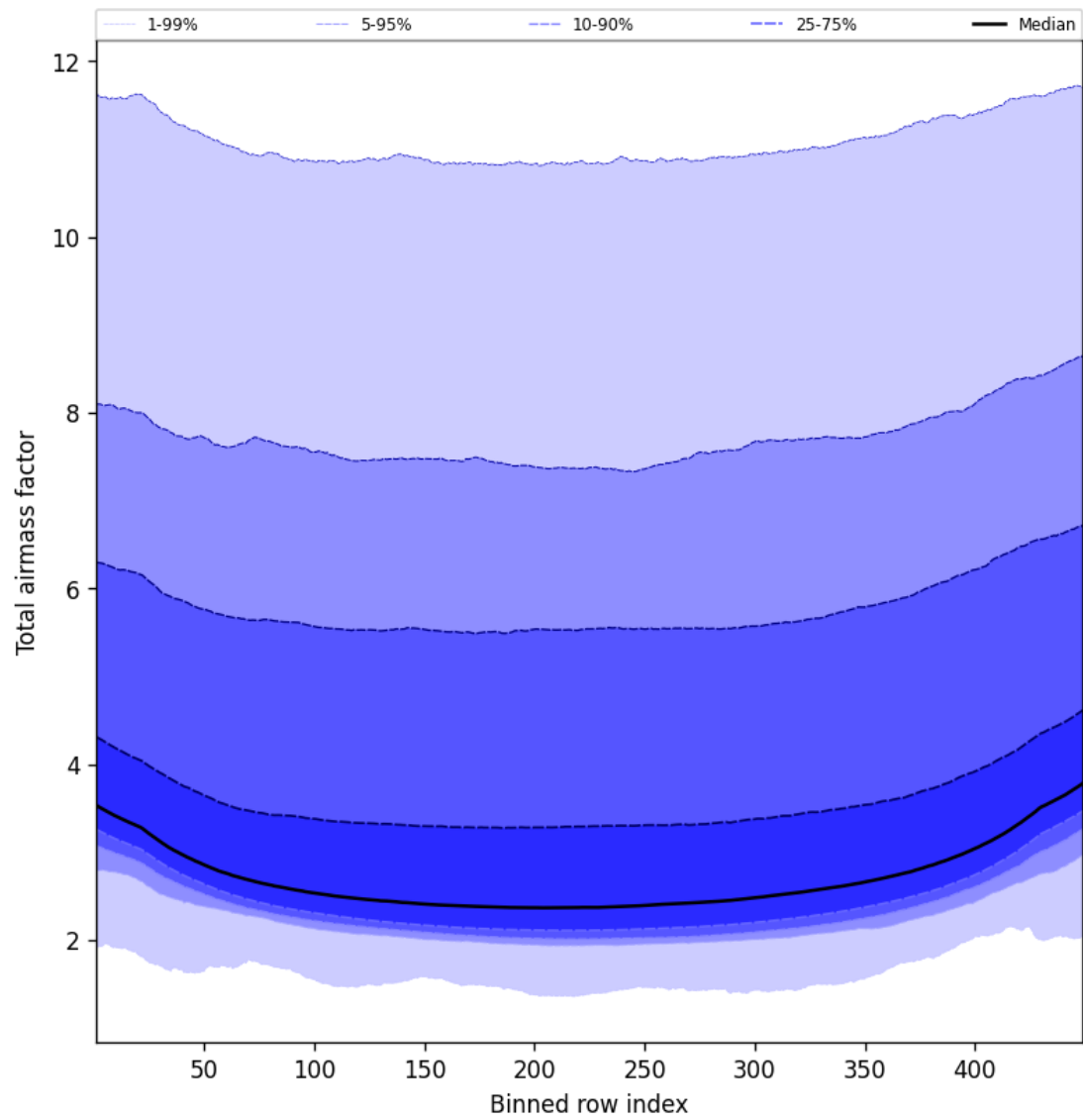
Figure 49: Along track statistics of “Total airmass factor” for 2025-11-18 to 2025-11-20
