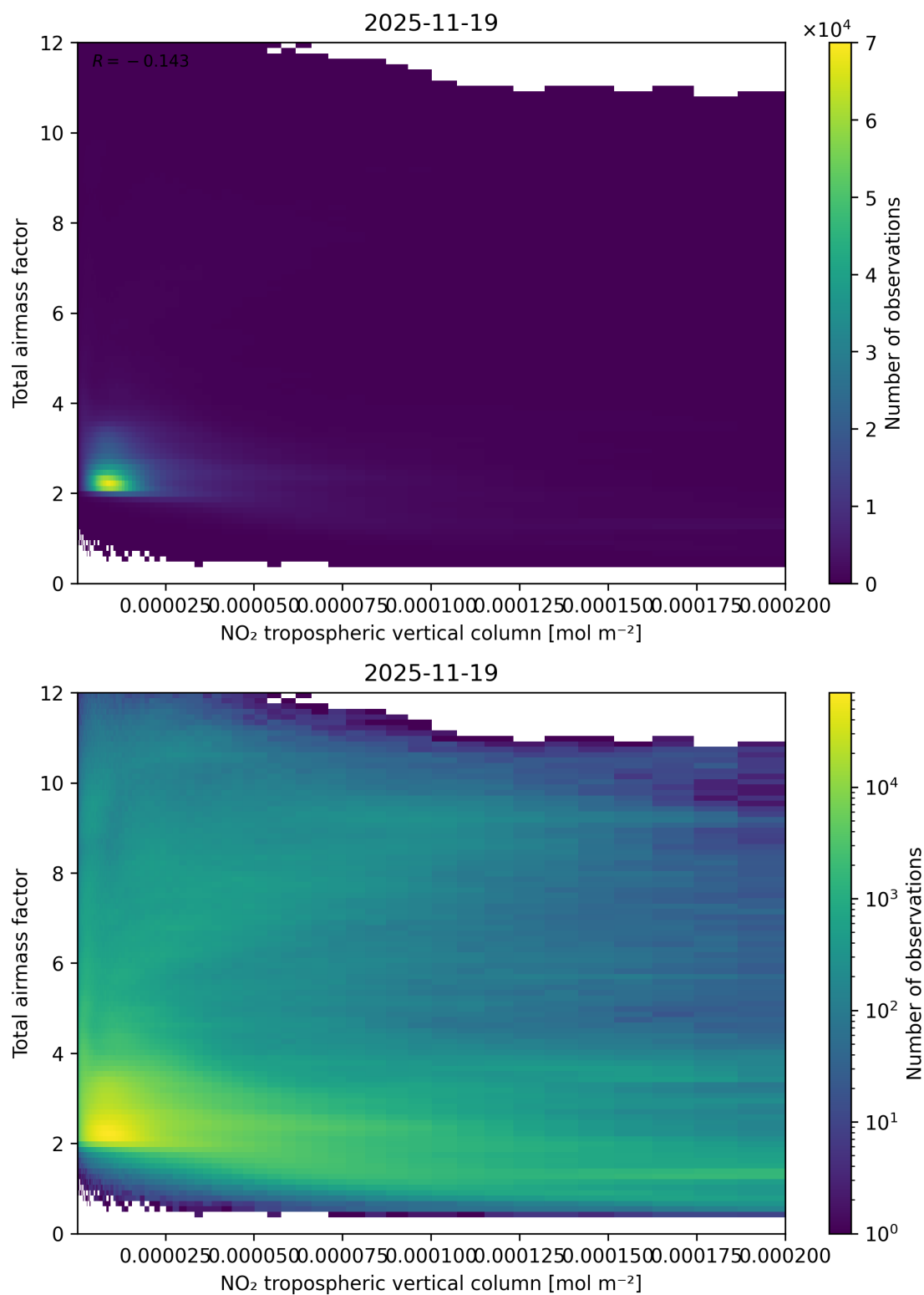
Figure 122: Scatter density plot of “NO 2 tropospheric vertical column” against “Total air mass factor” for 2025-11-18 to 2025-11-20.
