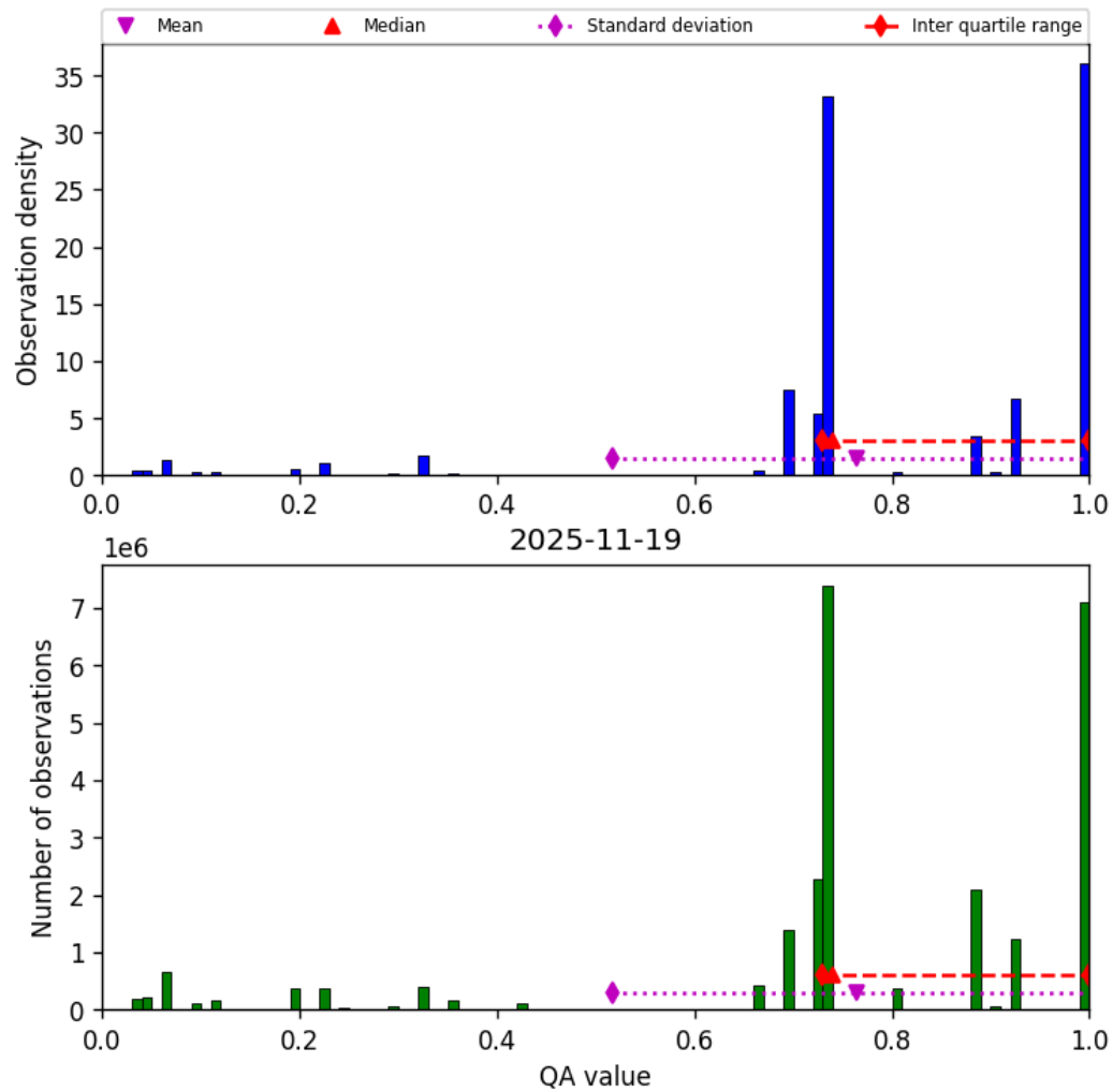
Figure 28: Histogram of “QA value” for 2025-11-18 to 2025-11-20
