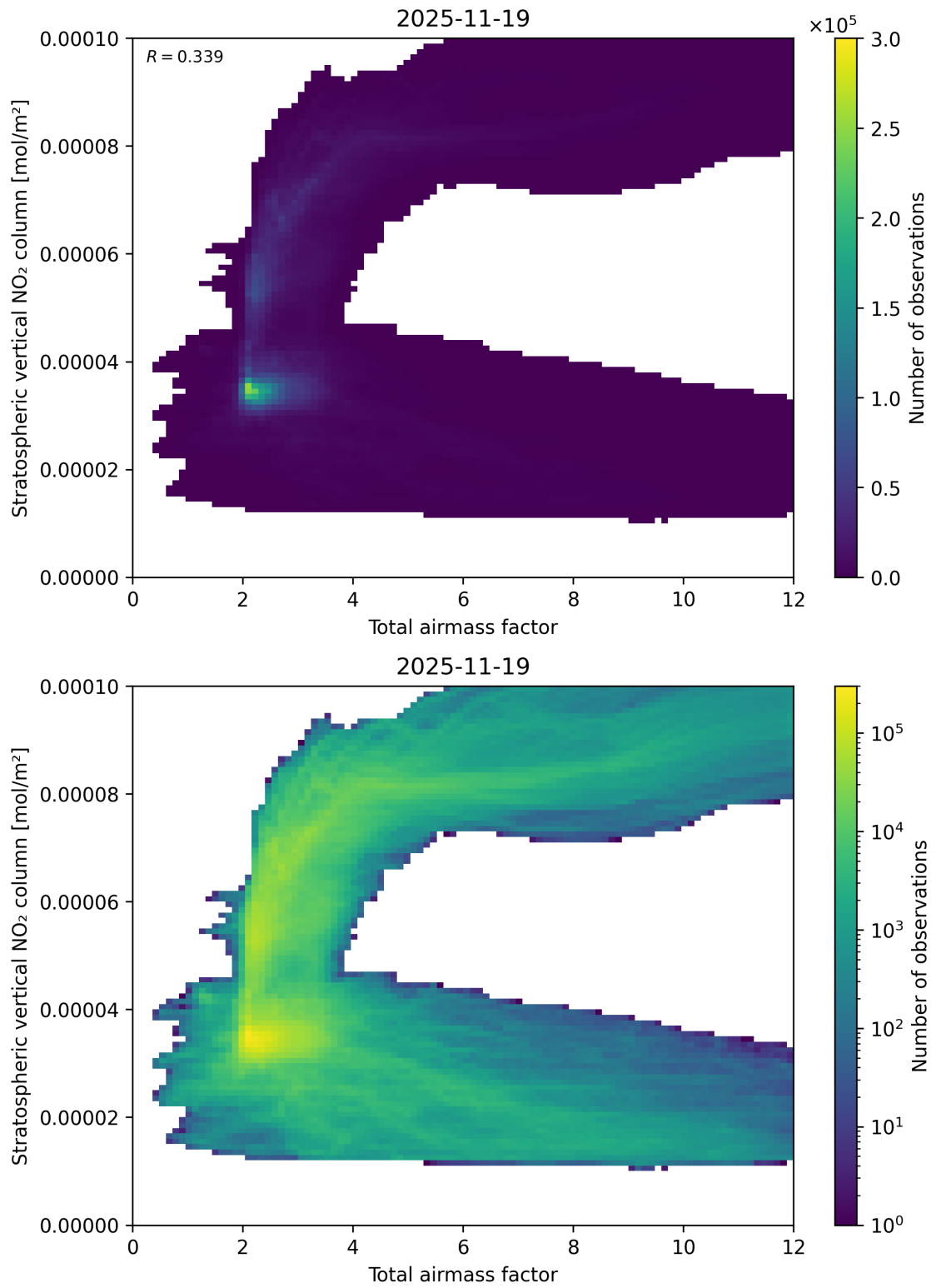
Figure 64: Scatter density plot of “Total airmass factor” against “Stratospheric vertical \text{NO}_2 column” for 2025-11-18 to 2025-11-20.
