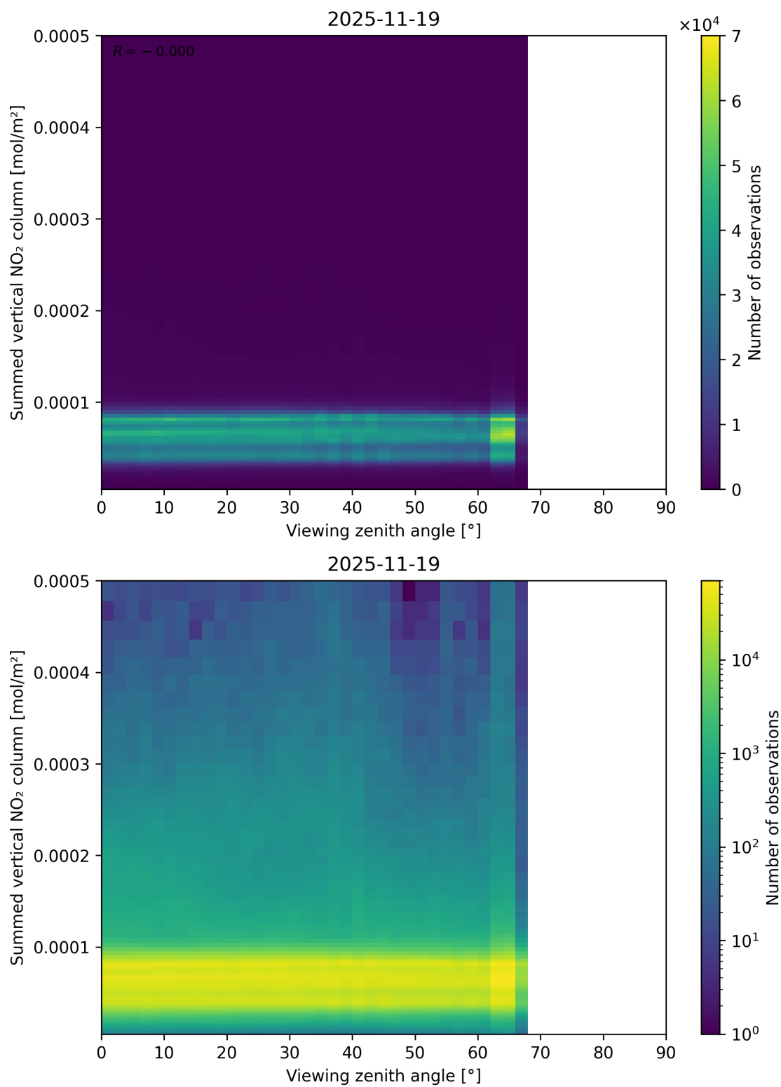
Figure 165: Scatter density plot of “Viewing zenith angle” against “Summed vertical NO 2 column” for 2025-11-18 to 2025-11-20.
