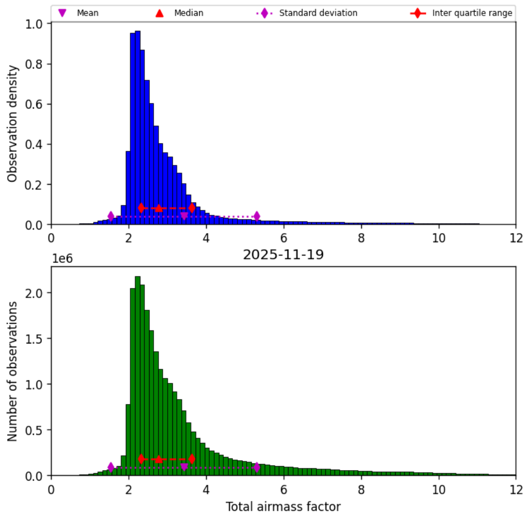
Figure 32: Histogram of “Total airmass factor” for 2025-11-18 to 2025-11-20
