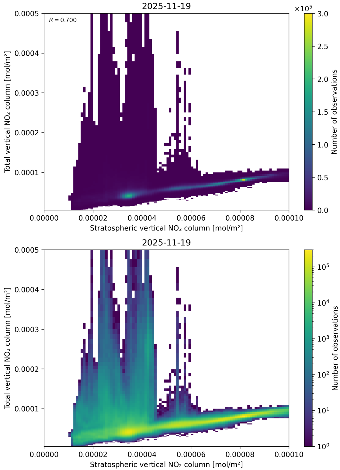
Figure 100: Scatter density plot of “Stratospheric vertical NO 2 column” against “Total vertical NO 2 column” for 2025-11-18 to 2025-11-20.
