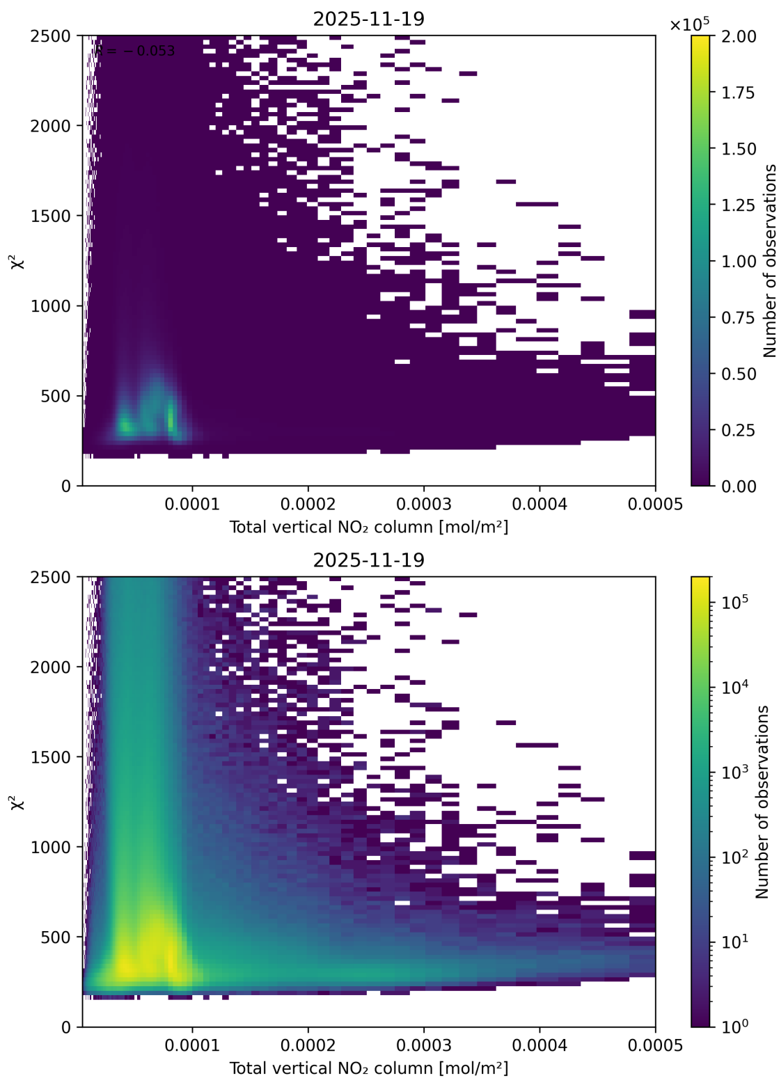
Figure 111: Scatter density plot of “Total vertical NO 2 column” against “ \chi^2 ” for 2025-11-18 to 2025-11-20.
