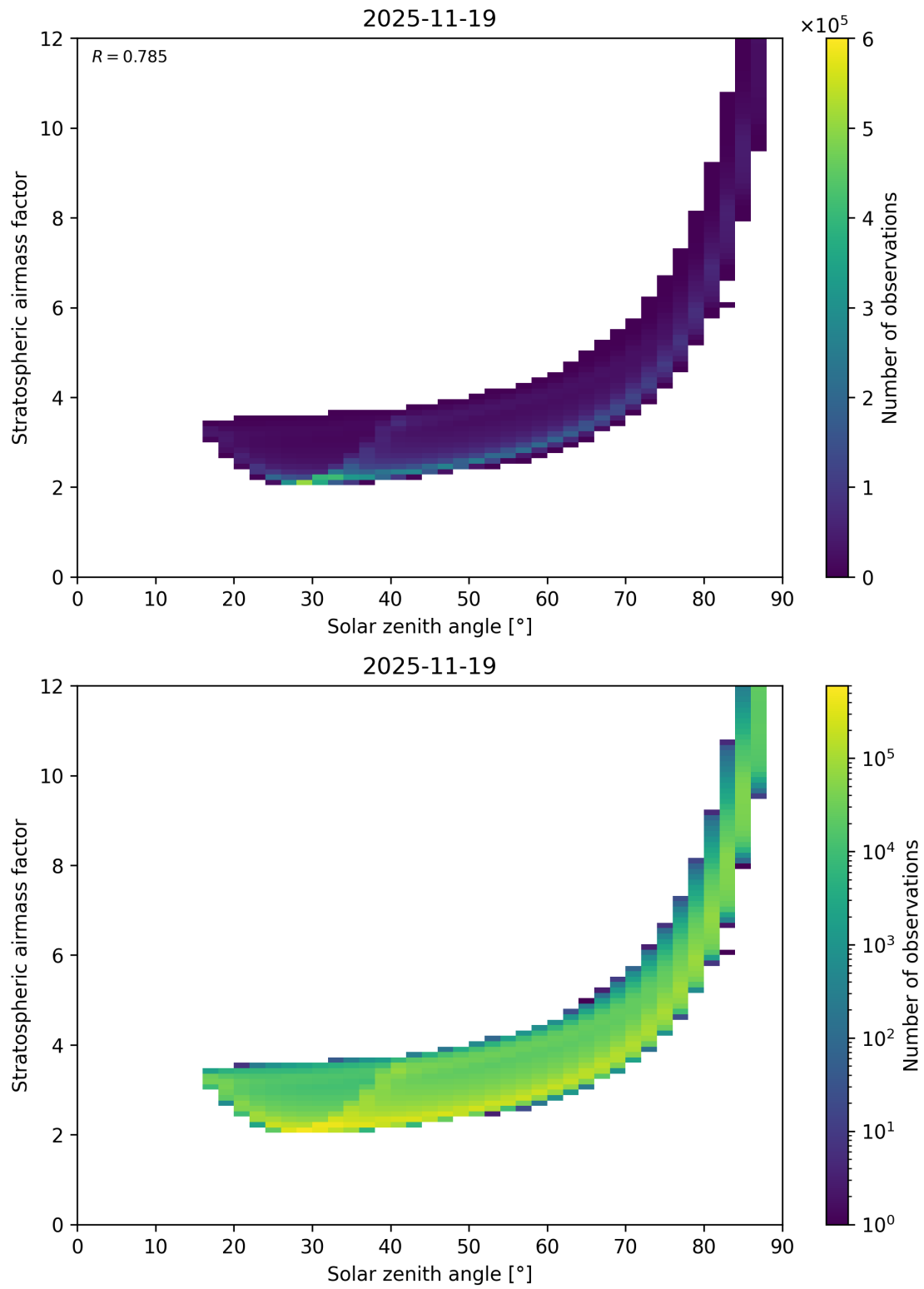
Figure 145: Scatter density plot of “Solar zenith angle” against “Stratospheric airmass factor” for 2025-11-18 to 2025-11-20.
