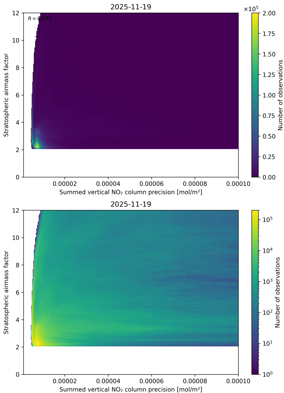
Figure 106: Scatter density plot of “Summed vertical NO 2 column precision” against “Stratospheric airmass factor” for 2025-11-18 to 2025-11-20.
