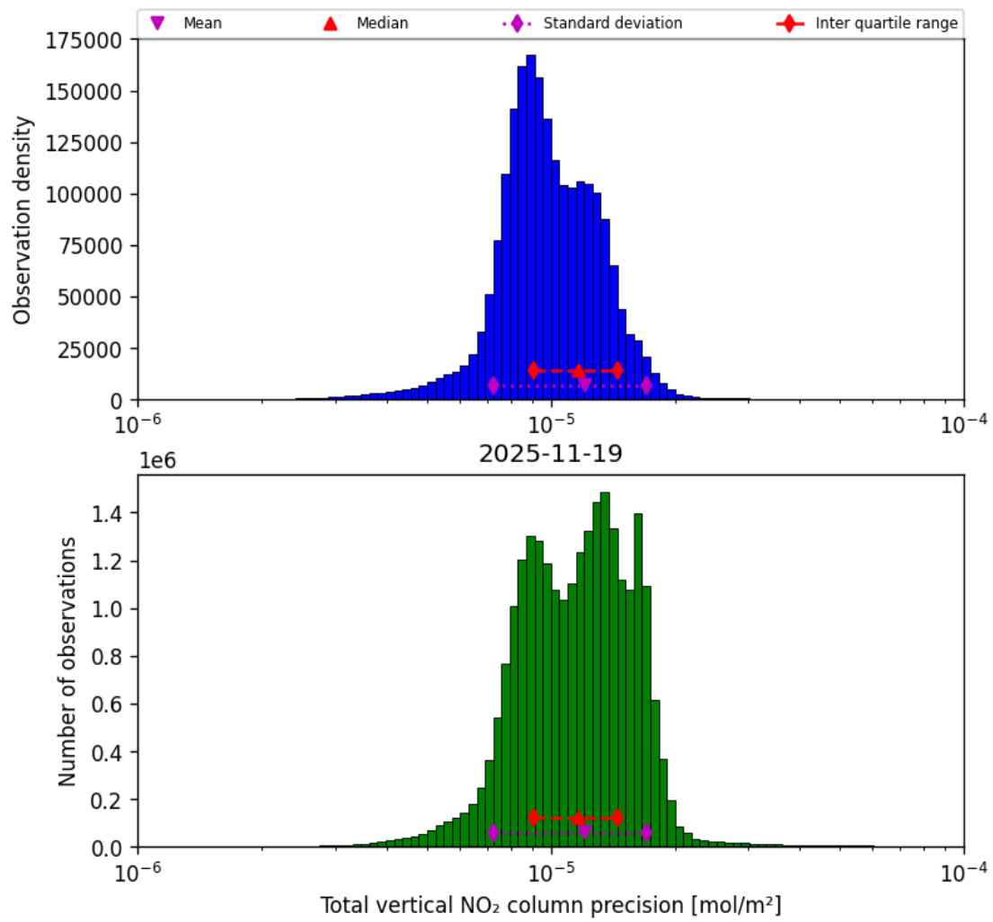
Figure 39: Histogram of “Total vertical NO 2 column precision” for 2025-11-18 to 2025-11-20
