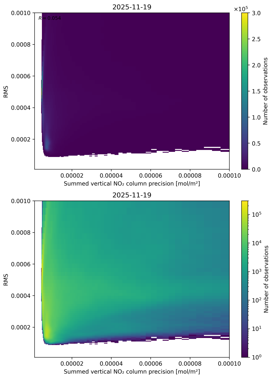
Figure 108: Scatter density plot of “Summed vertical NO 2 column precision” against “RMS” for 2025-11-18 to 2025-11-20.
