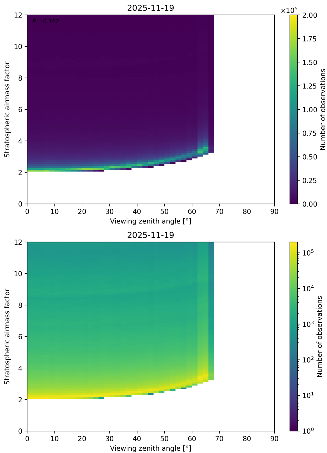
Figure 159: Scatter density plot of “Viewing zenith angle” against “Stratospheric airmass factor” for 2025-11-18 to 2025-11-20.
