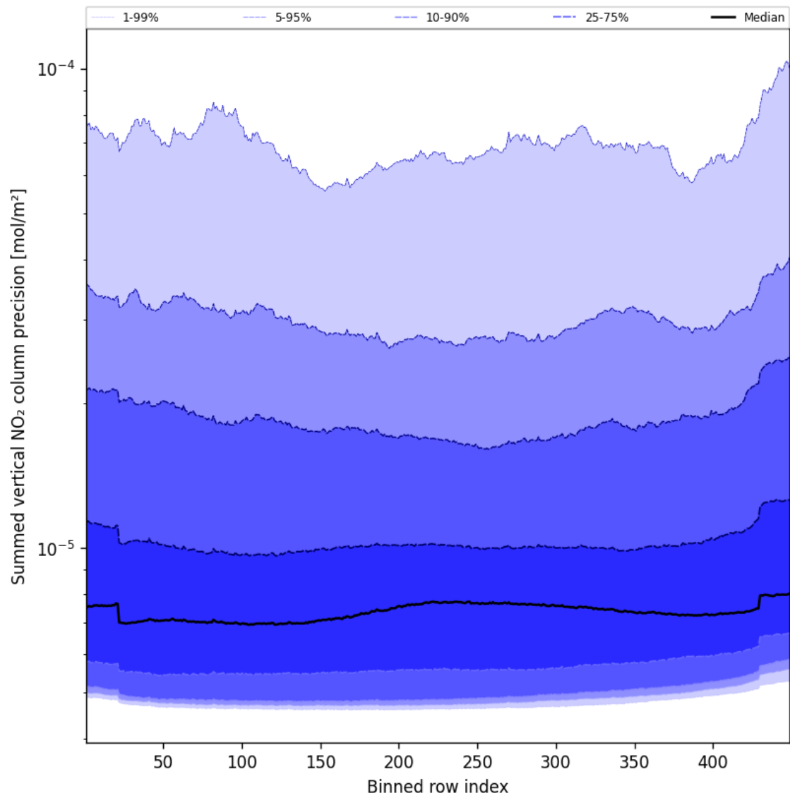
Figure 58: Along track statistics of “Summed vertical NO 2 column precision” for 2025-11-18 to 2025-11-20
