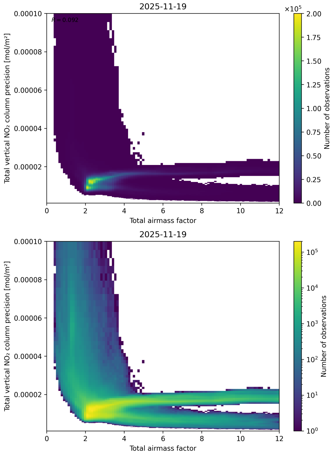
Figure 68: Scatter density plot of “Total airmass factor” against “Total vertical NO 2 column precision” for 2025-11-18 to 2025-11-20.
