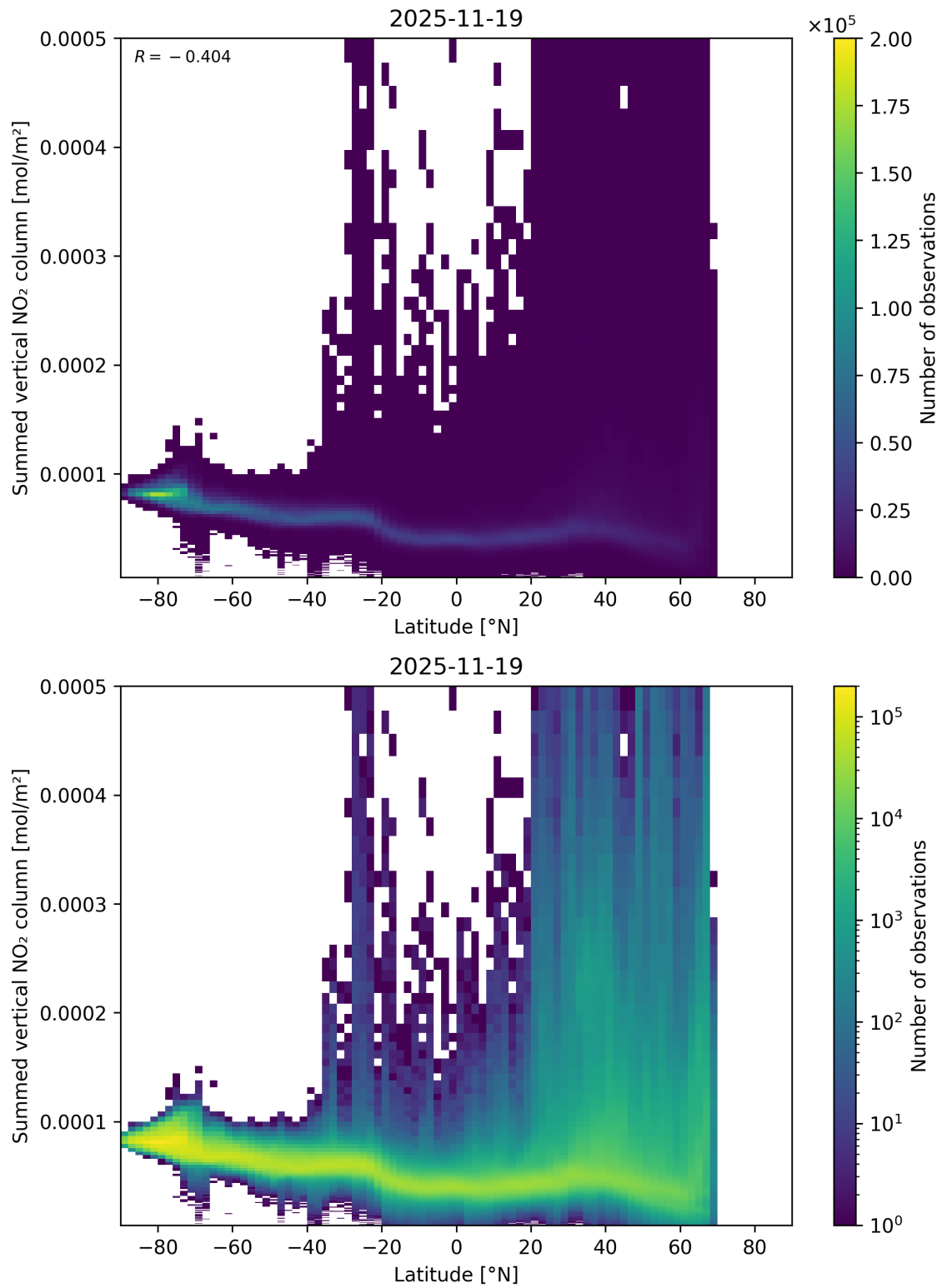
Figure 88: Scatter density plot of “Latitude” against “Summed vertical NO 2 column” for 2025-11-18 to 2025-11-20.
