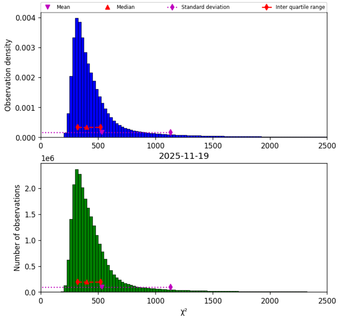
Figure 42: Histogram of “ \chi^2 ” for 2025-11-18 to 2025-11-20
