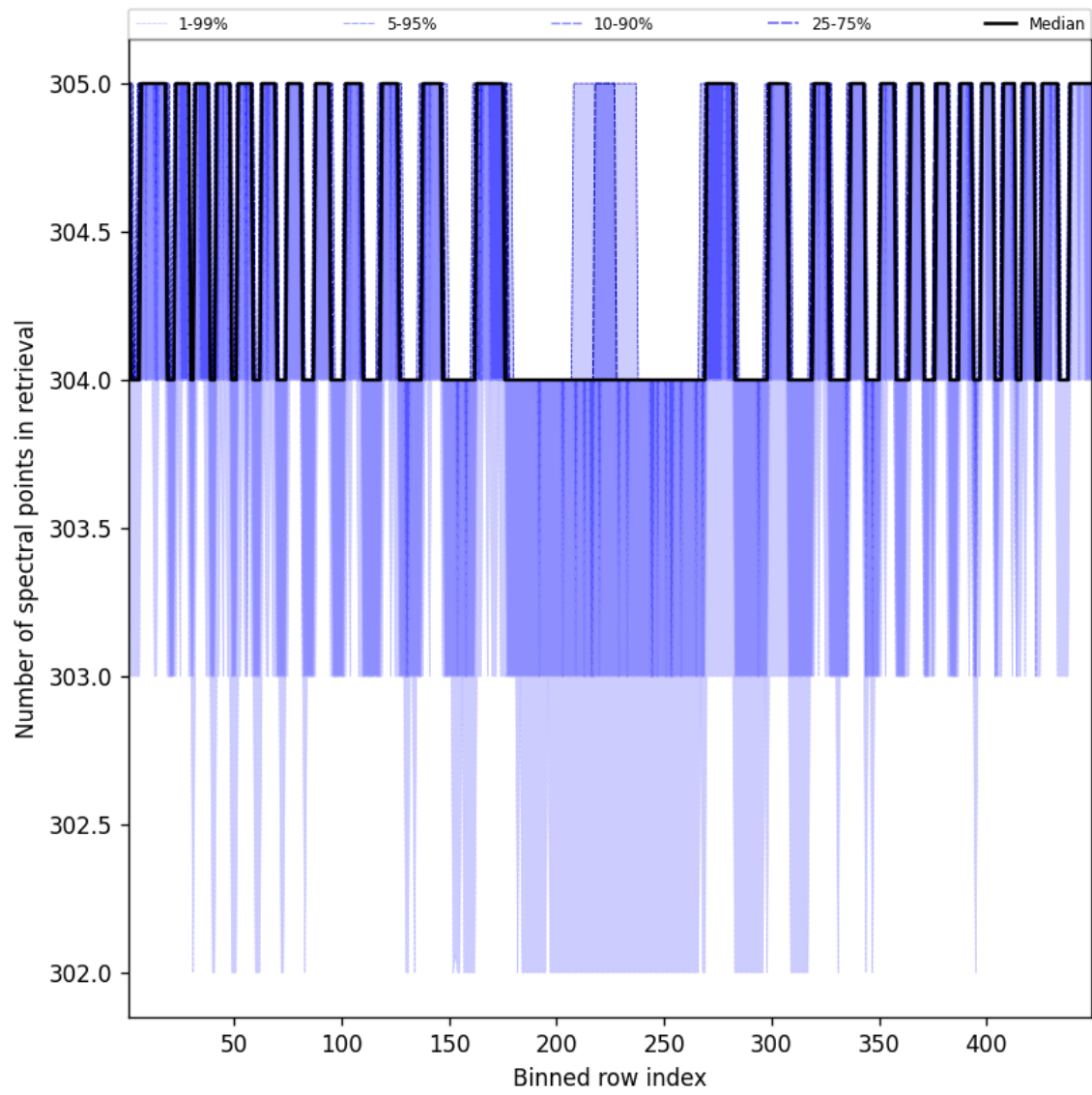
Figure 50: Along track statistics of “Number of spectral points in retrieval” for 2025-11-18 to 2025-11-20
