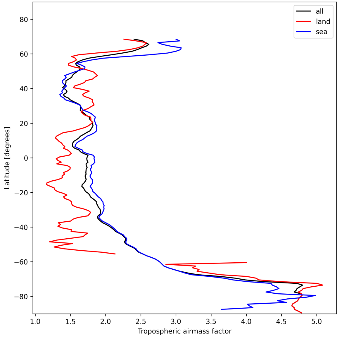
Figure 14: Zonal average of “Tropospheric airmass factor” for 2025-11-18 to 2025-11-20.
