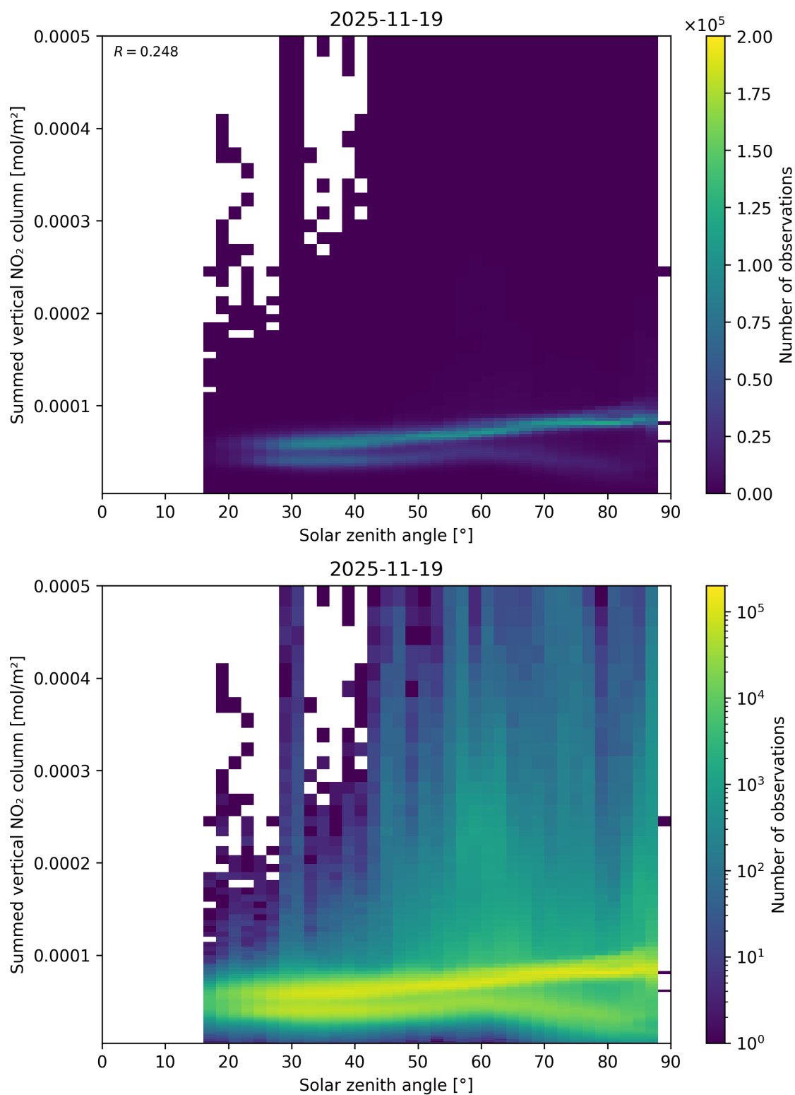
Figure 151: Scatter density plot of “Solar zenith angle” against “Summed vertical NO 2 column” for 2025-11-18 to 2025-11-20.
