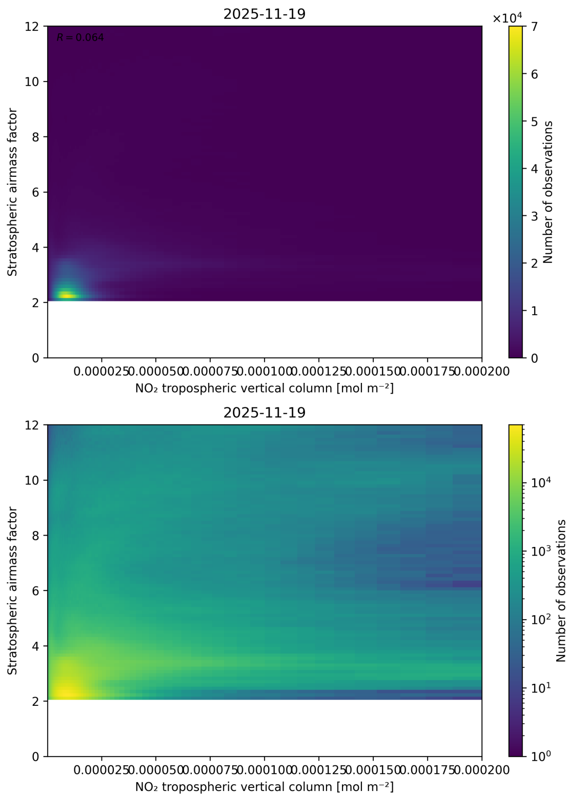
Figure 121: Scatter density plot of “NO 2 tropospheric vertical column” against “Stratospheric airmass factor” for 2025-11-18 to 2025-11-20.
