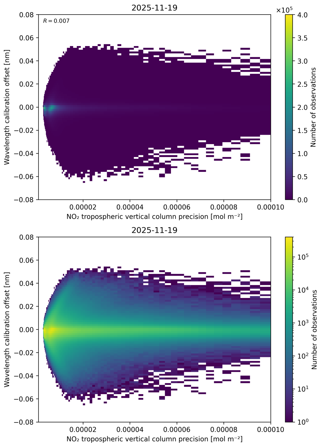
Figure 141: Scatter density plot of “NO 2 tropospheric vertical column precision” against “Wavelength calibration offset” for 2025-11-18 to 2025-11-20.
