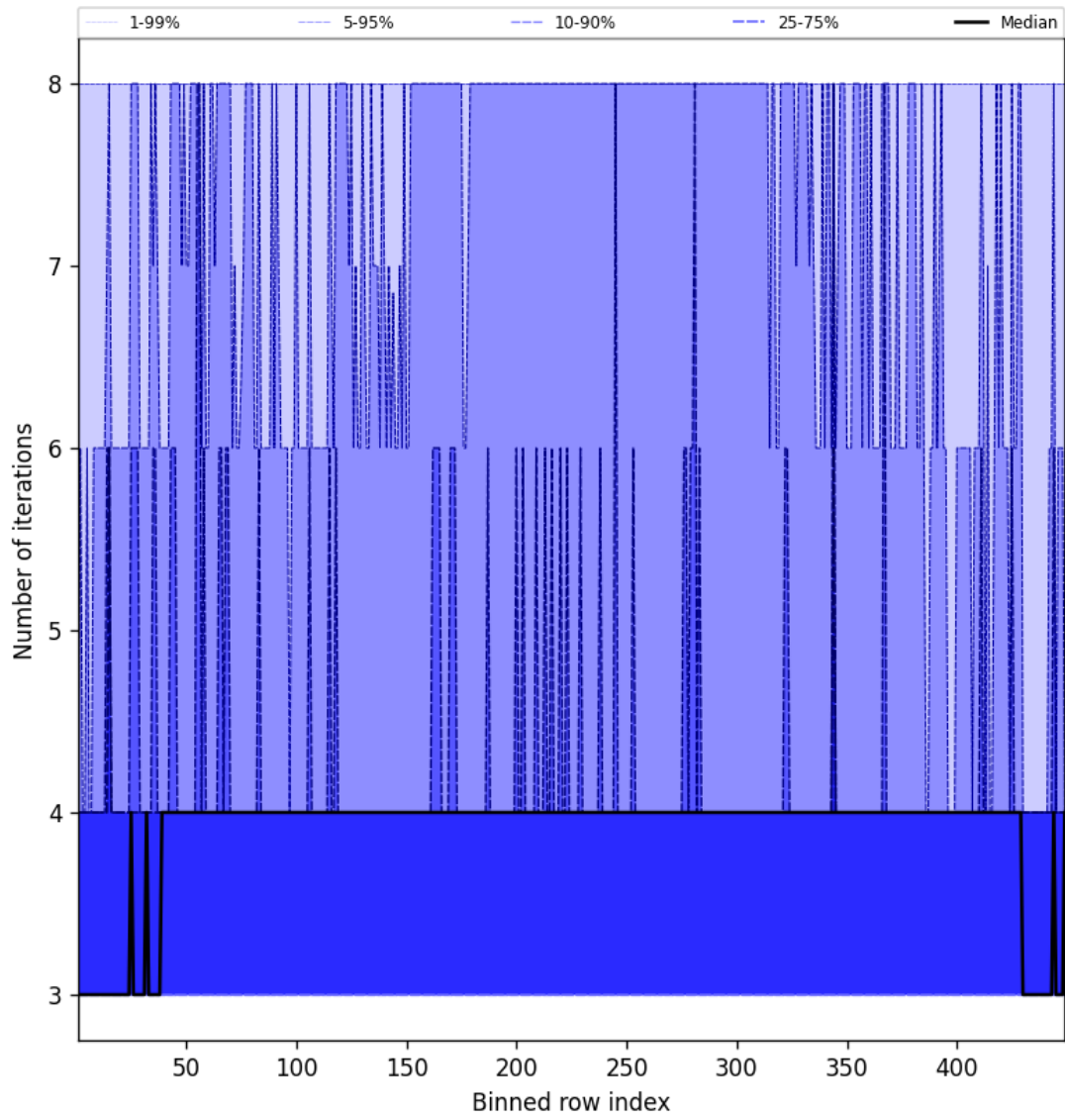
Figure 51: Along track statistics of “Number of iterations” for 2025-11-19 to 2025-11-21
