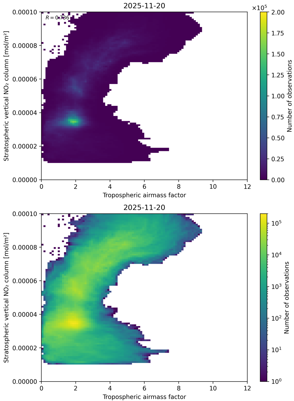
Figure 74: Scatter density plot of “Tropospheric air mass factor” against “Stratospheric vertical NO 2 column” for 2025-11-19 to 2025-11-21.
