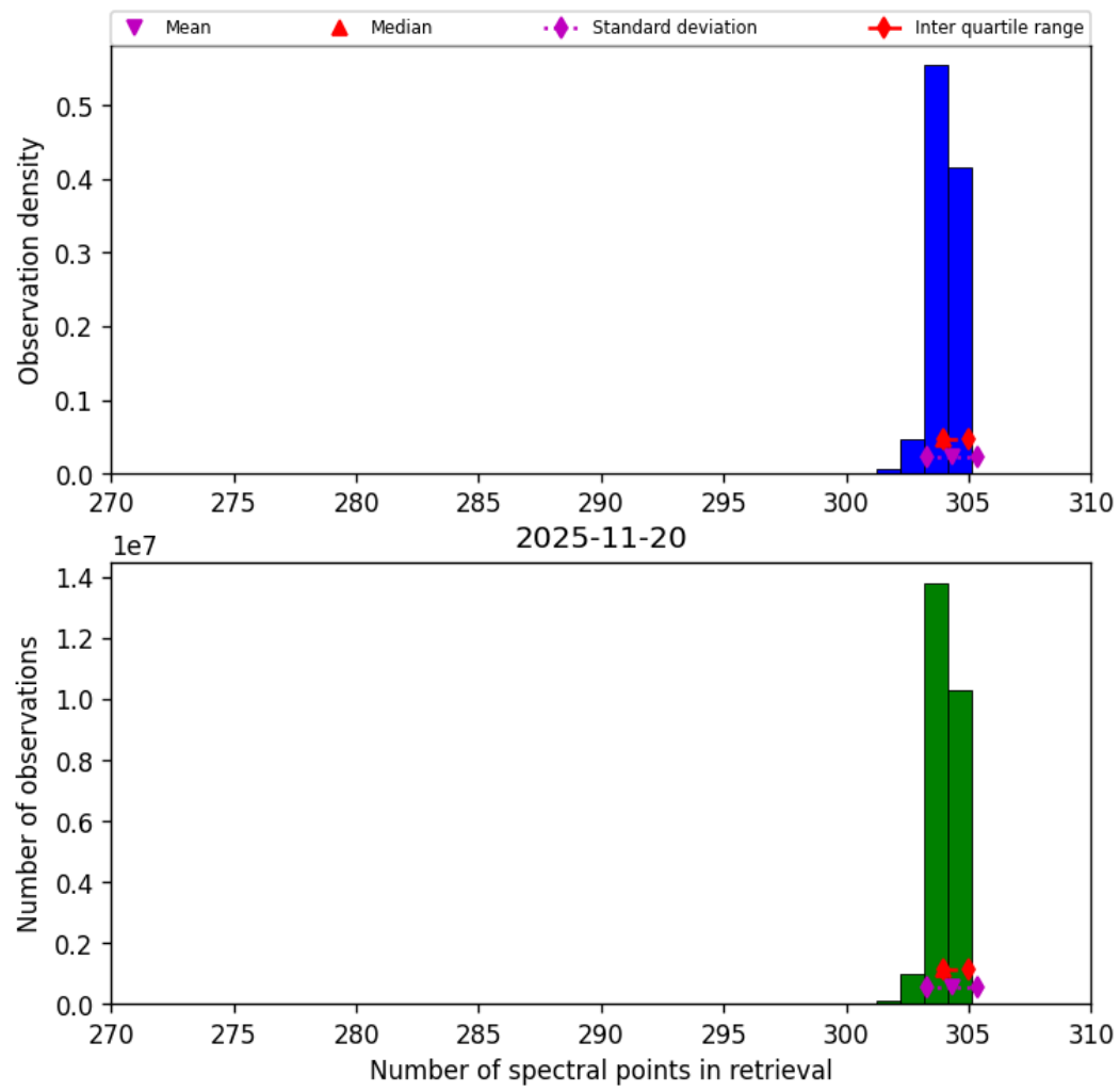
Figure 33: Histogram of “Number of spectral points in retrieval” for 2025-11-19 to 2025-11-21
