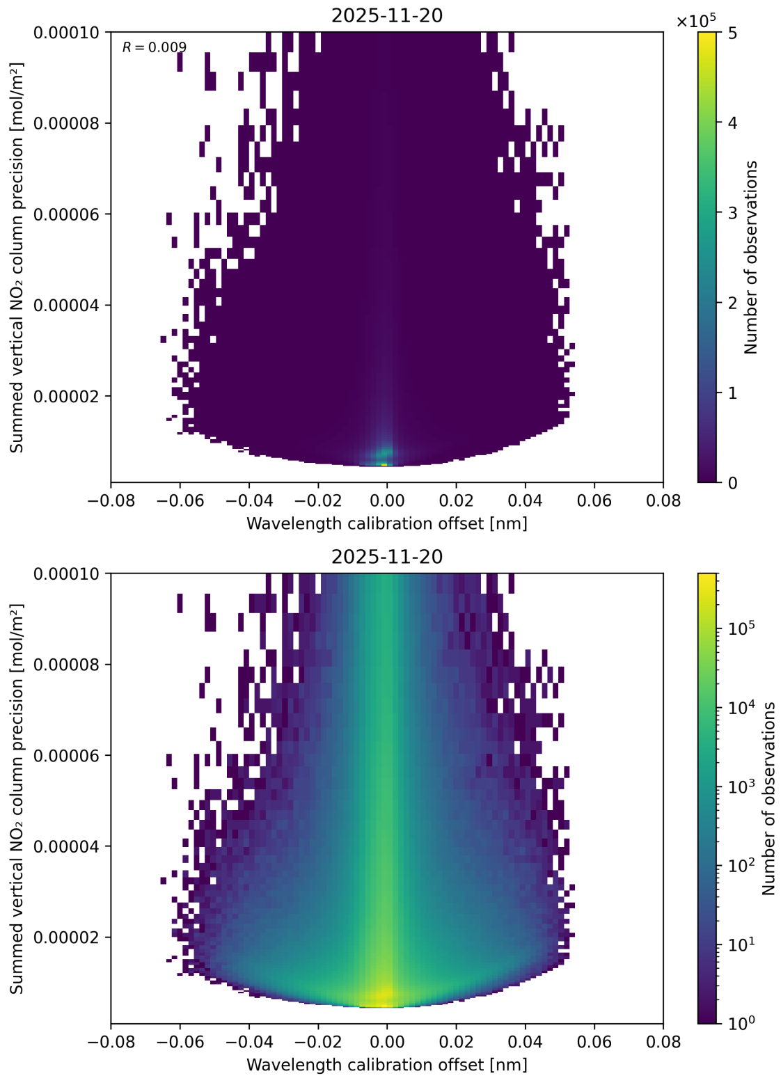
Figure 178: Scatter density plot of “Wavelength calibration offset” against “Summed vertical NO 2 column precision” for 2025-11-19 to 2025-11-21.
