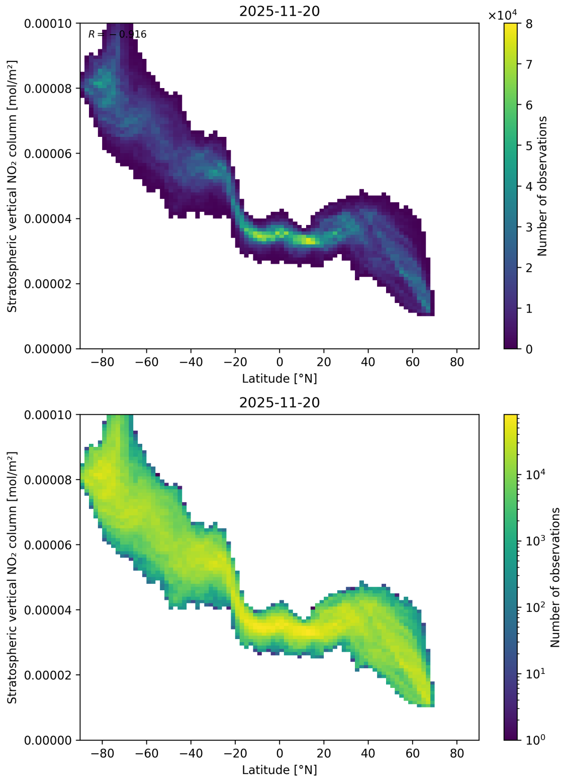
Figure 87: Scatter density plot of “Latitude” against “Stratospheric vertical NO 2 column” for 2025-11-19 to 2025-11-21.
