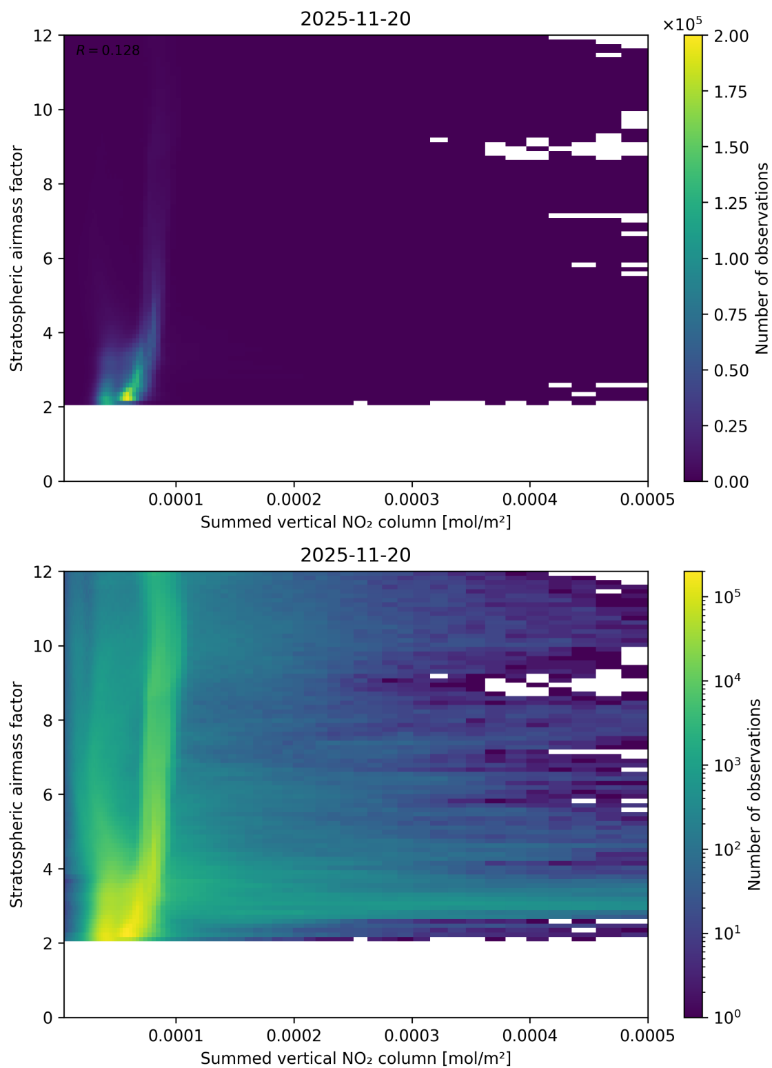
Figure 103: Scatter density plot of “Summed vertical NO 2 column” against “Stratospheric airmass factor” for 2025-11-19 to 2025-11-21.
