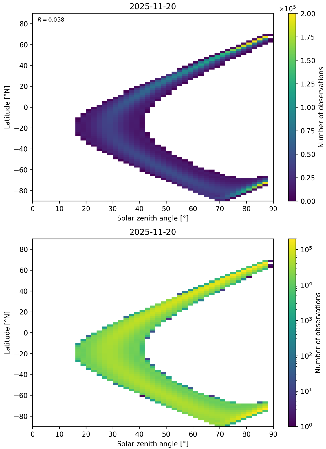
Figure 149: Scatter density plot of “Solar zenith angle” against “Latitude” for 2025-11-19 to 2025-11-21.
