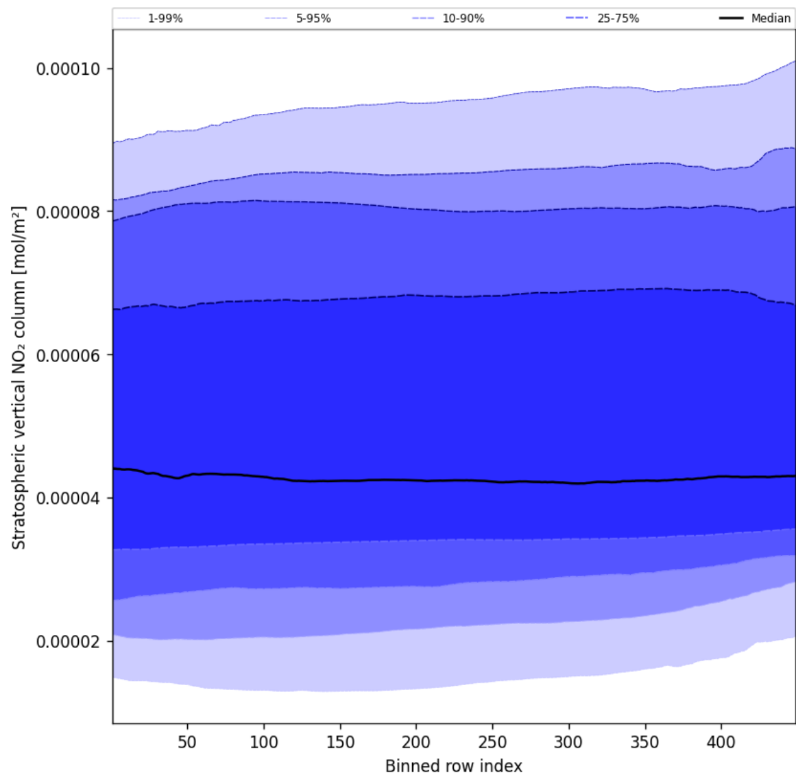
Figure 53: Along track statistics of “Stratospheric vertical NO 2 column” for 2025-11-19 to 2025-11-21
