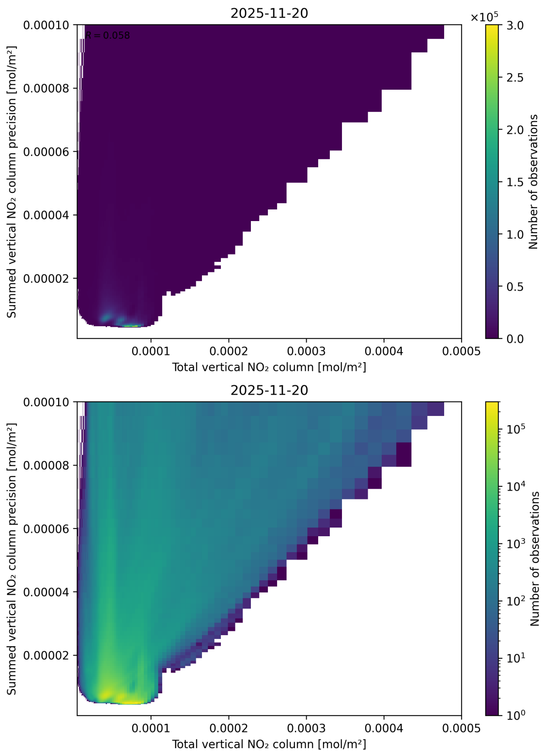
Figure 113: Scatter density plot of “Total vertical NO 2 column” against “Summed vertical NO 2 column precision” for 2025-11-19 to 2025-11-21.
