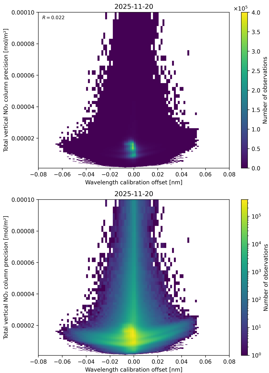
Figure 180: Scatter density plot of “Wavelength calibration offset” against “Total vertical NO 2 column precision” for 2025-11-19 to 2025-11-21.
