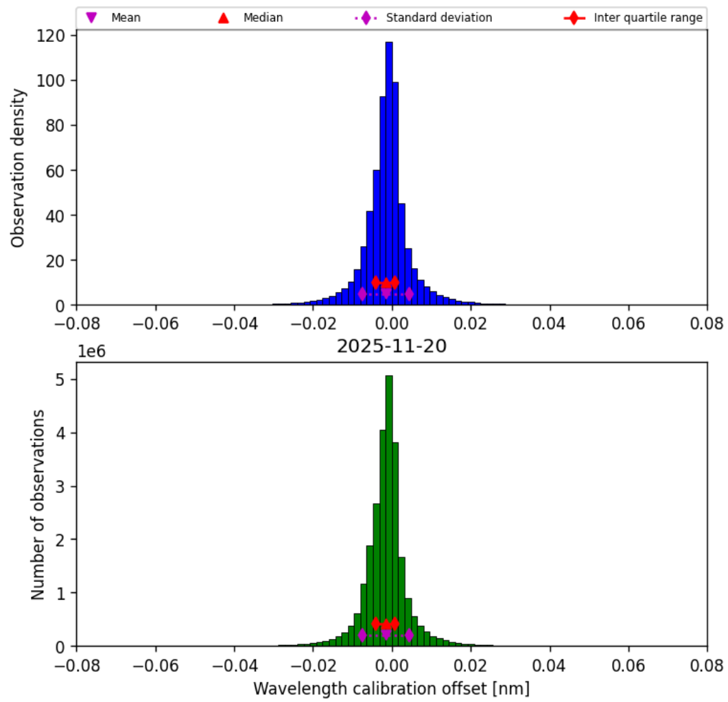
Figure 35: Histogram of “Wavelength calibration offset” for 2025-11-19 to 2025-11-21
