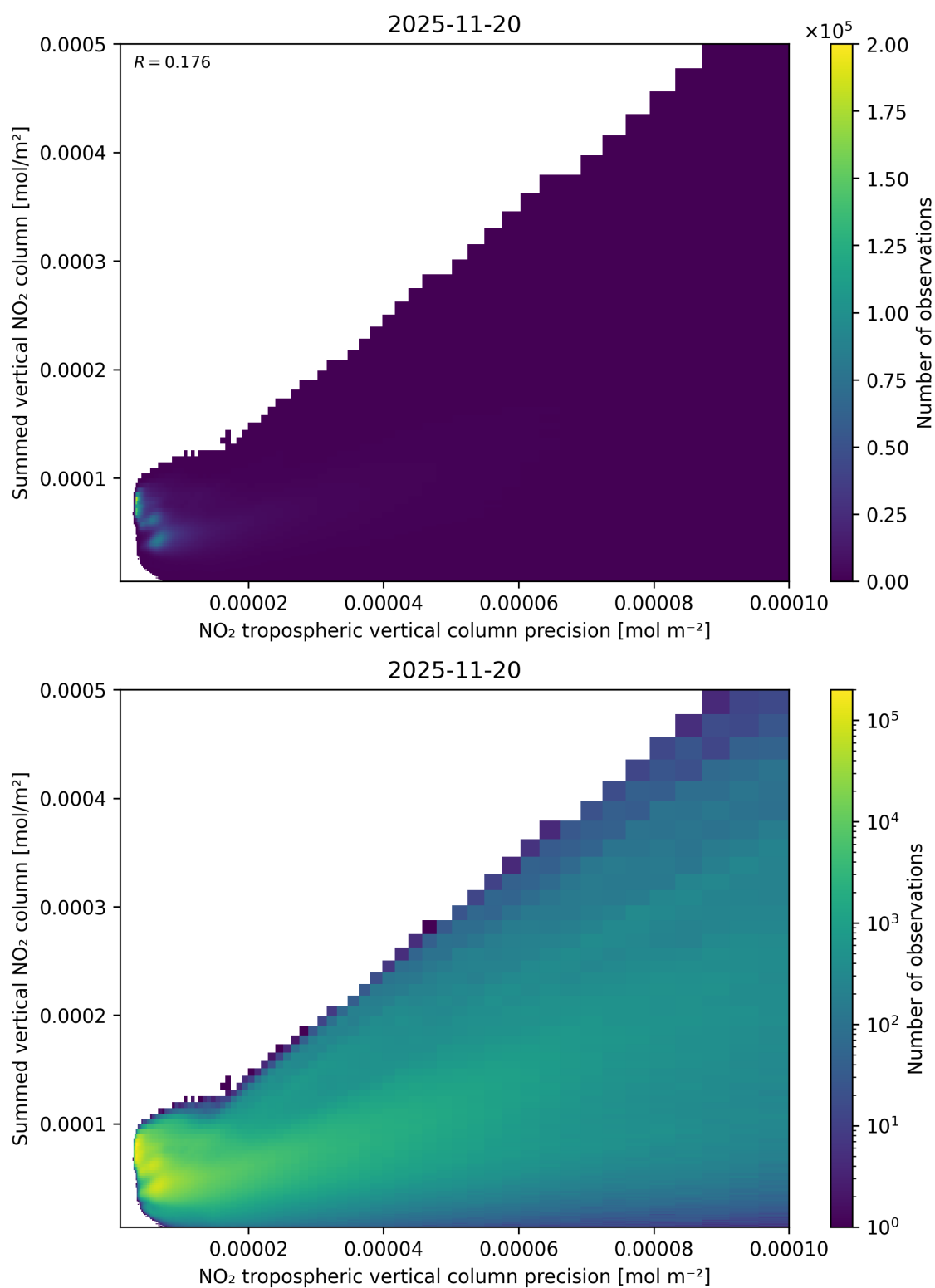
Figure 136: Scatter density plot of “NO 2 tropospheric vertical column precision” against “Summed vertical NO 2 column” for 2025-11-19 to 2025-11-21.
