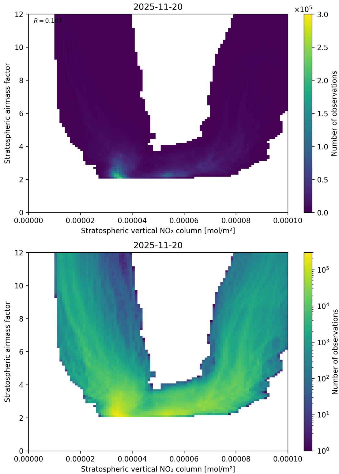
Figure 96: Scatter density plot of “Stratospheric vertical NO 2 column” against “Stratospheric airmass factor” for 2025-11-19 to 2025-11-21.
