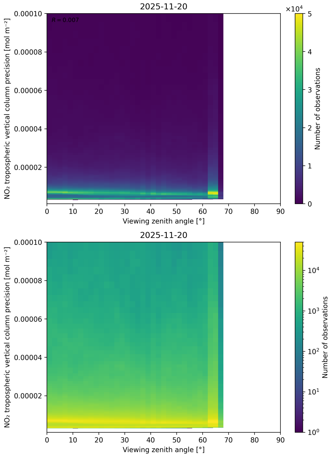
Figure 170: Scatter density plot of “Viewing zenith angle” against “NO 2 tropospheric vertical column precision” for 2025-11-19 to 2025-11-21.
