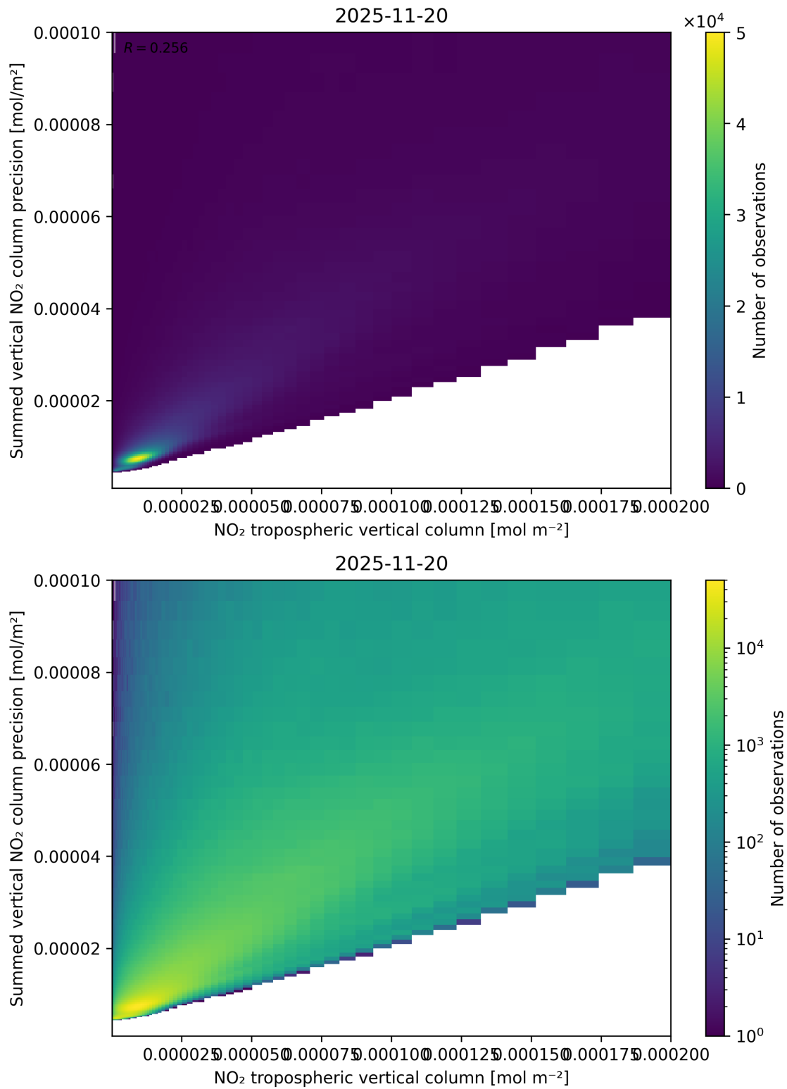
Figure 127: Scatter density plot of “NO 2 tropospheric vertical column” against “Summed vertical NO 2 column precision” for 2025-11-19 to 2025-11-21.
