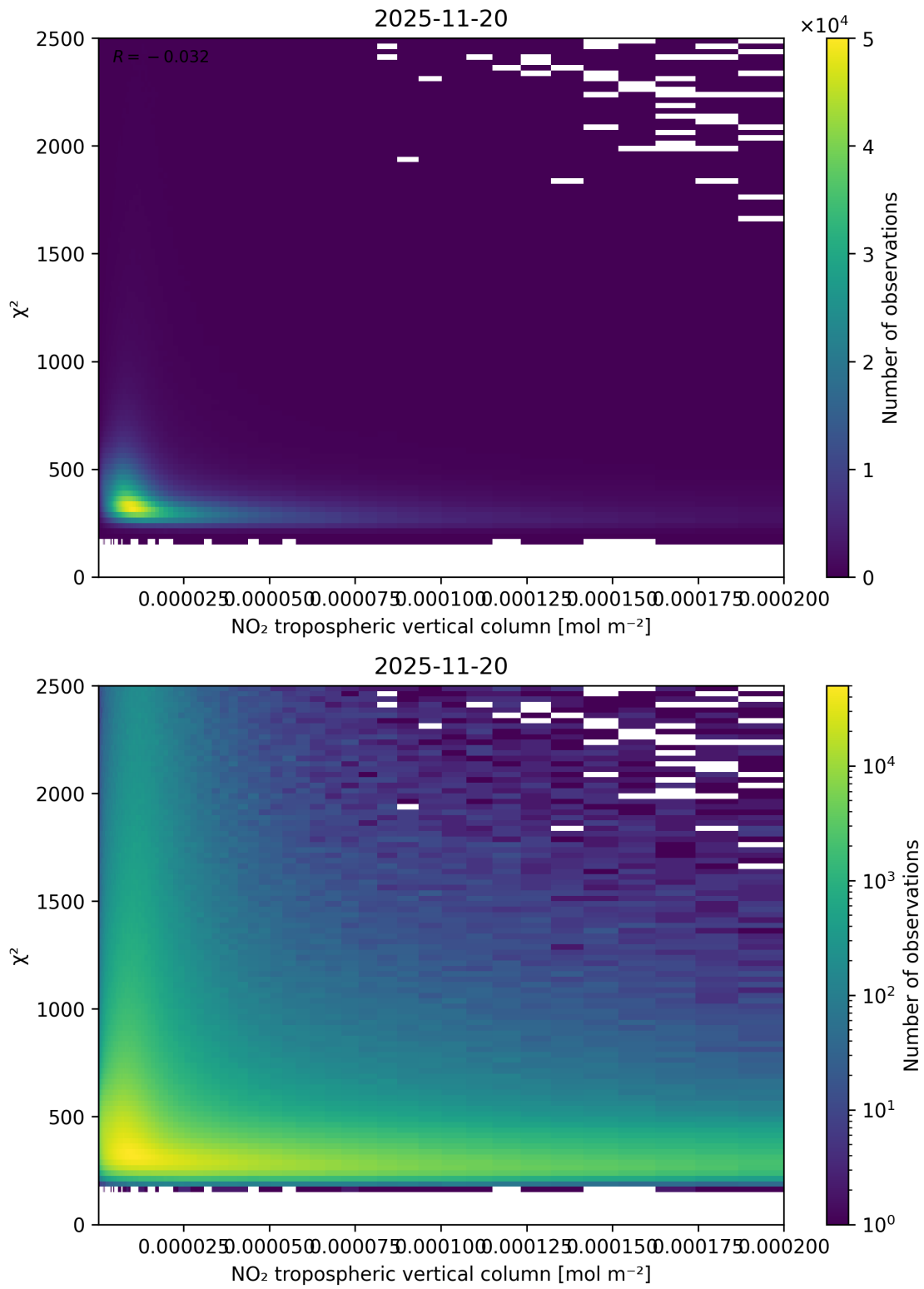
Figure 124: Scatter density plot of “NO 2 tropospheric vertical column” against “ \chi^2 ” for 2025-11-19 to 2025-11-21.
