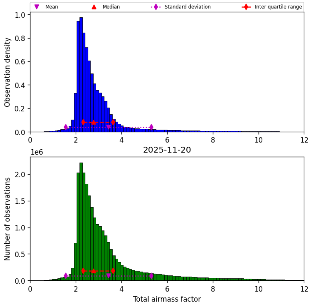
Figure 32: Histogram of “Total airmass factor” for 2025-11-19 to 2025-11-21
