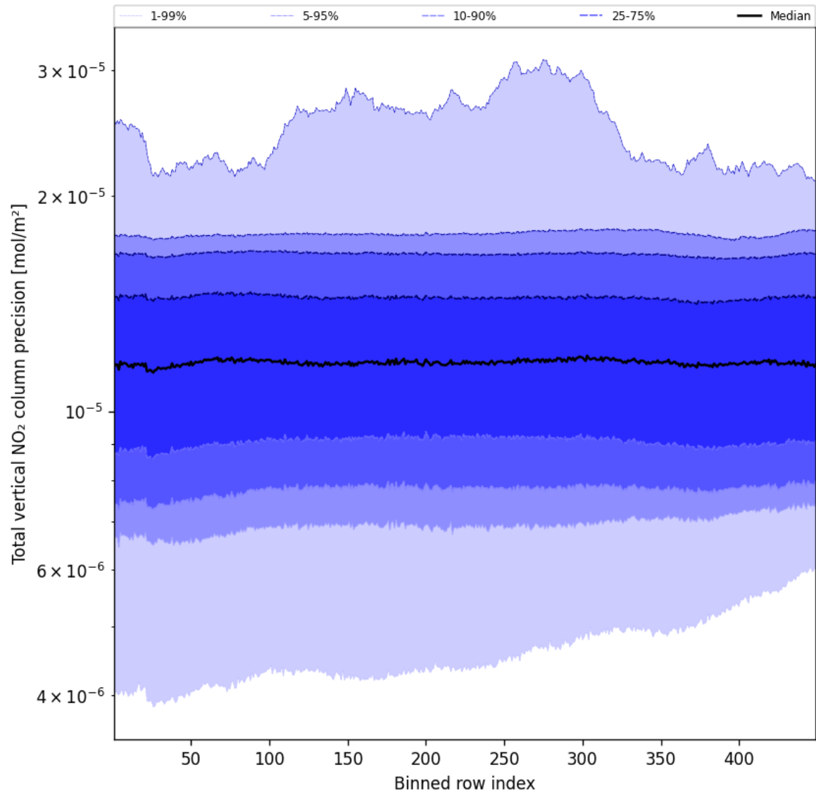
Figure 56: Along track statistics of “Total vertical NO 2 column precision” for 2025-11-19 to 2025-11-21
