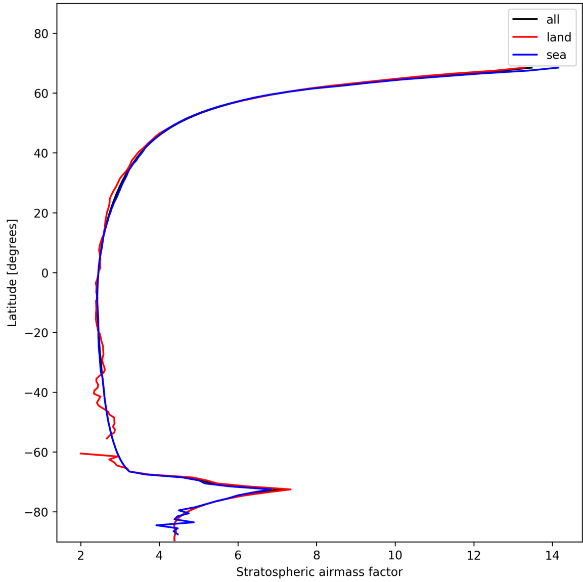
Figure 27: Zonal average of “Stratospheric air mass factor” for 2025-11-19 to 2025-11-21.
