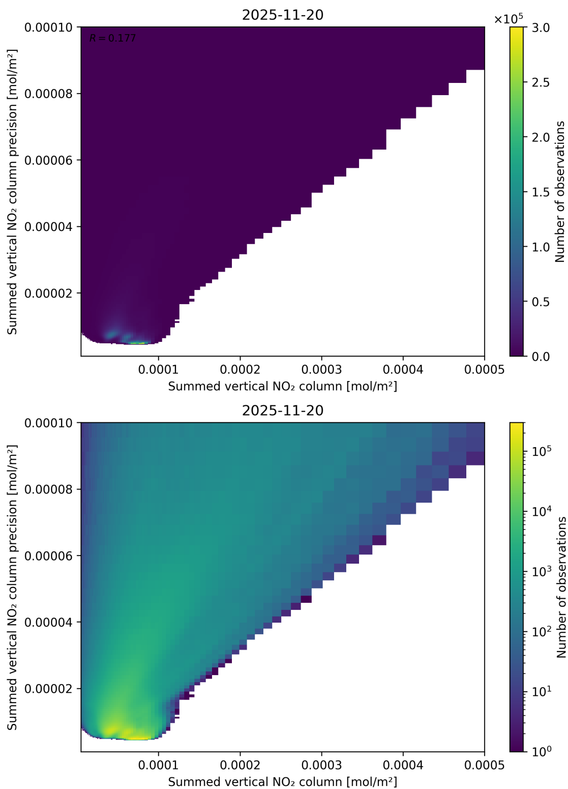
Figure 105: Scatter density plot of “Summed vertical NO 2 column” against “Summed vertical NO 2 column precision” for 2025-11-19 to 2025-11-21.
