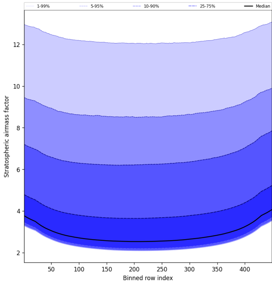
Figure 61: Along track statistics of “Stratospheric airmass factor” for 2025-11-19 to 2025-11-21
