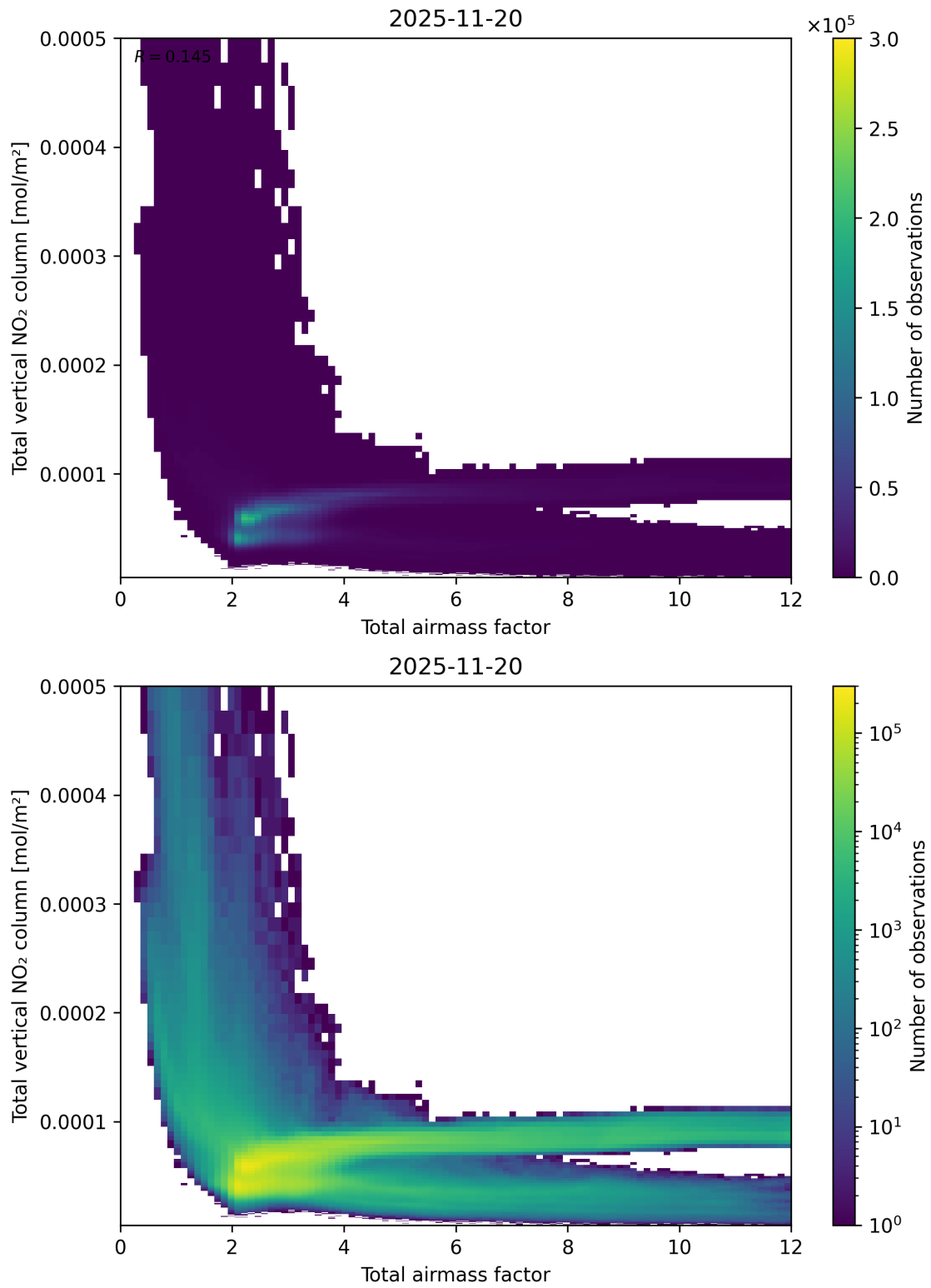
Figure 67: Scatter density plot of “Total airmass factor” against “Total vertical NO 2 column” for 2025-11-19 to 2025-11-21.
