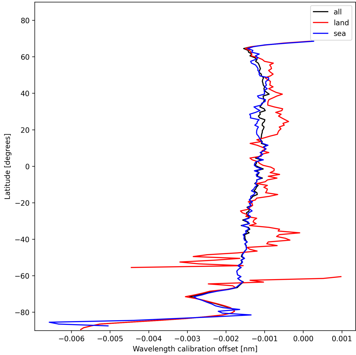
Figure 18: Zonal average of “Wavelength calibration offset” for 2025-11-19 to 2025-11-21.
