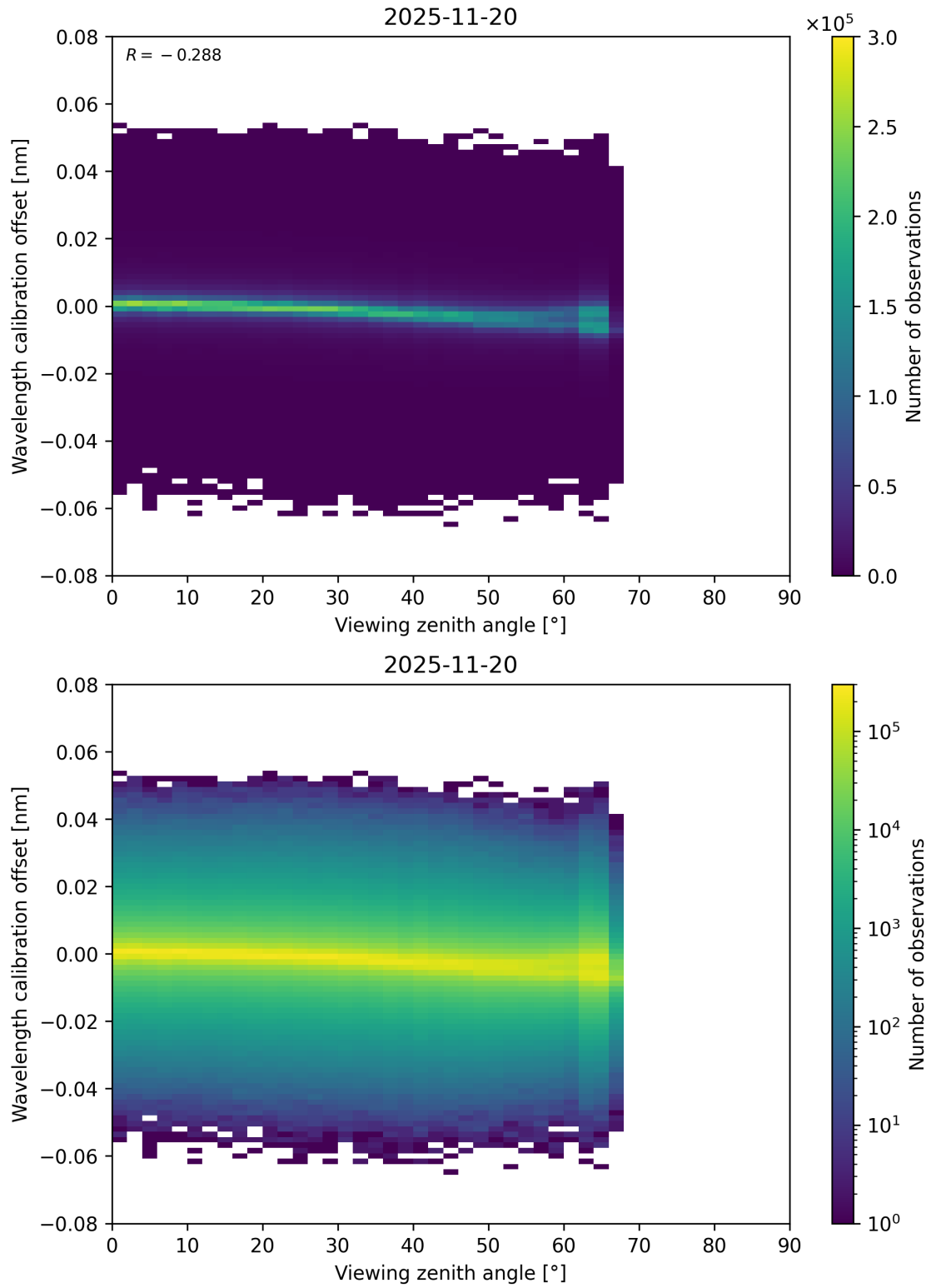
Figure 173: Scatter density plot of “Viewing zenith angle” against “Wavelength calibration offset” for 2025-11-19 to 2025-11-21.
