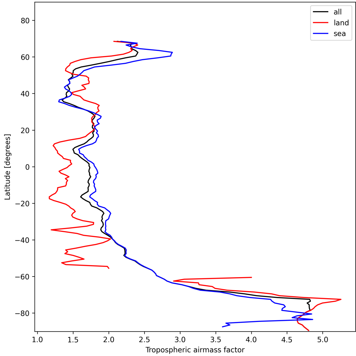
Figure 14: Zonal average of “Tropospheric airmass factor” for 2025-11-19 to 2025-11-21.
