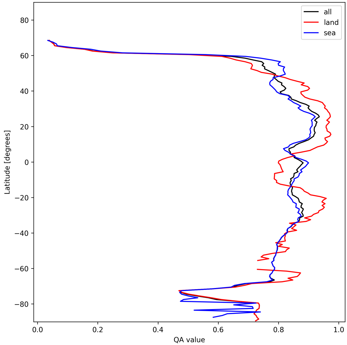
Figure 11: Zonal average of “QA value” for 2025-11-19 to 2025-11-21.
