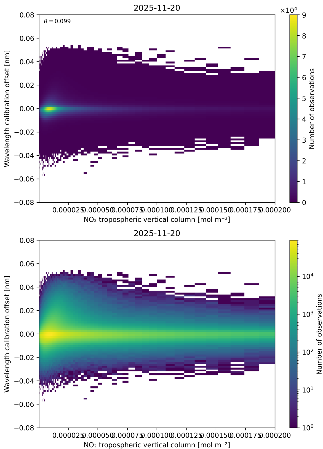
Figure 143: Scatter density plot of “NO 2 tropospheric vertical column” against “Wavelength calibration offset” for 2025-11-19 to 2025-11-21.
