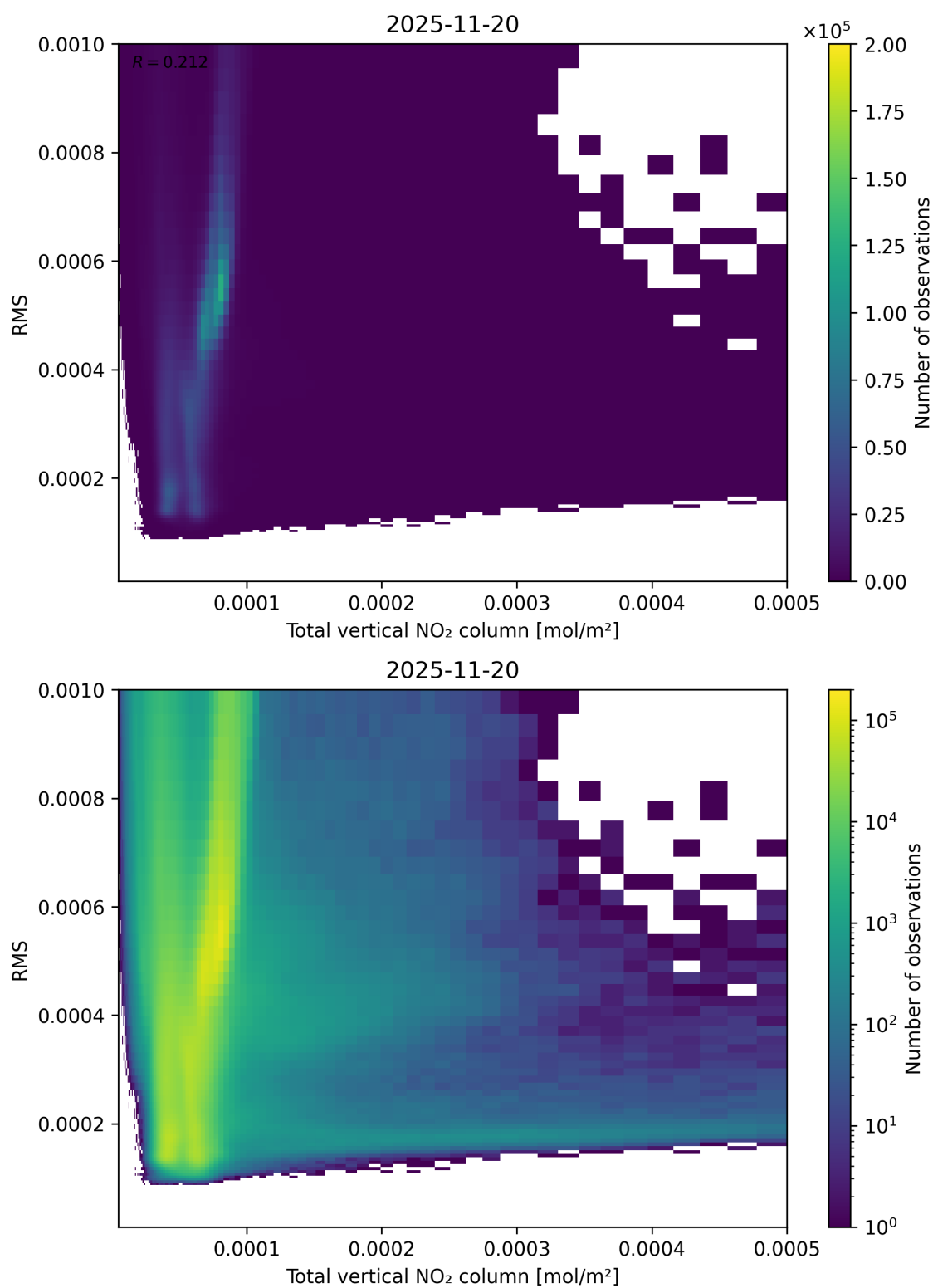
Figure 120: Scatter density plot of “Total vertical NO 2 column” against “RMS” for 2025-11-19 to 2025-11-21.
