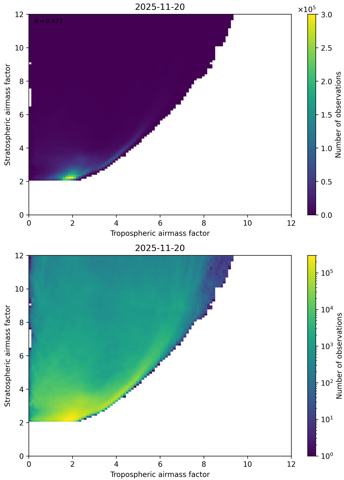
Figure 71: Scatter density plot of “Tropospheric airmass factor” against “Stratospheric airmass factor” for 2025-11-19 to 2025-11-21.
