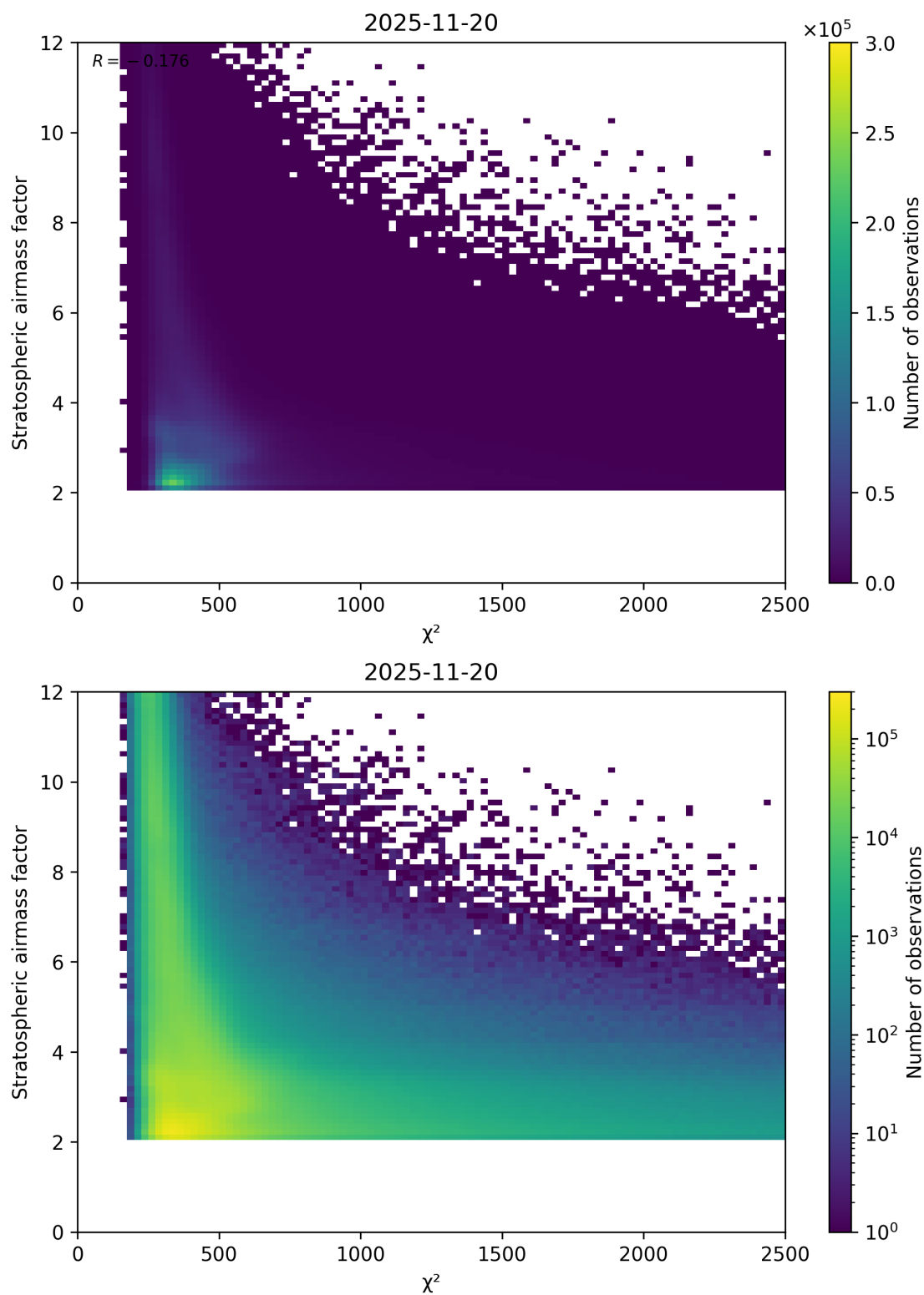
Figure 81: Scatter density plot of “ \chi^2 ” against “Stratospheric airmass factor” for 2025-11-19 to 2025-11-21.
