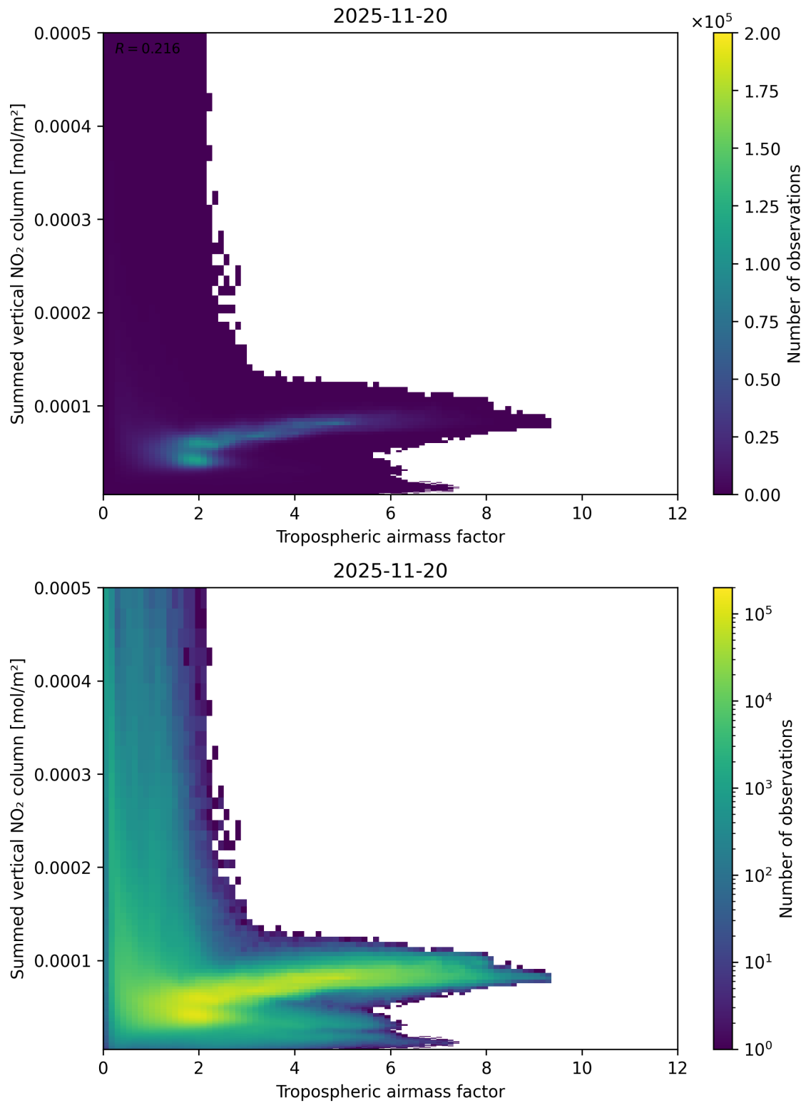
Figure 75: Scatter density plot of “Tropospheric air mass factor” against “Summed vertical NO 2 column” for 2025-11-19 to 2025-11-21.
