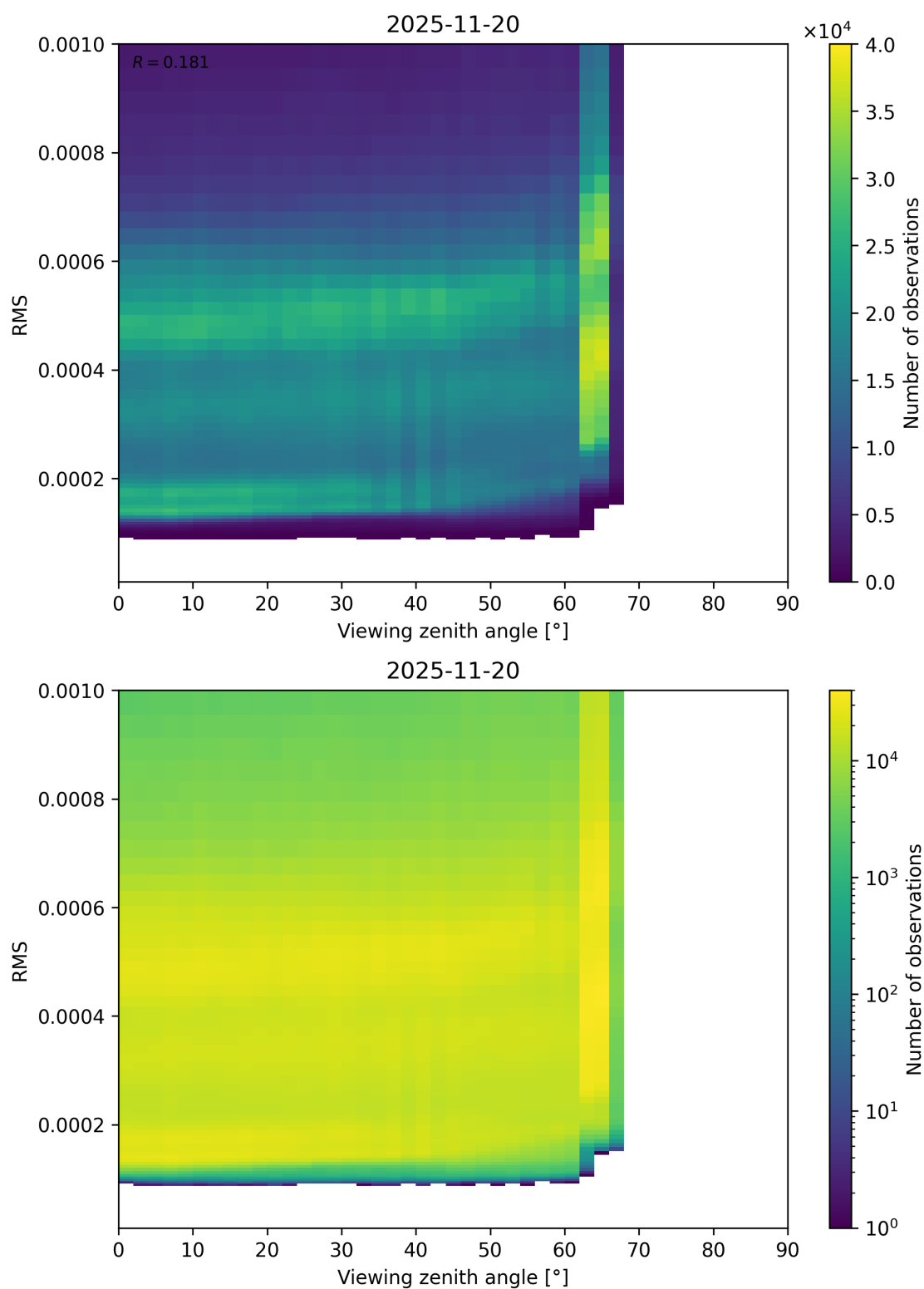
Figure 171: Scatter density plot of “Viewing zenith angle” against “RMS” for 2025-11-19 to 2025-11-21.
