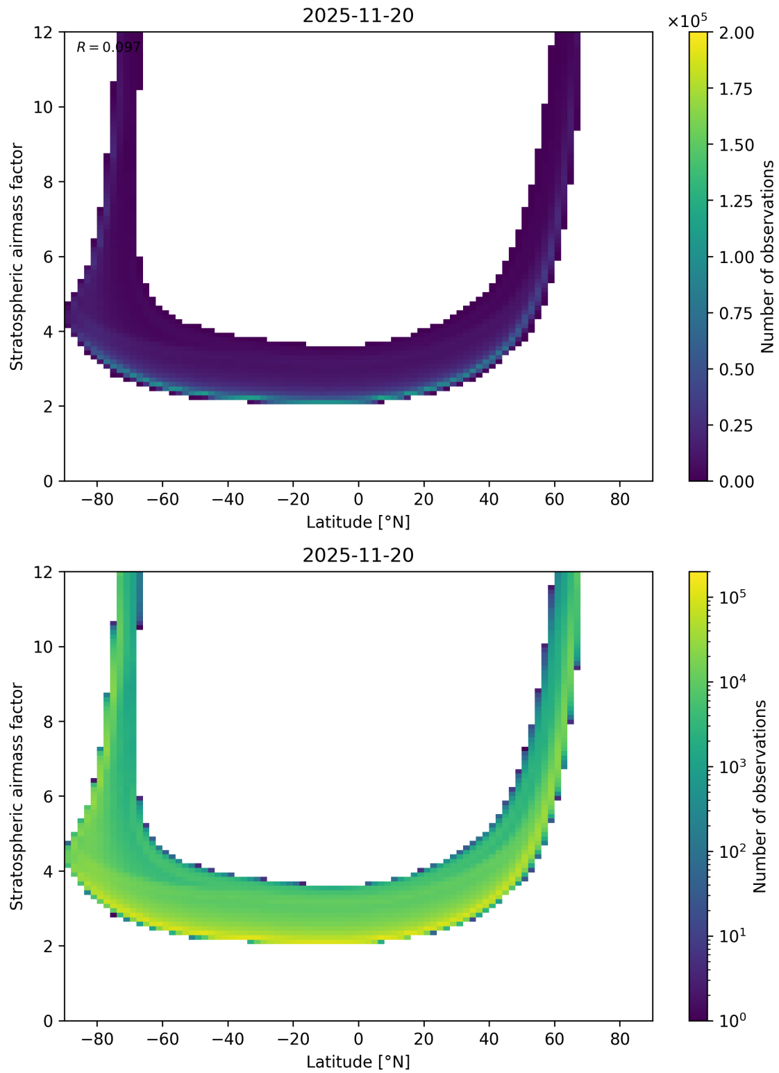
Figure 83: Scatter density plot of “Latitude” against “Stratospheric airmass factor” for 2025-11-19 to 2025-11-21.
