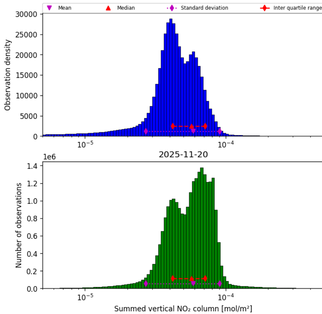
Figure 40: Histogram of “Summed vertical NO 2 column” for 2025-11-19 to 2025-11-21
