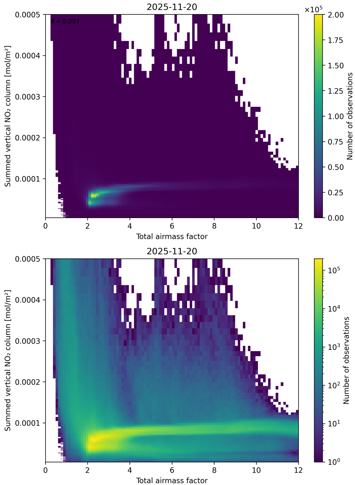
Figure 65: Scatter density plot of “Total airmass factor” against “Summed vertical NO 2 column” for 2025-11-19 to 2025-11-21.
