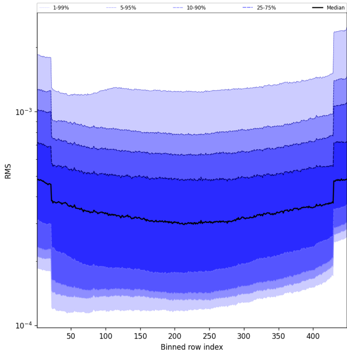
Figure 60: Along track statistics of “RMS” for 2025-11-19 to 2025-11-21
