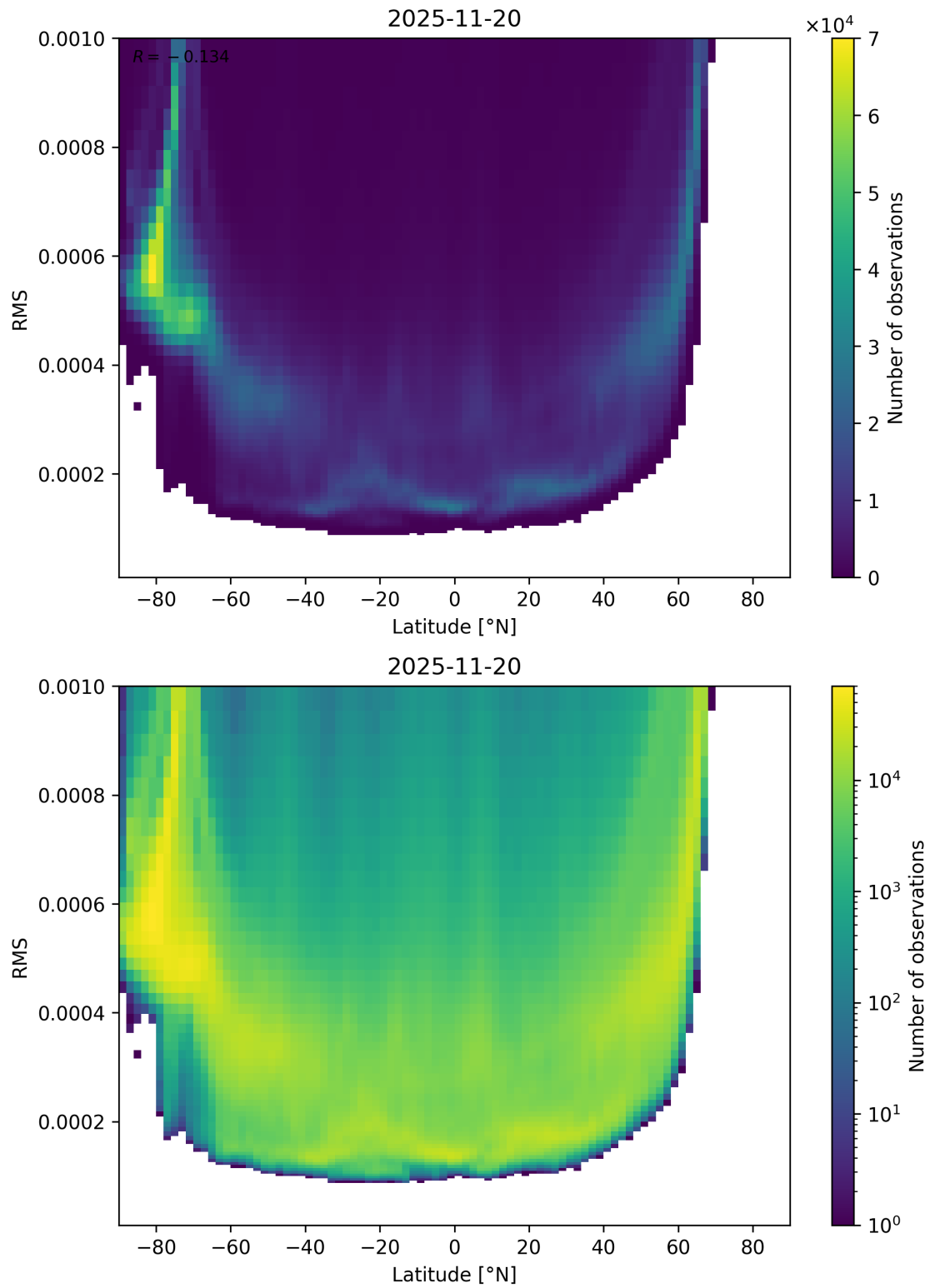
Figure 94: Scatter density plot of “Latitude” against “RMS” for 2025-11-19 to 2025-11-21.
