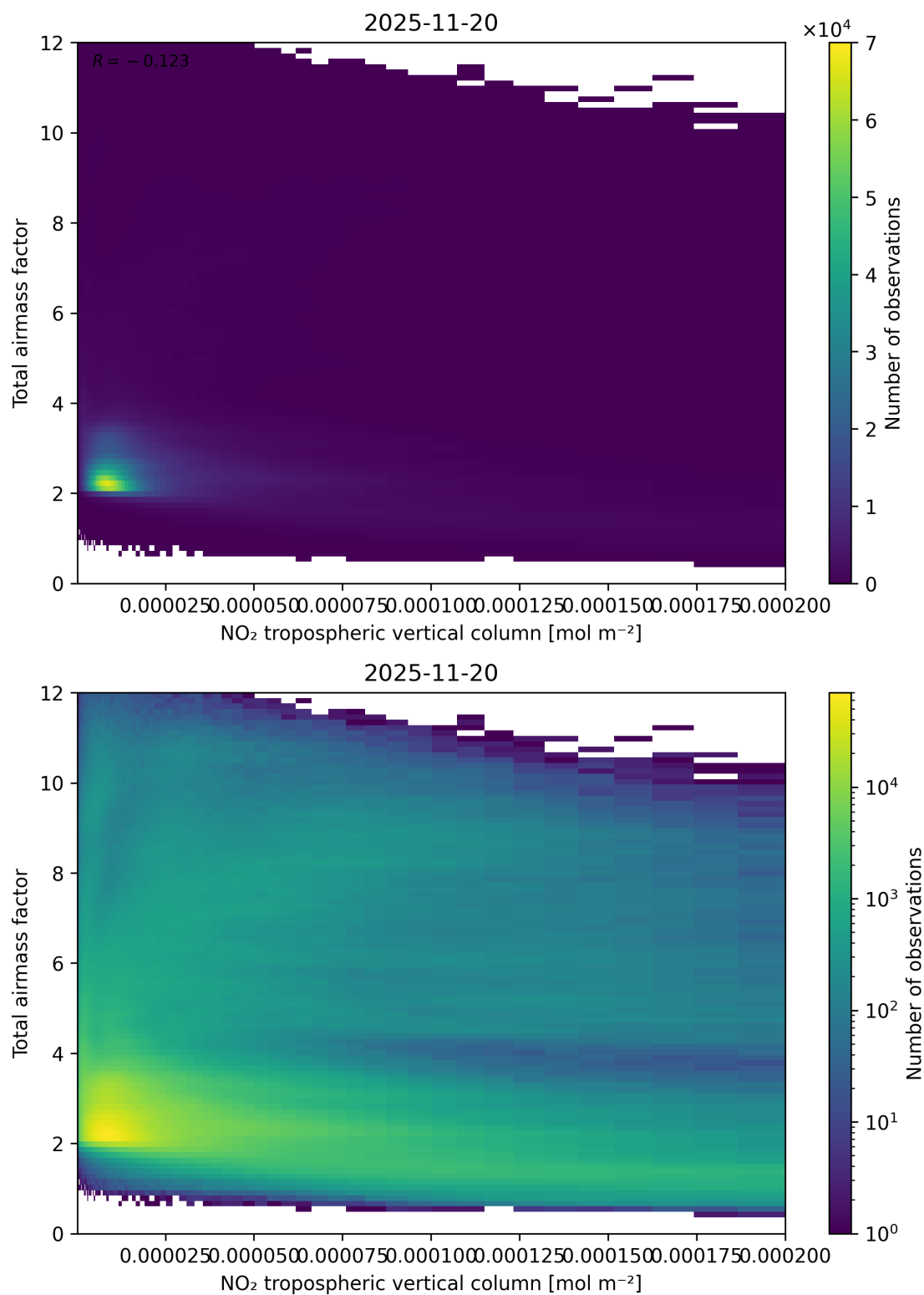
Figure 122: Scatter density plot of “NO 2 tropospheric vertical column” against “Total air mass factor” for 2025-11-19 to 2025-11-21.
