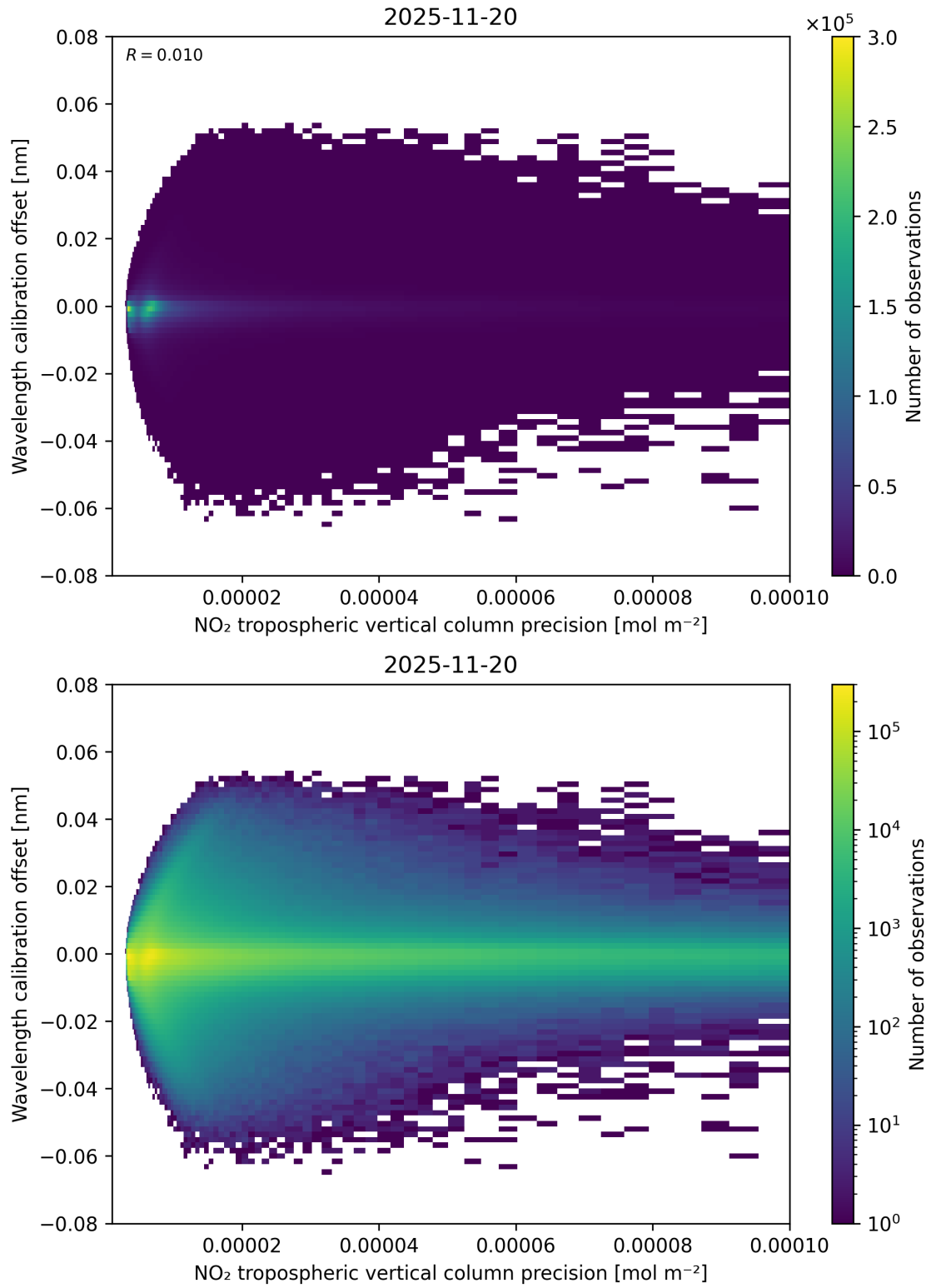
Figure 141: Scatter density plot of “NO 2 tropospheric vertical column precision” against “Wavelength calibration offset” for 2025-11-19 to 2025-11-21.
