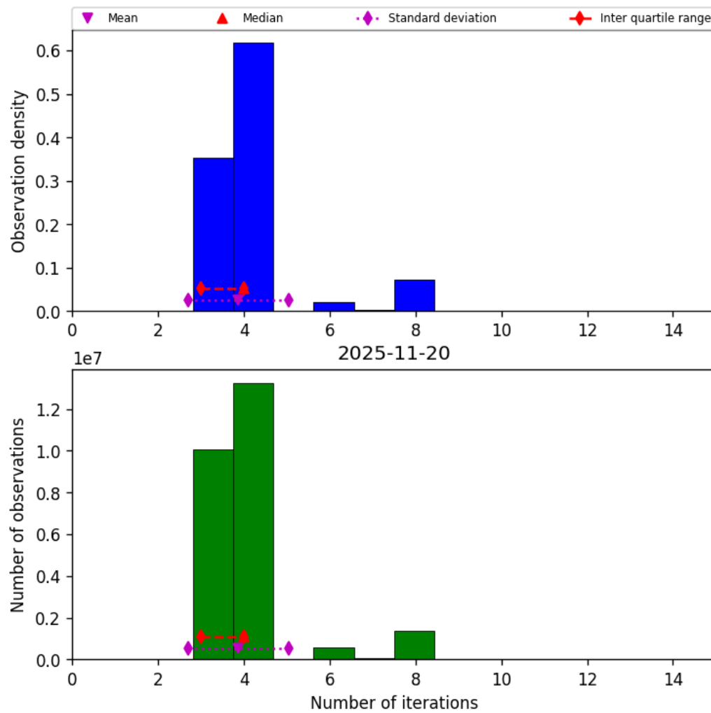
Figure 34: Histogram of “Number of iterations” for 2025-11-19 to 2025-11-21
