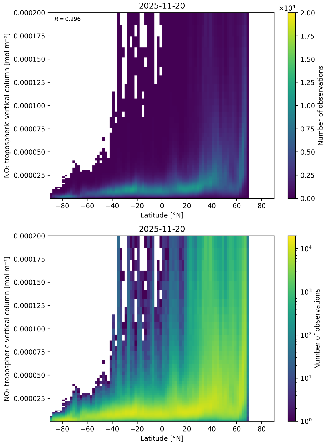
Figure 92: Scatter density plot of “Latitude” against “NO 2 tropospheric vertical column” for 2025-11-19 to 2025-11-21.
