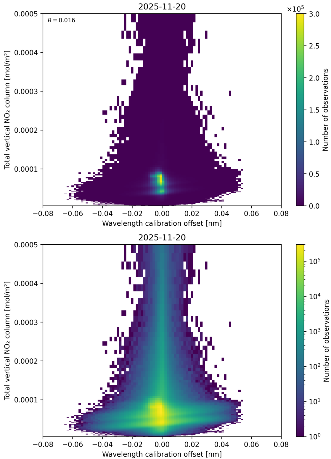
Figure 179: Scatter density plot of “Wavelength calibration offset” against “Total vertical NO 2 column” for 2025-11-19 to 2025-11-21.
