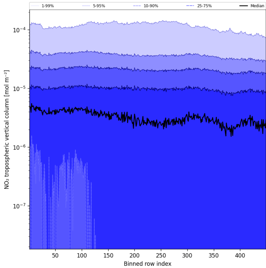
Figure 46: Along track statistics of “NO 2 tropospheric vertical column” for 2025-11-19 to 2025-11-21
