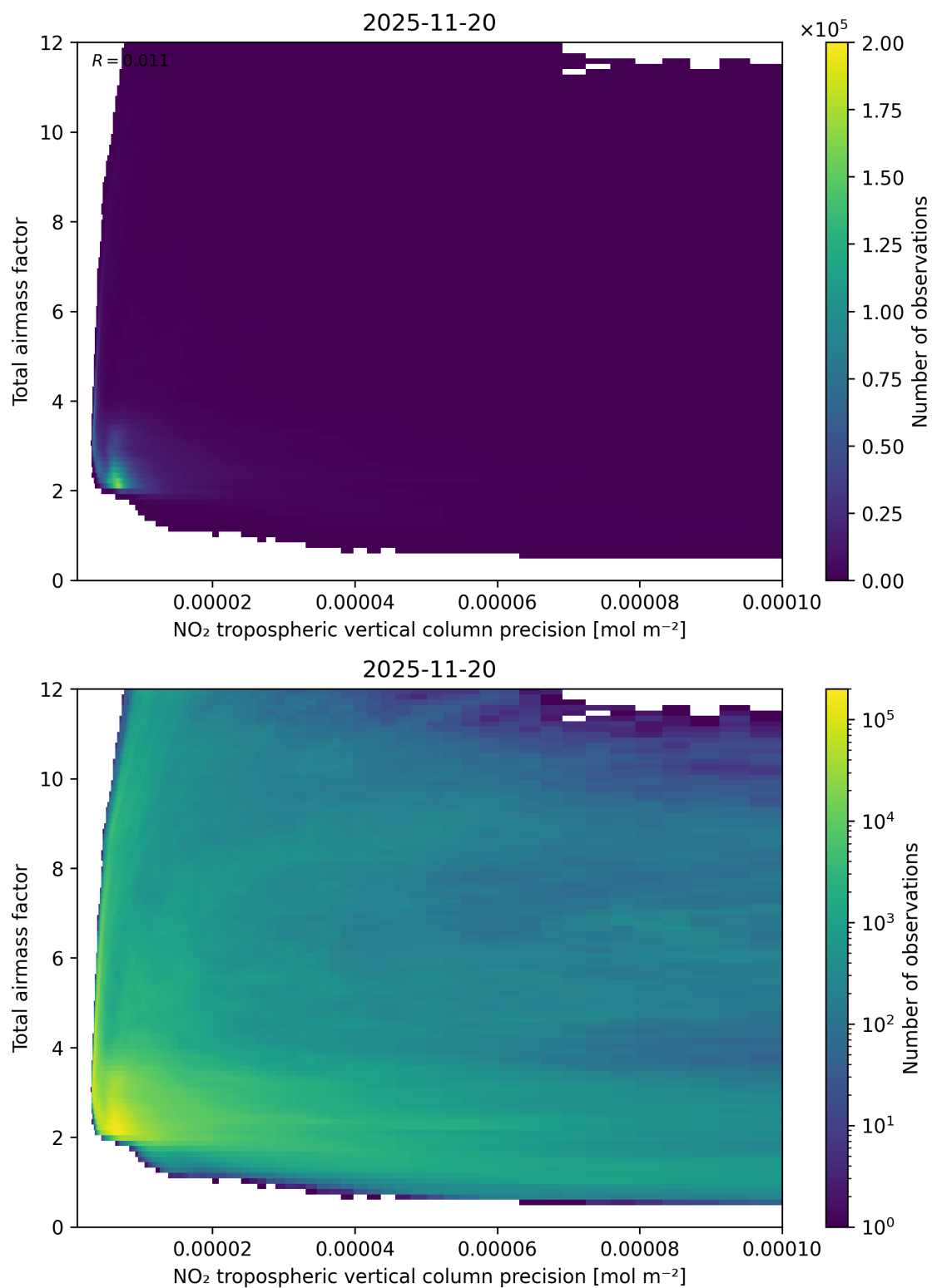
Figure 132: Scatter density plot of “NO 2 tropospheric vertical column precision” against “Total air mass factor” for 2025-11-19 to 2025-11-21.
