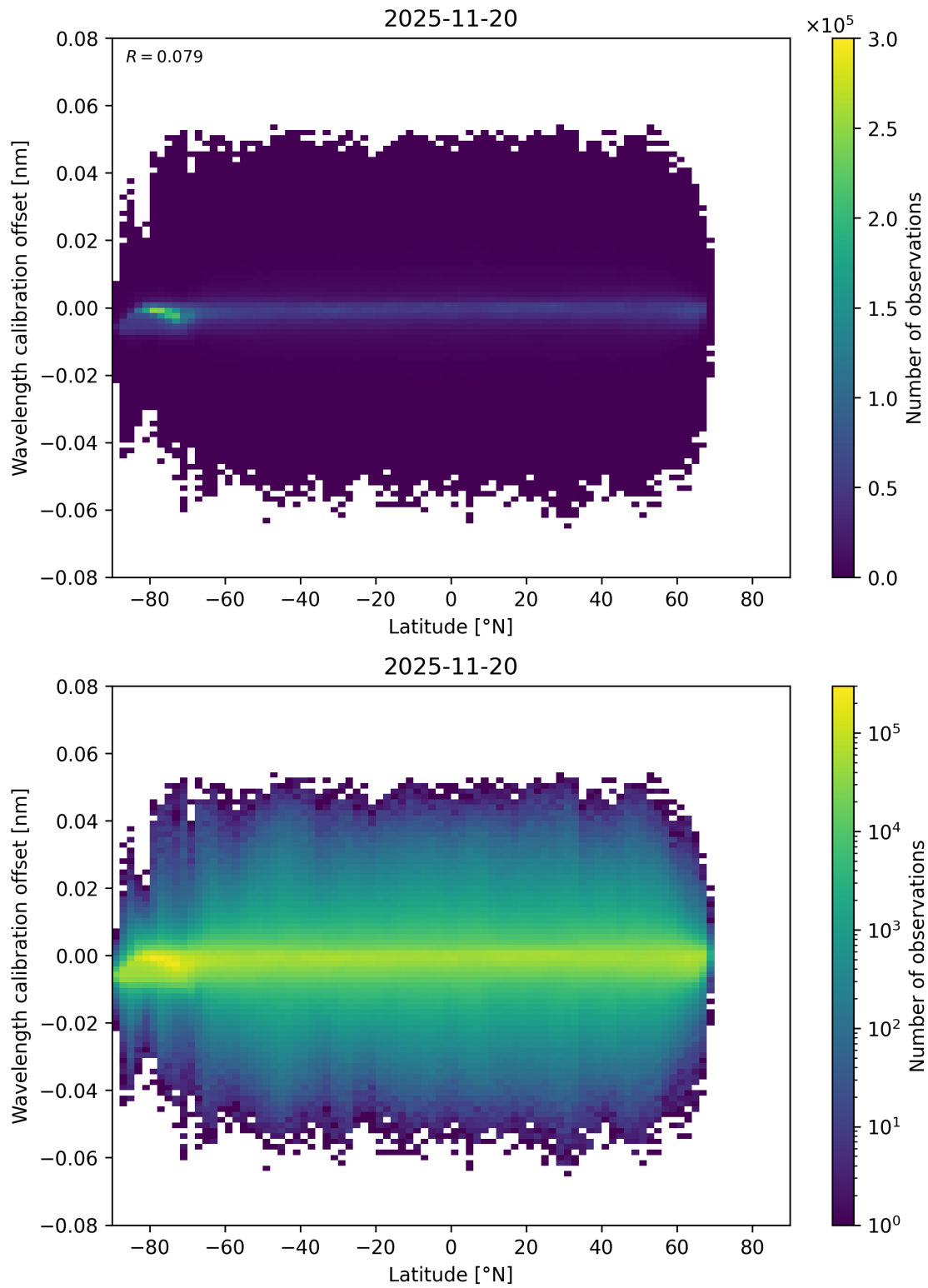
Figure 95: Scatter density plot of “Latitude” against “Wavelength calibration offset” for 2025-11-19 to 2025-11-21.
