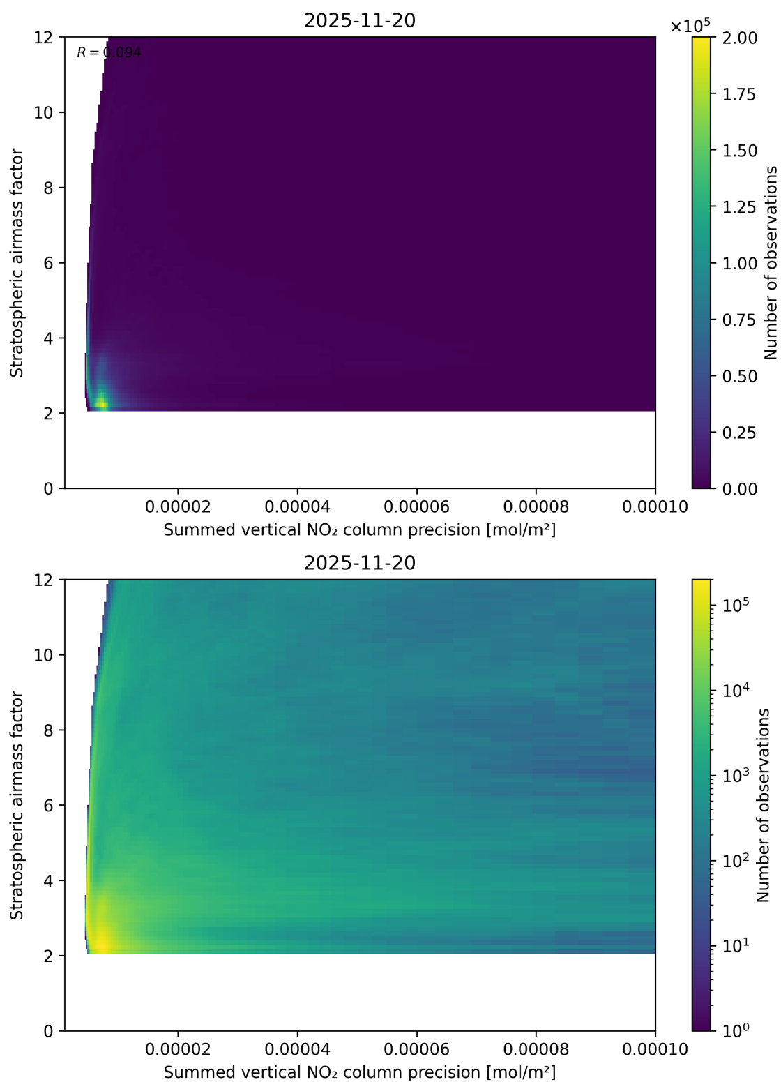
Figure 106: Scatter density plot of “Summed vertical NO 2 column precision” against “Stratospheric airmass factor” for 2025-11-19 to 2025-11-21.
