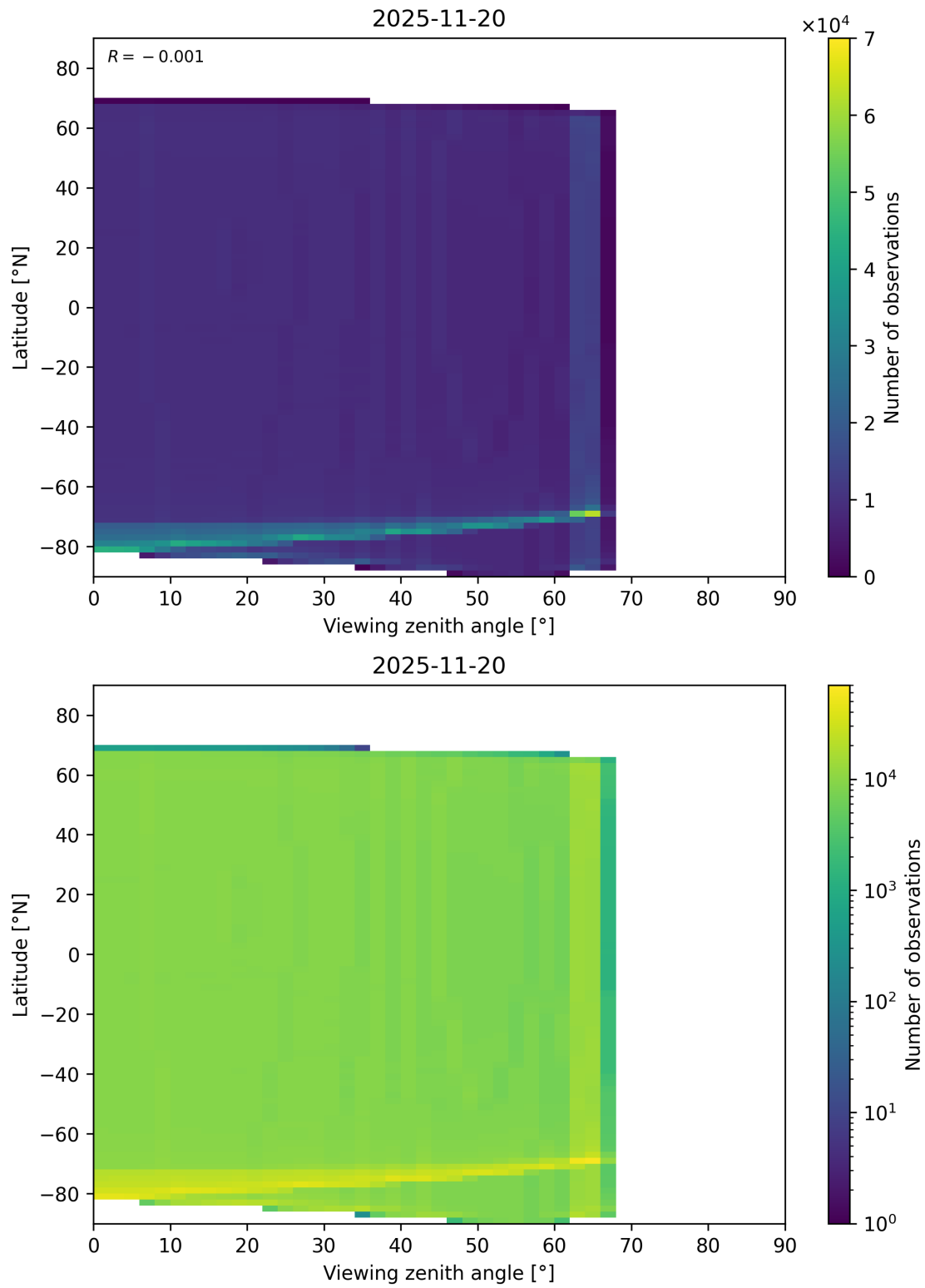
Figure 163: Scatter density plot of “Viewing zenith angle” against “Latitude” for 2025-11-19 to 2025-11-21.
