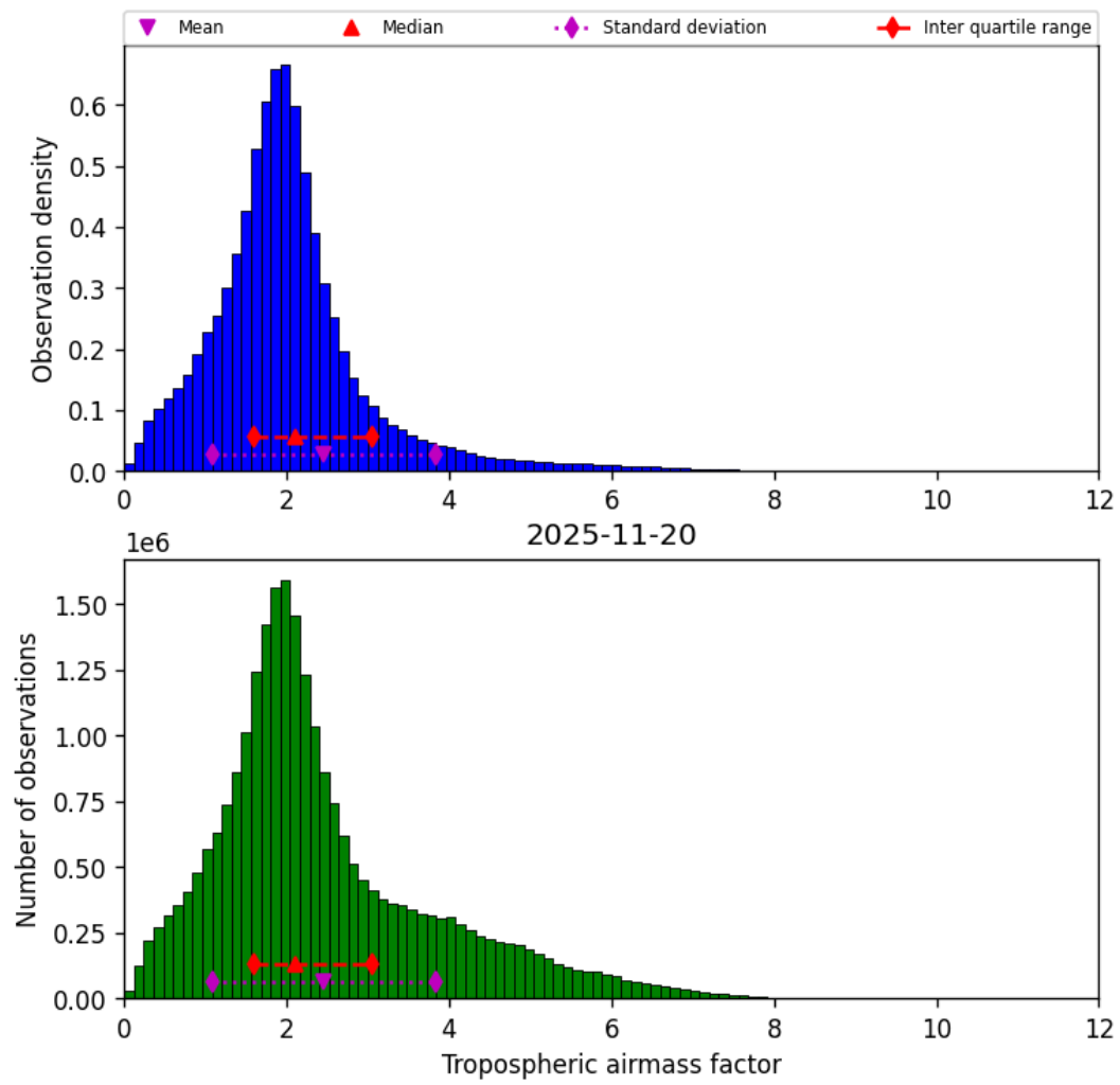
Figure 31: Histogram of “Tropospheric airmass factor” for 2025-11-19 to 2025-11-21
