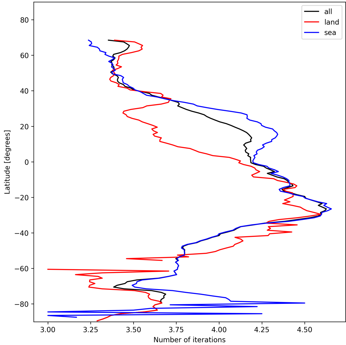
Figure 17: Zonal average of “Number of iterations” for 2025-11-19 to 2025-11-21.
