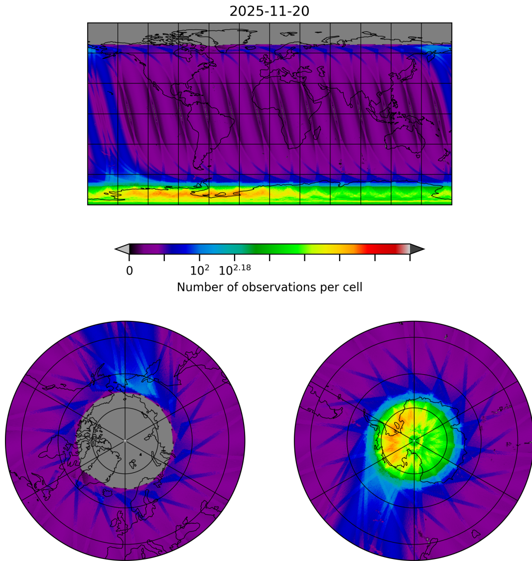
Figure 10: Map of the number of observations for 2025-11-19 to 2025-11-21
