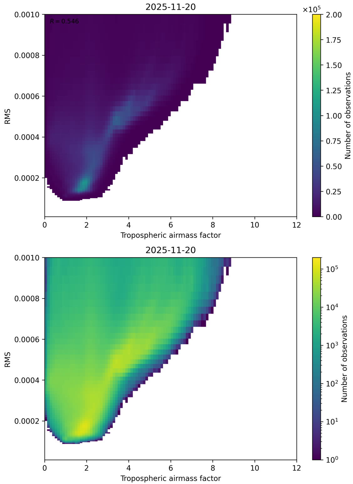
Figure 79: Scatter density plot of “Tropospheric airmass factor” against “RMS” for 2025-11-19 to 2025-11-21.
