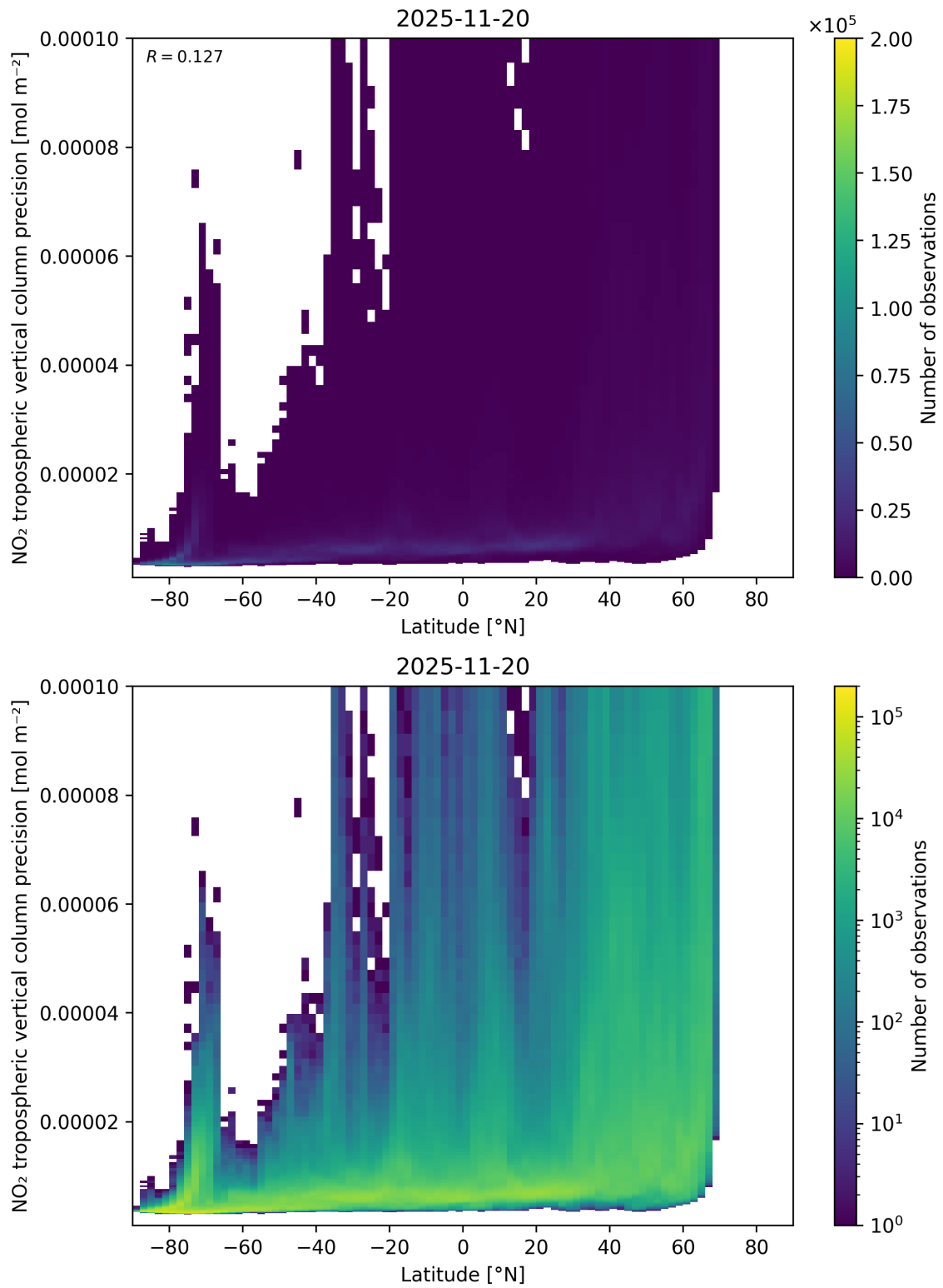
Figure 93: Scatter density plot of “Latitude” against “NO 2 tropospheric vertical column precision” for 2025-11-19 to 2025-11-21.
