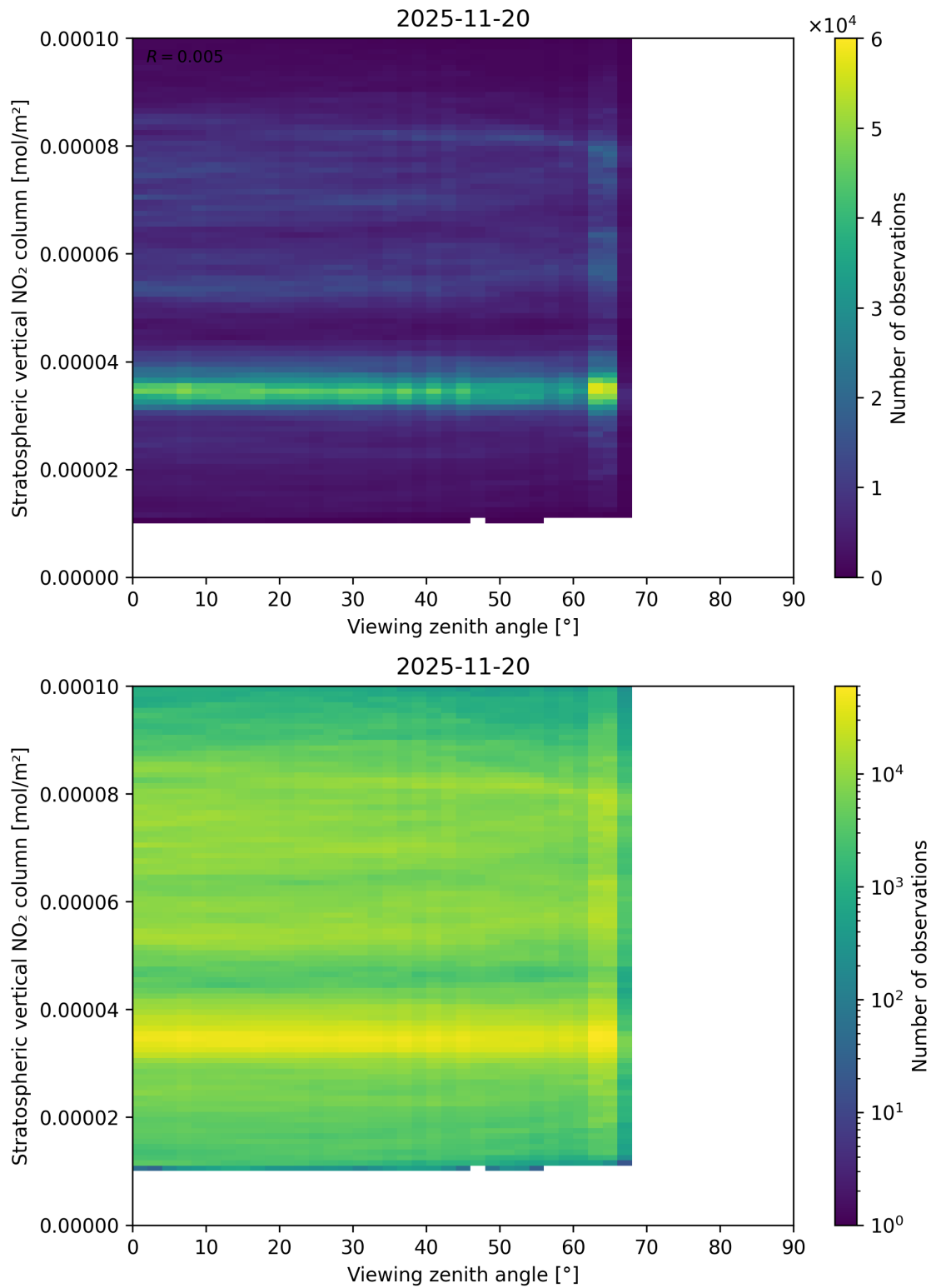
Figure 164: Scatter density plot of “Viewing zenith angle” against “Stratospheric vertical NO 2 column” for 2025-11-19 to 2025-11-21.
