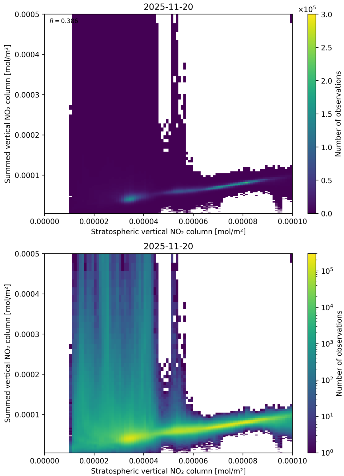
Figure 98: Scatter density plot of “Stratospheric vertical NO 2 column” against “Summed vertical NO 2 column” for 2025-11-19 to 2025-11-21.
