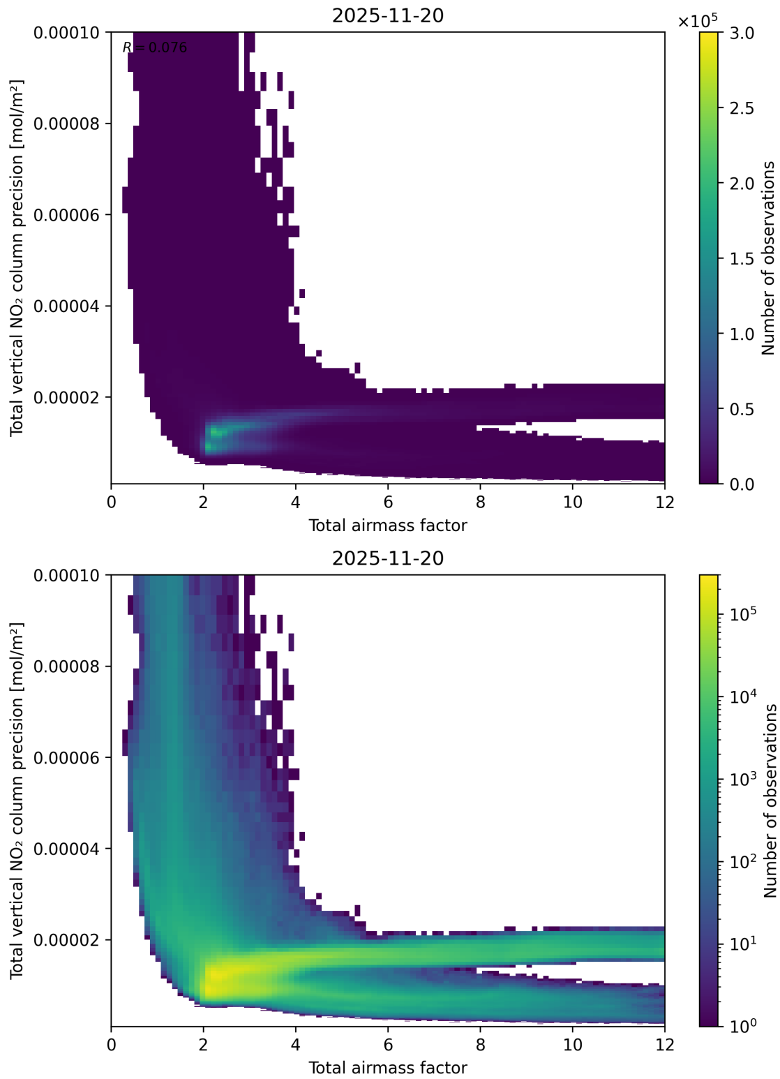
Figure 68: Scatter density plot of “Total airmass factor” against “Total vertical NO 2 column precision” for 2025-11-19 to 2025-11-21.
