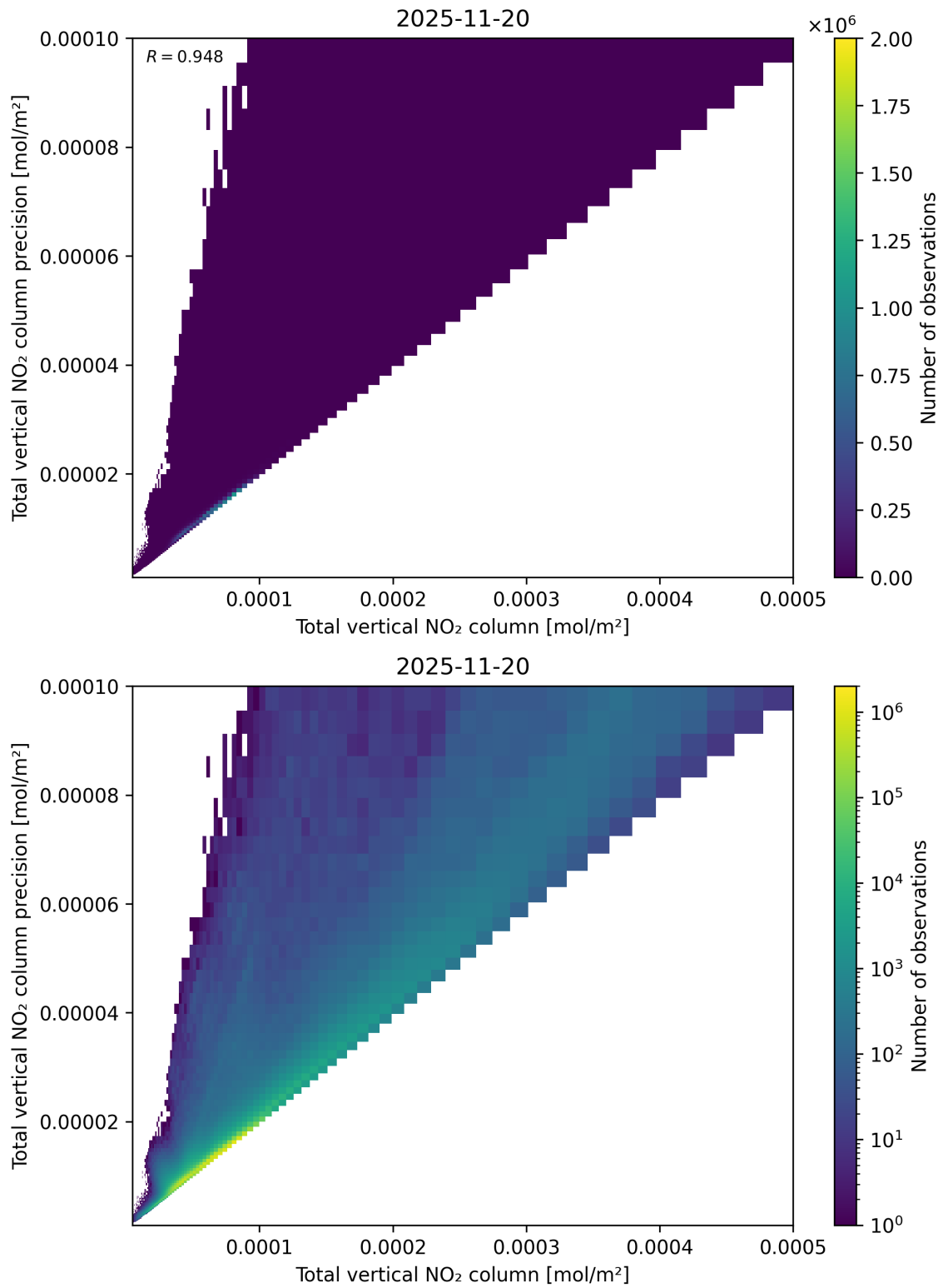
Figure 114: Scatter density plot of “Total vertical NO 2 column” against “Total vertical NO 2 column precision” for 2025-11-19 to 2025-11-21.
