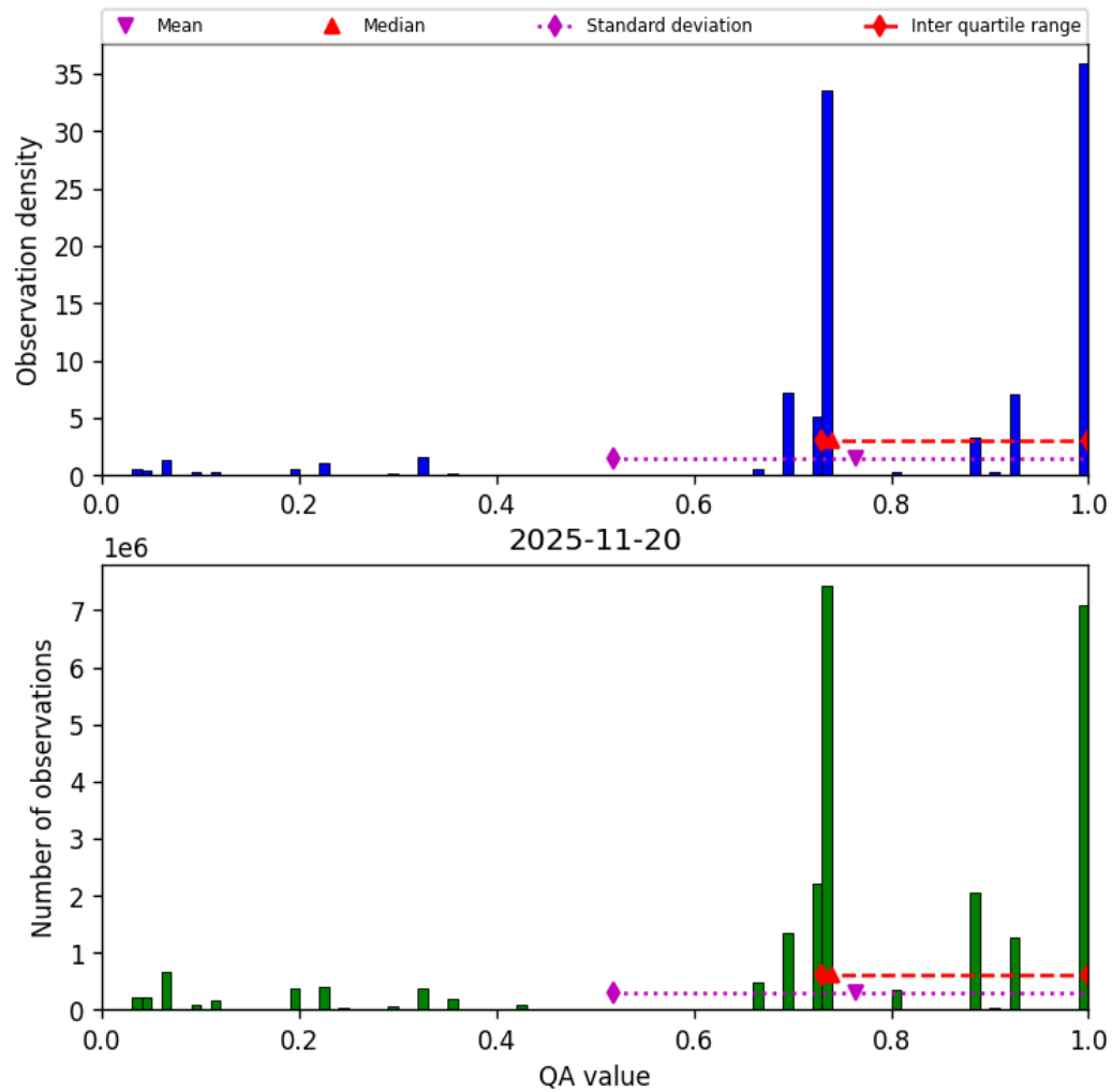
Figure 28: Histogram of “QA value” for 2025-11-19 to 2025-11-21
