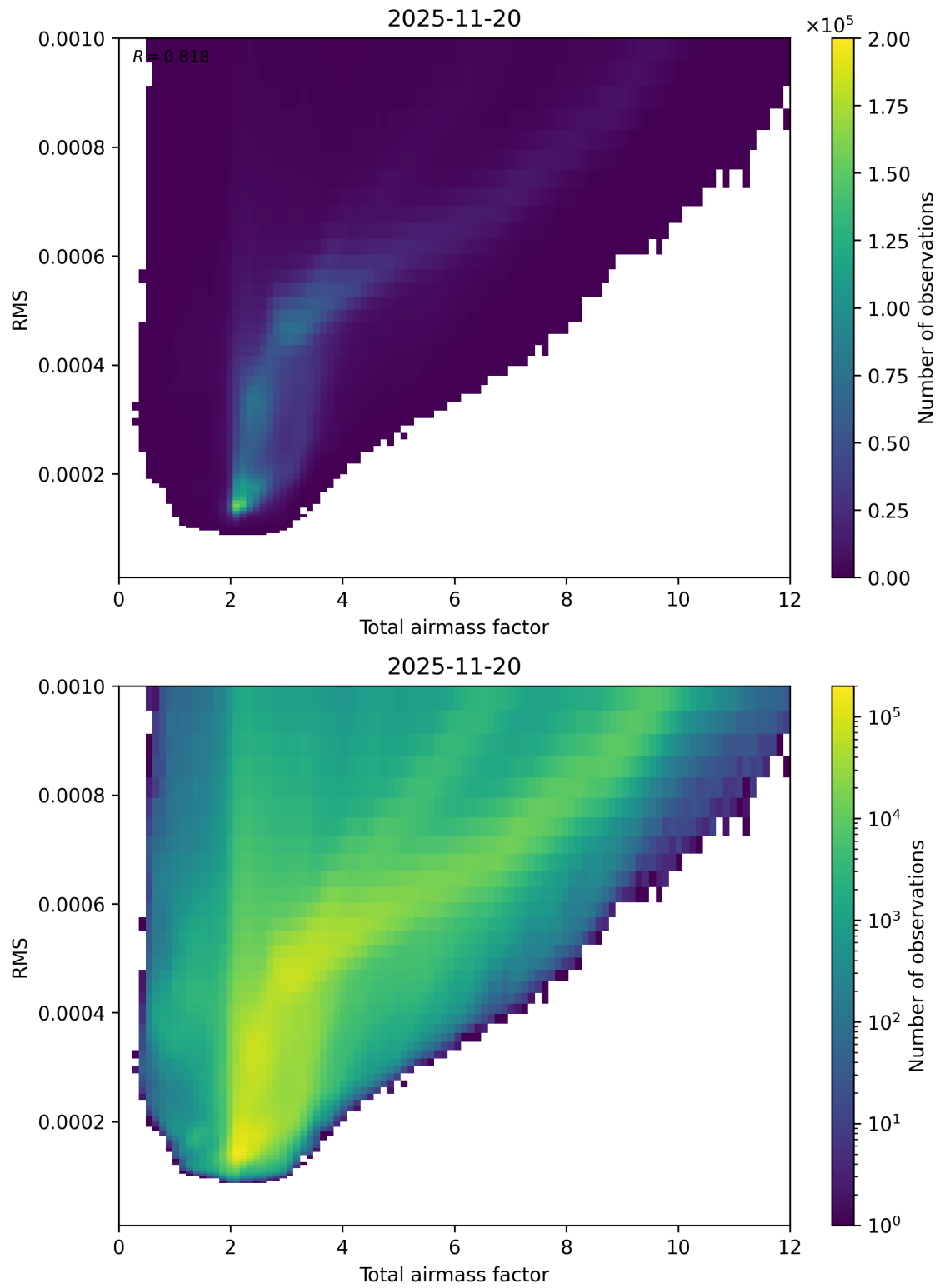
Figure 69: Scatter density plot of “Total airmass factor” against “RMS” for 2025-11-19 to 2025-11-21.
