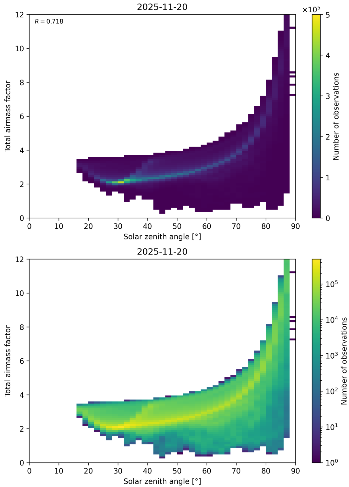
Figure 146: Scatter density plot of “Solar zenith angle” against “Total airmass factor” for 2025-11-19 to 2025-11-21.
