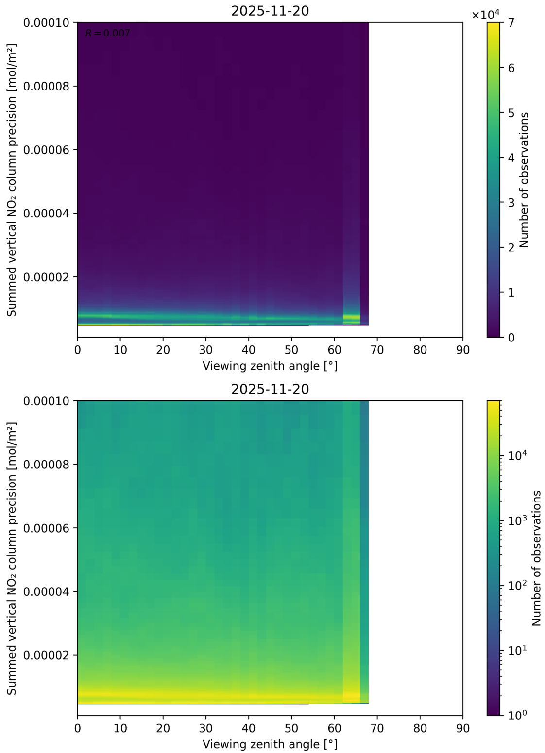
Figure 166: Scatter density plot of “Viewing zenith angle” against “Summed vertical NO 2 column precision” for 2025-11-19 to 2025-11-21.
