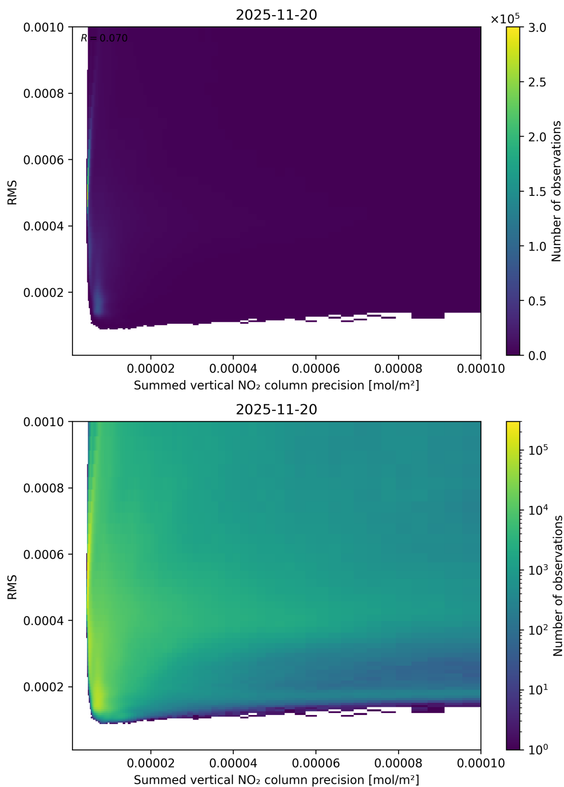
Figure 108: Scatter density plot of “Summed vertical NO 2 column precision” against “RMS” for 2025-11-19 to 2025-11-21.
