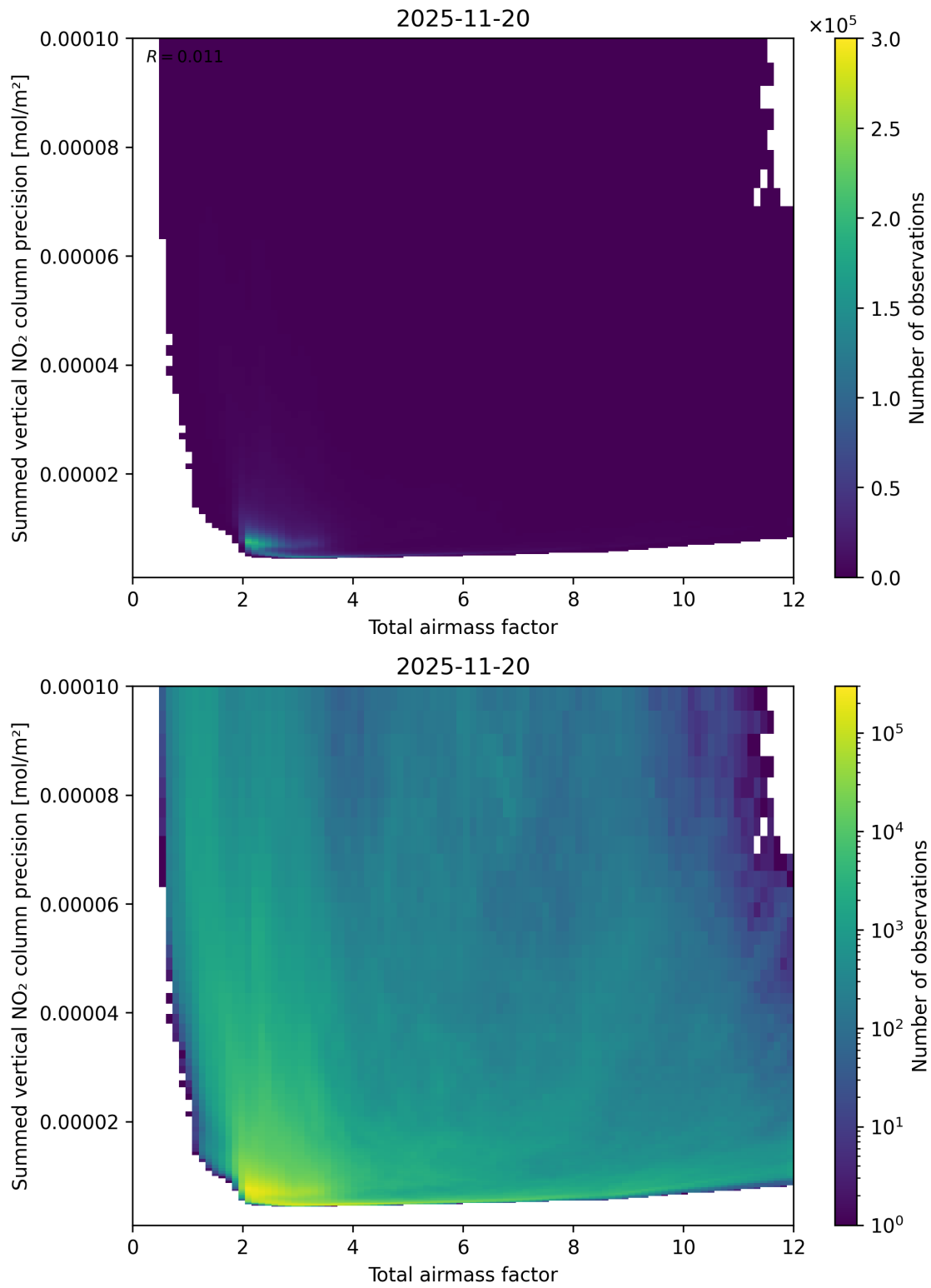
Figure 66: Scatter density plot of “Total airmass factor” against “Summed vertical NO 2 column precision” for 2025-11-19 to 2025-11-21.
