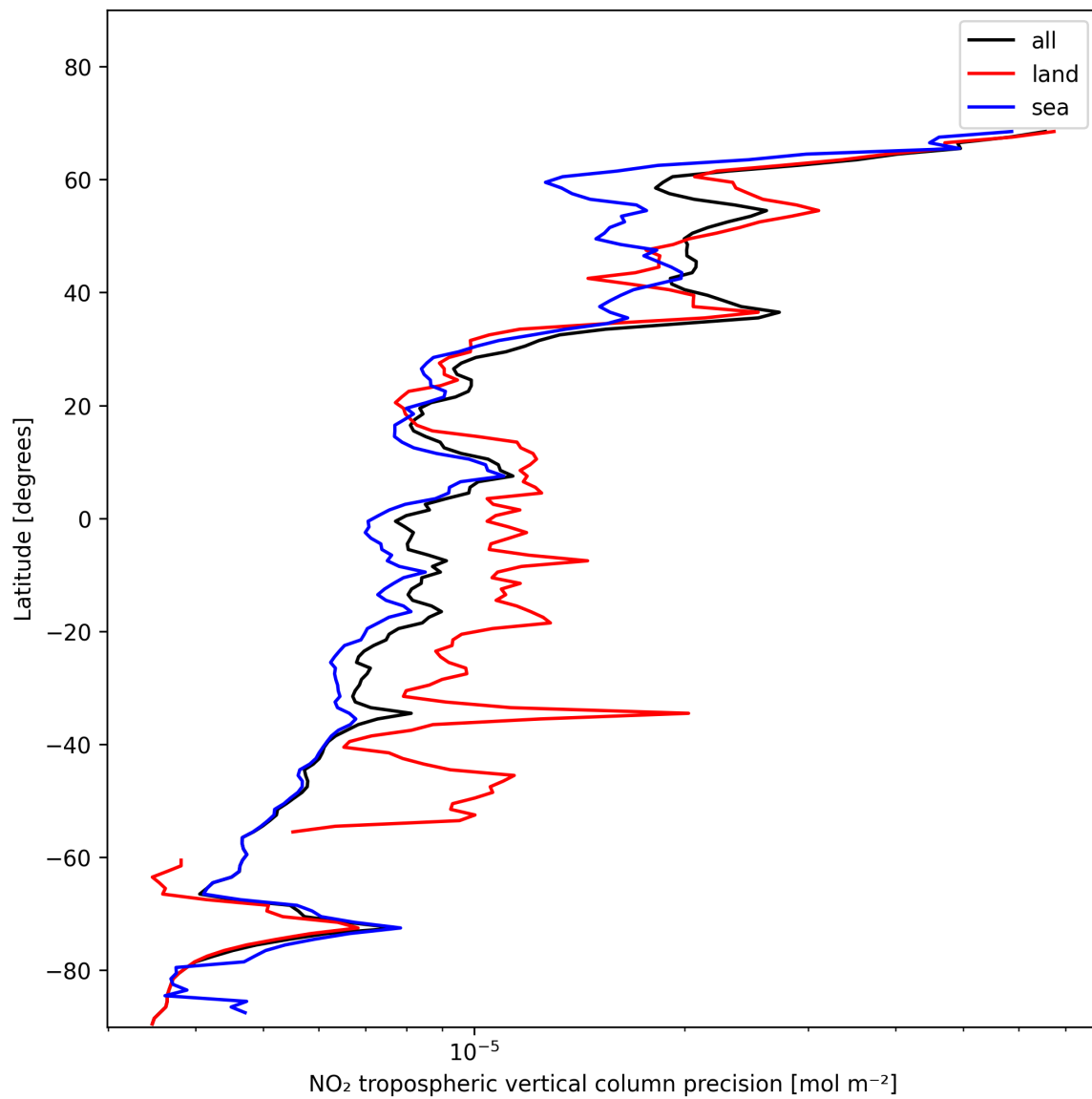
Figure 13: Zonal average of “NO 2 tropospheric vertical column precision” for 2025-11-19 to 2025-11-21.
