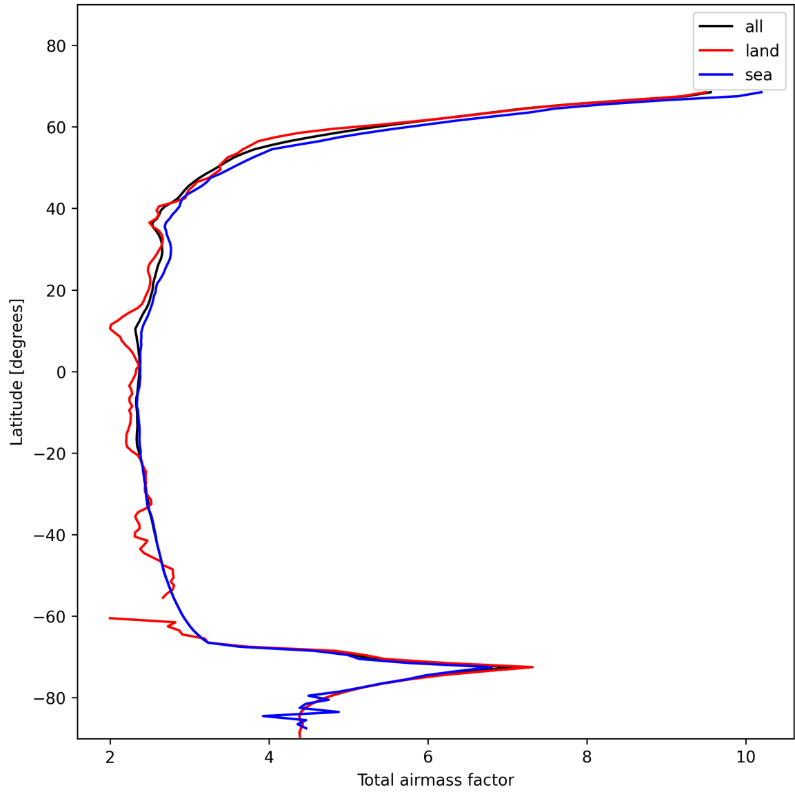
Figure 15: Zonal average of “Total airmass factor” for 2025-11-19 to 2025-11-21.
