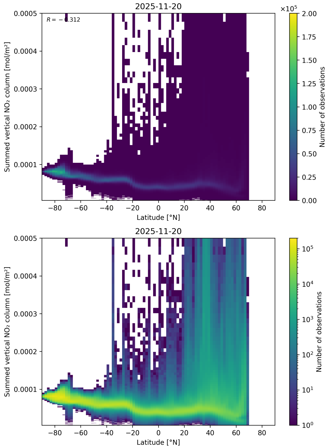
Figure 88: Scatter density plot of “Latitude” against “Summed vertical NO 2 column” for 2025-11-19 to 2025-11-21.
