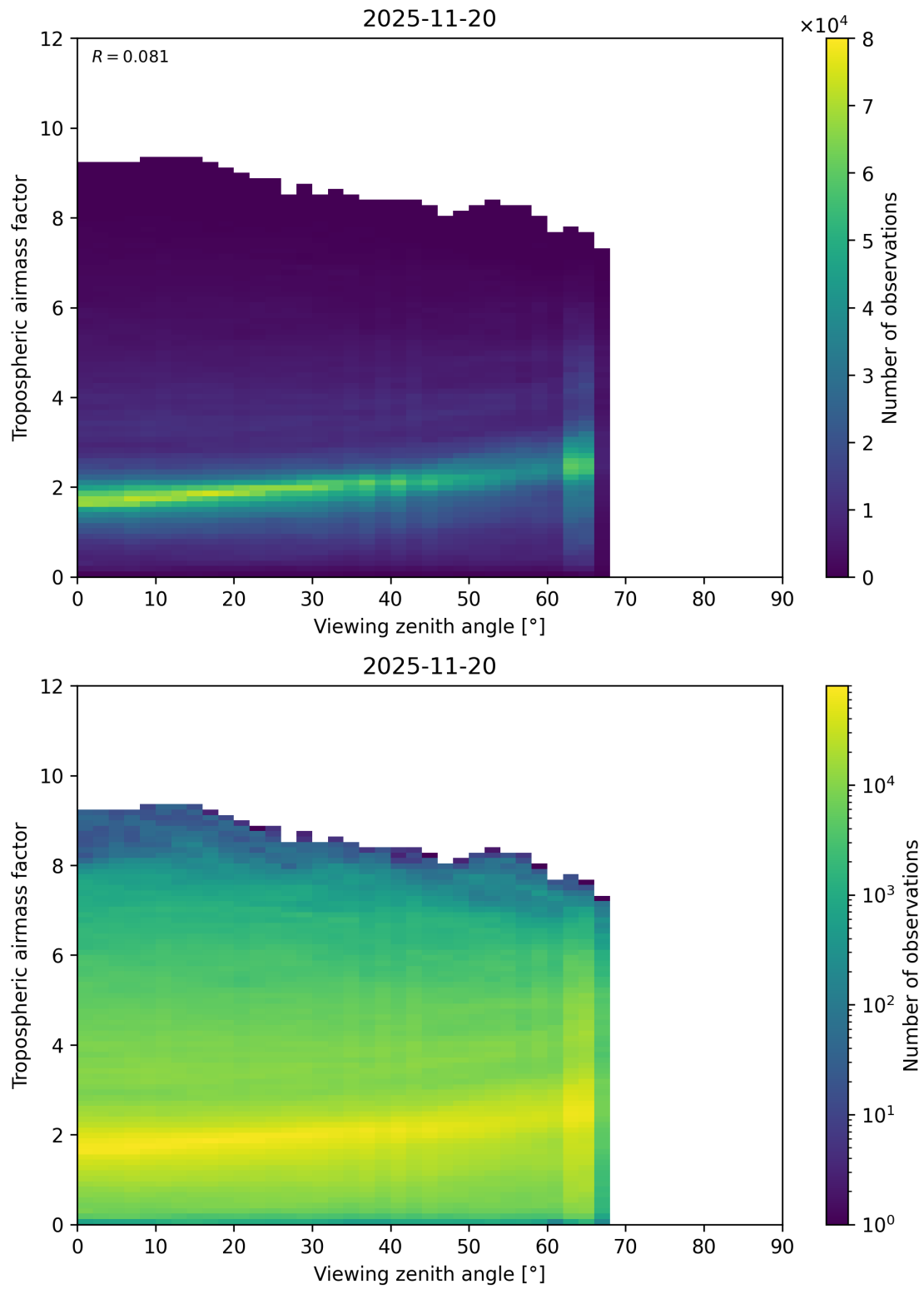
Figure 161: Scatter density plot of “Viewing zenith angle” against “Tropospheric airmass factor” for 2025-11-19 to 2025-11-21.
