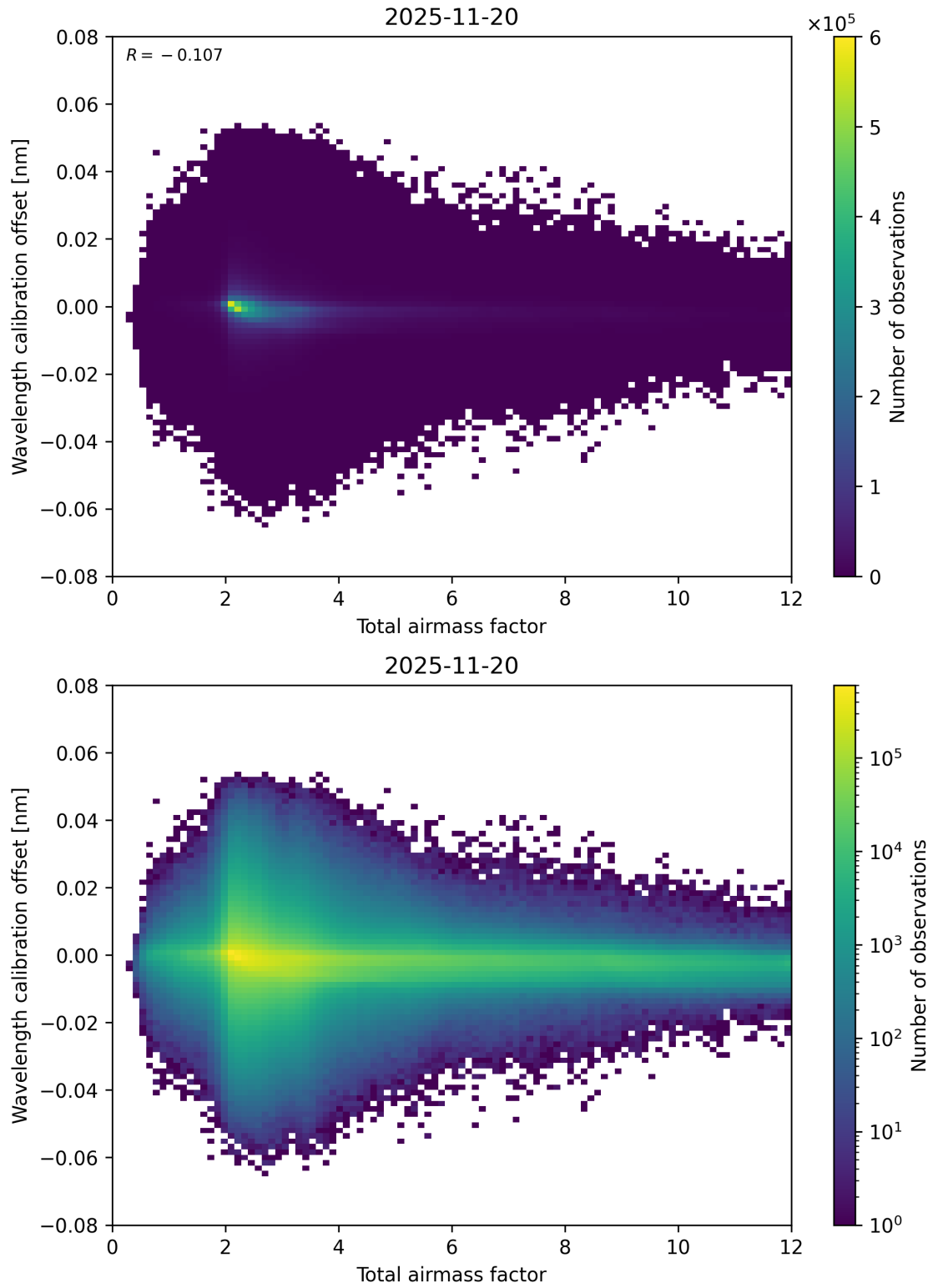
Figure 70: Scatter density plot of “Total airmass factor” against “Wavelength calibration offset” for 2025-11-19 to 2025-11-21.
