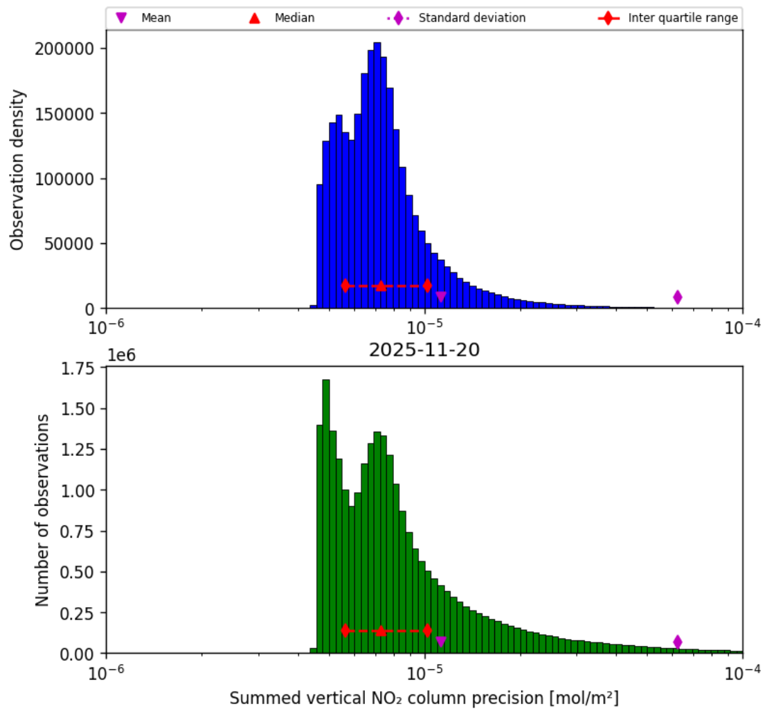
Figure 41: Histogram of "Summed vertical NO 2 column precision" for 2025-11-19 to 2025-11-21
