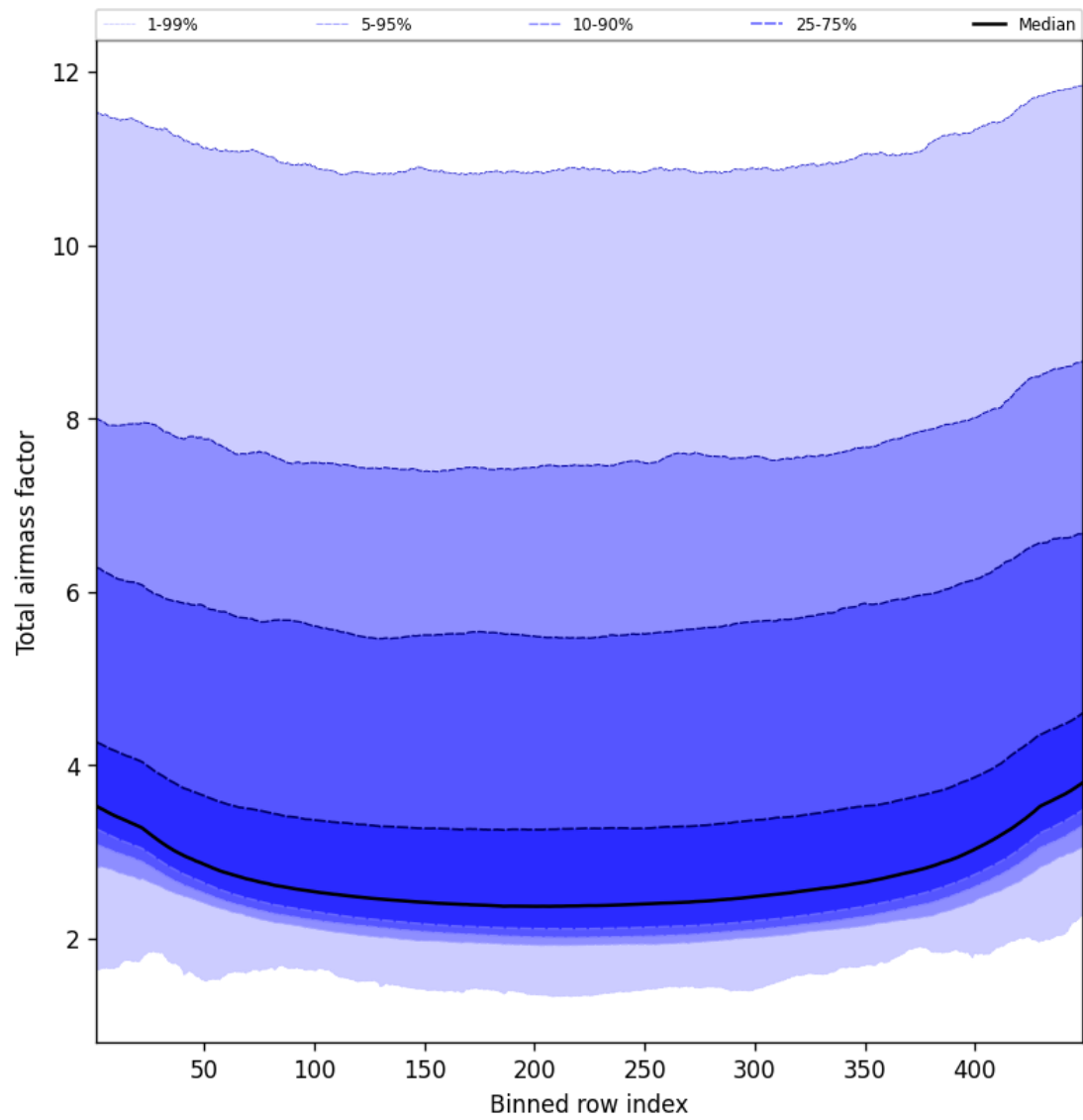
Figure 49: Along track statistics of “Total airmass factor” for 2025-11-19 to 2025-11-21
