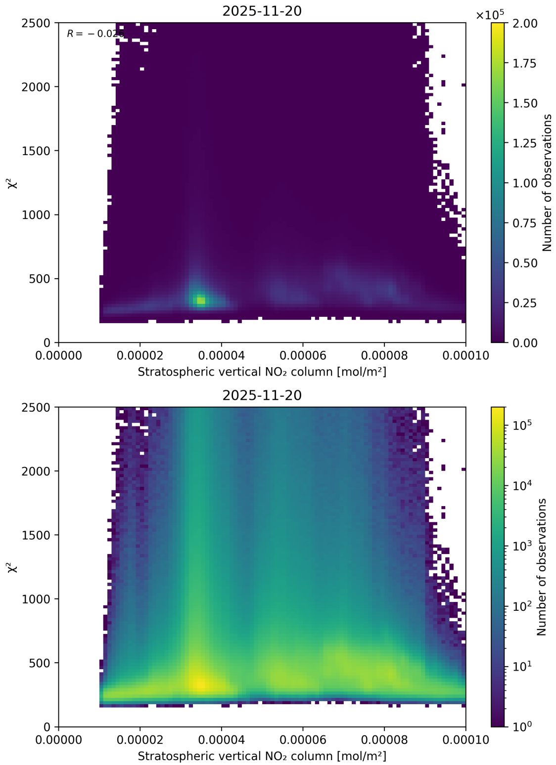
Figure 97: Scatter density plot of “Stratospheric vertical NO 2 column” against “ \chi^2 ” for 2025-11-19 to 2025-11-21.
