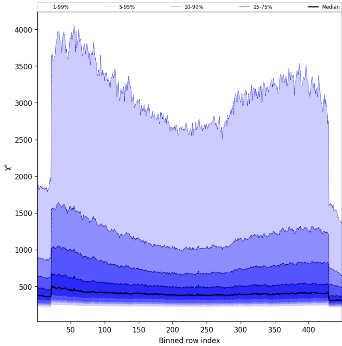
Figure 59: Along track statistics of “ \chi^2 ” for 2025-11-19 to 2025-11-21
