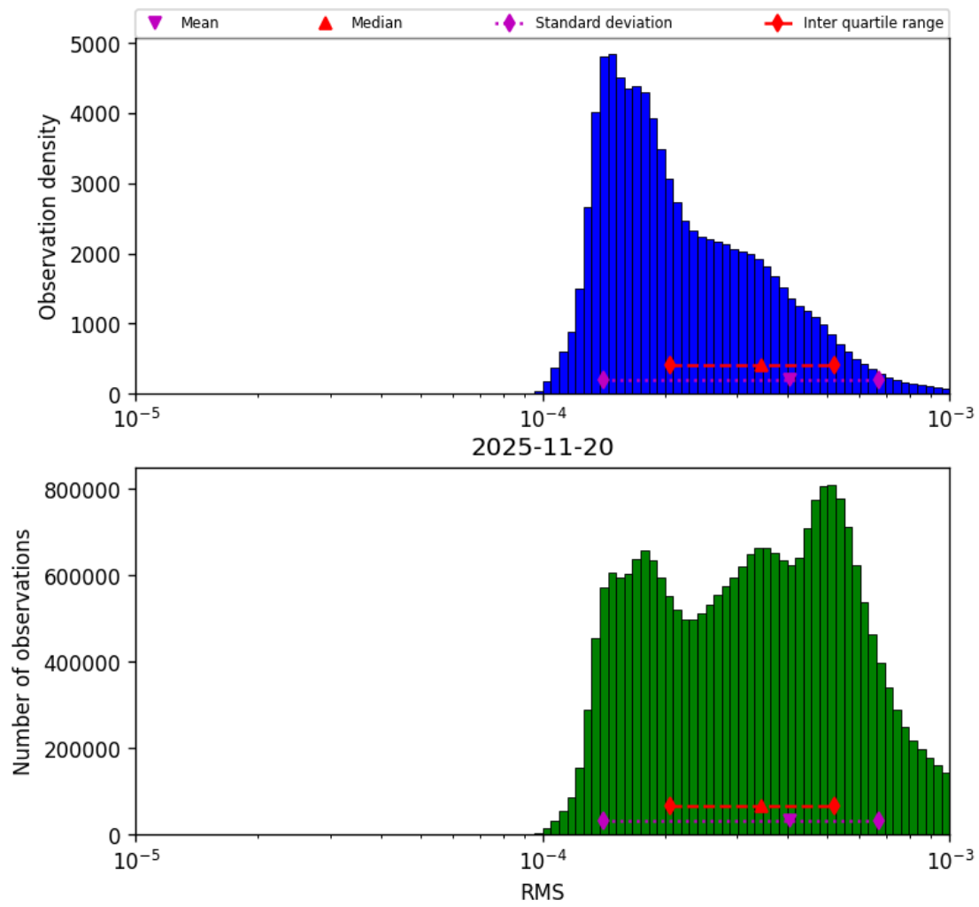
Figure 43: Histogram of “RMS” for 2025-11-19 to 2025-11-21
