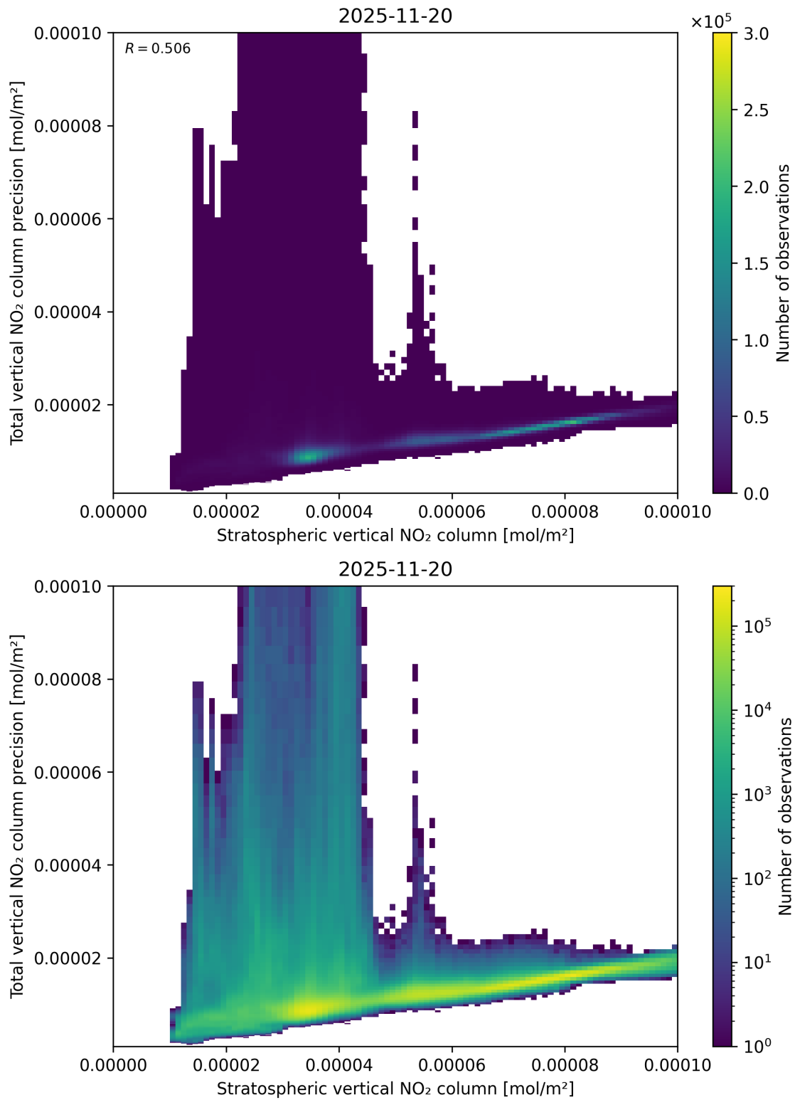
Figure 101: Scatter density plot of “Stratospheric vertical NO 2 column” against “Total vertical NO 2 column precision” for 2025-11-19 to 2025-11-21.
