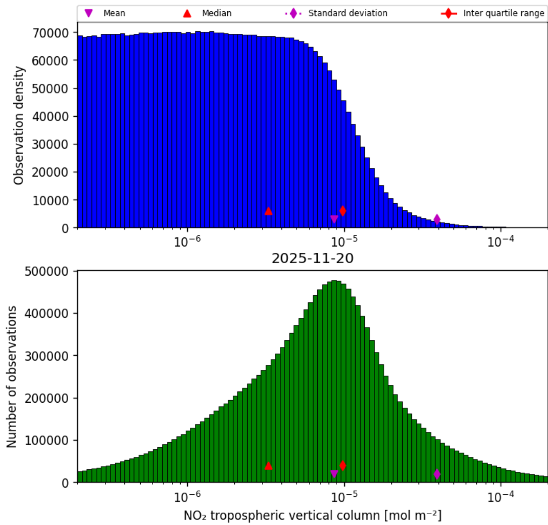
Figure 29: Histogram of “NO 2 tropospheric vertical column” for 2025-11-19 to 2025-11-21
