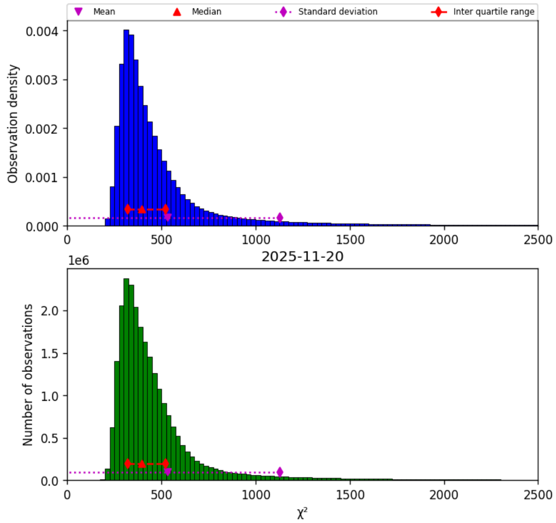
Figure 42: Histogram of “ \chi^2 ” for 2025-11-19 to 2025-11-21
