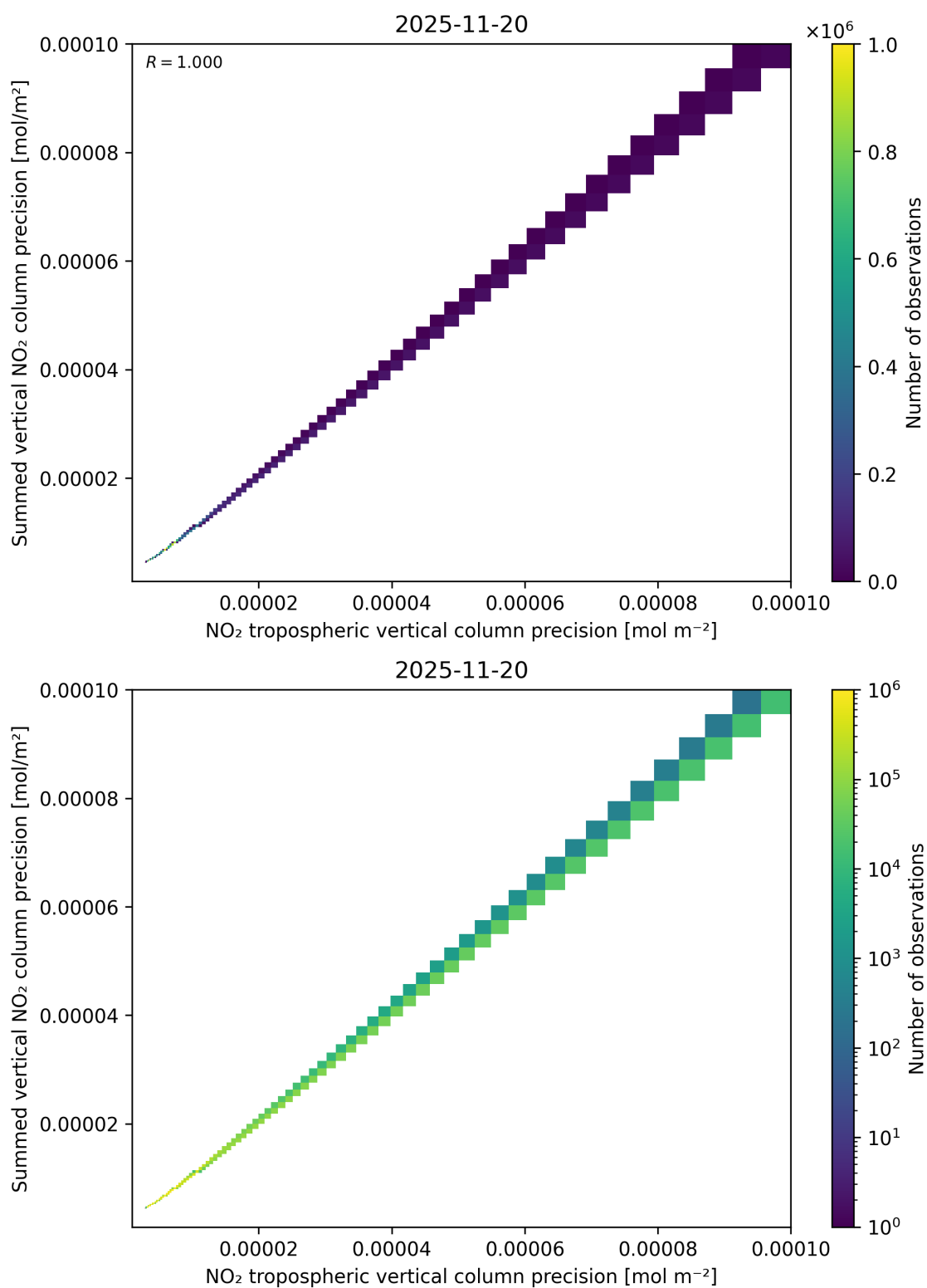
Figure 137: Scatter density plot of “NO 2 tropospheric vertical column precision” against “Summed vertical NO 2 column precision” for 2025-11-19 to 2025-11-21.
