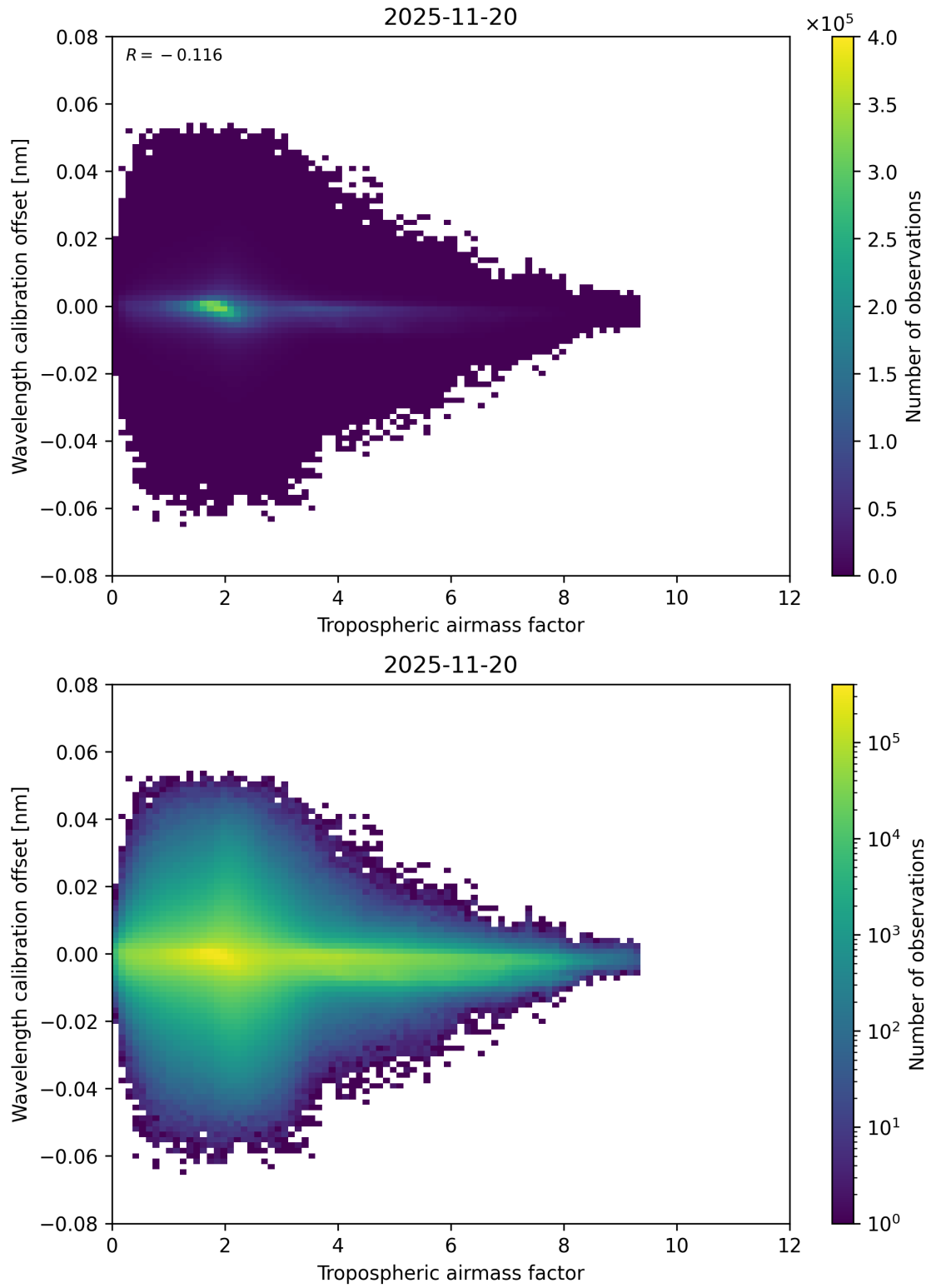
Figure 80: Scatter density plot of “Tropospheric airmass factor” against “Wavelength calibration offset” for 2025-11-19 to 2025-11-21.
