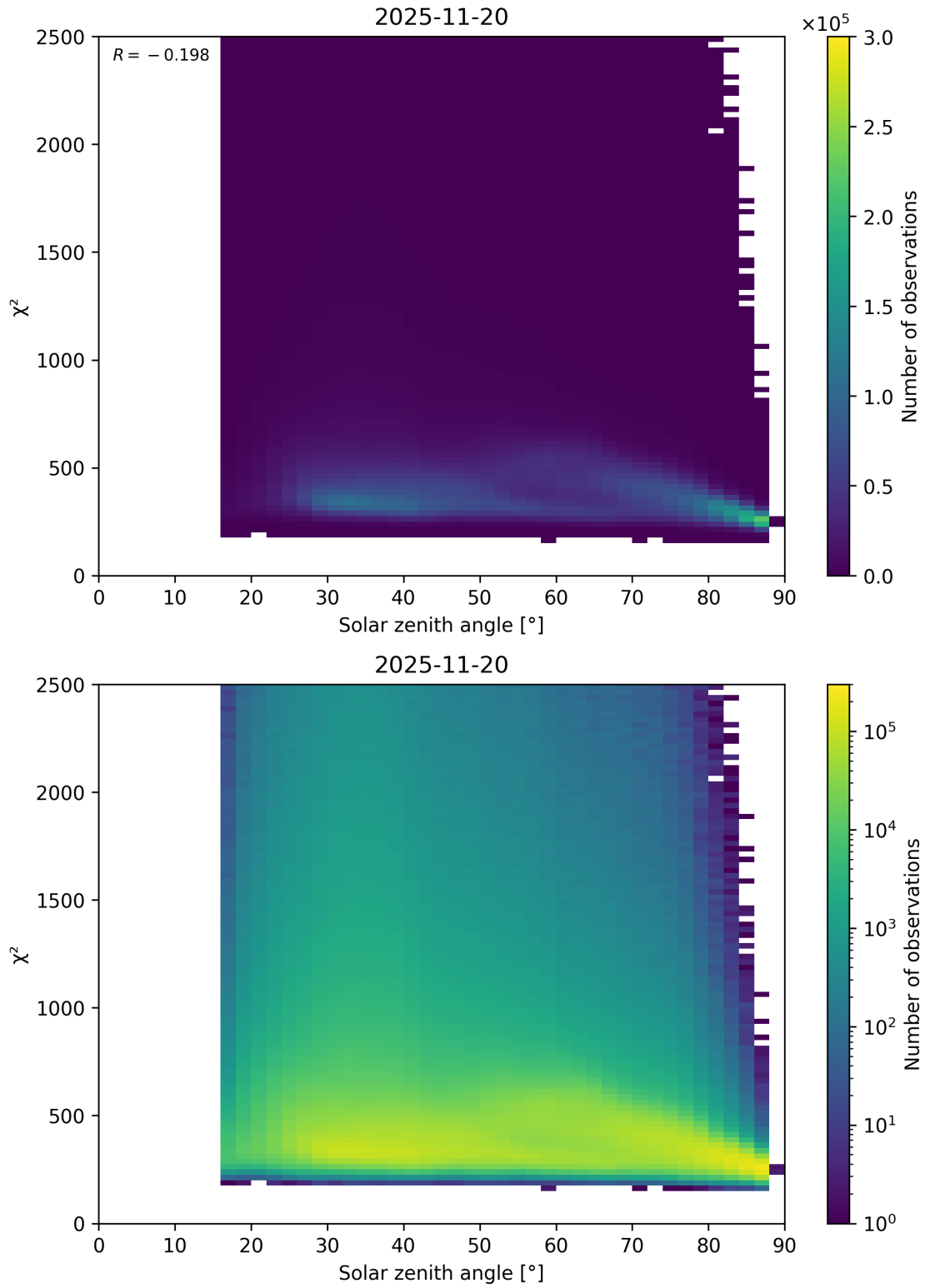
Figure 148: Scatter density plot of “Solar zenith angle” against “ \chi^2 ” for 2025-11-19 to 2025-11-21.
