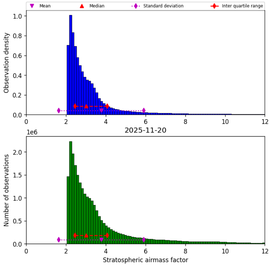
Figure 44: Histogram of “Stratospheric airmass factor” for 2025-11-19 to 2025-11-21
