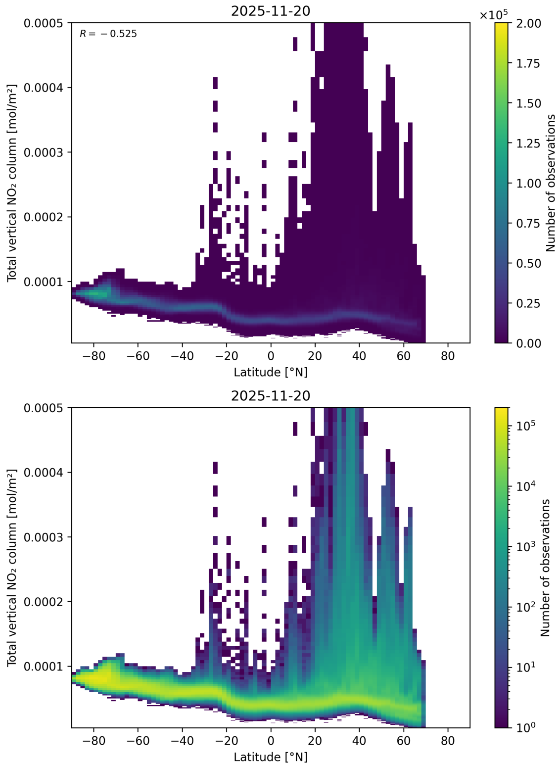
Figure 90: Scatter density plot of “Latitude” against “Total vertical NO 2 column” for 2025-11-19 to 2025-11-21.
