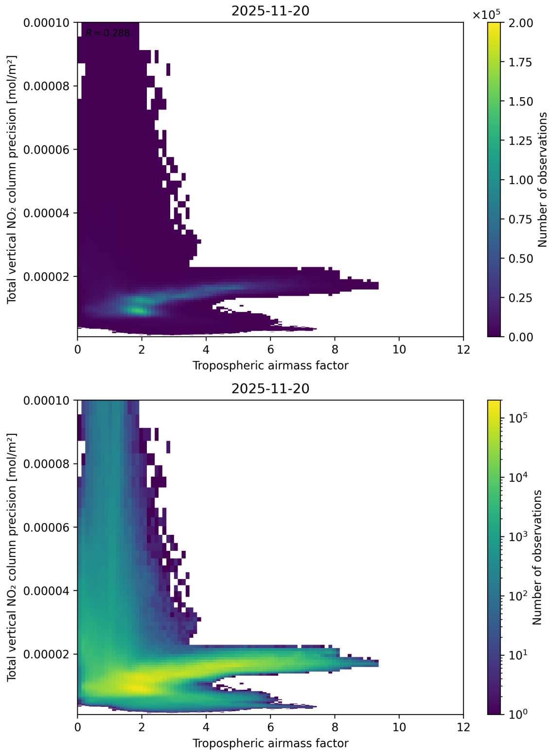
Figure 78: Scatter density plot of “Tropospheric air mass factor” against “Total vertical NO 2 column precision” for 2025-11-19 to 2025-11-21.
