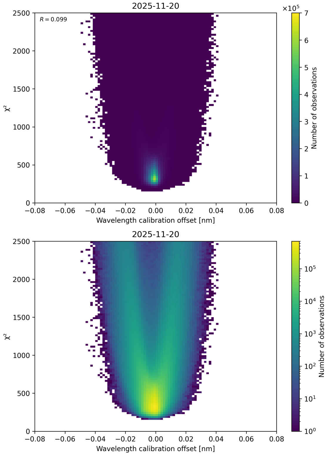
Figure 175: Scatter density plot of “Wavelength calibration offset” against “ \chi^2 ” for 2025-11-19 to 2025-11-21.
