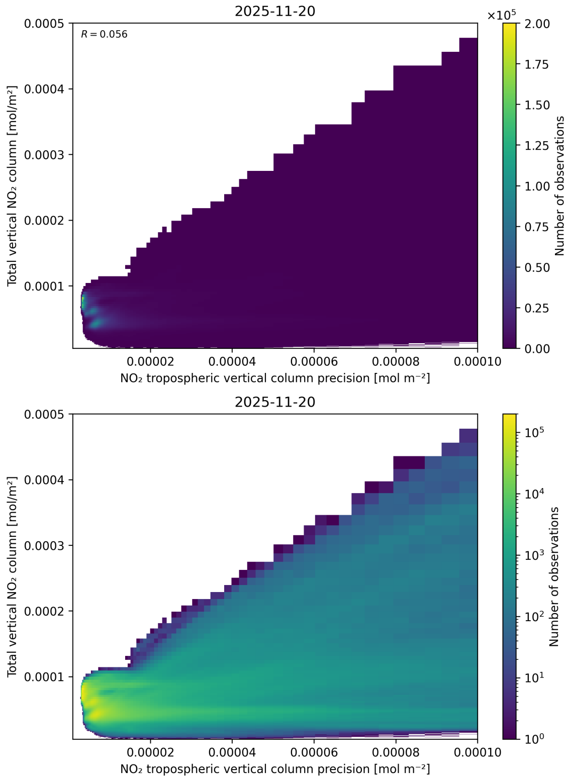
Figure 138: Scatter density plot of “NO 2 tropospheric vertical column precision” against “Total vertical NO 2 column” for 2025-11-19 to 2025-11-21.
