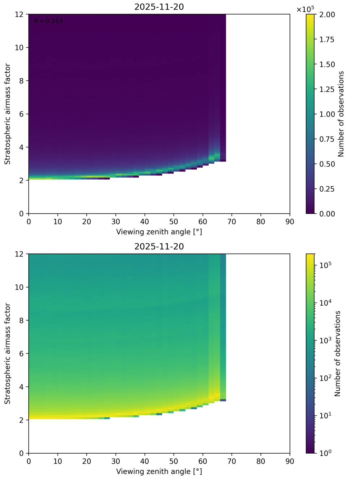
Figure 159: Scatter density plot of “Viewing zenith angle” against “Stratospheric airmass factor” for 2025-11-19 to 2025-11-21.
