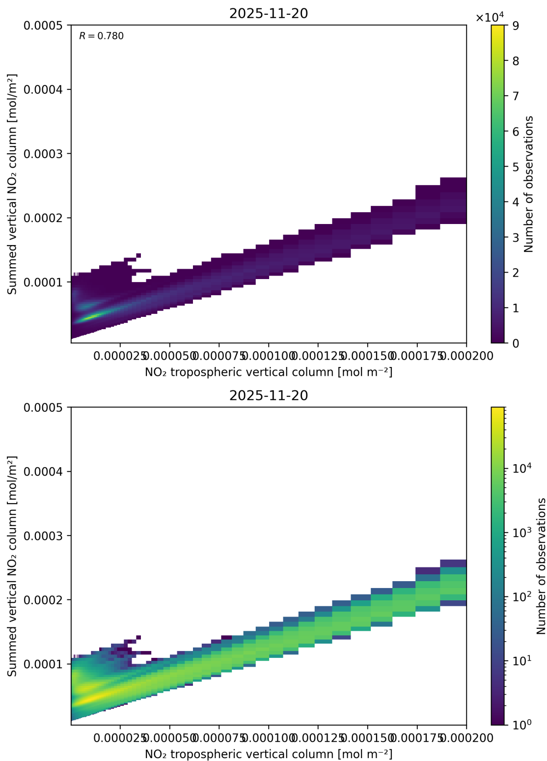
Figure 126: Scatter density plot of “NO 2 tropospheric vertical column” against “Summed vertical NO 2 column” for 2025-11-19 to 2025-11-21.
