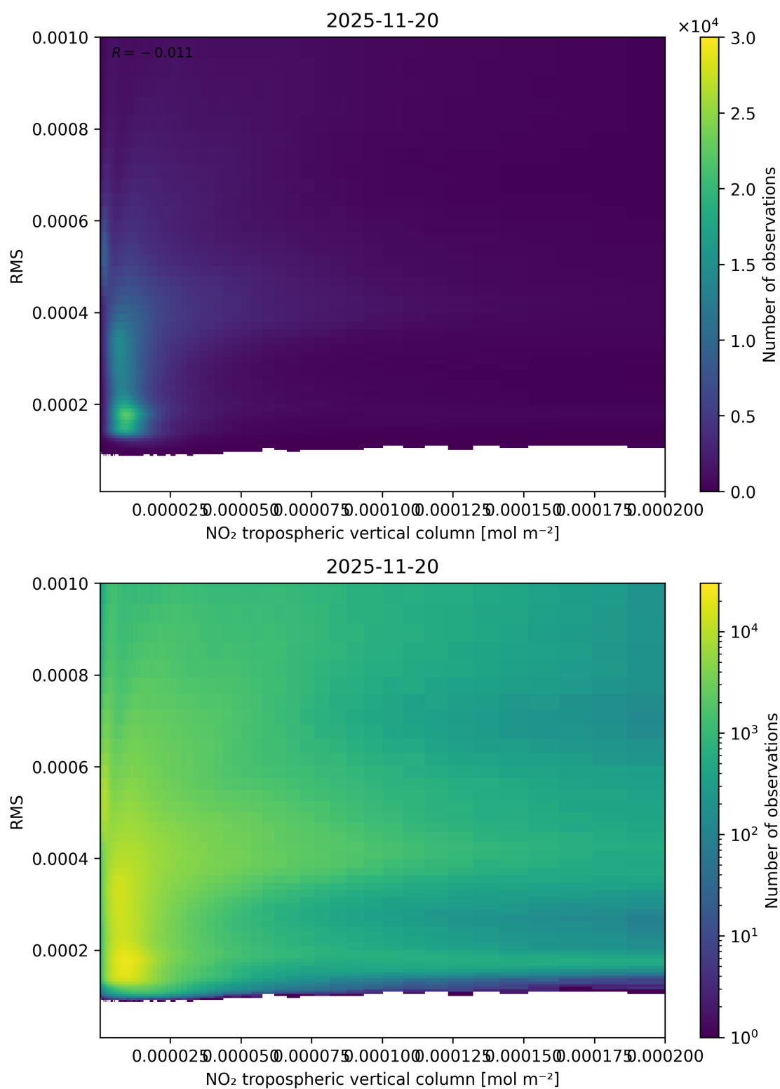
Figure 142: Scatter density plot of “NO 2 tropospheric vertical column” against “RMS” for 2025-11-19 to 2025-11-21.
