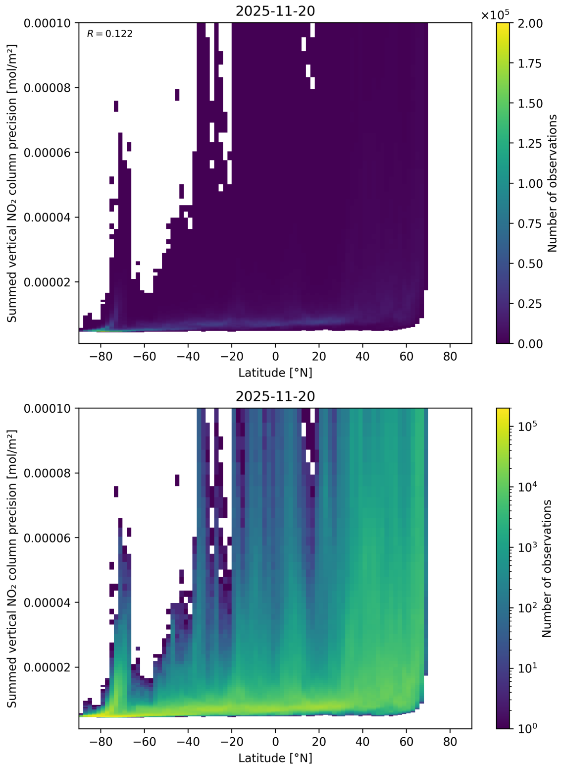
Figure 89: Scatter density plot of “Latitude” against “Summed vertical NO 2 column precision” for 2025-11-19 to 2025-11-21.
