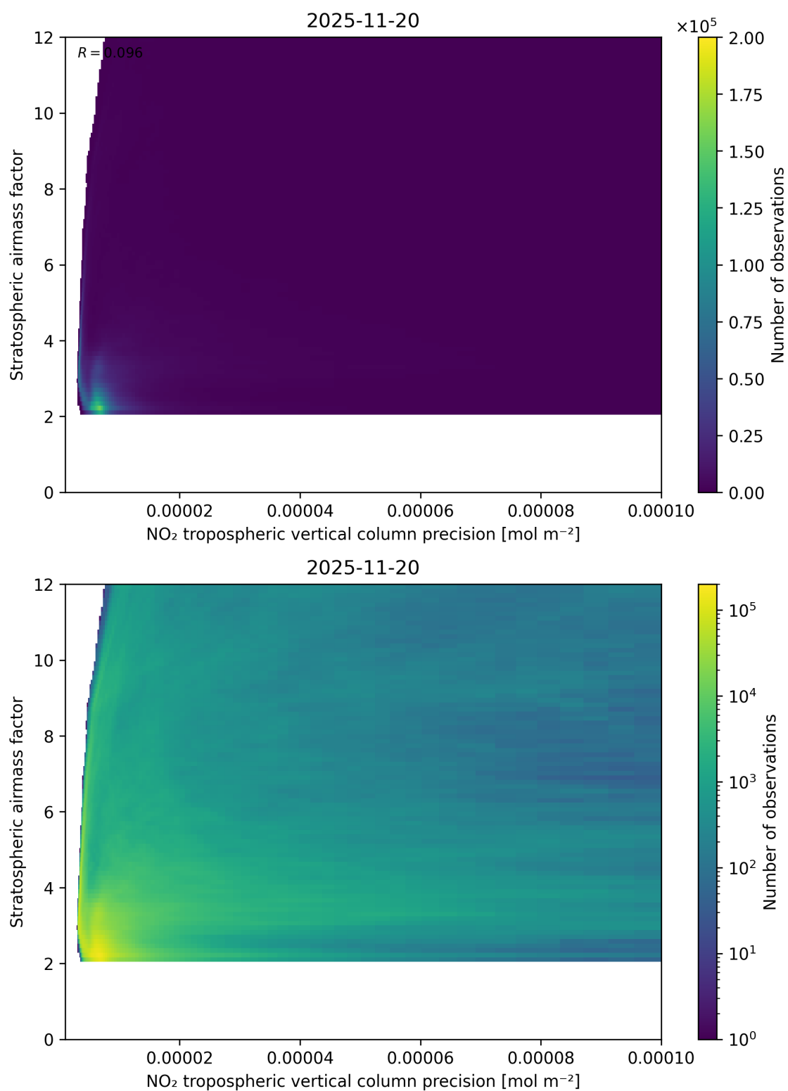
Figure 131: Scatter density plot of “NO 2 tropospheric vertical column precision” against “Stratospheric airmass factor” for 2025-11-19 to 2025-11-21.
