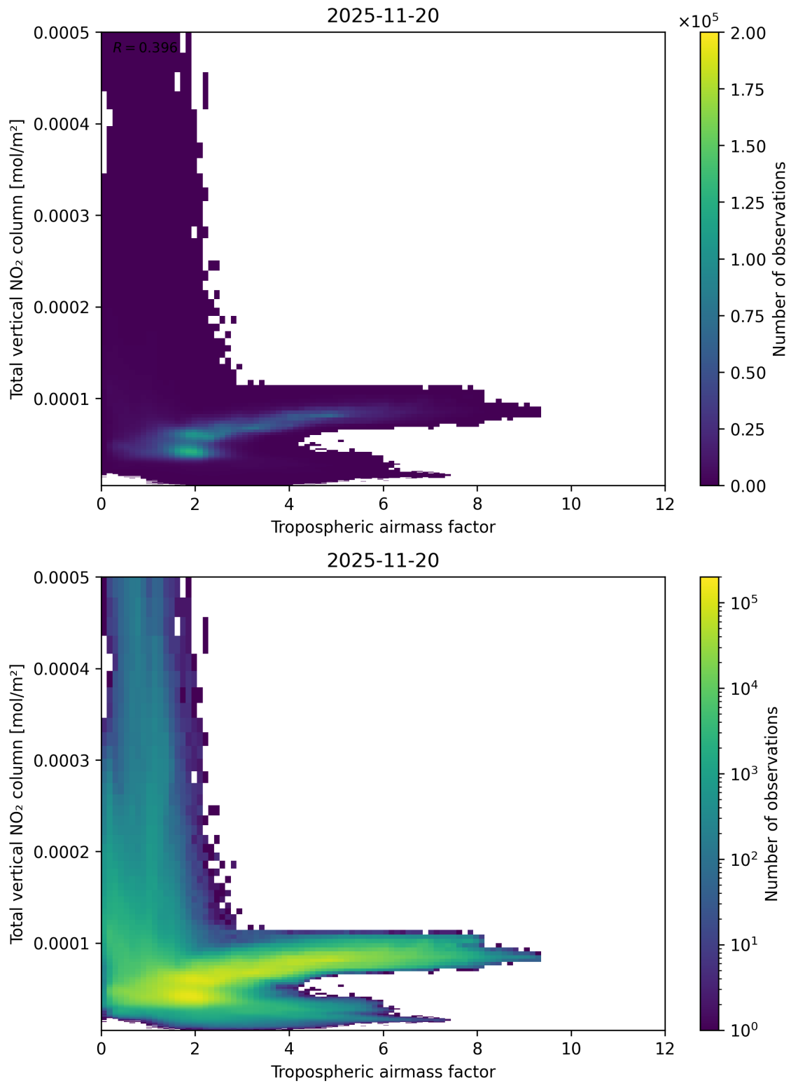
Figure 77: Scatter density plot of “Tropospheric airmass factor” against “Total vertical NO 2 column” for 2025-11-19 to 2025-11-21.
