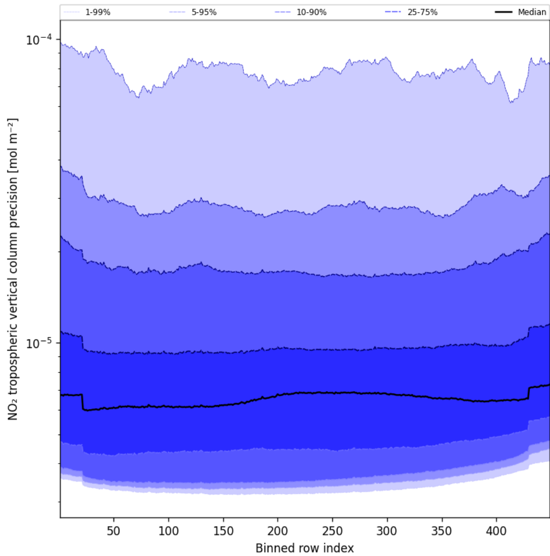
Figure 47: Along track statistics of “NO 2 tropospheric vertical column precision” for 2025-11-19 to 2025-11-21
