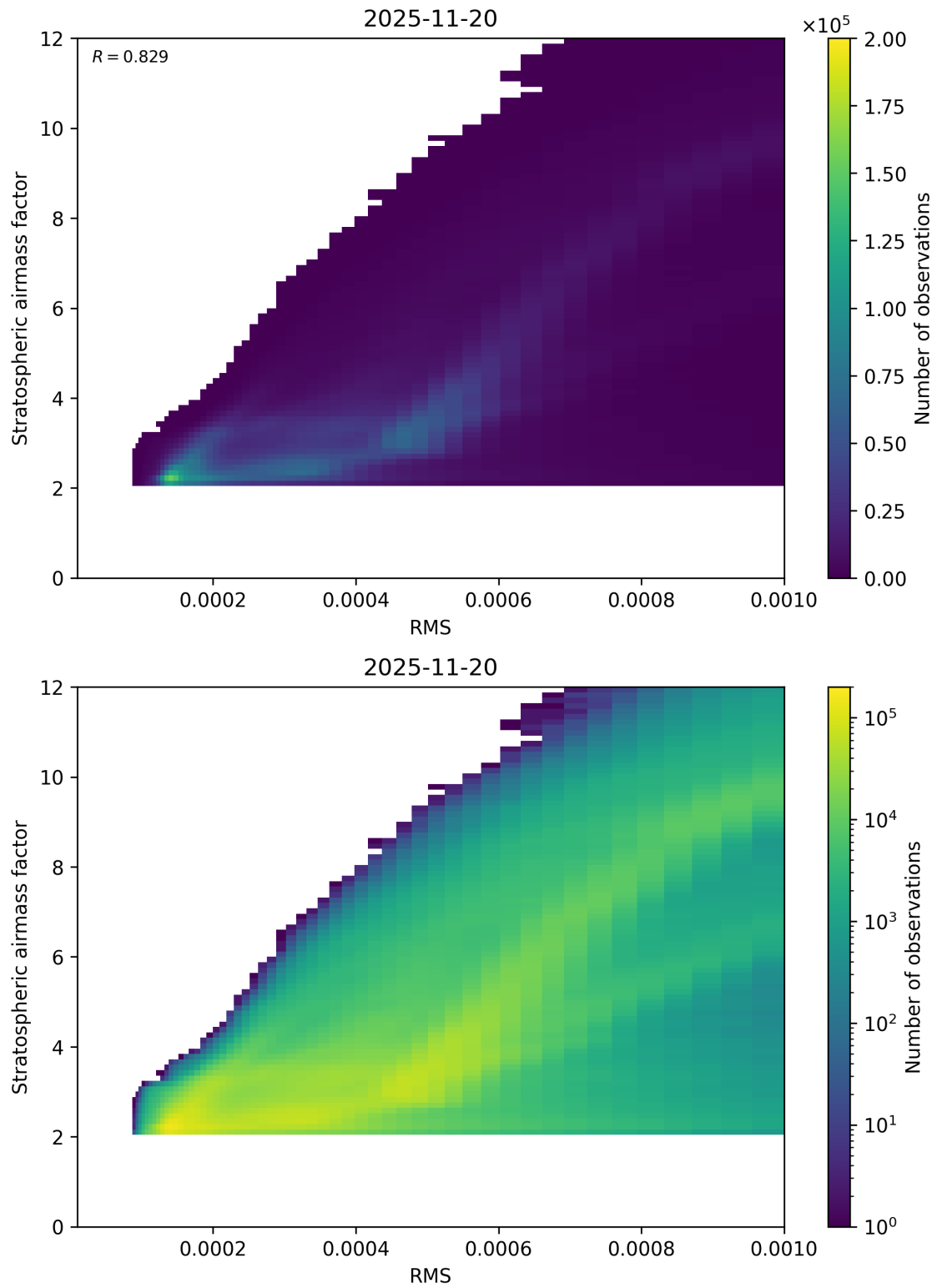
Figure 144: Scatter density plot of “RMS” against “Stratospheric airmass factor” for 2025-11-19 to 2025-11-21.
