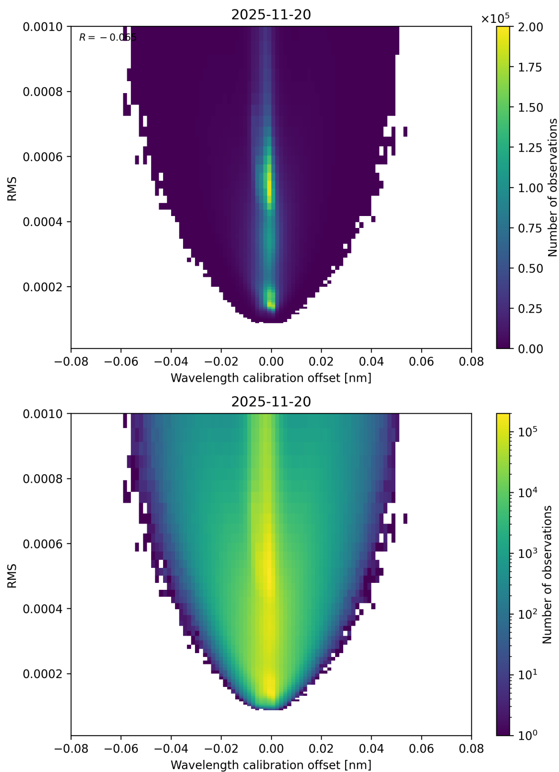
Figure 181: Scatter density plot of “Wavelength calibration offset” against “RMS” for 2025-11-19 to 2025-11-21.
