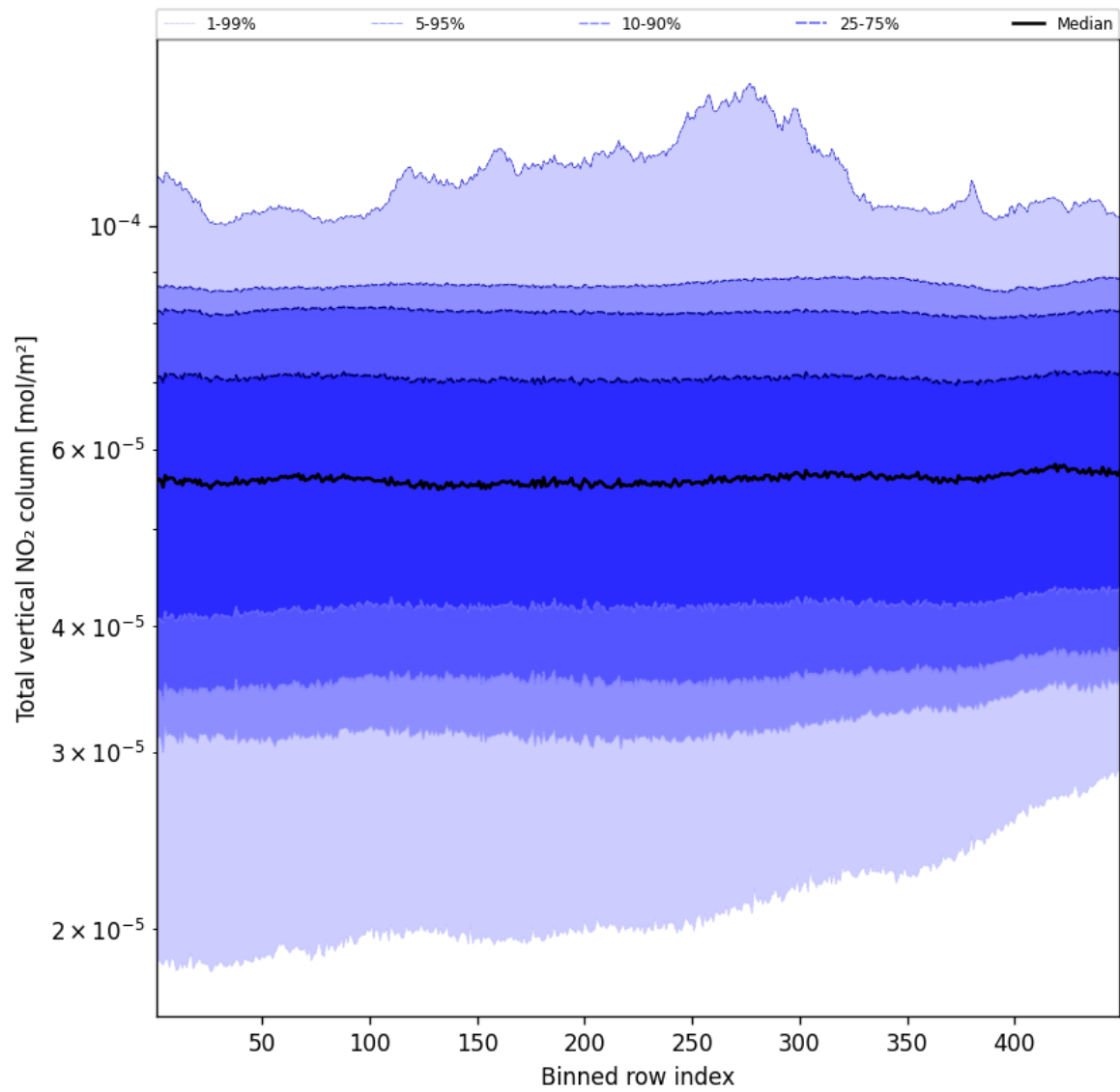
Figure 55: Along track statistics of “Total vertical NO 2 column” for 2025-11-19 to 2025-11-21
