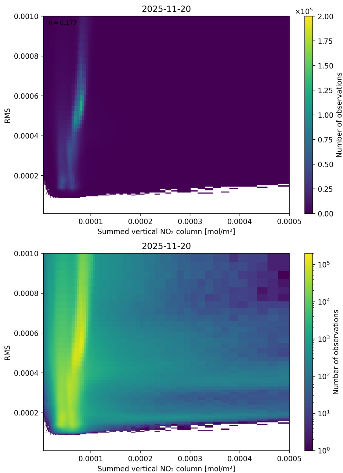
Figure 109: Scatter density plot of “Summed vertical NO 2 column” against “RMS” for 2025-11-19 to 2025-11-21.
