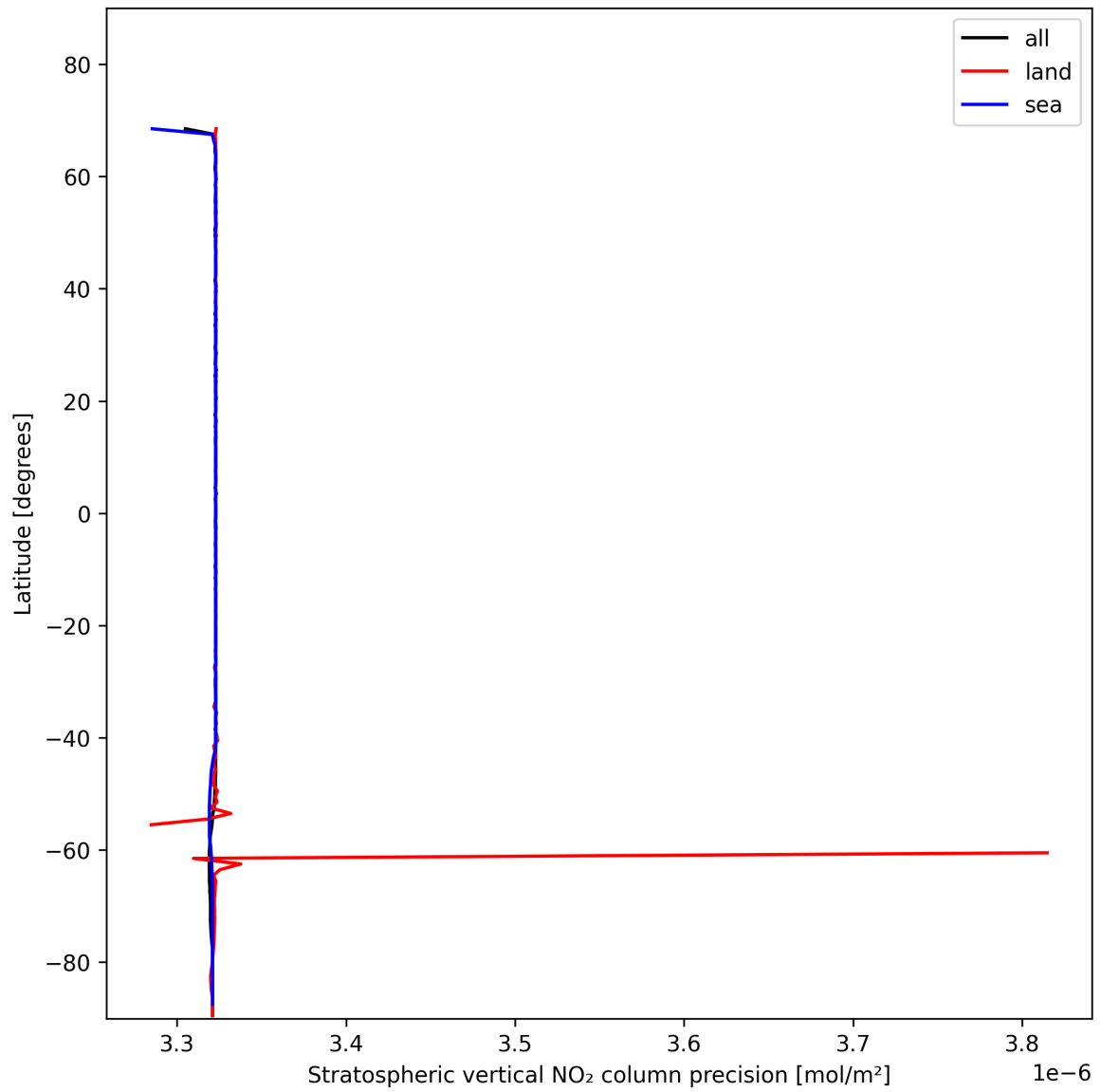
Figure 20: Zonal average of “Stratospheric vertical NO 2 column precision” for 2025-11-19 to 2025-11-21.
