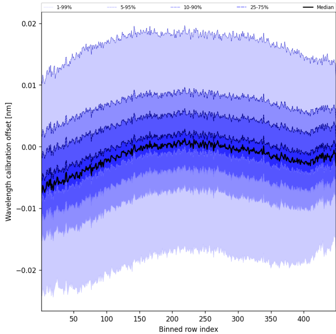
Figure 52: Along track statistics of “Wavelength calibration offset” for 2025-11-19 to 2025-11-21
