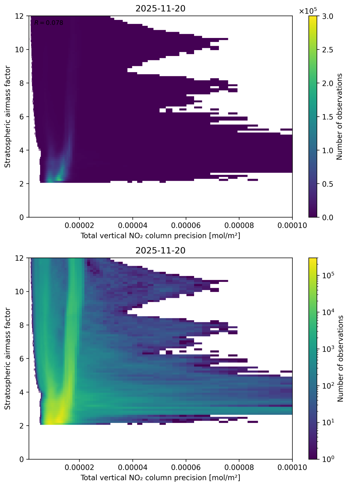
Figure 115: Scatter density plot of “Total vertical NO 2 column precision” against “Stratospheric air mass factor” for 2025-11-19 to 2025-11-21.
