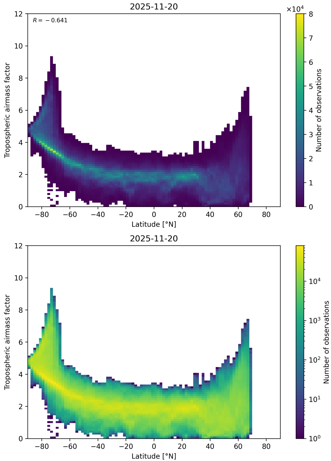
Figure 85: Scatter density plot of “Latitude” against “Tropospheric airmass factor” for 2025-11-19 to 2025-11-21.
