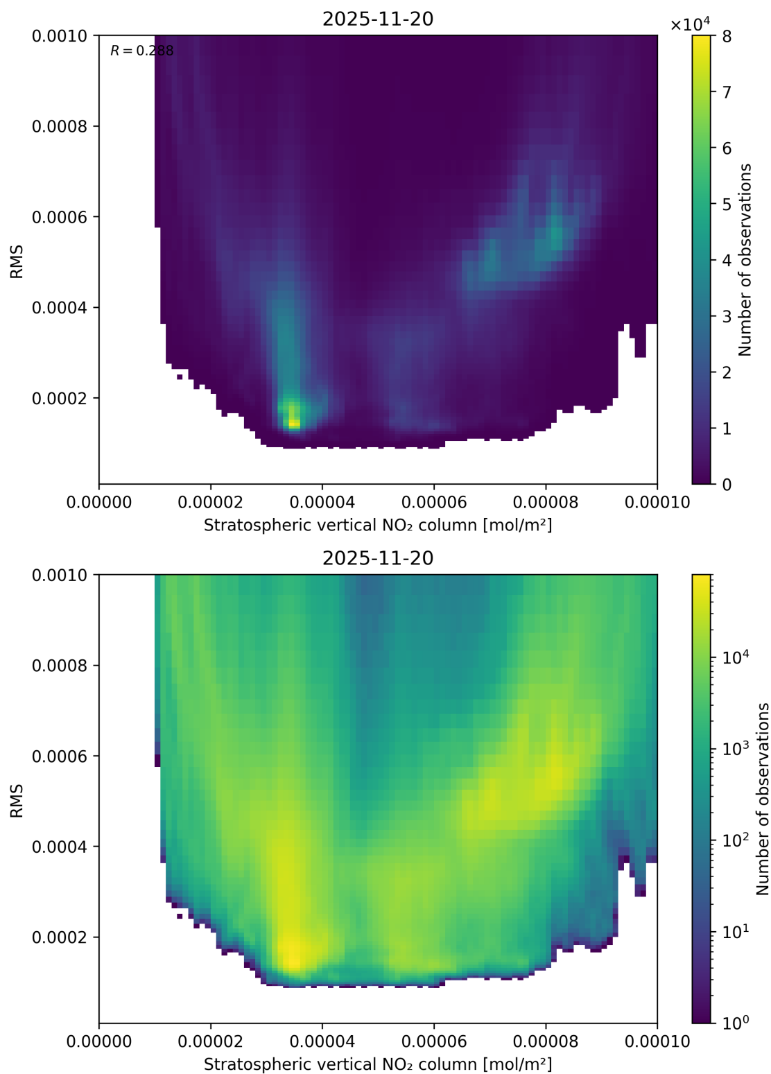
Figure 102: Scatter density plot of “Stratospheric vertical NO 2 column” against “RMS” for 2025-11-19 to 2025-11-21.
