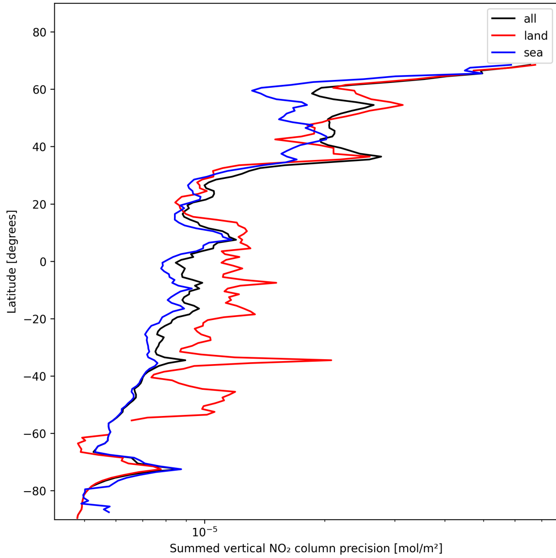
Figure 24: Zonal average of “Summed vertical NO 2 column precision” for 2025-11-19 to 2025-11-21.
