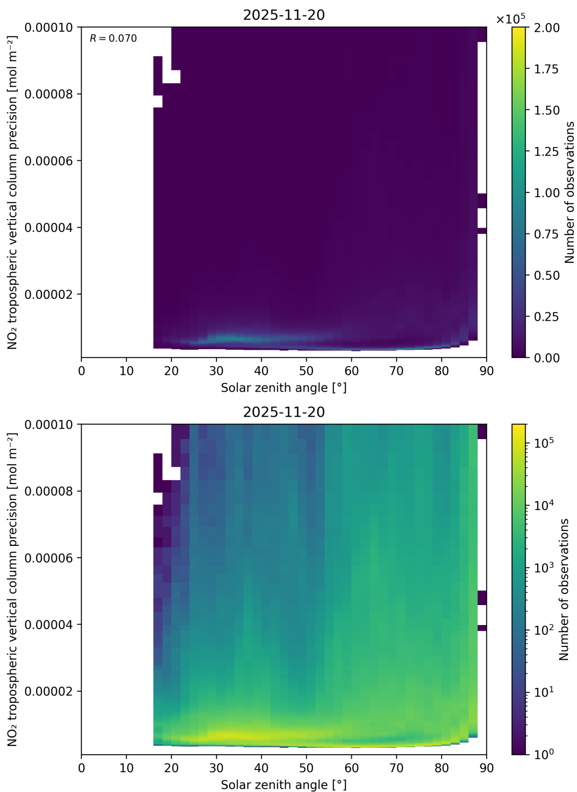
Figure 156: Scatter density plot of “Solar zenith angle” against “NO 2 tropospheric vertical column precision” for 2025-11-19 to 2025-11-21.
