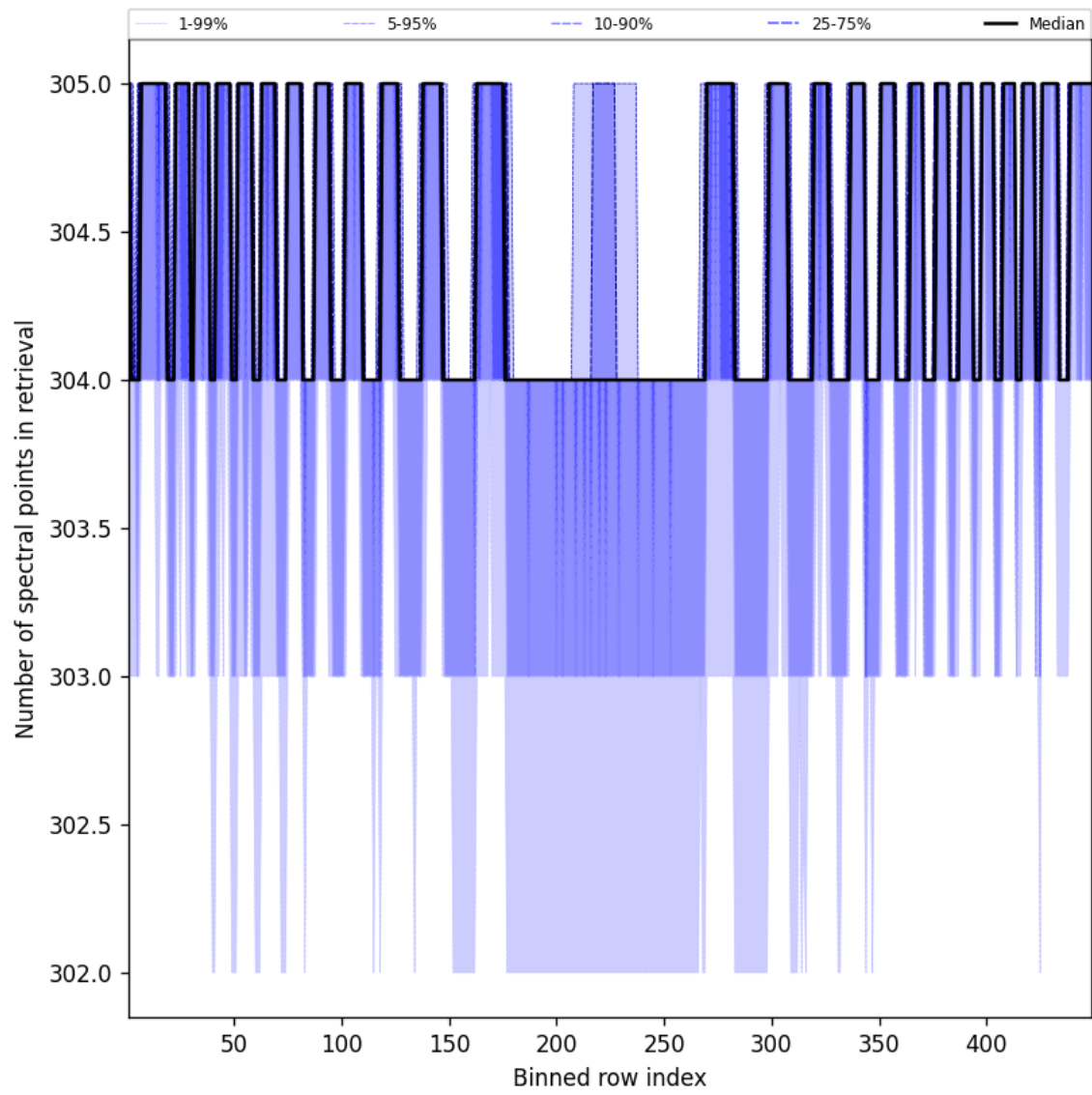
Figure 50: Along track statistics of “Number of spectral points in retrieval” for 2025-11-19 to 2025-11-21
