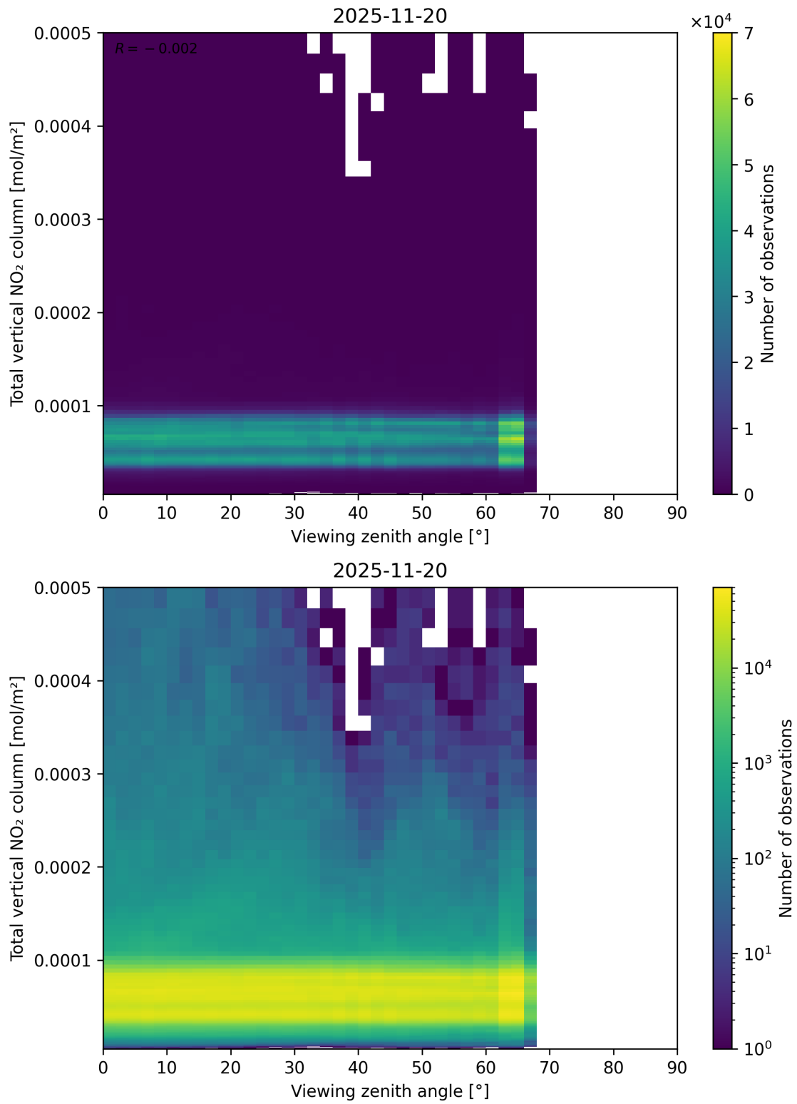
Figure 167: Scatter density plot of “Viewing zenith angle” against “Total vertical NO 2 column” for 2025-11-19 to 2025-11-21.
