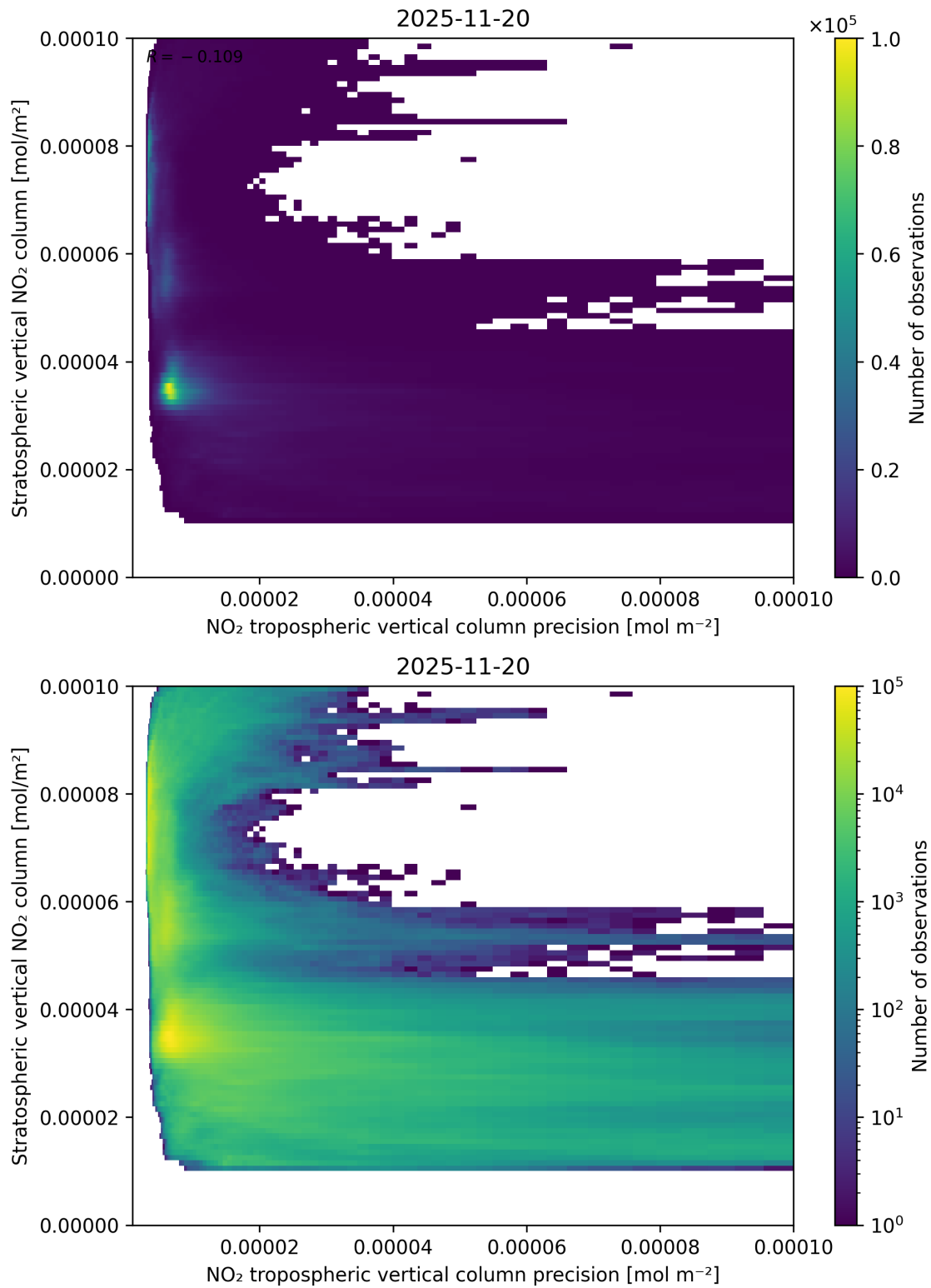
Figure 135: Scatter density plot of “NO 2 tropospheric vertical column precision” against “Stratospheric vertical NO 2 column” for 2025-11-19 to 2025-11-21.
