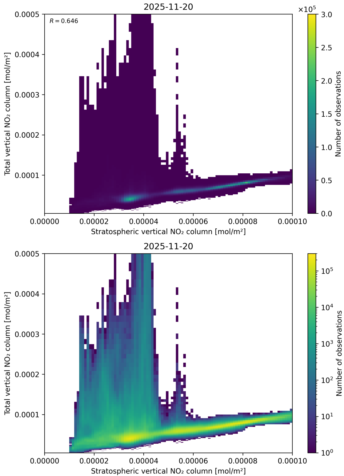
Figure 100: Scatter density plot of “Stratospheric vertical NO 2 column” against “Total vertical NO 2 column” for 2025-11-19 to 2025-11-21.
