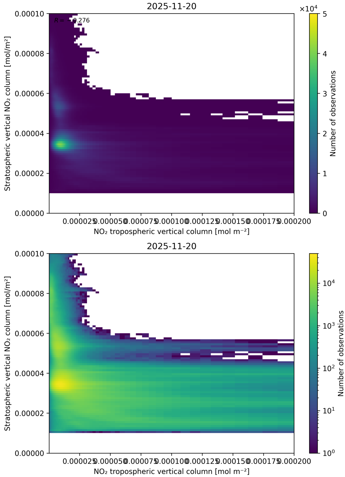
Figure 125: Scatter density plot of “NO 2 tropospheric vertical column” against “Stratospheric vertical NO 2 column” for 2025-11-19 to 2025-11-21.
