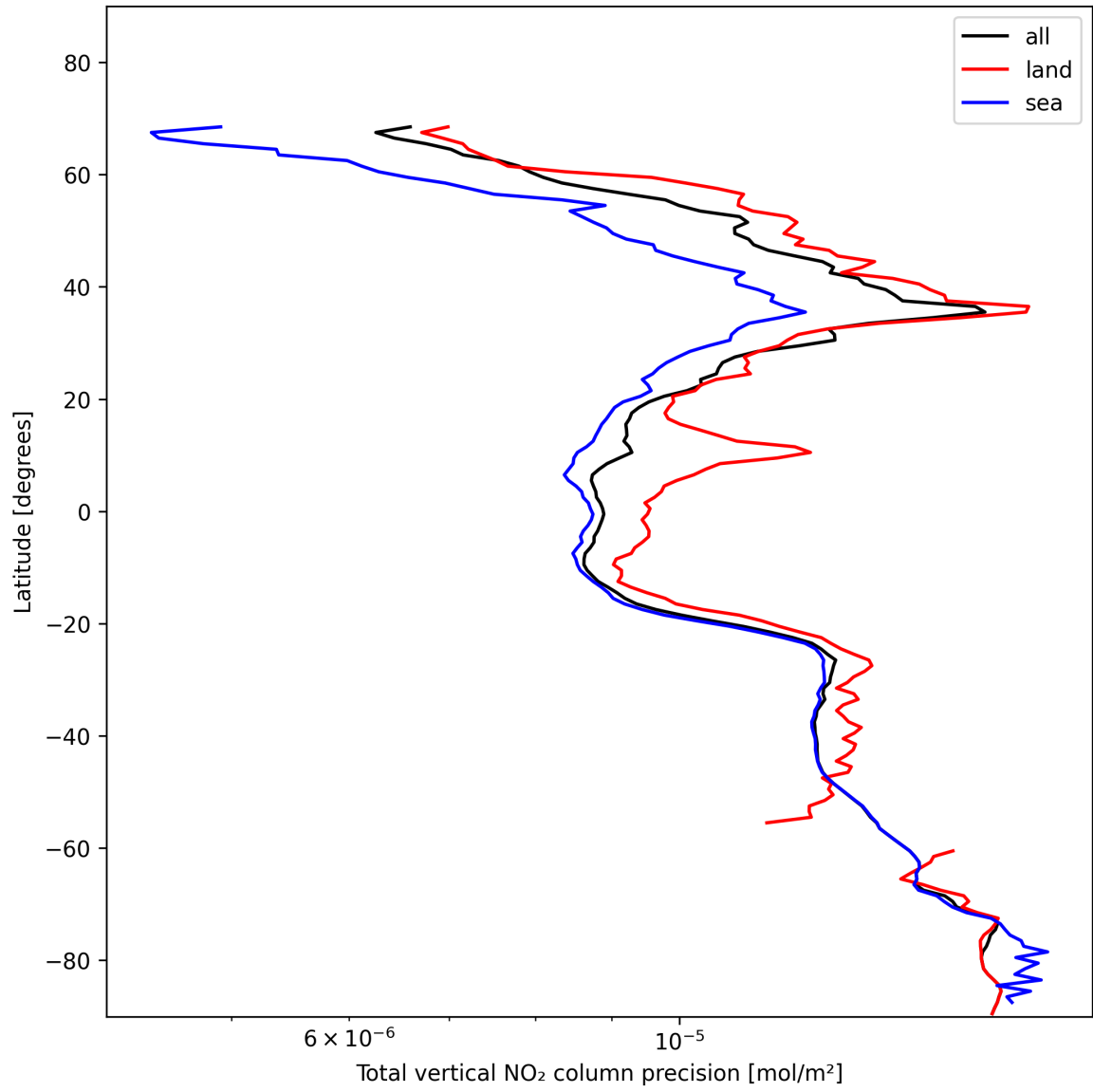
Figure 22: Zonal average of “Total vertical NO 2 column precision” for 2025-11-19 to 2025-11-21.
