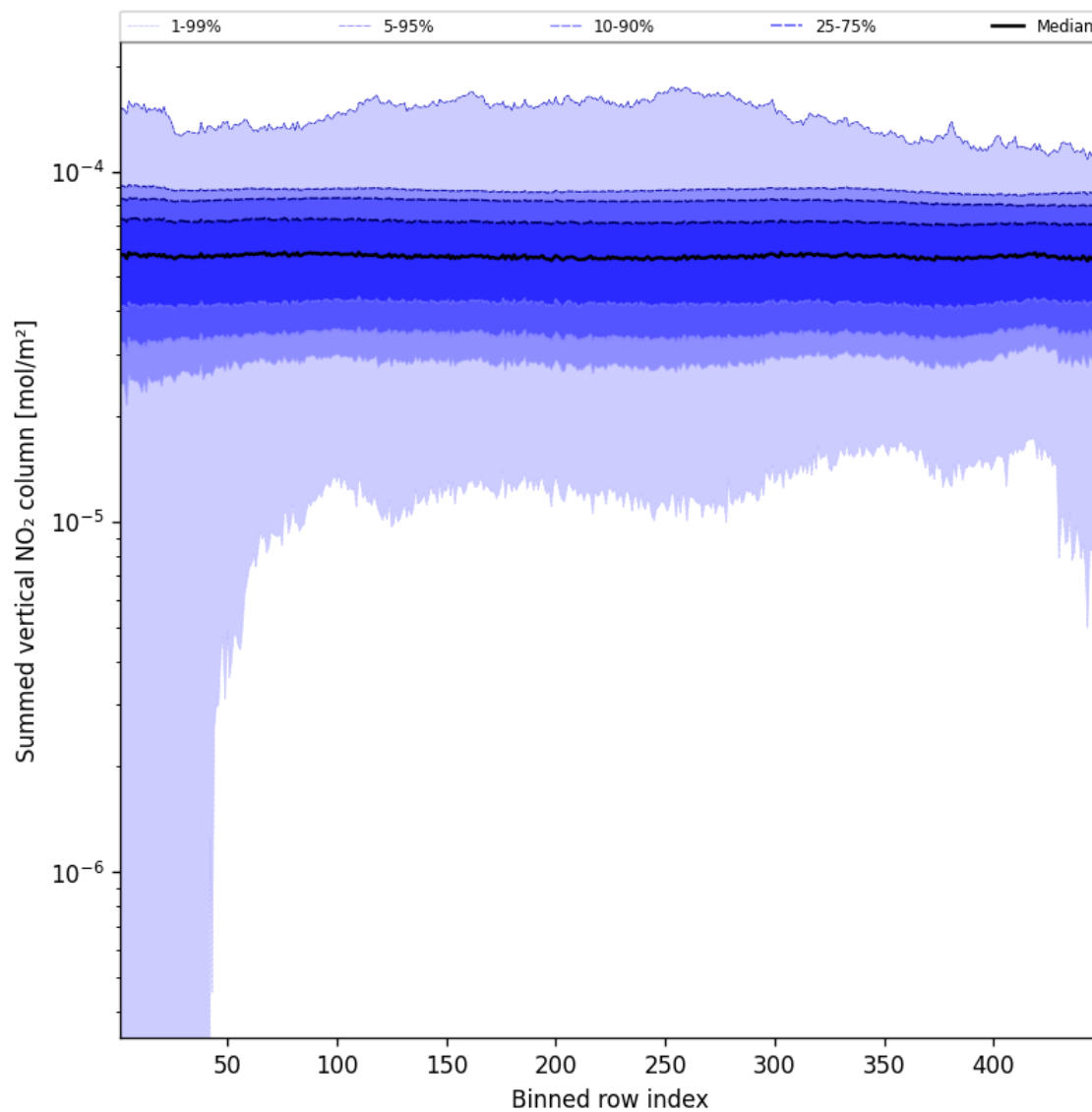
Figure 57: Along track statistics of “Summed vertical NO 2 column” for 2025-11-19 to 2025-11-21
