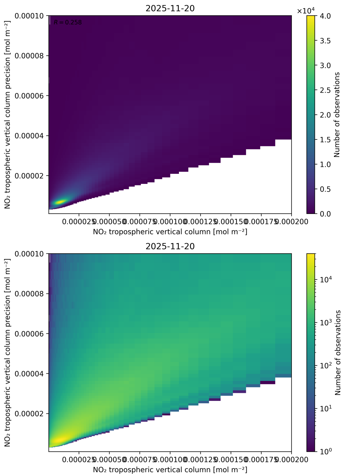
Figure 130: Scatter density plot of “NO 2 tropospheric vertical column” against “NO 2 tropospheric vertical column precision” for 2025-11-19 to 2025-11-21.
