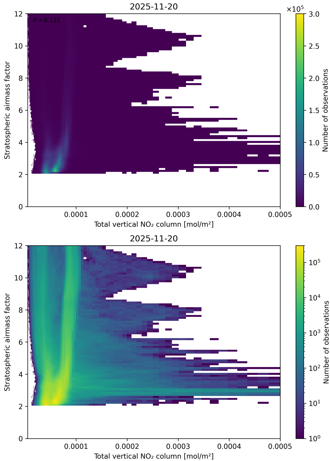
Figure 110: Scatter density plot of “Total vertical NO 2 column” against “Stratospheric airmass factor” for 2025-11-19 to 2025-11-21.
