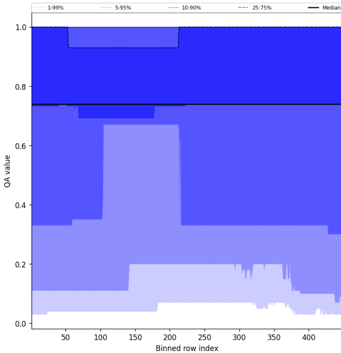
Figure 45: Along track statistics of “QA value” for 2025-11-19 to 2025-11-21
