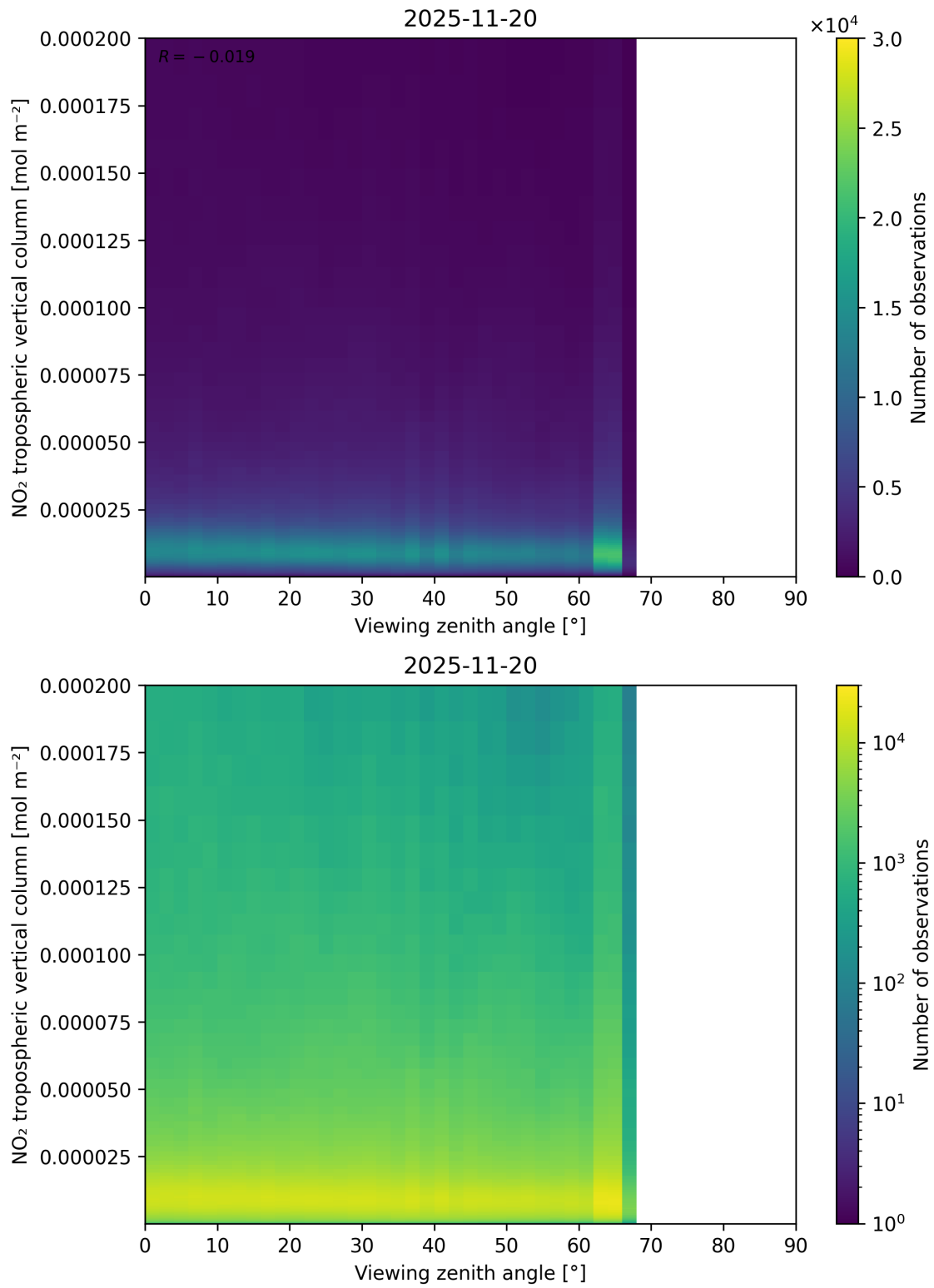
Figure 169: Scatter density plot of “Viewing zenith angle” against “NO 2 tropospheric vertical column” for 2025-11-19 to 2025-11-21.
