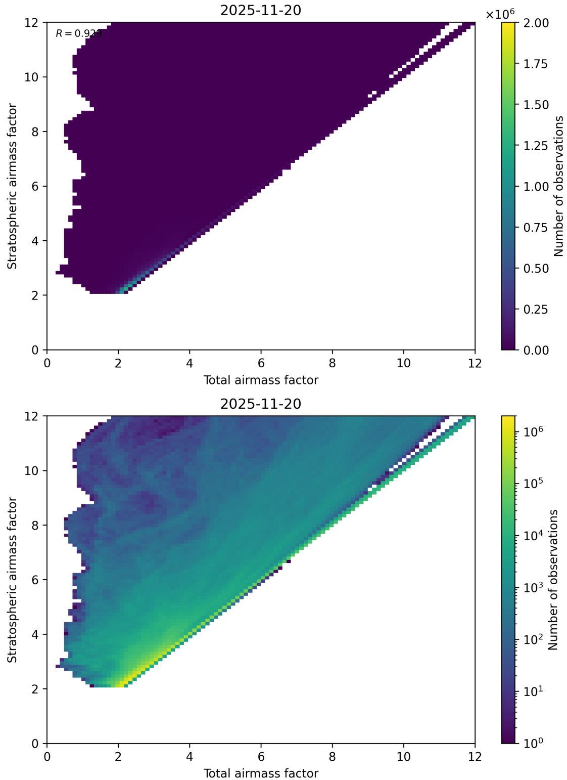
Figure 62: Scatter density plot of “Total airmass factor” against “Stratospheric airmass factor” for 2025-11-19 to 2025-11-21.
