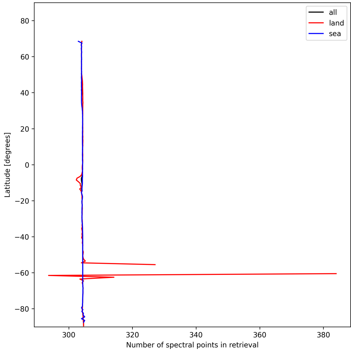
Figure 16: Zonal average of “Number of spectral points in retrieval” for 2025-11-19 to 2025-11-21.
