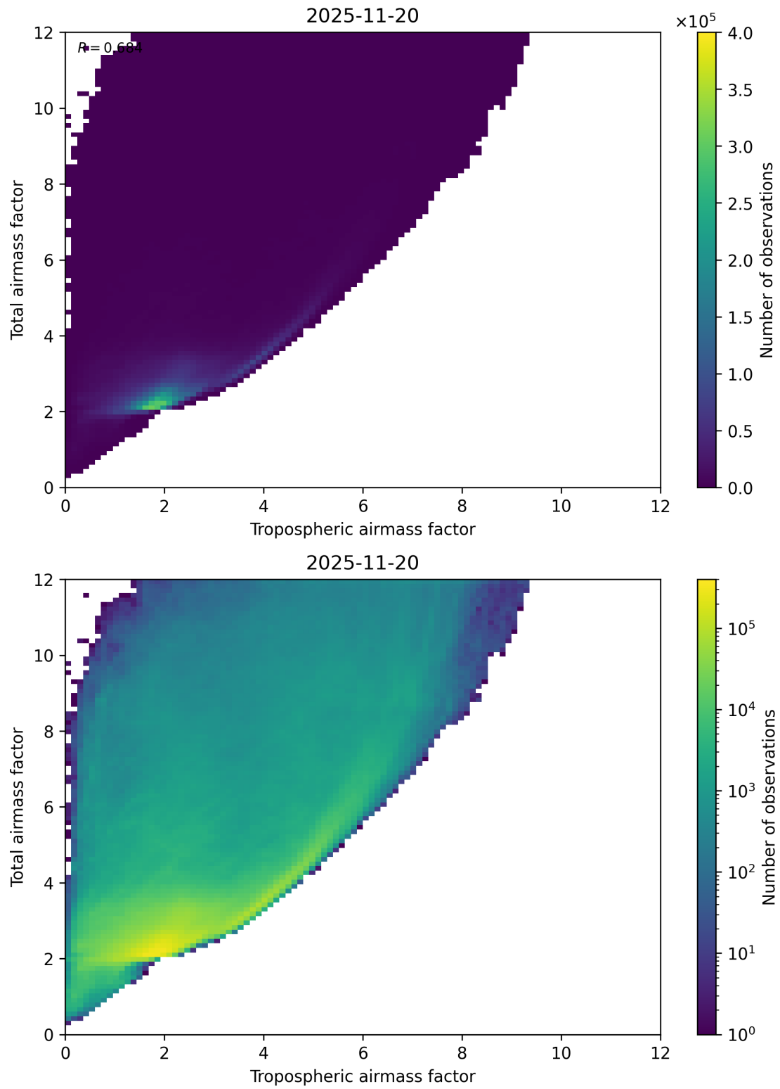
Figure 72: Scatter density plot of “Tropospheric airmass factor” against “Total airmass factor” for 2025-11-19 to 2025-11-21.
