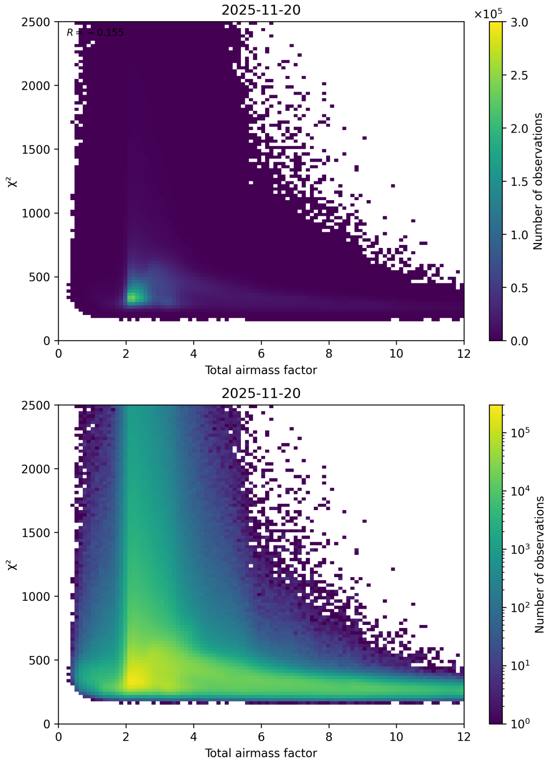
Figure 63: Scatter density plot of “Total airmass factor” against “ \chi^2 ” for 2025-11-19 to 2025-11-21.
