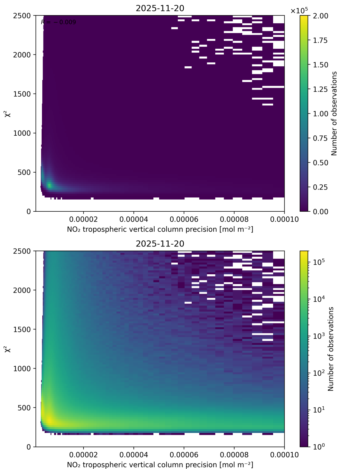
Figure 134: Scatter density plot of “NO 2 tropospheric vertical column precision” against “ \chi^2 ” for 2025-11-19 to 2025-11-21.
