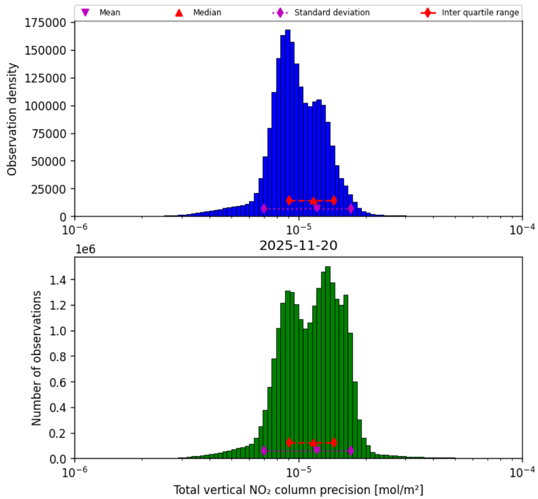
Figure 39: Histogram of “Total vertical NO 2 column precision” for 2025-11-19 to 2025-11-21
