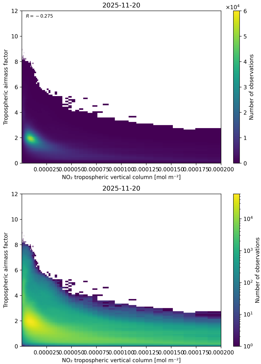
Figure 123: Scatter density plot of “NO 2 tropospheric vertical column” against “Tropospheric air mass factor” for 2025-11-19 to 2025-11-21.
