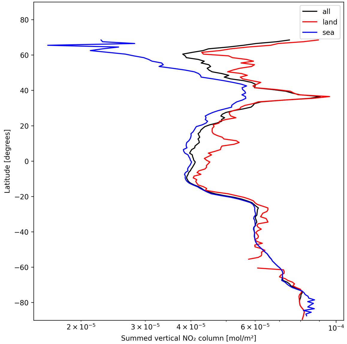
Figure 23: Zonal average of “Summed vertical NO 2 column” for 2025-11-19 to 2025-11-21.
