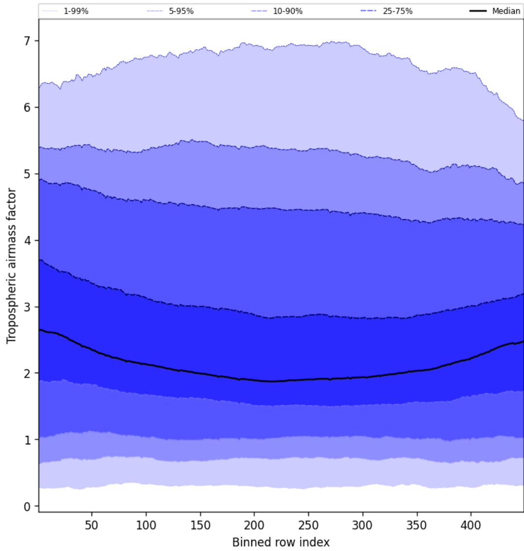
Figure 48: Along track statistics of “Tropospheric airmass factor” for 2025-11-19 to 2025-11-21
