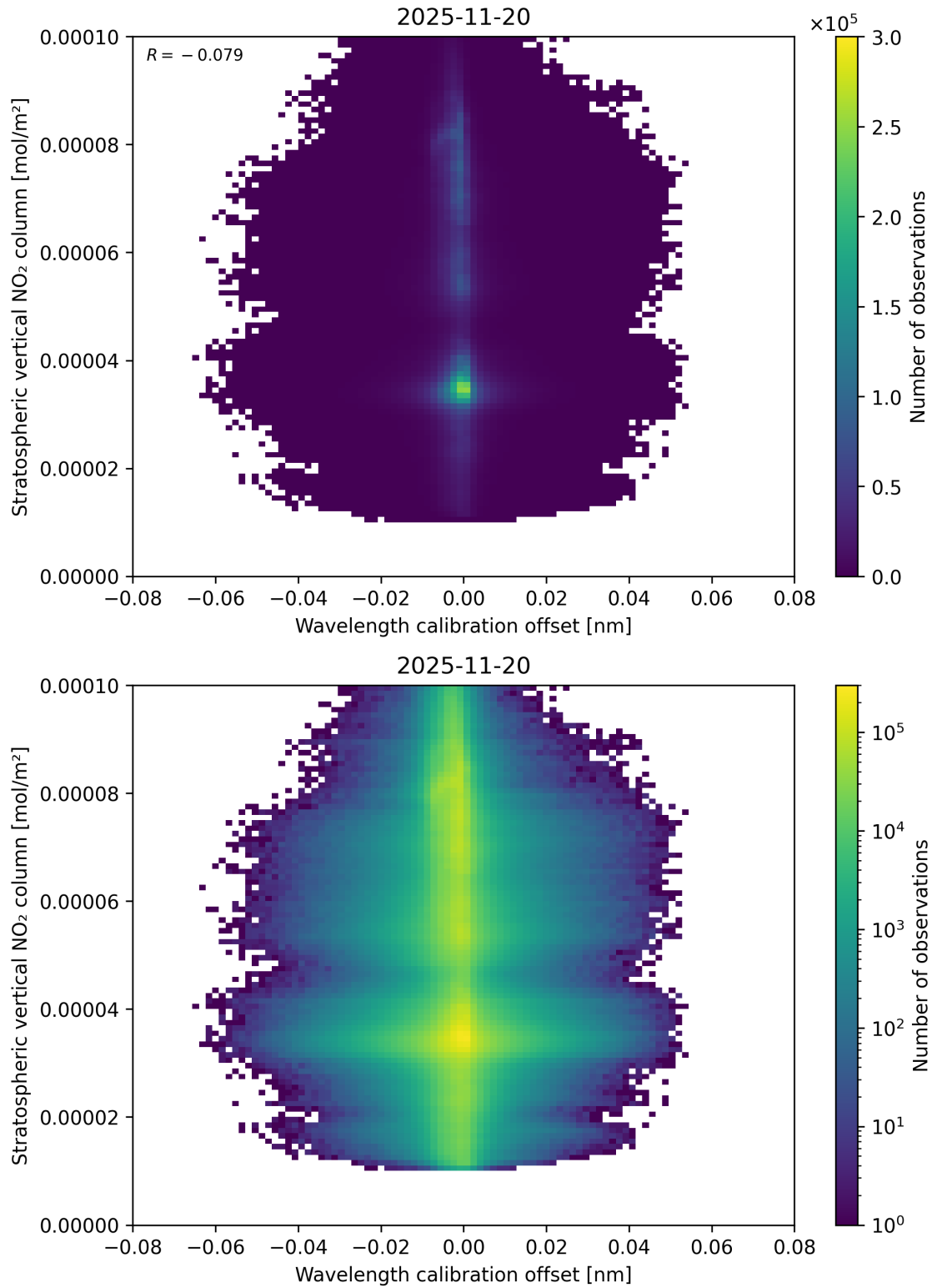
Figure 176: Scatter density plot of “Wavelength calibration offset” against “Stratospheric vertical NO 2 column” for 2025-11-19 to 2025-11-21.
