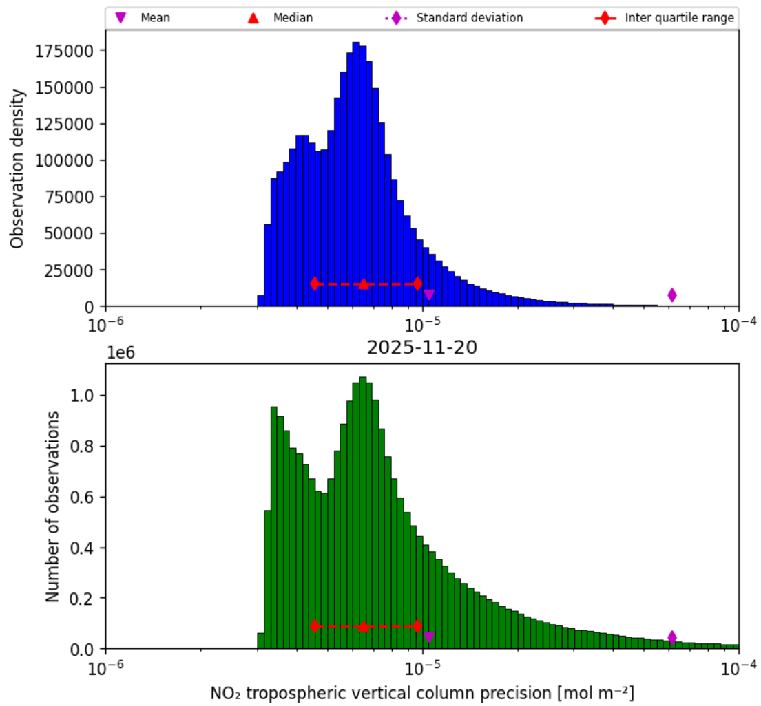
Figure 30: Histogram of "NO 2 tropospheric vertical column precision" for 2025-11-19 to 2025-11-21
