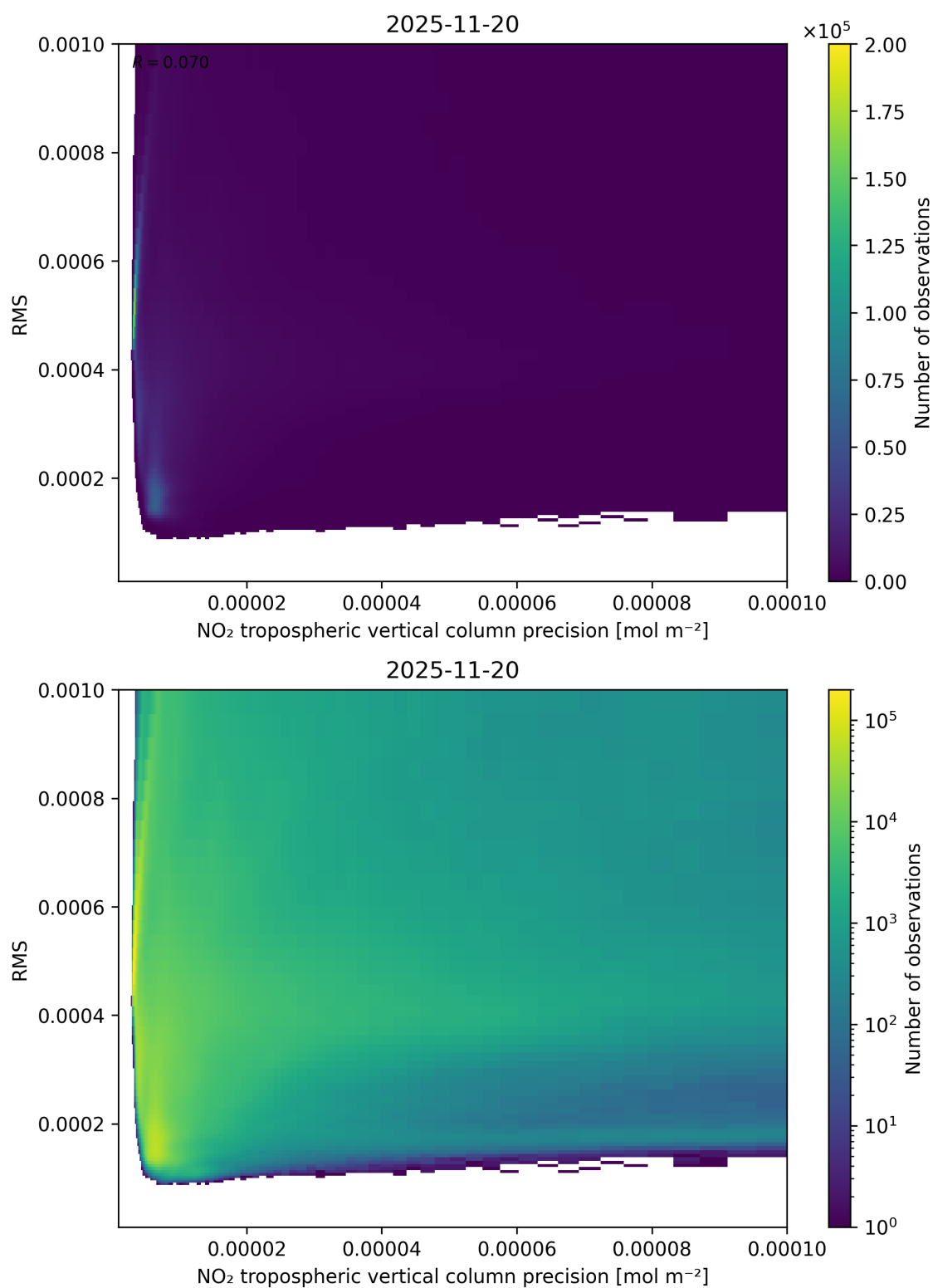
Figure 140: Scatter density plot of “NO 2 tropospheric vertical column precision” against “RMS” for 2025-11-19 to 2025-11-21.
