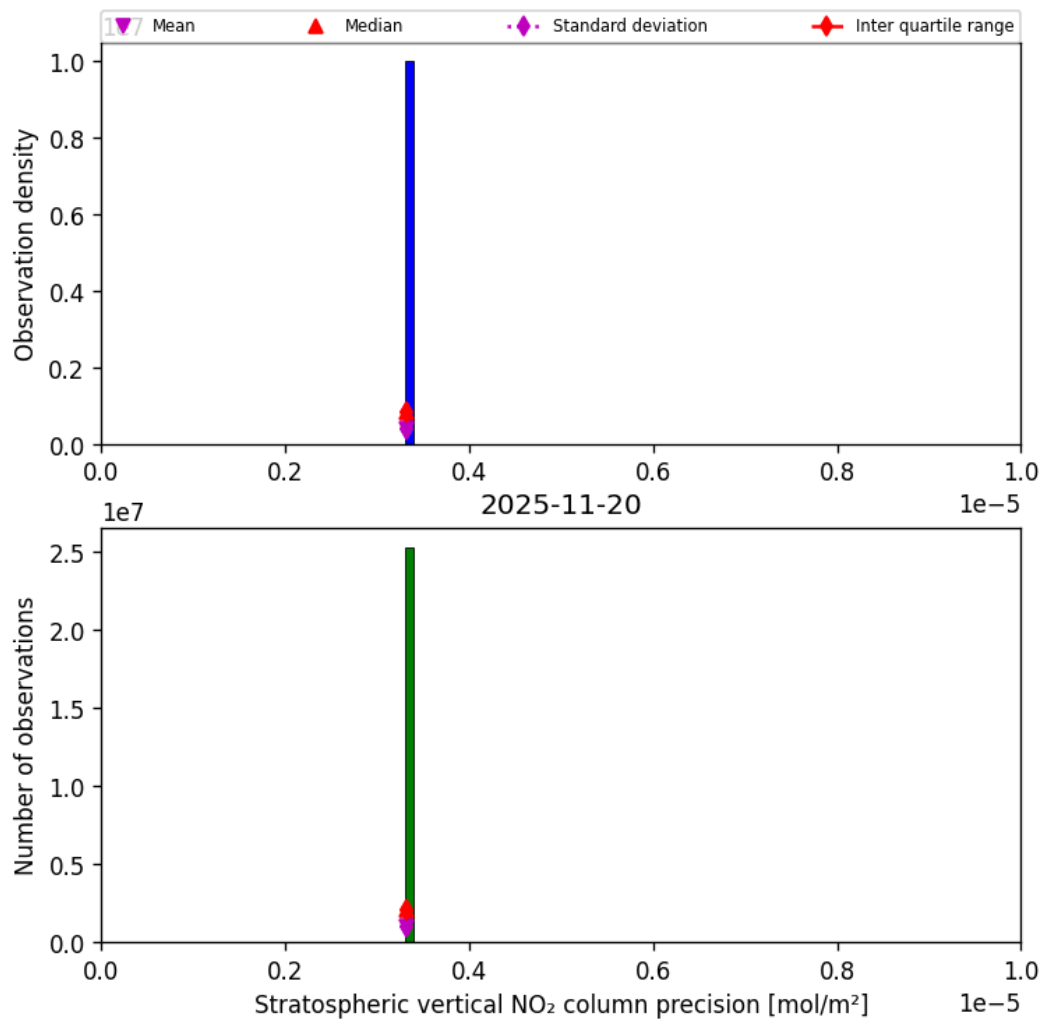
Figure 37: Histogram of “Stratospheric vertical NO 2 column precision” for 2025-11-19 to 2025-11-21
