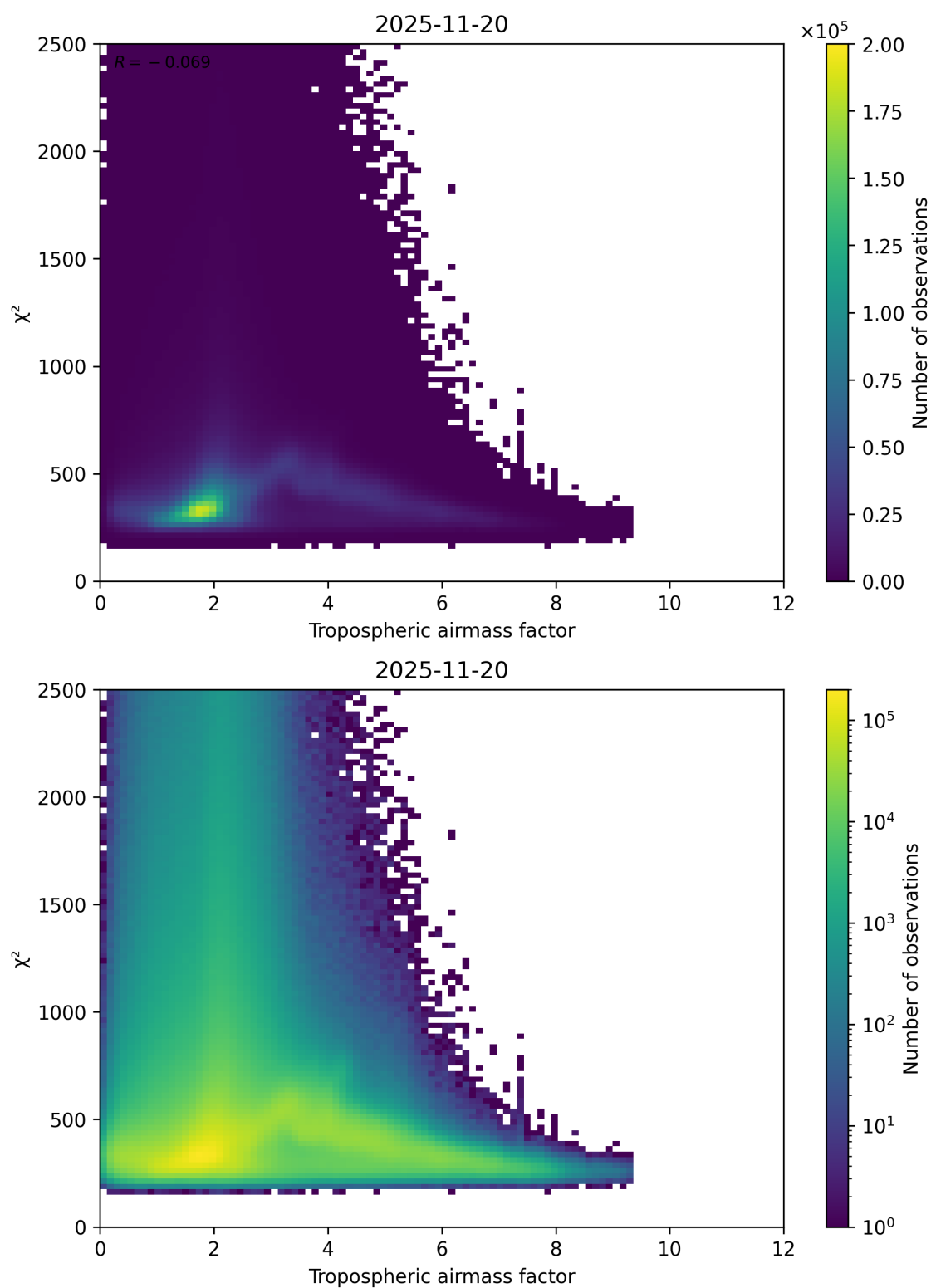
Figure 73: Scatter density plot of “Tropospheric airmass factor” against “ \chi^2 ” for 2025-11-19 to 2025-11-21.
