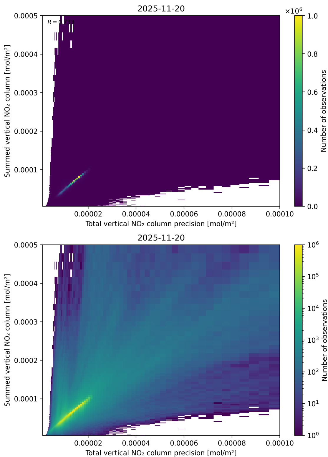
Figure 117: Scatter density plot of “Total vertical NO 2 column precision” against “Summed vertical NO 2 column” for 2025-11-19 to 2025-11-21.
