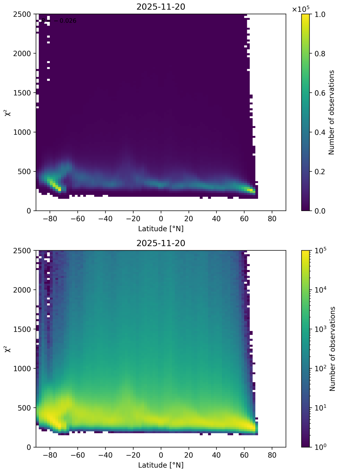
Figure 86: Scatter density plot of “Latitude” against “ \chi^2 ” for 2025-11-19 to 2025-11-21.
