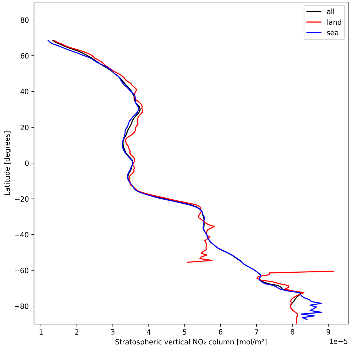
Figure 19: Zonal average of “Stratospheric vertical NO 2 column” for 2025-11-19 to 2025-11-21.
