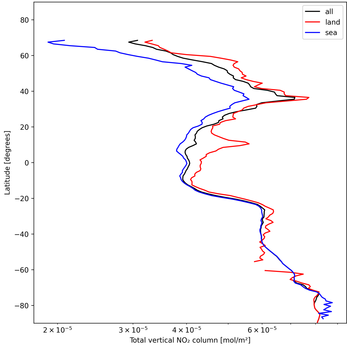
Figure 21: Zonal average of “Total vertical NO 2 column” for 2025-11-19 to 2025-11-21.
