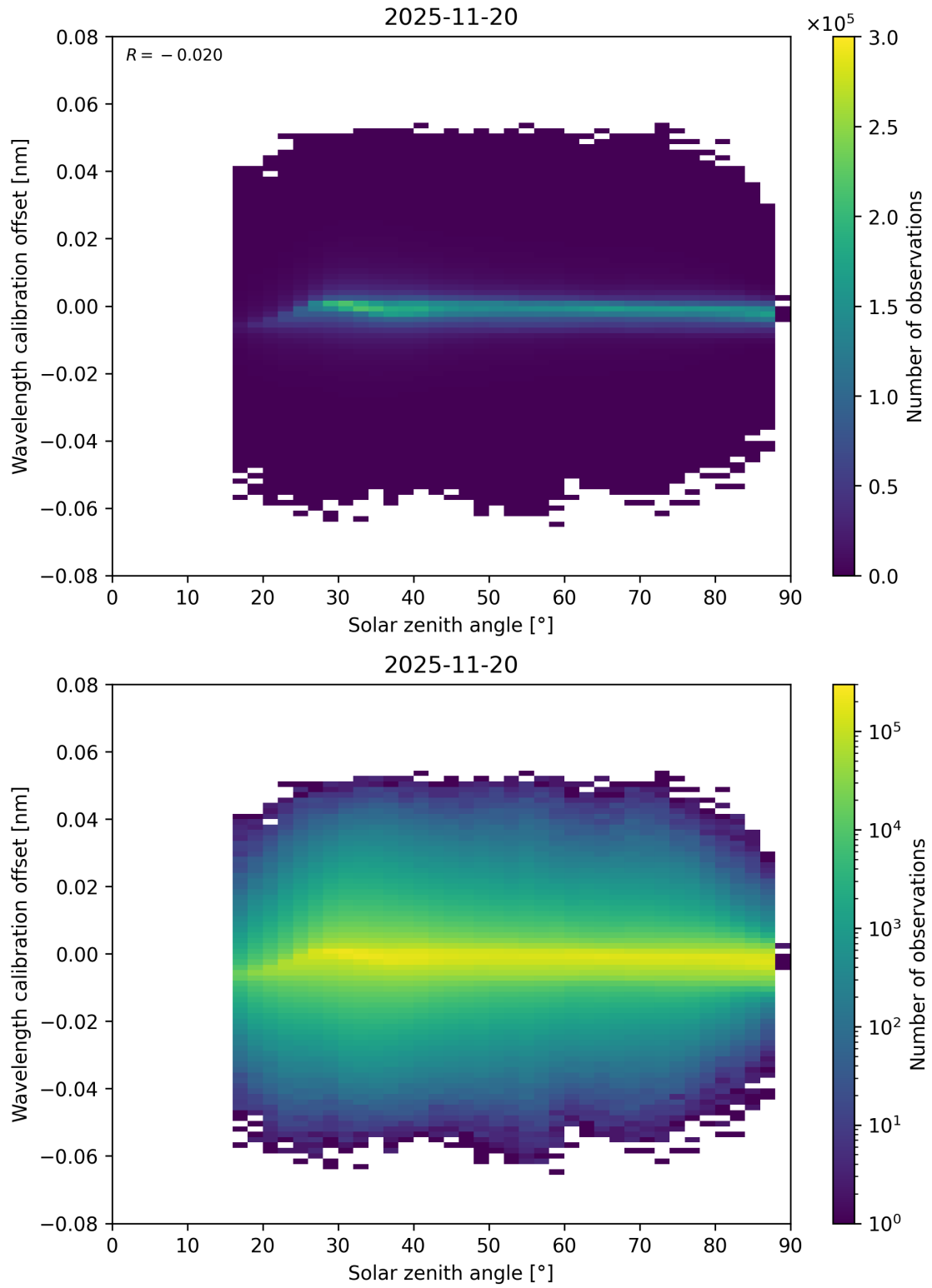
Figure 158: Scatter density plot of “Solar zenith angle” against “Wavelength calibration offset” for 2025-11-19 to 2025-11-21.
