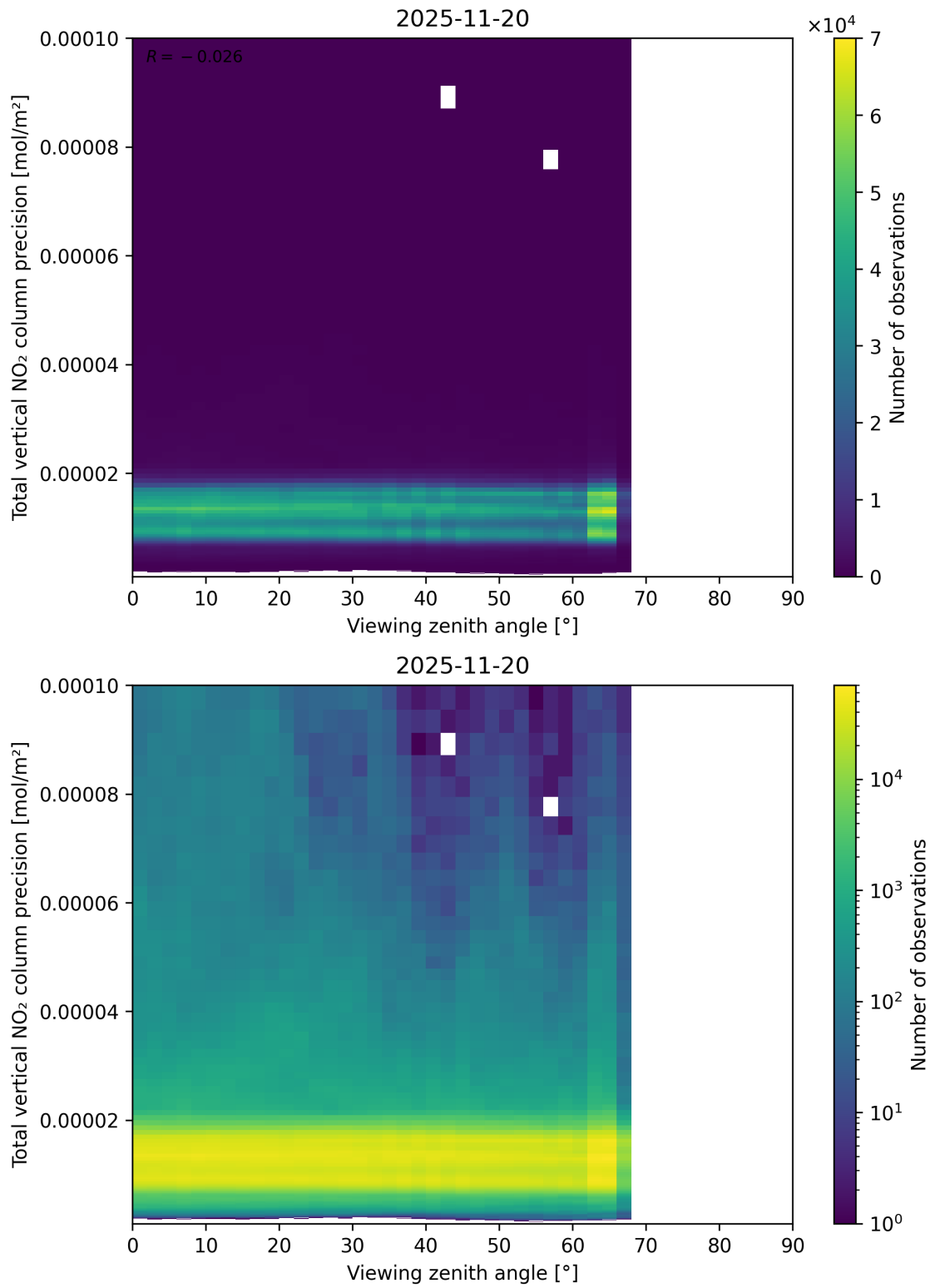
Figure 168: Scatter density plot of “Viewing zenith angle” against “Total vertical NO 2 column precision” for 2025-11-19 to 2025-11-21.
