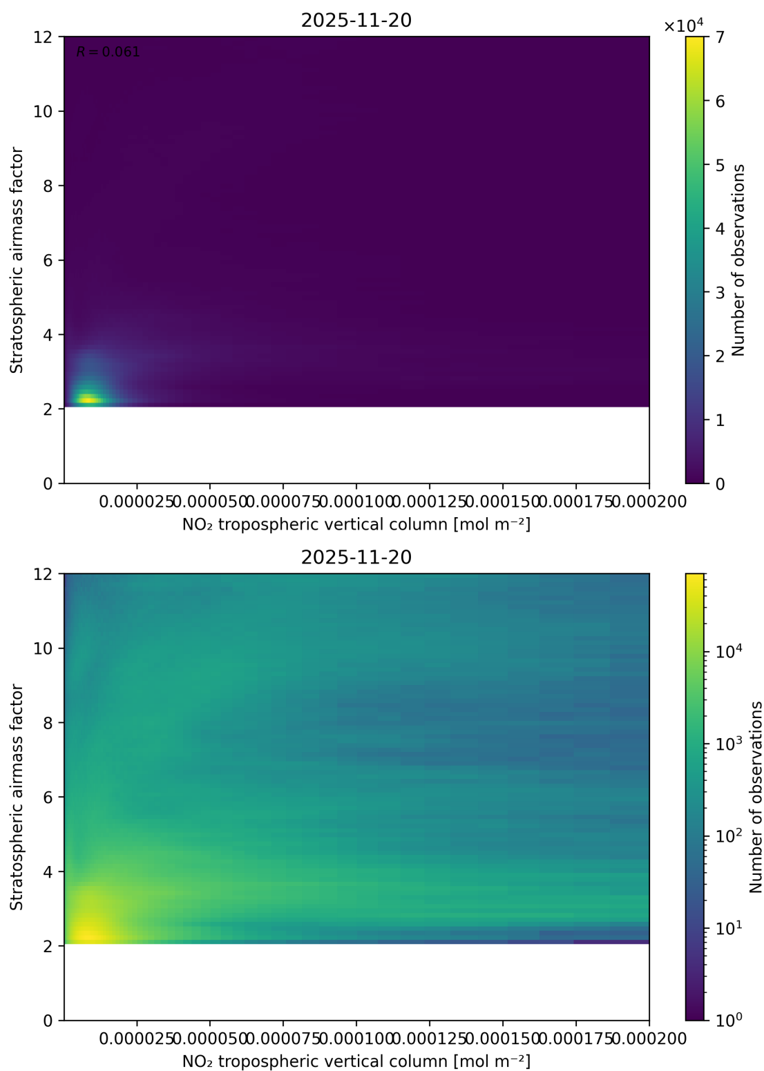
Figure 121: Scatter density plot of “NO 2 tropospheric vertical column” against “Stratospheric airmass factor” for 2025-11-19 to 2025-11-21.
