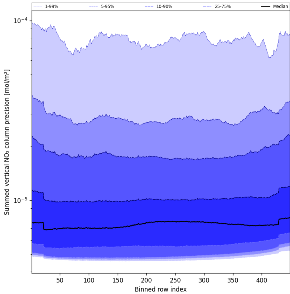
Figure 58: Along track statistics of “Summed vertical NO 2 column precision” for 2025-11-19 to 2025-11-21
