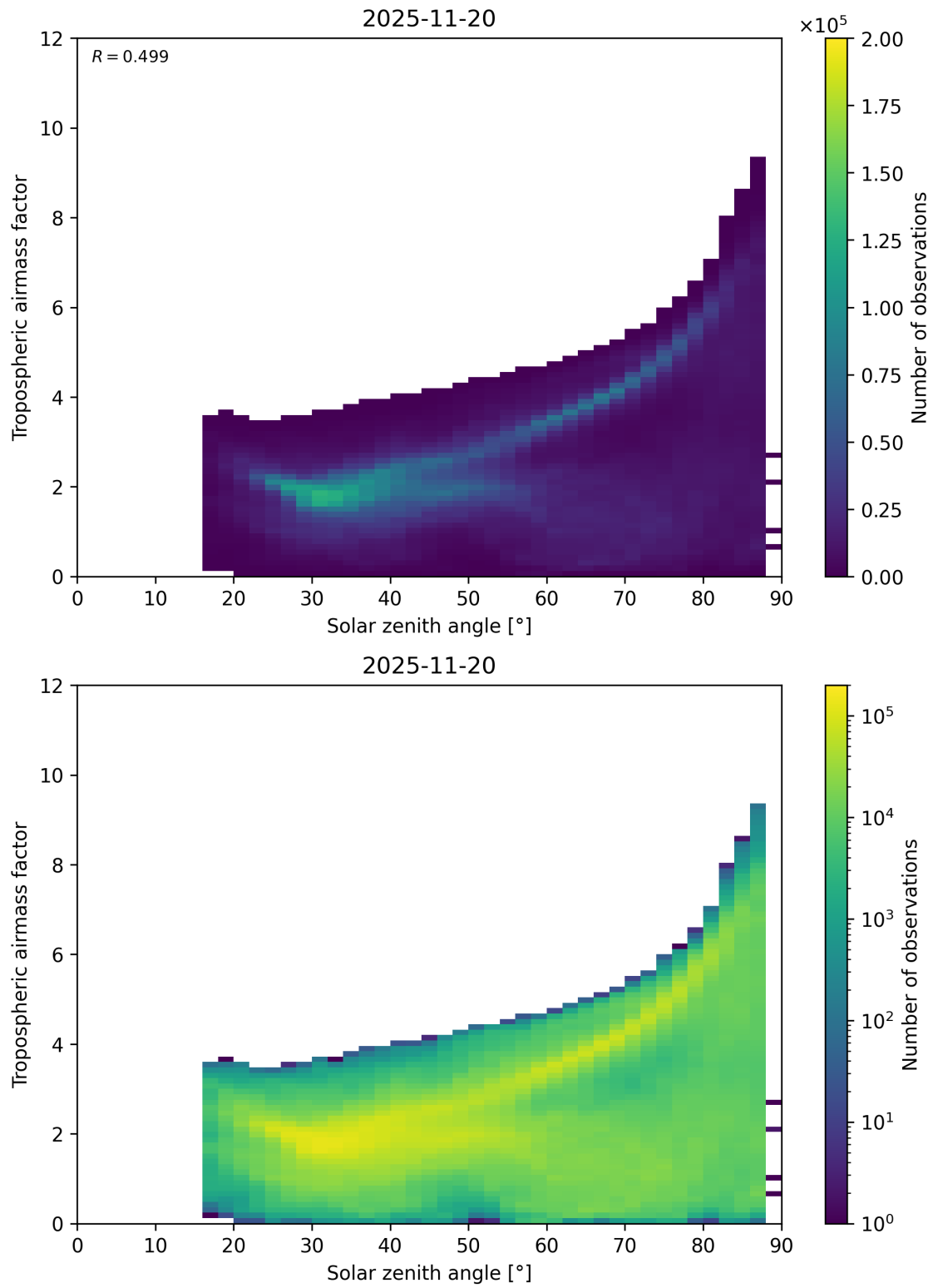
Figure 147: Scatter density plot of “Solar zenith angle” against “Tropospheric airmass factor” for 2025-11-19 to 2025-11-21.
