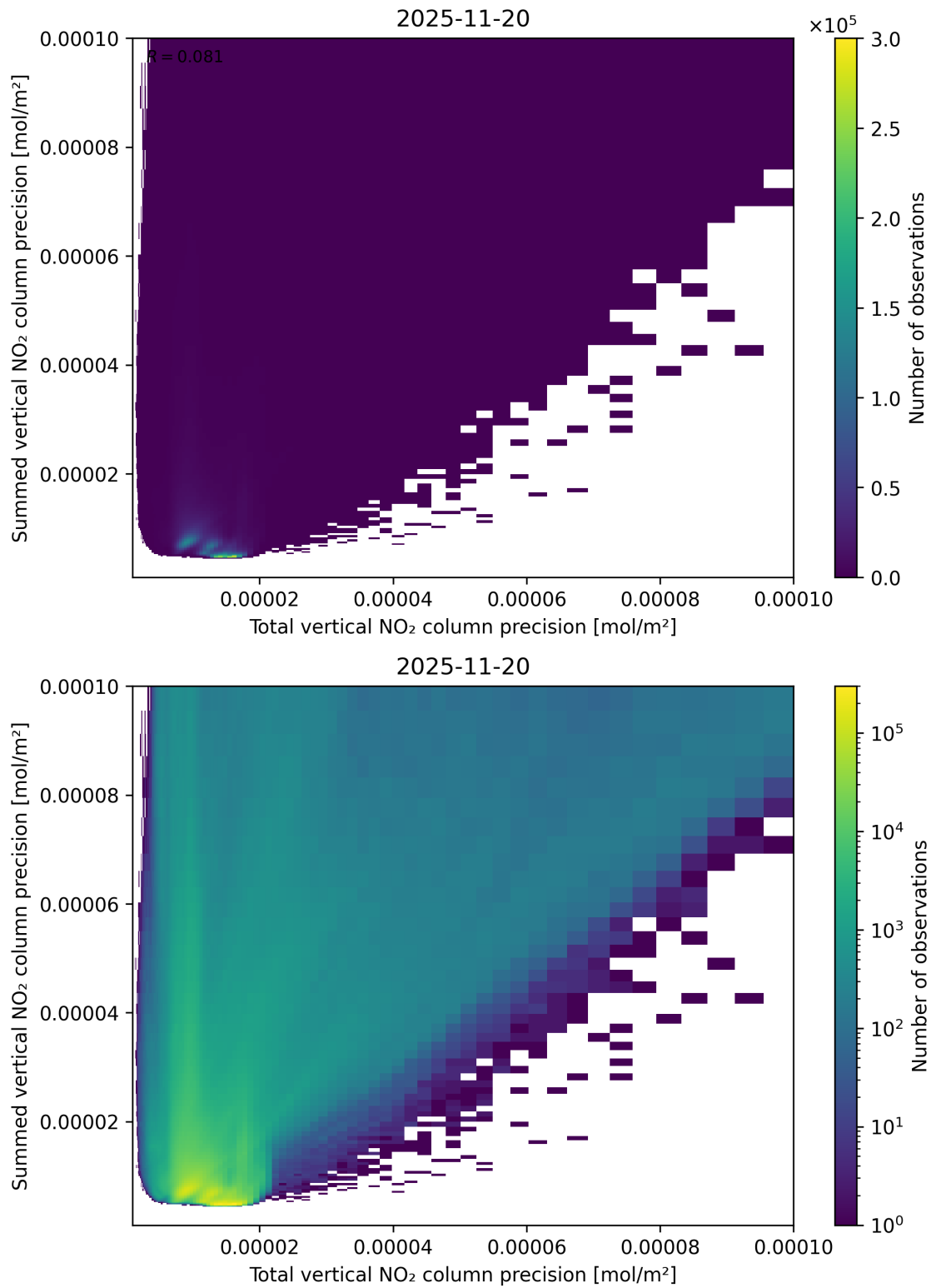
Figure 118: Scatter density plot of “Total vertical NO 2 column precision” against “Summed vertical NO 2 column precision” for 2025-11-19 to 2025-11-21.
