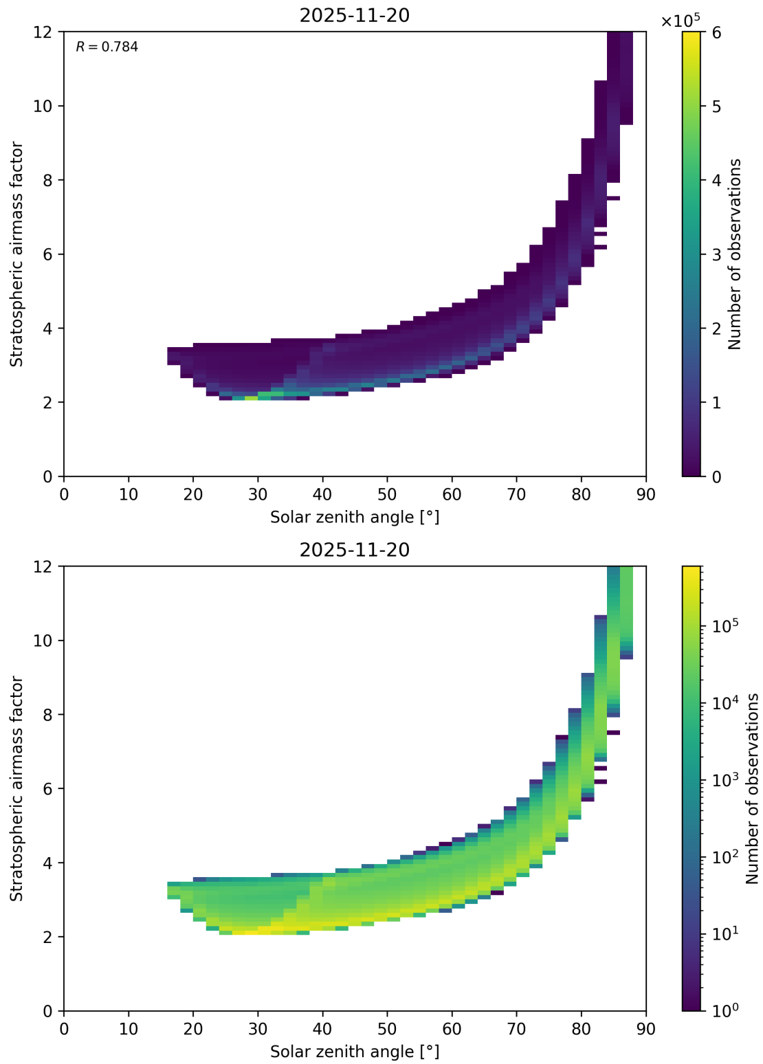
Figure 145: Scatter density plot of “Solar zenith angle” against “Stratospheric airmass factor” for 2025-11-19 to 2025-11-21.
