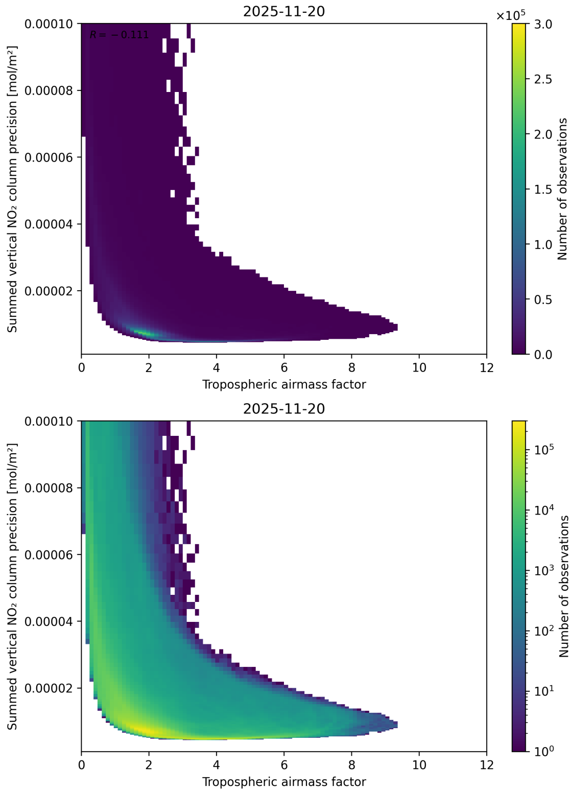
Figure 76: Scatter density plot of “Tropospheric airmass factor” against “Summed vertical NO 2 column precision” for 2025-11-19 to 2025-11-21.
