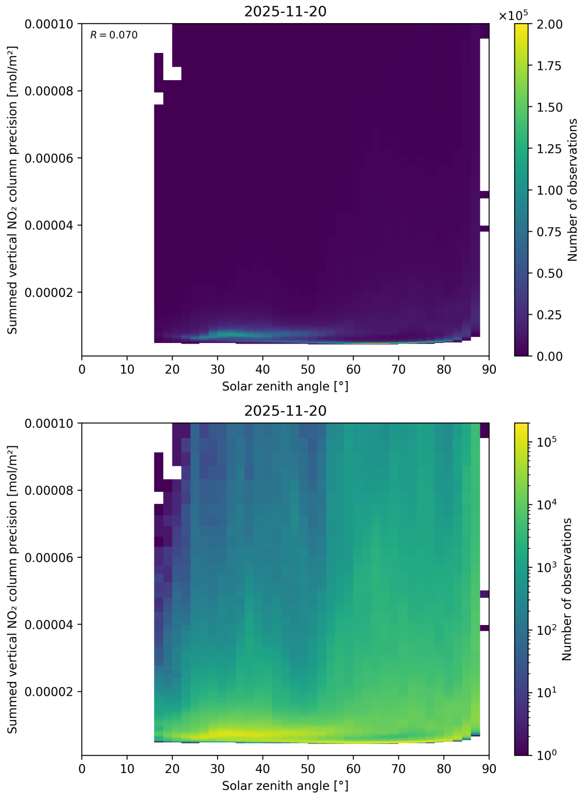
Figure 152: Scatter density plot of “Solar zenith angle” against “Summed vertical NO 2 column precision” for 2025-11-19 to 2025-11-21.
