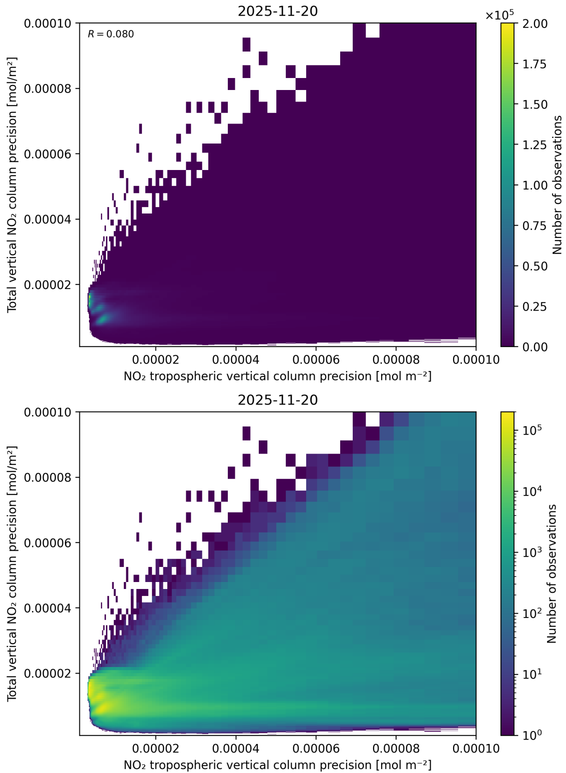
Figure 139: Scatter density plot of “NO 2 tropospheric vertical column precision” against “Total vertical NO 2 column precision” for 2025-11-19 to 2025-11-21.
