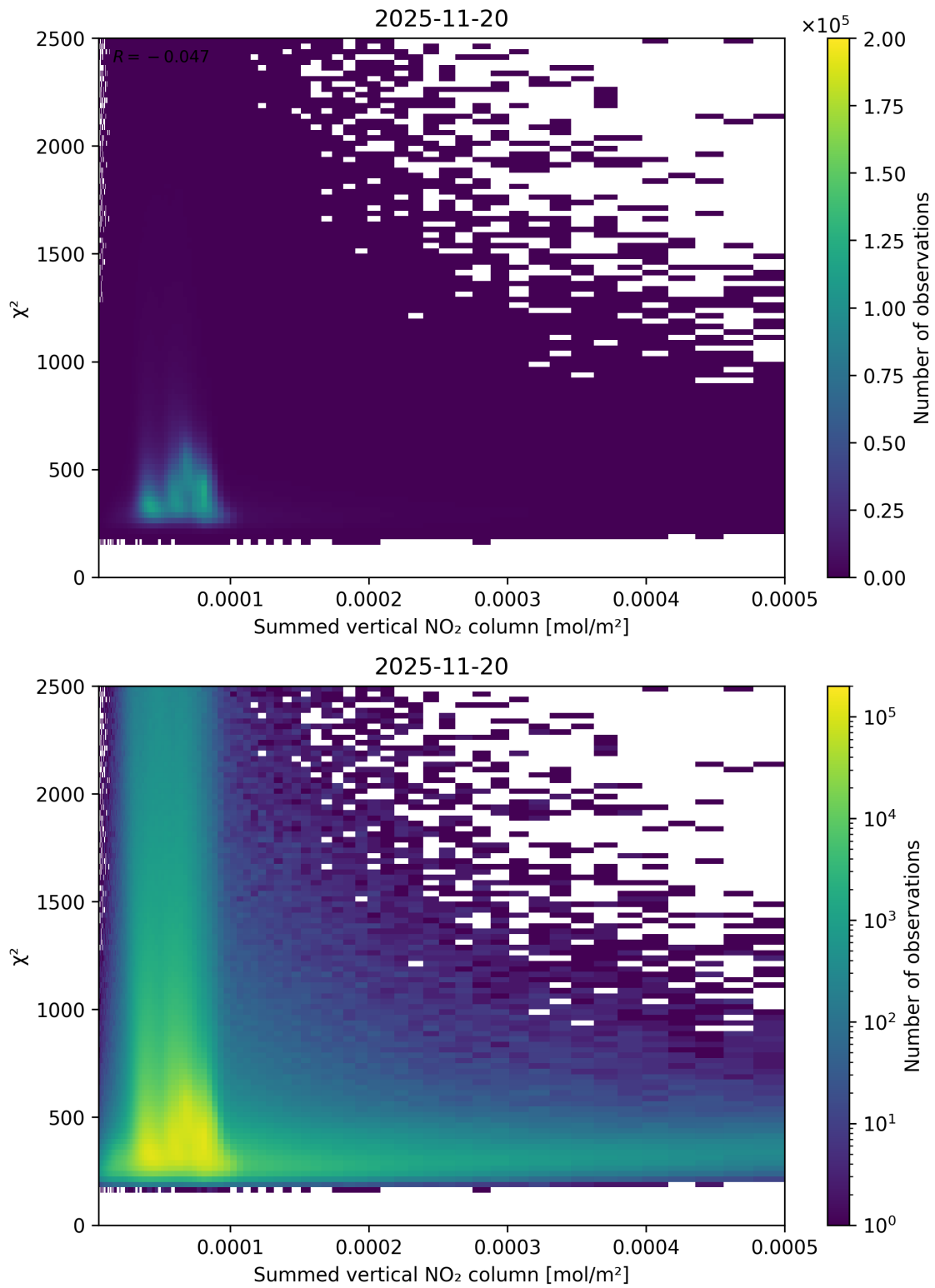
Figure 104: Scatter density plot of “Summed vertical NO 2 column” against “ \chi^2 ” for 2025-11-19 to 2025-11-21.
