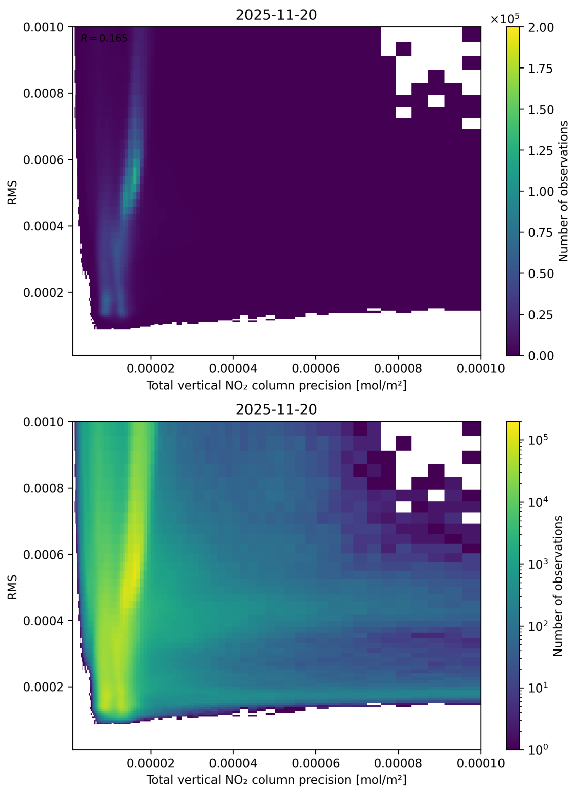
Figure 119: Scatter density plot of “Total vertical NO 2 column precision” against “RMS” for 2025-11-19 to 2025-11-21.
