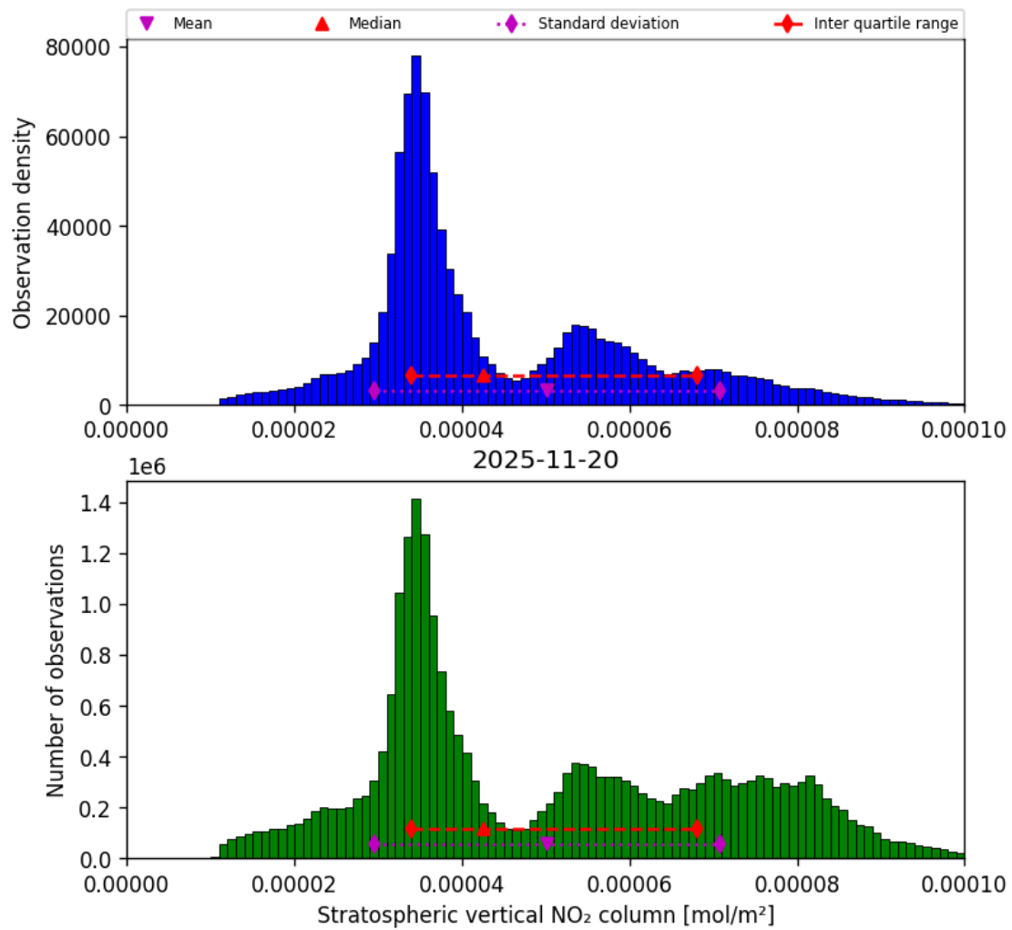
Figure 36: Histogram of “Stratospheric vertical NO 2 column” for 2025-11-19 to 2025-11-21
