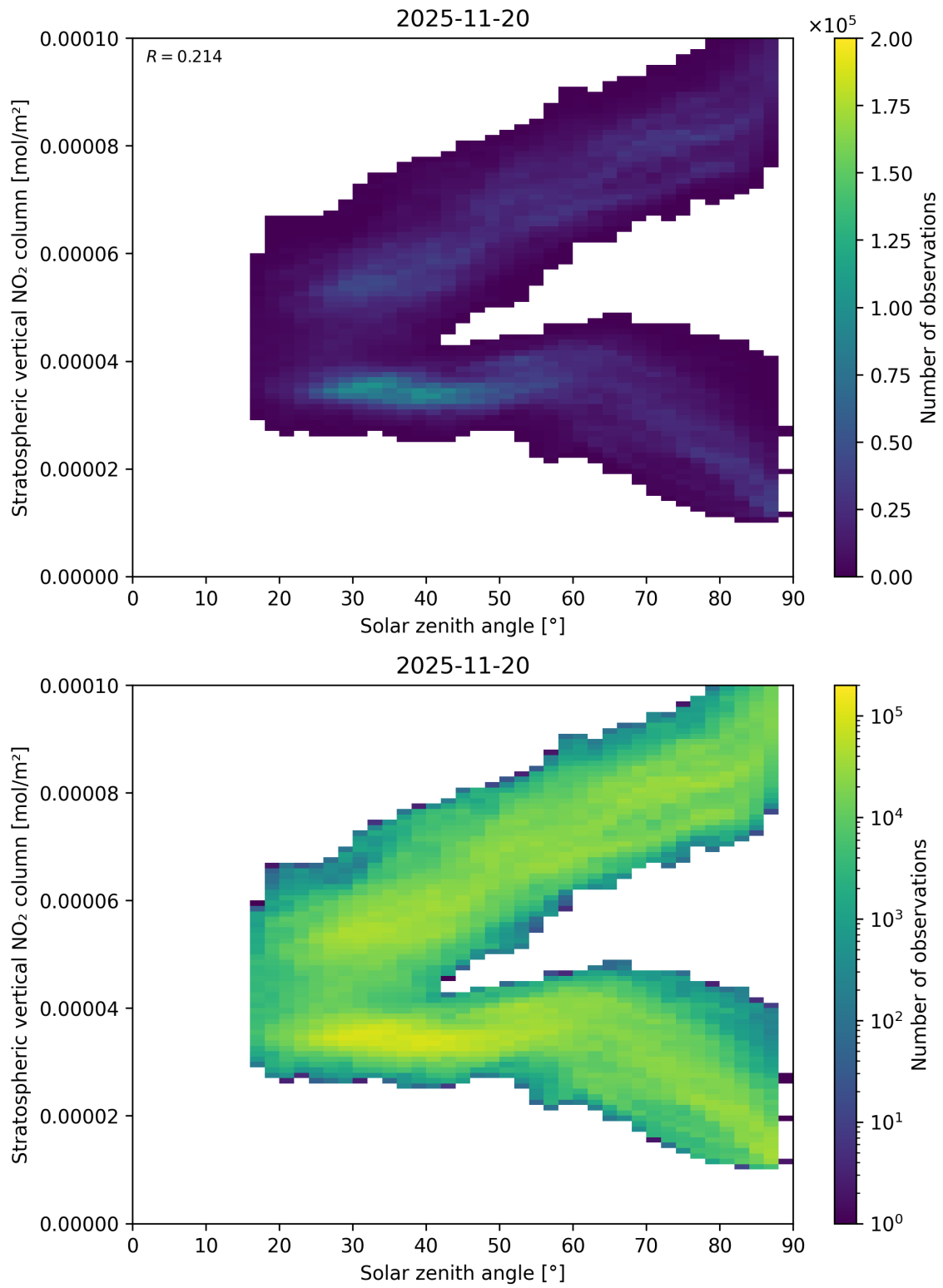
Figure 150: Scatter density plot of “Solar zenith angle” against “Stratospheric vertical NO 2 column” for 2025-11-19 to 2025-11-21.
