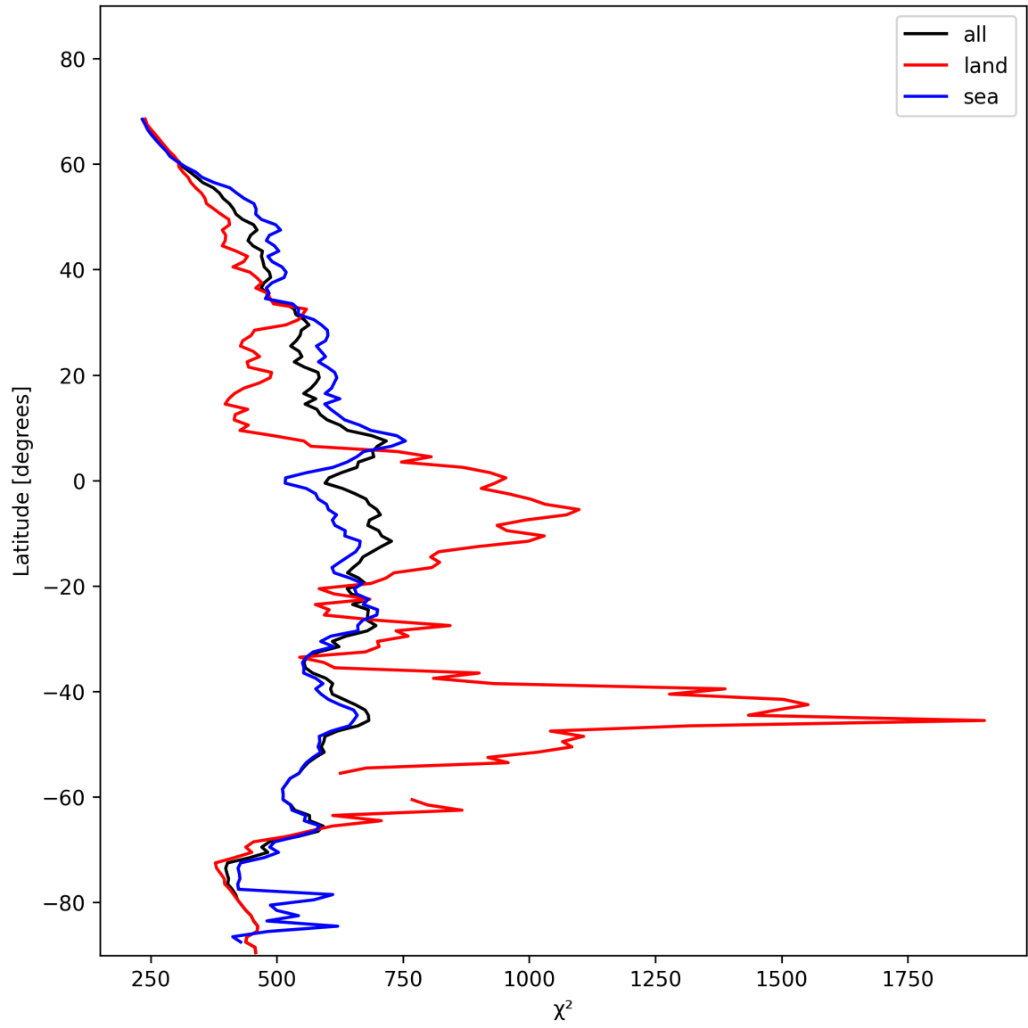
Figure 25: Zonal average of “ \chi^2 ” for 2025-11-19 to 2025-11-21.
