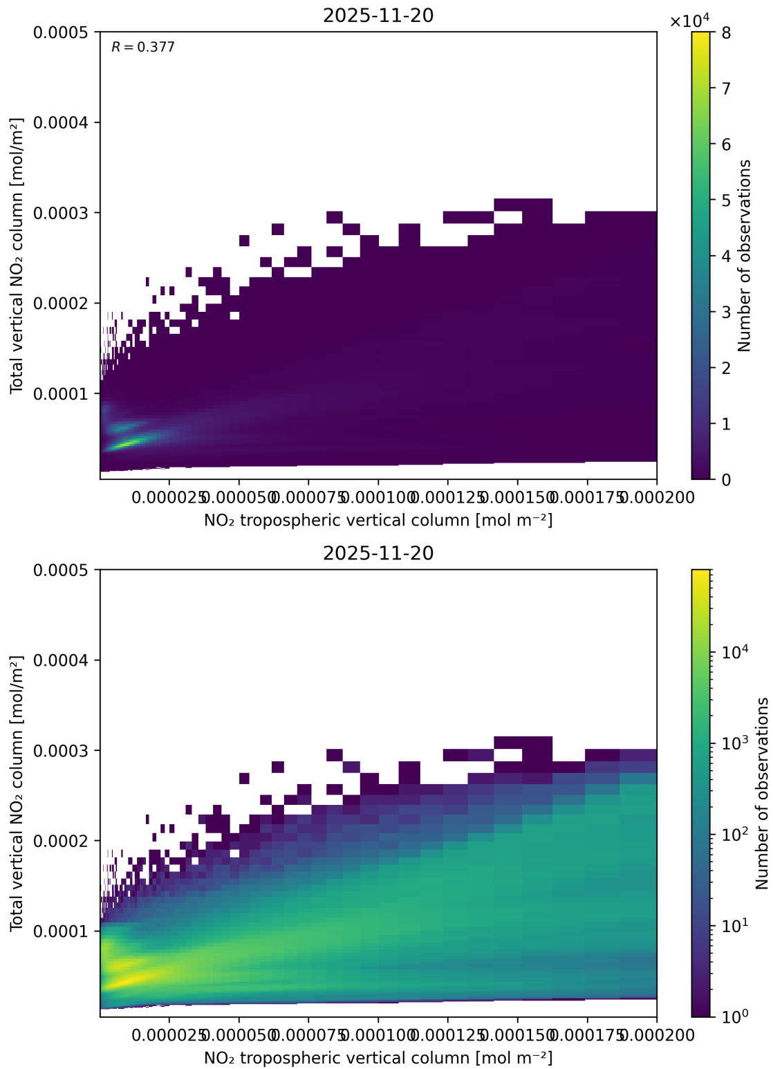
Figure 128: Scatter density plot of “NO 2 tropospheric vertical column” against “Total vertical NO 2 column” for 2025-11-19 to 2025-11-21.
