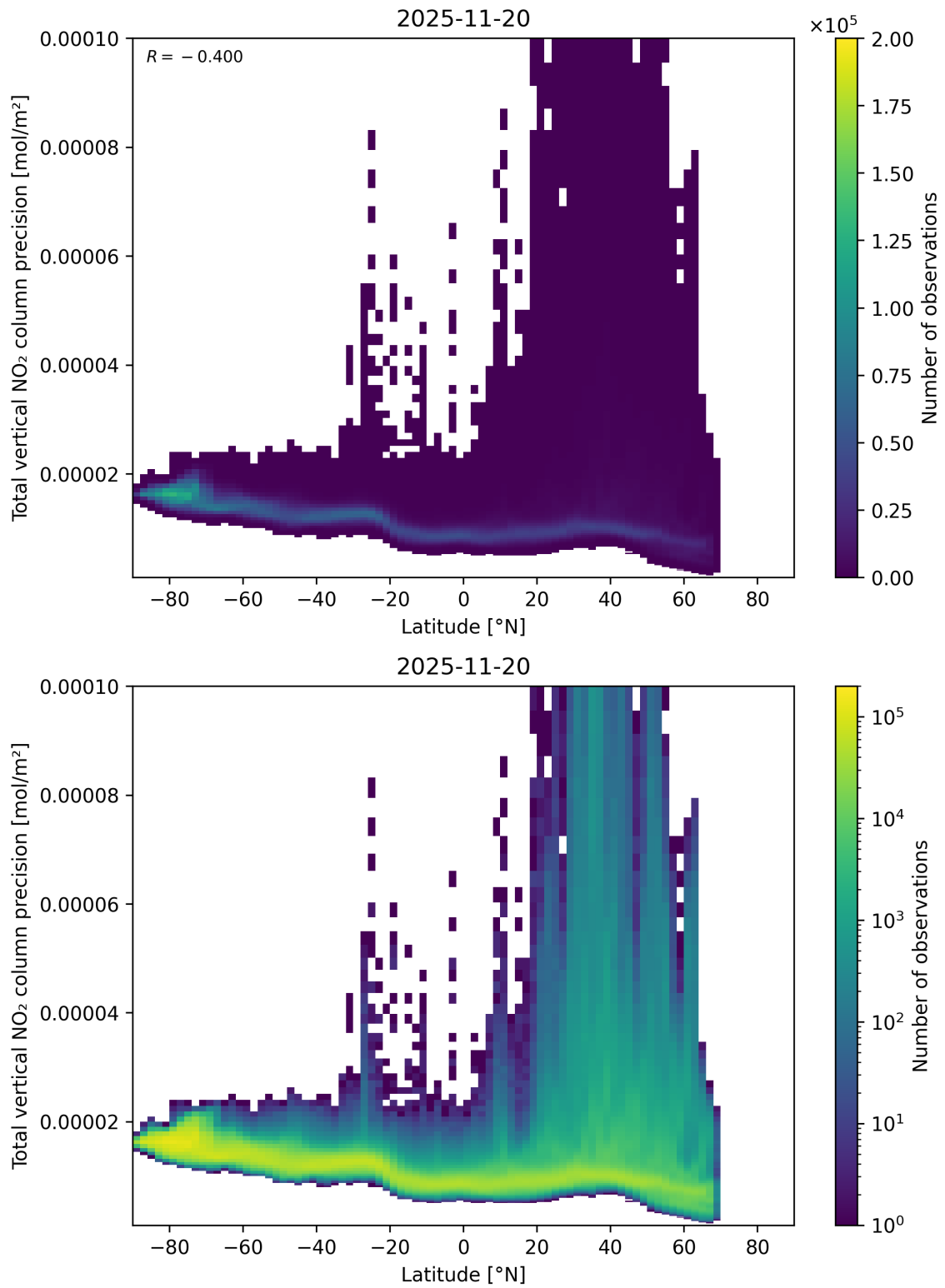
Figure 91: Scatter density plot of “Latitude” against “Total vertical NO 2 column precision” for 2025-11-19 to 2025-11-21.
