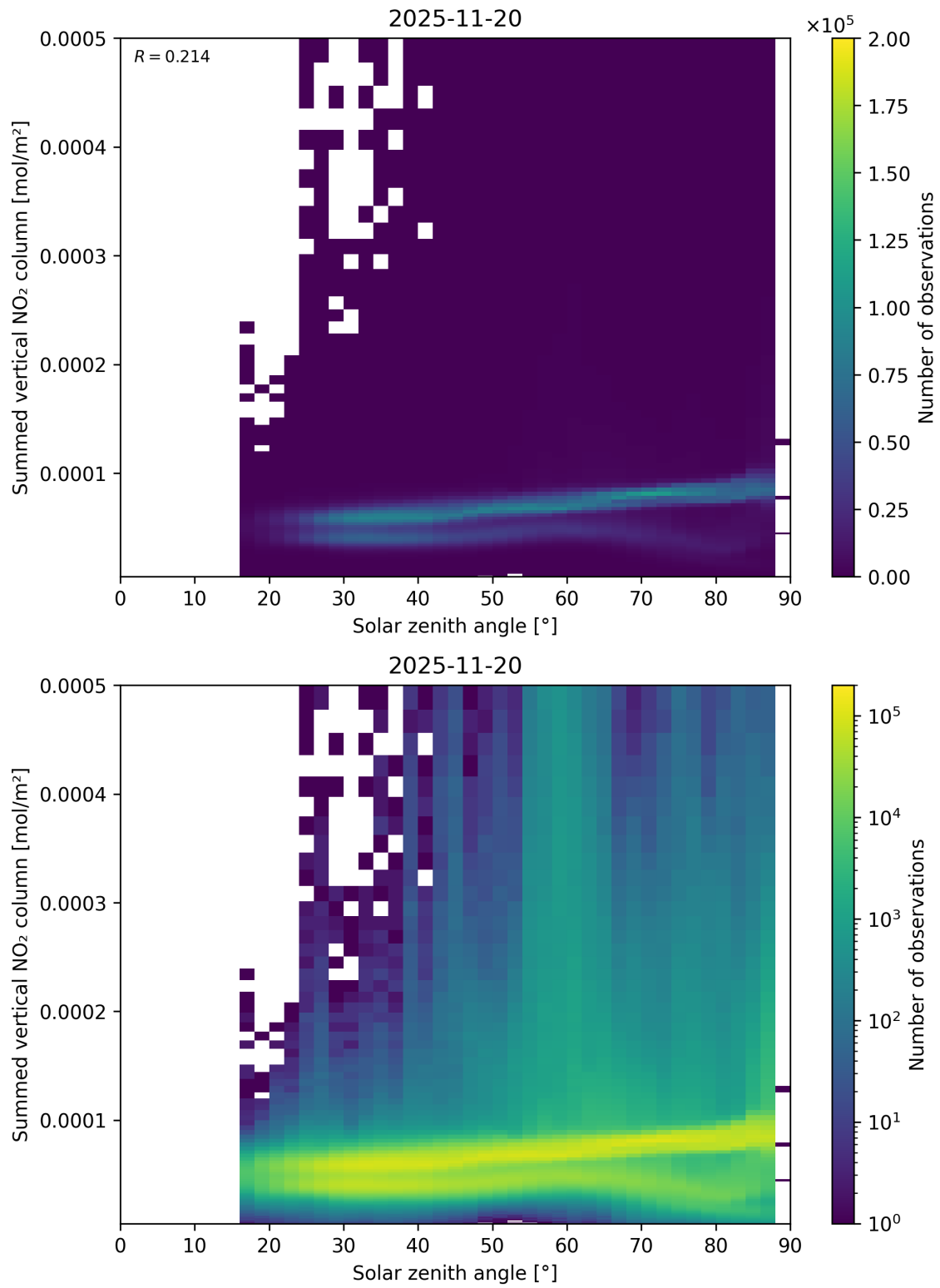
Figure 151: Scatter density plot of “Solar zenith angle” against “Summed vertical NO 2 column” for 2025-11-19 to 2025-11-21.
