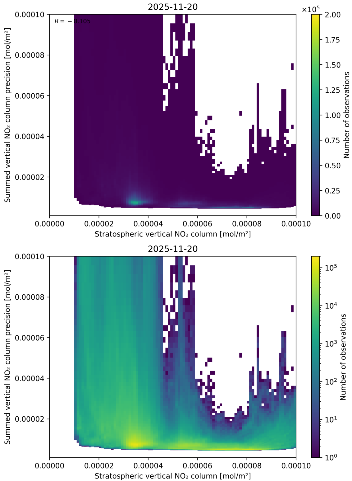
Figure 99: Scatter density plot of “Stratospheric vertical NO 2 column” against “Summed vertical NO 2 column precision” for 2025-11-19 to 2025-11-21.
