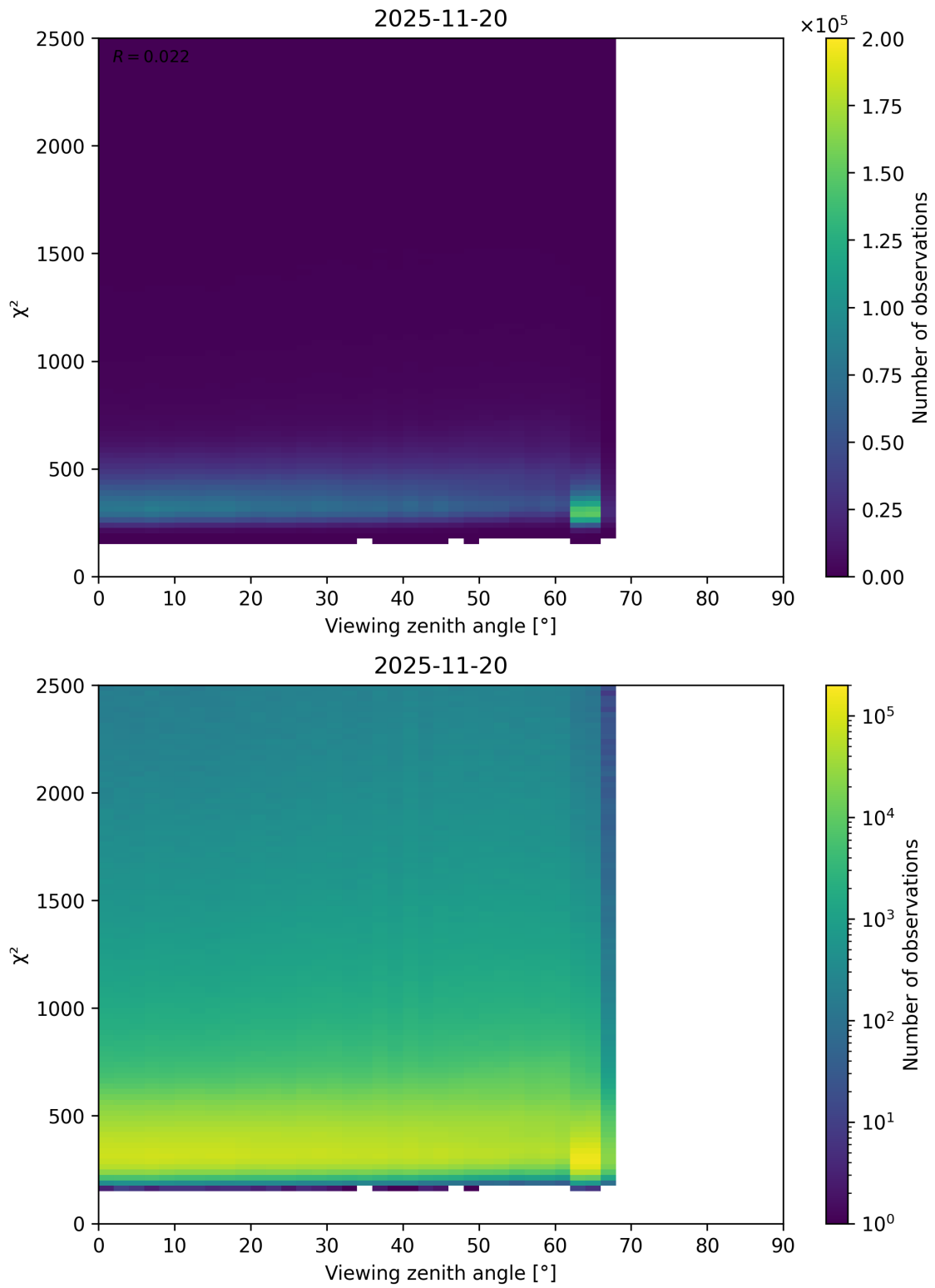
Figure 162: Scatter density plot of “Viewing zenith angle” against “ \chi^2 ” for 2025-11-19 to 2025-11-21.
