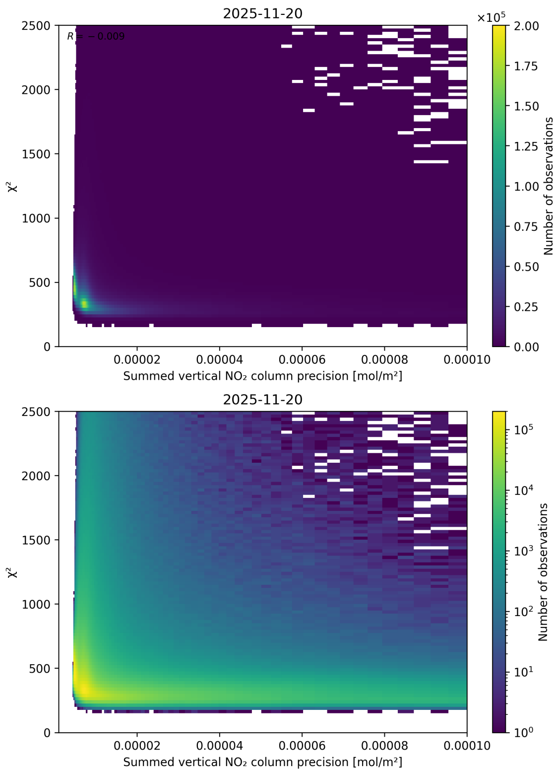
Figure 107: Scatter density plot of “Summed vertical NO 2 column precision” against “ \chi^2 ” for 2025-11-19 to 2025-11-21.
