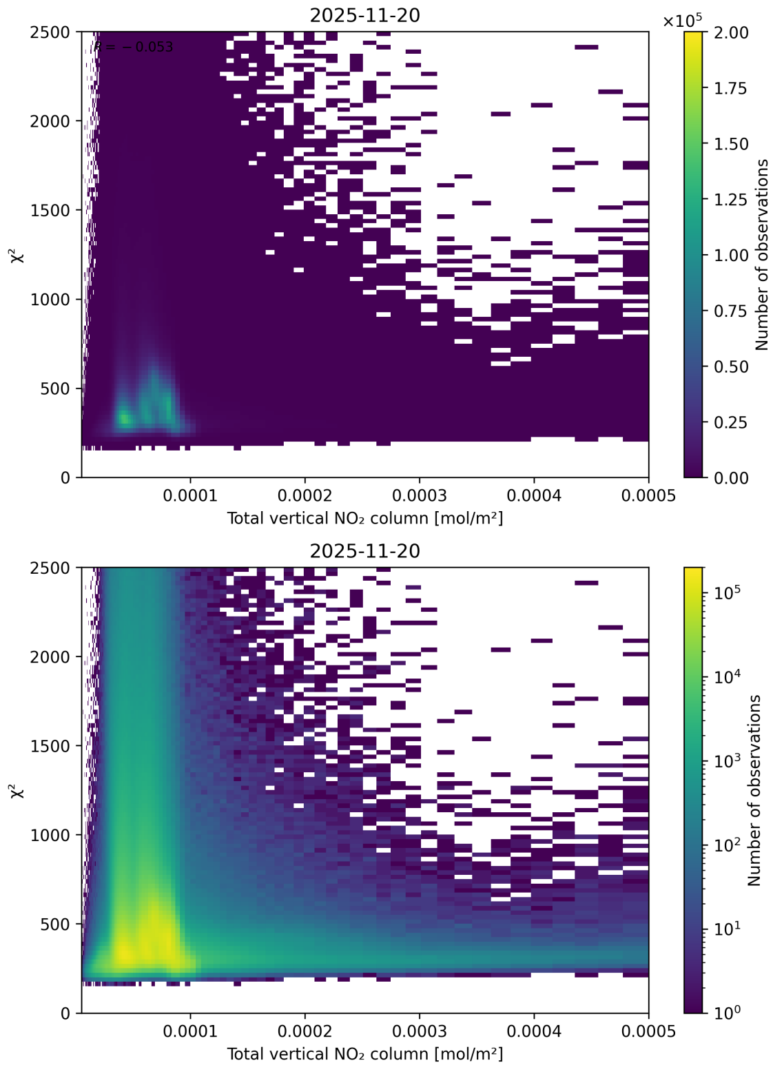
Figure 111: Scatter density plot of “Total vertical NO 2 column” against “ \chi^2 ” for 2025-11-19 to 2025-11-21.
