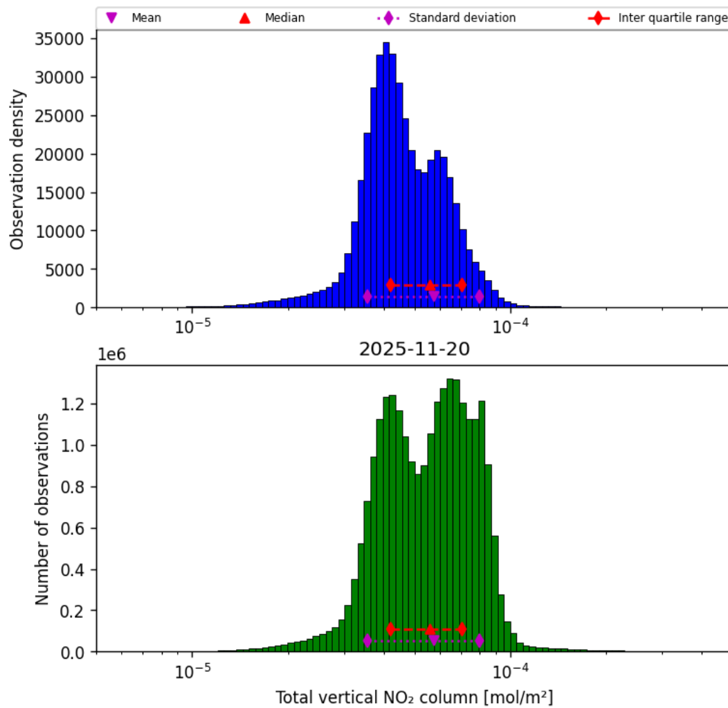
Figure 38: Histogram of "Total vertical NO 2 column" for 2025-11-19 to 2025-11-21
