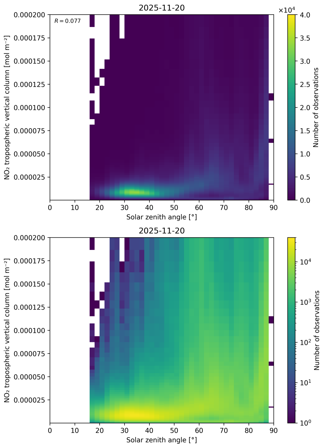
Figure 155: Scatter density plot of “Solar zenith angle” against “NO 2 tropospheric vertical column” for 2025-11-19 to 2025-11-21.
