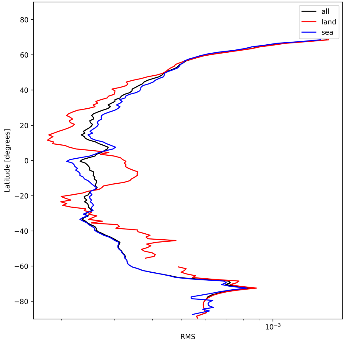
Figure 26: Zonal average of “RMS” for 2025-11-19 to 2025-11-21.
