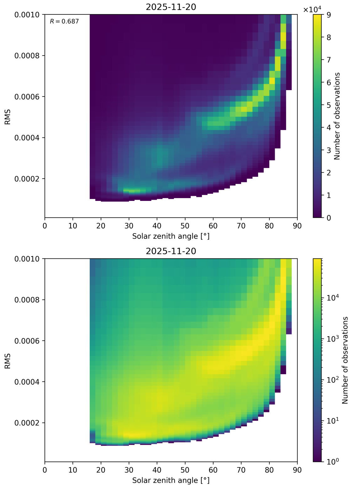
Figure 157: Scatter density plot of “Solar zenith angle” against “RMS” for 2025-11-19 to 2025-11-21.
