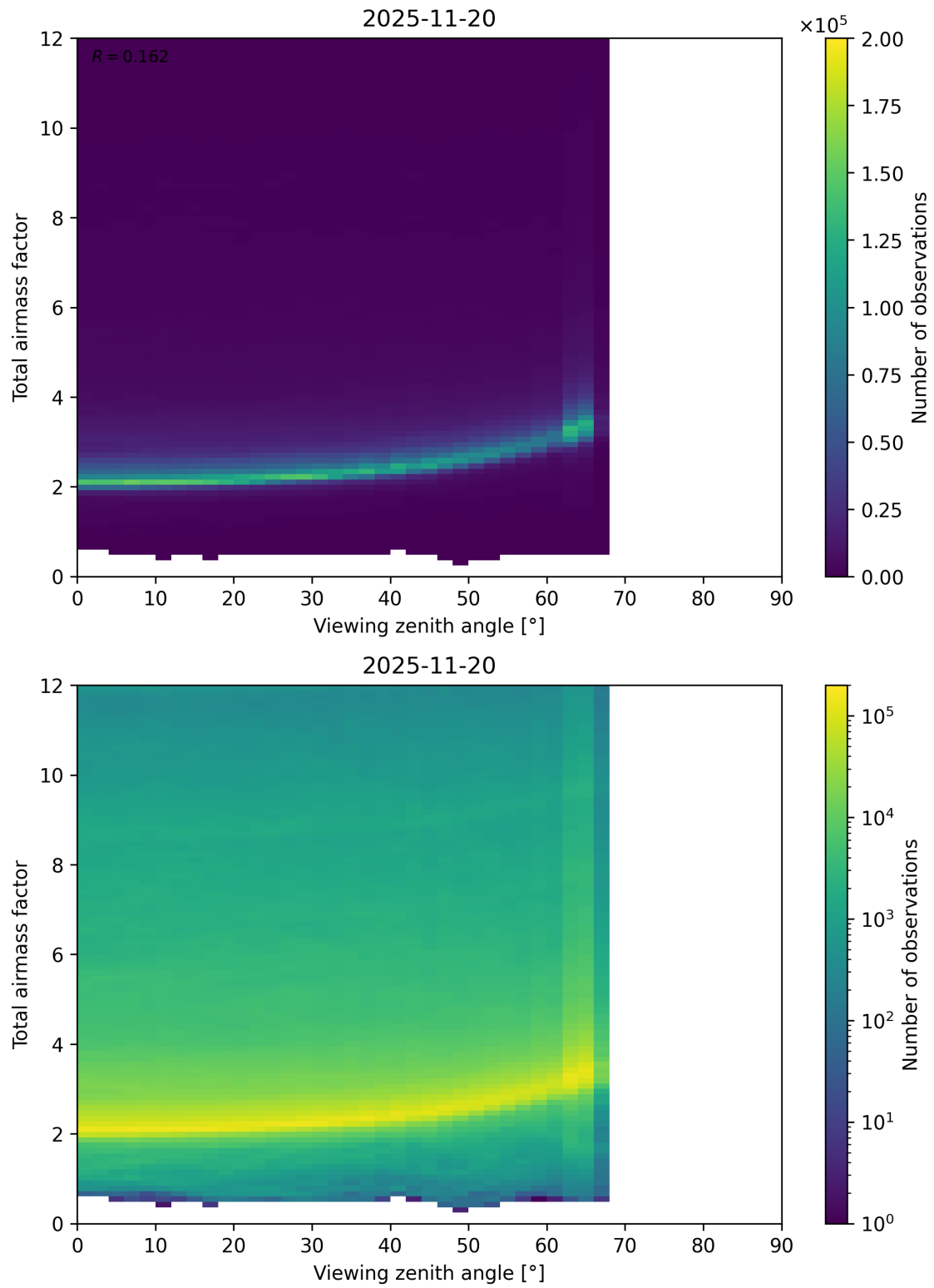
Figure 160: Scatter density plot of “Viewing zenith angle” against “Total airmass factor” for 2025-11-19 to 2025-11-21.
