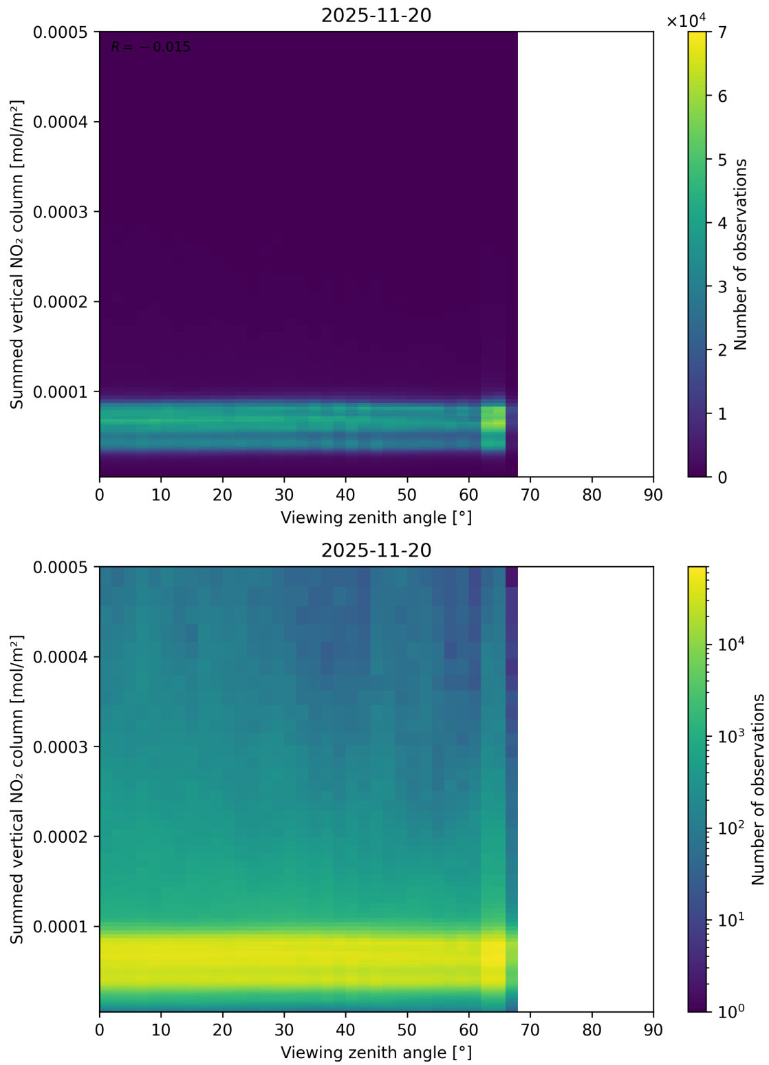
Figure 165: Scatter density plot of “Viewing zenith angle” against “Summed vertical NO 2 column” for 2025-11-19 to 2025-11-21.
