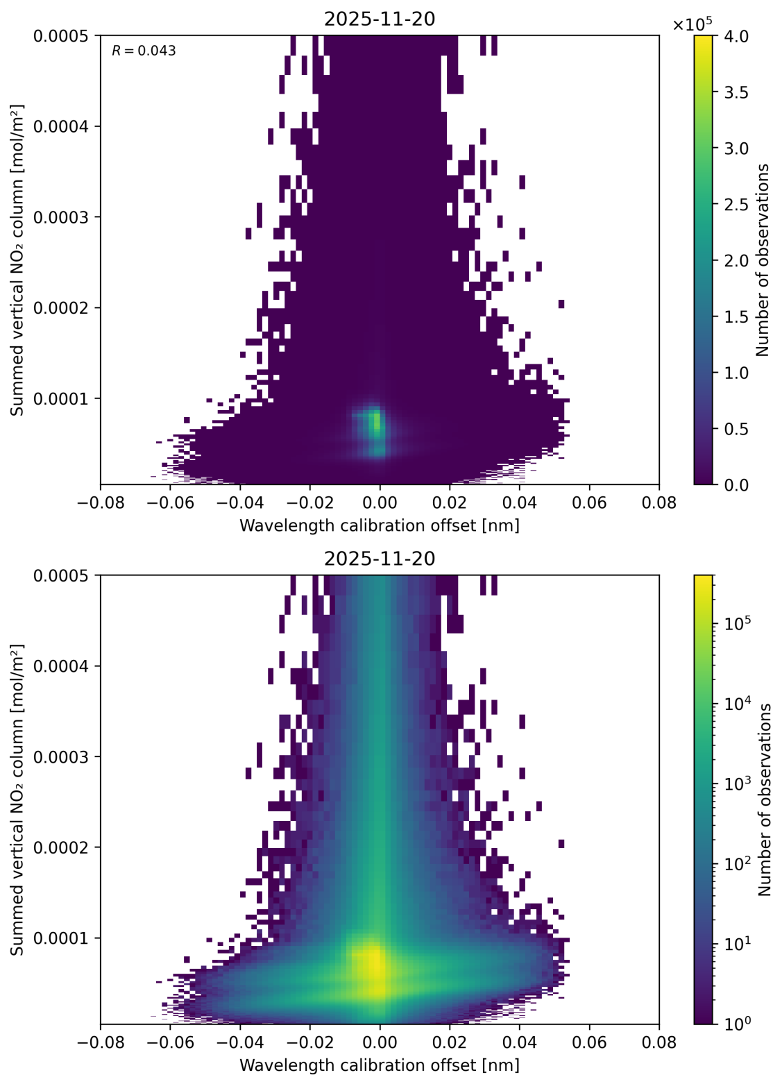
Figure 177: Scatter density plot of “Wavelength calibration offset” against “Summed vertical NO 2 column” for 2025-11-19 to 2025-11-21.
