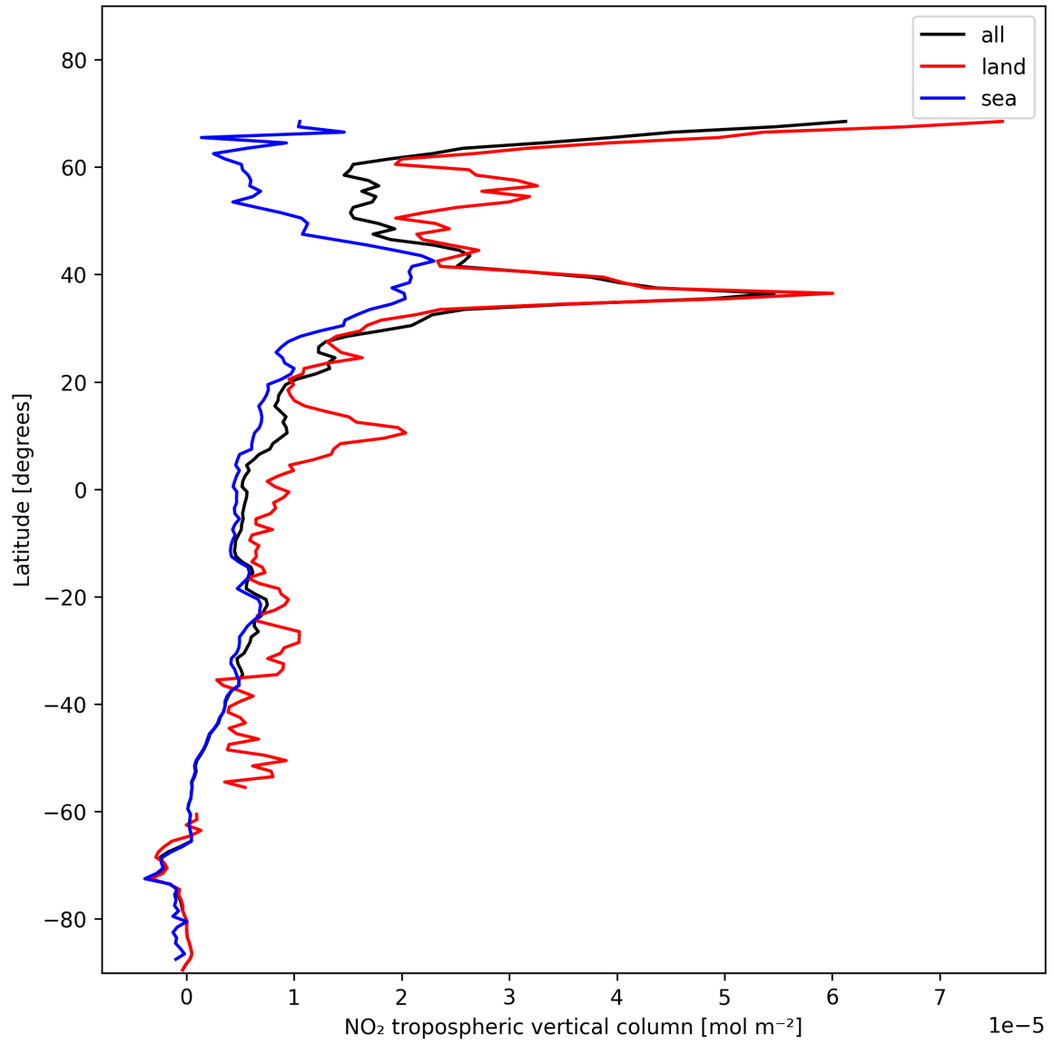
Figure 12: Zonal average of “NO 2 tropospheric vertical column” for 2025-11-19 to 2025-11-21.
