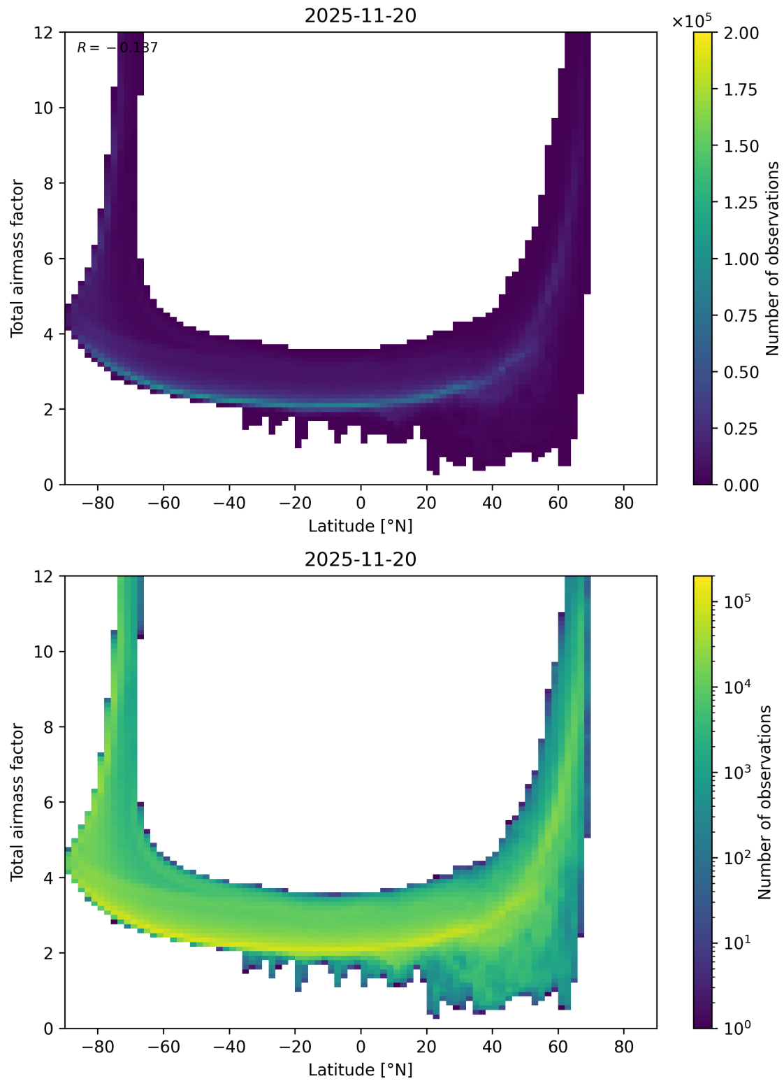
Figure 84: Scatter density plot of “Latitude” against “Total airmass factor” for 2025-11-19 to 2025-11-21.
