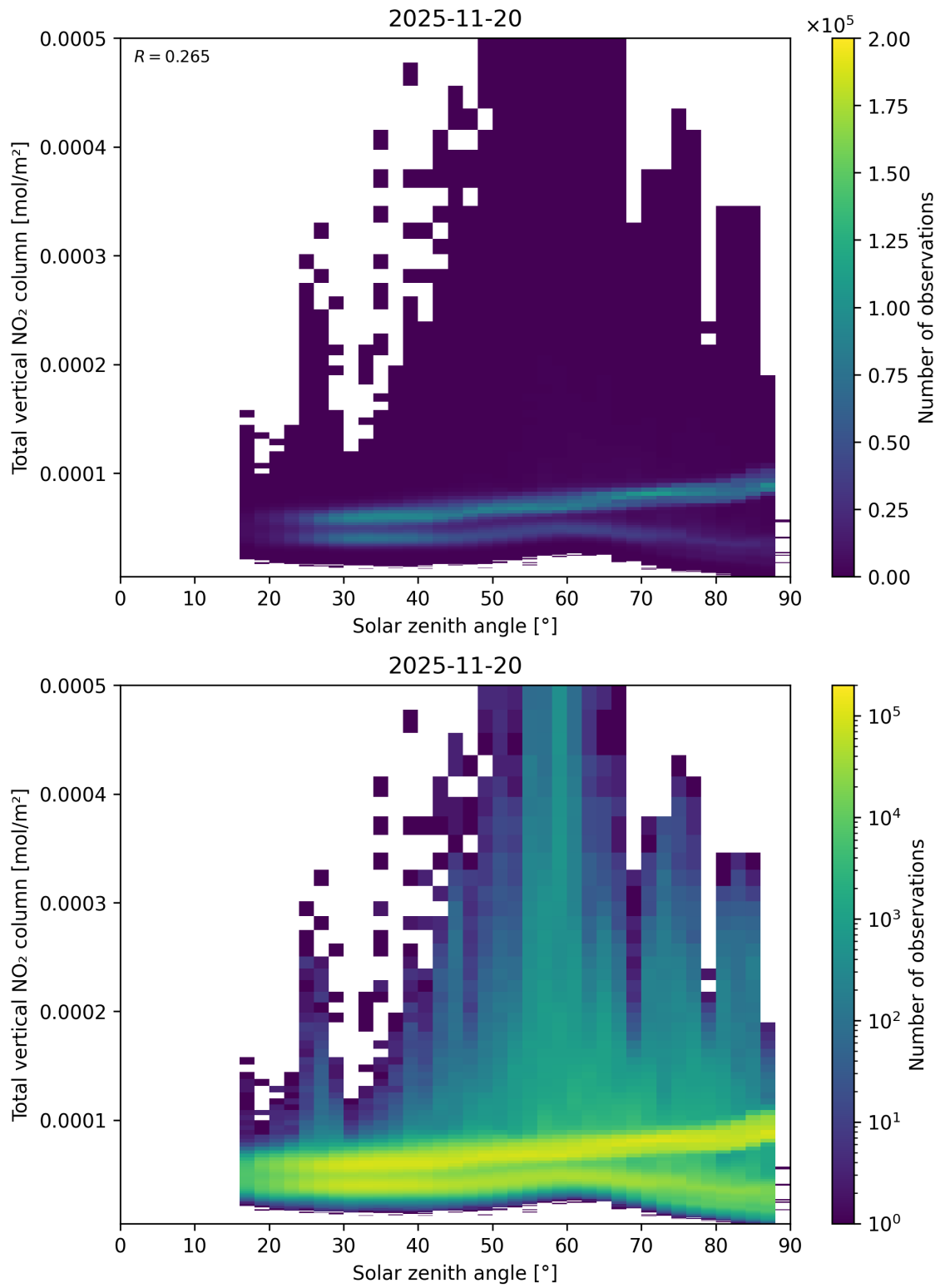
Figure 153: Scatter density plot of “Solar zenith angle” against “Total vertical NO 2 column” for 2025-11-19 to 2025-11-21.
