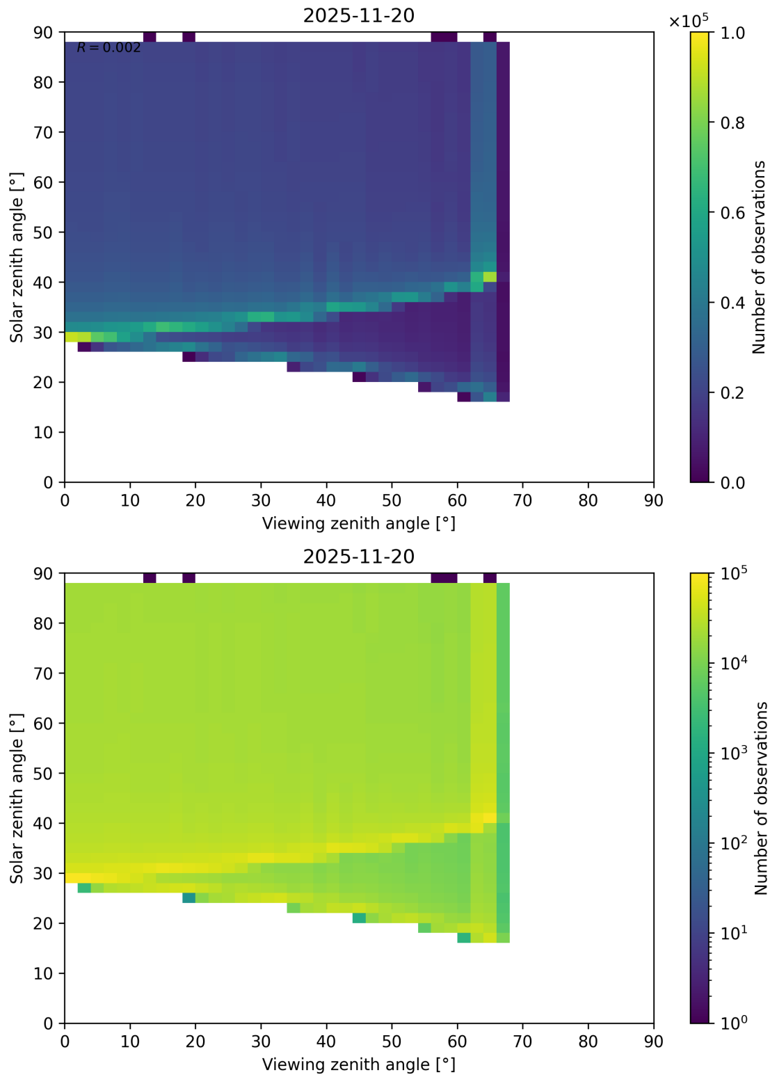
Figure 172: Scatter density plot of “Viewing zenith angle” against “Solar zenith angle” for 2025-11-19 to 2025-11-21.
