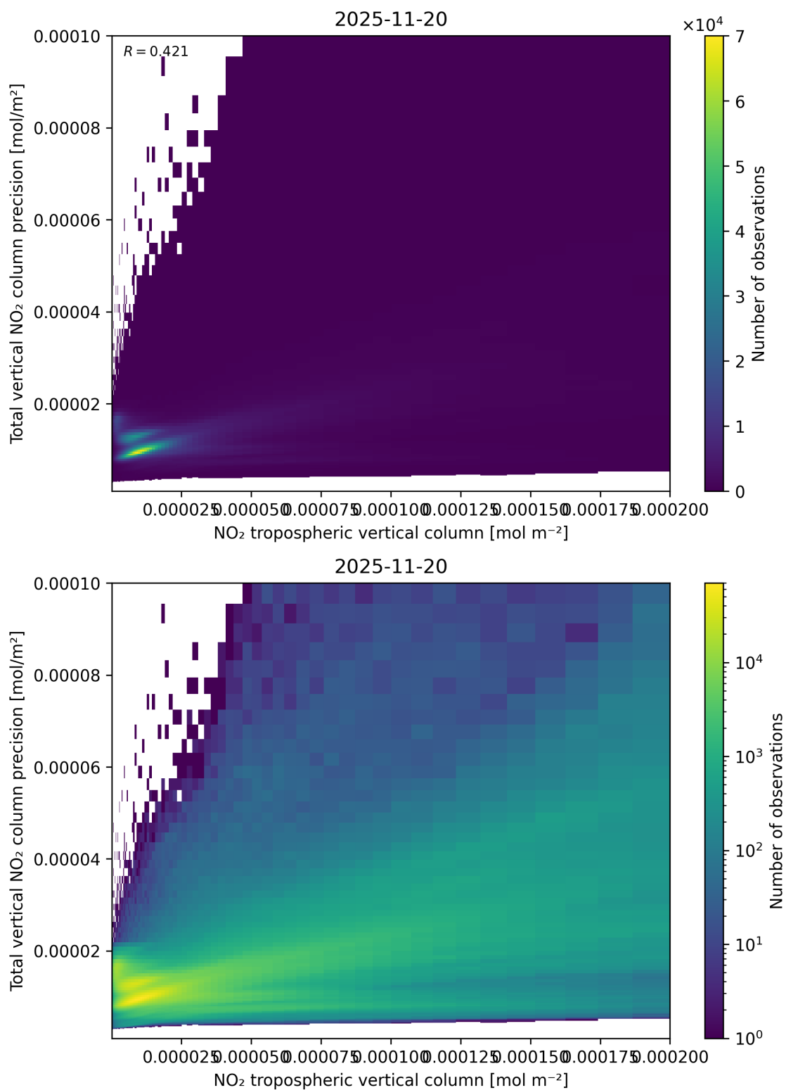
Figure 129: Scatter density plot of “NO 2 tropospheric vertical column” against “Total vertical NO 2 column precision” for 2025-11-19 to 2025-11-21.
