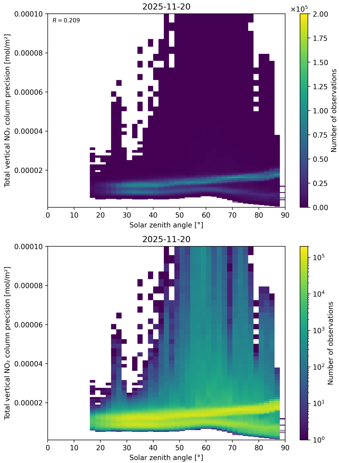
Figure 154: Scatter density plot of “Solar zenith angle” against “Total vertical NO 2 column precision” for 2025-11-19 to 2025-11-21.
