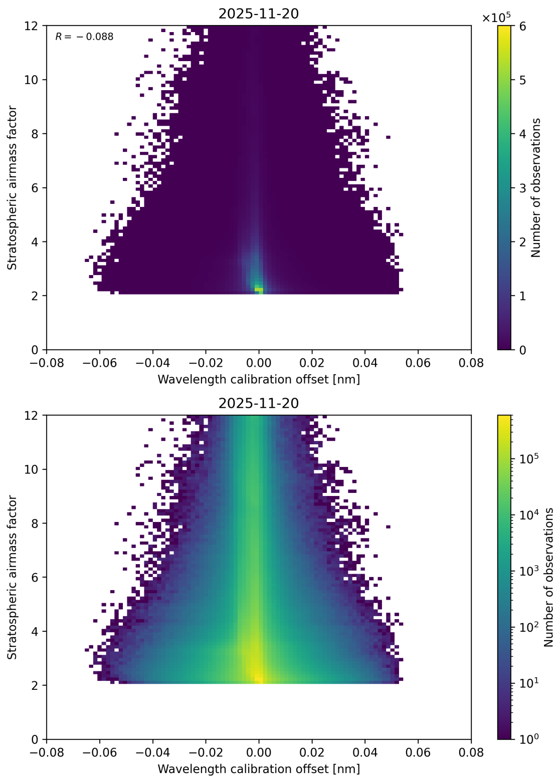
Figure 174: Scatter density plot of “Wavelength calibration offset” against “Stratospheric airmass factor” for 2025-11-19 to 2025-11-21.
