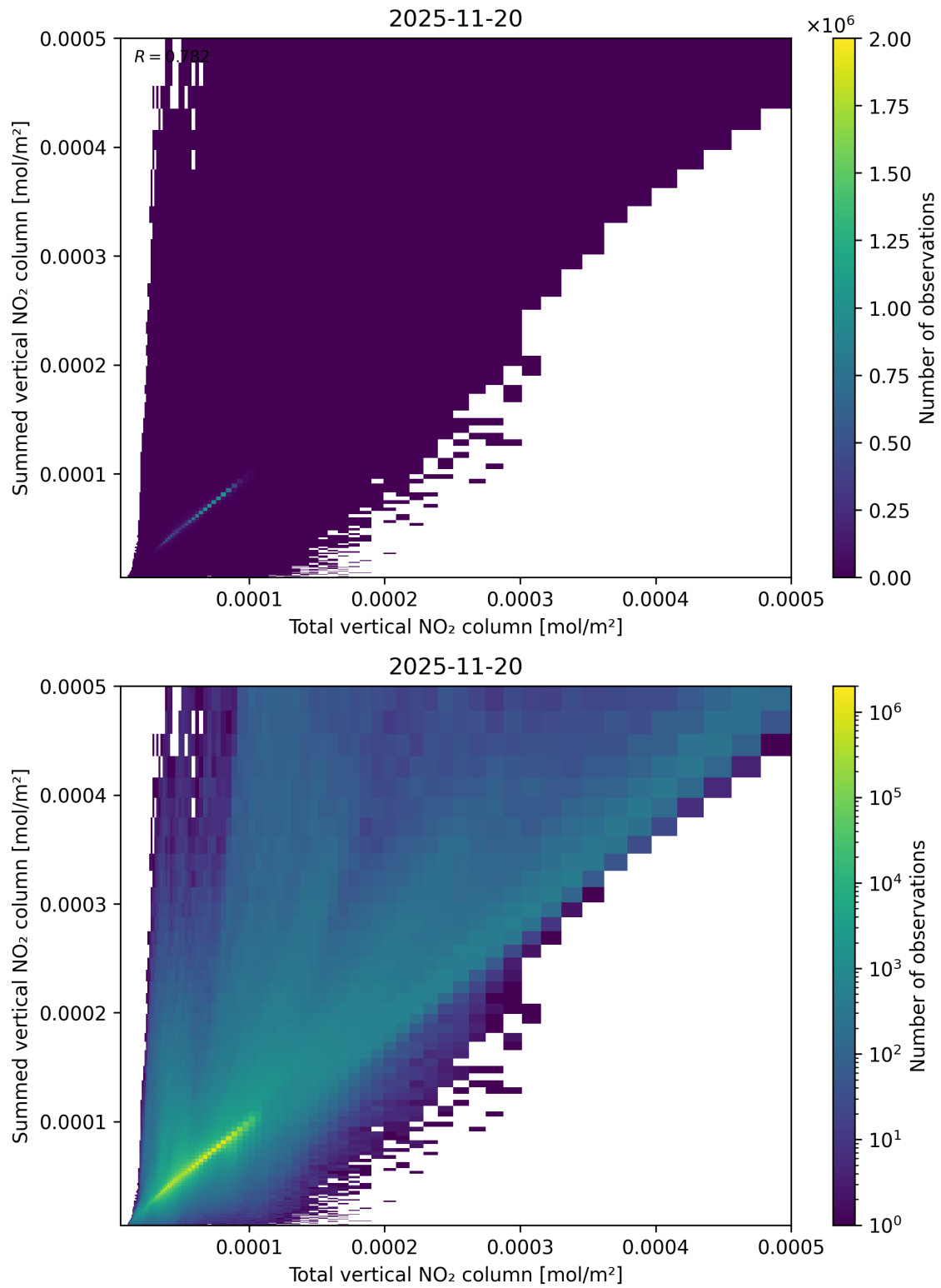
Figure 112: Scatter density plot of “Total vertical NO 2 column” against “Summed vertical NO 2 column” for 2025-11-19 to 2025-11-21.
