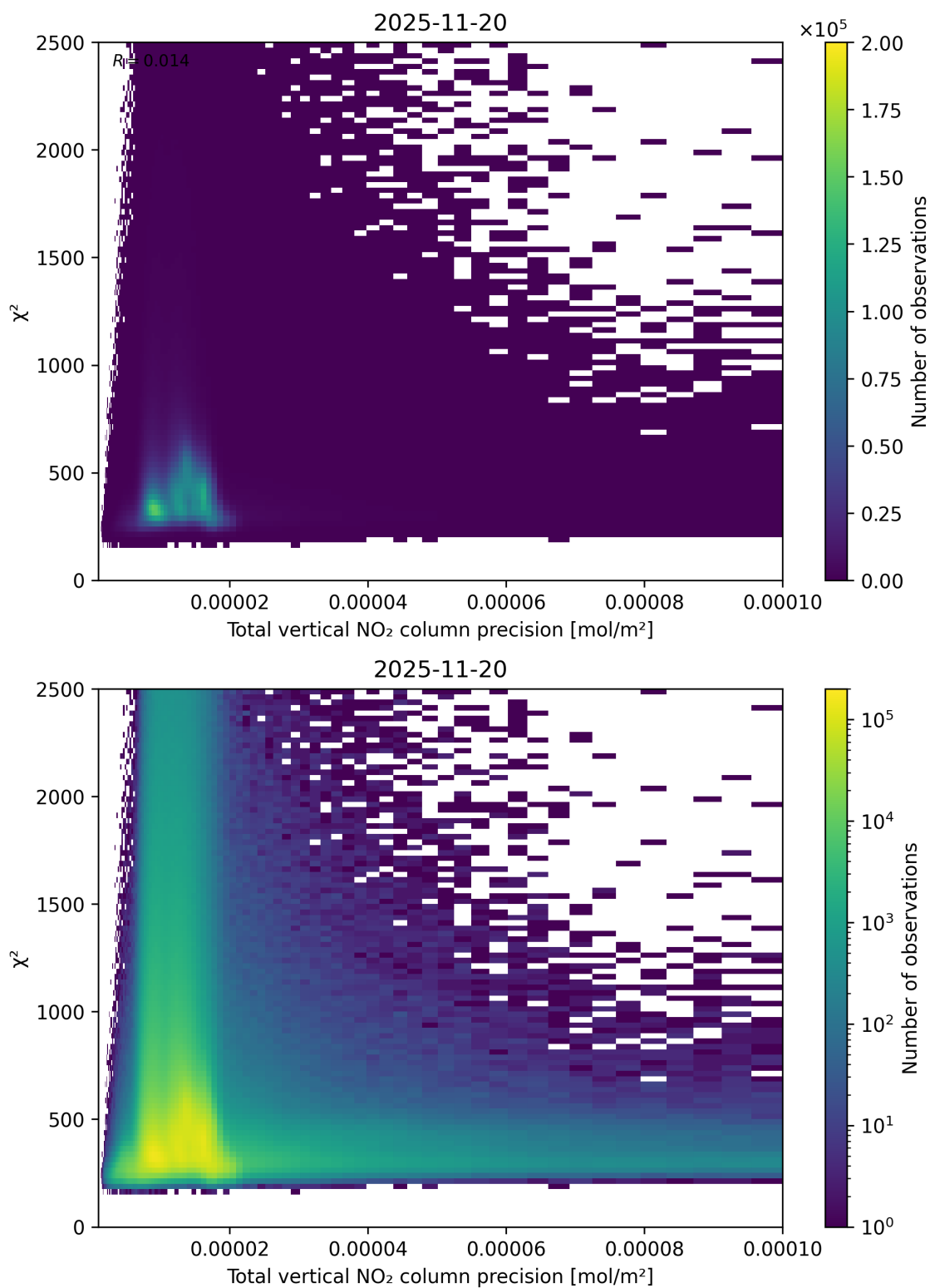
Figure 116: Scatter density plot of “Total vertical NO 2 column precision” against “ \chi^2 ” for 2025-11-19 to 2025-11-21.
