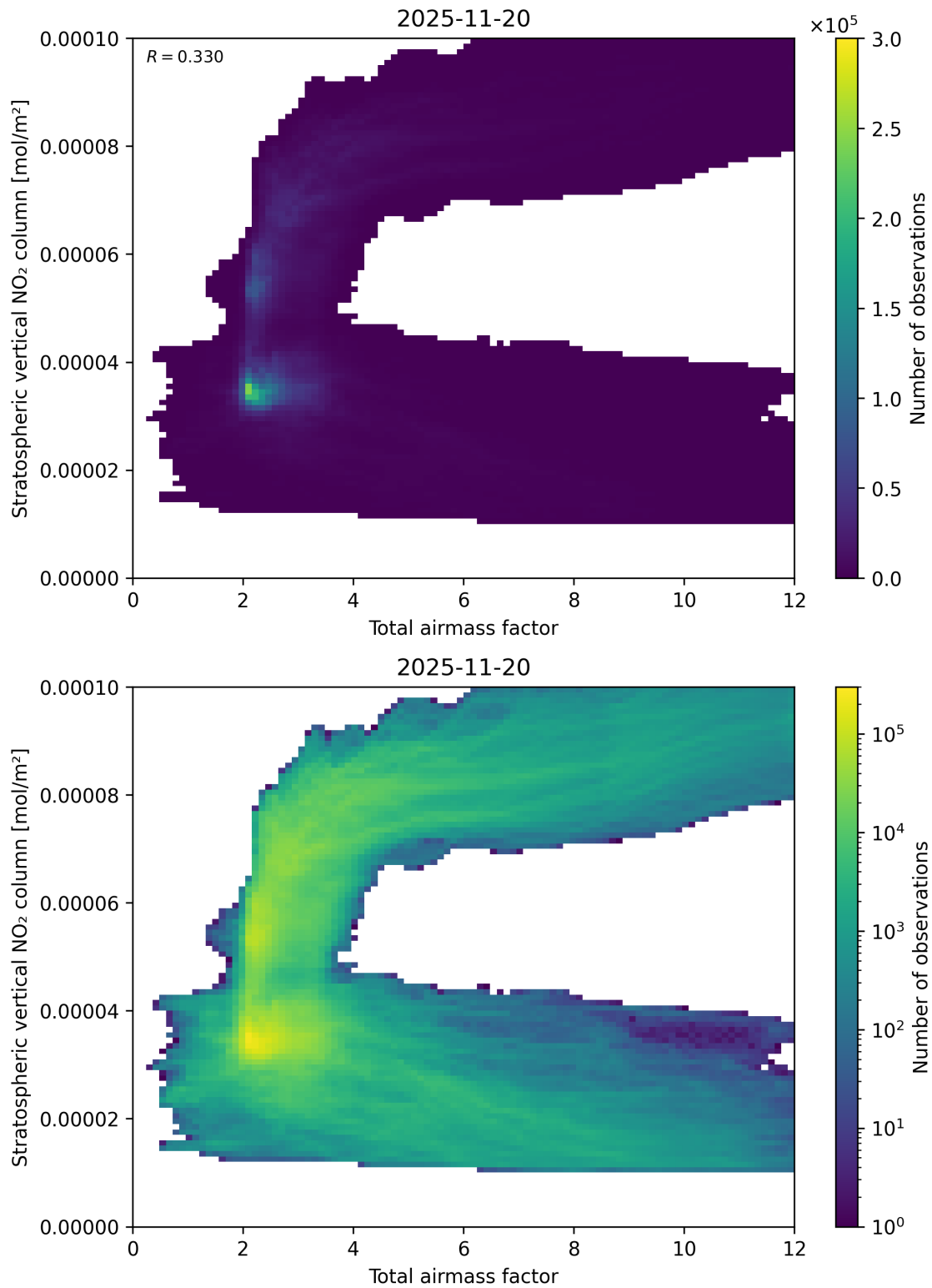
Figure 64: Scatter density plot of “Total airmass factor” against “Stratospheric vertical \text{NO}_2 column” for 2025-11-19 to 2025-11-21.
