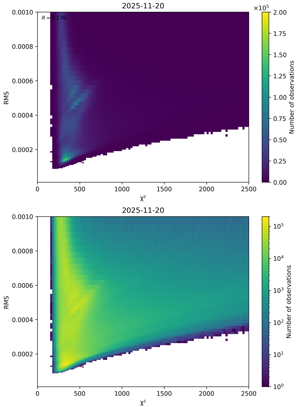
Figure 82: Scatter density plot of “ \chi^2 ” against “RMS” for 2025-11-19 to 2025-11-21.
