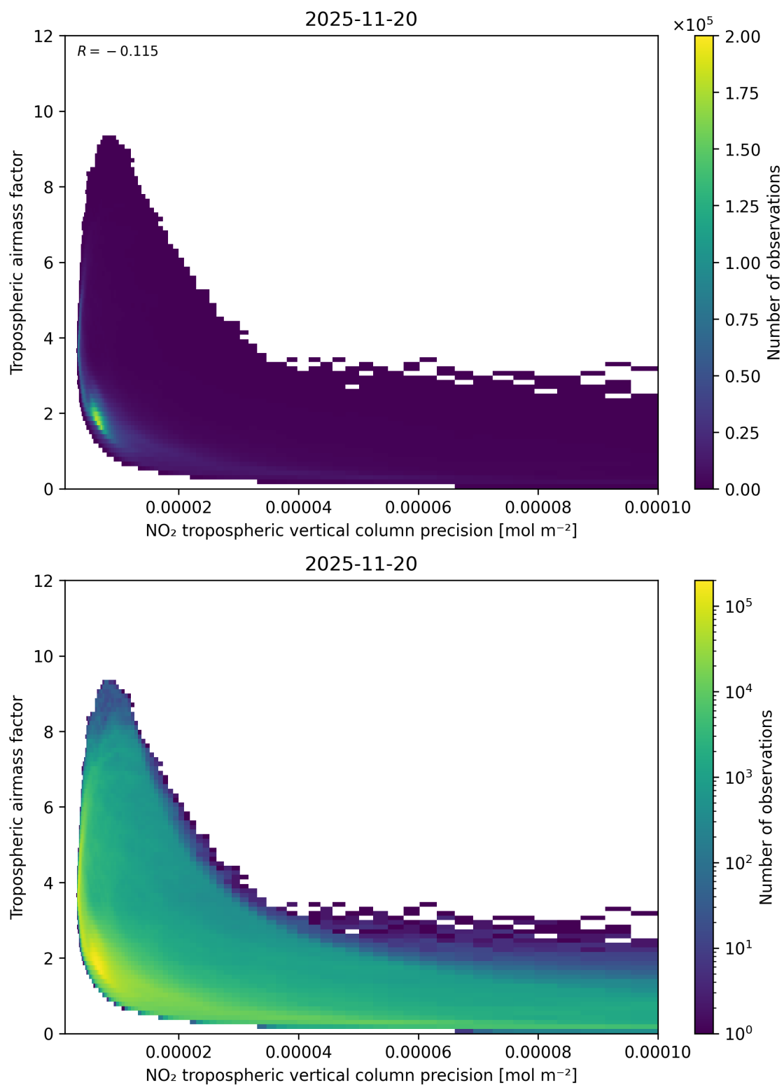
Figure 133: Scatter density plot of “NO 2 tropospheric vertical column precision” against “Tropospheric airmass factor” for 2025-11-19 to 2025-11-21.
