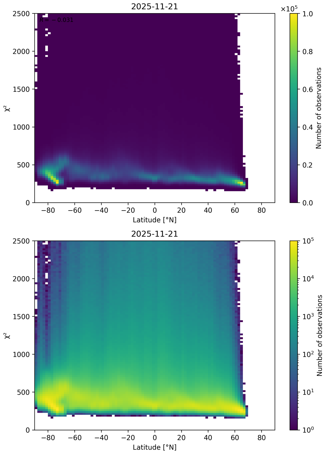
Figure 86: Scatter density plot of “Latitude” against “ \chi^2 ” for 2025-11-20 to 2025-11-22.
