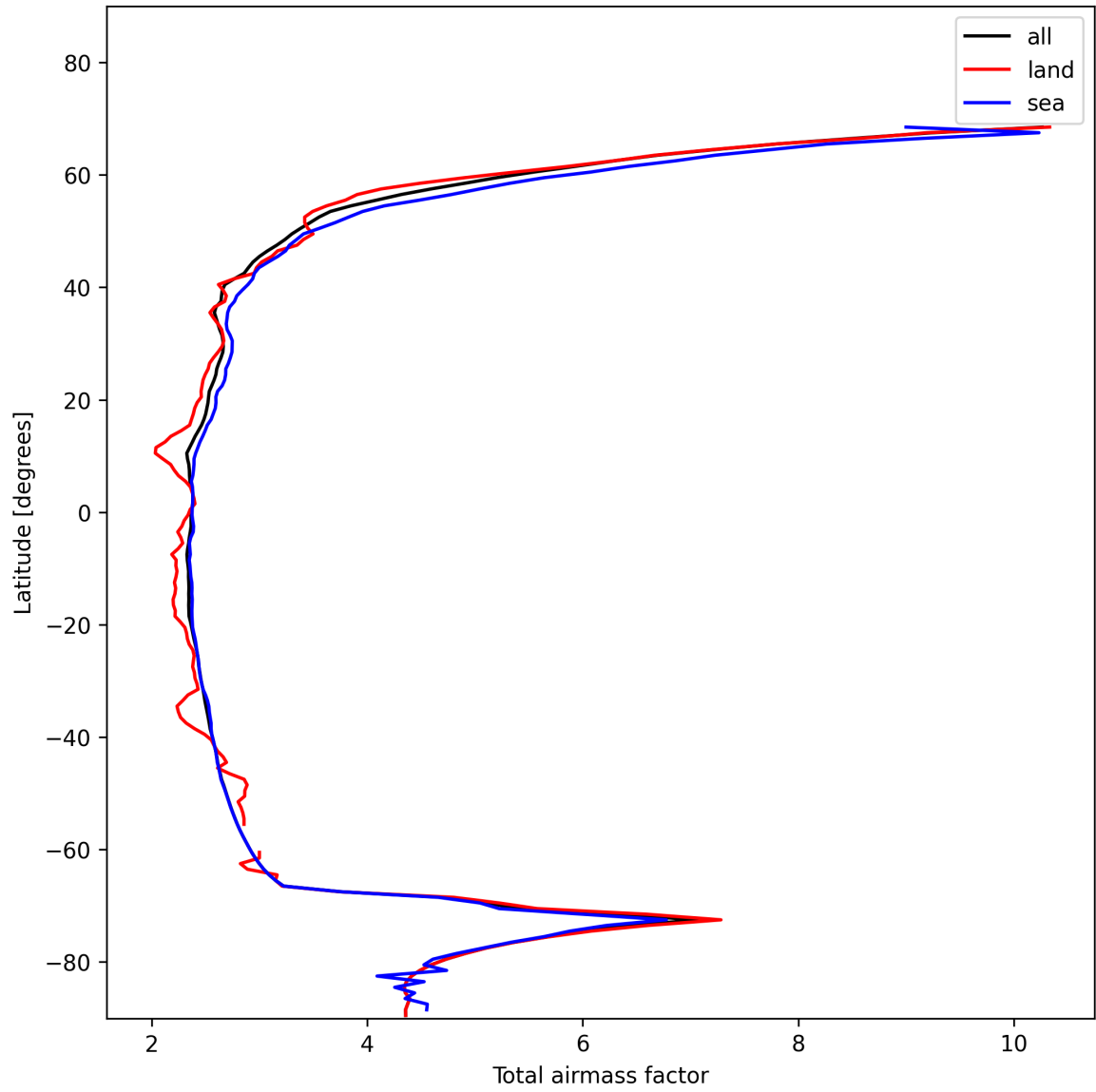
Figure 15: Zonal average of “Total airmass factor” for 2025-11-20 to 2025-11-22.
