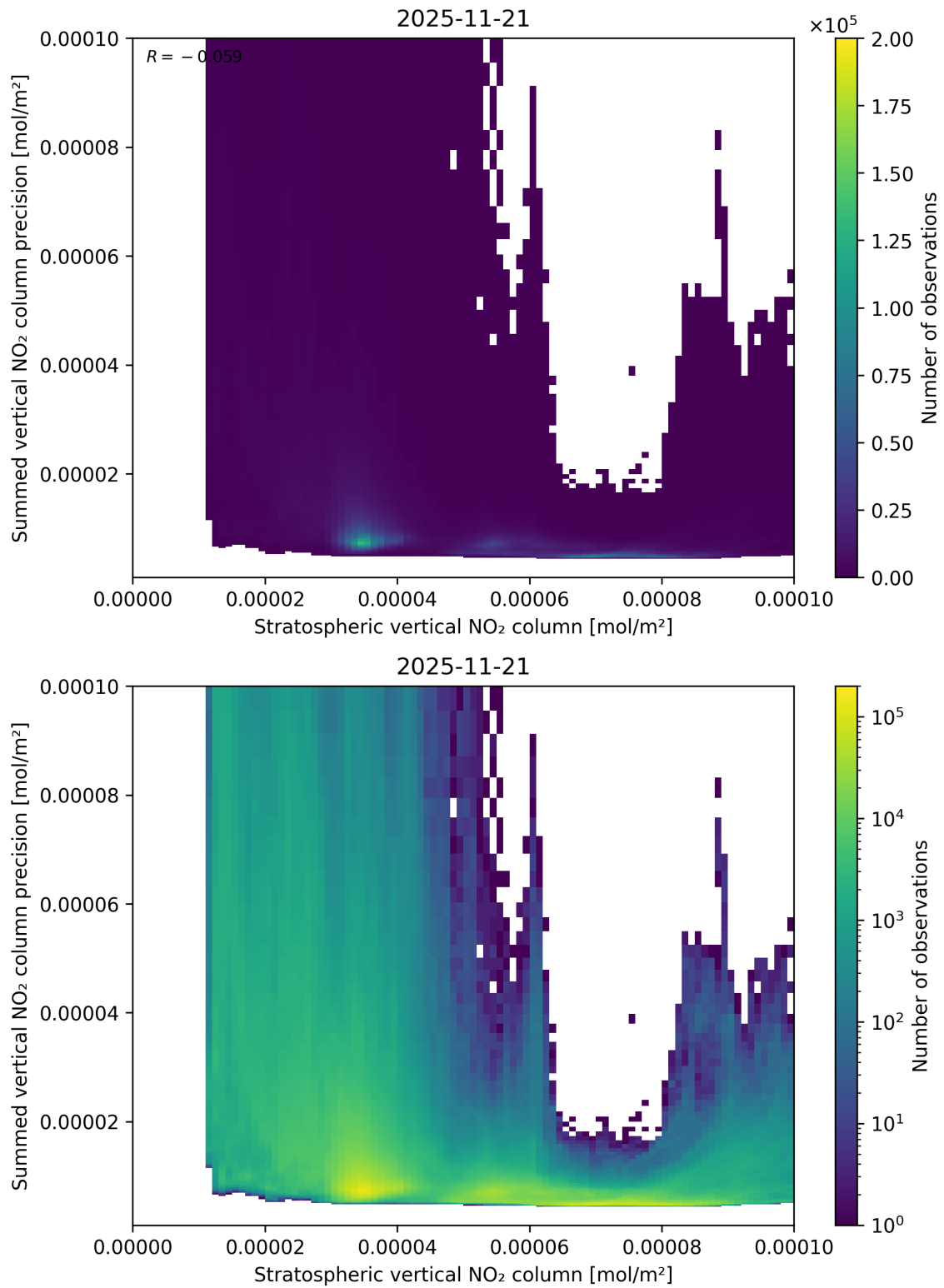
Figure 99: Scatter density plot of “Stratospheric vertical NO 2 column” against “Summed vertical NO 2 column precision” for 2025-11-20 to 2025-11-22.
