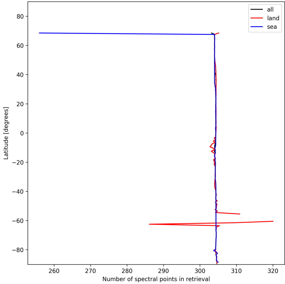
Figure 16: Zonal average of “Number of spectral points in retrieval” for 2025-11-20 to 2025-11-22.
