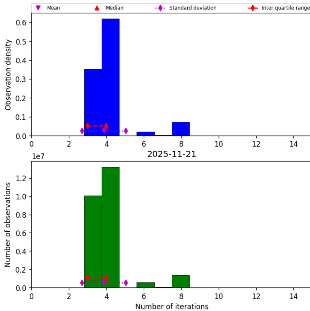
Figure 34: Histogram of “Number of iterations” for 2025-11-20 to 2025-11-22
