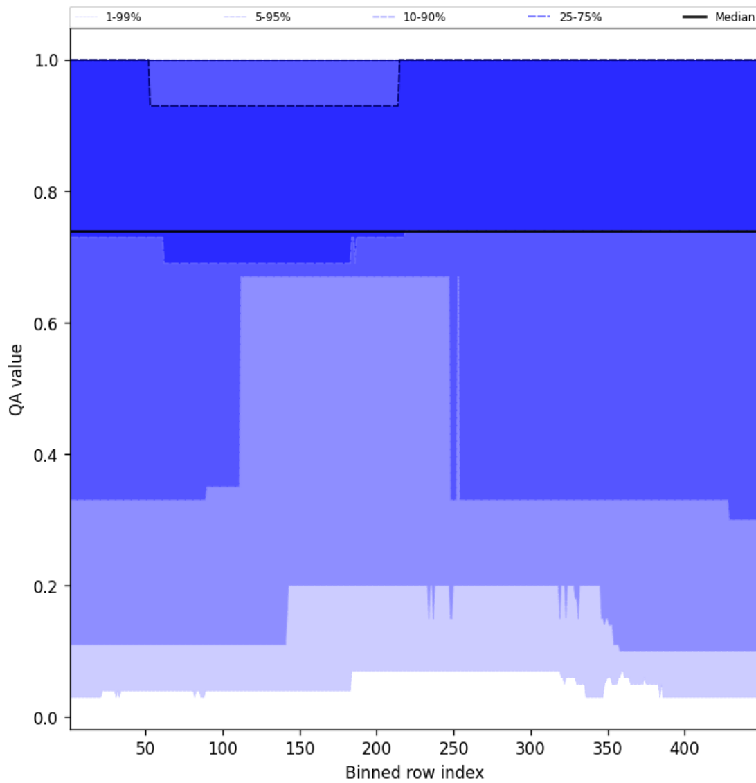
Figure 45: Along track statistics of “QA value” for 2025-11-20 to 2025-11-22
