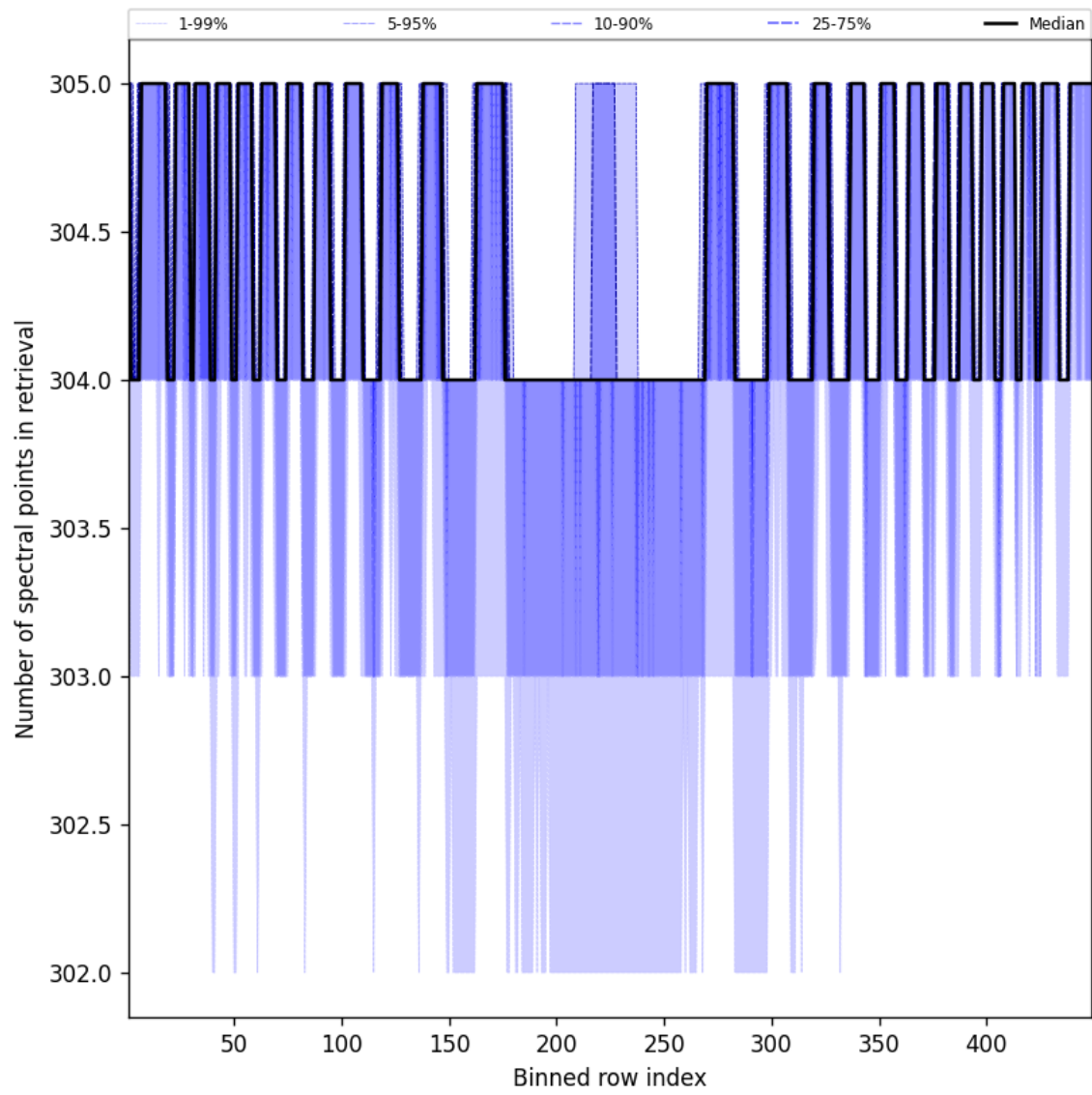
Figure 50: Along track statistics of “Number of spectral points in retrieval” for 2025-11-20 to 2025-11-22
