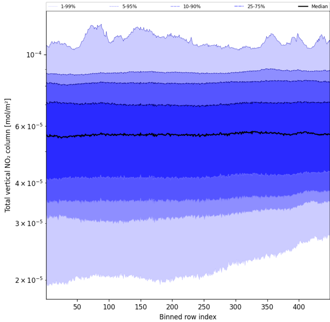
Figure 55: Along track statistics of “Total vertical NO 2 column” for 2025-11-20 to 2025-11-22
