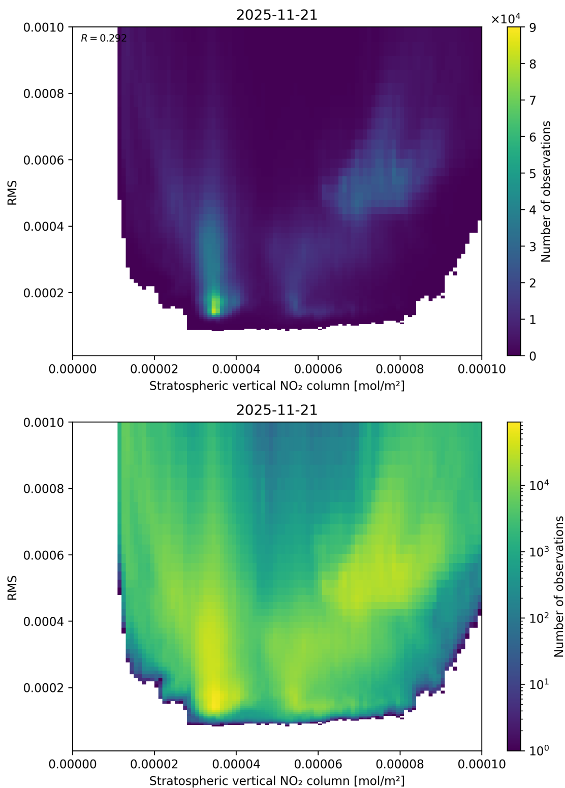
Figure 102: Scatter density plot of “Stratospheric vertical NO 2 column” against “RMS” for 2025-11-20 to 2025-11-22.
