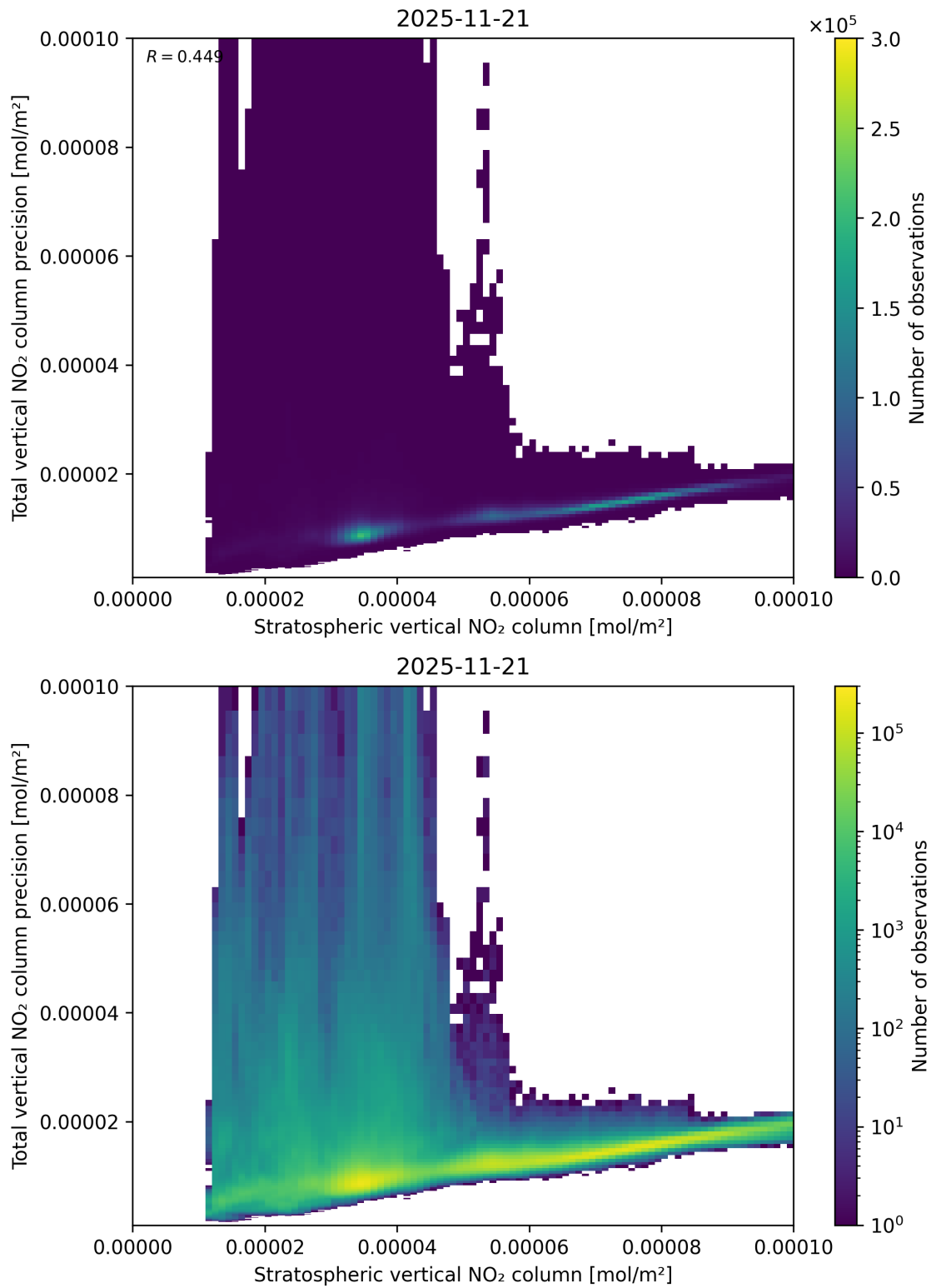
Figure 101: Scatter density plot of “Stratospheric vertical NO 2 column” against “Total vertical NO 2 column precision” for 2025-11-20 to 2025-11-22.
