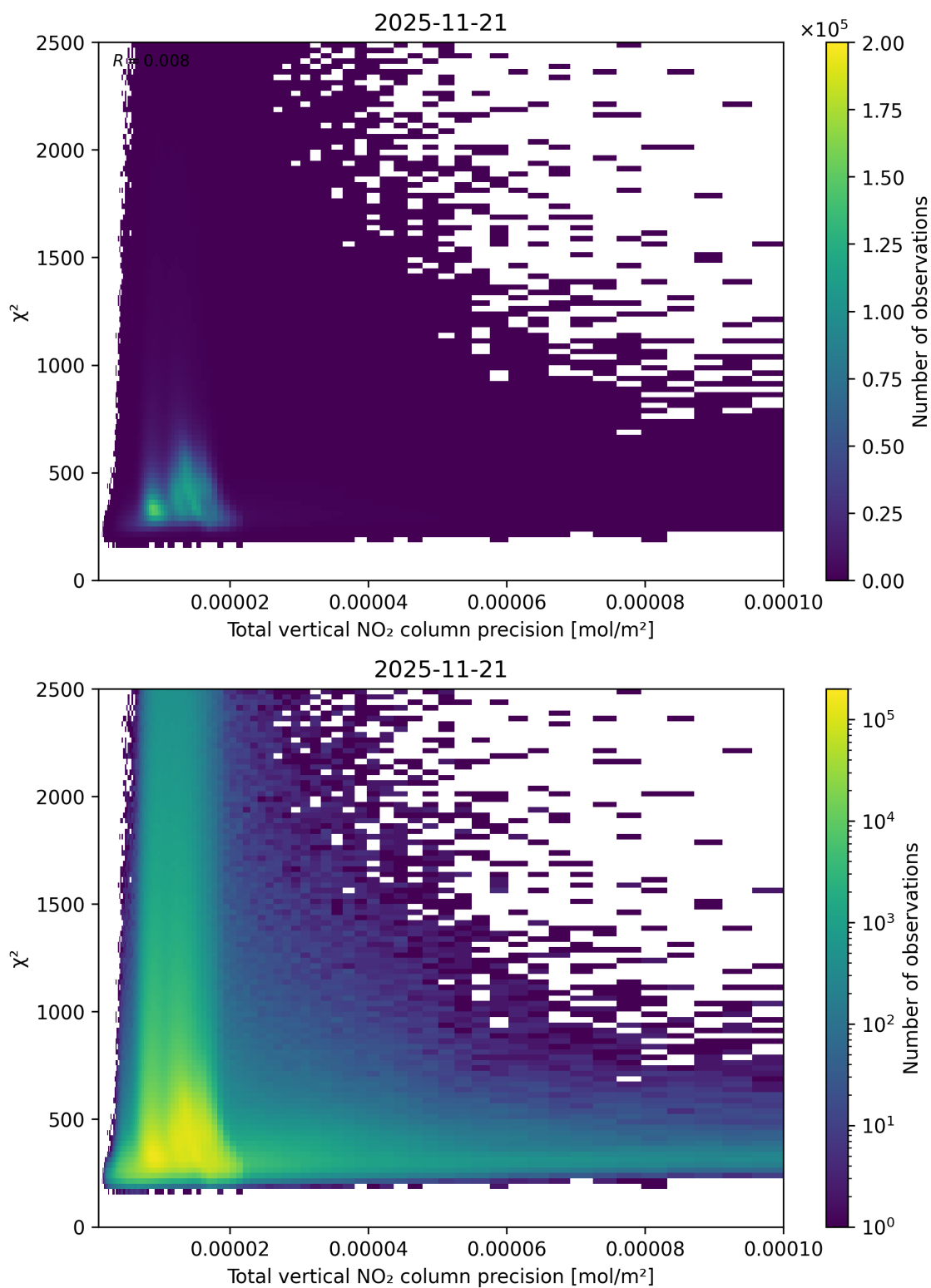
Figure 116: Scatter density plot of “Total vertical NO 2 column precision” against “ \chi^2 ” for 2025-11-20 to 2025-11-22.
