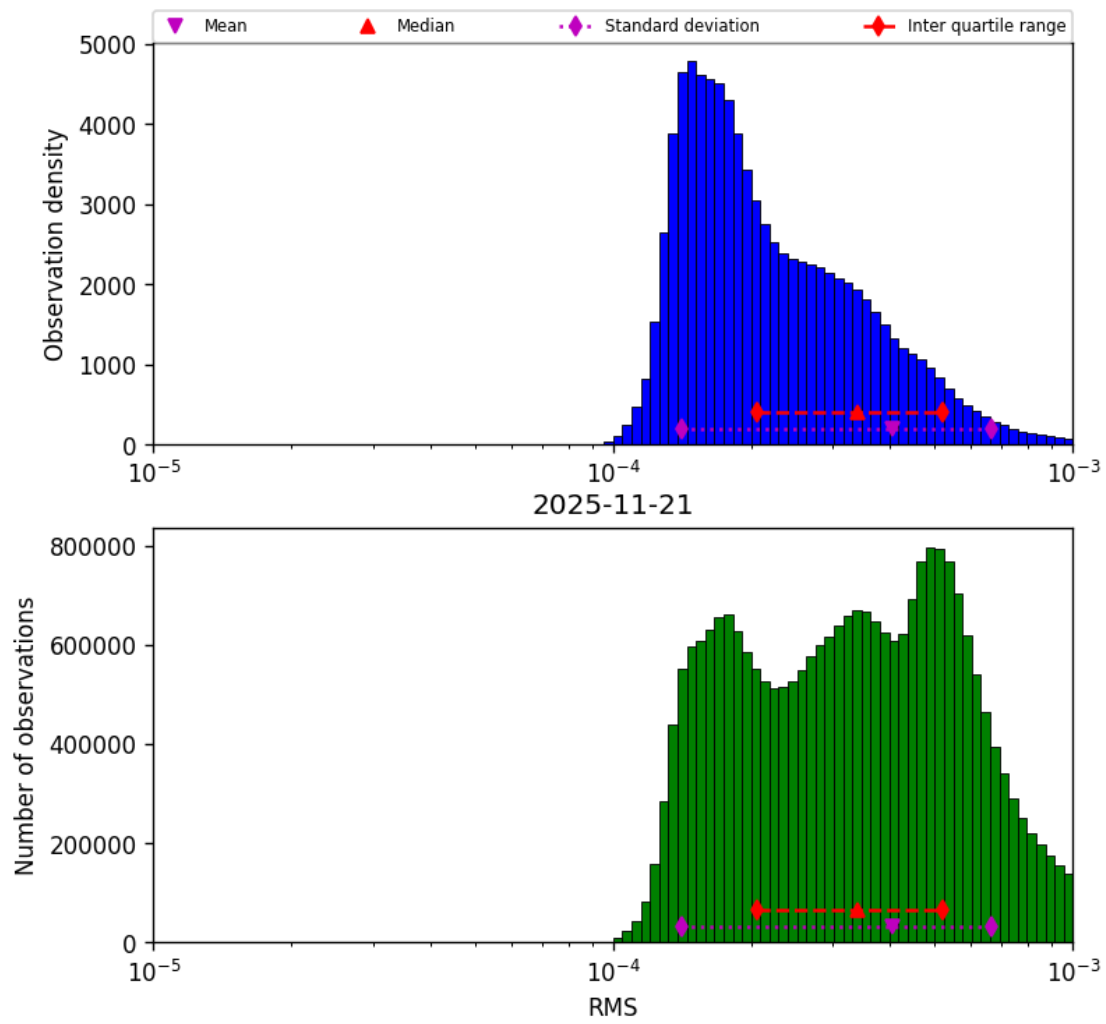
Figure 43: Histogram of “RMS” for 2025-11-20 to 2025-11-22
