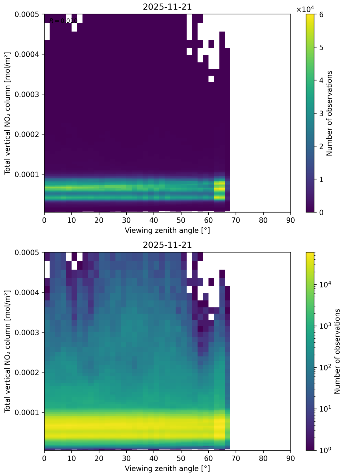
Figure 167: Scatter density plot of “Viewing zenith angle” against “Total vertical NO 2 column” for 2025-11-20 to 2025-11-22.
