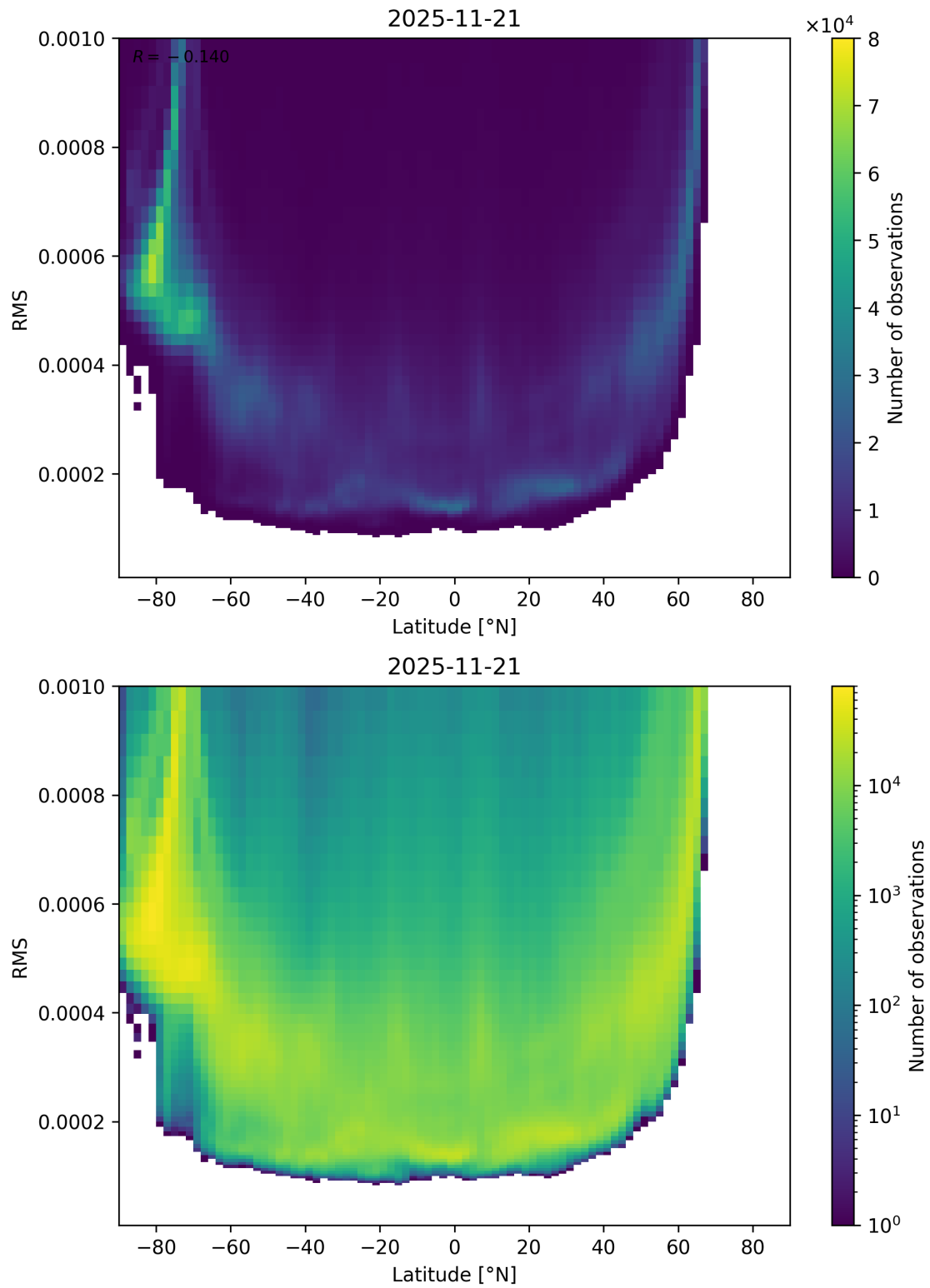
Figure 94: Scatter density plot of “Latitude” against “RMS” for 2025-11-20 to 2025-11-22.
