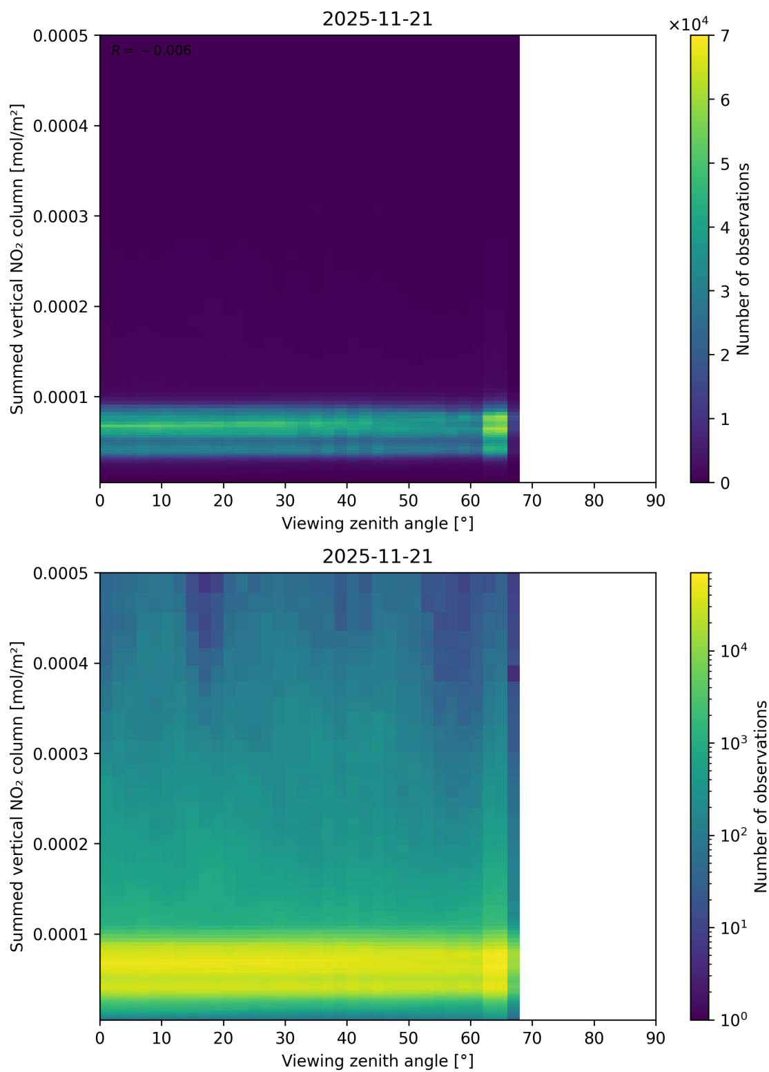
Figure 165: Scatter density plot of “Viewing zenith angle” against “Summed vertical NO 2 column” for 2025-11-20 to 2025-11-22.
