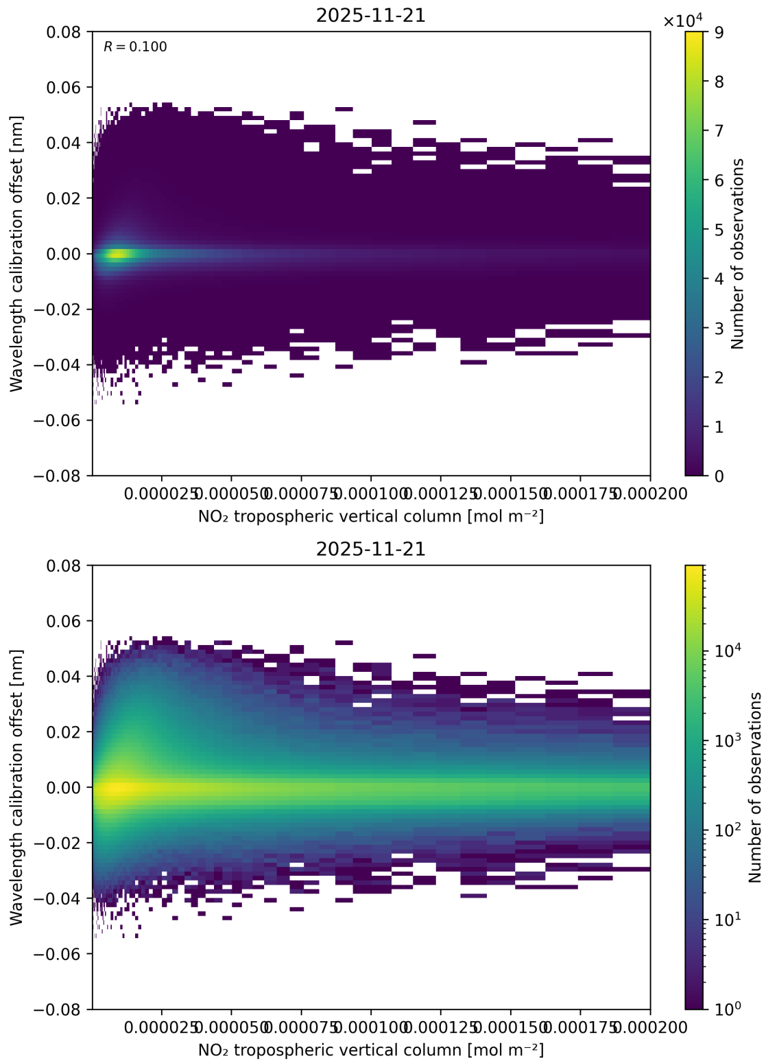
Figure 143: Scatter density plot of “NO 2 tropospheric vertical column” against “Wavelength calibration offset” for 2025-11-20 to 2025-11-22.
