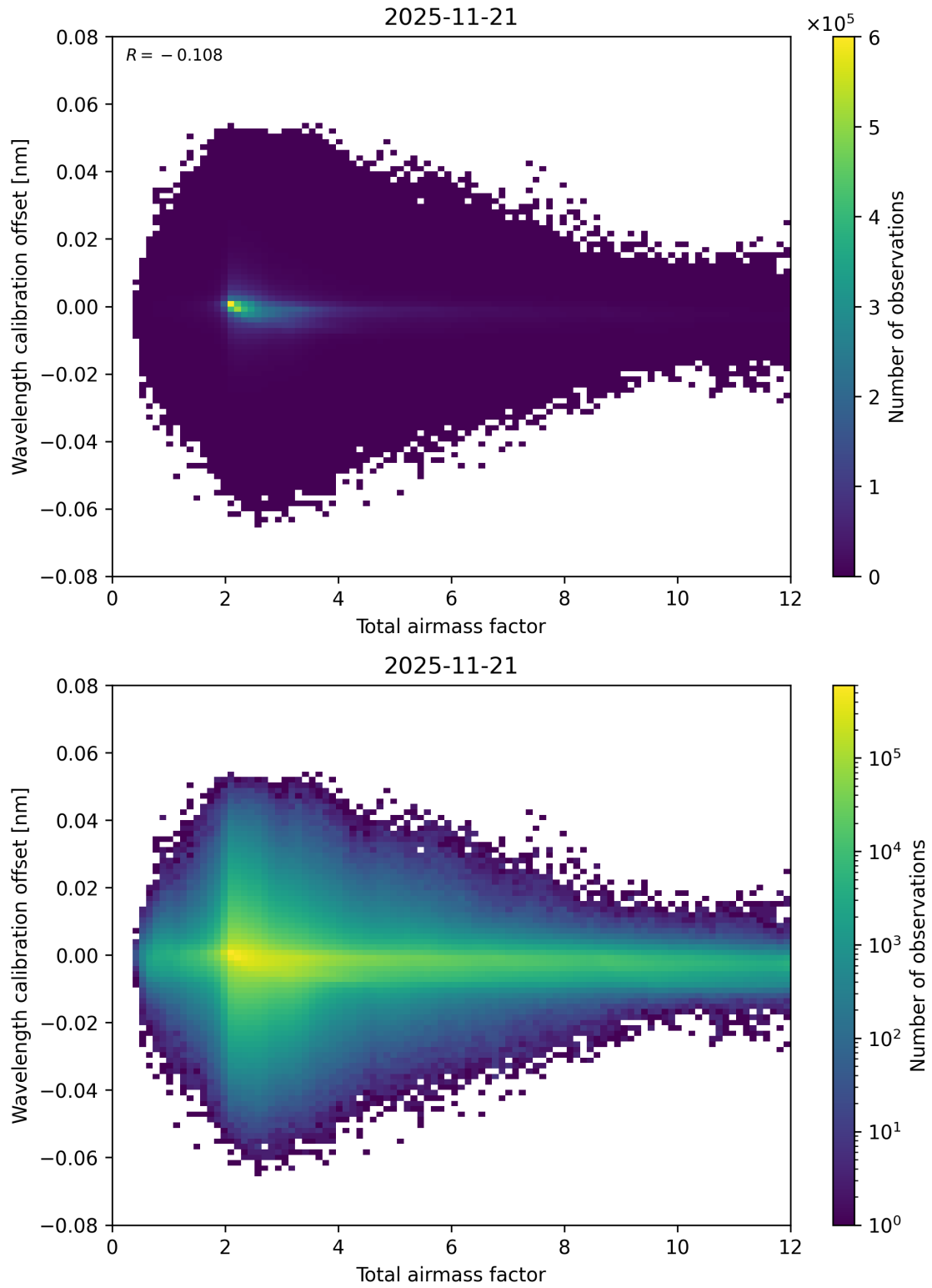
Figure 70: Scatter density plot of “Total airmass factor” against “Wavelength calibration offset” for 2025-11-20 to 2025-11-22.
