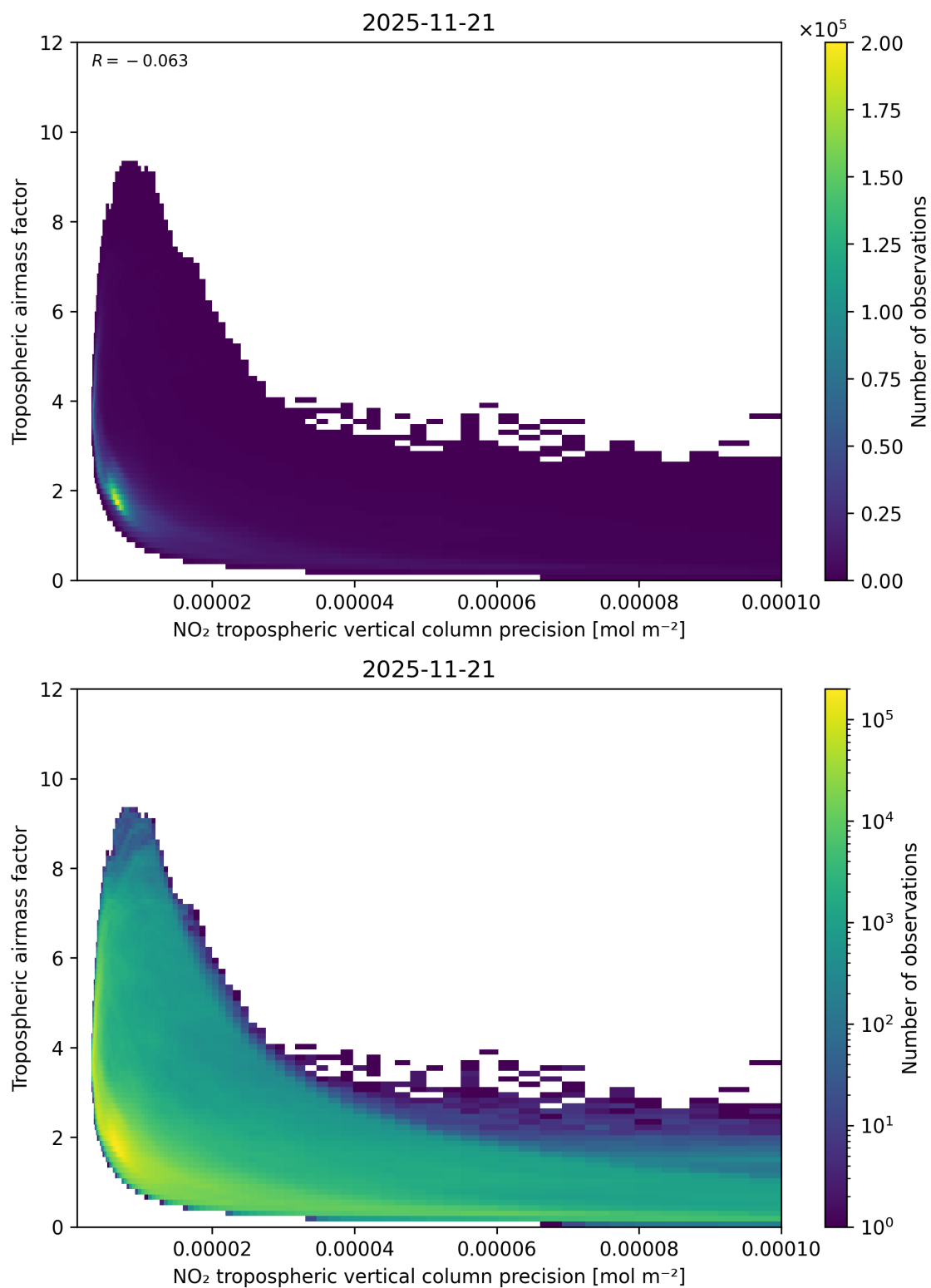
Figure 133: Scatter density plot of “NO 2 tropospheric vertical column precision” against “Tropospheric airmass factor” for 2025-11-20 to 2025-11-22.
