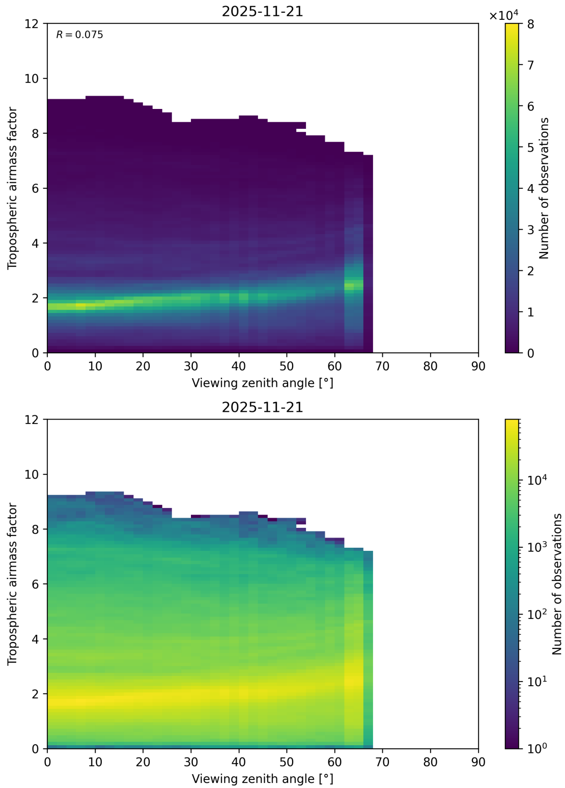
Figure 161: Scatter density plot of “Viewing zenith angle” against “Tropospheric airmass factor” for 2025-11-20 to 2025-11-22.
