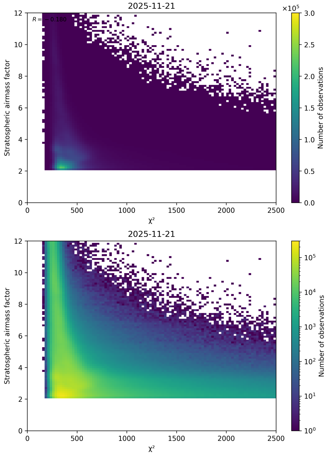
Figure 81: Scatter density plot of “ \chi^2 ” against “Stratospheric airmass factor” for 2025-11-20 to 2025-11-22.
