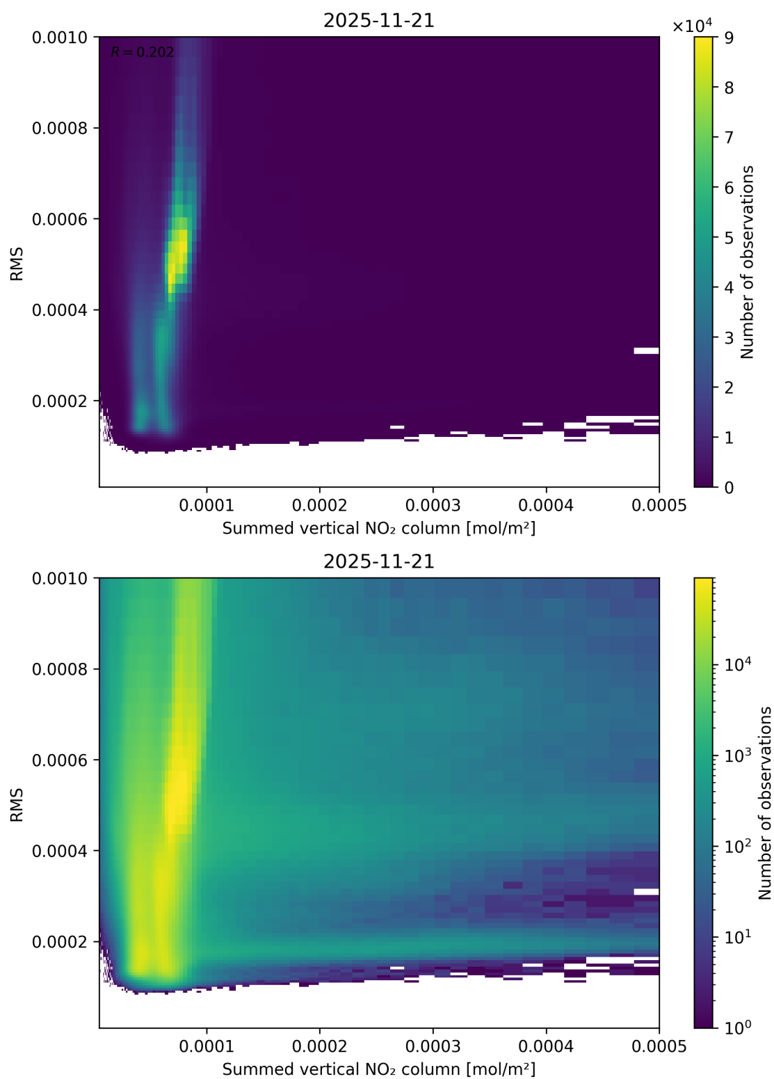
Figure 109: Scatter density plot of “Summed vertical NO 2 column” against “RMS” for 2025-11-20 to 2025-11-22.
