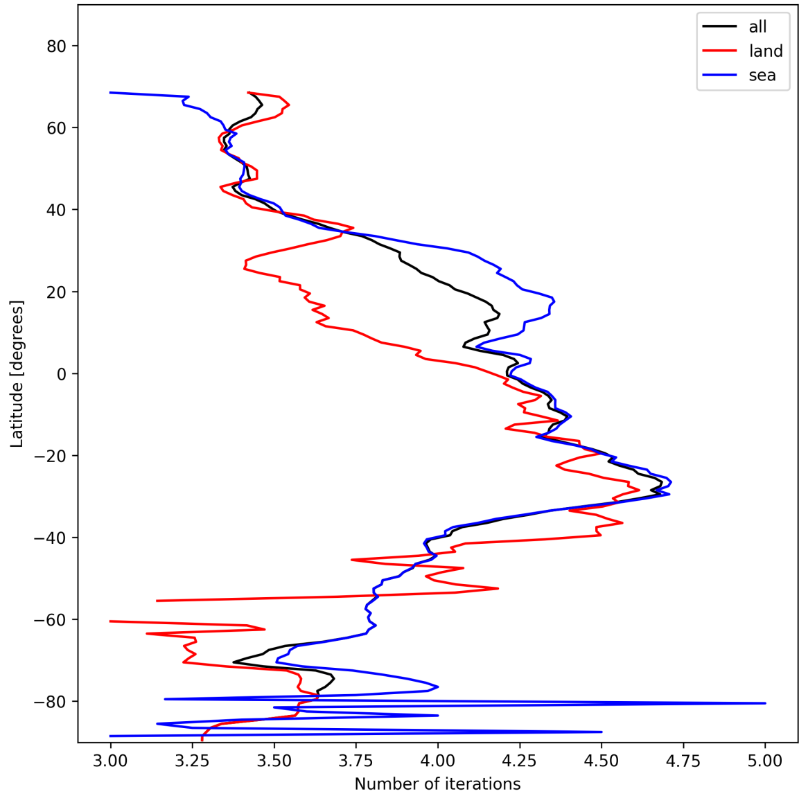
Figure 17: Zonal average of “Number of iterations” for 2025-11-20 to 2025-11-22.
