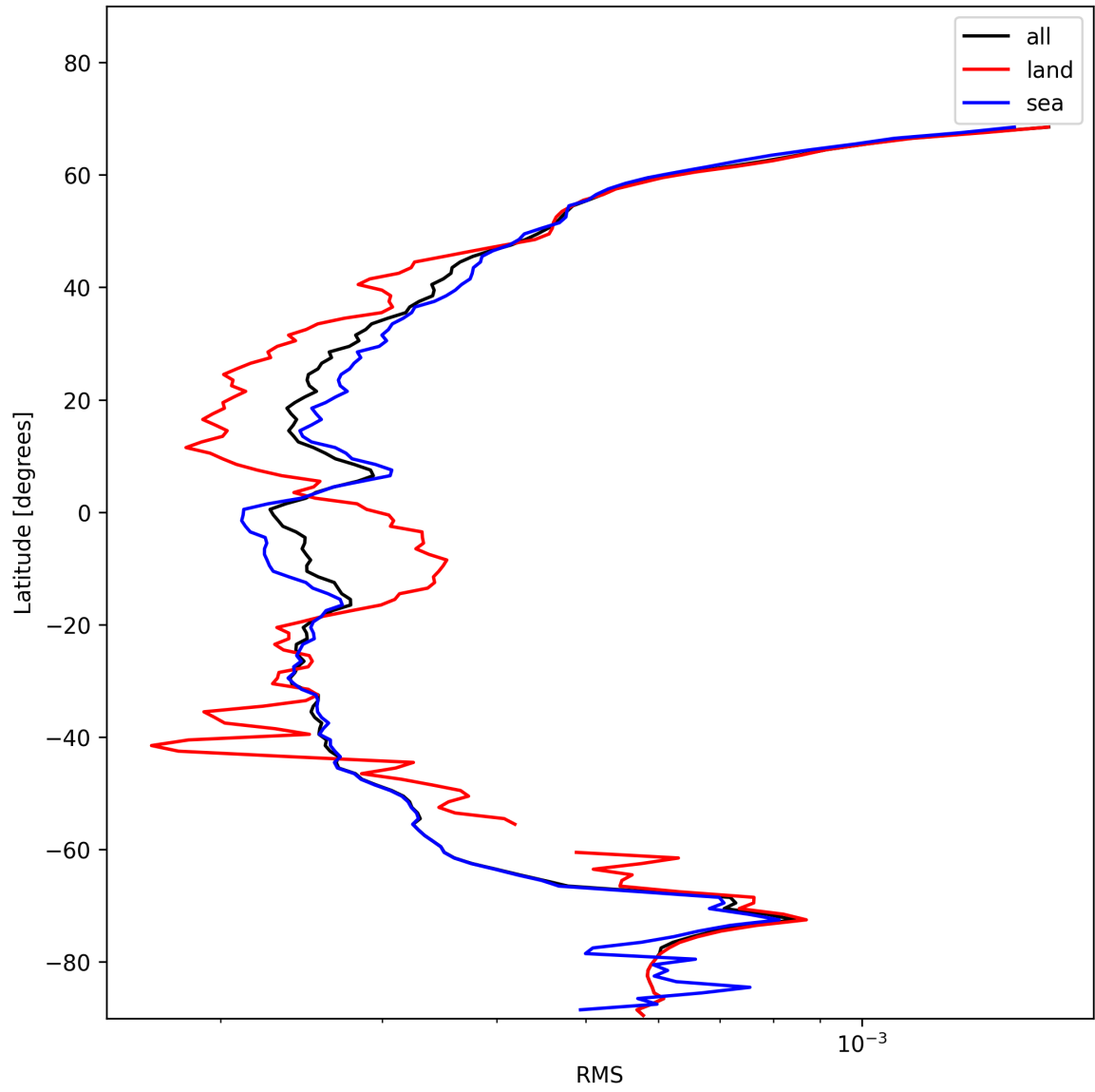
Figure 26: Zonal average of “RMS” for 2025-11-20 to 2025-11-22.
