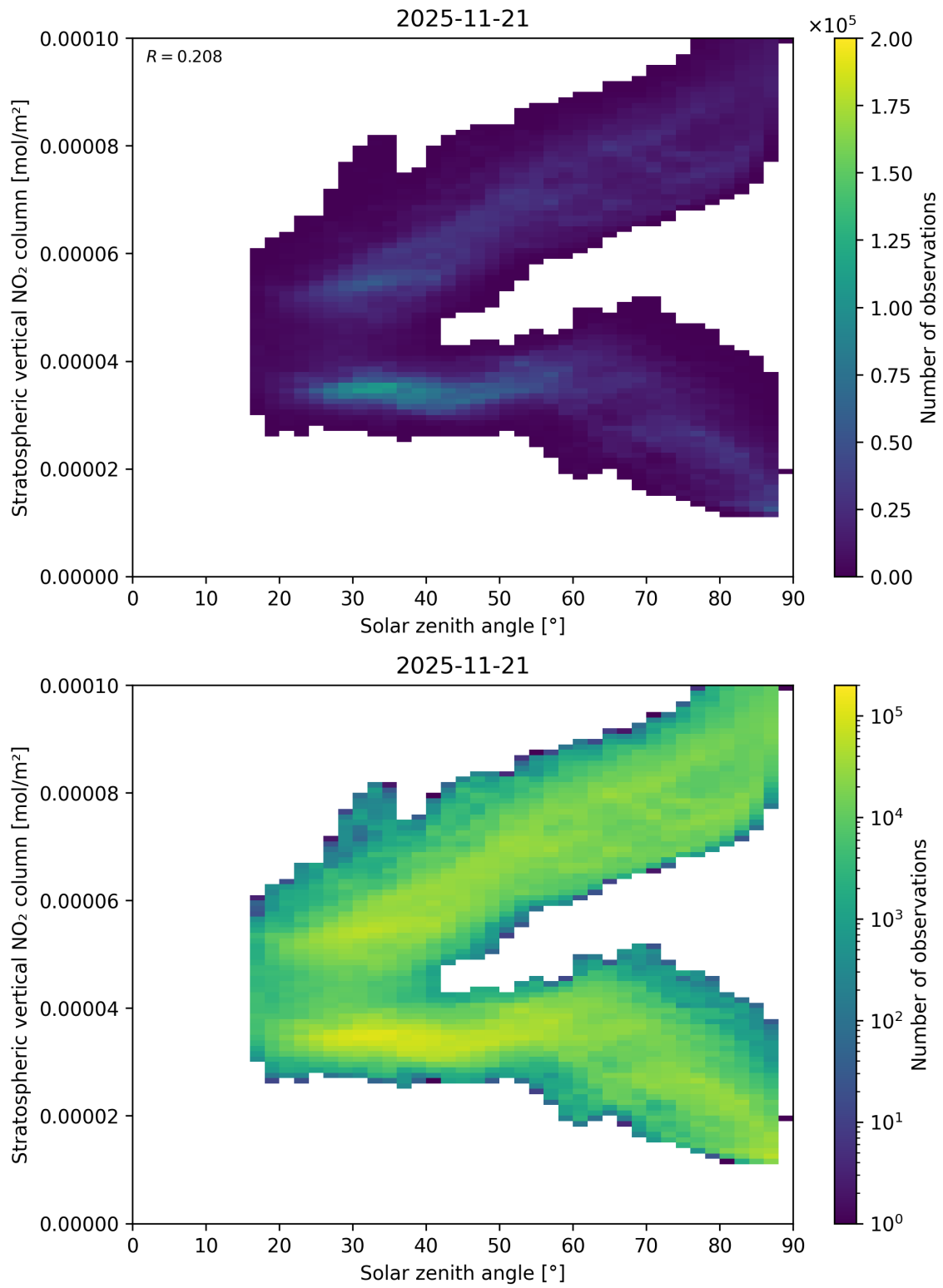
Figure 150: Scatter density plot of “Solar zenith angle” against “Stratospheric vertical NO 2 column” for 2025-11-20 to 2025-11-22.
