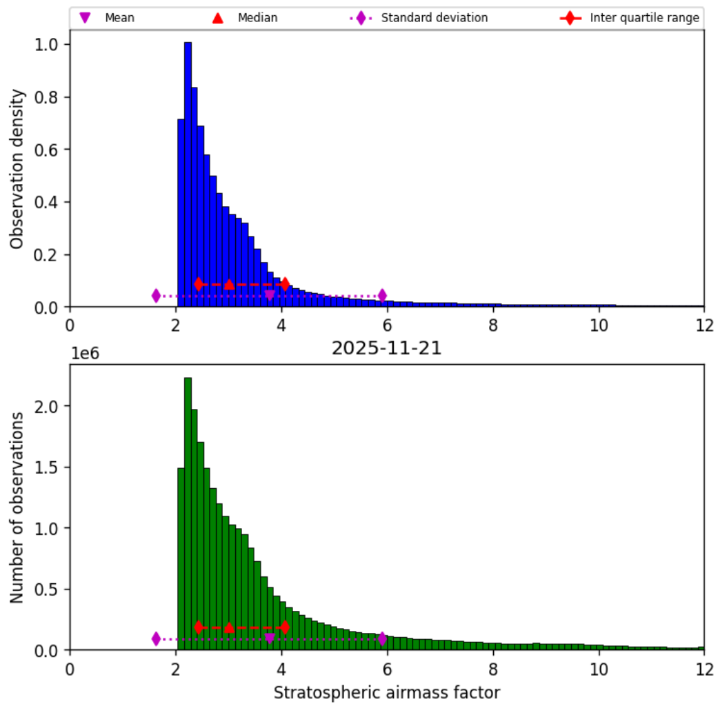
Figure 44: Histogram of “Stratospheric airmass factor” for 2025-11-20 to 2025-11-22
