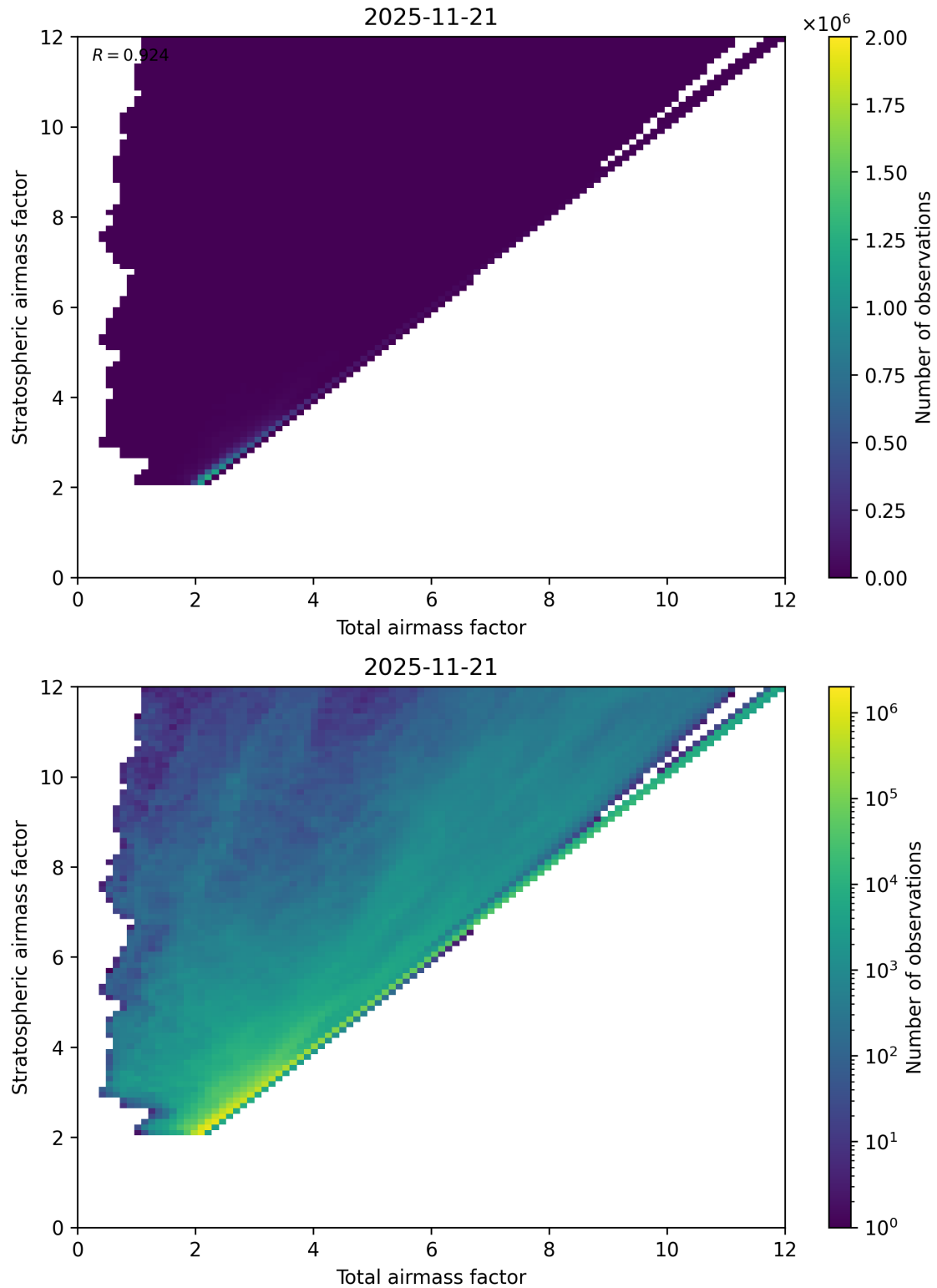
Figure 62: Scatter density plot of “Total airmass factor” against “Stratospheric airmass factor” for 2025-11-20 to 2025-11-22.
