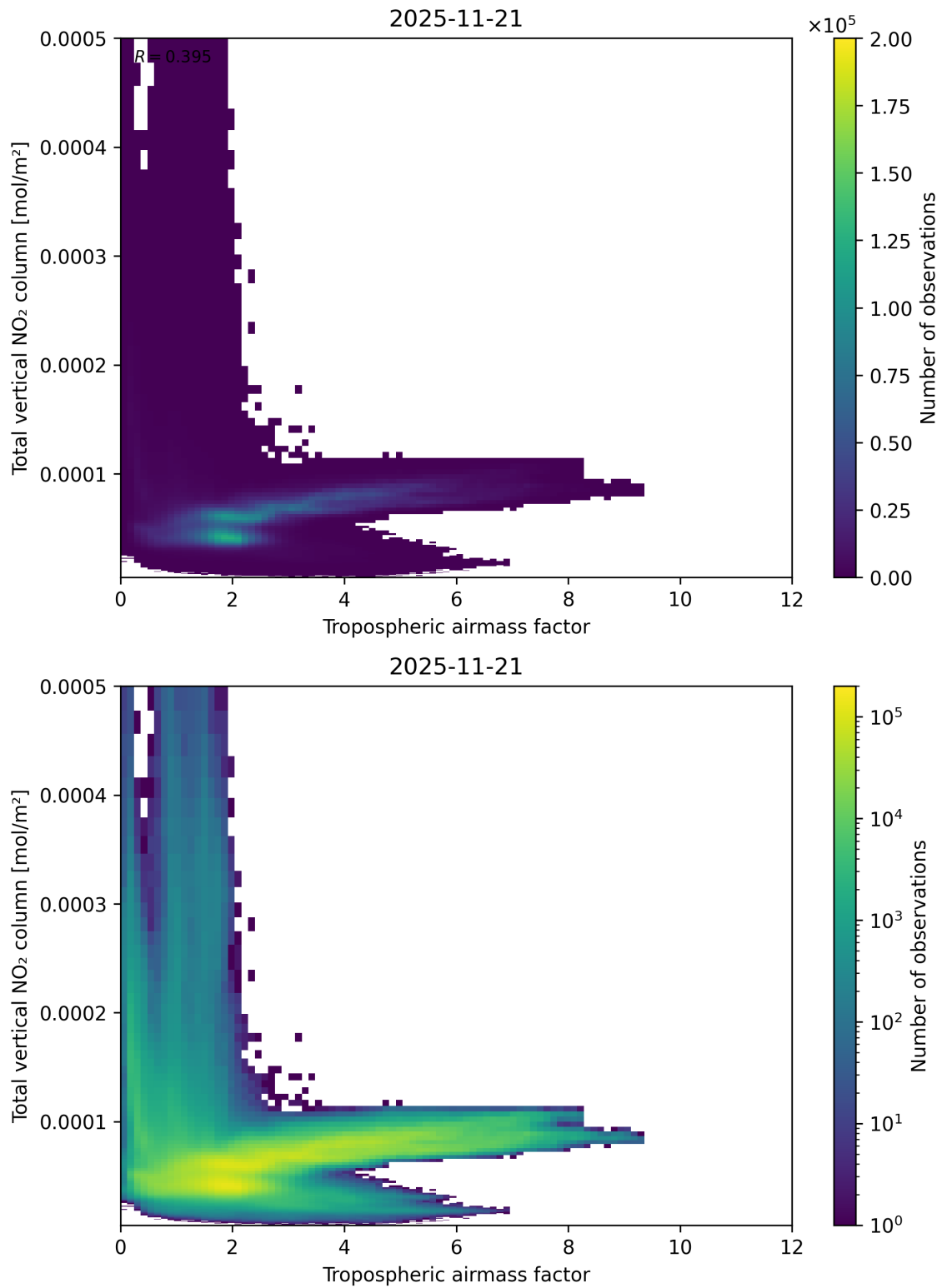
Figure 77: Scatter density plot of “Tropospheric airmass factor” against “Total vertical NO 2 column” for 2025-11-20 to 2025-11-22.
