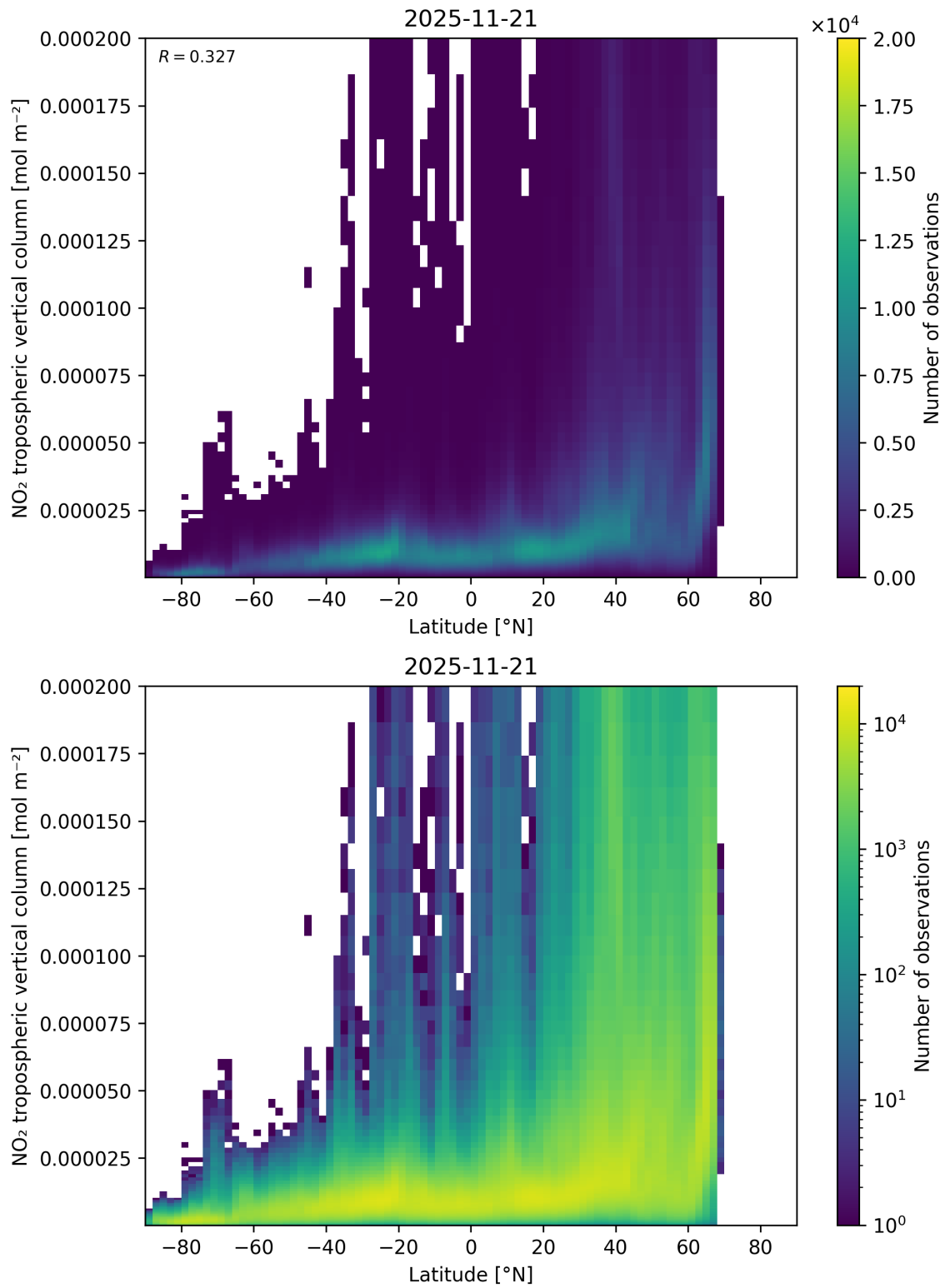
Figure 92: Scatter density plot of “Latitude” against “NO 2 tropospheric vertical column” for 2025-11-20 to 2025-11-22.
