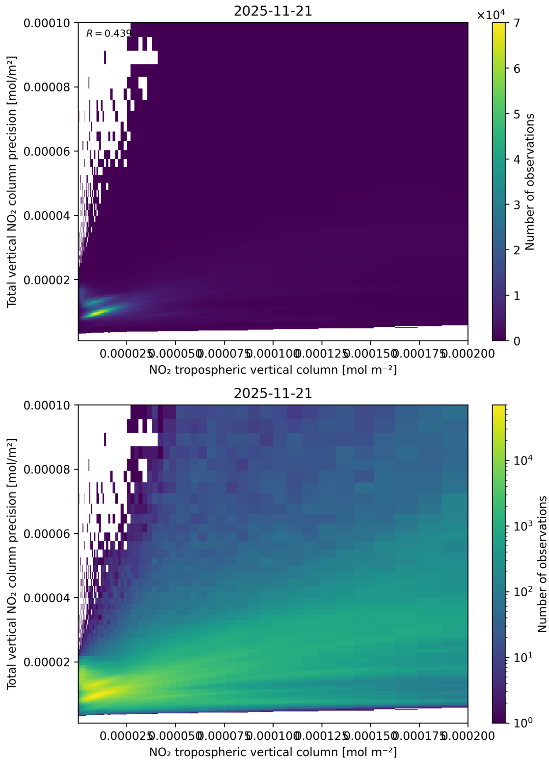
Figure 129: Scatter density plot of “NO 2 tropospheric vertical column” against “Total vertical NO 2 column precision” for 2025-11-20 to 2025-11-22.
