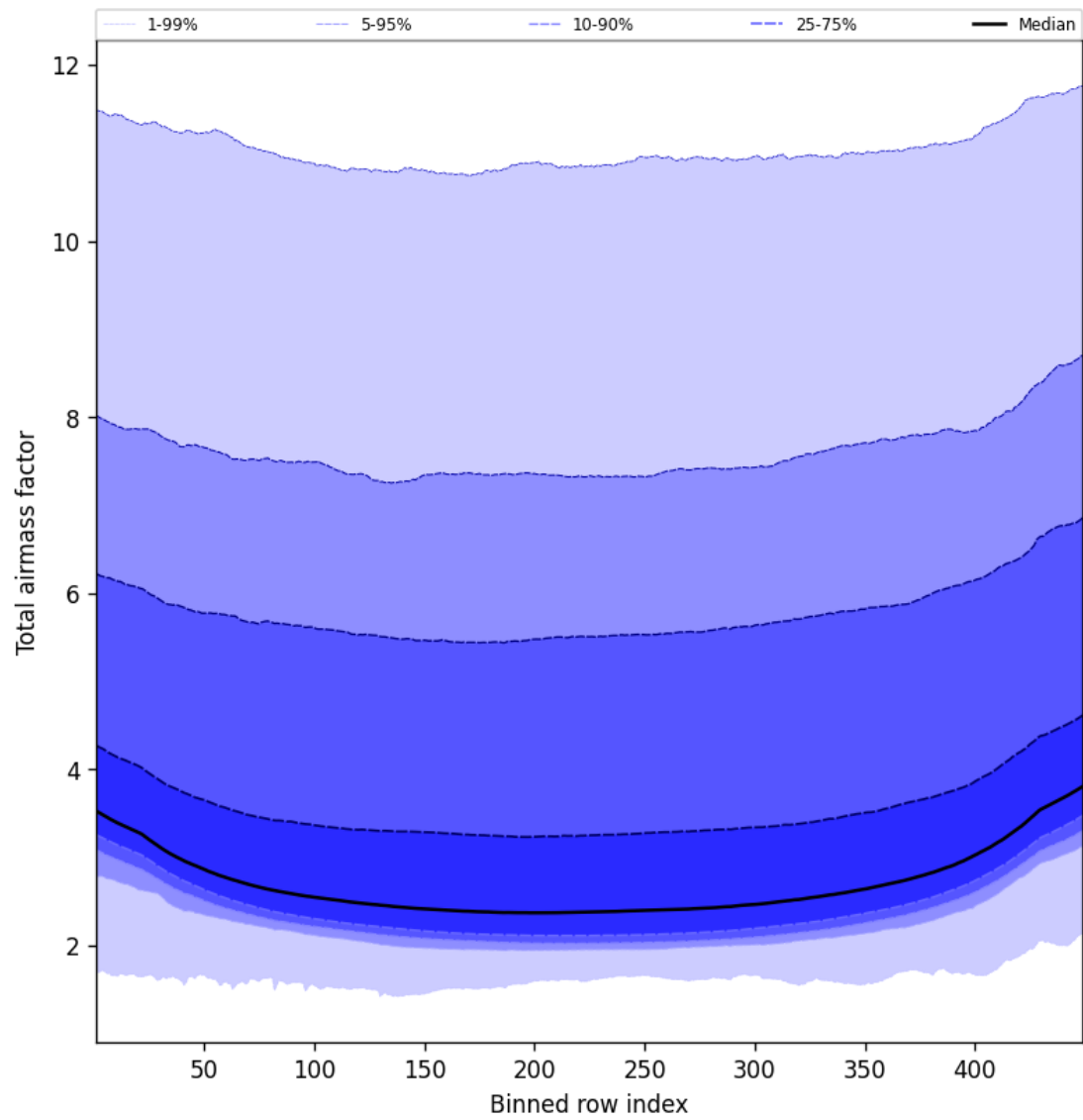
Figure 49: Along track statistics of “Total airmass factor” for 2025-11-20 to 2025-11-22
