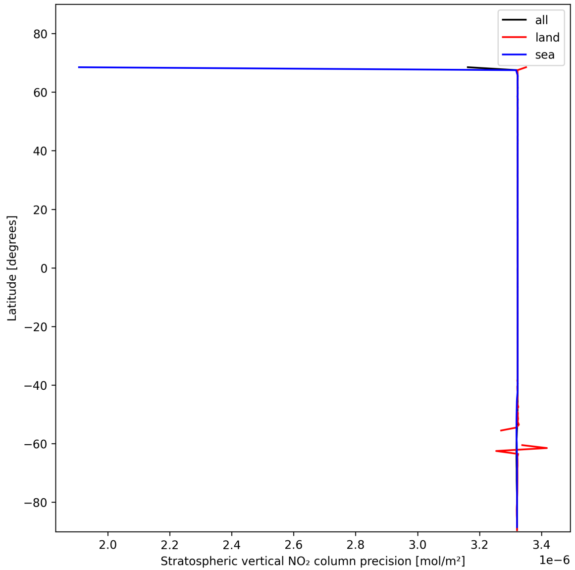
Figure 20: Zonal average of “Stratospheric vertical NO 2 column precision” for 2025-11-20 to 2025-11-22.
