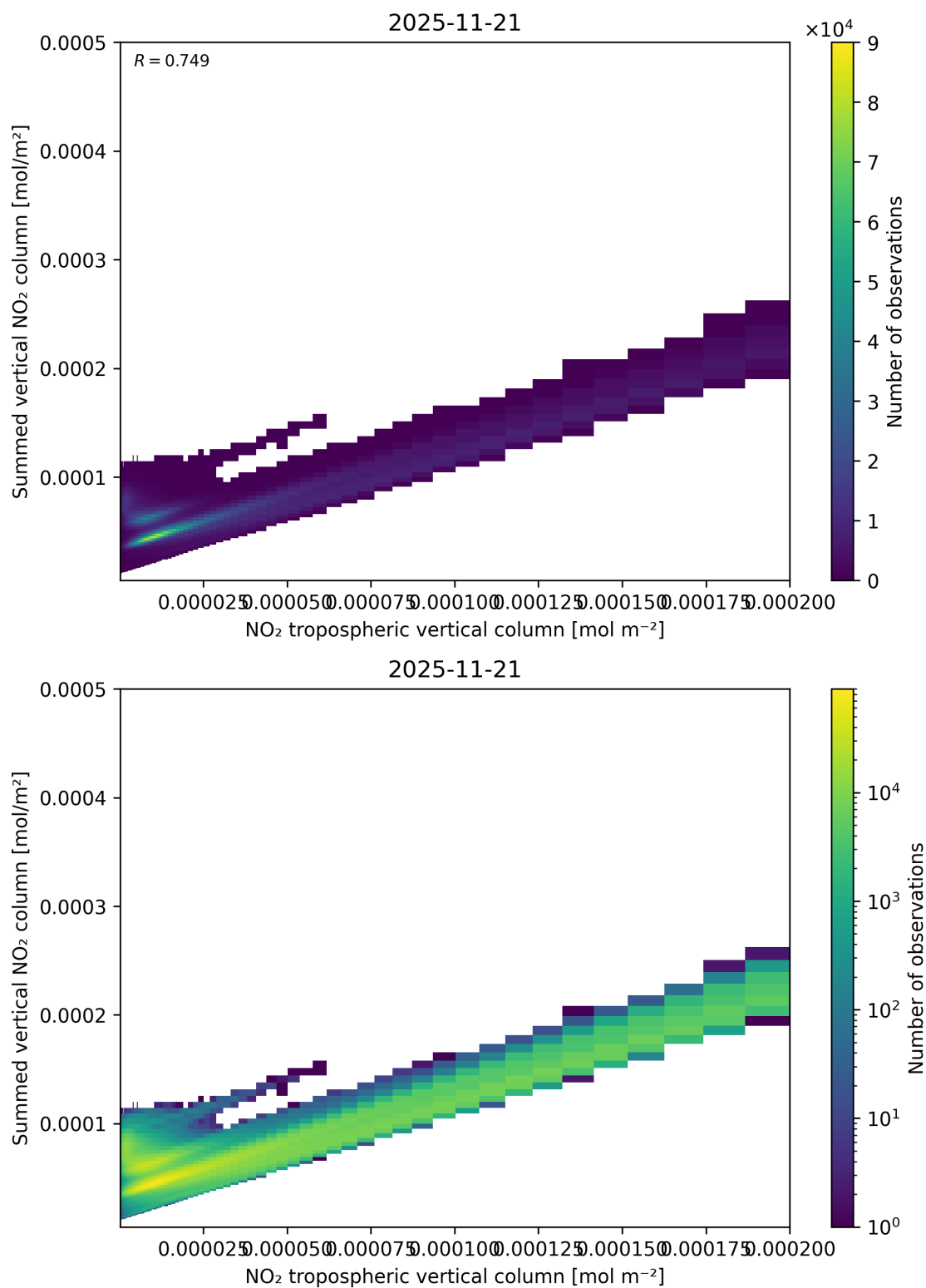
Figure 126: Scatter density plot of “NO 2 tropospheric vertical column” against “Summed vertical NO 2 column” for 2025-11-20 to 2025-11-22.
