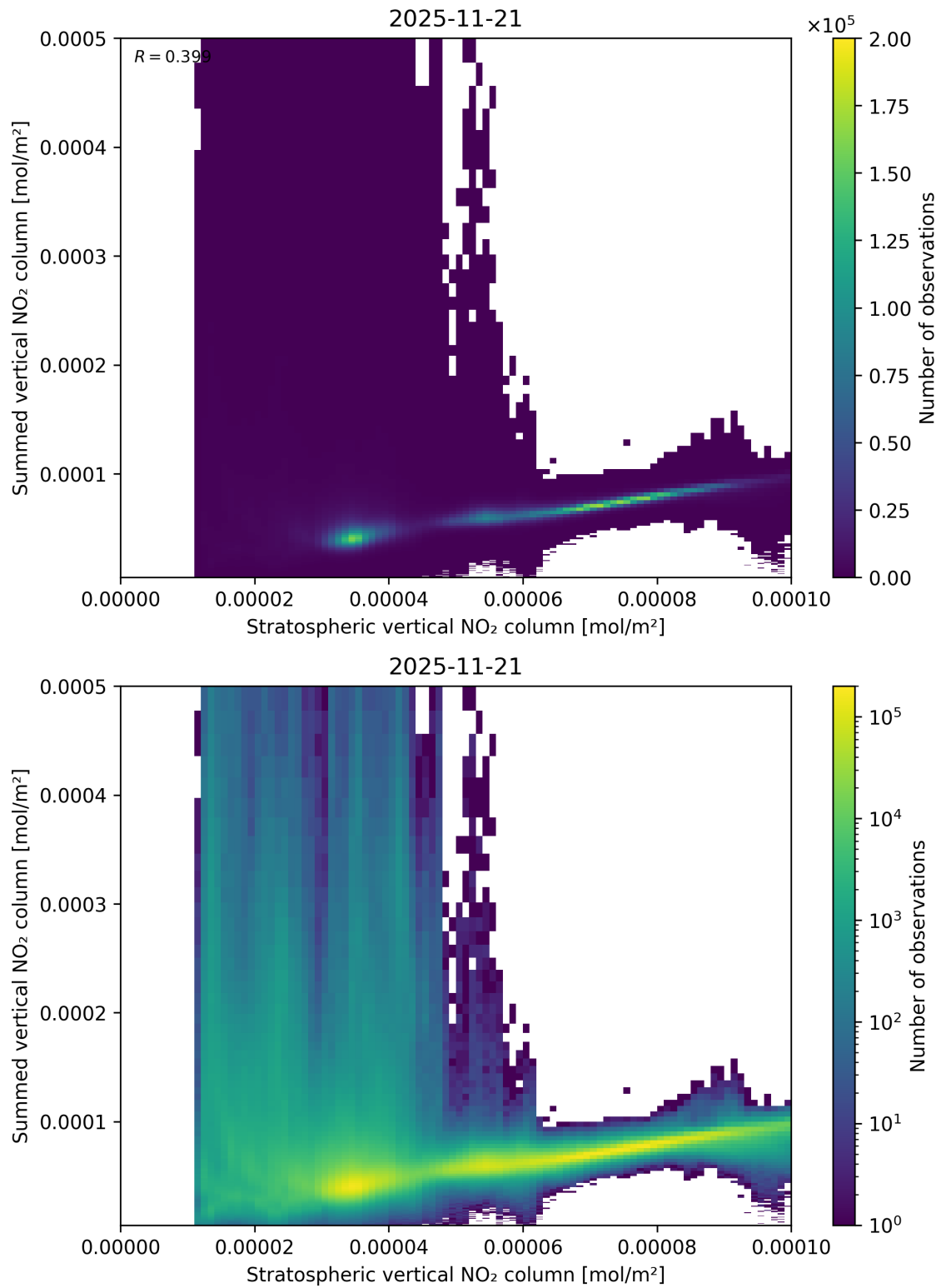
Figure 98: Scatter density plot of “Stratospheric vertical NO 2 column” against “Summed vertical NO 2 column” for 2025-11-20 to 2025-11-22.
