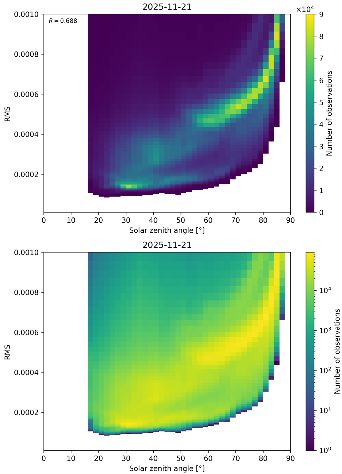
Figure 157: Scatter density plot of “Solar zenith angle” against “RMS” for 2025-11-20 to 2025-11-22.
