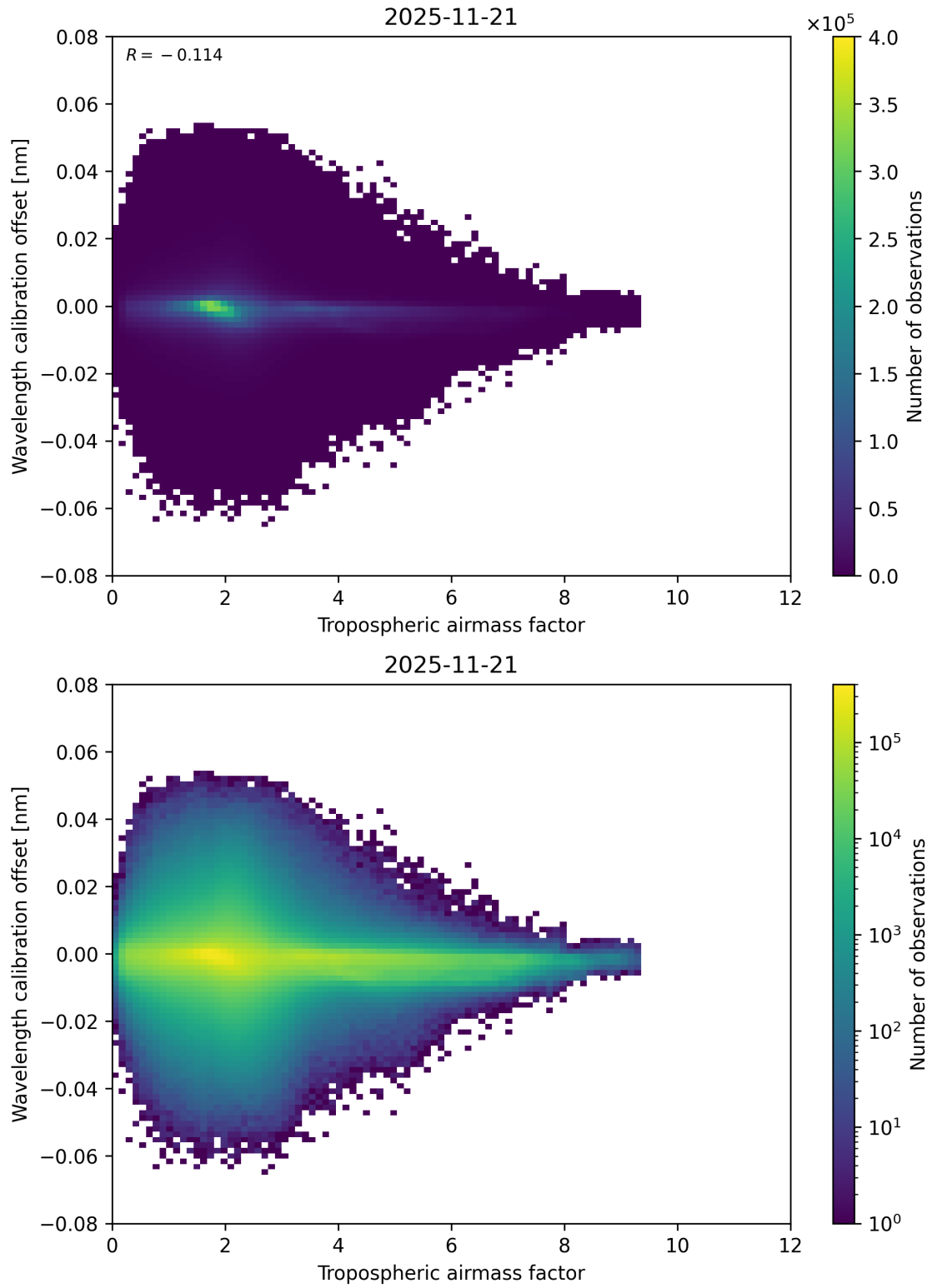
Figure 80: Scatter density plot of “Tropospheric airmass factor” against “Wavelength calibration offset” for 2025-11-20 to 2025-11-22.
