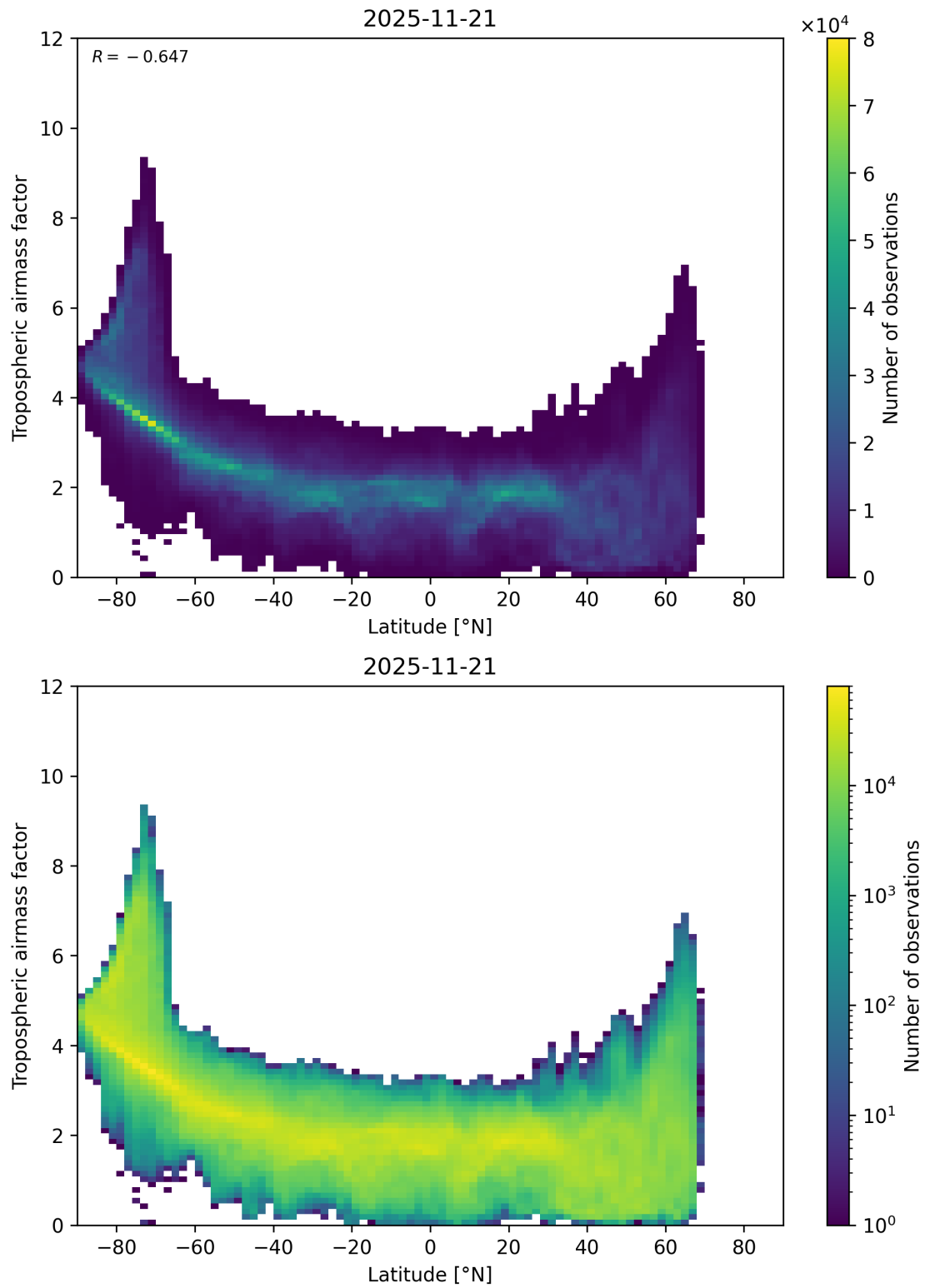
Figure 85: Scatter density plot of “Latitude” against “Tropospheric airmass factor” for 2025-11-20 to 2025-11-22.
