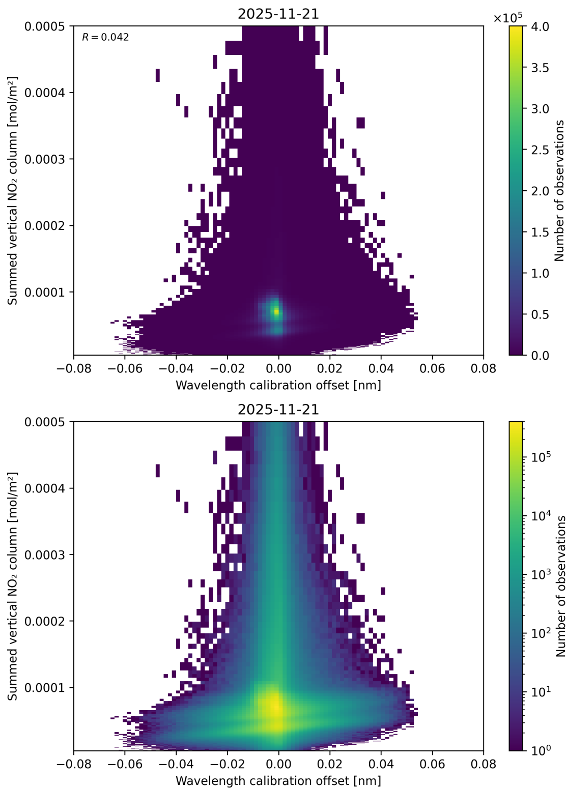
Figure 177: Scatter density plot of “Wavelength calibration offset” against “Summed vertical NO 2 column” for 2025-11-20 to 2025-11-22.
