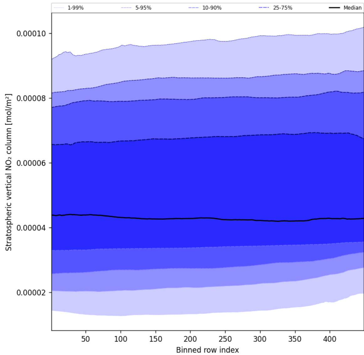
Figure 53: Along track statistics of “Stratospheric vertical NO 2 column” for 2025-11-20 to 2025-11-22
