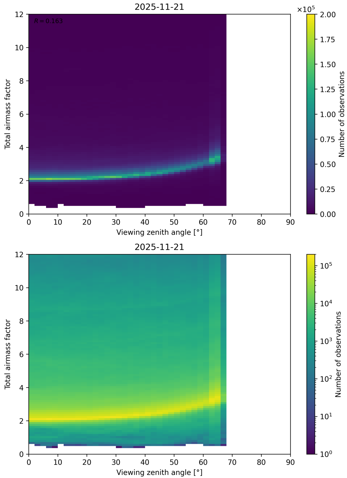
Figure 160: Scatter density plot of “Viewing zenith angle” against “Total airmass factor” for 2025-11-20 to 2025-11-22.
