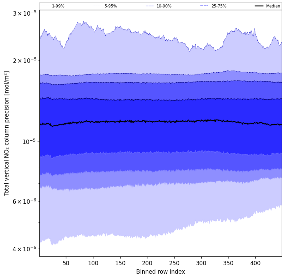
Figure 56: Along track statistics of “Total vertical NO 2 column precision” for 2025-11-20 to 2025-11-22
