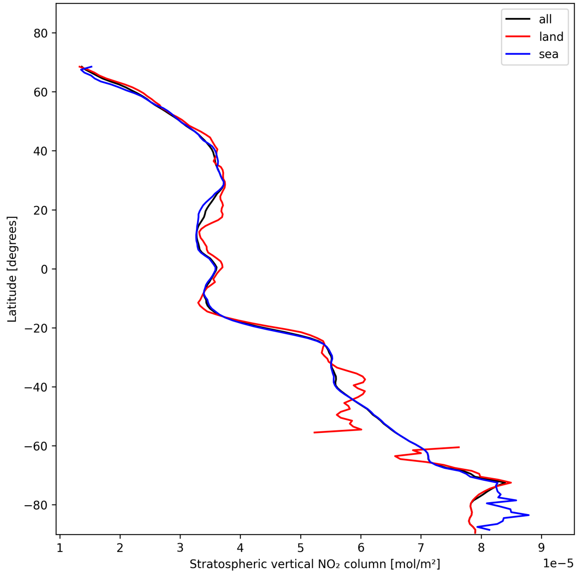
Figure 19: Zonal average of “Stratospheric vertical NO 2 column” for 2025-11-20 to 2025-11-22.
