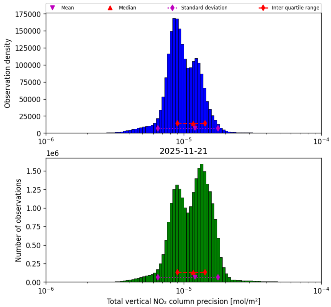
Figure 39: Histogram of “Total vertical NO 2 column precision” for 2025-11-20 to 2025-11-22
