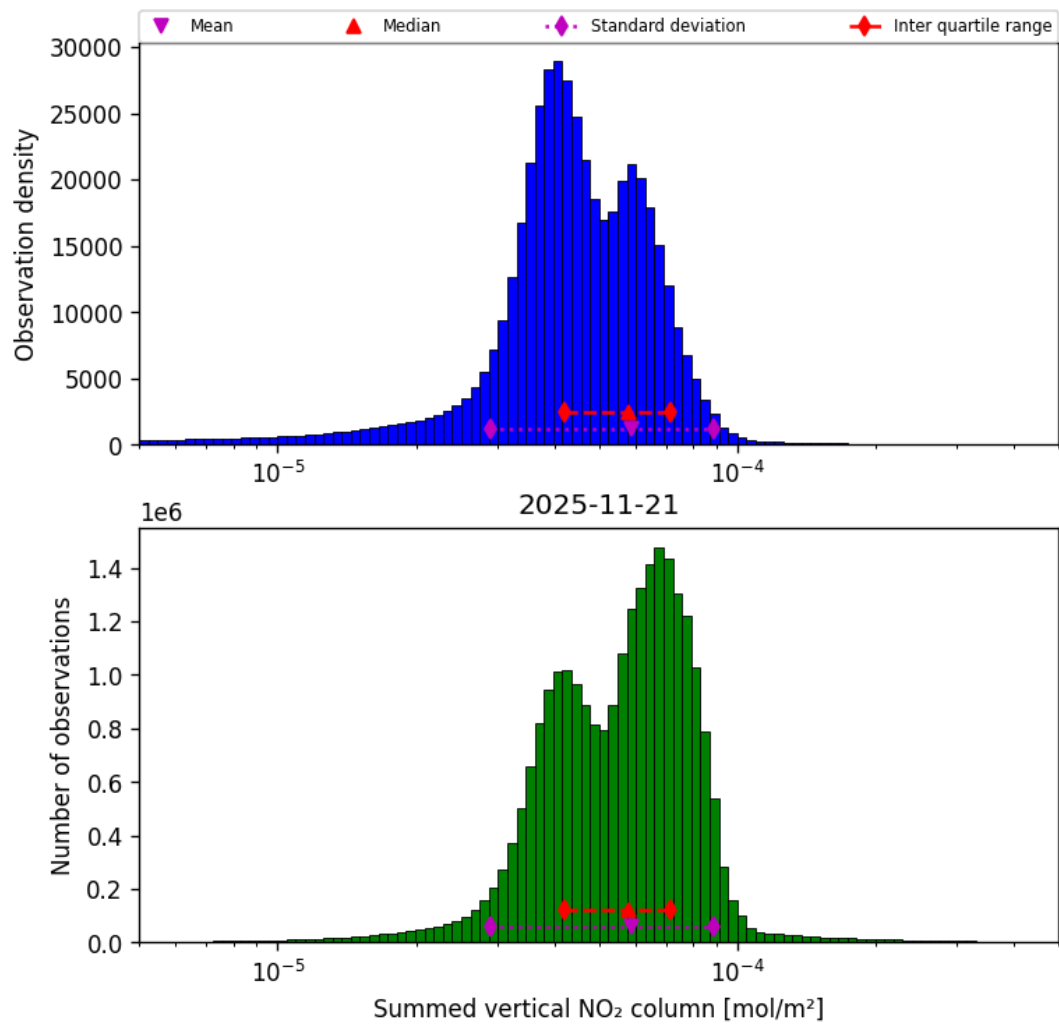
Figure 40: Histogram of “Summed vertical NO 2 column” for 2025-11-20 to 2025-11-22
