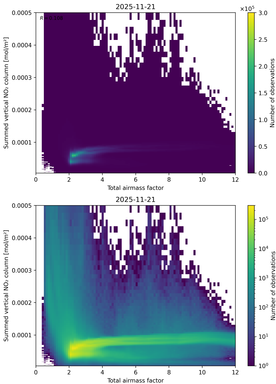
Figure 65: Scatter density plot of “Total airmass factor” against “Summed vertical NO 2 column” for 2025-11-20 to 2025-11-22.
