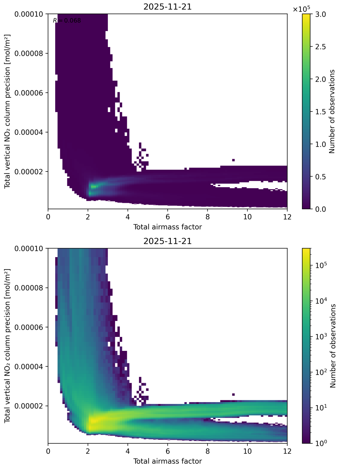
Figure 68: Scatter density plot of “Total airmass factor” against “Total vertical NO 2 column precision” for 2025-11-20 to 2025-11-22.
