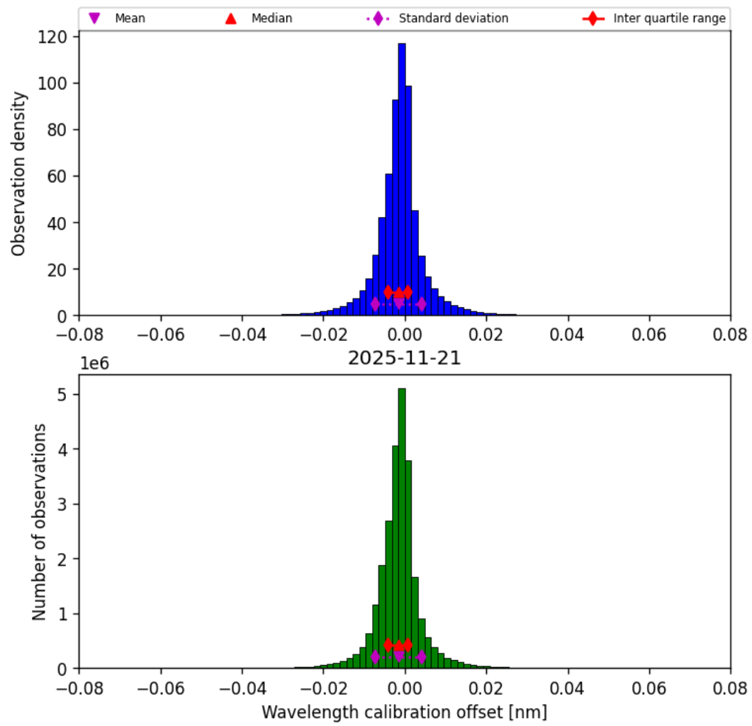
Figure 35: Histogram of “Wavelength calibration offset” for 2025-11-20 to 2025-11-22
