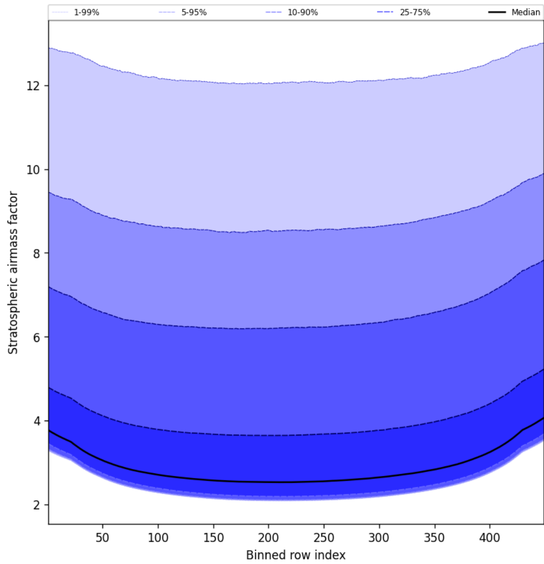
Figure 61: Along track statistics of “Stratospheric airmass factor” for 2025-11-20 to 2025-11-22
