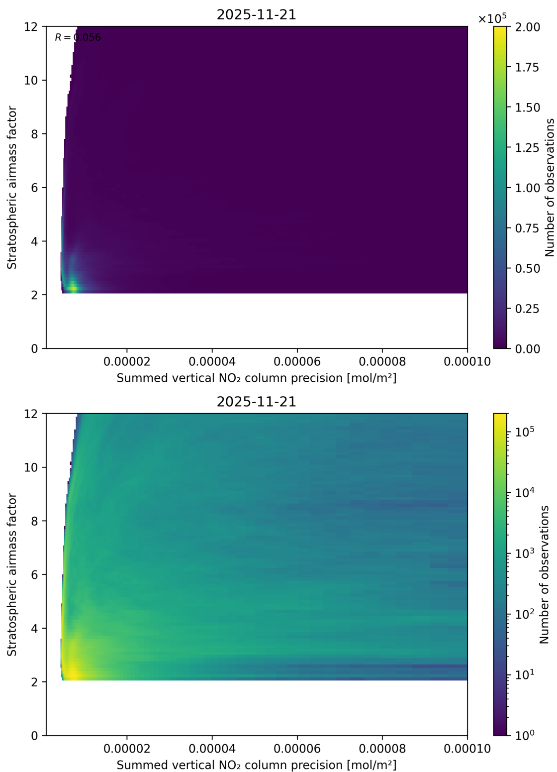
Figure 106: Scatter density plot of “Summed vertical NO 2 column precision” against “Stratospheric airmass factor” for 2025-11-20 to 2025-11-22.
