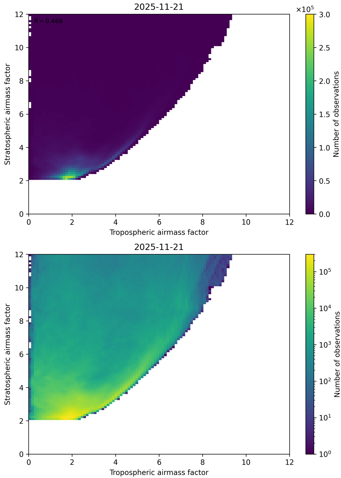
Figure 71: Scatter density plot of “Tropospheric airmass factor” against “Stratospheric airmass factor” for 2025-11-20 to 2025-11-22.
