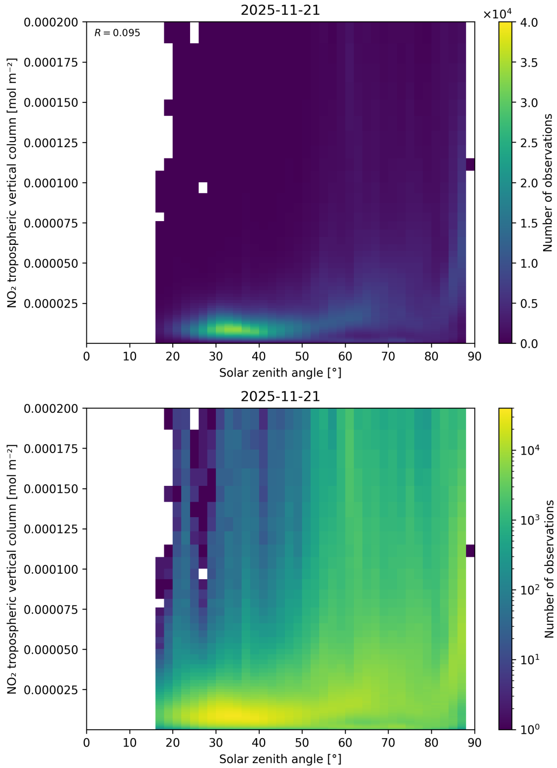
Figure 155: Scatter density plot of “Solar zenith angle” against “NO 2 tropospheric vertical column” for 2025-11-20 to 2025-11-22.
