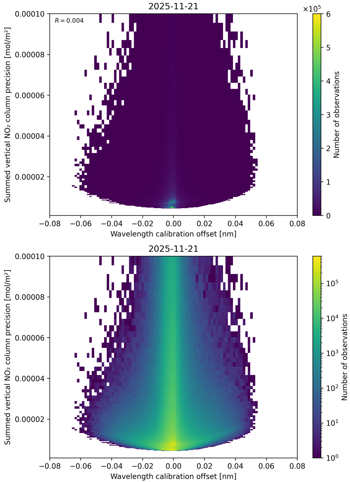
Figure 178: Scatter density plot of “Wavelength calibration offset” against “Summed vertical NO 2 column precision” for 2025-11-20 to 2025-11-22.
