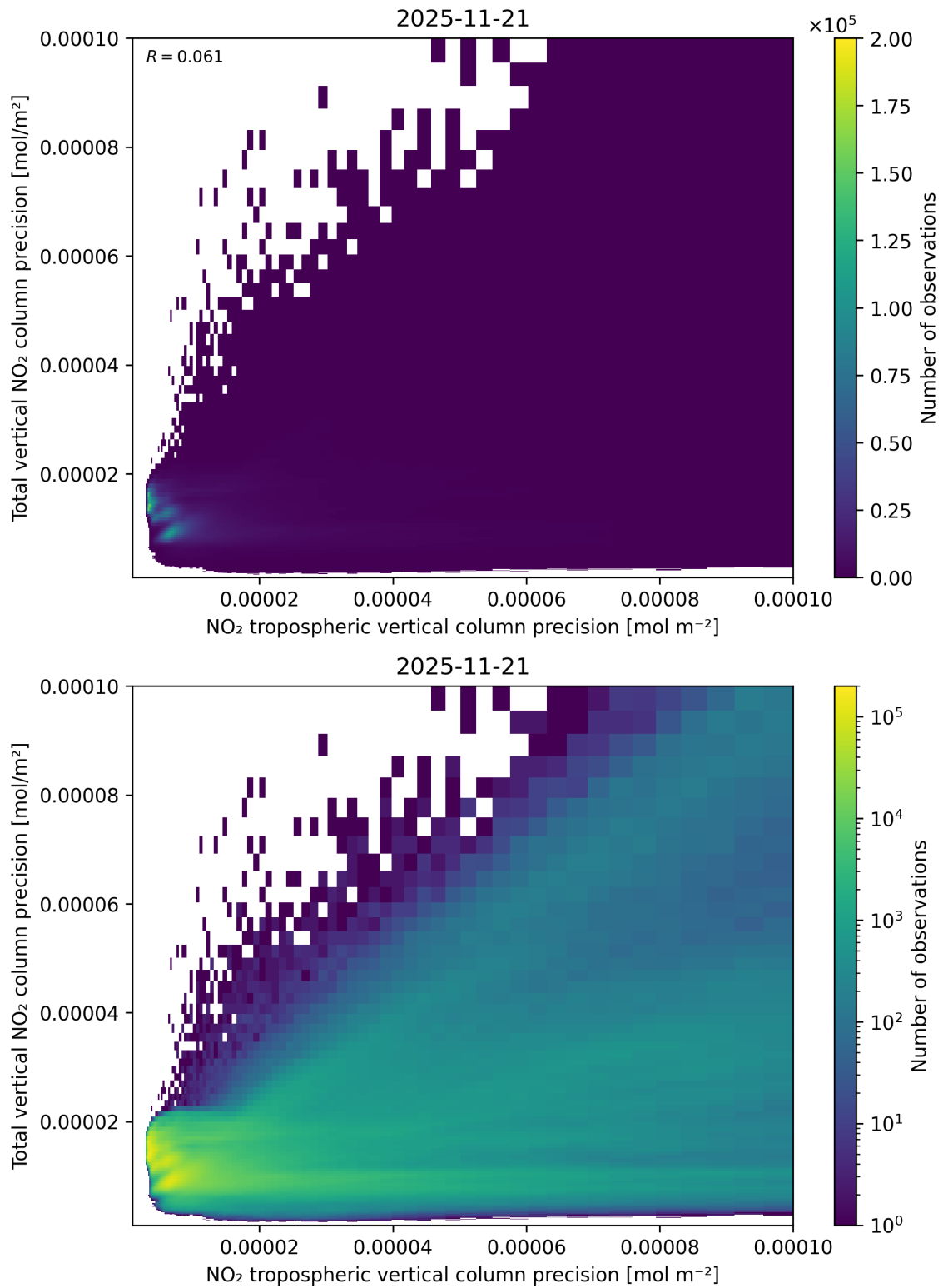
Figure 139: Scatter density plot of “NO 2 tropospheric vertical column precision” against “Total vertical NO 2 column precision” for 2025-11-20 to 2025-11-22.
