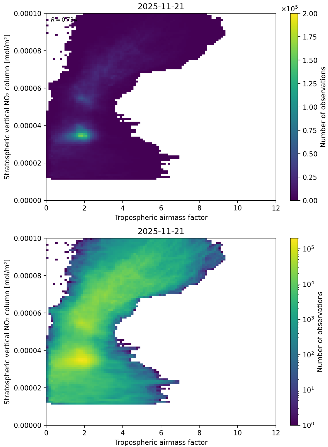
Figure 74: Scatter density plot of “Tropospheric air mass factor” against “Stratospheric vertical NO 2 column” for 2025-11-20 to 2025-11-22.
