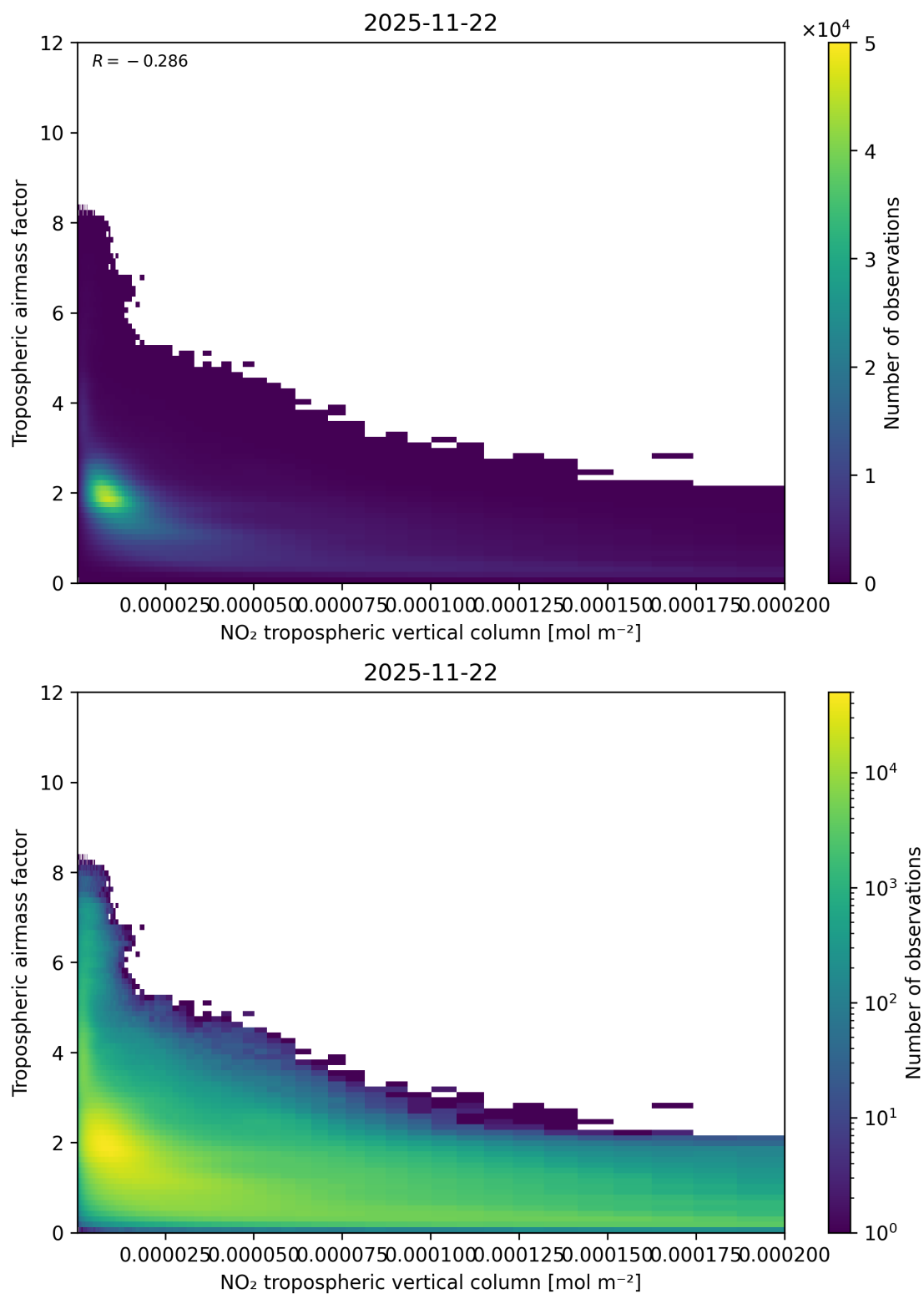
Figure 123: Scatter density plot of “NO 2 tropospheric vertical column” against “Tropospheric air mass factor” for 2025-11-21 to 2025-11-23.
