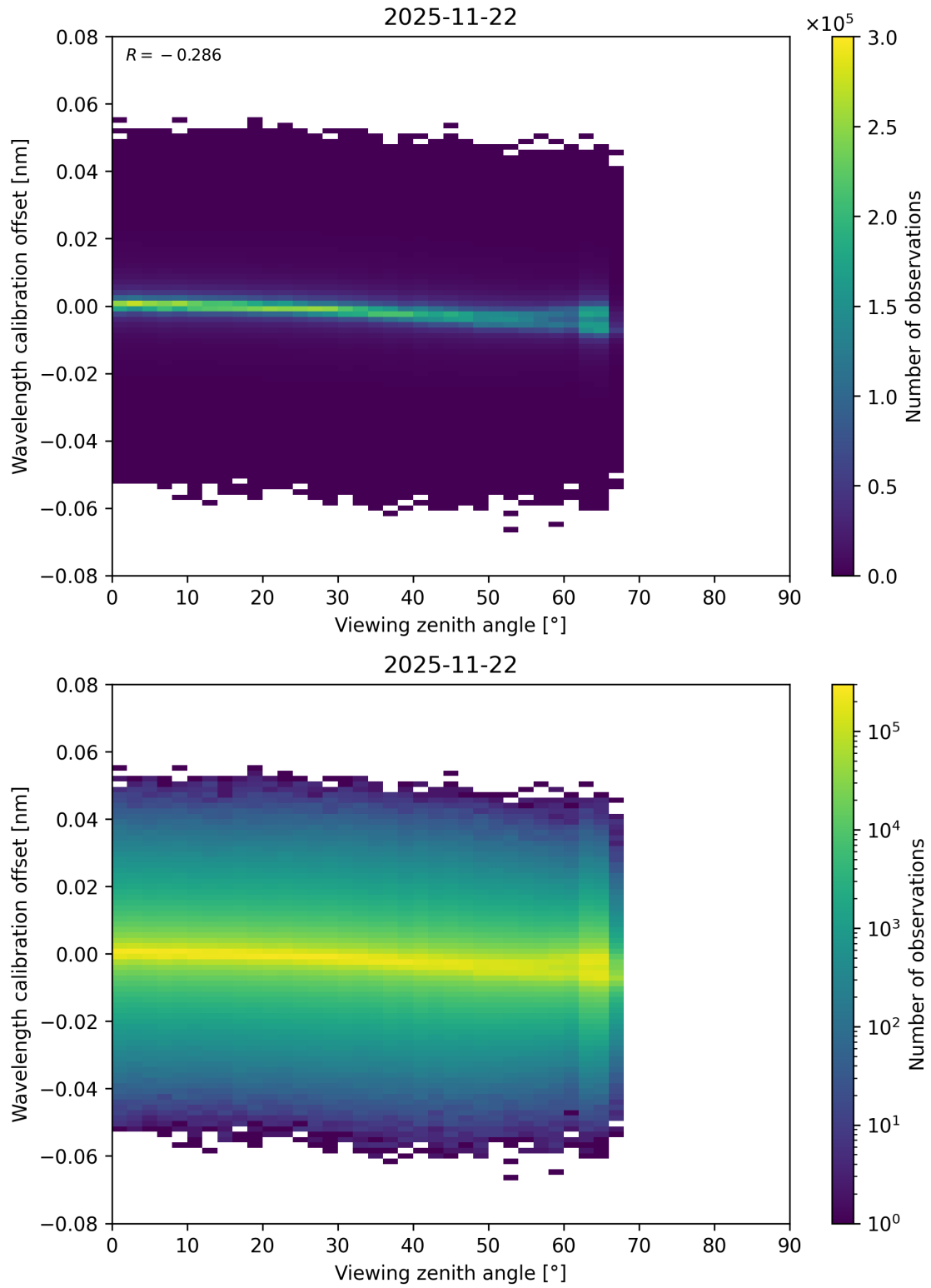
Figure 173: Scatter density plot of “Viewing zenith angle” against “Wavelength calibration offset” for 2025-11-21 to 2025-11-23.
