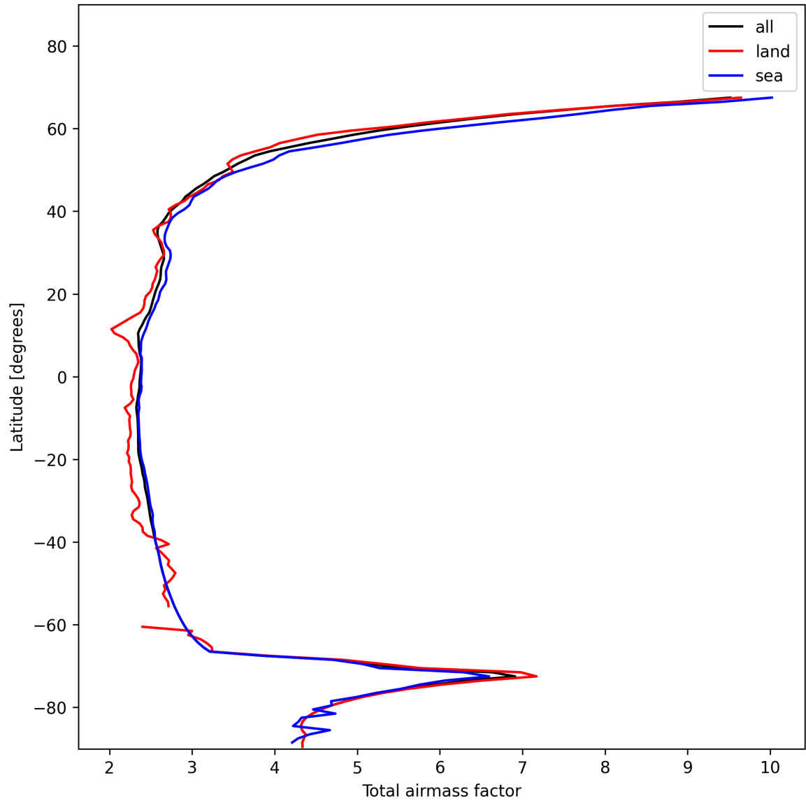
Figure 15: Zonal average of “Total airmass factor” for 2025-11-21 to 2025-11-23.
