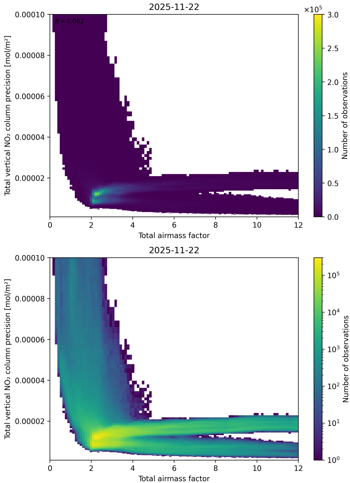
Figure 68: Scatter density plot of “Total airmass factor” against “Total vertical NO 2 column precision” for 2025-11-21 to 2025-11-23.
