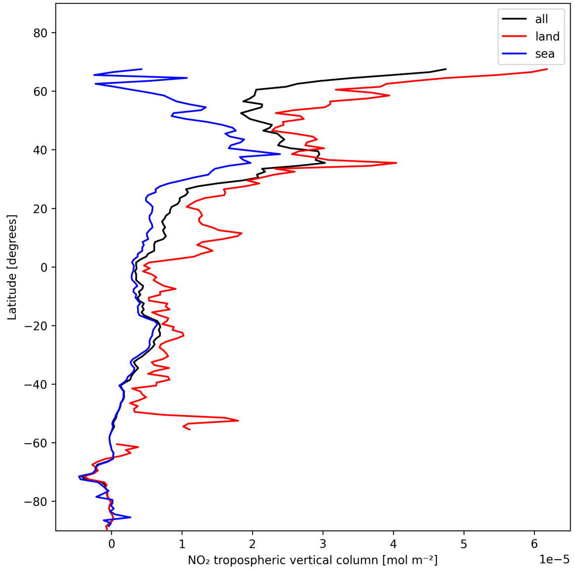
Figure 12: Zonal average of “NO 2 tropospheric vertical column” for 2025-11-21 to 2025-11-23.
