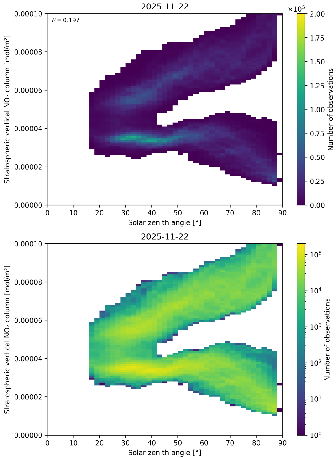
Figure 150: Scatter density plot of “Solar zenith angle” against “Stratospheric vertical NO 2 column” for 2025-11-21 to 2025-11-23.
