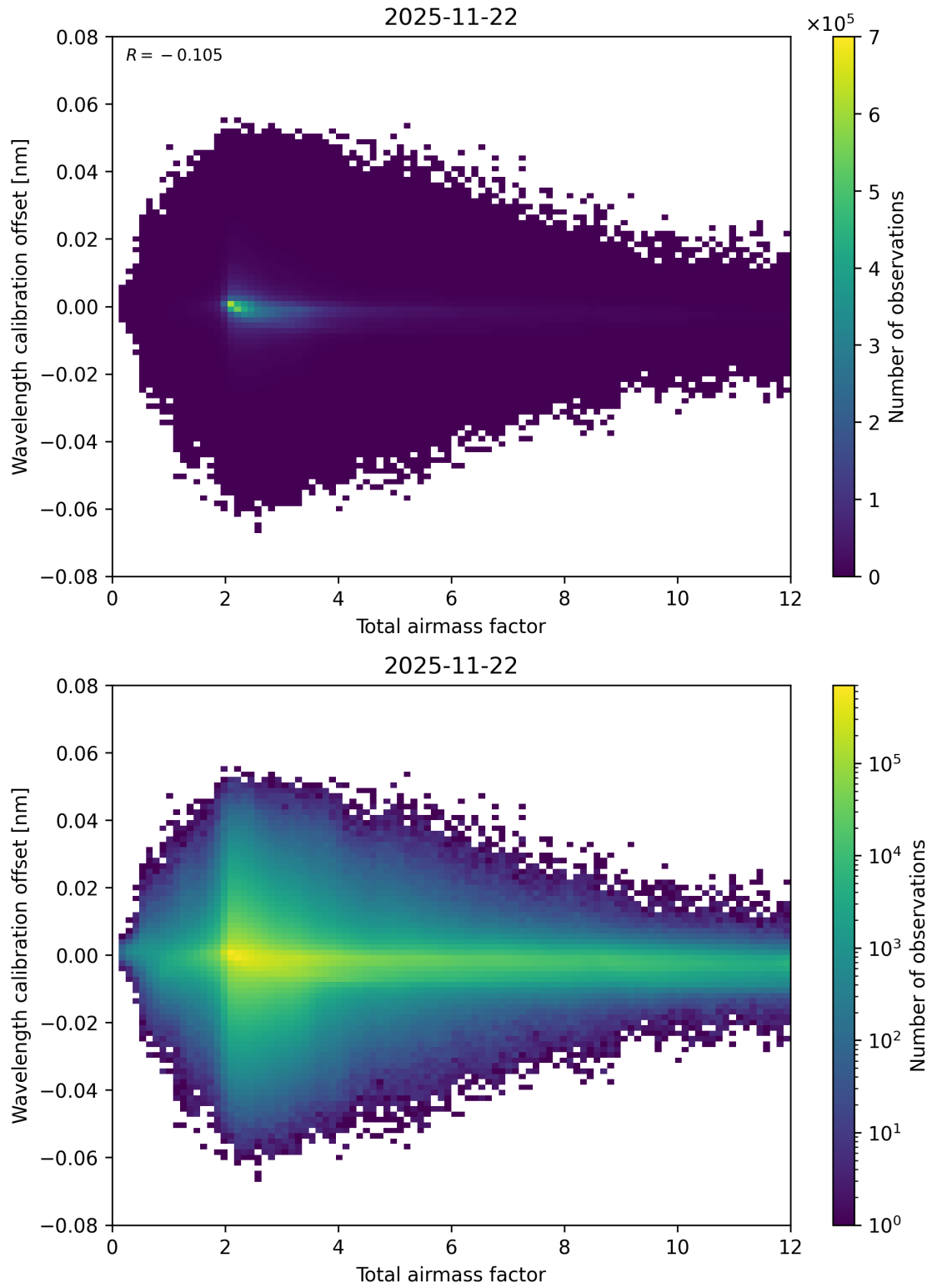
Figure 70: Scatter density plot of “Total airmass factor” against “Wavelength calibration offset” for 2025-11-21 to 2025-11-23.
