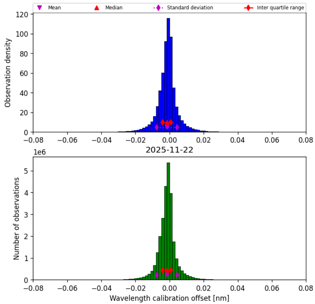
Figure 35: Histogram of “Wavelength calibration offset” for 2025-11-21 to 2025-11-23
