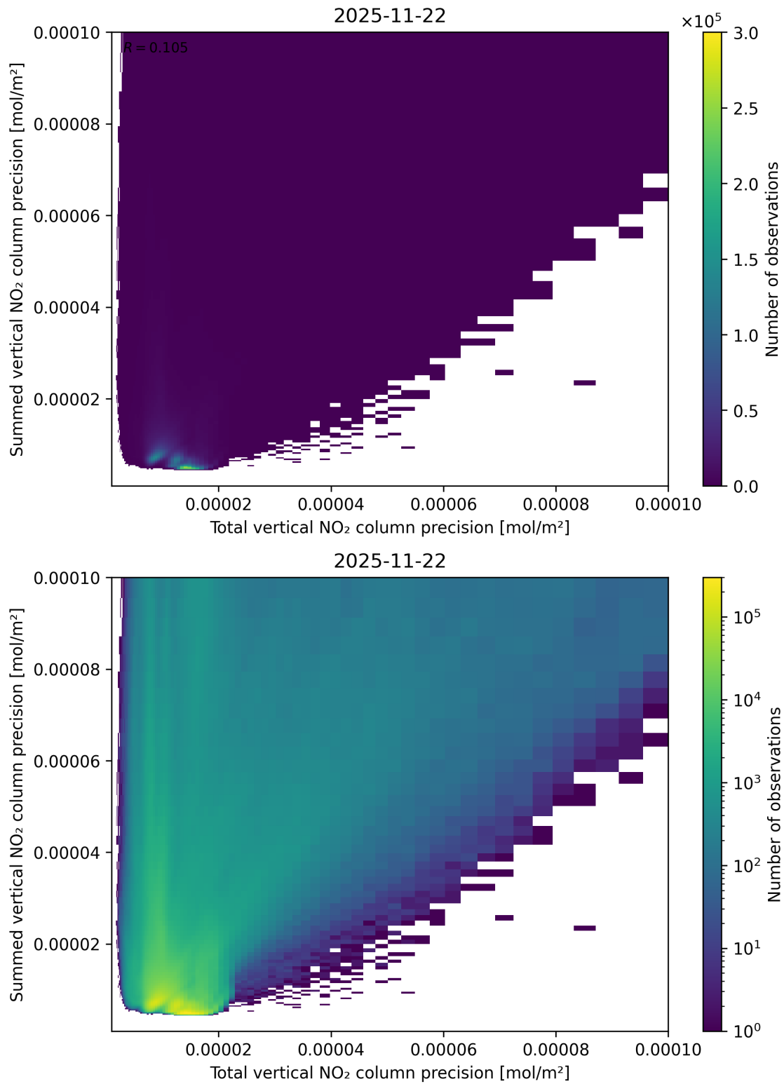
Figure 118: Scatter density plot of “Total vertical NO 2 column precision” against “Summed vertical NO 2 column precision” for 2025-11-21 to 2025-11-23.
