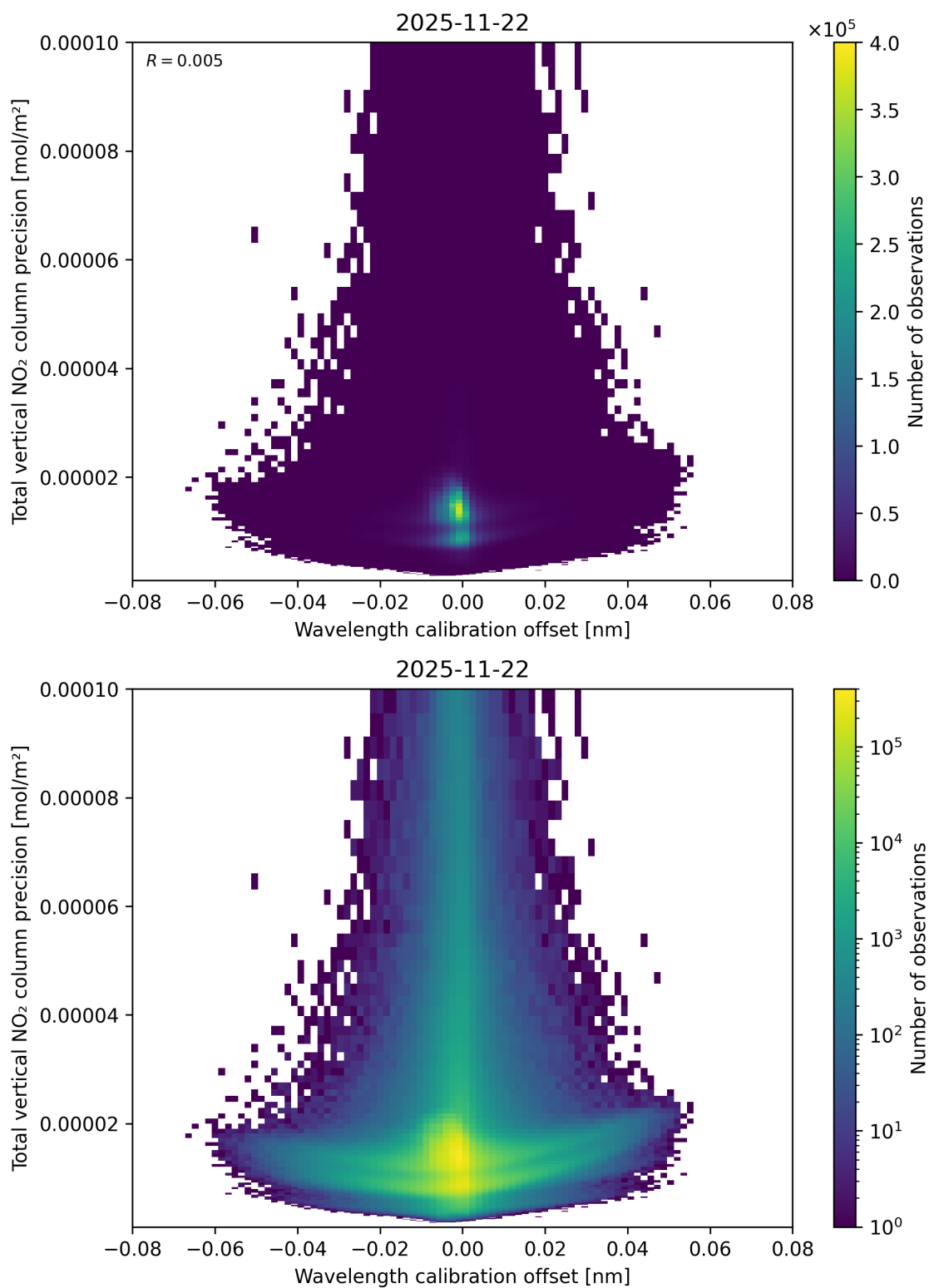
Figure 180: Scatter density plot of “Wavelength calibration offset” against “Total vertical NO 2 column precision” for 2025-11-21 to 2025-11-23.
