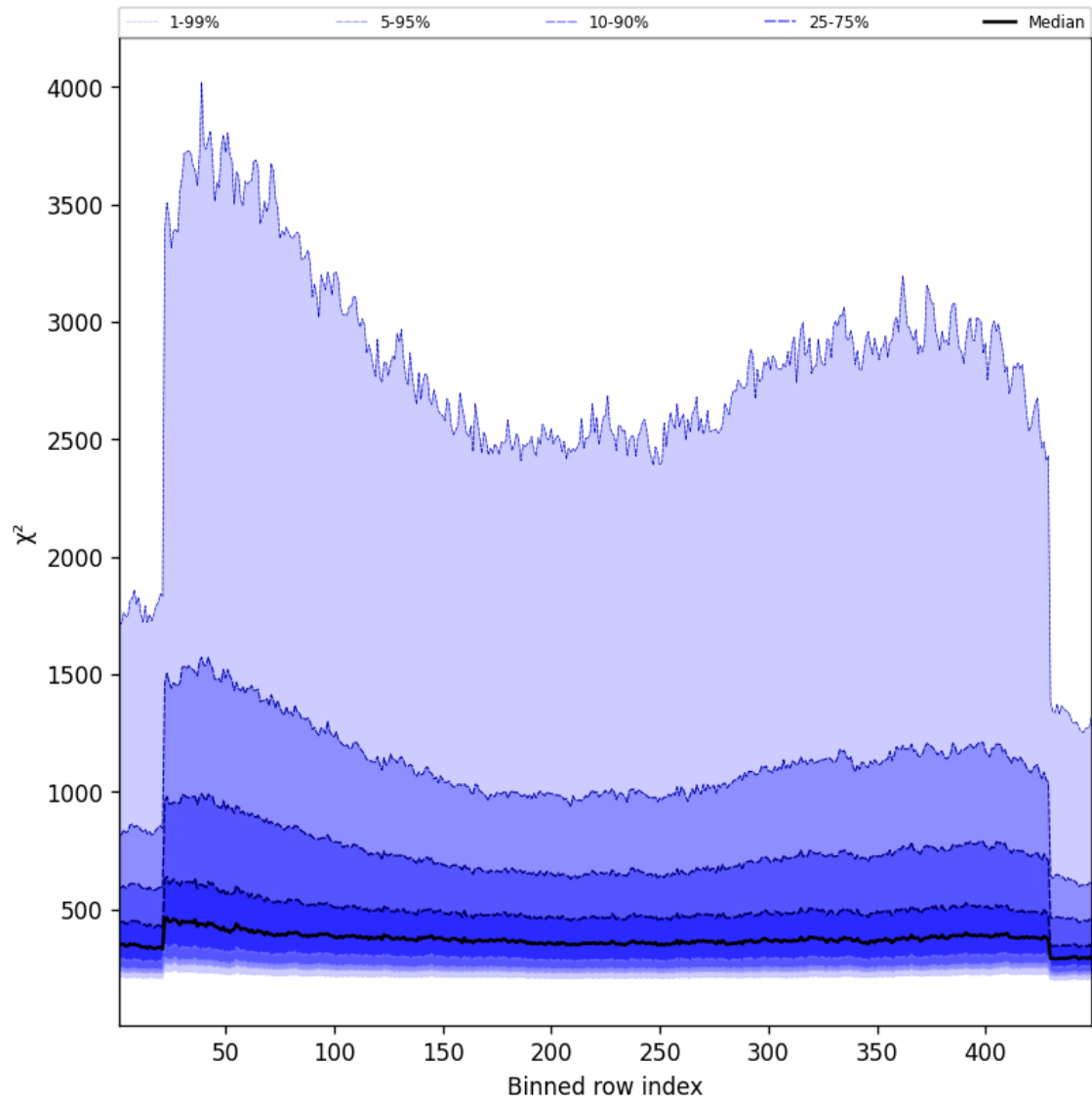
Figure 59: Along track statistics of “ \chi^2 ” for 2025-11-21 to 2025-11-23
