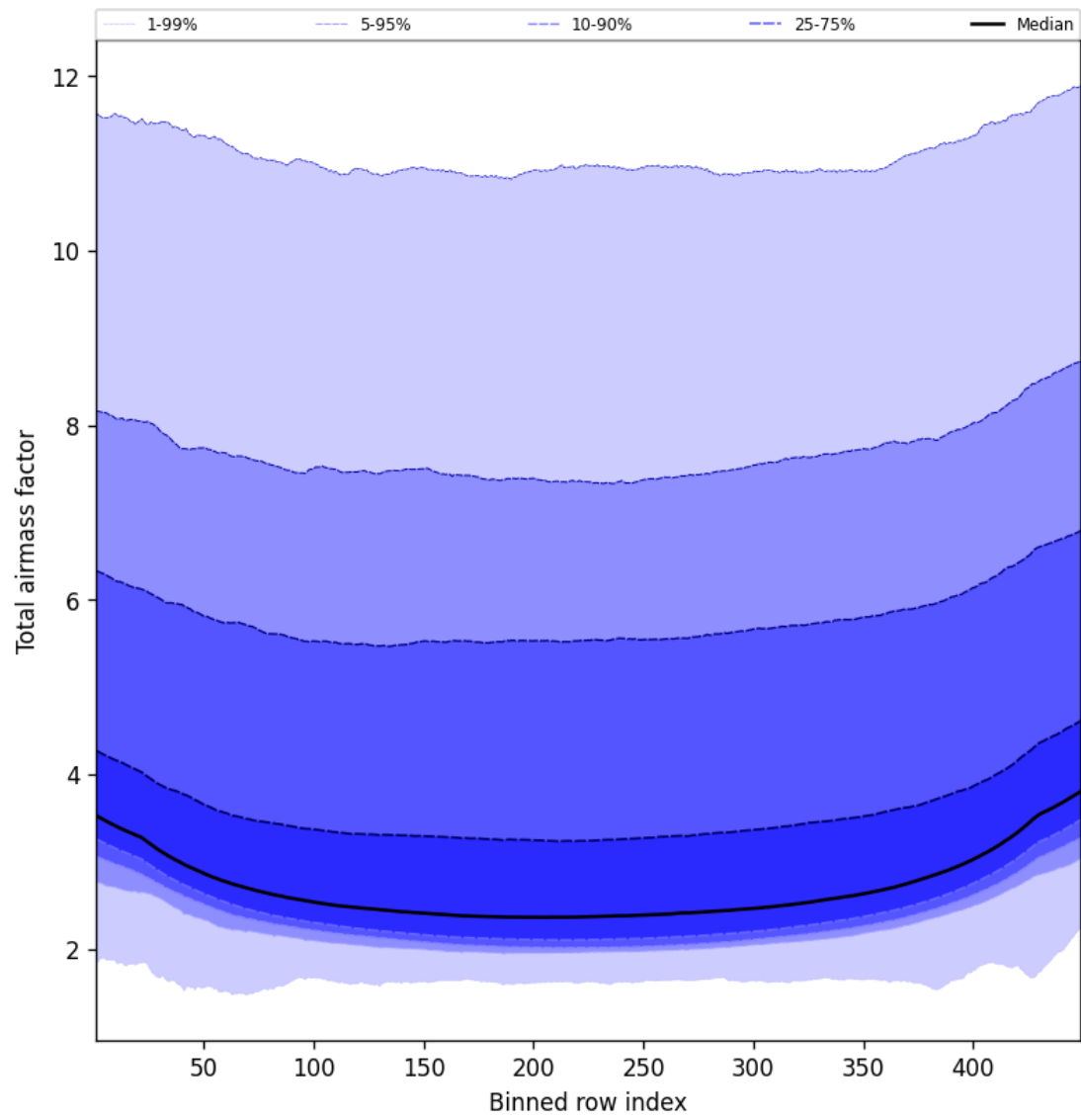
Figure 49: Along track statistics of “Total airmass factor” for 2025-11-21 to 2025-11-23
