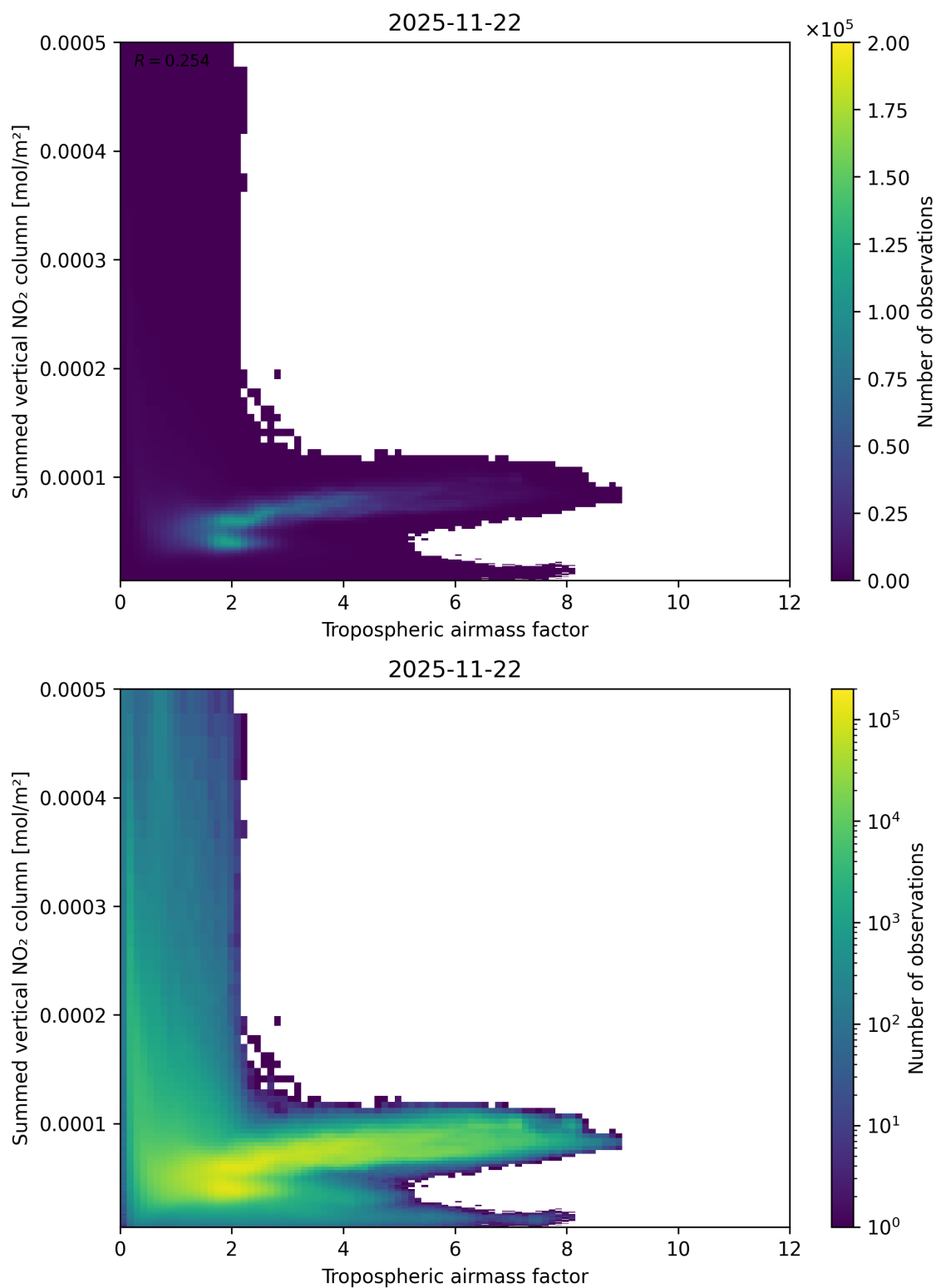
Figure 75: Scatter density plot of “Tropospheric air mass factor” against “Summed vertical NO 2 column” for 2025-11-21 to 2025-11-23.
