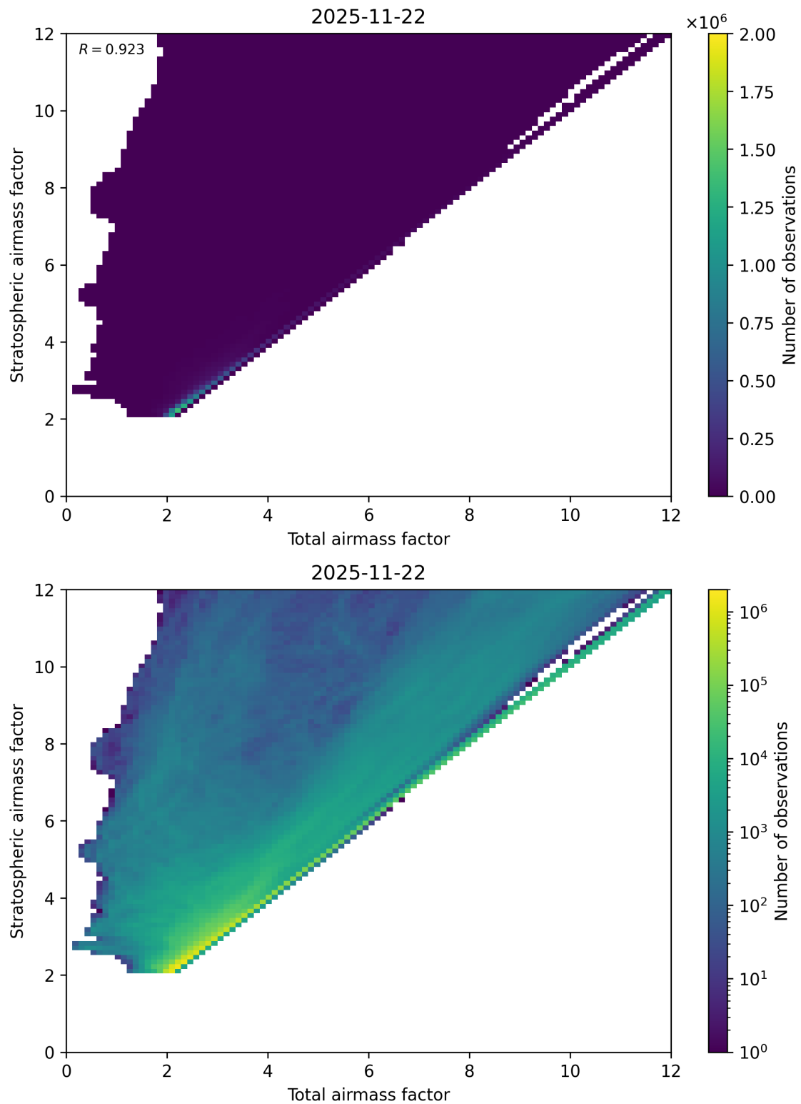
Figure 62: Scatter density plot of “Total airmass factor” against “Stratospheric airmass factor” for 2025-11-21 to 2025-11-23.
