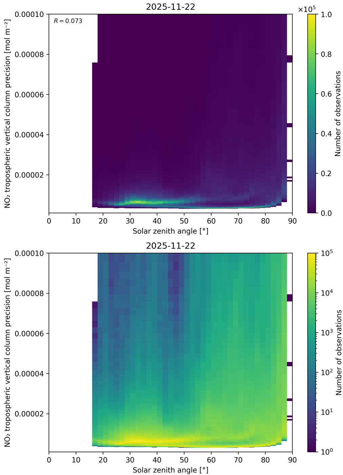
Figure 156: Scatter density plot of “Solar zenith angle” against “NO 2 tropospheric vertical column precision” for 2025-11-21 to 2025-11-23.
