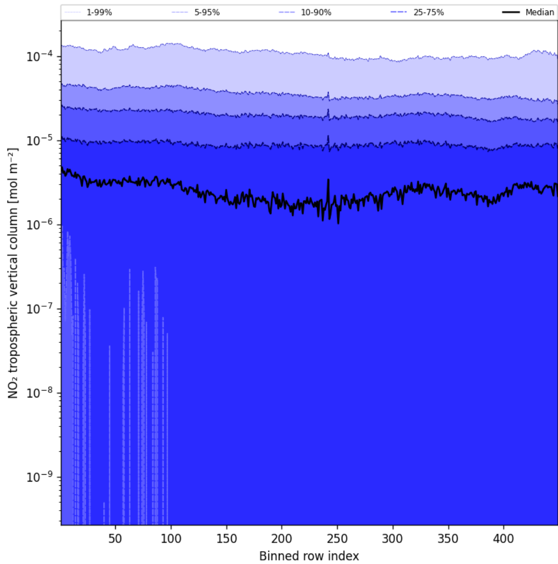
Figure 46: Along track statistics of “NO 2 tropospheric vertical column” for 2025-11-21 to 2025-11-23
