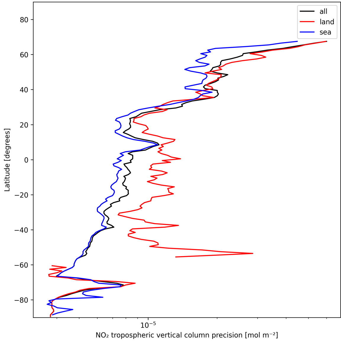
Figure 13: Zonal average of “NO 2 tropospheric vertical column precision” for 2025-11-21 to 2025-11-23.
