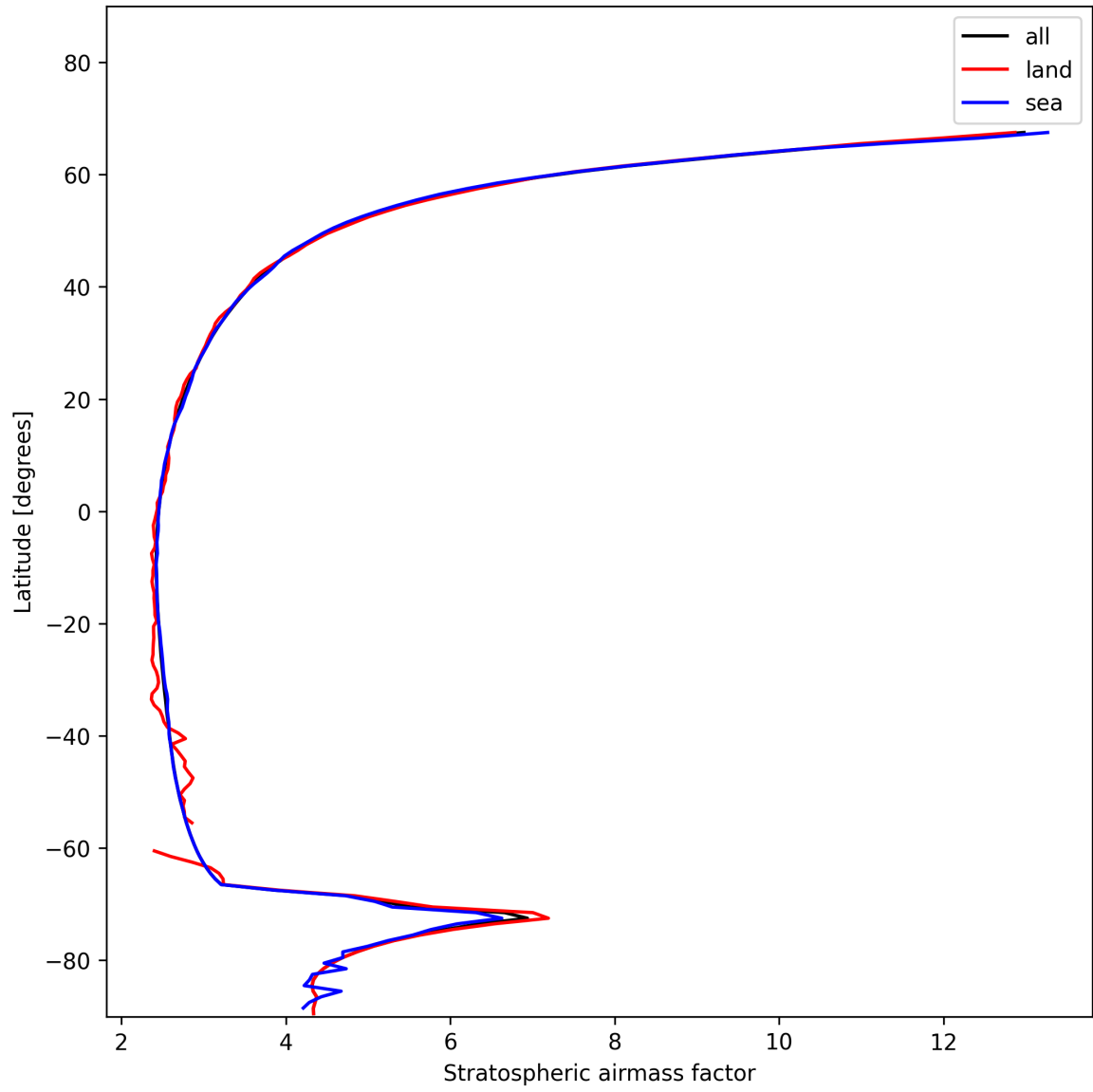
Figure 27: Zonal average of “Stratospheric air mass factor” for 2025-11-21 to 2025-11-23.
