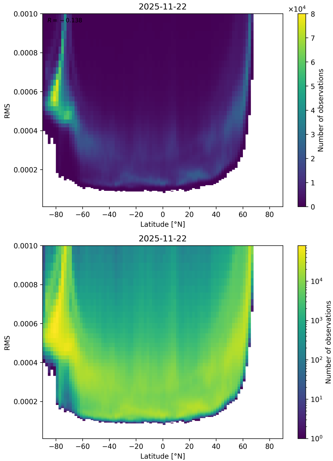
Figure 94: Scatter density plot of “Latitude” against “RMS” for 2025-11-21 to 2025-11-23.
