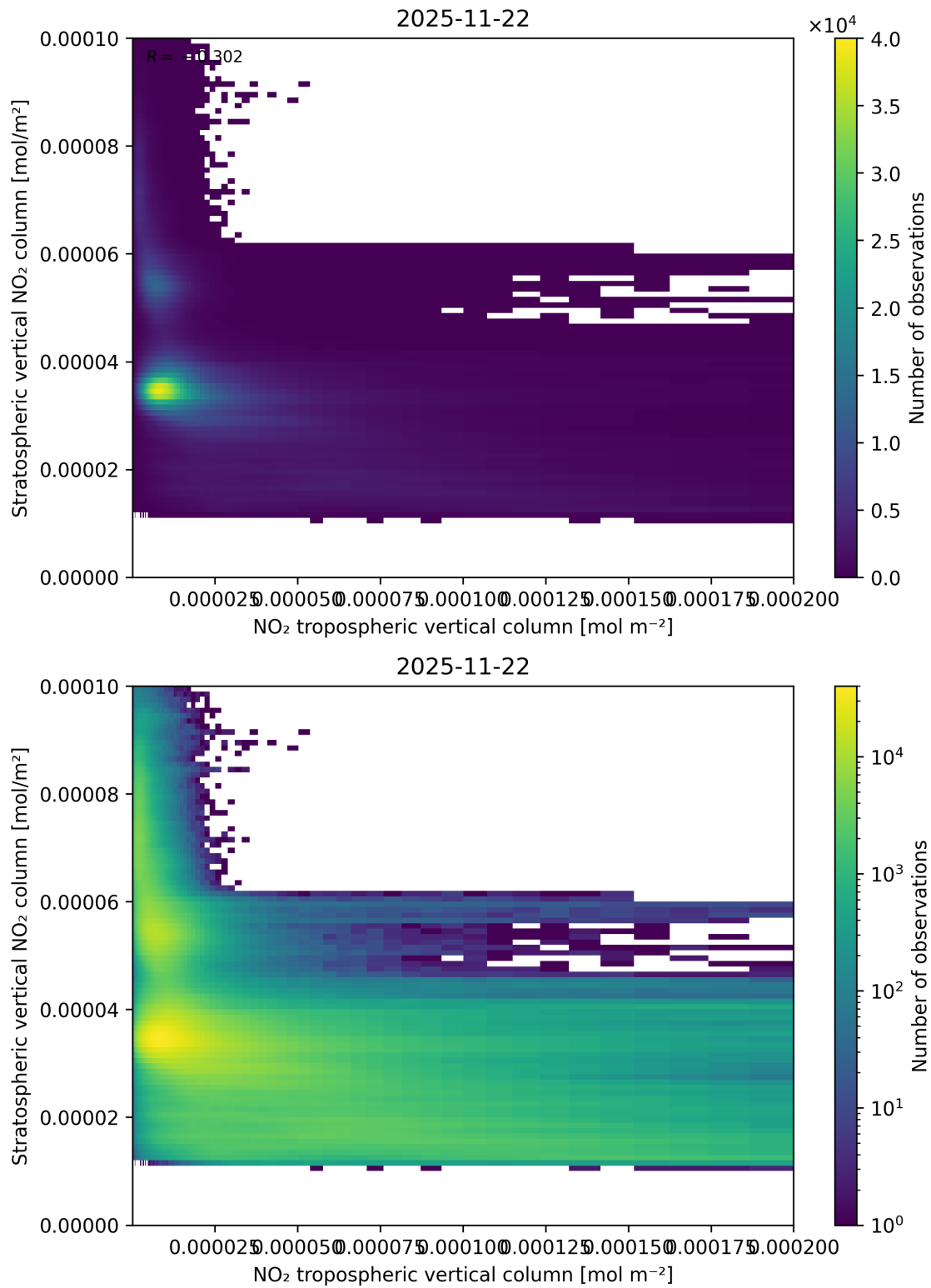
Figure 125: Scatter density plot of “NO 2 tropospheric vertical column” against “Stratospheric vertical NO 2 column” for 2025-11-21 to 2025-11-23.
