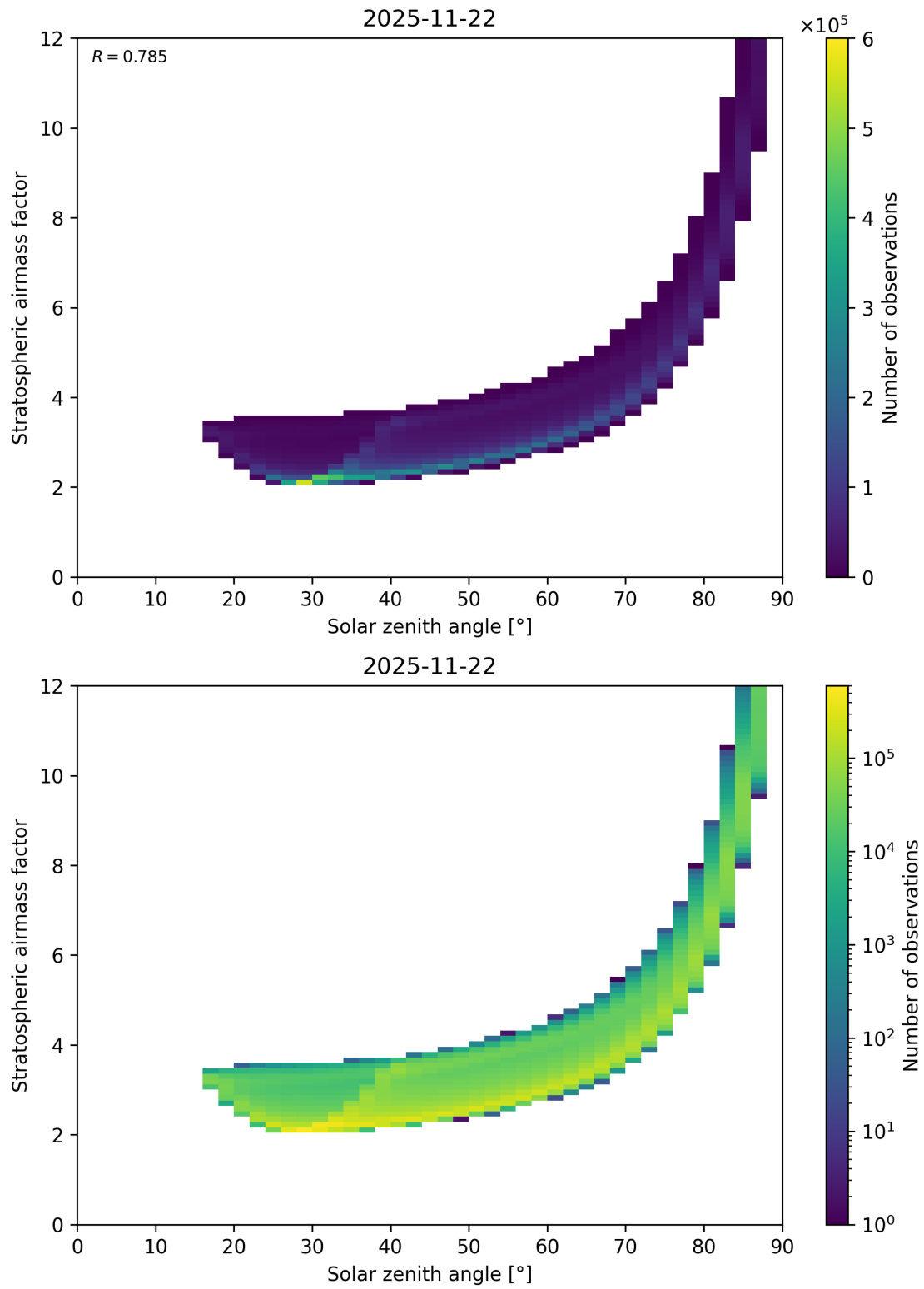
Figure 145: Scatter density plot of “Solar zenith angle” against “Stratospheric airmass factor” for 2025-11-21 to 2025-11-23.
