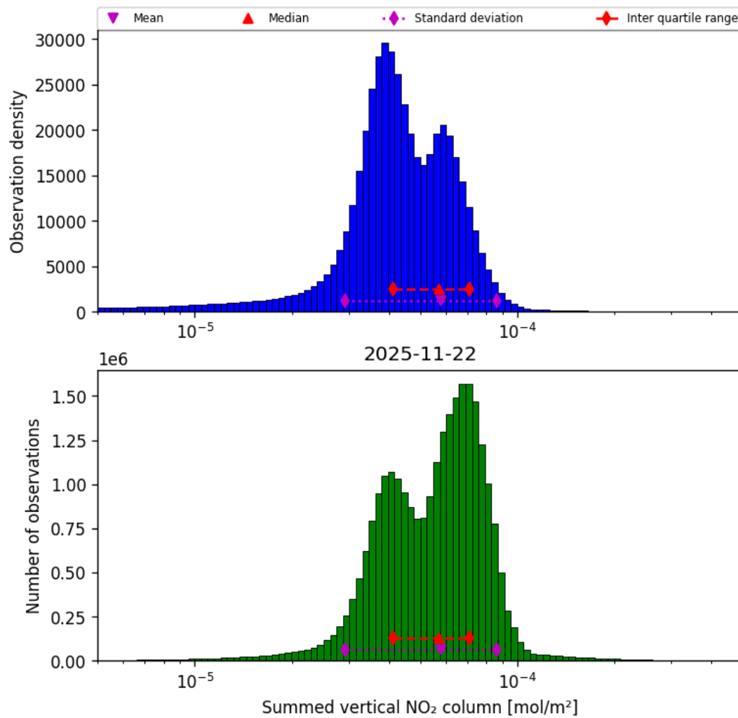
Figure 40: Histogram of “Summed vertical NO 2 column” for 2025-11-21 to 2025-11-23
