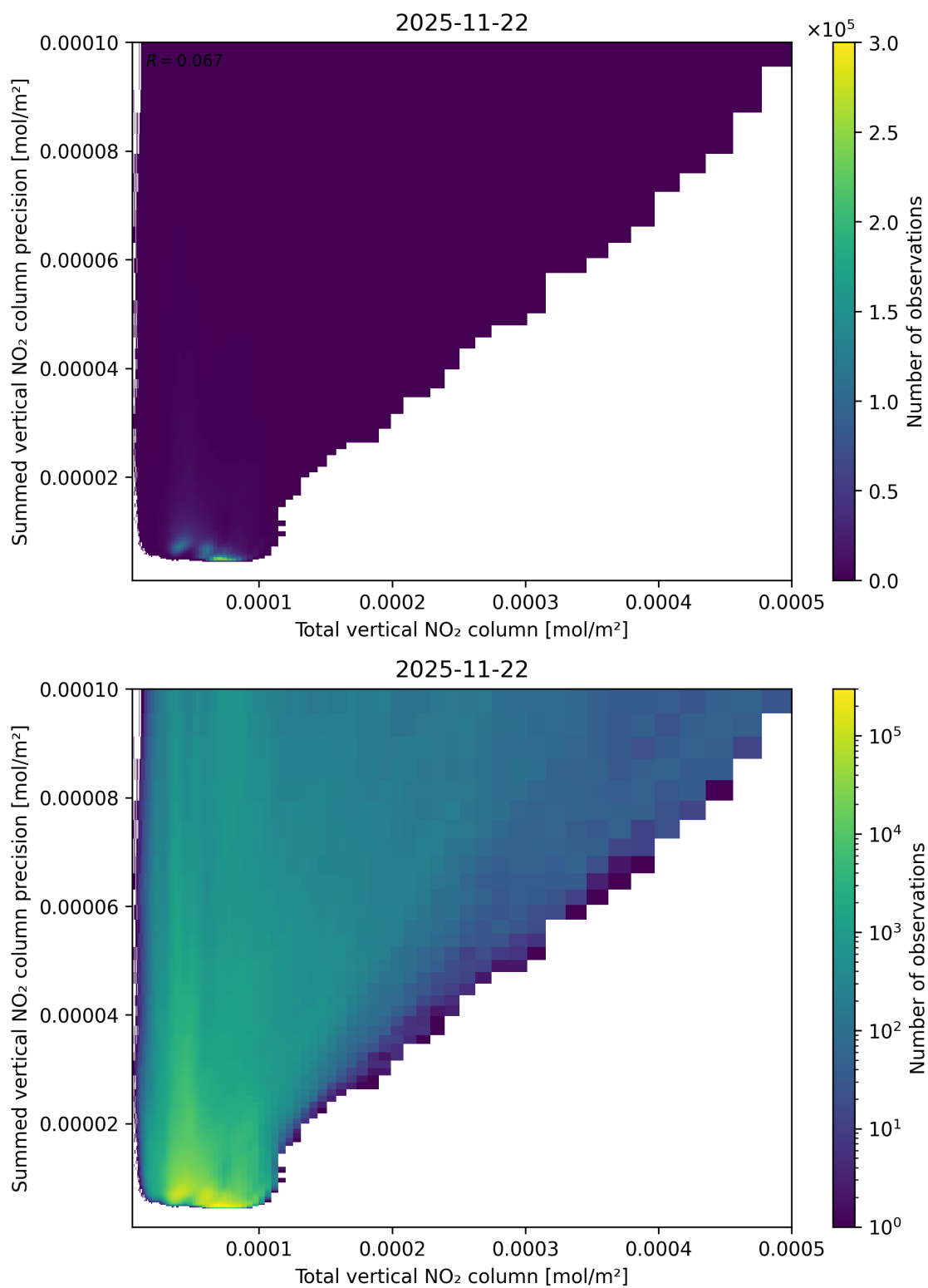
Figure 113: Scatter density plot of “Total vertical NO 2 column” against “Summed vertical NO 2 column precision” for 2025-11-21 to 2025-11-23.
