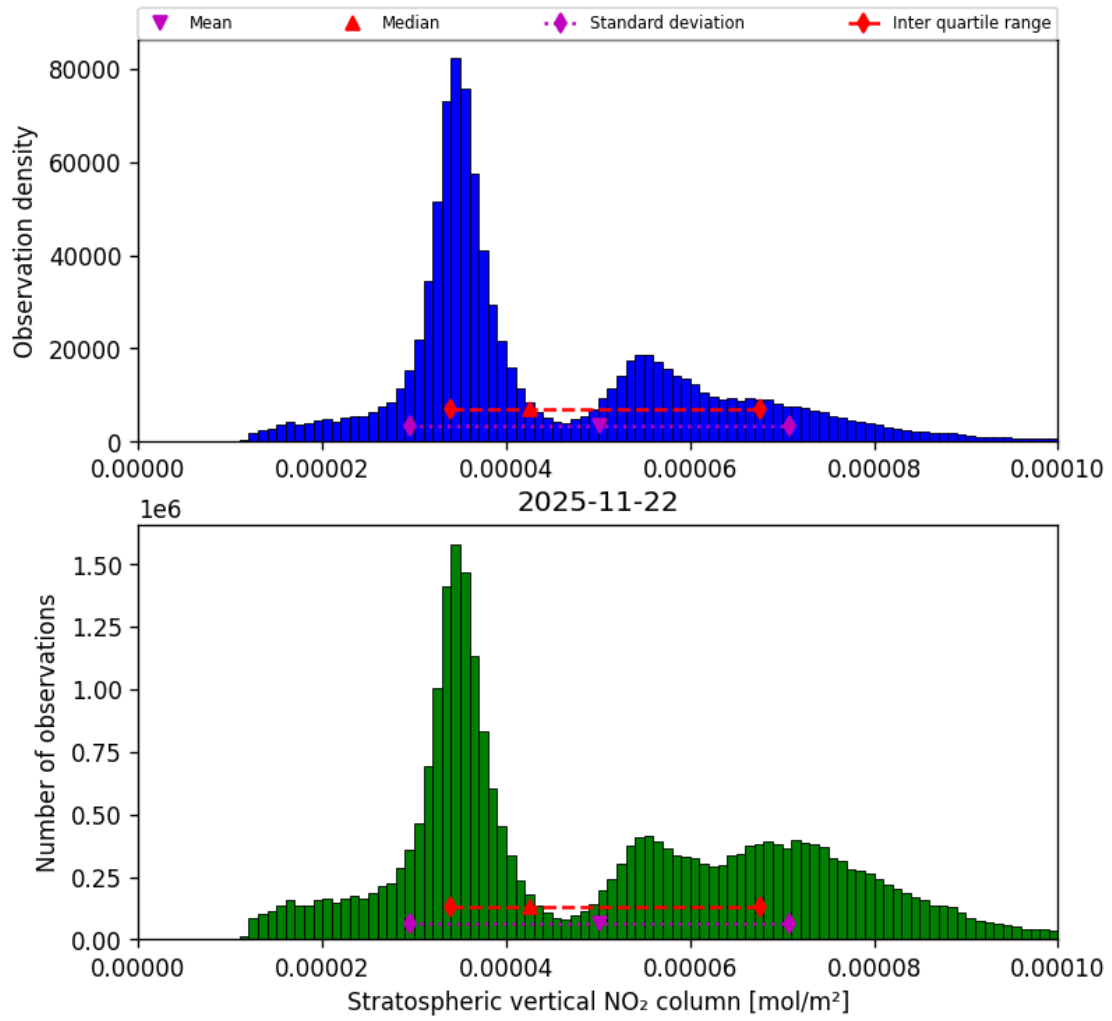
Figure 36: Histogram of “Stratospheric vertical NO 2 column” for 2025-11-21 to 2025-11-23
