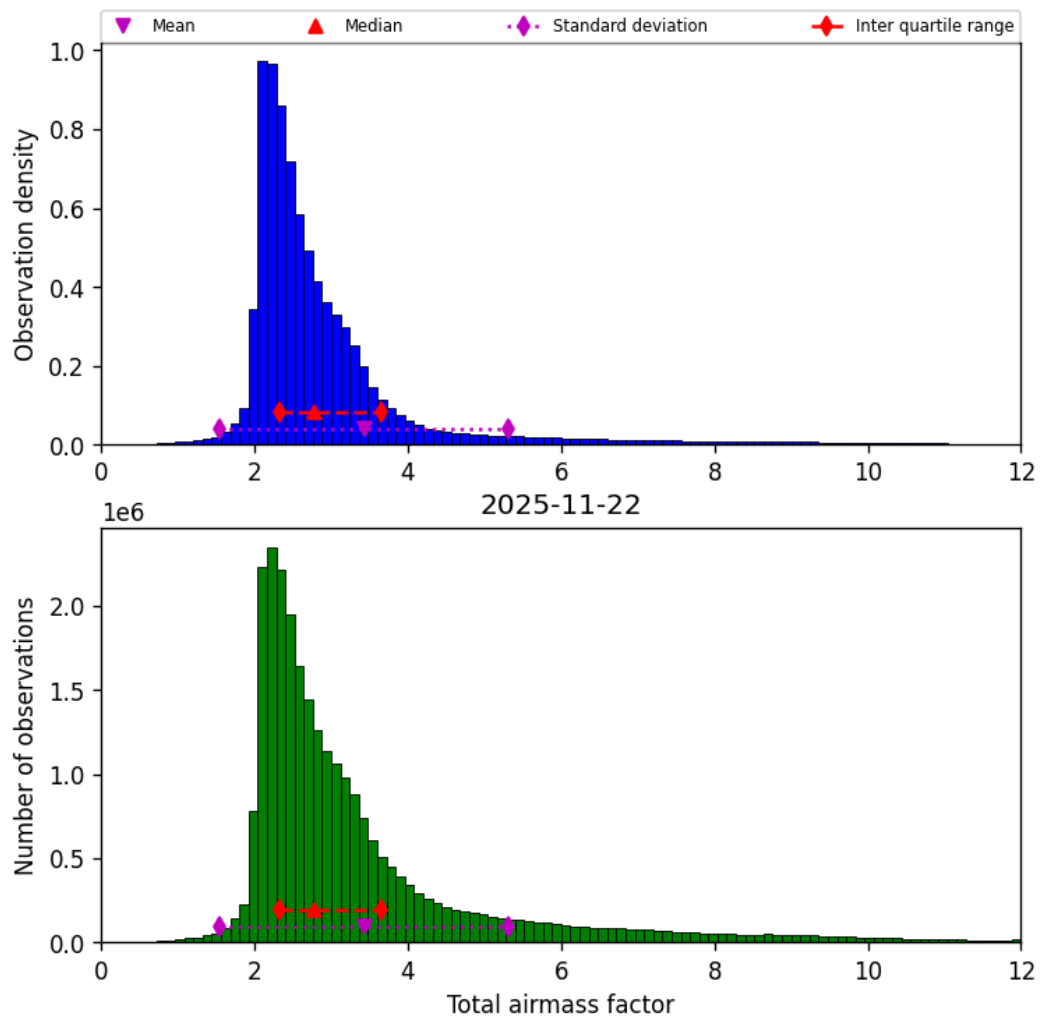
Figure 32: Histogram of “Total airmass factor” for 2025-11-21 to 2025-11-23
