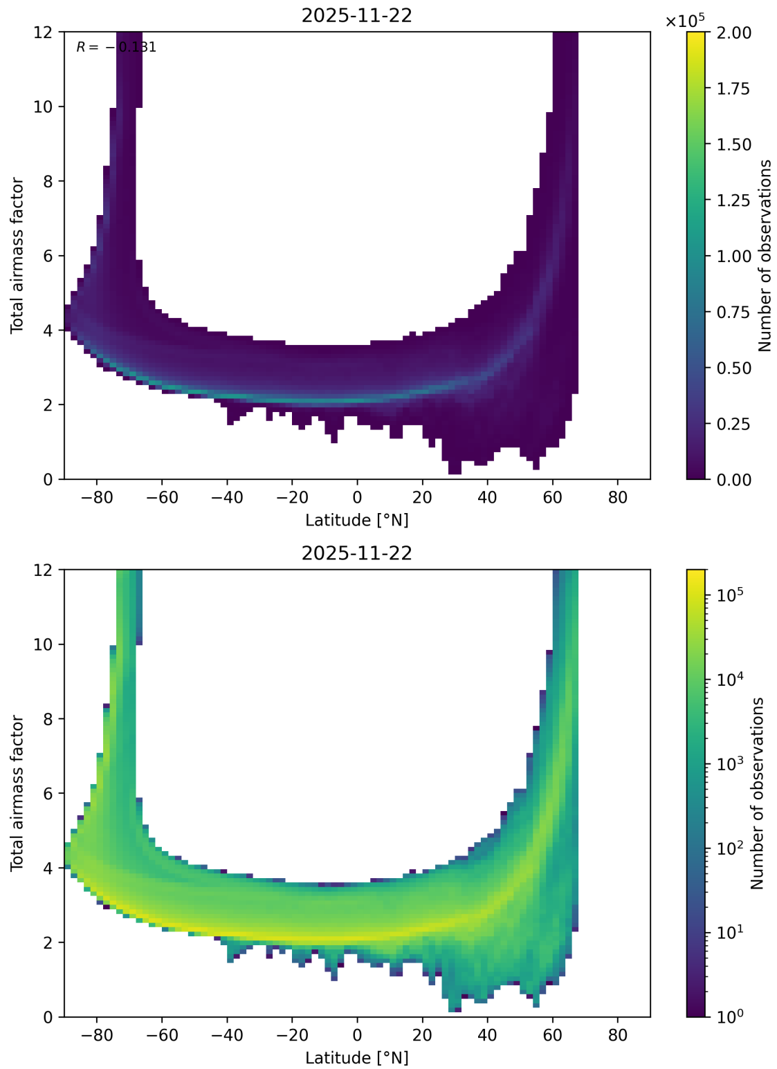
Figure 84: Scatter density plot of “Latitude” against “Total airmass factor” for 2025-11-21 to 2025-11-23.
