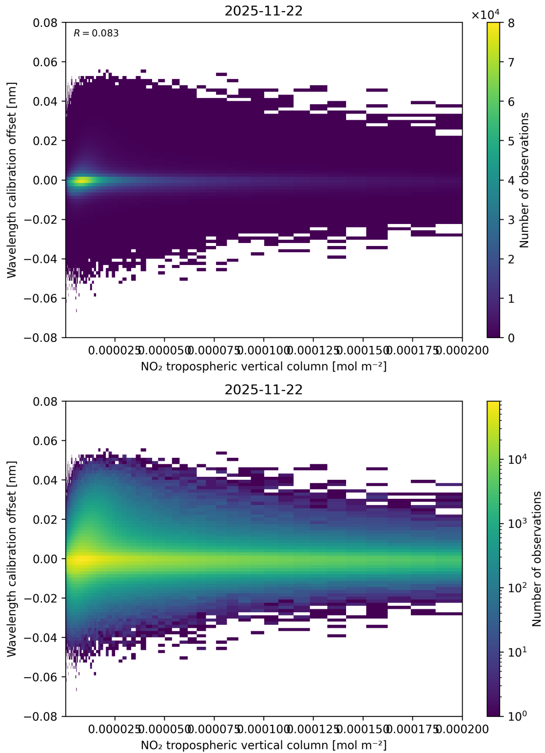
Figure 143: Scatter density plot of “NO 2 tropospheric vertical column” against “Wavelength calibration offset” for 2025-11-21 to 2025-11-23.
