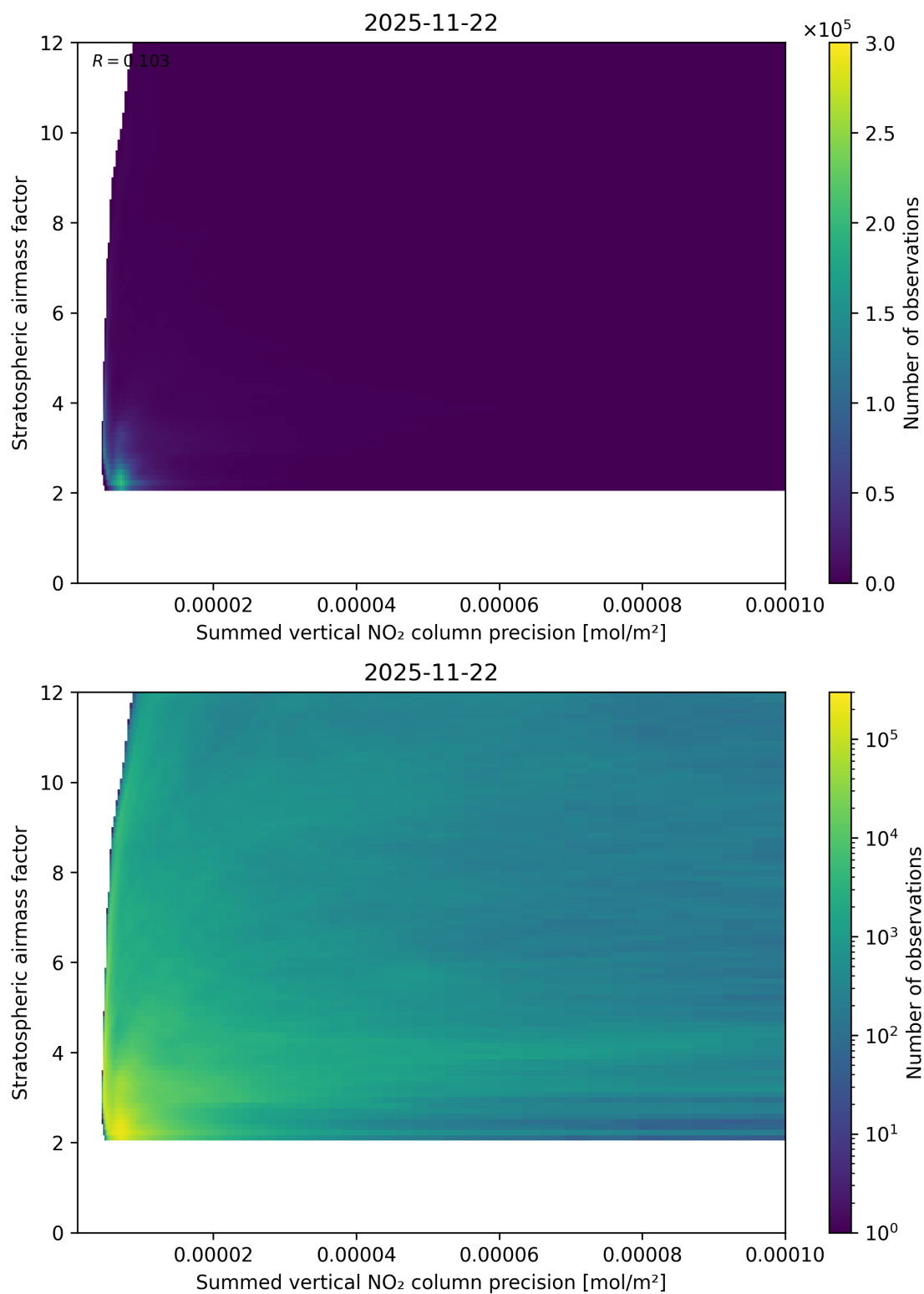
Figure 106: Scatter density plot of “Summed vertical NO 2 column precision” against “Stratospheric airmass factor” for 2025-11-21 to 2025-11-23.
