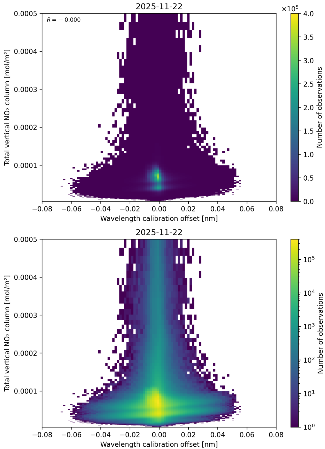
Figure 179: Scatter density plot of “Wavelength calibration offset” against “Total vertical NO 2 column” for 2025-11-21 to 2025-11-23.
