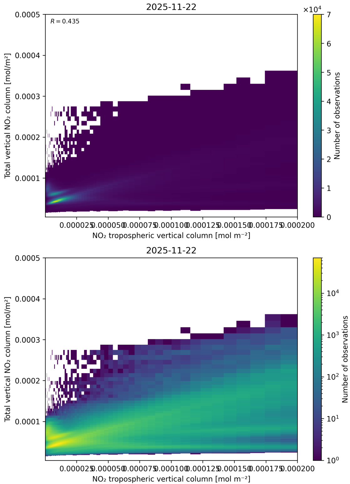
Figure 128: Scatter density plot of “NO 2 tropospheric vertical column” against “Total vertical NO 2 column” for 2025-11-21 to 2025-11-23.
