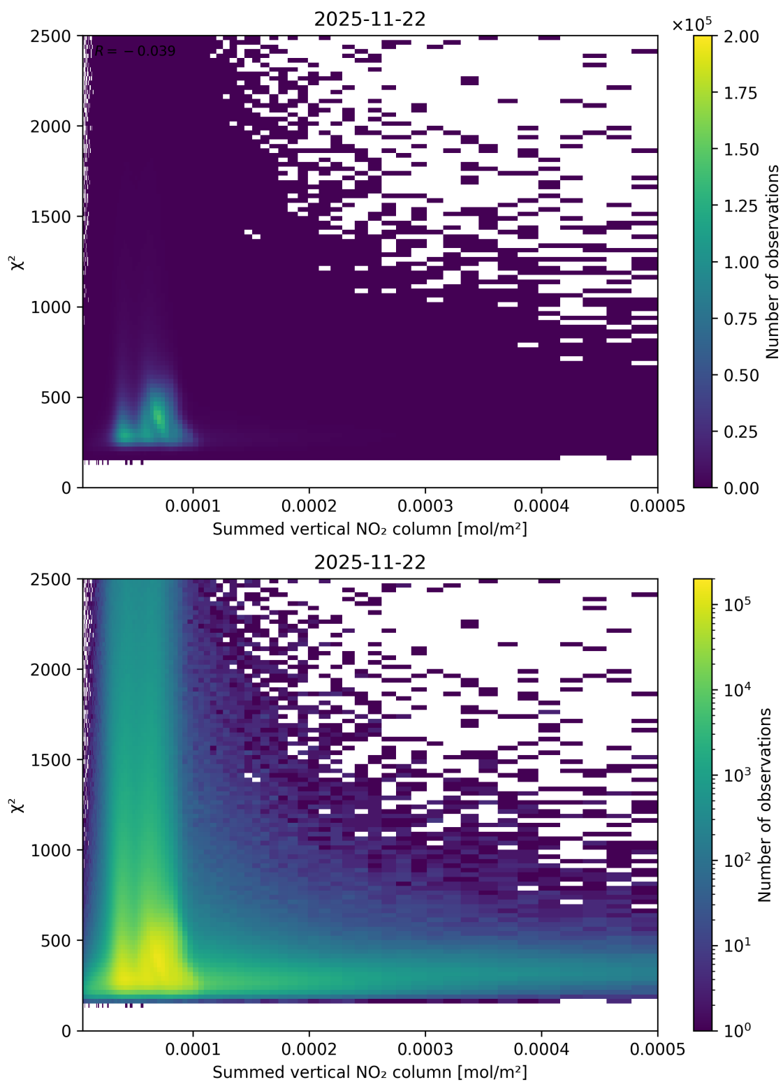
Figure 104: Scatter density plot of “Summed vertical NO 2 column” against “ \chi^2 ” for 2025-11-21 to 2025-11-23.
