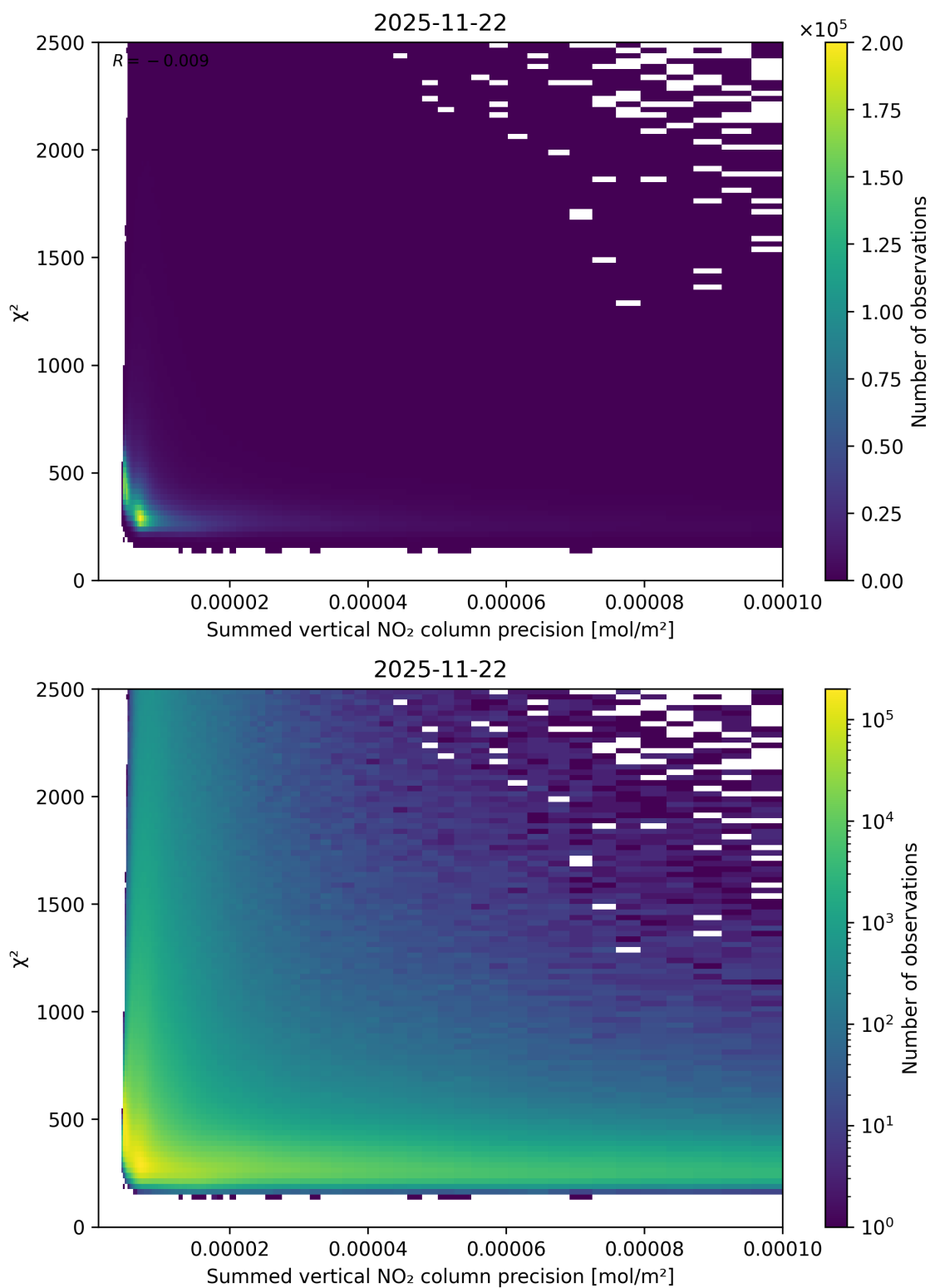
Figure 107: Scatter density plot of “Summed vertical NO 2 column precision” against “ \chi^2 ” for 2025-11-21 to 2025-11-23.
