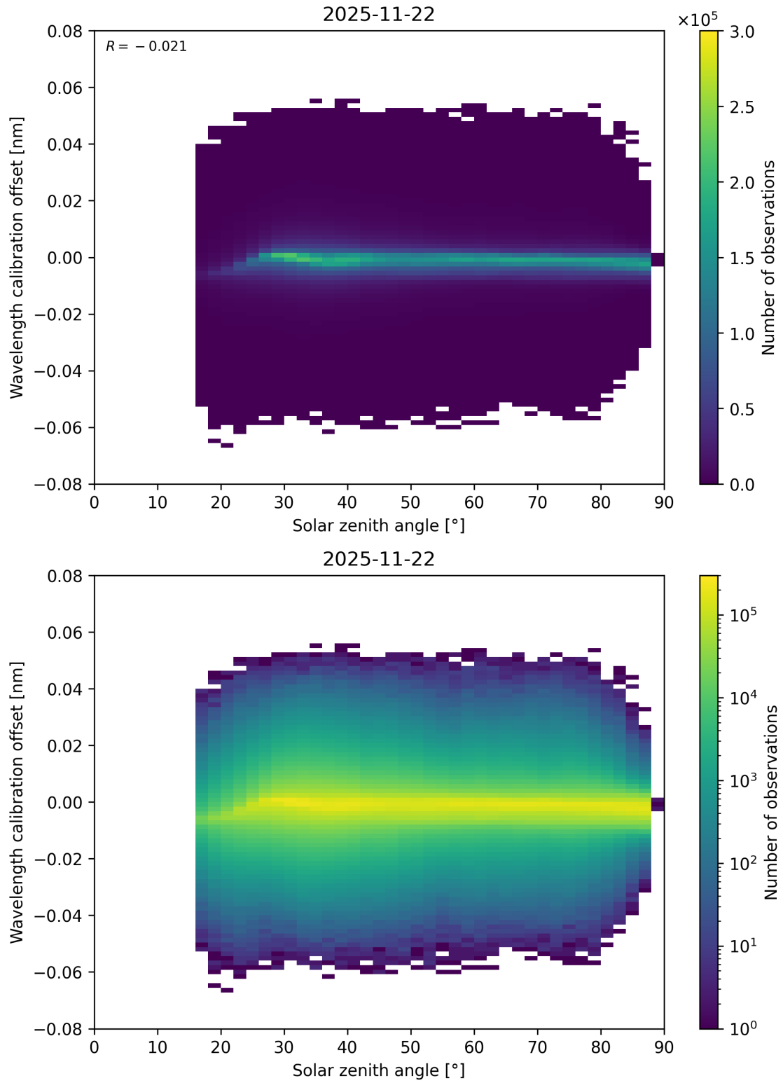
Figure 158: Scatter density plot of “Solar zenith angle” against “Wavelength calibration offset” for 2025-11-21 to 2025-11-23.
