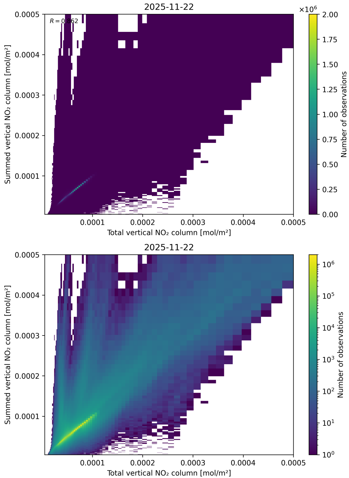
Figure 112: Scatter density plot of “Total vertical NO 2 column” against “Summed vertical NO 2 column” for 2025-11-21 to 2025-11-23.
