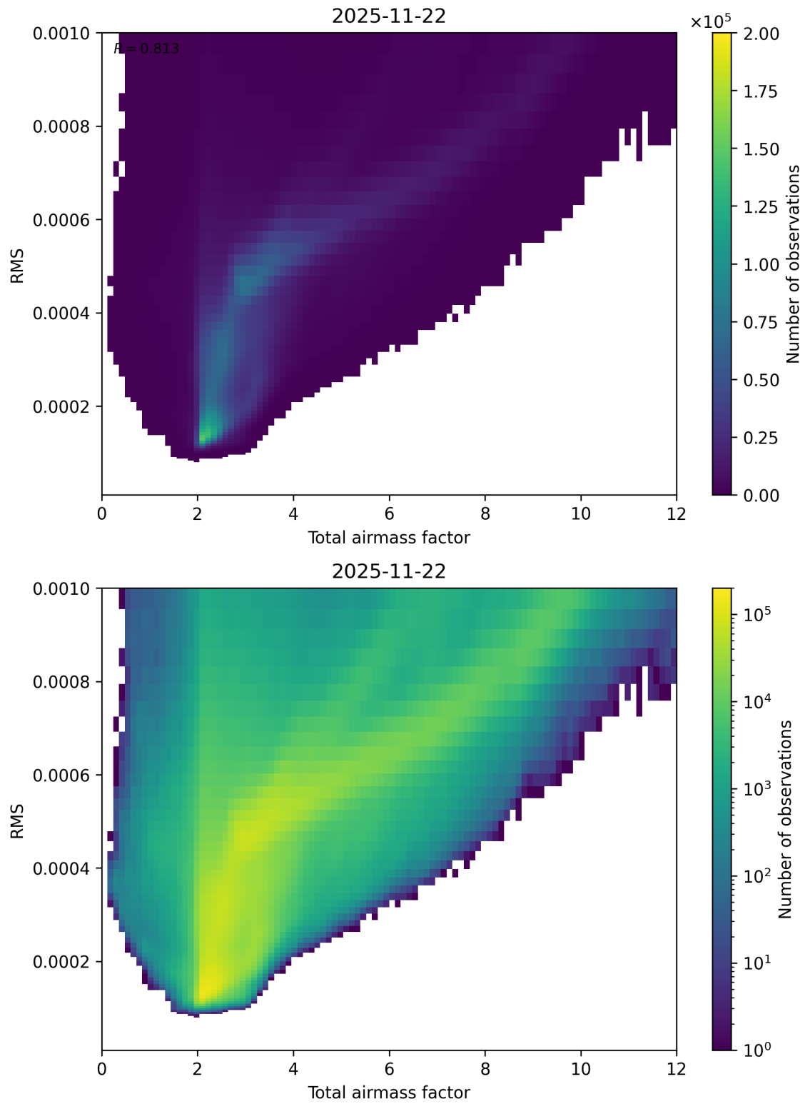
Figure 69: Scatter density plot of “Total airmass factor” against “RMS” for 2025-11-21 to 2025-11-23.
