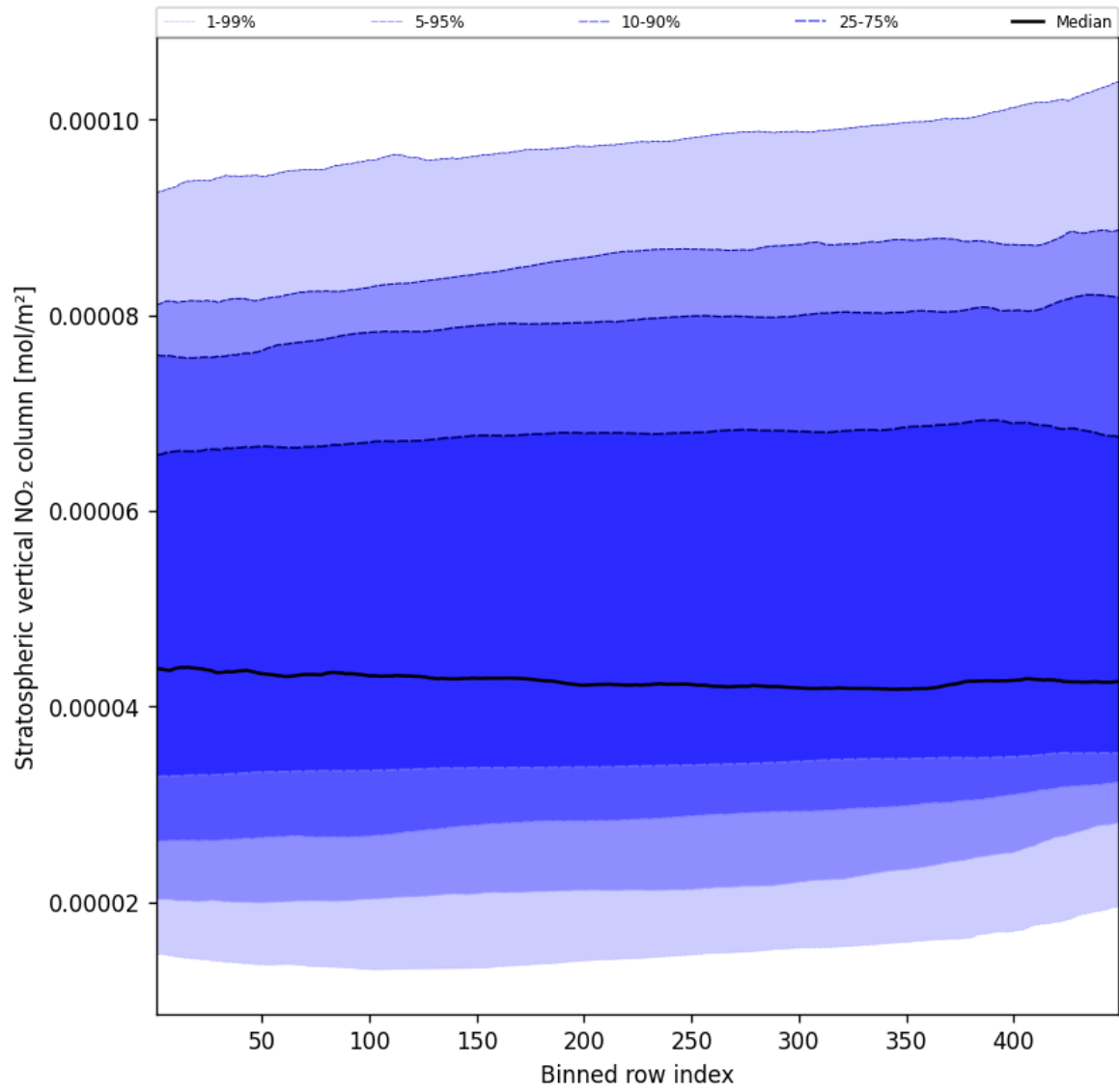
Figure 53: Along track statistics of “Stratospheric vertical NO 2 column” for 2025-11-21 to 2025-11-23
