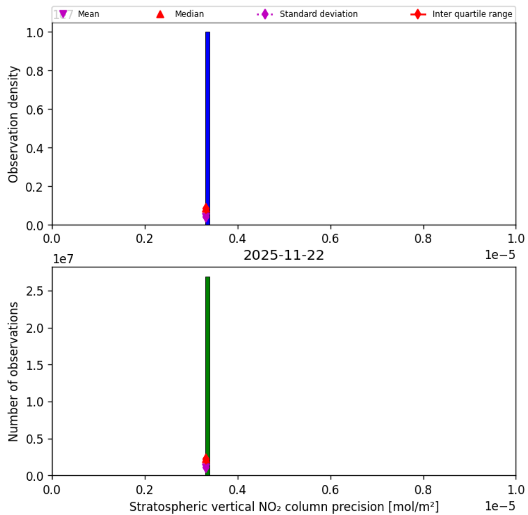
Figure 37: Histogram of “Stratospheric vertical NO 2 column precision” for 2025-11-21 to 2025-11-23
