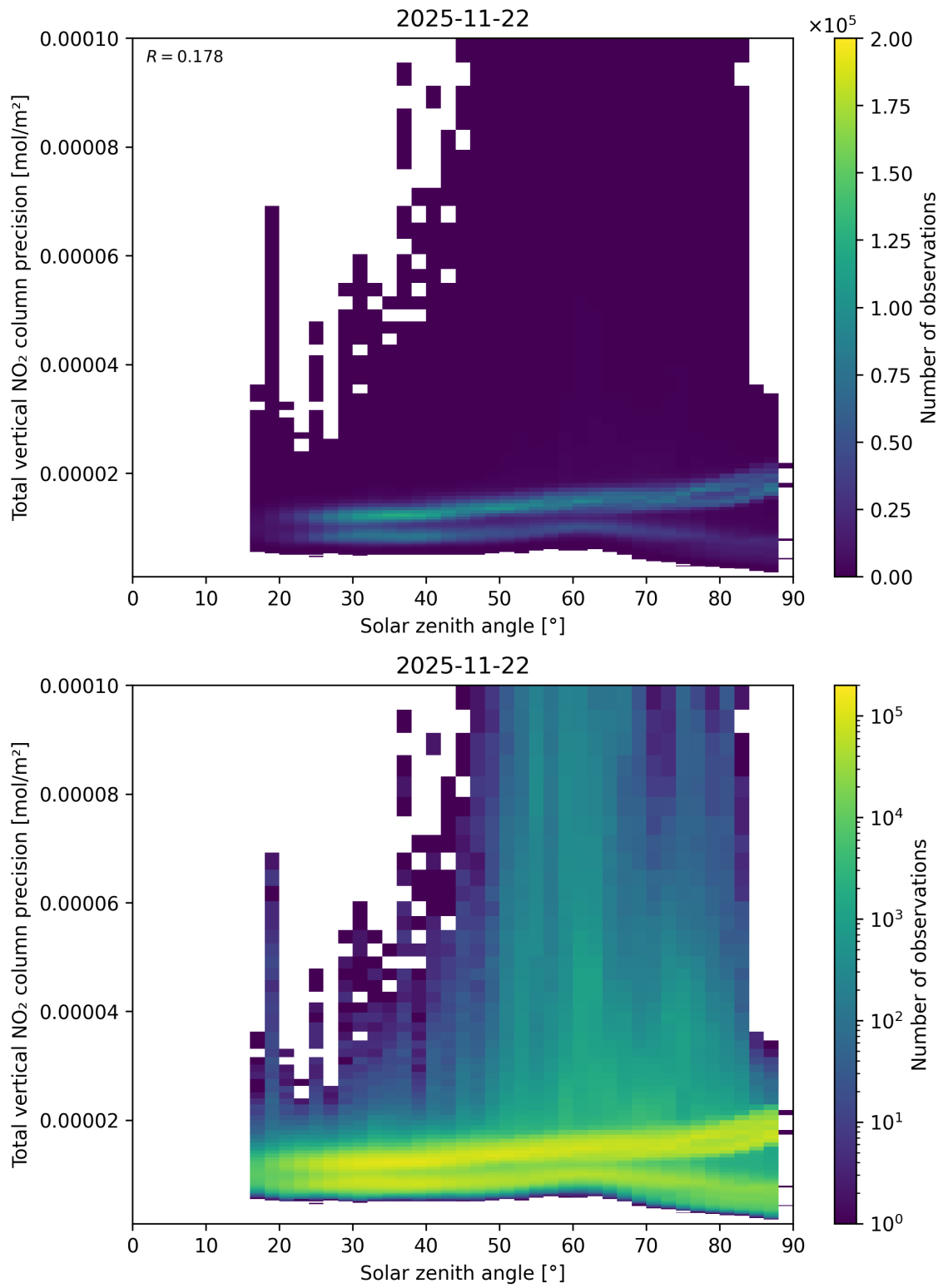
Figure 154: Scatter density plot of “Solar zenith angle” against “Total vertical NO 2 column precision” for 2025-11-21 to 2025-11-23.
