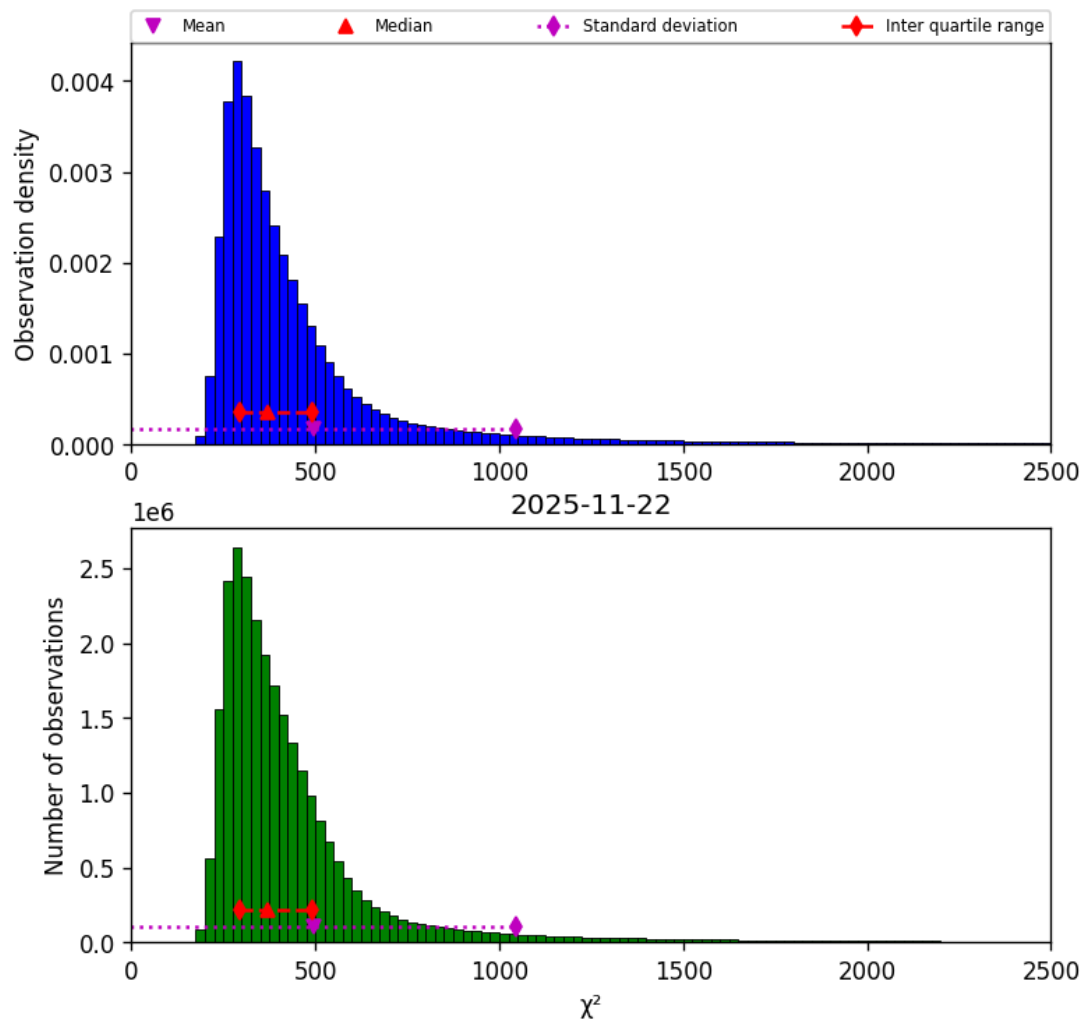
Figure 42: Histogram of “ \chi^2 ” for 2025-11-21 to 2025-11-23
