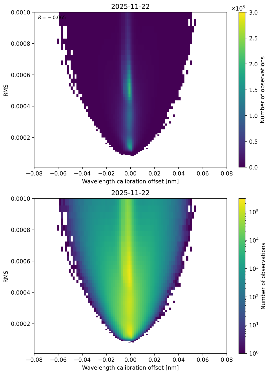
Figure 181: Scatter density plot of “Wavelength calibration offset” against “RMS” for 2025-11-21 to 2025-11-23.
