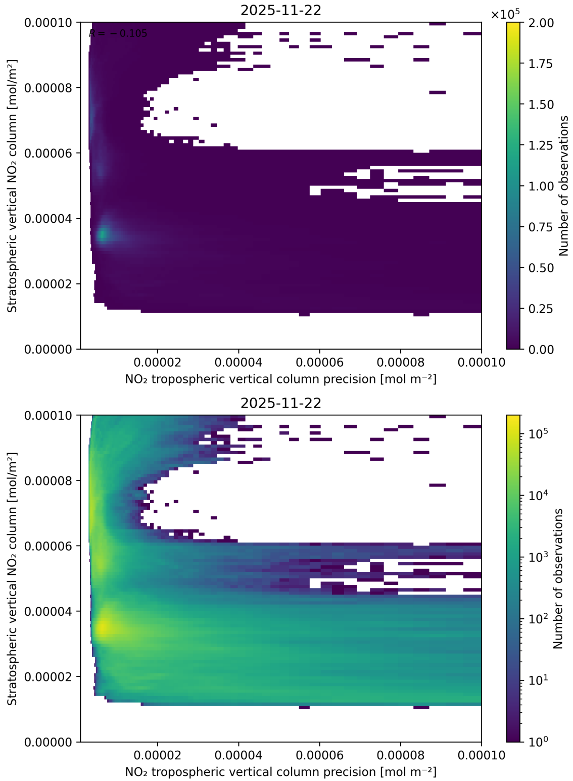
Figure 135: Scatter density plot of “NO 2 tropospheric vertical column precision” against “Stratospheric vertical NO 2 column” for 2025-11-21 to 2025-11-23.
