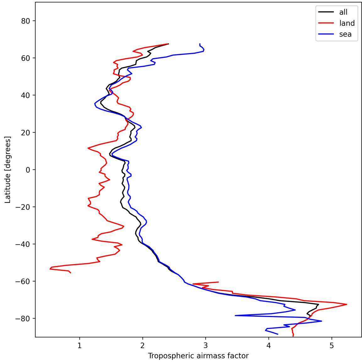
Figure 14: Zonal average of “Tropospheric air mass factor” for 2025-11-21 to 2025-11-23.
