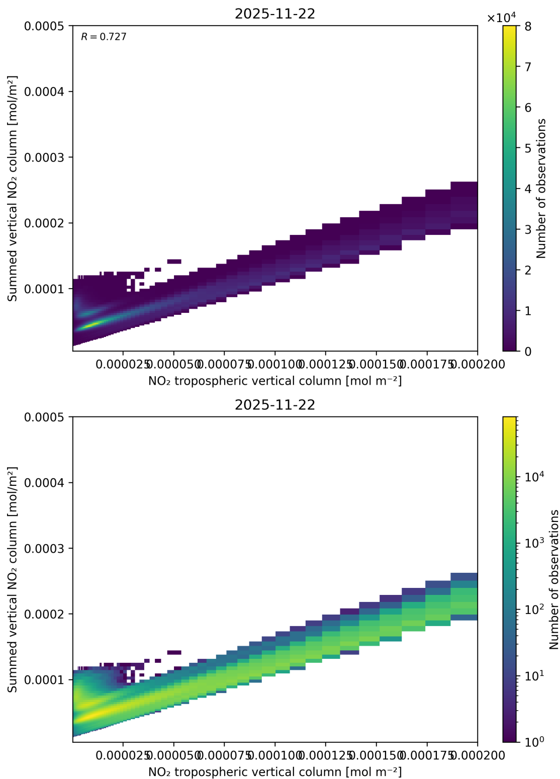
Figure 126: Scatter density plot of “NO 2 tropospheric vertical column” against “Summed vertical NO 2 column” for 2025-11-21 to 2025-11-23.
