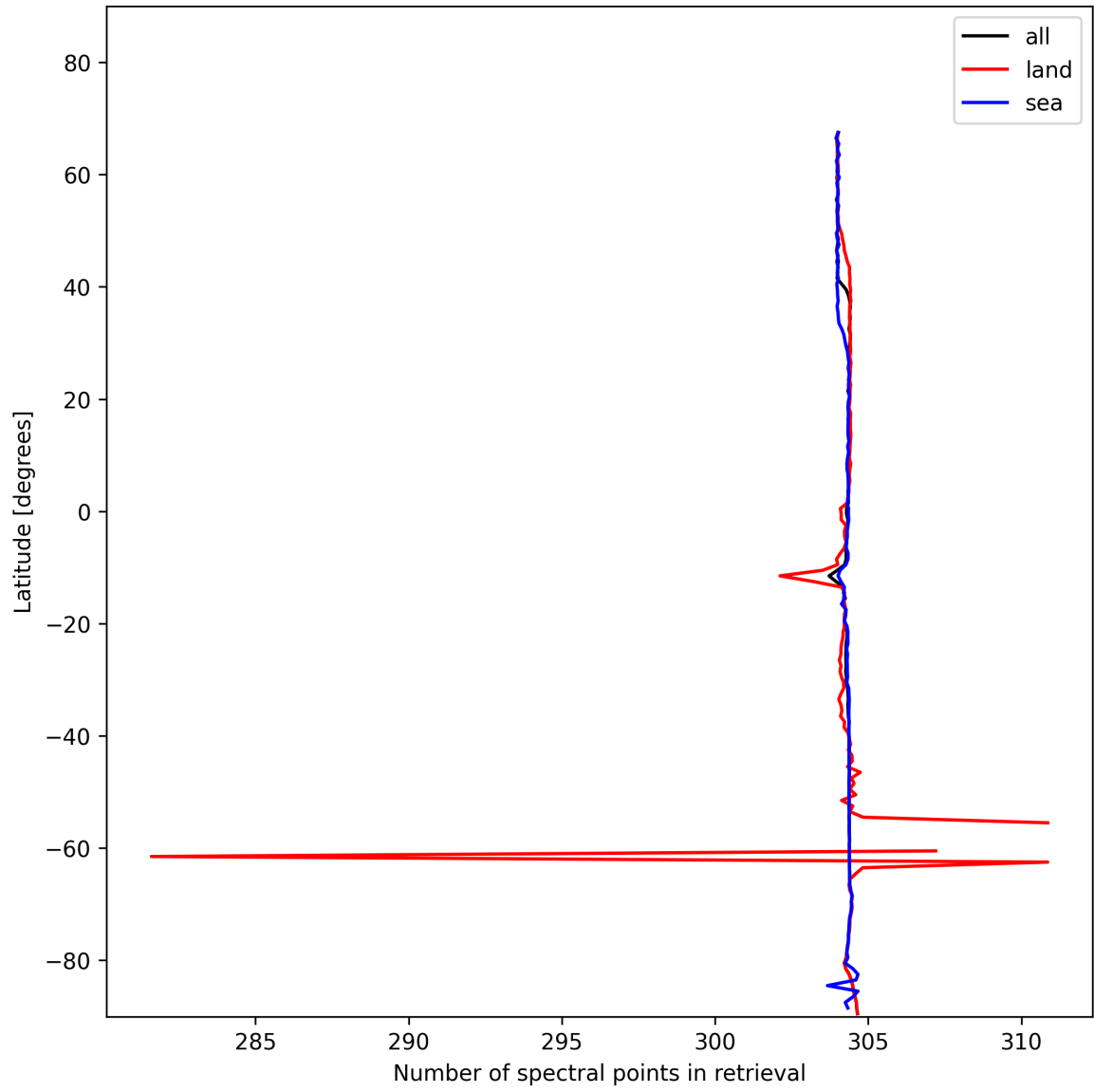
Figure 16: Zonal average of “Number of spectral points in retrieval” for 2025-11-21 to 2025-11-23.
