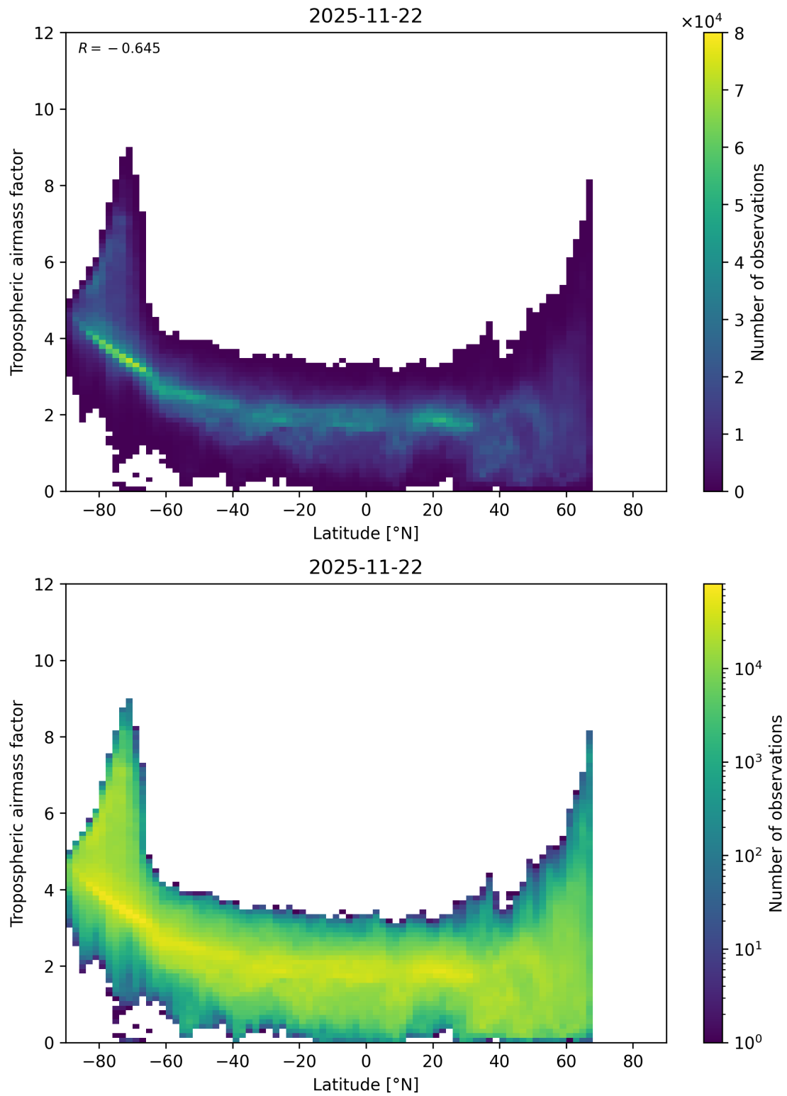
Figure 85: Scatter density plot of “Latitude” against “Tropospheric airmass factor” for 2025-11-21 to 2025-11-23.
