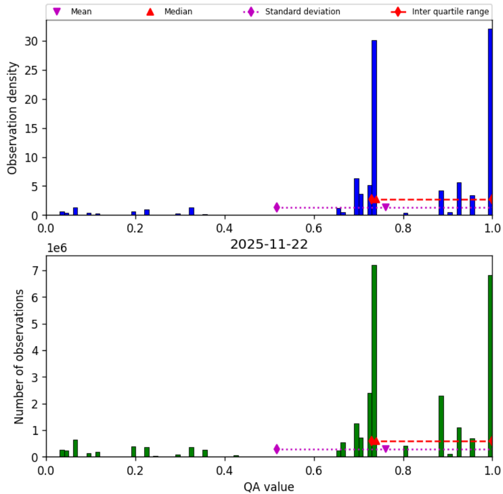
Figure 28: Histogram of “QA value” for 2025-11-21 to 2025-11-23
