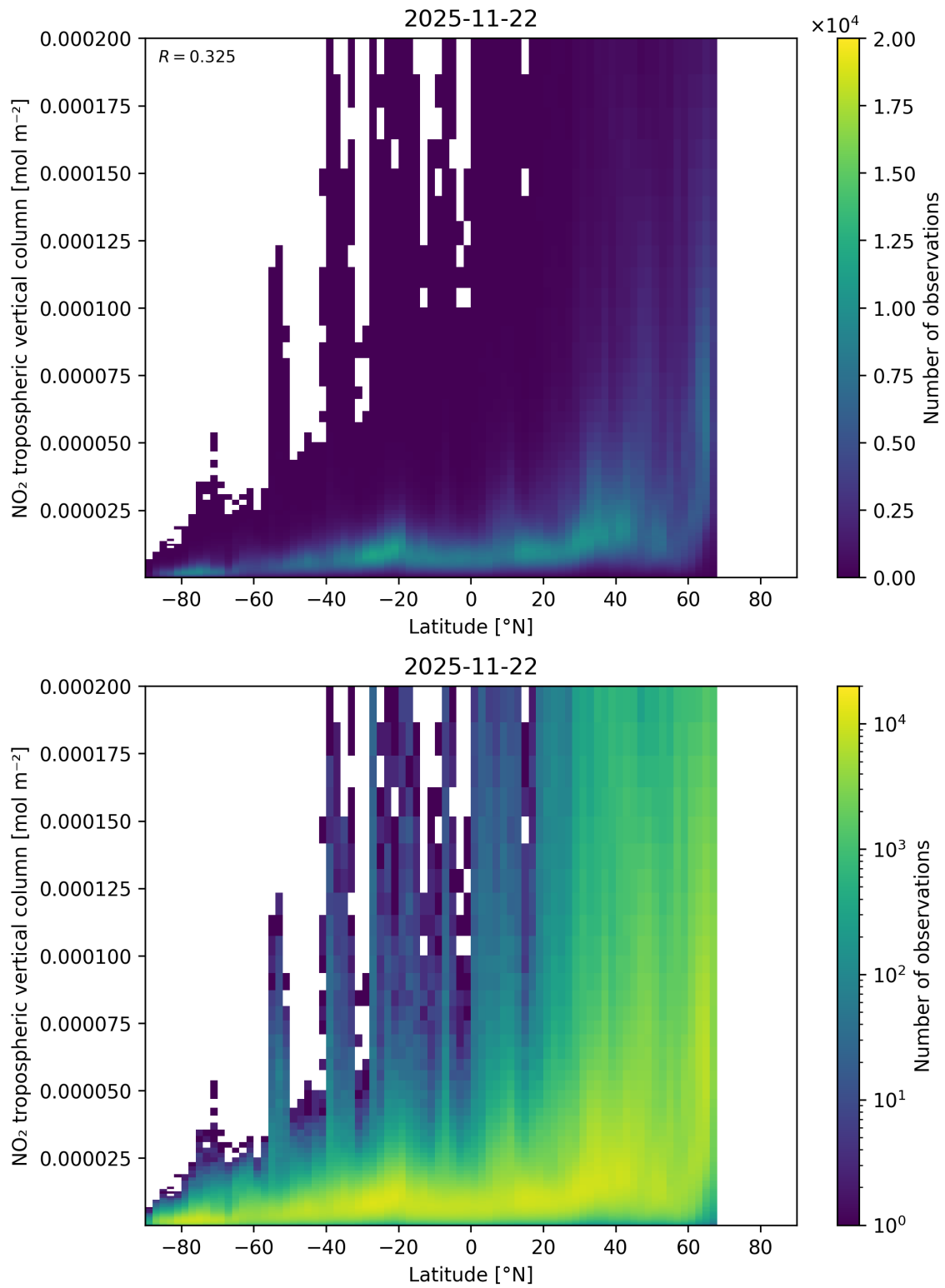
Figure 92: Scatter density plot of “Latitude” against “NO 2 tropospheric vertical column” for 2025-11-21 to 2025-11-23.
