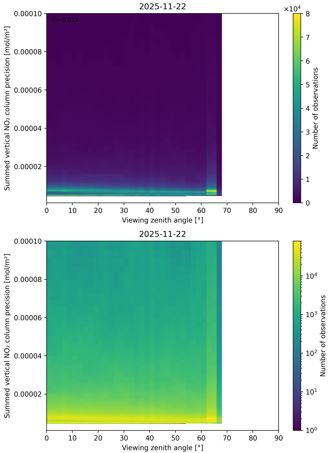
Figure 166: Scatter density plot of “Viewing zenith angle” against “Summed vertical NO 2 column precision” for 2025-11-21 to 2025-11-23.
