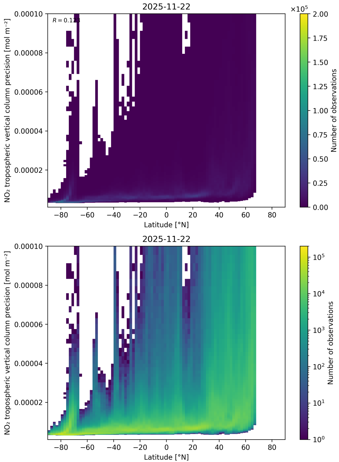
Figure 93: Scatter density plot of “Latitude” against “NO 2 tropospheric vertical column precision” for 2025-11-21 to 2025-11-23.
