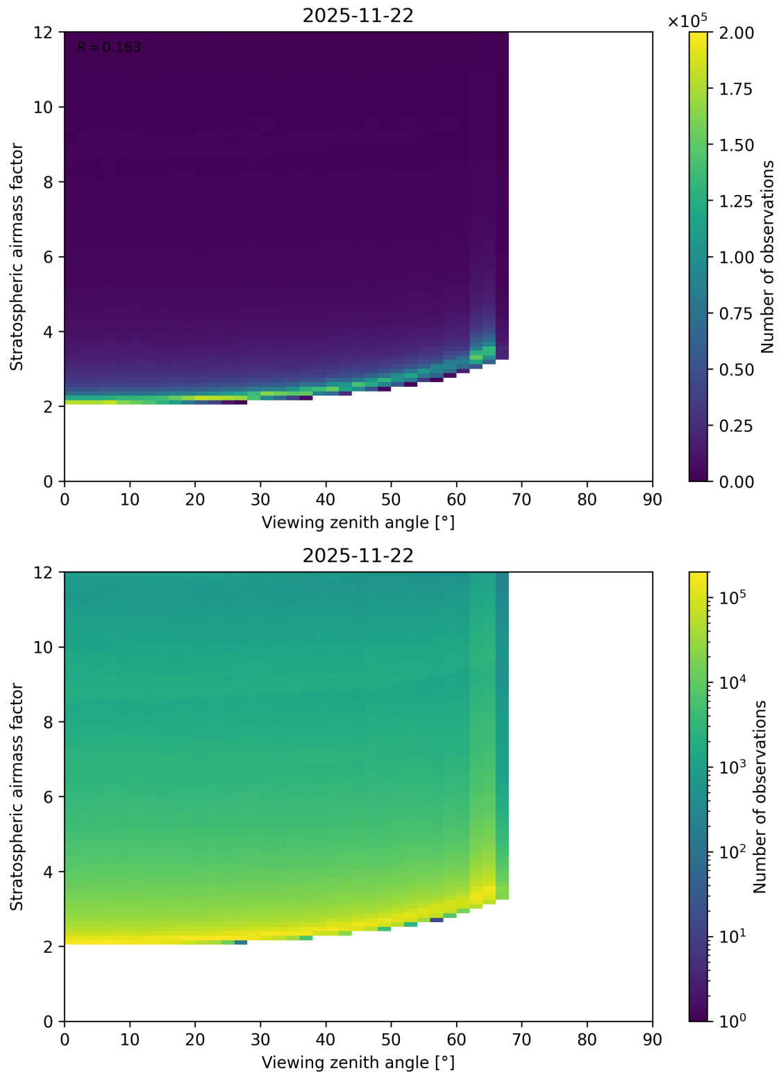
Figure 159: Scatter density plot of “Viewing zenith angle” against “Stratospheric airmass factor” for 2025-11-21 to 2025-11-23.
