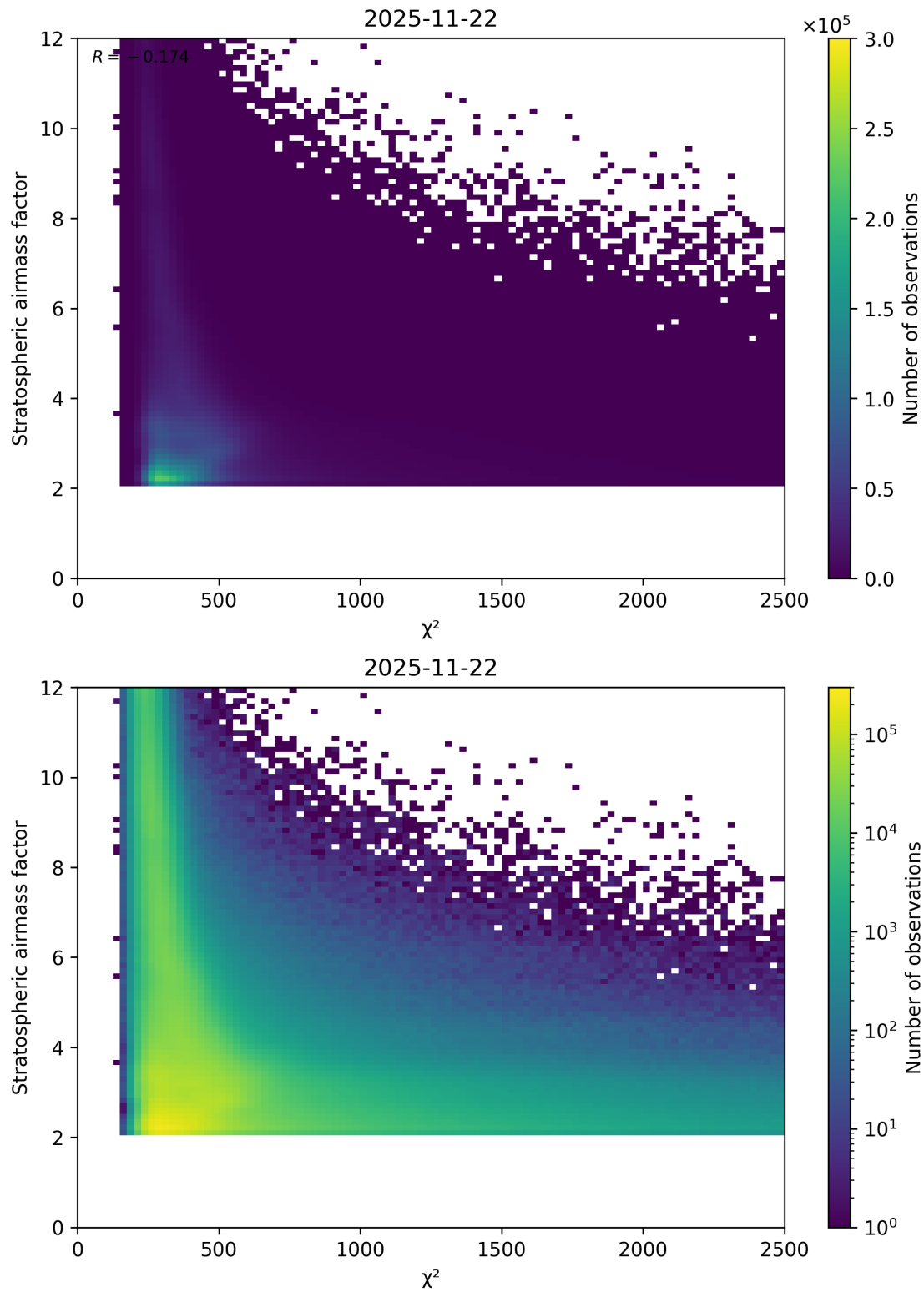
Figure 81: Scatter density plot of “ \chi^2 ” against “Stratospheric airmass factor” for 2025-11-21 to 2025-11-23.
