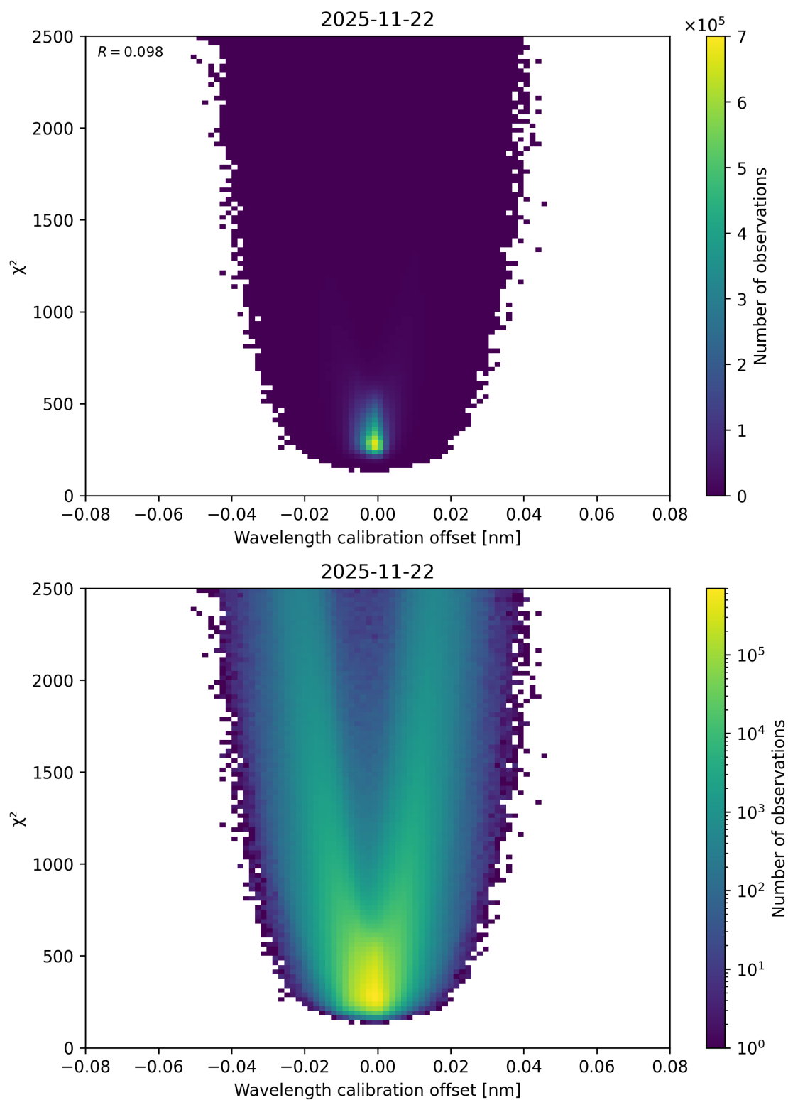
Figure 175: Scatter density plot of “Wavelength calibration offset” against “ \chi^2 ” for 2025-11-21 to 2025-11-23.
