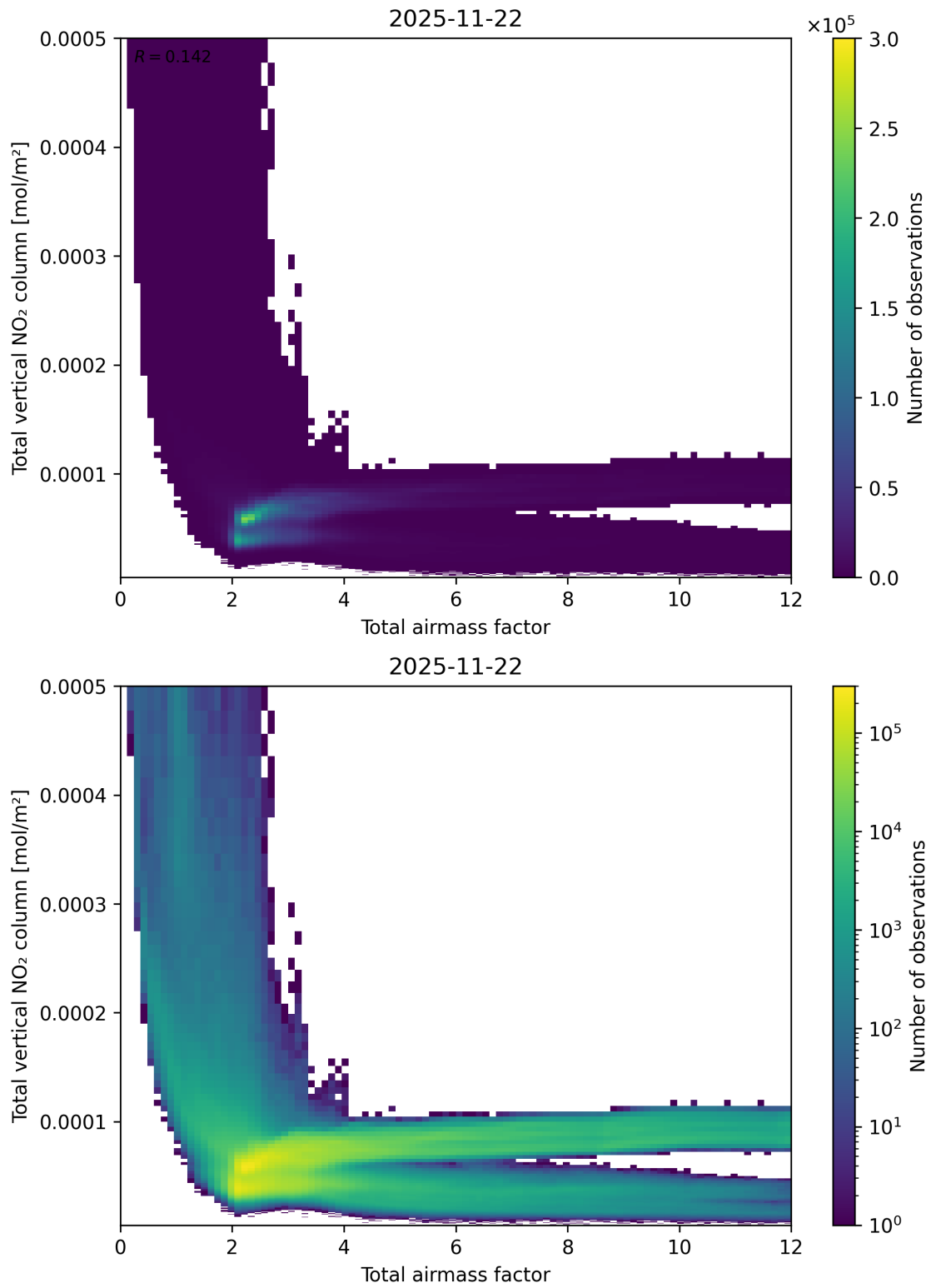
Figure 67: Scatter density plot of “Total airmass factor” against “Total vertical NO 2 column” for 2025-11-21 to 2025-11-23.
