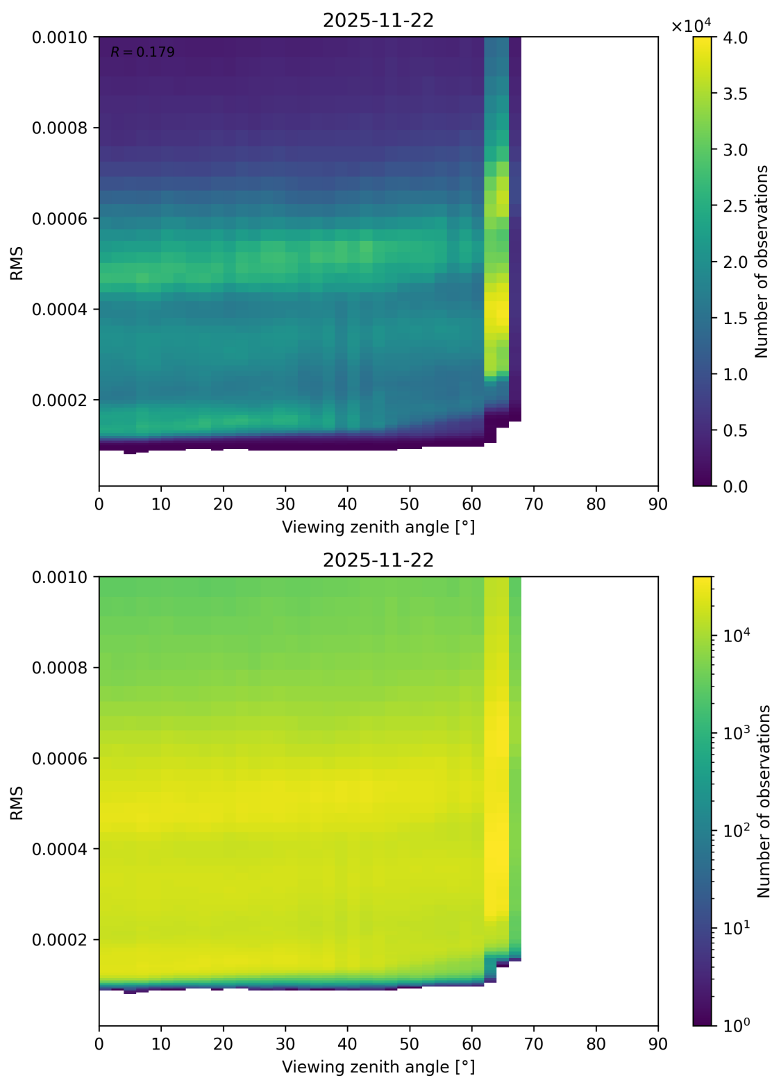
Figure 171: Scatter density plot of “Viewing zenith angle” against “RMS” for 2025-11-21 to 2025-11-23.
