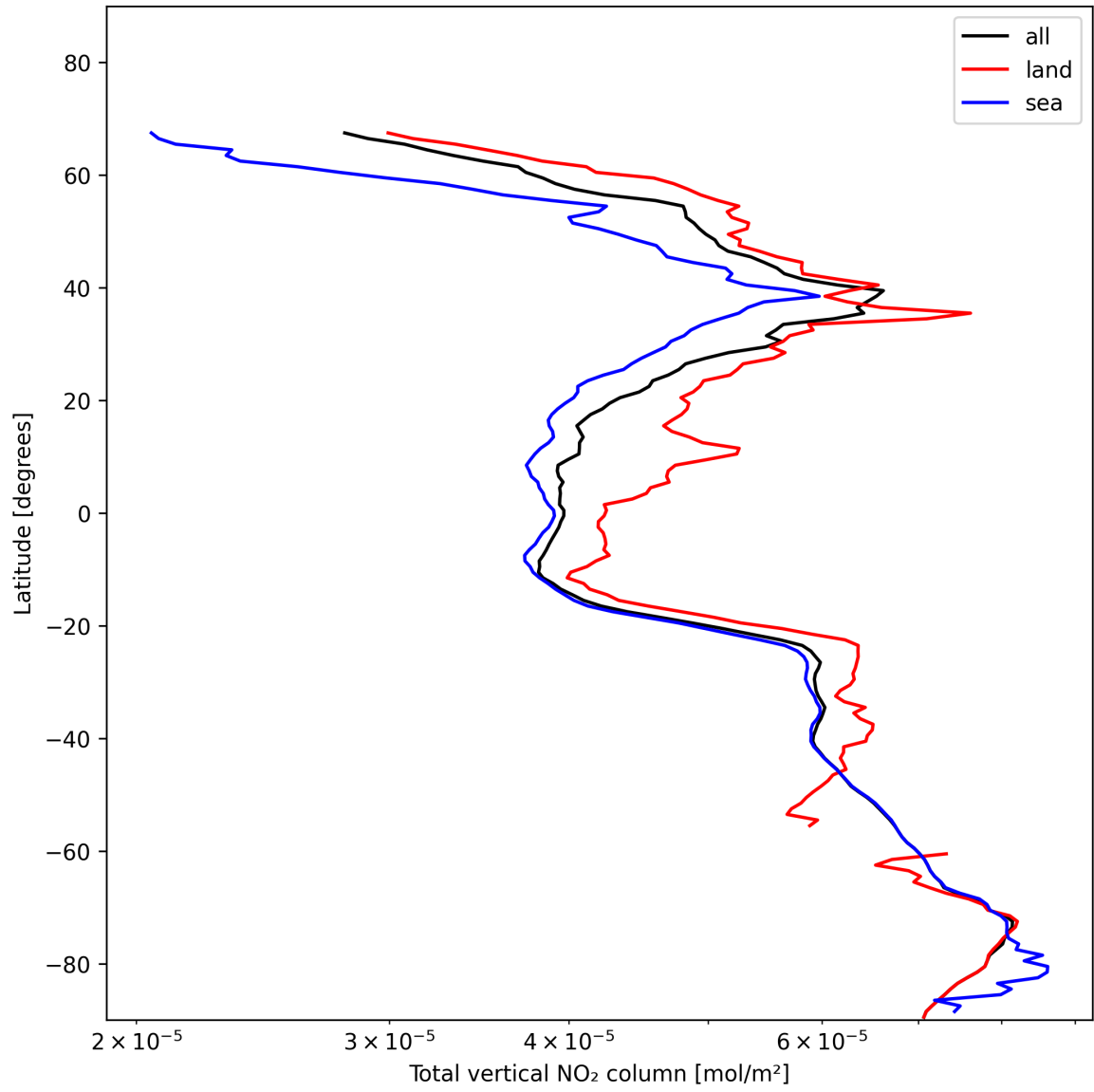
Figure 21: Zonal average of “Total vertical NO 2 column” for 2025-11-21 to 2025-11-23.
