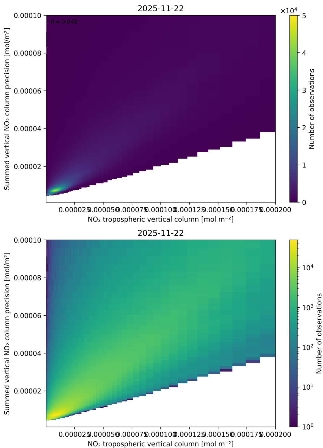
Figure 127: Scatter density plot of “NO 2 tropospheric vertical column” against “Summed vertical NO 2 column precision” for 2025-11-21 to 2025-11-23.
