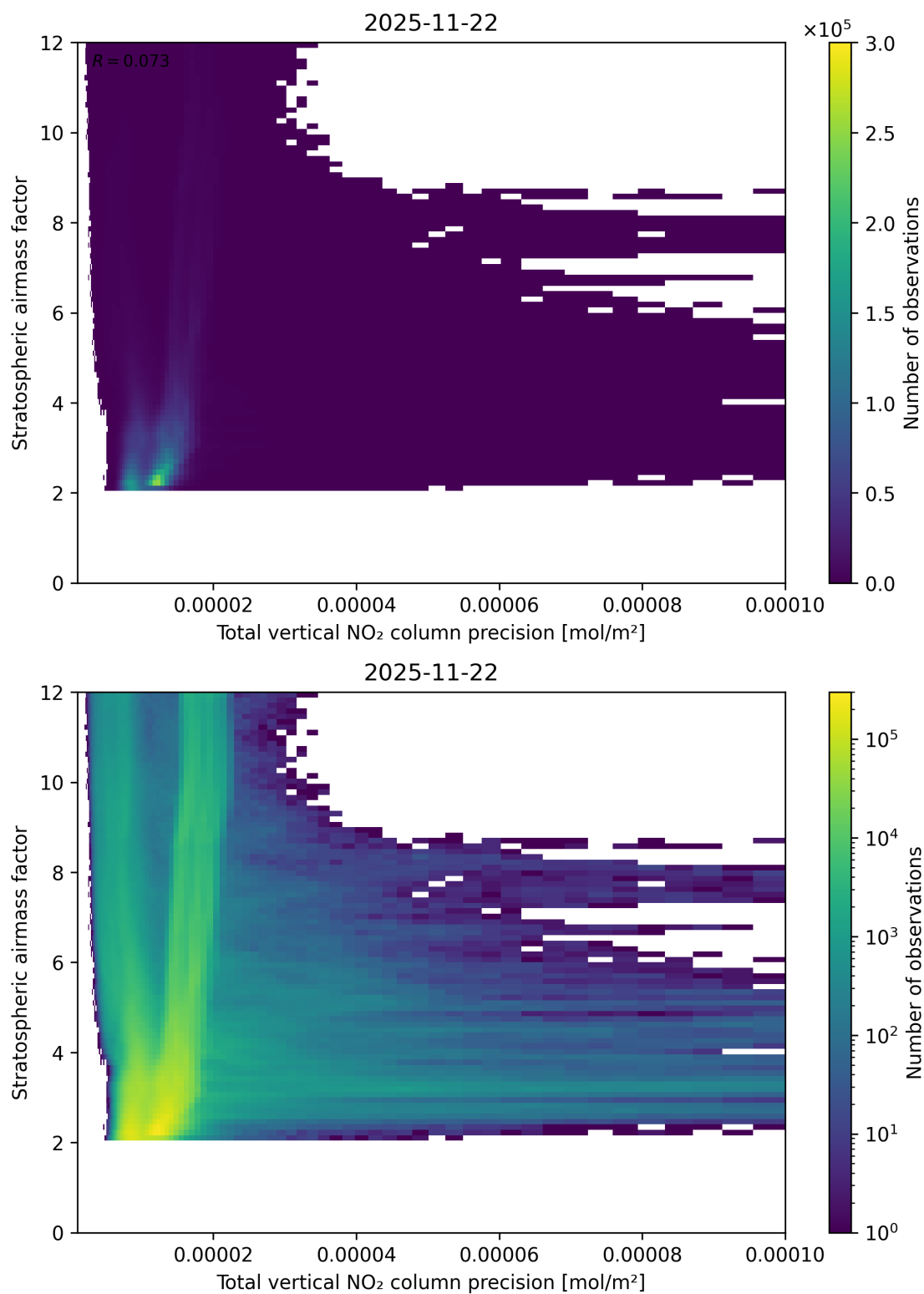
Figure 115: Scatter density plot of “Total vertical NO 2 column precision” against “Stratospheric air mass factor” for 2025-11-21 to 2025-11-23.
