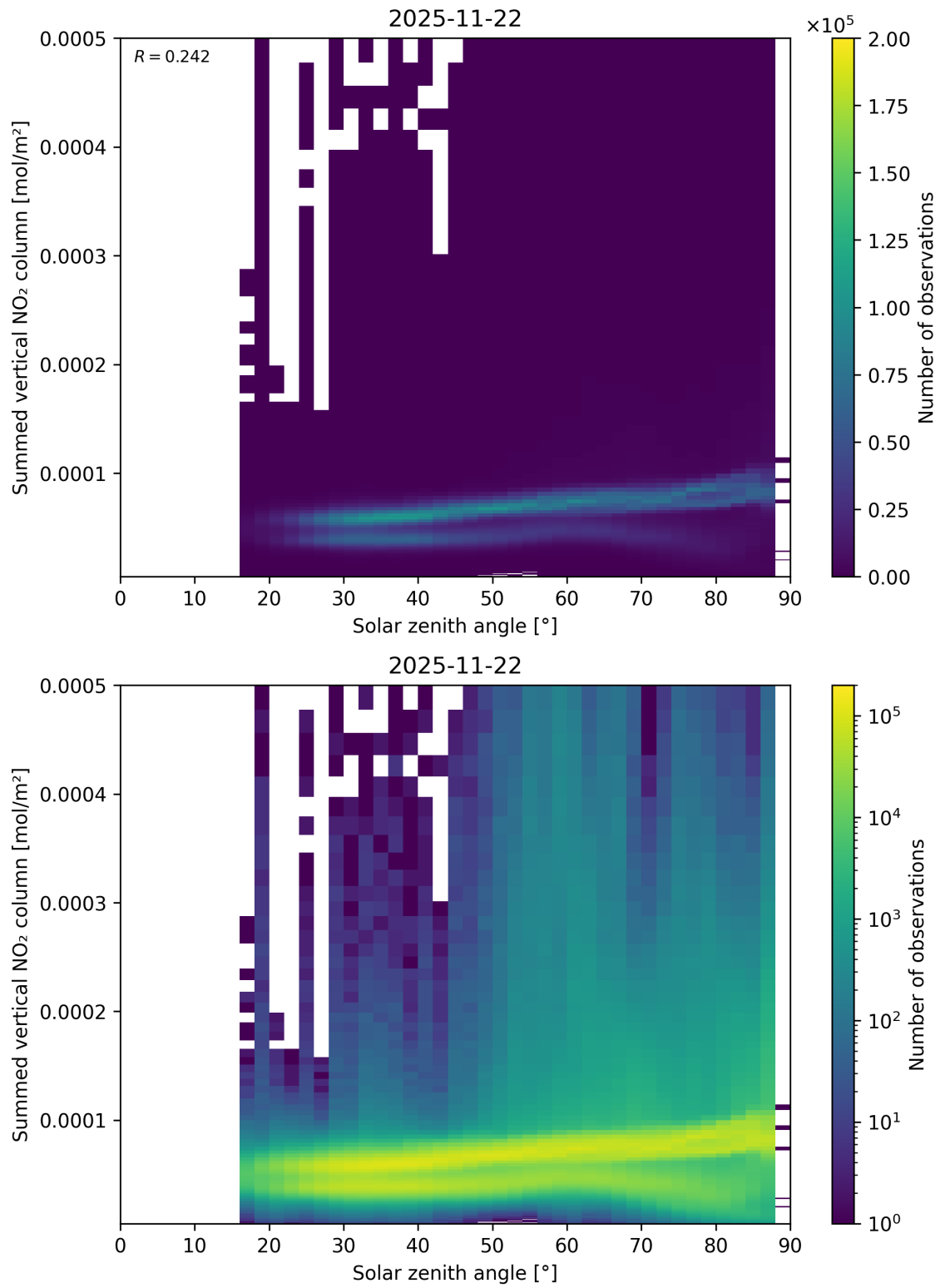
Figure 151: Scatter density plot of “Solar zenith angle” against “Summed vertical NO 2 column” for 2025-11-21 to 2025-11-23.
