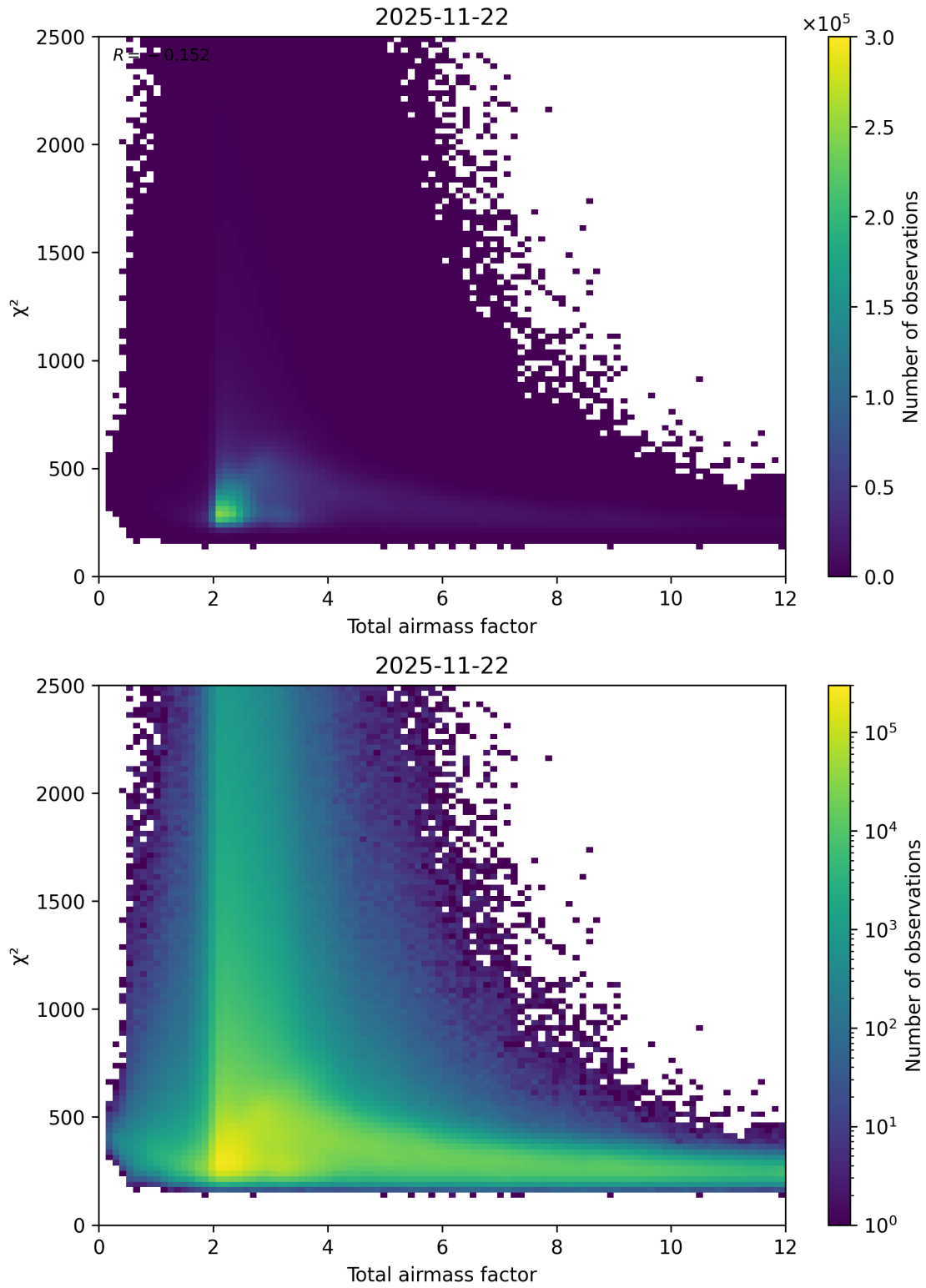
Figure 63: Scatter density plot of “Total airmass factor” against “ \chi^2 ” for 2025-11-21 to 2025-11-23.
