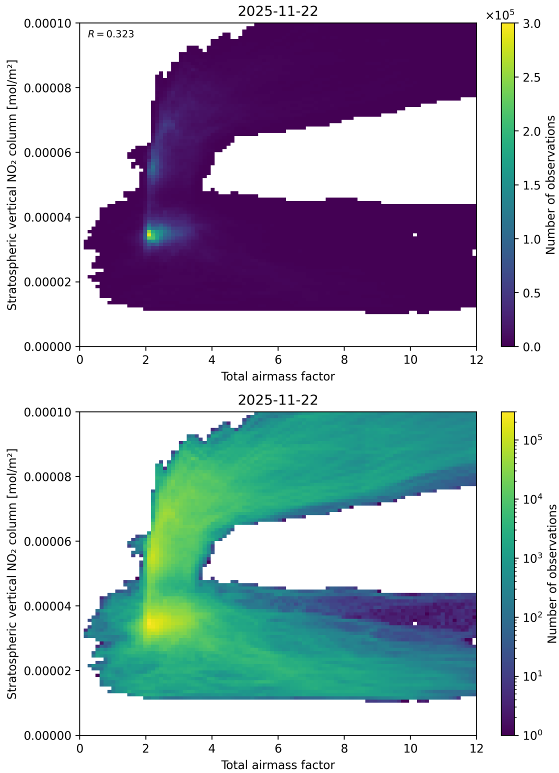
Figure 64: Scatter density plot of “Total airmass factor” against “Stratospheric vertical \text{NO}_2 column” for 2025-11-21 to 2025-11-23.
