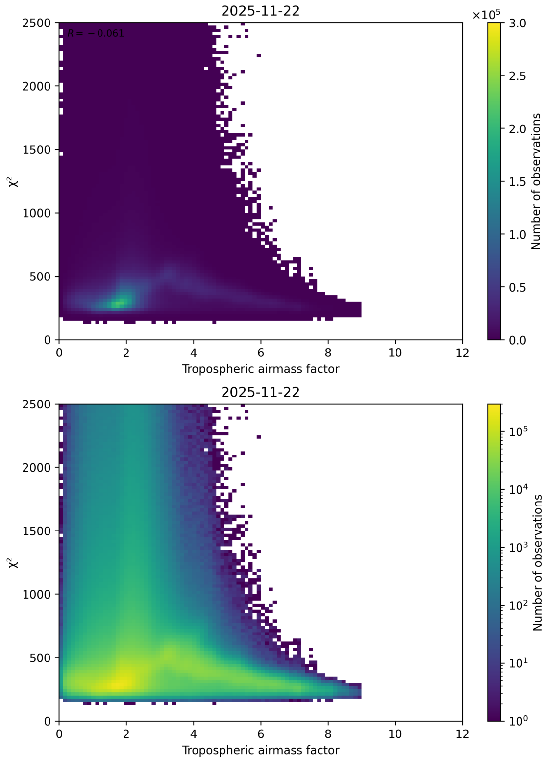
Figure 73: Scatter density plot of “Tropospheric airmass factor” against “ \chi^2 ” for 2025-11-21 to 2025-11-23.
