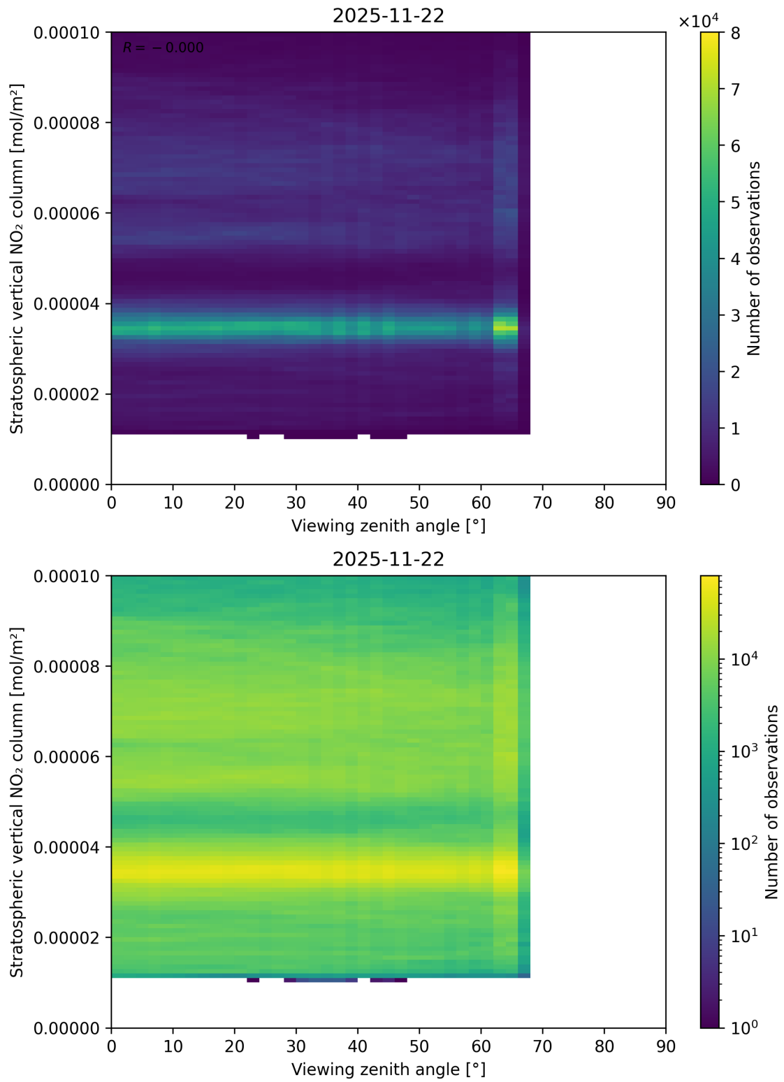
Figure 164: Scatter density plot of “Viewing zenith angle” against “Stratospheric vertical NO 2 column” for 2025-11-21 to 2025-11-23.
