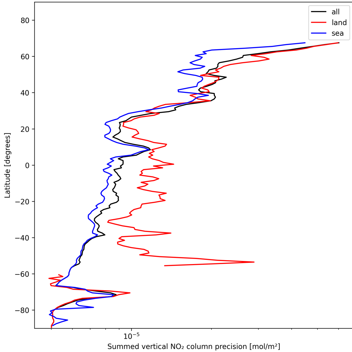
Figure 24: Zonal average of “Summed vertical NO 2 column precision” for 2025-11-21 to 2025-11-23.
