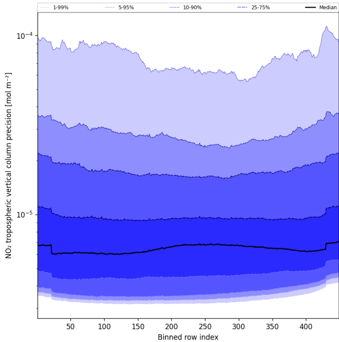
Figure 47: Along track statistics of “NO 2 tropospheric vertical column precision” for 2025-11-21 to 2025-11-23
