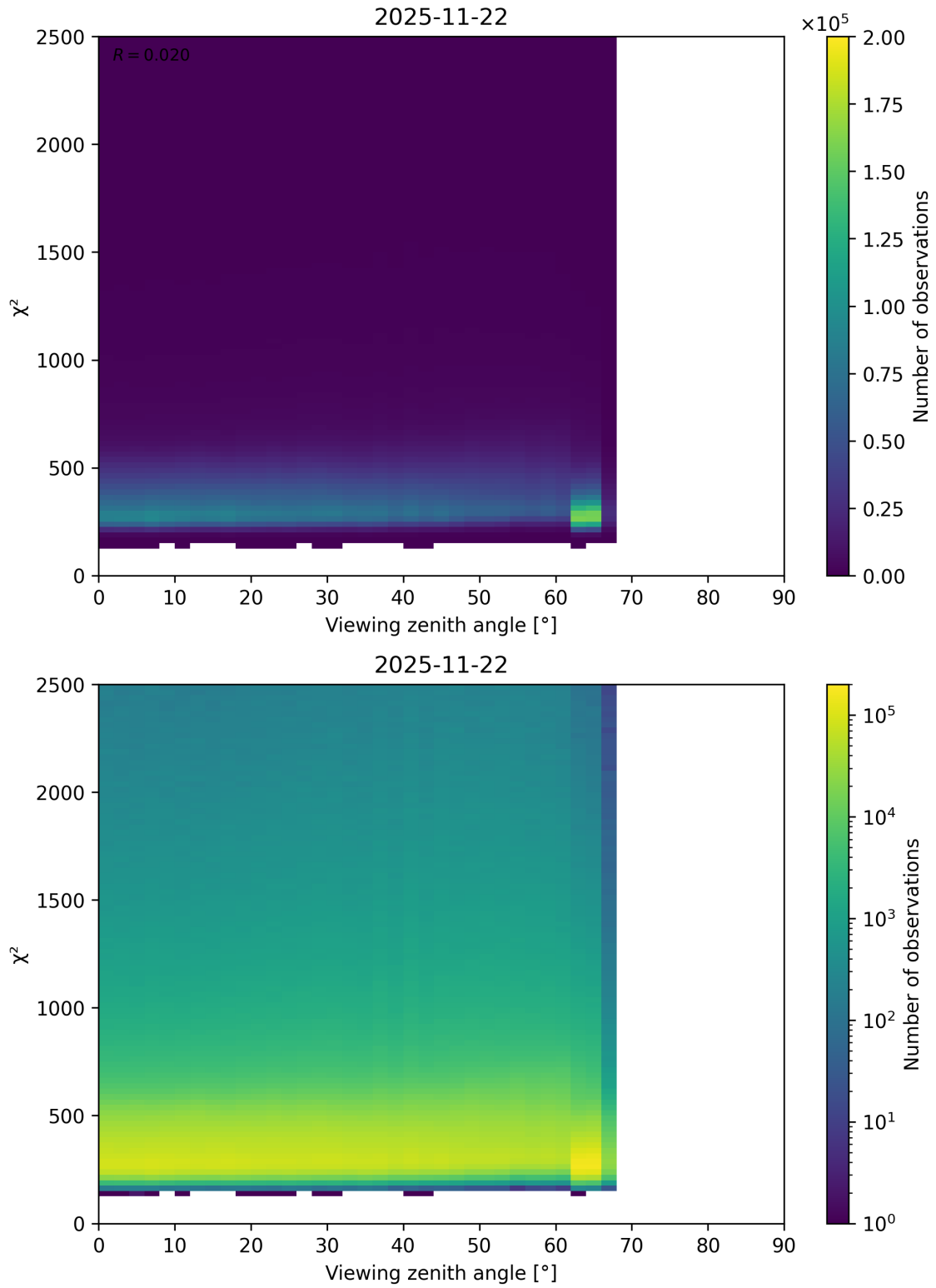
Figure 162: Scatter density plot of “Viewing zenith angle” against “ \chi^2 ” for 2025-11-21 to 2025-11-23.
