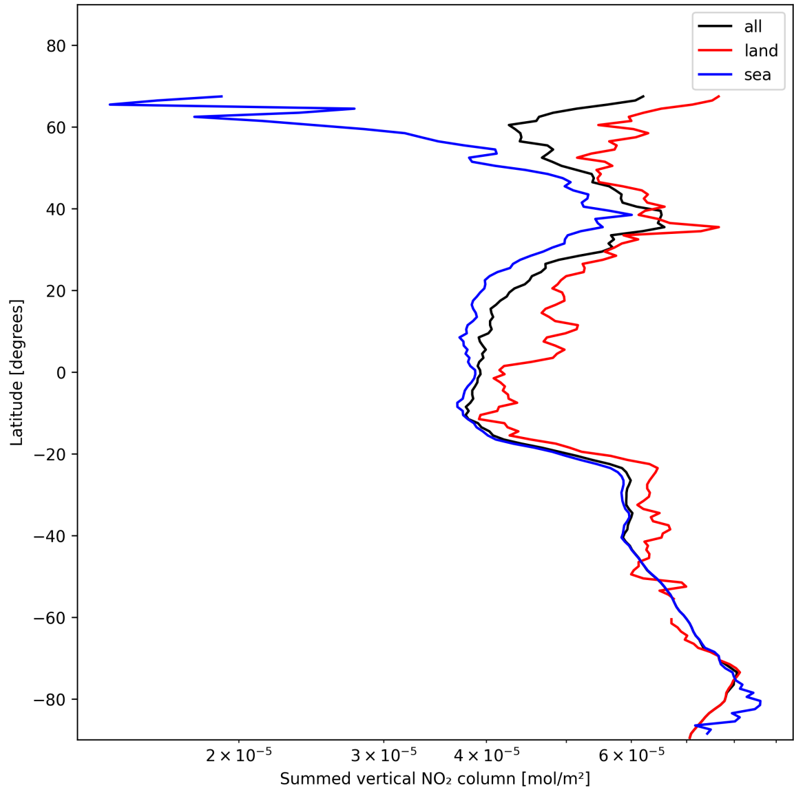
Figure 23: Zonal average of “Summed vertical NO 2 column” for 2025-11-21 to 2025-11-23.
