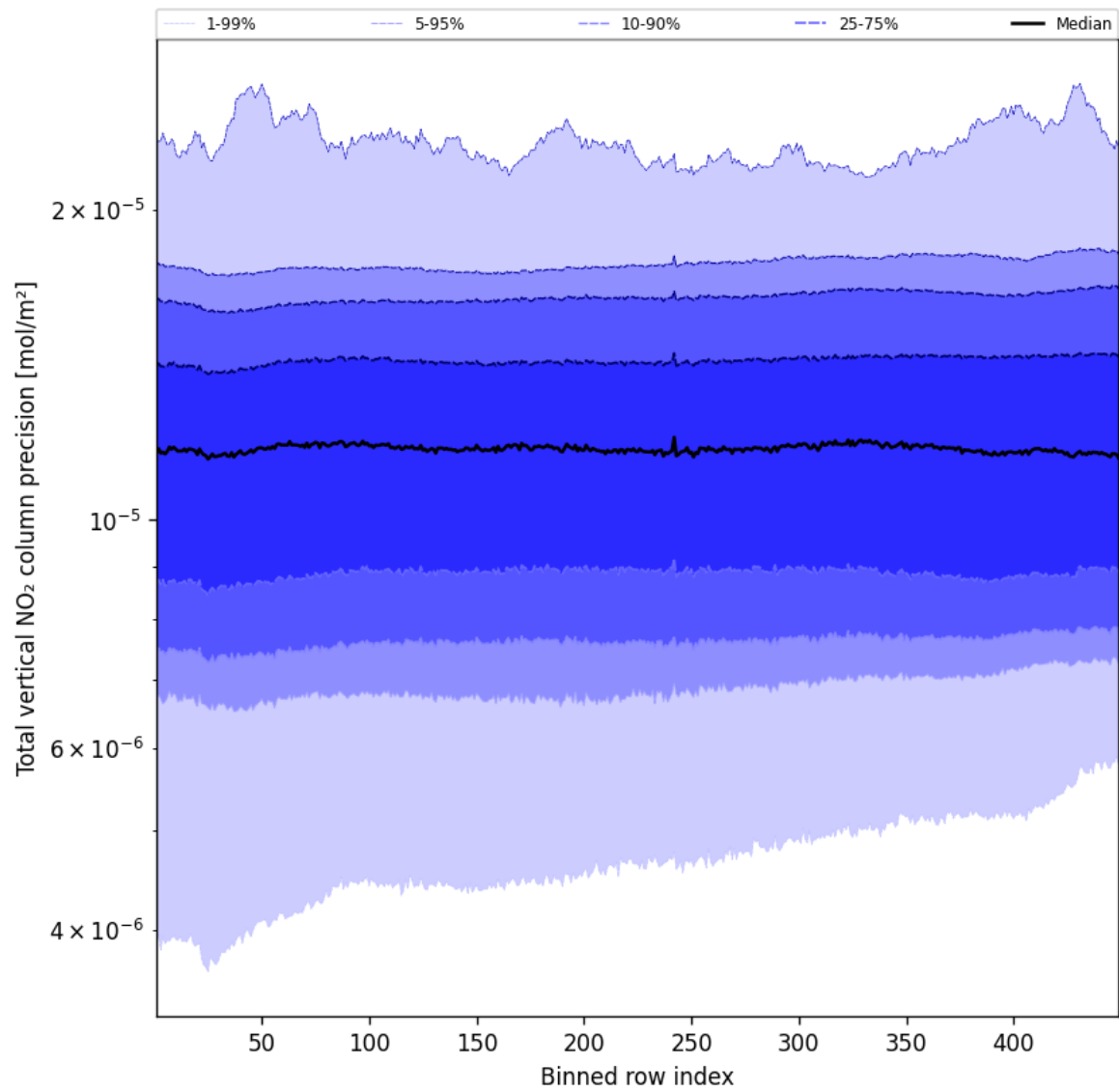
Figure 56: Along track statistics of “Total vertical NO 2 column precision” for 2025-11-21 to 2025-11-23
