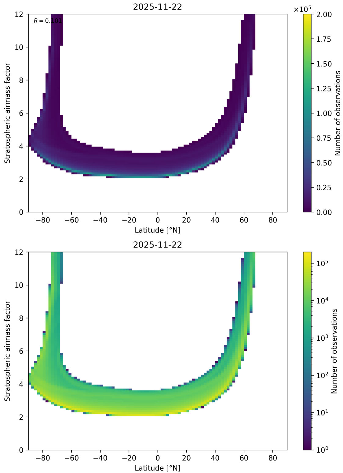
Figure 83: Scatter density plot of “Latitude” against “Stratospheric air mass factor” for 2025-11-21 to 2025-11-23.
