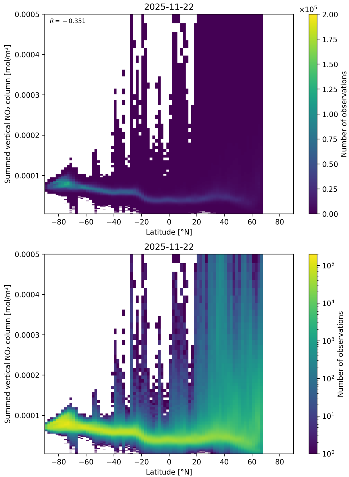
Figure 88: Scatter density plot of “Latitude” against “Summed vertical NO 2 column” for 2025-11-21 to 2025-11-23.
