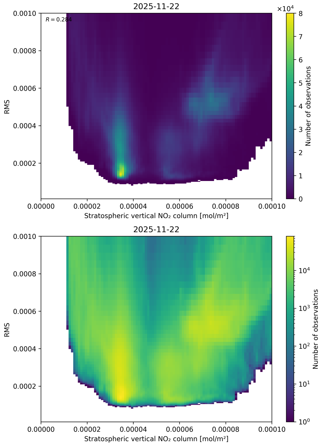
Figure 102: Scatter density plot of “Stratospheric vertical NO 2 column” against “RMS” for 2025-11-21 to 2025-11-23.
