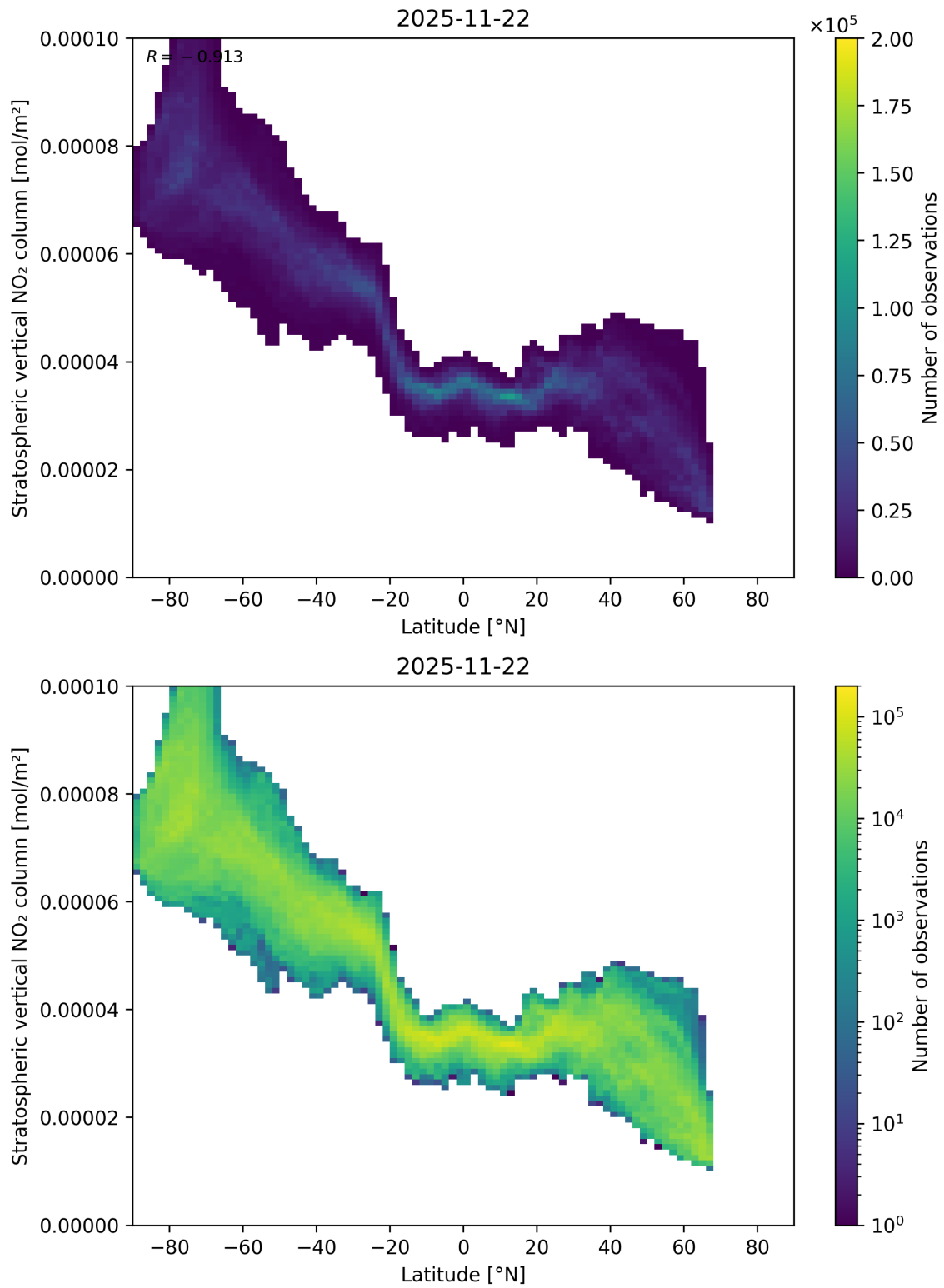
Figure 87: Scatter density plot of “Latitude” against “Stratospheric vertical NO 2 column” for 2025-11-21 to 2025-11-23.
