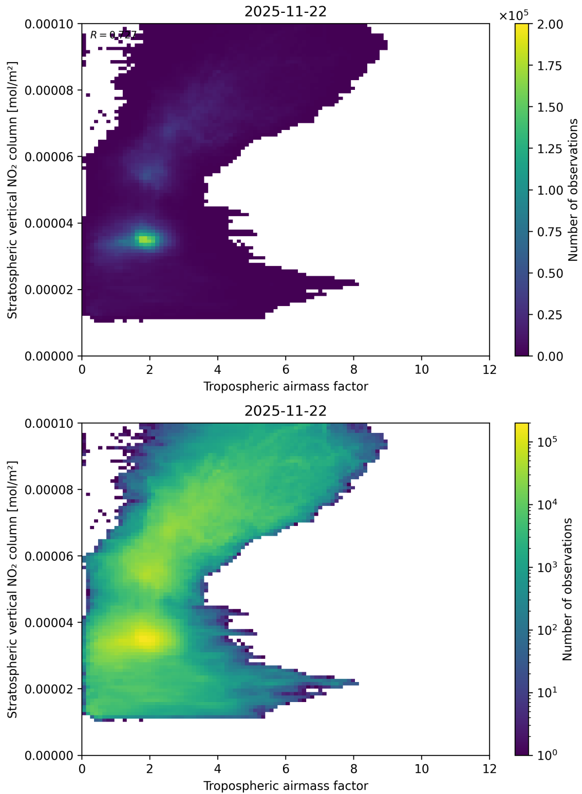
Figure 74: Scatter density plot of “Tropospheric airmass factor” against “Stratospheric vertical NO 2 column” for 2025-11-21 to 2025-11-23.
