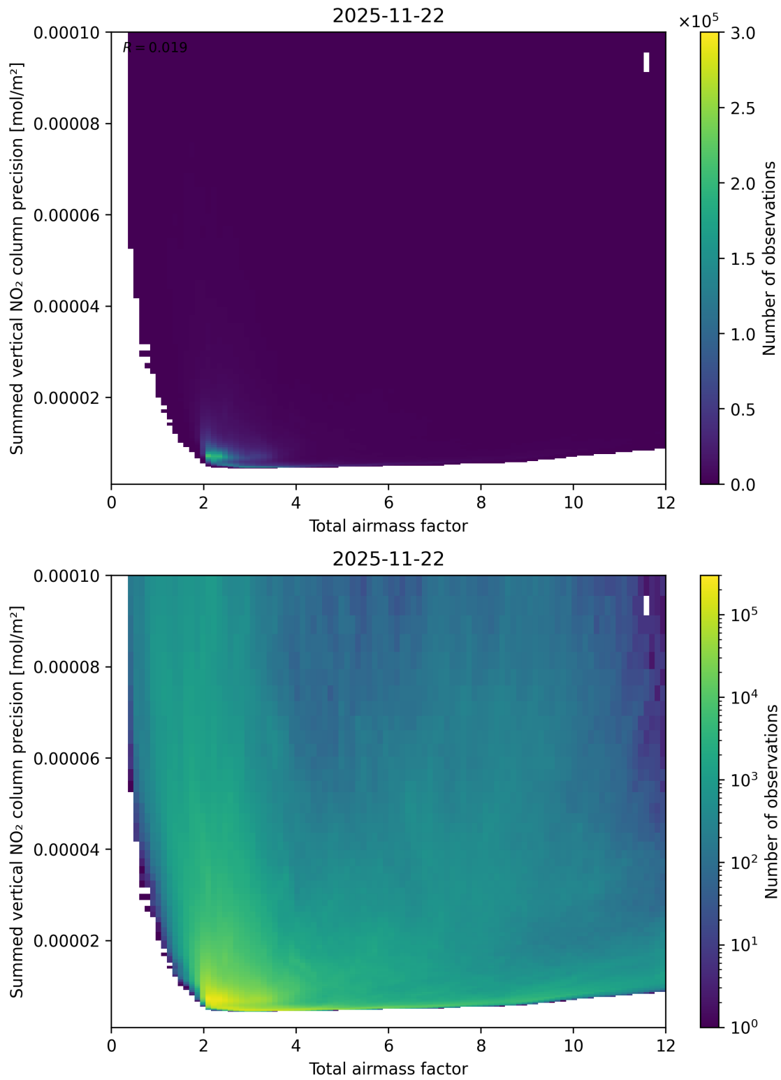
Figure 66: Scatter density plot of “Total airmass factor” against “Summed vertical NO 2 column precision” for 2025-11-21 to 2025-11-23.
