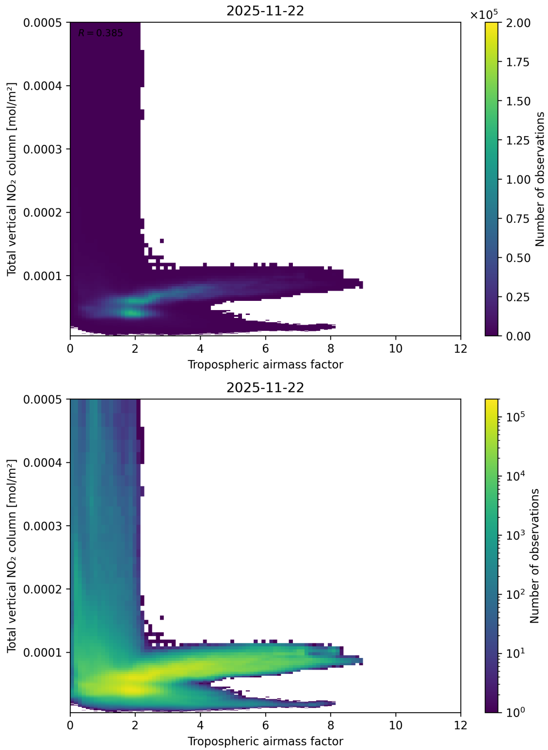
Figure 77: Scatter density plot of “Tropospheric airmass factor” against “Total vertical NO 2 column” for 2025-11-21 to 2025-11-23.
