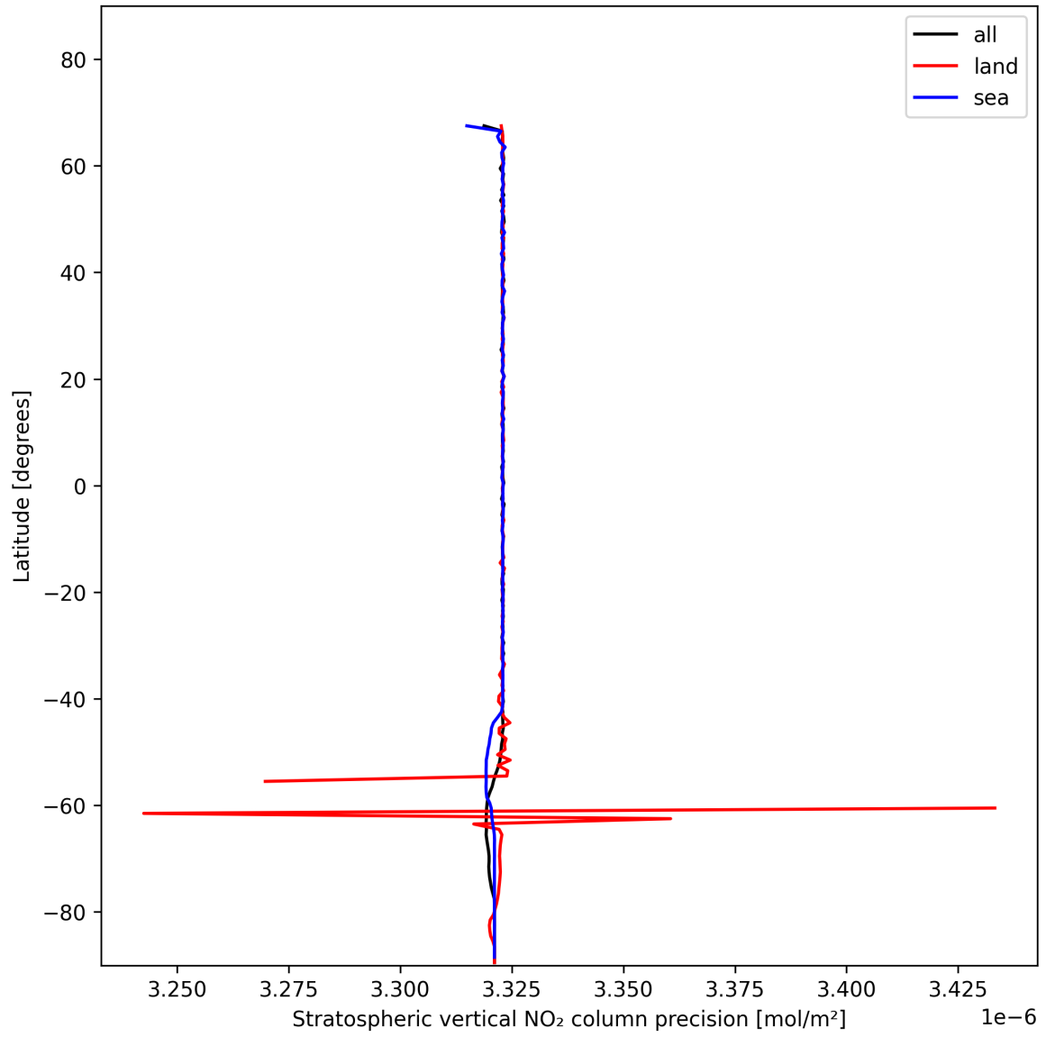
Figure 20: Zonal average of “Stratospheric vertical NO 2 column precision” for 2025-11-21 to 2025-11-23.
