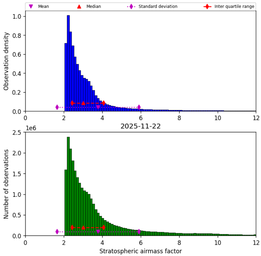
Figure 44: Histogram of “Stratospheric airmass factor” for 2025-11-21 to 2025-11-23
