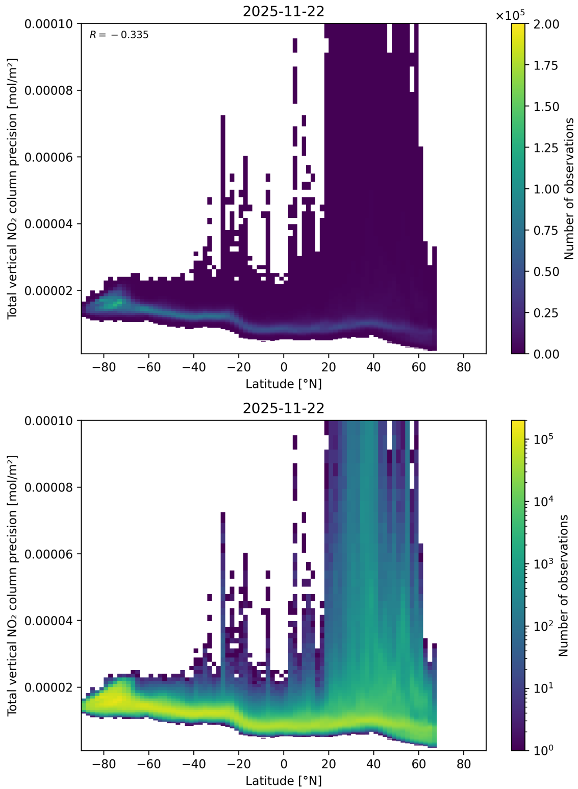
Figure 91: Scatter density plot of “Latitude” against “Total vertical NO 2 column precision” for 2025-11-21 to 2025-11-23.
