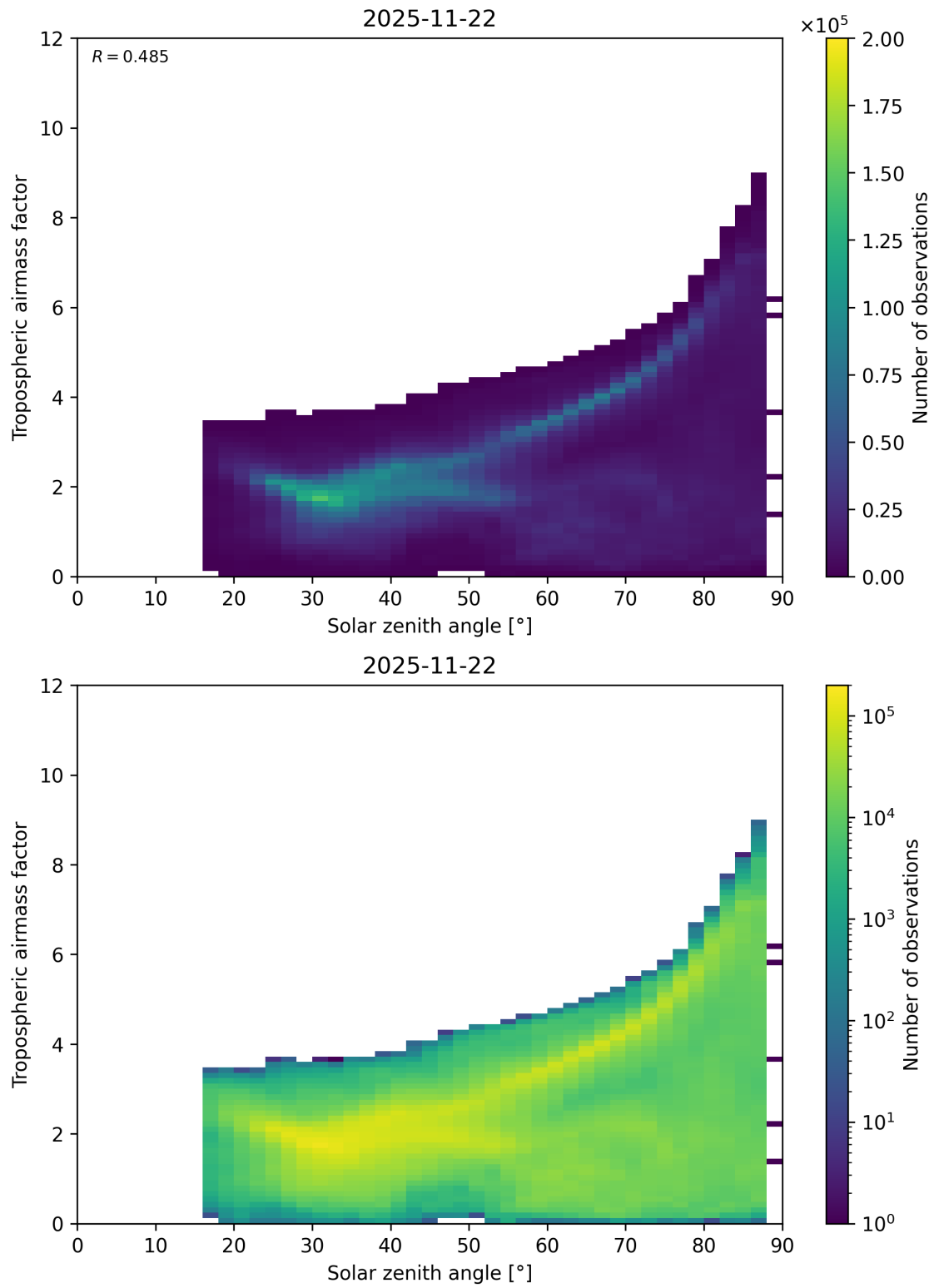
Figure 147: Scatter density plot of “Solar zenith angle” against “Tropospheric airmass factor” for 2025-11-21 to 2025-11-23.
