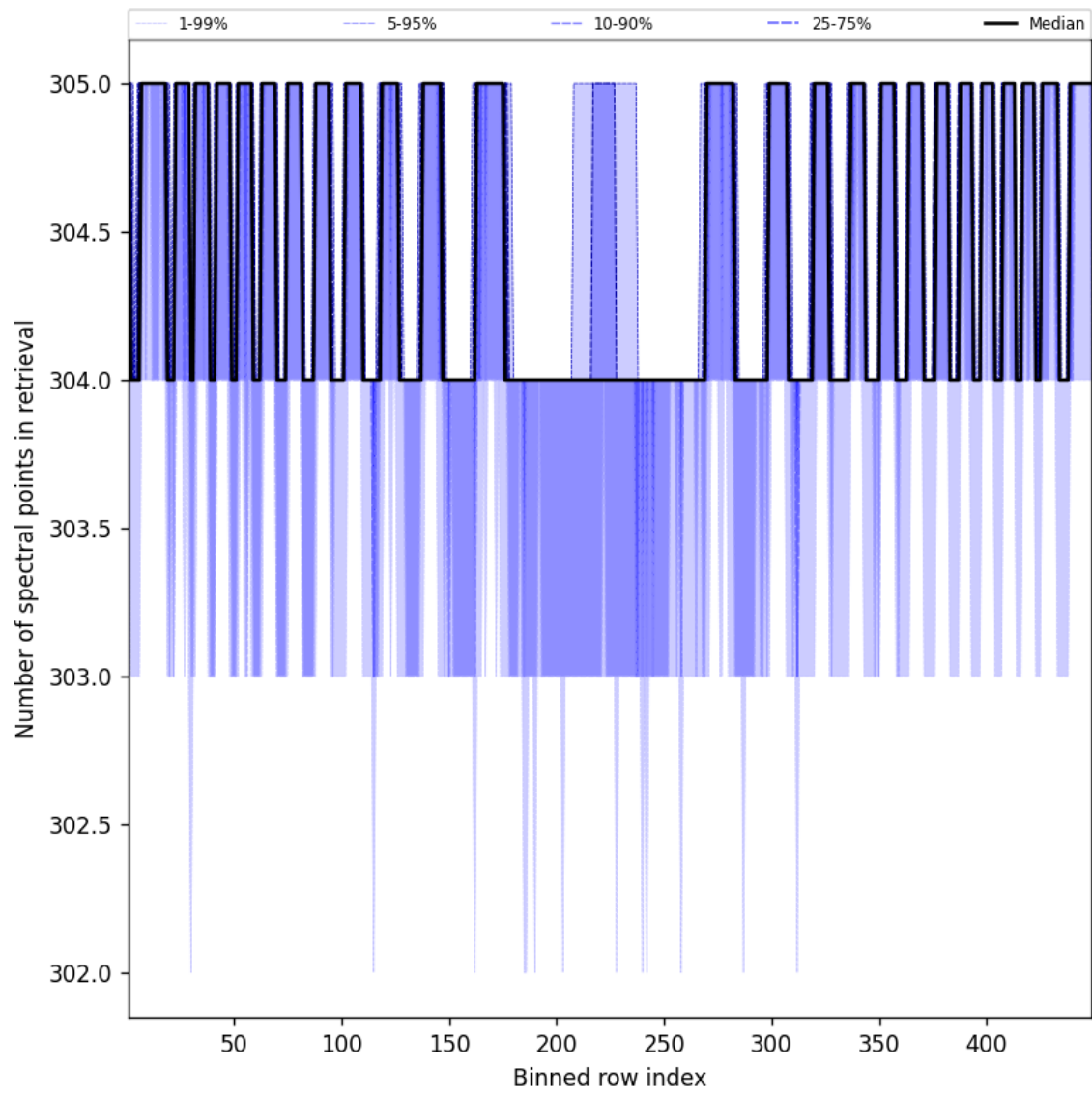
Figure 50: Along track statistics of “Number of spectral points in retrieval” for 2025-11-21 to 2025-11-23
