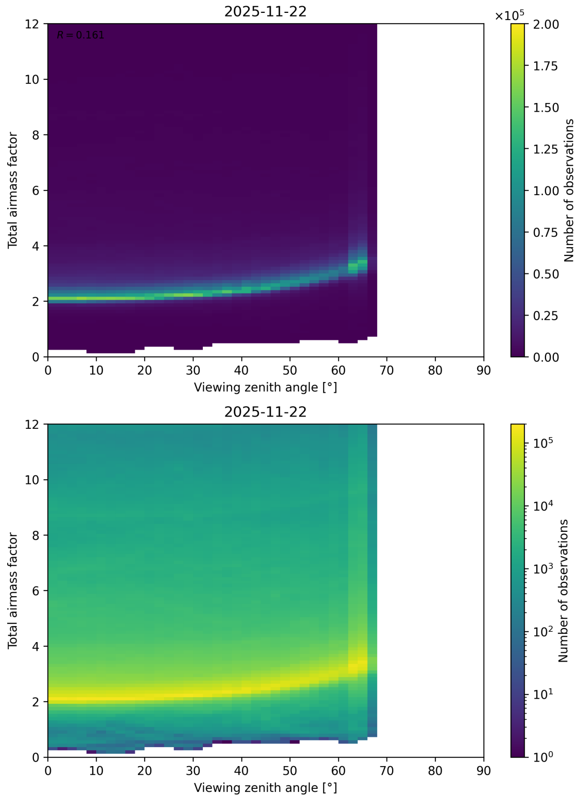
Figure 160: Scatter density plot of “Viewing zenith angle” against “Total airmass factor” for 2025-11-21 to 2025-11-23.
