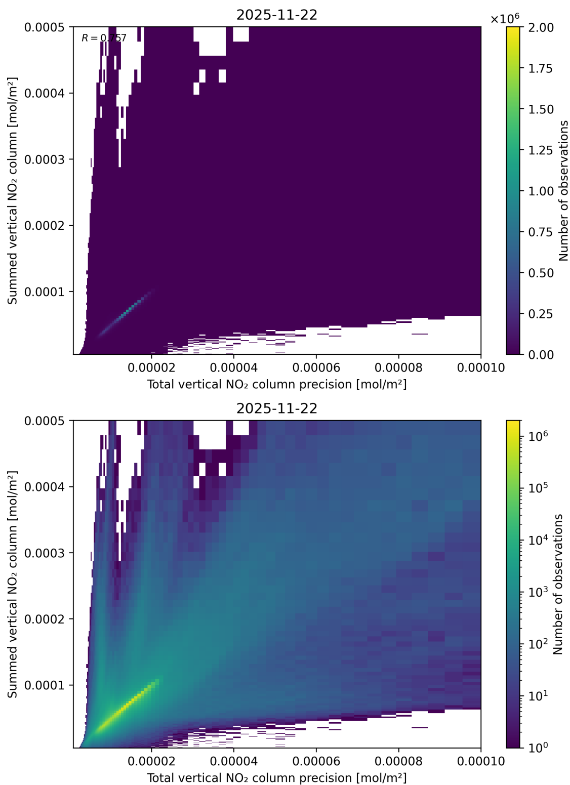
Figure 117: Scatter density plot of “Total vertical NO 2 column precision” against “Summed vertical NO 2 column” for 2025-11-21 to 2025-11-23.
