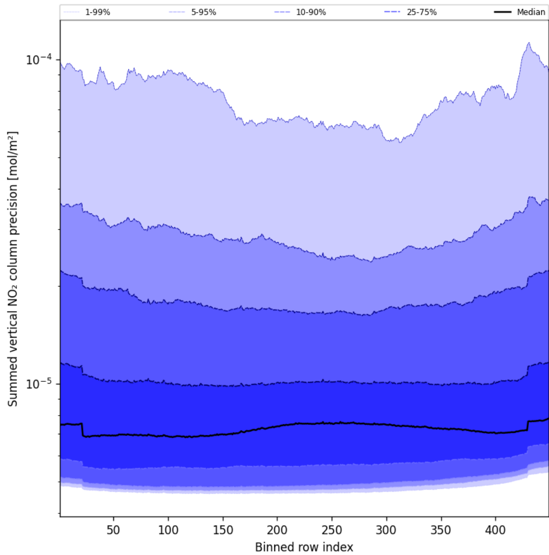
Figure 58: Along track statistics of “Summed vertical NO 2 column precision” for 2025-11-21 to 2025-11-23
