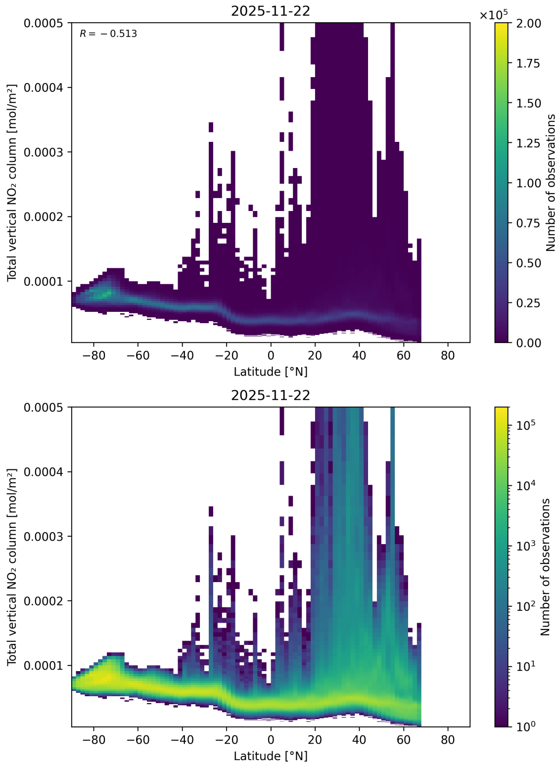
Figure 90: Scatter density plot of “Latitude” against “Total vertical NO 2 column” for 2025-11-21 to 2025-11-23.
