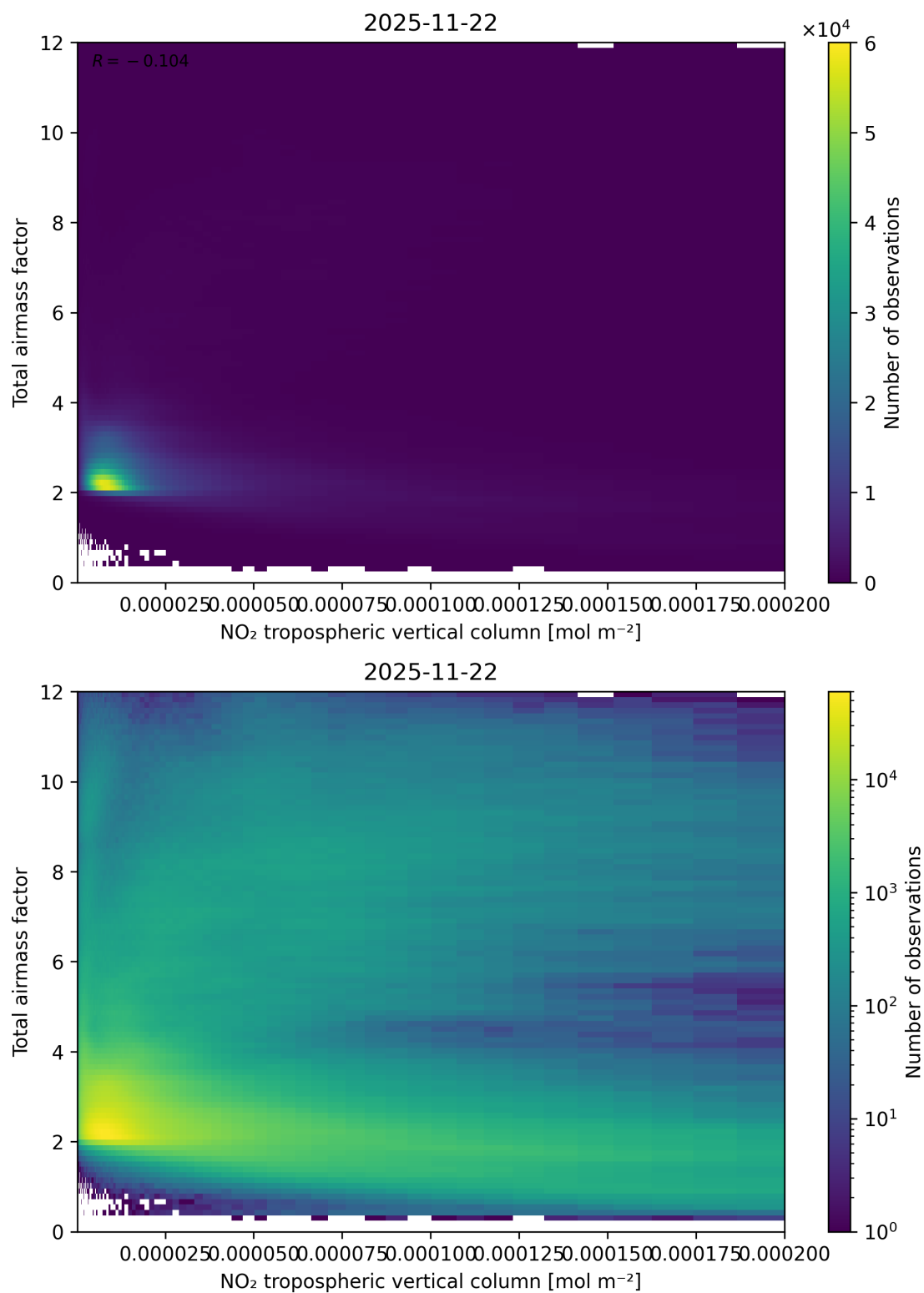
Figure 122: Scatter density plot of “NO 2 tropospheric vertical column” against “Total air mass factor” for 2025-11-21 to 2025-11-23.
