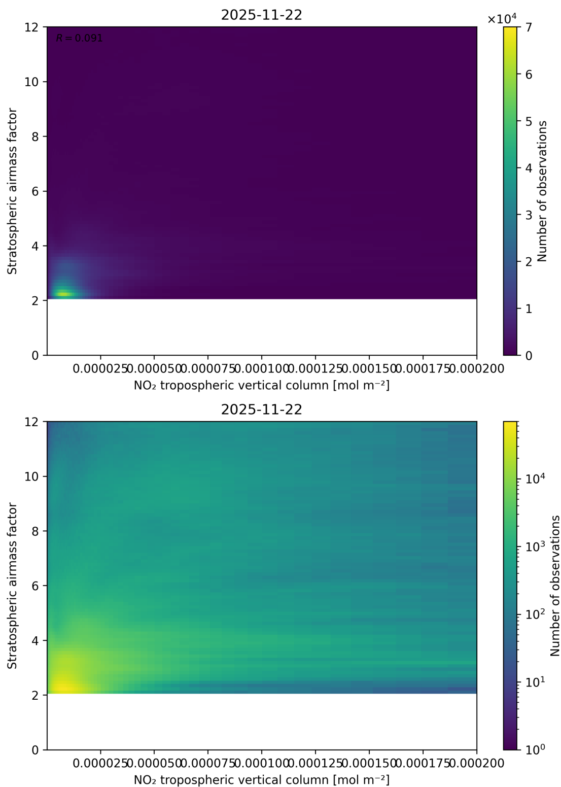
Figure 121: Scatter density plot of “NO 2 tropospheric vertical column” against “Stratospheric airmass factor” for 2025-11-21 to 2025-11-23.
