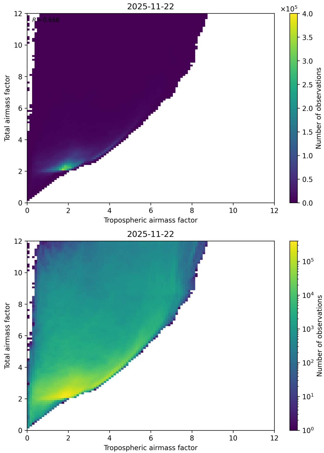
Figure 72: Scatter density plot of “Tropospheric airmass factor” against “Total airmass factor” for 2025-11-21 to 2025-11-23.
