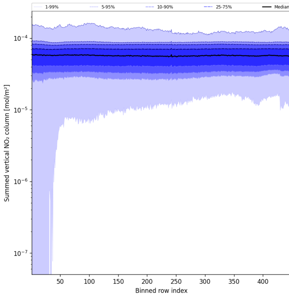
Figure 57: Along track statistics of “Summed vertical NO 2 column” for 2025-11-21 to 2025-11-23
