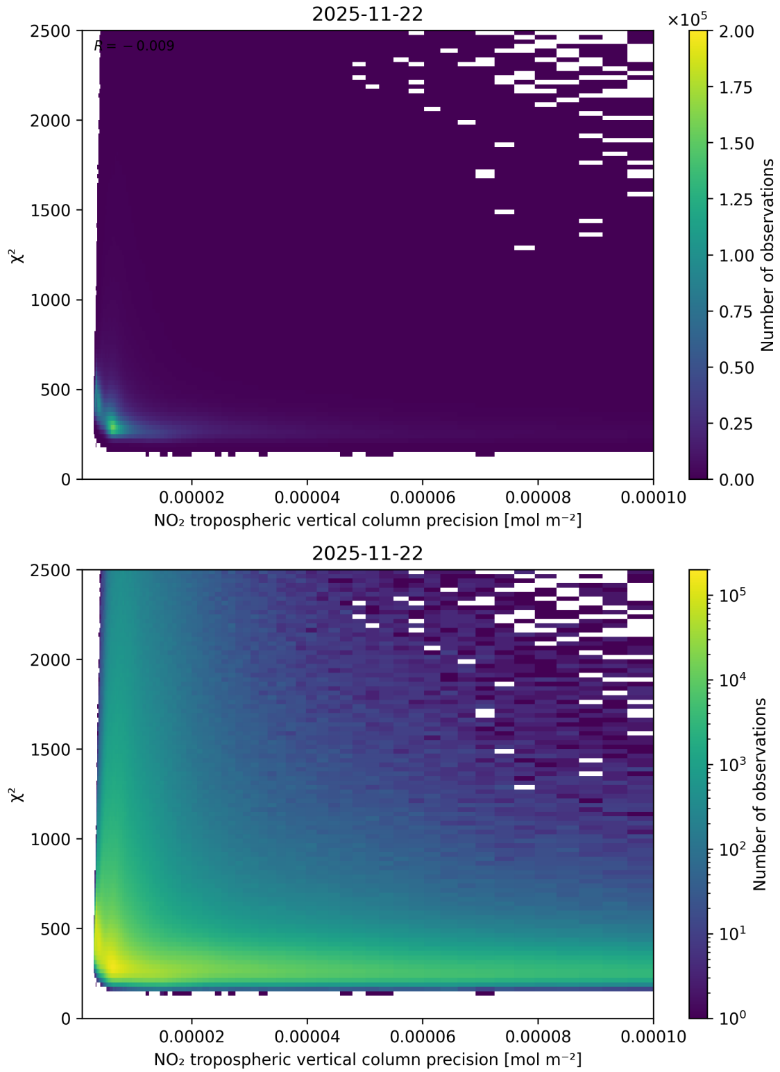
Figure 134: Scatter density plot of “NO 2 tropospheric vertical column precision” against “ \chi^2 ” for 2025-11-21 to 2025-11-23.
