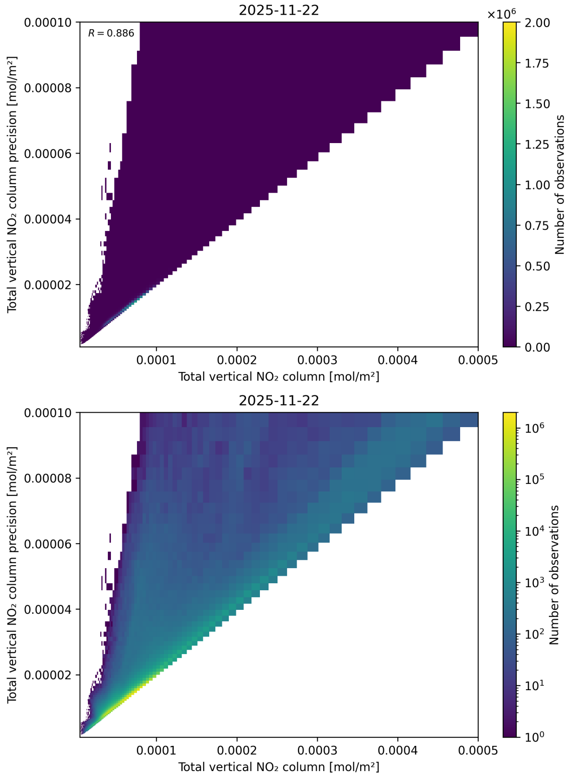
Figure 114: Scatter density plot of “Total vertical NO 2 column” against “Total vertical NO 2 column precision” for 2025-11-21 to 2025-11-23.
