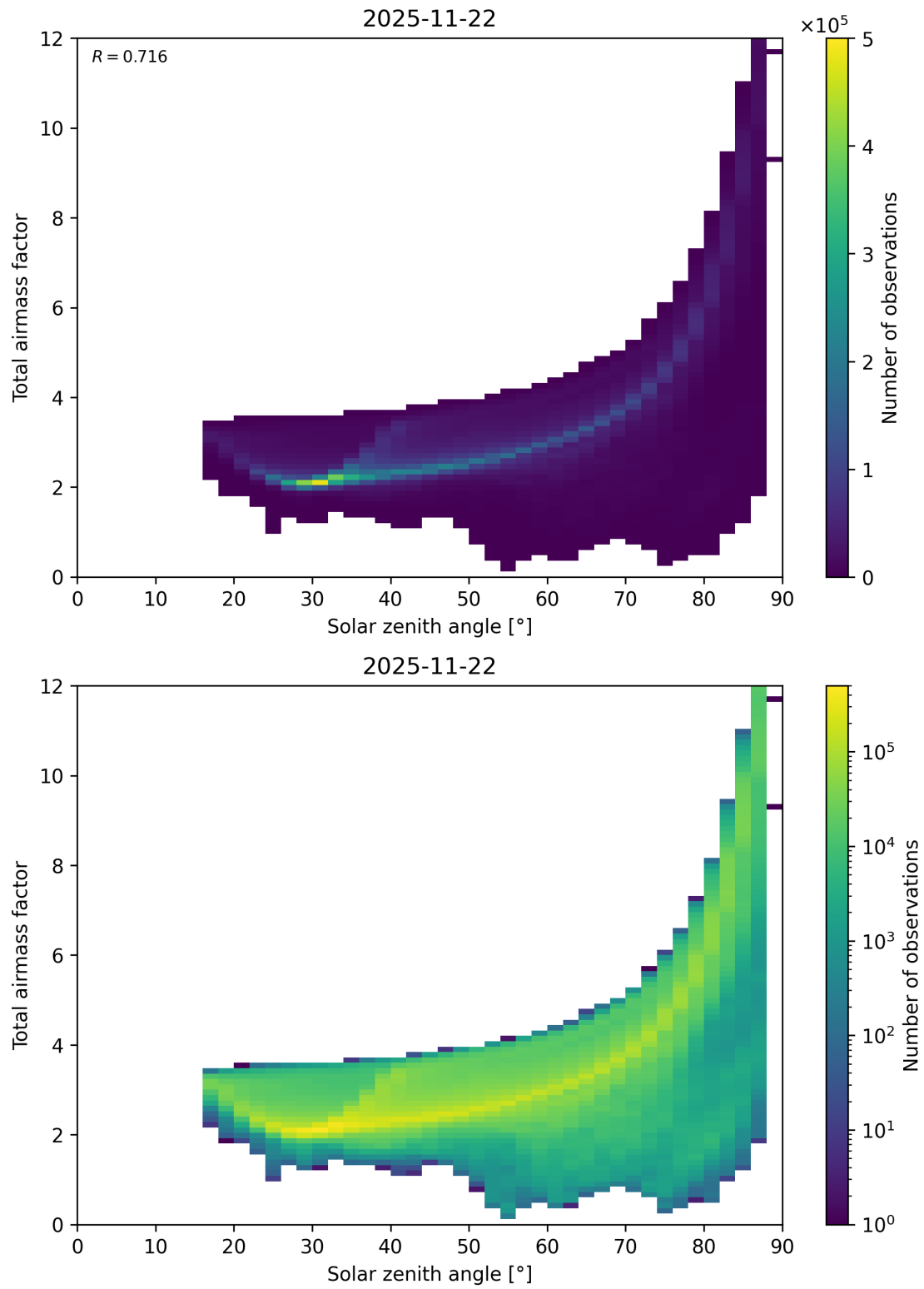
Figure 146: Scatter density plot of “Solar zenith angle” against “Total airmass factor” for 2025-11-21 to 2025-11-23.
