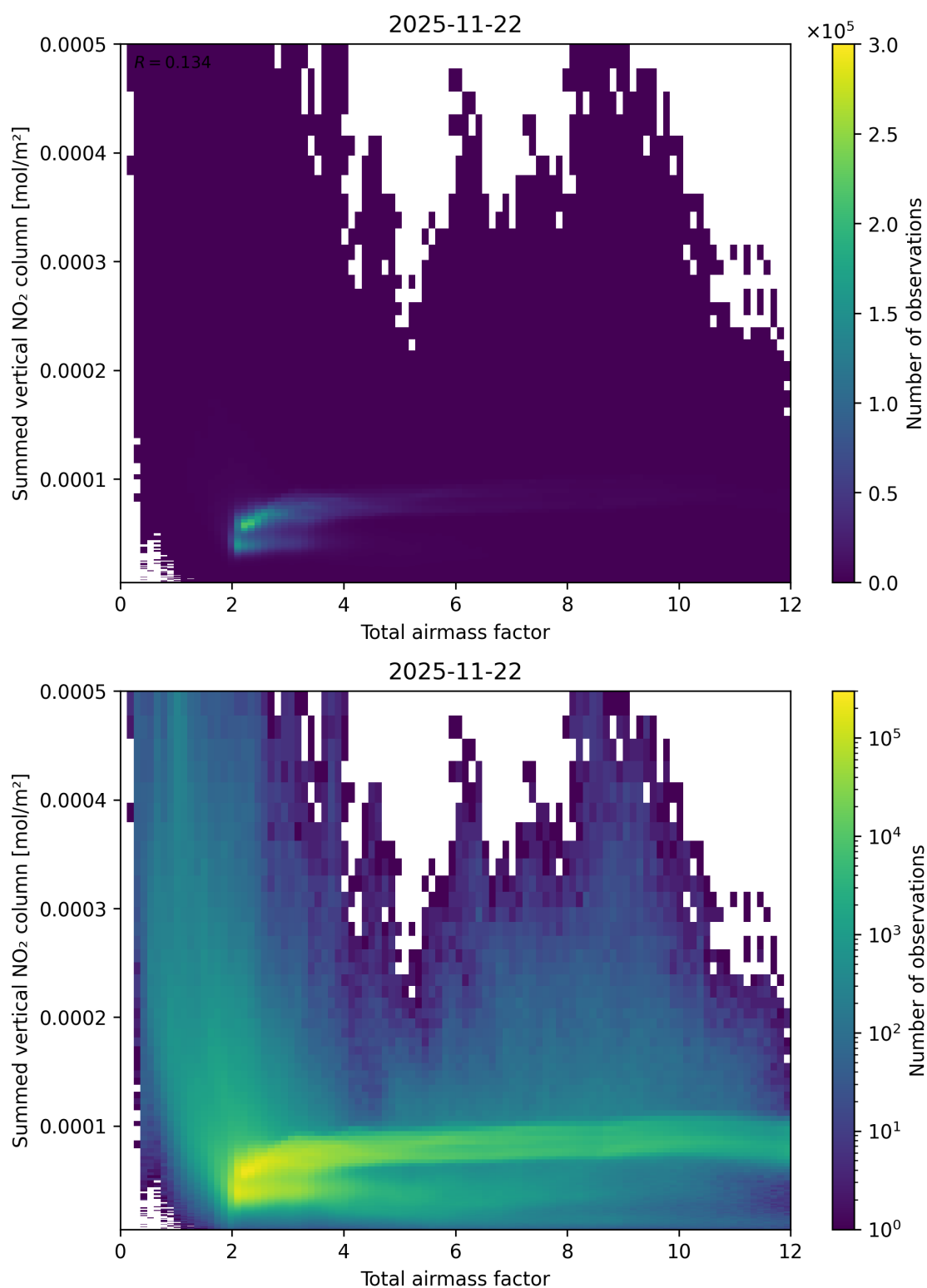
Figure 65: Scatter density plot of “Total airmass factor” against “Summed vertical NO 2 column” for 2025-11-21 to 2025-11-23.
