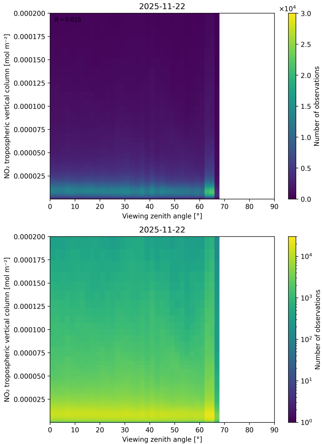
Figure 169: Scatter density plot of “Viewing zenith angle” against “NO 2 tropospheric vertical column” for 2025-11-21 to 2025-11-23.
