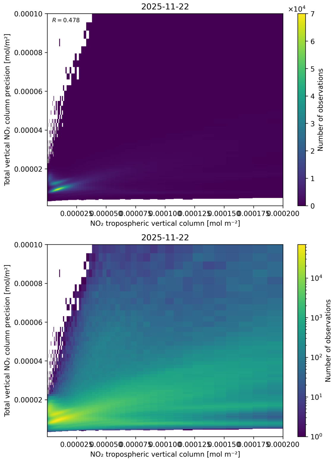
Figure 129: Scatter density plot of “NO 2 tropospheric vertical column” against “Total vertical NO 2 column precision” for 2025-11-21 to 2025-11-23.
