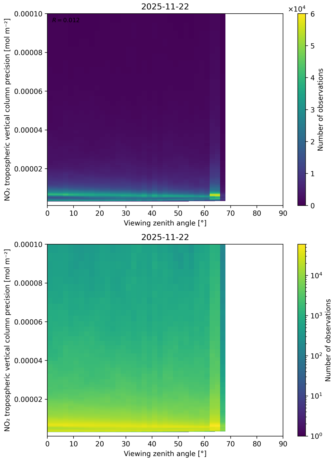
Figure 170: Scatter density plot of “Viewing zenith angle” against “NO 2 tropospheric vertical column precision” for 2025-11-21 to 2025-11-23.
