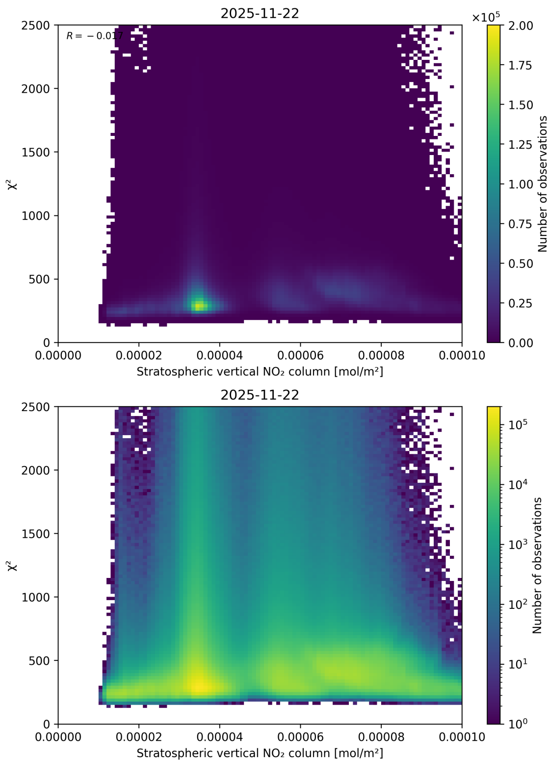
Figure 97: Scatter density plot of “Stratospheric vertical NO 2 column” against “ \chi^2 ” for 2025-11-21 to 2025-11-23.
