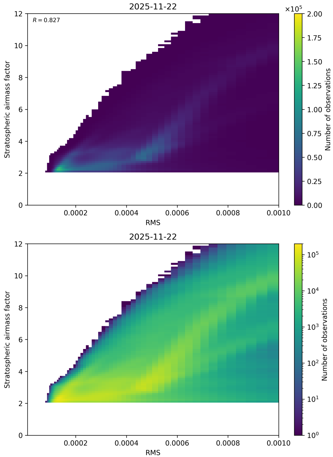
Figure 144: Scatter density plot of “RMS” against “Stratospheric airmass factor” for 2025-11-21 to 2025-11-23.
