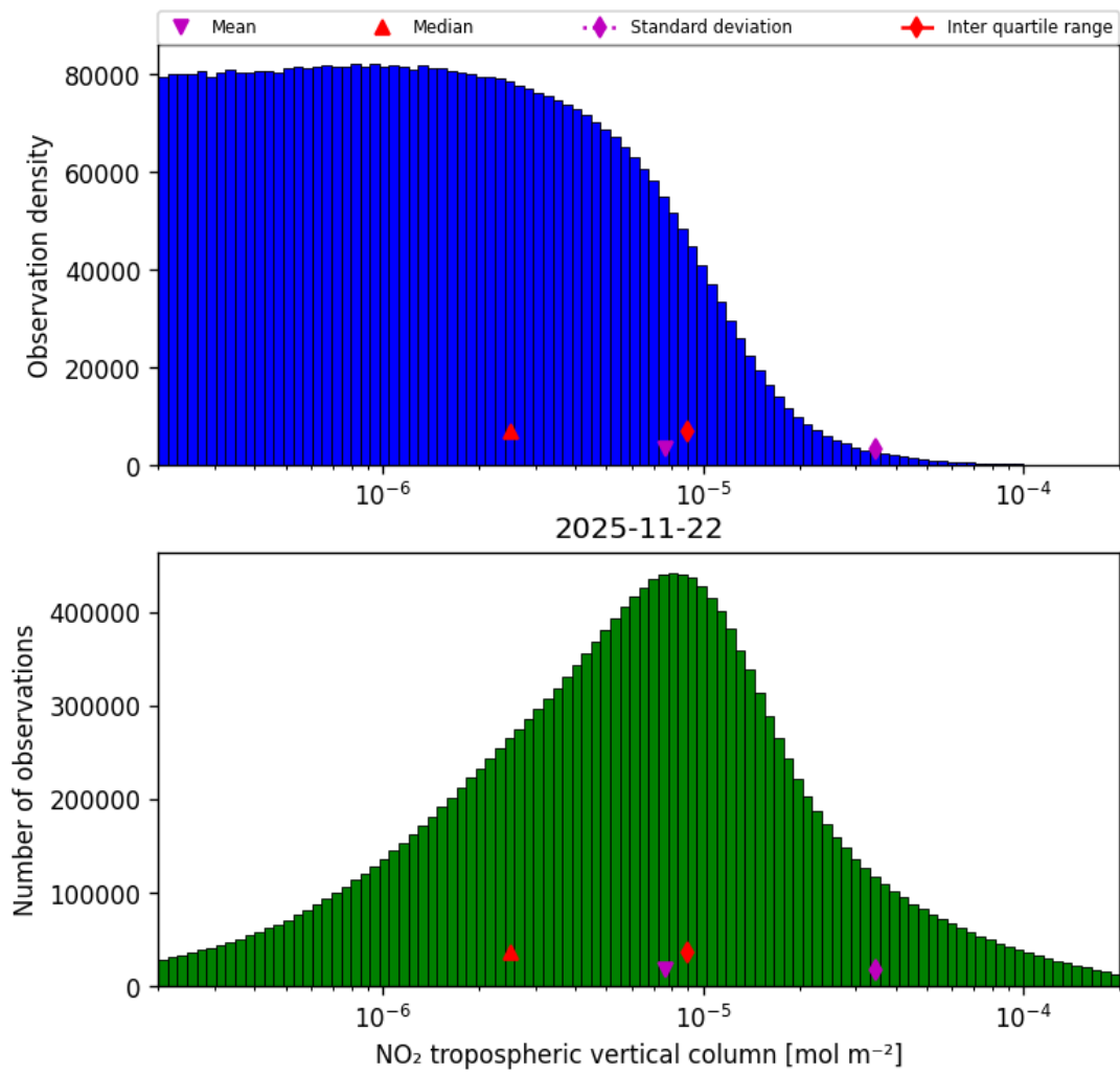
Figure 29: Histogram of “NO 2 tropospheric vertical column” for 2025-11-21 to 2025-11-23
