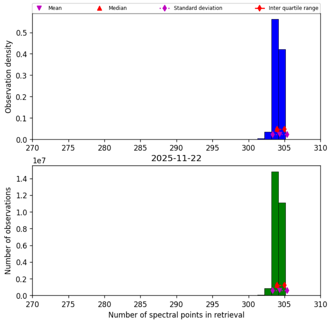
Figure 33: Histogram of “Number of spectral points in retrieval” for 2025-11-21 to 2025-11-23
