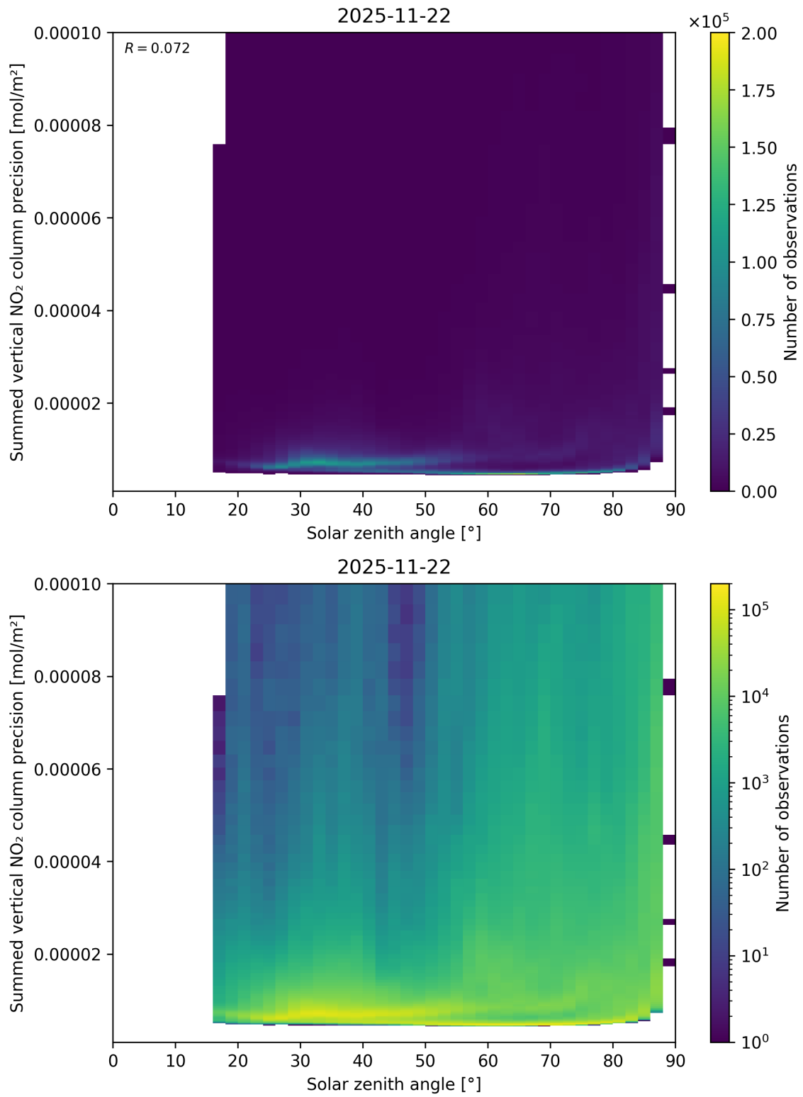
Figure 152: Scatter density plot of “Solar zenith angle” against “Summed vertical NO 2 column precision” for 2025-11-21 to 2025-11-23.
