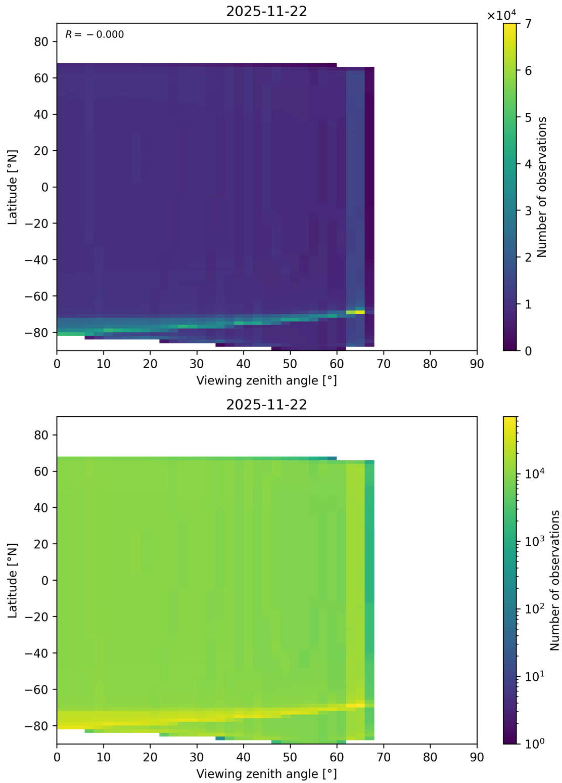
Figure 163: Scatter density plot of “Viewing zenith angle” against “Latitude” for 2025-11-21 to 2025-11-23.
