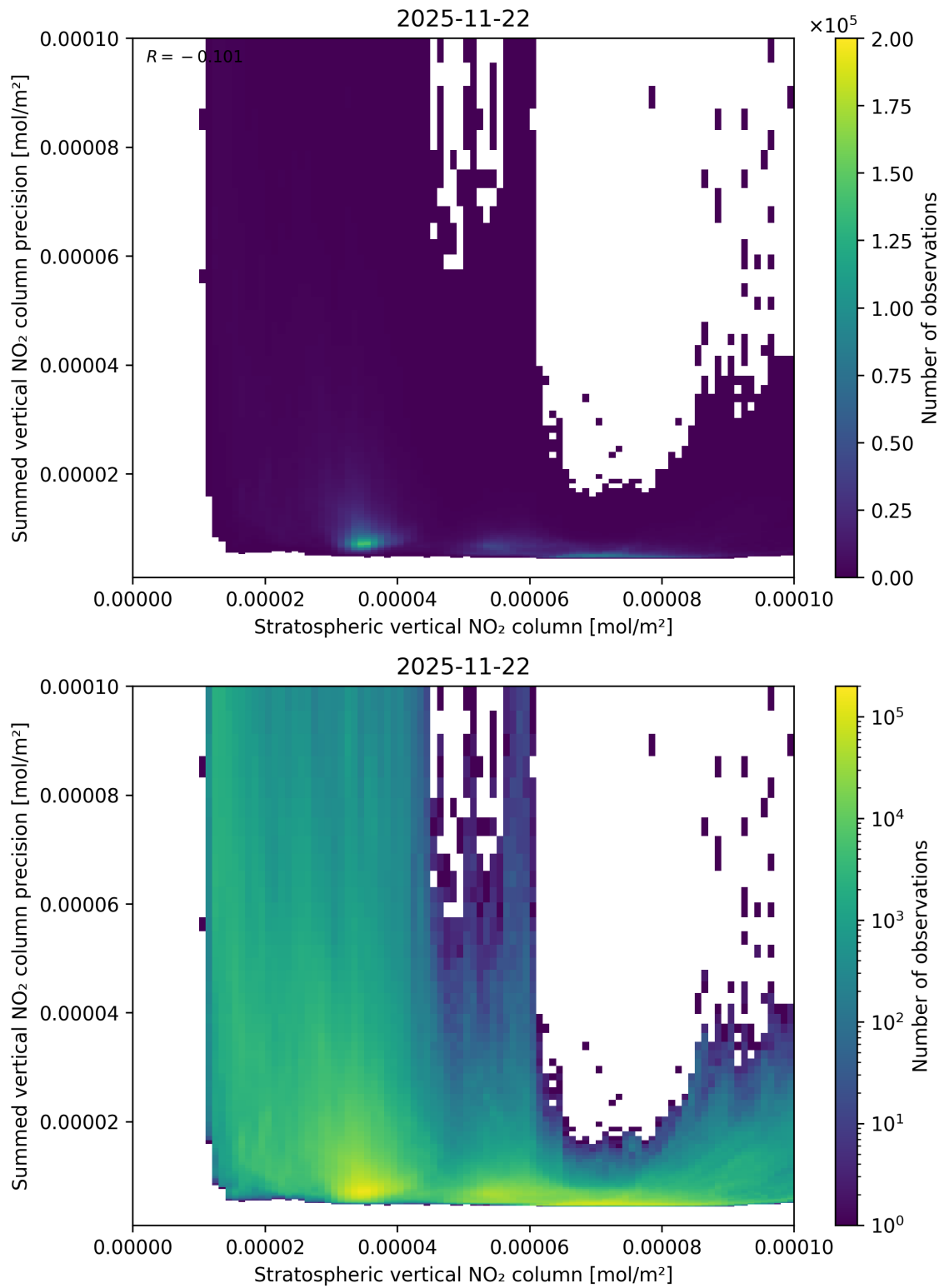
Figure 99: Scatter density plot of “Stratospheric vertical NO 2 column” against “Summed vertical NO 2 column precision” for 2025-11-21 to 2025-11-23.
