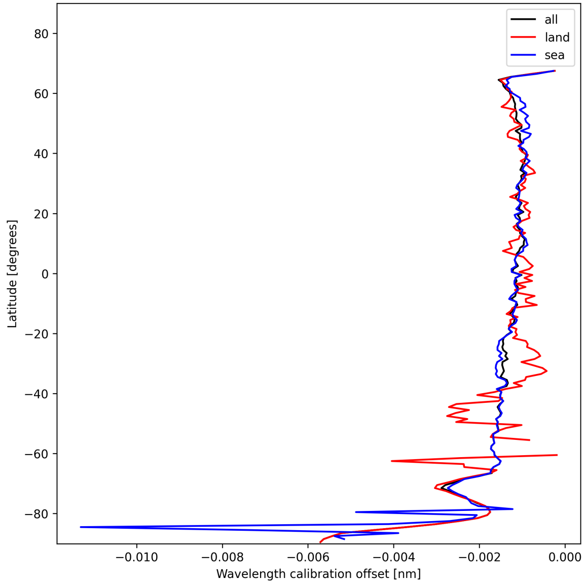
Figure 18: Zonal average of “Wavelength calibration offset” for 2025-11-21 to 2025-11-23.
