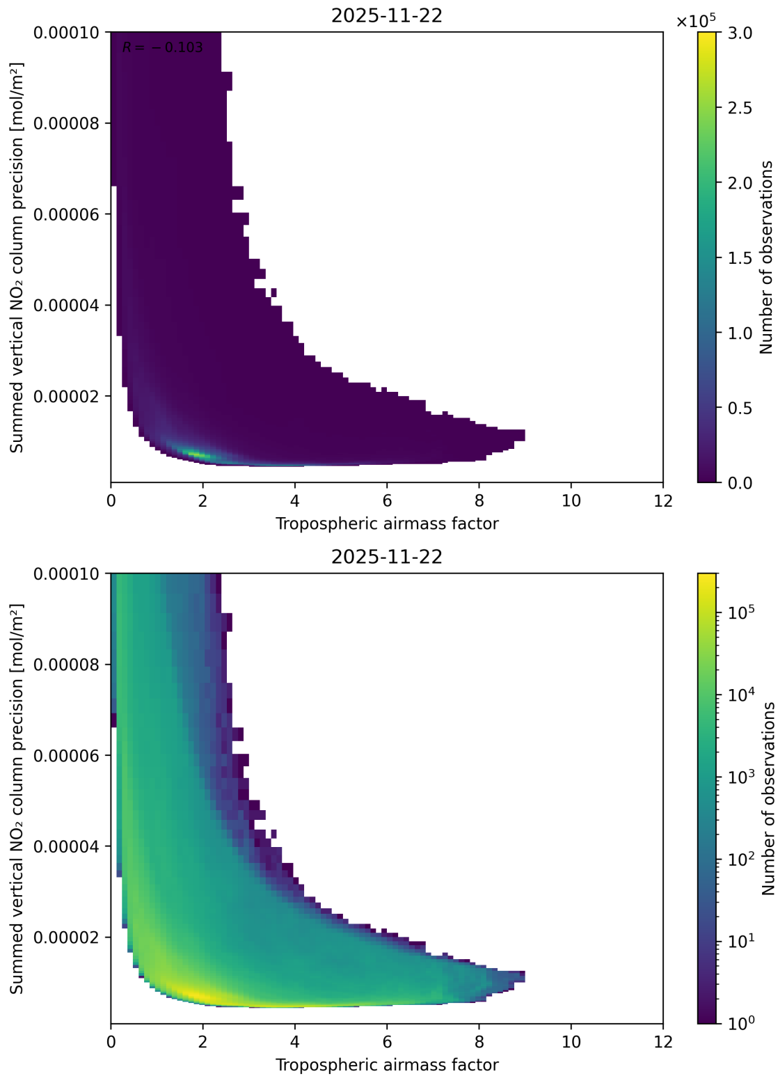
Figure 76: Scatter density plot of “Tropospheric air mass factor” against “Summed vertical NO 2 column precision” for 2025-11-21 to 2025-11-23.
