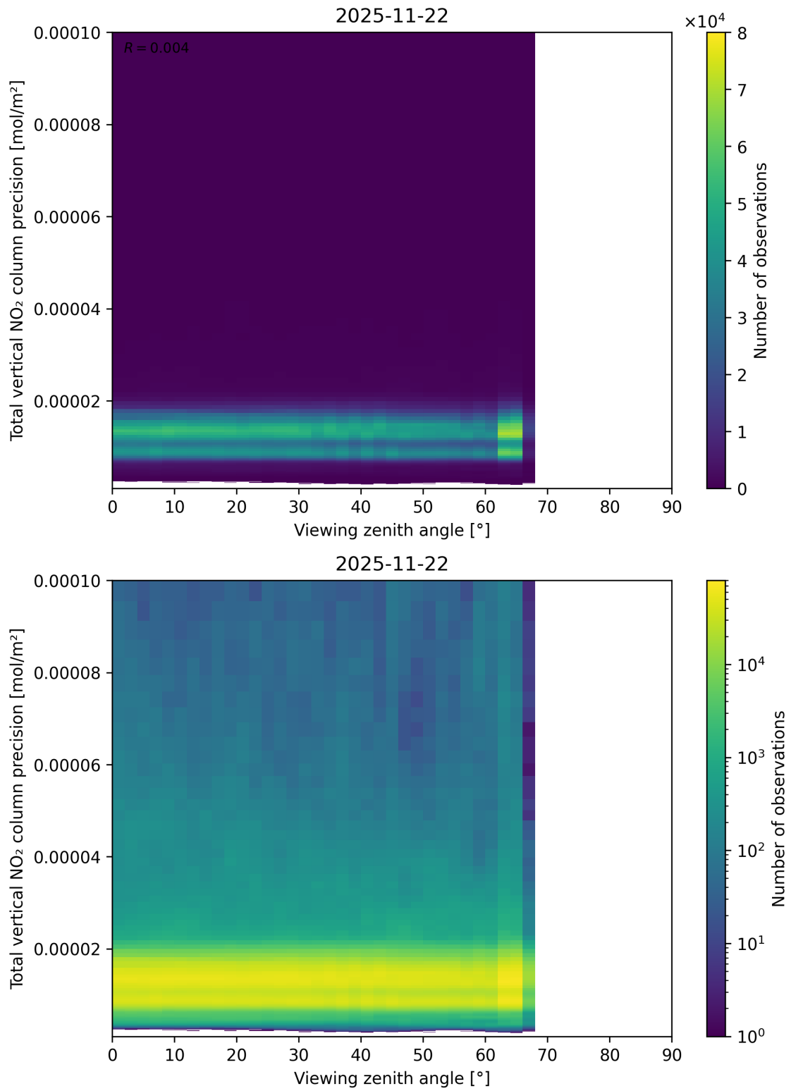
Figure 168: Scatter density plot of “Viewing zenith angle” against “Total vertical NO 2 column precision” for 2025-11-21 to 2025-11-23.
