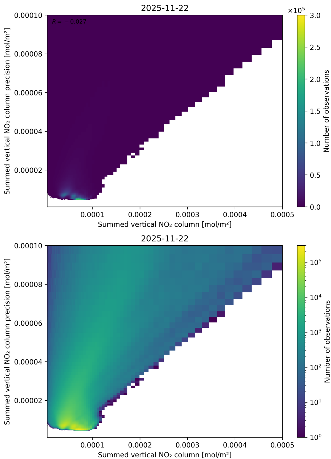
Figure 105: Scatter density plot of “Summed vertical NO 2 column” against “Summed vertical NO 2 column precision” for 2025-11-21 to 2025-11-23.
