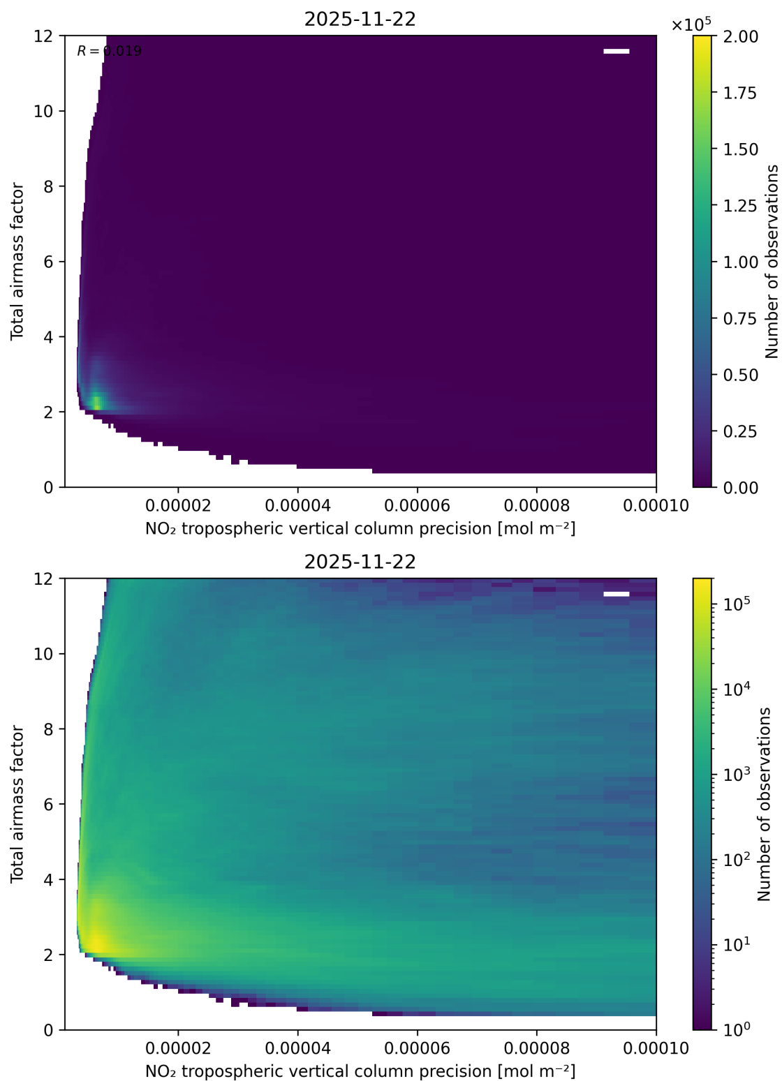
Figure 132: Scatter density plot of “NO 2 tropospheric vertical column precision” against “Total air mass factor” for 2025-11-21 to 2025-11-23.
