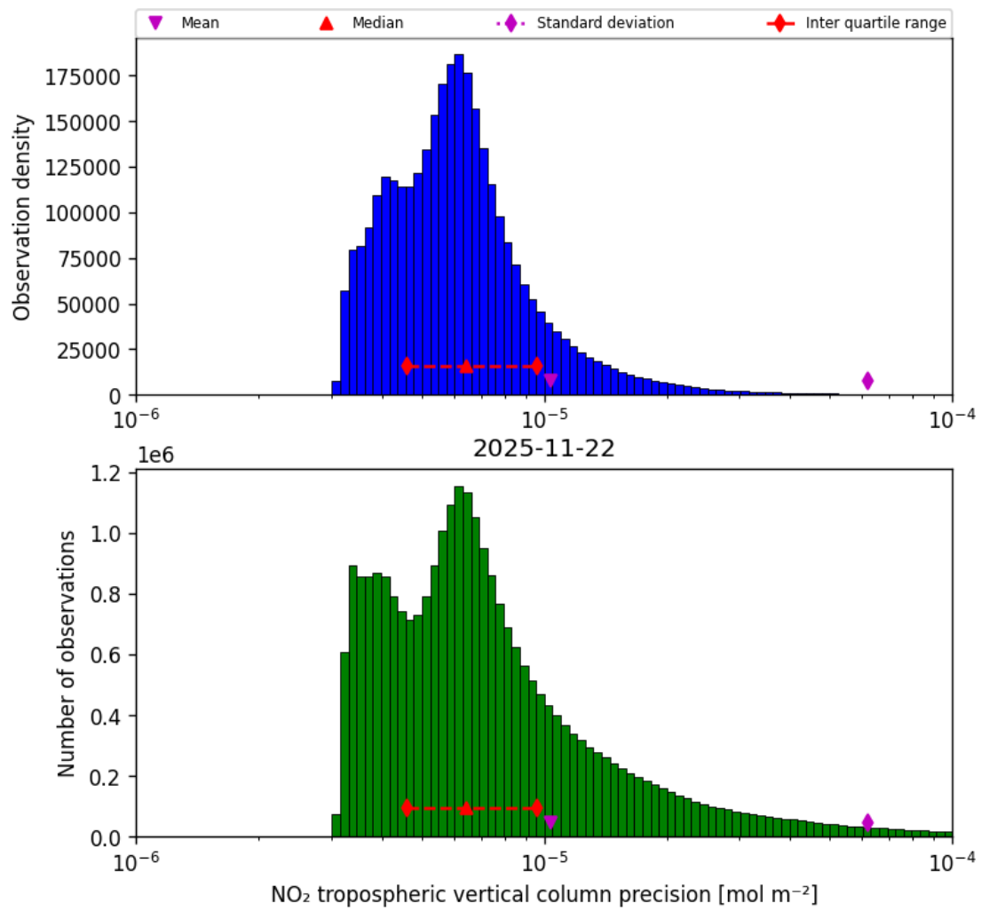
Figure 30: Histogram of “NO 2 tropospheric vertical column precision” for 2025-11-21 to 2025-11-23
