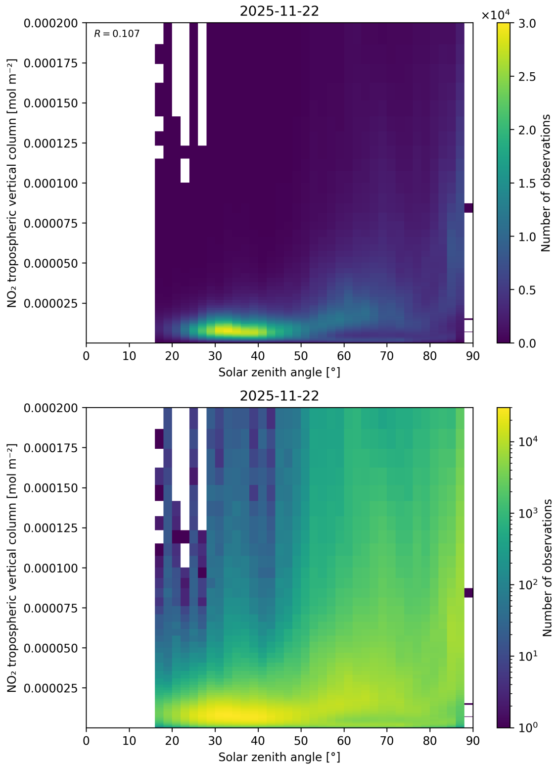
Figure 155: Scatter density plot of “Solar zenith angle” against “NO 2 tropospheric vertical column” for 2025-11-21 to 2025-11-23.
