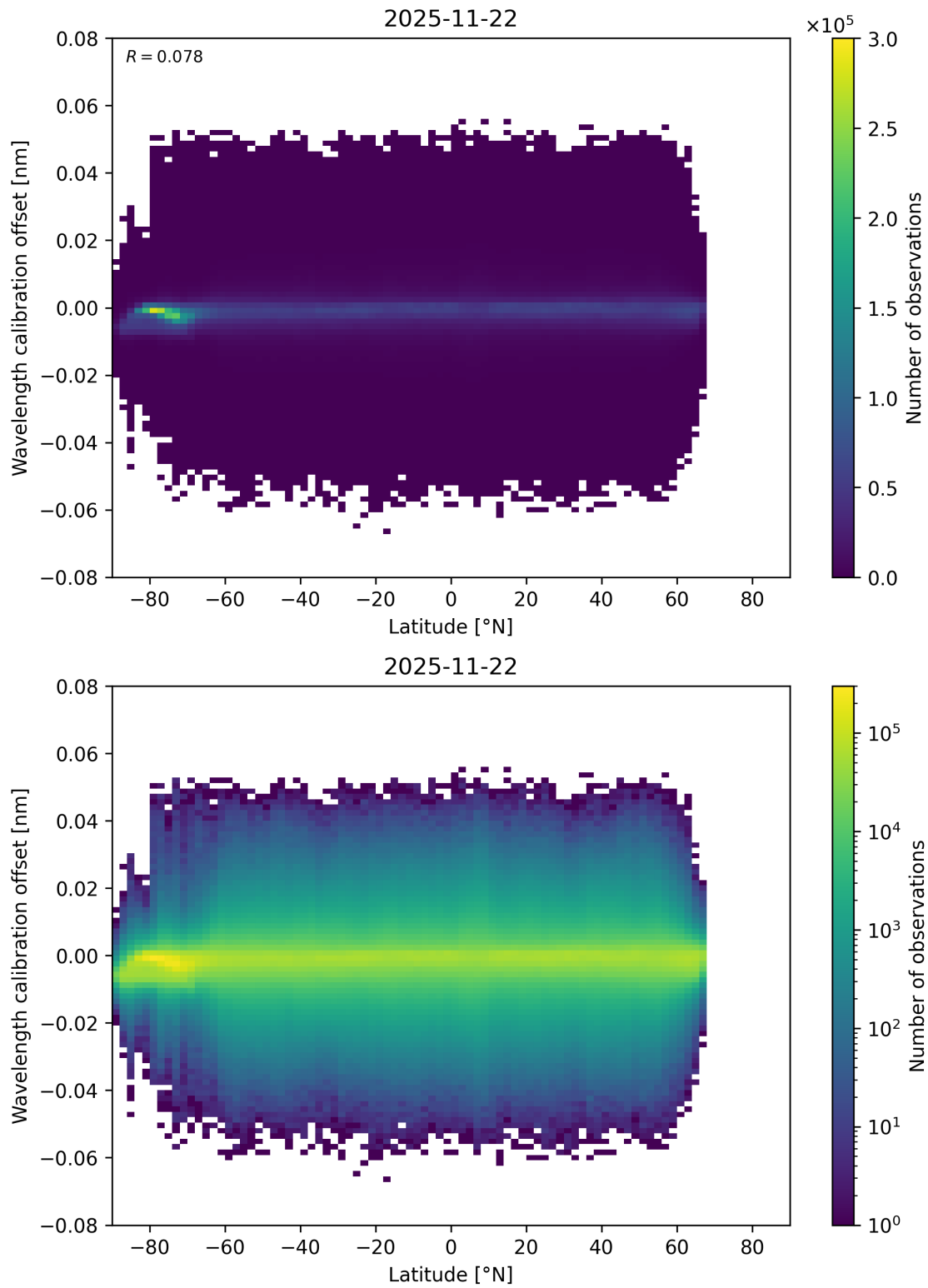
Figure 95: Scatter density plot of “Latitude” against “Wavelength calibration offset” for 2025-11-21 to 2025-11-23.
