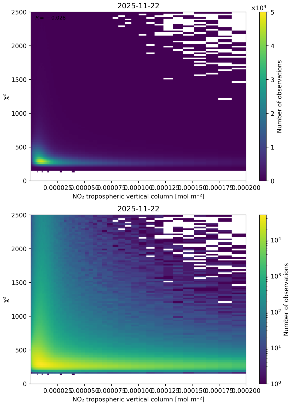
Figure 124: Scatter density plot of “NO 2 tropospheric vertical column” against “ \chi^2 ” for 2025-11-21 to 2025-11-23.
