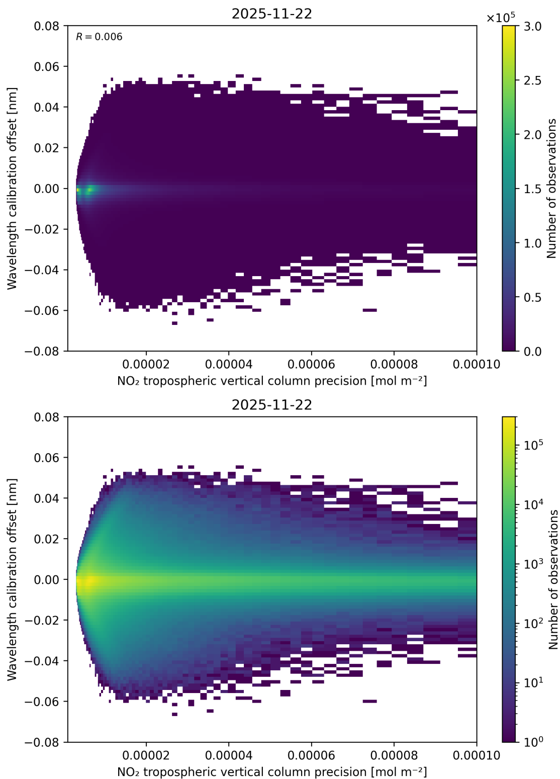
Figure 141: Scatter density plot of “NO 2 tropospheric vertical column precision” against “Wavelength calibration offset” for 2025-11-21 to 2025-11-23.
