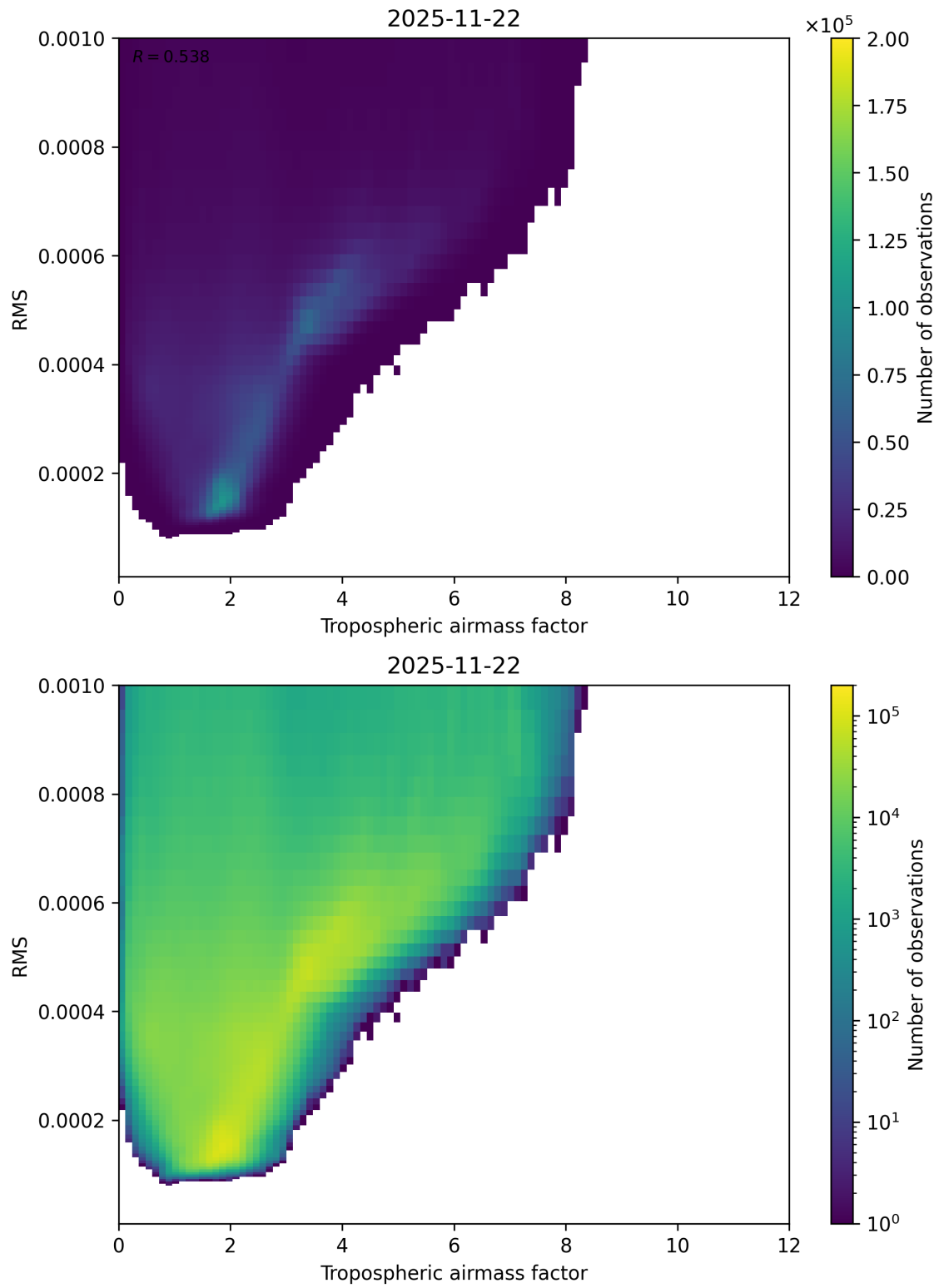
Figure 79: Scatter density plot of “Tropospheric airmass factor” against “RMS” for 2025-11-21 to 2025-11-23.
