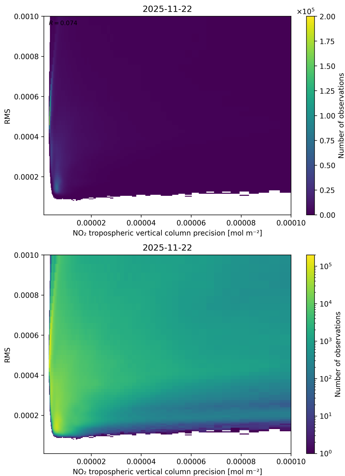
Figure 140: Scatter density plot of “NO 2 tropospheric vertical column precision” against “RMS” for 2025-11-21 to 2025-11-23.
