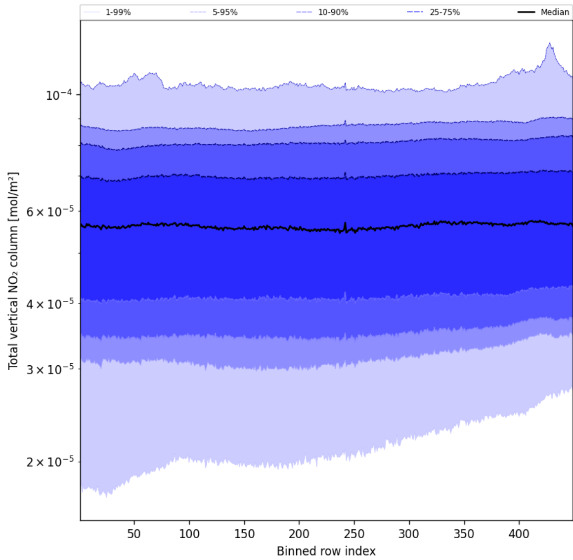
Figure 55: Along track statistics of “Total vertical NO 2 column” for 2025-11-21 to 2025-11-23
