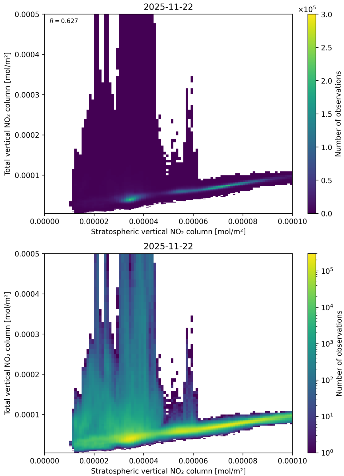
Figure 100: Scatter density plot of “Stratospheric vertical NO 2 column” against “Total vertical NO 2 column” for 2025-11-21 to 2025-11-23.
