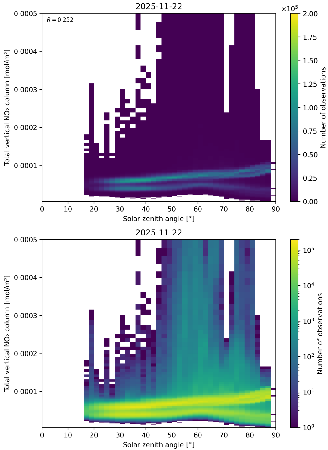
Figure 153: Scatter density plot of “Solar zenith angle” against “Total vertical NO 2 column” for 2025-11-21 to 2025-11-23.
