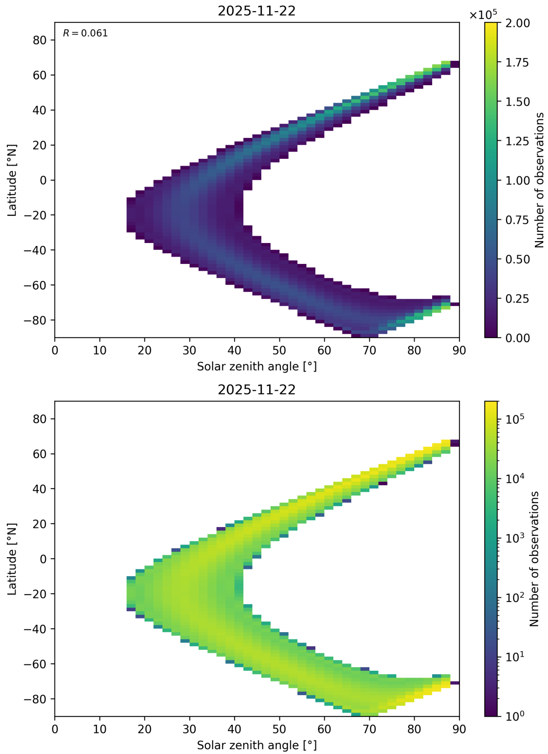
Figure 149: Scatter density plot of “Solar zenith angle” against “Latitude” for 2025-11-21 to 2025-11-23.
