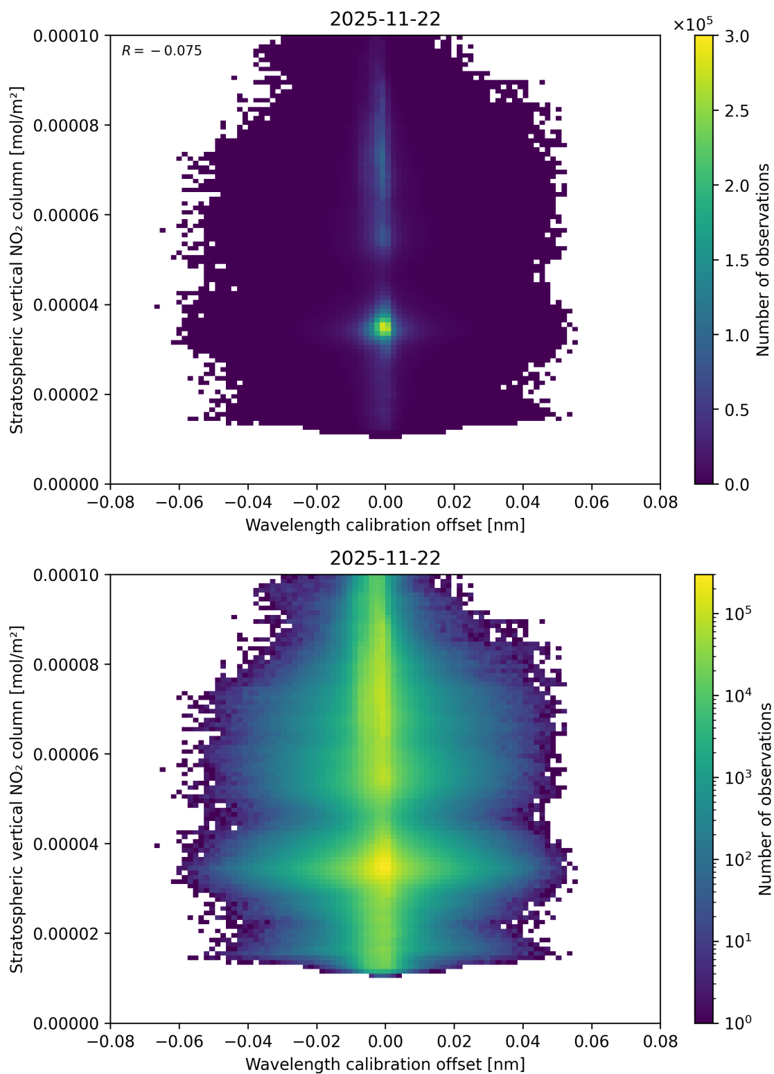
Figure 176: Scatter density plot of “Wavelength calibration offset” against “Stratospheric vertical NO 2 column” for 2025-11-21 to 2025-11-23.
