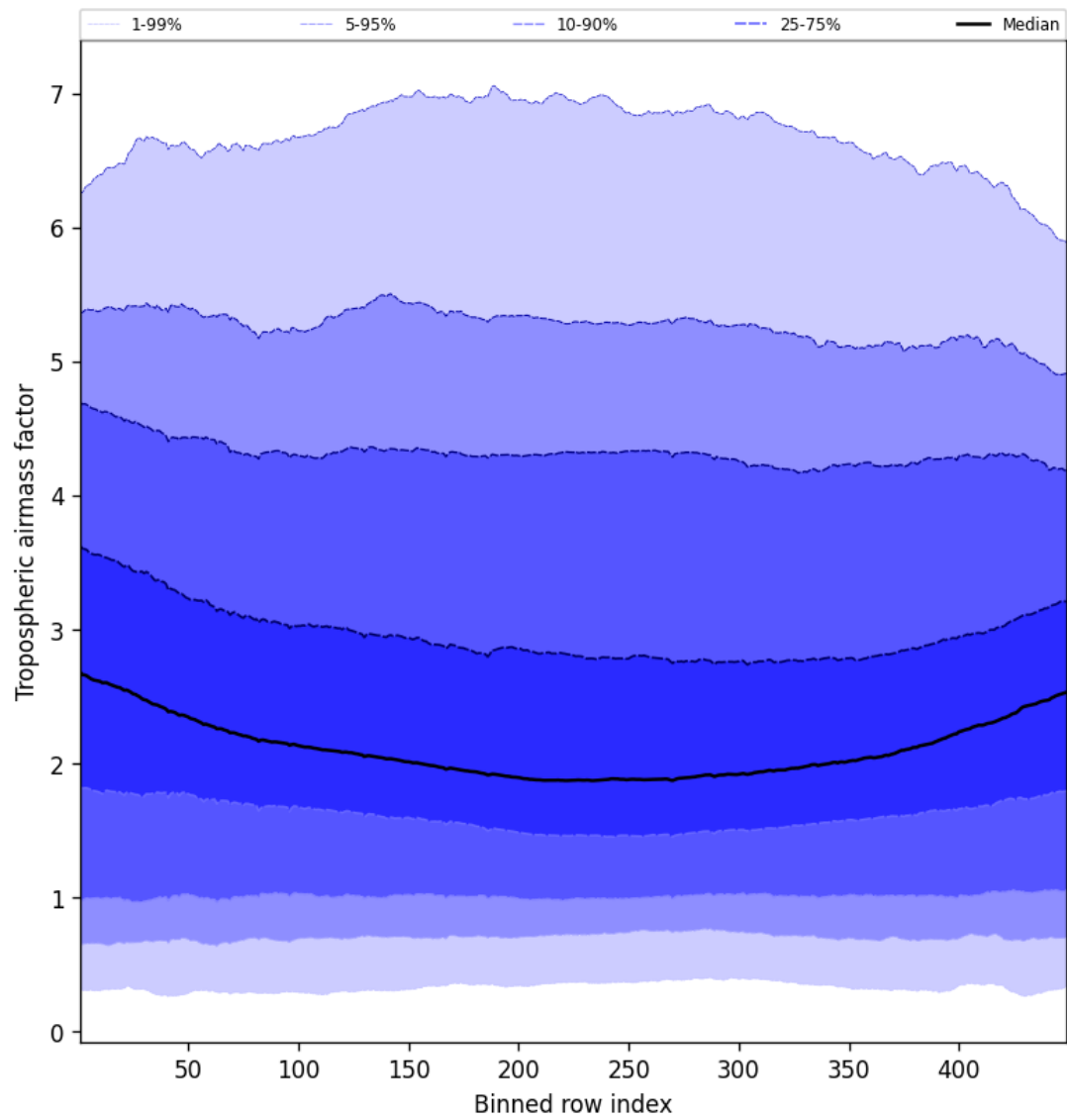
Figure 48: Along track statistics of “Tropospheric air mass factor” for 2025-11-21 to 2025-11-23
