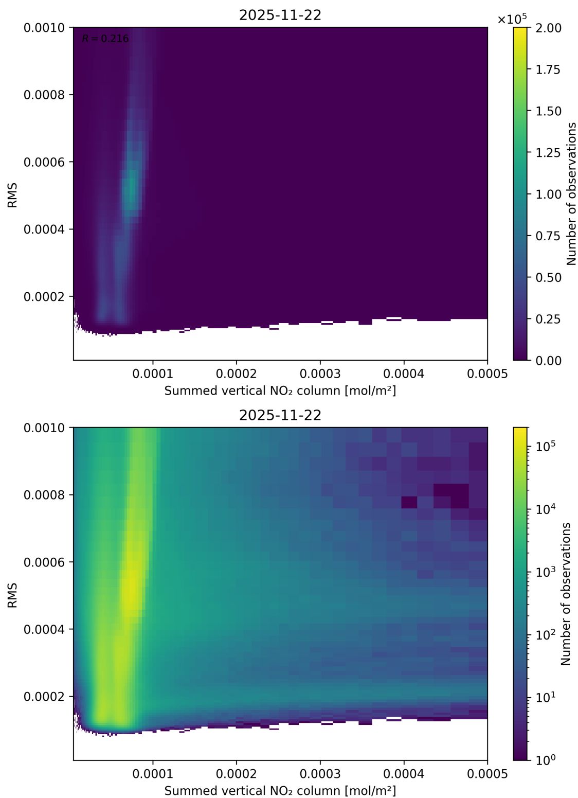
Figure 109: Scatter density plot of “Summed vertical NO 2 column” against “RMS” for 2025-11-21 to 2025-11-23.
