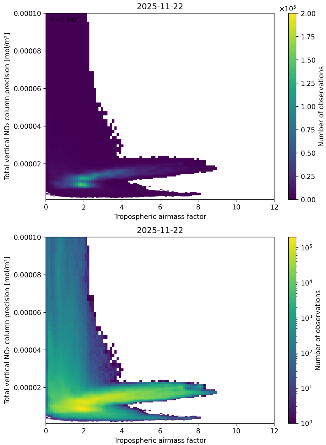
Figure 78: Scatter density plot of “Tropospheric air mass factor” against “Total vertical NO 2 column precision” for 2025-11-21 to 2025-11-23.
