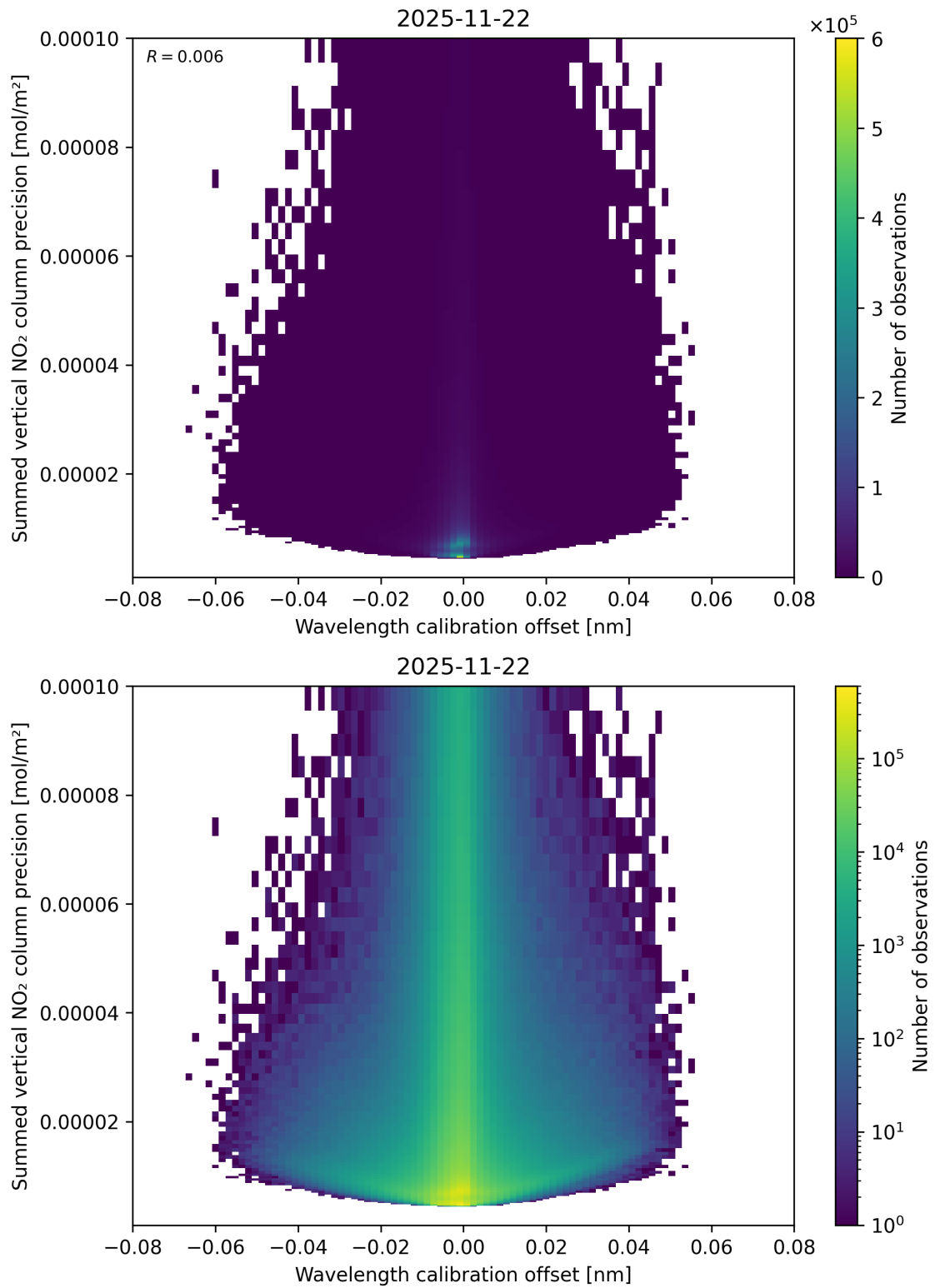
Figure 178: Scatter density plot of “Wavelength calibration offset” against “Summed vertical NO 2 column precision” for 2025-11-21 to 2025-11-23.
