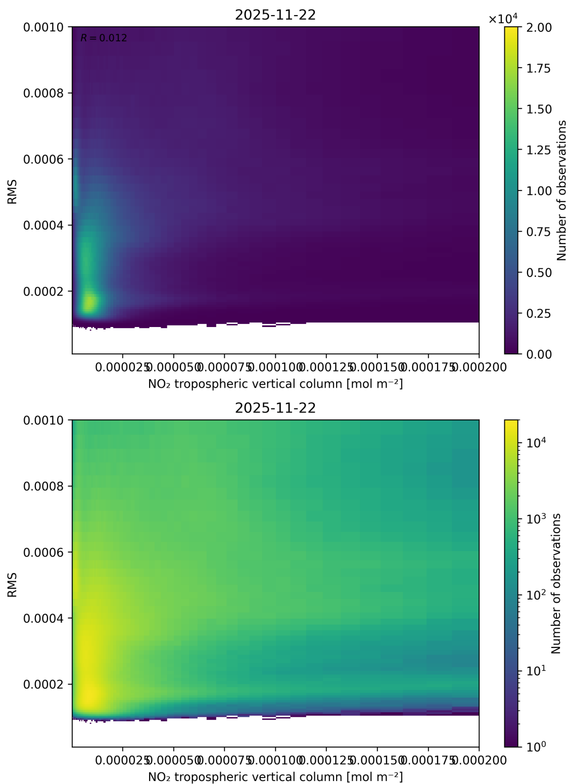
Figure 142: Scatter density plot of “NO 2 tropospheric vertical column” against “RMS” for 2025-11-21 to 2025-11-23.
