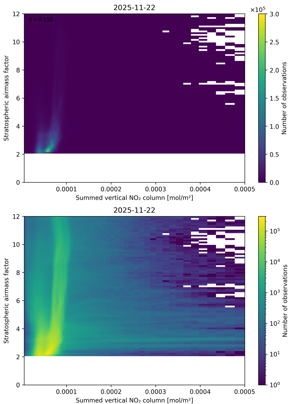
Figure 103: Scatter density plot of “Summed vertical NO 2 column” against “Stratospheric airmass factor” for 2025-11-21 to 2025-11-23.
