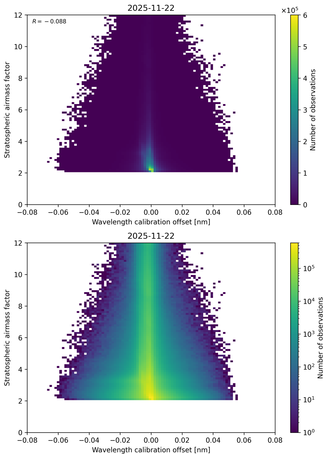
Figure 174: Scatter density plot of “Wavelength calibration offset” against “Stratospheric airmass factor” for 2025-11-21 to 2025-11-23.
