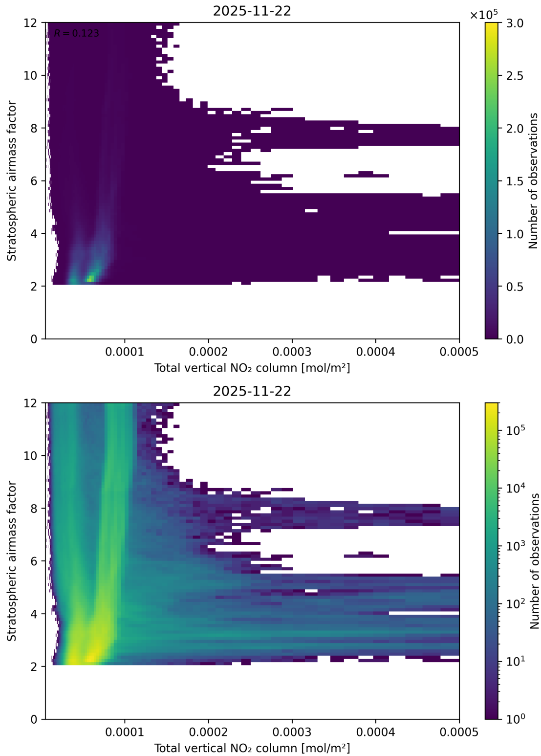
Figure 110: Scatter density plot of “Total vertical NO 2 column” against “Stratospheric airmass factor” for 2025-11-21 to 2025-11-23.
