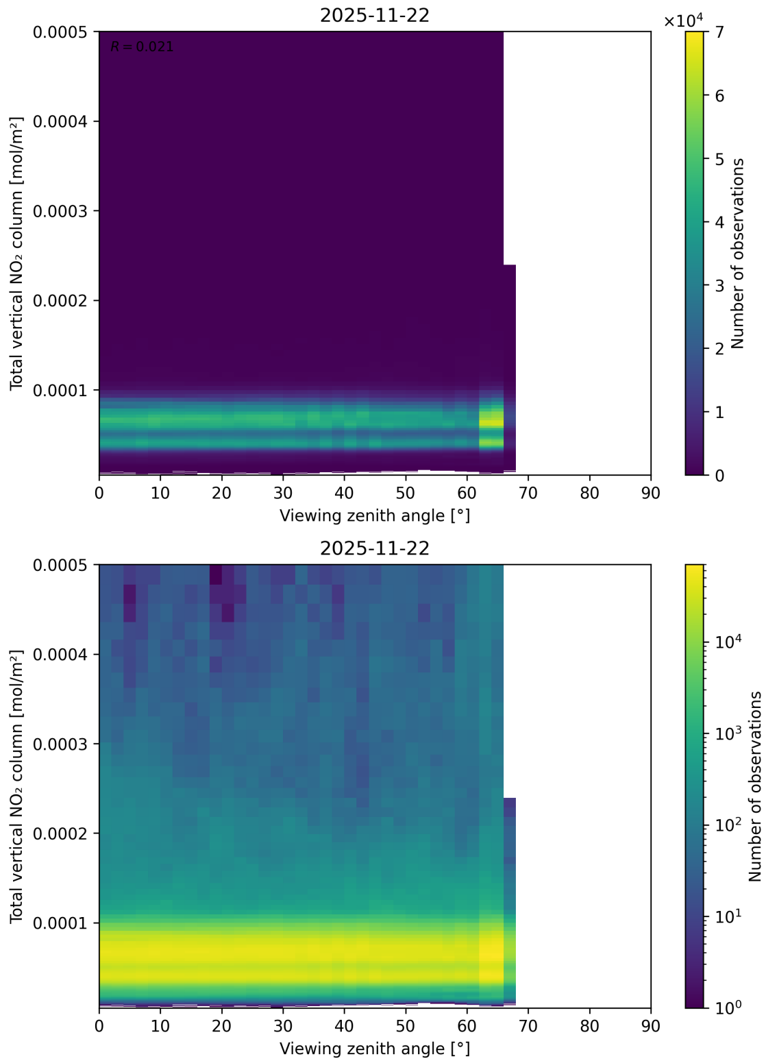
Figure 167: Scatter density plot of “Viewing zenith angle” against “Total vertical NO 2 column” for 2025-11-21 to 2025-11-23.
