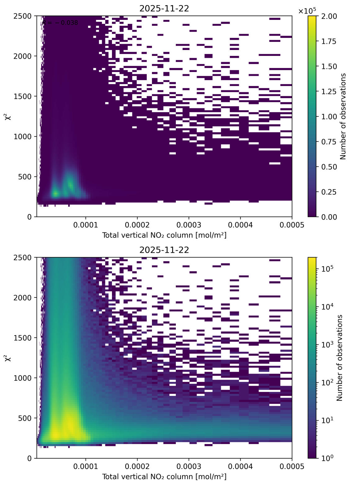
Figure 111: Scatter density plot of “Total vertical NO 2 column” against “ \chi^2 ” for 2025-11-21 to 2025-11-23.
