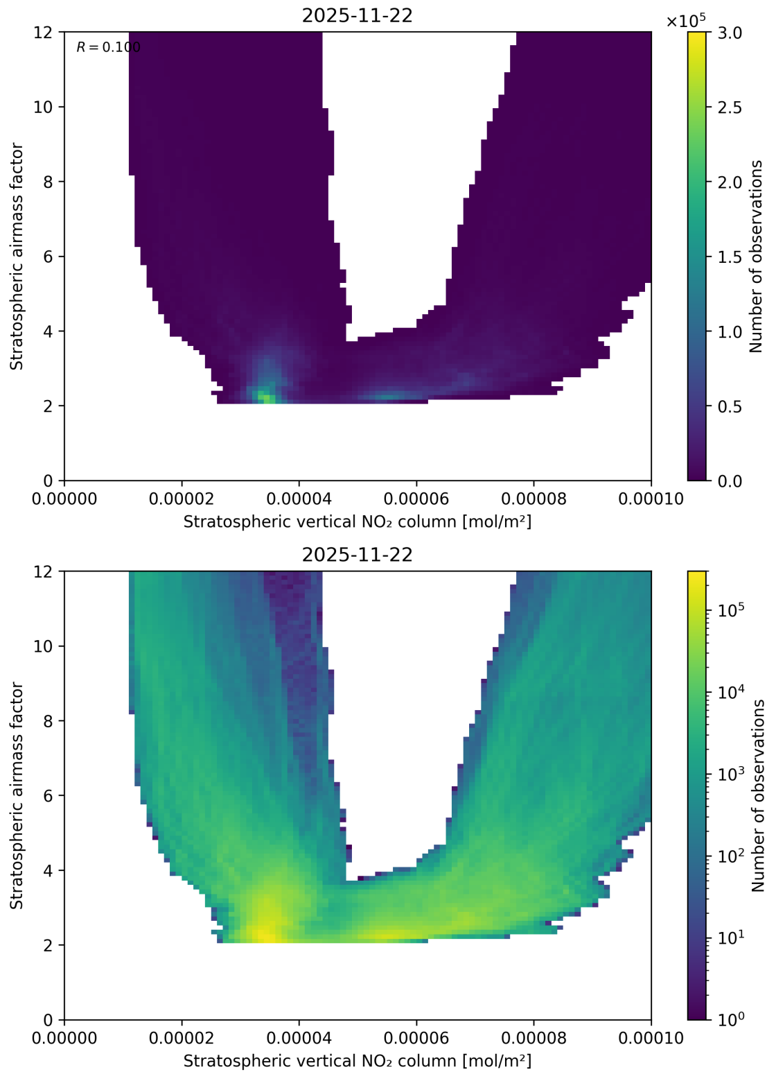
Figure 96: Scatter density plot of “Stratospheric vertical NO 2 column” against “Stratospheric airmass factor” for 2025-11-21 to 2025-11-23.
