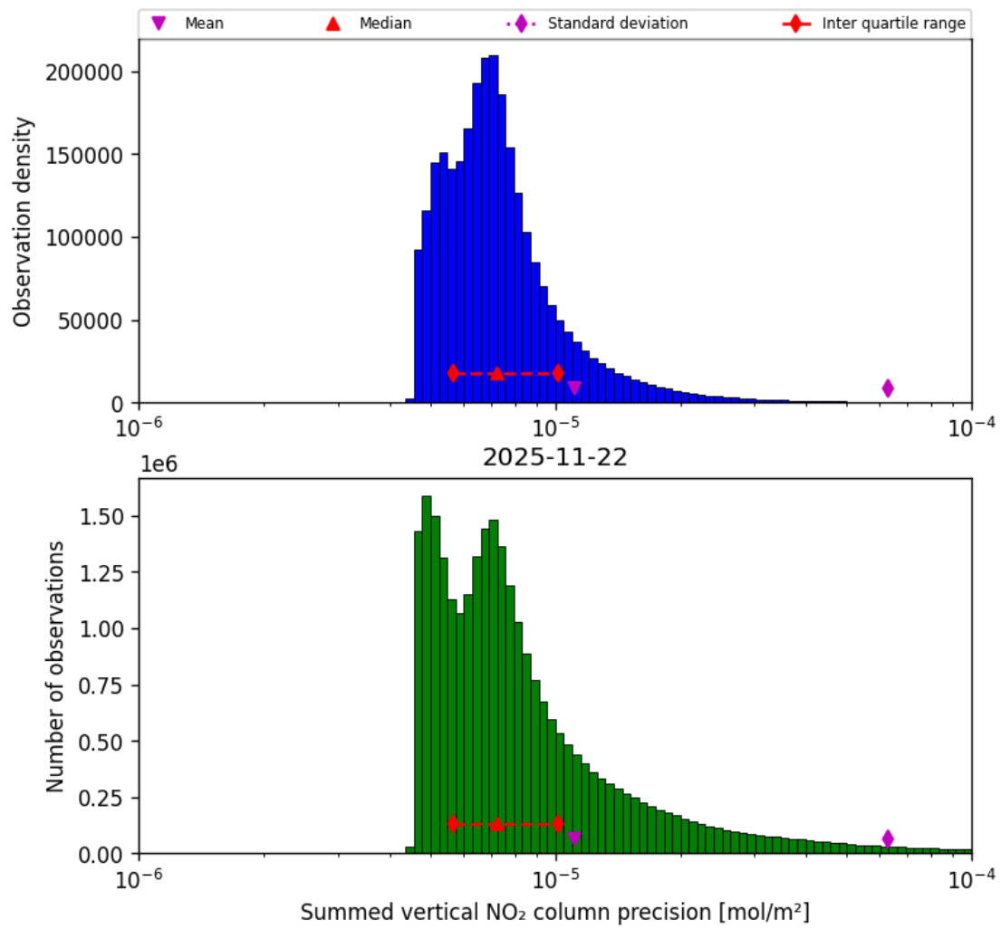
Figure 41: Histogram of "Summed vertical NO 2 column precision" for 2025-11-21 to 2025-11-23
