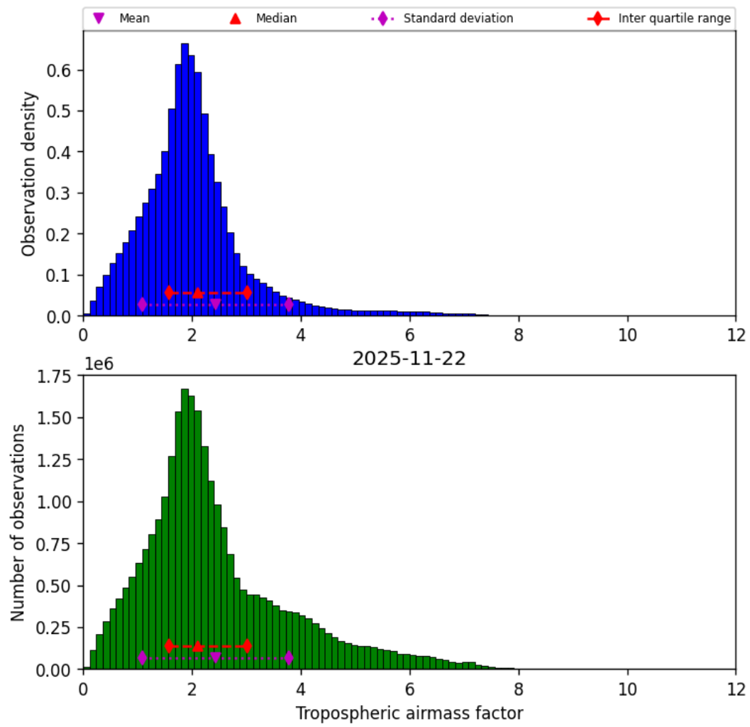
Figure 31: Histogram of “Tropospheric airmass factor” for 2025-11-21 to 2025-11-23
