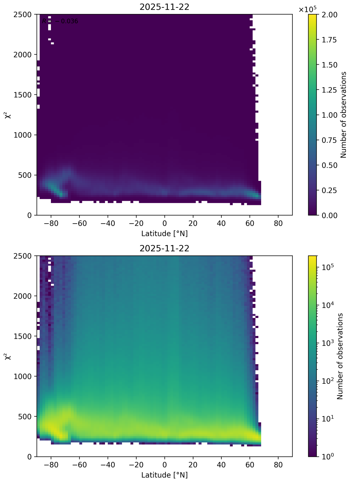
Figure 86: Scatter density plot of “Latitude” against “ \chi^2 ” for 2025-11-21 to 2025-11-23.
