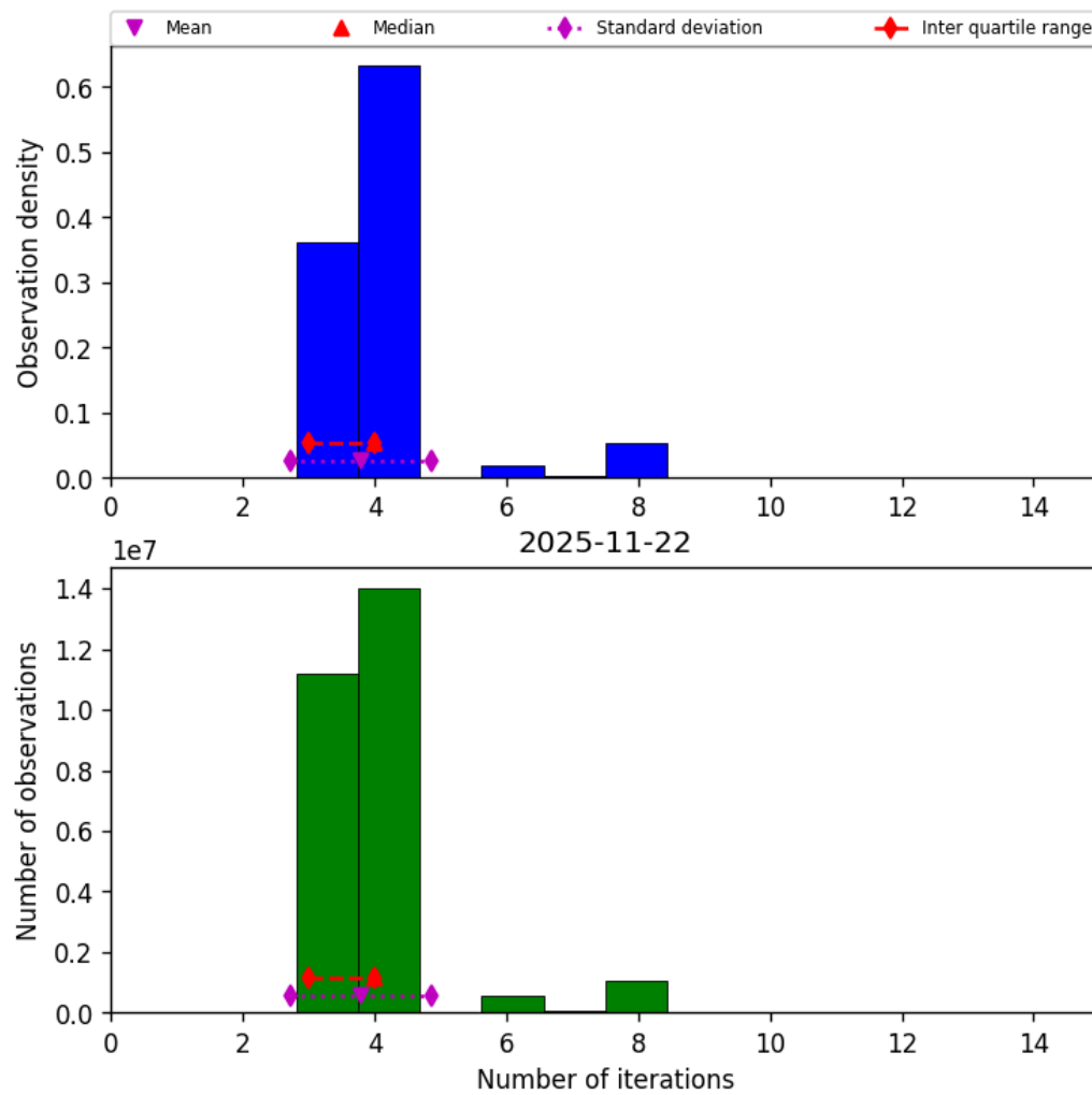
Figure 34: Histogram of “Number of iterations” for 2025-11-21 to 2025-11-23
