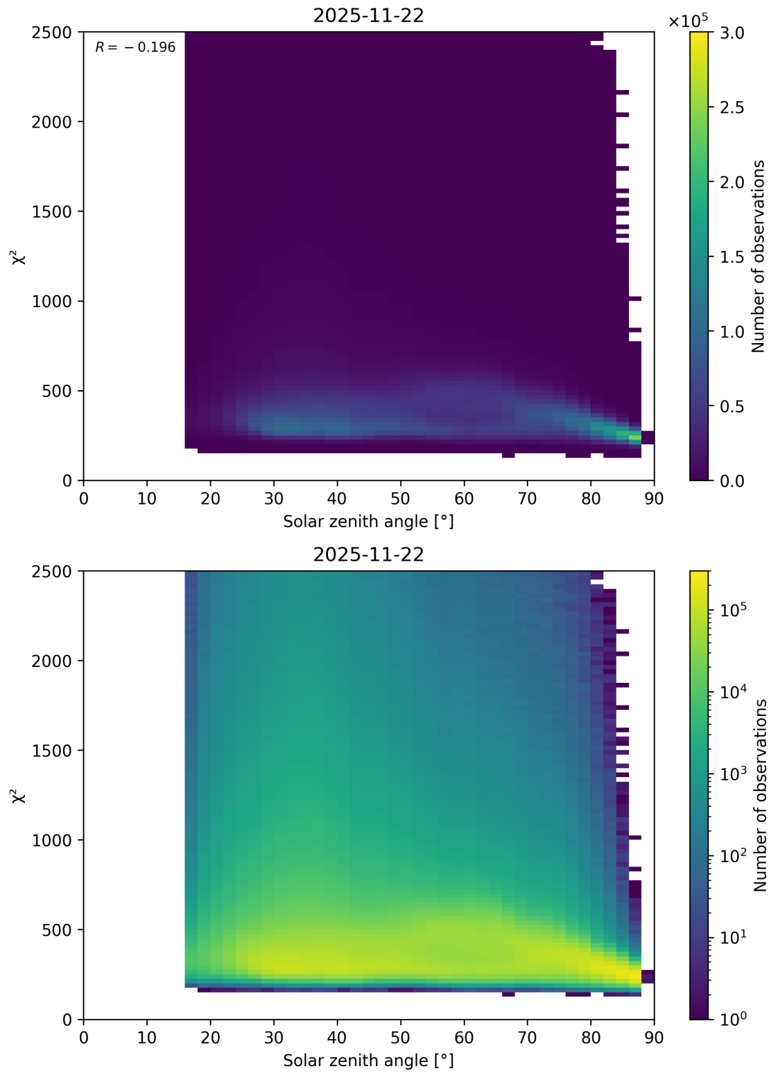
Figure 148: Scatter density plot of “Solar zenith angle” against “ \chi^2 ” for 2025-11-21 to 2025-11-23.
