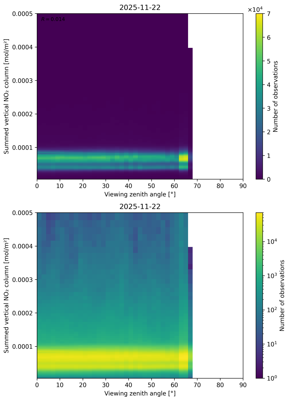
Figure 165: Scatter density plot of “Viewing zenith angle” against “Summed vertical NO 2 column” for 2025-11-21 to 2025-11-23.
