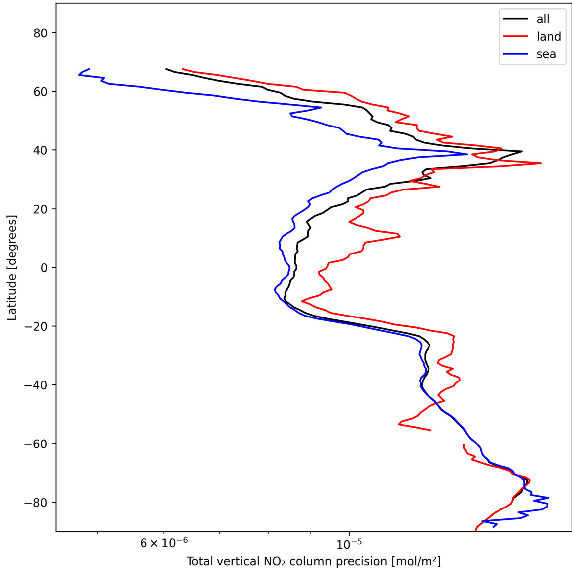
Figure 22: Zonal average of “Total vertical NO 2 column precision” for 2025-11-21 to 2025-11-23.
