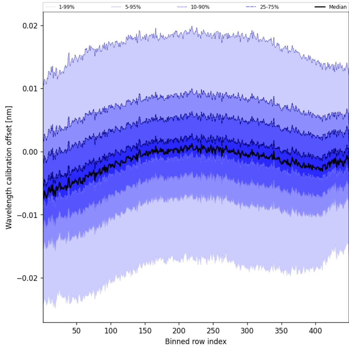
Figure 52: Along track statistics of “Wavelength calibration offset” for 2025-11-21 to 2025-11-23
