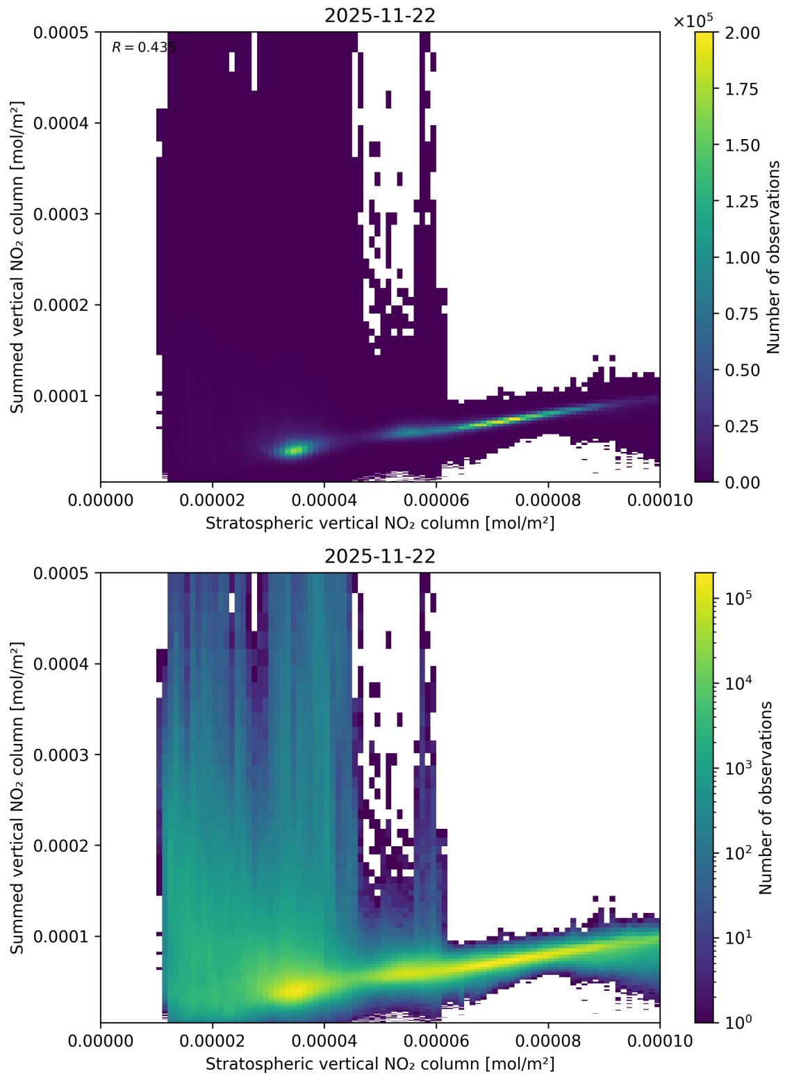
Figure 98: Scatter density plot of “Stratospheric vertical NO 2 column” against “Summed vertical NO 2 column” for 2025-11-21 to 2025-11-23.
