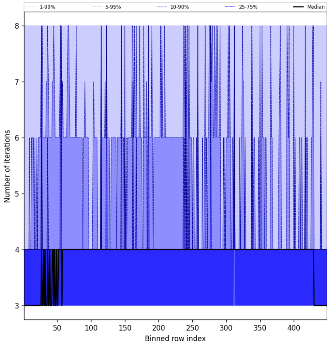
Figure 51: Along track statistics of “Number of iterations” for 2025-11-21 to 2025-11-23
