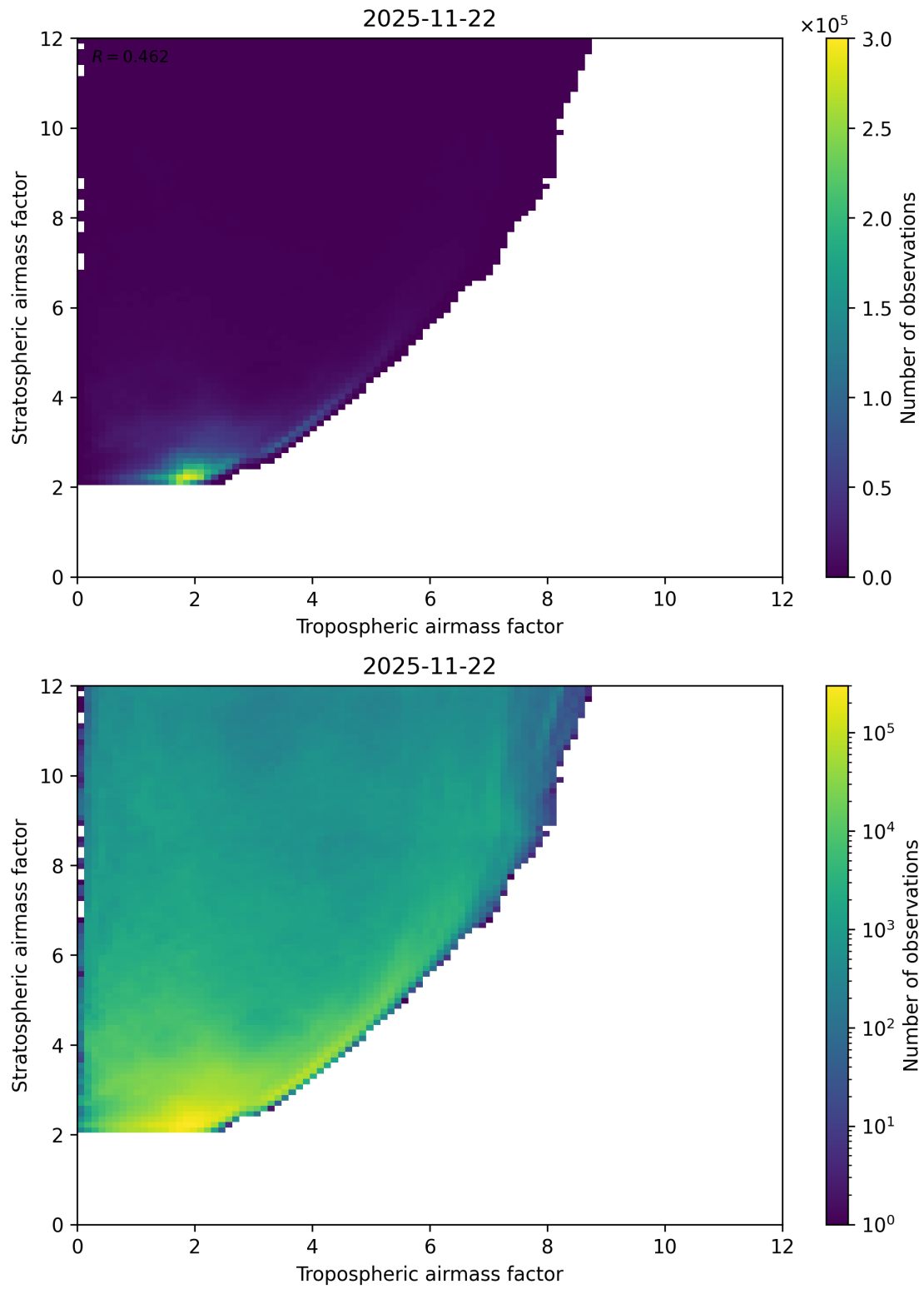
Figure 71: Scatter density plot of “Tropospheric airmass factor” against “Stratospheric airmass factor” for 2025-11-21 to 2025-11-23.
