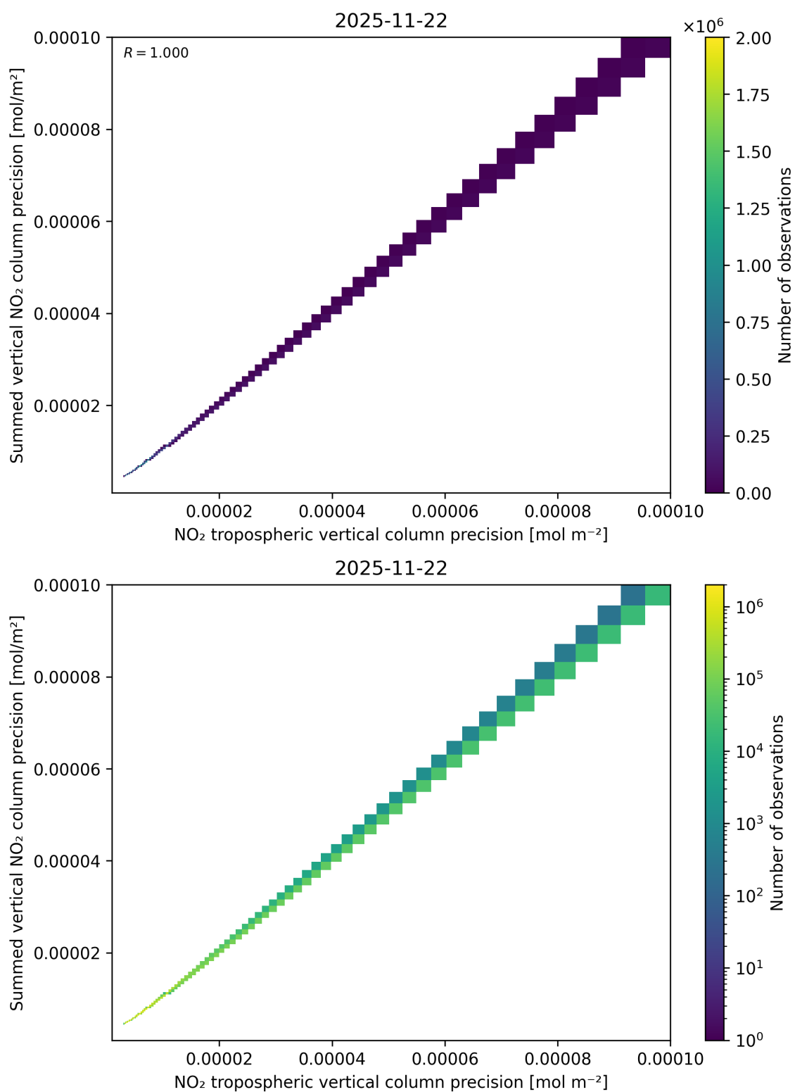
Figure 137: Scatter density plot of “NO 2 tropospheric vertical column precision” against “Summed vertical NO 2 column precision” for 2025-11-21 to 2025-11-23.
