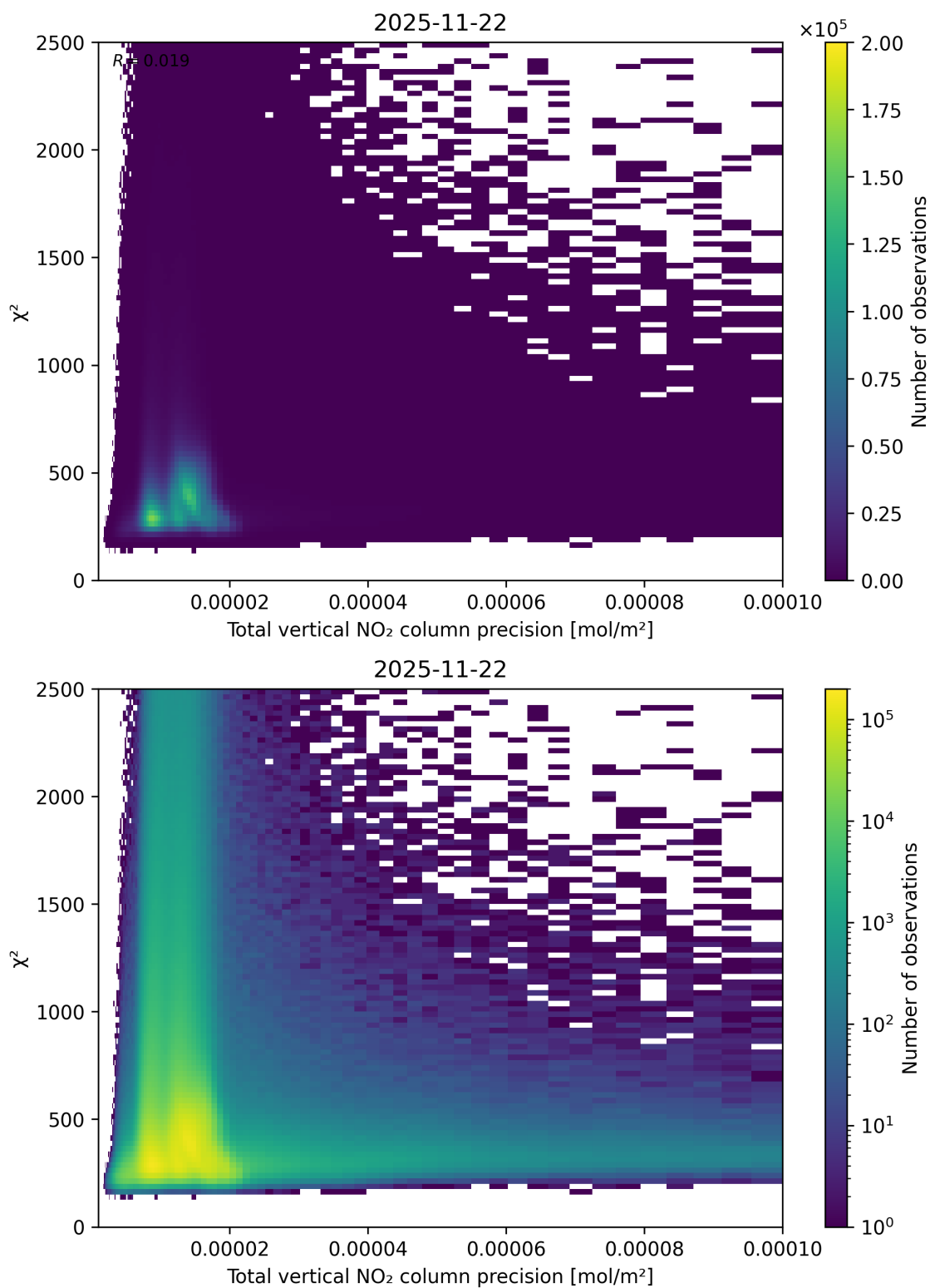
Figure 116: Scatter density plot of “Total vertical NO 2 column precision” against “ \chi^2 ” for 2025-11-21 to 2025-11-23.
