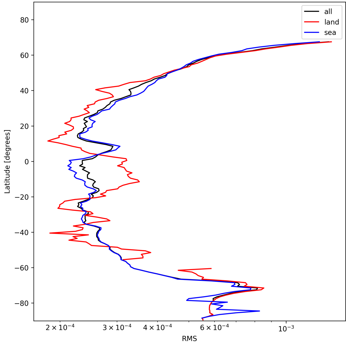
Figure 26: Zonal average of “RMS” for 2025-11-21 to 2025-11-23.
