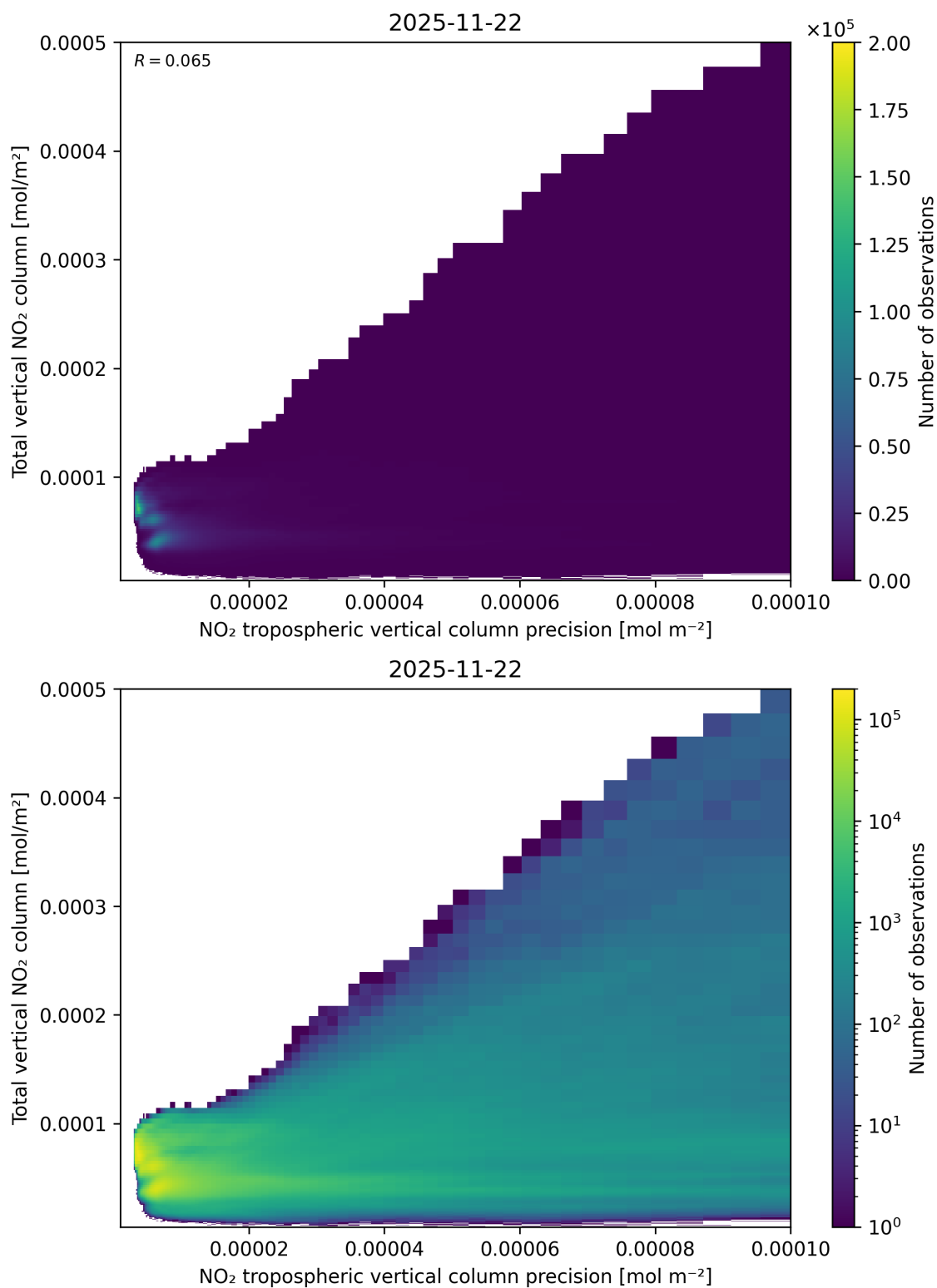
Figure 138: Scatter density plot of “NO 2 tropospheric vertical column precision” against “Total vertical NO 2 column” for 2025-11-21 to 2025-11-23.
