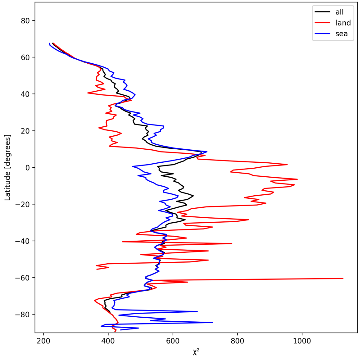
Figure 25: Zonal average of “ \chi^2 ” for 2025-11-21 to 2025-11-23.
