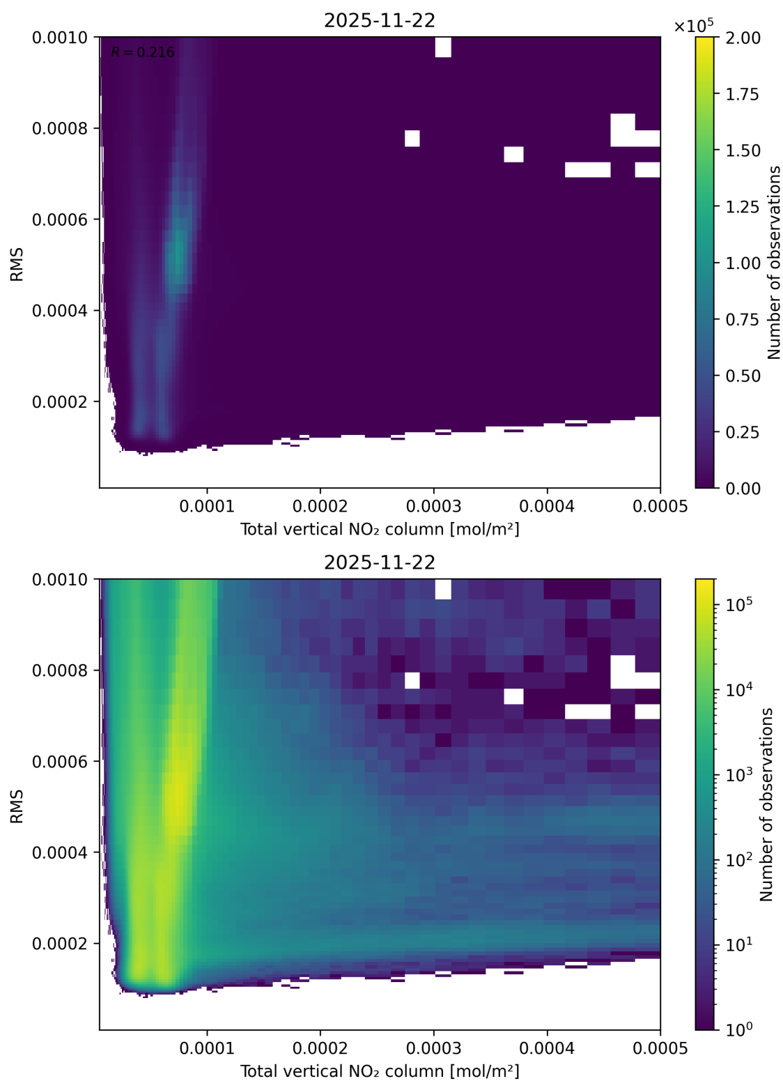
Figure 120: Scatter density plot of “Total vertical NO 2 column” against “RMS” for 2025-11-21 to 2025-11-23.
