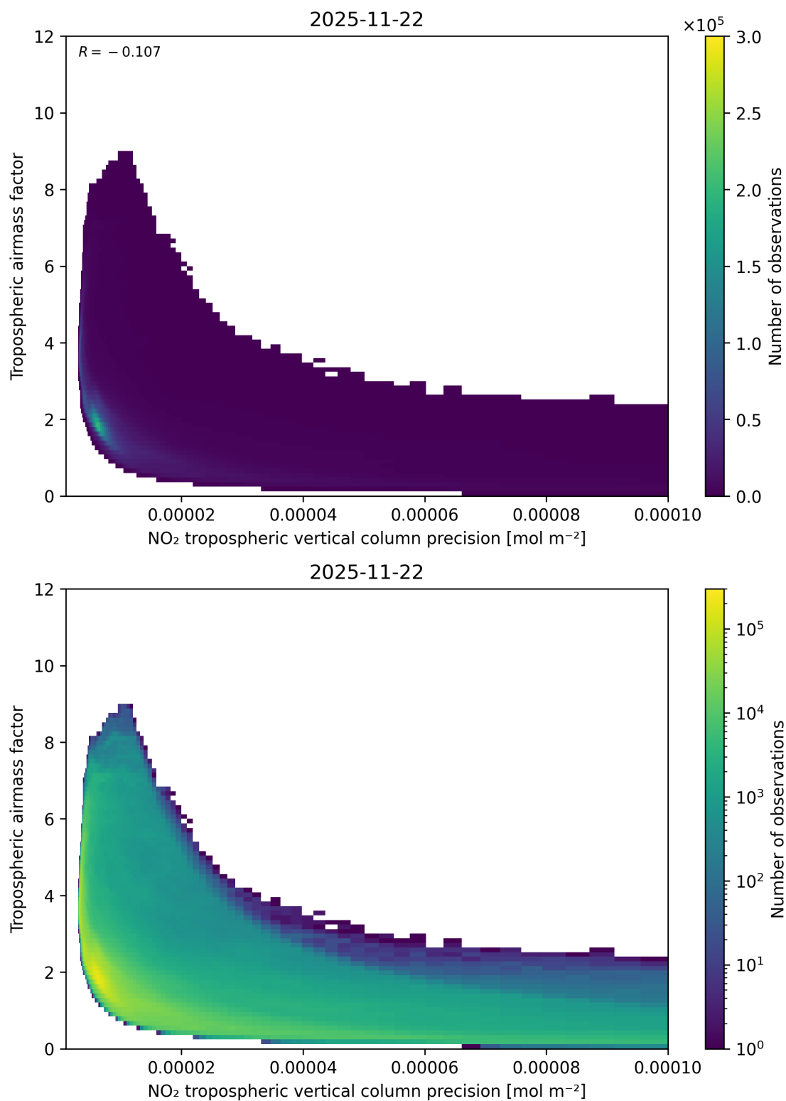
Figure 133: Scatter density plot of “NO 2 tropospheric vertical column precision” against “Tropospheric airmass factor” for 2025-11-21 to 2025-11-23.
