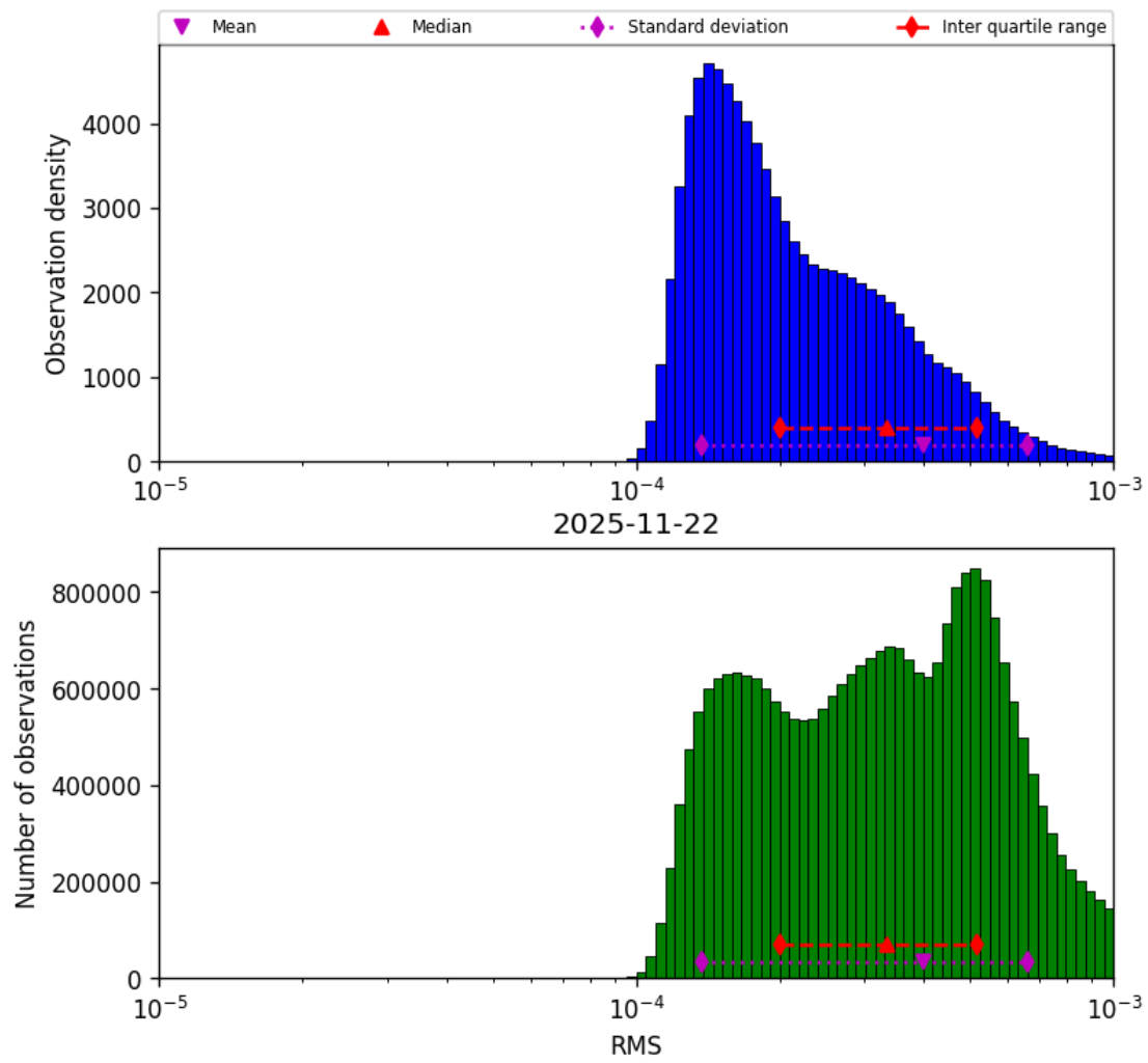
Figure 43: Histogram of “RMS” for 2025-11-21 to 2025-11-23
