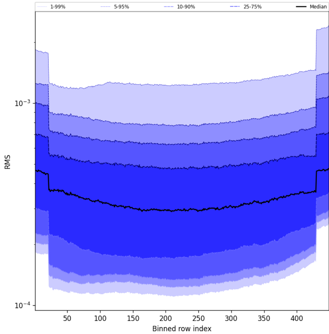
Figure 60: Along track statistics of “RMS” for 2025-11-21 to 2025-11-23
