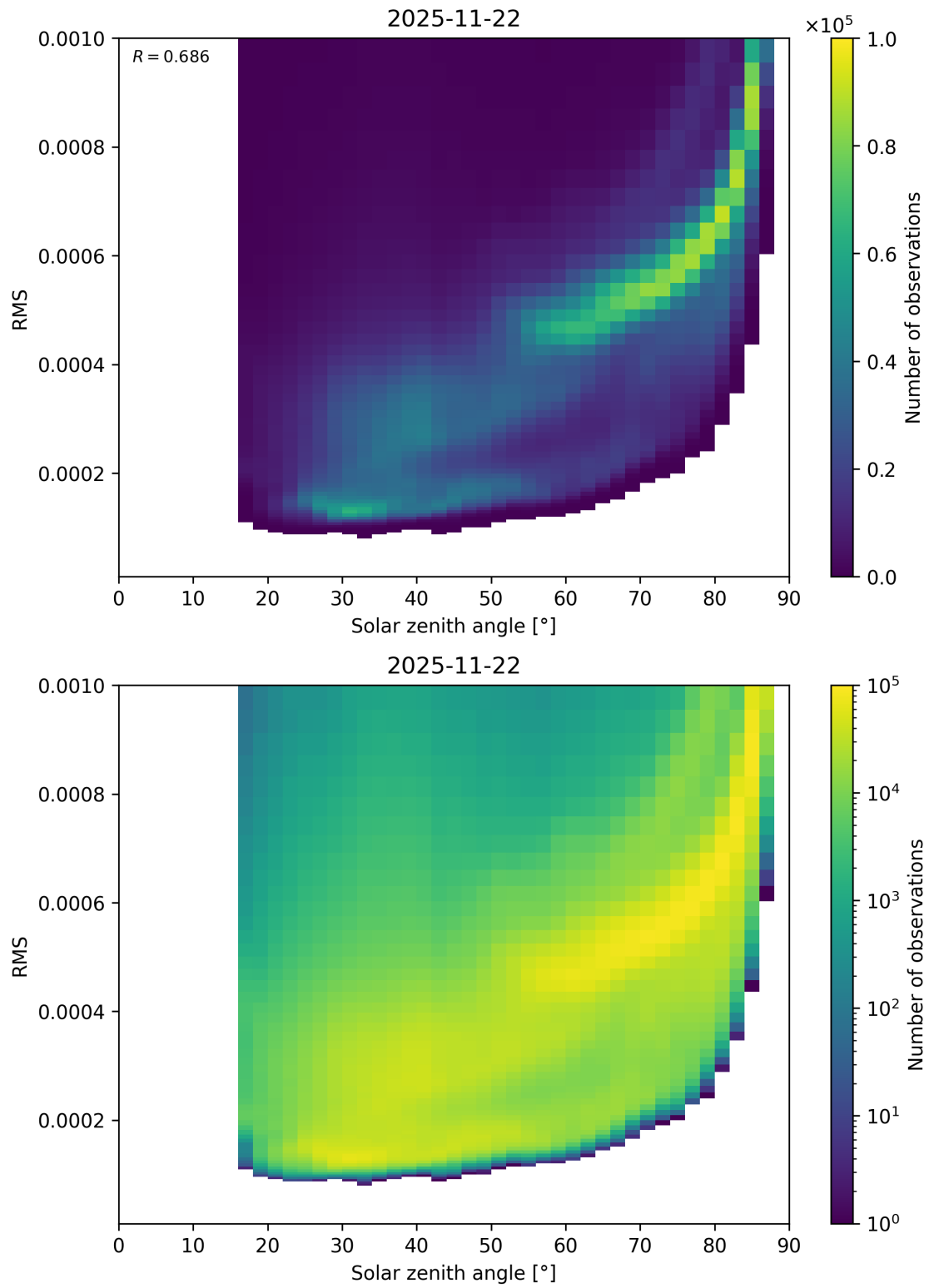
Figure 157: Scatter density plot of “Solar zenith angle” against “RMS” for 2025-11-21 to 2025-11-23.
