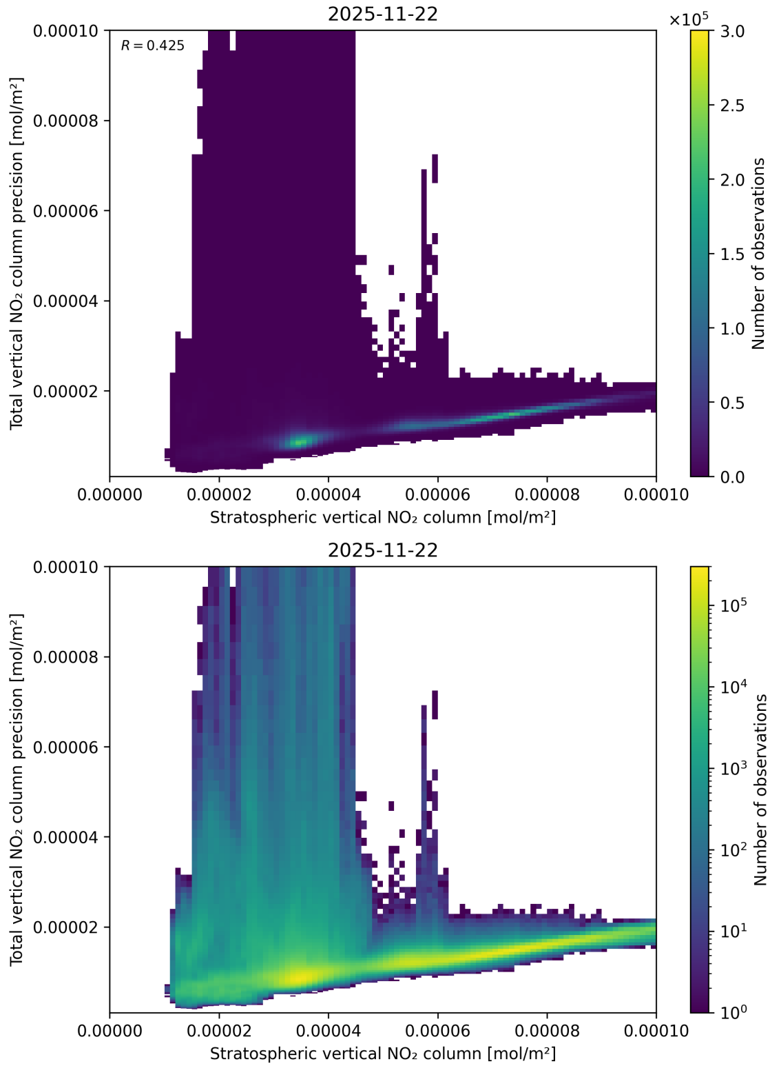
Figure 101: Scatter density plot of “Stratospheric vertical NO 2 column” against “Total vertical NO 2 column precision” for 2025-11-21 to 2025-11-23.
