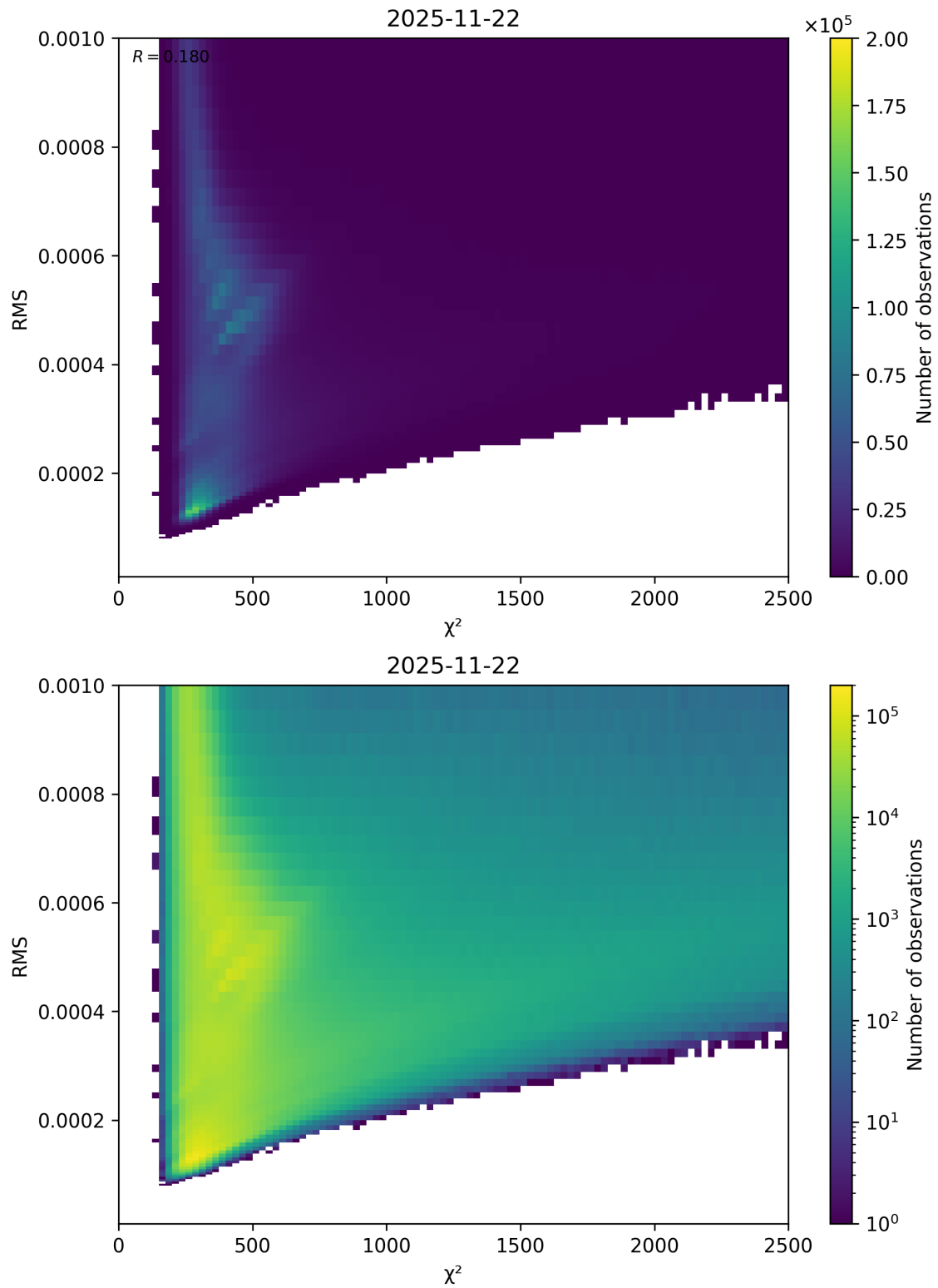
Figure 82: Scatter density plot of “ \chi^2 ” against “RMS” for 2025-11-21 to 2025-11-23.
