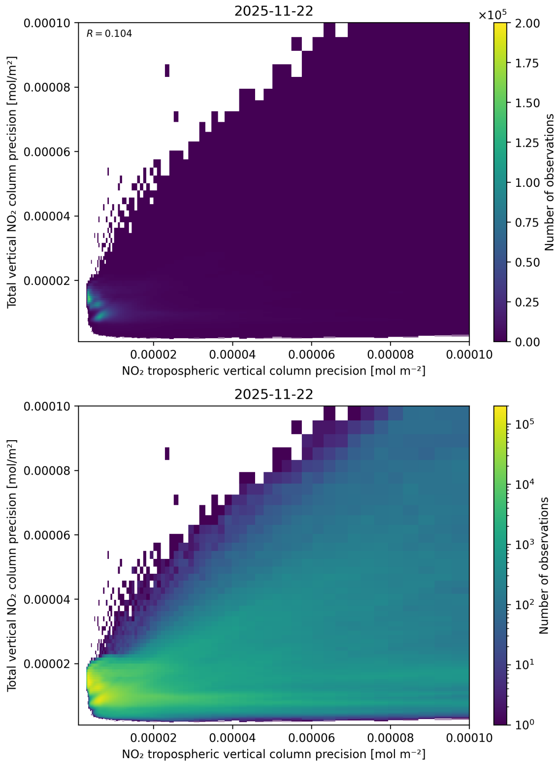
Figure 139: Scatter density plot of “NO 2 tropospheric vertical column precision” against “Total vertical NO 2 column precision” for 2025-11-21 to 2025-11-23.
