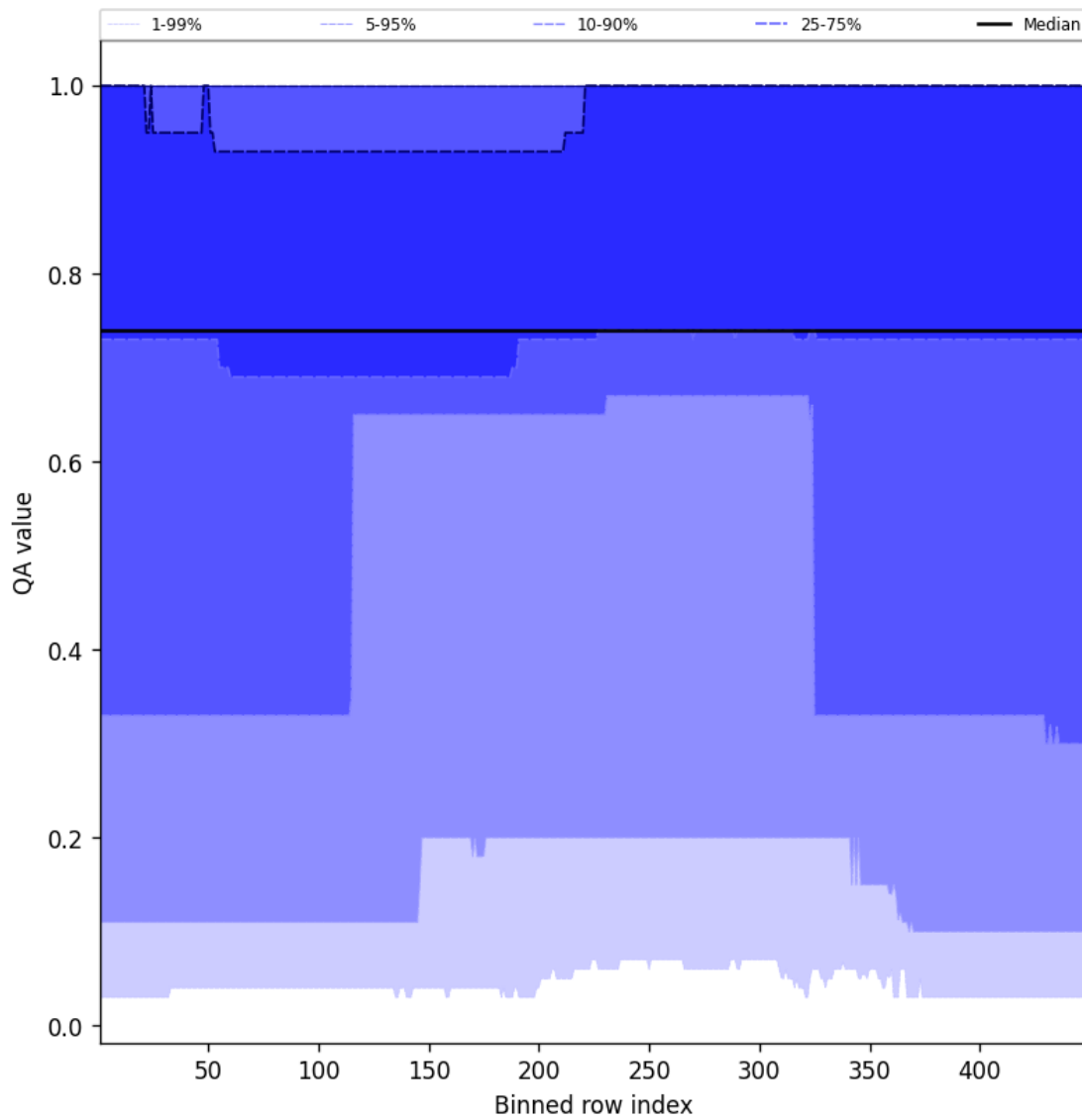
Figure 45: Along track statistics of “QA value” for 2025-11-21 to 2025-11-23
