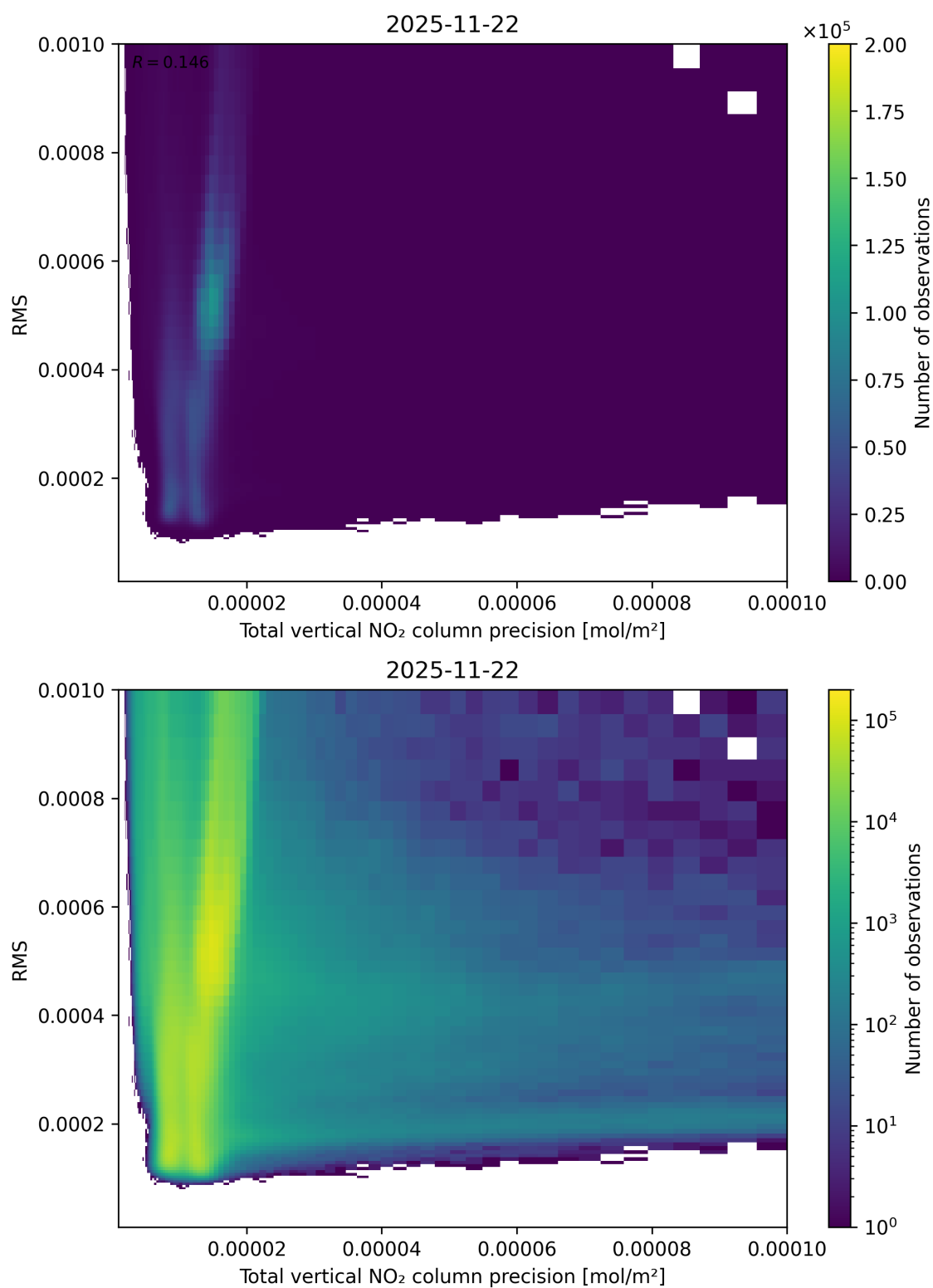
Figure 119: Scatter density plot of “Total vertical NO 2 column precision” against “RMS” for 2025-11-21 to 2025-11-23.
