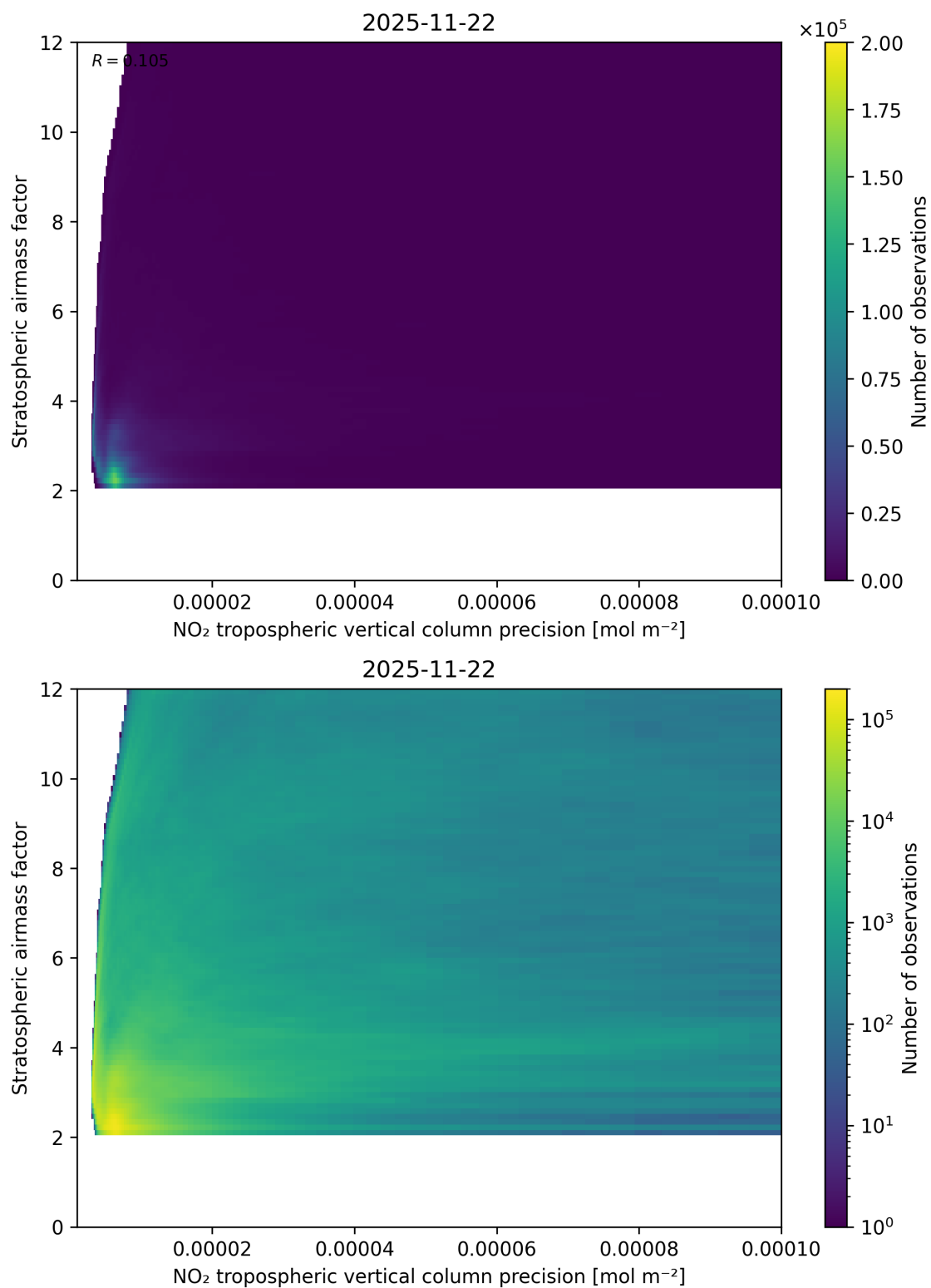
Figure 131: Scatter density plot of “NO 2 tropospheric vertical column precision” against “Stratospheric airmass factor” for 2025-11-21 to 2025-11-23.
