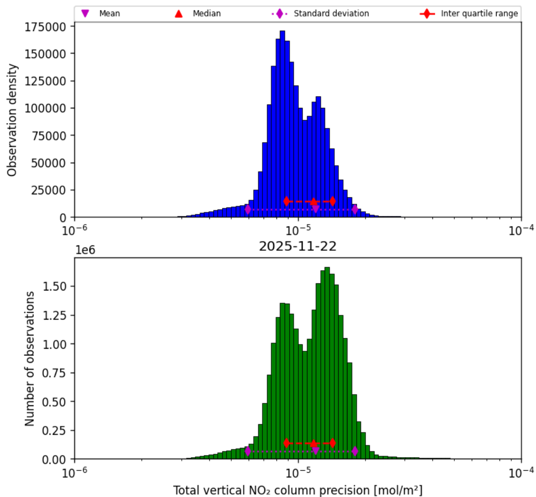
Figure 39: Histogram of “Total vertical NO 2 column precision” for 2025-11-21 to 2025-11-23
