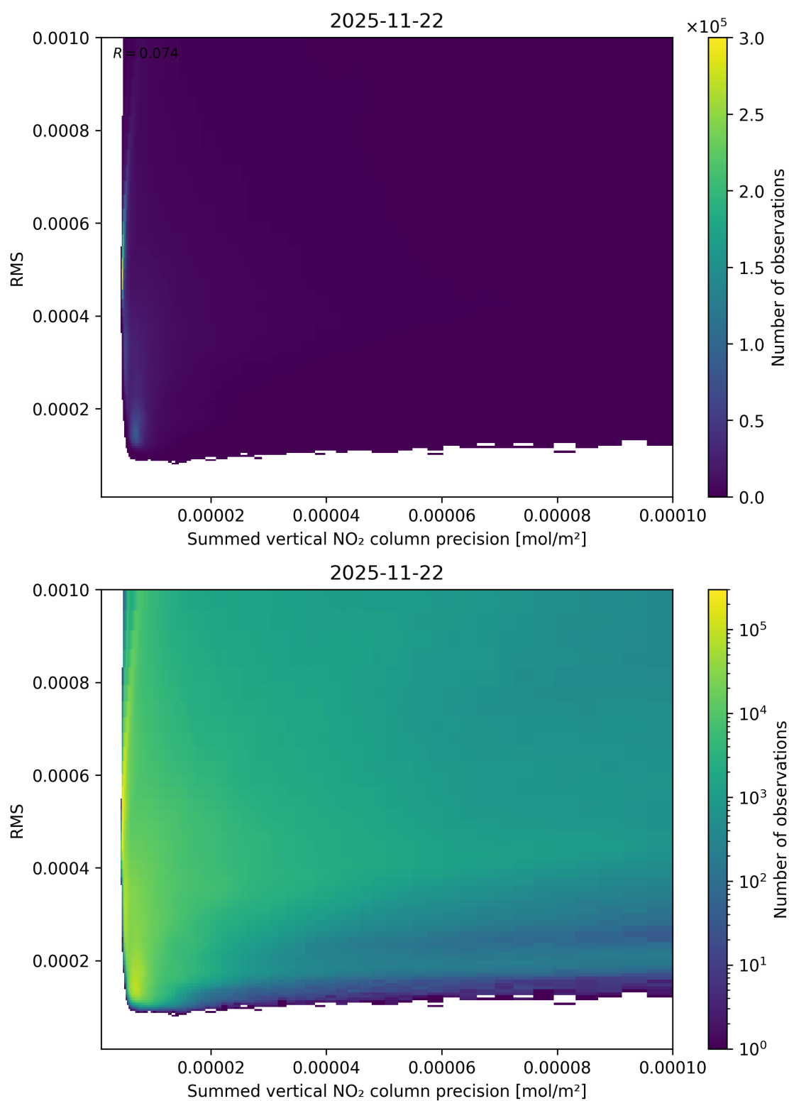
Figure 108: Scatter density plot of “Summed vertical NO 2 column precision” against “RMS” for 2025-11-21 to 2025-11-23.
