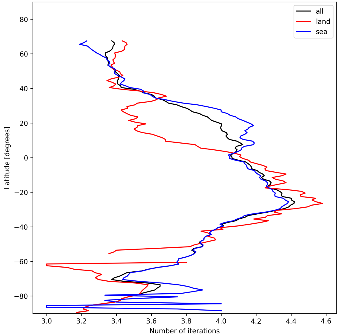
Figure 17: Zonal average of “Number of iterations” for 2025-11-21 to 2025-11-23.
