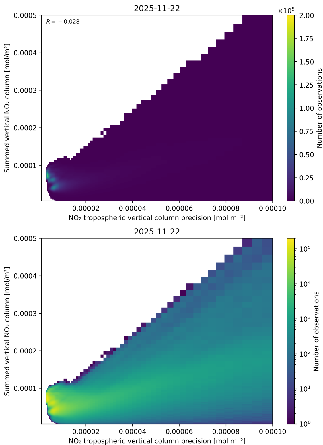
Figure 136: Scatter density plot of “NO 2 tropospheric vertical column precision” against “Summed vertical NO 2 column” for 2025-11-21 to 2025-11-23.
