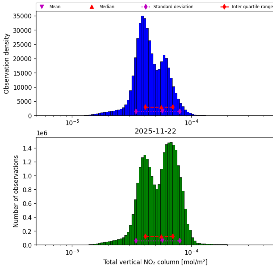
Figure 38: Histogram of “Total vertical NO 2 column” for 2025-11-21 to 2025-11-23
