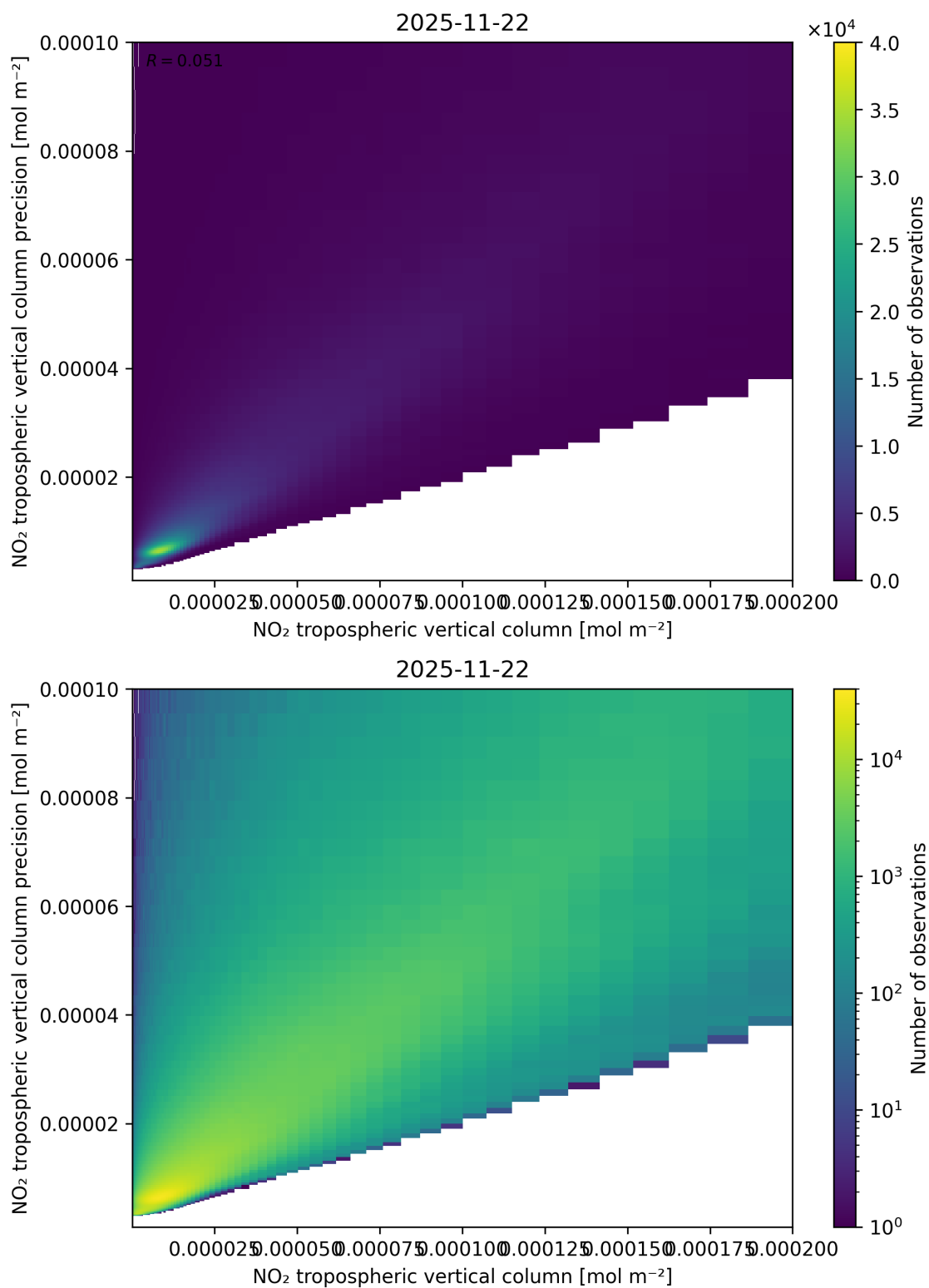
Figure 130: Scatter density plot of “NO 2 tropospheric vertical column” against “NO 2 tropospheric vertical column precision” for 2025-11-21 to 2025-11-23.
