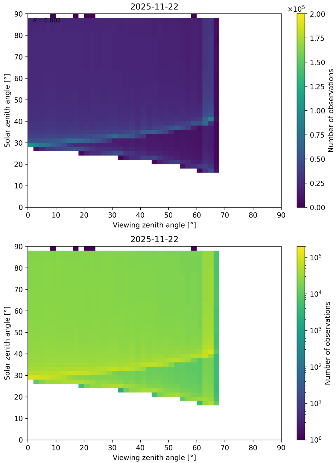
Figure 172: Scatter density plot of “Viewing zenith angle” against “Solar zenith angle” for 2025-11-21 to 2025-11-23.
