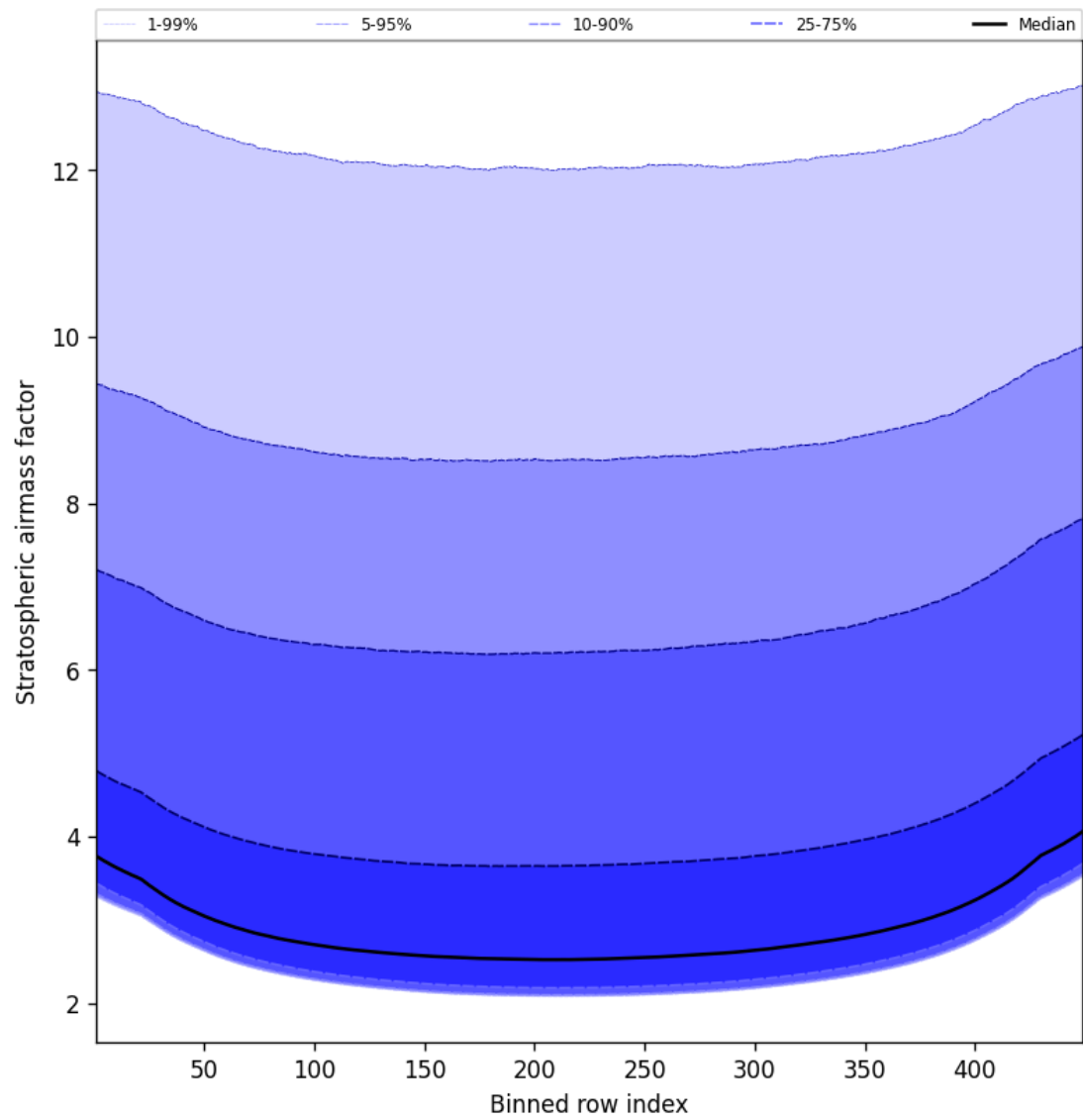
Figure 61: Along track statistics of “Stratospheric air mass factor” for 2025-11-21 to 2025-11-23
