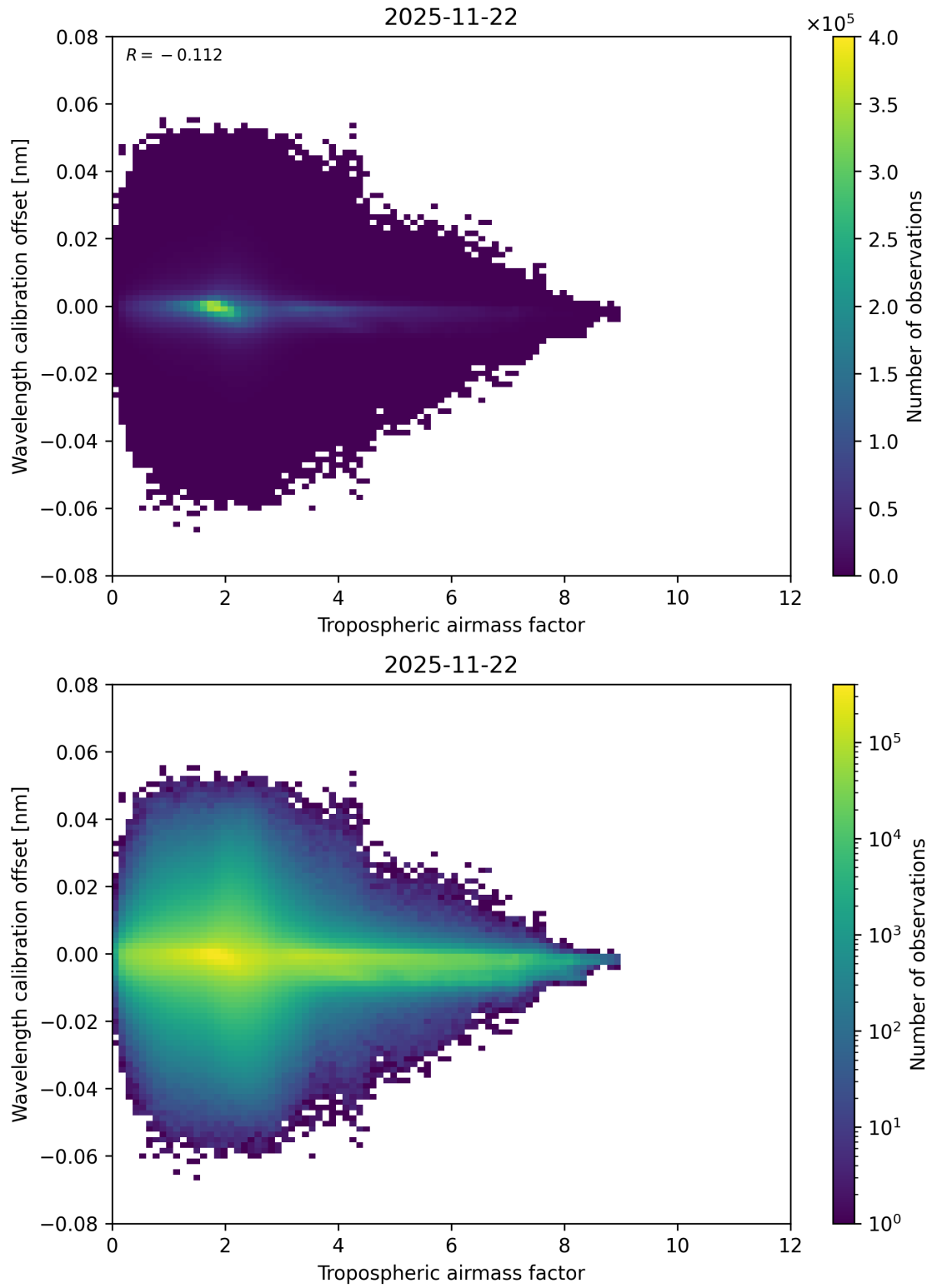
Figure 80: Scatter density plot of “Tropospheric airmass factor” against “Wavelength calibration offset” for 2025-11-21 to 2025-11-23.
