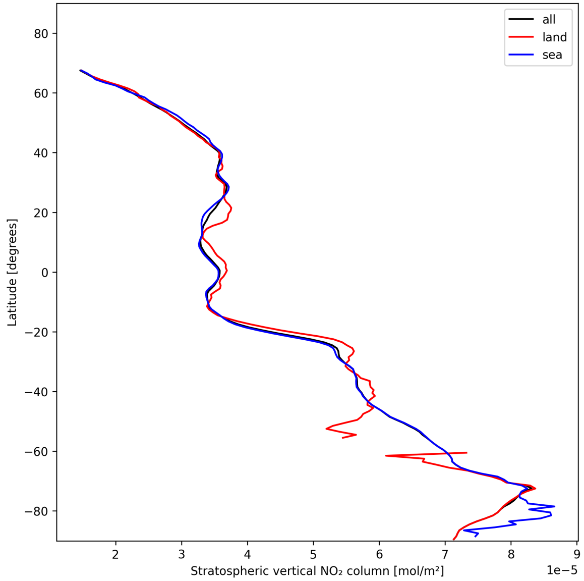
Figure 19: Zonal average of “Stratospheric vertical NO 2 column” for 2025-11-21 to 2025-11-23.
