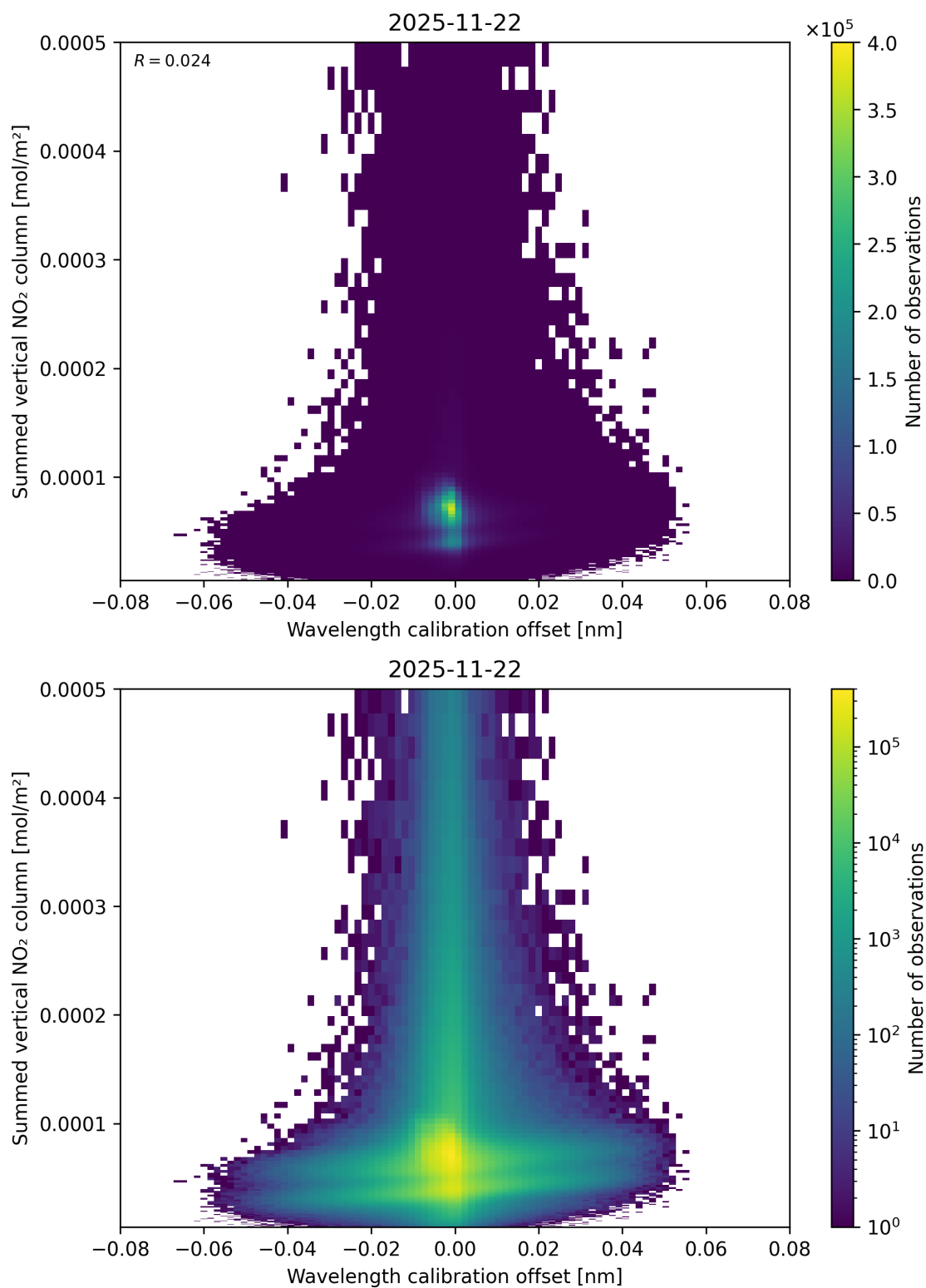
Figure 177: Scatter density plot of “Wavelength calibration offset” against “Summed vertical NO 2 column” for 2025-11-21 to 2025-11-23.
