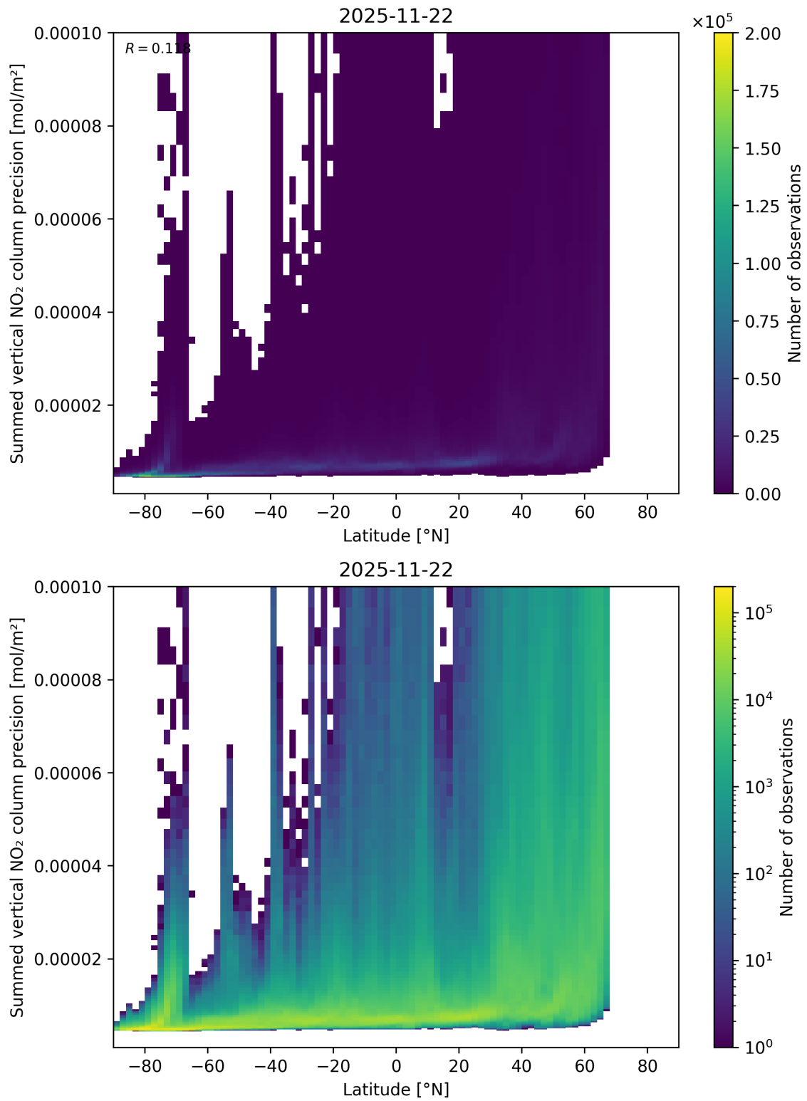
Figure 89: Scatter density plot of “Latitude” against “Summed vertical NO 2 column precision” for 2025-11-21 to 2025-11-23.
