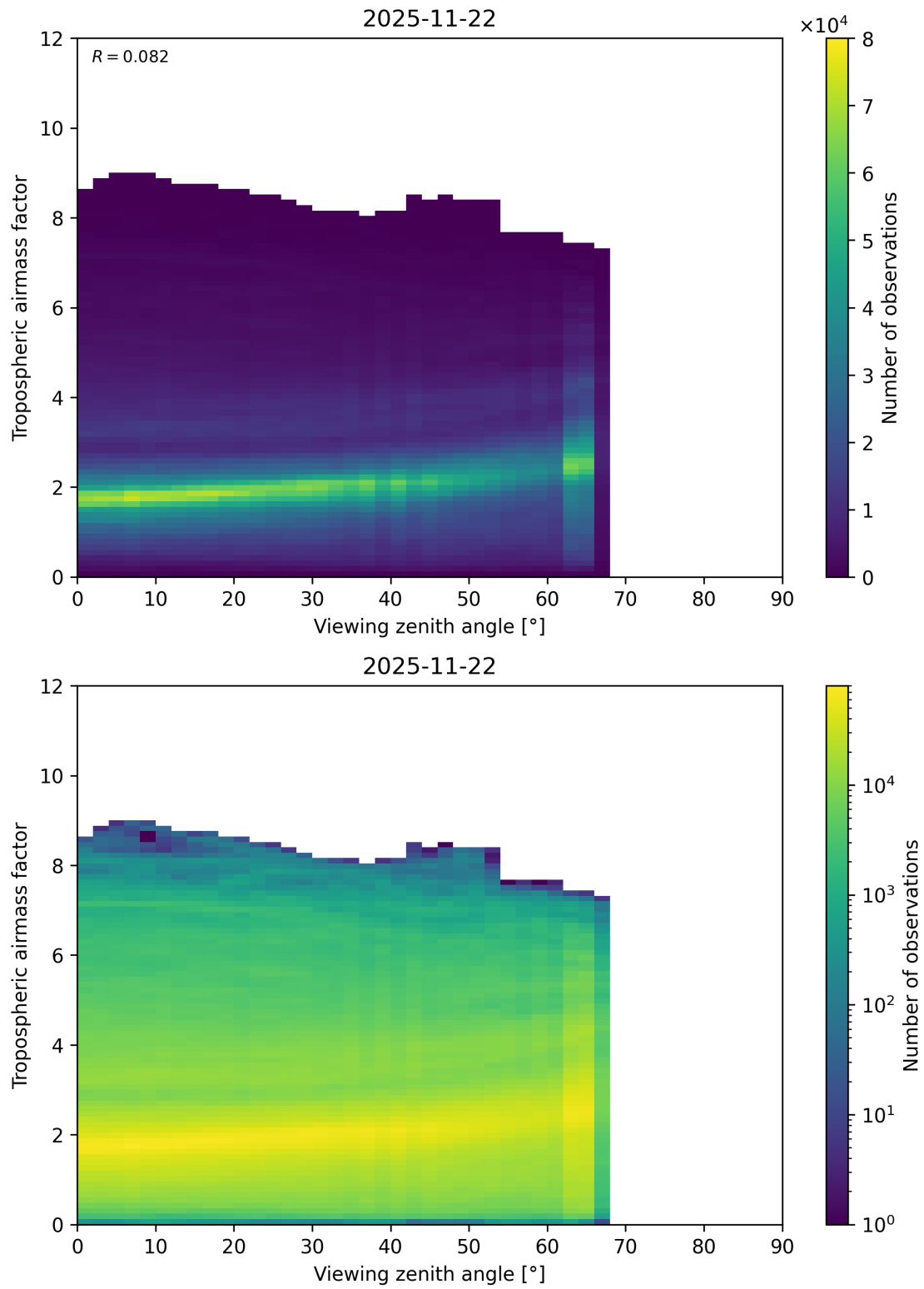
Figure 161: Scatter density plot of “Viewing zenith angle” against “Tropospheric airmass factor” for 2025-11-21 to 2025-11-23.
