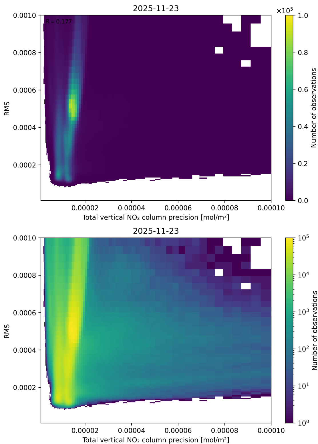
Figure 119: Scatter density plot of “Total vertical NO 2 column precision” against “RMS” for 2025-11-23 to 2025-11-24.
