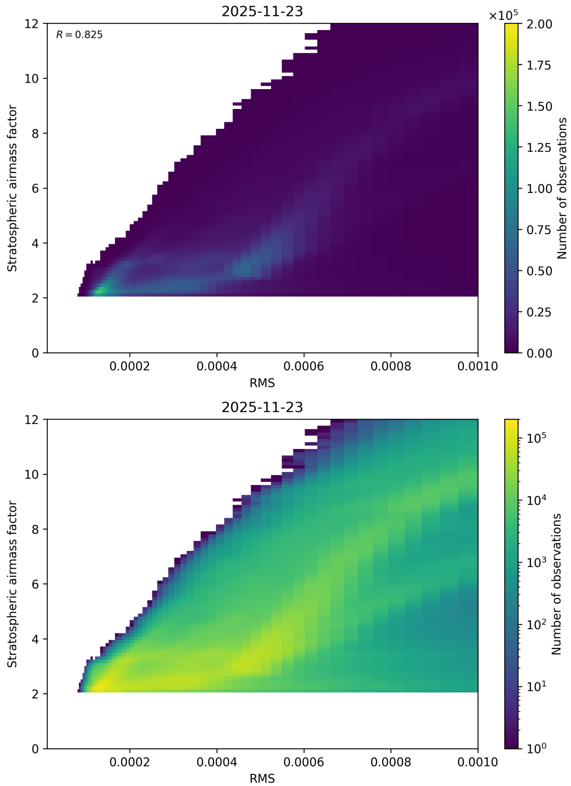
Figure 144: Scatter density plot of “RMS” against “Stratospheric airmass factor” for 2025-11-23 to 2025-11-24.
