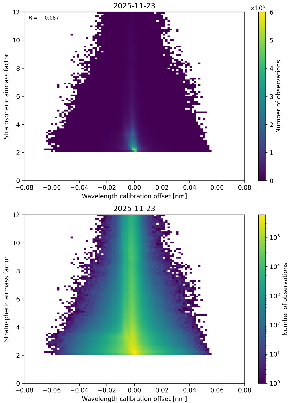
Figure 174: Scatter density plot of “Wavelength calibration offset” against “Stratospheric airmass factor” for 2025-11-23 to 2025-11-24.
