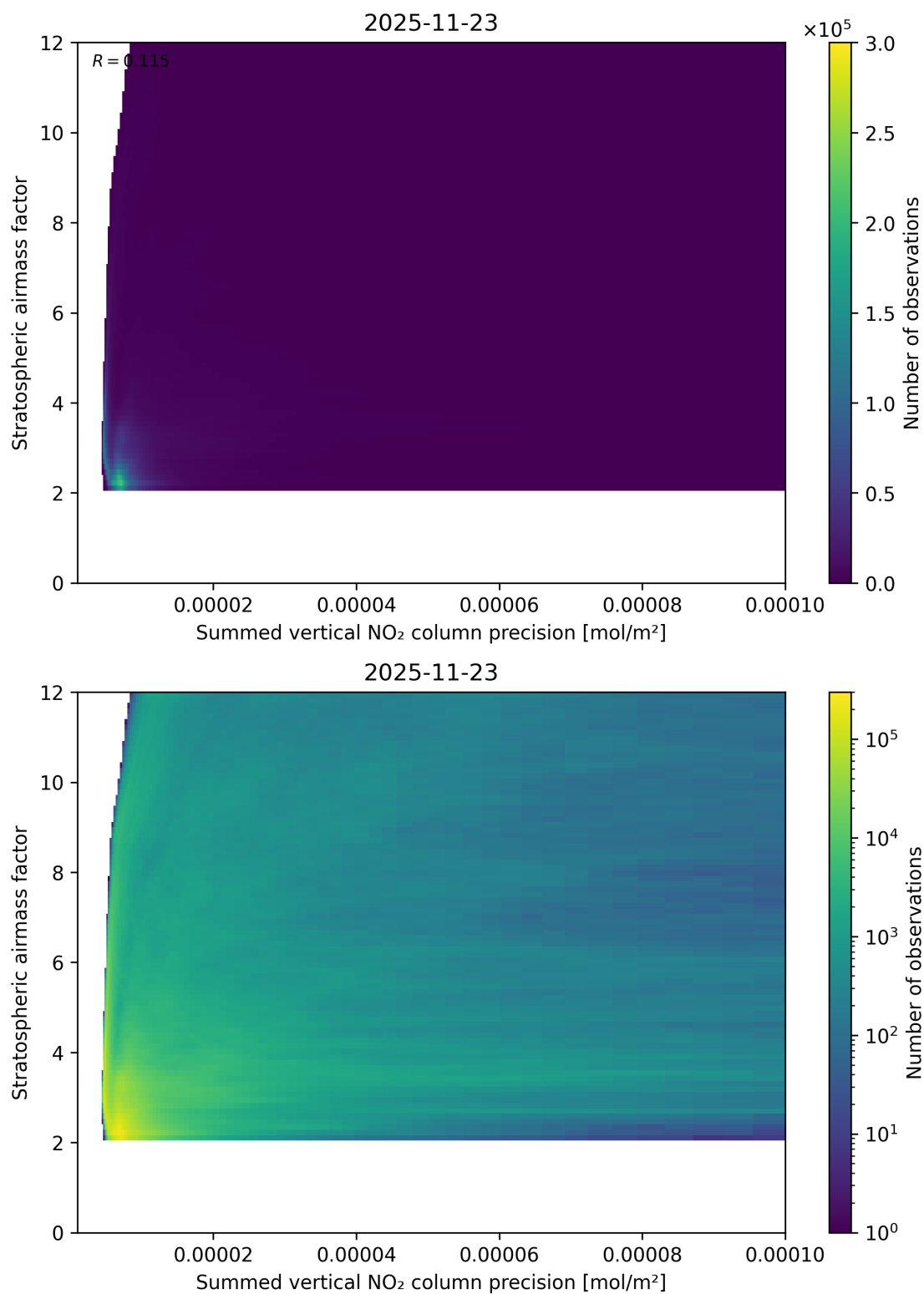
Figure 106: Scatter density plot of “Summed vertical NO 2 column precision” against “Stratospheric airmass factor” for 2025-11-23 to 2025-11-24.
