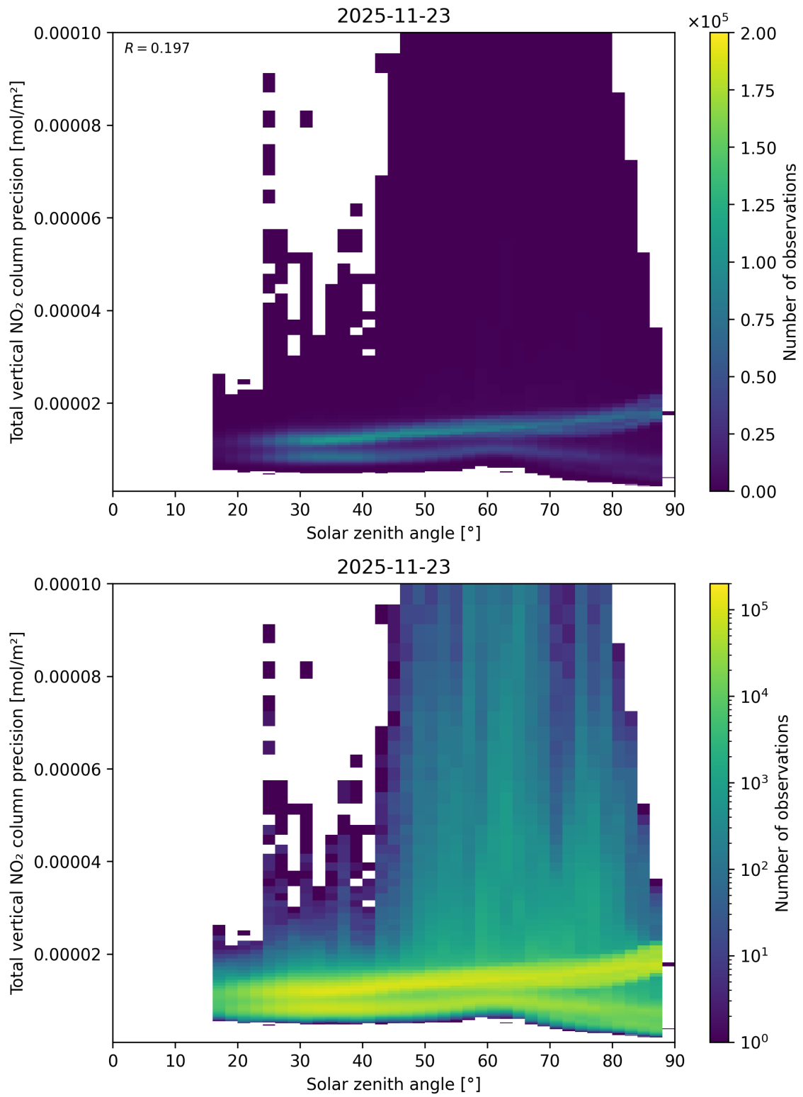
Figure 154: Scatter density plot of “Solar zenith angle” against “Total vertical NO 2 column precision” for 2025-11-23 to 2025-11-24.
