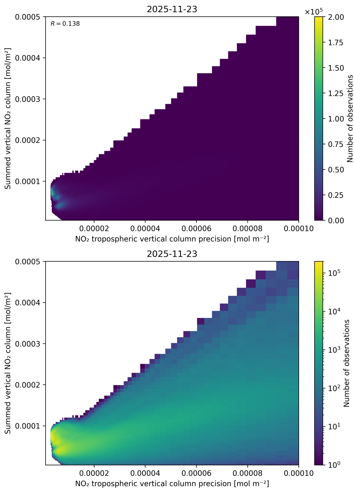
Figure 136: Scatter density plot of “NO 2 tropospheric vertical column precision” against “Summed vertical NO 2 column” for 2025-11-23 to 2025-11-24.
