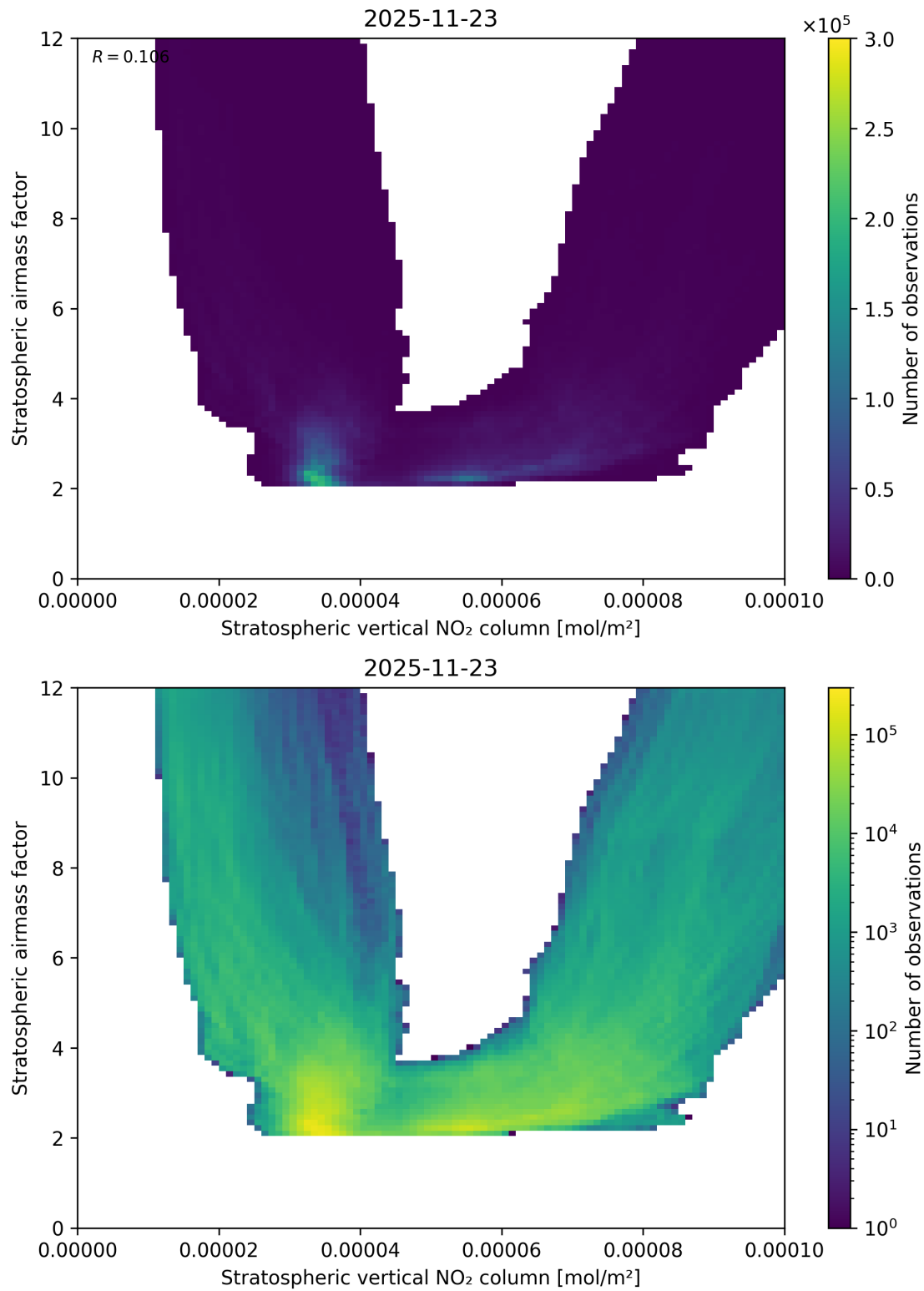
Figure 96: Scatter density plot of “Stratospheric vertical NO 2 column” against “Stratospheric airmass factor” for 2025-11-23 to 2025-11-24.
