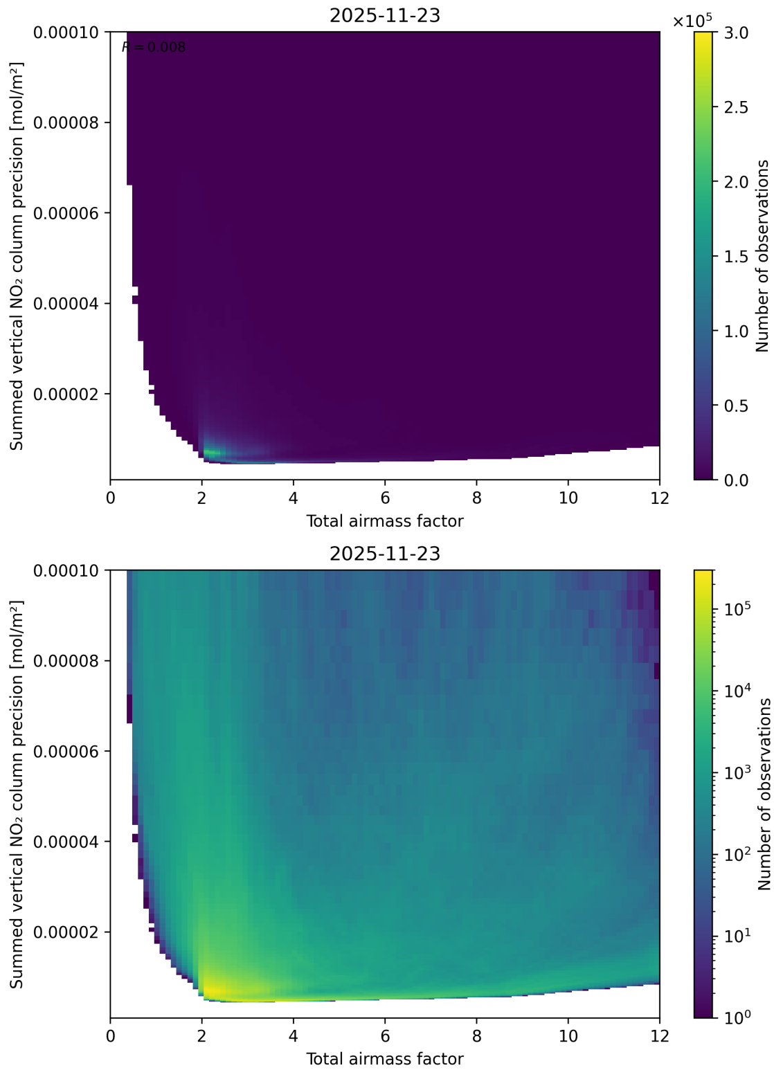
Figure 66: Scatter density plot of “Total airmass factor” against “Summed vertical NO 2 column precision” for 2025-11-23 to 2025-11-24.
