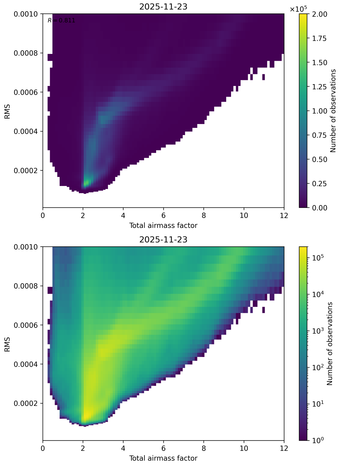
Figure 69: Scatter density plot of “Total airmass factor” against “RMS” for 2025-11-23 to 2025-11-24.
