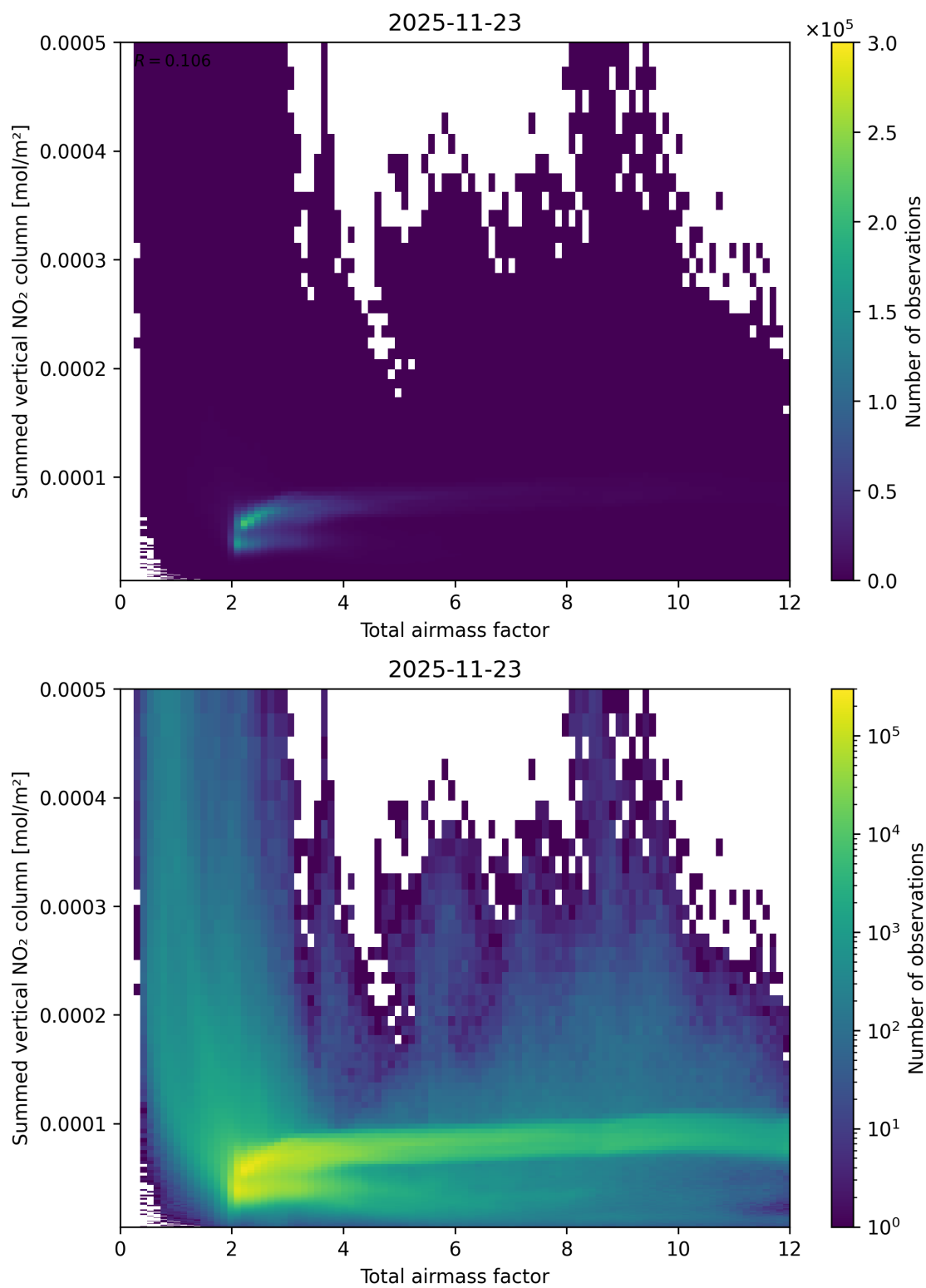
Figure 65: Scatter density plot of “Total airmass factor” against “Summed vertical NO 2 column” for 2025-11-23 to 2025-11-24.
