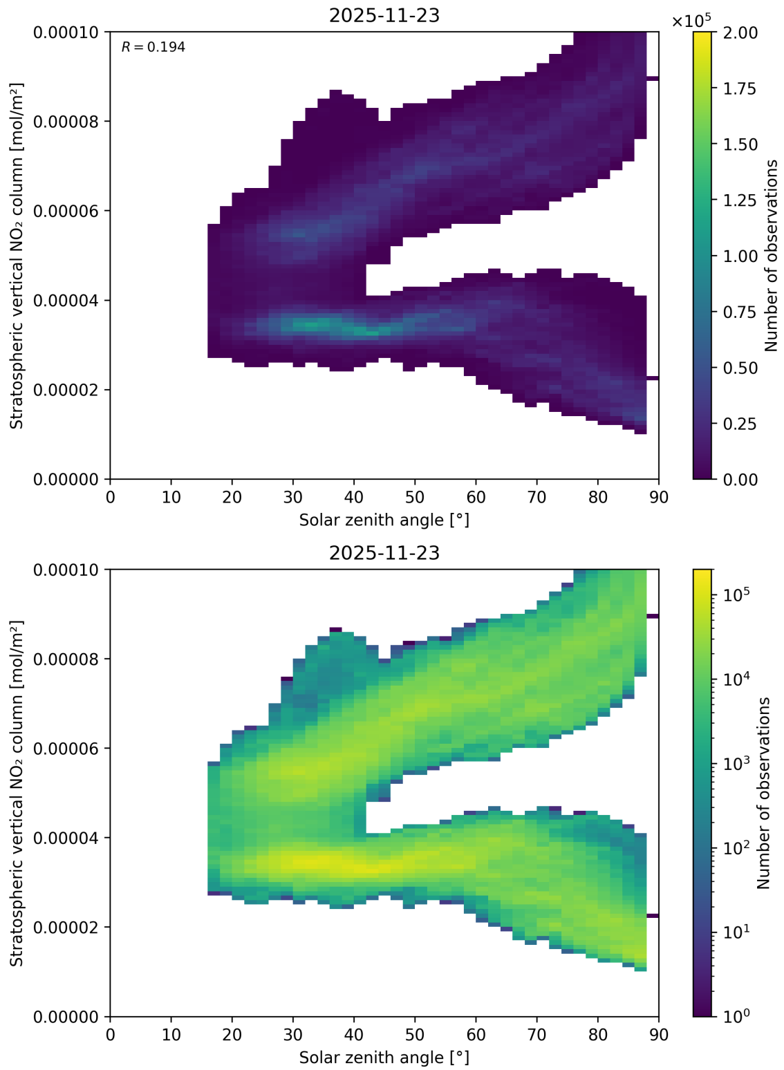
Figure 150: Scatter density plot of “Solar zenith angle” against “Stratospheric vertical NO 2 column” for 2025-11-23 to 2025-11-24.
