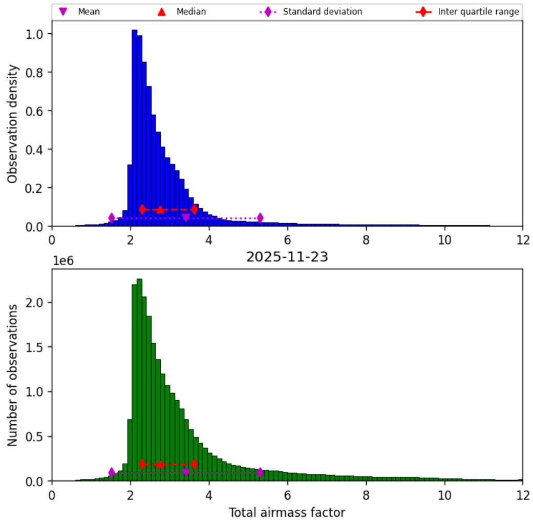
Figure 32: Histogram of “Total airmass factor” for 2025-11-23 to 2025-11-24
