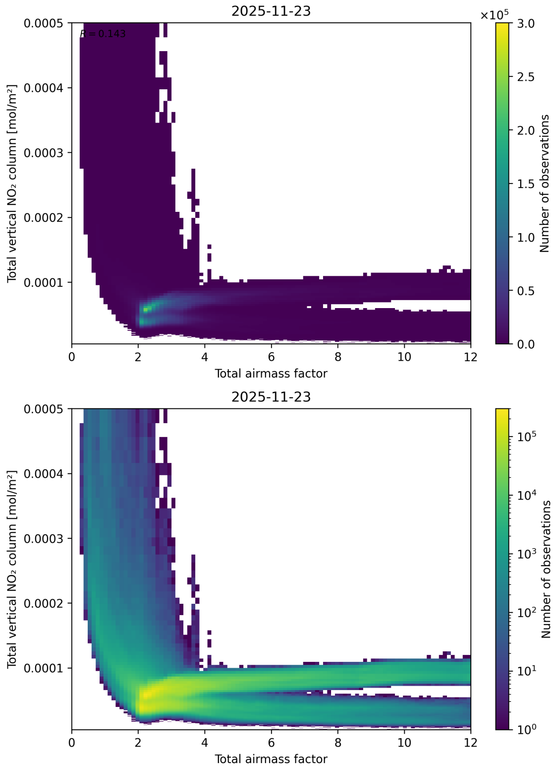
Figure 67: Scatter density plot of “Total airmass factor” against “Total vertical NO 2 column” for 2025-11-23 to 2025-11-24.
