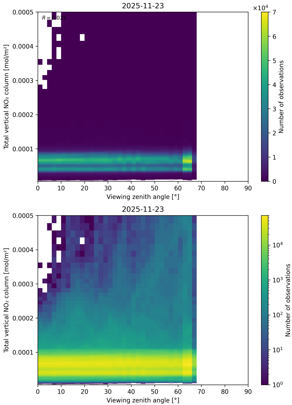
Figure 167: Scatter density plot of “Viewing zenith angle” against “Total vertical NO 2 column” for 2025-11-23 to 2025-11-24.
