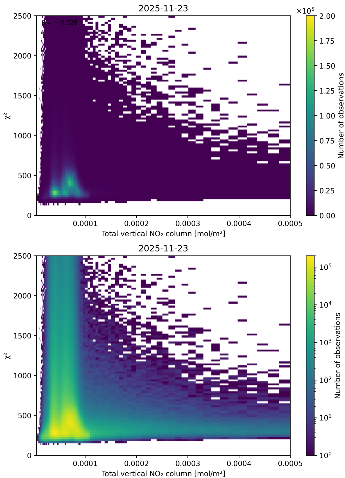
Figure 111: Scatter density plot of “Total vertical NO 2 column” against “ \chi^2 ” for 2025-11-23 to 2025-11-24.
