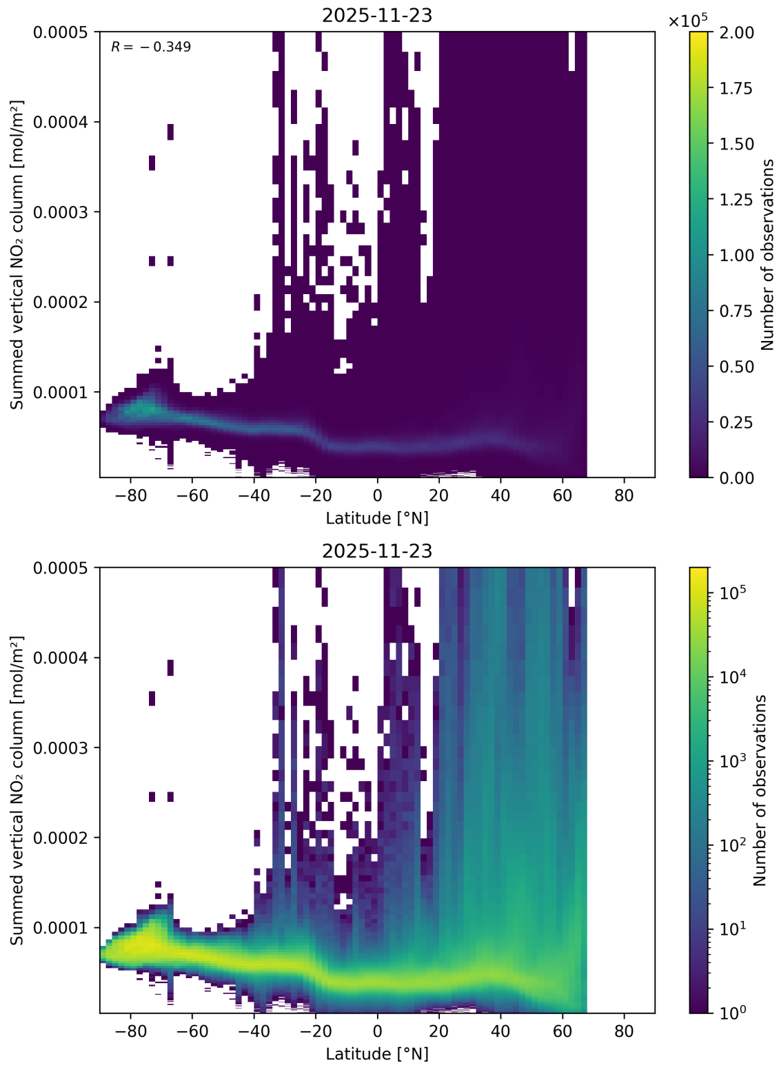
Figure 88: Scatter density plot of “Latitude” against “Summed vertical NO 2 column” for 2025-11-23 to 2025-11-24.
