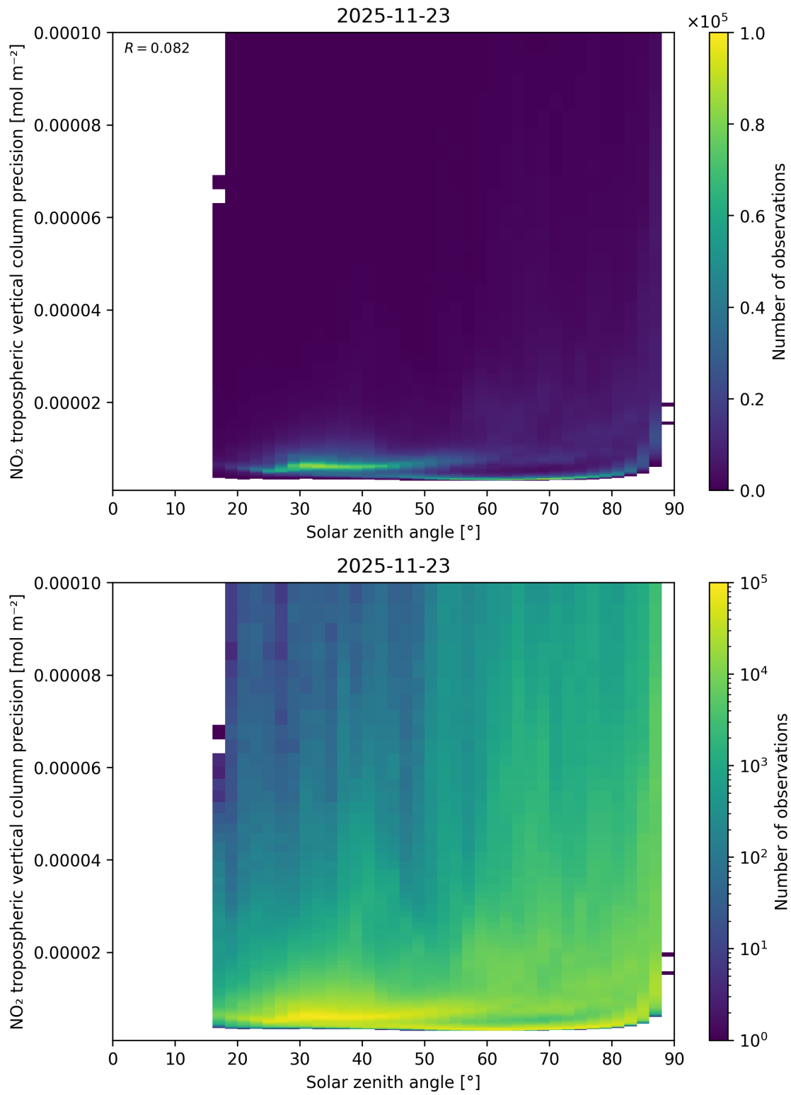
Figure 156: Scatter density plot of “Solar zenith angle” against “NO 2 tropospheric vertical column precision” for 2025-11-23 to 2025-11-24.
