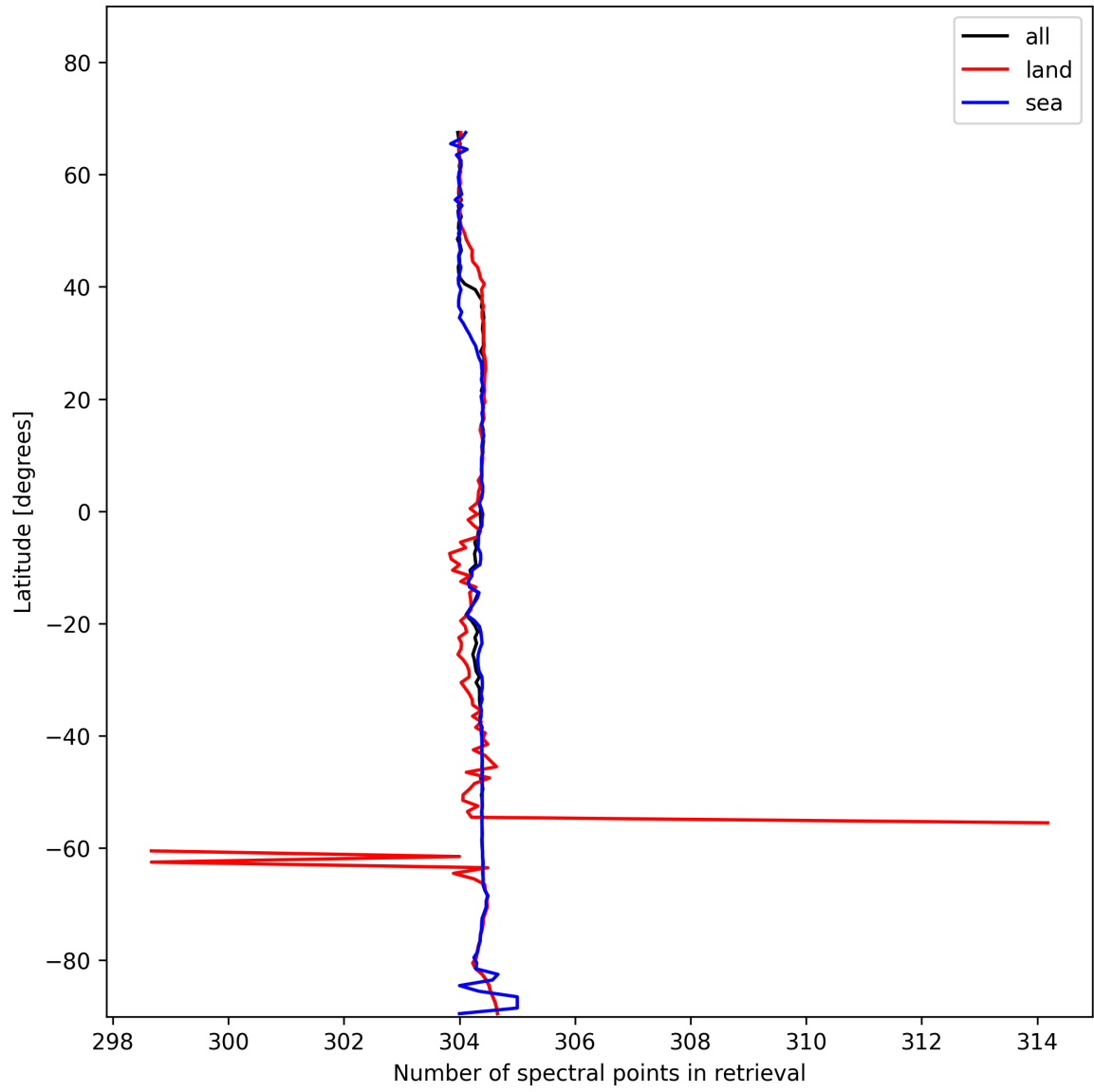
Figure 16: Zonal average of “Number of spectral points in retrieval” for 2025-11-23 to 2025-11-24.
