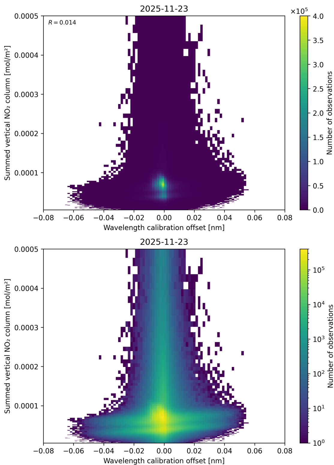
Figure 177: Scatter density plot of “Wavelength calibration offset” against “Summed vertical NO 2 column” for 2025-11-23 to 2025-11-24.
