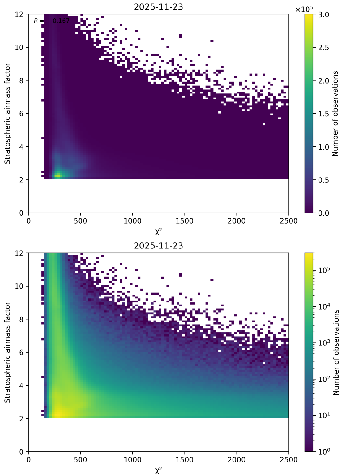
Figure 81: Scatter density plot of “ \chi^2 ” against “Stratospheric airmass factor” for 2025-11-23 to 2025-11-24.
