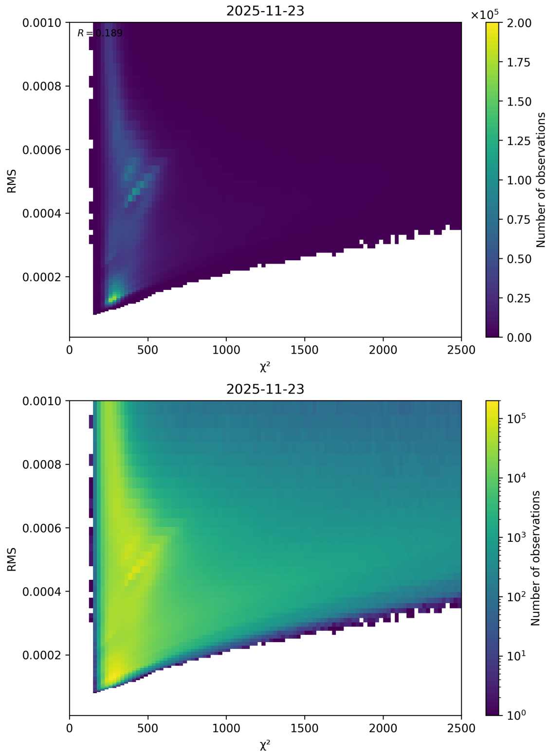
Figure 82: Scatter density plot of “ \chi^2 ” against “RMS” for 2025-11-23 to 2025-11-24.
