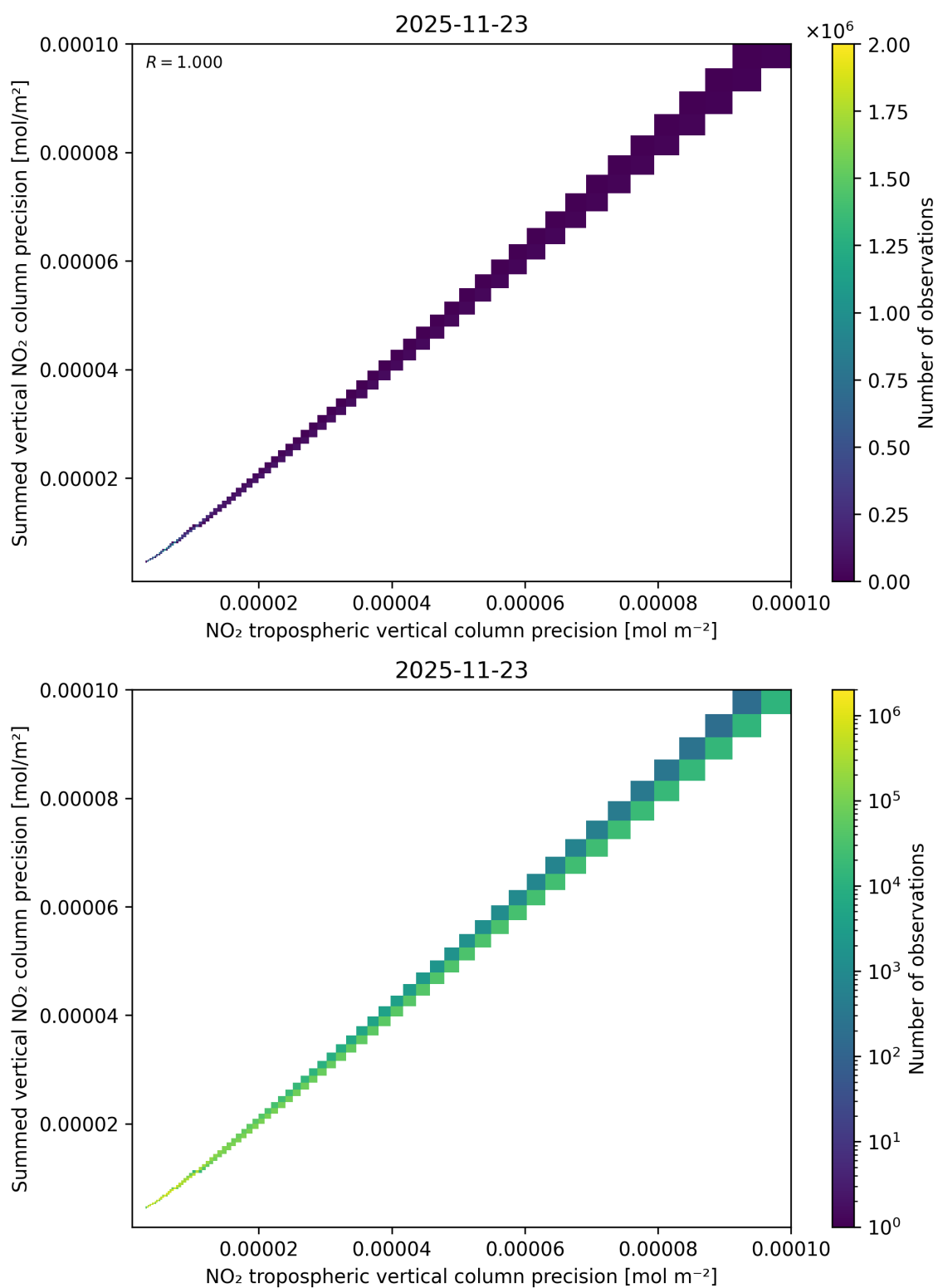
Figure 137: Scatter density plot of “NO 2 tropospheric vertical column precision” against “Summed vertical NO 2 column precision” for 2025-11-23 to 2025-11-24.
