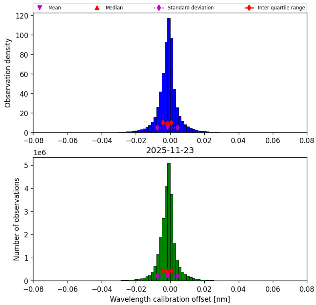
Figure 35: Histogram of “Wavelength calibration offset” for 2025-11-23 to 2025-11-24
