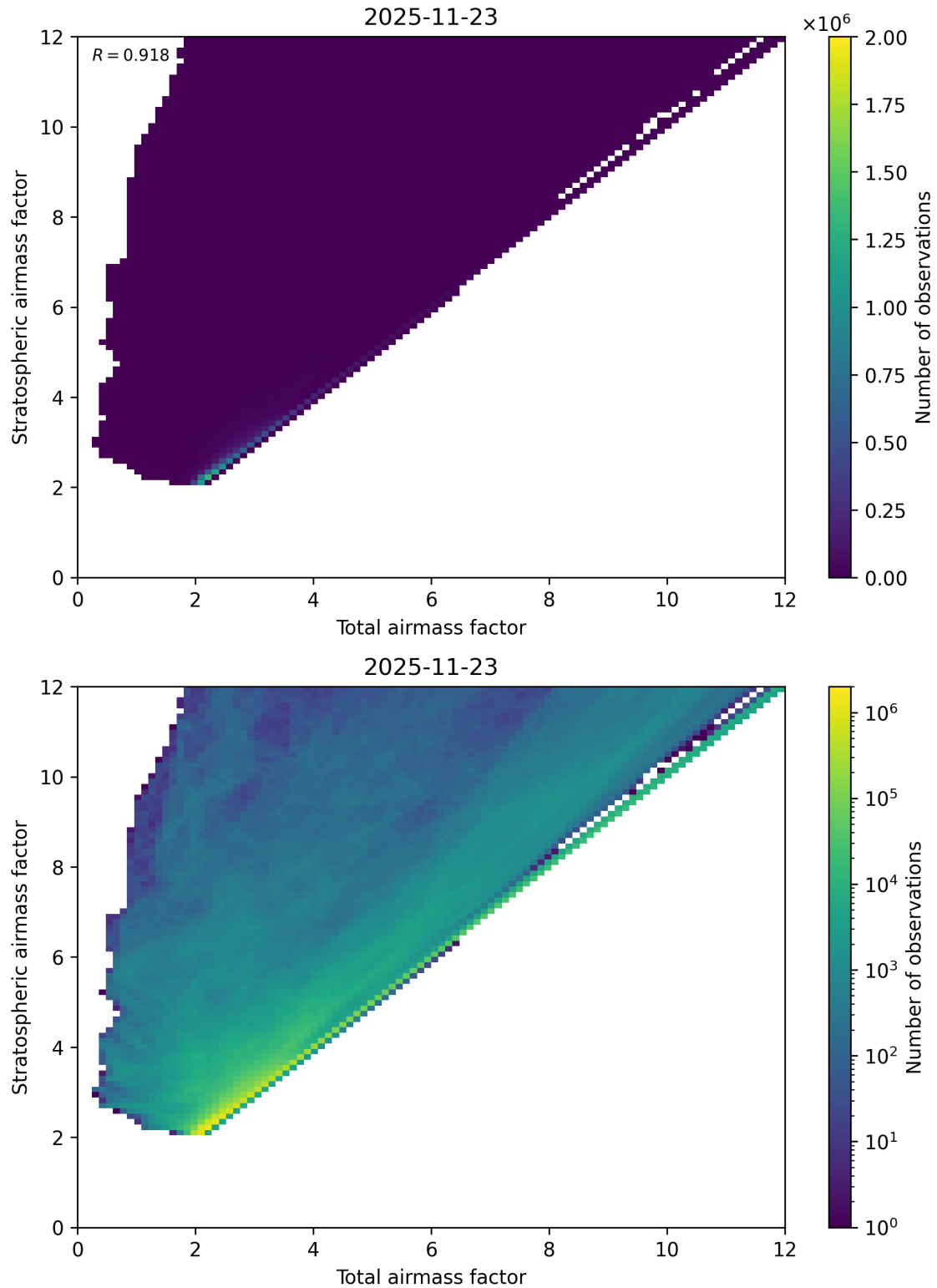
Figure 62: Scatter density plot of “Total airmass factor” against “Stratospheric airmass factor” for 2025-11-23 to 2025-11-24.
