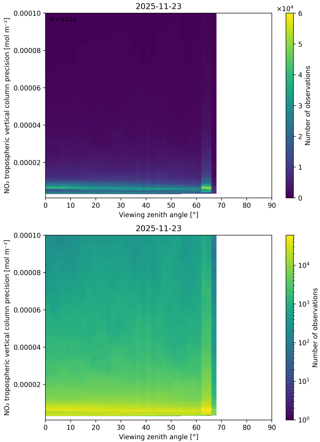
Figure 170: Scatter density plot of “Viewing zenith angle” against “NO 2 tropospheric vertical column precision” for 2025-11-23 to 2025-11-24.
