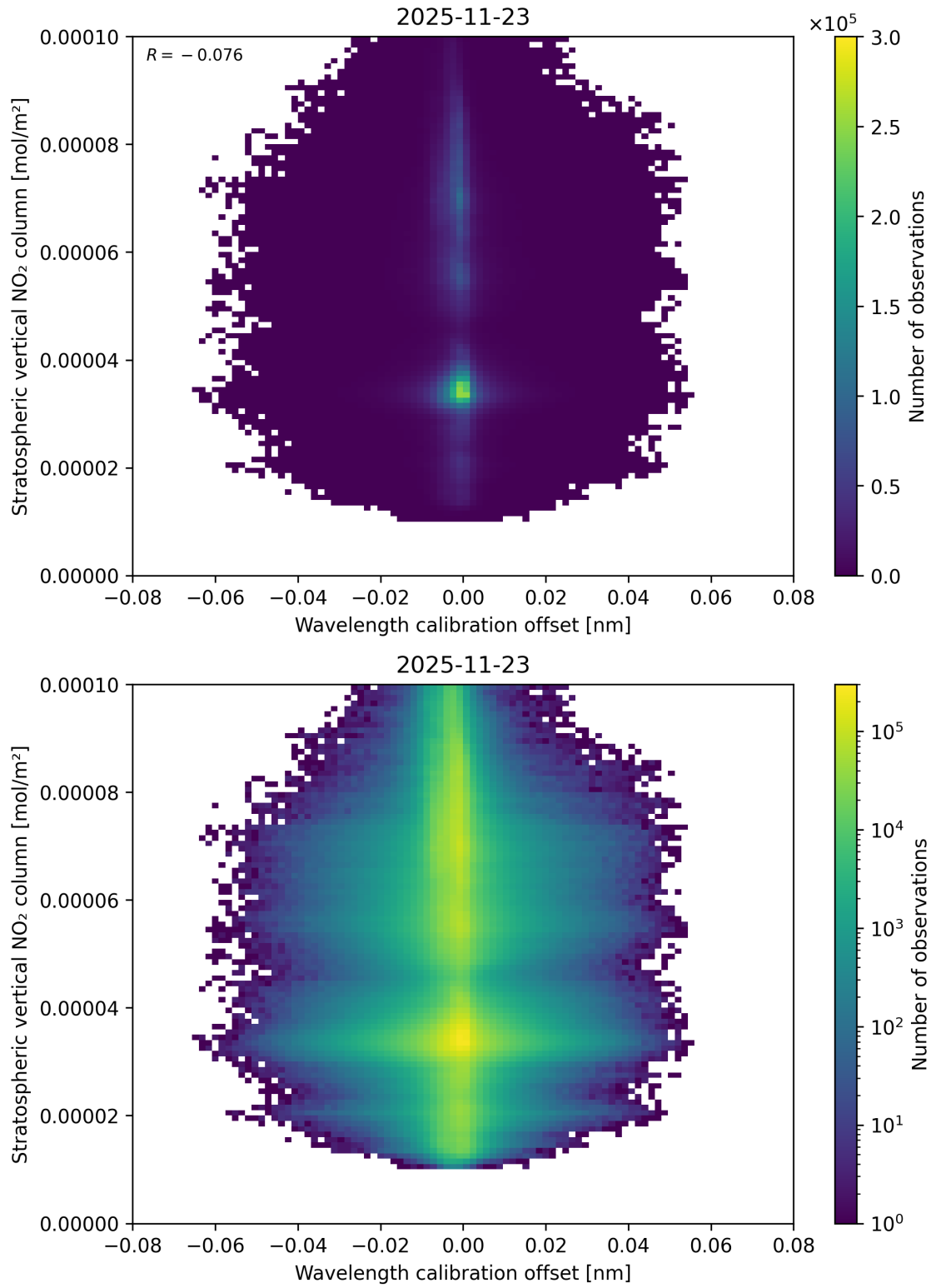
Figure 176: Scatter density plot of “Wavelength calibration offset” against “Stratospheric vertical NO 2 column” for 2025-11-23 to 2025-11-24.
