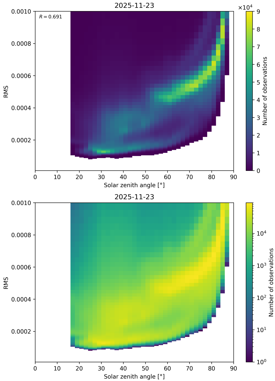
Figure 157: Scatter density plot of “Solar zenith angle” against “RMS” for 2025-11-23 to 2025-11-24.
