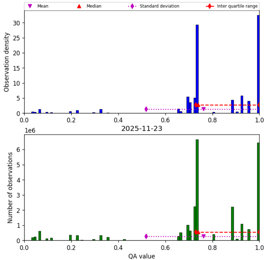
Figure 28: Histogram of “QA value” for 2025-11-23 to 2025-11-24
