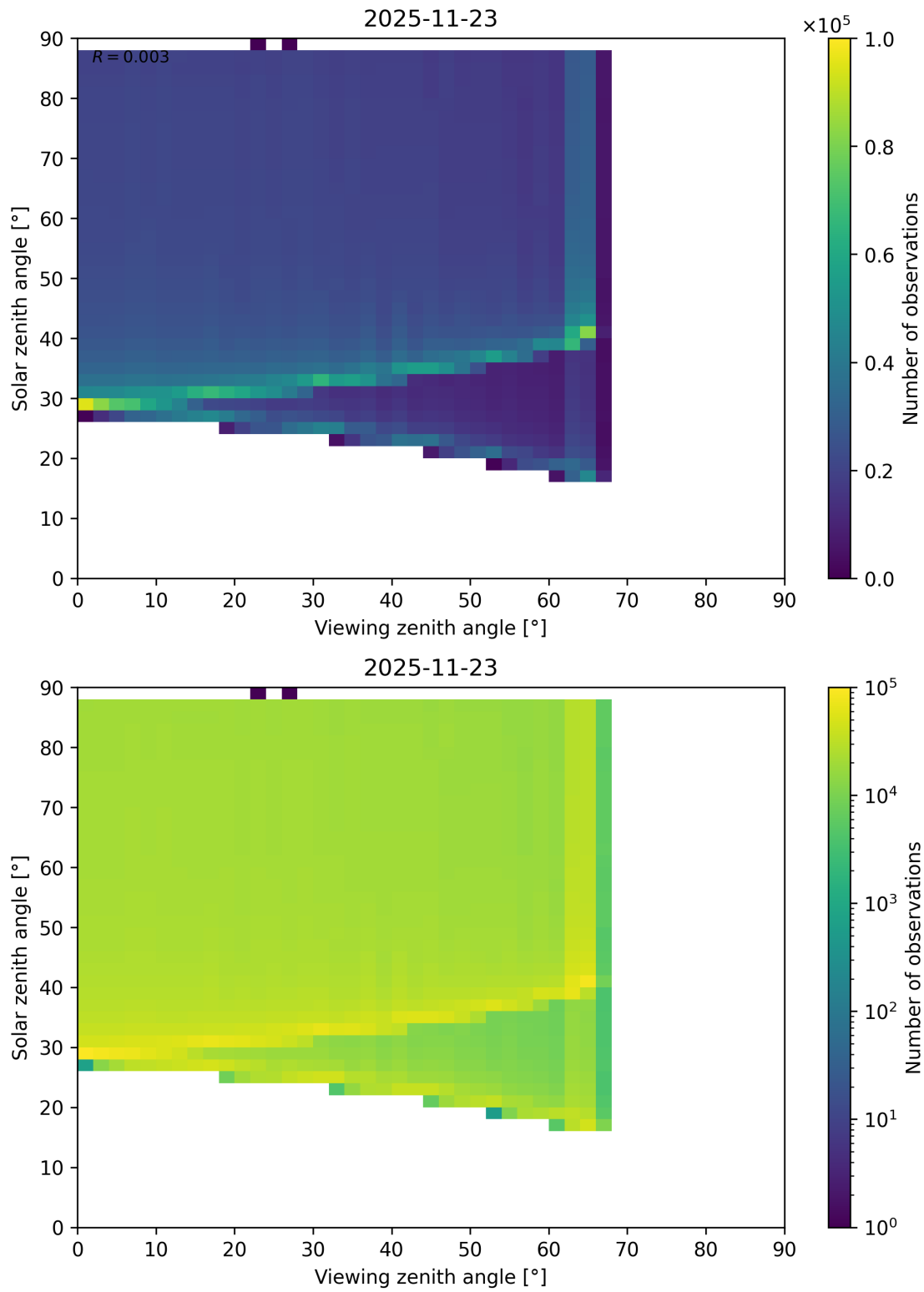
Figure 172: Scatter density plot of “Viewing zenith angle” against “Solar zenith angle” for 2025-11-23 to 2025-11-24.
