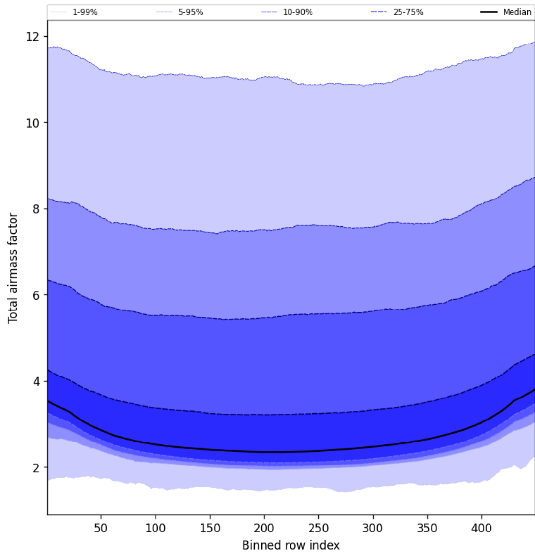
Figure 49: Along track statistics of “Total airmass factor” for 2025-11-23 to 2025-11-24
