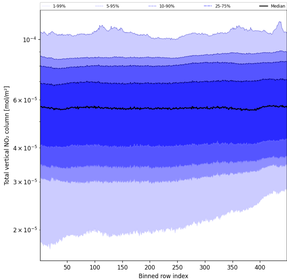
Figure 55: Along track statistics of “Total vertical NO 2 column” for 2025-11-23 to 2025-11-24
