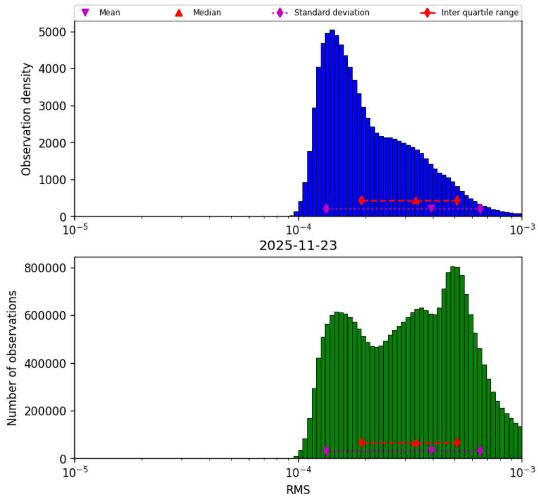
Figure 43: Histogram of “RMS” for 2025-11-23 to 2025-11-24
