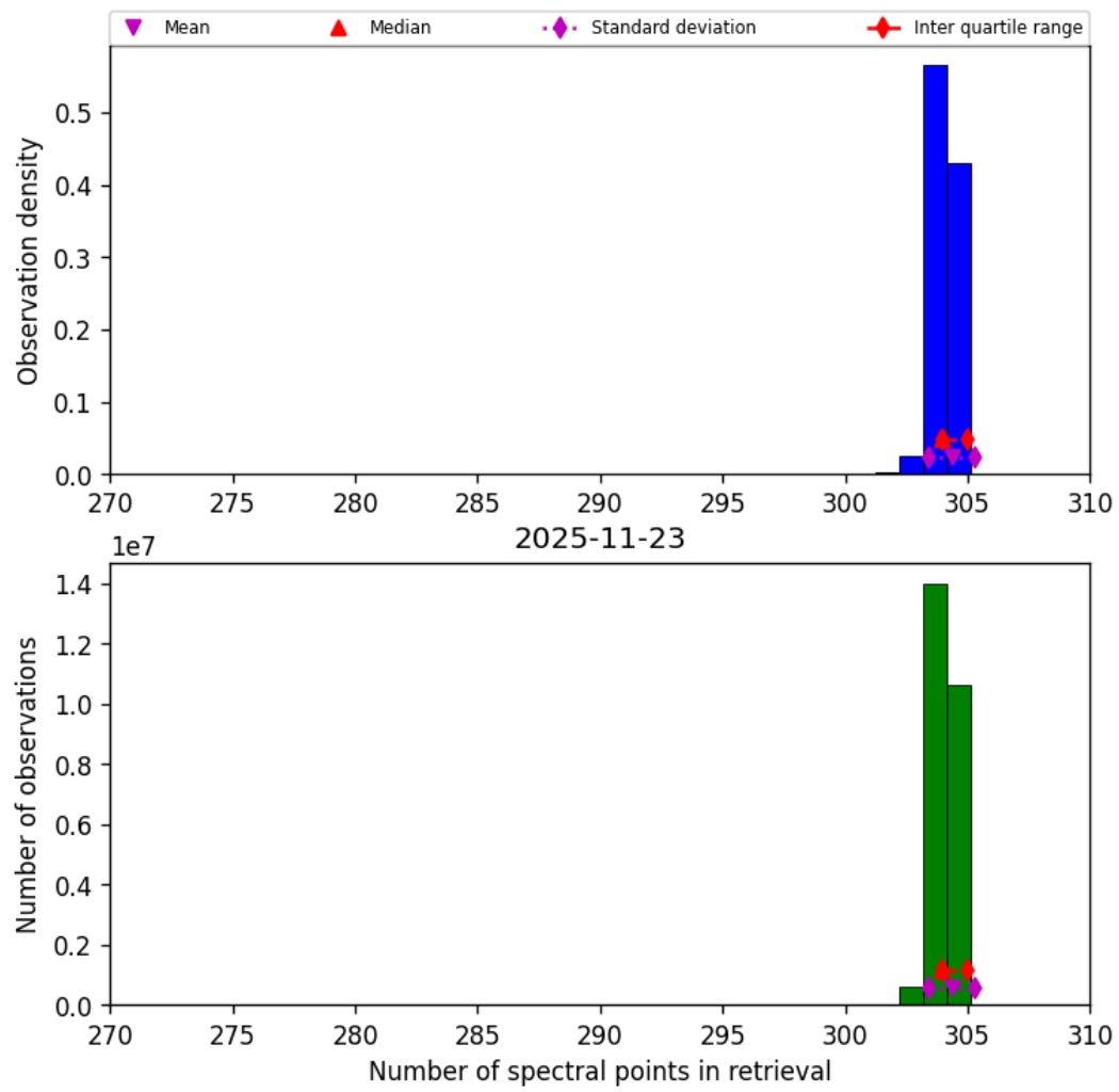
Figure 33: Histogram of “Number of spectral points in retrieval” for 2025-11-23 to 2025-11-24
