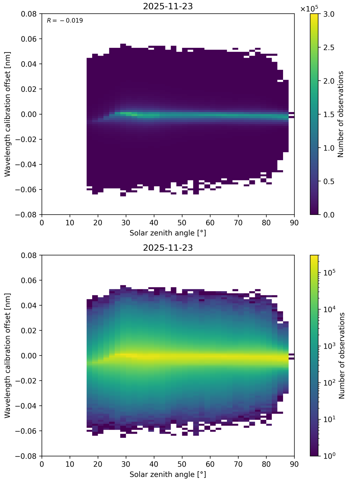
Figure 158: Scatter density plot of “Solar zenith angle” against “Wavelength calibration offset” for 2025-11-23 to 2025-11-24.
