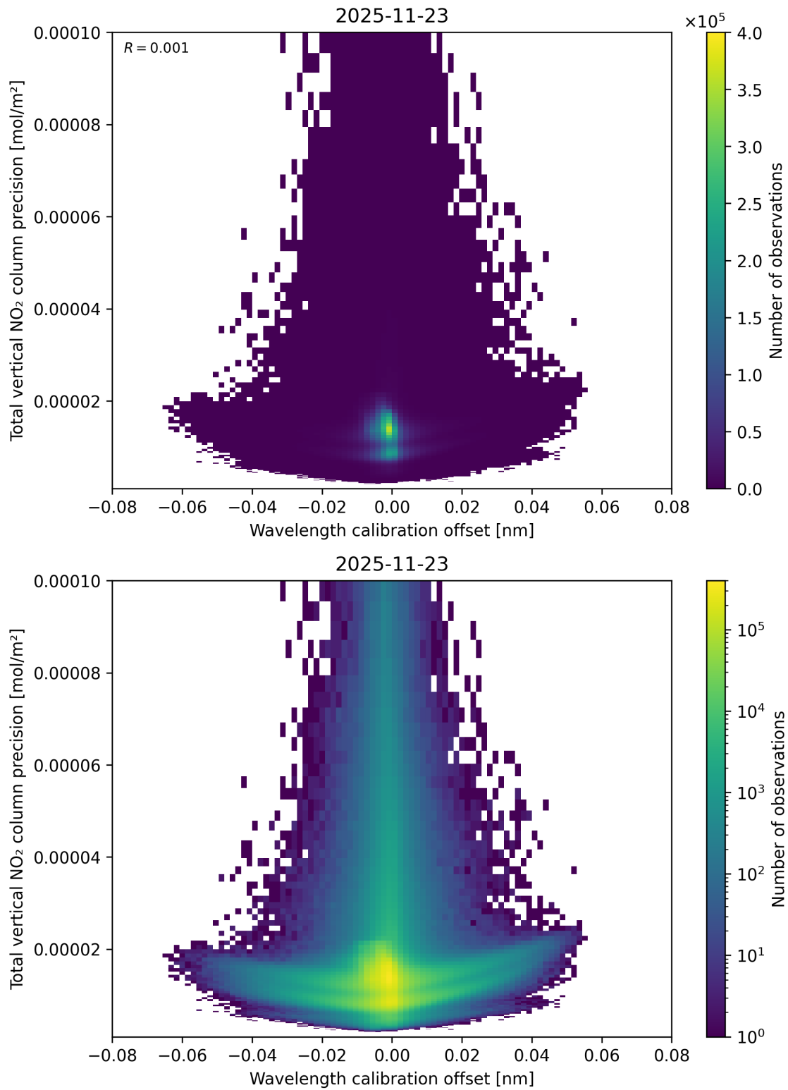
Figure 180: Scatter density plot of “Wavelength calibration offset” against “Total vertical NO 2 column precision” for 2025-11-23 to 2025-11-24.
