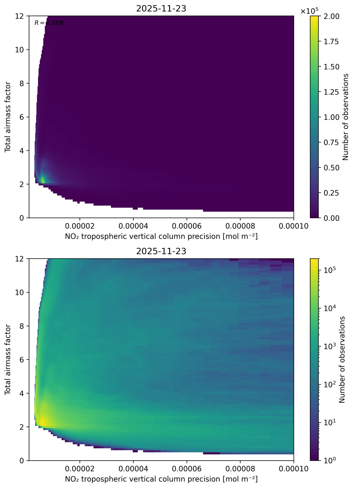
Figure 132: Scatter density plot of “NO 2 tropospheric vertical column precision” against “Total air mass factor” for 2025-11-23 to 2025-11-24.
