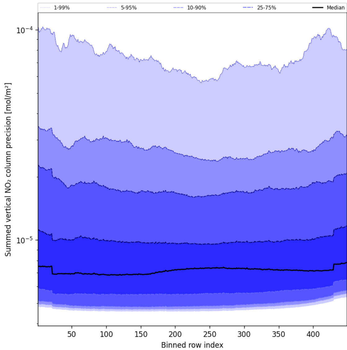
Figure 58: Along track statistics of “Summed vertical NO 2 column precision” for 2025-11-23 to 2025-11-24
