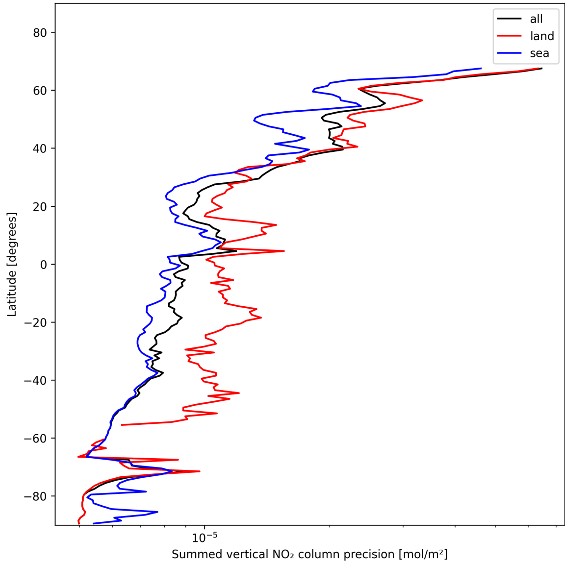
Figure 24: Zonal average of “Summed vertical NO 2 column precision” for 2025-11-23 to 2025-11-24.
