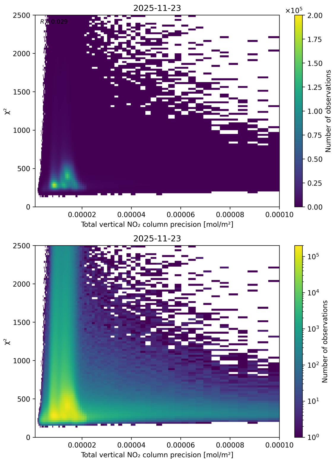
Figure 116: Scatter density plot of “Total vertical NO 2 column precision” against “ \chi^2 ” for 2025-11-23 to 2025-11-24.
