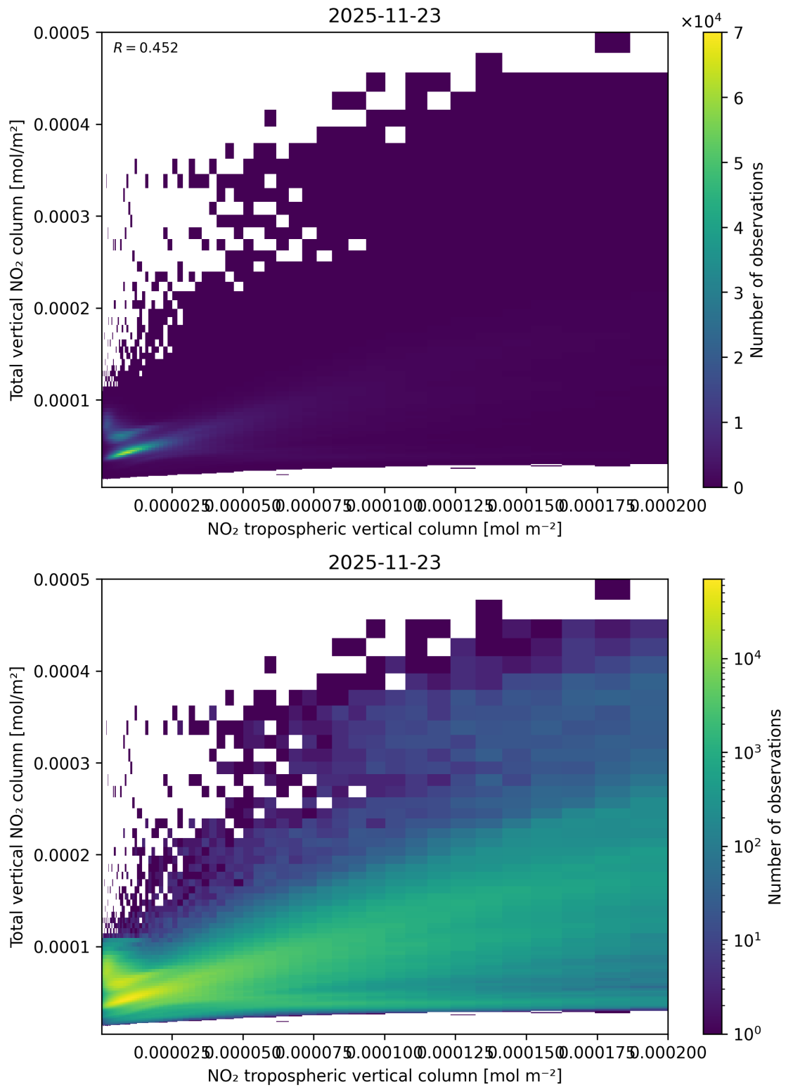
Figure 128: Scatter density plot of “NO 2 tropospheric vertical column” against “Total vertical NO 2 column” for 2025-11-23 to 2025-11-24.
