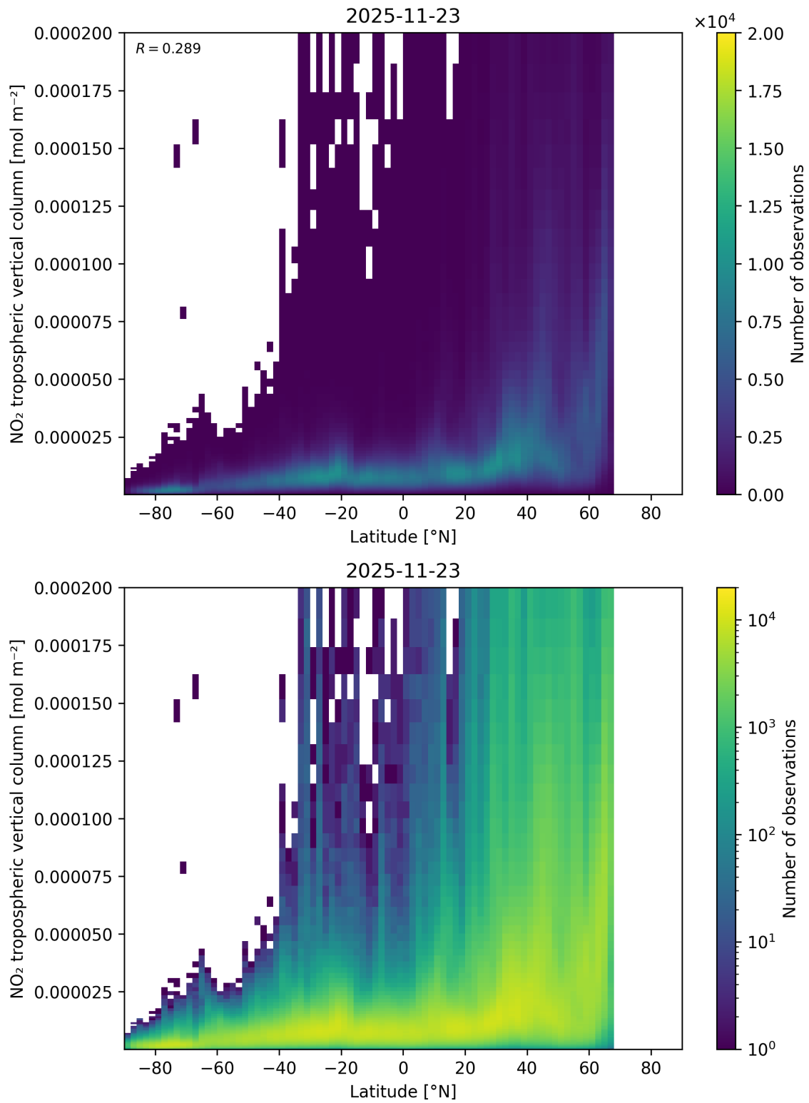
Figure 92: Scatter density plot of “Latitude” against “NO 2 tropospheric vertical column” for 2025-11-23 to 2025-11-24.
