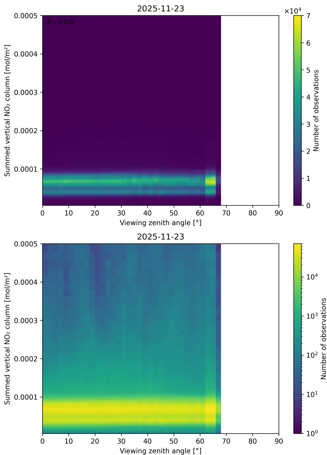
Figure 165: Scatter density plot of “Viewing zenith angle” against “Summed vertical NO 2 column” for 2025-11-23 to 2025-11-24.
