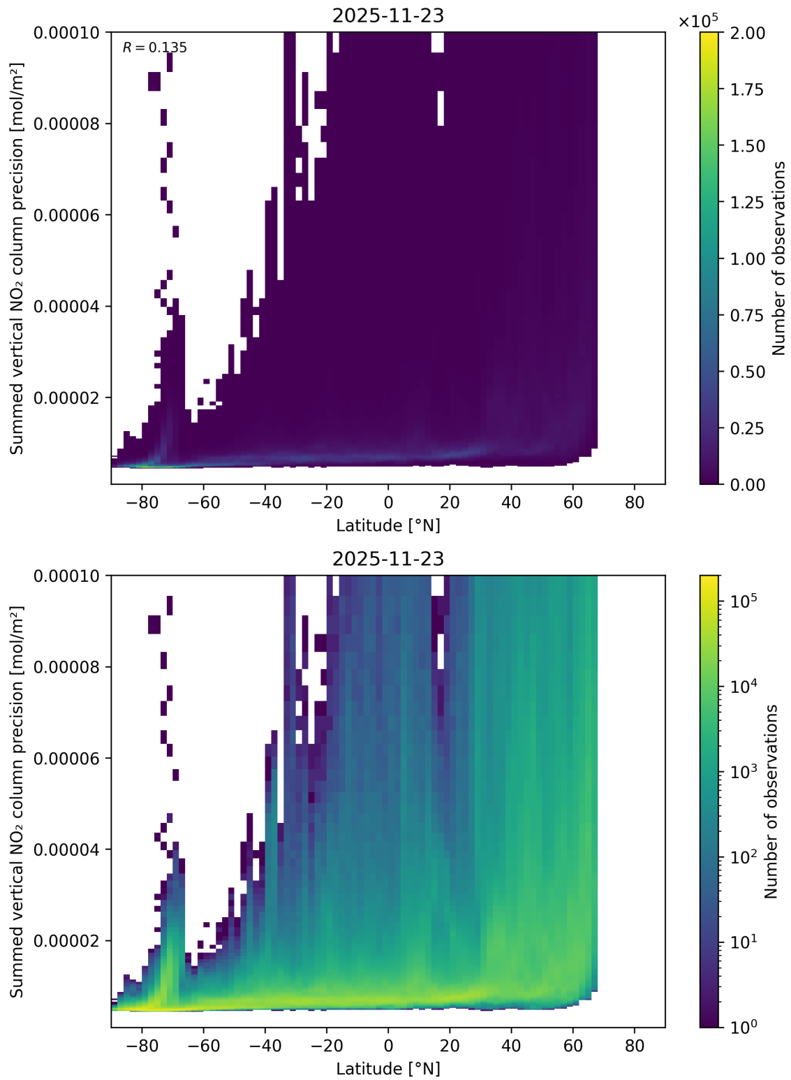
Figure 89: Scatter density plot of “Latitude” against “Summed vertical NO 2 column precision” for 2025-11-23 to 2025-11-24.
