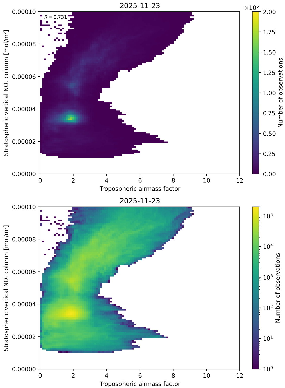
Figure 74: Scatter density plot of “Tropospheric airmass factor” against “Stratospheric vertical NO 2 column” for 2025-11-23 to 2025-11-24.
