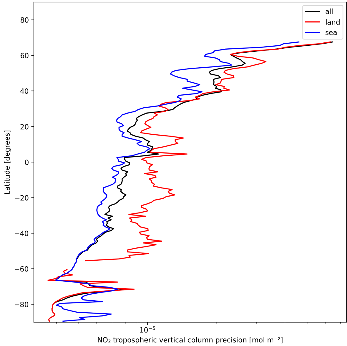
Figure 13: Zonal average of “NO 2 tropospheric vertical column precision” for 2025-11-23 to 2025-11-24.
