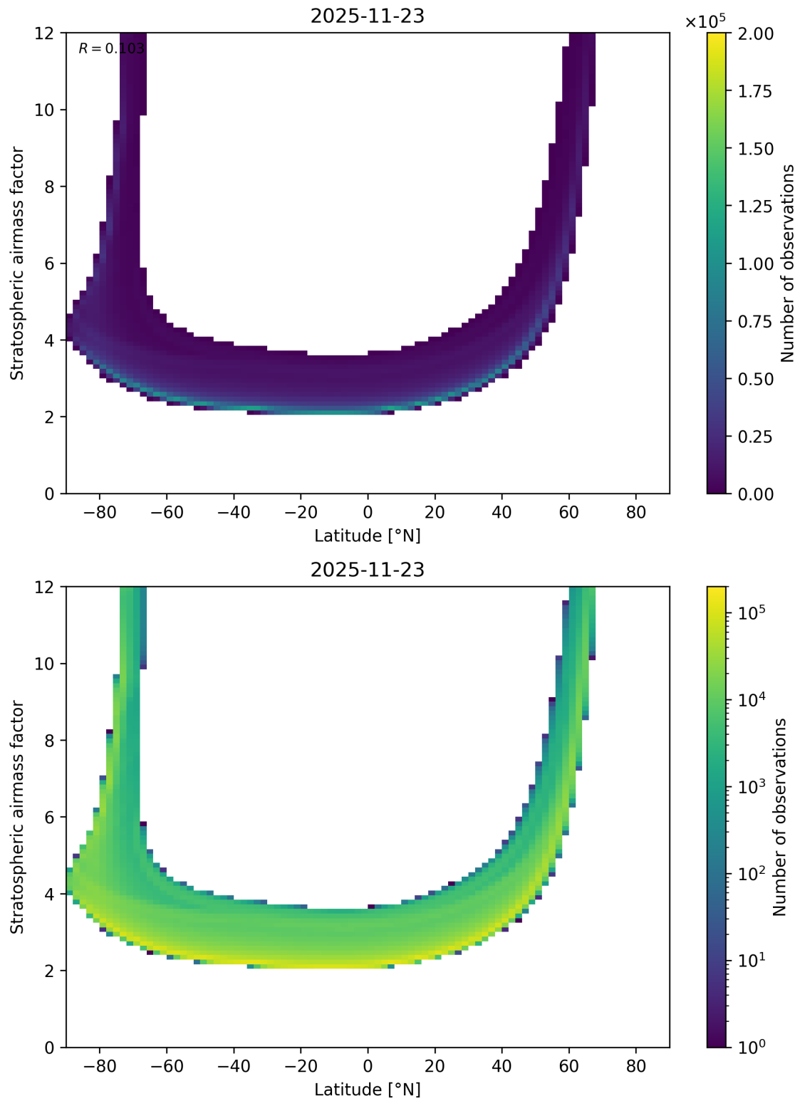
Figure 83: Scatter density plot of “Latitude” against “Stratospheric air mass factor” for 2025-11-23 to 2025-11-24.
