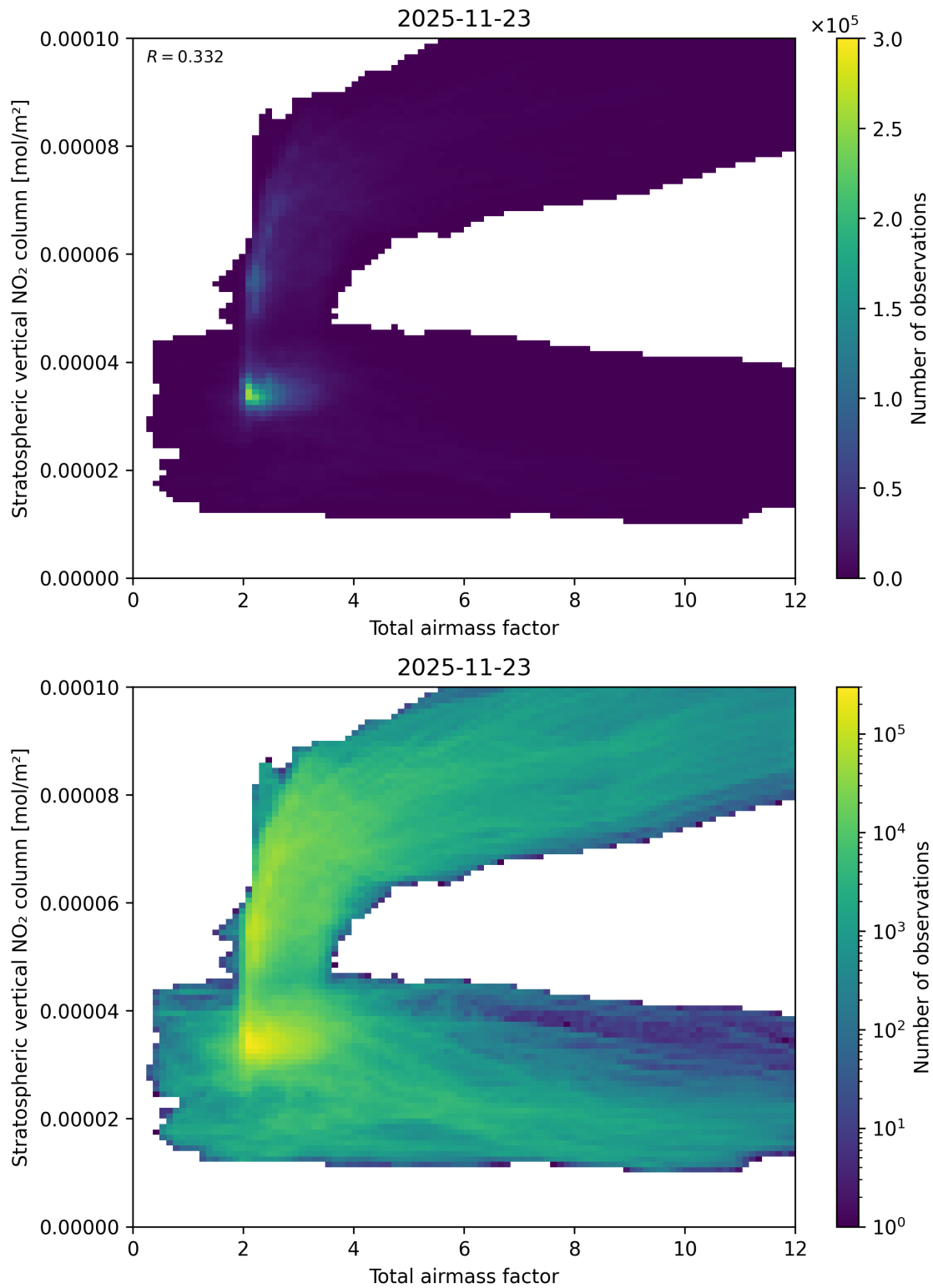
Figure 64: Scatter density plot of “Total airmass factor” against “Stratospheric vertical NO 2 column” for 2025-11-23 to 2025-11-24.
