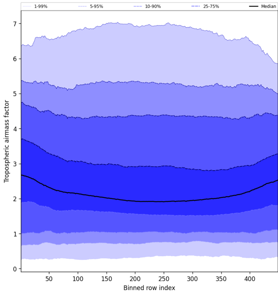
Figure 48: Along track statistics of “Tropospheric air mass factor” for 2025-11-23 to 2025-11-24
