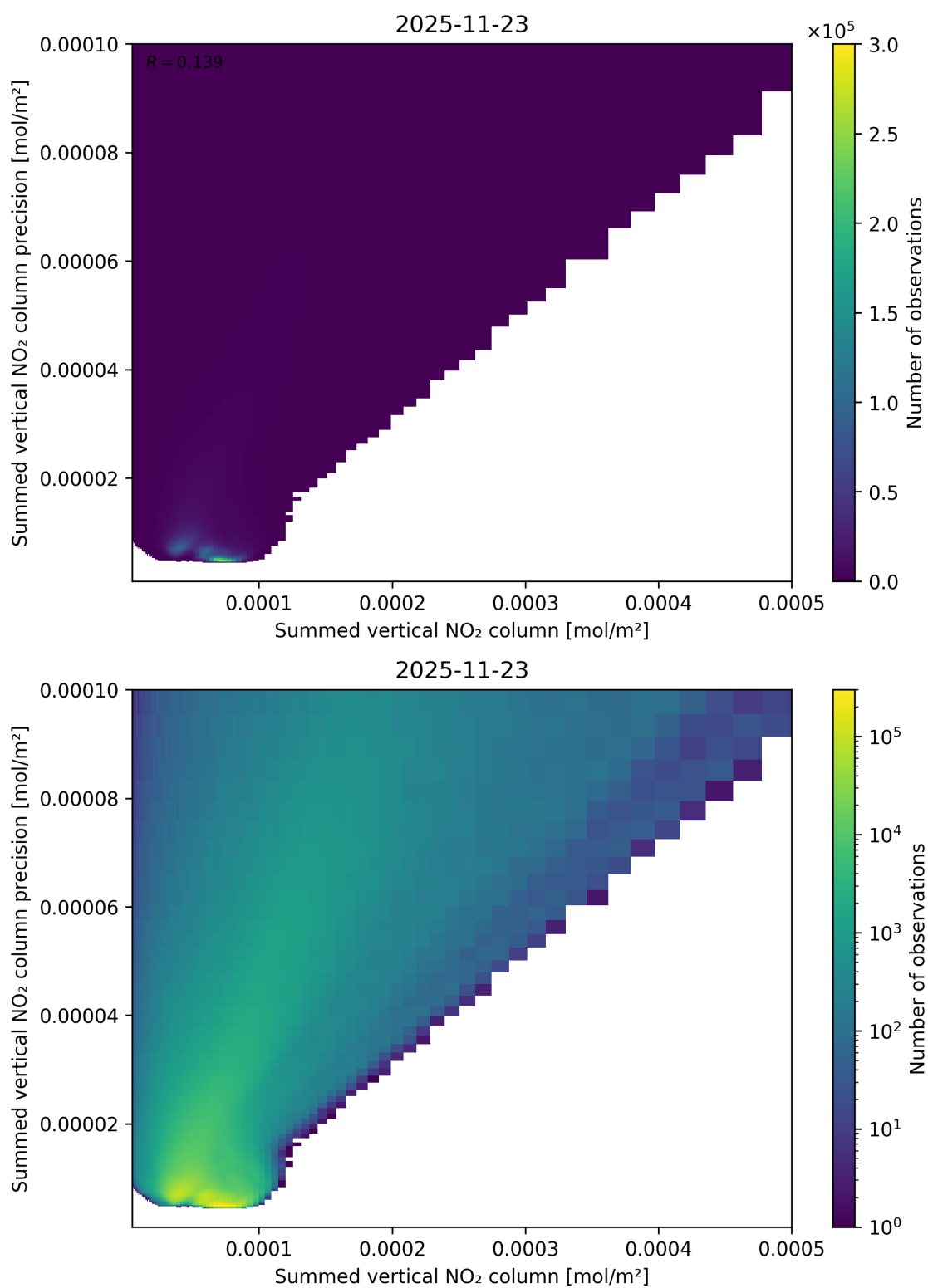
Figure 105: Scatter density plot of “Summed vertical NO 2 column” against “Summed vertical NO 2 column precision” for 2025-11-23 to 2025-11-24.
