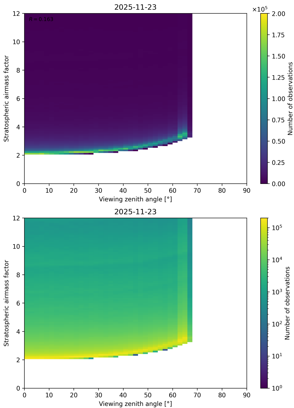
Figure 159: Scatter density plot of “Viewing zenith angle” against “Stratospheric airmass factor” for 2025-11-23 to 2025-11-24.
