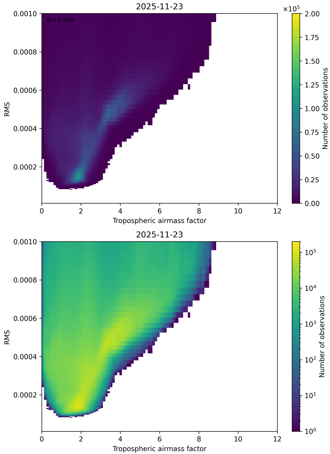
Figure 79: Scatter density plot of “Tropospheric airmass factor” against “RMS” for 2025-11-23 to 2025-11-24.
