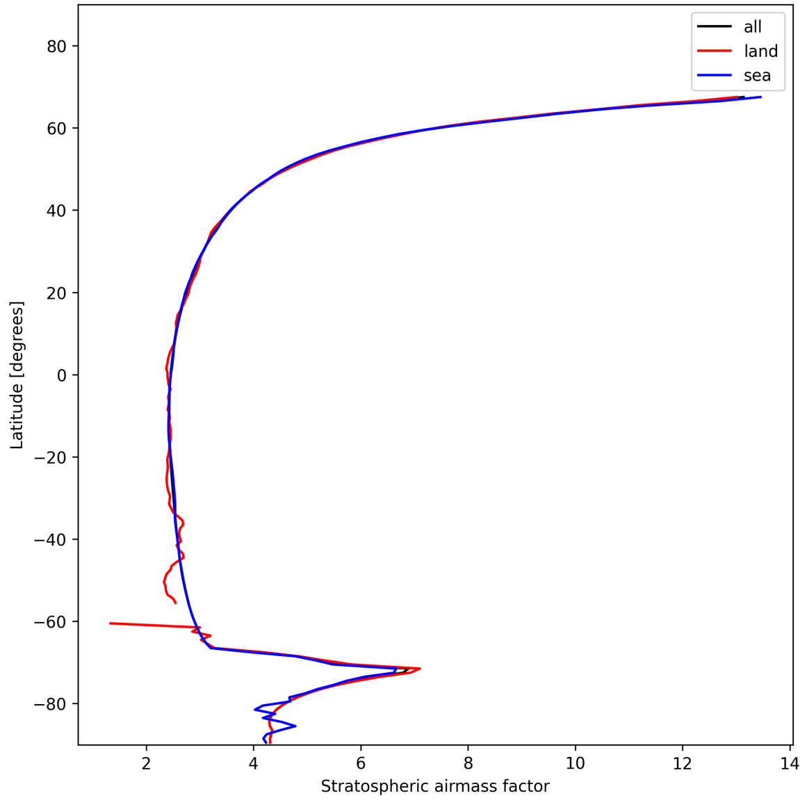
Figure 27: Zonal average of “Stratospheric air mass factor” for 2025-11-23 to 2025-11-24.
