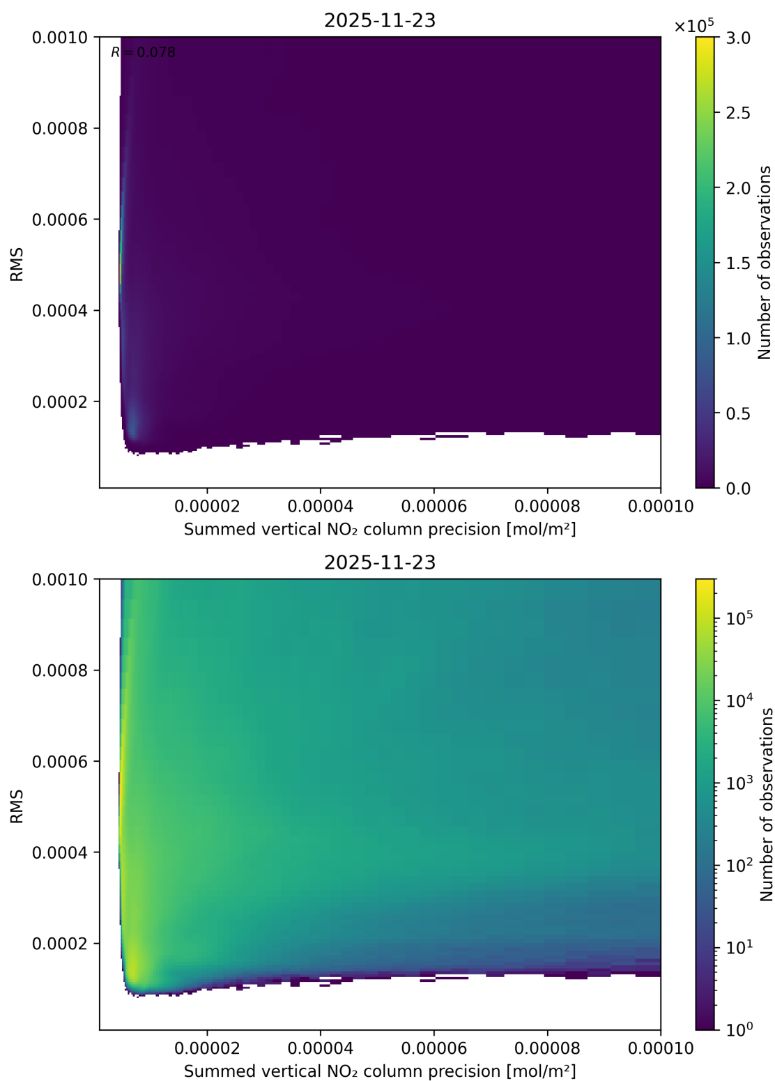
Figure 108: Scatter density plot of “Summed vertical NO 2 column precision” against “RMS” for 2025-11-23 to 2025-11-24.
