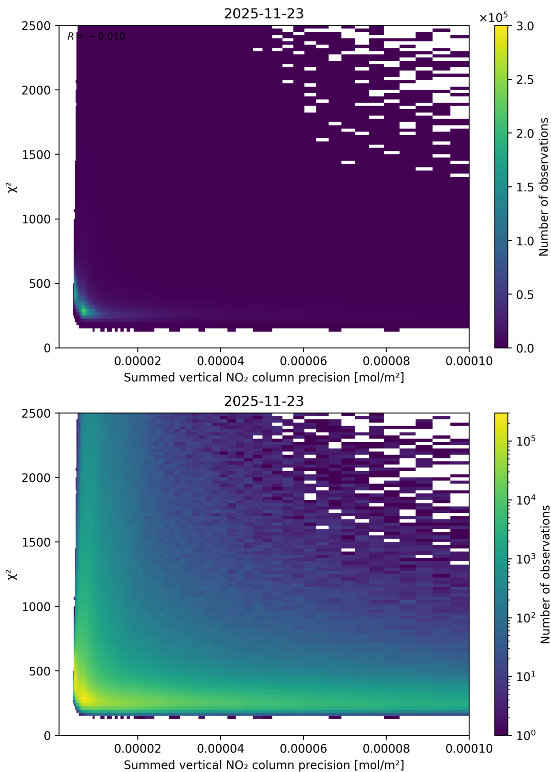
Figure 107: Scatter density plot of “Summed vertical NO 2 column precision” against “ \chi^2 ” for 2025-11-23 to 2025-11-24.
