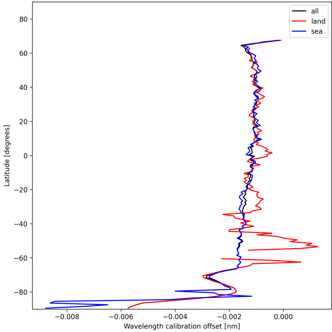
Figure 18: Zonal average of “Wavelength calibration offset” for 2025-11-23 to 2025-11-24.
