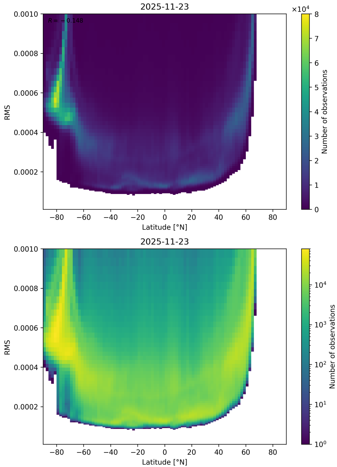
Figure 94: Scatter density plot of “Latitude” against “RMS” for 2025-11-23 to 2025-11-24.
