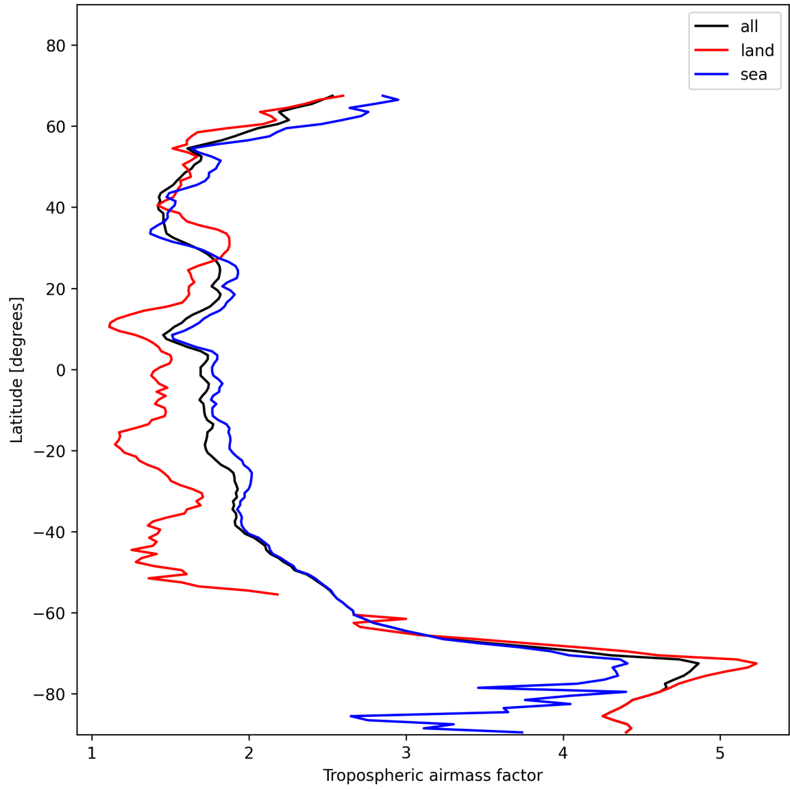
Figure 14: Zonal average of “Tropospheric airmass factor” for 2025-11-23 to 2025-11-24.
