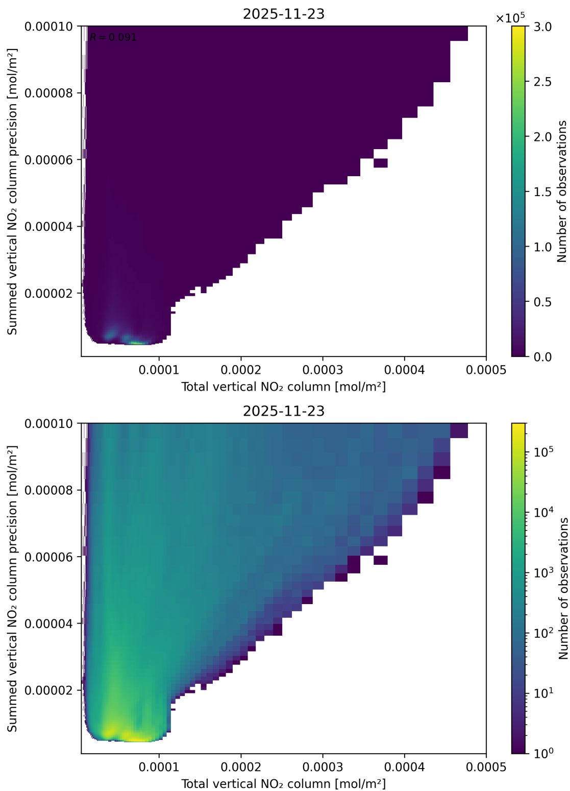
Figure 113: Scatter density plot of “Total vertical NO 2 column” against “Summed vertical NO 2 column precision” for 2025-11-23 to 2025-11-24.
