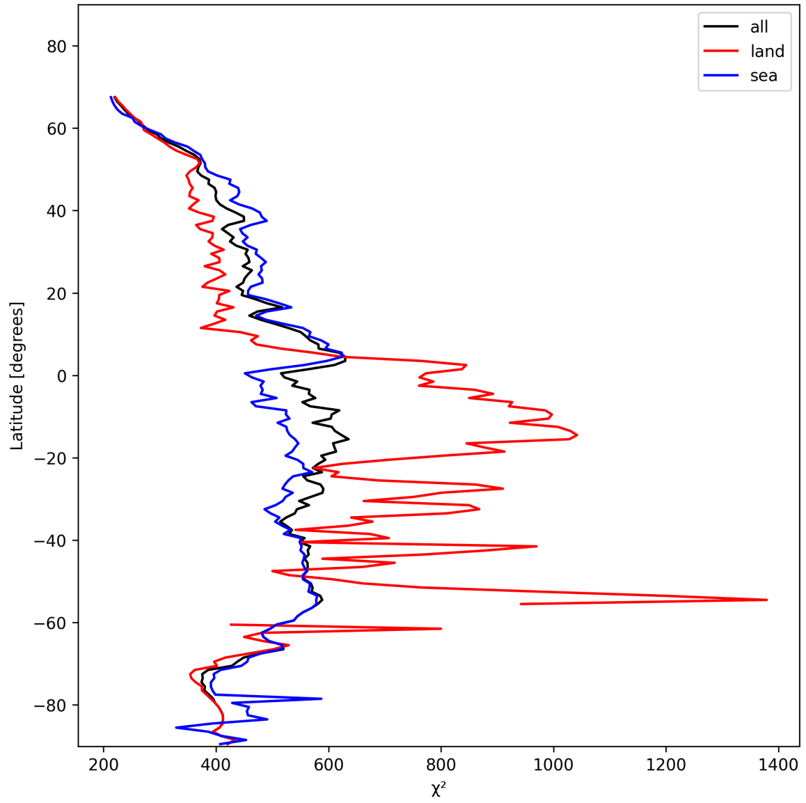
Figure 25: Zonal average of “ \chi^2 ” for 2025-11-23 to 2025-11-24.
