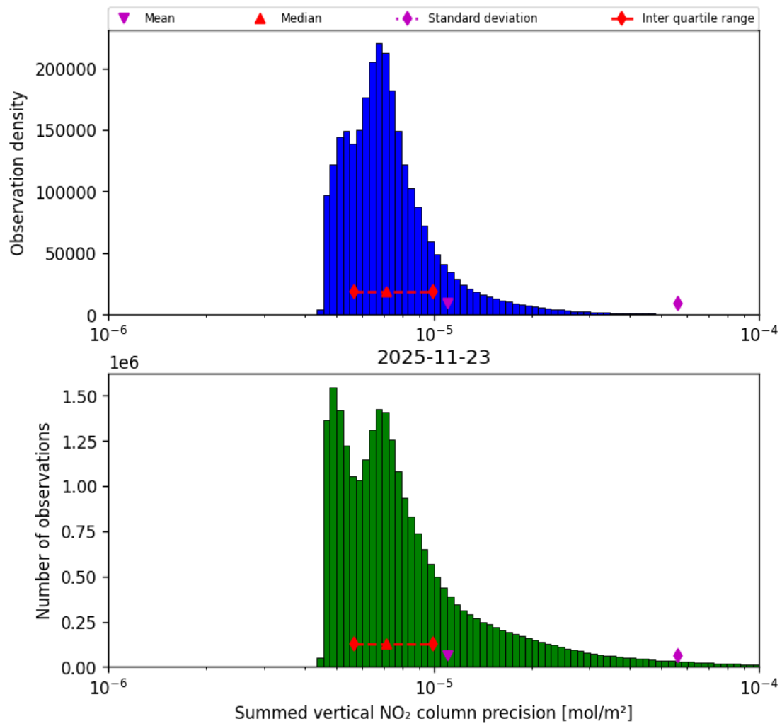
Figure 41: Histogram of “Summed vertical NO 2 column precision” for 2025-11-23 to 2025-11-24
