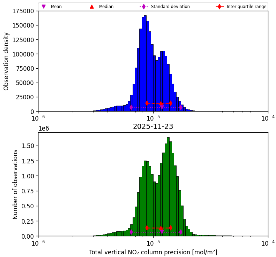
Figure 39: Histogram of “Total vertical NO 2 column precision” for 2025-11-23 to 2025-11-24
