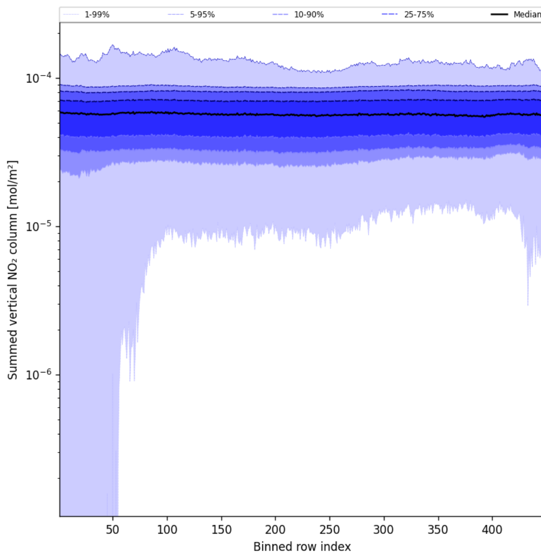
Figure 57: Along track statistics of “Summed vertical NO 2 column” for 2025-11-23 to 2025-11-24
