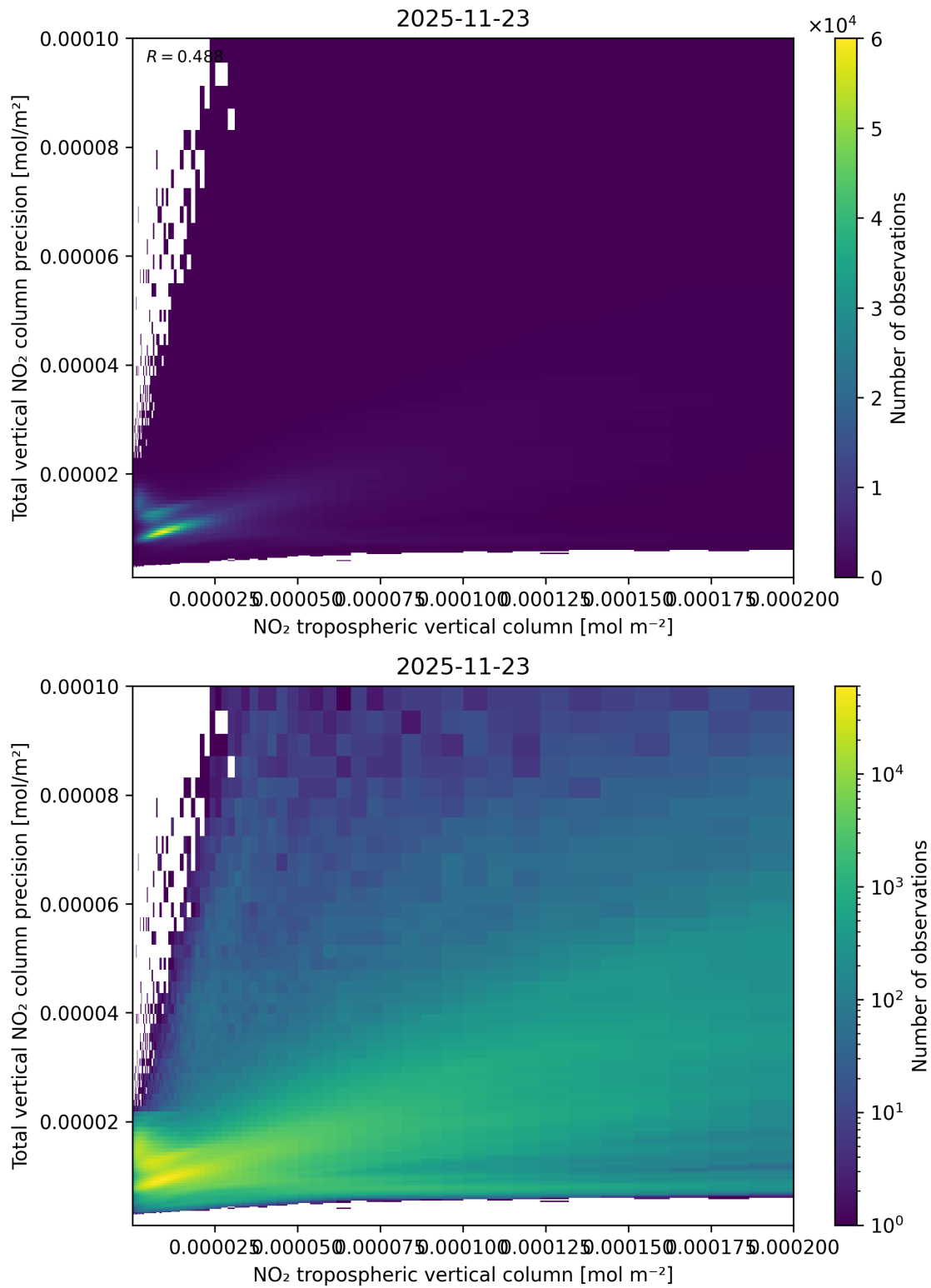
Figure 129: Scatter density plot of “NO 2 tropospheric vertical column” against “Total vertical NO 2 column precision” for 2025-11-23 to 2025-11-24.
