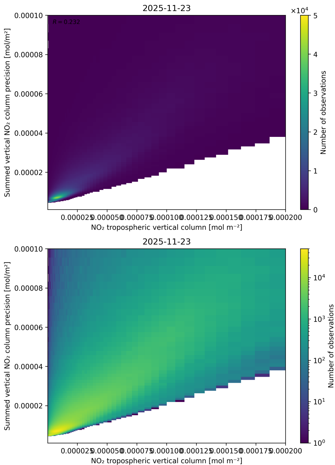
Figure 127: Scatter density plot of “NO 2 tropospheric vertical column” against “Summed vertical NO 2 column precision” for 2025-11-23 to 2025-11-24.
