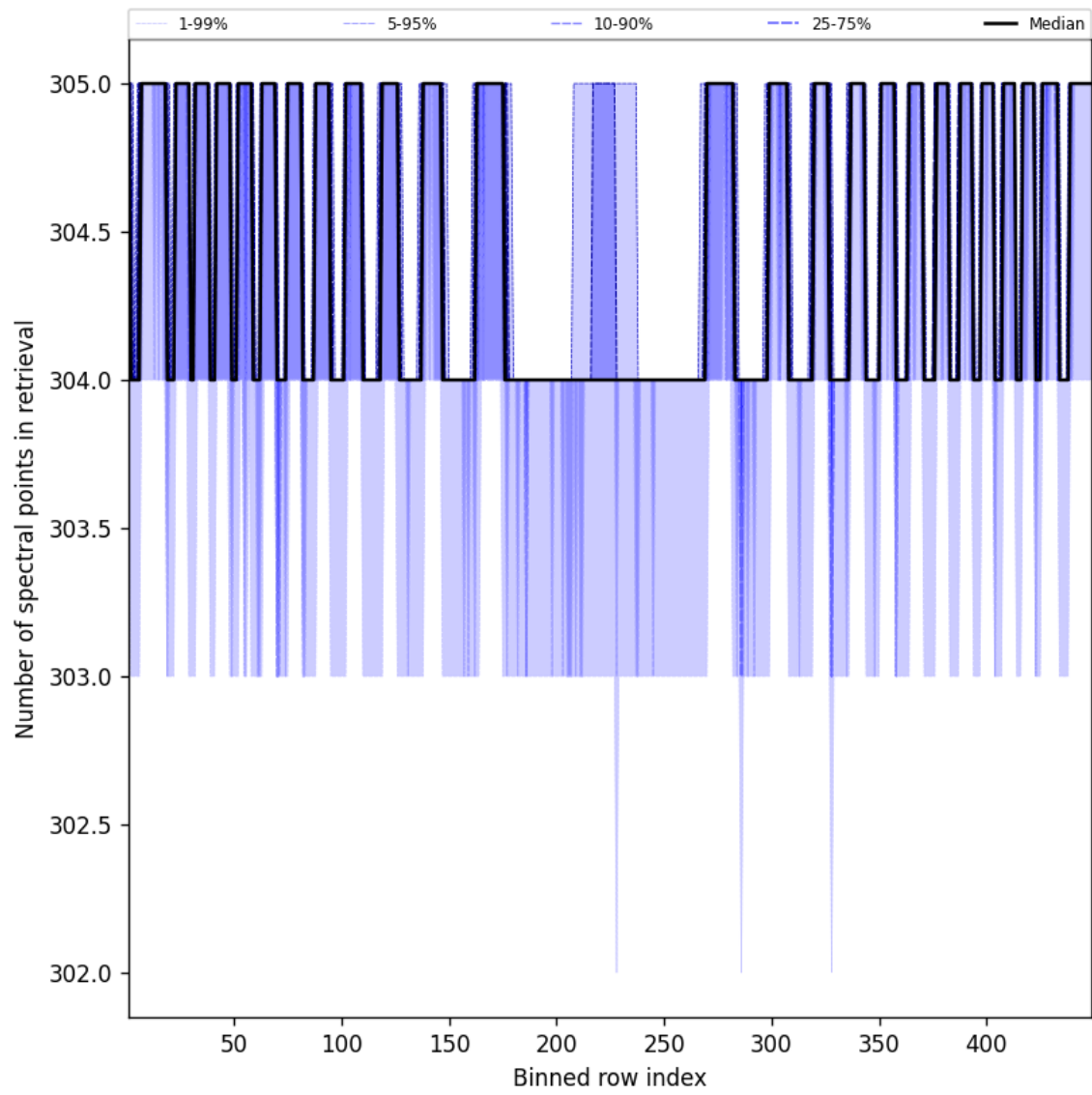
Figure 50: Along track statistics of “Number of spectral points in retrieval” for 2025-11-23 to 2025-11-24
