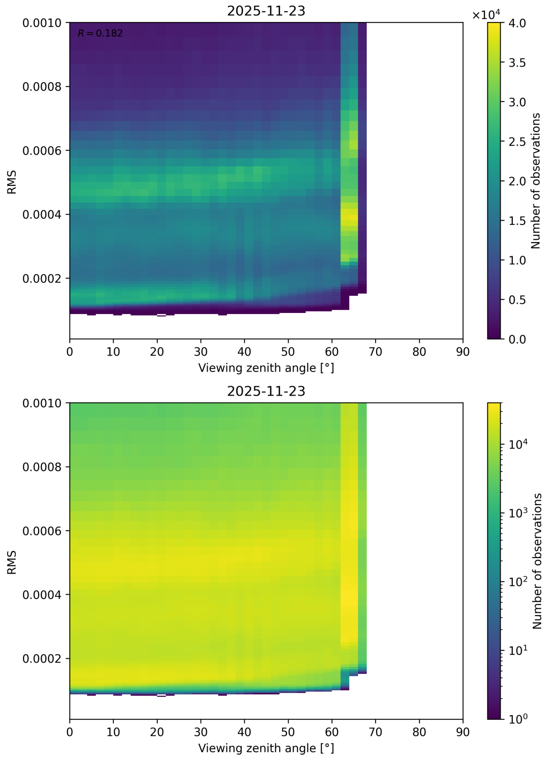
Figure 171: Scatter density plot of “Viewing zenith angle” against “RMS” for 2025-11-23 to 2025-11-24.
