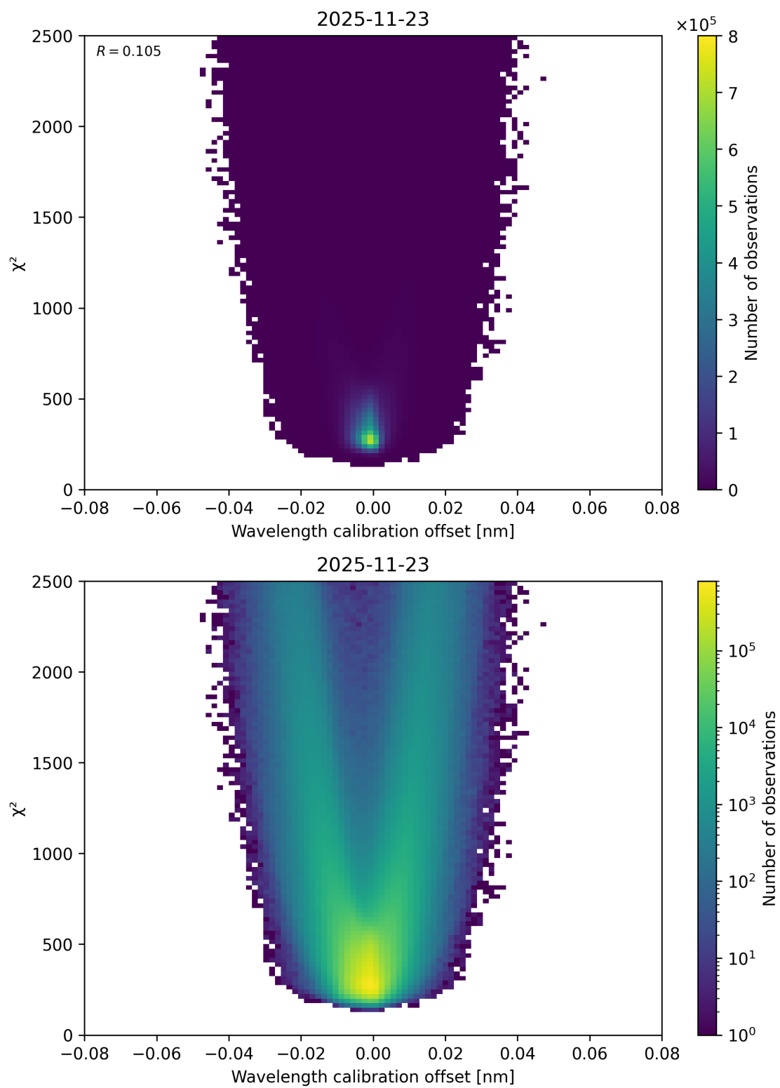
Figure 175: Scatter density plot of “Wavelength calibration offset” against “ \chi^2 ” for 2025-11-23 to 2025-11-24.
