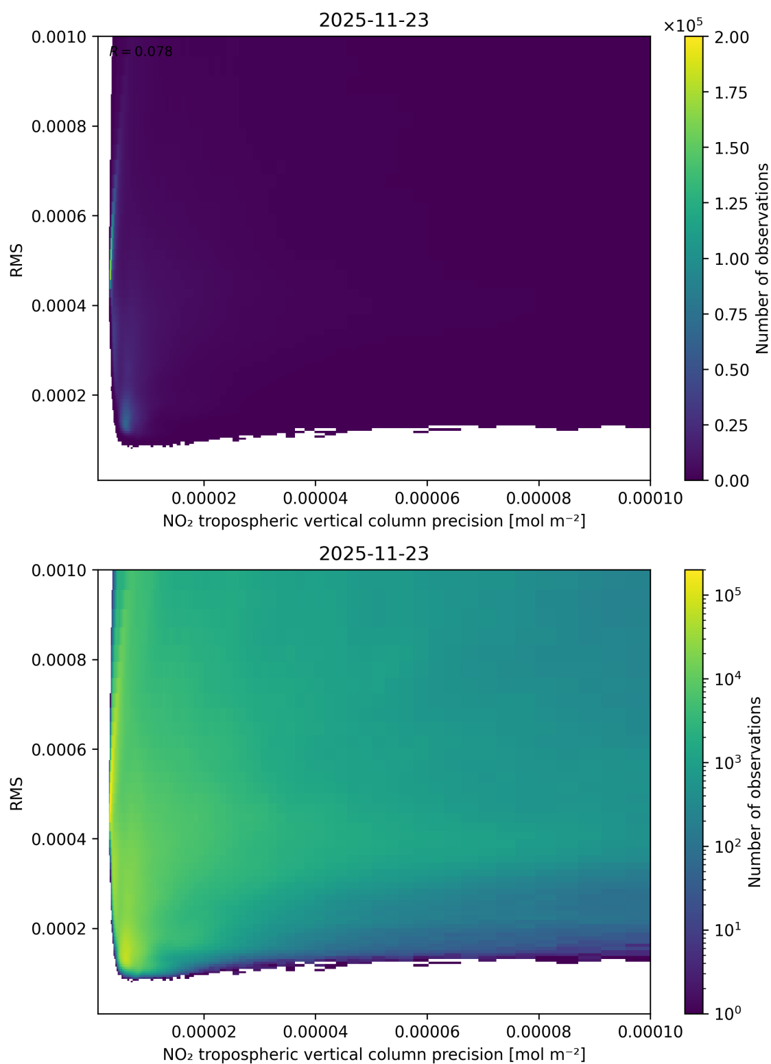
Figure 140: Scatter density plot of “NO 2 tropospheric vertical column precision” against “RMS” for 2025-11-23 to 2025-11-24.
