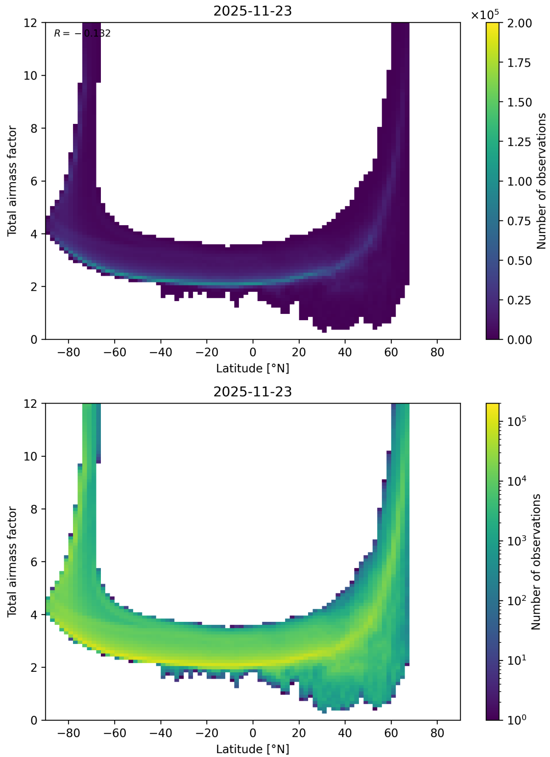
Figure 84: Scatter density plot of “Latitude” against “Total airmass factor” for 2025-11-23 to 2025-11-24.
