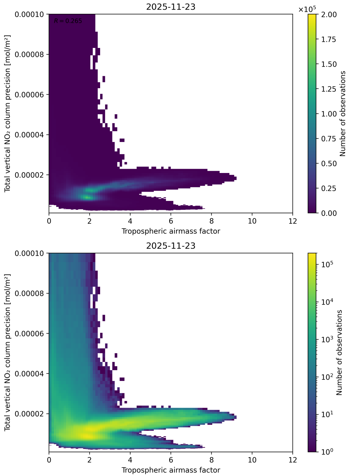
Figure 78: Scatter density plot of “Tropospheric air mass factor” against “Total vertical NO 2 column precision” for 2025-11-23 to 2025-11-24.
