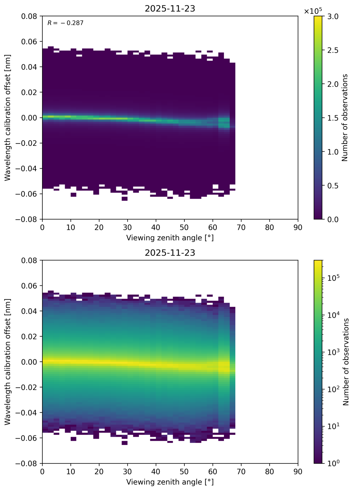
Figure 173: Scatter density plot of “Viewing zenith angle” against “Wavelength calibration offset” for 2025-11-23 to 2025-11-24.
