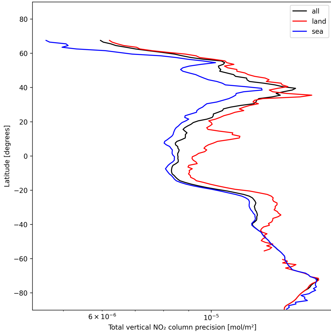
Figure 22: Zonal average of “Total vertical NO 2 column precision” for 2025-11-23 to 2025-11-24.
