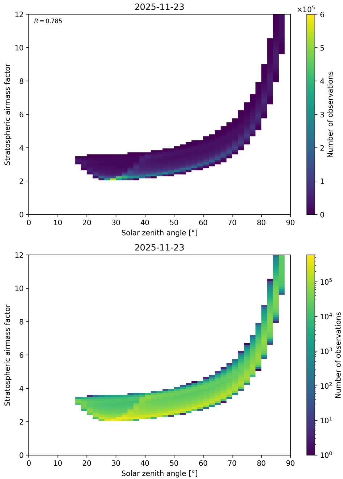
Figure 145: Scatter density plot of “Solar zenith angle” against “Stratospheric airmass factor” for 2025-11-23 to 2025-11-24.
