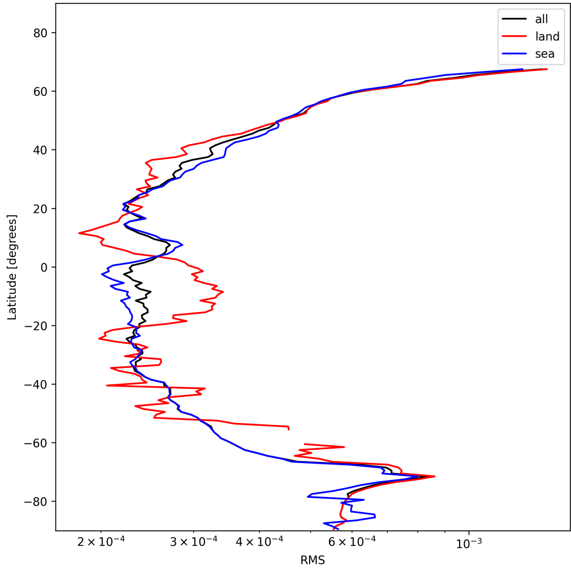
Figure 26: Zonal average of “RMS” for 2025-11-23 to 2025-11-24.
