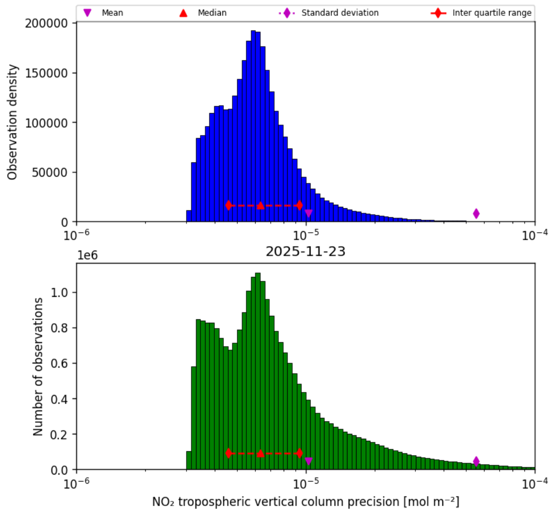
Figure 30: Histogram of “NO 2 tropospheric vertical column precision” for 2025-11-23 to 2025-11-24
