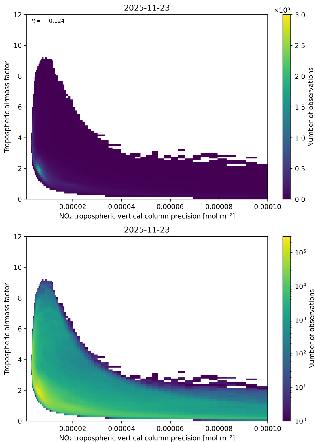
Figure 133: Scatter density plot of “NO 2 tropospheric vertical column precision” against “Tropospheric airmass factor” for 2025-11-23 to 2025-11-24.
