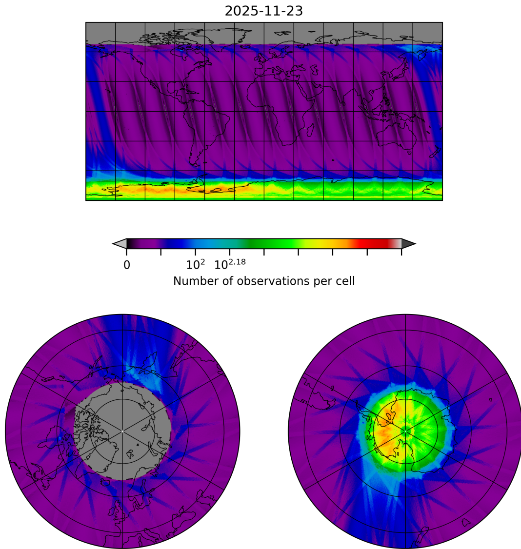
Figure 10: Map of the number of observations for 2025-11-23 to 2025-11-24
