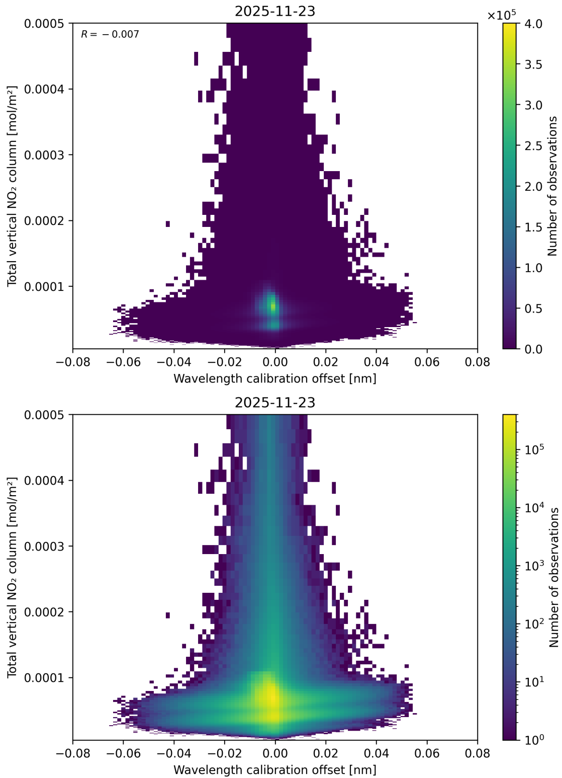
Figure 179: Scatter density plot of “Wavelength calibration offset” against “Total vertical NO 2 column” for 2025-11-23 to 2025-11-24.
