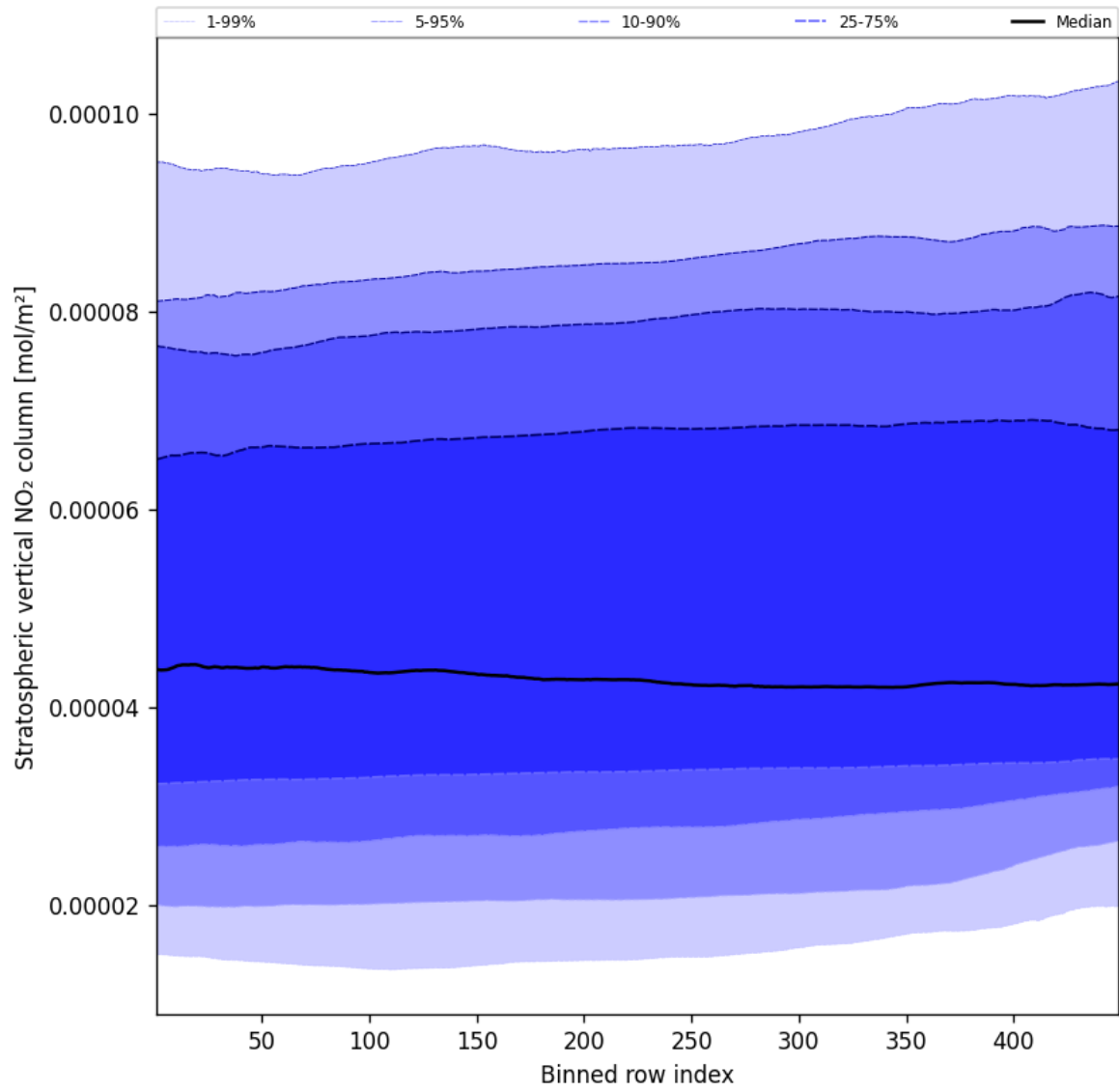
Figure 53: Along track statistics of “Stratospheric vertical NO 2 column” for 2025-11-23 to 2025-11-24
