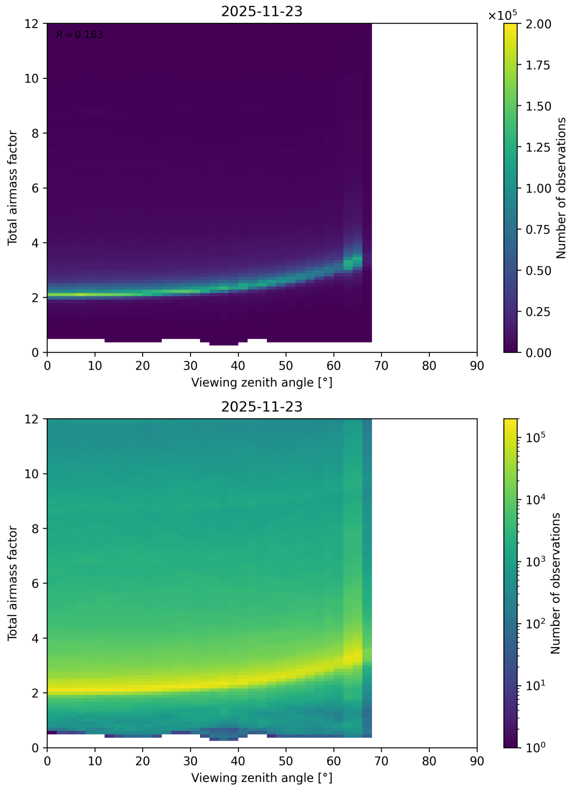
Figure 160: Scatter density plot of “Viewing zenith angle” against “Total airmass factor” for 2025-11-23 to 2025-11-24.
