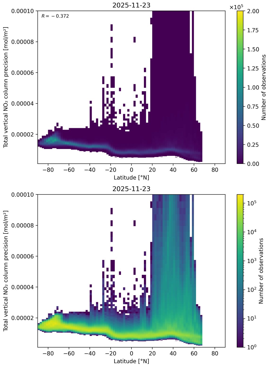
Figure 91: Scatter density plot of “Latitude” against “Total vertical NO 2 column precision” for 2025-11-23 to 2025-11-24.
