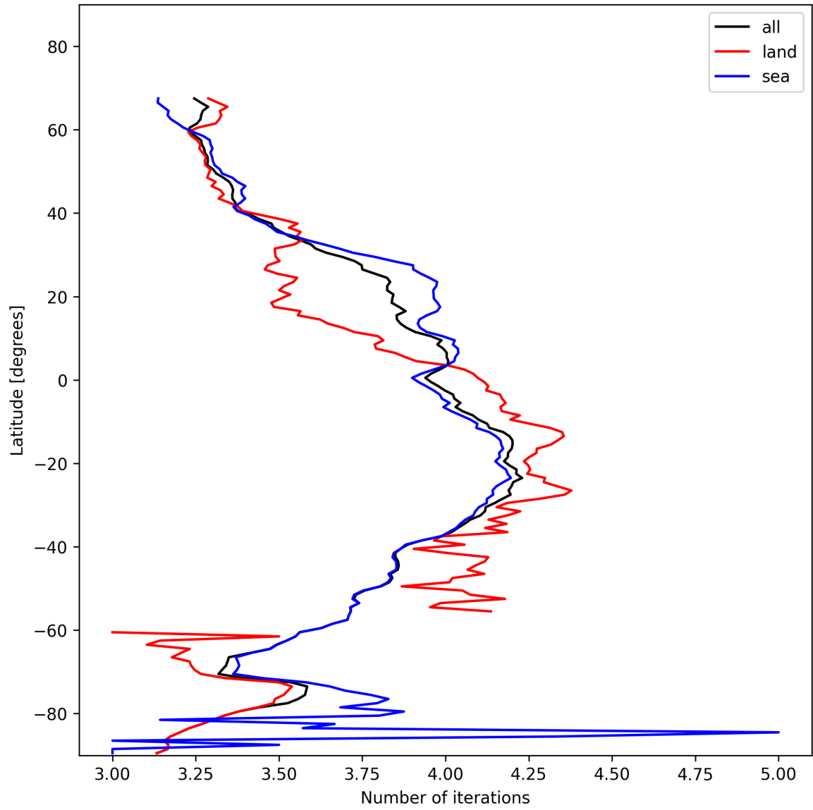
Figure 17: Zonal average of “Number of iterations” for 2025-11-23 to 2025-11-24.
