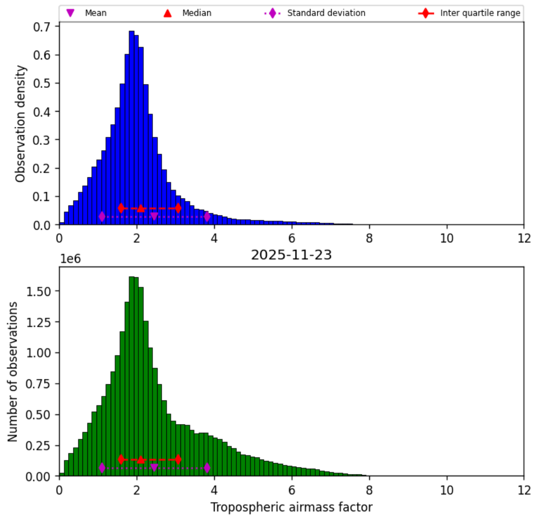
Figure 31: Histogram of “Tropospheric airmass factor” for 2025-11-23 to 2025-11-24
