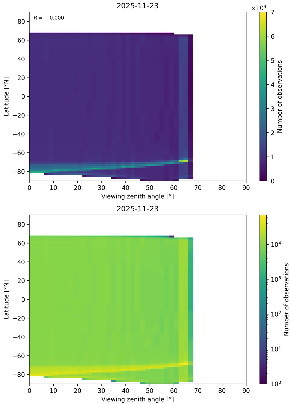
Figure 163: Scatter density plot of “Viewing zenith angle” against “Latitude” for 2025-11-23 to 2025-11-24.
