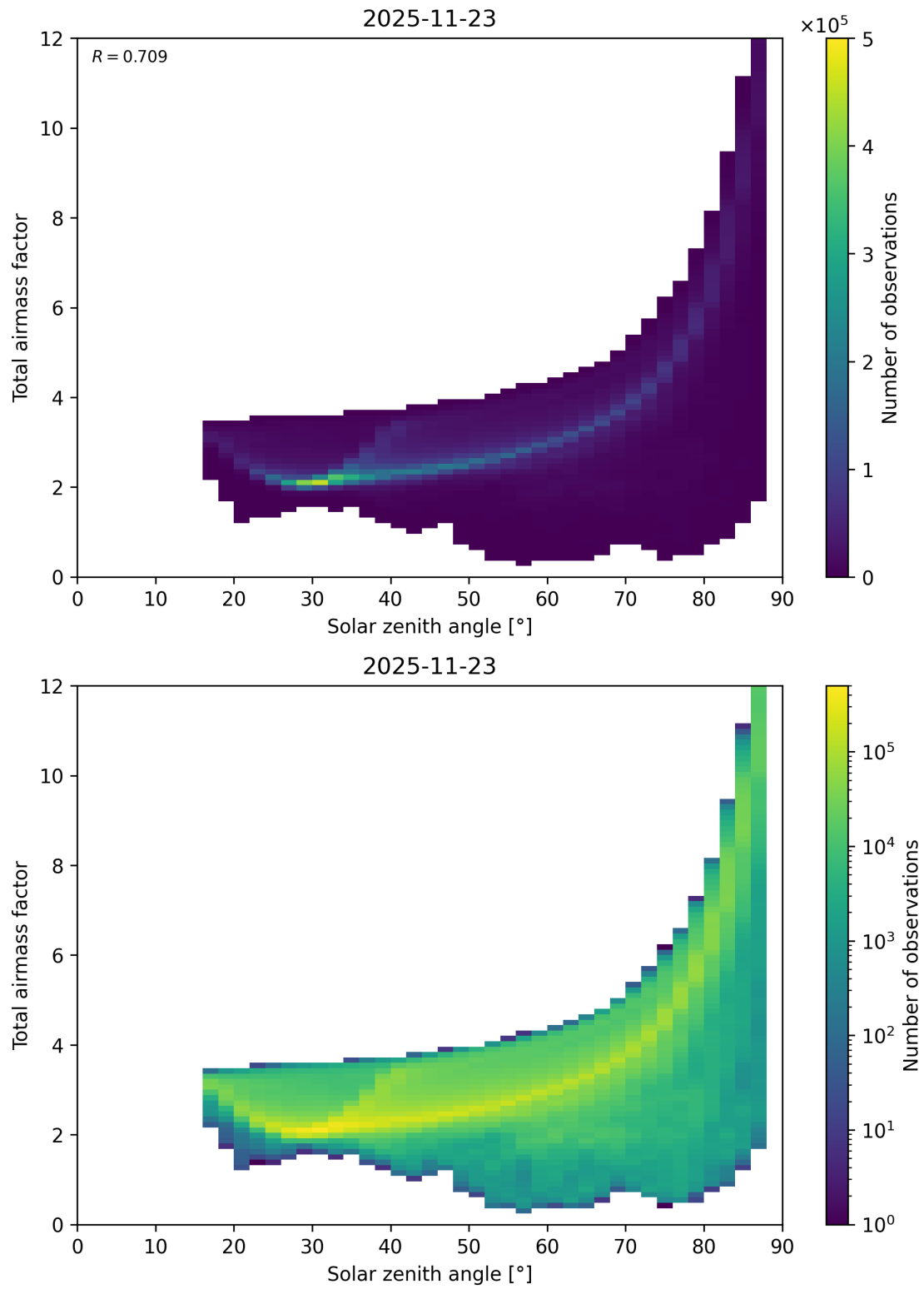
Figure 146: Scatter density plot of “Solar zenith angle” against “Total airmass factor” for 2025-11-23 to 2025-11-24.
