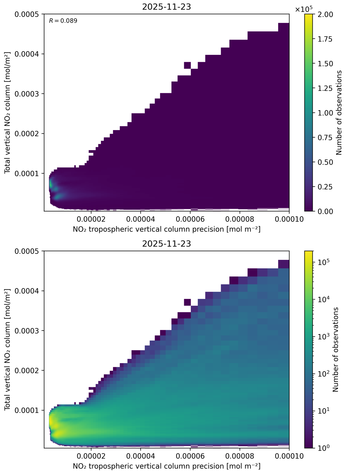
Figure 138: Scatter density plot of “NO 2 tropospheric vertical column precision” against “Total vertical NO 2 column” for 2025-11-23 to 2025-11-24.
