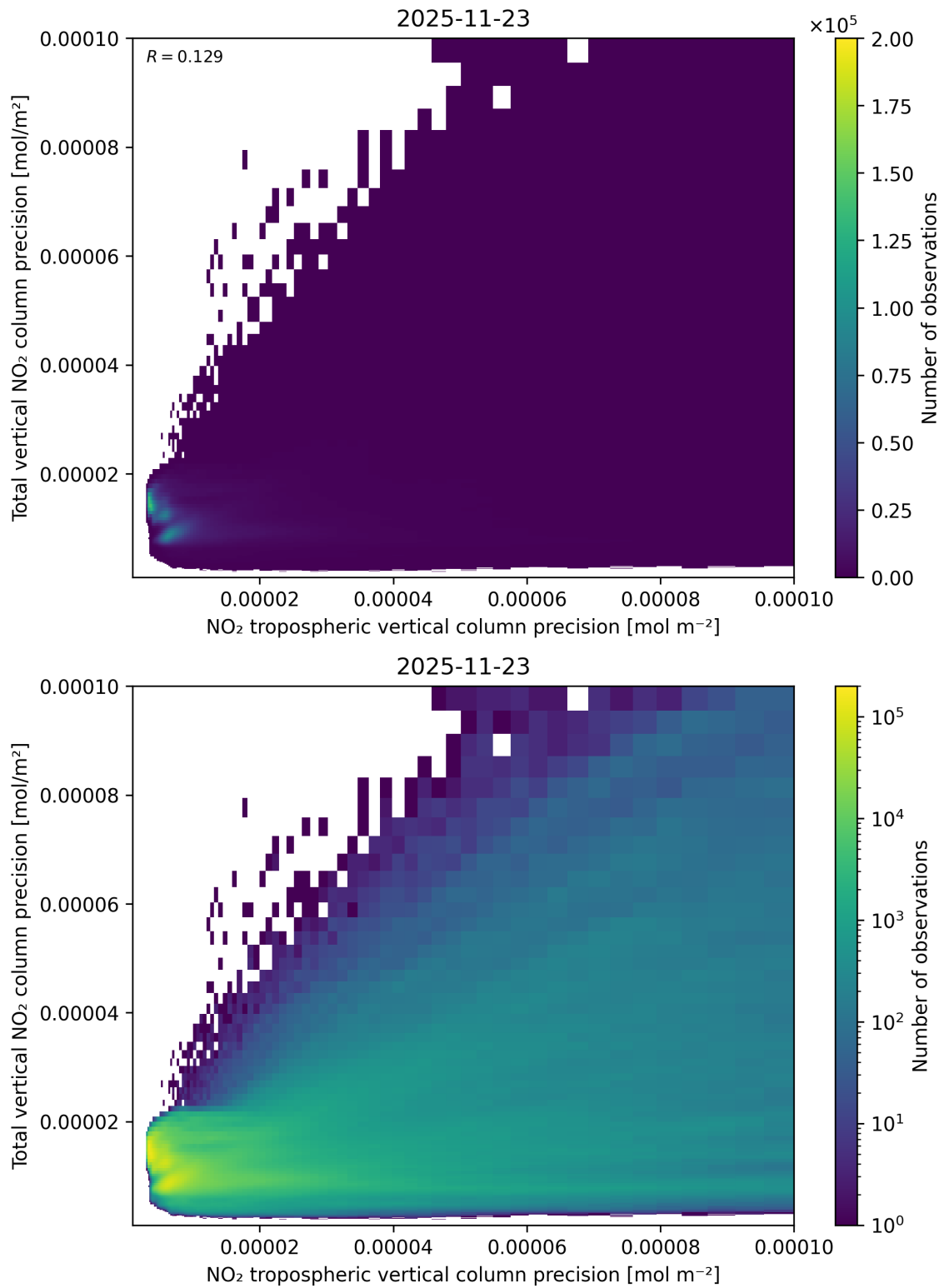
Figure 139: Scatter density plot of “NO 2 tropospheric vertical column precision” against “Total vertical NO 2 column precision” for 2025-11-23 to 2025-11-24.
