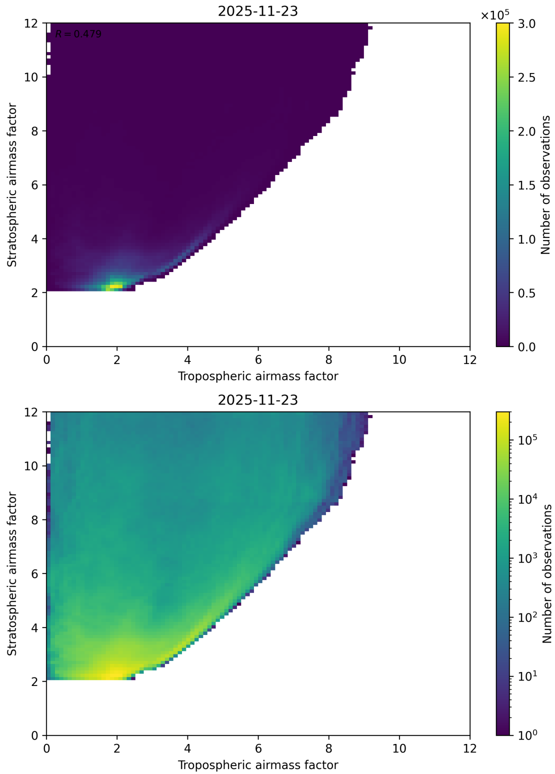
Figure 71: Scatter density plot of “Tropospheric airmass factor” against “Stratospheric airmass factor” for 2025-11-23 to 2025-11-24.
