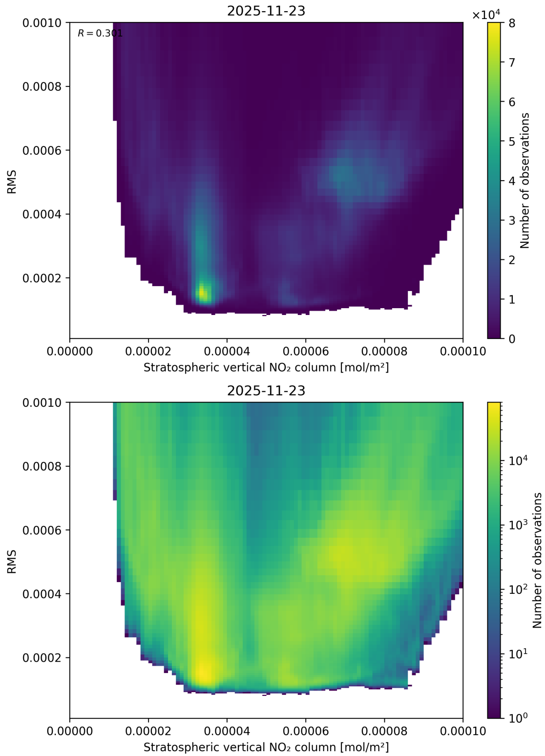
Figure 102: Scatter density plot of “Stratospheric vertical NO 2 column” against “RMS” for 2025-11-23 to 2025-11-24.
