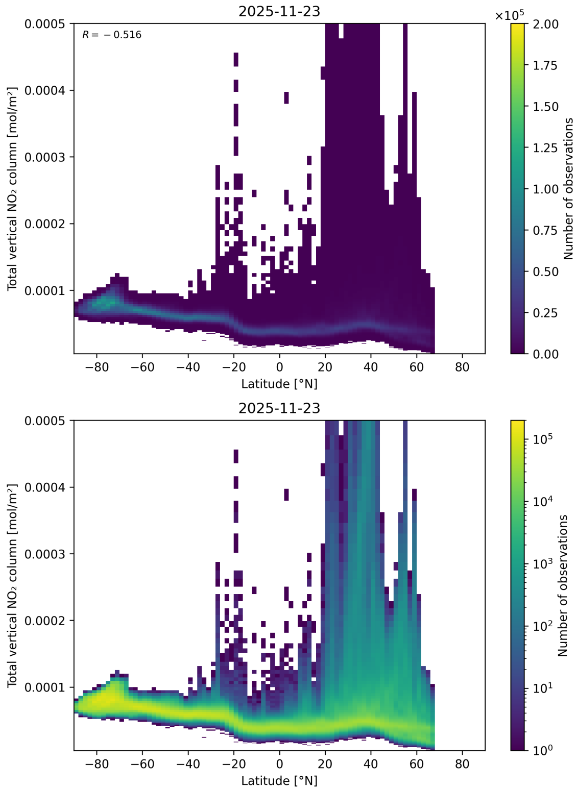
Figure 90: Scatter density plot of “Latitude” against “Total vertical NO 2 column” for 2025-11-23 to 2025-11-24.
