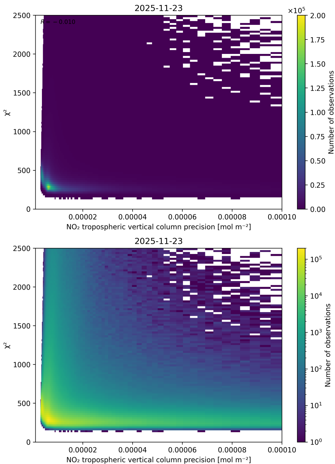
Figure 134: Scatter density plot of “NO 2 tropospheric vertical column precision” against “ \chi^2 ” for 2025-11-23 to 2025-11-24.
