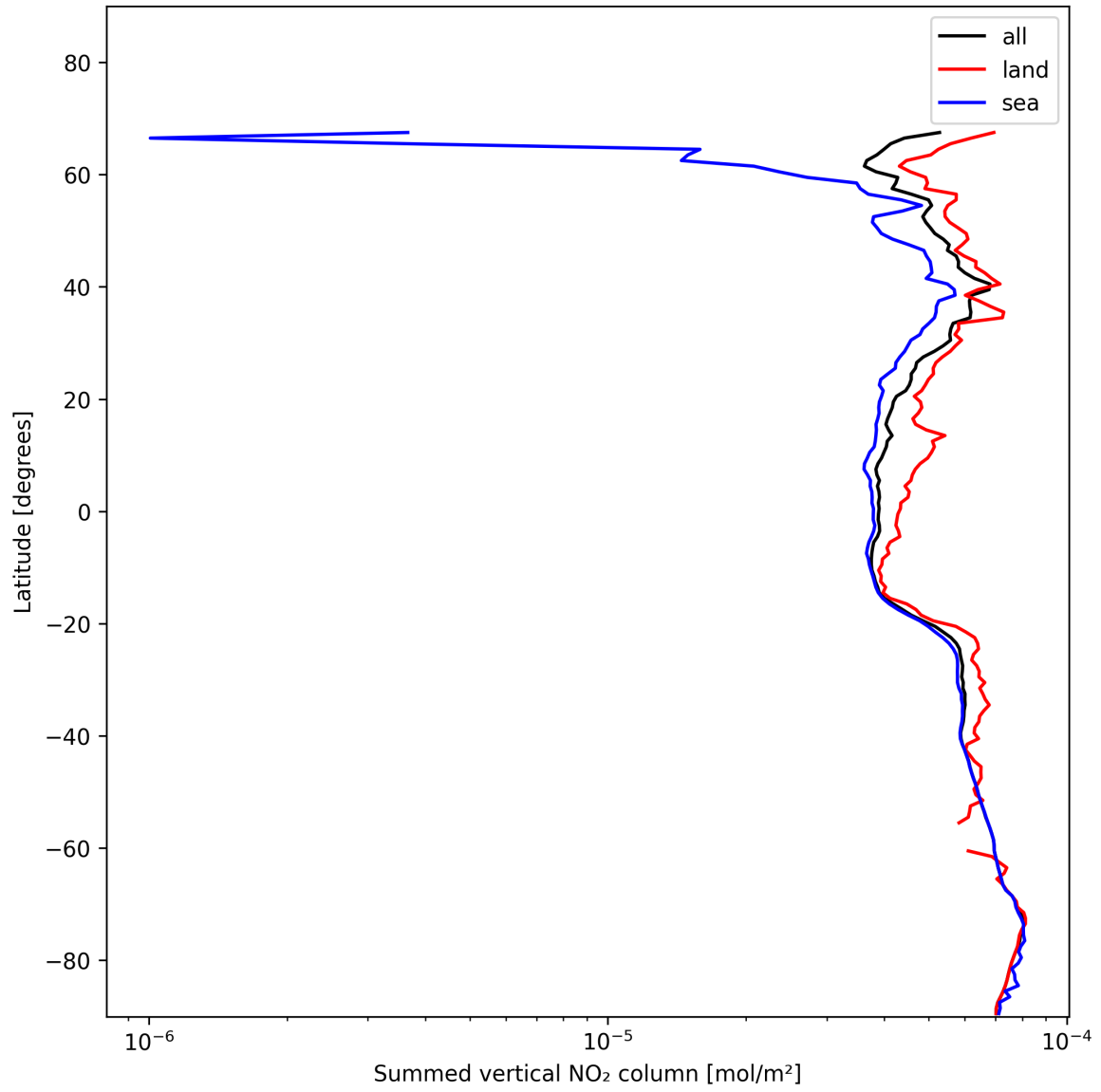
Figure 23: Zonal average of “Summed vertical NO 2 column” for 2025-11-23 to 2025-11-24.
