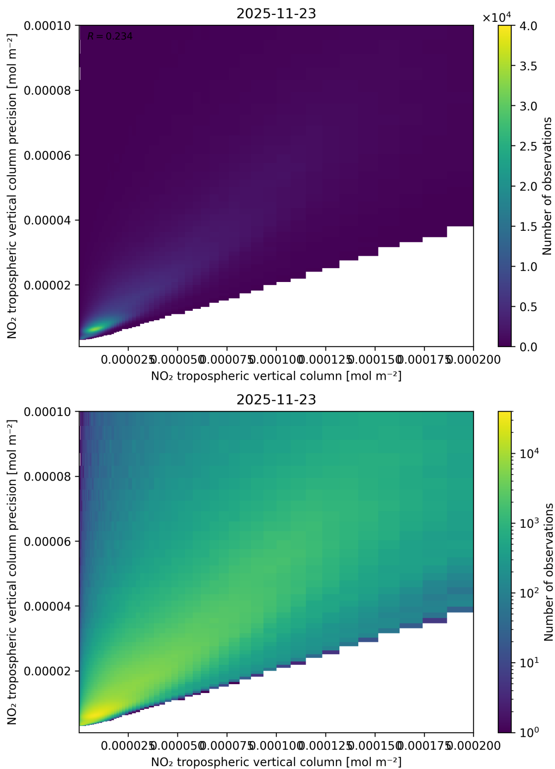
Figure 130: Scatter density plot of “NO 2 tropospheric vertical column” against “NO 2 tropospheric vertical column precision” for 2025-11-23 to 2025-11-24.
