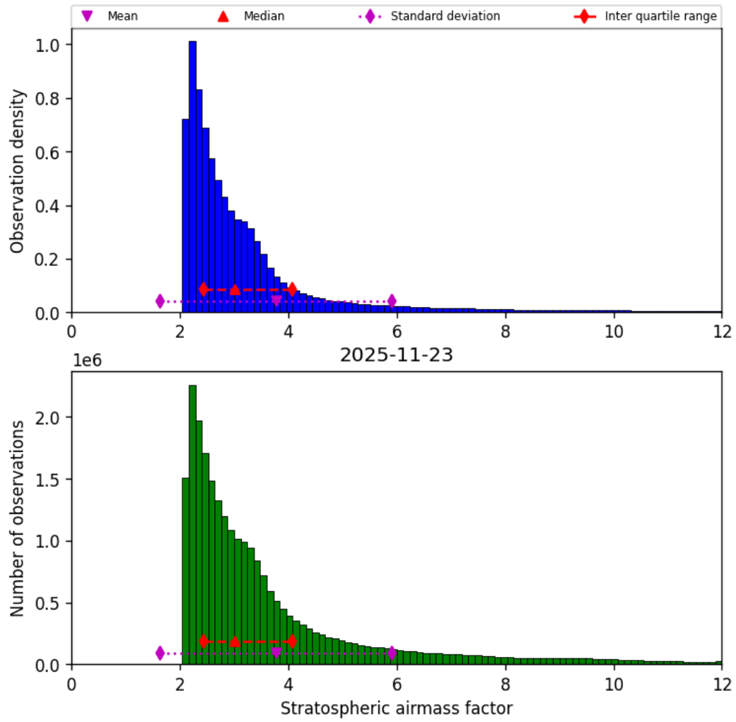
Figure 44: Histogram of “Stratospheric airmass factor” for 2025-11-23 to 2025-11-24
