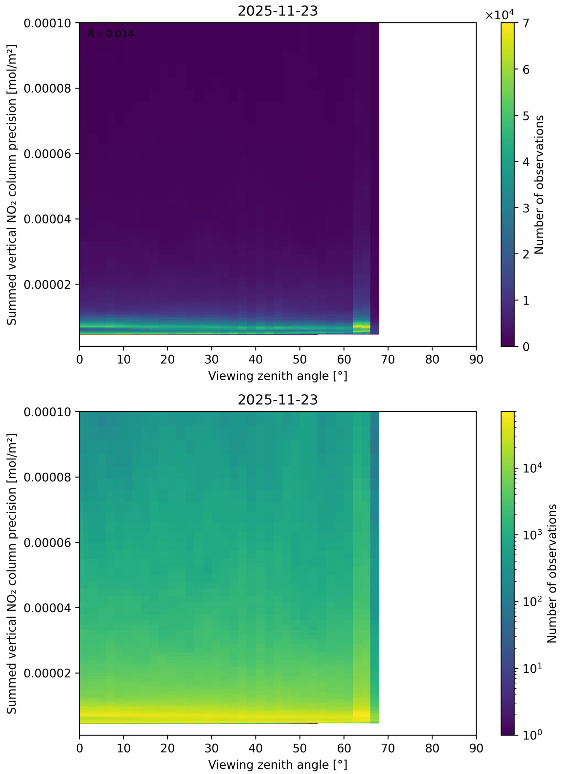
Figure 166: Scatter density plot of “Viewing zenith angle” against “Summed vertical NO 2 column precision” for 2025-11-23 to 2025-11-24.
