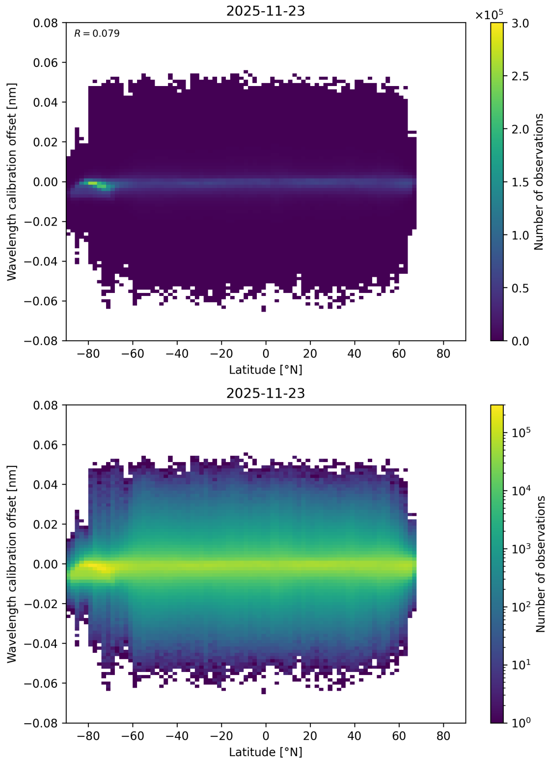
Figure 95: Scatter density plot of “Latitude” against “Wavelength calibration offset” for 2025-11-23 to 2025-11-24.
