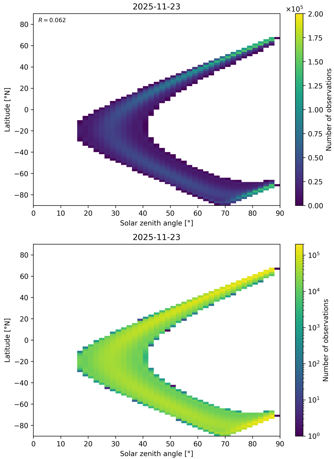
Figure 149: Scatter density plot of “Solar zenith angle” against “Latitude” for 2025-11-23 to 2025-11-24.
