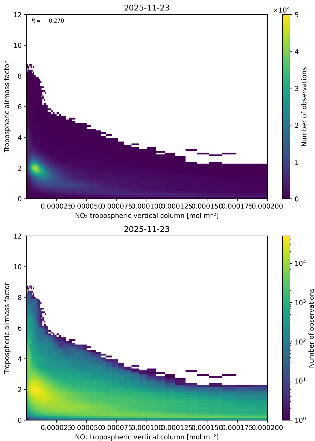
Figure 123: Scatter density plot of “NO 2 tropospheric vertical column” against “Tropospheric air mass factor” for 2025-11-23 to 2025-11-24.
