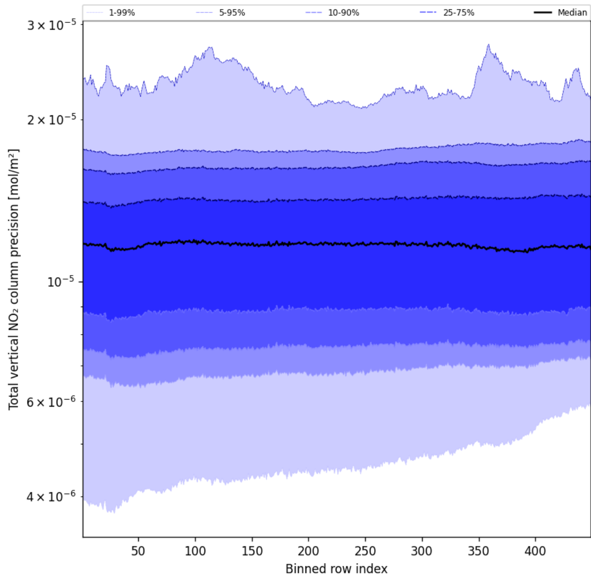
Figure 56: Along track statistics of “Total vertical NO 2 column precision” for 2025-11-23 to 2025-11-24
