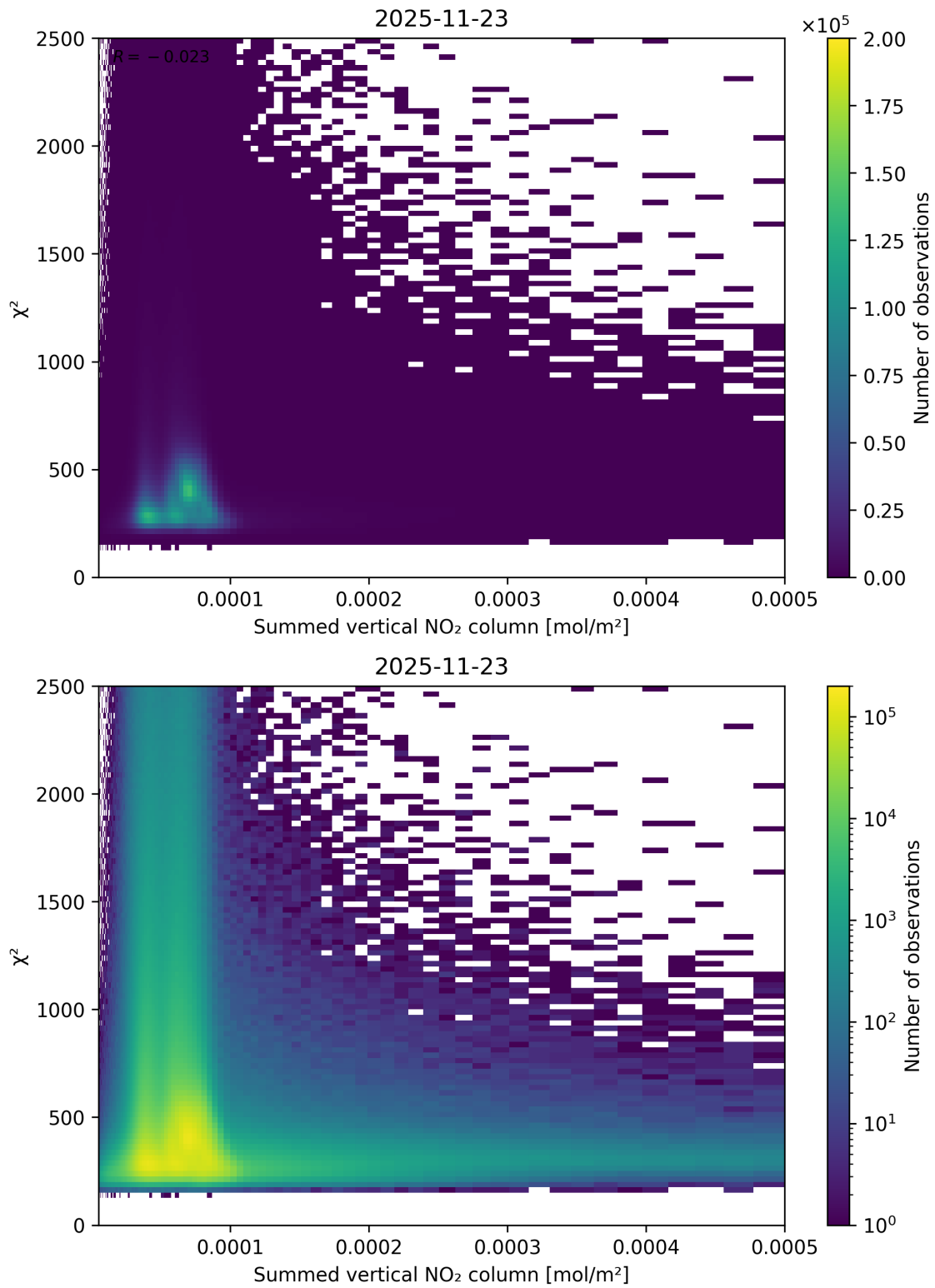
Figure 104: Scatter density plot of “Summed vertical NO 2 column” against “ \chi^2 ” for 2025-11-23 to 2025-11-24.
