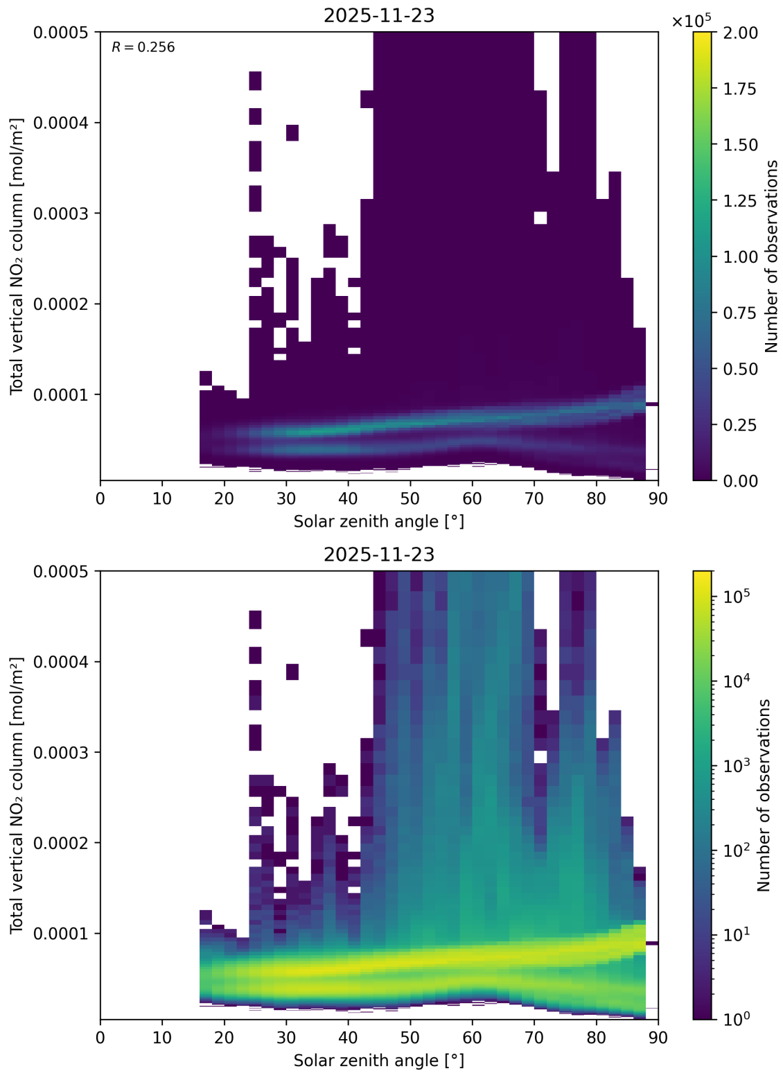
Figure 153: Scatter density plot of “Solar zenith angle” against “Total vertical NO 2 column” for 2025-11-23 to 2025-11-24.
