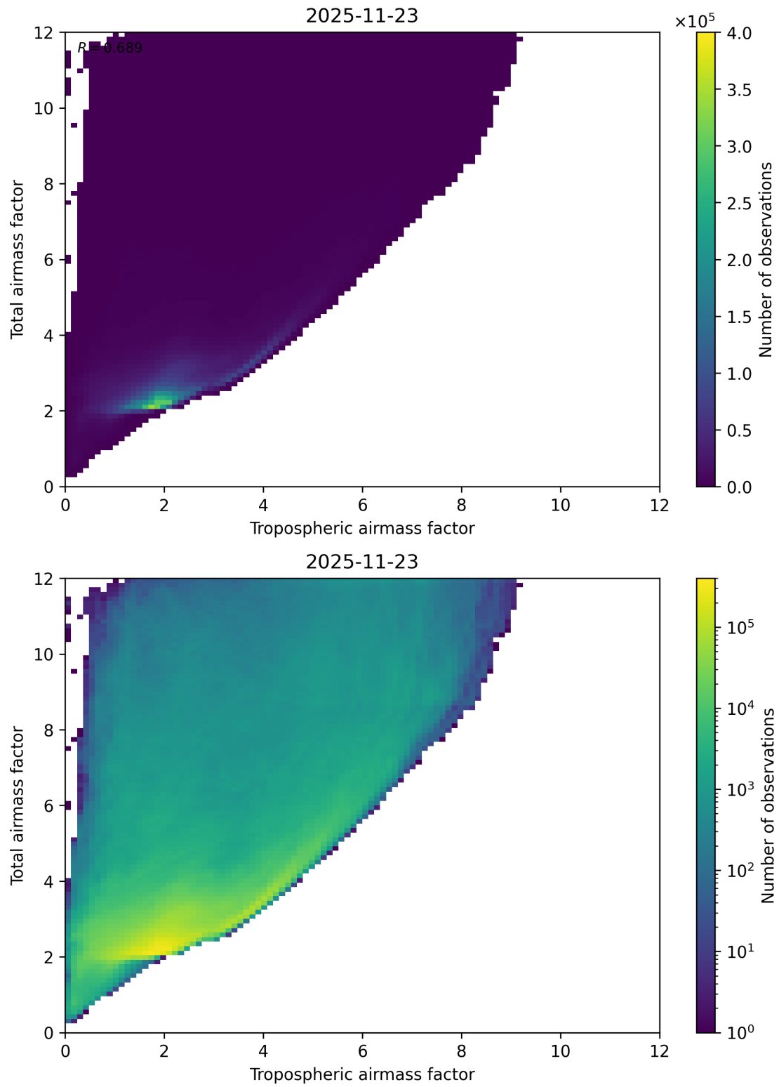
Figure 72: Scatter density plot of “Tropospheric airmass factor” against “Total airmass factor” for 2025-11-23 to 2025-11-24.
