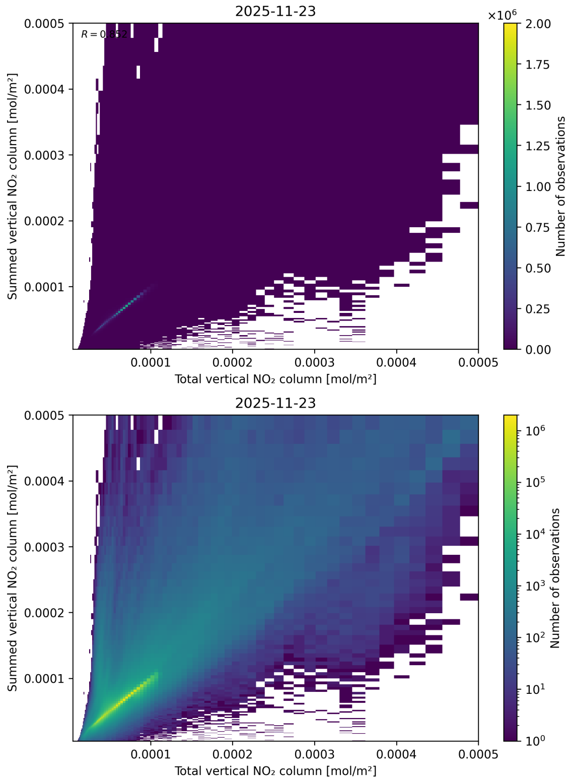
Figure 112: Scatter density plot of “Total vertical NO 2 column” against “Summed vertical NO 2 column” for 2025-11-23 to 2025-11-24.
