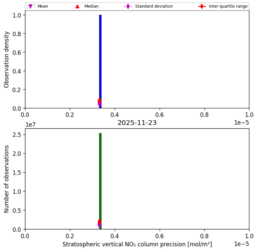
Figure 37: Histogram of “Stratospheric vertical NO 2 column precision” for 2025-11-23 to 2025-11-24
