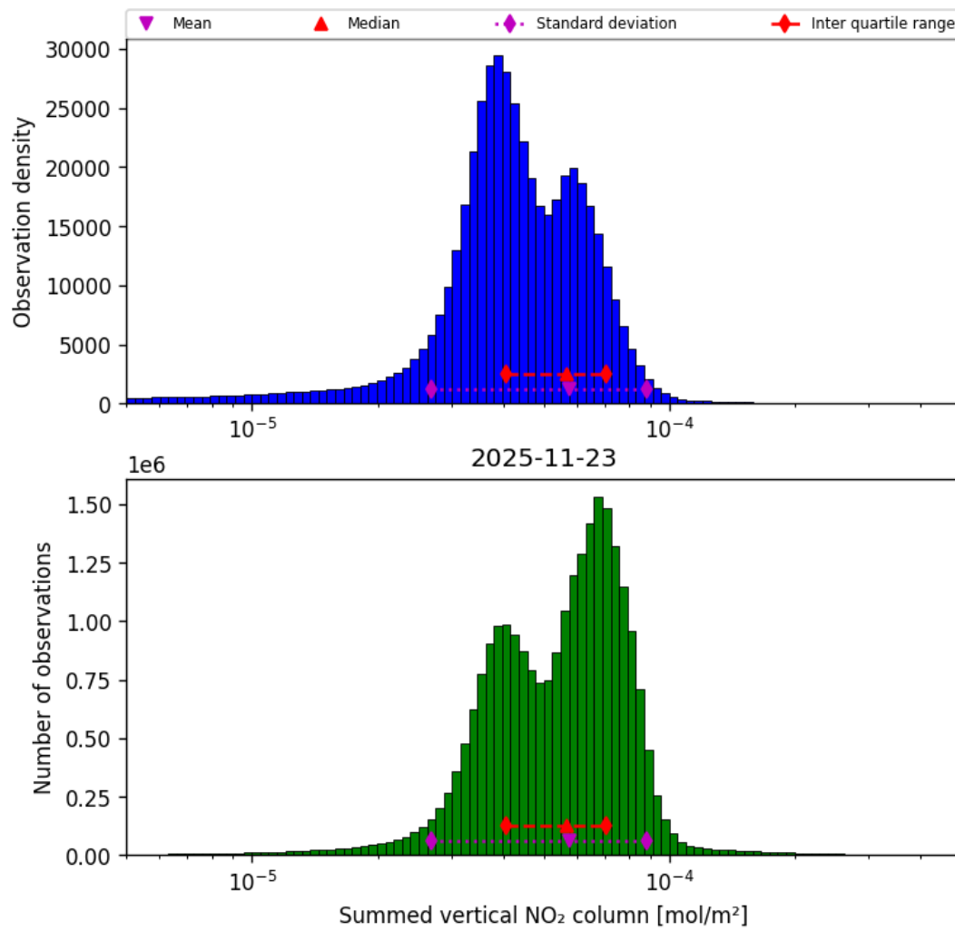
Figure 40: Histogram of “Summed vertical NO 2 column” for 2025-11-23 to 2025-11-24
