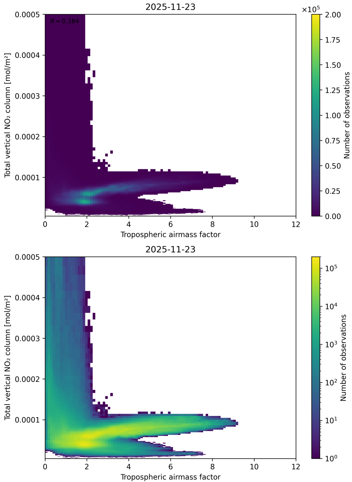
Figure 77: Scatter density plot of “Tropospheric airmass factor” against “Total vertical \text{NO}_2 column” for 2025-11-23 to 2025-11-24.
