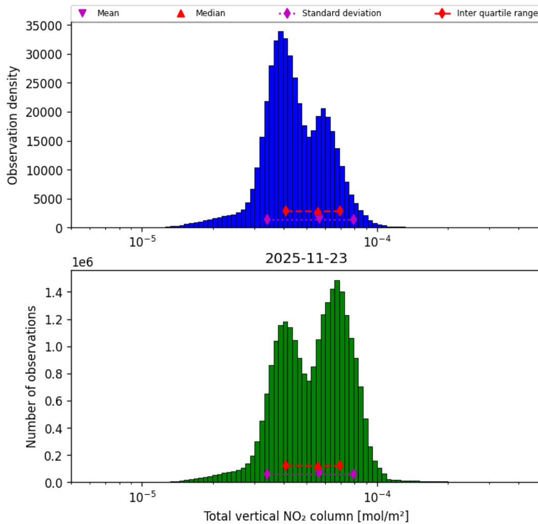
Figure 38: Histogram of “Total vertical NO 2 column” for 2025-11-23 to 2025-11-24
