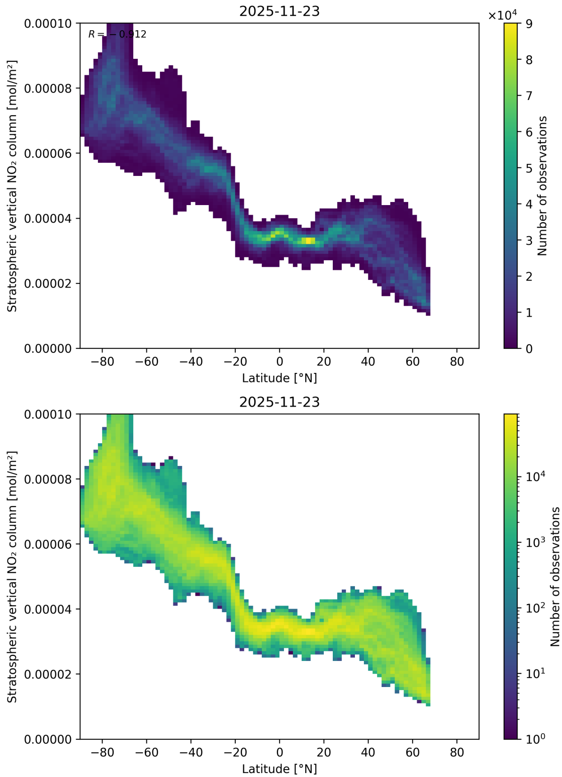
Figure 87: Scatter density plot of “Latitude” against “Stratospheric vertical NO 2 column” for 2025-11-23 to 2025-11-24.
