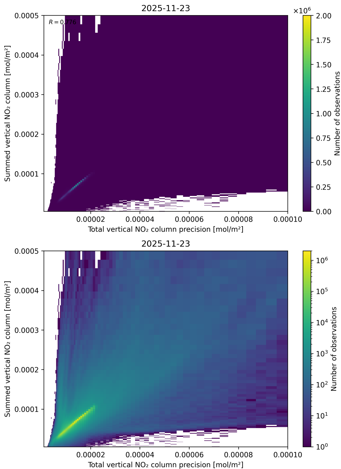
Figure 117: Scatter density plot of “Total vertical NO 2 column precision” against “Summed vertical NO 2 column” for 2025-11-23 to 2025-11-24.
