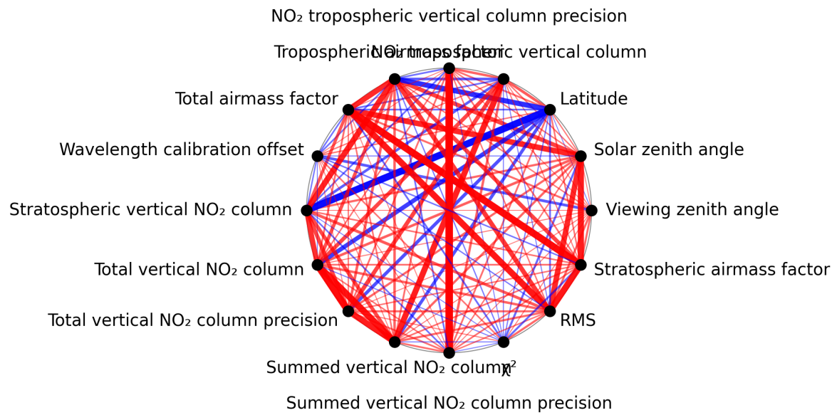
Figure 1: Map of correlation graph for 2025-11-23 to 2025-11-24.
