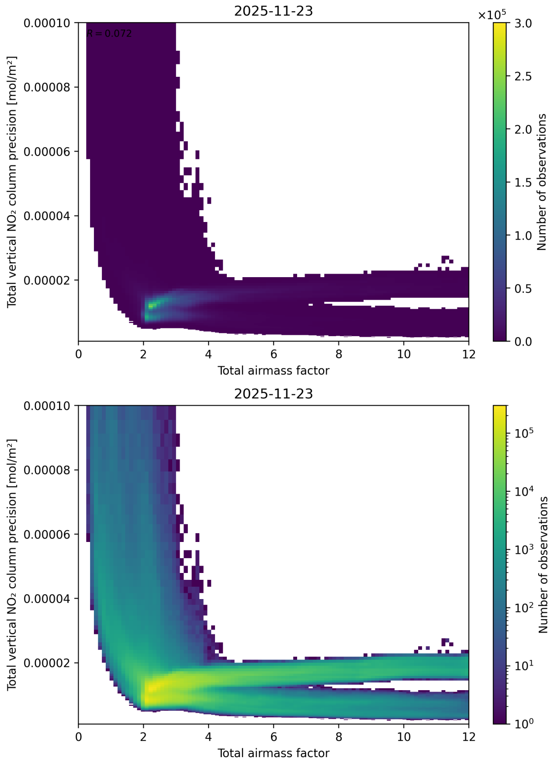
Figure 68: Scatter density plot of “Total airmass factor” against “Total vertical NO 2 column precision” for 2025-11-23 to 2025-11-24.
