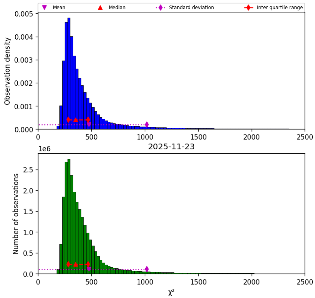
Figure 42: Histogram of “ \chi^2 ” for 2025-11-23 to 2025-11-24
