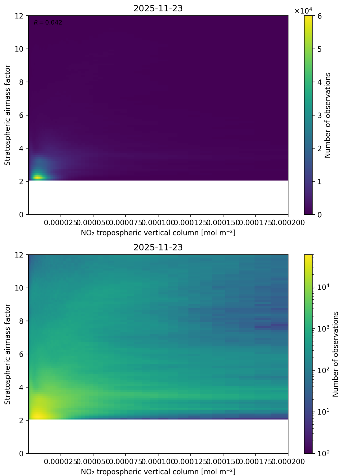
Figure 121: Scatter density plot of “NO 2 tropospheric vertical column” against “Stratospheric airmass factor” for 2025-11-23 to 2025-11-24.
