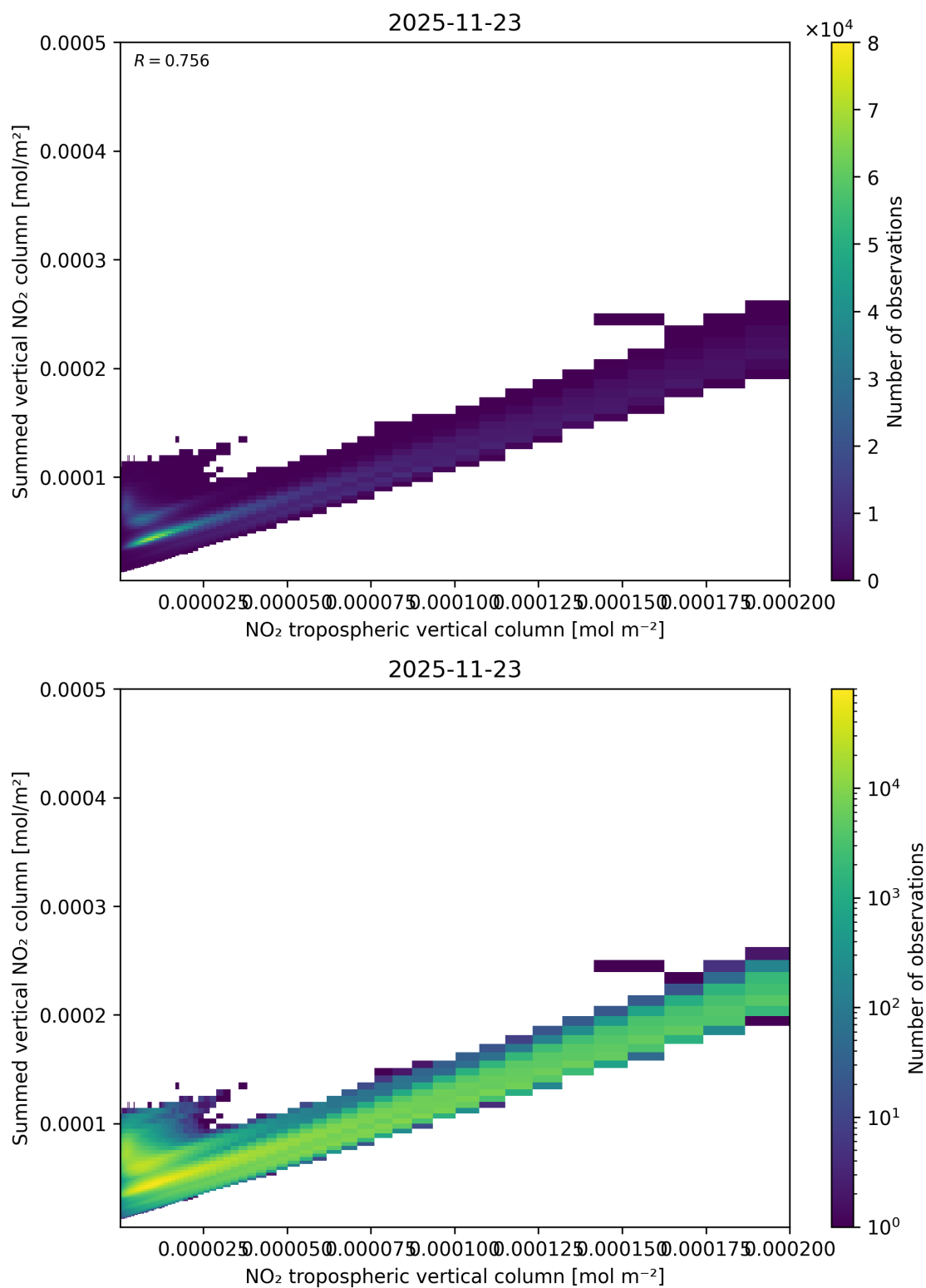
Figure 126: Scatter density plot of “NO 2 tropospheric vertical column” against “Summed vertical NO 2 column” for 2025-11-23 to 2025-11-24.
