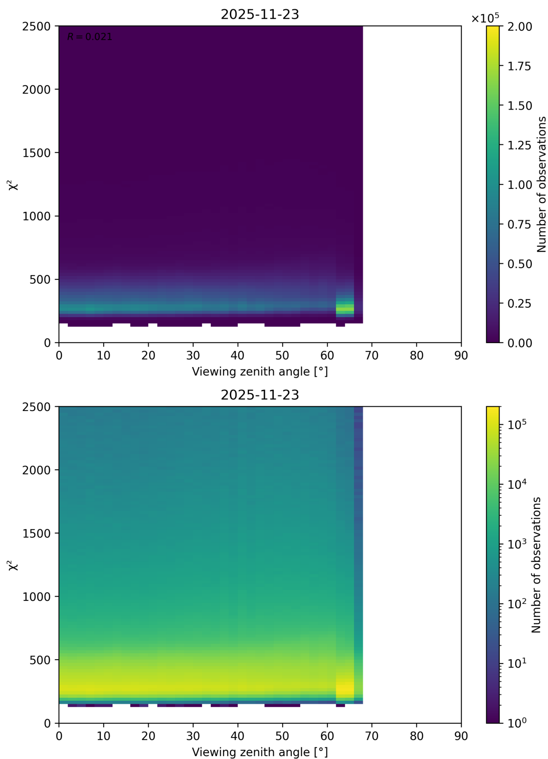
Figure 162: Scatter density plot of “Viewing zenith angle” against “ \chi^2 ” for 2025-11-23 to 2025-11-24.
