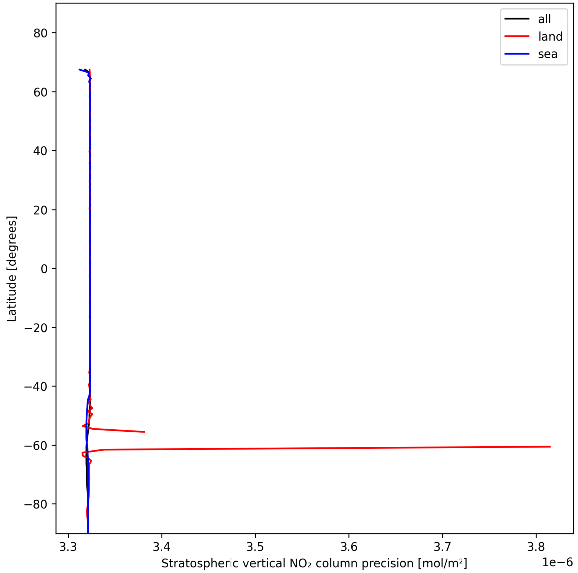
Figure 20: Zonal average of “Stratospheric vertical NO 2 column precision” for 2025-11-23 to 2025-11-24.
