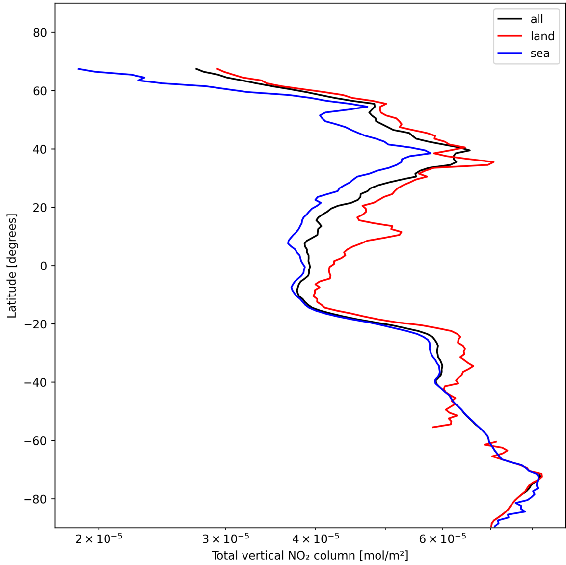
Figure 21: Zonal average of “Total vertical NO 2 column” for 2025-11-23 to 2025-11-24.
