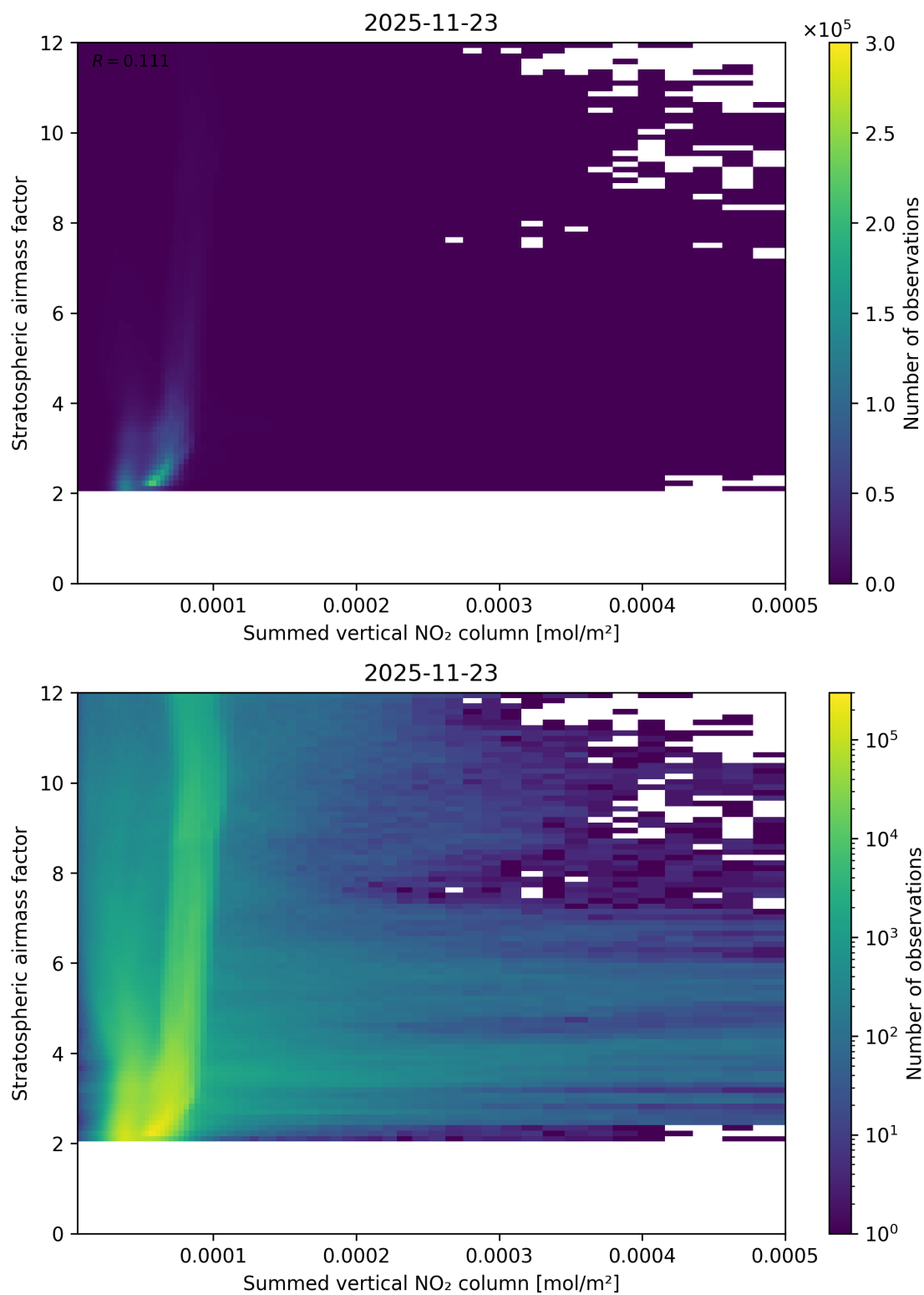
Figure 103: Scatter density plot of “Summed vertical NO 2 column” against “Stratospheric airmass factor” for 2025-11-23 to 2025-11-24.
