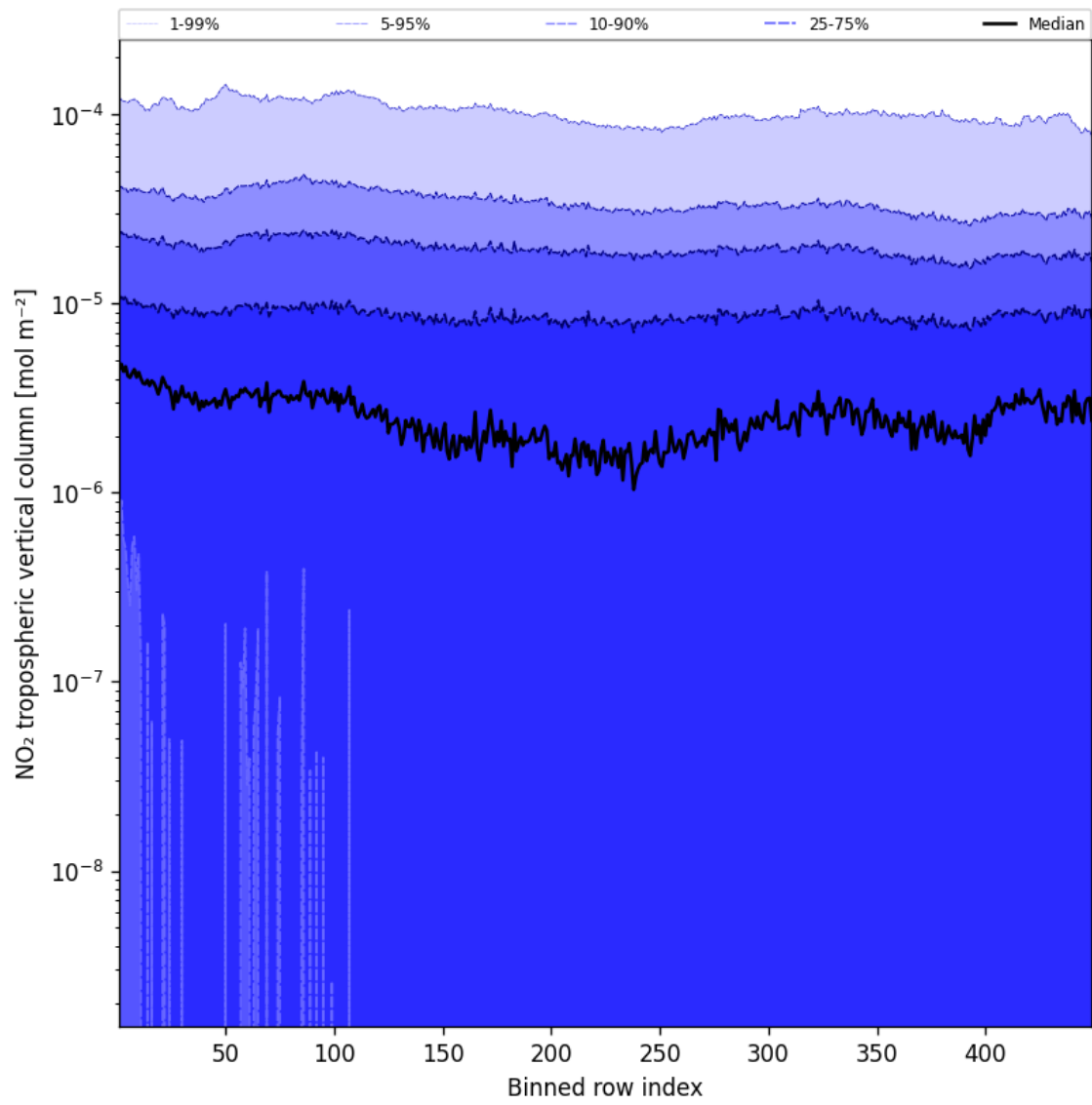
Figure 46: Along track statistics of “NO 2 tropospheric vertical column” for 2025-11-23 to 2025-11-24
