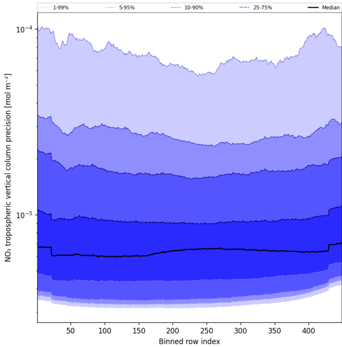
Figure 47: Along track statistics of “NO 2 tropospheric vertical column precision” for 2025-11-23 to 2025-11-24
