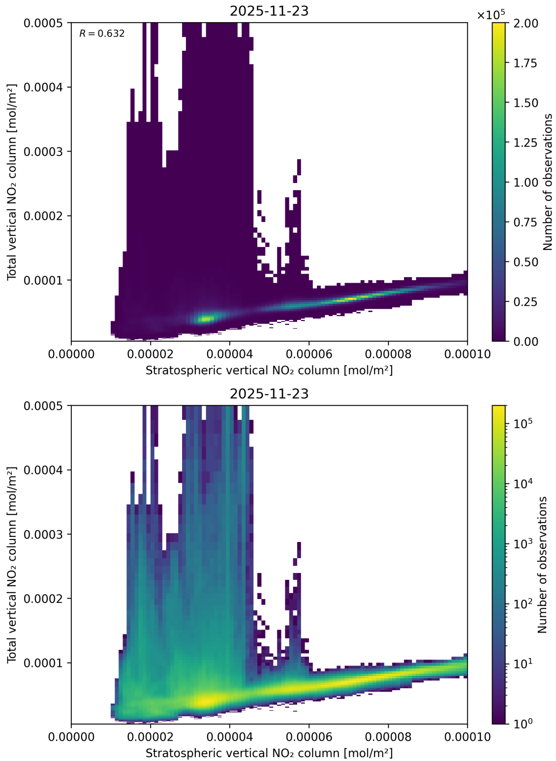
Figure 100: Scatter density plot of “Stratospheric vertical NO 2 column” against “Total vertical NO 2 column” for 2025-11-23 to 2025-11-24.
