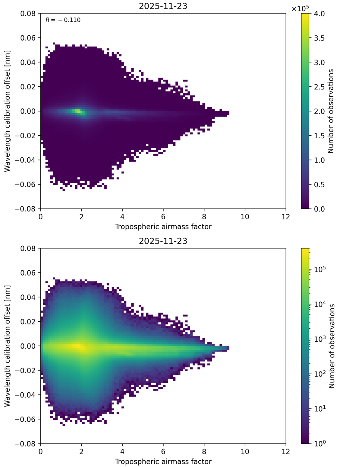
Figure 80: Scatter density plot of “Tropospheric airmass factor” against “Wavelength calibration offset” for 2025-11-23 to 2025-11-24.
