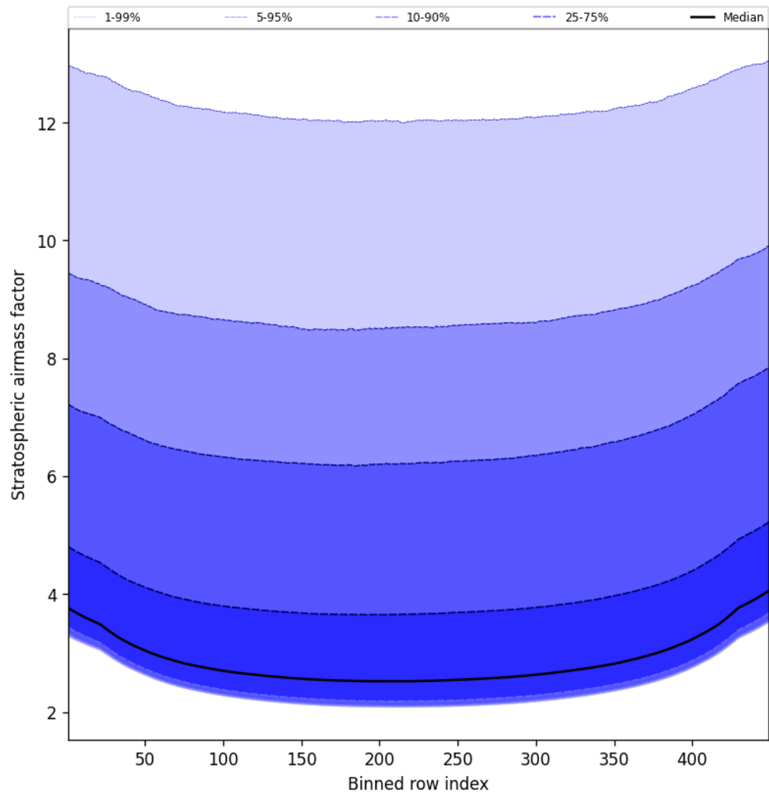
Figure 61: Along track statistics of “Stratospheric air mass factor” for 2025-11-23 to 2025-11-24
