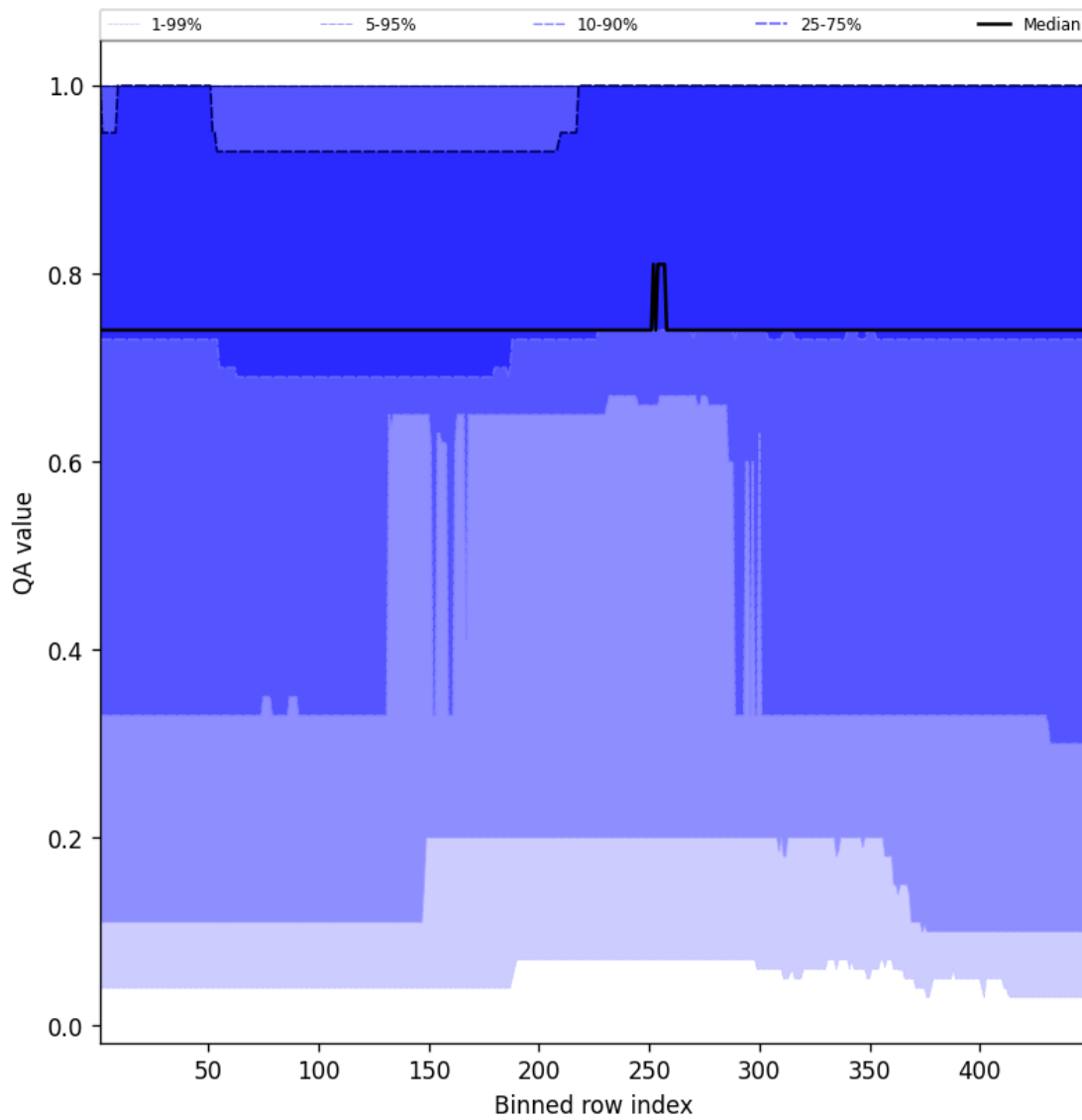
Figure 45: Along track statistics of “QA value” for 2025-11-23 to 2025-11-24
