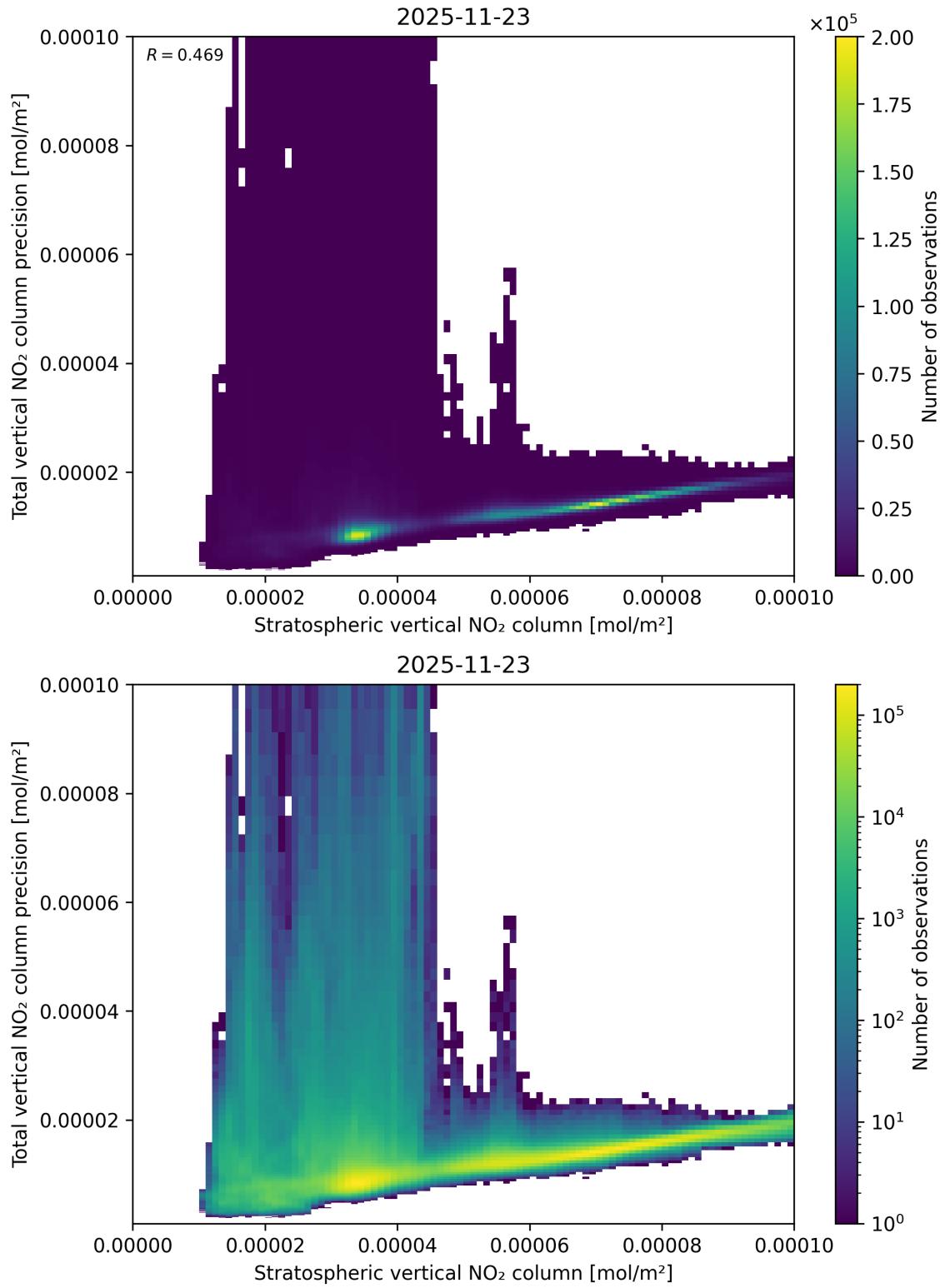
Figure 101: Scatter density plot of “Stratospheric vertical NO 2 column” against “Total vertical NO 2 column precision” for 2025-11-23 to 2025-11-24.
