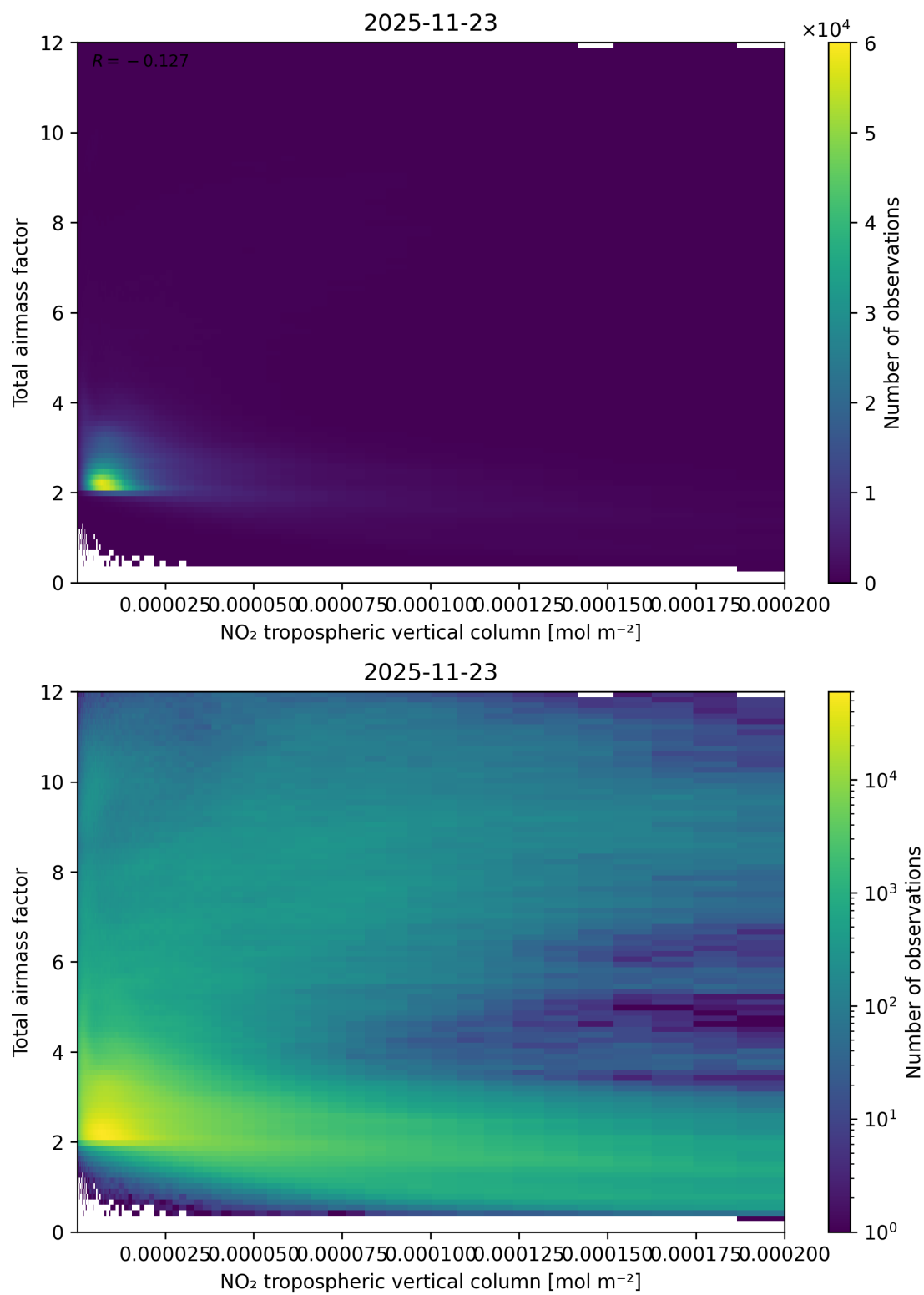
Figure 122: Scatter density plot of “NO 2 tropospheric vertical column” against “Total air mass factor” for 2025-11-23 to 2025-11-24.
