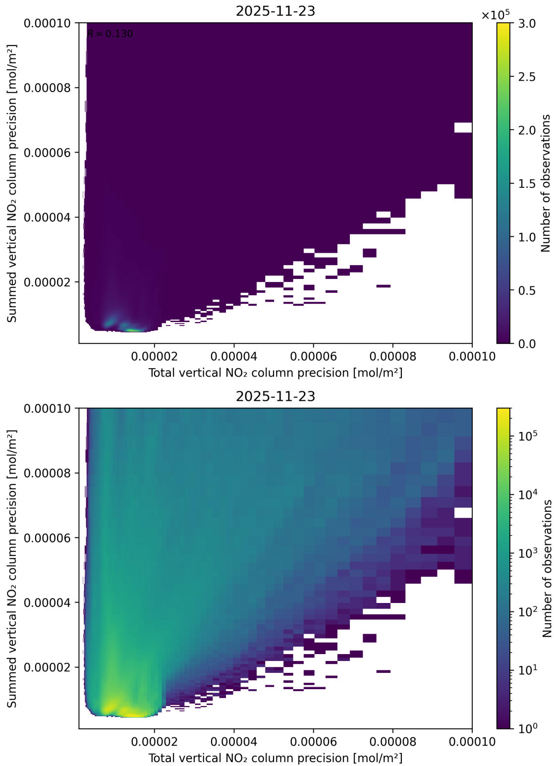
Figure 118: Scatter density plot of “Total vertical NO 2 column precision” against “Summed vertical NO 2 column precision” for 2025-11-23 to 2025-11-24.
