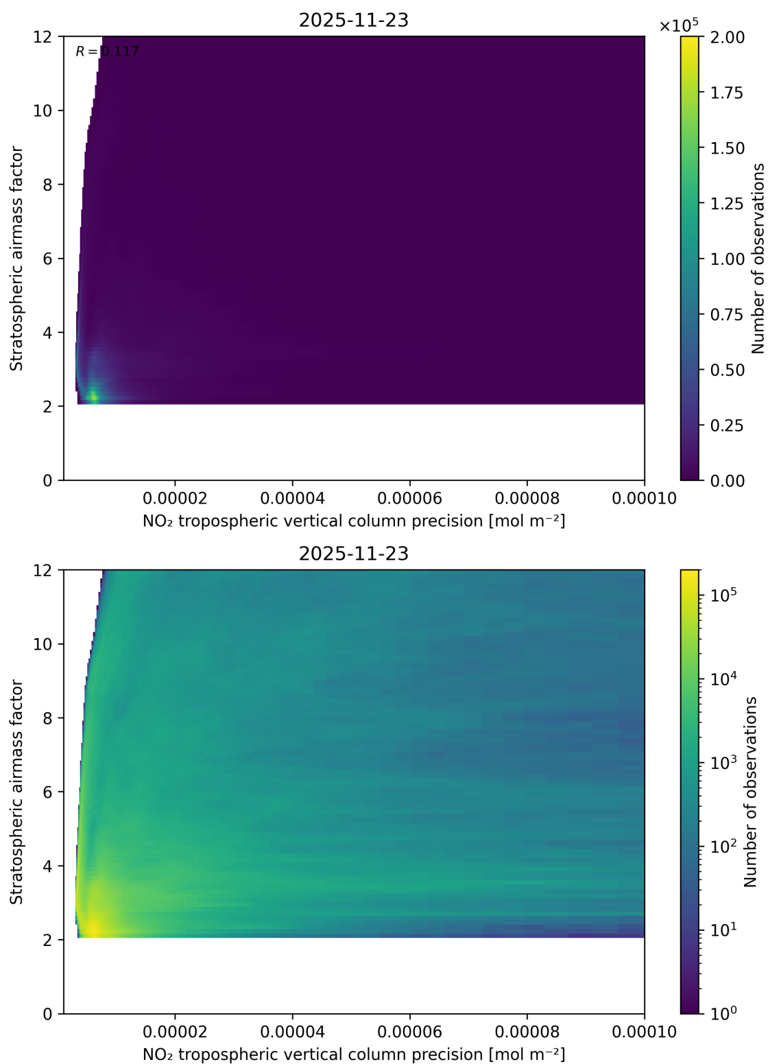
Figure 131: Scatter density plot of “NO 2 tropospheric vertical column precision” against “Stratospheric airmass factor” for 2025-11-23 to 2025-11-24.
