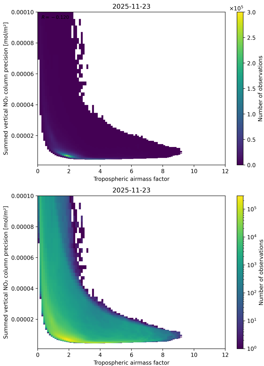
Figure 76: Scatter density plot of “Tropospheric air mass factor” against “Summed vertical NO 2 column precision” for 2025-11-23 to 2025-11-24.
