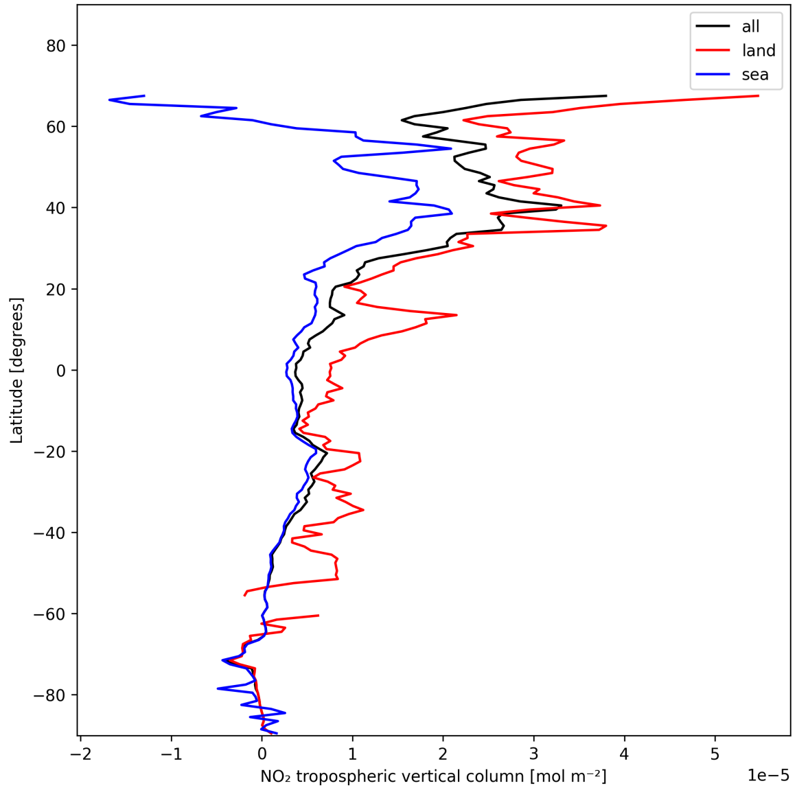
Figure 12: Zonal average of “NO 2 tropospheric vertical column” for 2025-11-23 to 2025-11-24.
