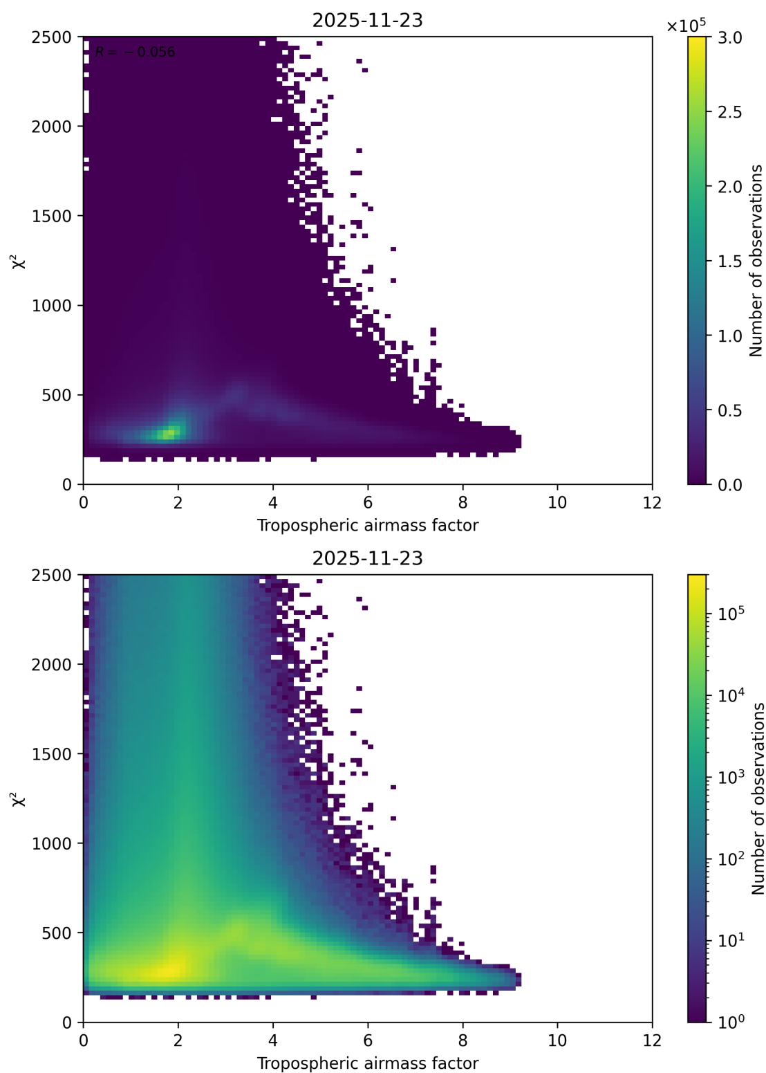
Figure 73: Scatter density plot of “Tropospheric airmass factor” against “ \chi^2 ” for 2025-11-23 to 2025-11-24.
