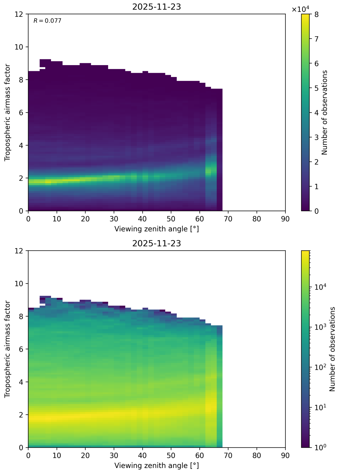
Figure 161: Scatter density plot of “Viewing zenith angle” against “Tropospheric airmass factor” for 2025-11-23 to 2025-11-24.
