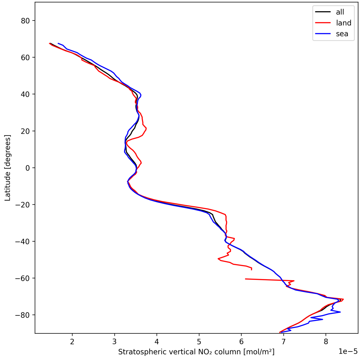
Figure 19: Zonal average of “Stratospheric vertical NO 2 column” for 2025-11-23 to 2025-11-24.
