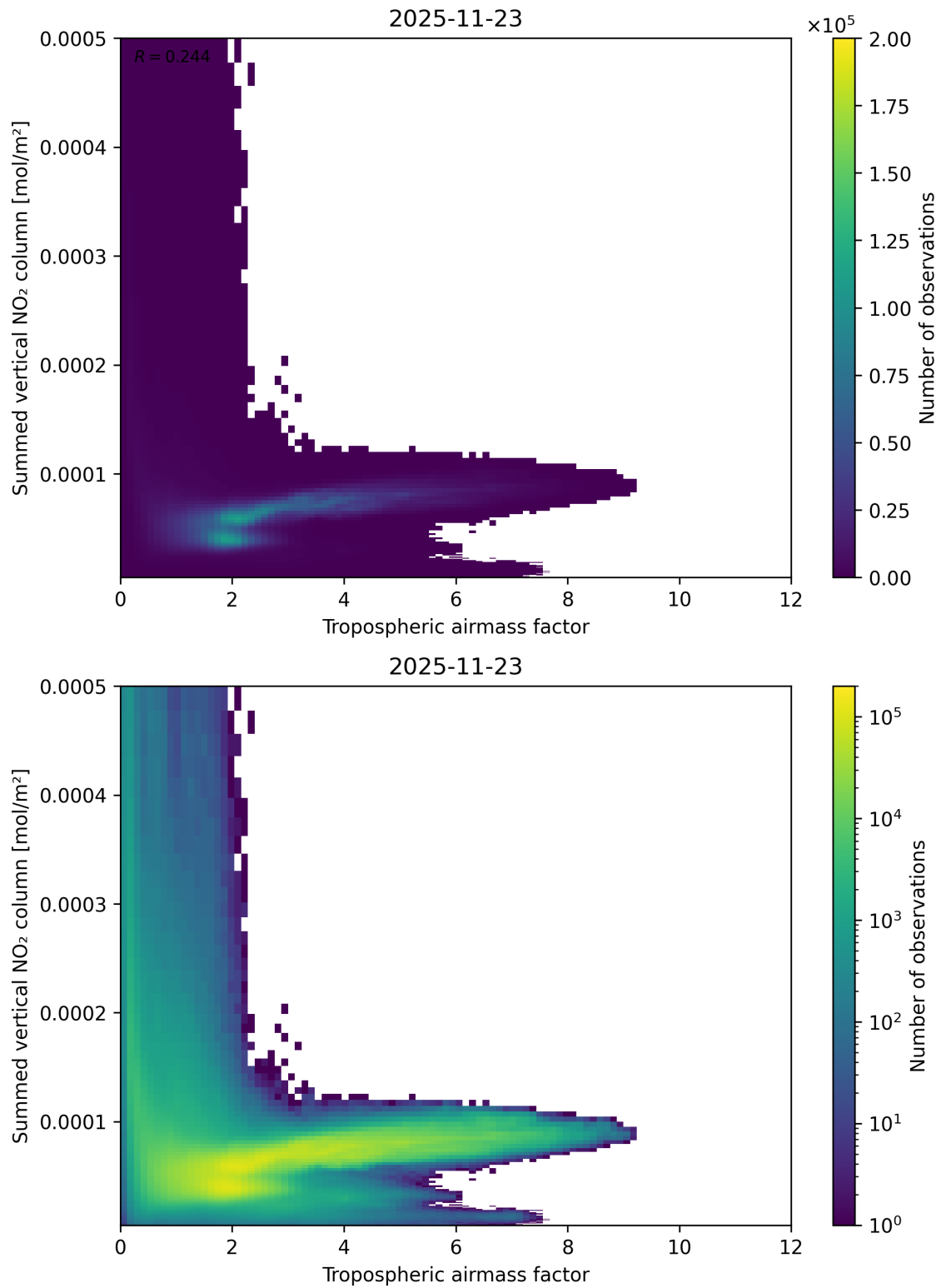
Figure 75: Scatter density plot of “Tropospheric air mass factor” against “Summed vertical NO 2 column” for 2025-11-23 to 2025-11-24.
