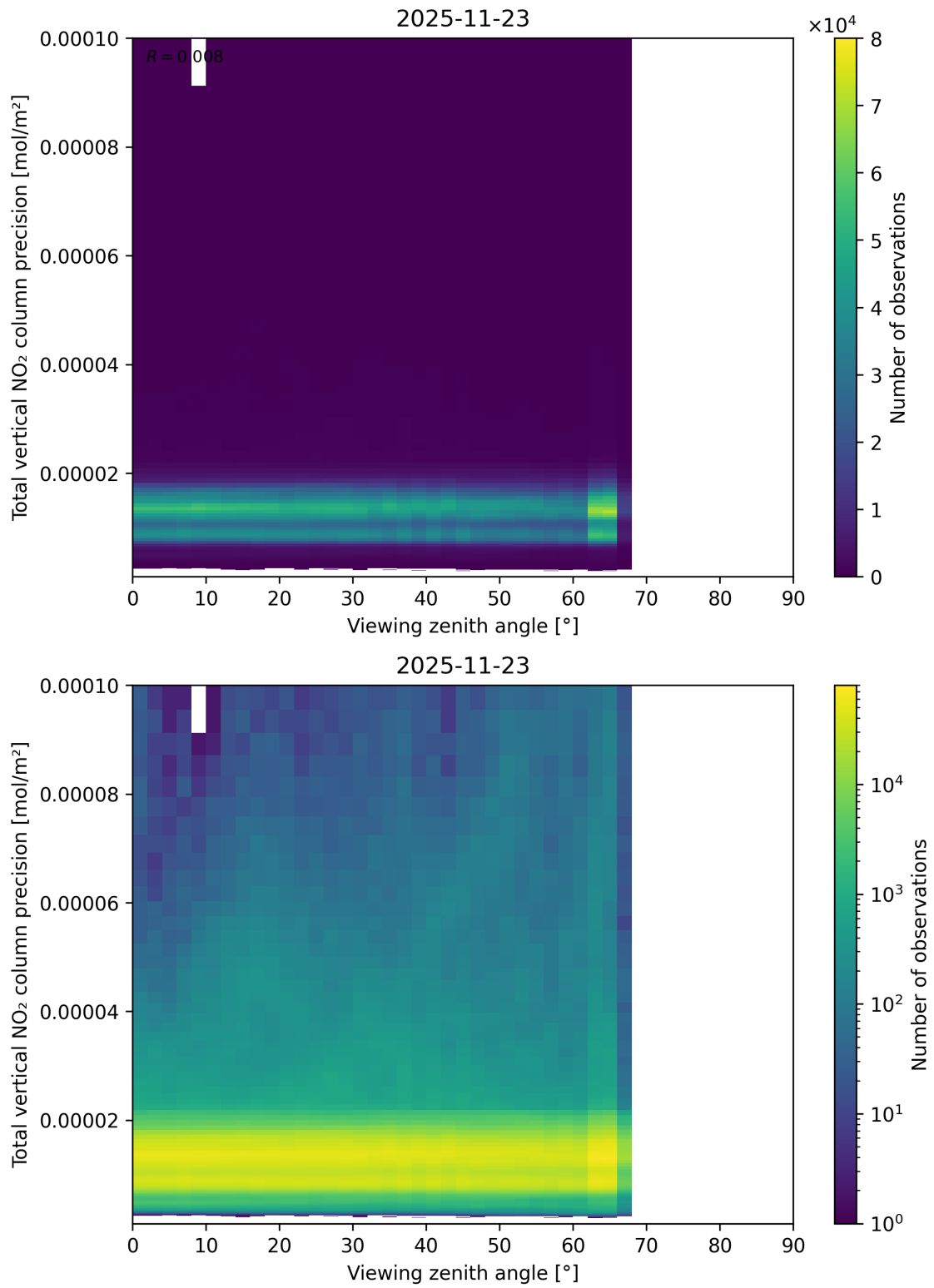
Figure 168: Scatter density plot of “Viewing zenith angle” against “Total vertical NO 2 column precision” for 2025-11-23 to 2025-11-24.
