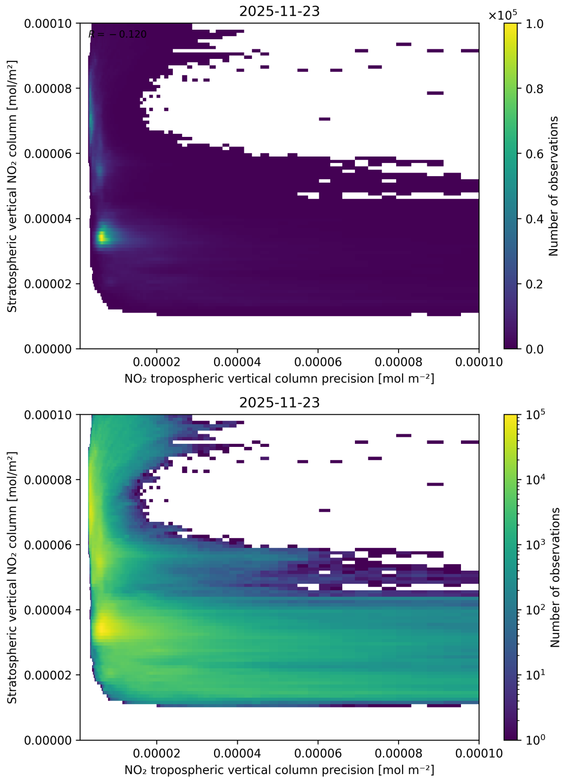
Figure 135: Scatter density plot of “NO 2 tropospheric vertical column precision” against “Stratospheric vertical NO 2 column” for 2025-11-23 to 2025-11-24.
