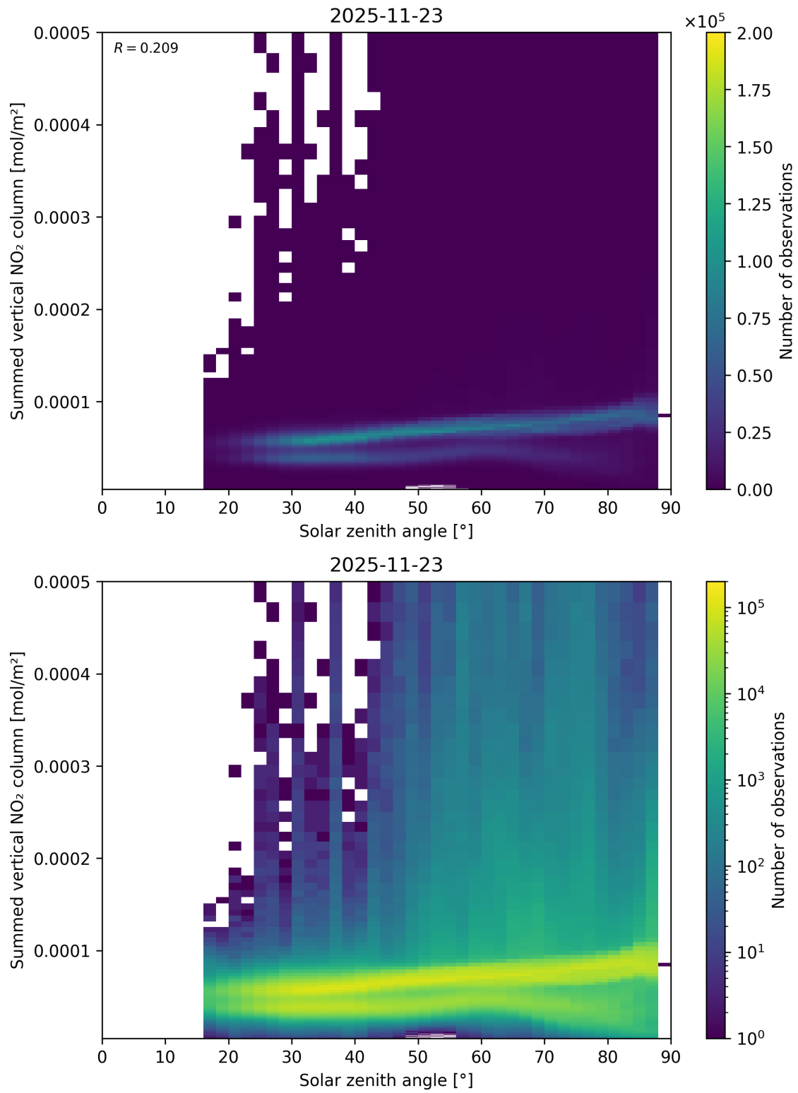
Figure 151: Scatter density plot of “Solar zenith angle” against “Summed vertical NO 2 column” for 2025-11-23 to 2025-11-24.
