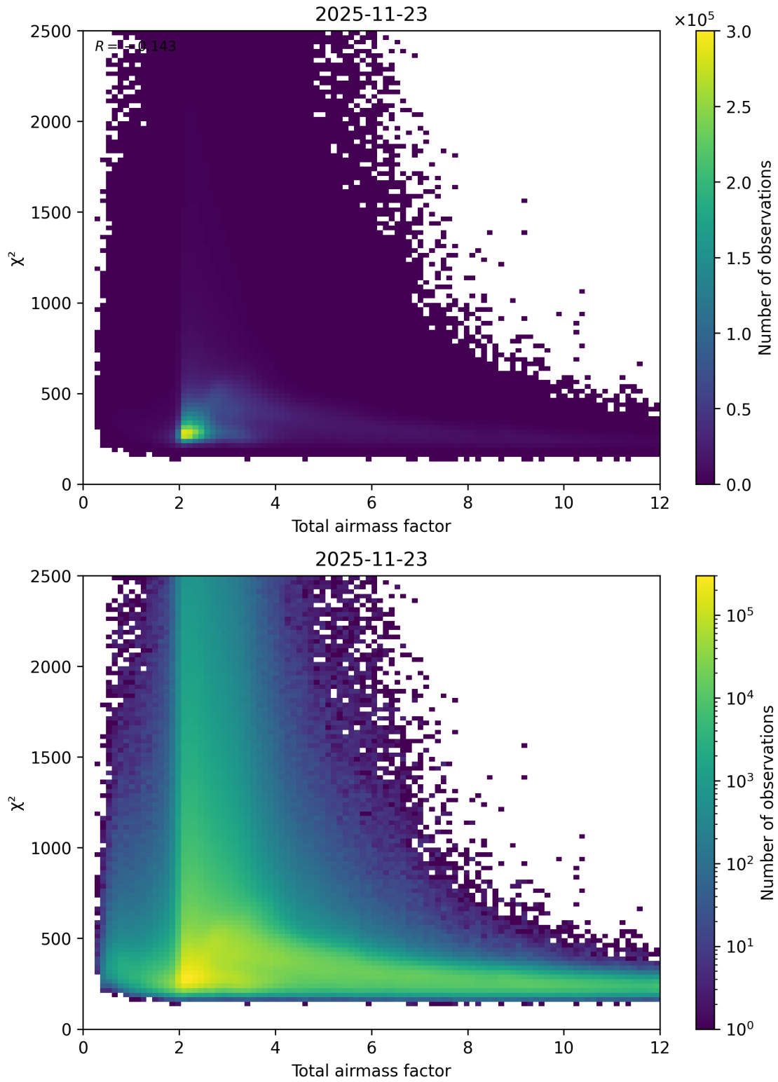
Figure 63: Scatter density plot of “Total airmass factor” against “ \chi^2 ” for 2025-11-23 to 2025-11-24.
