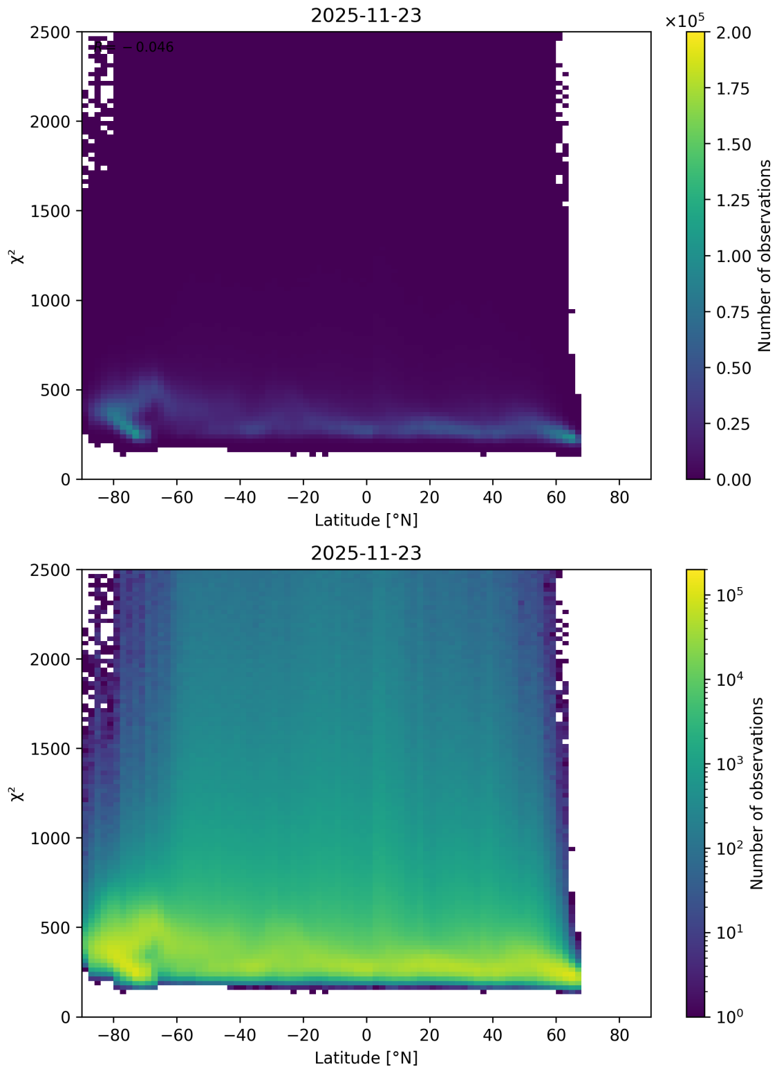
Figure 86: Scatter density plot of “Latitude” against “ \chi^2 ” for 2025-11-23 to 2025-11-24.
