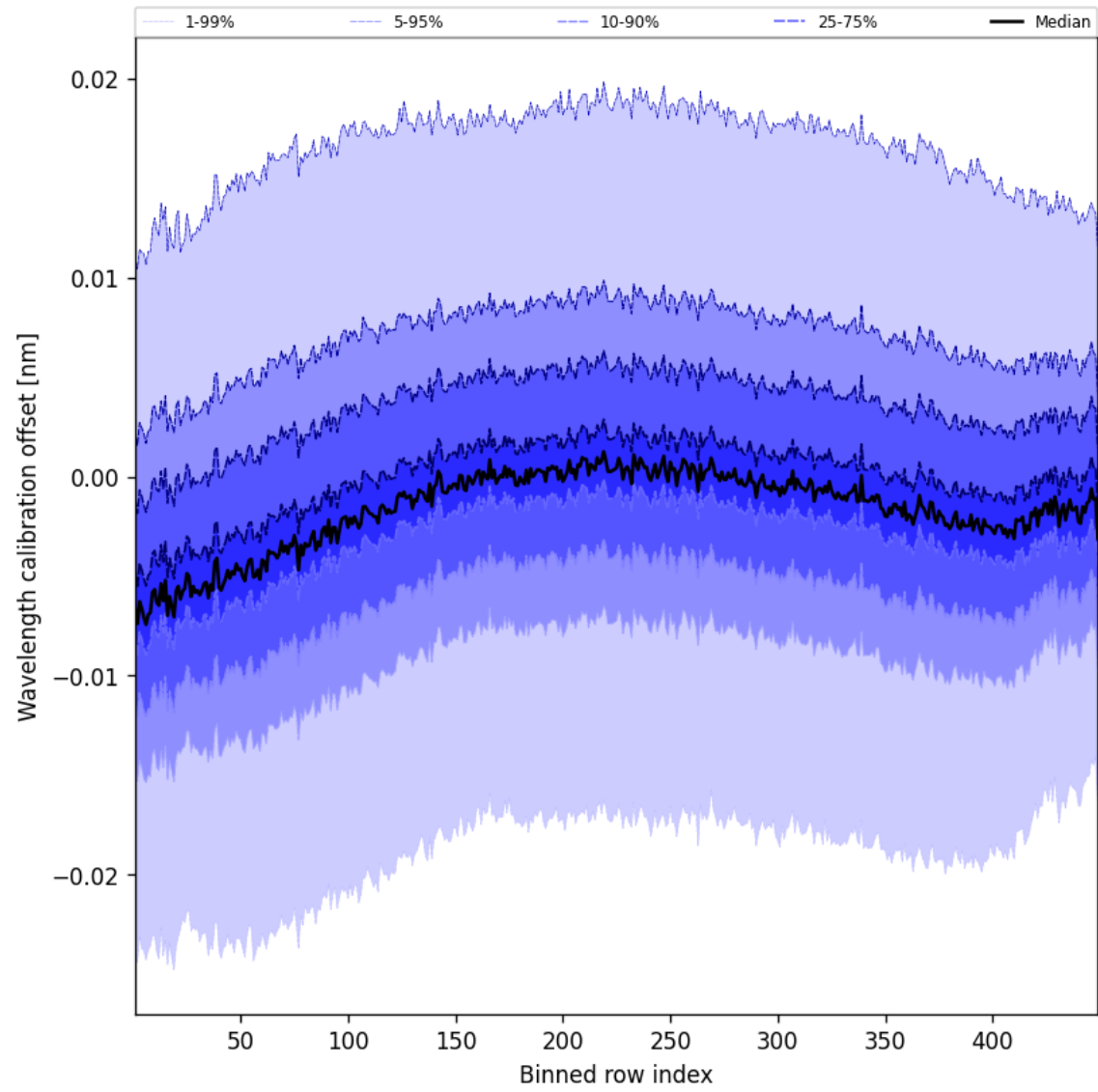
Figure 52: Along track statistics of “Wavelength calibration offset” for 2025-11-23 to 2025-11-24
