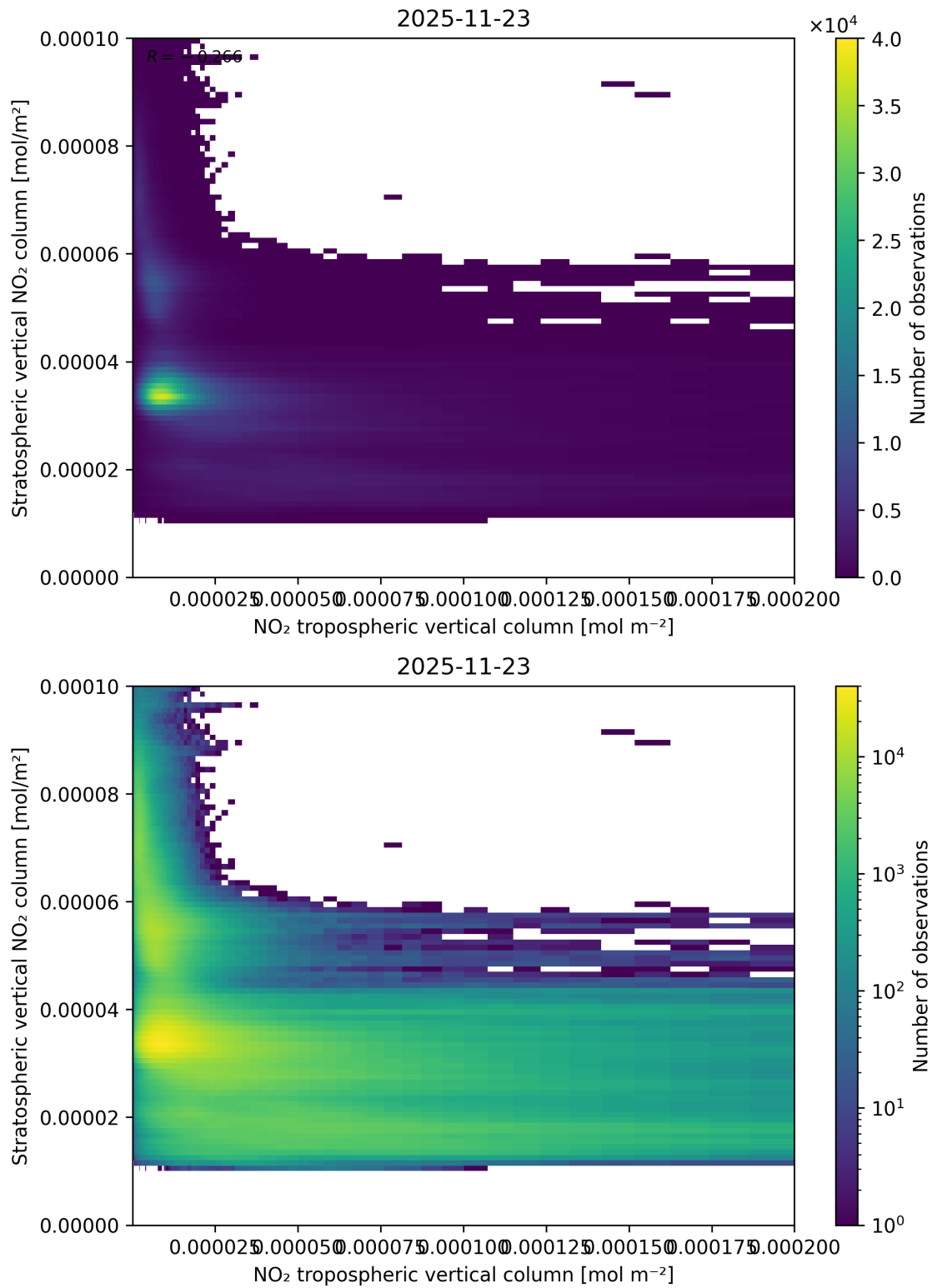
Figure 125: Scatter density plot of “NO 2 tropospheric vertical column” against “Stratospheric vertical NO 2 column” for 2025-11-23 to 2025-11-24.
