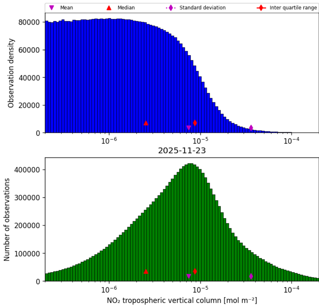
Figure 29: Histogram of “NO 2 tropospheric vertical column” for 2025-11-23 to 2025-11-24
