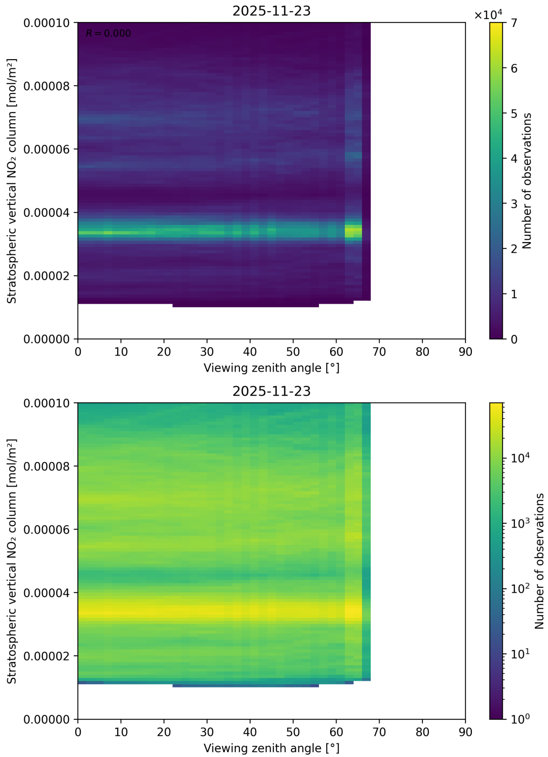
Figure 164: Scatter density plot of “Viewing zenith angle” against “Stratospheric vertical NO 2 column” for 2025-11-23 to 2025-11-24.
