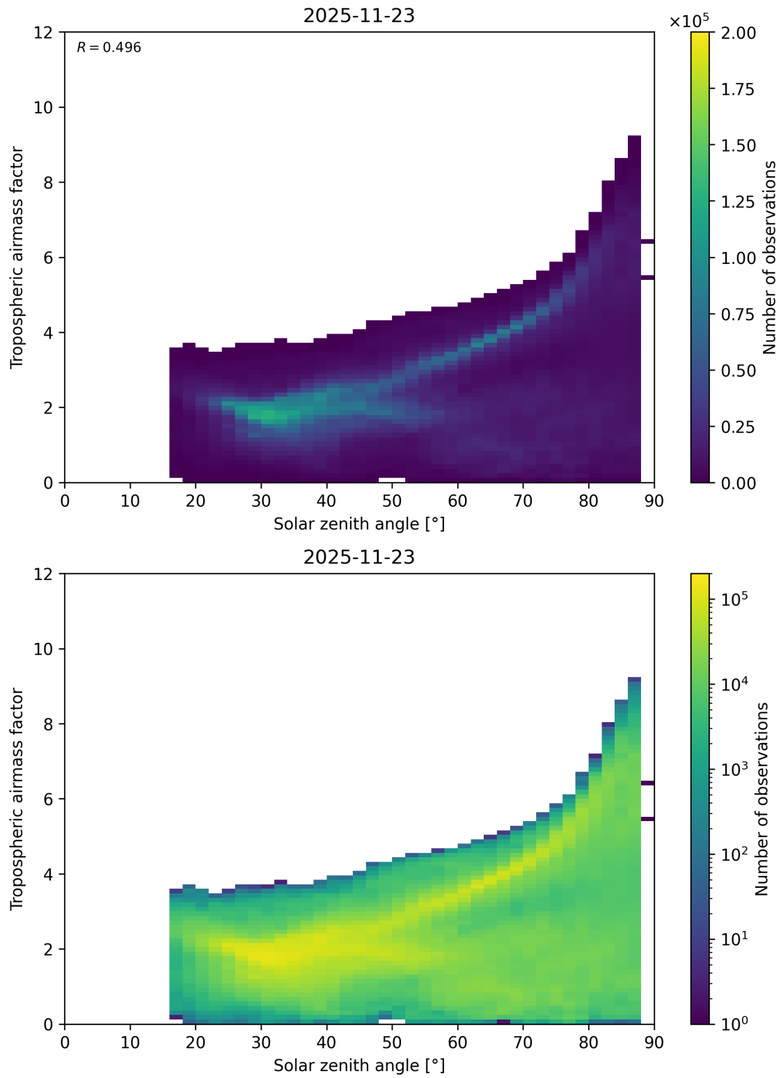
Figure 147: Scatter density plot of “Solar zenith angle” against “Tropospheric airmass factor” for 2025-11-23 to 2025-11-24.
