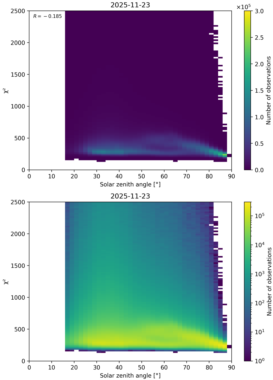
Figure 148: Scatter density plot of “Solar zenith angle” against “ \chi^2 ” for 2025-11-23 to 2025-11-24.
