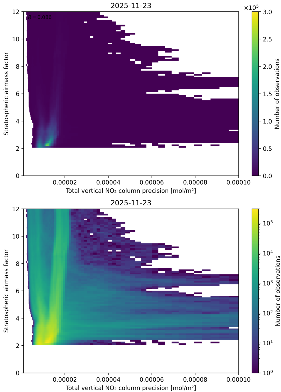
Figure 115: Scatter density plot of “Total vertical NO 2 column precision” against “Stratospheric air mass factor” for 2025-11-23 to 2025-11-24.
