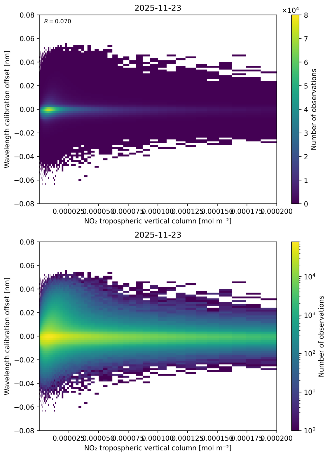
Figure 143: Scatter density plot of “NO 2 tropospheric vertical column” against “Wavelength calibration offset” for 2025-11-23 to 2025-11-24.
