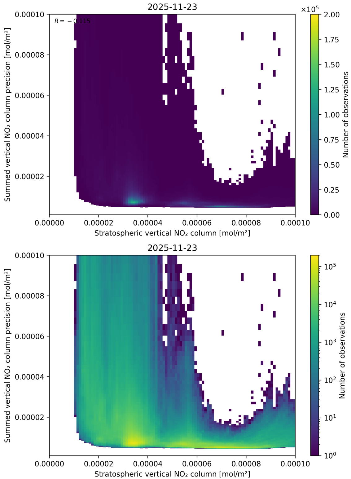
Figure 99: Scatter density plot of “Stratospheric vertical NO 2 column” against “Summed vertical NO 2 column precision” for 2025-11-23 to 2025-11-24.
