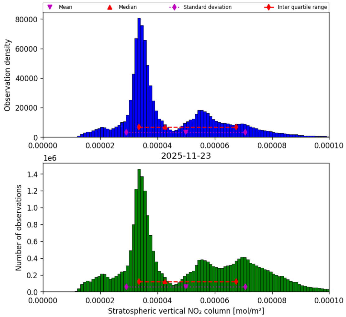
Figure 36: Histogram of “Stratospheric vertical NO 2 column” for 2025-11-23 to 2025-11-24
