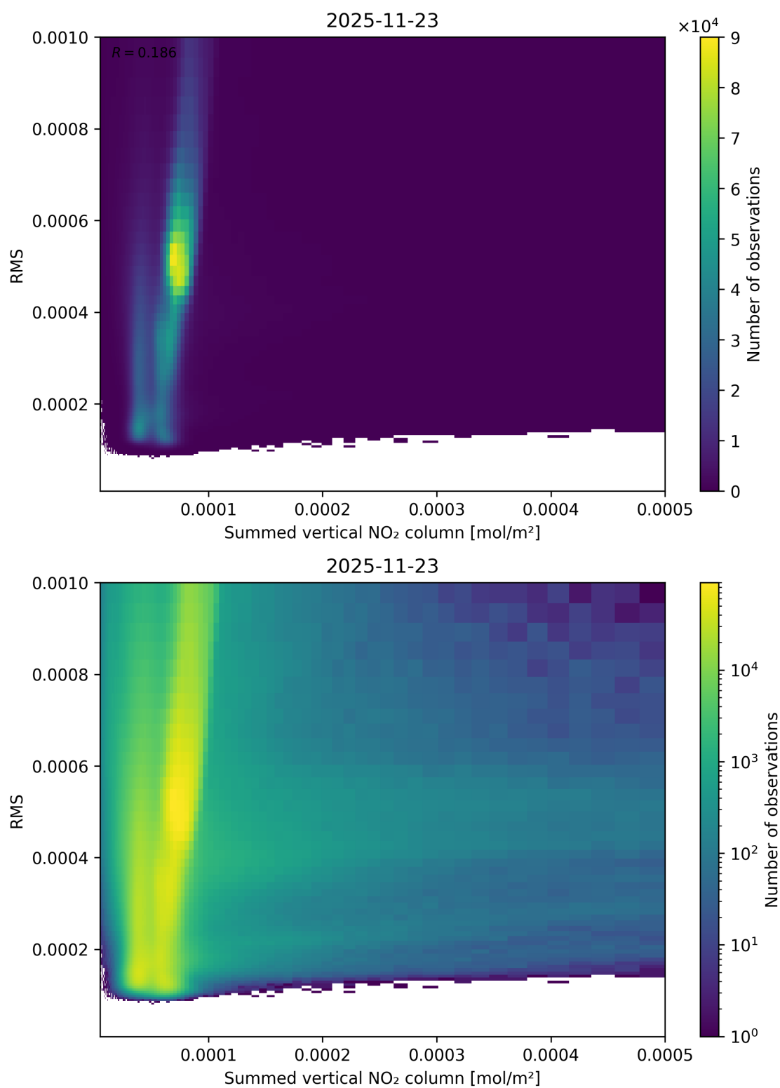
Figure 109: Scatter density plot of “Summed vertical NO 2 column” against “RMS” for 2025-11-23 to 2025-11-24.
