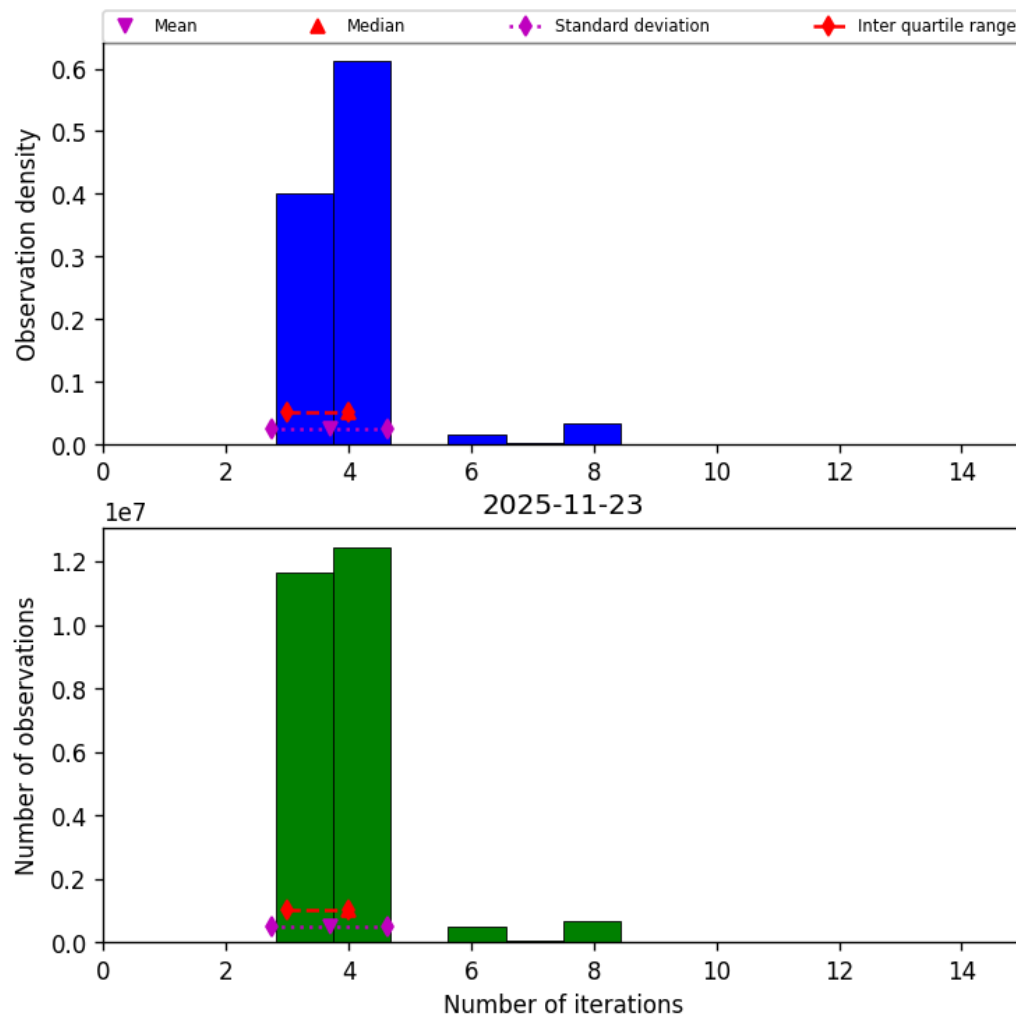
Figure 34: Histogram of “Number of iterations” for 2025-11-23 to 2025-11-24
