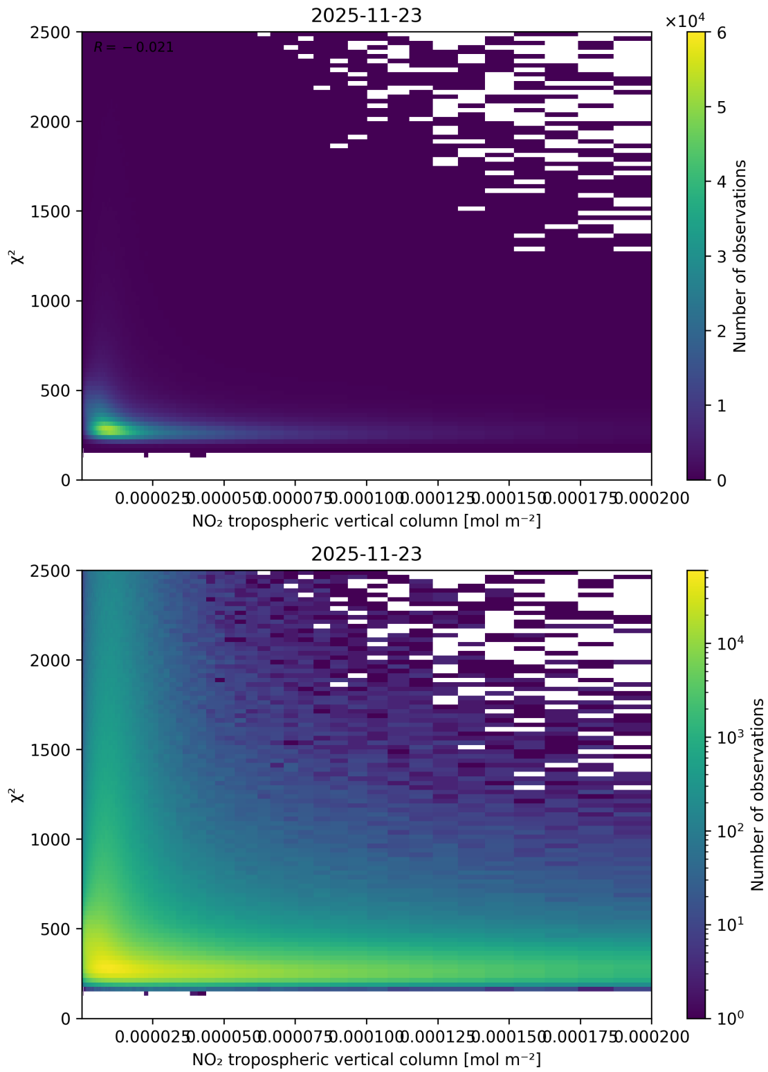
Figure 124: Scatter density plot of “NO 2 tropospheric vertical column” against “ \chi^2 ” for 2025-11-23 to 2025-11-24.
