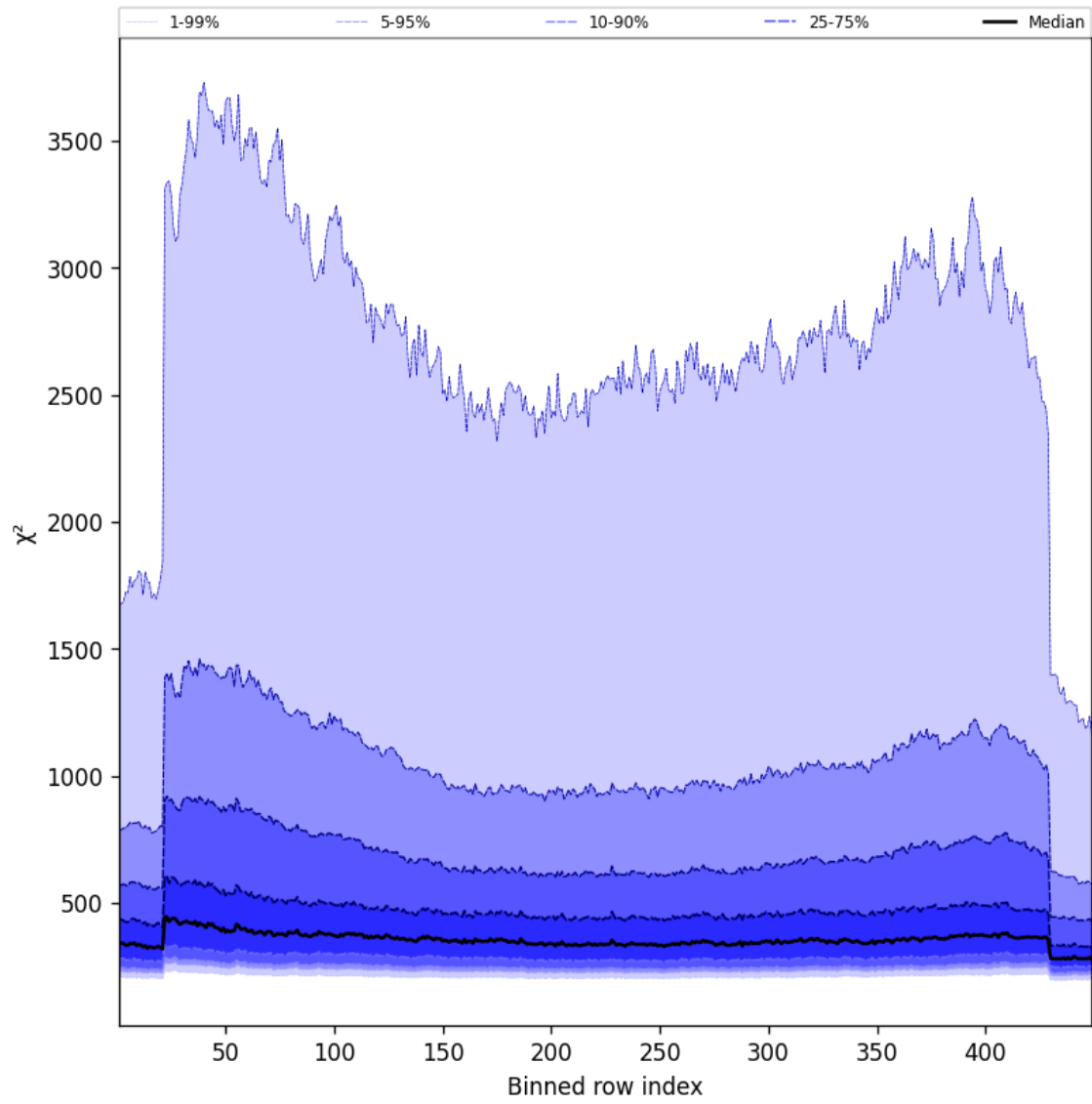
Figure 59: Along track statistics of “ \chi^2 ” for 2025-11-23 to 2025-11-24
