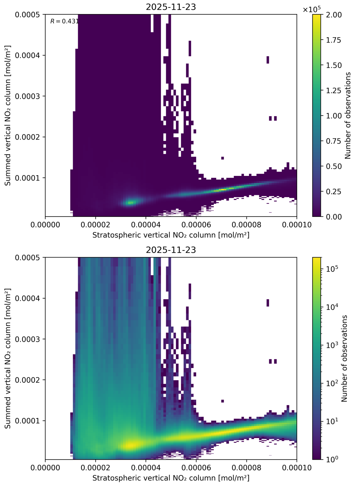
Figure 98: Scatter density plot of “Stratospheric vertical NO 2 column” against “Summed vertical NO 2 column” for 2025-11-23 to 2025-11-24.
