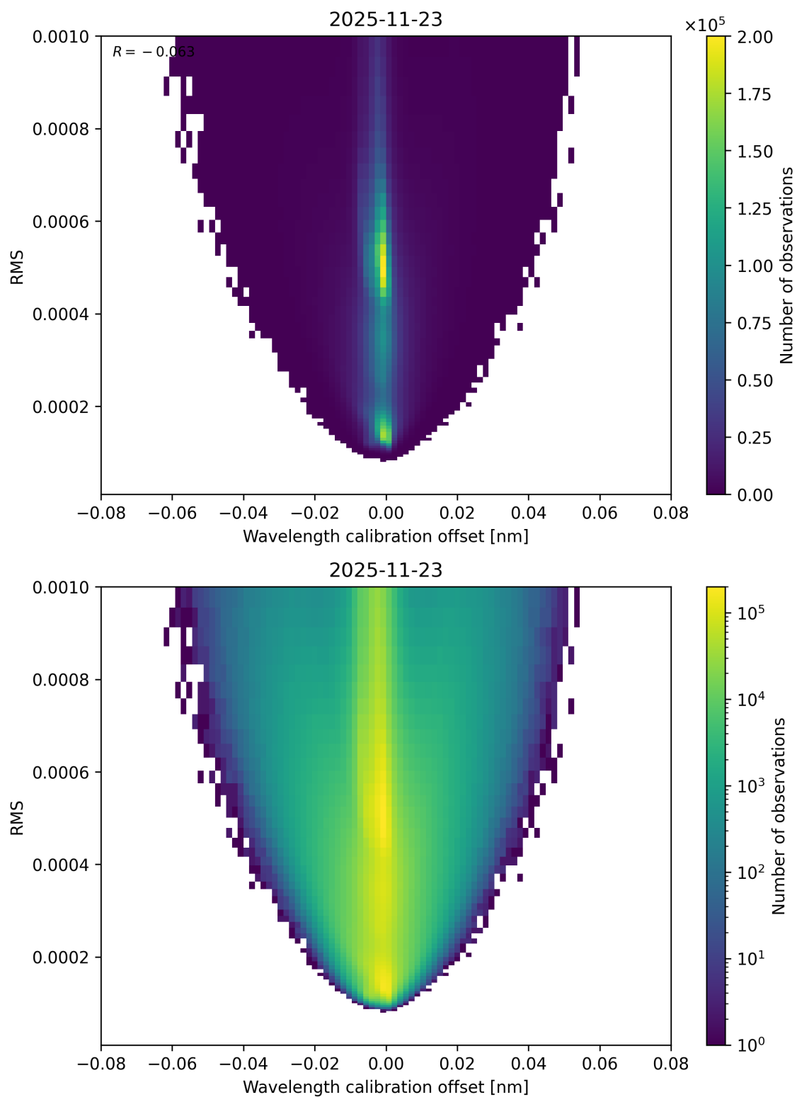
Figure 181: Scatter density plot of “Wavelength calibration offset” against “RMS” for 2025-11-23 to 2025-11-24.
