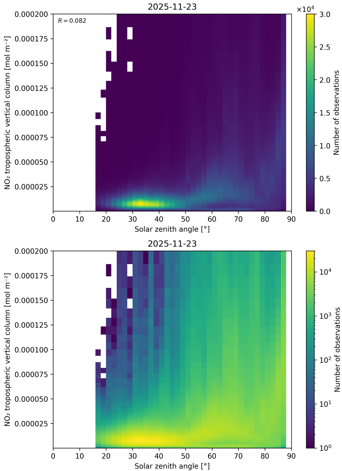
Figure 155: Scatter density plot of “Solar zenith angle” against “NO 2 tropospheric vertical column” for 2025-11-23 to 2025-11-24.
