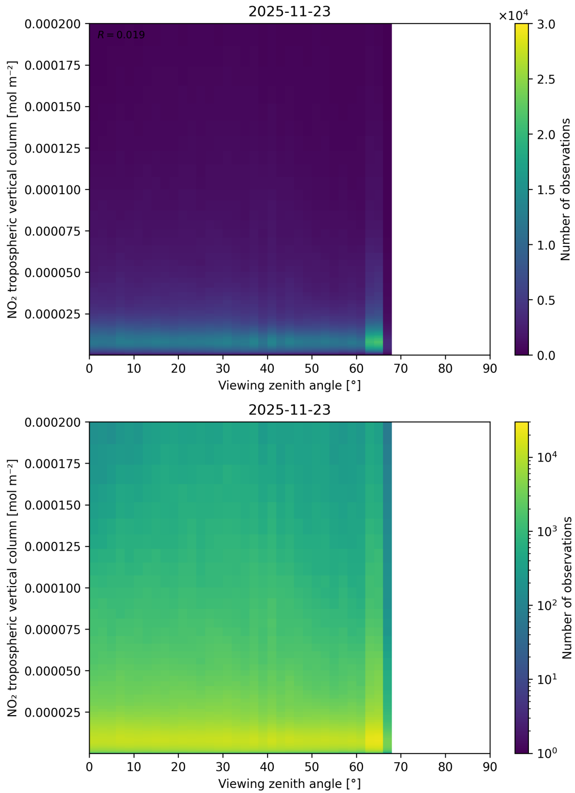
Figure 169: Scatter density plot of “Viewing zenith angle” against “NO 2 tropospheric vertical column” for 2025-11-23 to 2025-11-24.
