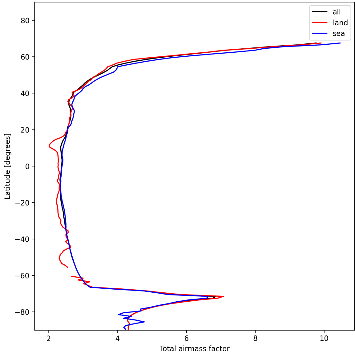
Figure 15: Zonal average of “Total airmass factor” for 2025-11-23 to 2025-11-24.
