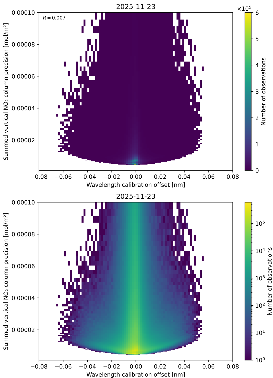
Figure 178: Scatter density plot of “Wavelength calibration offset” against “Summed vertical NO 2 column precision” for 2025-11-23 to 2025-11-24.
