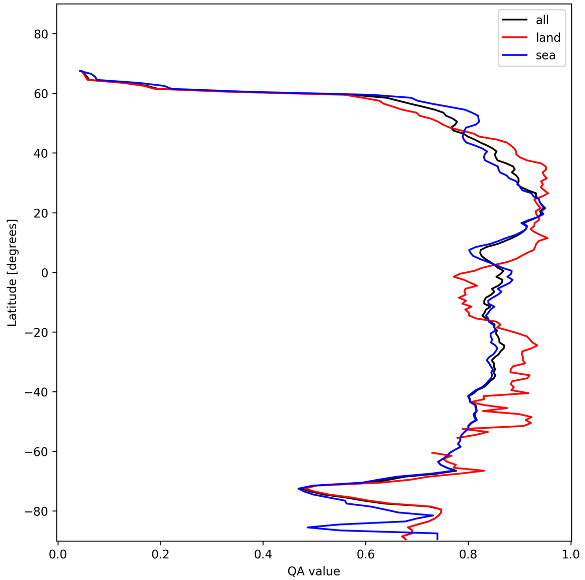
Figure 11: Zonal average of “QA value” for 2025-11-23 to 2025-11-24.
