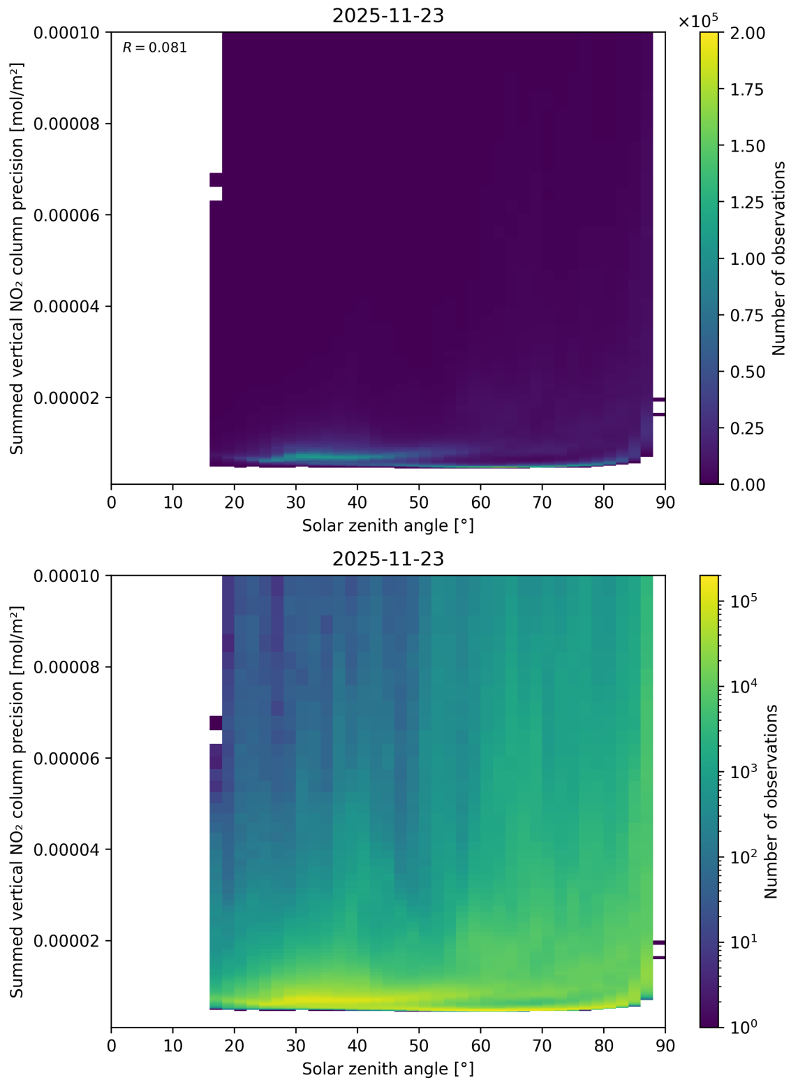
Figure 152: Scatter density plot of “Solar zenith angle” against “Summed vertical NO 2 column precision” for 2025-11-23 to 2025-11-24.
