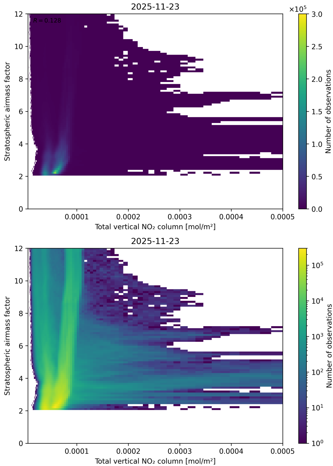
Figure 110: Scatter density plot of “Total vertical NO 2 column” against “Stratospheric airmass factor” for 2025-11-23 to 2025-11-24.
