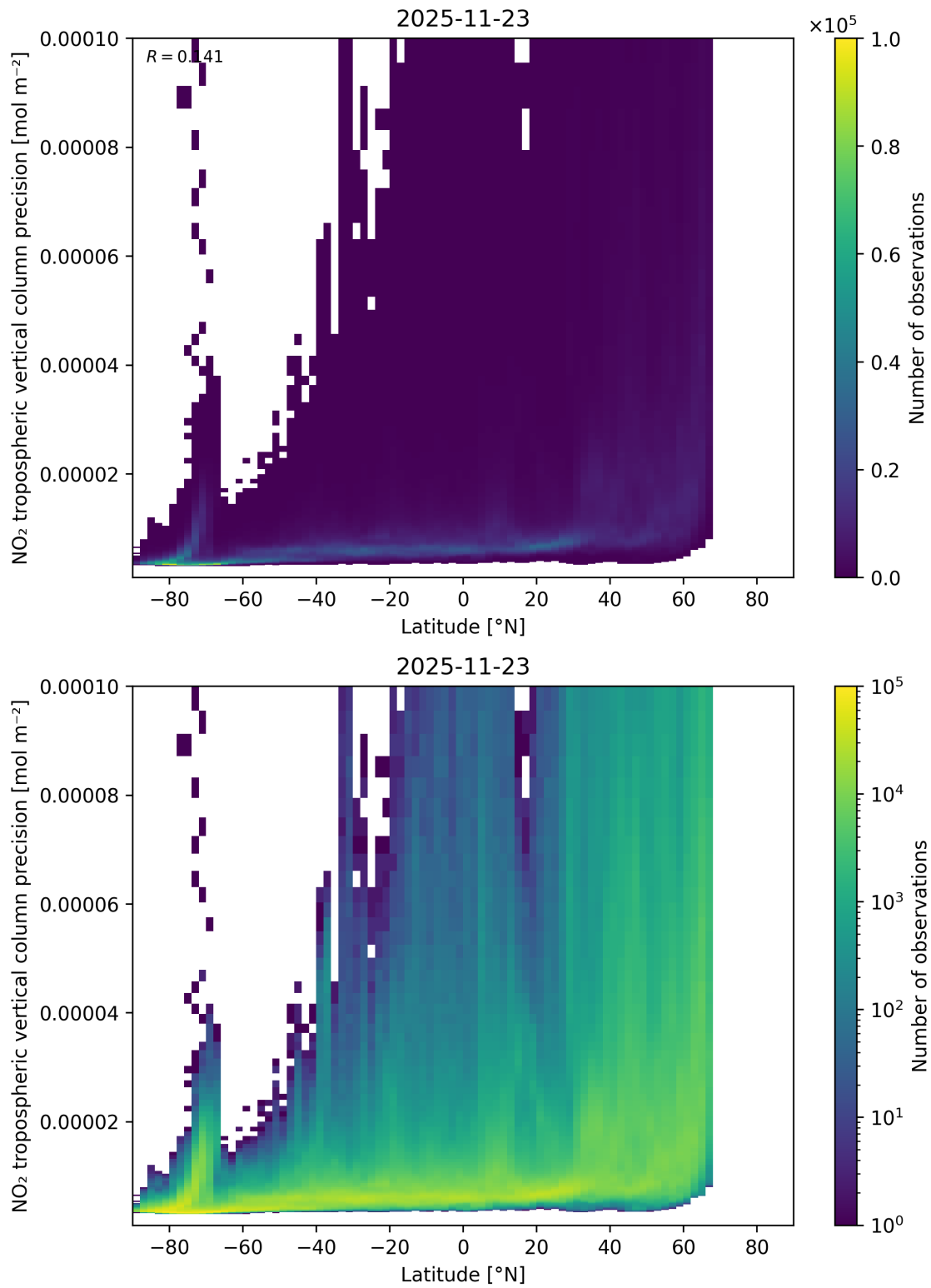
Figure 93: Scatter density plot of “Latitude” against “NO 2 tropospheric vertical column precision” for 2025-11-23 to 2025-11-24.
