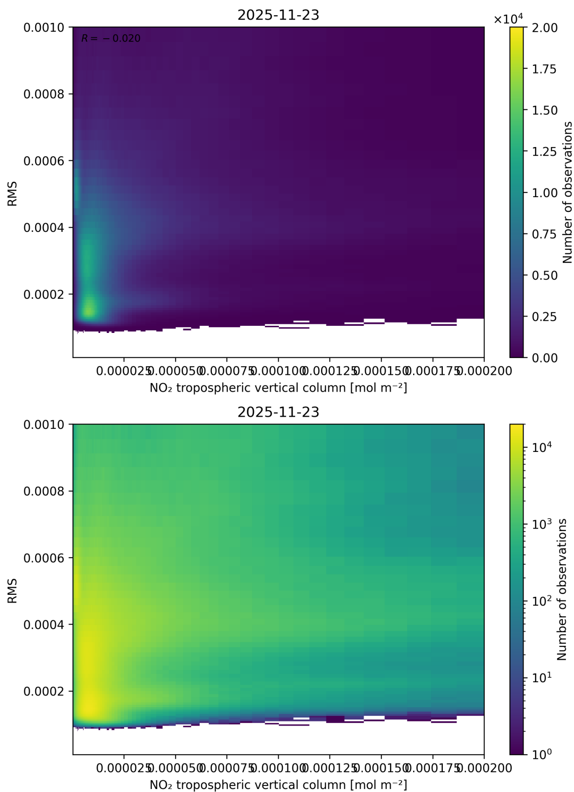
Figure 142: Scatter density plot of “NO 2 tropospheric vertical column” against “RMS” for 2025-11-23 to 2025-11-24.
