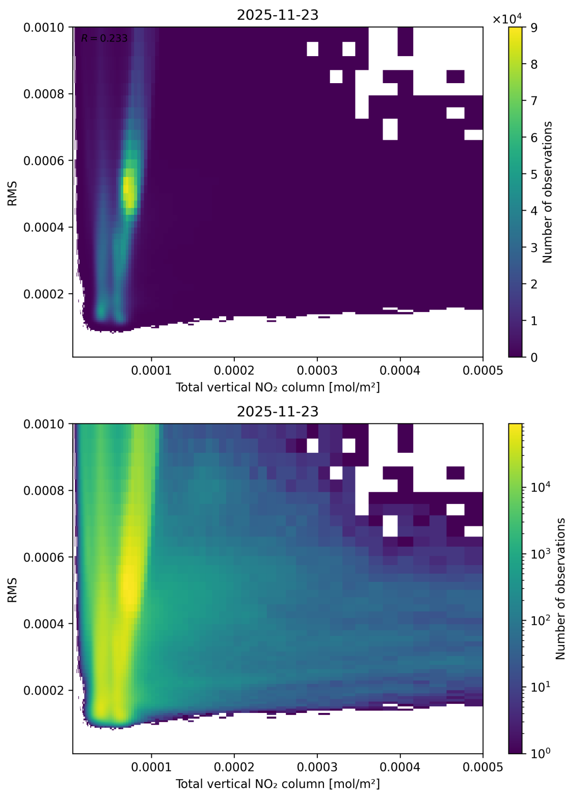
Figure 120: Scatter density plot of “Total vertical NO 2 column” against “RMS” for 2025-11-23 to 2025-11-24.
