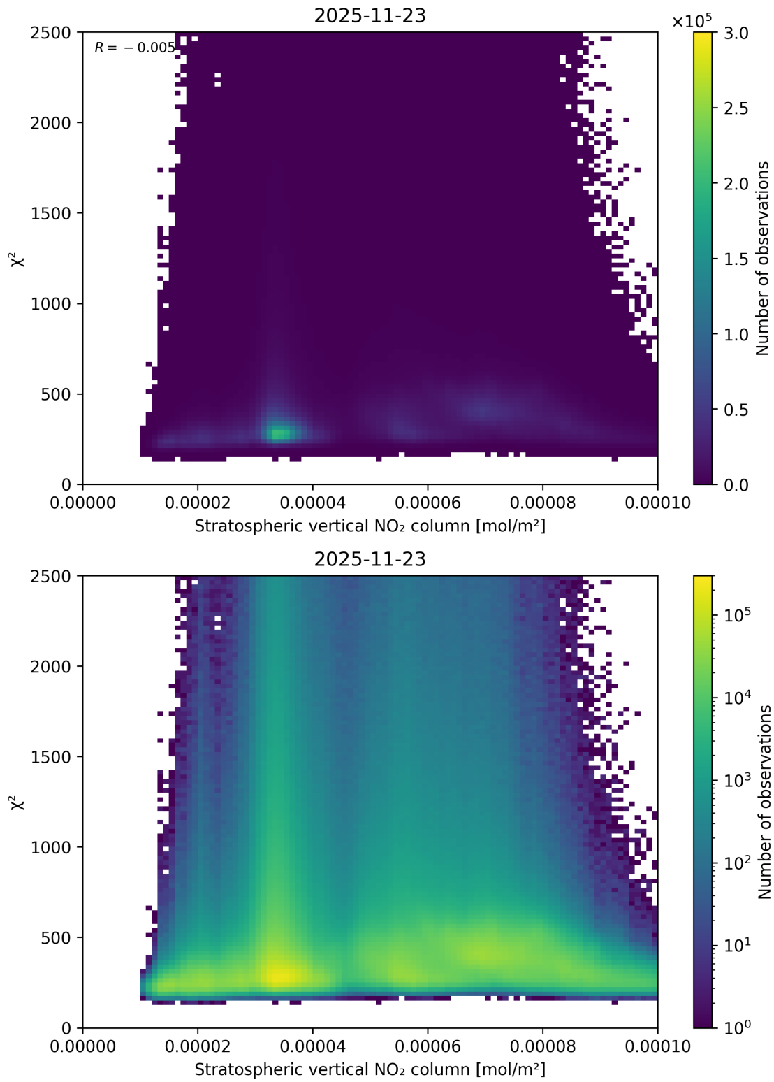
Figure 97: Scatter density plot of “Stratospheric vertical NO 2 column” against “ \chi^2 ” for 2025-11-23 to 2025-11-24.
