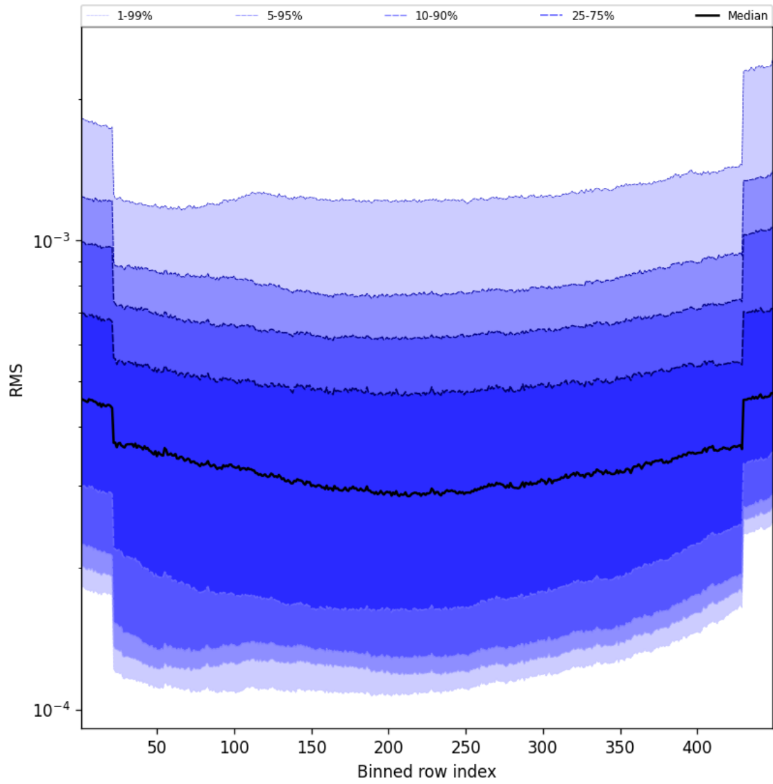
Figure 60: Along track statistics of “RMS” for 2025-11-23 to 2025-11-24
