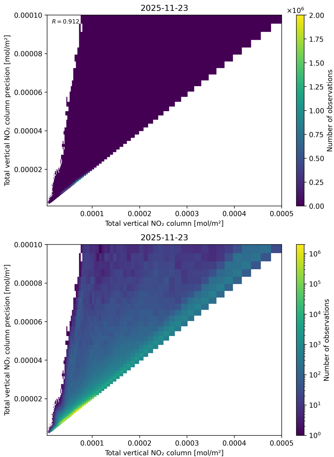
Figure 114: Scatter density plot of “Total vertical NO 2 column” against “Total vertical NO 2 column precision” for 2025-11-23 to 2025-11-24.
