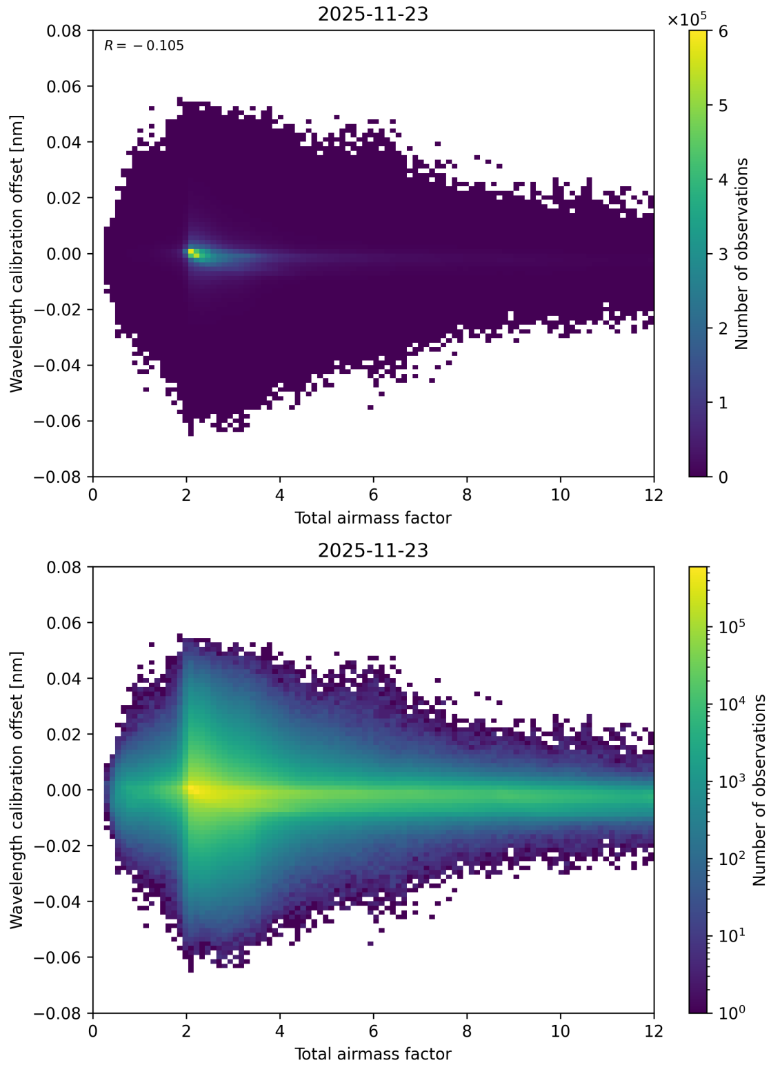
Figure 70: Scatter density plot of “Total airmass factor” against “Wavelength calibration offset” for 2025-11-23 to 2025-11-24.
