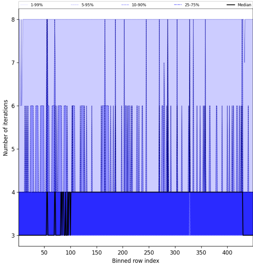
Figure 51: Along track statistics of “Number of iterations” for 2025-11-23 to 2025-11-24
