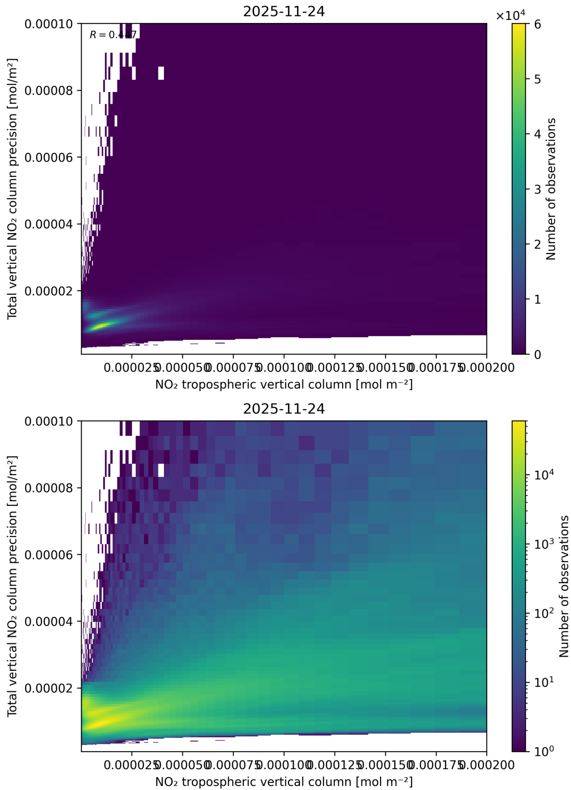
Figure 129: Scatter density plot of “NO 2 tropospheric vertical column” against “Total vertical NO 2 column precision” for 2025-11-23 to 2025-11-25.
