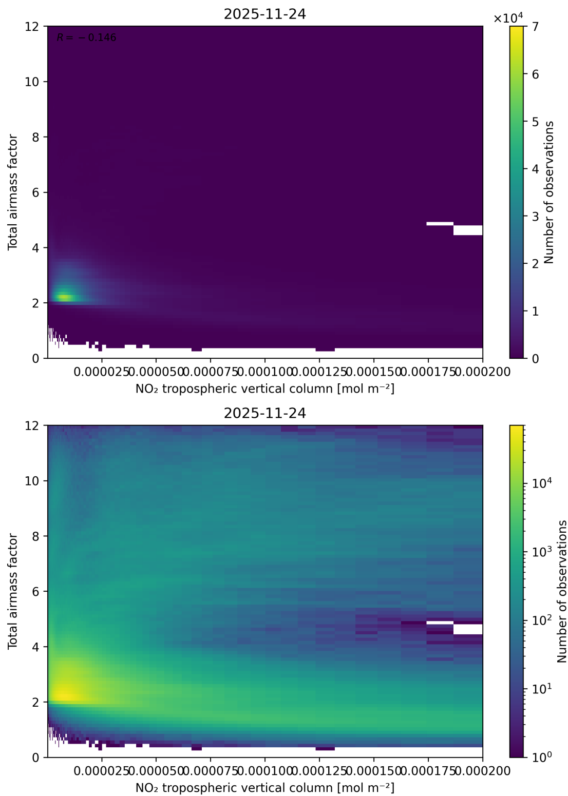
Figure 122: Scatter density plot of “NO 2 tropospheric vertical column” against “Total air mass factor” for 2025-11-23 to 2025-11-25.
