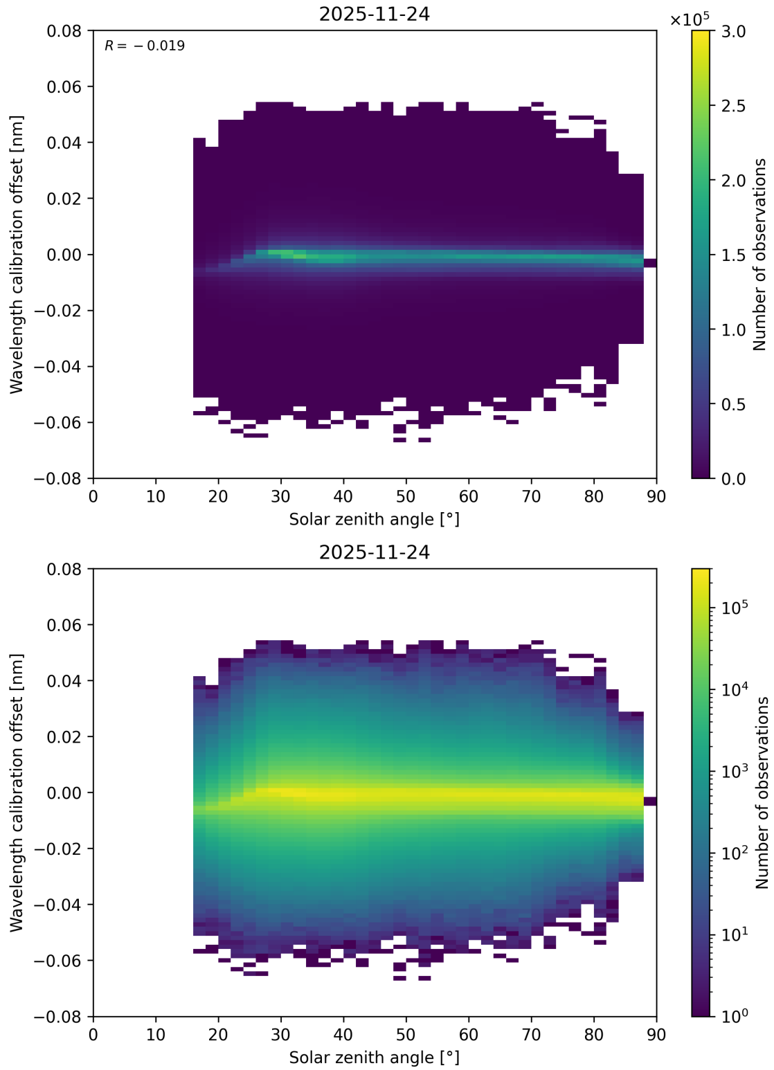
Figure 158: Scatter density plot of “Solar zenith angle” against “Wavelength calibration offset” for 2025-11-23 to 2025-11-25.
