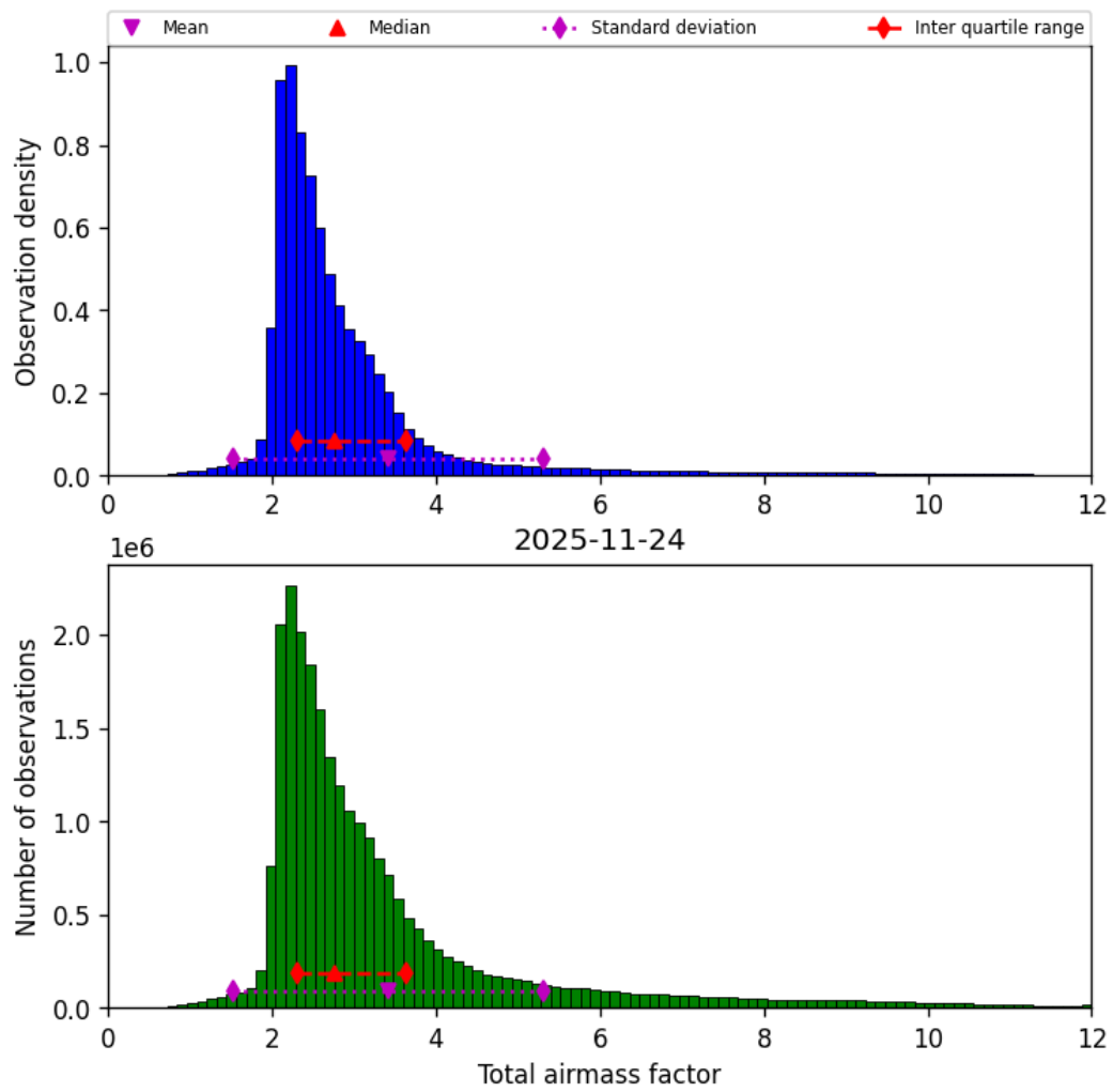
Figure 32: Histogram of “Total airmass factor” for 2025-11-23 to 2025-11-25
