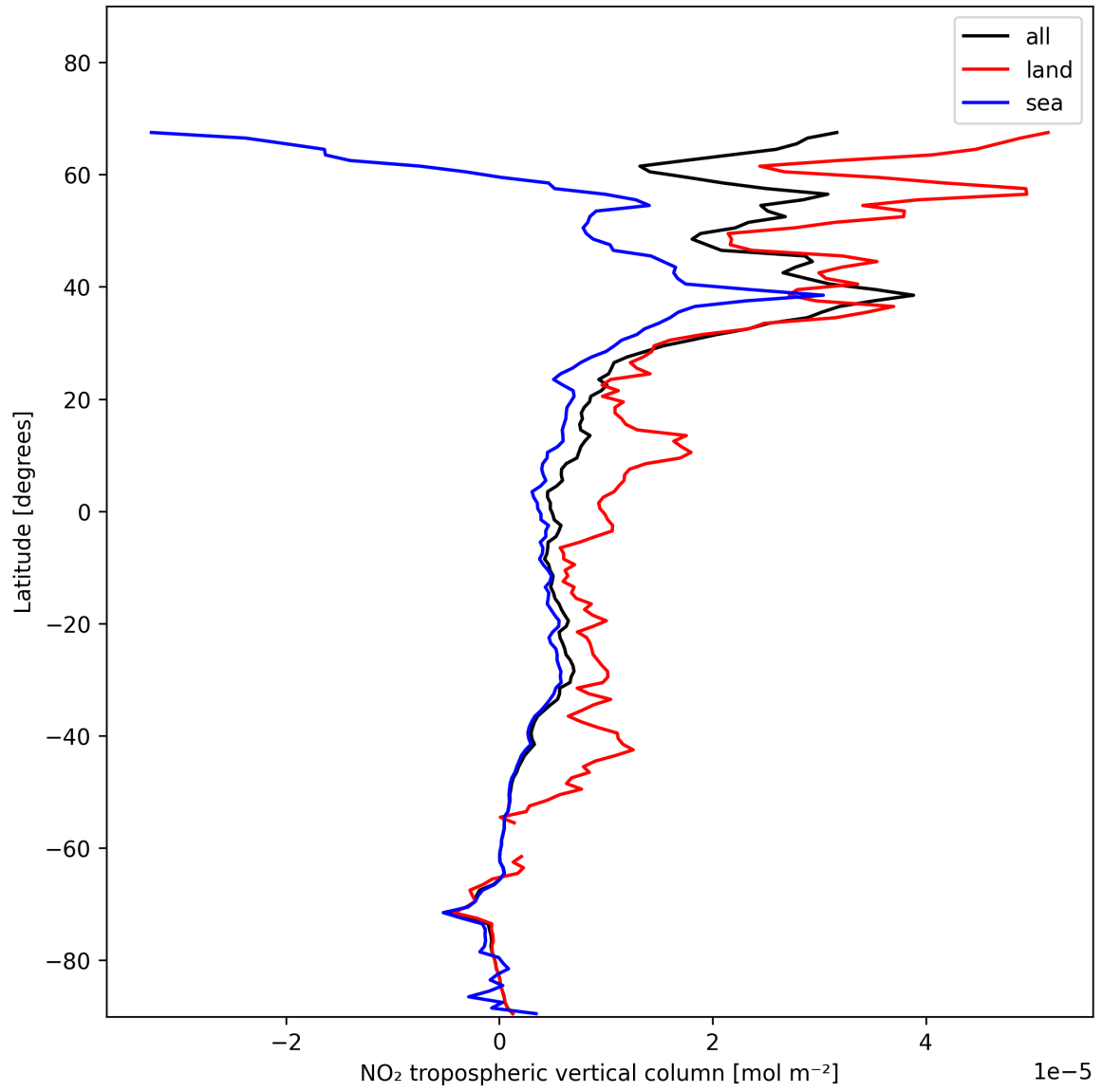
Figure 12: Zonal average of “NO 2 tropospheric vertical column” for 2025-11-23 to 2025-11-25.
