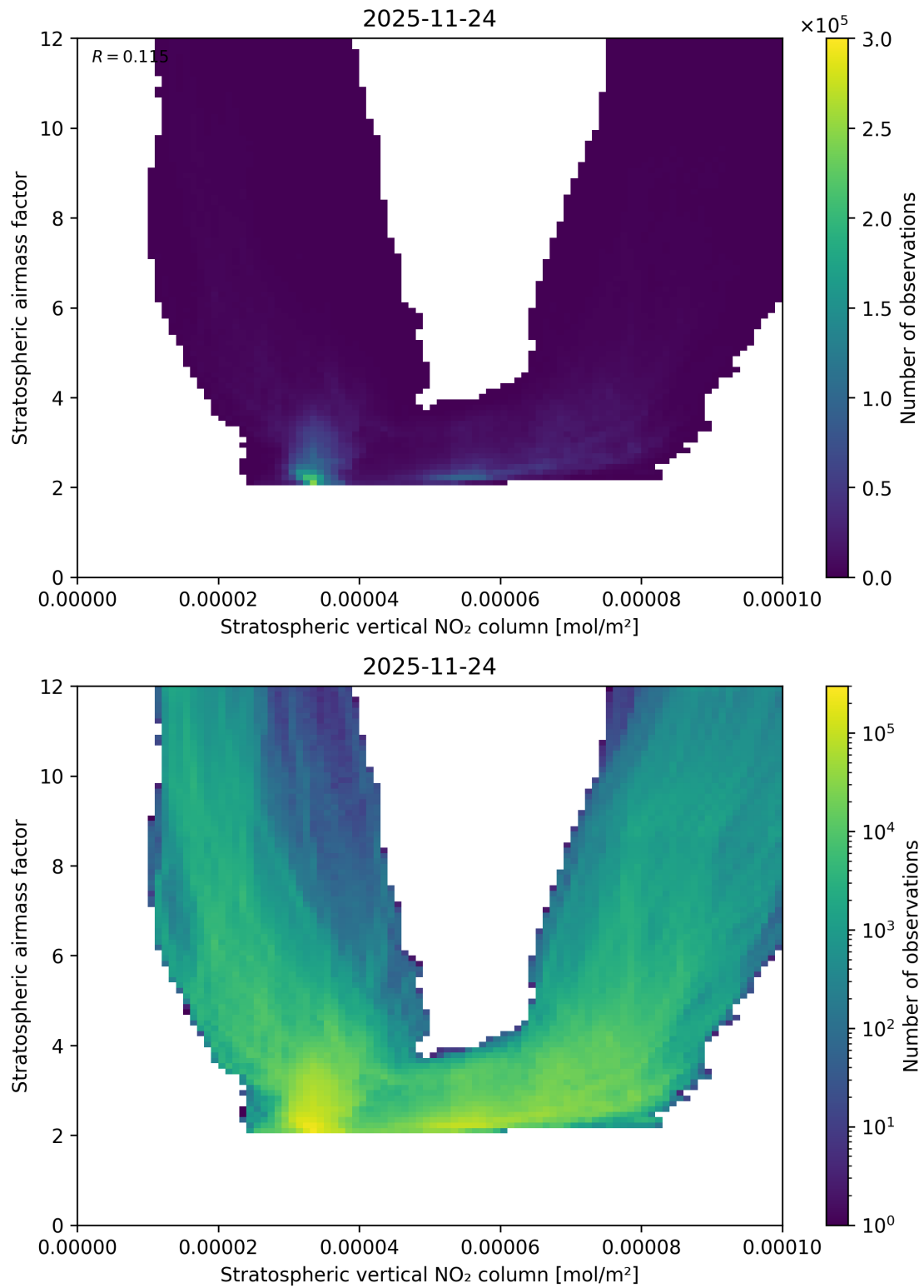
Figure 96: Scatter density plot of “Stratospheric vertical NO 2 column” against “Stratospheric airmass factor” for 2025-11-23 to 2025-11-25.
