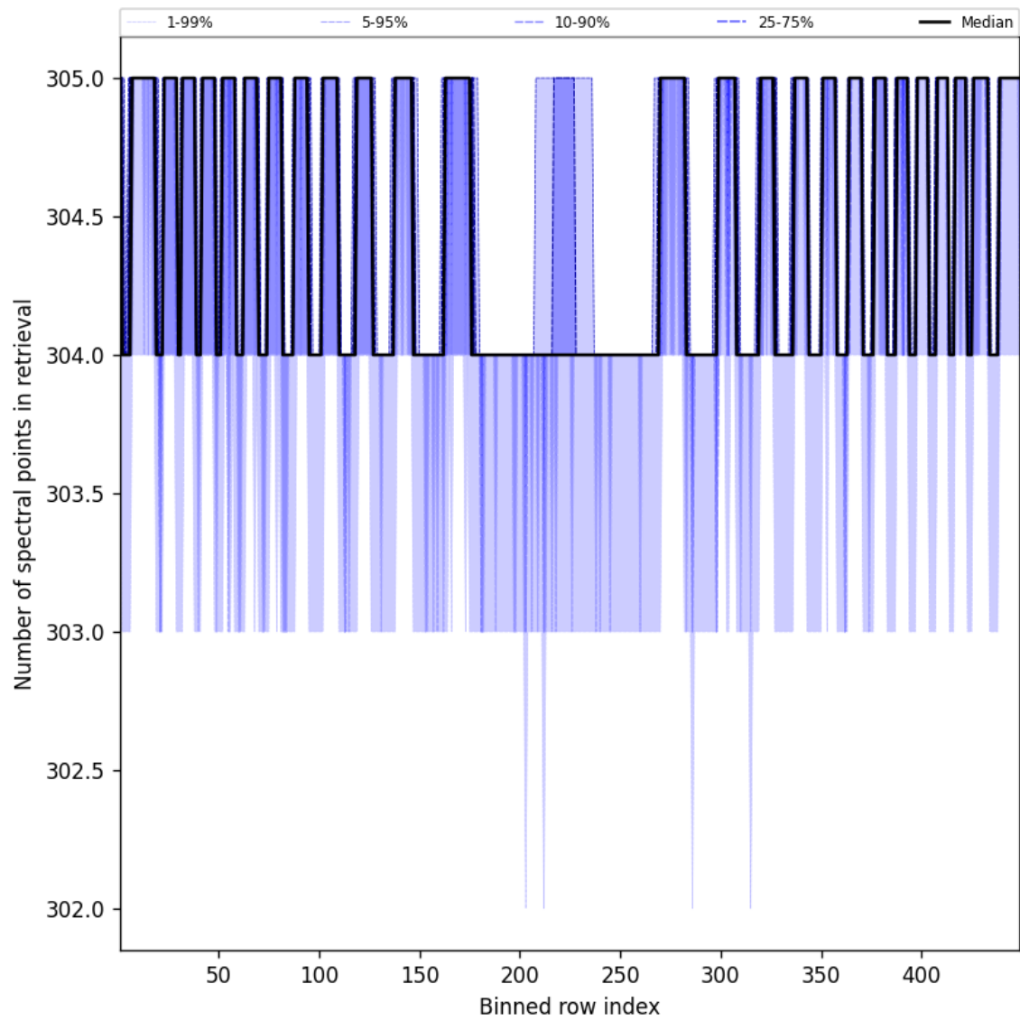
Figure 50: Along track statistics of “Number of spectral points in retrieval” for 2025-11-23 to 2025-11-25
