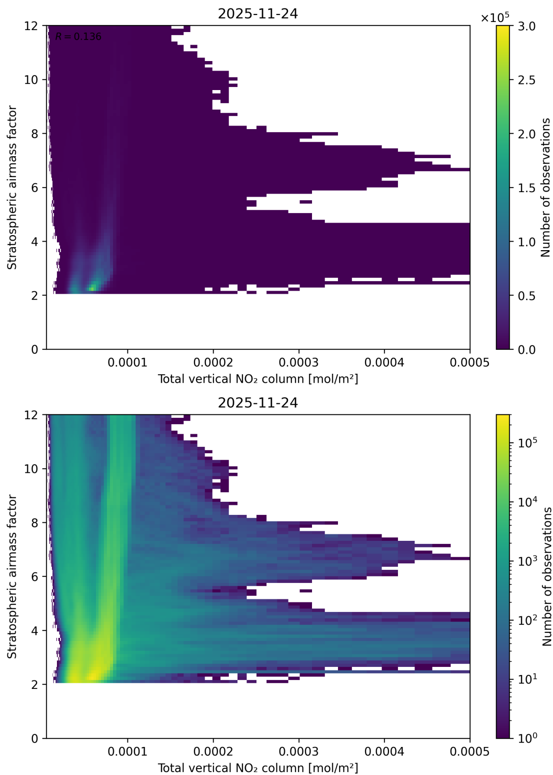
Figure 110: Scatter density plot of “Total vertical NO 2 column” against “Stratospheric air mass factor” for 2025-11-23 to 2025-11-25.
