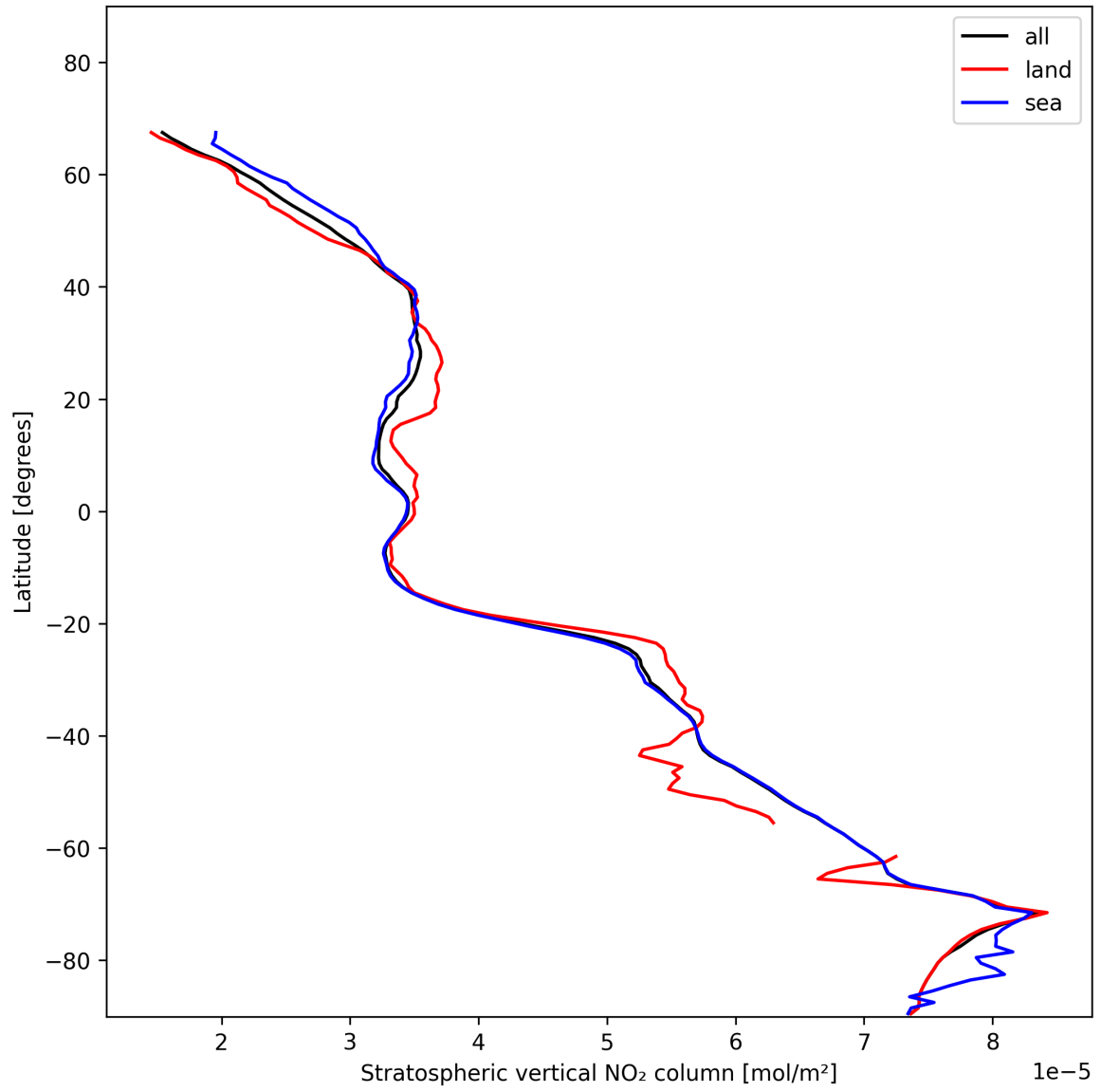
Figure 19: Zonal average of “Stratospheric vertical NO 2 column” for 2025-11-23 to 2025-11-25.
