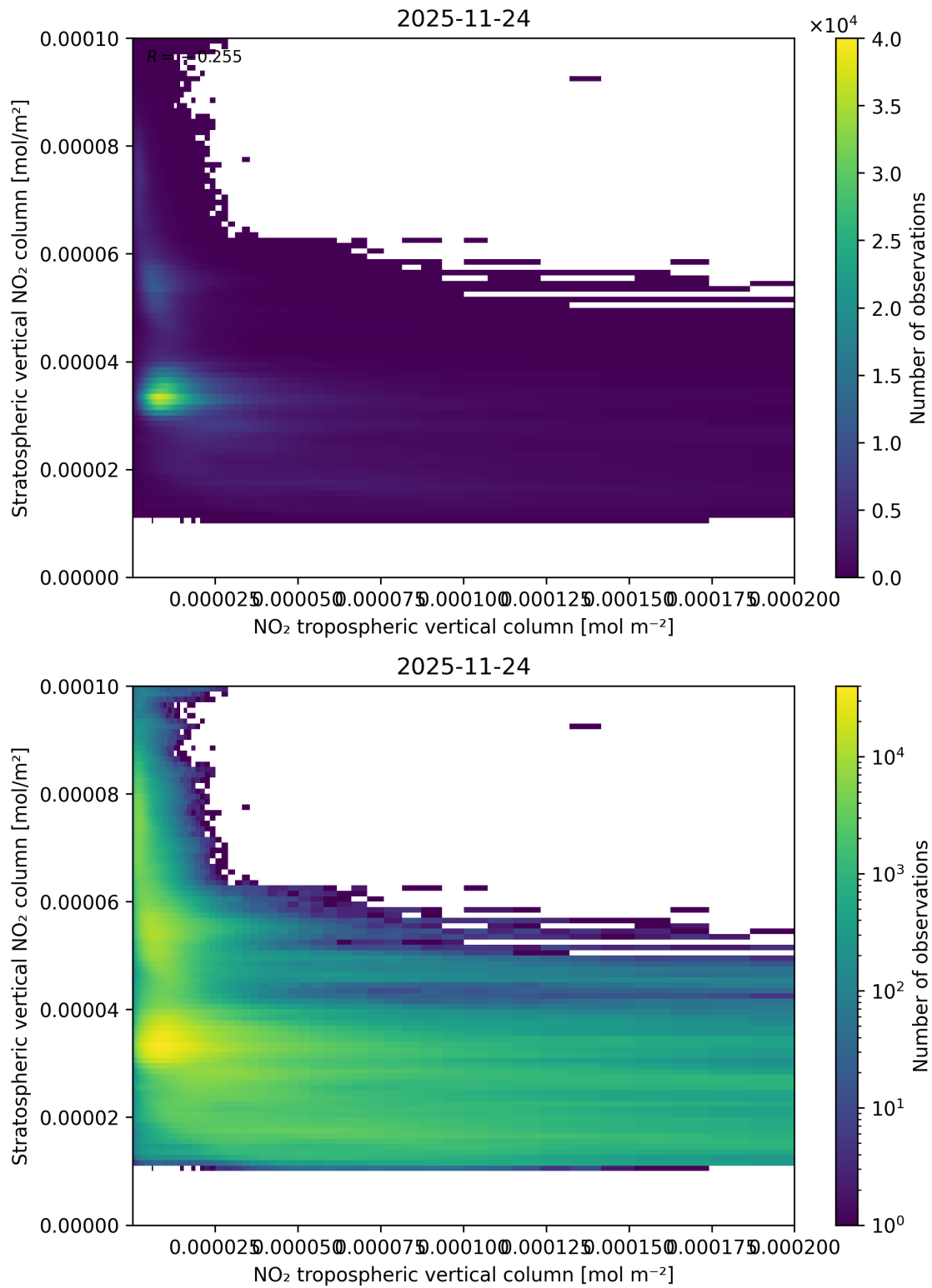
Figure 125: Scatter density plot of “NO 2 tropospheric vertical column” against “Stratospheric vertical NO 2 column” for 2025-11-23 to 2025-11-25.
