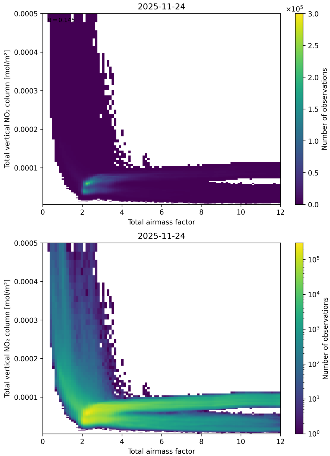
Figure 67: Scatter density plot of “Total airmass factor” against “Total vertical NO 2 column” for 2025-11-23 to 2025-11-25.
