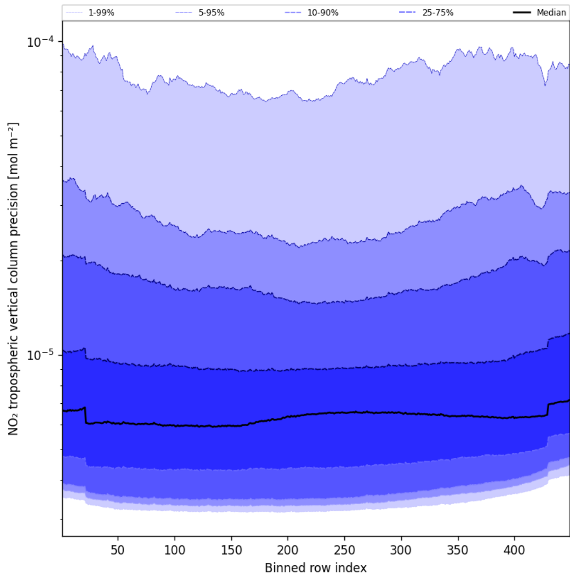
Figure 47: Along track statistics of “NO 2 tropospheric vertical column precision” for 2025-11-23 to 2025-11-25
