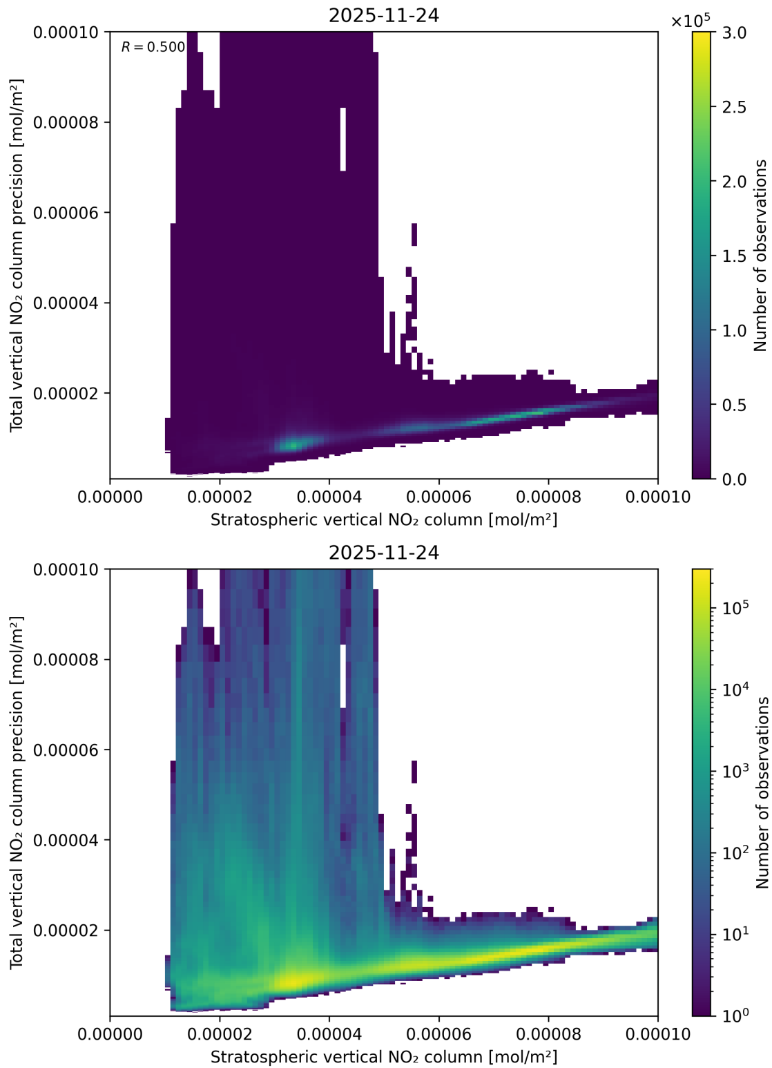
Figure 101: Scatter density plot of “Stratospheric vertical NO 2 column” against “Total vertical NO 2 column precision” for 2025-11-23 to 2025-11-25.
