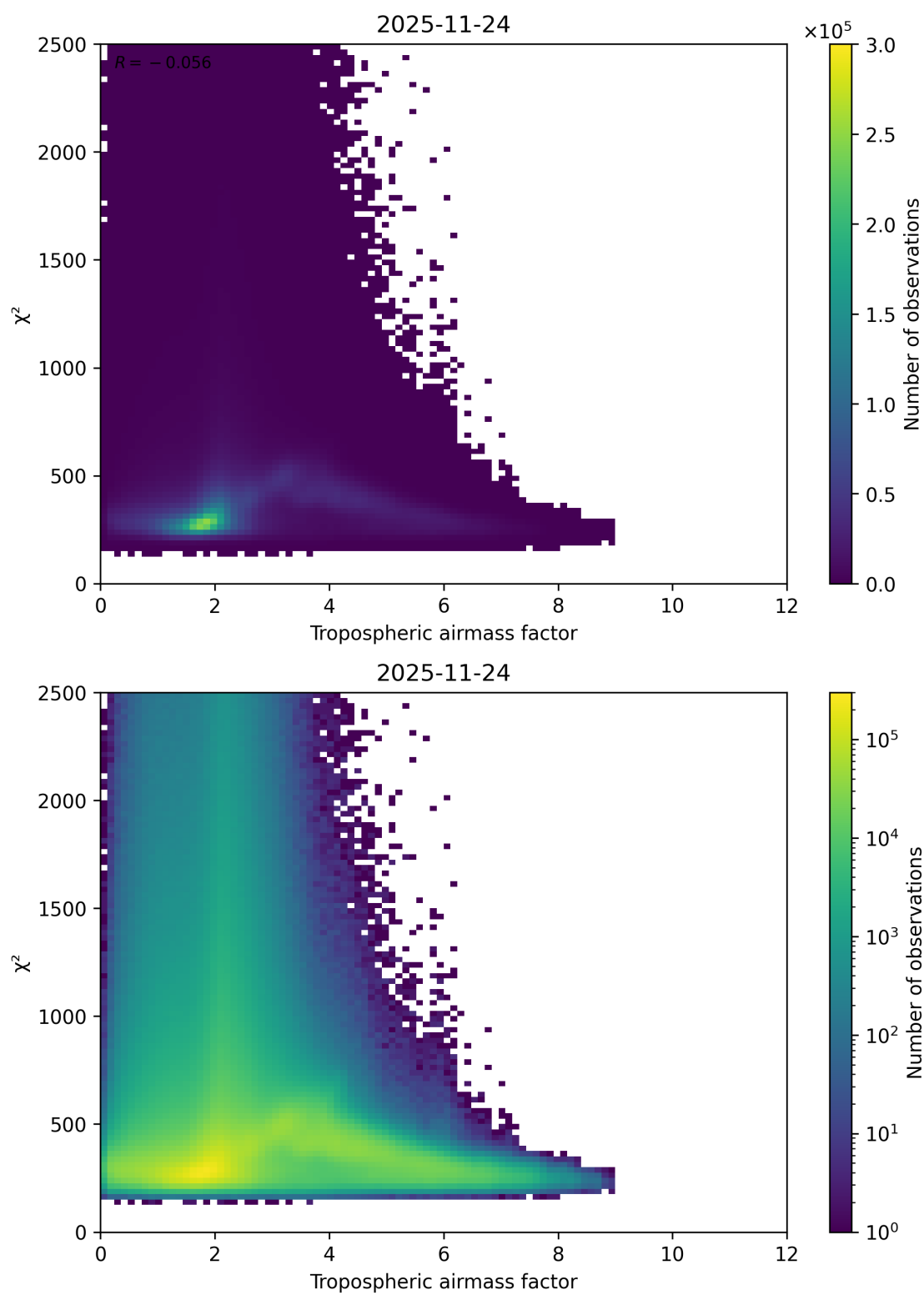
Figure 73: Scatter density plot of “Tropospheric airmass factor” against “ \chi^2 ” for 2025-11-23 to 2025-11-25.
