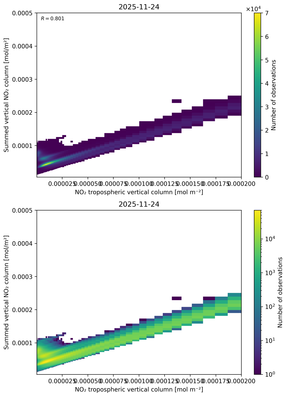
Figure 126: Scatter density plot of “NO 2 tropospheric vertical column” against “Summed vertical NO 2 column” for 2025-11-23 to 2025-11-25.
