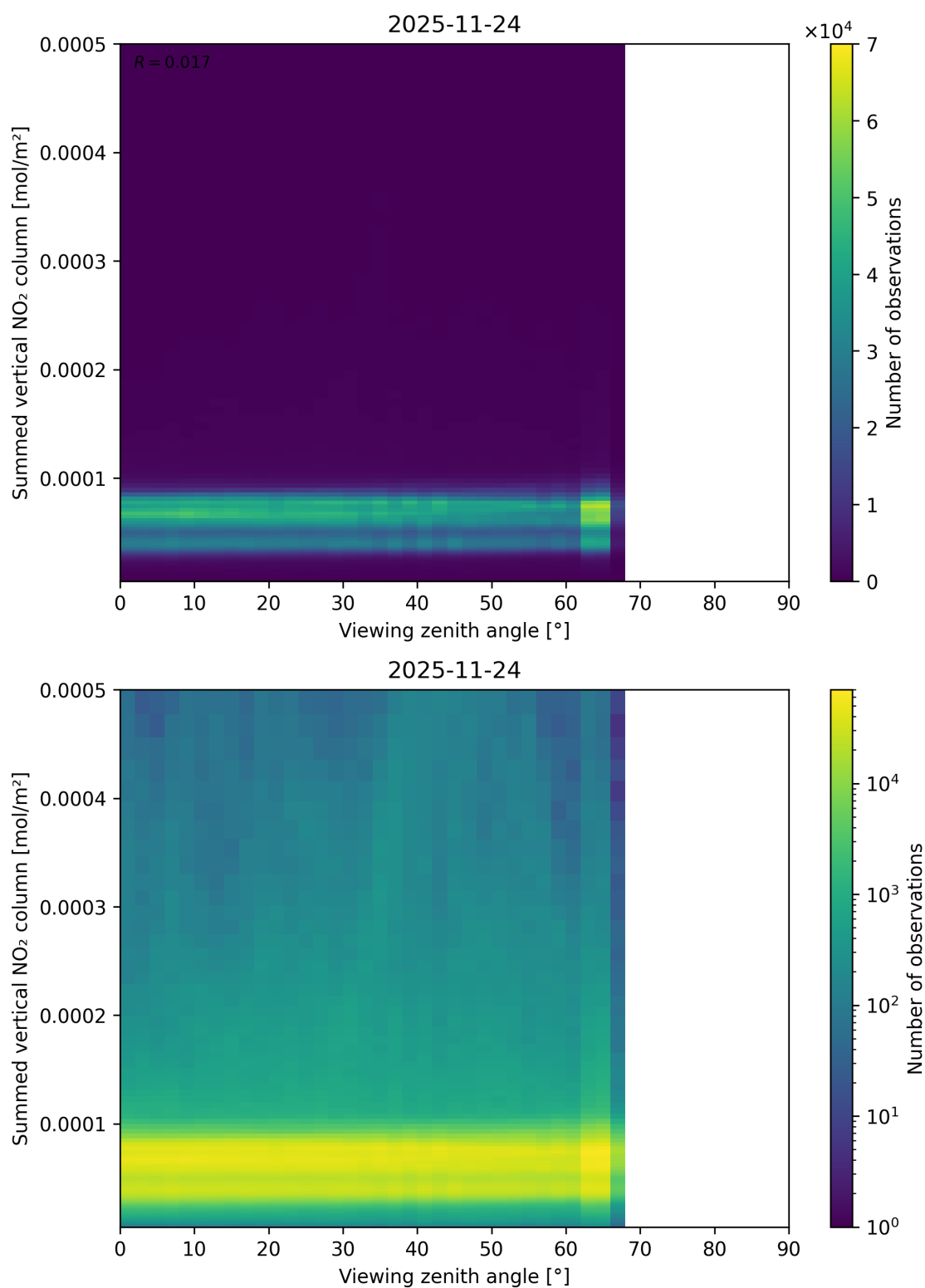
Figure 165: Scatter density plot of “Viewing zenith angle” against “Summed vertical NO 2 column” for 2025-11-23 to 2025-11-25.
