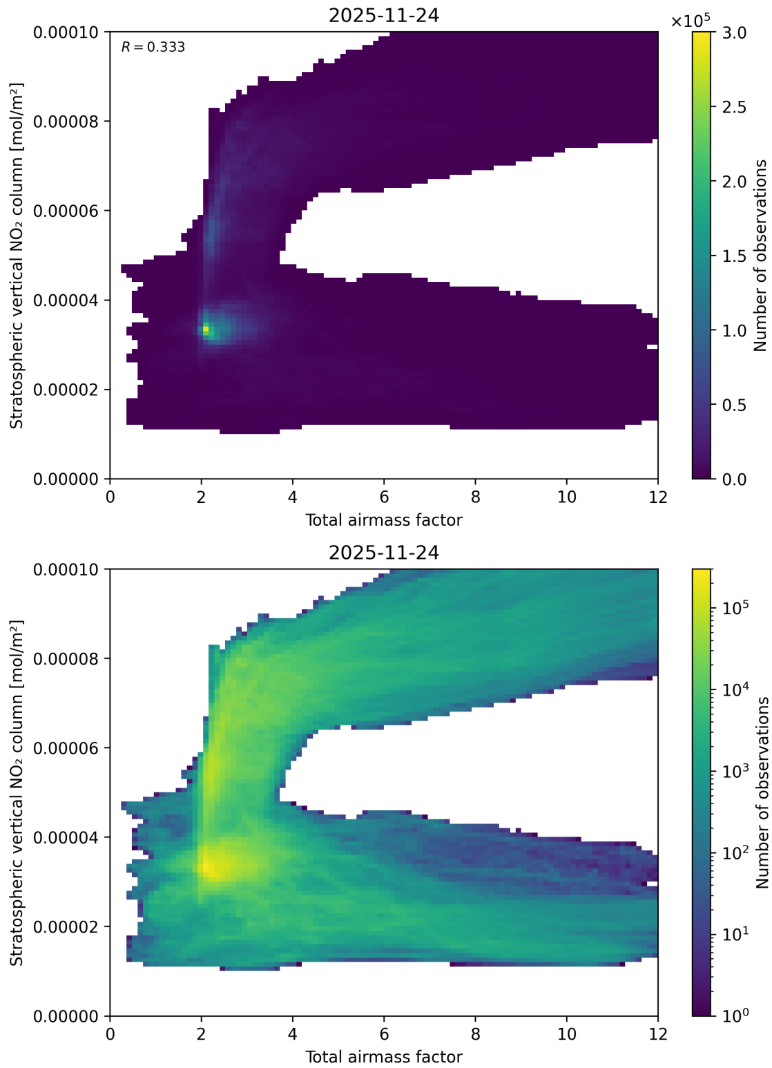
Figure 64: Scatter density plot of “Total airmass factor” against “Stratospheric vertical \text{NO}_2 column” for 2025-11-23 to 2025-11-25.
