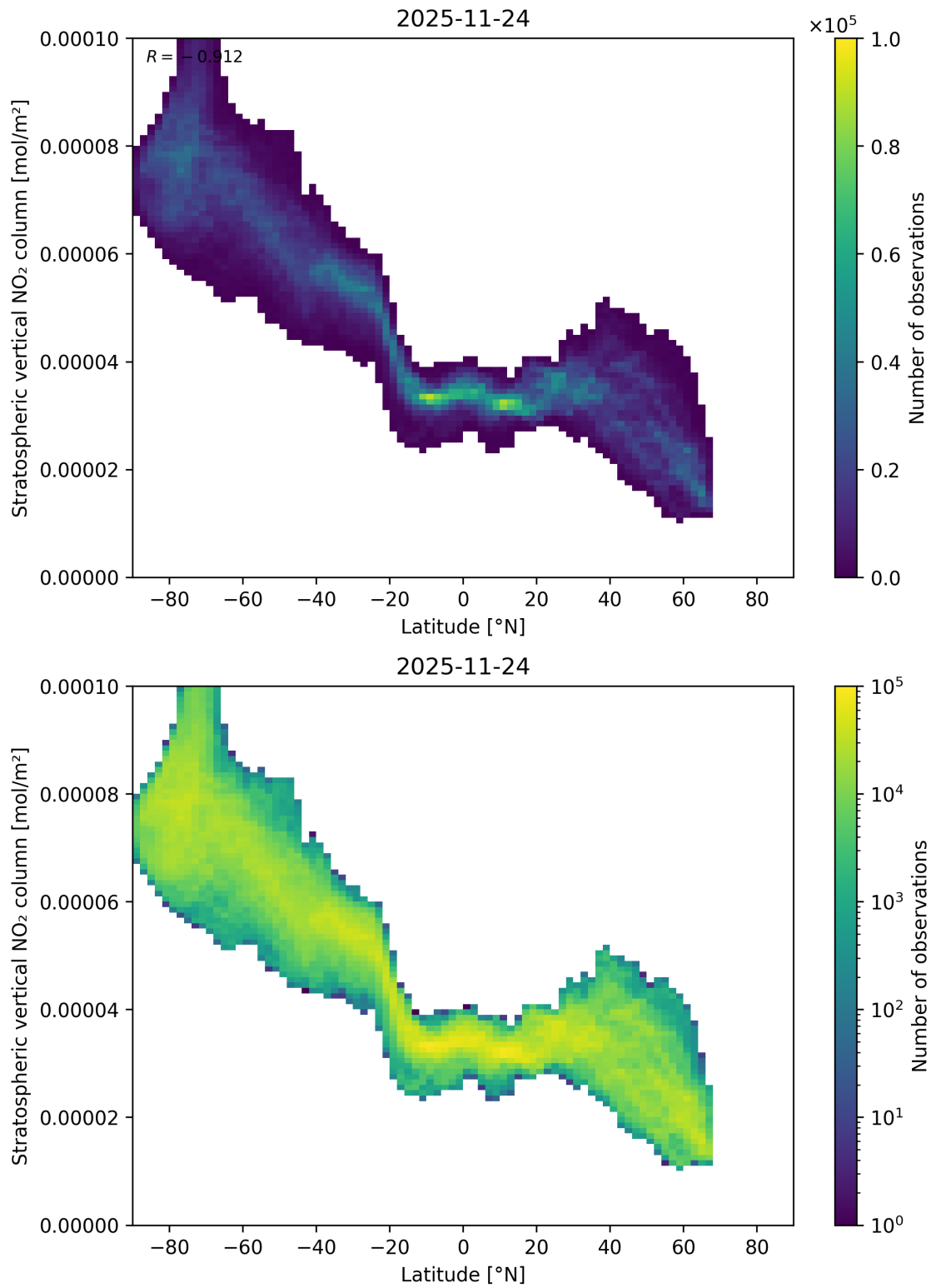
Figure 87: Scatter density plot of “Latitude” against “Stratospheric vertical NO 2 column” for 2025-11-23 to 2025-11-25.
