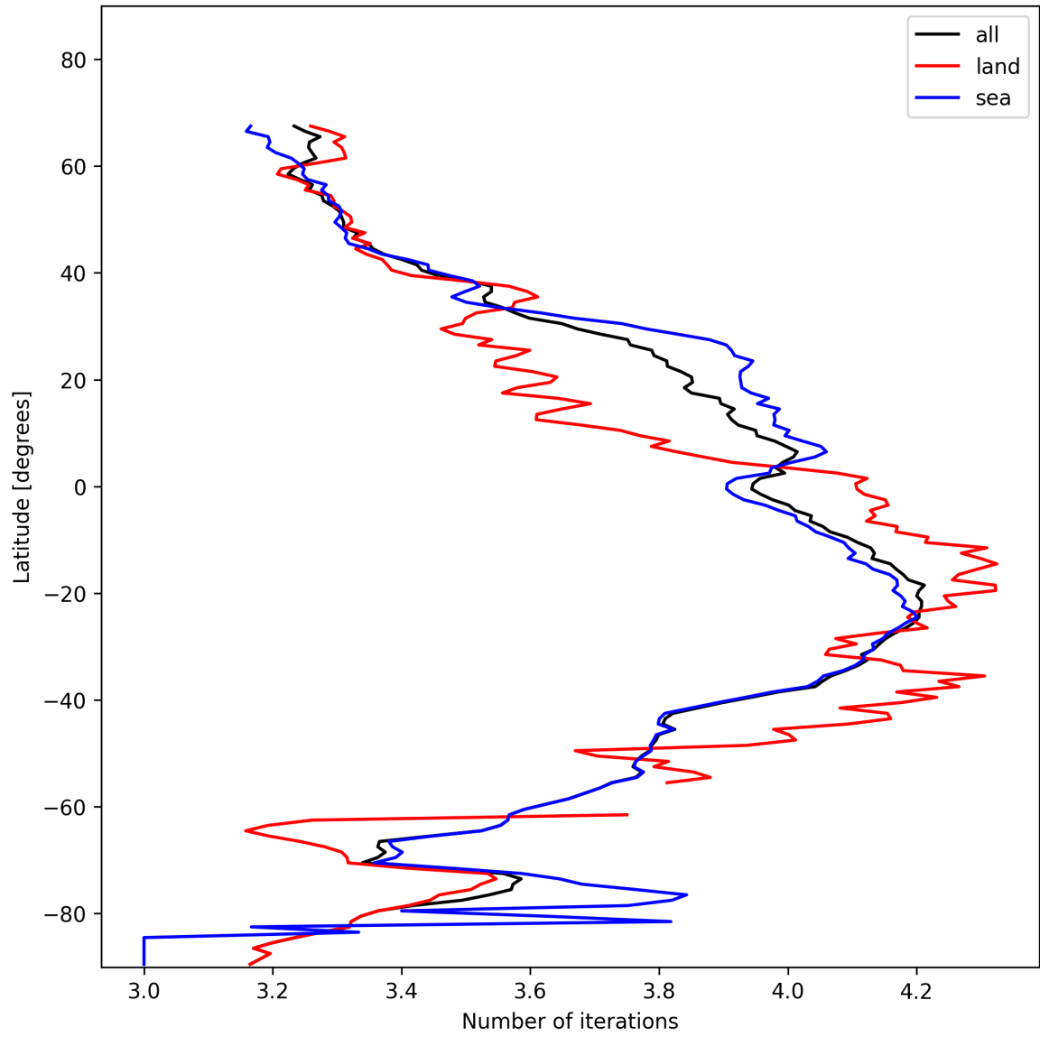
Figure 17: Zonal average of “Number of iterations” for 2025-11-23 to 2025-11-25.
