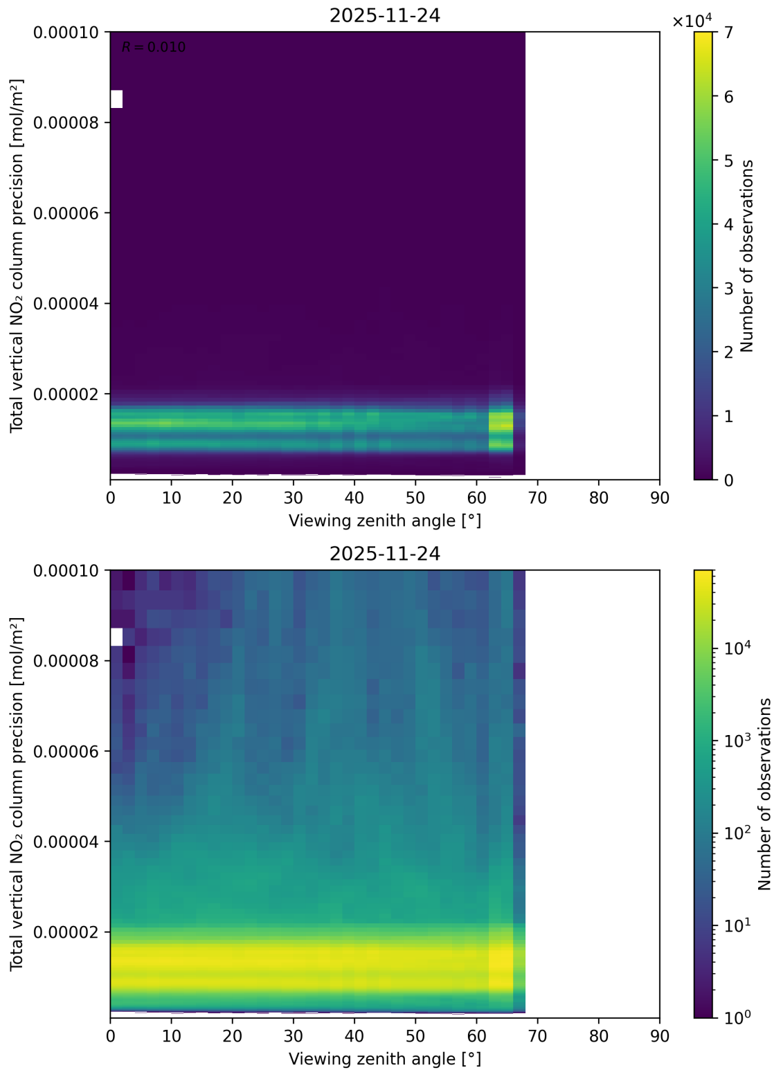
Figure 168: Scatter density plot of “Viewing zenith angle” against “Total vertical NO 2 column precision” for 2025-11-23 to 2025-11-25.
