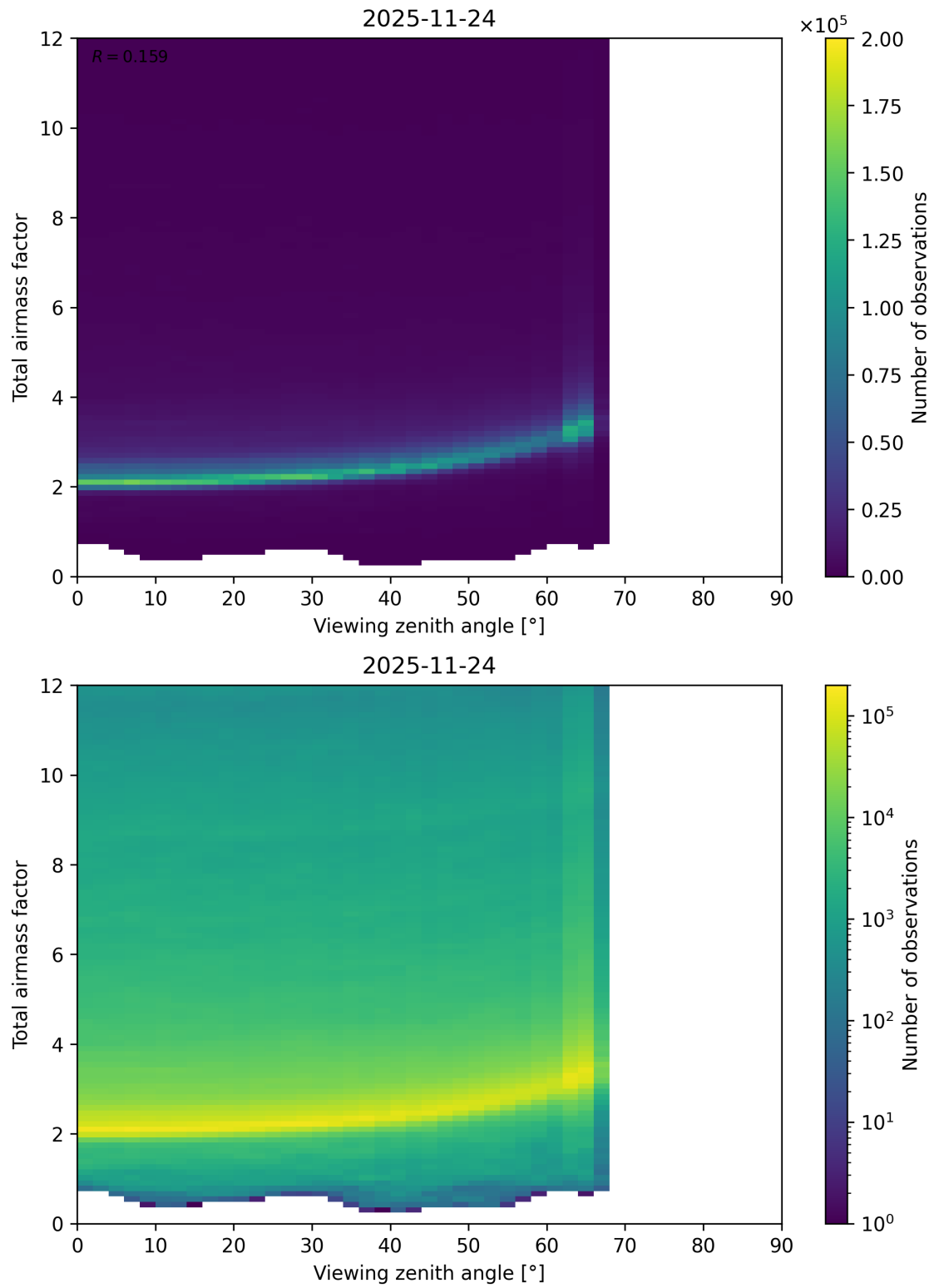
Figure 160: Scatter density plot of “Viewing zenith angle” against “Total airmass factor” for 2025-11-23 to 2025-11-25.
