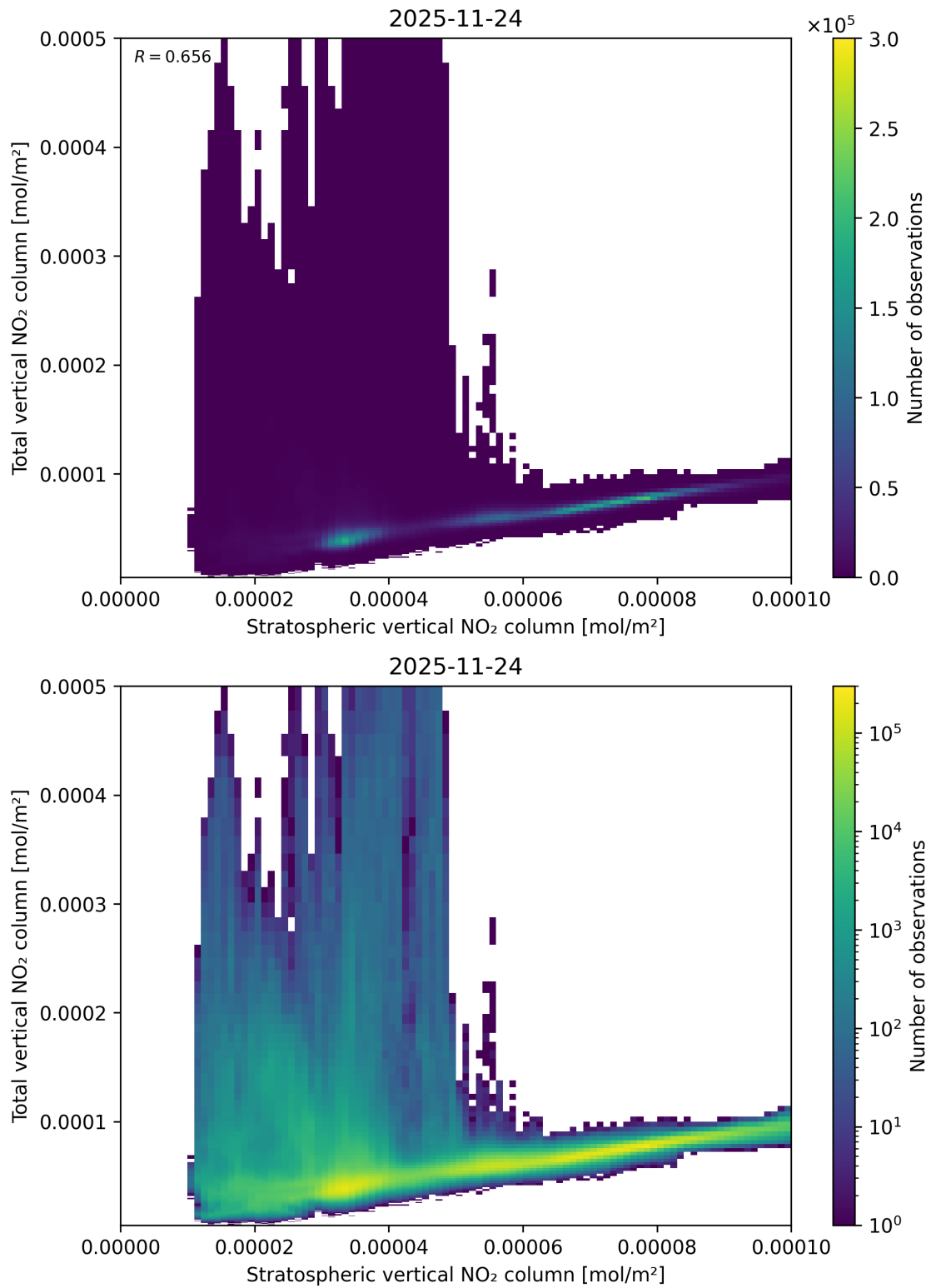
Figure 100: Scatter density plot of “Stratospheric vertical NO 2 column” against “Total vertical NO 2 column” for 2025-11-23 to 2025-11-25.
