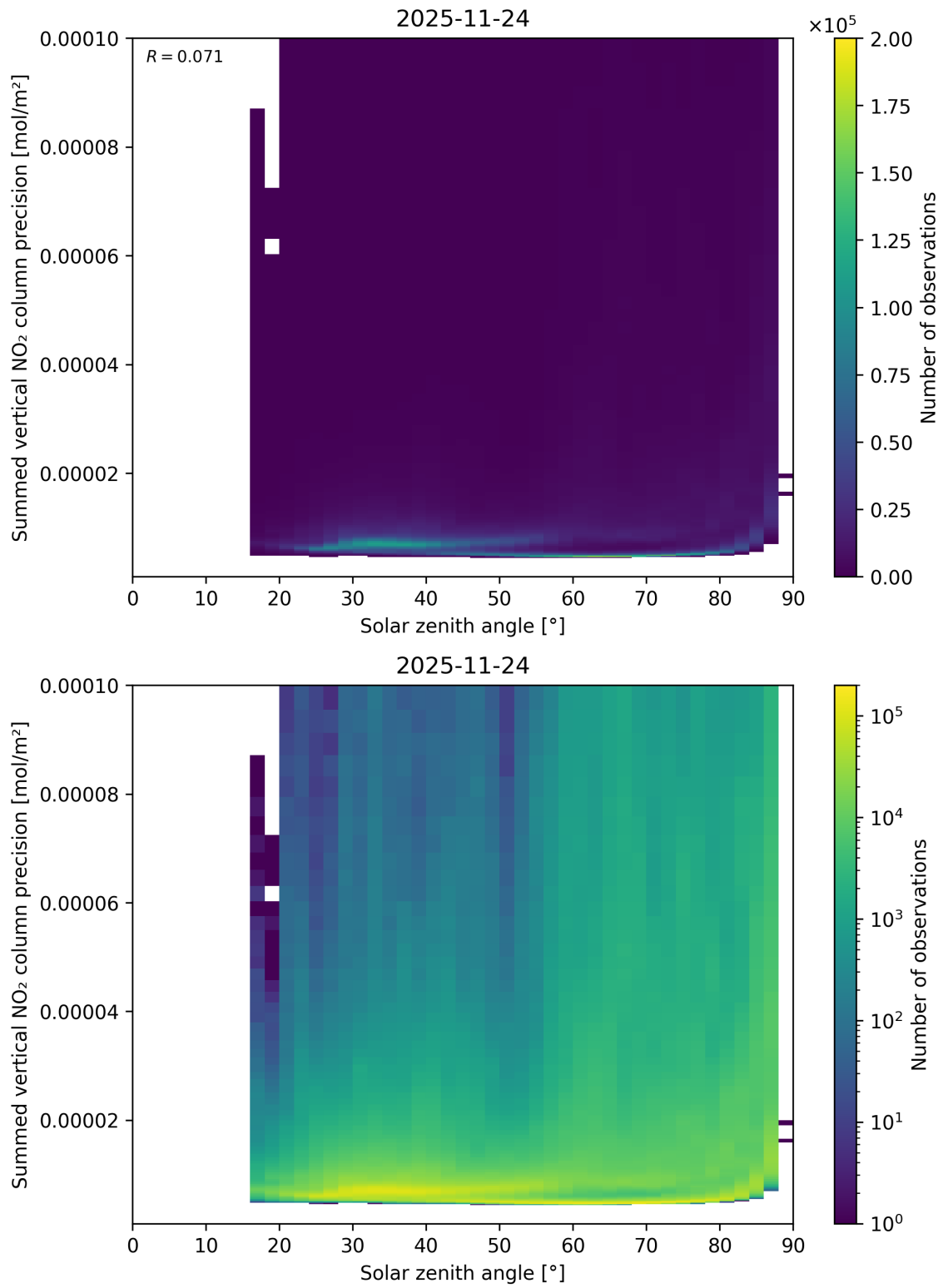
Figure 152: Scatter density plot of “Solar zenith angle” against “Summed vertical NO 2 column precision” for 2025-11-23 to 2025-11-25.
