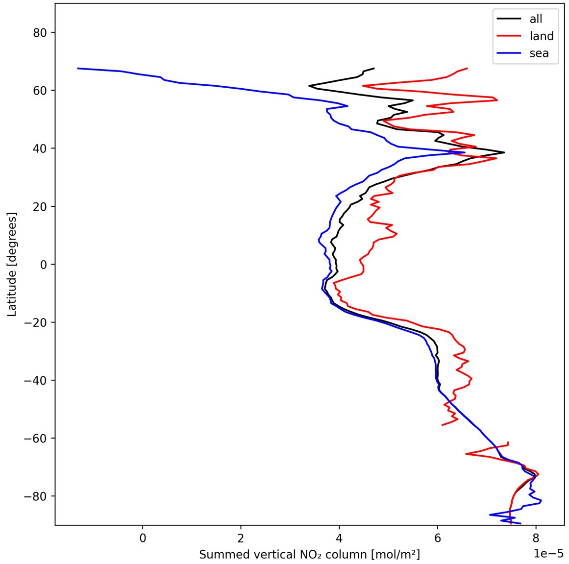
Figure 23: Zonal average of “Summed vertical NO 2 column” for 2025-11-23 to 2025-11-25.
