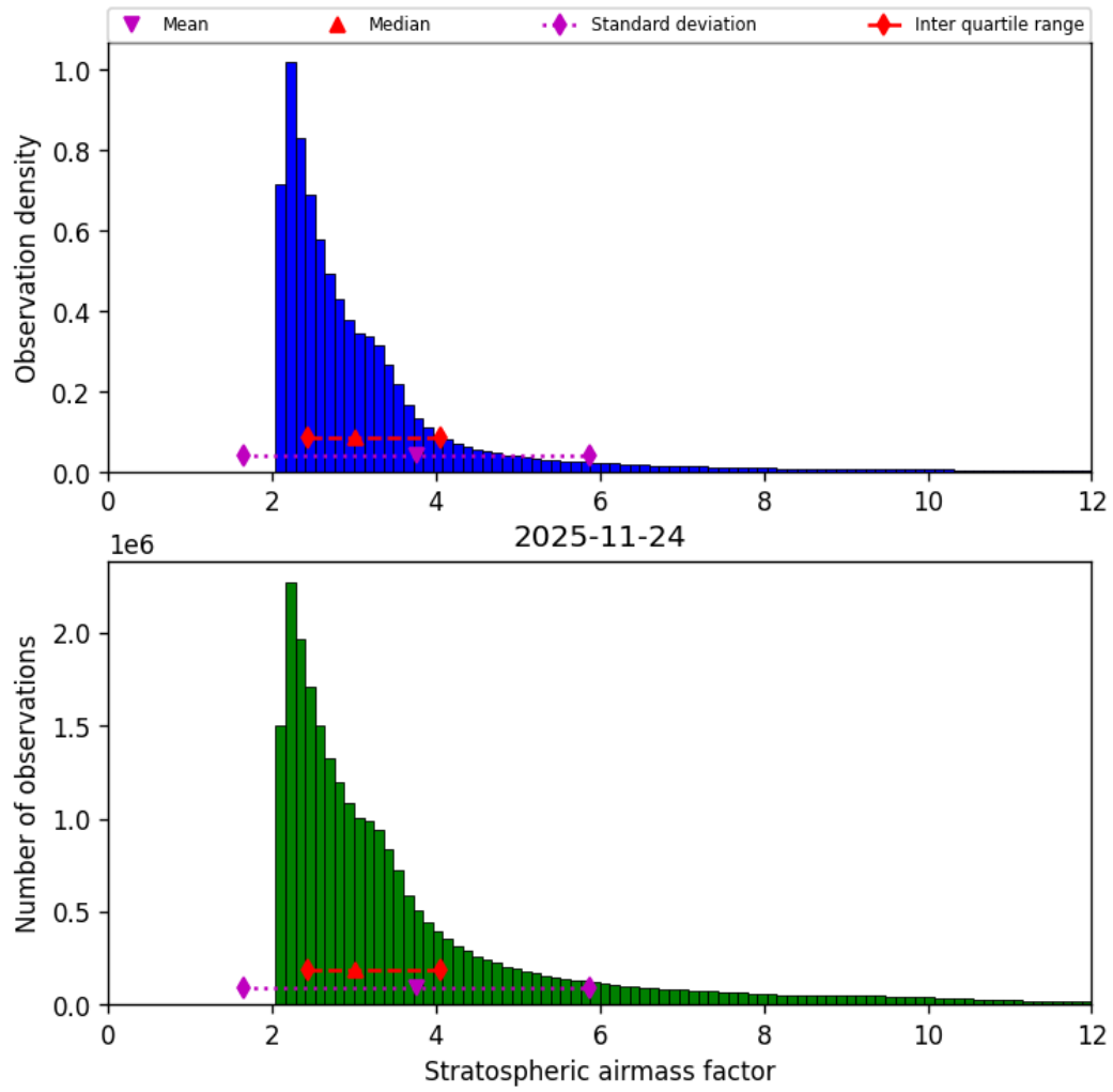
Figure 44: Histogram of “Stratospheric airmass factor” for 2025-11-23 to 2025-11-25
