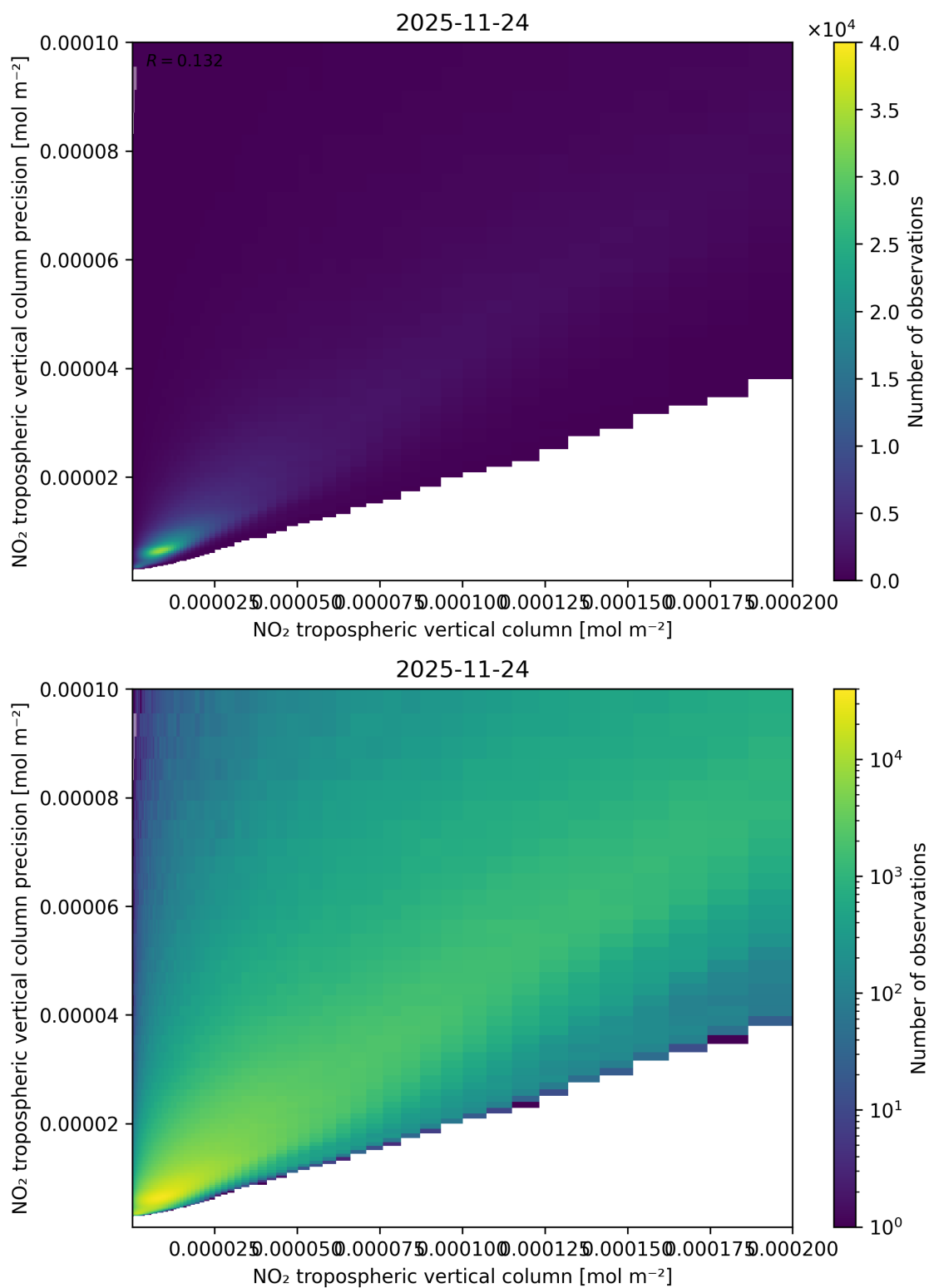
Figure 130: Scatter density plot of “NO 2 tropospheric vertical column” against “NO 2 tropospheric vertical column precision” for 2025-11-23 to 2025-11-25.
