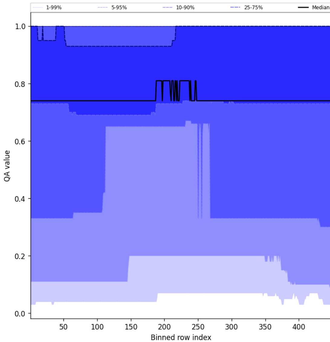
Figure 45: Along track statistics of “QA value” for 2025-11-23 to 2025-11-25
