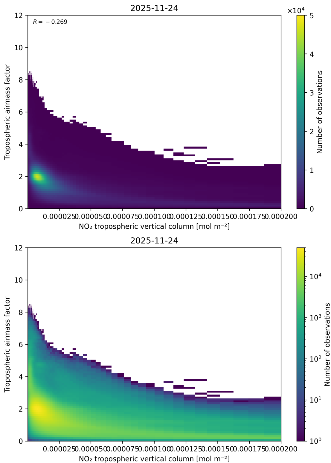
Figure 123: Scatter density plot of “NO 2 tropospheric vertical column” against “Tropospheric airmass factor” for 2025-11-23 to 2025-11-25.
