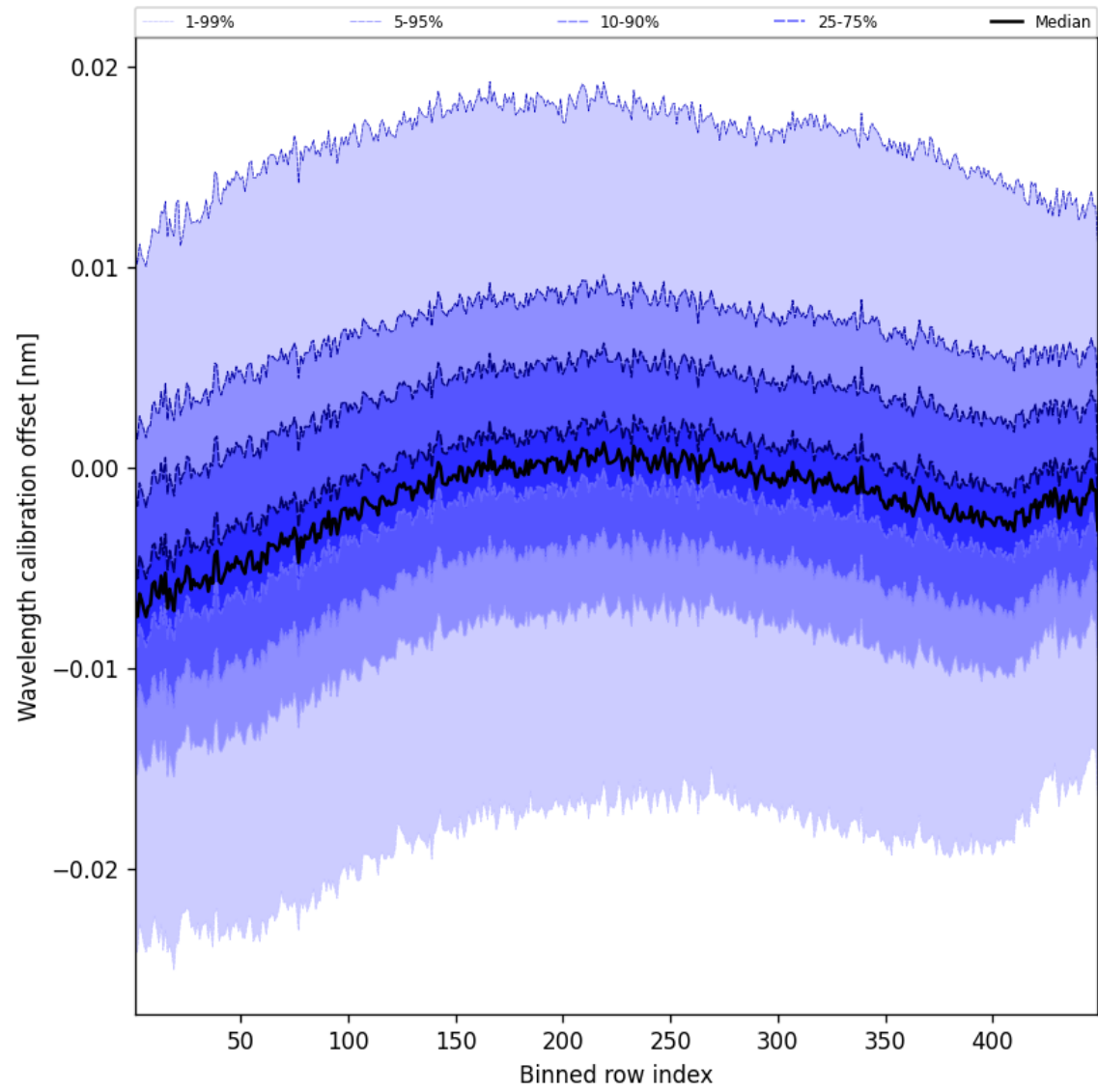
Figure 52: Along track statistics of “Wavelength calibration offset” for 2025-11-23 to 2025-11-25
