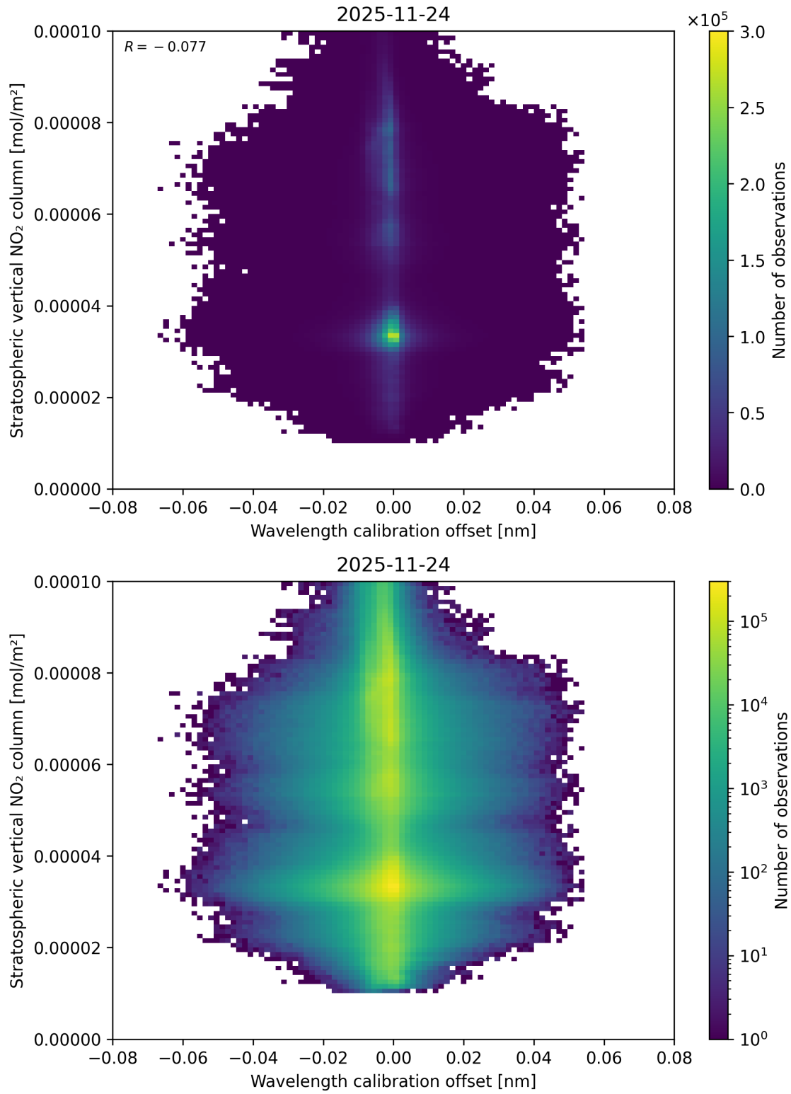
Figure 176: Scatter density plot of “Wavelength calibration offset” against “Stratospheric vertical NO 2 column” for 2025-11-23 to 2025-11-25.
