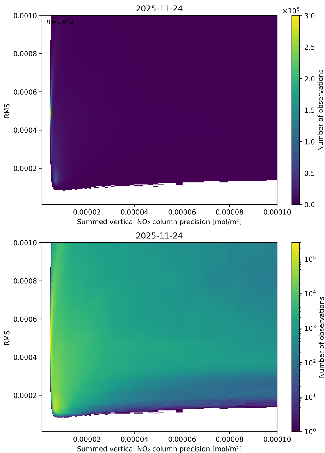
Figure 108: Scatter density plot of “Summed vertical NO 2 column precision” against “RMS” for 2025-11-23 to 2025-11-25.
