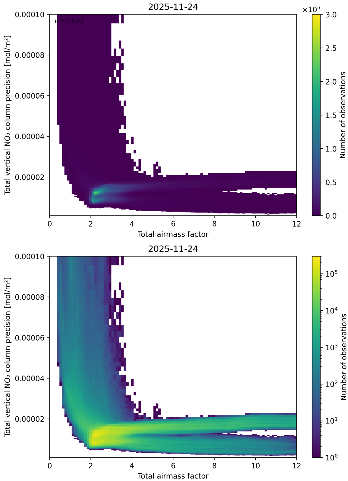
Figure 68: Scatter density plot of “Total airmass factor” against “Total vertical NO 2 column precision” for 2025-11-23 to 2025-11-25.
