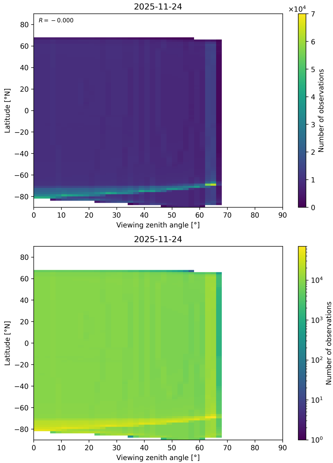
Figure 163: Scatter density plot of “Viewing zenith angle” against “Latitude” for 2025-11-23 to 2025-11-25.
