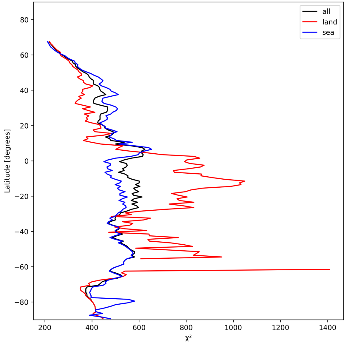
Figure 25: Zonal average of “ \chi^2 ” for 2025-11-23 to 2025-11-25.
