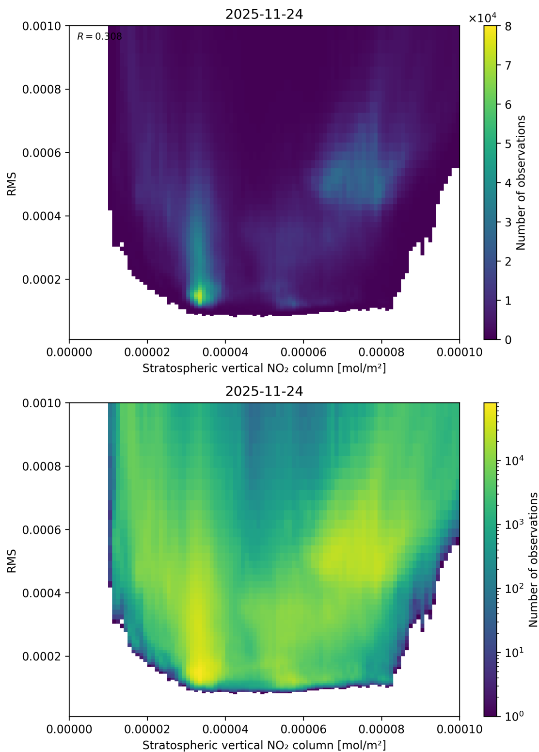
Figure 102: Scatter density plot of “Stratospheric vertical NO 2 column” against “RMS” for 2025-11-23 to 2025-11-25.
