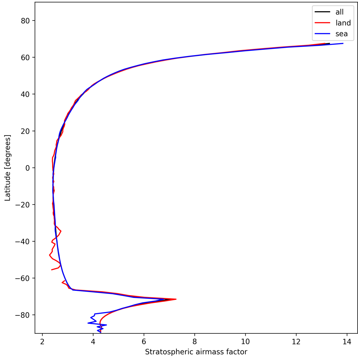
Figure 27: Zonal average of “Stratospheric airmass factor” for 2025-11-23 to 2025-11-25.
