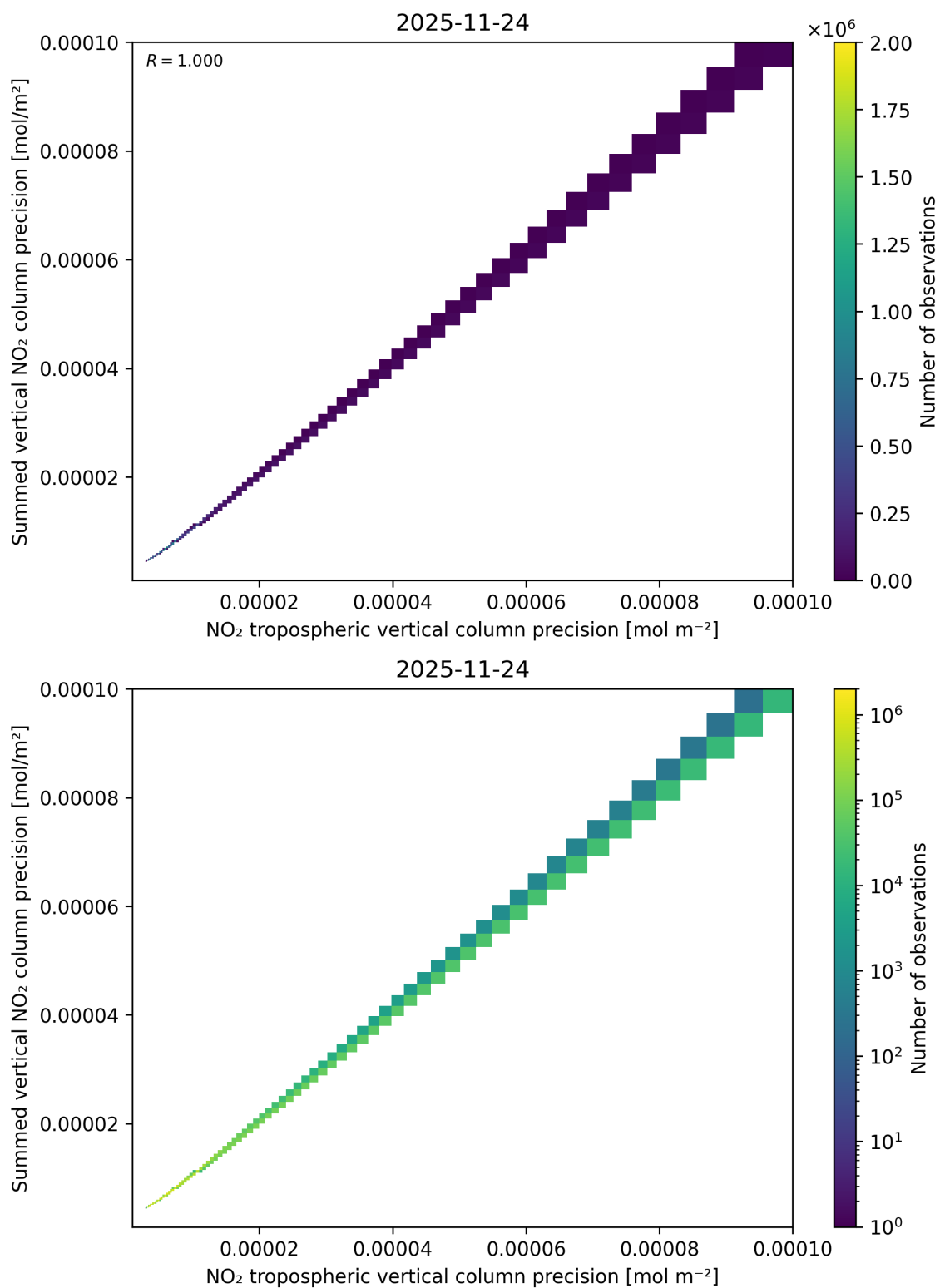
Figure 137: Scatter density plot of “NO 2 tropospheric vertical column precision” against “Summed vertical NO 2 column precision” for 2025-11-23 to 2025-11-25.
