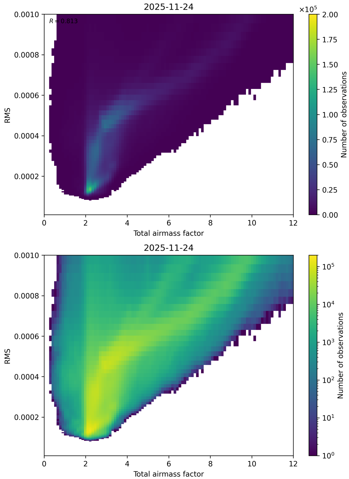
Figure 69: Scatter density plot of “Total airmass factor” against “RMS” for 2025-11-23 to 2025-11-25.
