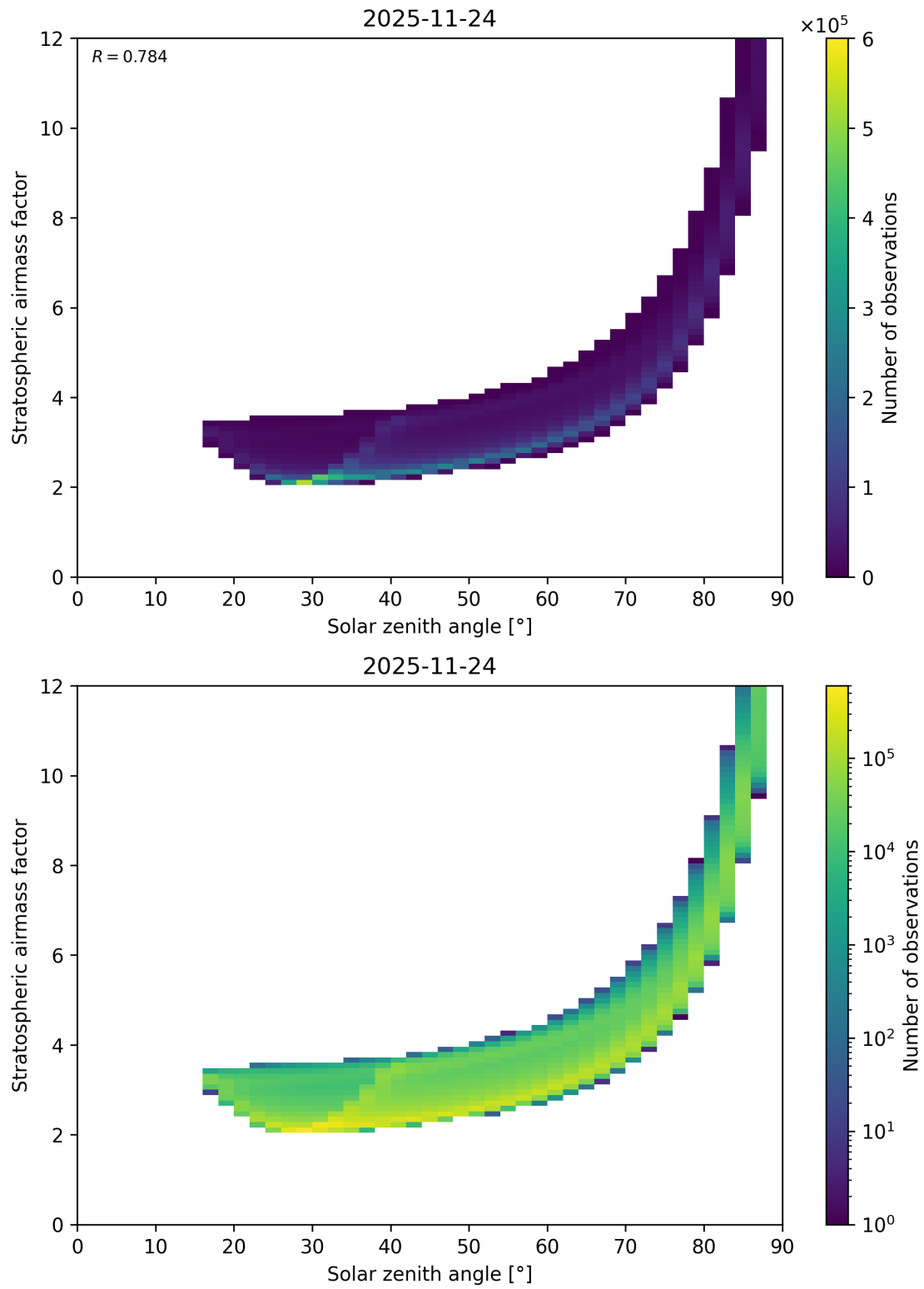
Figure 145: Scatter density plot of “Solar zenith angle” against “Stratospheric airmass factor” for 2025-11-23 to 2025-11-25.
