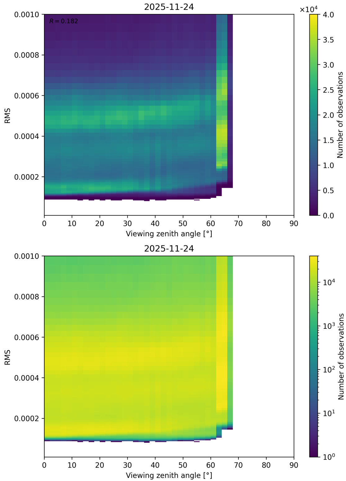
Figure 171: Scatter density plot of “Viewing zenith angle” against “RMS” for 2025-11-23 to 2025-11-25.
