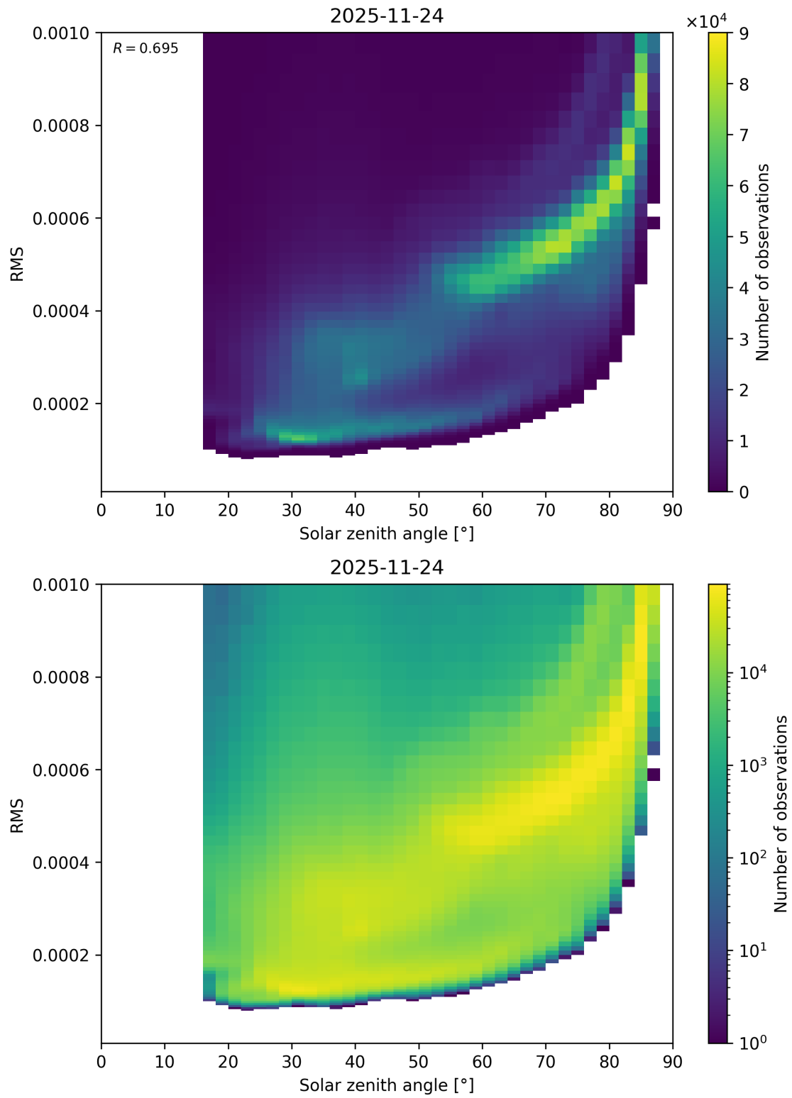
Figure 157: Scatter density plot of “Solar zenith angle” against “RMS” for 2025-11-23 to 2025-11-25.
