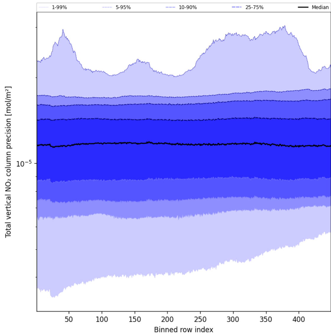
Figure 56: Along track statistics of “Total vertical NO 2 column precision” for 2025-11-23 to 2025-11-25
