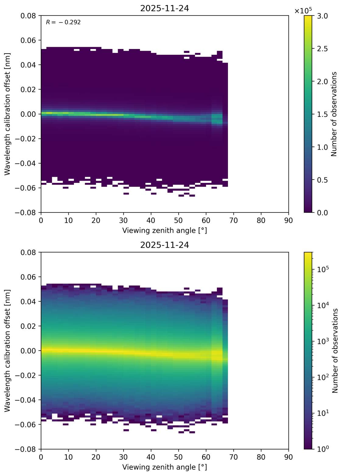
Figure 173: Scatter density plot of “Viewing zenith angle” against “Wavelength calibration offset” for 2025-11-23 to 2025-11-25.
