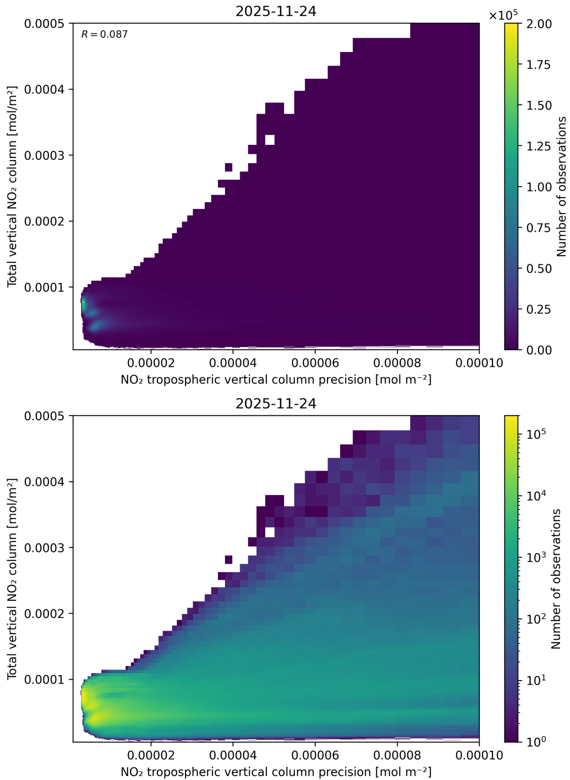
Figure 138: Scatter density plot of “NO 2 tropospheric vertical column precision” against “Total vertical NO 2 column” for 2025-11-23 to 2025-11-25.
