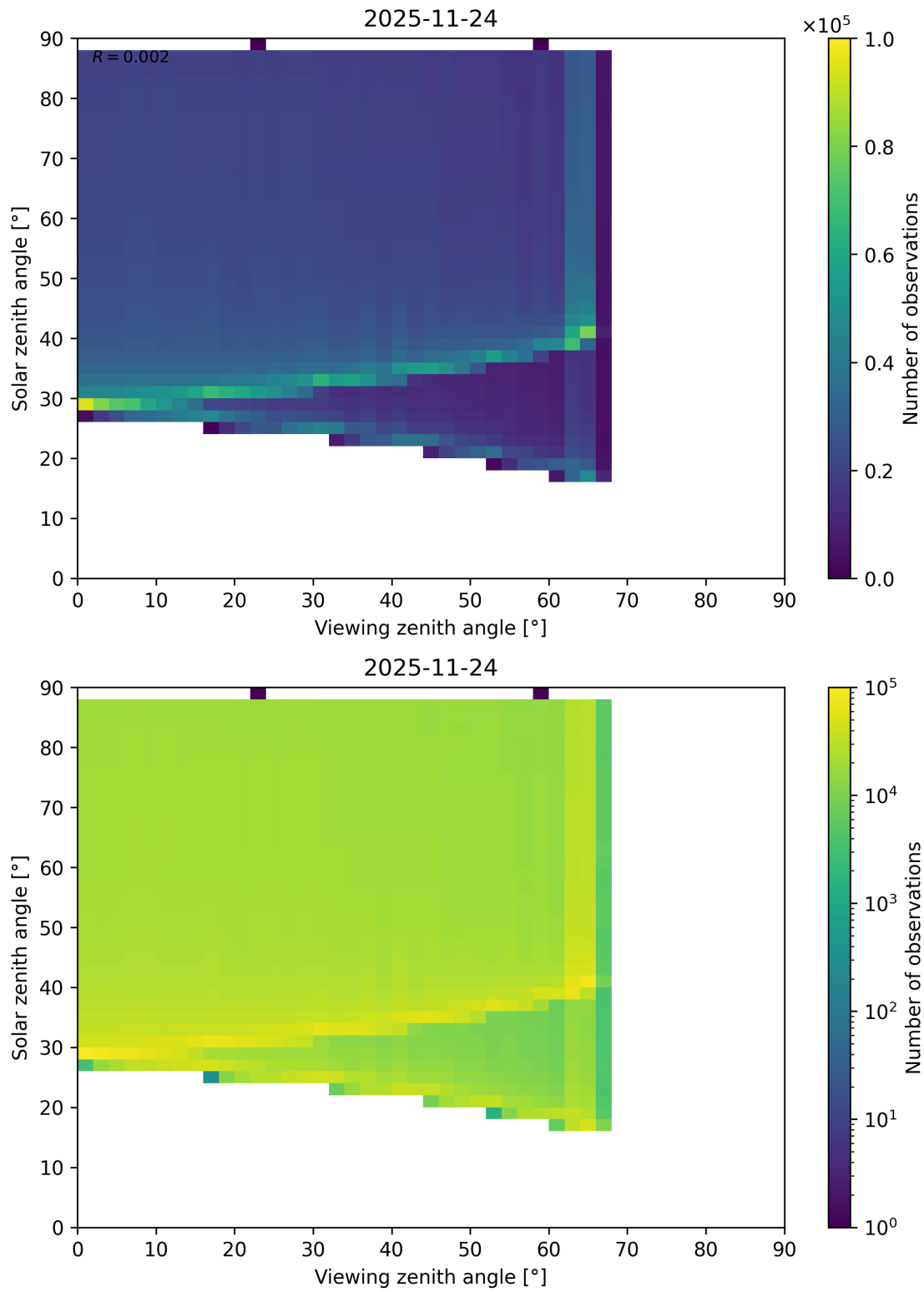
Figure 172: Scatter density plot of “Viewing zenith angle” against “Solar zenith angle” for 2025-11-23 to 2025-11-25.
