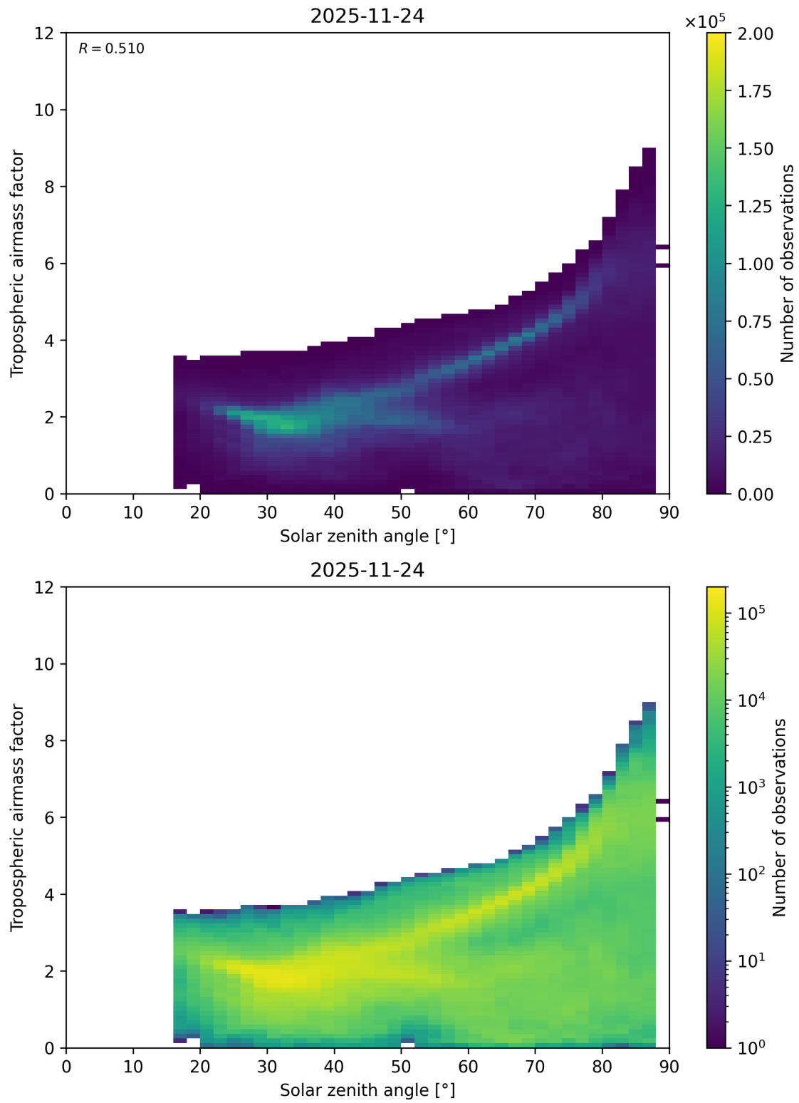
Figure 147: Scatter density plot of “Solar zenith angle” against “Tropospheric airmass factor” for 2025-11-23 to 2025-11-25.
