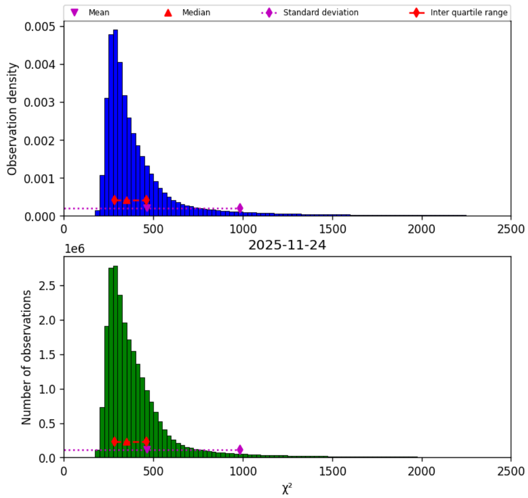
Figure 42: Histogram of “ \chi^2 ” for 2025-11-23 to 2025-11-25
