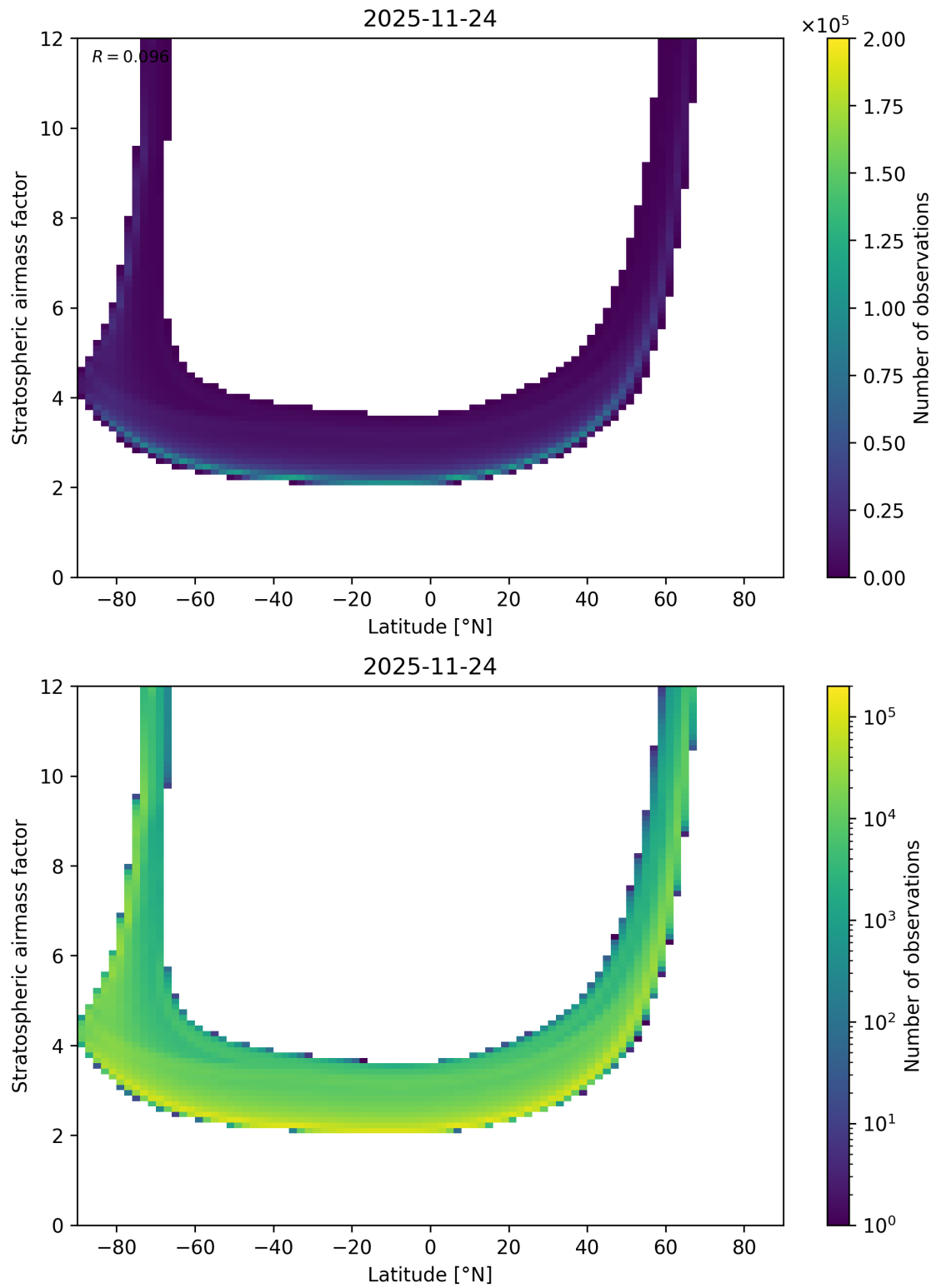
Figure 83: Scatter density plot of “Latitude” against “Stratospheric airmass factor” for 2025-11-23 to 2025-11-25.
