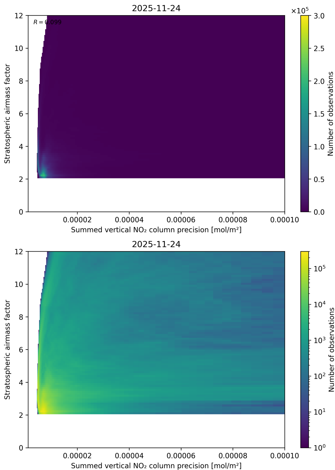
Figure 106: Scatter density plot of “Summed vertical NO 2 column precision” against “Stratospheric airmass factor” for 2025-11-23 to 2025-11-25.
