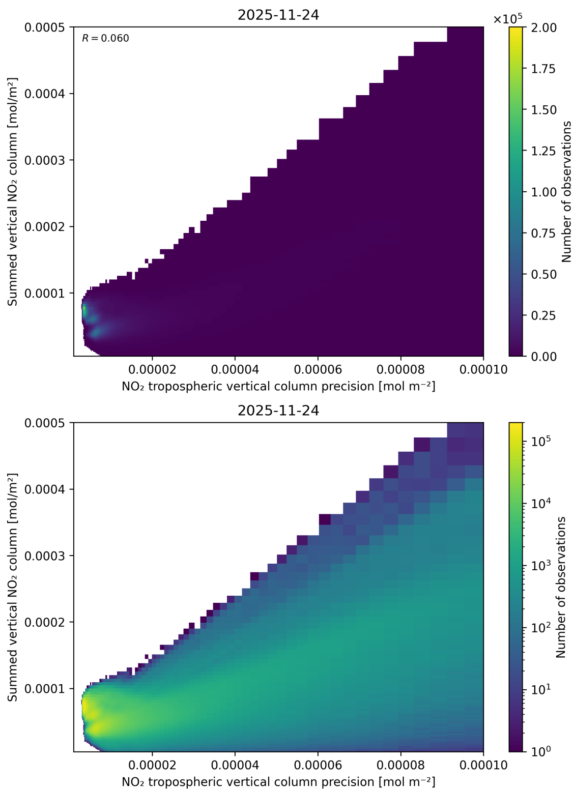
Figure 136: Scatter density plot of “NO 2 tropospheric vertical column precision” against “Summed vertical NO 2 column” for 2025-11-23 to 2025-11-25.
