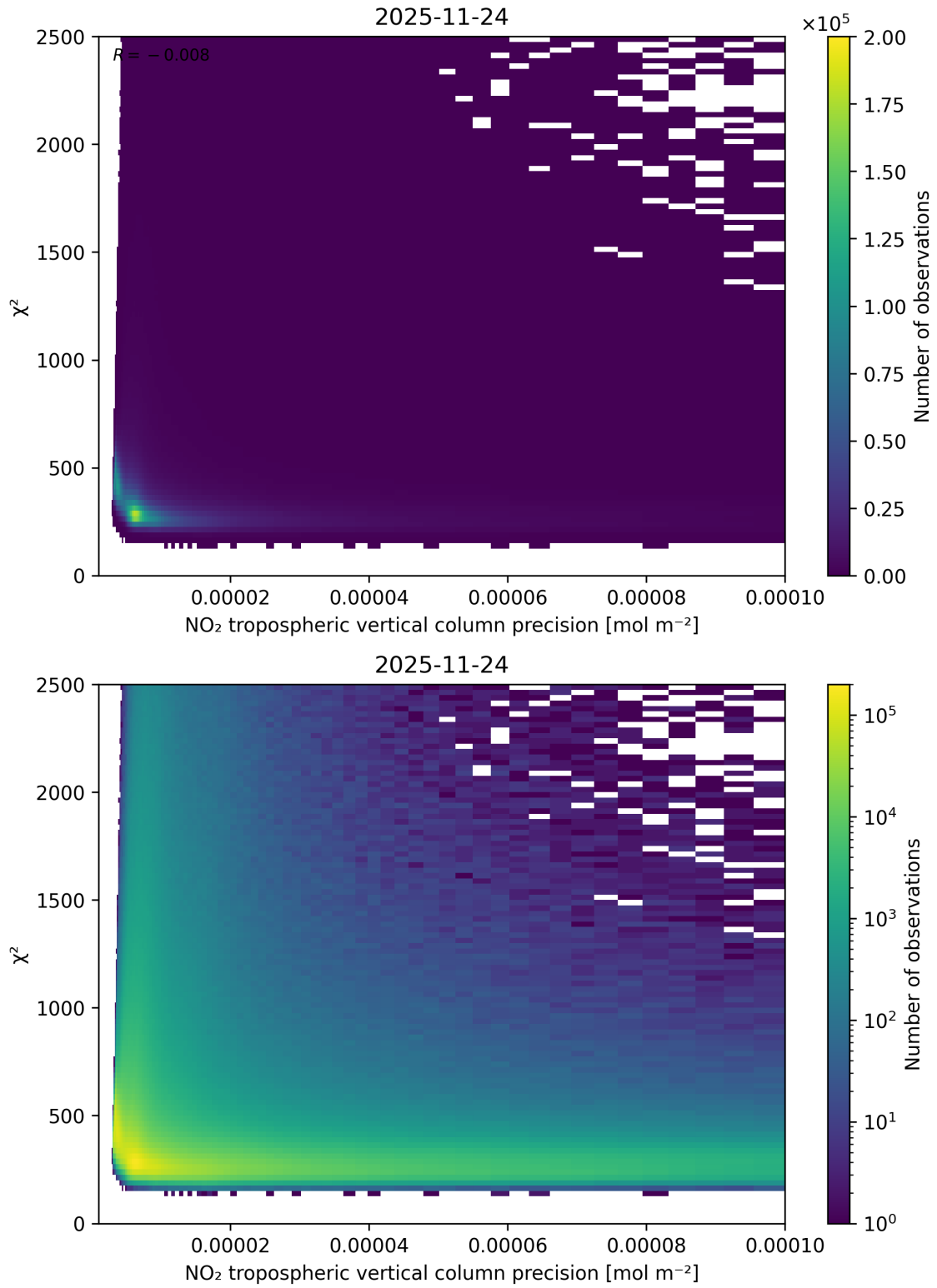
Figure 134: Scatter density plot of “NO 2 tropospheric vertical column precision” against “ \chi^2 ” for 2025-11-23 to 2025-11-25.
