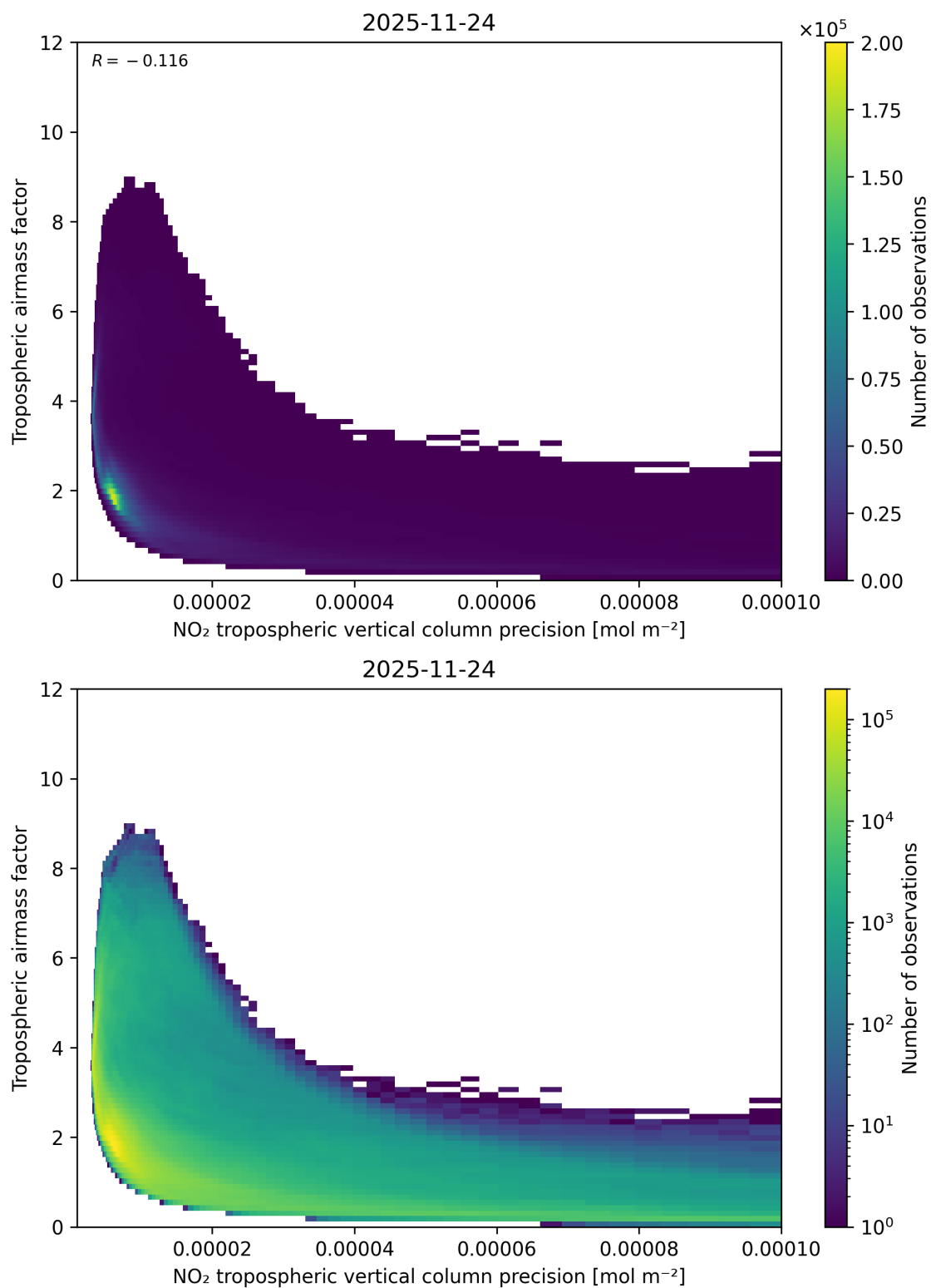
Figure 133: Scatter density plot of “NO 2 tropospheric vertical column precision” against “Tropospheric airmass factor” for 2025-11-23 to 2025-11-25.
