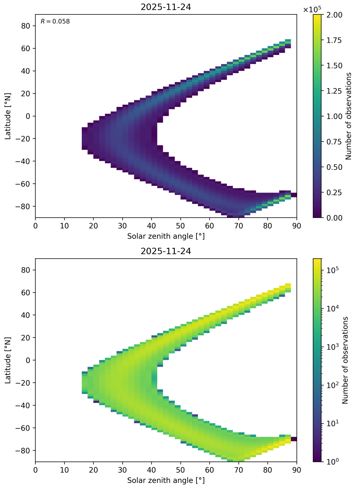
Figure 149: Scatter density plot of “Solar zenith angle” against “Latitude” for 2025-11-23 to 2025-11-25.
