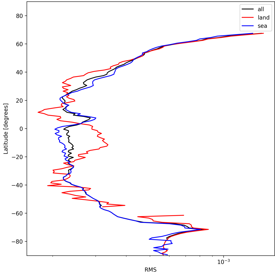
Figure 26: Zonal average of “RMS” for 2025-11-23 to 2025-11-25.
