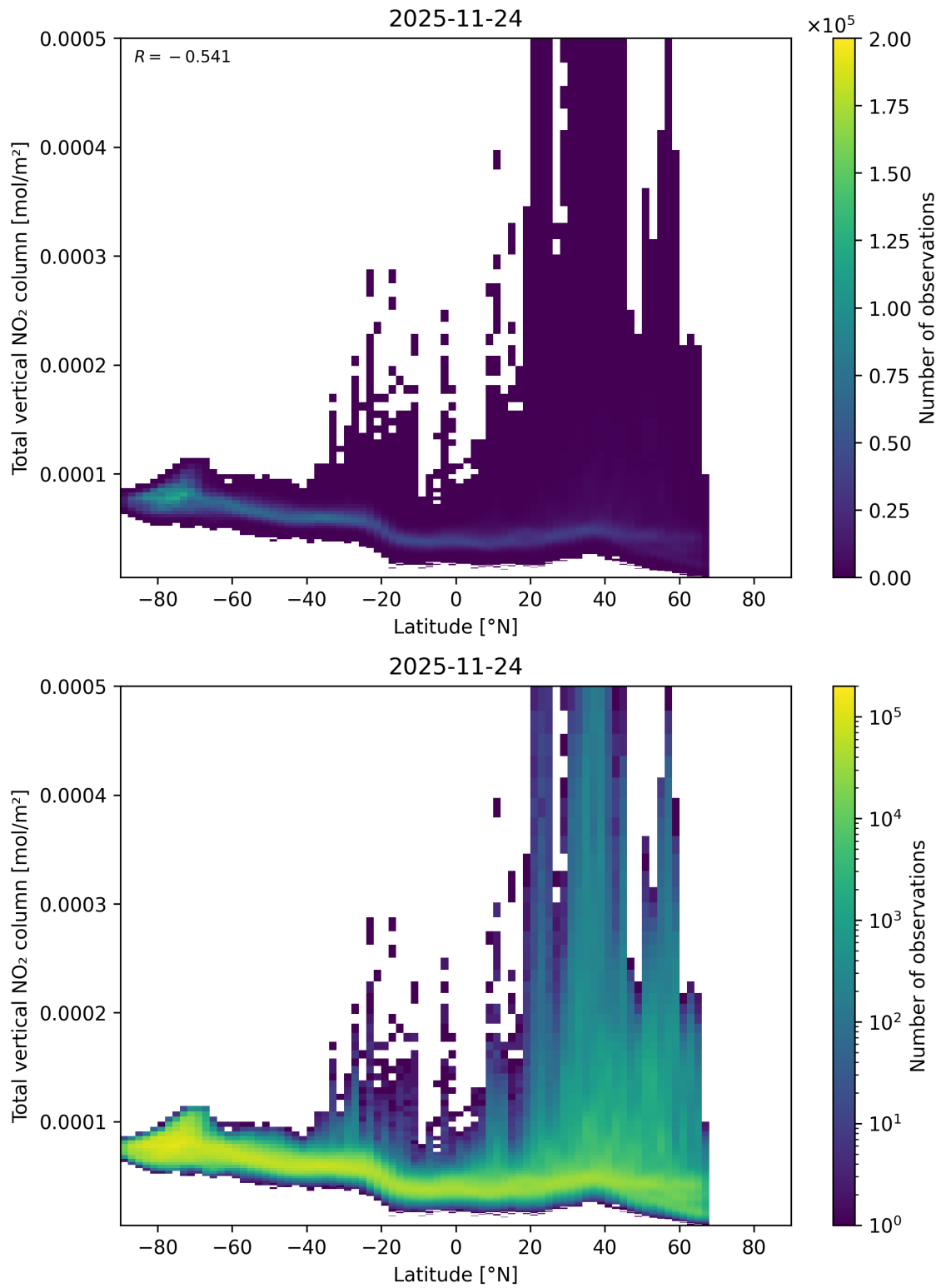
Figure 90: Scatter density plot of “Latitude” against “Total vertical NO 2 column” for 2025-11-23 to 2025-11-25.
