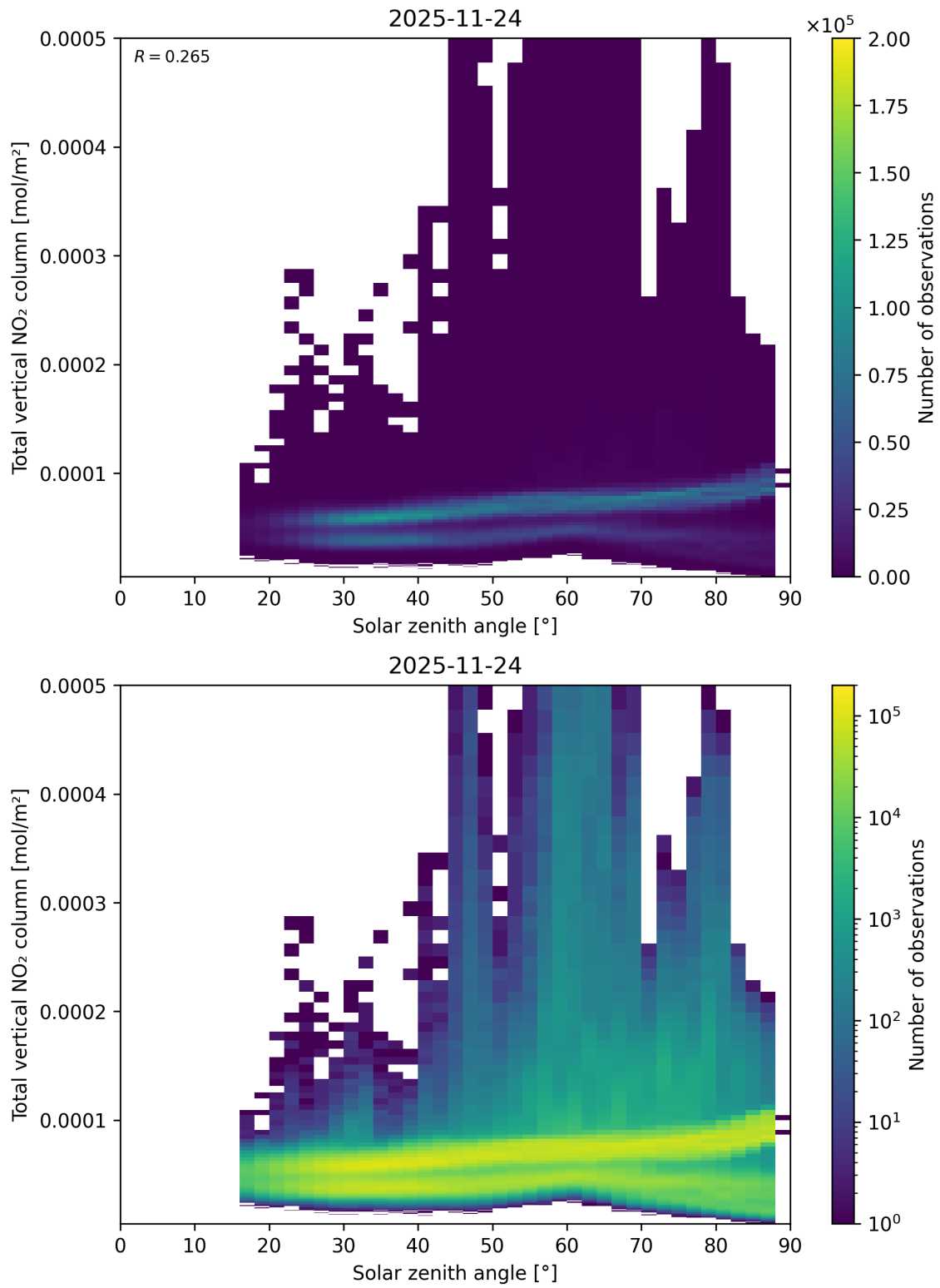
Figure 153: Scatter density plot of “Solar zenith angle” against “Total vertical NO 2 column” for 2025-11-23 to 2025-11-25.
