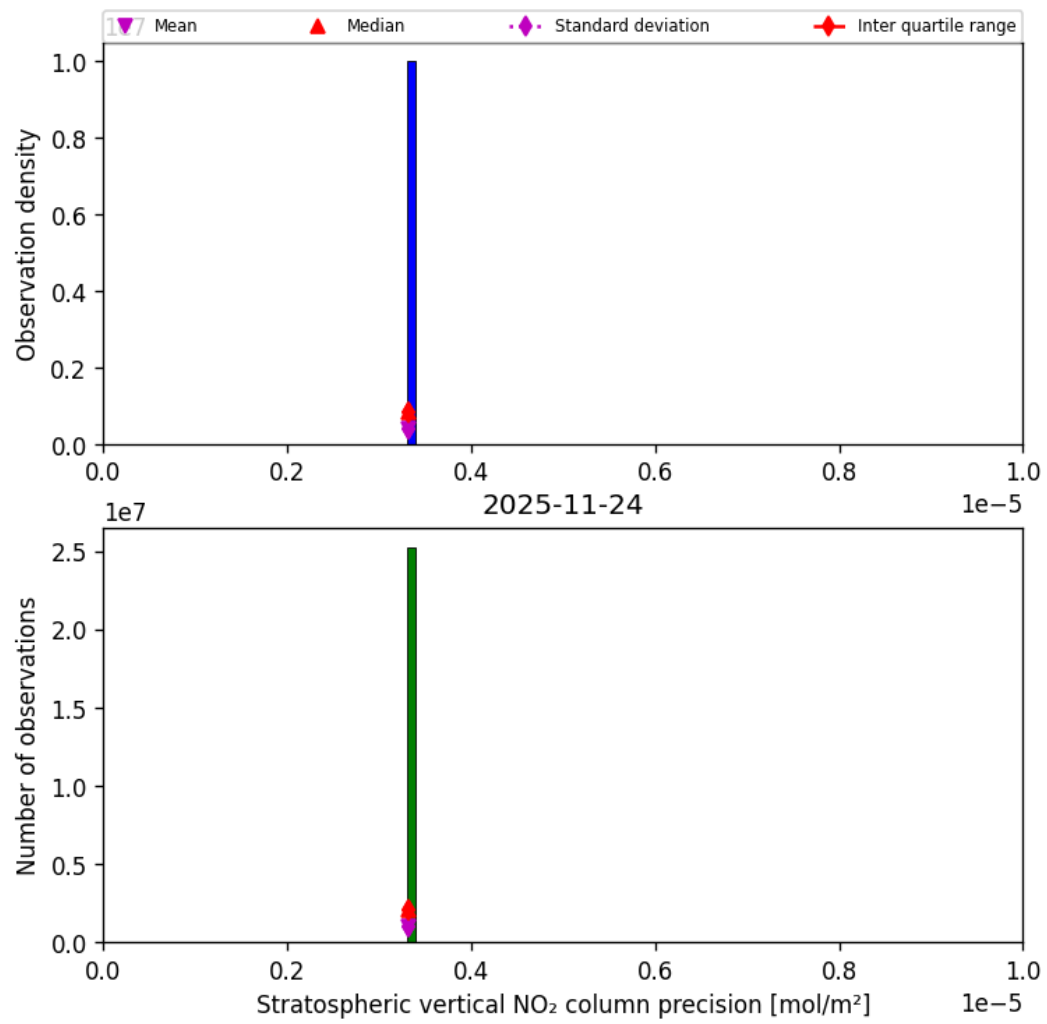
Figure 37: Histogram of “Stratospheric vertical NO 2 column precision” for 2025-11-23 to 2025-11-25
