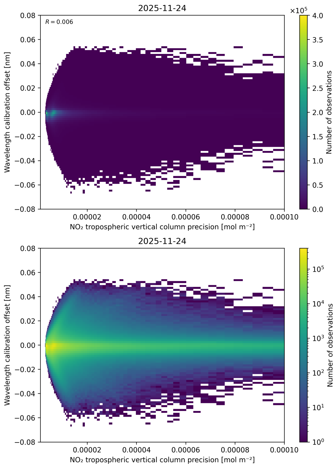
Figure 141: Scatter density plot of “NO 2 tropospheric vertical column precision” against “Wavelength calibration offset” for 2025-11-23 to 2025-11-25.
