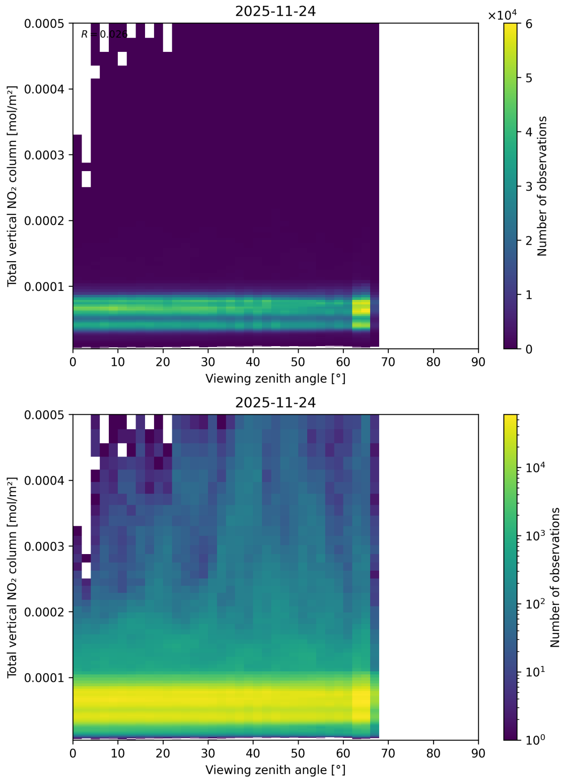
Figure 167: Scatter density plot of “Viewing zenith angle” against “Total vertical NO 2 column” for 2025-11-23 to 2025-11-25.
