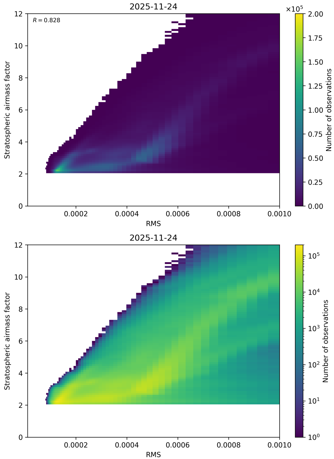
Figure 144: Scatter density plot of “RMS” against “Stratospheric airmass factor” for 2025-11-23 to 2025-11-25.
