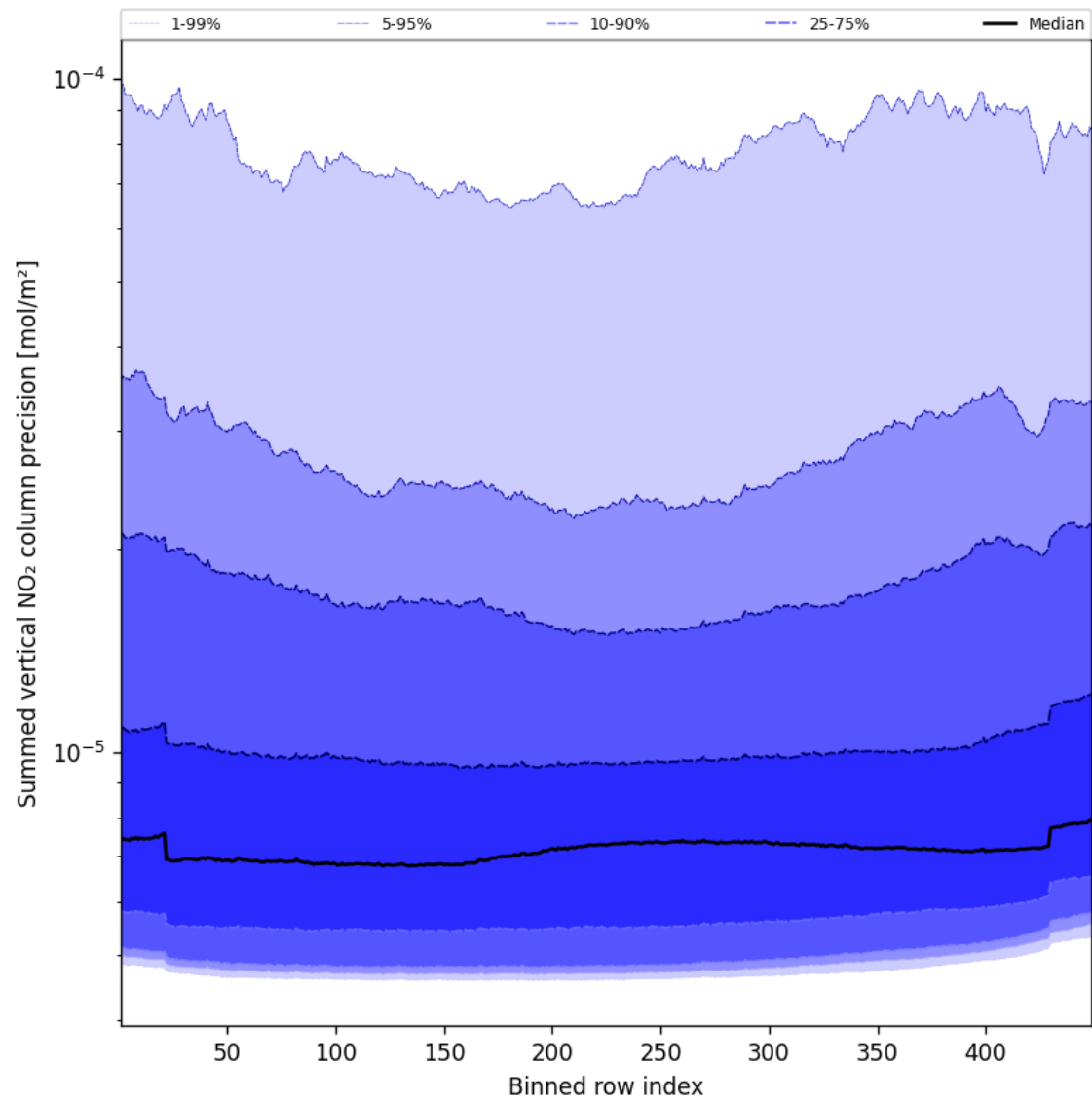
Figure 58: Along track statistics of “Summed vertical NO 2 column precision” for 2025-11-23 to 2025-11-25
