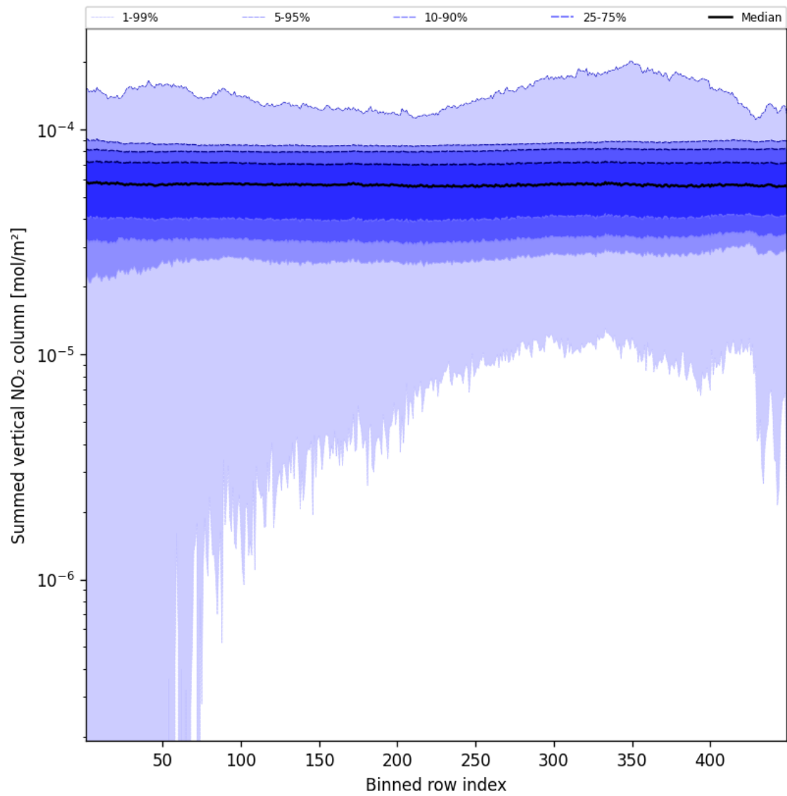
Figure 57: Along track statistics of “Summed vertical NO 2 column” for 2025-11-23 to 2025-11-25
