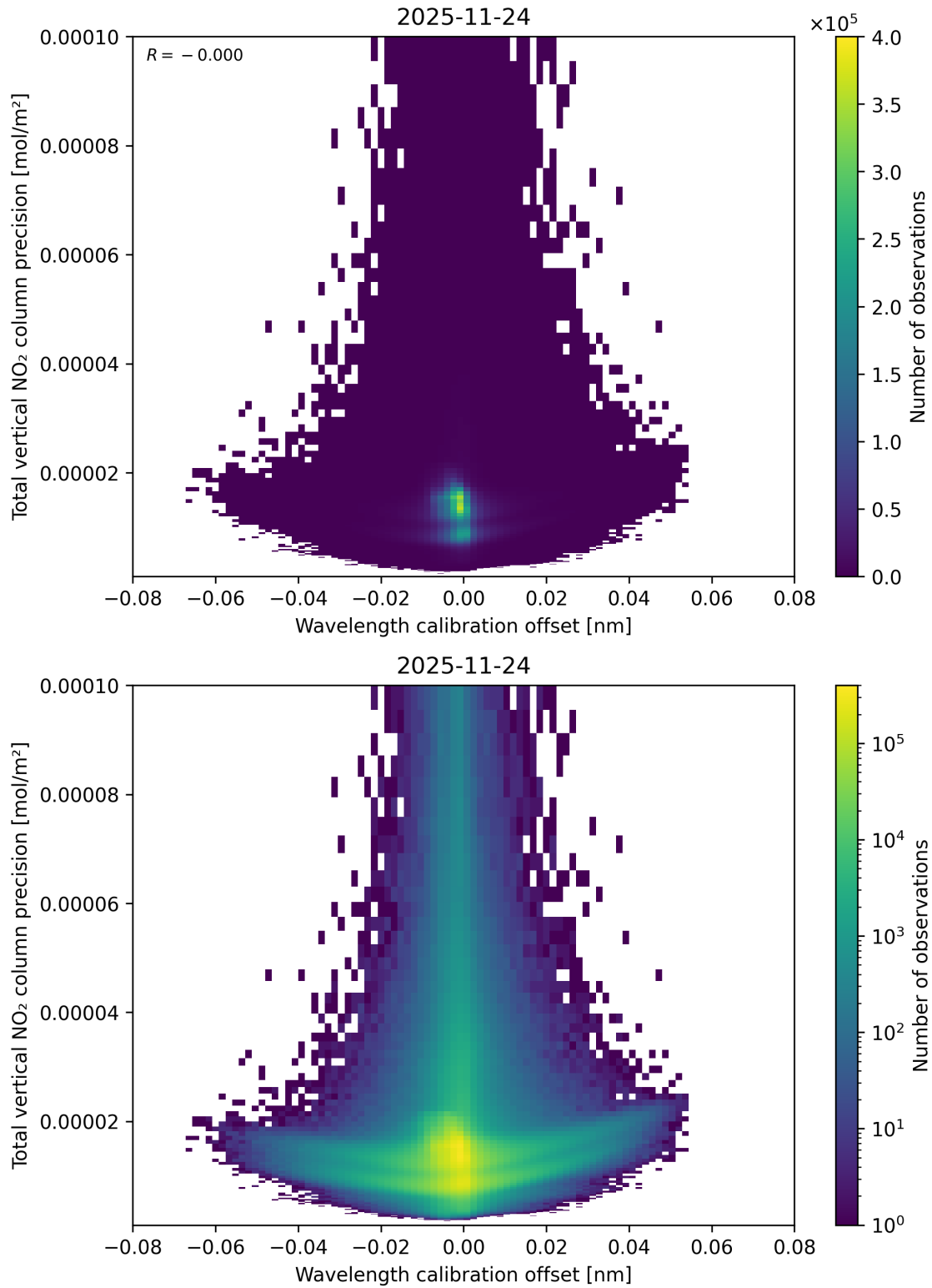
Figure 180: Scatter density plot of “Wavelength calibration offset” against “Total vertical NO 2 column precision” for 2025-11-23 to 2025-11-25.
