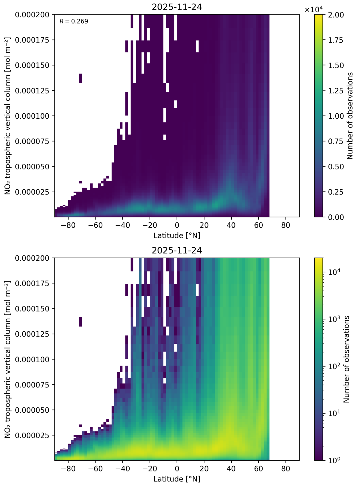
Figure 92: Scatter density plot of “Latitude” against “NO 2 tropospheric vertical column” for 2025-11-23 to 2025-11-25.
