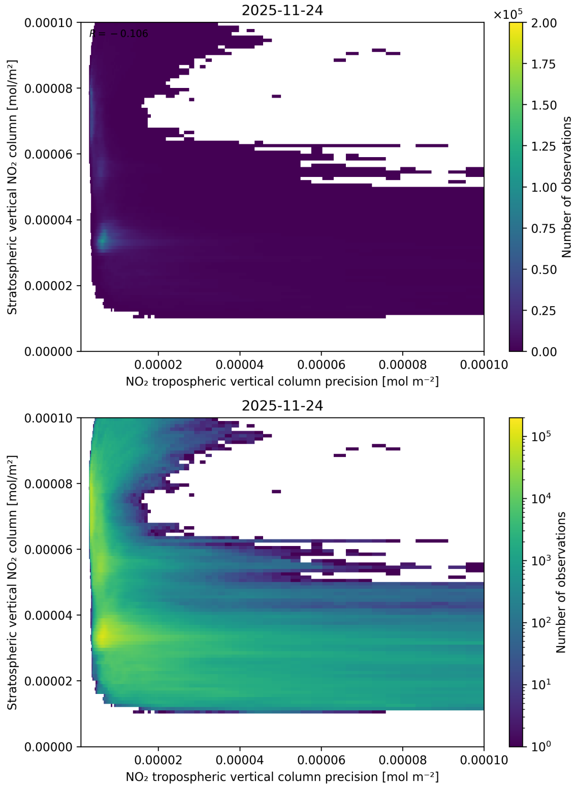
Figure 135: Scatter density plot of “NO 2 tropospheric vertical column precision” against “Stratospheric vertical NO 2 column” for 2025-11-23 to 2025-11-25.
