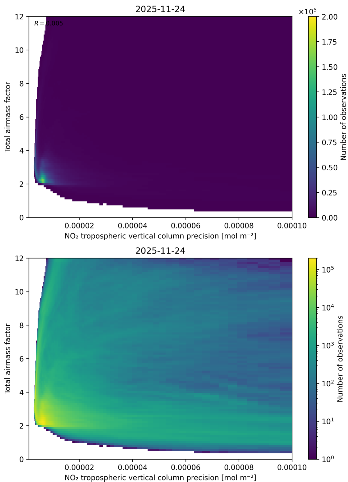
Figure 132: Scatter density plot of “NO 2 tropospheric vertical column precision” against “Total air mass factor” for 2025-11-23 to 2025-11-25.
