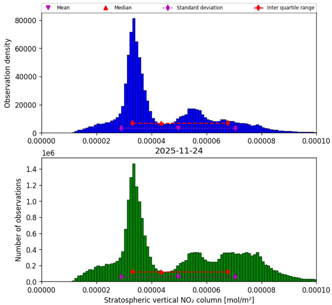
Figure 36: Histogram of “Stratospheric vertical NO 2 column” for 2025-11-23 to 2025-11-25
