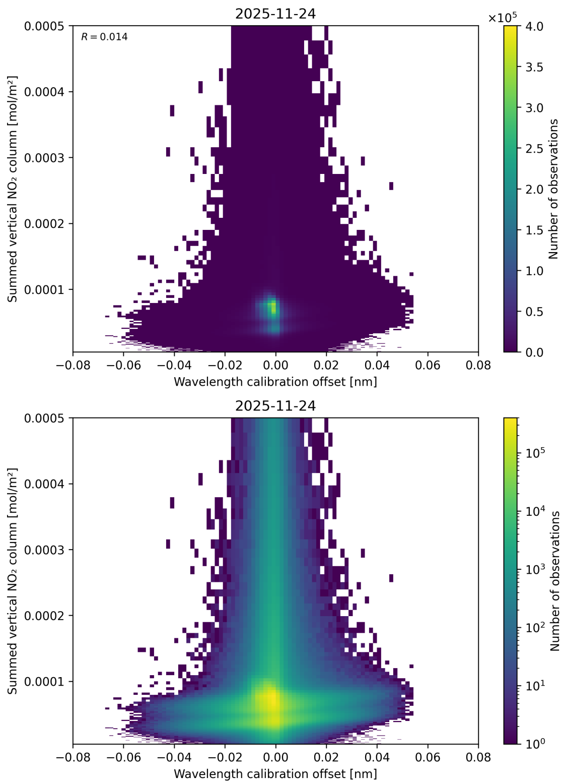
Figure 177: Scatter density plot of “Wavelength calibration offset” against “Summed vertical NO 2 column” for 2025-11-23 to 2025-11-25.
