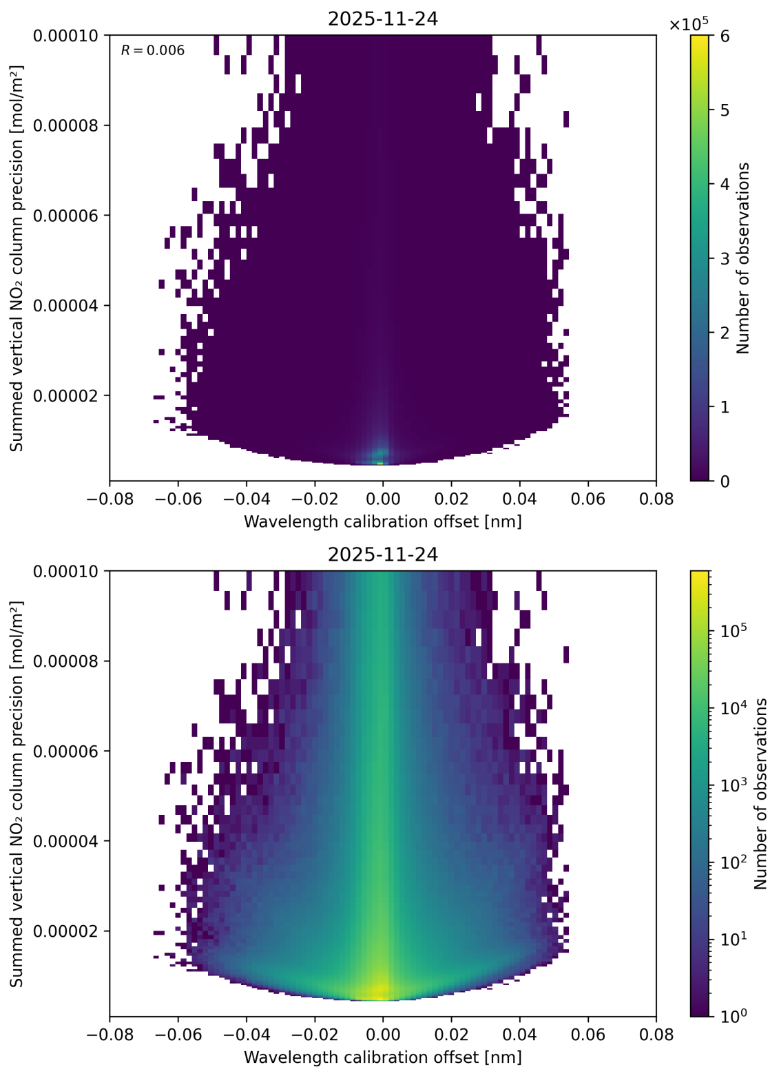
Figure 178: Scatter density plot of “Wavelength calibration offset” against “Summed vertical NO 2 column precision” for 2025-11-23 to 2025-11-25.
