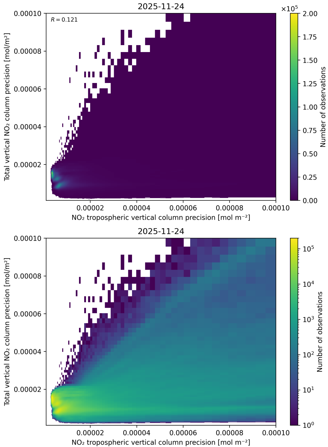
Figure 139: Scatter density plot of “NO 2 tropospheric vertical column precision” against “Total vertical NO 2 column precision” for 2025-11-23 to 2025-11-25.
