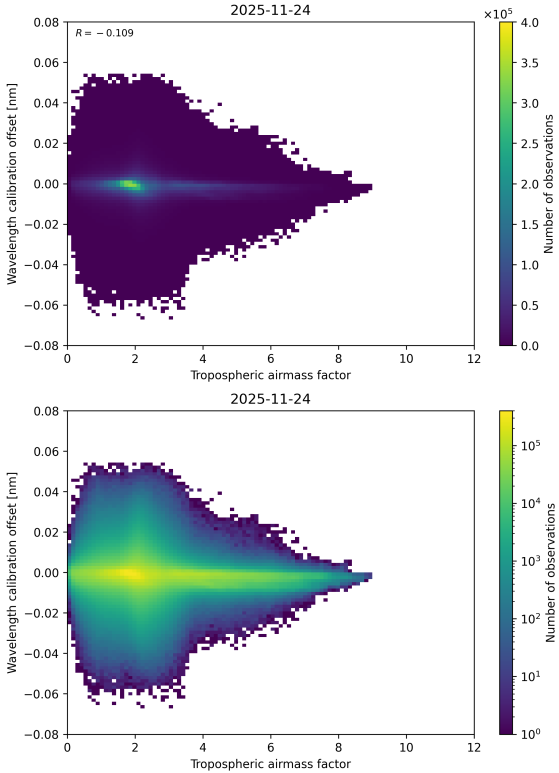
Figure 80: Scatter density plot of “Tropospheric airmass factor” against “Wavelength calibration offset” for 2025-11-23 to 2025-11-25.
