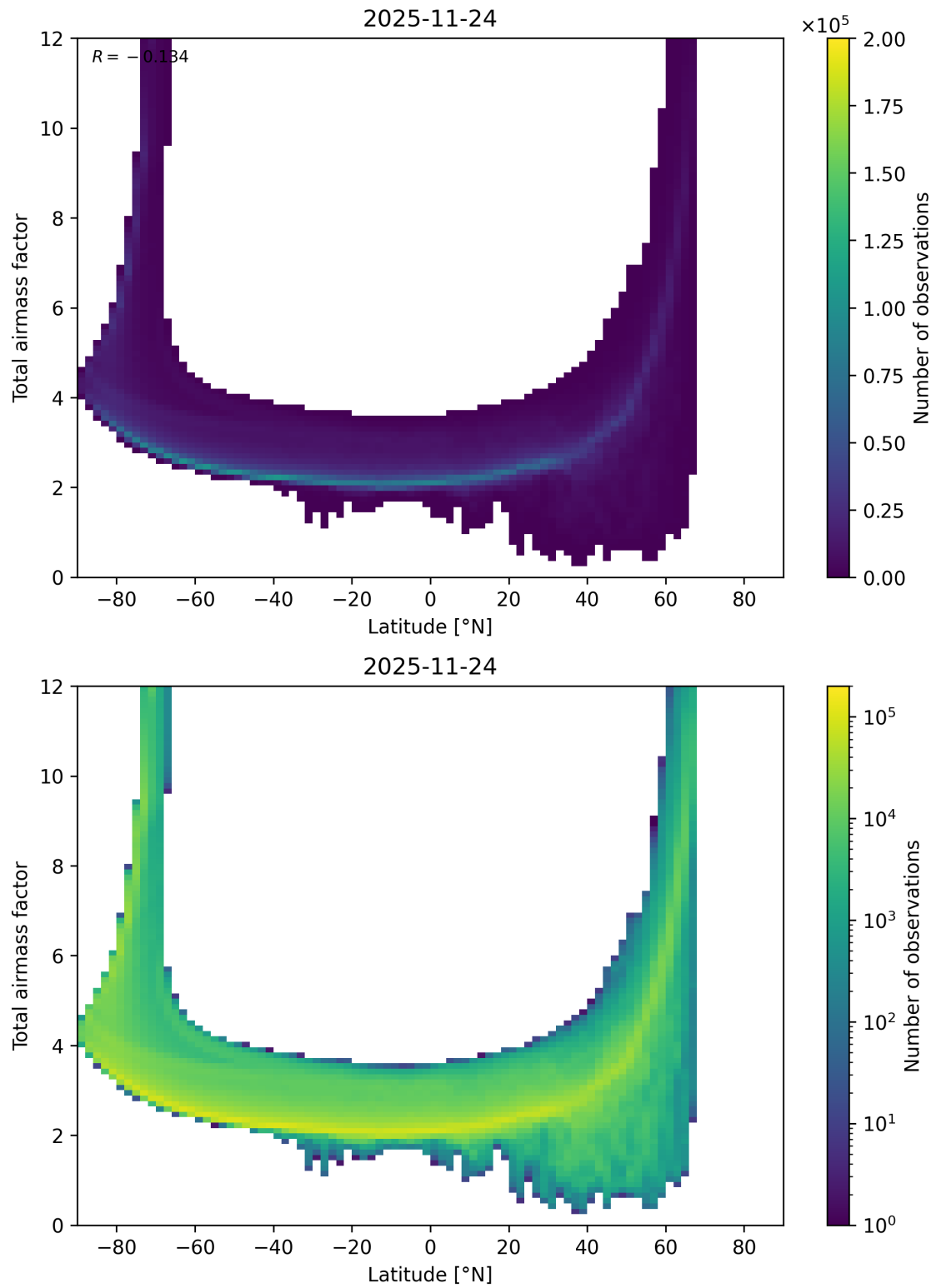
Figure 84: Scatter density plot of “Latitude” against “Total airmass factor” for 2025-11-23 to 2025-11-25.
