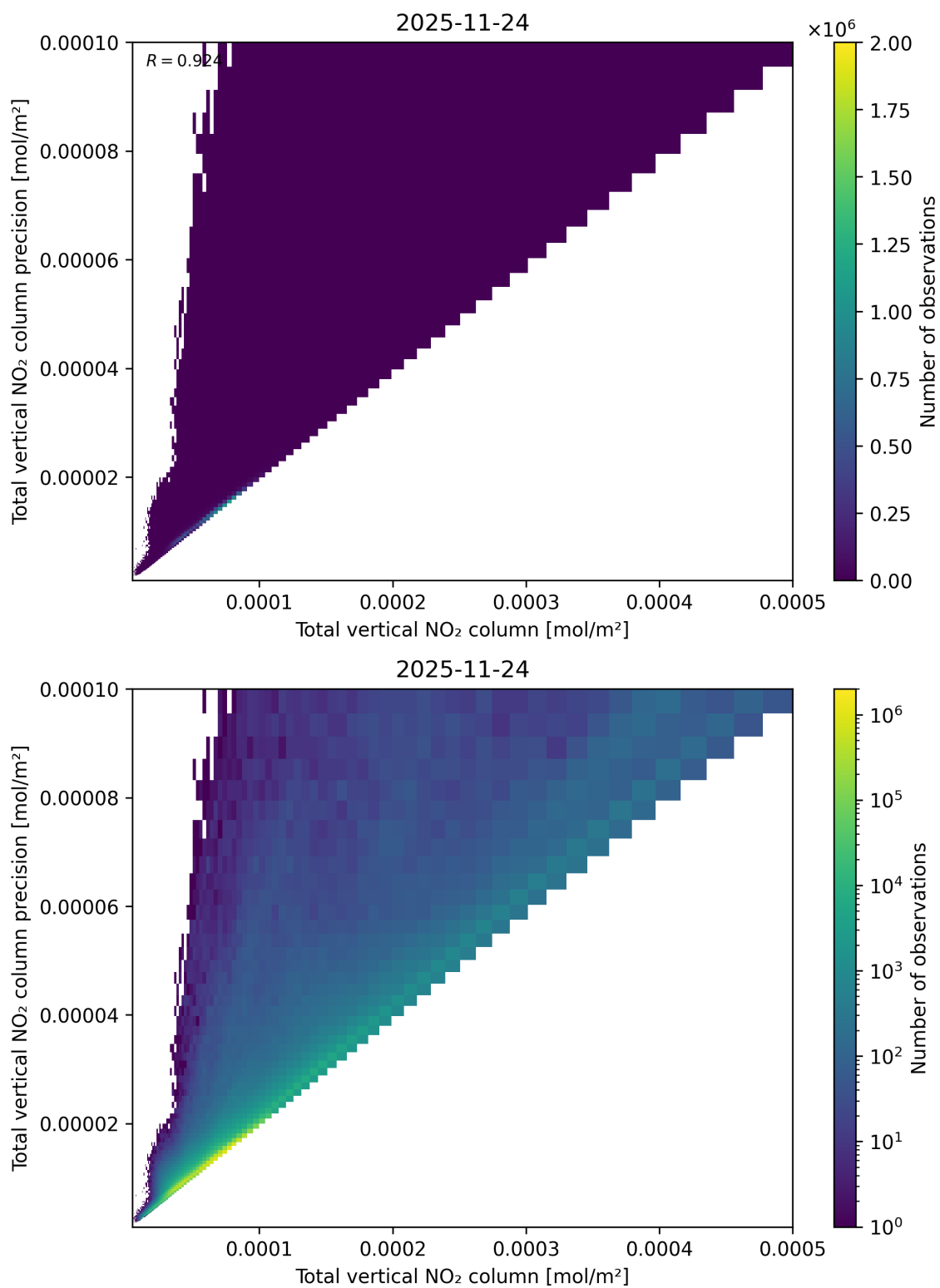
Figure 114: Scatter density plot of “Total vertical NO 2 column” against “Total vertical NO 2 column precision” for 2025-11-23 to 2025-11-25.
