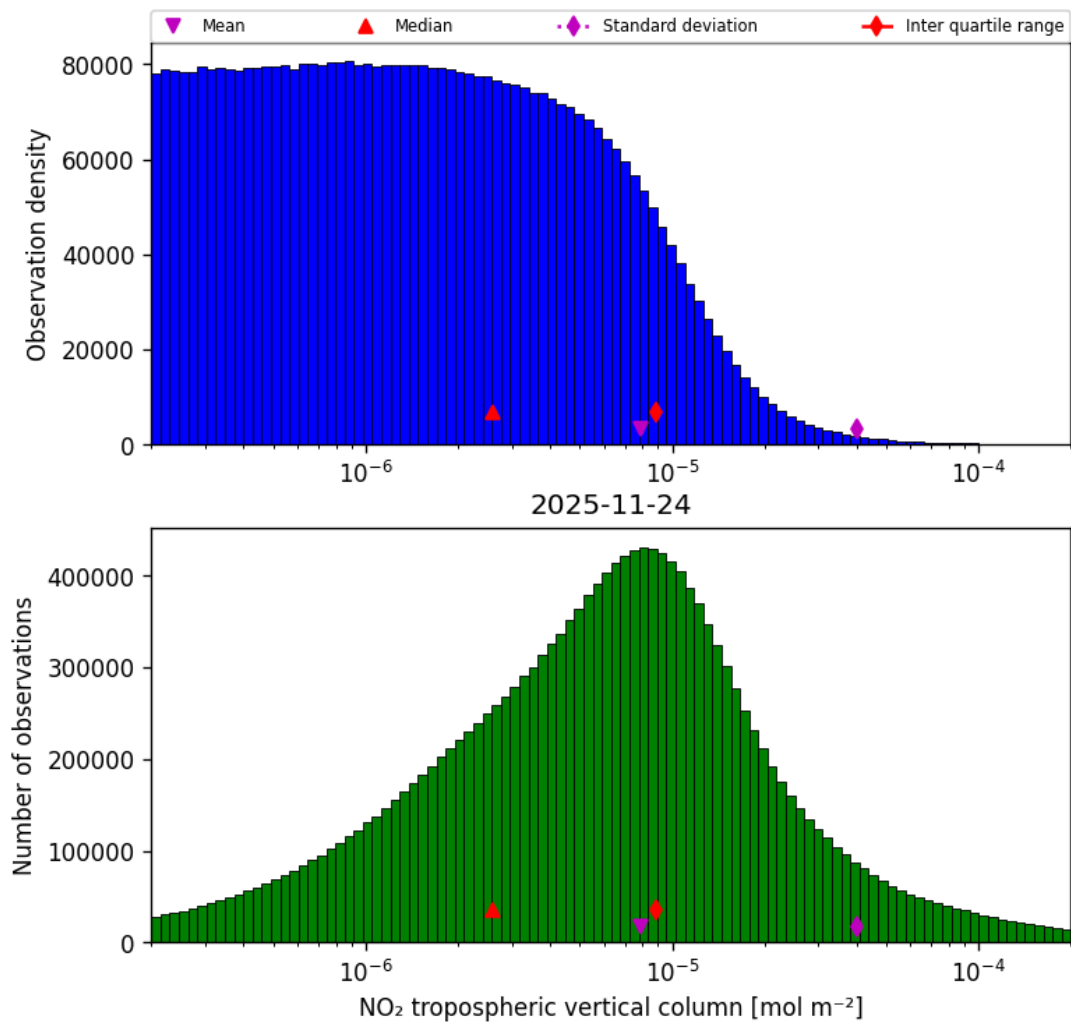
Figure 29: Histogram of “NO 2 tropospheric vertical column” for 2025-11-23 to 2025-11-25
