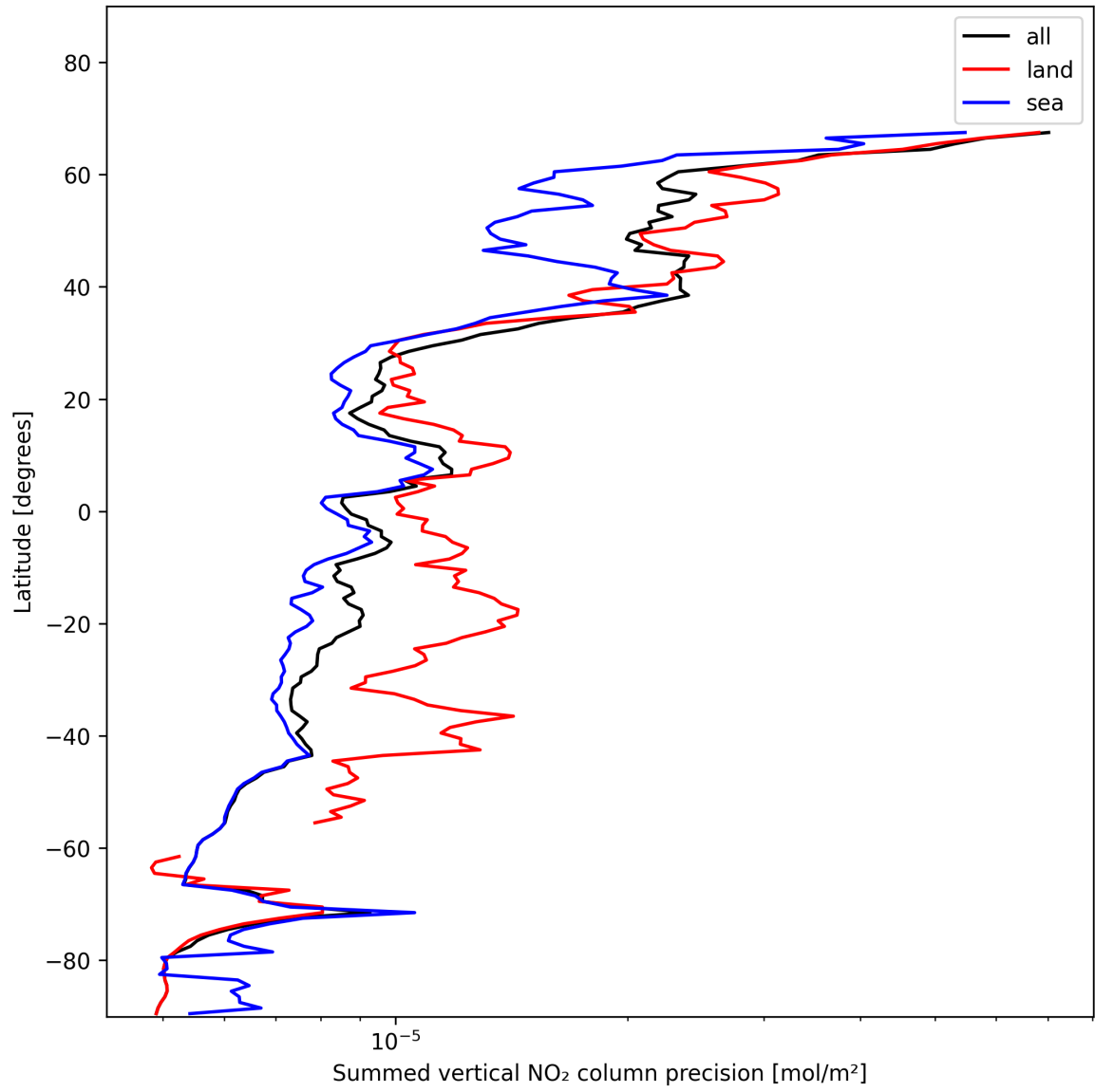
Figure 24: Zonal average of “Summed vertical NO 2 column precision” for 2025-11-23 to 2025-11-25.
