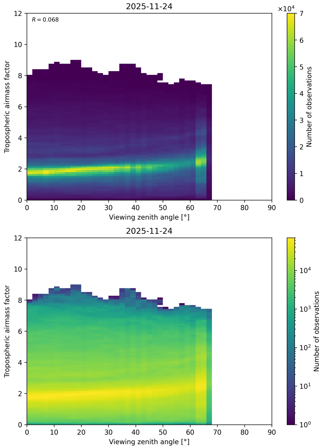
Figure 161: Scatter density plot of “Viewing zenith angle” against “Tropospheric airmass factor” for 2025-11-23 to 2025-11-25.
