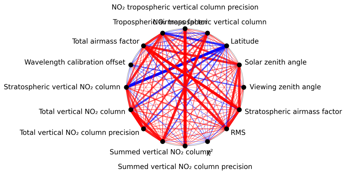
Figure 1: Map of correlation graph for 2025-11-23 to 2025-11-25.
