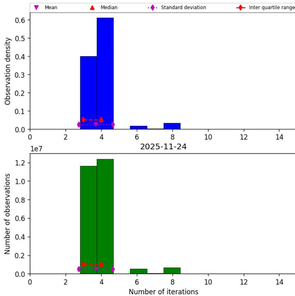
Figure 34: Histogram of “Number of iterations” for 2025-11-23 to 2025-11-25
