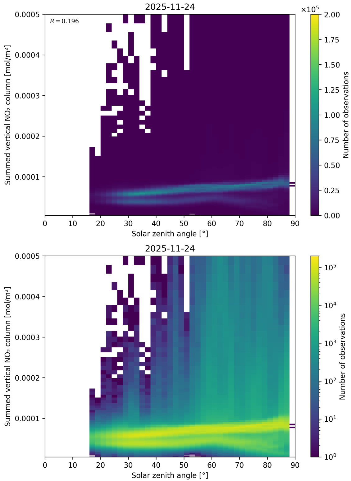
Figure 151: Scatter density plot of “Solar zenith angle” against “Summed vertical NO 2 column” for 2025-11-23 to 2025-11-25.
