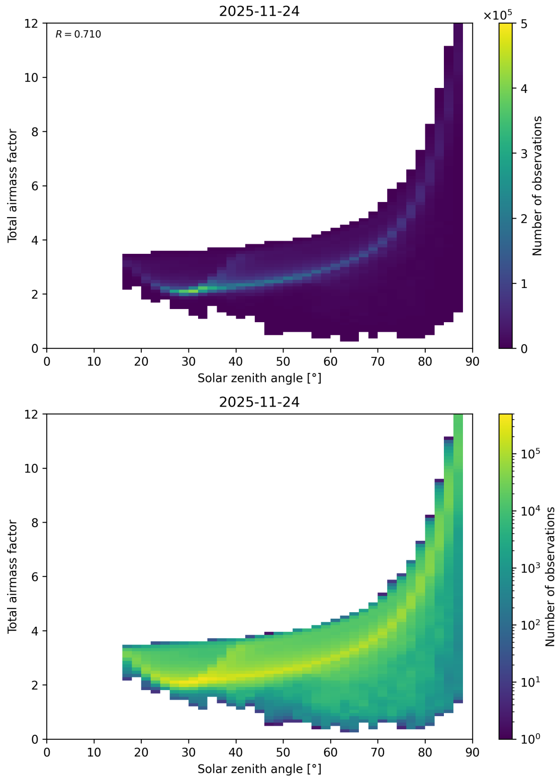
Figure 146: Scatter density plot of “Solar zenith angle” against “Total air mass factor” for 2025-11-23 to 2025-11-25.
