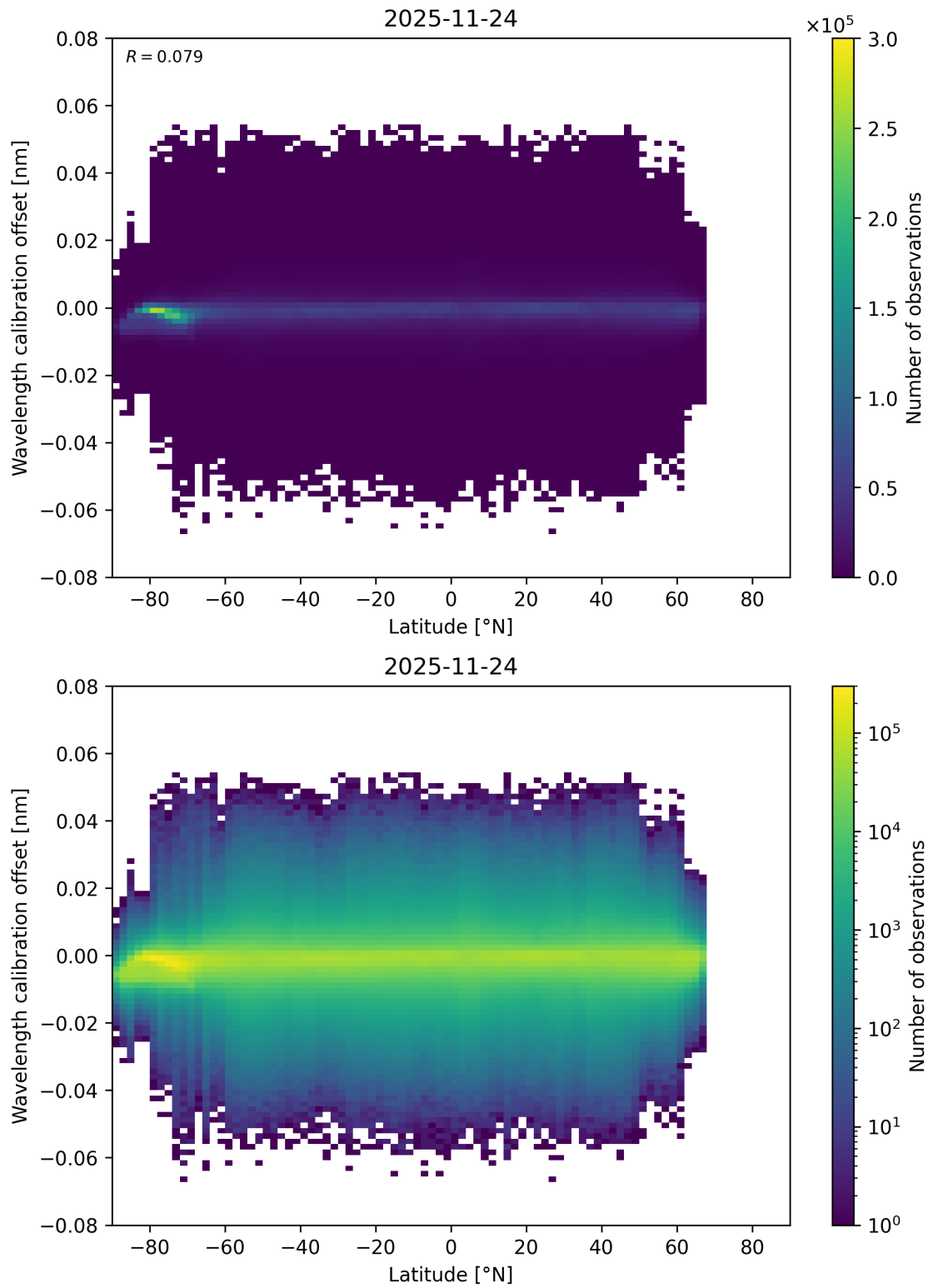
Figure 95: Scatter density plot of “Latitude” against “Wavelength calibration offset” for 2025-11-23 to 2025-11-25.
