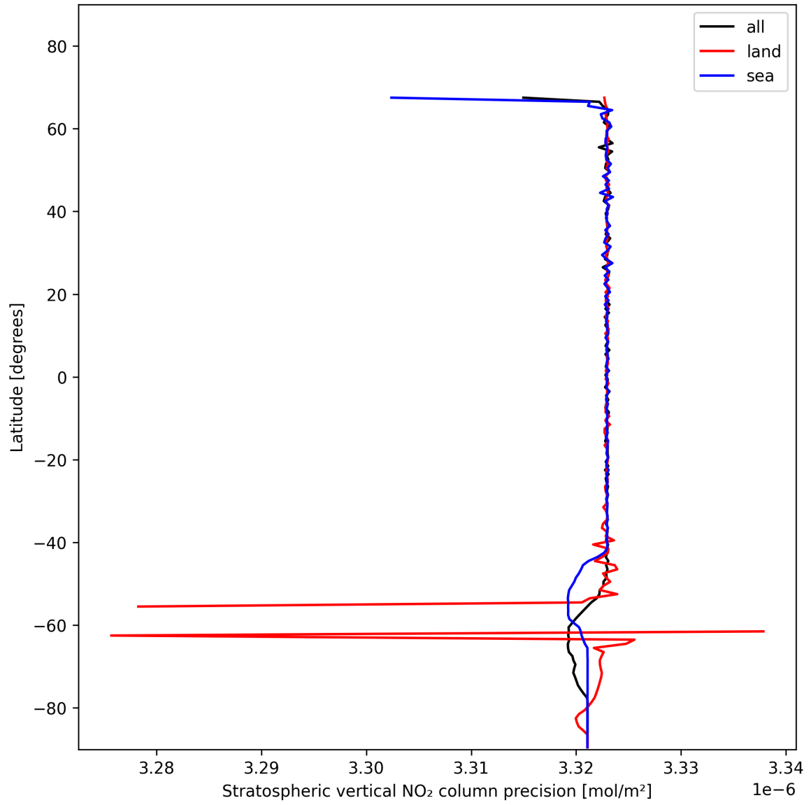
Figure 20: Zonal average of "Stratospheric vertical NO 2 column precision" for 2025-11-23 to 2025-11-25.
