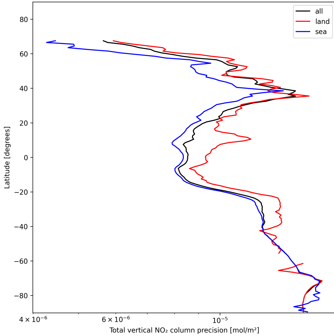
Figure 22: Zonal average of “Total vertical NO 2 column precision” for 2025-11-23 to 2025-11-25.
