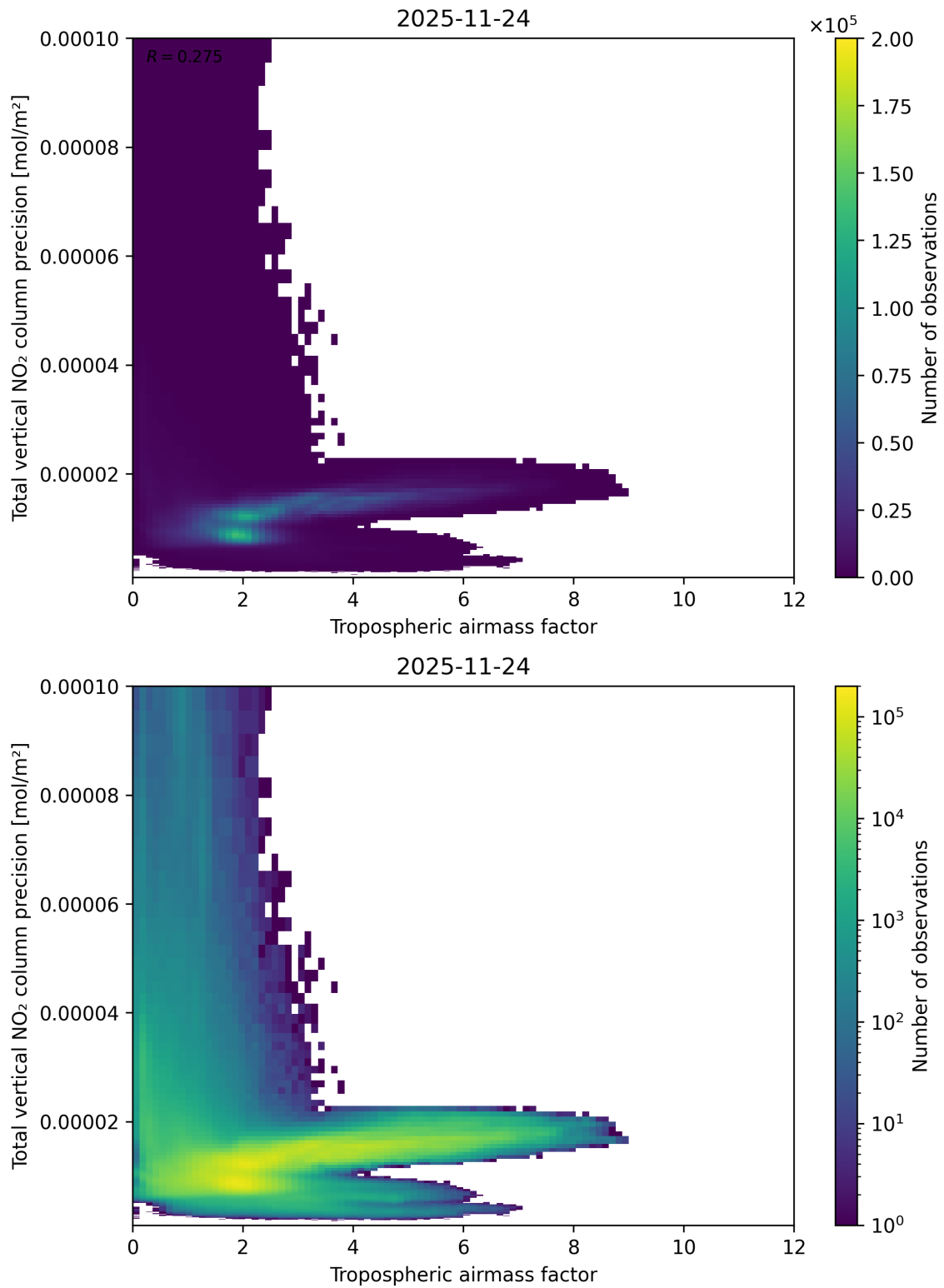
Figure 78: Scatter density plot of “Tropospheric air mass factor” against “Total vertical NO 2 column precision” for 2025-11-23 to 2025-11-25.
