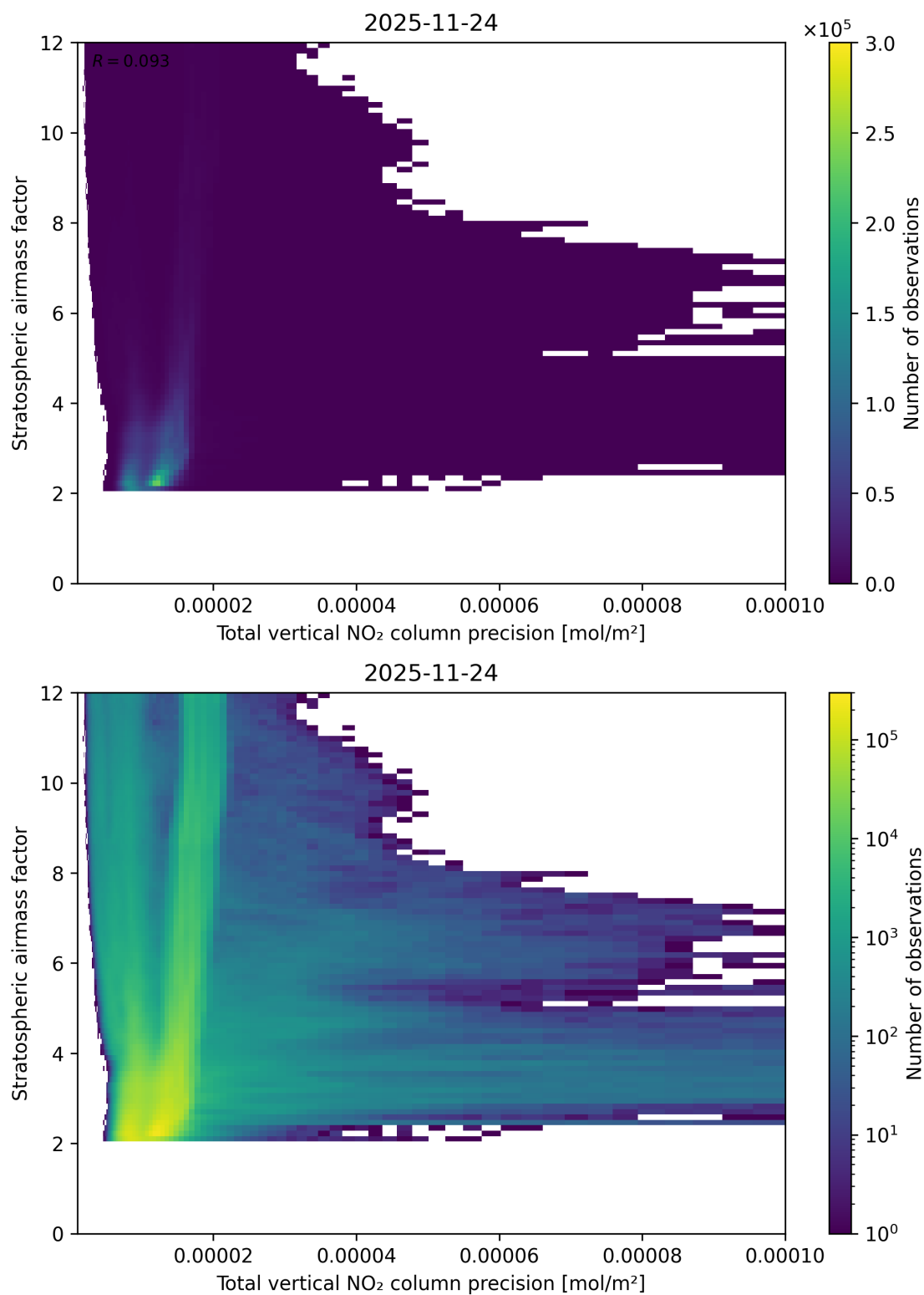
Figure 115: Scatter density plot of “Total vertical NO 2 column precision” against “Stratospheric air mass factor” for 2025-11-23 to 2025-11-25.
