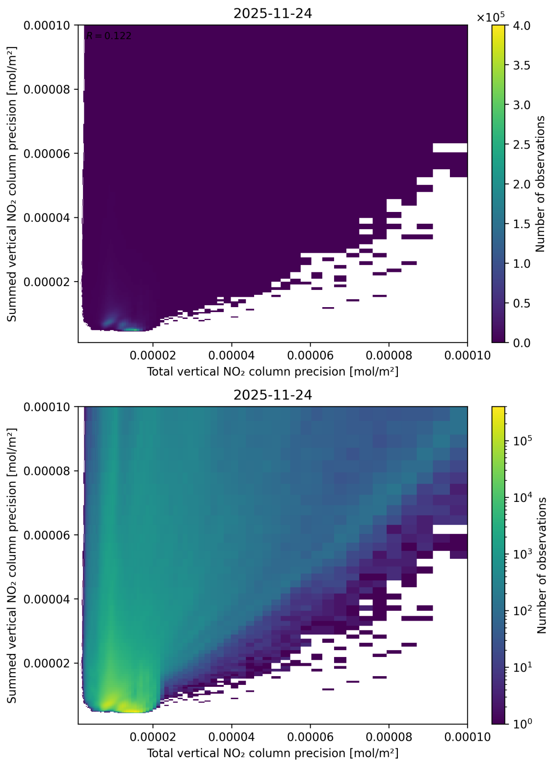
Figure 118: Scatter density plot of “Total vertical NO 2 column precision” against “Summed vertical NO 2 column precision” for 2025-11-23 to 2025-11-25.
