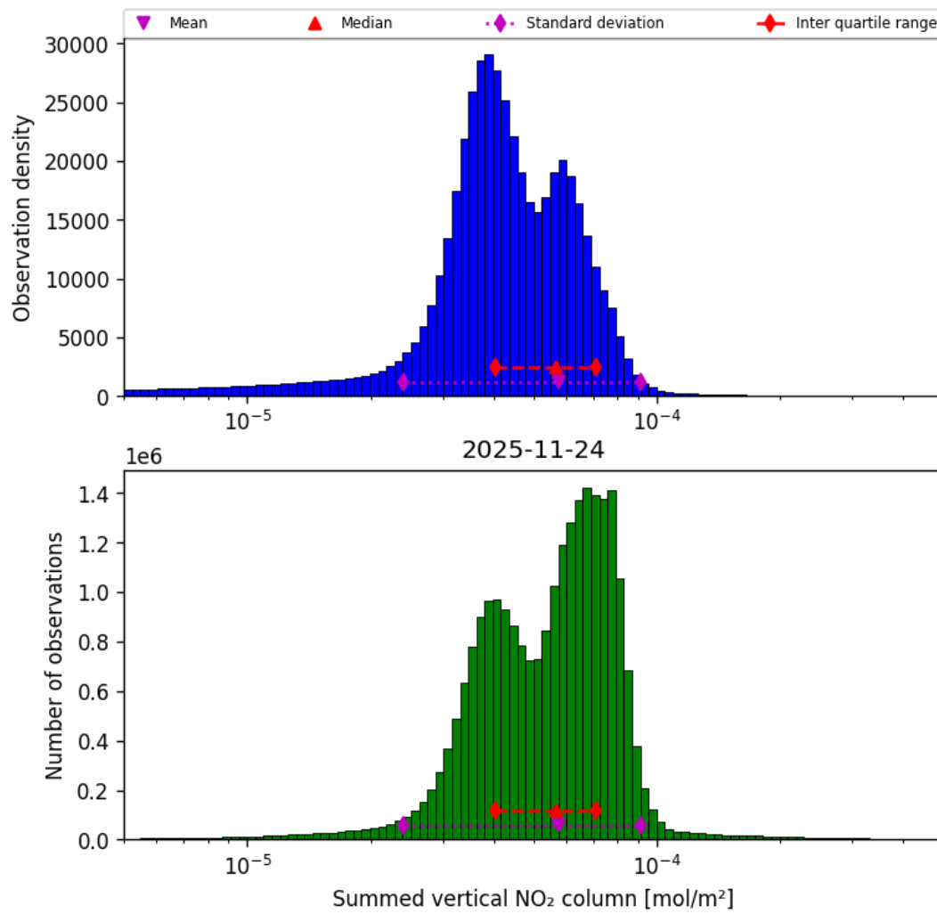
Figure 40: Histogram of “Summed vertical NO 2 column” for 2025-11-23 to 2025-11-25
