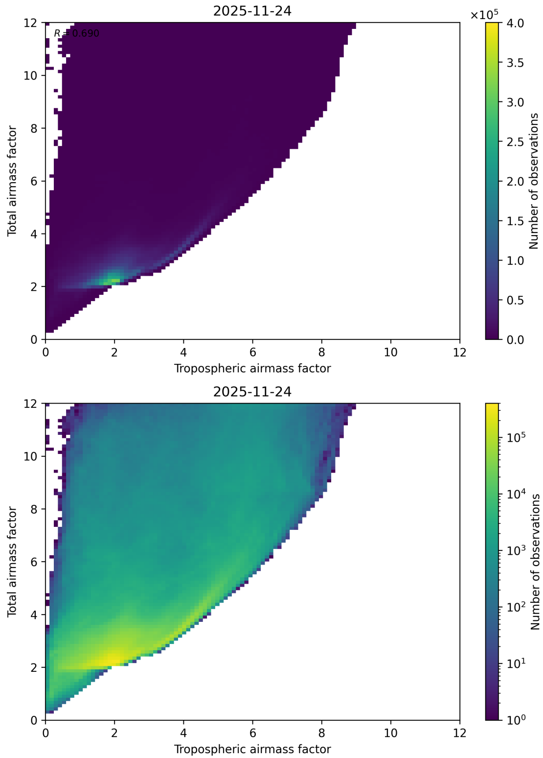
Figure 72: Scatter density plot of “Tropospheric airmass factor” against “Total airmass factor” for 2025-11-23 to 2025-11-25.
