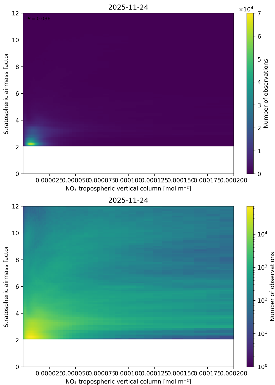
Figure 121: Scatter density plot of “NO 2 tropospheric vertical column” against “Stratospheric airmass factor” for 2025-11-23 to 2025-11-25.
