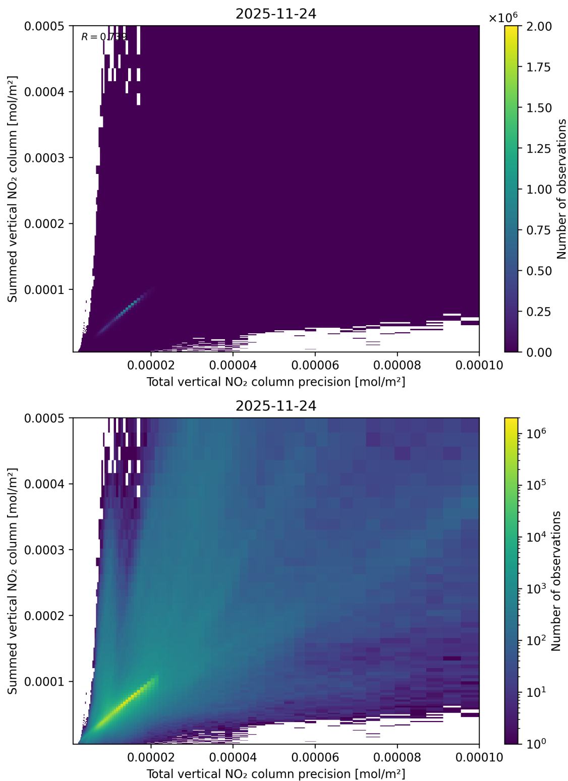
Figure 117: Scatter density plot of “Total vertical NO 2 column precision” against “Summed vertical NO 2 column” for 2025-11-23 to 2025-11-25.
