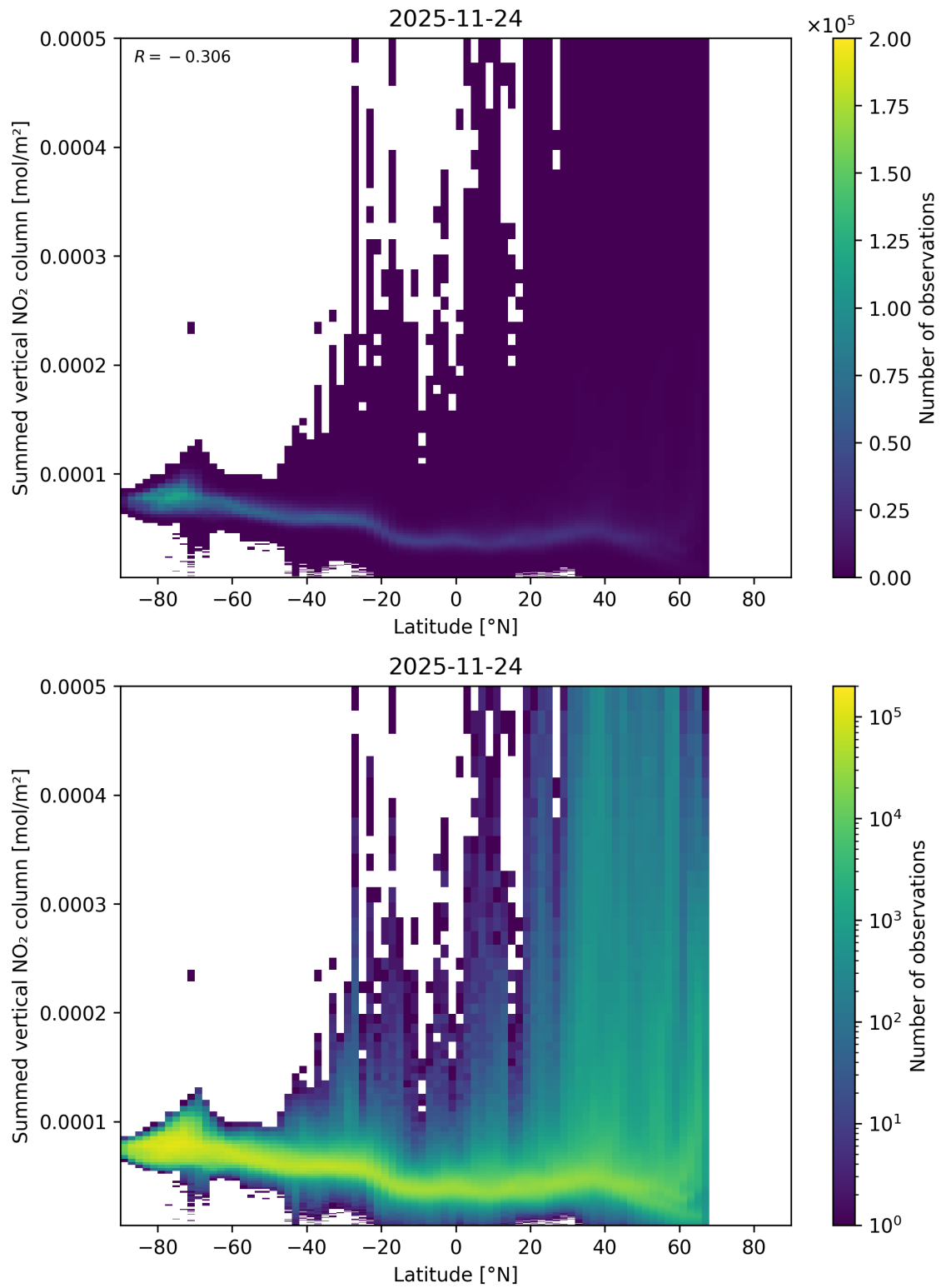
Figure 88: Scatter density plot of “Latitude” against “Summed vertical NO 2 column” for 2025-11-23 to 2025-11-25.
