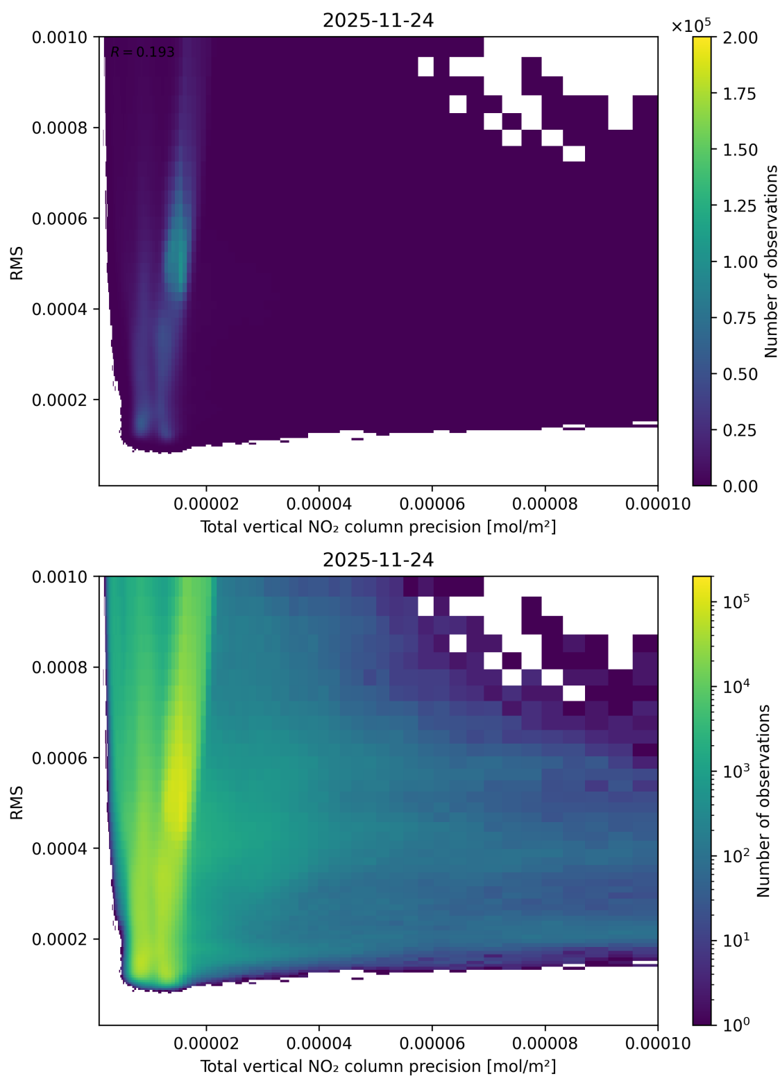
Figure 119: Scatter density plot of “Total vertical NO 2 column precision” against “RMS” for 2025-11-23 to 2025-11-25.
