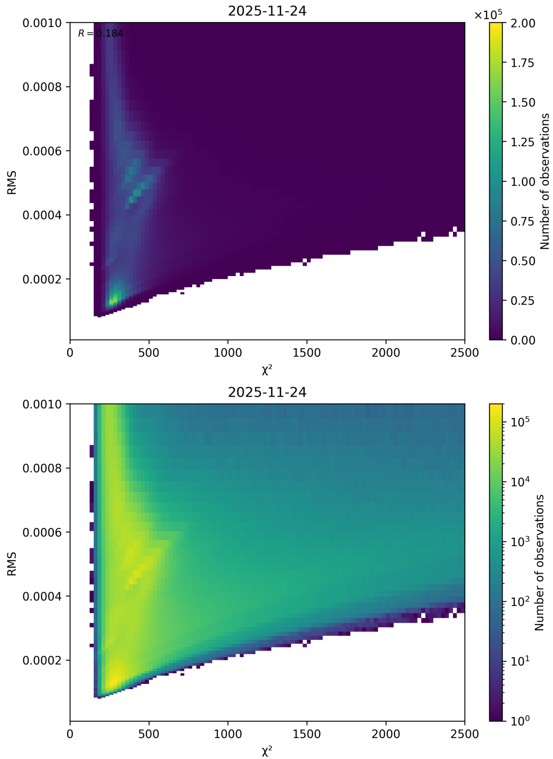
Figure 82: Scatter density plot of “ \chi^2 ” against “RMS” for 2025-11-23 to 2025-11-25.
