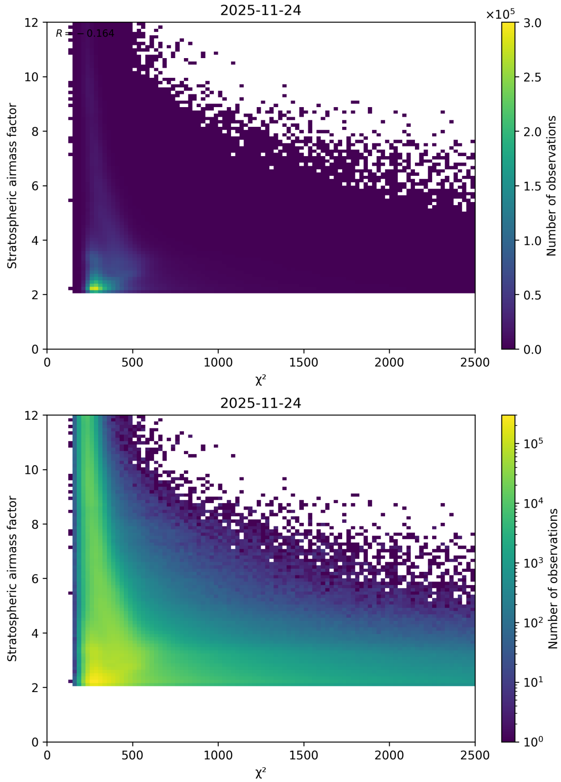
Figure 81: Scatter density plot of “ \chi^2 ” against “Stratospheric airmass factor” for 2025-11-23 to 2025-11-25.
