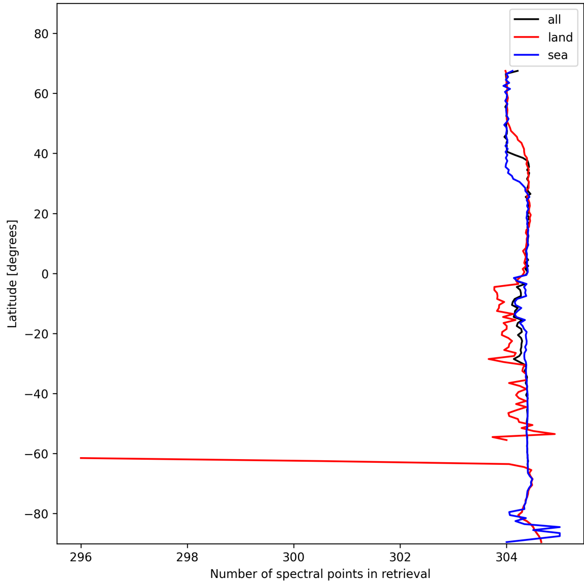
Figure 16: Zonal average of “Number of spectral points in retrieval” for 2025-11-23 to 2025-11-25.
