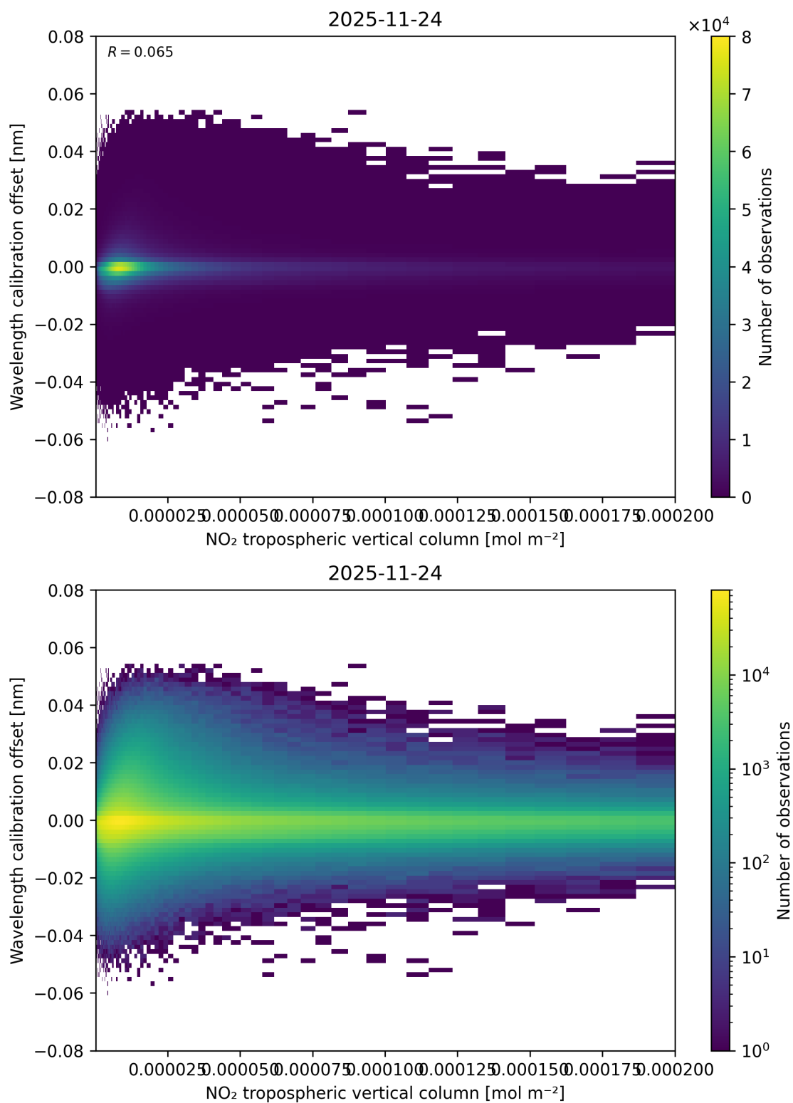
Figure 143: Scatter density plot of “NO 2 tropospheric vertical column” against “Wavelength calibration offset” for 2025-11-23 to 2025-11-25.
