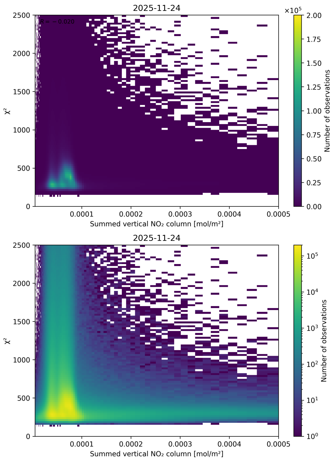
Figure 104: Scatter density plot of “Summed vertical NO 2 column” against “ \chi^2 ” for 2025-11-23 to 2025-11-25.
