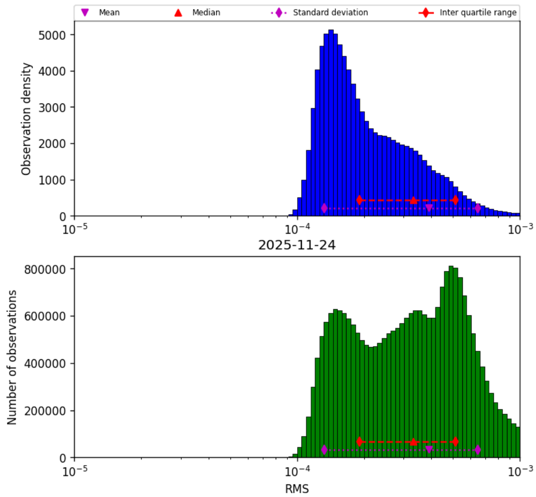
Figure 43: Histogram of “RMS” for 2025-11-23 to 2025-11-25
