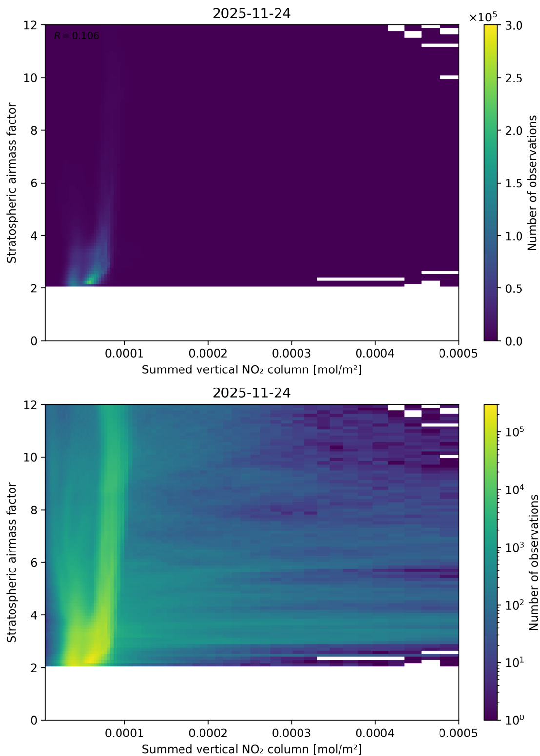
Figure 103: Scatter density plot of “Summed vertical NO 2 column” against “Stratospheric airmass factor” for 2025-11-23 to 2025-11-25.
