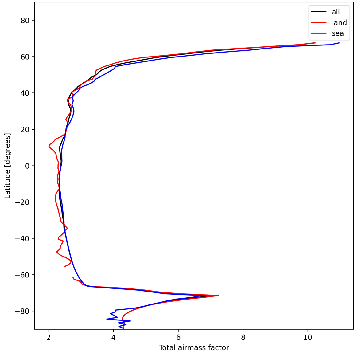
Figure 15: Zonal average of “Total airmass factor” for 2025-11-23 to 2025-11-25.
