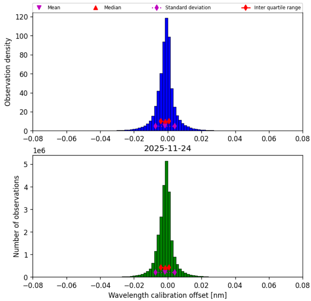
Figure 35: Histogram of “Wavelength calibration offset” for 2025-11-23 to 2025-11-25
