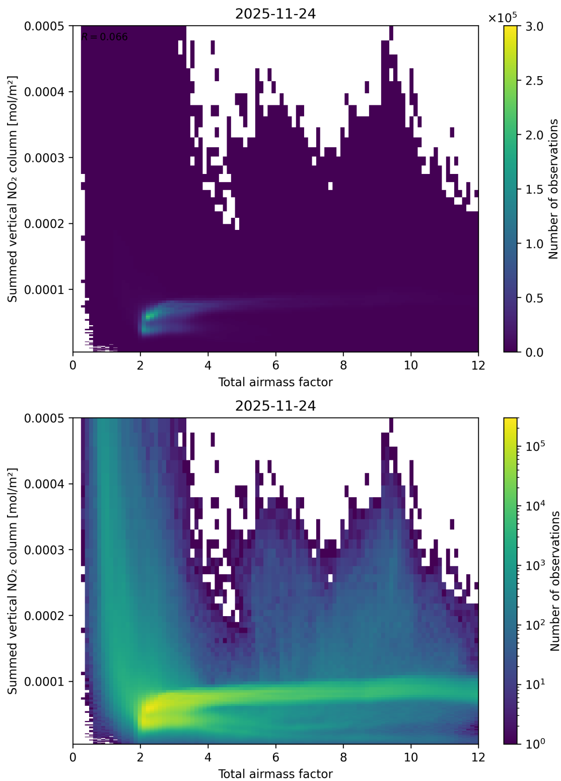
Figure 65: Scatter density plot of “Total airmass factor” against “Summed vertical NO 2 column” for 2025-11-23 to 2025-11-25.
