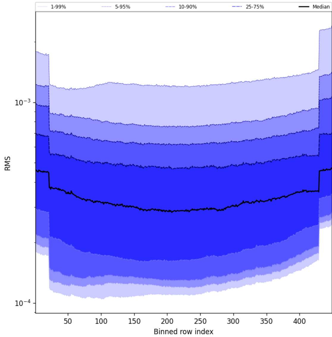
Figure 60: Along track statistics of “RMS” for 2025-11-23 to 2025-11-25
