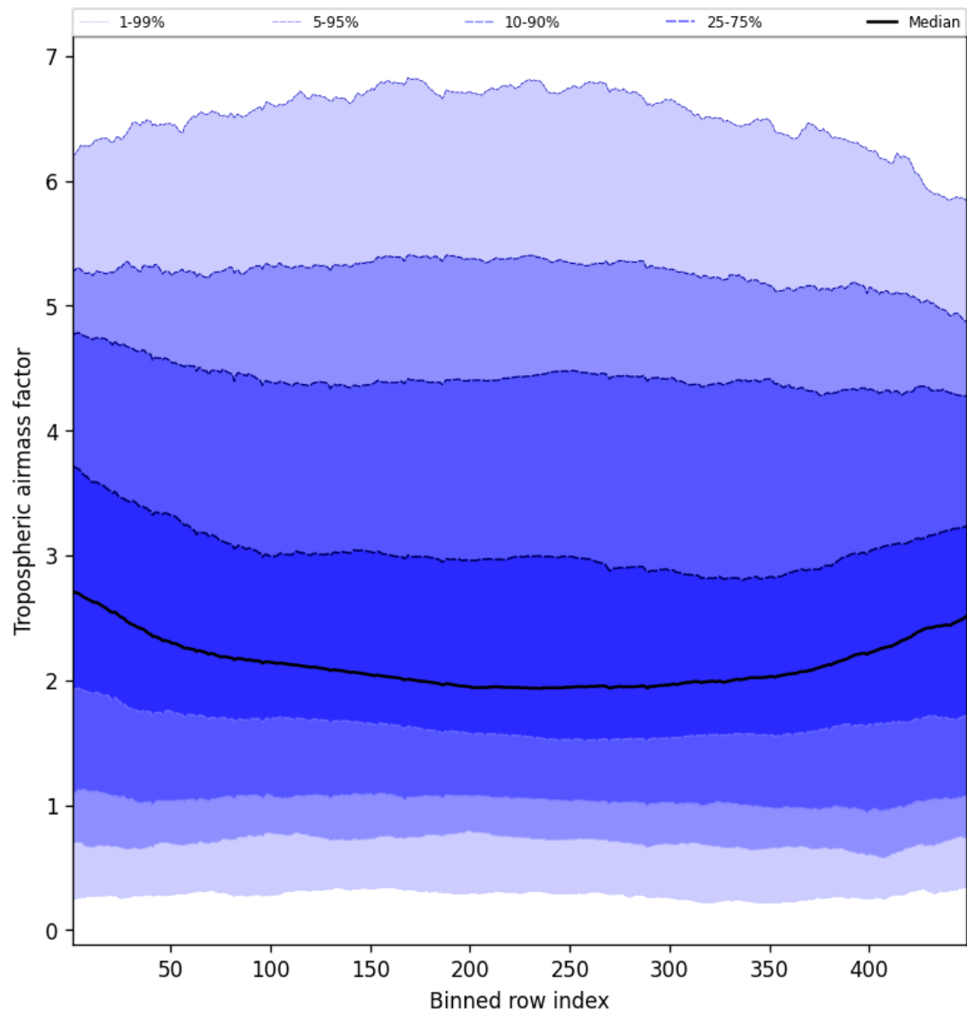
Figure 48: Along track statistics of “Tropospheric airmass factor” for 2025-11-23 to 2025-11-25
