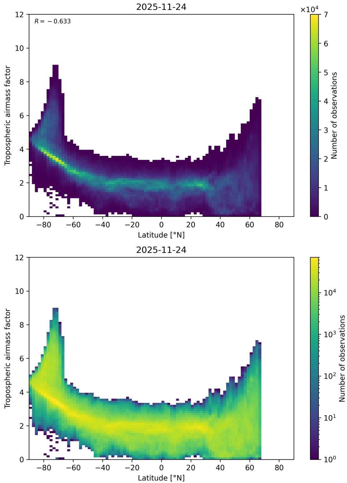
Figure 85: Scatter density plot of “Latitude” against “Tropospheric air mass factor” for 2025-11-23 to 2025-11-25.
