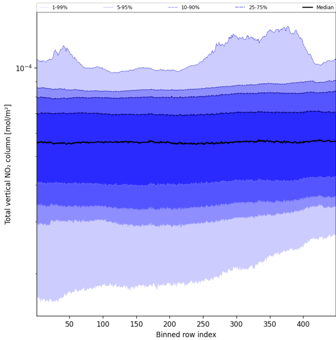
Figure 55: Along track statistics of “Total vertical NO 2 column” for 2025-11-23 to 2025-11-25
