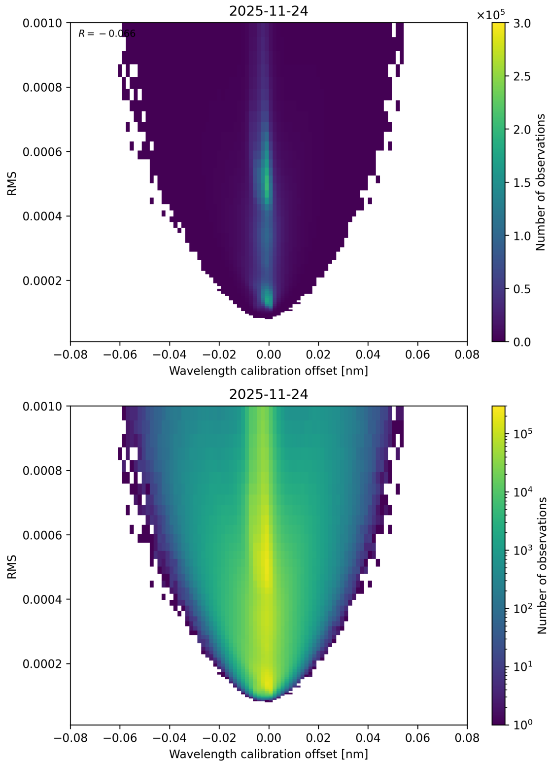
Figure 181: Scatter density plot of “Wavelength calibration offset” against “RMS” for 2025-11-23 to 2025-11-25.
