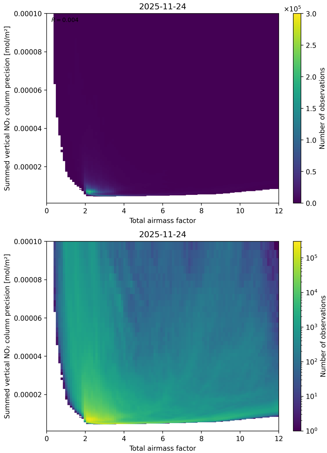
Figure 66: Scatter density plot of “Total airmass factor” against “Summed vertical NO 2 column precision” for 2025-11-23 to 2025-11-25.
