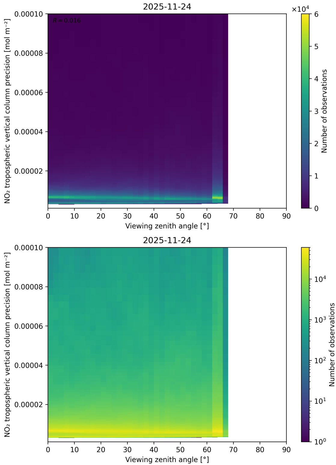
Figure 170: Scatter density plot of “Viewing zenith angle” against “NO 2 tropospheric vertical column precision” for 2025-11-23 to 2025-11-25.
