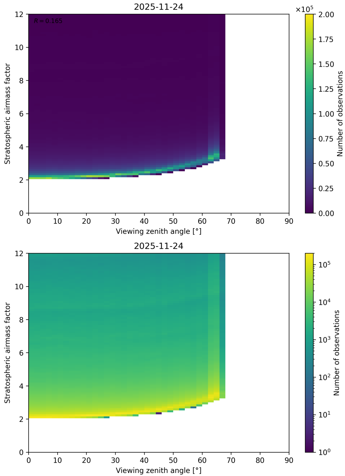
Figure 159: Scatter density plot of “Viewing zenith angle” against “Stratospheric airmass factor” for 2025-11-23 to 2025-11-25.
