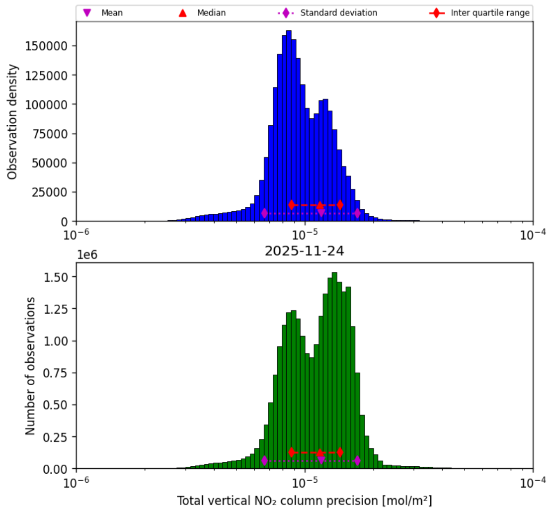
Figure 39: Histogram of “Total vertical NO 2 column precision” for 2025-11-23 to 2025-11-25
