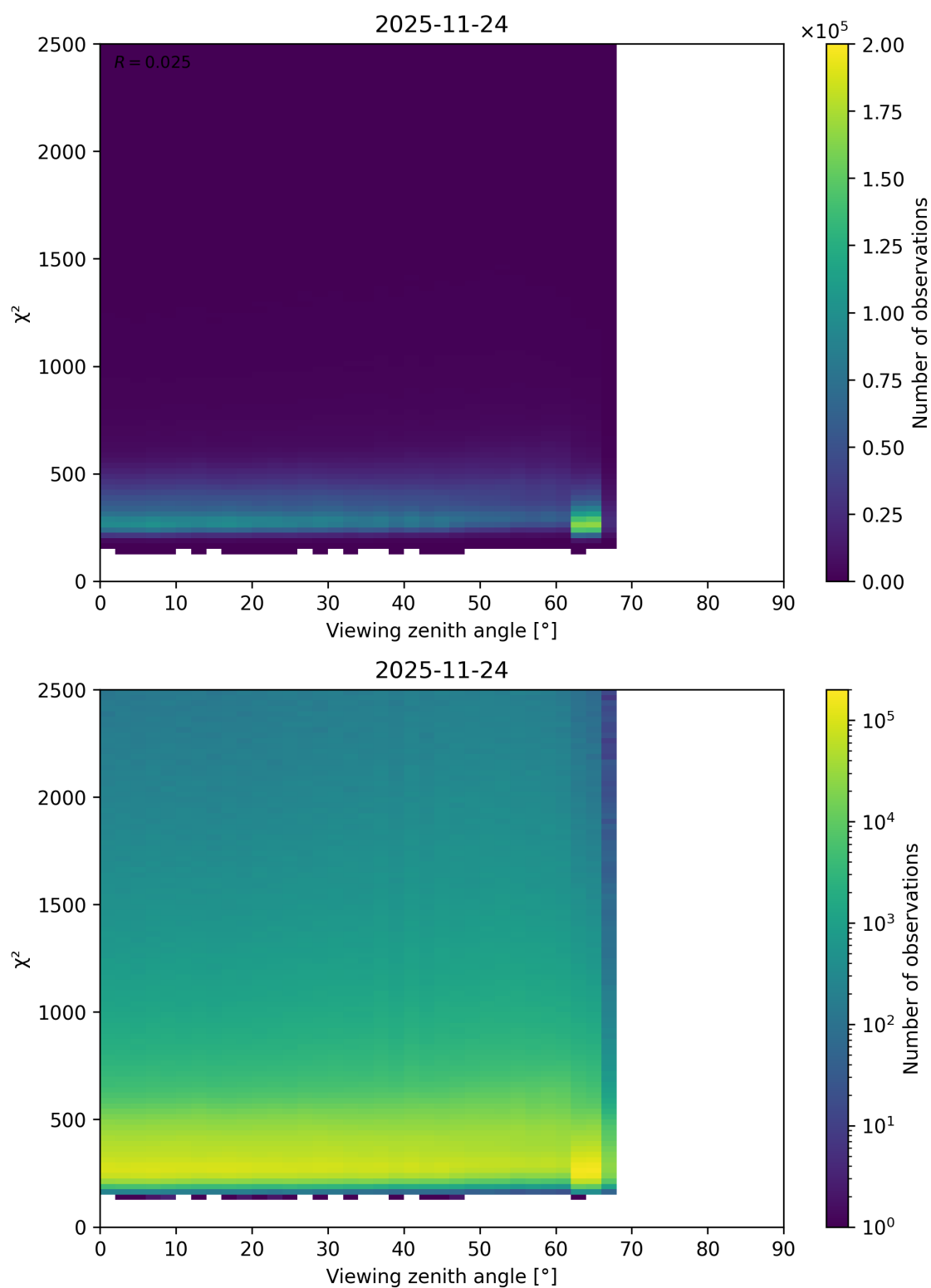
Figure 162: Scatter density plot of “Viewing zenith angle” against “ \chi^2 ” for 2025-11-23 to 2025-11-25.
