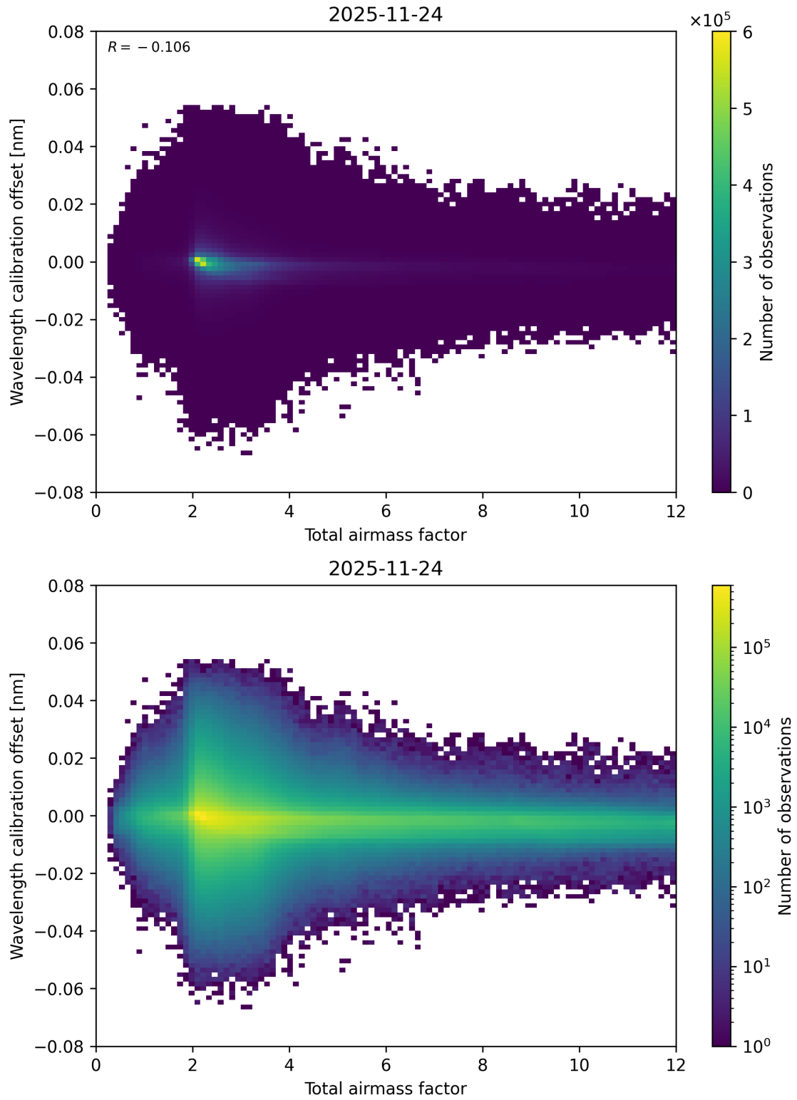
Figure 70: Scatter density plot of “Total airmass factor” against “Wavelength calibration offset” for 2025-11-23 to 2025-11-25.
