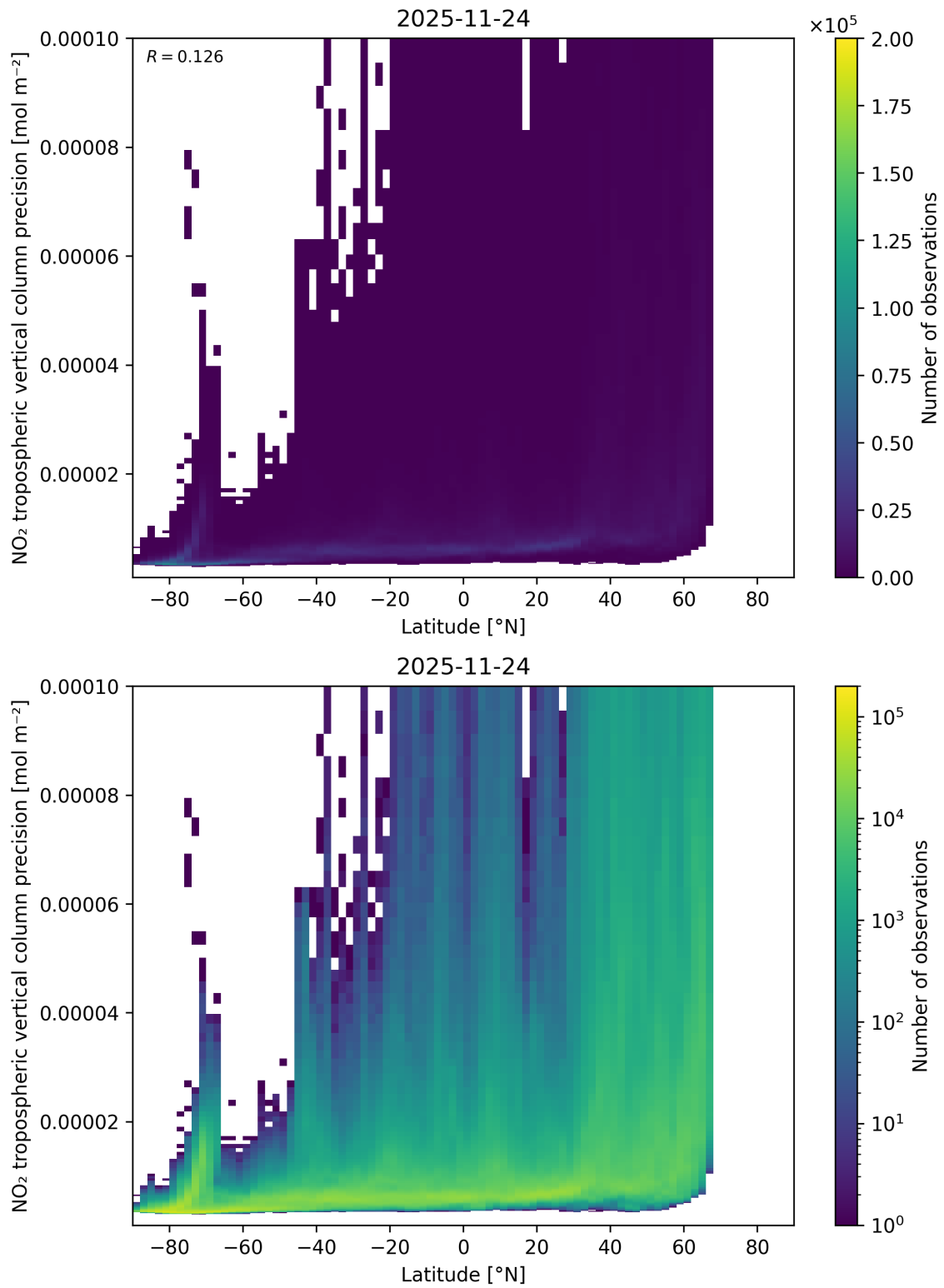
Figure 93: Scatter density plot of “Latitude” against “NO 2 tropospheric vertical column precision” for 2025-11-23 to 2025-11-25.
