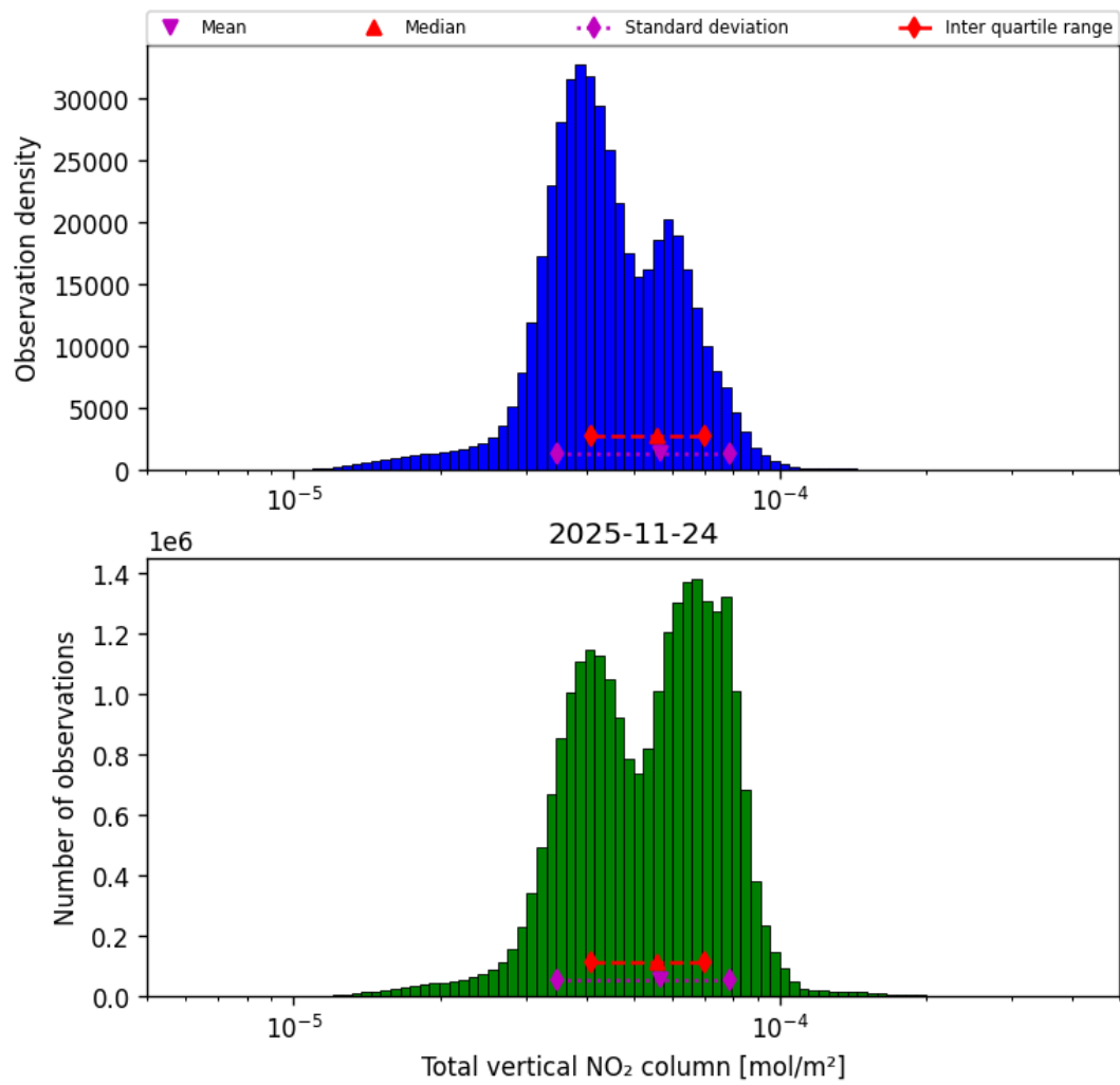
Figure 38: Histogram of “Total vertical NO 2 column” for 2025-11-23 to 2025-11-25
