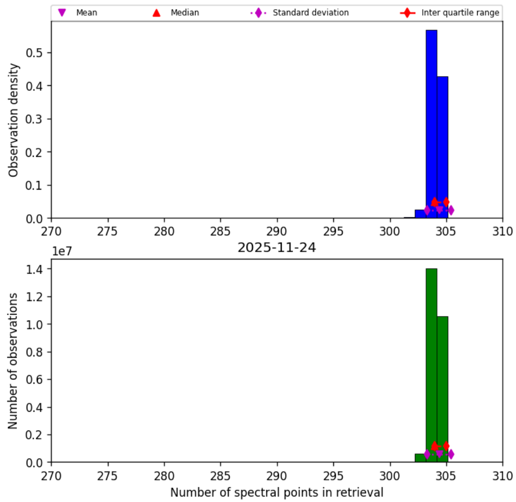
Figure 33: Histogram of “Number of spectral points in retrieval” for 2025-11-23 to 2025-11-25
