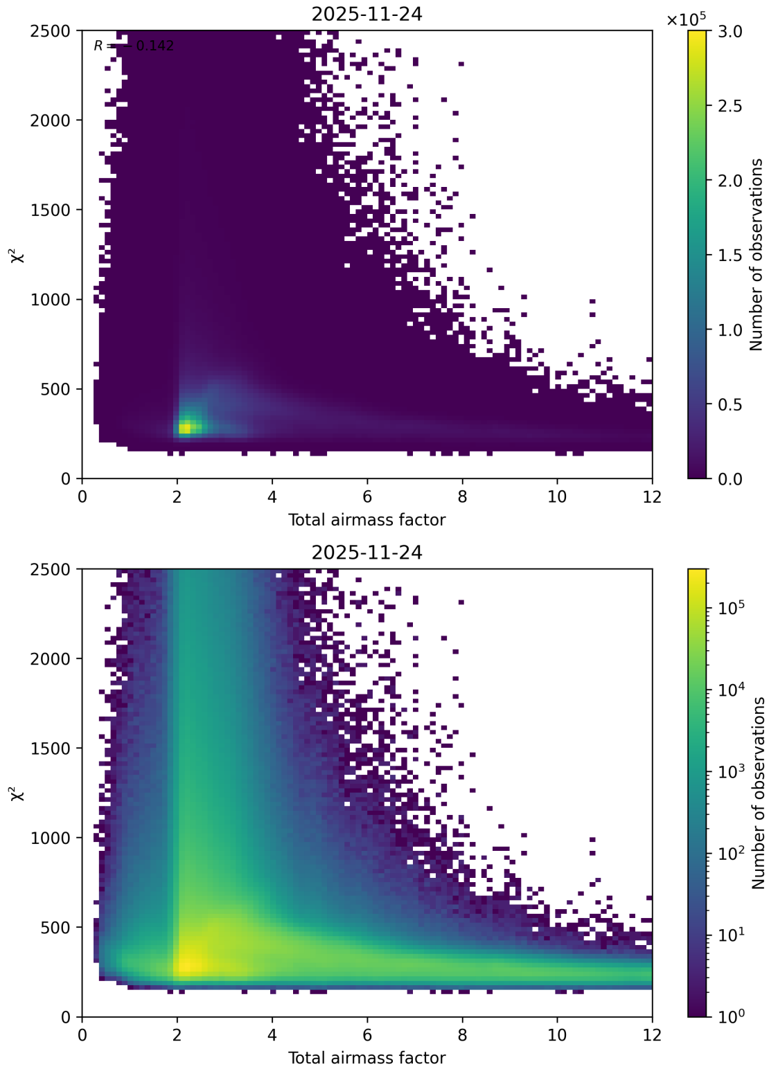
Figure 63: Scatter density plot of “Total airmass factor” against “ \chi^2 ” for 2025-11-23 to 2025-11-25.
