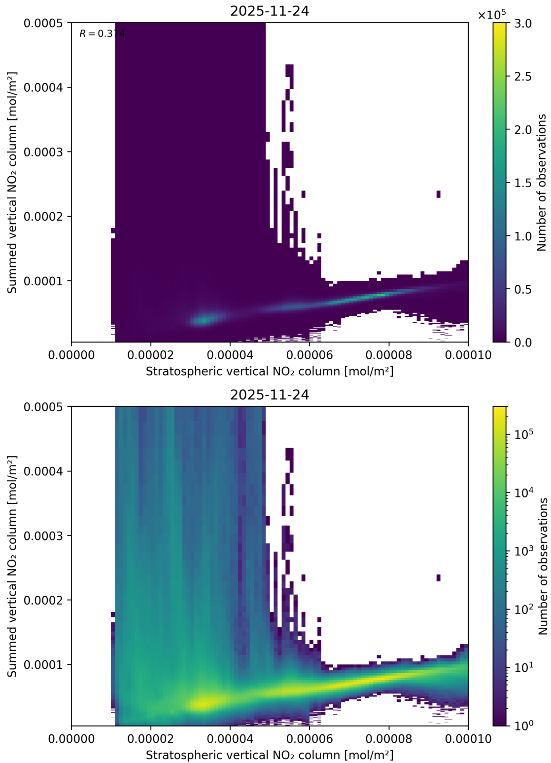
Figure 98: Scatter density plot of “Stratospheric vertical NO 2 column” against “Summed vertical NO 2 column” for 2025-11-23 to 2025-11-25.
