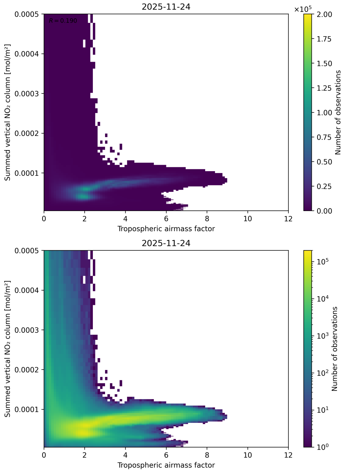
Figure 75: Scatter density plot of “Tropospheric air mass factor” against “Summed vertical NO 2 column” for 2025-11-23 to 2025-11-25.
