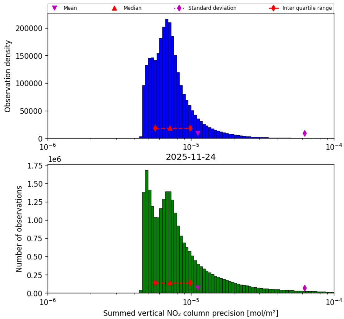
Figure 41: Histogram of "Summed vertical NO 2 column precision" for 2025-11-23 to 2025-11-25
