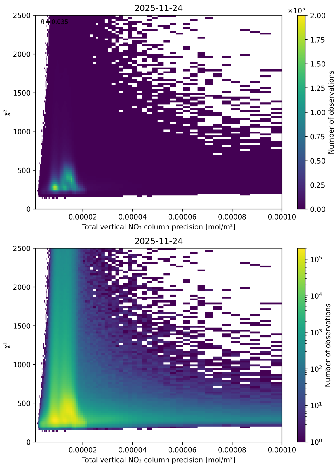
Figure 116: Scatter density plot of “Total vertical NO 2 column precision” against “ \chi^2 ” for 2025-11-23 to 2025-11-25.
