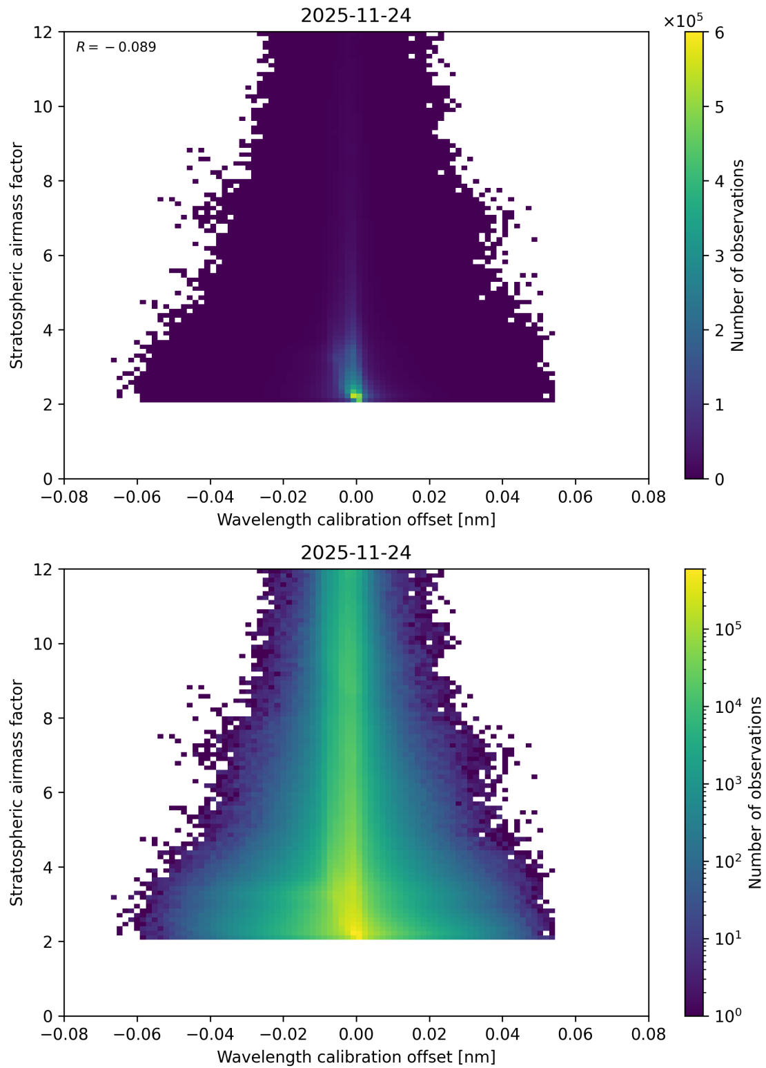
Figure 174: Scatter density plot of “Wavelength calibration offset” against “Stratospheric airmass factor” for 2025-11-23 to 2025-11-25.
