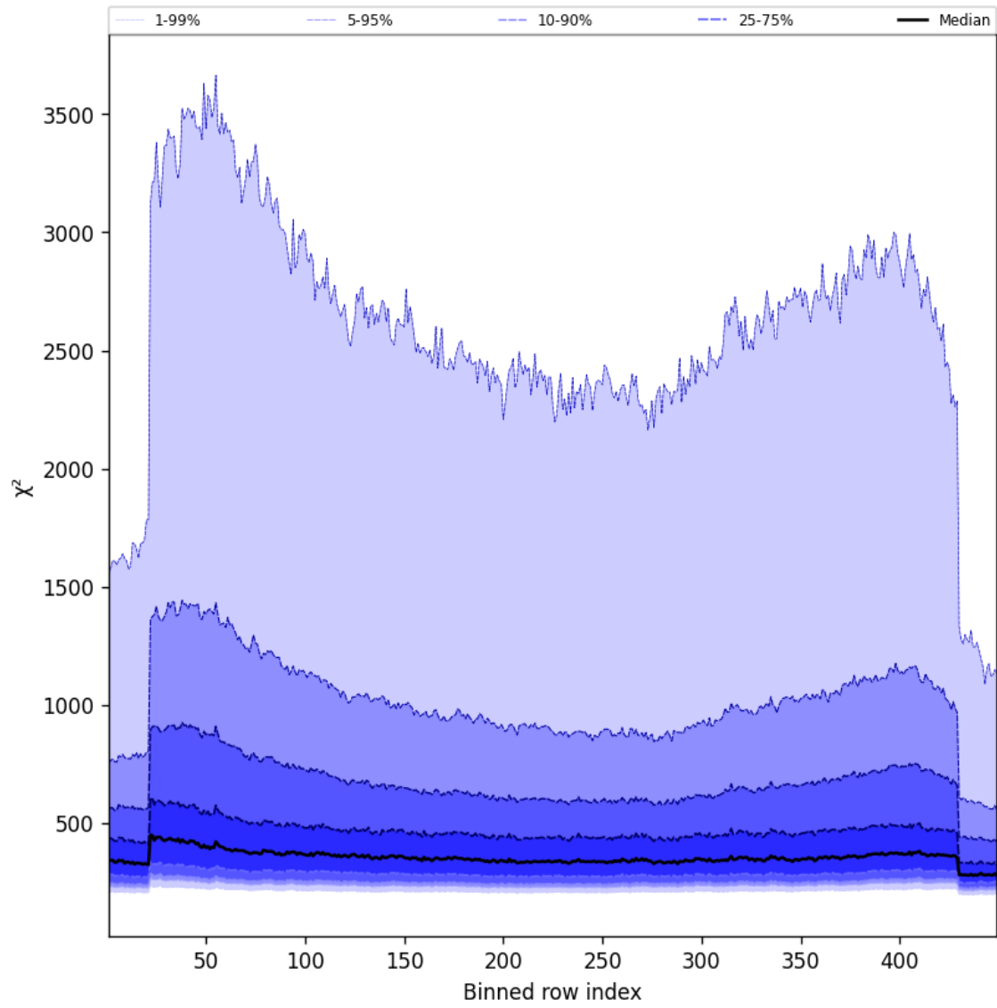
Figure 59: Along track statistics of “ \chi^2 ” for 2025-11-23 to 2025-11-25
