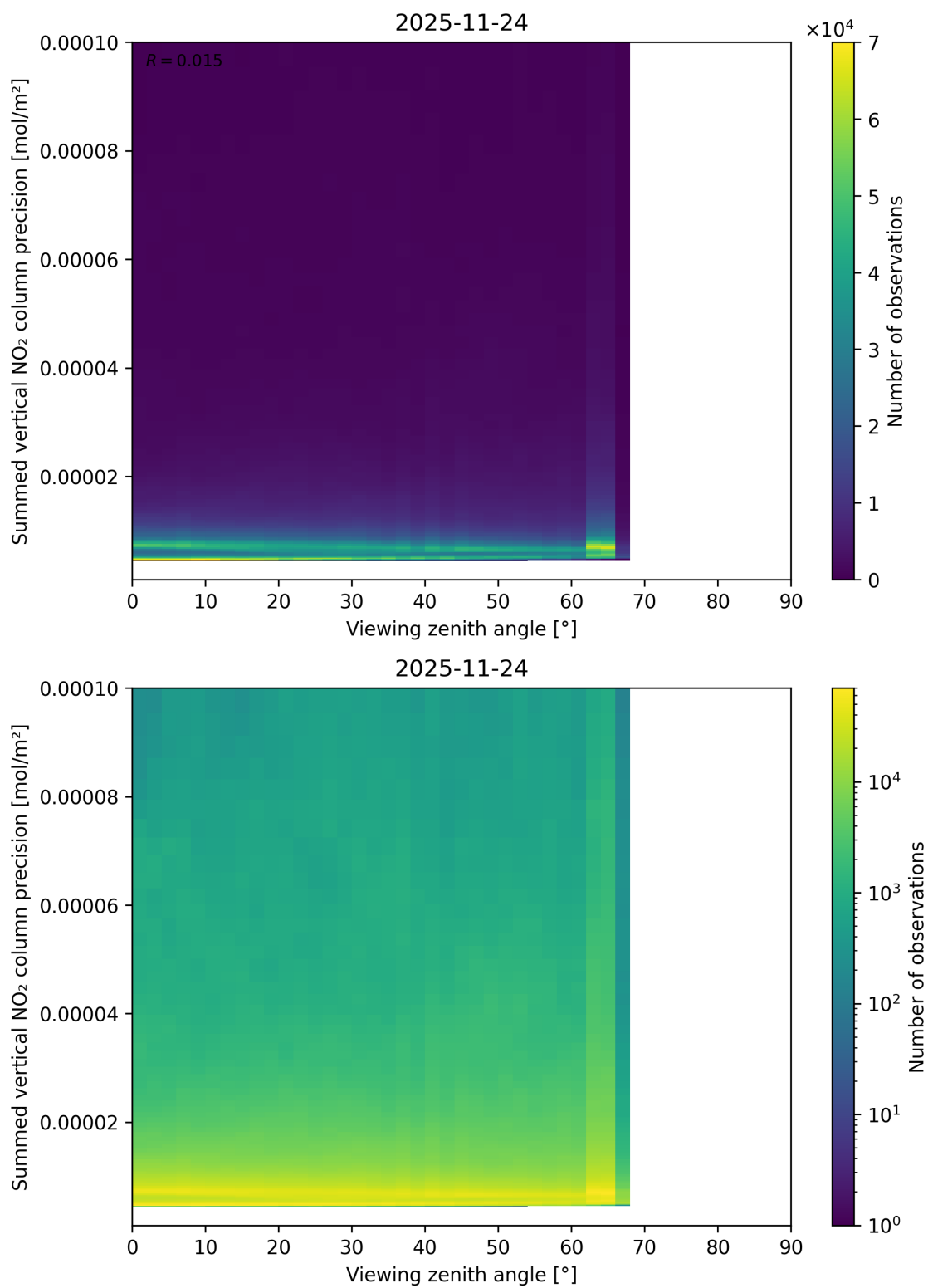
Figure 166: Scatter density plot of “Viewing zenith angle” against “Summed vertical NO 2 column precision” for 2025-11-23 to 2025-11-25.
