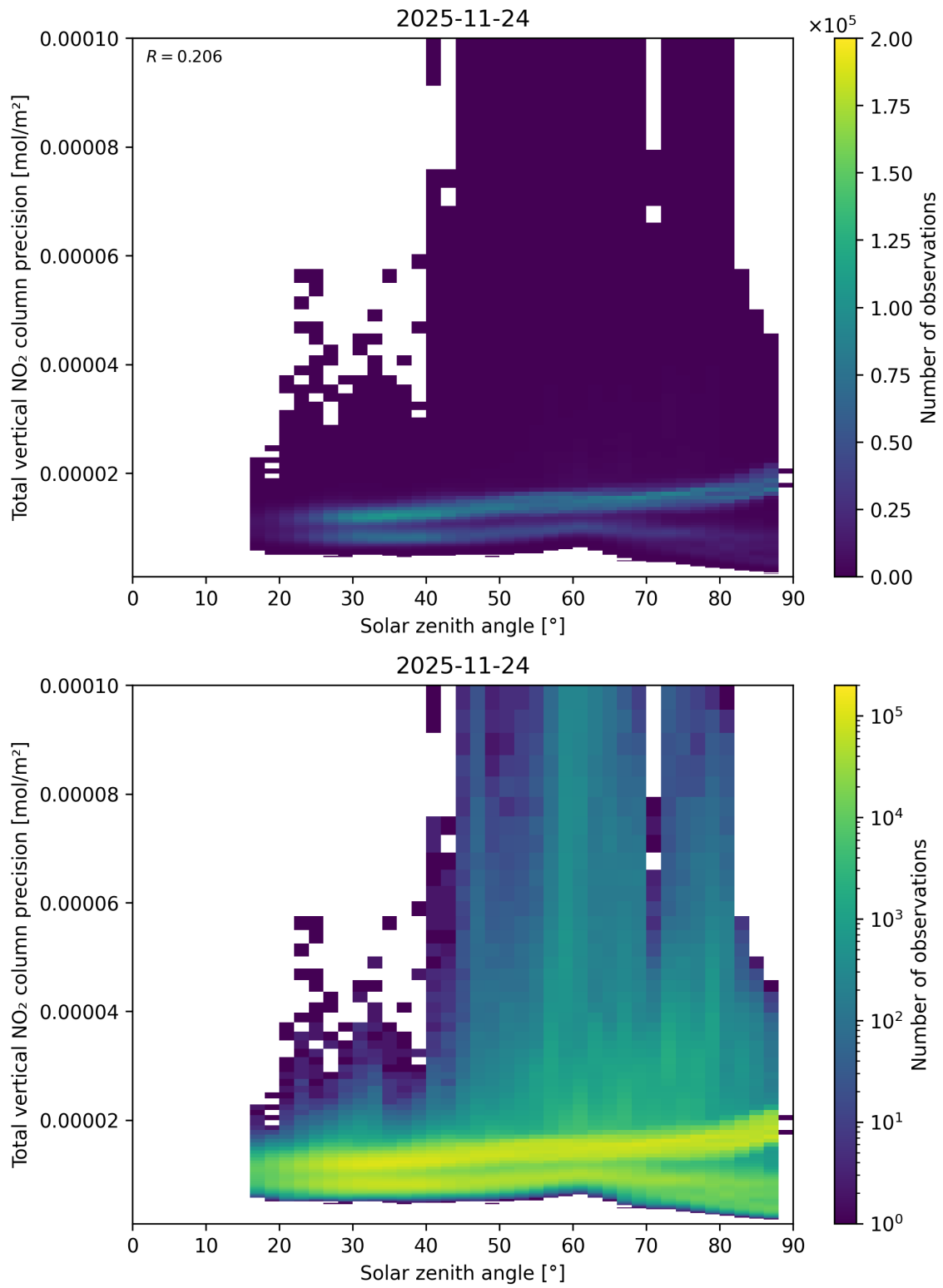
Figure 154: Scatter density plot of “Solar zenith angle” against “Total vertical NO 2 column precision” for 2025-11-23 to 2025-11-25.
