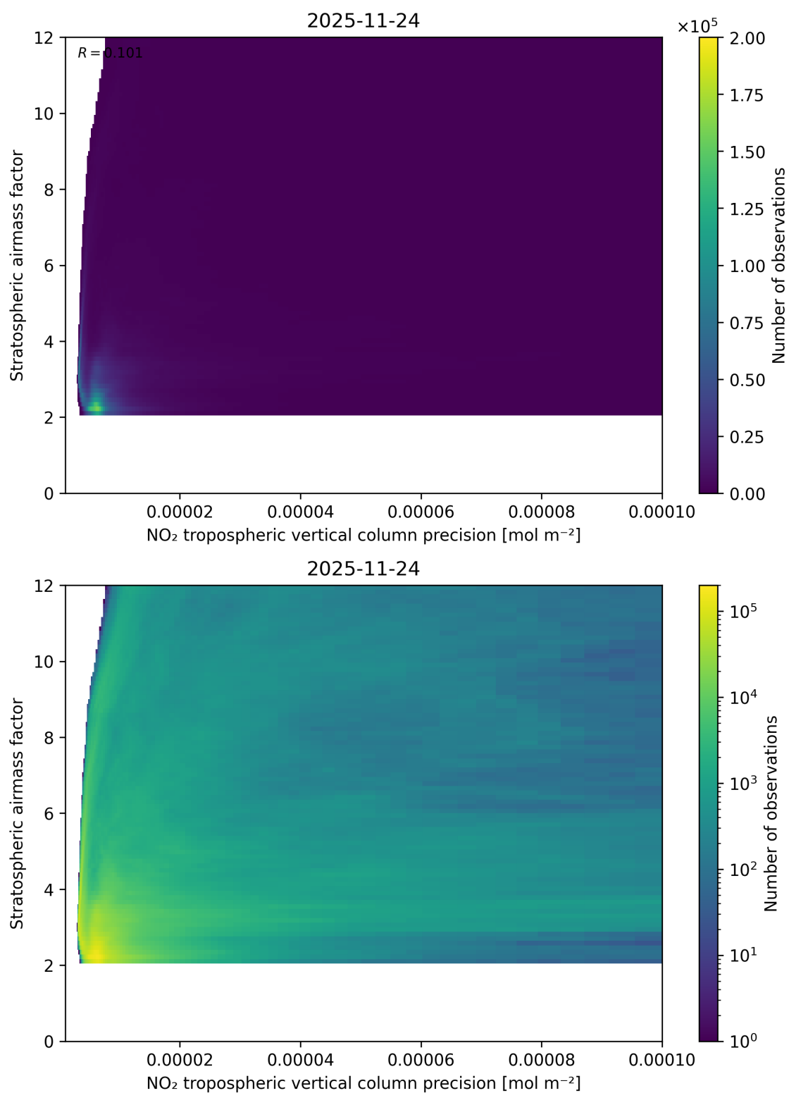
Figure 131: Scatter density plot of “NO 2 tropospheric vertical column precision” against “Stratospheric airmass factor” for 2025-11-23 to 2025-11-25.
