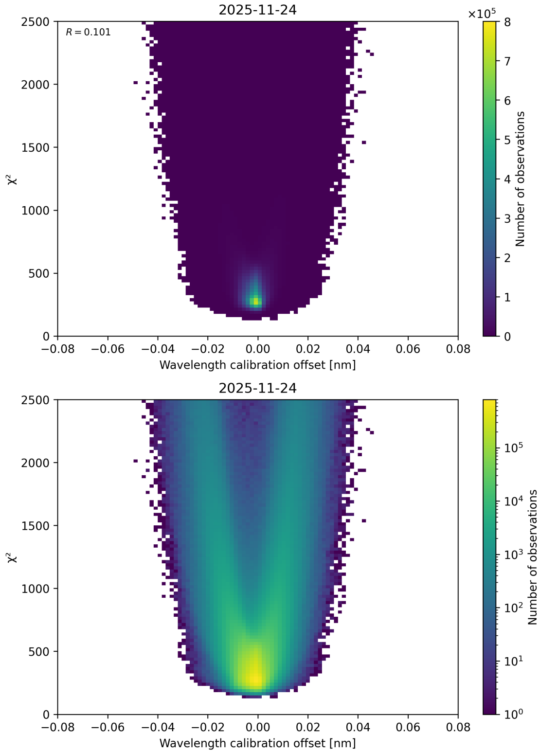
Figure 175: Scatter density plot of “Wavelength calibration offset” against “ \chi^2 ” for 2025-11-23 to 2025-11-25.
