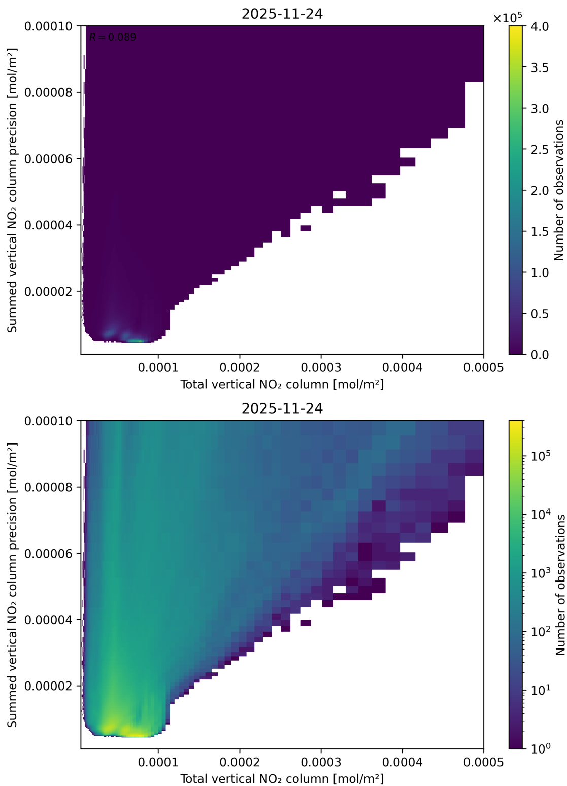
Figure 113: Scatter density plot of “Total vertical NO 2 column” against “Summed vertical NO 2 column precision” for 2025-11-23 to 2025-11-25.
