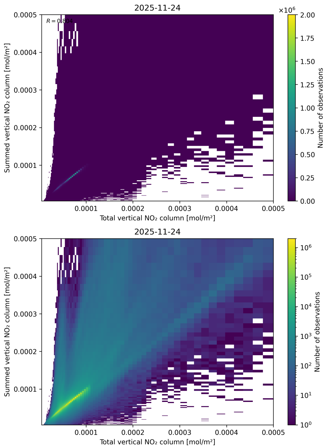
Figure 112: Scatter density plot of “Total vertical NO 2 column” against “Summed vertical NO 2 column” for 2025-11-23 to 2025-11-25.
