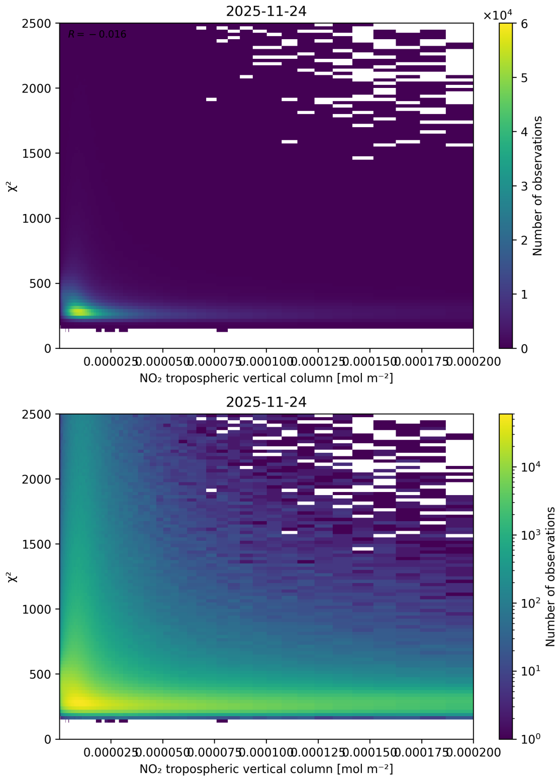
Figure 124: Scatter density plot of “NO 2 tropospheric vertical column” against “ \chi^2 ” for 2025-11-23 to 2025-11-25.
