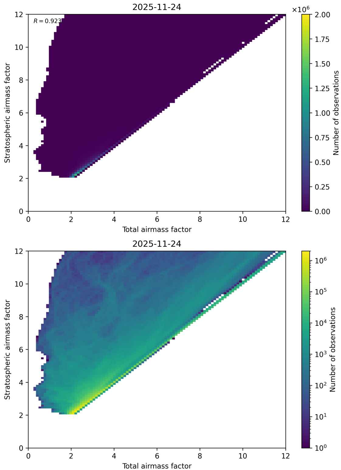
Figure 62: Scatter density plot of “Total airmass factor” against “Stratospheric airmass factor” for 2025-11-23 to 2025-11-25.
