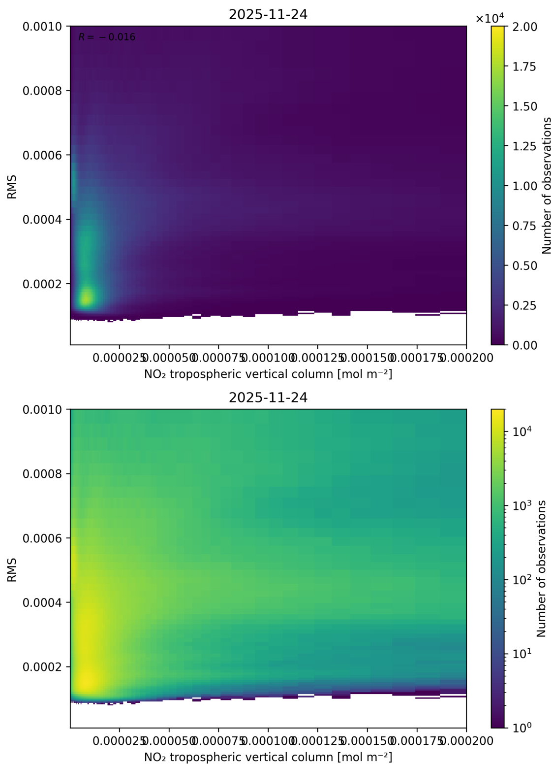
Figure 142: Scatter density plot of “NO 2 tropospheric vertical column” against “RMS” for 2025-11-23 to 2025-11-25.
