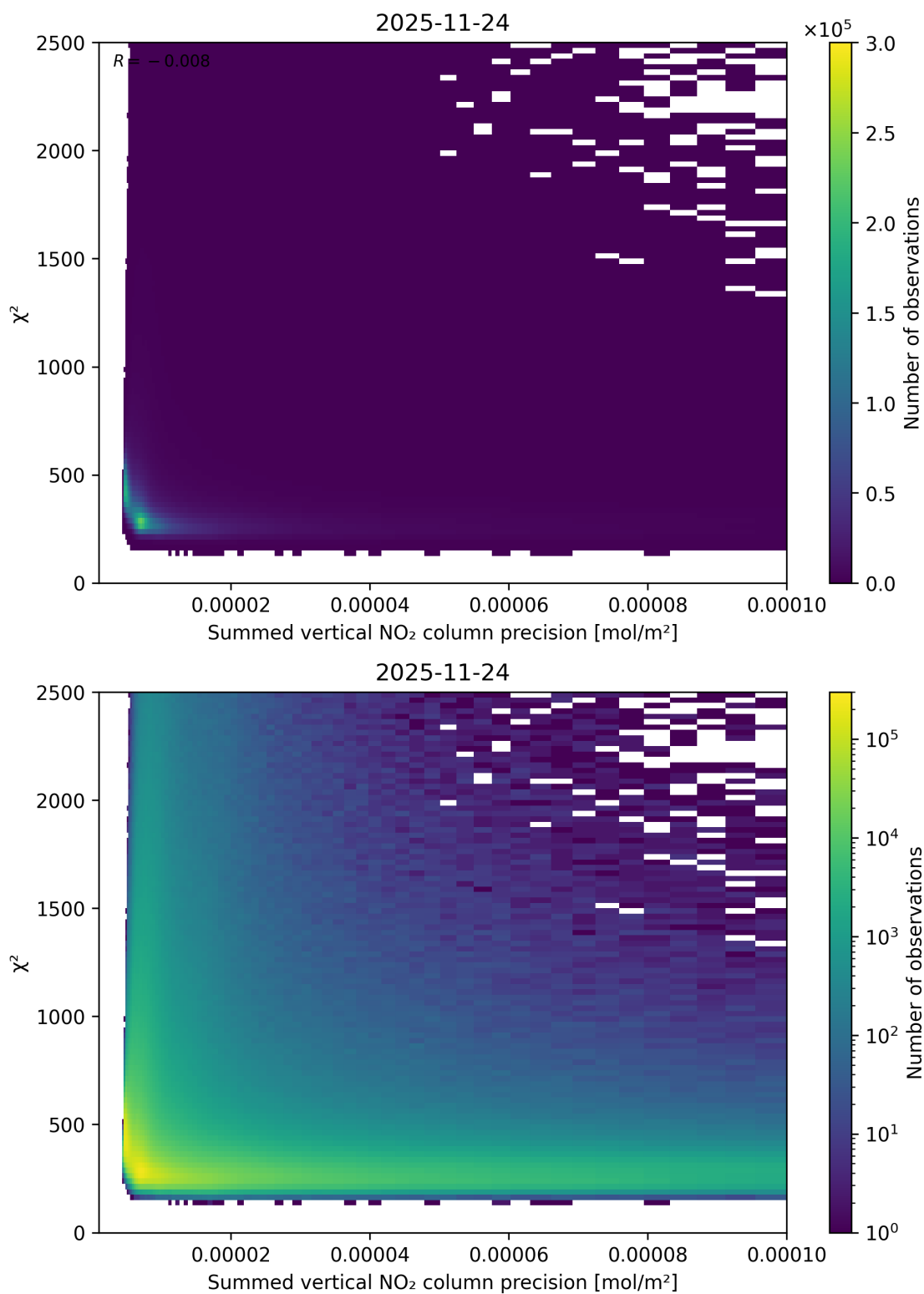
Figure 107: Scatter density plot of “Summed vertical NO 2 column precision” against “ \chi^2 ” for 2025-11-23 to 2025-11-25.
