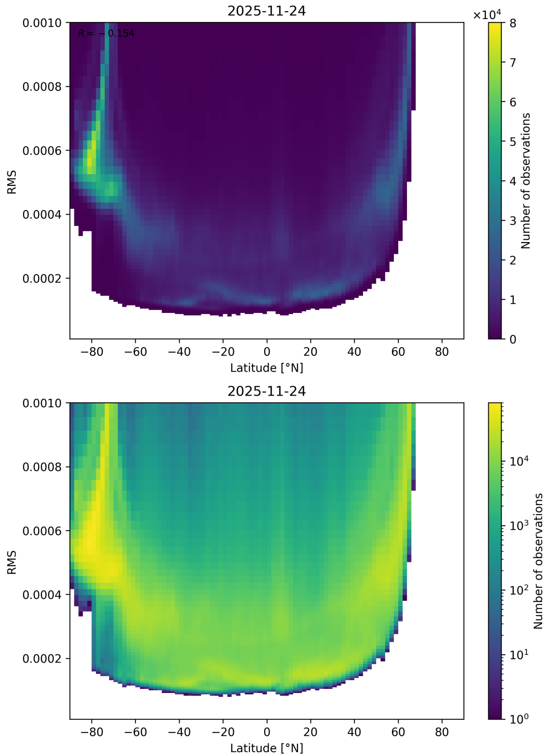
Figure 94: Scatter density plot of “Latitude” against “RMS” for 2025-11-23 to 2025-11-25.
