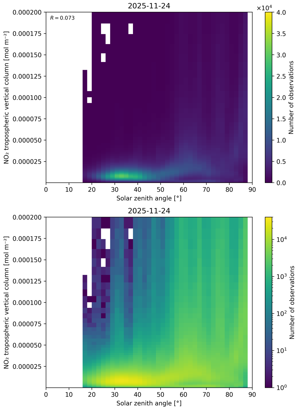
Figure 155: Scatter density plot of “Solar zenith angle” against “NO 2 tropospheric vertical column” for 2025-11-23 to 2025-11-25.
