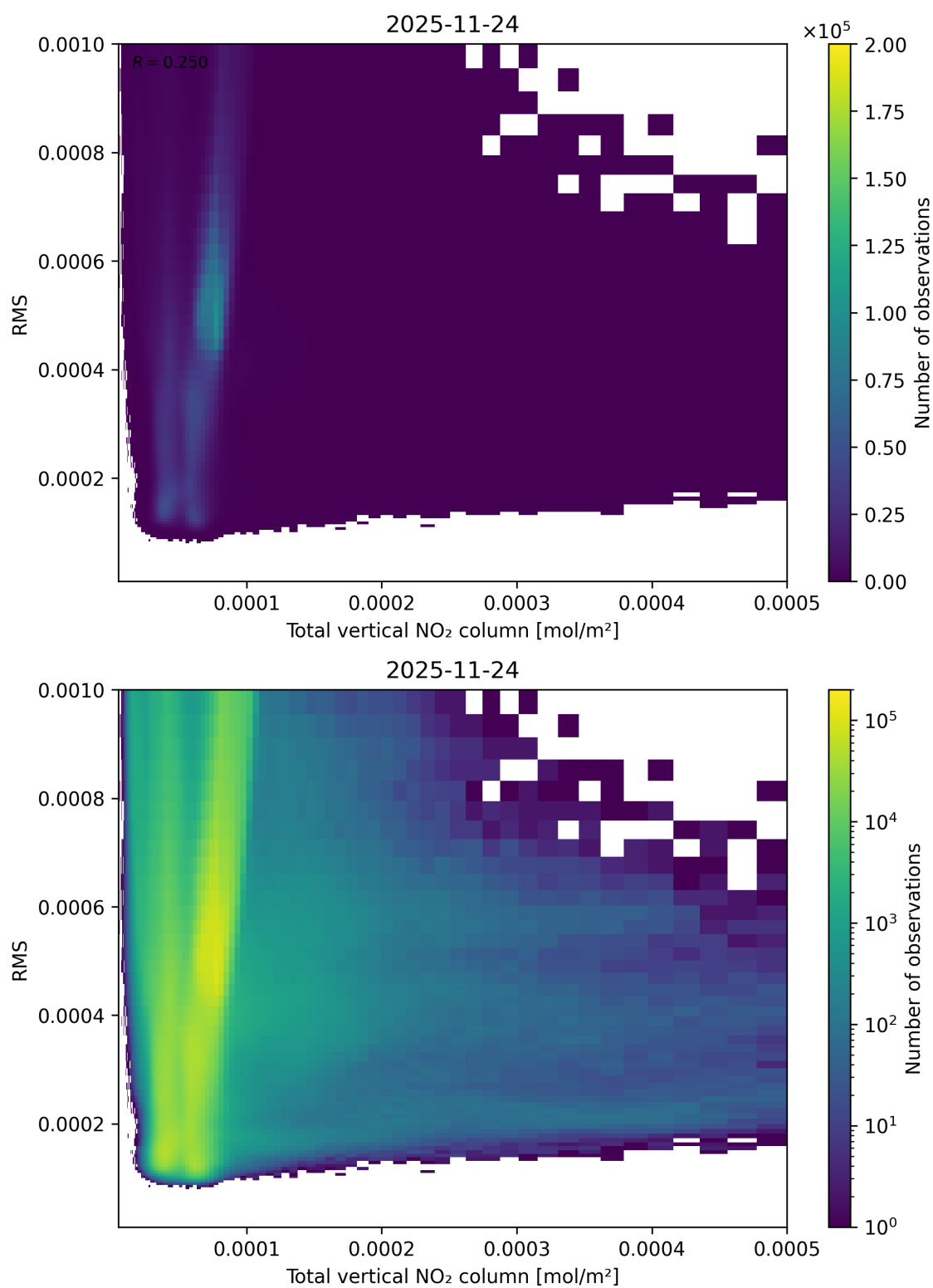
Figure 120: Scatter density plot of “Total vertical NO 2 column” against “RMS” for 2025-11-23 to 2025-11-25.
