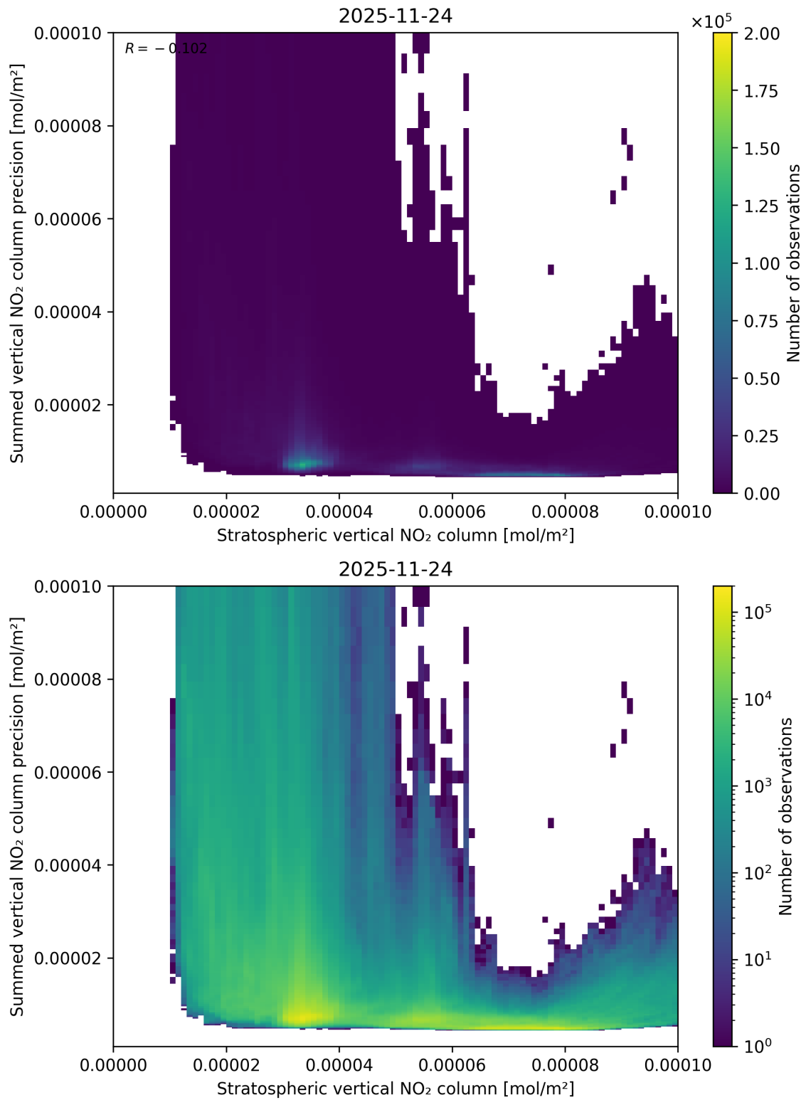
Figure 99: Scatter density plot of “Stratospheric vertical NO 2 column” against “Summed vertical NO 2 column precision” for 2025-11-23 to 2025-11-25.
