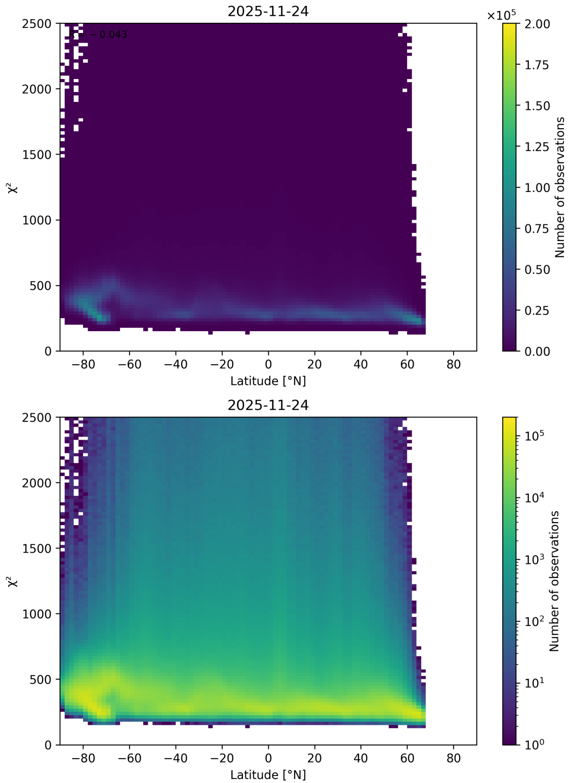
Figure 86: Scatter density plot of “Latitude” against “ \chi^2 ” for 2025-11-23 to 2025-11-25.
