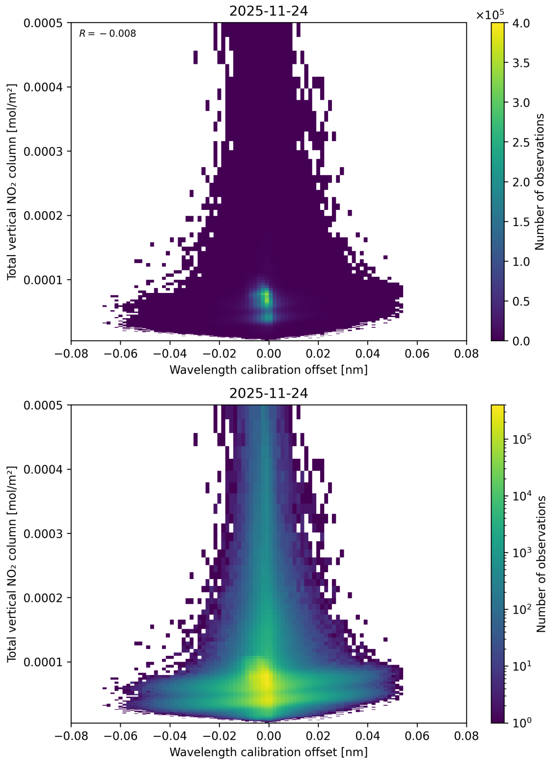
Figure 179: Scatter density plot of “Wavelength calibration offset” against “Total vertical NO 2 column” for 2025-11-23 to 2025-11-25.
