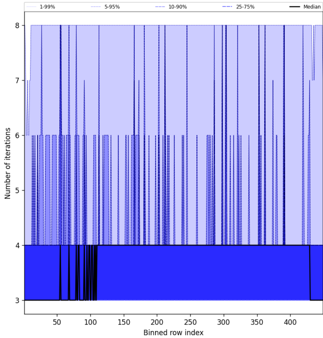
Figure 51: Along track statistics of “Number of iterations” for 2025-11-23 to 2025-11-25
