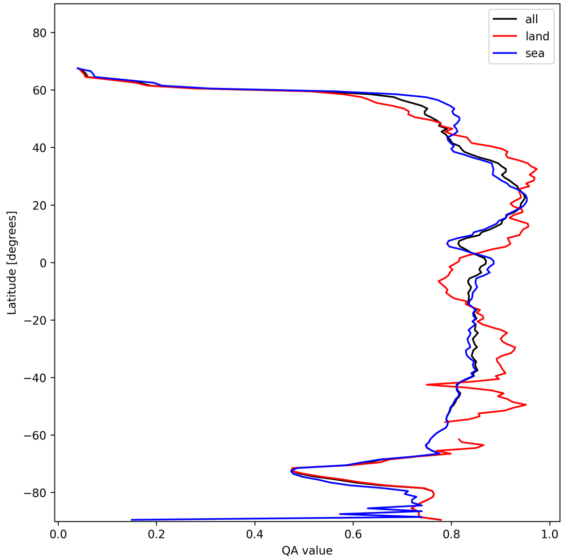
Figure 11: Zonal average of “QA value” for 2025-11-23 to 2025-11-25.
