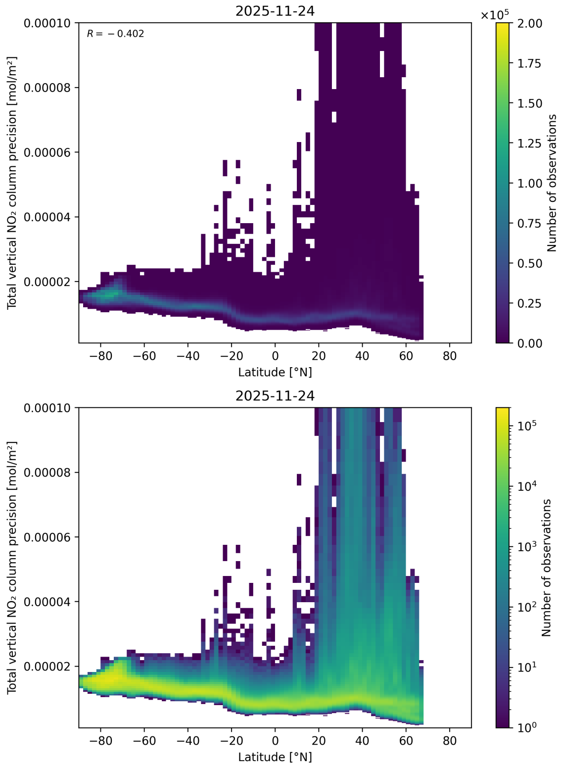
Figure 91: Scatter density plot of “Latitude” against “Total vertical NO 2 column precision” for 2025-11-23 to 2025-11-25.
