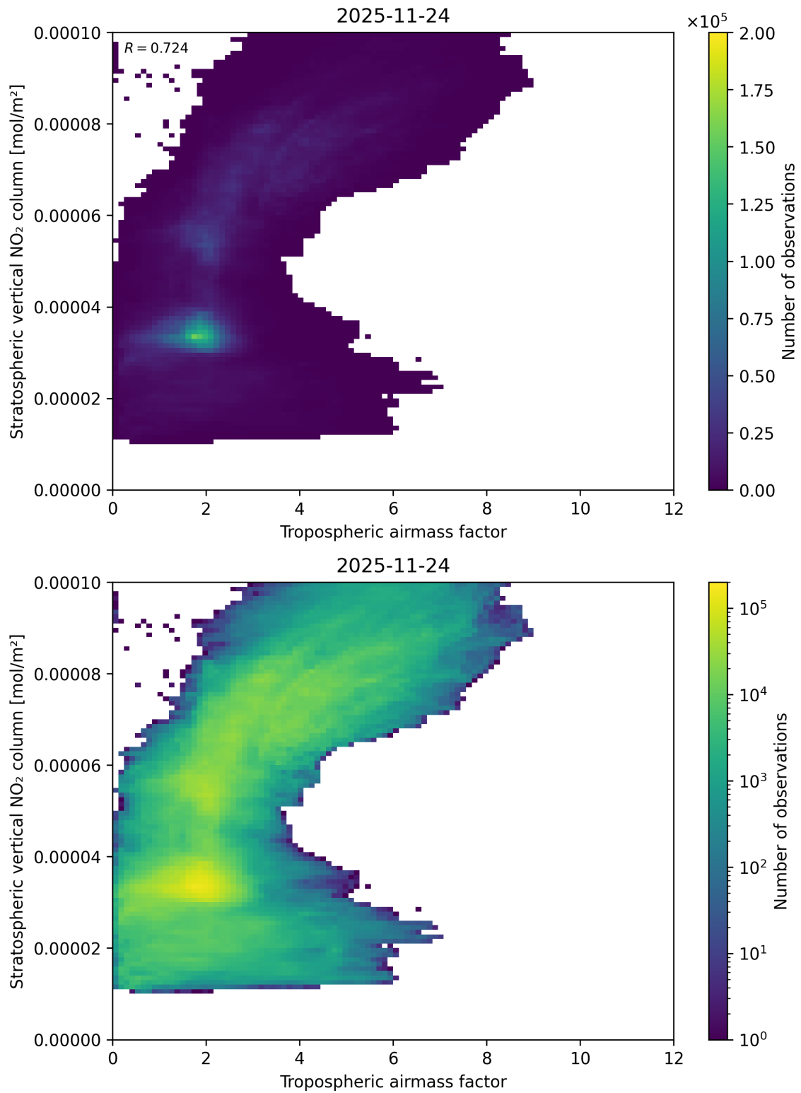
Figure 74: Scatter density plot of “Tropospheric air mass factor” against “Stratospheric vertical NO 2 column” for 2025-11-23 to 2025-11-25.
