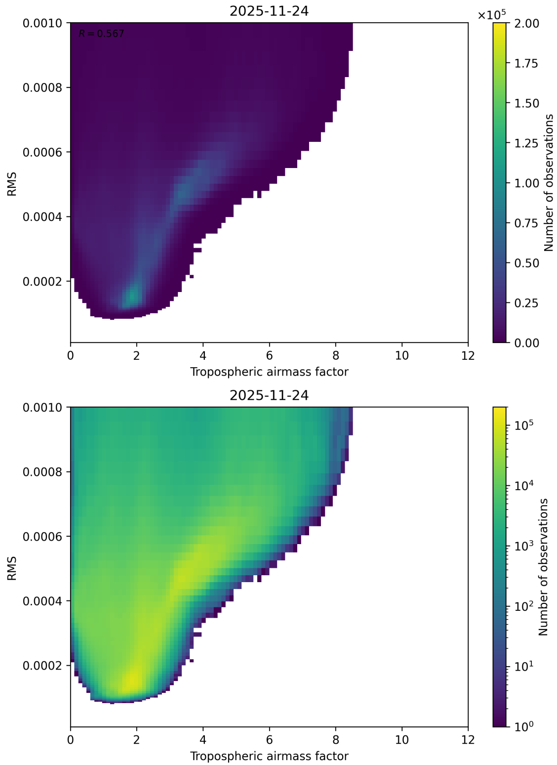
Figure 79: Scatter density plot of “Tropospheric airmass factor” against “RMS” for 2025-11-23 to 2025-11-25.
