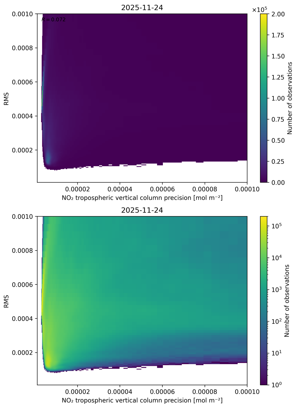
Figure 140: Scatter density plot of “NO 2 tropospheric vertical column precision” against “RMS” for 2025-11-23 to 2025-11-25.
