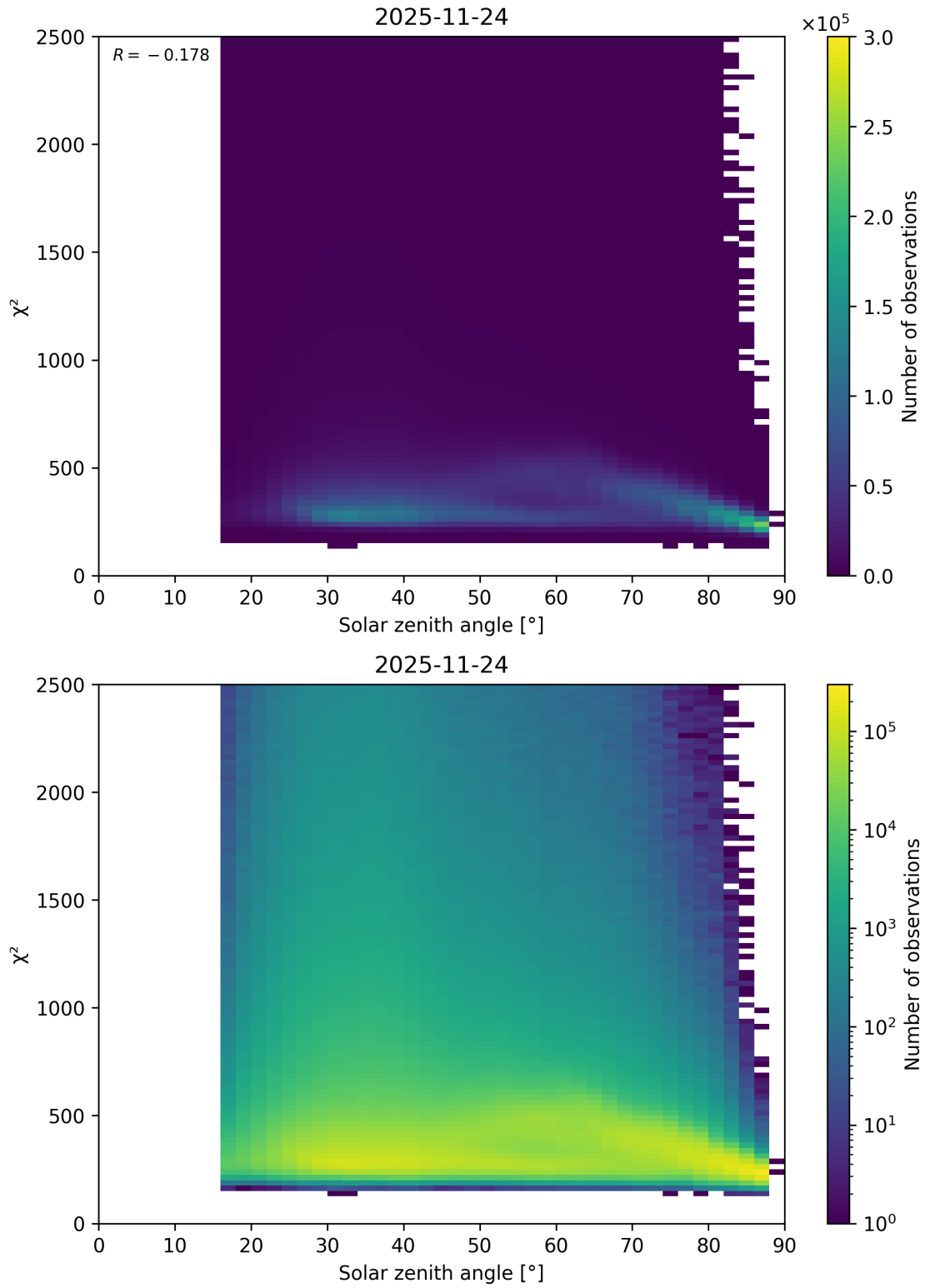
Figure 148: Scatter density plot of “Solar zenith angle” against “ \chi^2 ” for 2025-11-23 to 2025-11-25.
