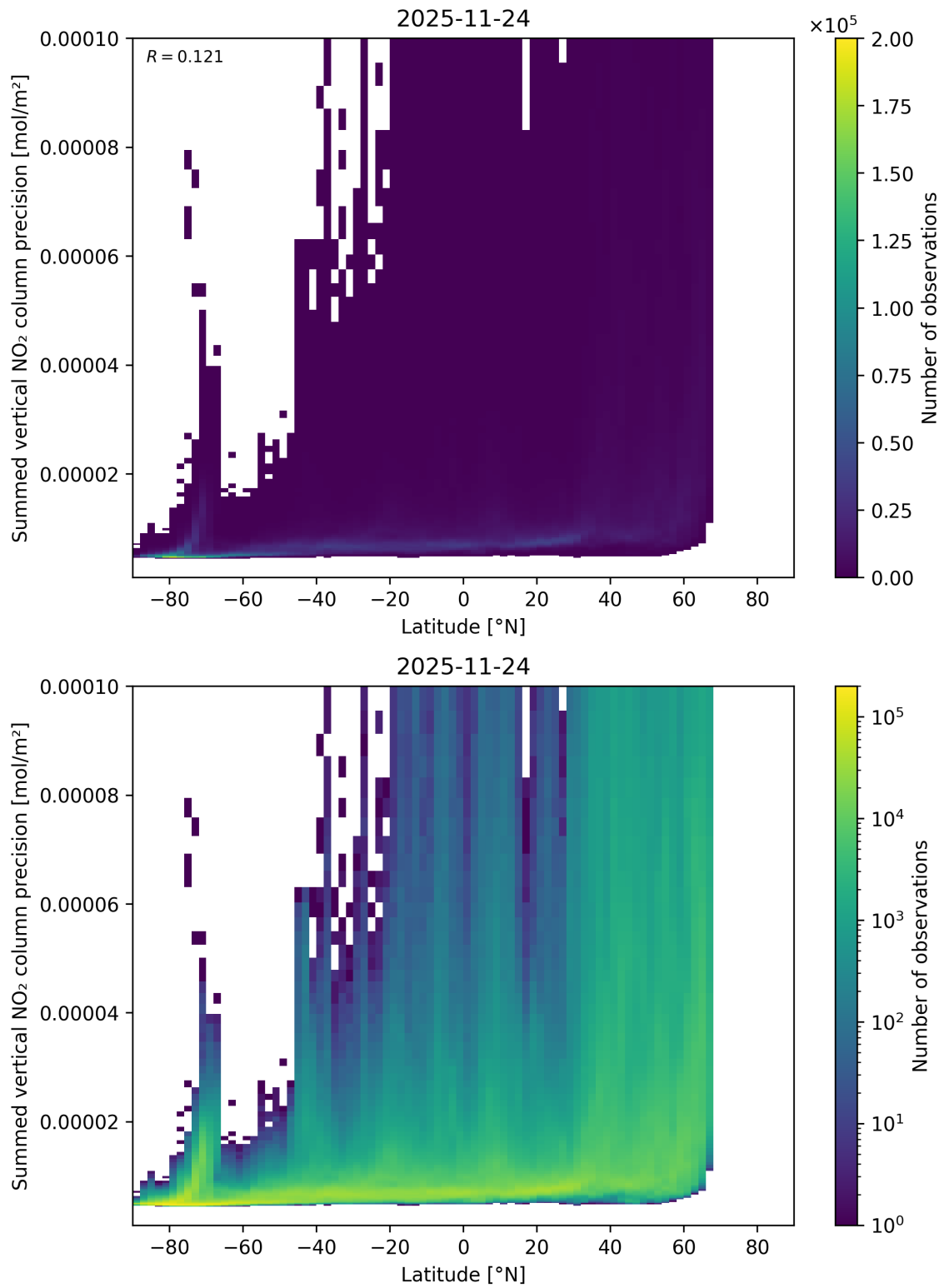
Figure 89: Scatter density plot of “Latitude” against “Summed vertical NO 2 column precision” for 2025-11-23 to 2025-11-25.
