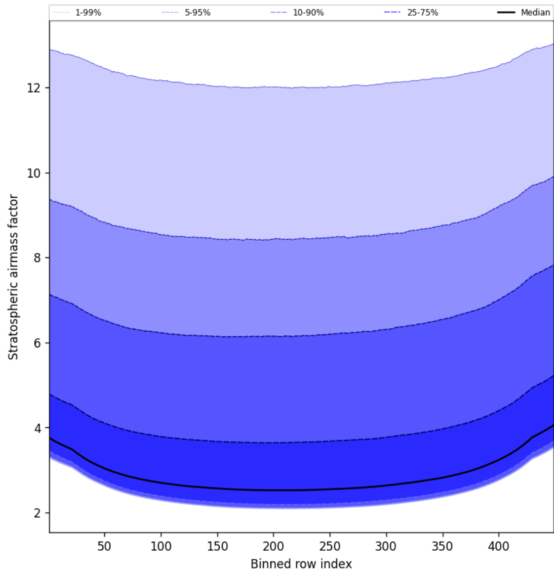
Figure 61: Along track statistics of “Stratospheric air mass factor” for 2025-11-23 to 2025-11-25
