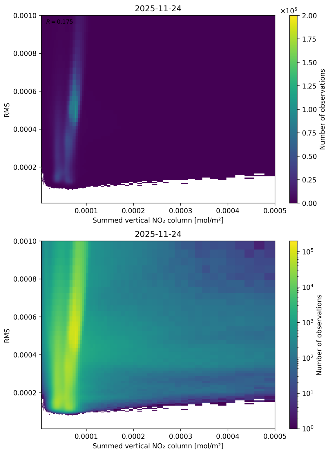
Figure 109: Scatter density plot of “Summed vertical NO 2 column” against “RMS” for 2025-11-23 to 2025-11-25.
