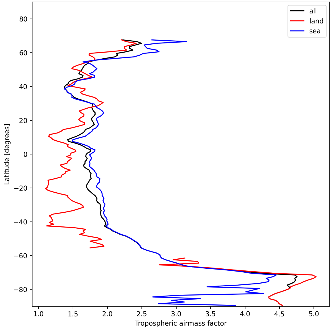
Figure 14: Zonal average of “Tropospheric airmass factor” for 2025-11-23 to 2025-11-25.
