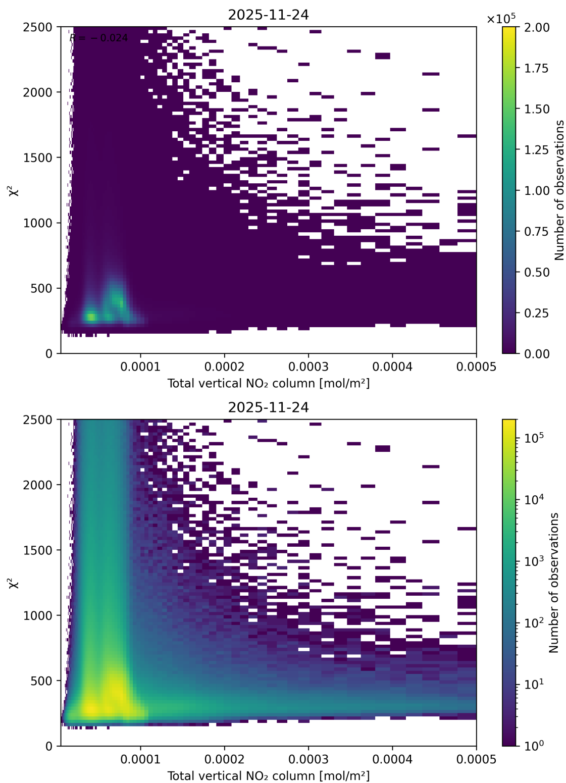
Figure 111: Scatter density plot of “Total vertical NO 2 column” against “ \chi^2 ” for 2025-11-23 to 2025-11-25.
