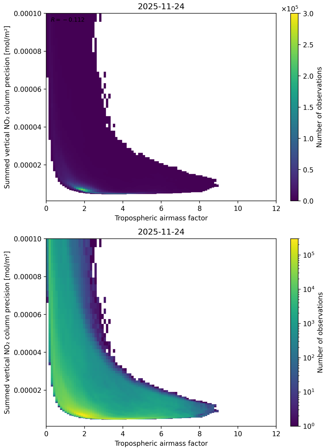
Figure 76: Scatter density plot of “Tropospheric air mass factor” against “Summed vertical NO 2 column precision” for 2025-11-23 to 2025-11-25.
