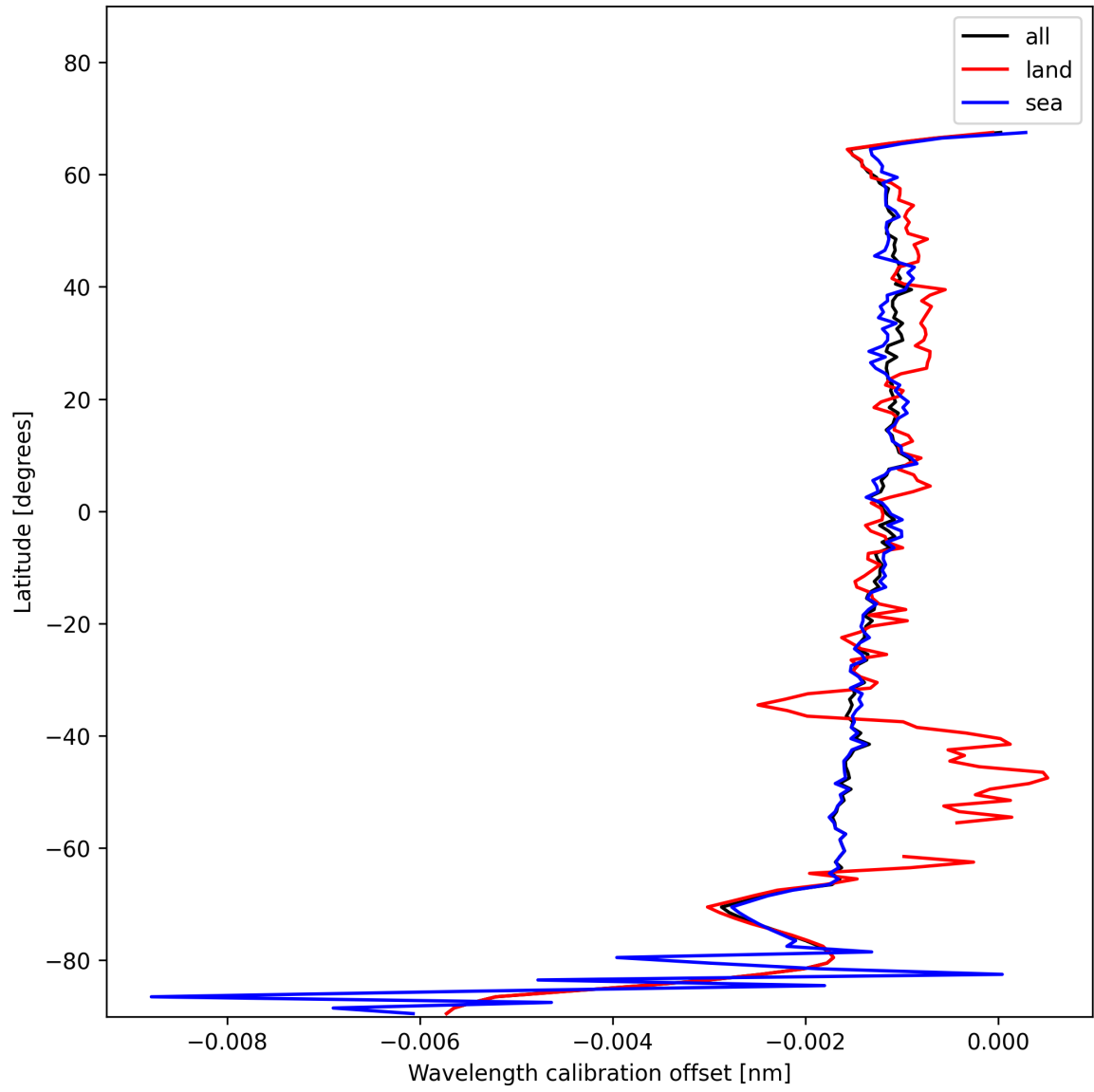
Figure 18: Zonal average of “Wavelength calibration offset” for 2025-11-23 to 2025-11-25.
