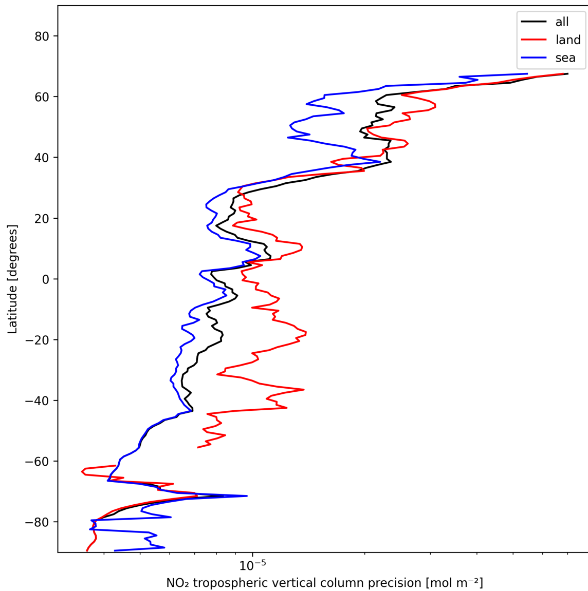
Figure 13: Zonal average of “NO 2 tropospheric vertical column precision” for 2025-11-23 to 2025-11-25.
