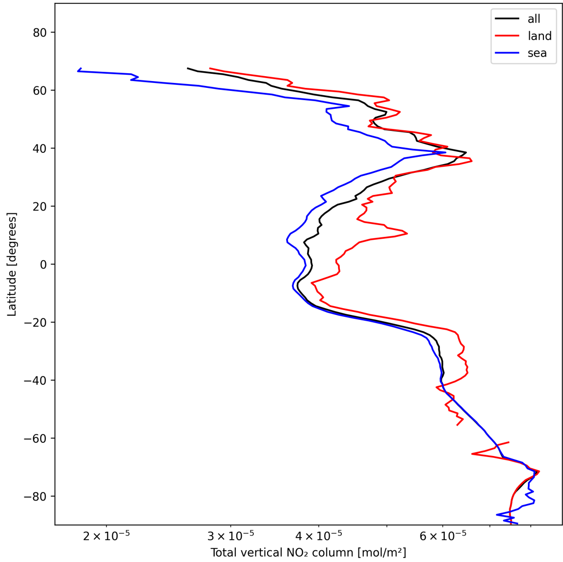
Figure 21: Zonal average of “Total vertical NO 2 column” for 2025-11-23 to 2025-11-25.
