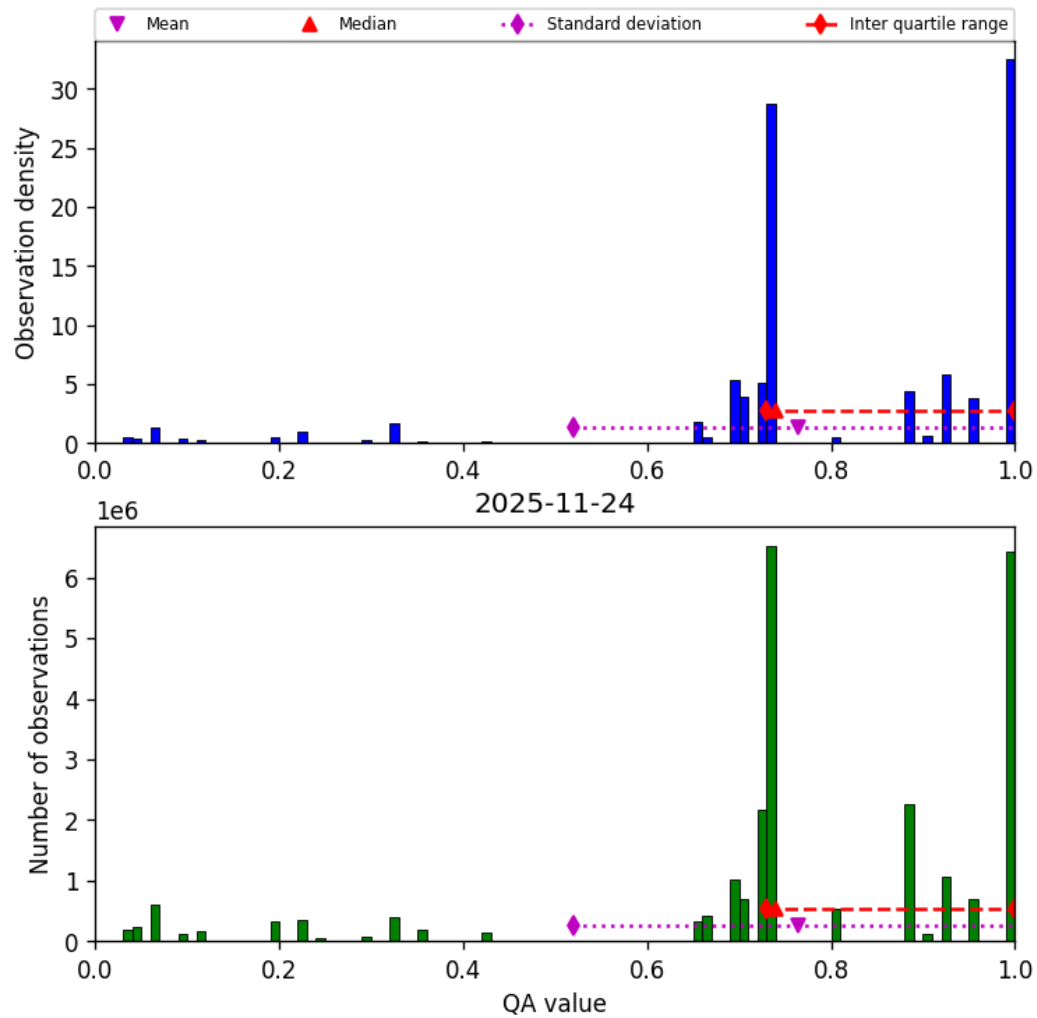
Figure 28: Histogram of “QA value” for 2025-11-23 to 2025-11-25
