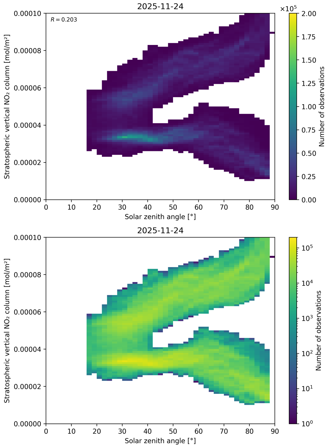
Figure 150: Scatter density plot of “Solar zenith angle” against “Stratospheric vertical NO 2 column” for 2025-11-23 to 2025-11-25.
