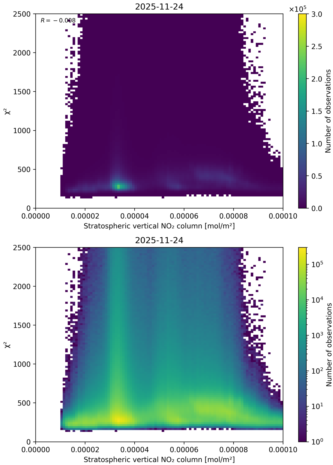
Figure 97: Scatter density plot of “Stratospheric vertical NO 2 column” against “ \chi^2 ” for 2025-11-23 to 2025-11-25.
