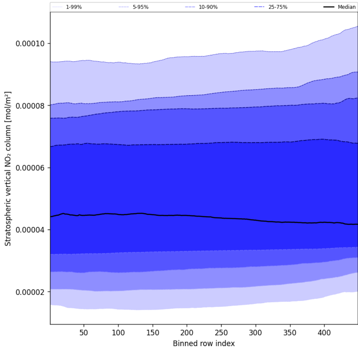
Figure 53: Along track statistics of “Stratospheric vertical NO 2 column” for 2025-11-23 to 2025-11-25
