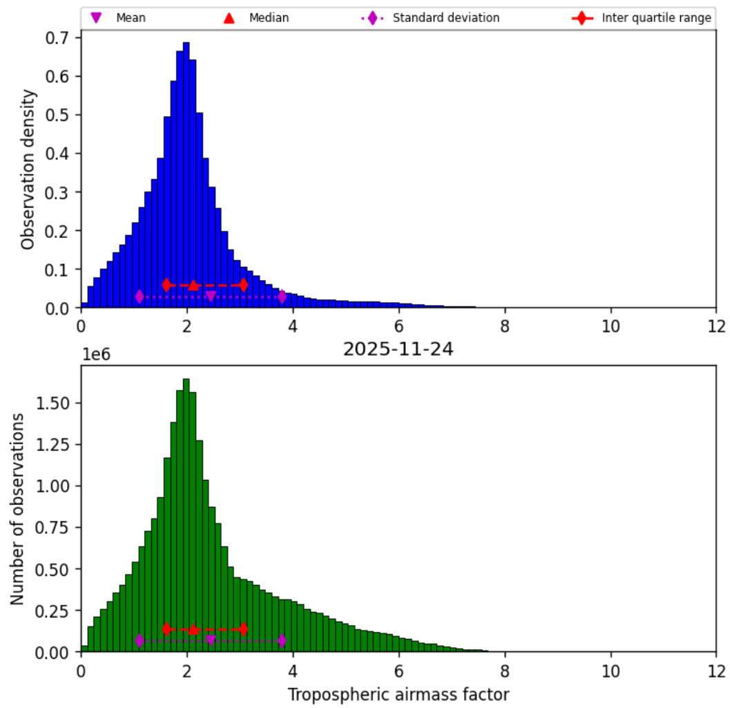
Figure 31: Histogram of “Tropospheric airmass factor” for 2025-11-23 to 2025-11-25
