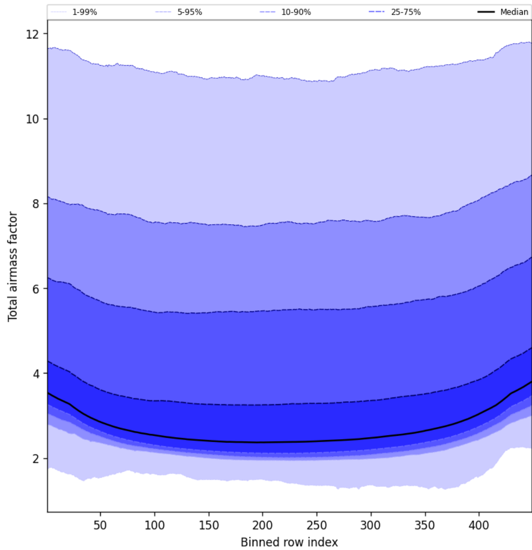
Figure 49: Along track statistics of “Total airmass factor” for 2025-11-23 to 2025-11-25
