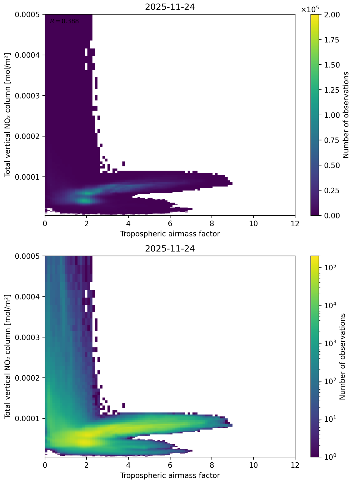
Figure 77: Scatter density plot of “Tropospheric airmass factor” against “Total vertical NO 2 column” for 2025-11-23 to 2025-11-25.
