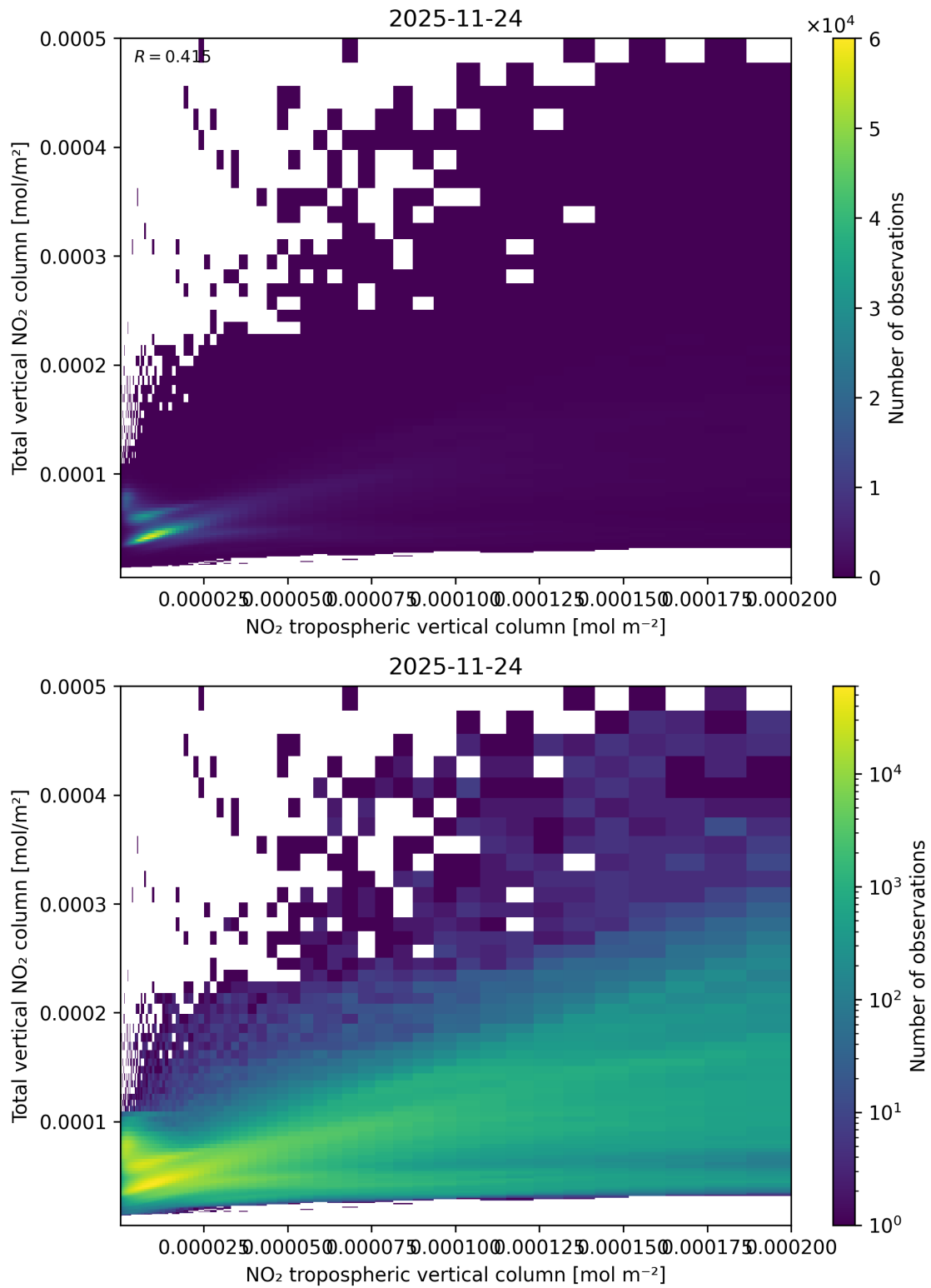
Figure 128: Scatter density plot of “NO 2 tropospheric vertical column” against “Total vertical NO 2 column” for 2025-11-23 to 2025-11-25.
