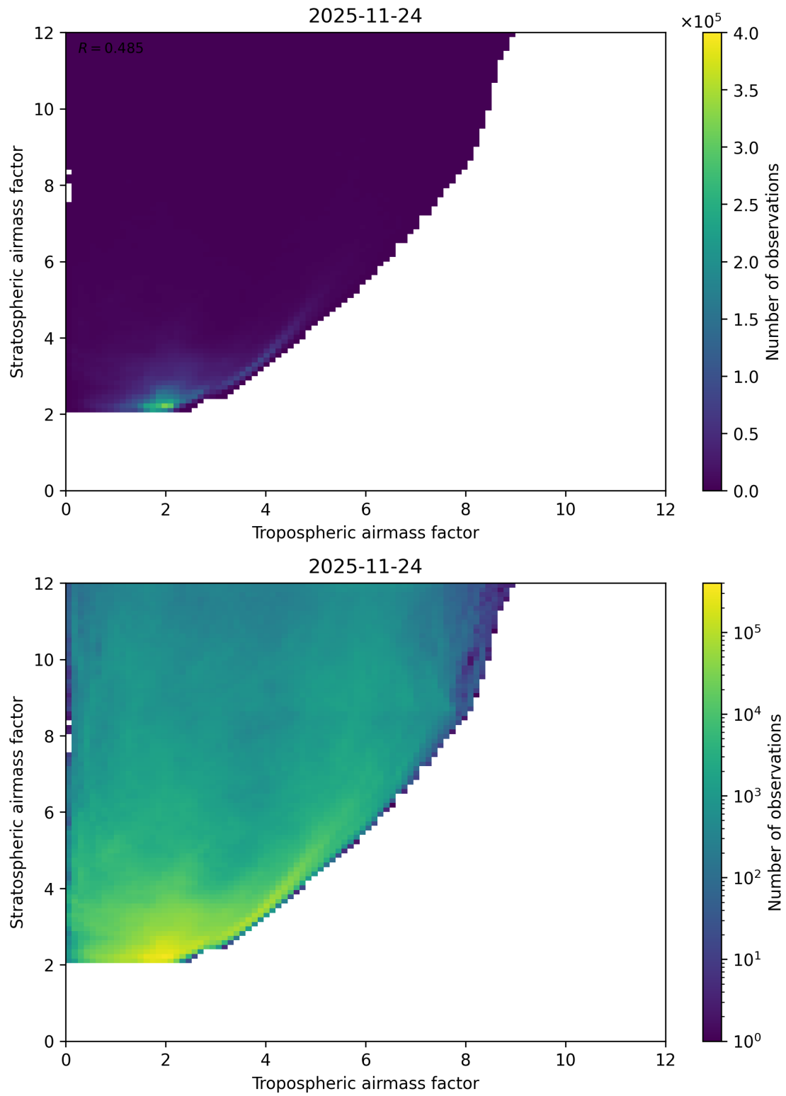
Figure 71: Scatter density plot of “Tropospheric airmass factor” against “Stratospheric airmass factor” for 2025-11-23 to 2025-11-25.
