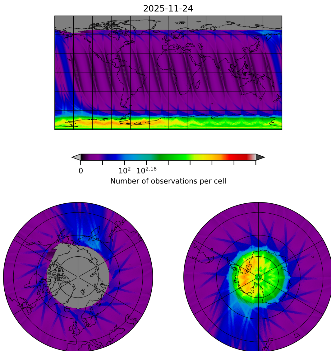
Figure 10: Map of the number of observations for 2025-11-23 to 2025-11-25
