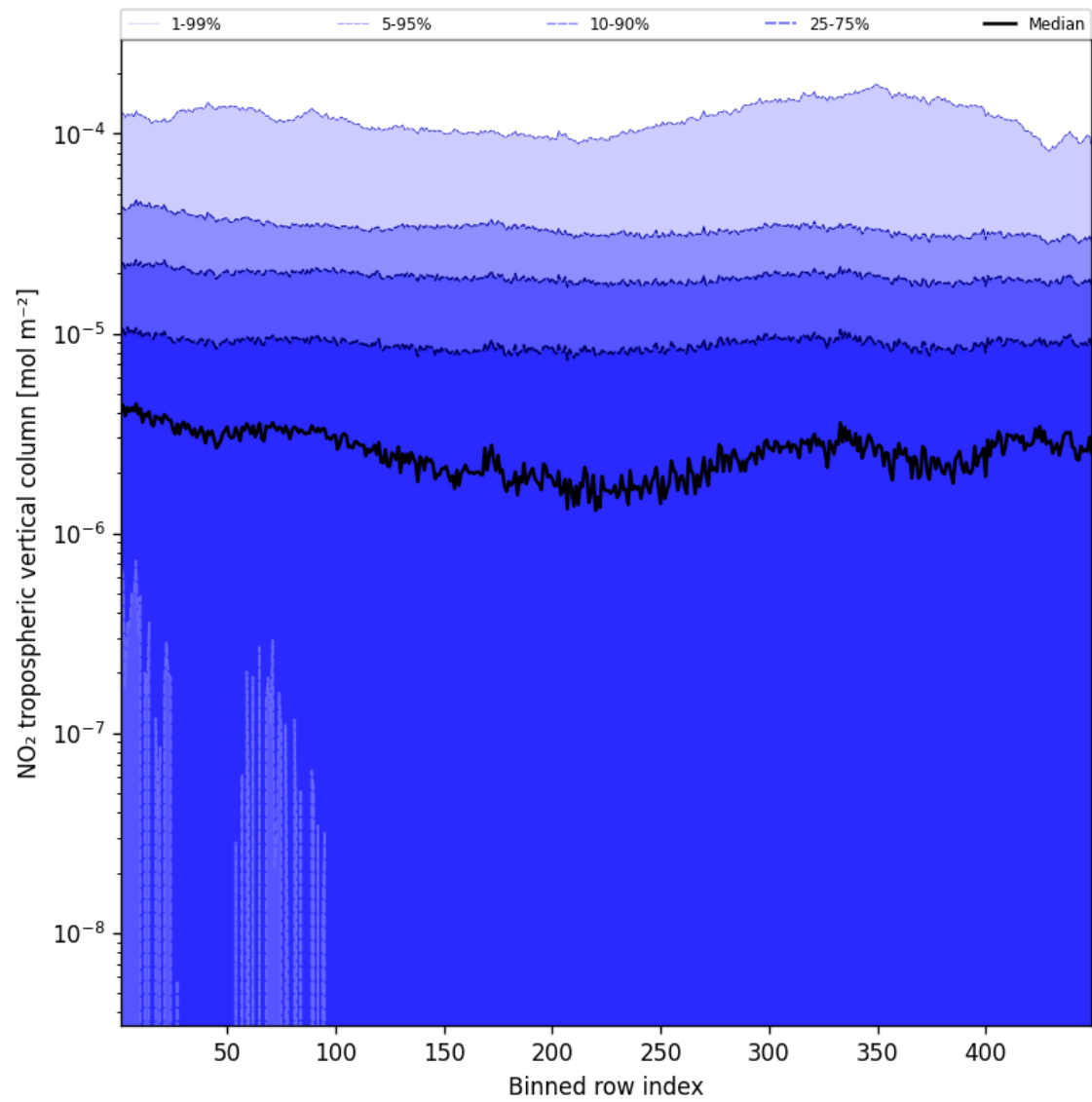
Figure 46: Along track statistics of “NO 2 tropospheric vertical column” for 2025-11-23 to 2025-11-25
