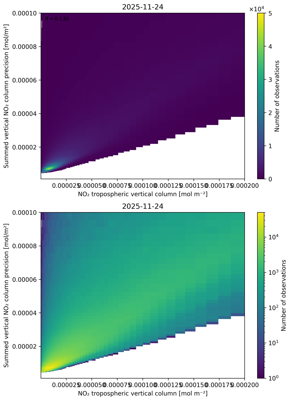
Figure 127: Scatter density plot of “NO 2 tropospheric vertical column” against “Summed vertical NO 2 column precision” for 2025-11-23 to 2025-11-25.
