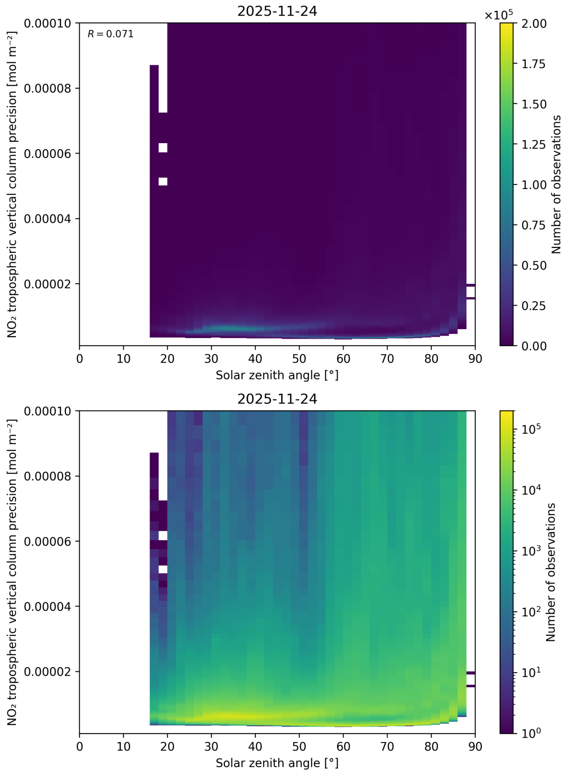
Figure 156: Scatter density plot of “Solar zenith angle” against “NO 2 tropospheric vertical column precision” for 2025-11-23 to 2025-11-25.
