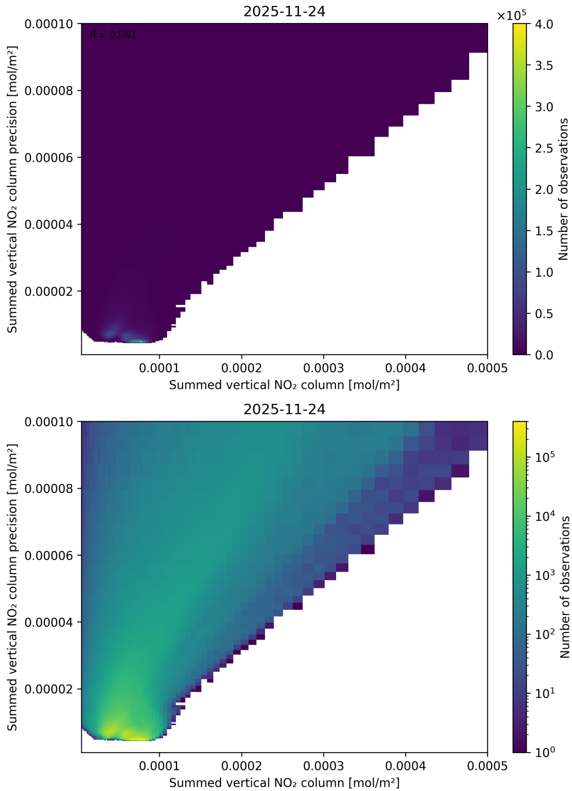
Figure 105: Scatter density plot of “Summed vertical NO 2 column” against “Summed vertical NO 2 column precision” for 2025-11-23 to 2025-11-25.
