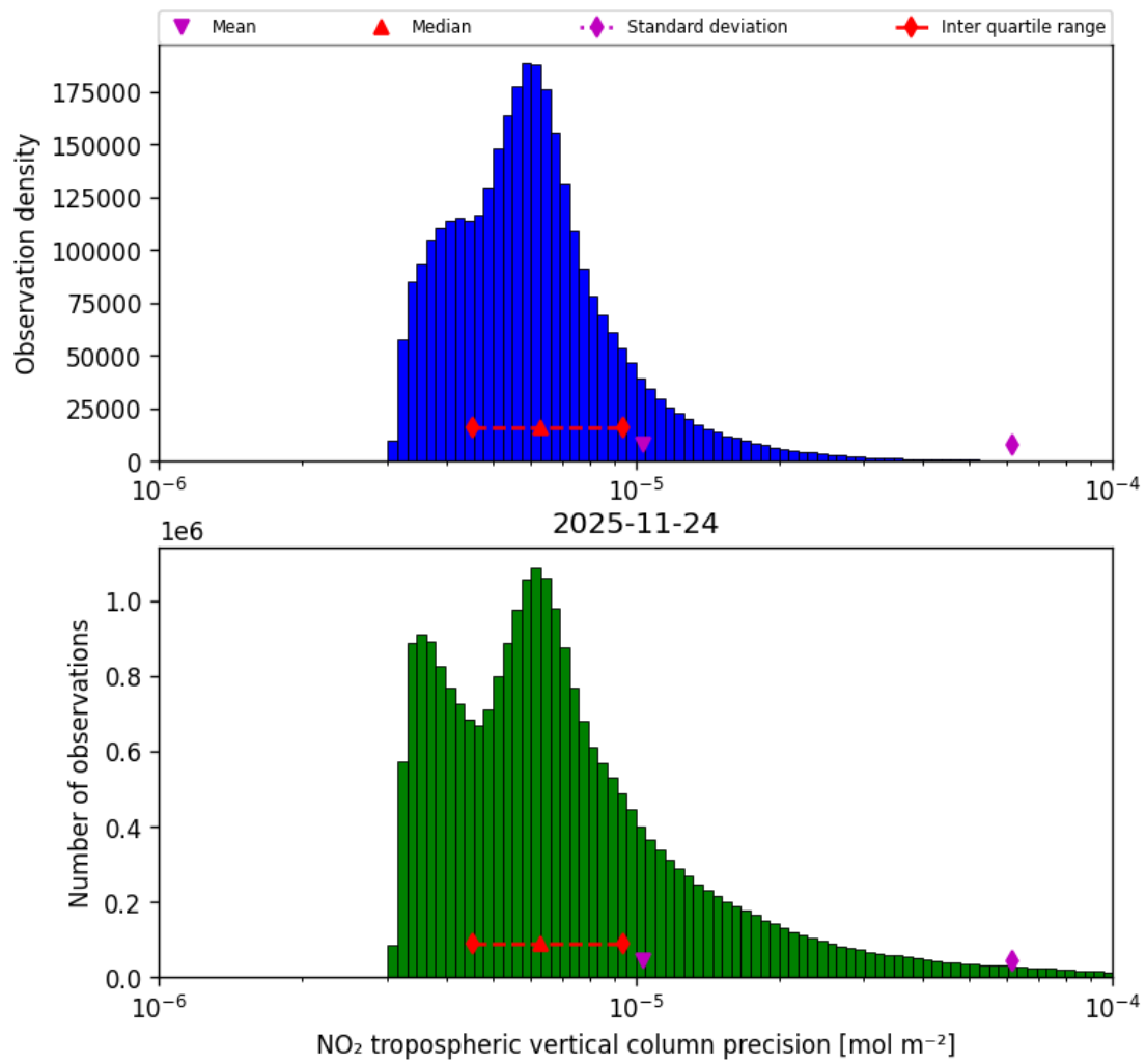
Figure 30: Histogram of “NO 2 tropospheric vertical column precision” for 2025-11-23 to 2025-11-25
