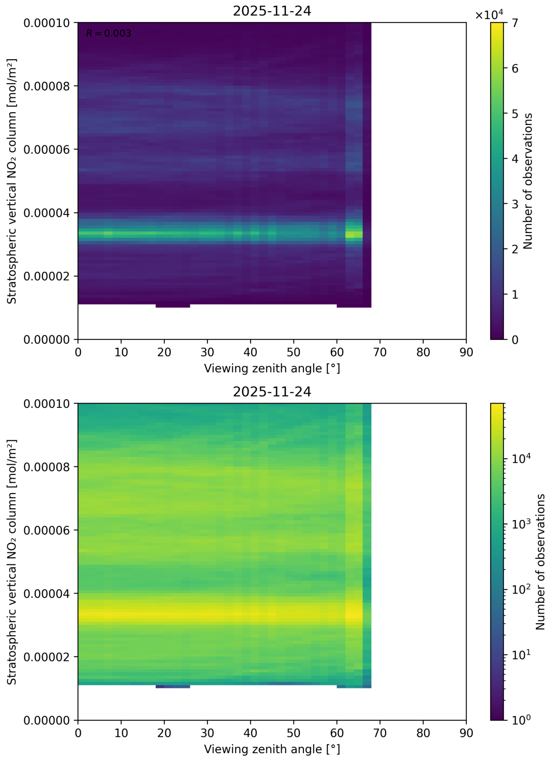
Figure 164: Scatter density plot of “Viewing zenith angle” against “Stratospheric vertical NO 2 column” for 2025-11-23 to 2025-11-25.
