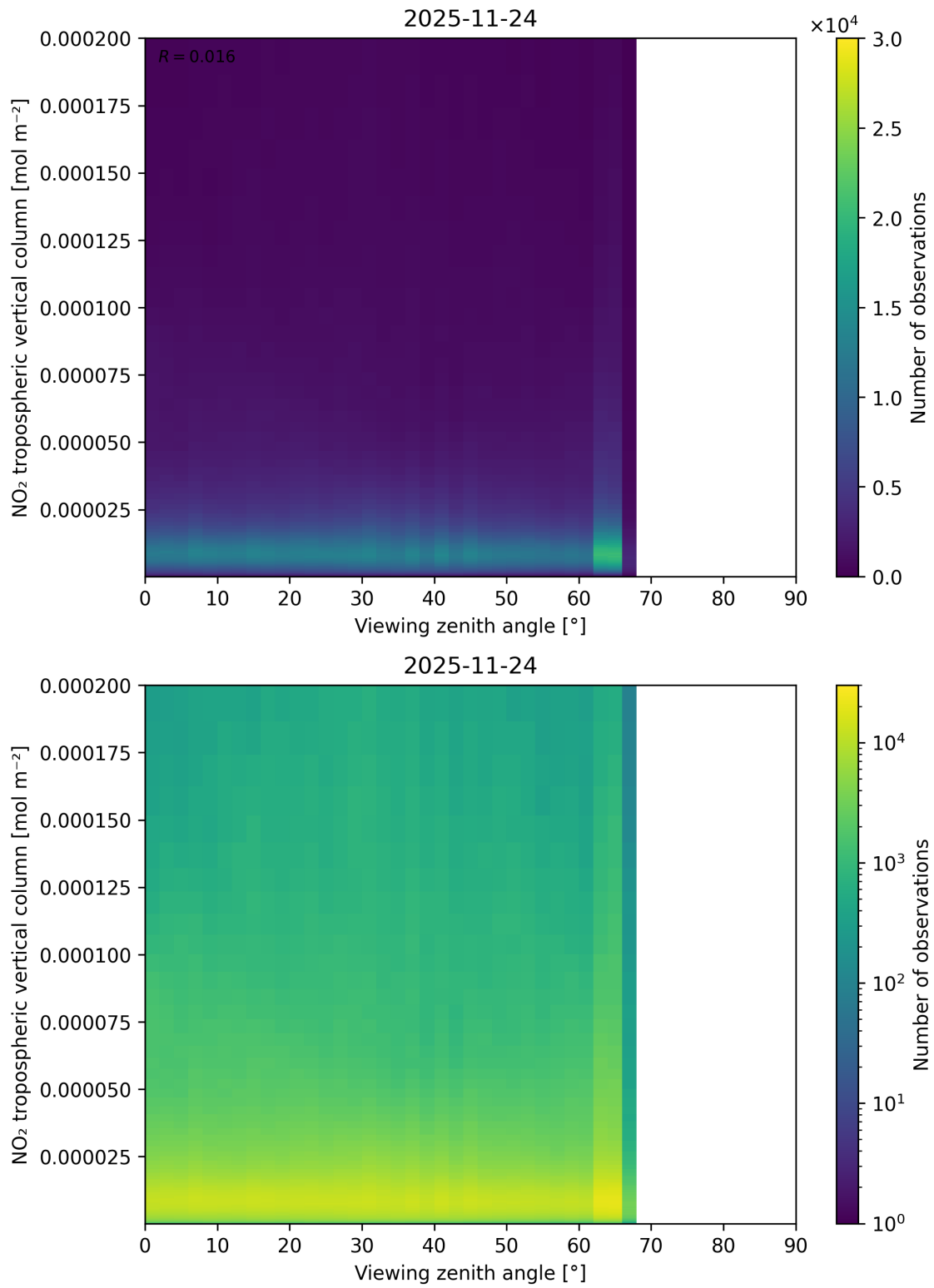
Figure 169: Scatter density plot of “Viewing zenith angle” against “NO 2 tropospheric vertical column” for 2025-11-23 to 2025-11-25.
