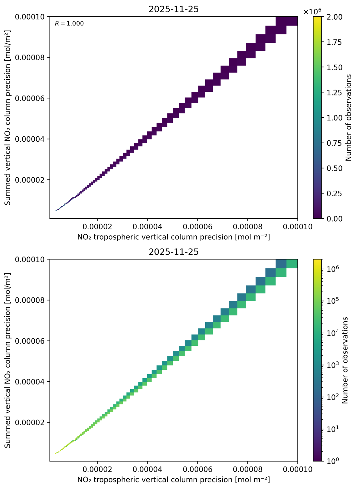
Figure 137: Scatter density plot of “NO 2 tropospheric vertical column precision” against “Summed vertical NO 2 column precision” for 2025-11-24 to 2025-11-26.
