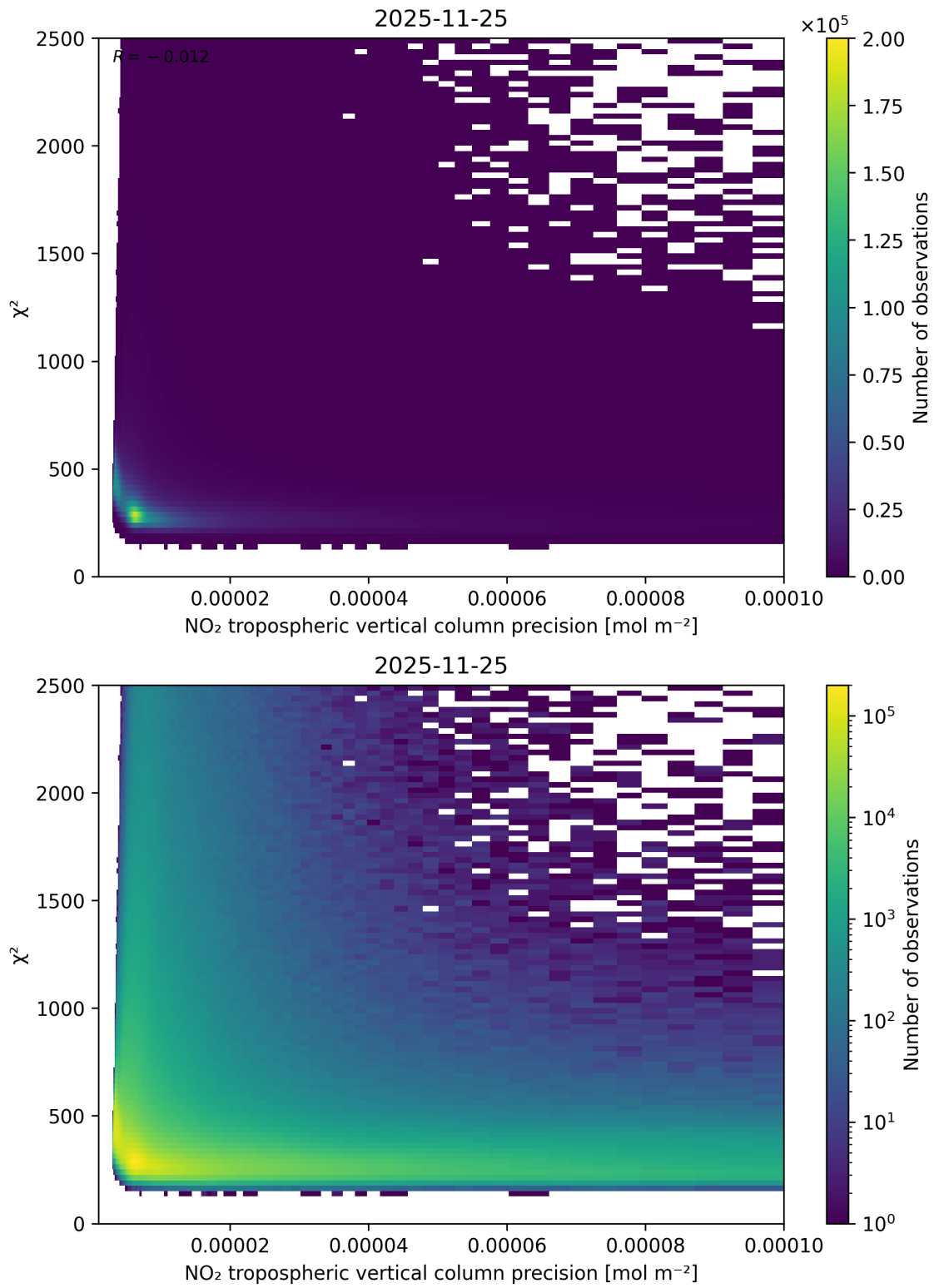
Figure 134: Scatter density plot of “NO 2 tropospheric vertical column precision” against “ \chi^2 ” for 2025-11-24 to 2025-11-26.
