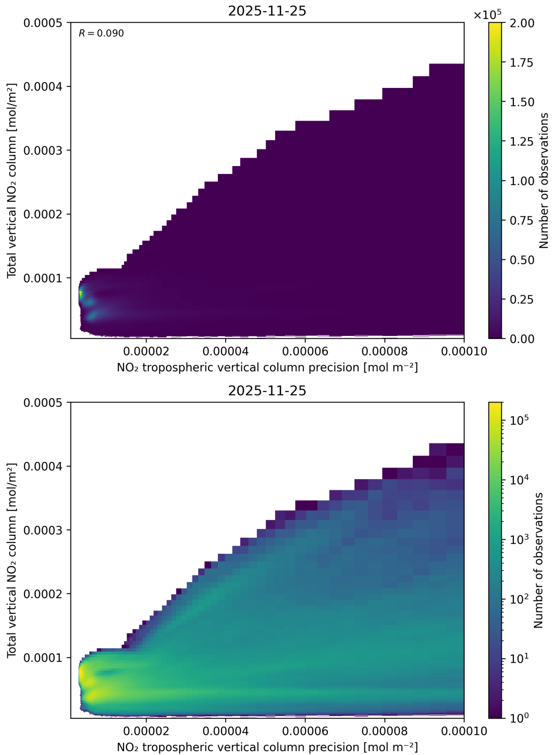
Figure 138: Scatter density plot of “NO 2 tropospheric vertical column precision” against “Total vertical NO 2 column” for 2025-11-24 to 2025-11-26.
