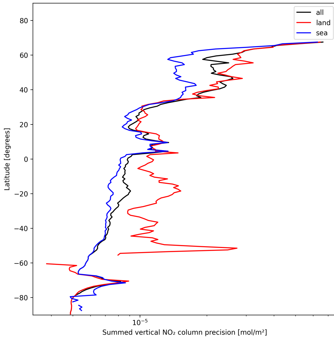
Figure 24: Zonal average of “Summed vertical NO 2 column precision” for 2025-11-24 to 2025-11-26.
