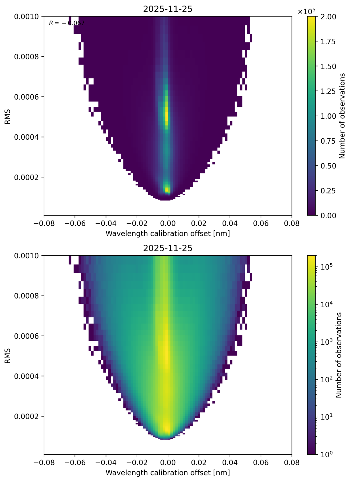
Figure 181: Scatter density plot of “Wavelength calibration offset” against “RMS” for 2025-11-24 to 2025-11-26.
