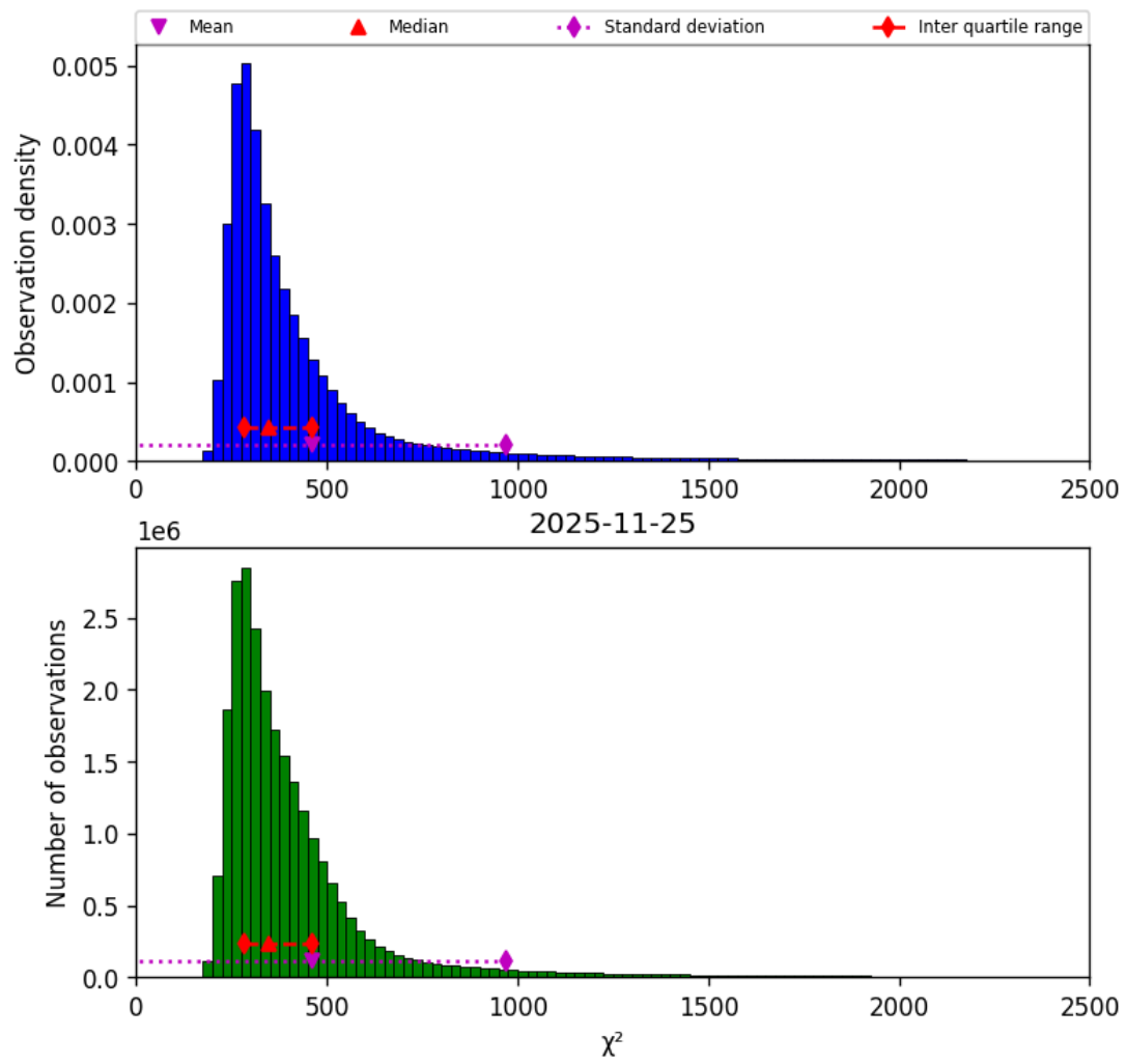
Figure 42: Histogram of “ \chi^2 ” for 2025-11-24 to 2025-11-26
