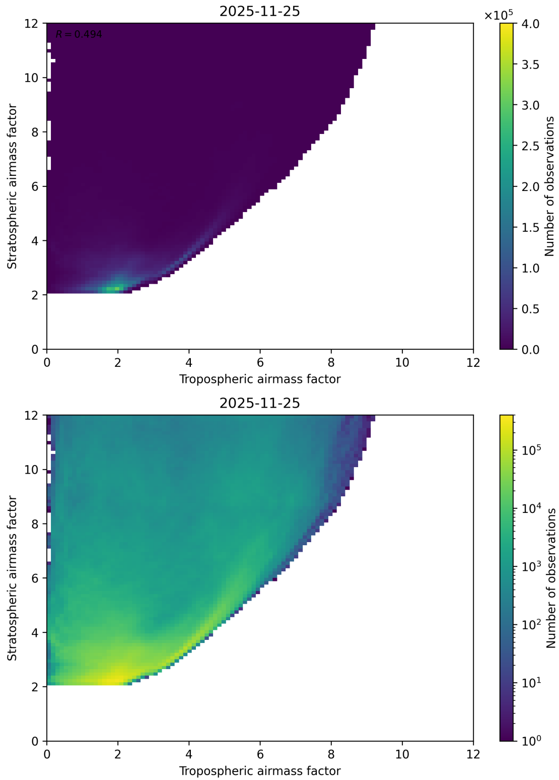
Figure 71: Scatter density plot of “Tropospheric airmass factor” against “Stratospheric airmass factor” for 2025-11-24 to 2025-11-26.
