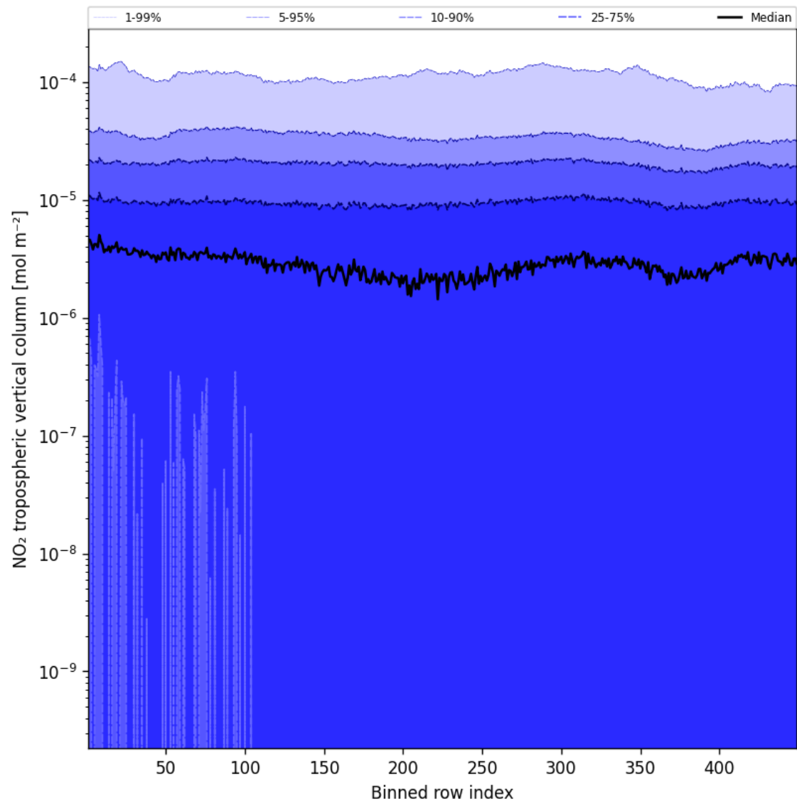
Figure 46: Along track statistics of “NO 2 tropospheric vertical column” for 2025-11-24 to 2025-11-26
