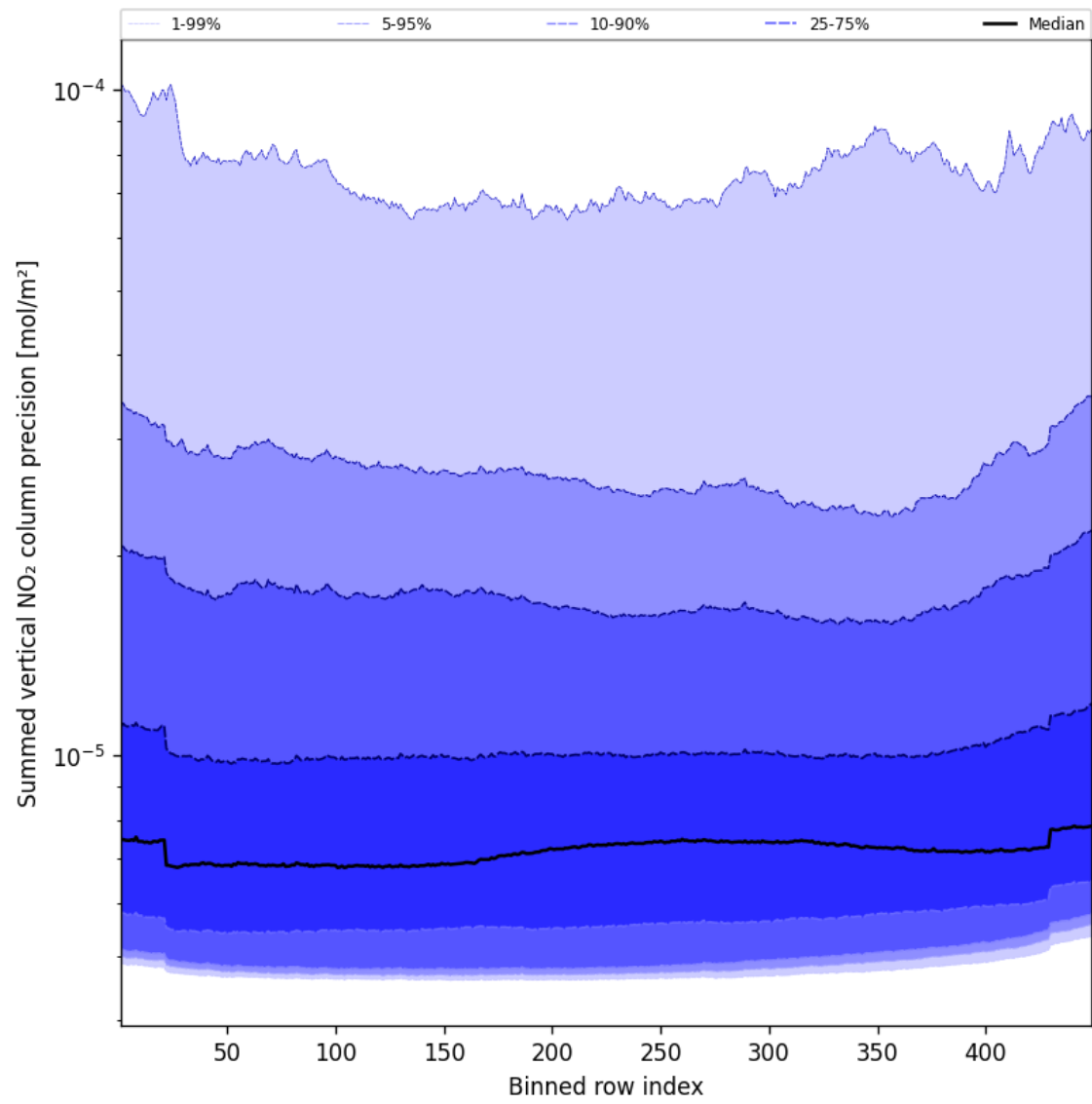
Figure 58: Along track statistics of “Summed vertical NO 2 column precision” for 2025-11-24 to 2025-11-26
