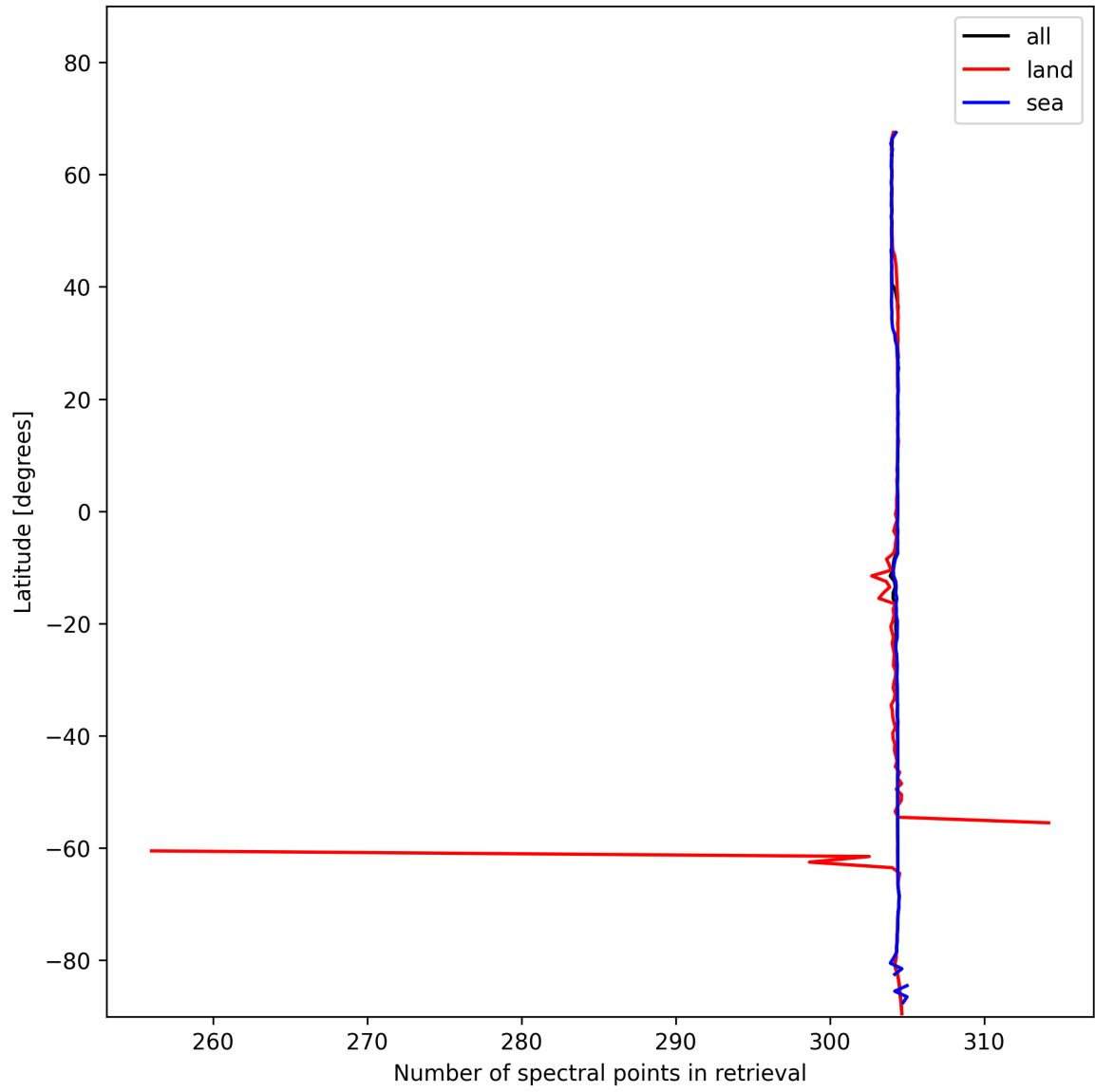
Figure 16: Zonal average of “Number of spectral points in retrieval” for 2025-11-24 to 2025-11-26.
