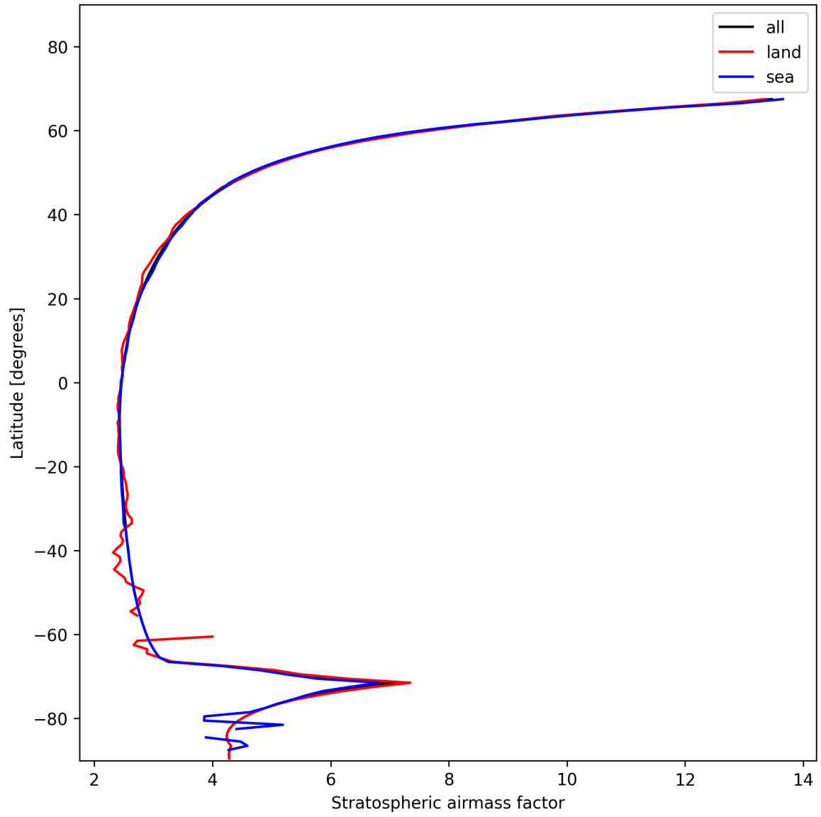
Figure 27: Zonal average of “Stratospheric air mass factor” for 2025-11-24 to 2025-11-26.
