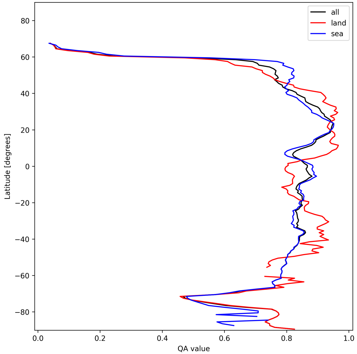
Figure 11: Zonal average of “QA value” for 2025-11-24 to 2025-11-26.
