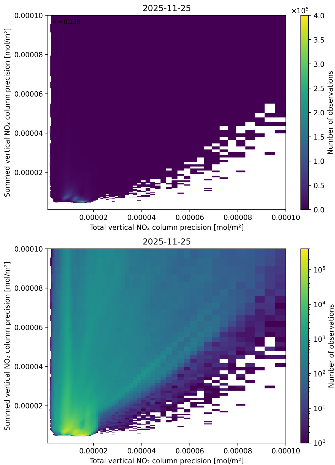
Figure 118: Scatter density plot of “Total vertical NO 2 column precision” against “Summed vertical NO 2 column precision” for 2025-11-24 to 2025-11-26.
