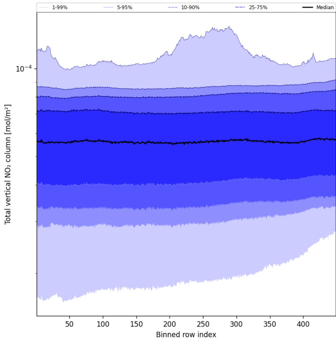
Figure 55: Along track statistics of “Total vertical NO 2 column” for 2025-11-24 to 2025-11-26
