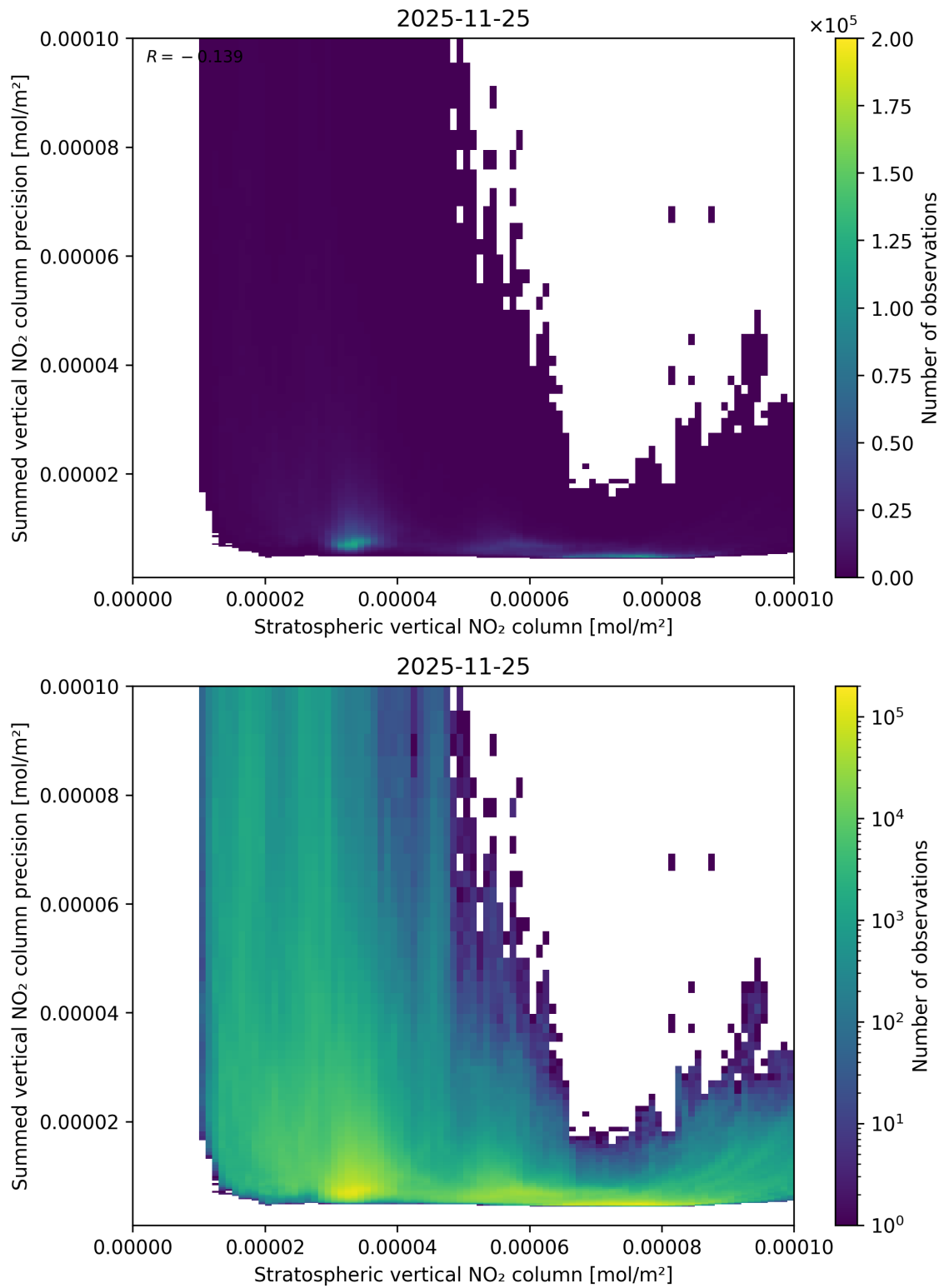
Figure 99: Scatter density plot of “Stratospheric vertical NO 2 column” against “Summed vertical NO 2 column precision” for 2025-11-24 to 2025-11-26.
