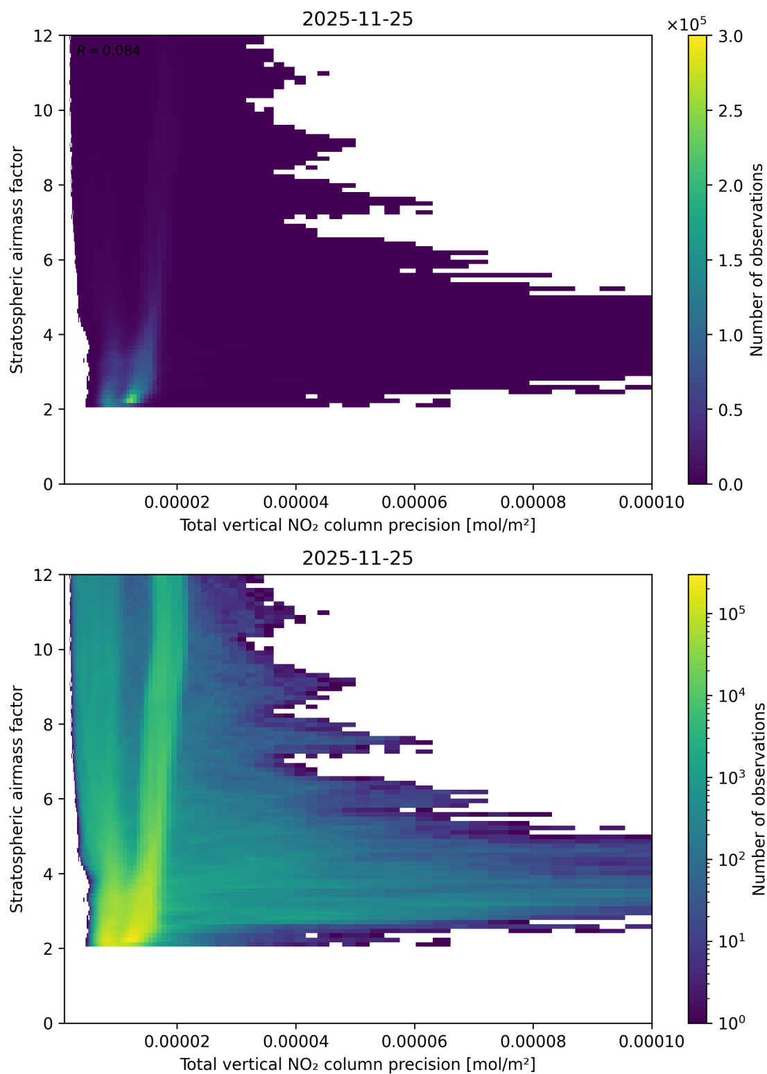
Figure 115: Scatter density plot of “Total vertical NO 2 column precision” against “Stratospheric air mass factor” for 2025-11-24 to 2025-11-26.
