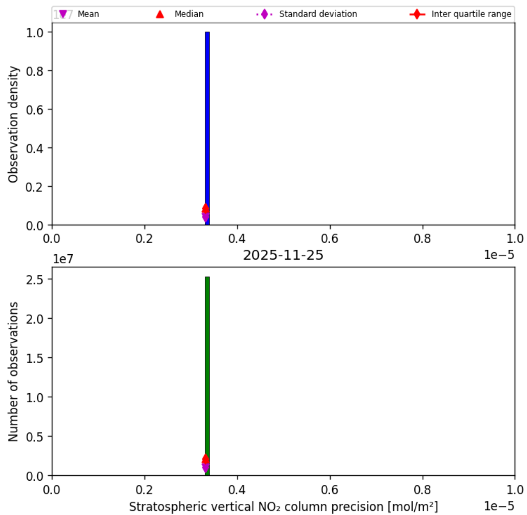
Figure 37: Histogram of “Stratospheric vertical NO 2 column precision” for 2025-11-24 to 2025-11-26
