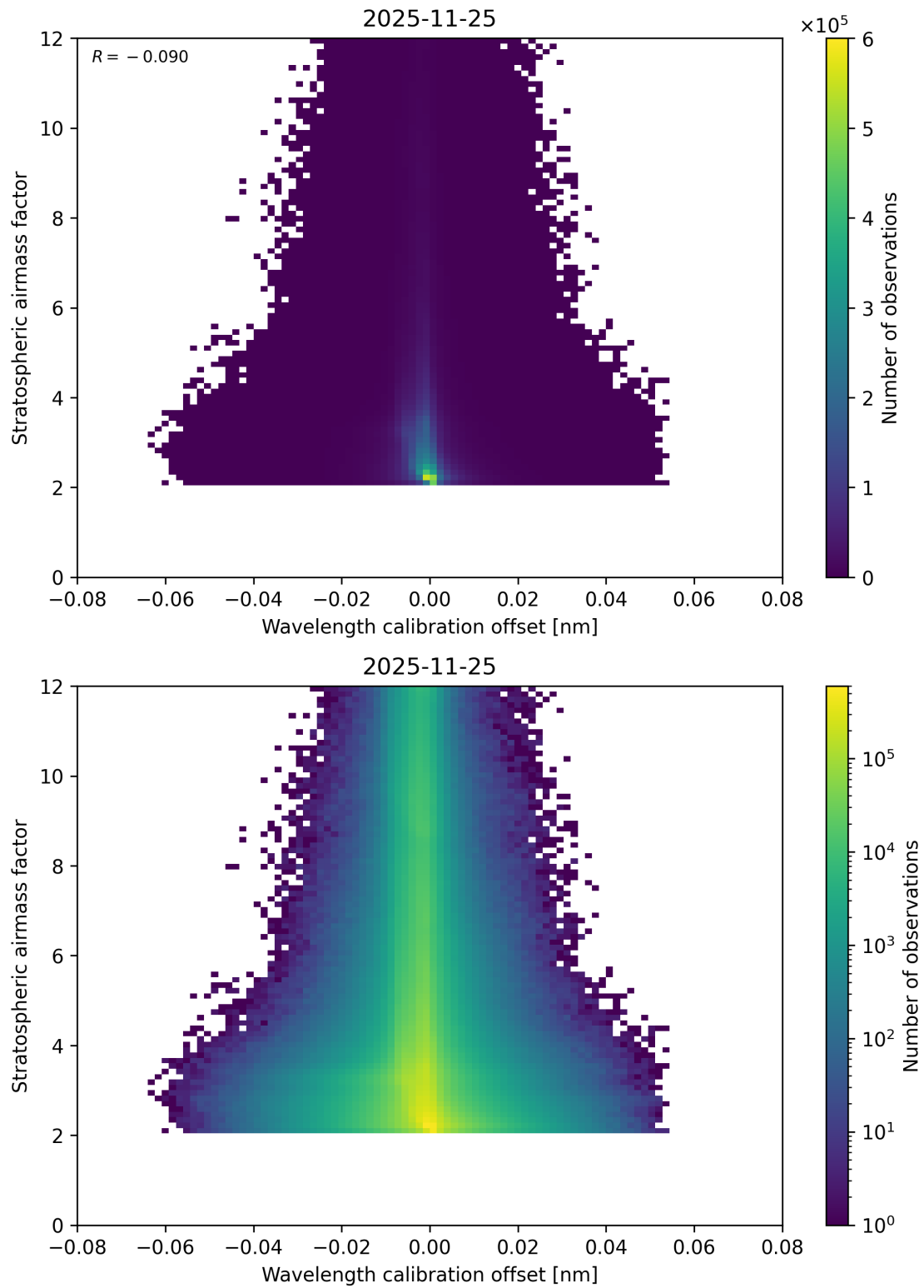
Figure 174: Scatter density plot of “Wavelength calibration offset” against “Stratospheric airmass factor” for 2025-11-24 to 2025-11-26.
