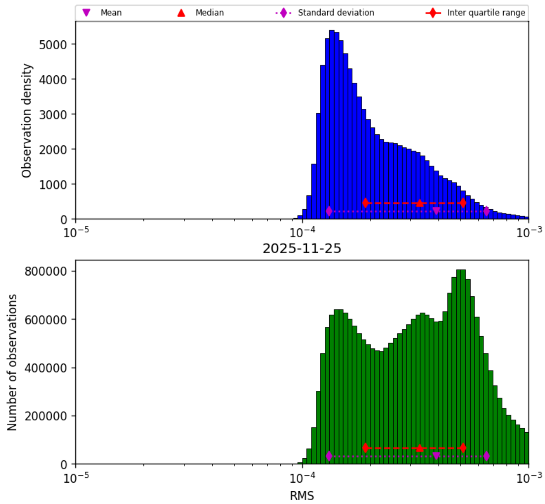
Figure 43: Histogram of “RMS” for 2025-11-24 to 2025-11-26
