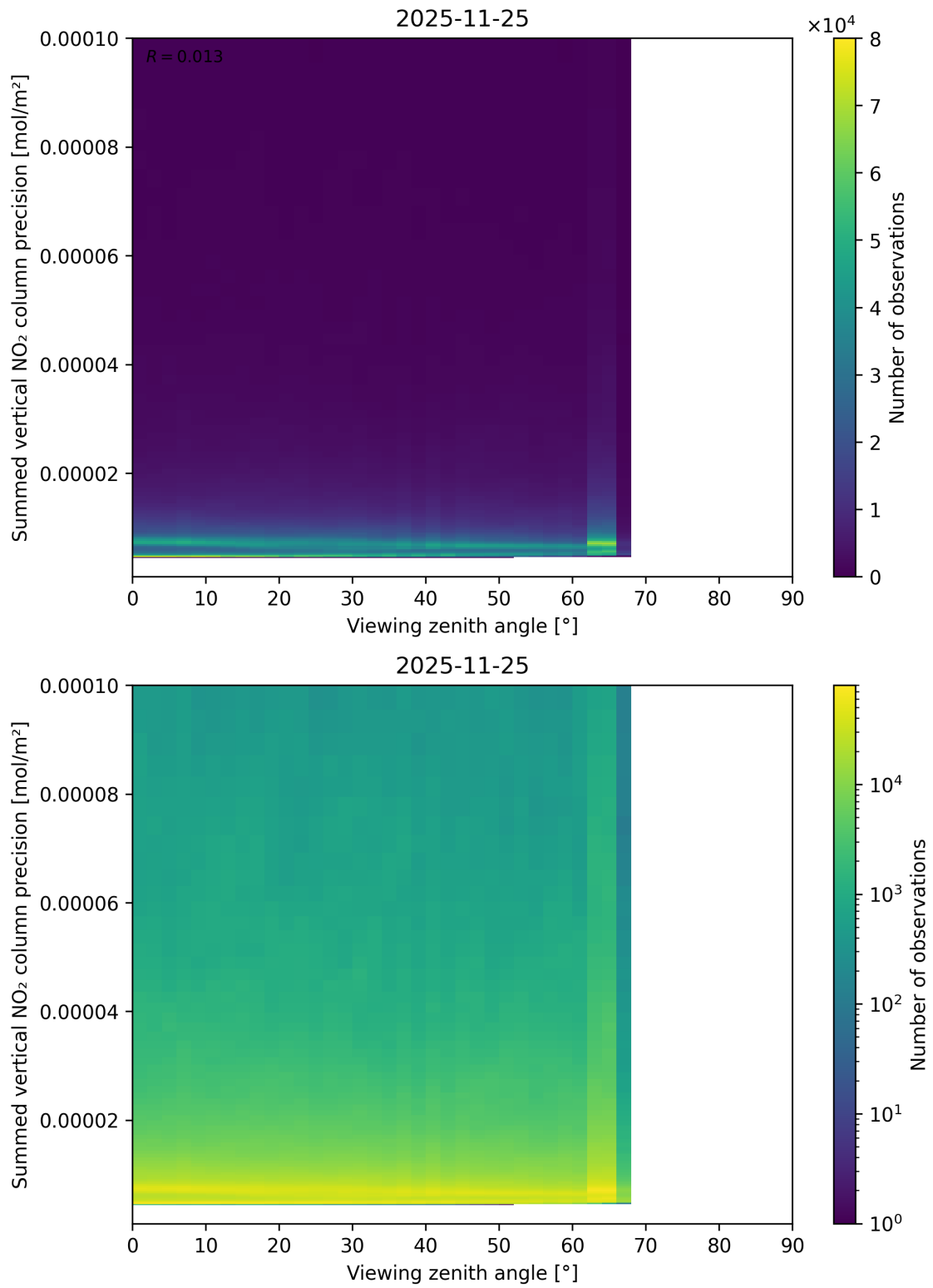
Figure 166: Scatter density plot of “Viewing zenith angle” against “Summed vertical NO 2 column precision” for 2025-11-24 to 2025-11-26.
