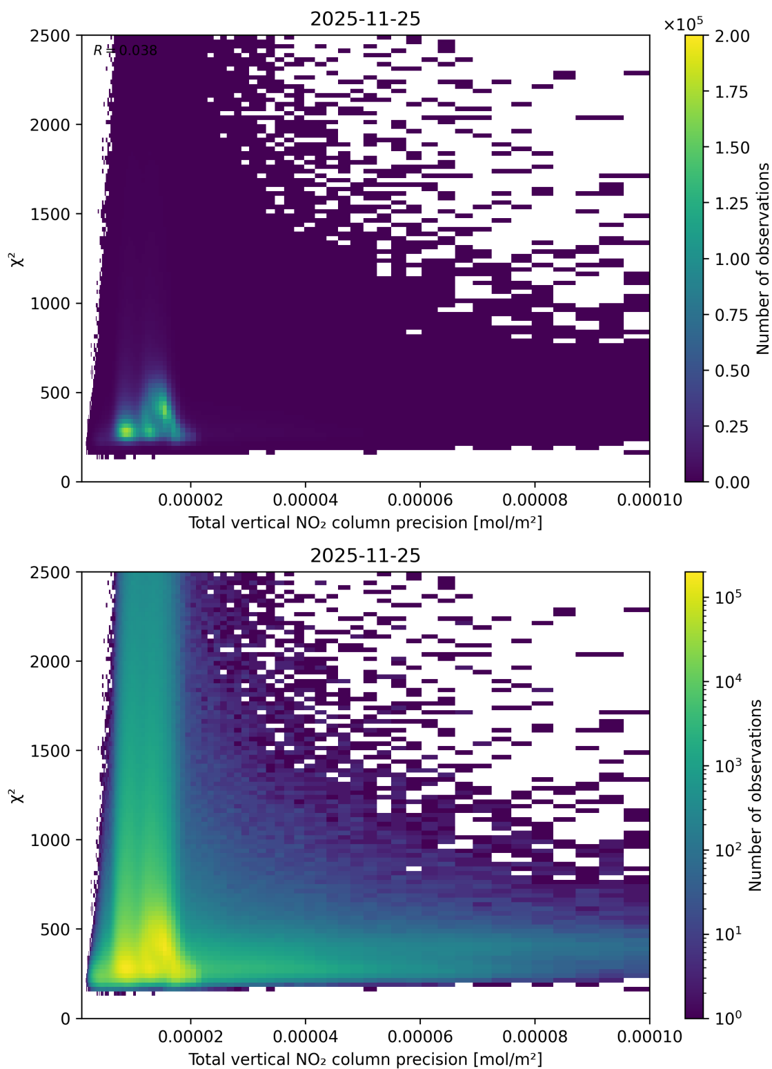
Figure 116: Scatter density plot of “Total vertical NO 2 column precision” against “ \chi^2 ” for 2025-11-24 to 2025-11-26.
