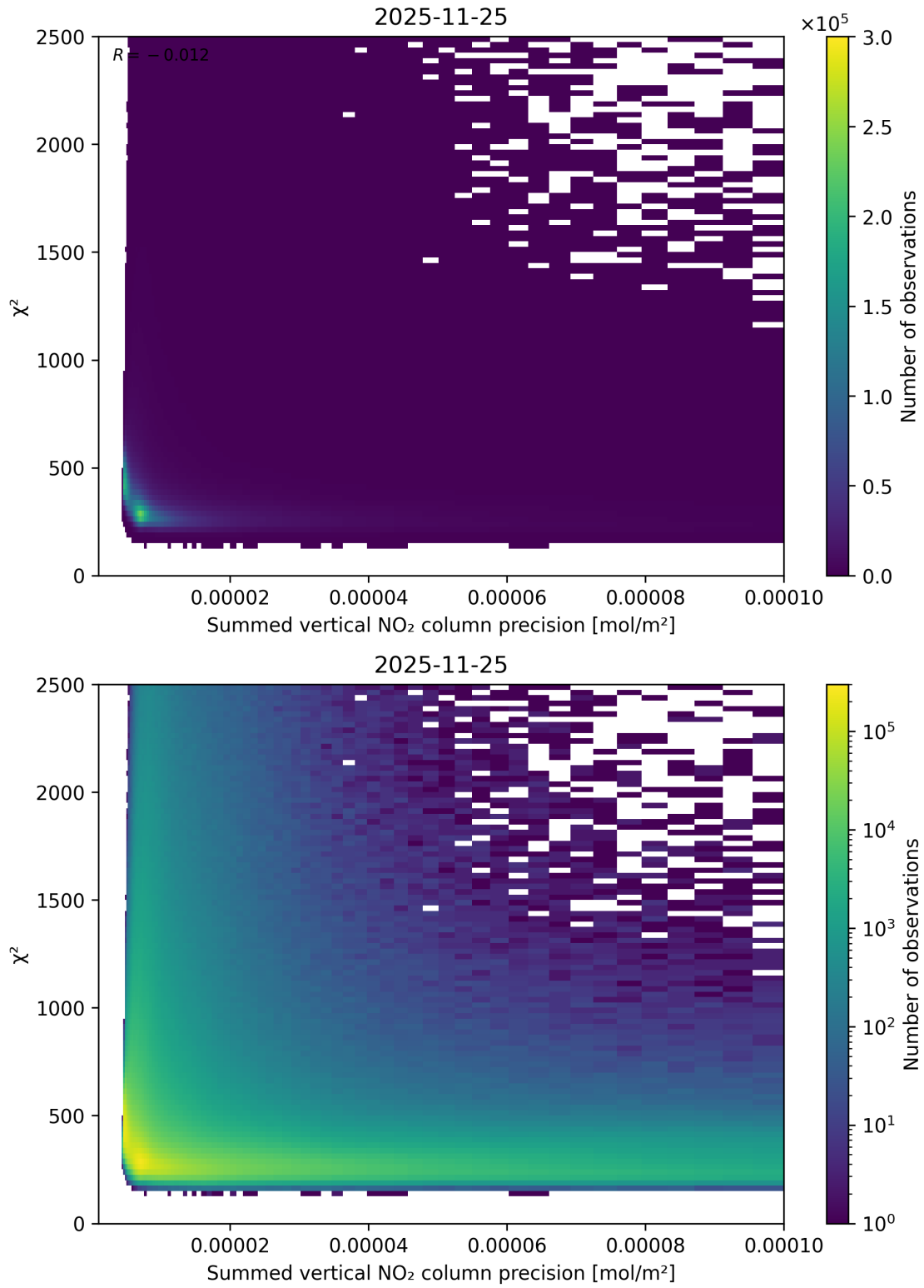
Figure 107: Scatter density plot of “Summed vertical NO 2 column precision” against “ \chi^2 ” for 2025-11-24 to 2025-11-26.
