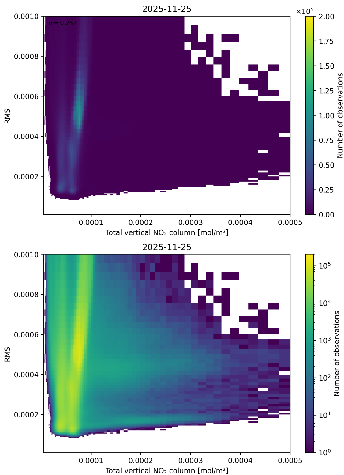
Figure 120: Scatter density plot of “Total vertical NO 2 column” against “RMS” for 2025-11-24 to 2025-11-26.
