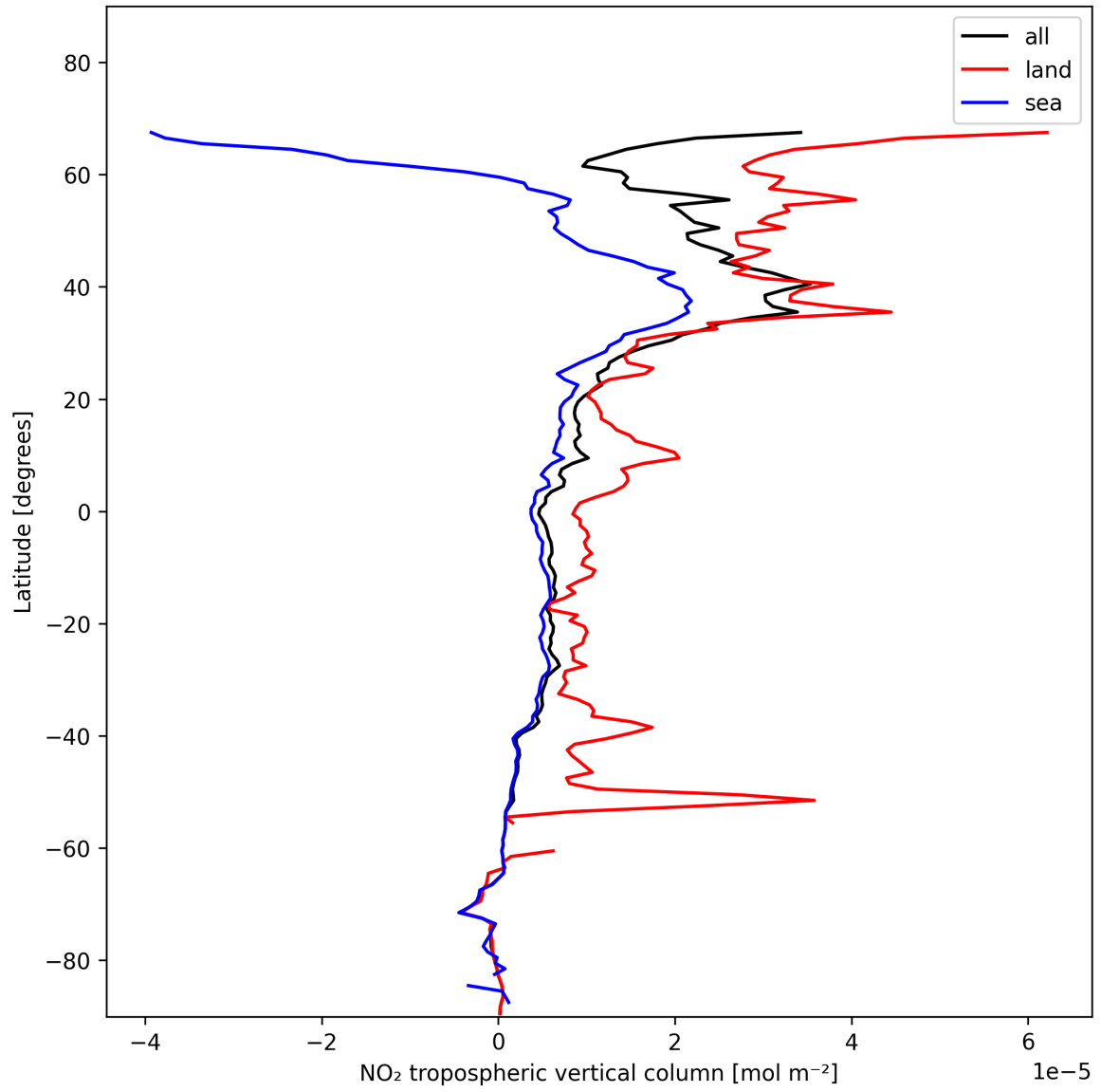
Figure 12: Zonal average of “NO 2 tropospheric vertical column” for 2025-11-24 to 2025-11-26.
