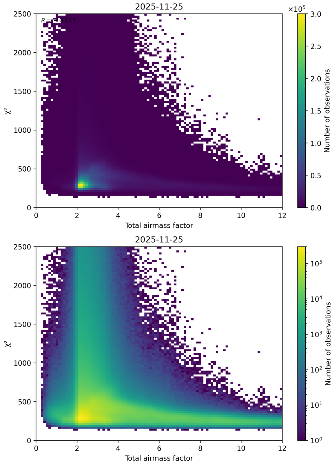
Figure 63: Scatter density plot of “Total airmass factor” against “ \chi^2 ” for 2025-11-24 to 2025-11-26.
