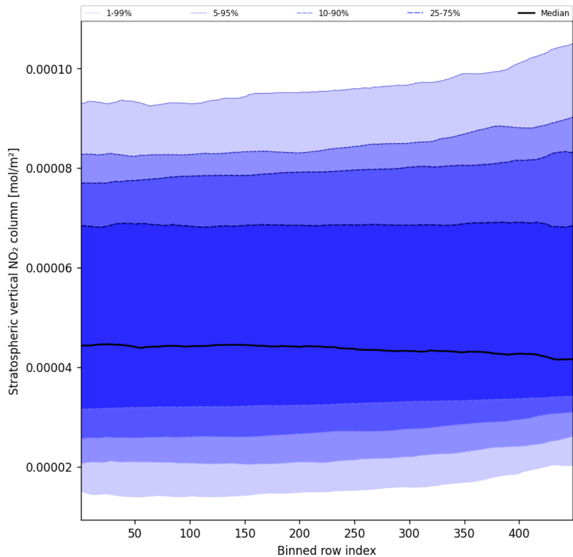
Figure 53: Along track statistics of “Stratospheric vertical NO 2 column” for 2025-11-24 to 2025-11-26
