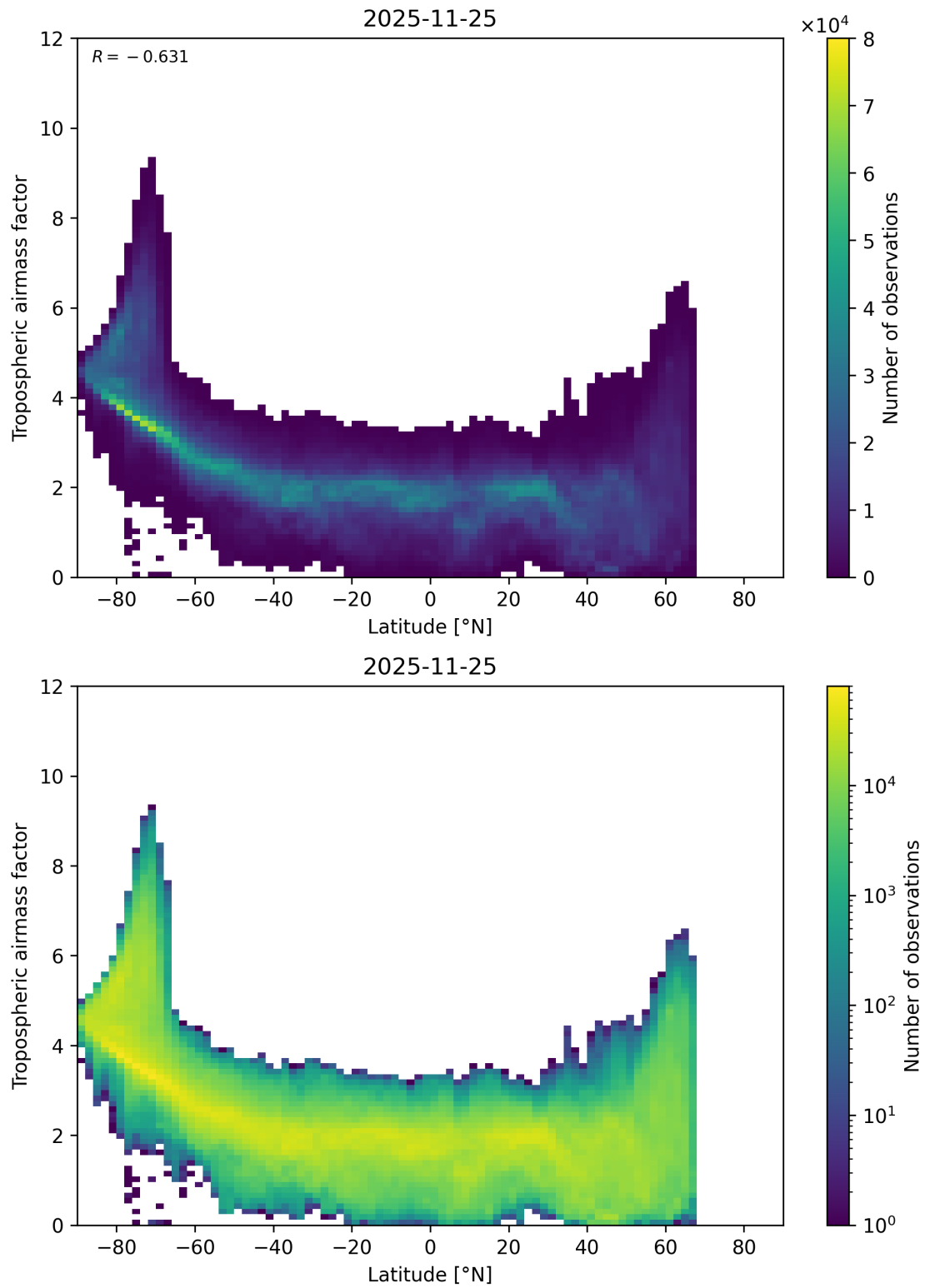
Figure 85: Scatter density plot of “Latitude” against “Tropospheric airmass factor” for 2025-11-24 to 2025-11-26.
