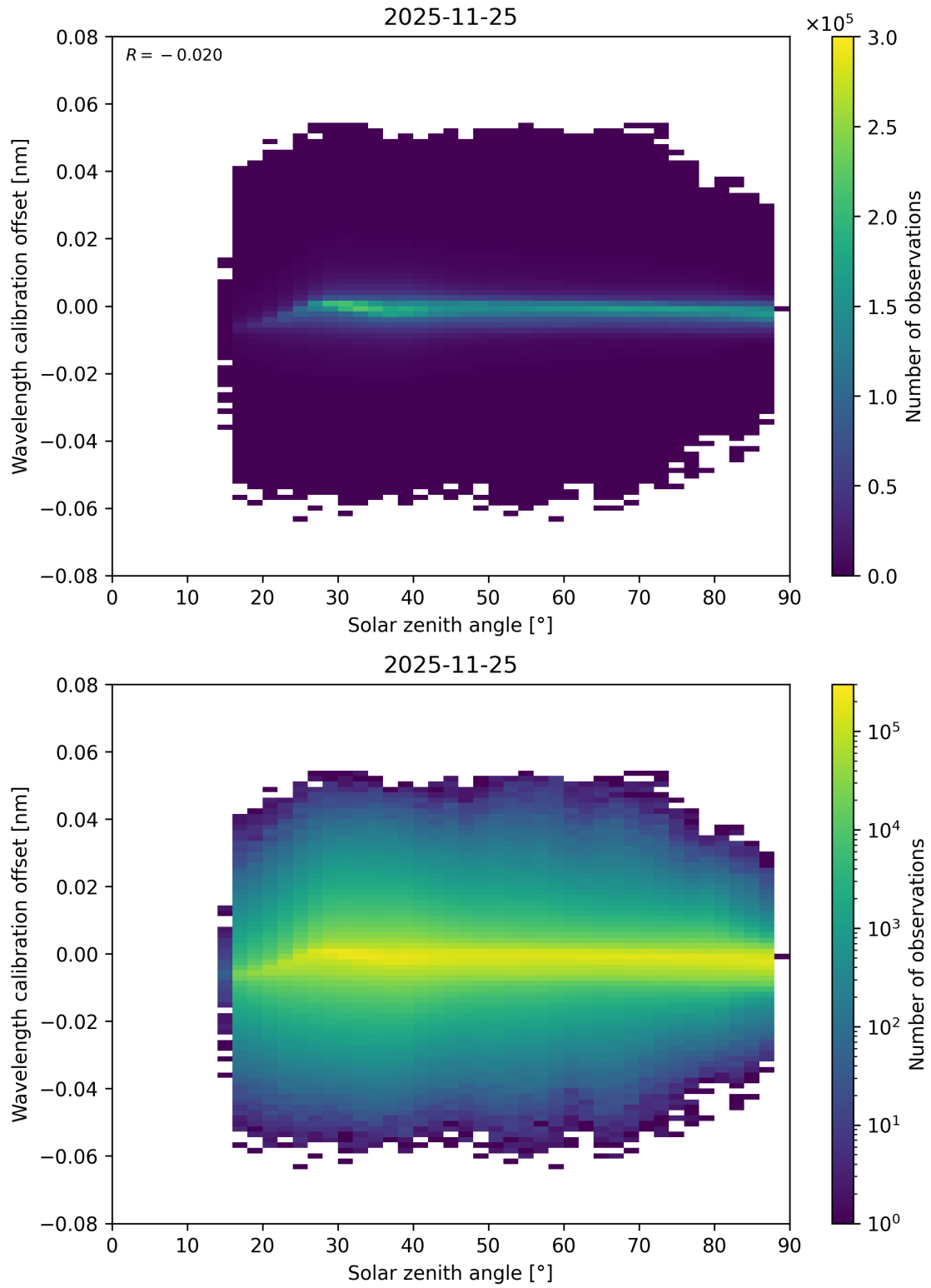
Figure 158: Scatter density plot of “Solar zenith angle” against “Wavelength calibration offset” for 2025-11-24 to 2025-11-26.
