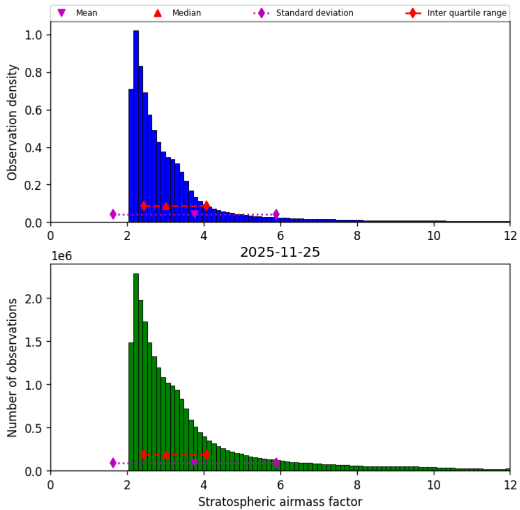
Figure 44: Histogram of “Stratospheric airmass factor” for 2025-11-24 to 2025-11-26
