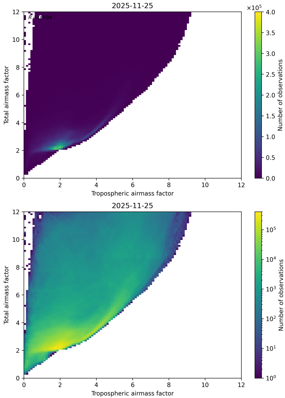
Figure 72: Scatter density plot of “Tropospheric airmass factor” against “Total airmass factor” for 2025-11-24 to 2025-11-26.
