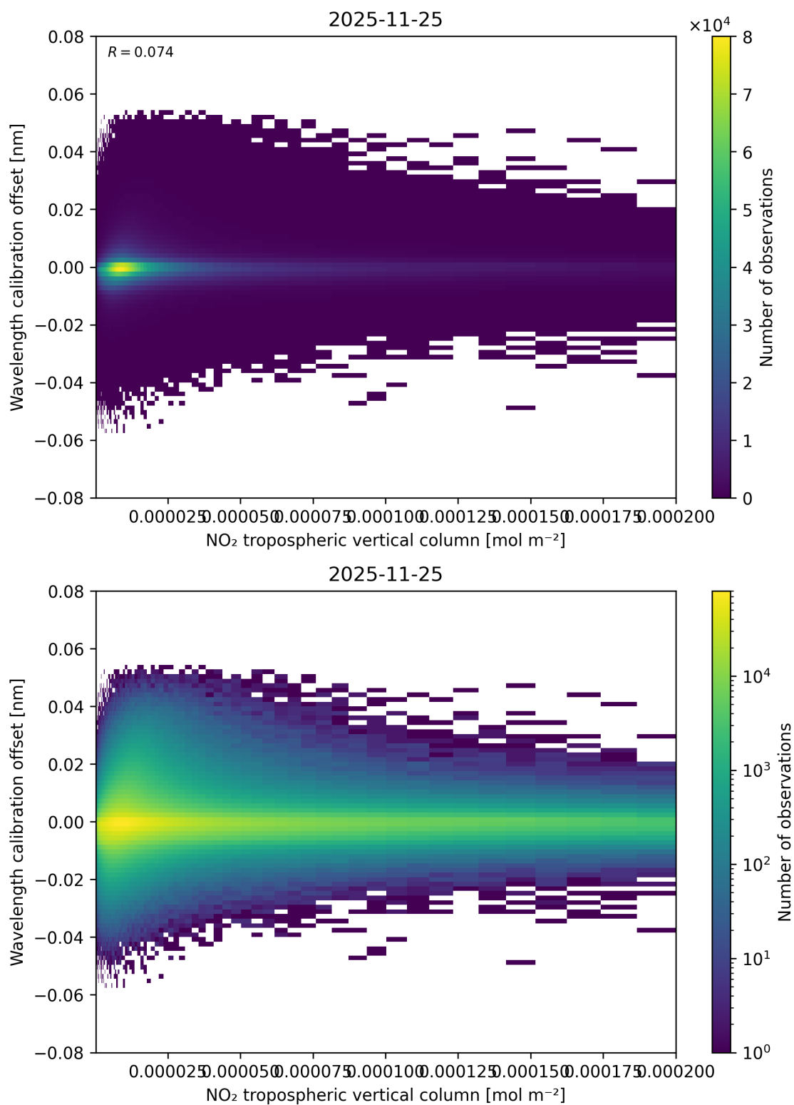
Figure 143: Scatter density plot of “NO 2 tropospheric vertical column” against “Wavelength calibration offset” for 2025-11-24 to 2025-11-26.
