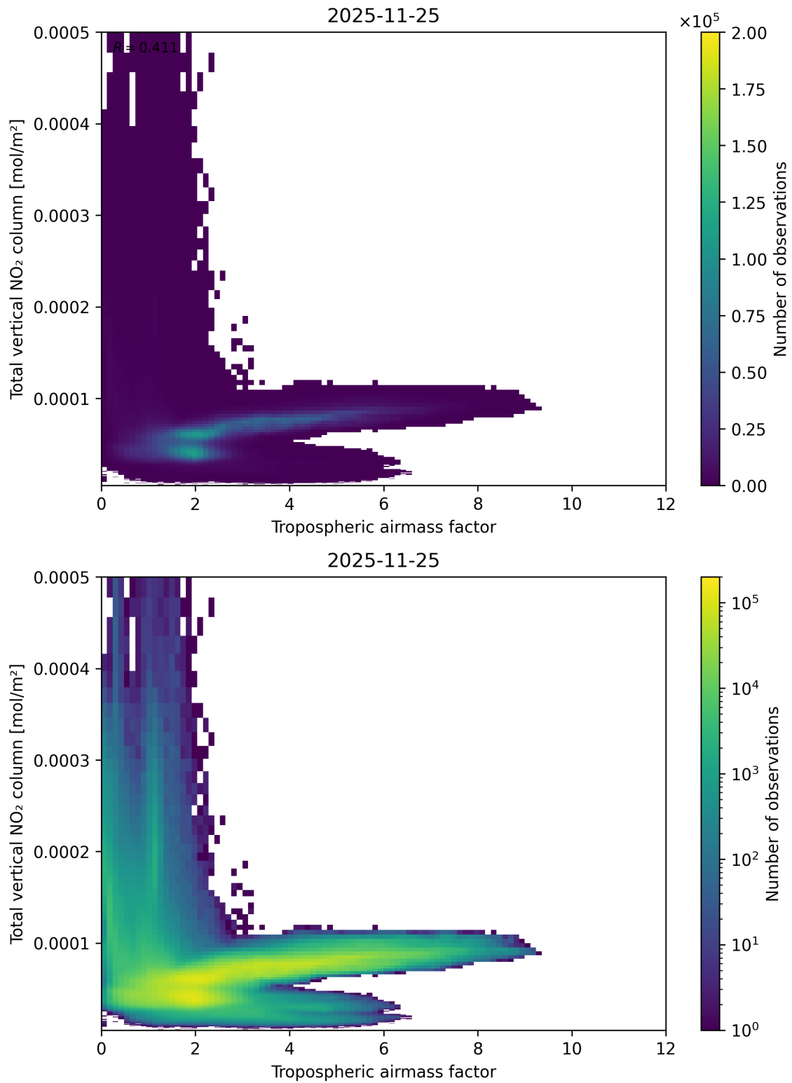
Figure 77: Scatter density plot of “Tropospheric airmass factor” against “Total vertical NO 2 column” for 2025-11-24 to 2025-11-26.
