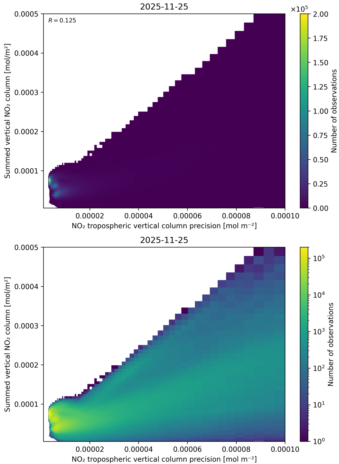
Figure 136: Scatter density plot of “NO 2 tropospheric vertical column precision” against “Summed vertical NO 2 column” for 2025-11-24 to 2025-11-26.
