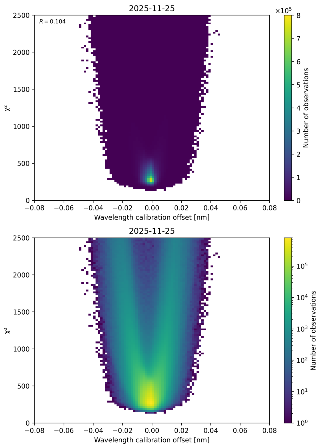
Figure 175: Scatter density plot of “Wavelength calibration offset” against “ \chi^2 ” for 2025-11-24 to 2025-11-26.
