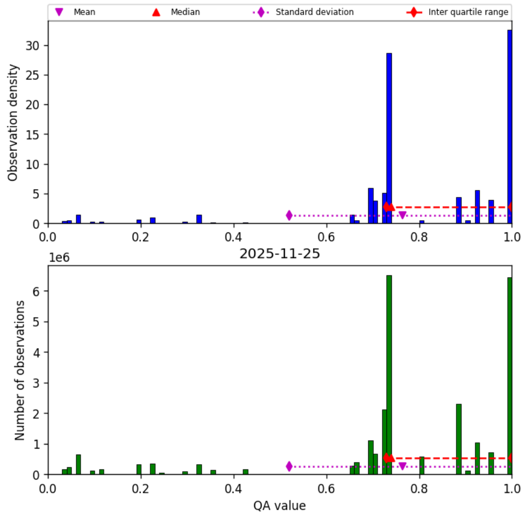
Figure 28: Histogram of “QA value” for 2025-11-24 to 2025-11-26
