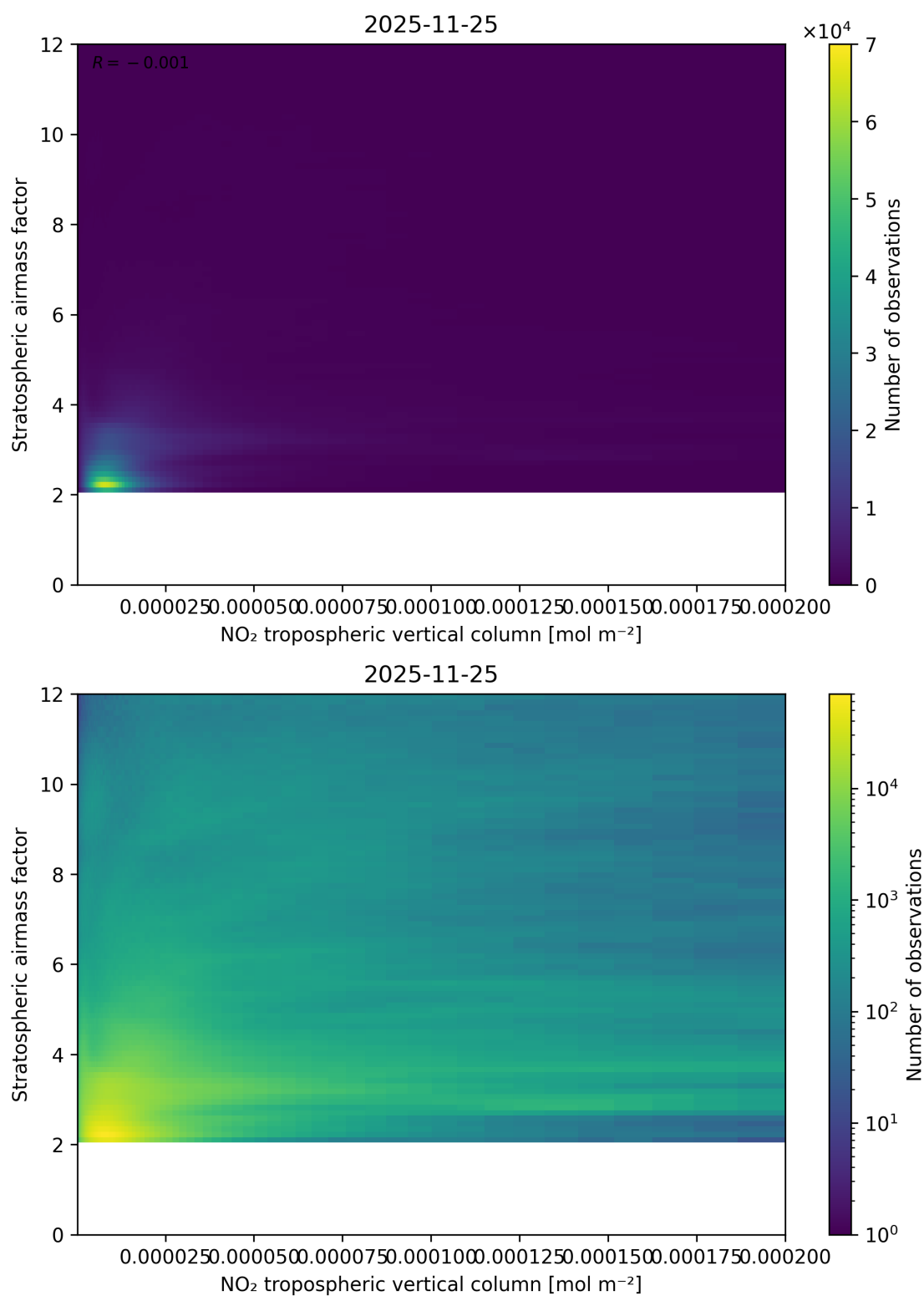
Figure 121: Scatter density plot of “NO 2 tropospheric vertical column” against “Stratospheric airmass factor” for 2025-11-24 to 2025-11-26.
