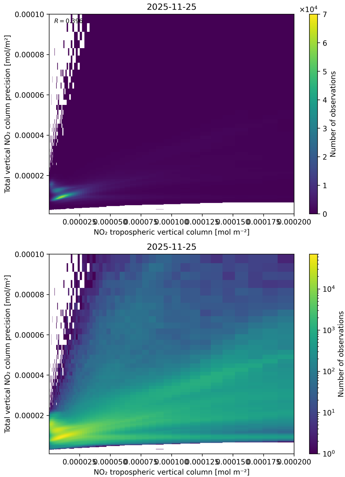
Figure 129: Scatter density plot of “NO 2 tropospheric vertical column” against “Total vertical NO 2 column precision” for 2025-11-24 to 2025-11-26.
