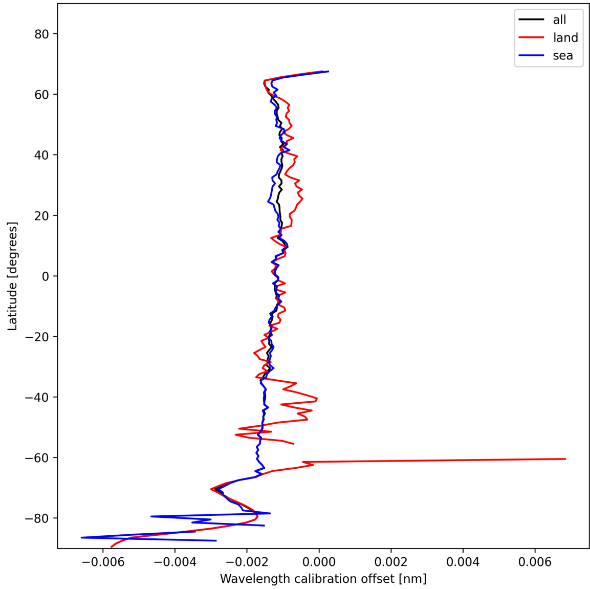
Figure 18: Zonal average of “Wavelength calibration offset” for 2025-11-24 to 2025-11-26.
