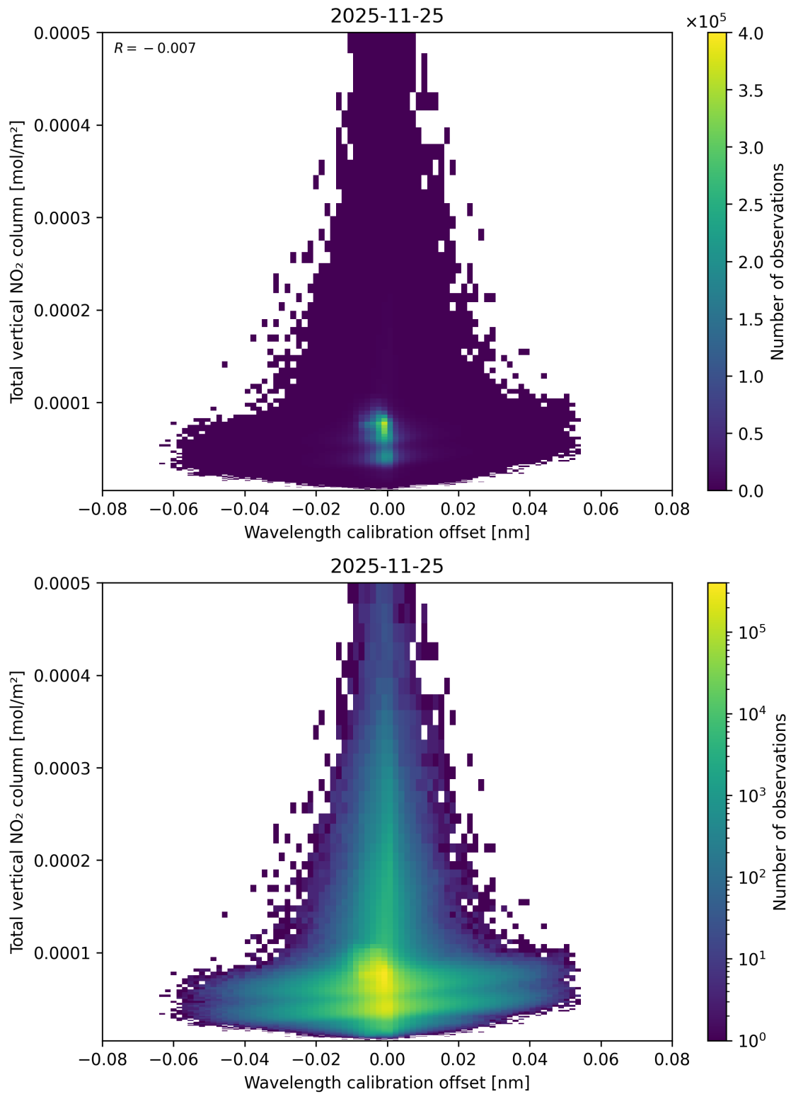
Figure 179: Scatter density plot of “Wavelength calibration offset” against “Total vertical NO 2 column” for 2025-11-24 to 2025-11-26.
