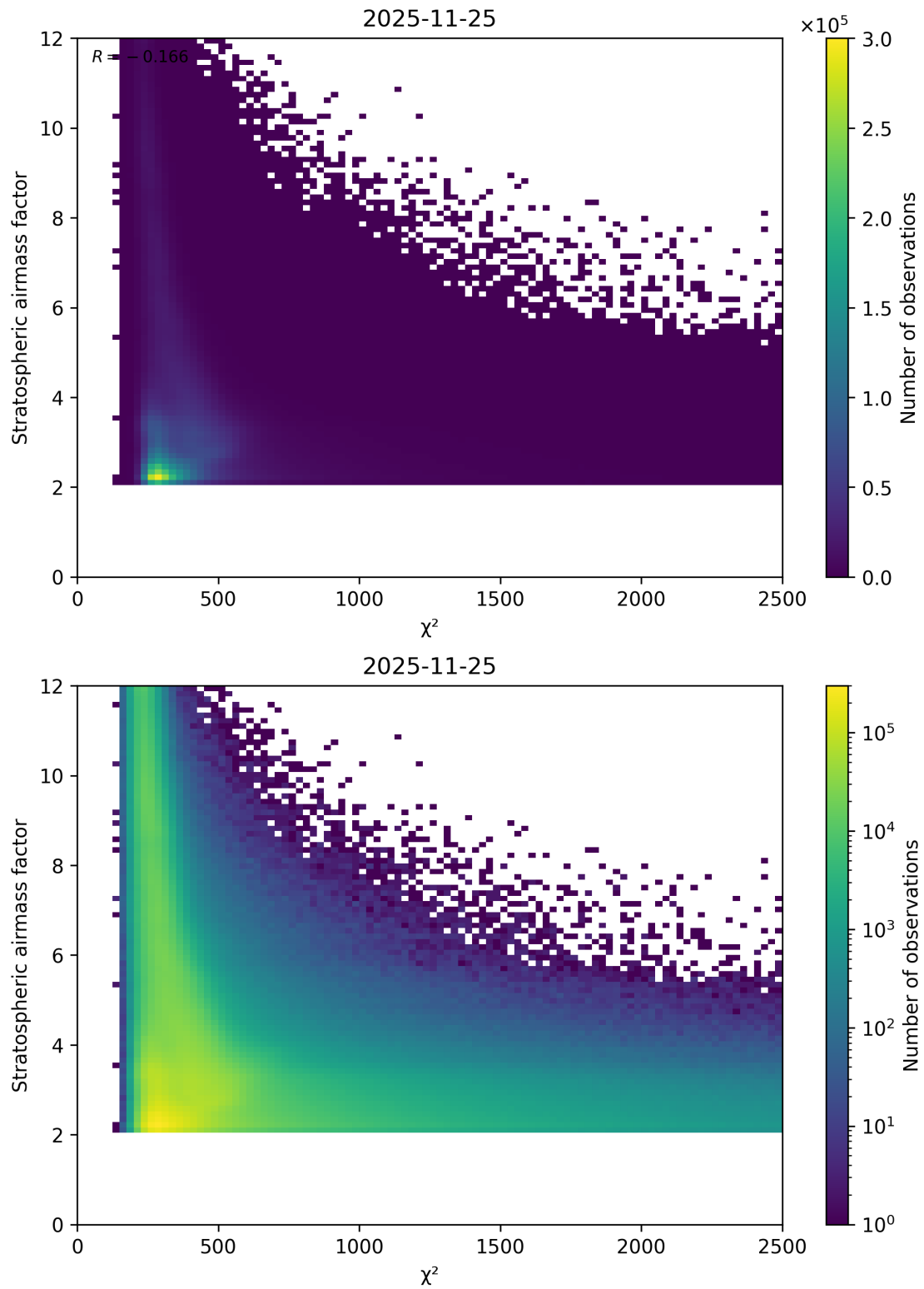
Figure 81: Scatter density plot of “ \chi^2 ” against “Stratospheric airmass factor” for 2025-11-24 to 2025-11-26.
