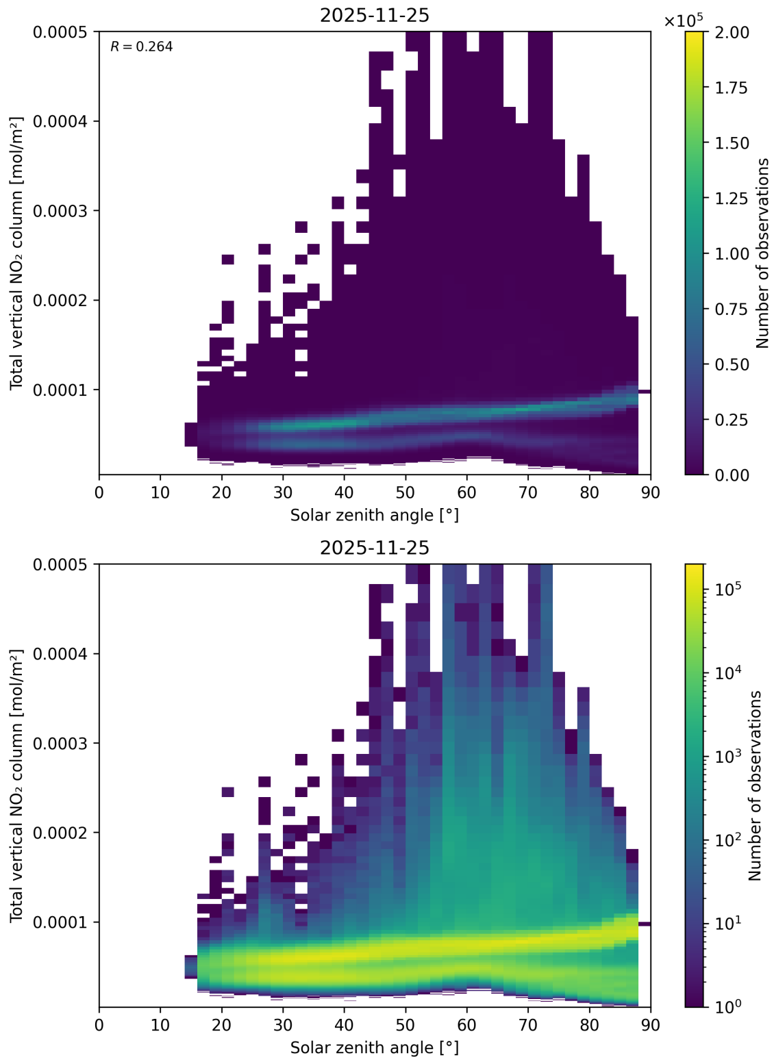
Figure 153: Scatter density plot of “Solar zenith angle” against “Total vertical NO 2 column” for 2025-11-24 to 2025-11-26.
