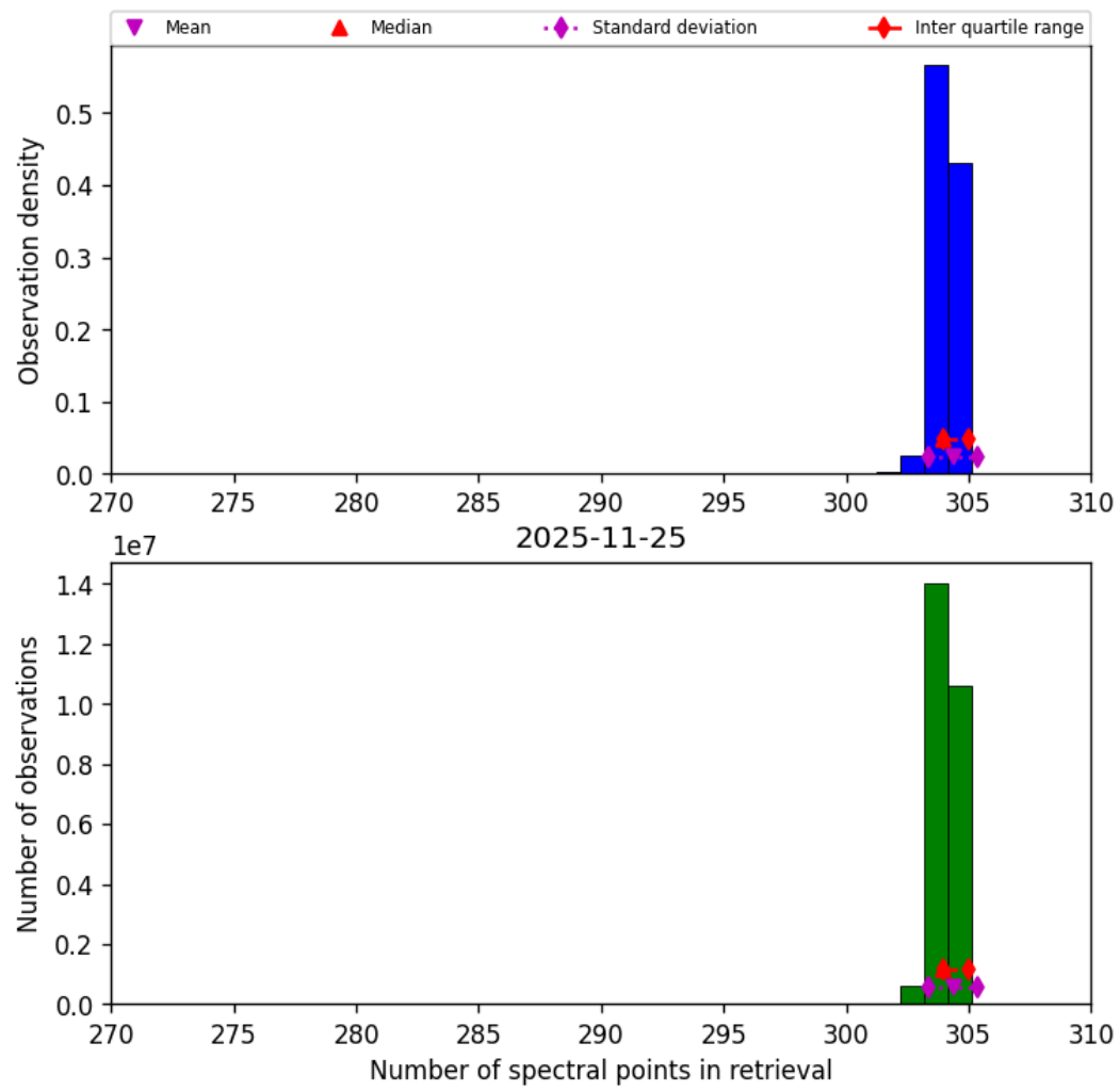
Figure 33: Histogram of “Number of spectral points in retrieval” for 2025-11-24 to 2025-11-26
