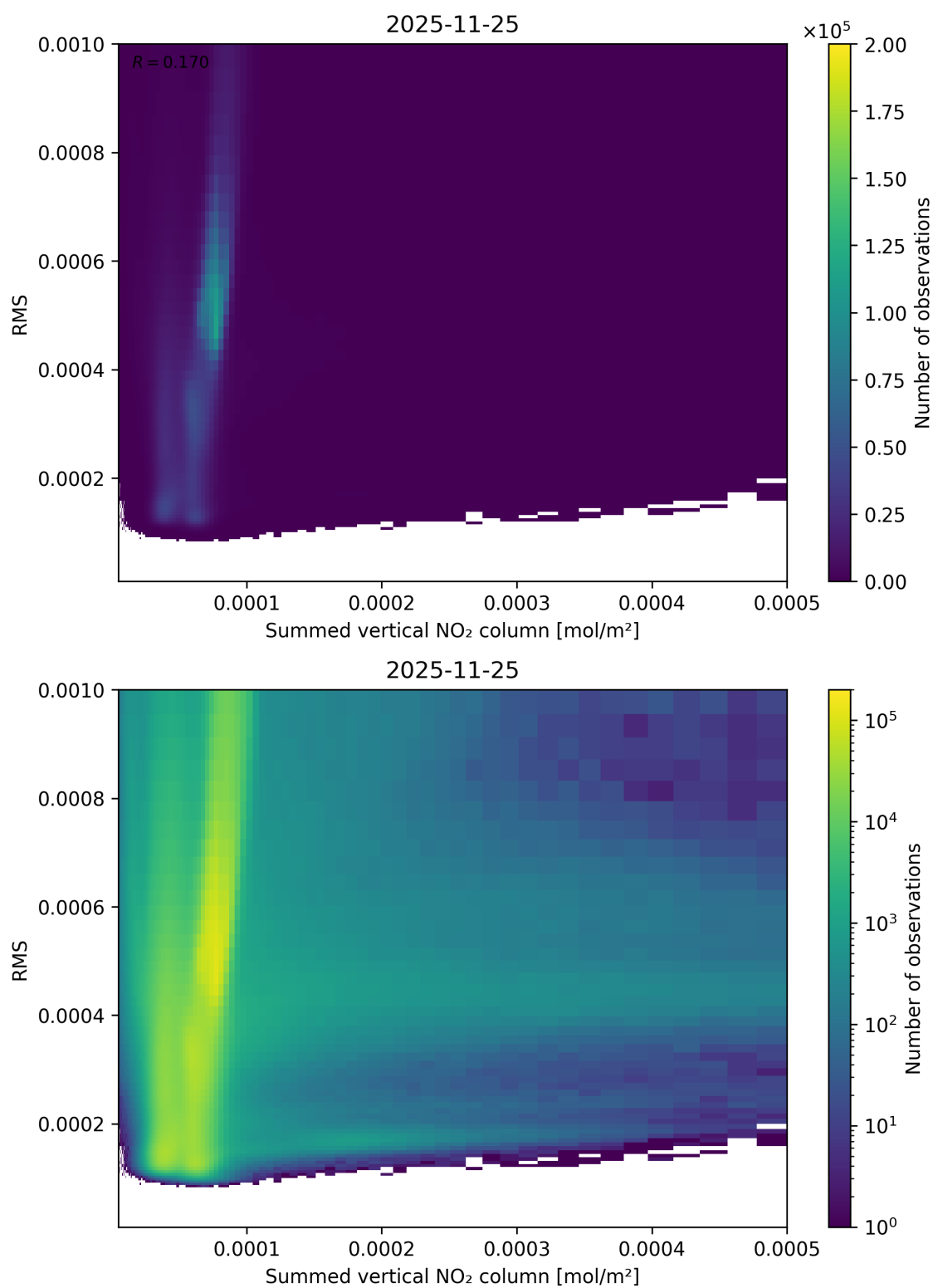
Figure 109: Scatter density plot of “Summed vertical NO 2 column” against “RMS” for 2025-11-24 to 2025-11-26.
