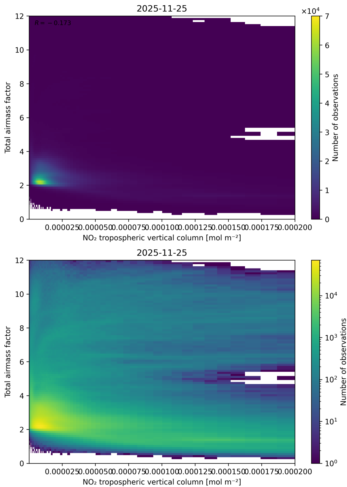
Figure 122: Scatter density plot of “NO 2 tropospheric vertical column” against “Total air mass factor” for 2025-11-24 to 2025-11-26.
