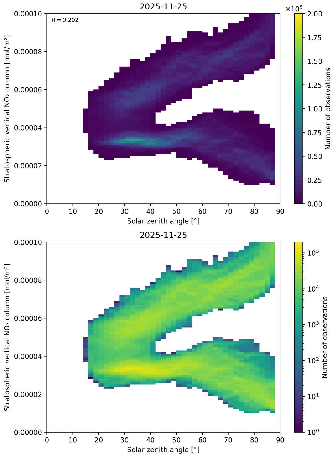
Figure 150: Scatter density plot of “Solar zenith angle” against “Stratospheric vertical NO 2 column” for 2025-11-24 to 2025-11-26.
