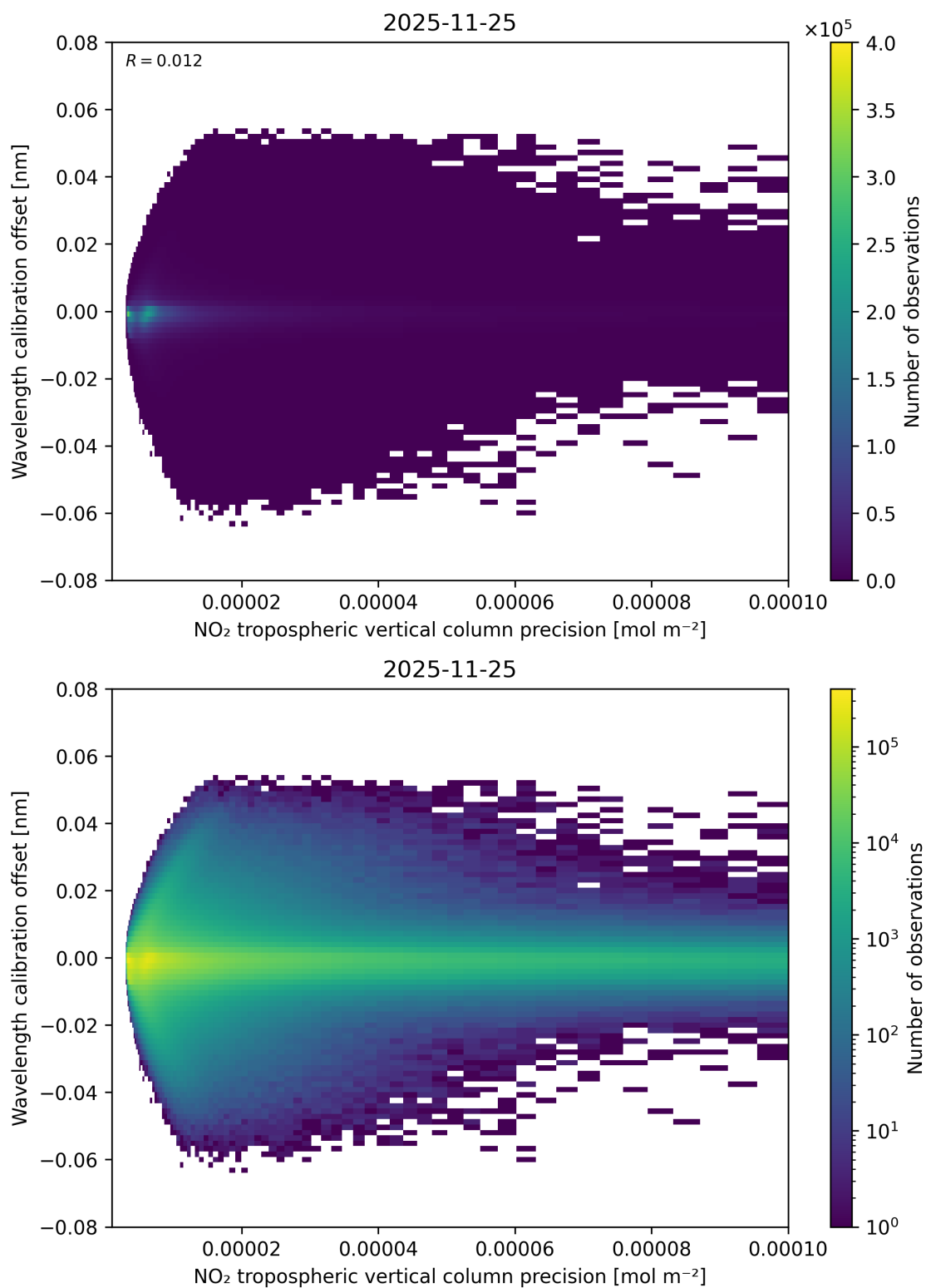
Figure 141: Scatter density plot of “NO 2 tropospheric vertical column precision” against “Wavelength calibration offset” for 2025-11-24 to 2025-11-26.
