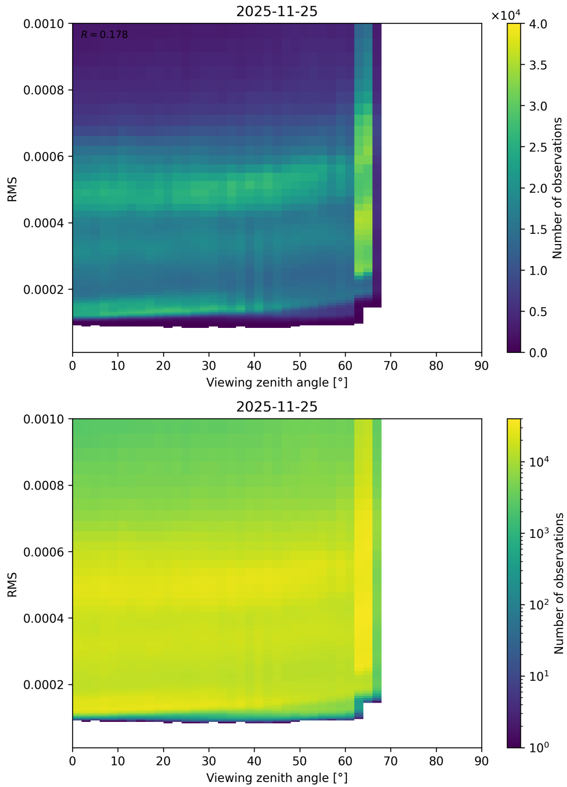
Figure 171: Scatter density plot of “Viewing zenith angle” against “RMS” for 2025-11-24 to 2025-11-26.
