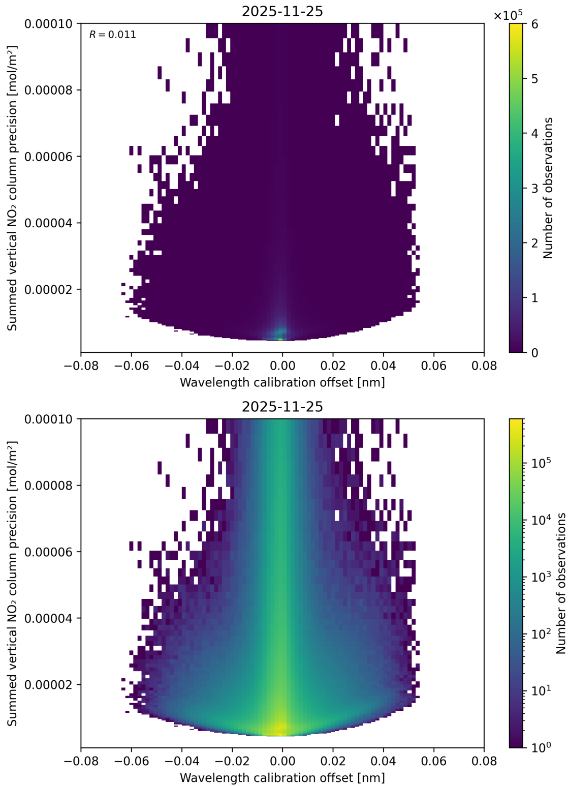
Figure 178: Scatter density plot of “Wavelength calibration offset” against “Summed vertical NO 2 column precision” for 2025-11-24 to 2025-11-26.
