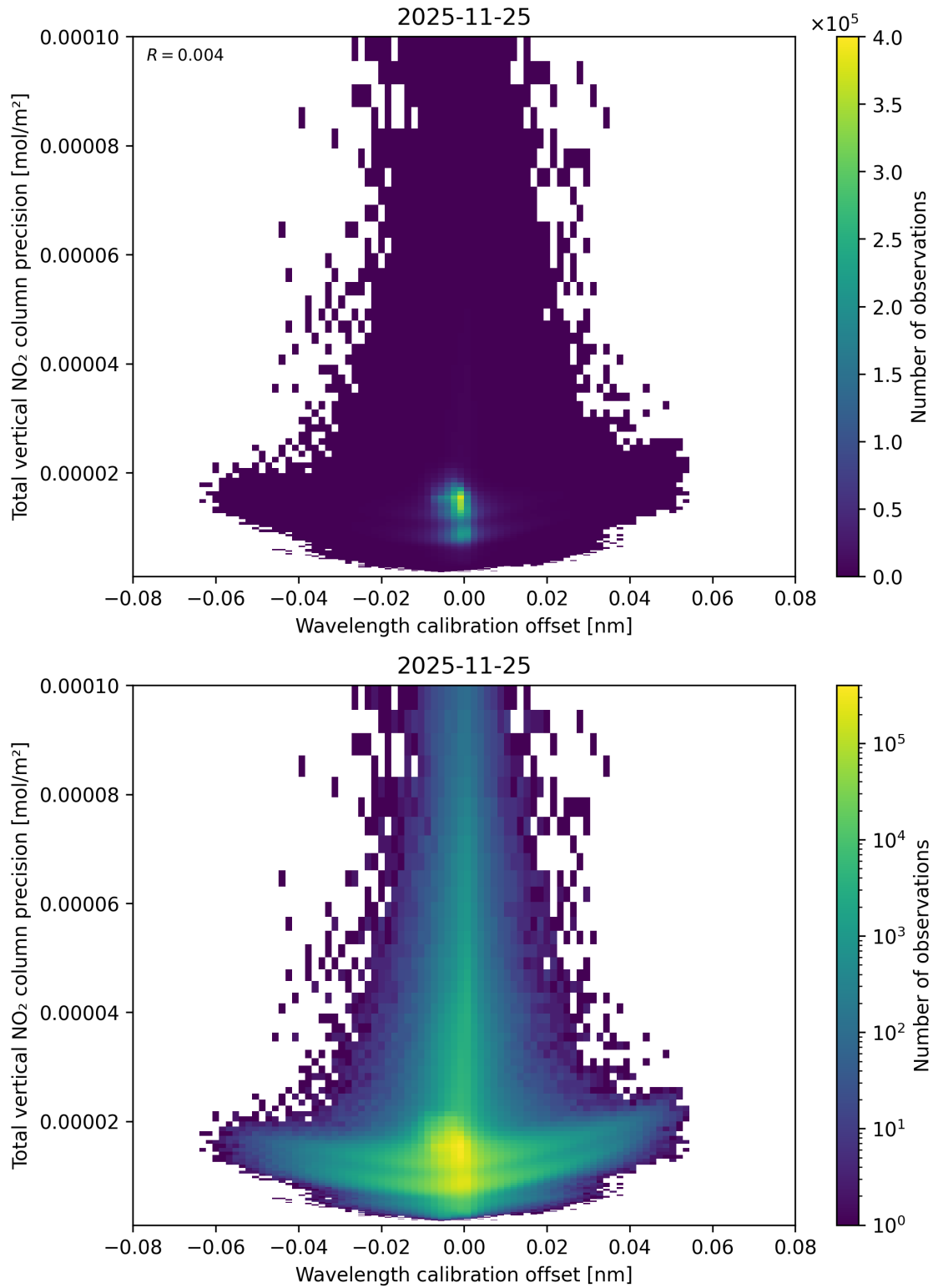
Figure 180: Scatter density plot of “Wavelength calibration offset” against “Total vertical NO 2 column precision” for 2025-11-24 to 2025-11-26.
