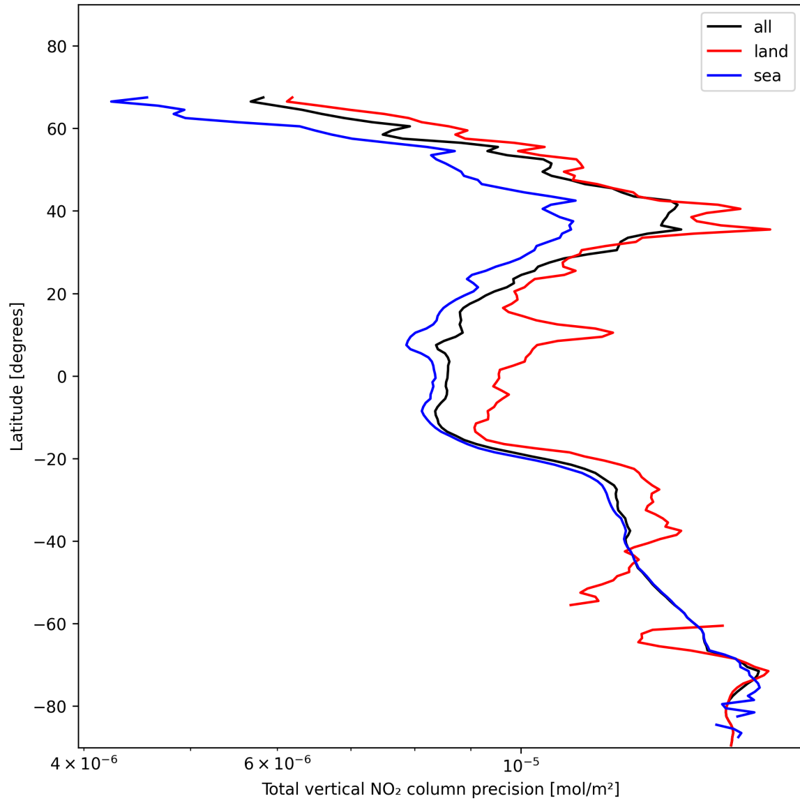
Figure 22: Zonal average of “Total vertical NO 2 column precision” for 2025-11-24 to 2025-11-26.
