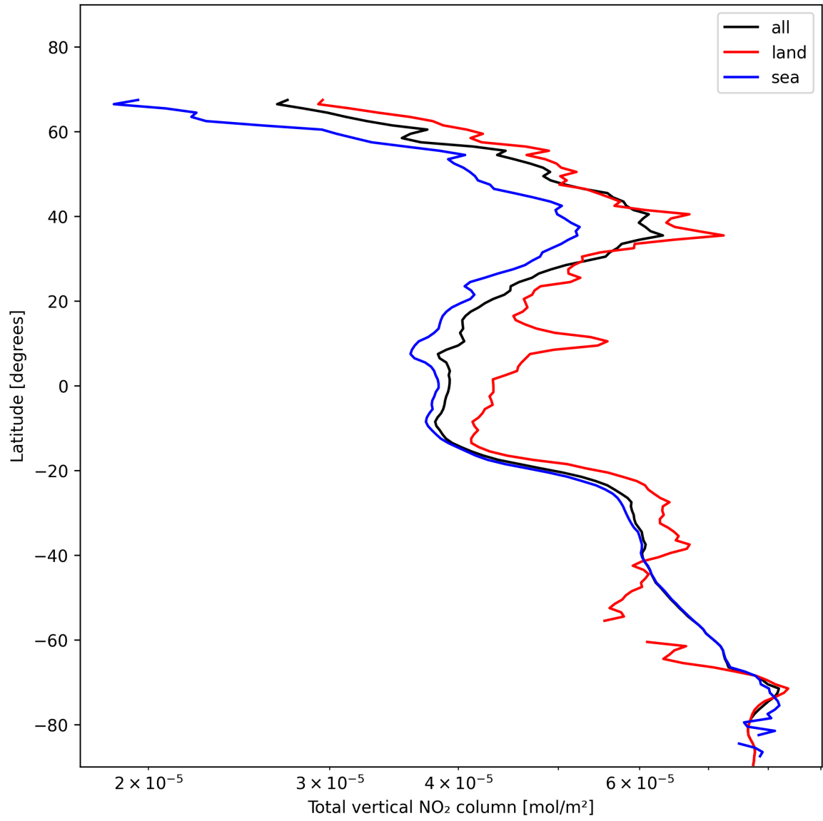
Figure 21: Zonal average of “Total vertical NO 2 column” for 2025-11-24 to 2025-11-26.
