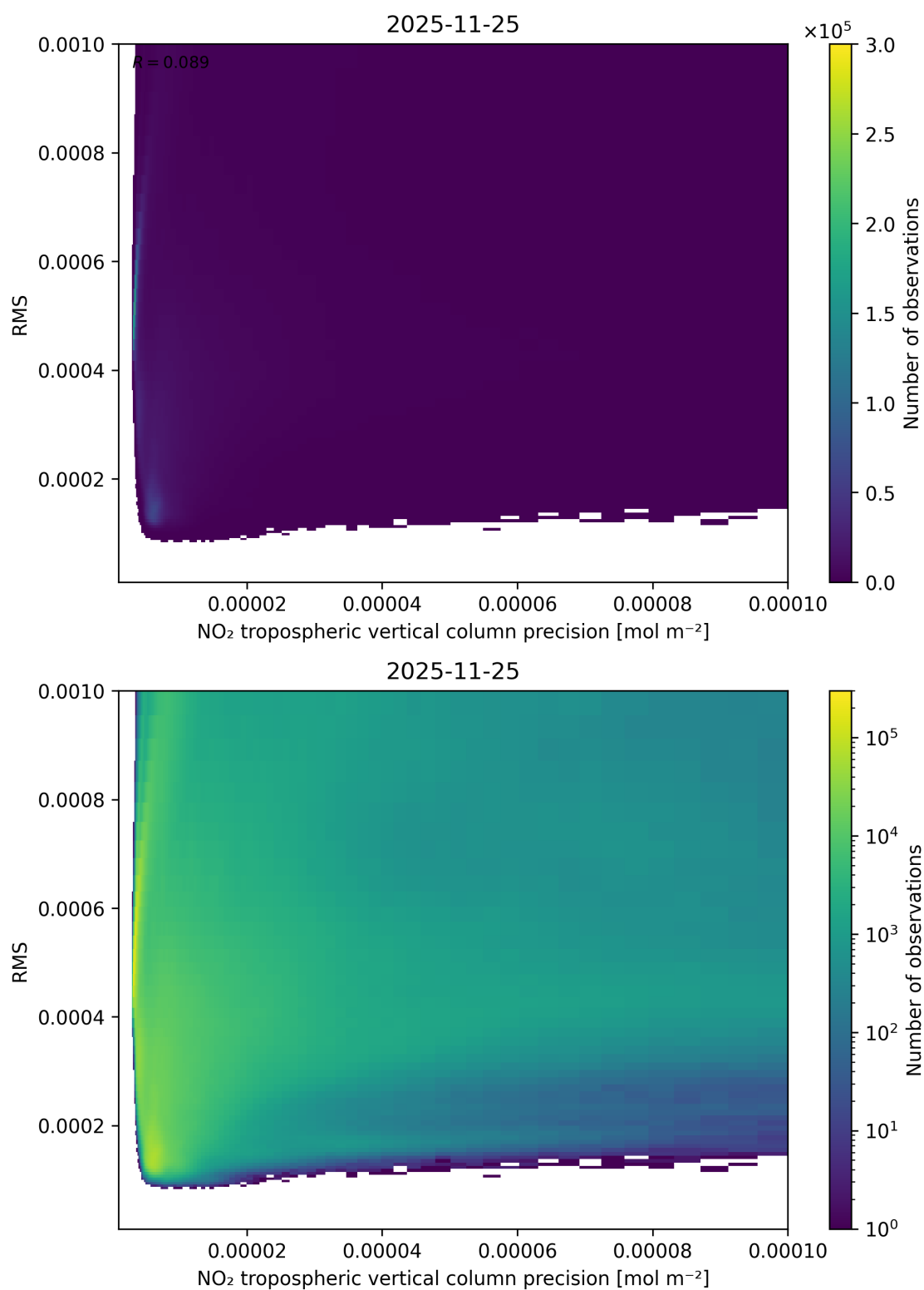
Figure 140: Scatter density plot of “NO 2 tropospheric vertical column precision” against “RMS” for 2025-11-24 to 2025-11-26.
