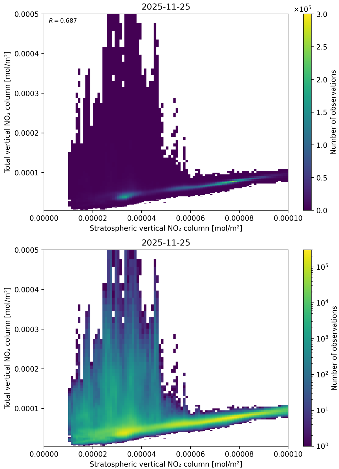
Figure 100: Scatter density plot of “Stratospheric vertical NO 2 column” against “Total vertical NO 2 column” for 2025-11-24 to 2025-11-26.
