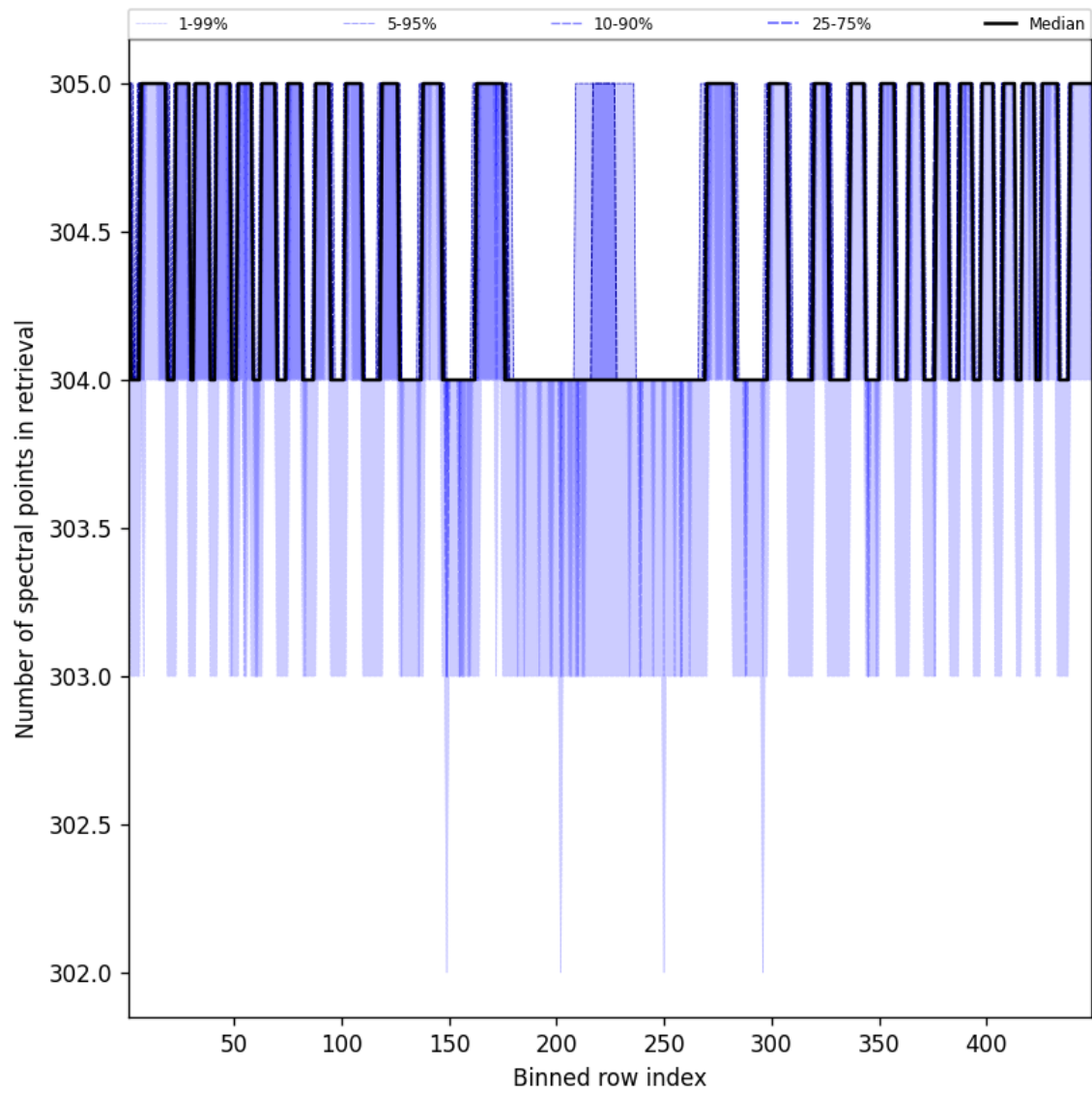
Figure 50: Along track statistics of “Number of spectral points in retrieval” for 2025-11-24 to 2025-11-26
