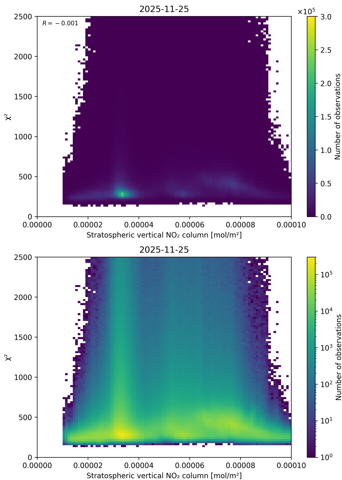
Figure 97: Scatter density plot of “Stratospheric vertical NO 2 column” against “ \chi^2 ” for 2025-11-24 to 2025-11-26.
