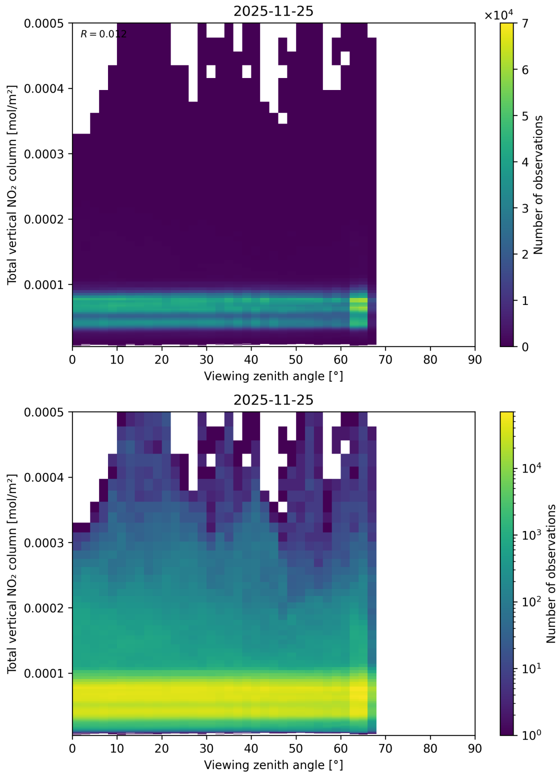
Figure 167: Scatter density plot of “Viewing zenith angle” against “Total vertical NO 2 column” for 2025-11-24 to 2025-11-26.
