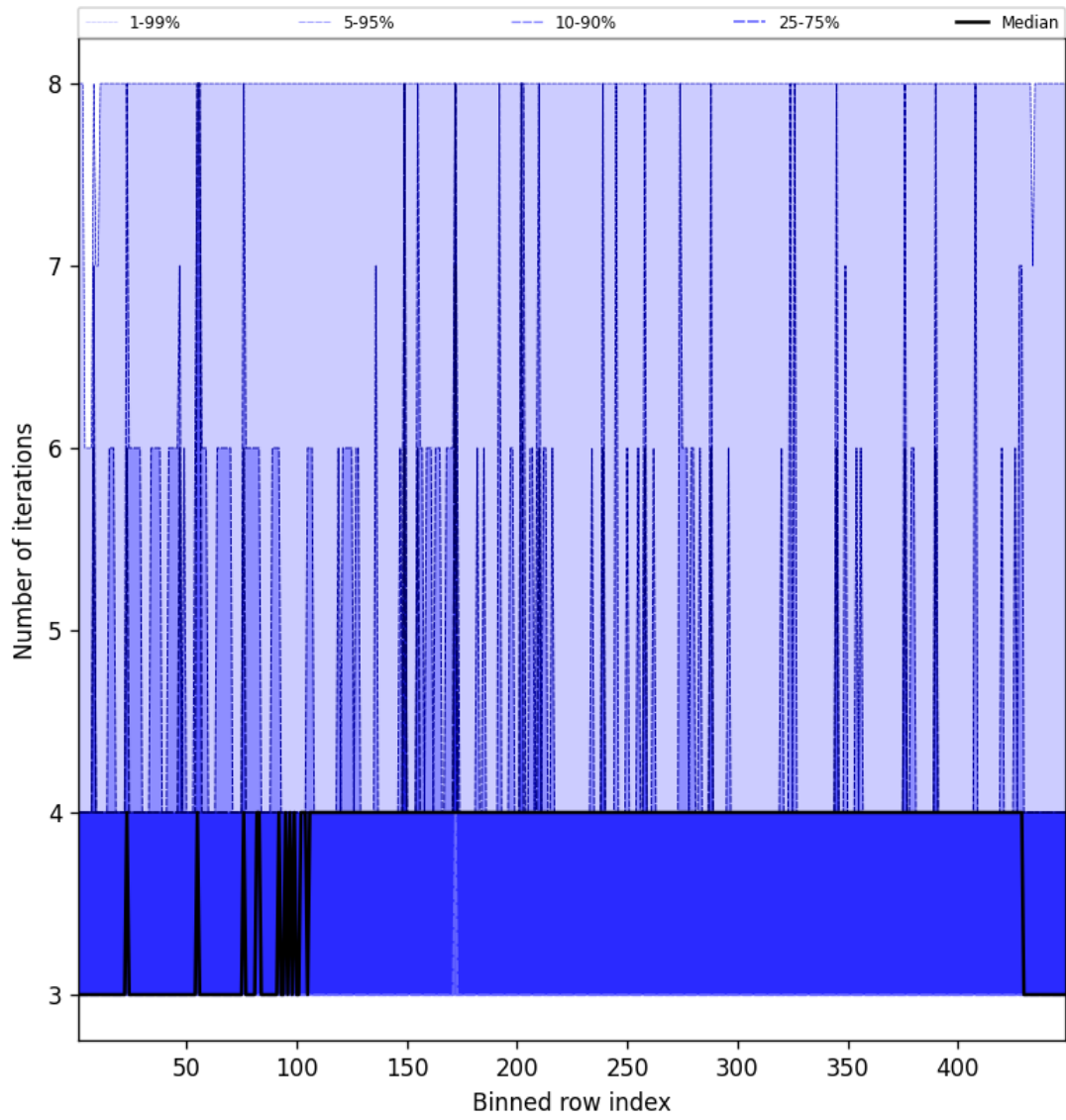
Figure 51: Along track statistics of “Number of iterations” for 2025-11-24 to 2025-11-26
