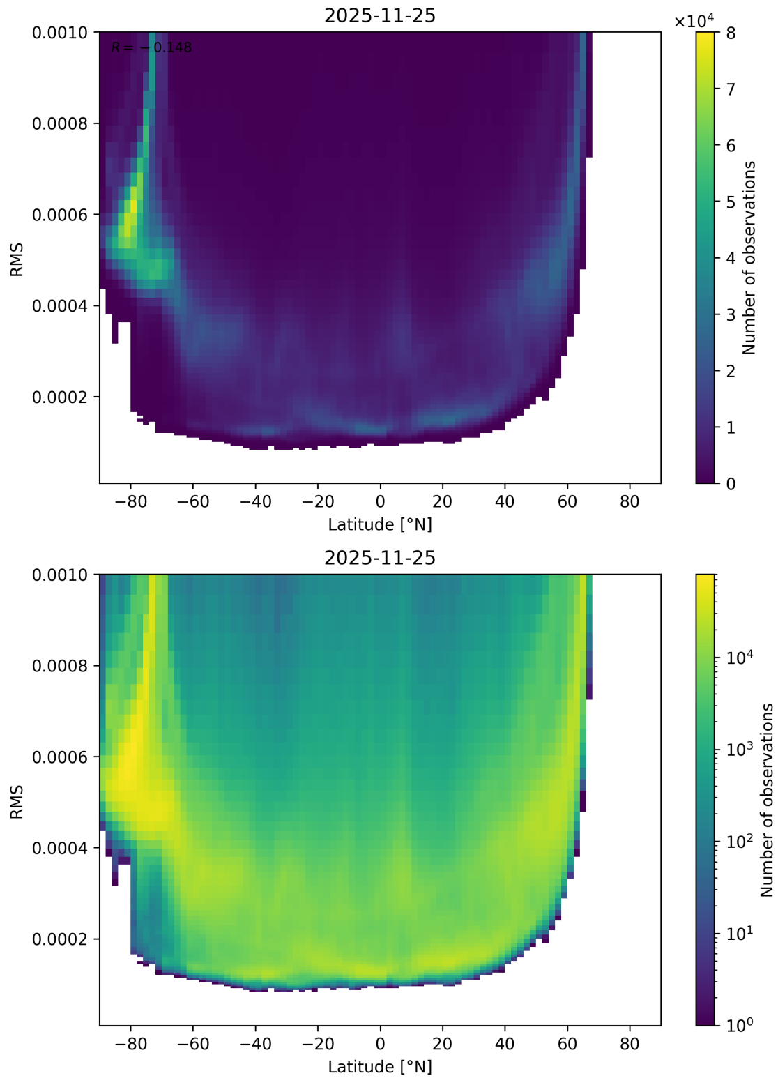
Figure 94: Scatter density plot of “Latitude” against “RMS” for 2025-11-24 to 2025-11-26.
