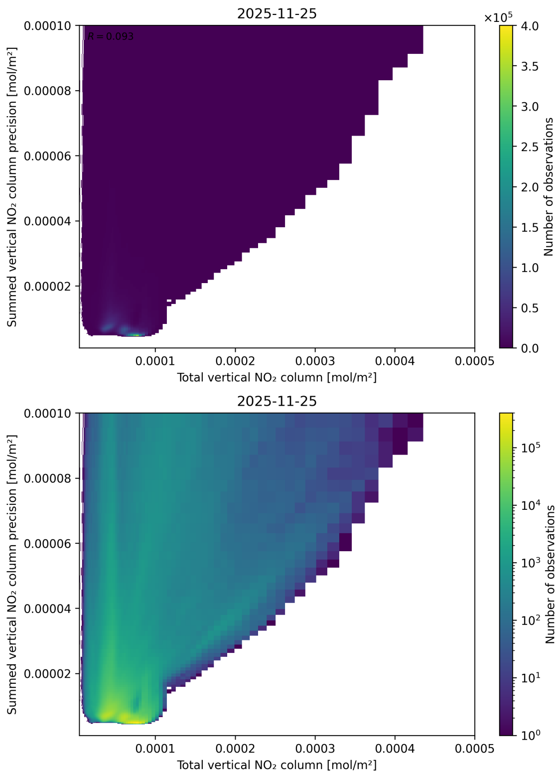
Figure 113: Scatter density plot of “Total vertical NO 2 column” against “Summed vertical NO 2 column precision” for 2025-11-24 to 2025-11-26.
