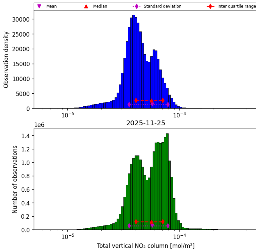
Figure 38: Histogram of “Total vertical NO 2 column” for 2025-11-24 to 2025-11-26
