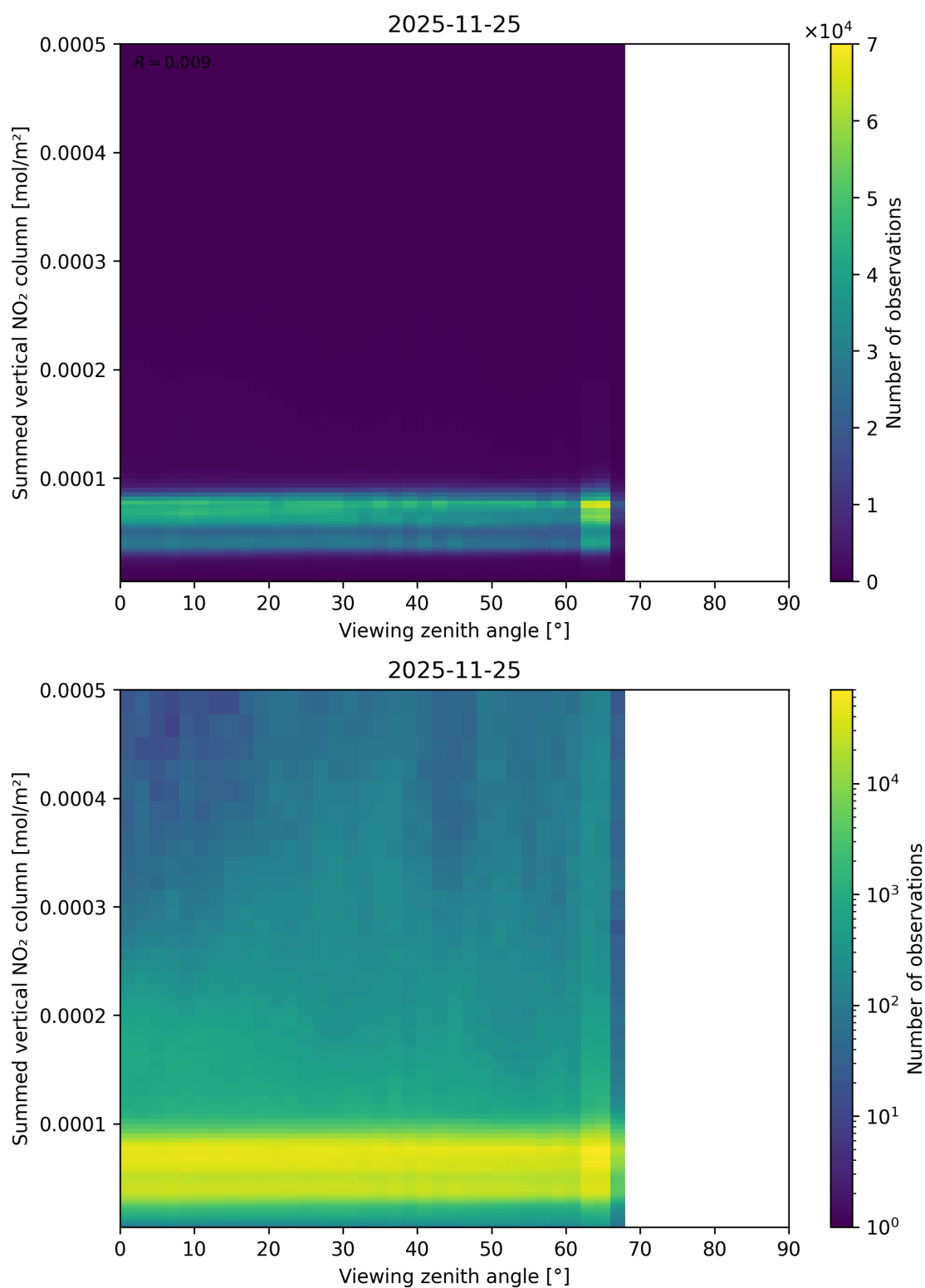
Figure 165: Scatter density plot of “Viewing zenith angle” against “Summed vertical NO 2 column” for 2025-11-24 to 2025-11-26.
