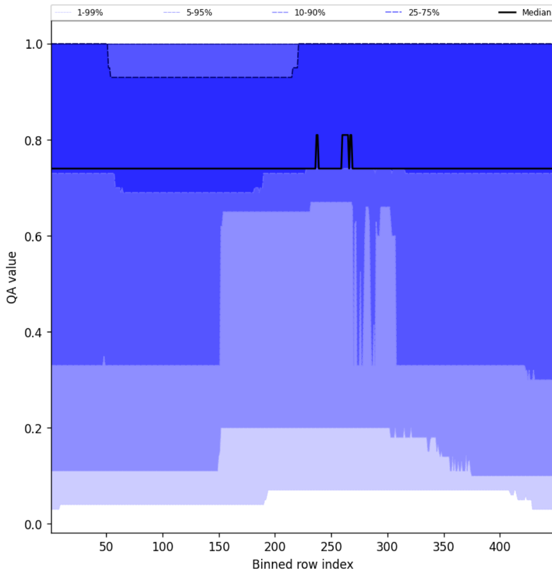
Figure 45: Along track statistics of "QA value" for 2025-11-24 to 2025-11-26
