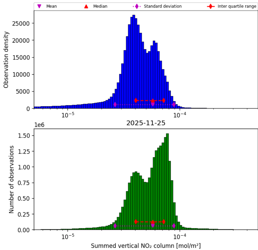
Figure 40: Histogram of “Summed vertical NO 2 column” for 2025-11-24 to 2025-11-26
