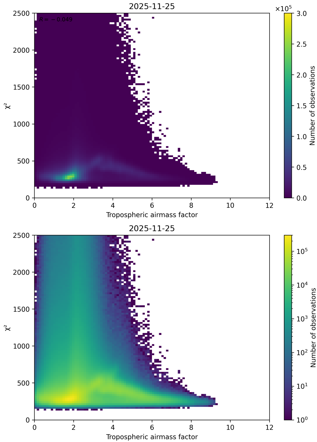
Figure 73: Scatter density plot of “Tropospheric airmass factor” against “ \chi^2 ” for 2025-11-24 to 2025-11-26.
