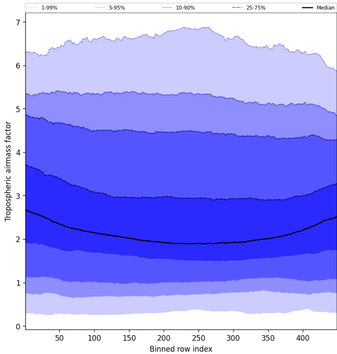
Figure 48: Along track statistics of “Tropospheric air mass factor” for 2025-11-24 to 2025-11-26
