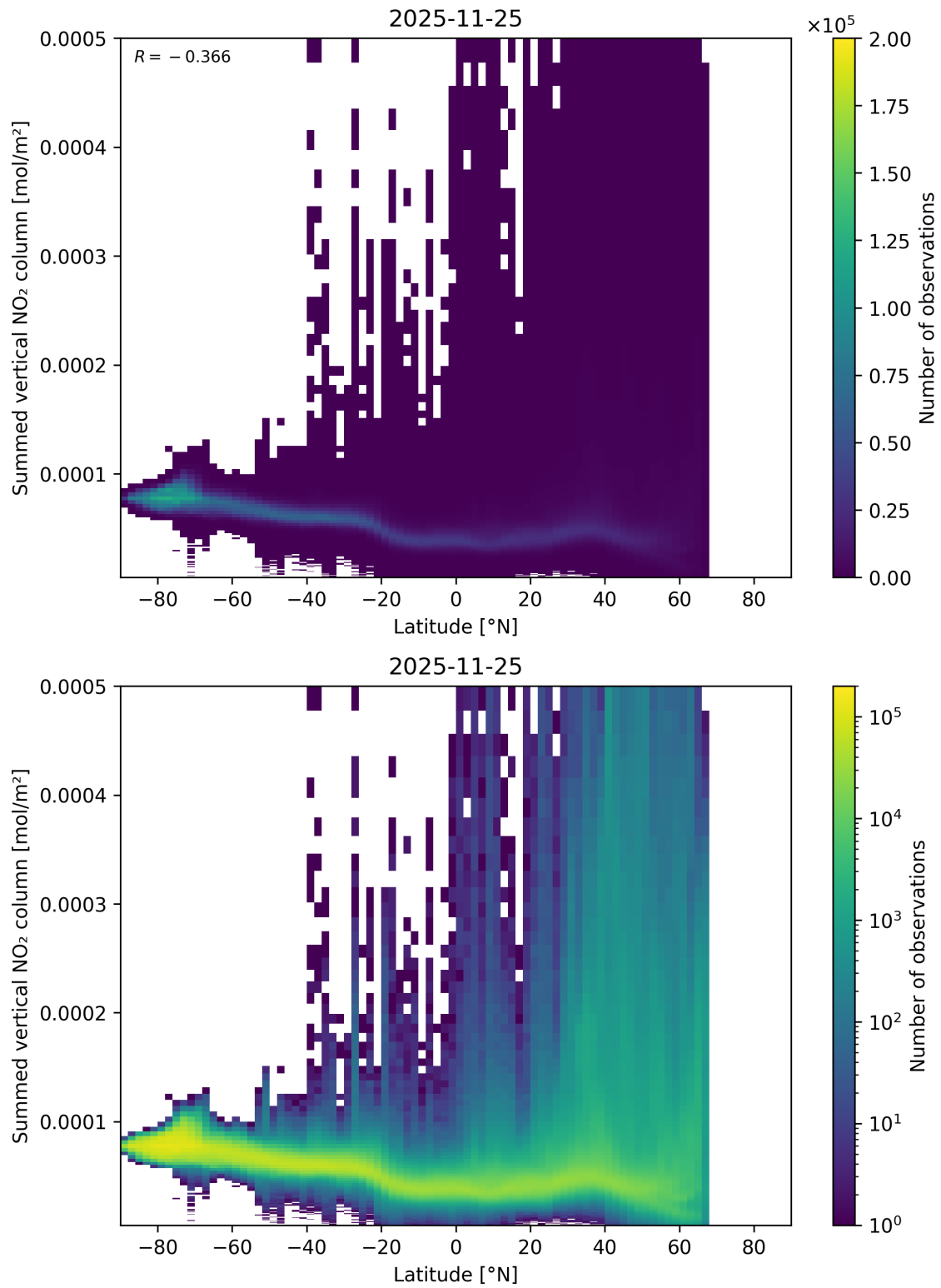
Figure 88: Scatter density plot of “Latitude” against “Summed vertical NO 2 column” for 2025-11-24 to 2025-11-26.
