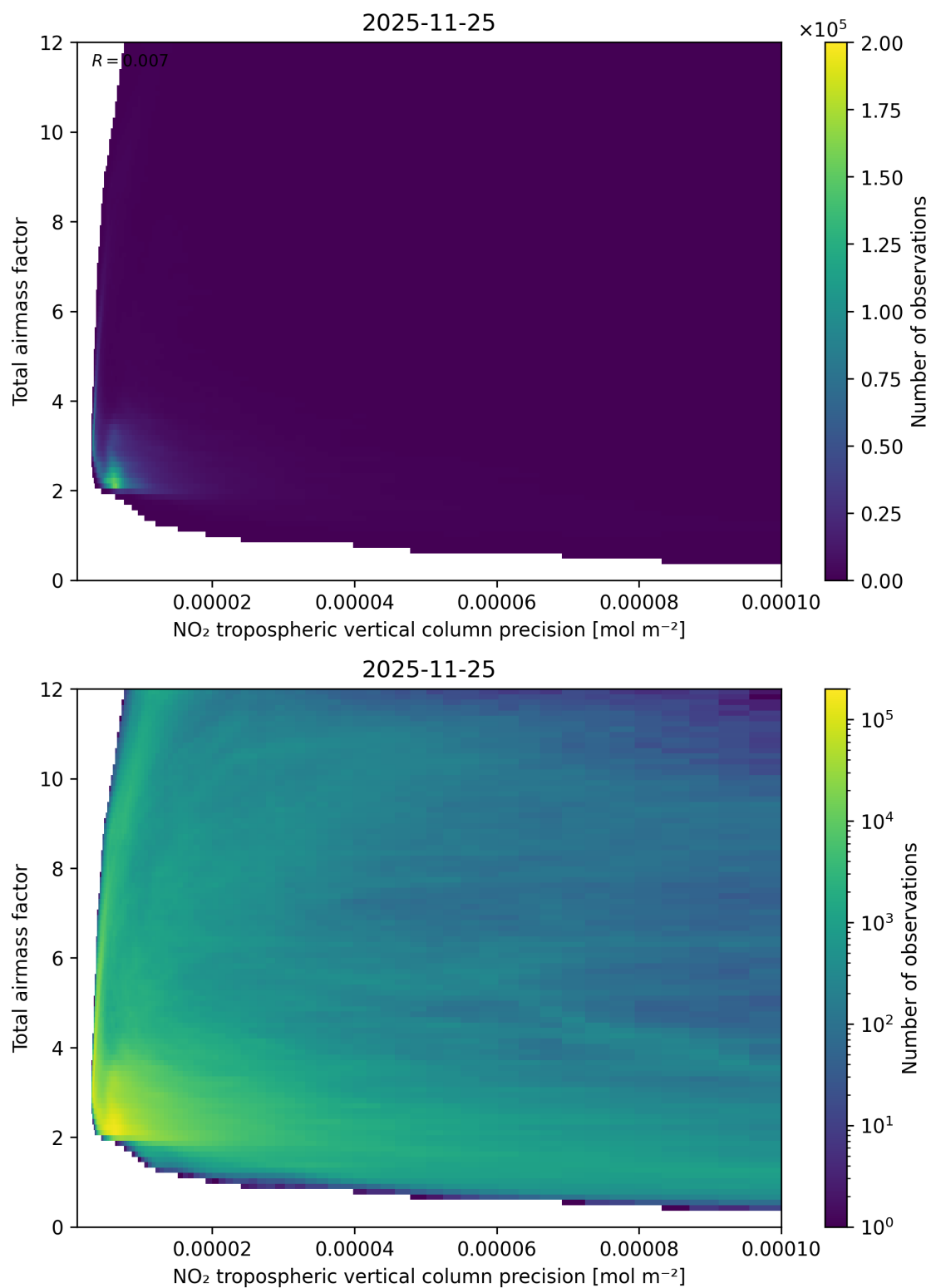
Figure 132: Scatter density plot of “NO 2 tropospheric vertical column precision” against “Total air mass factor” for 2025-11-24 to 2025-11-26.
