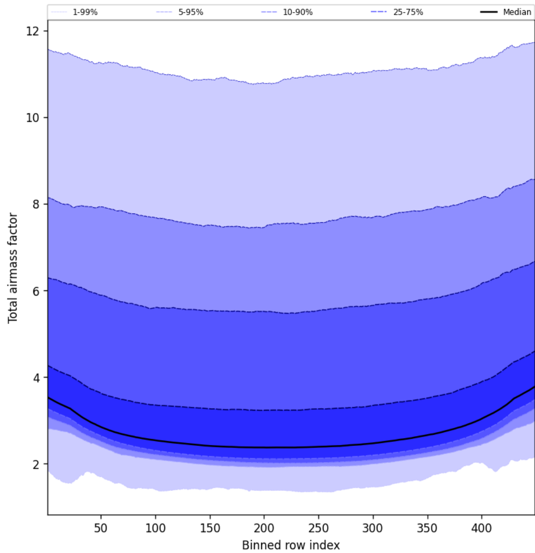
Figure 49: Along track statistics of “Total airmass factor” for 2025-11-24 to 2025-11-26
