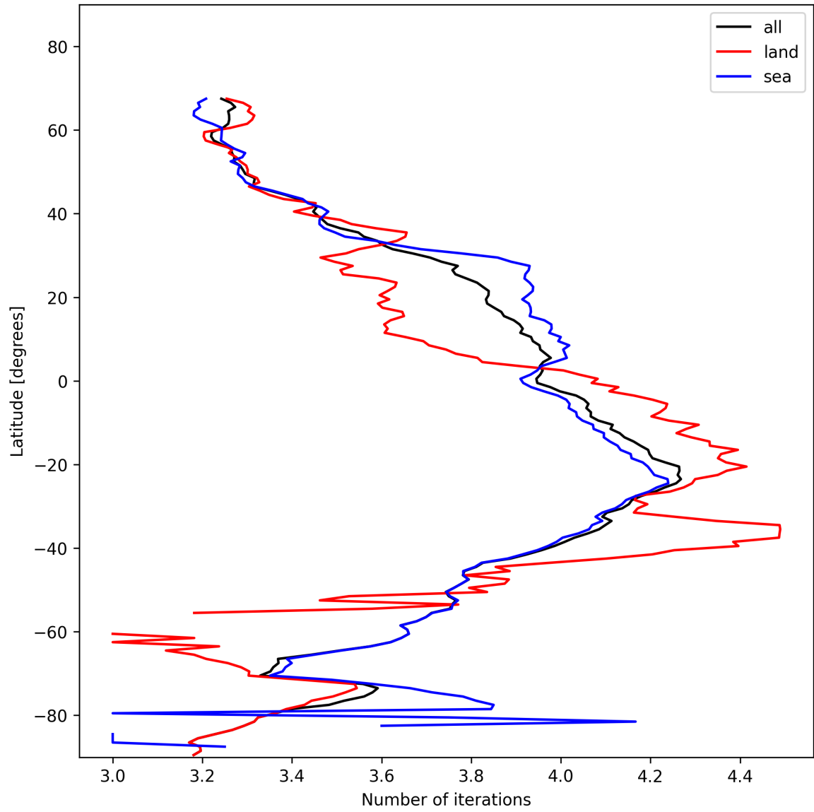
Figure 17: Zonal average of “Number of iterations” for 2025-11-24 to 2025-11-26.
