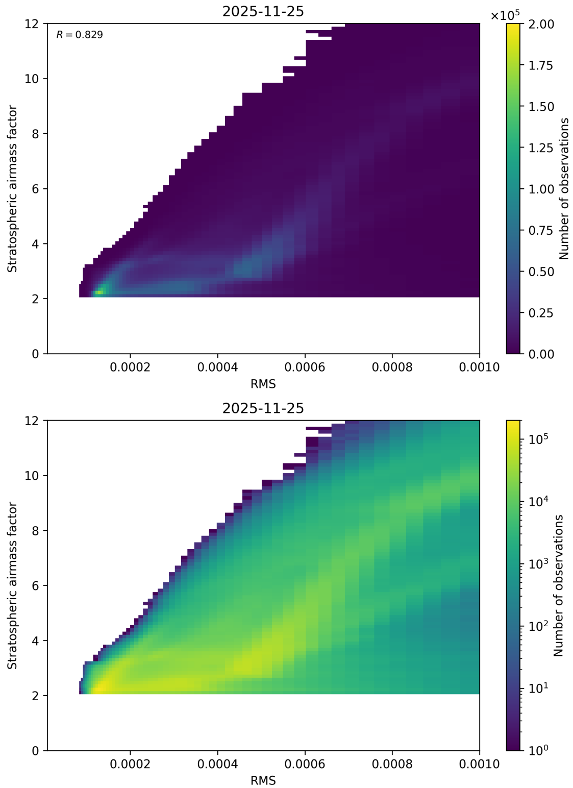
Figure 144: Scatter density plot of “RMS” against “Stratospheric airmass factor” for 2025-11-24 to 2025-11-26.
