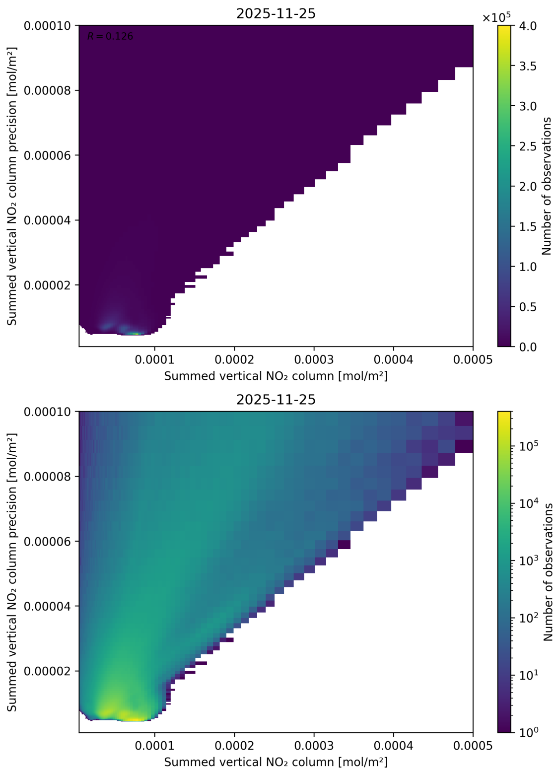
Figure 105: Scatter density plot of “Summed vertical NO 2 column” against “Summed vertical NO 2 column precision” for 2025-11-24 to 2025-11-26.
