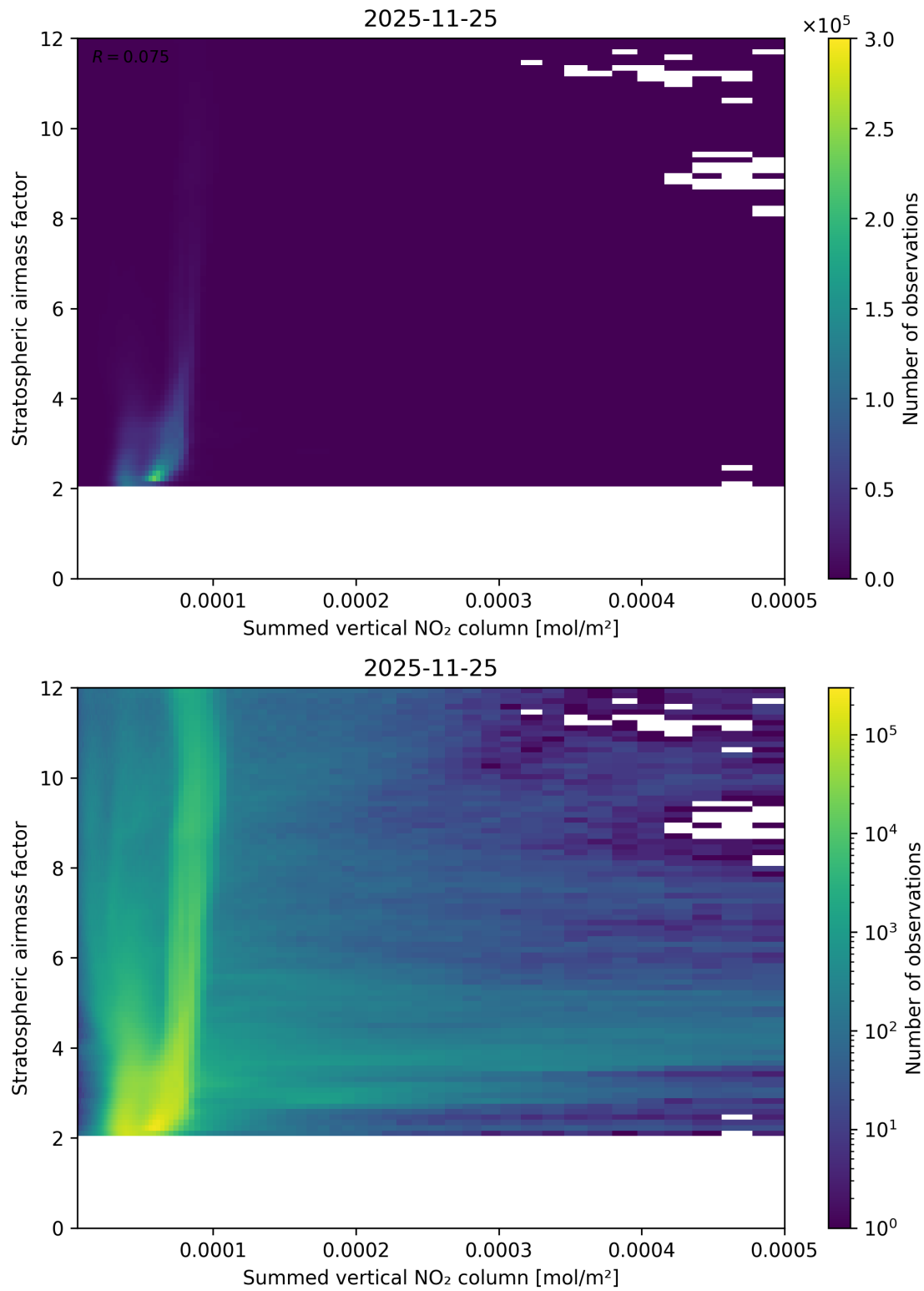
Figure 103: Scatter density plot of “Summed vertical NO 2 column” against “Stratospheric air mass factor” for 2025-11-24 to 2025-11-26.
