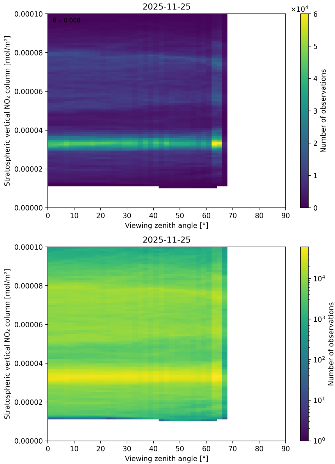
Figure 164: Scatter density plot of “Viewing zenith angle” against “Stratospheric vertical NO 2 column” for 2025-11-24 to 2025-11-26.
