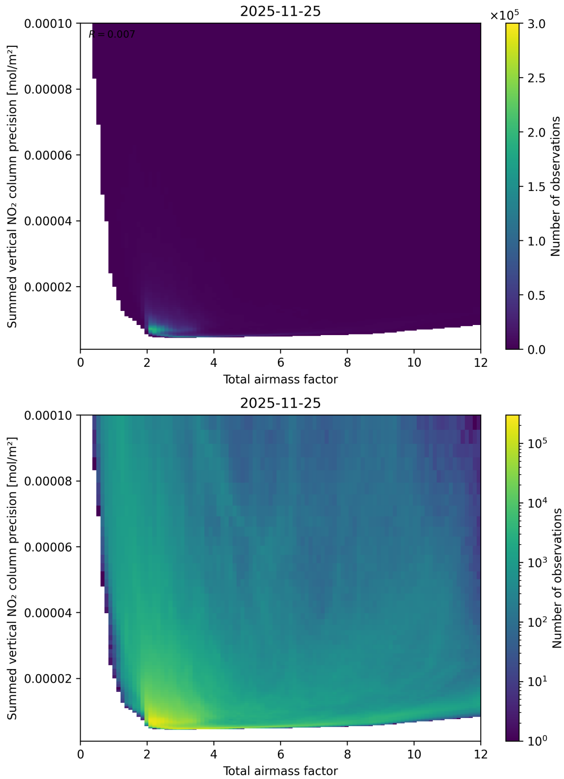
Figure 66: Scatter density plot of “Total airmass factor” against “Summed vertical NO 2 column precision” for 2025-11-24 to 2025-11-26.
