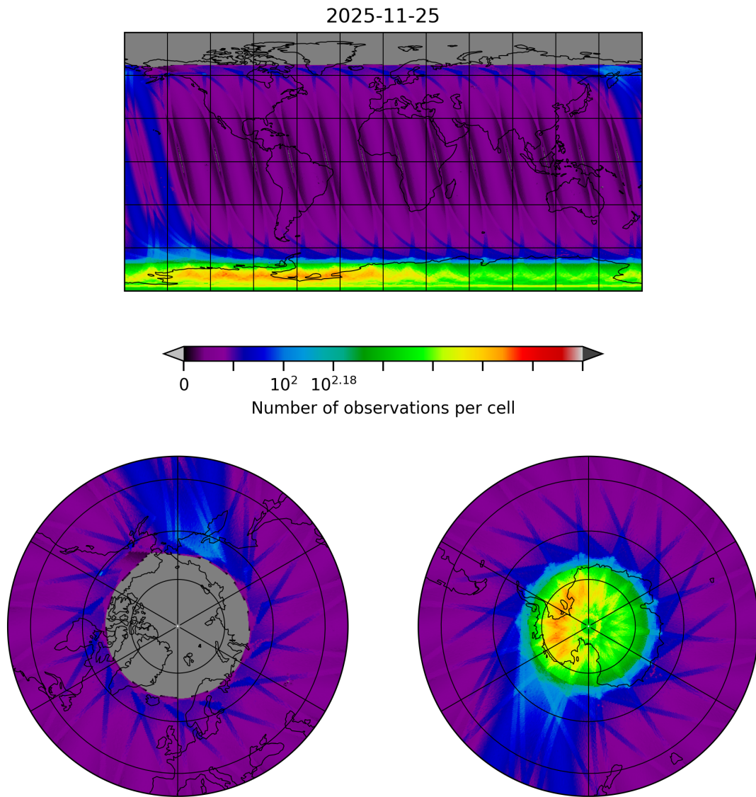
Figure 10: Map of the number of observations for 2025-11-24 to 2025-11-26
