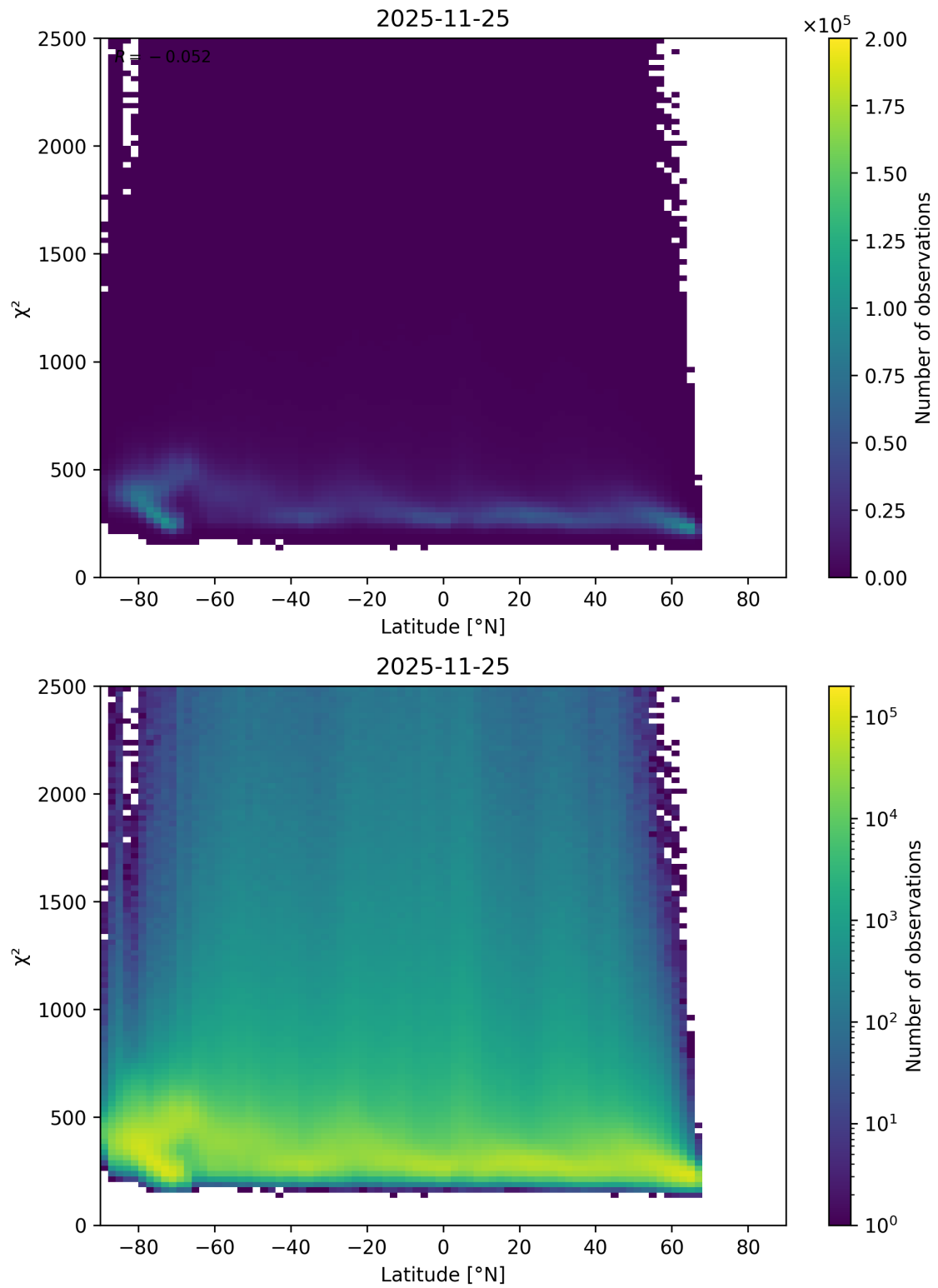
Figure 86: Scatter density plot of “Latitude” against “ \chi^2 ” for 2025-11-24 to 2025-11-26.
