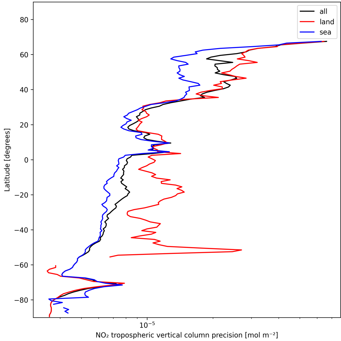
Figure 13: Zonal average of “NO 2 tropospheric vertical column precision” for 2025-11-24 to 2025-11-26.
