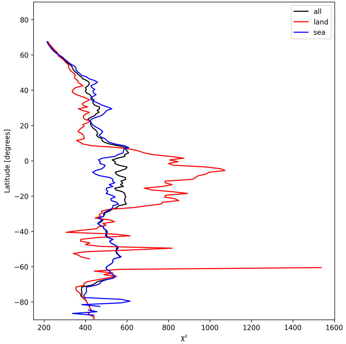
Figure 25: Zonal average of “ \chi^2 ” for 2025-11-24 to 2025-11-26.
