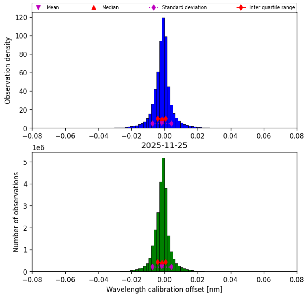
Figure 35: Histogram of “Wavelength calibration offset” for 2025-11-24 to 2025-11-26
