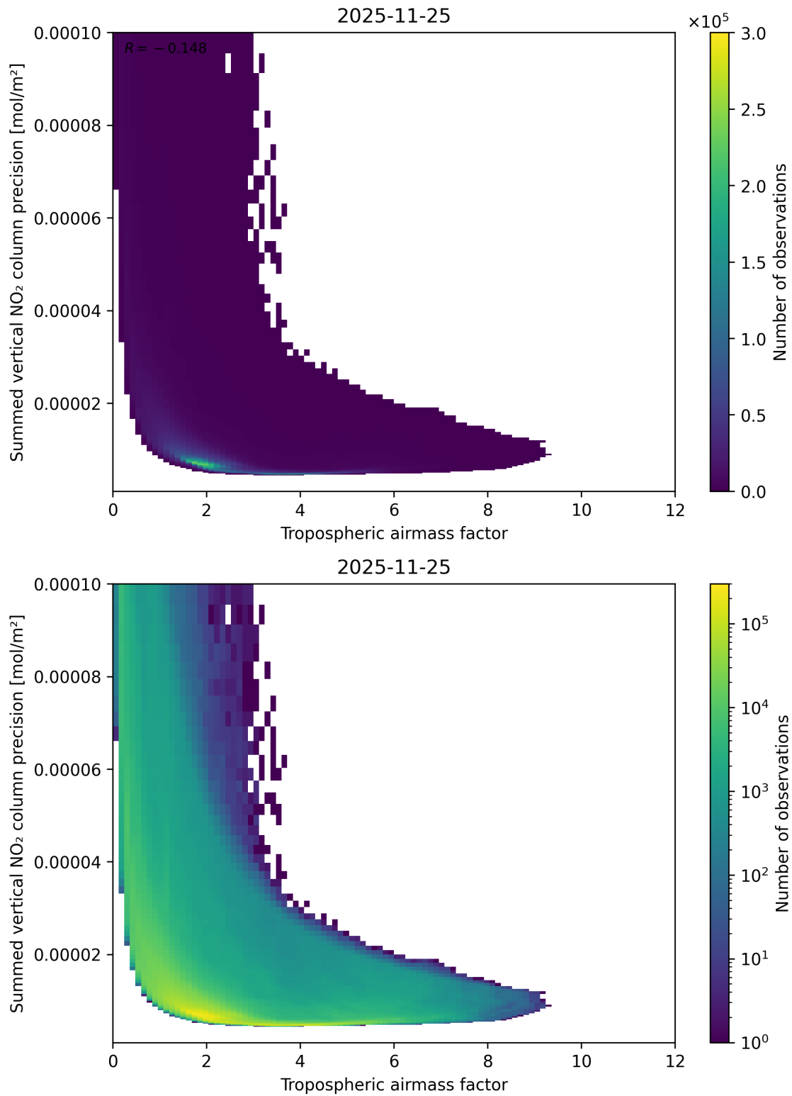
Figure 76: Scatter density plot of “Tropospheric air mass factor” against “Summed vertical NO 2 column precision” for 2025-11-24 to 2025-11-26.
