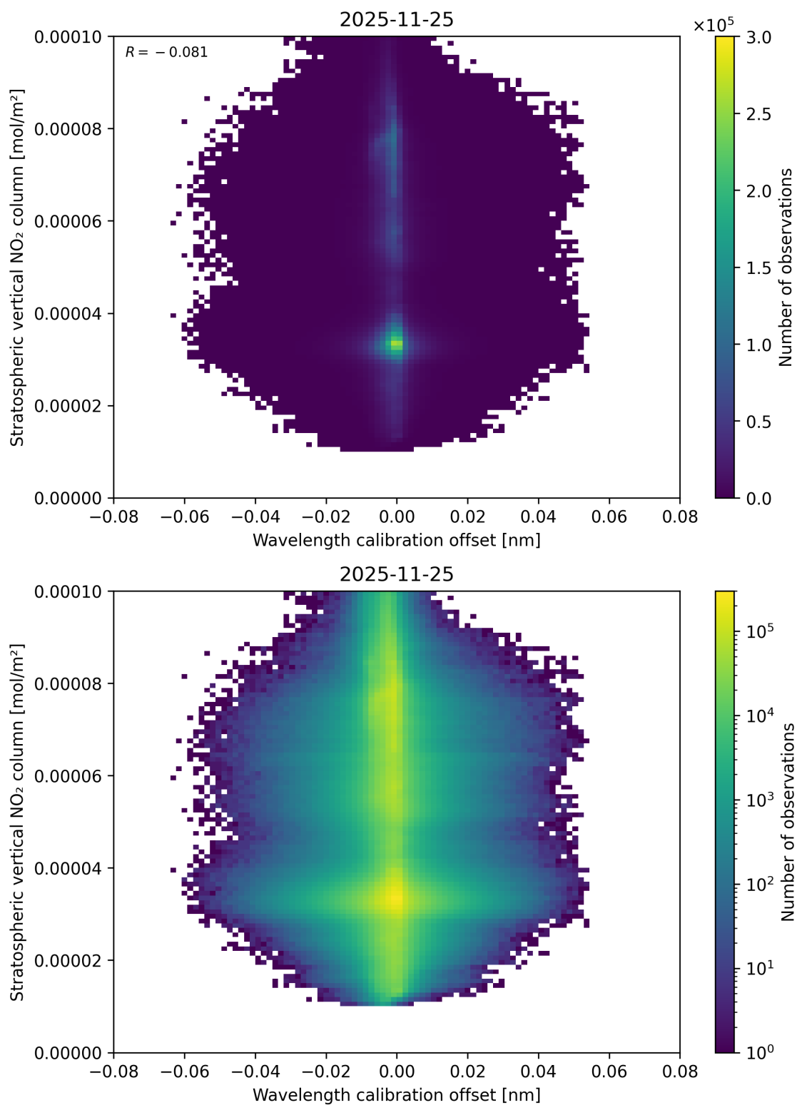
Figure 176: Scatter density plot of “Wavelength calibration offset” against “Stratospheric vertical NO 2 column” for 2025-11-24 to 2025-11-26.
