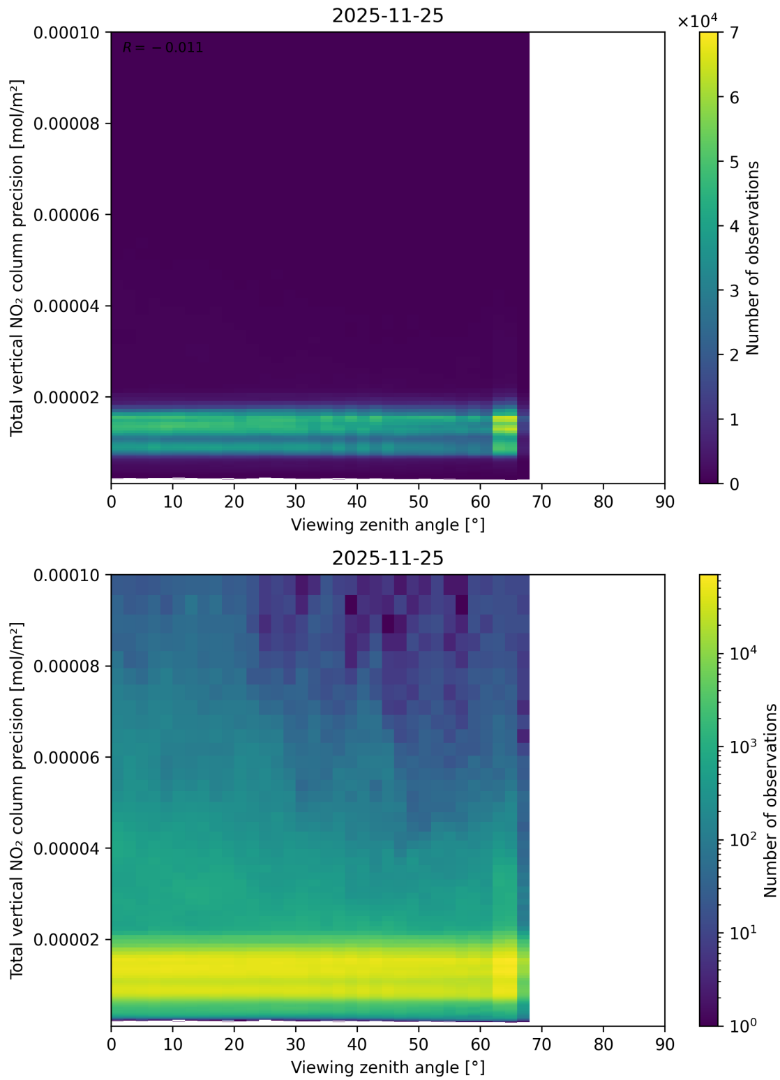
Figure 168: Scatter density plot of “Viewing zenith angle” against “Total vertical NO 2 column precision” for 2025-11-24 to 2025-11-26.
