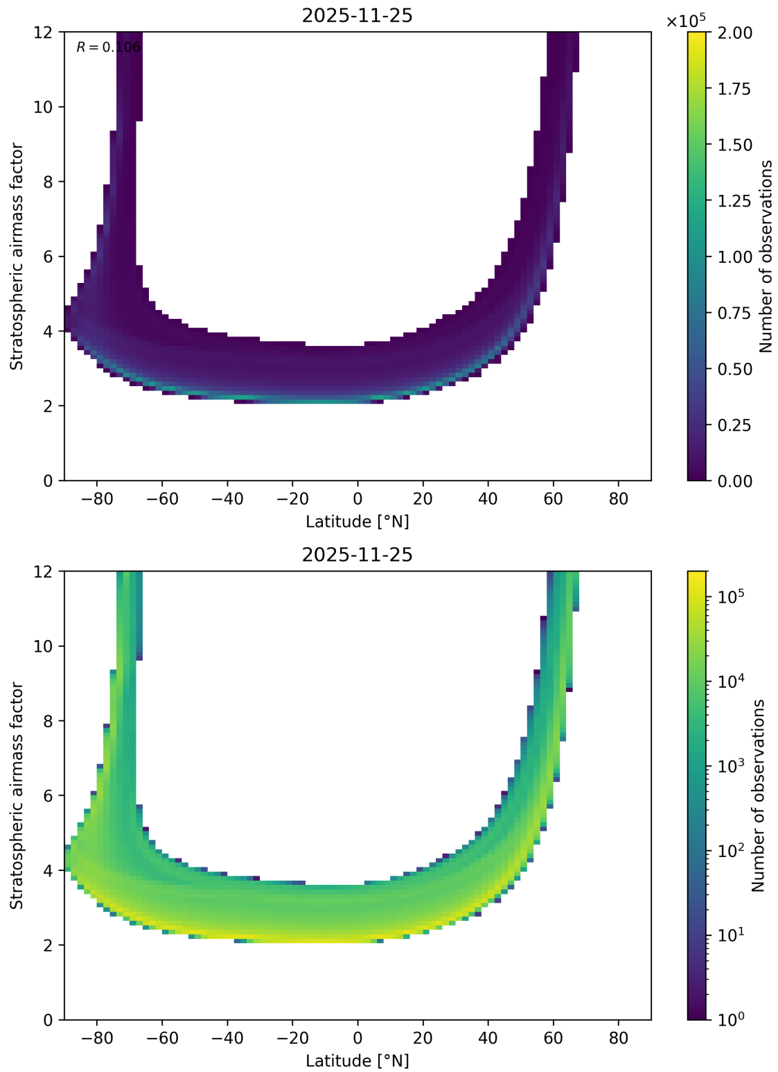
Figure 83: Scatter density plot of “Latitude” against “Stratospheric air mass factor” for 2025-11-24 to 2025-11-26.
