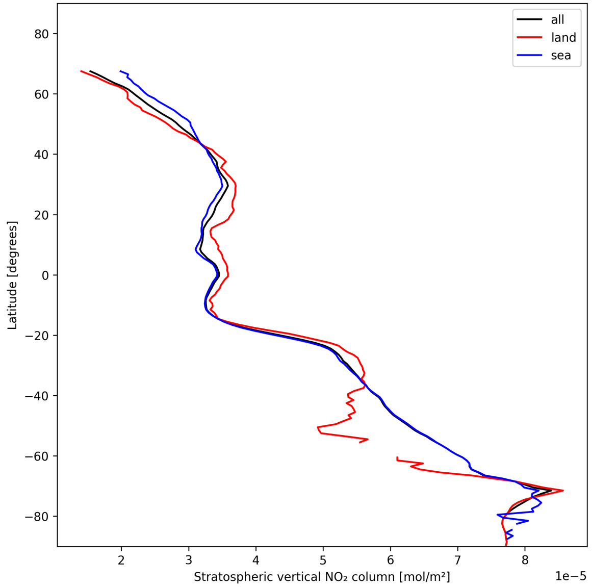
Figure 19: Zonal average of “Stratospheric vertical NO 2 column” for 2025-11-24 to 2025-11-26.
