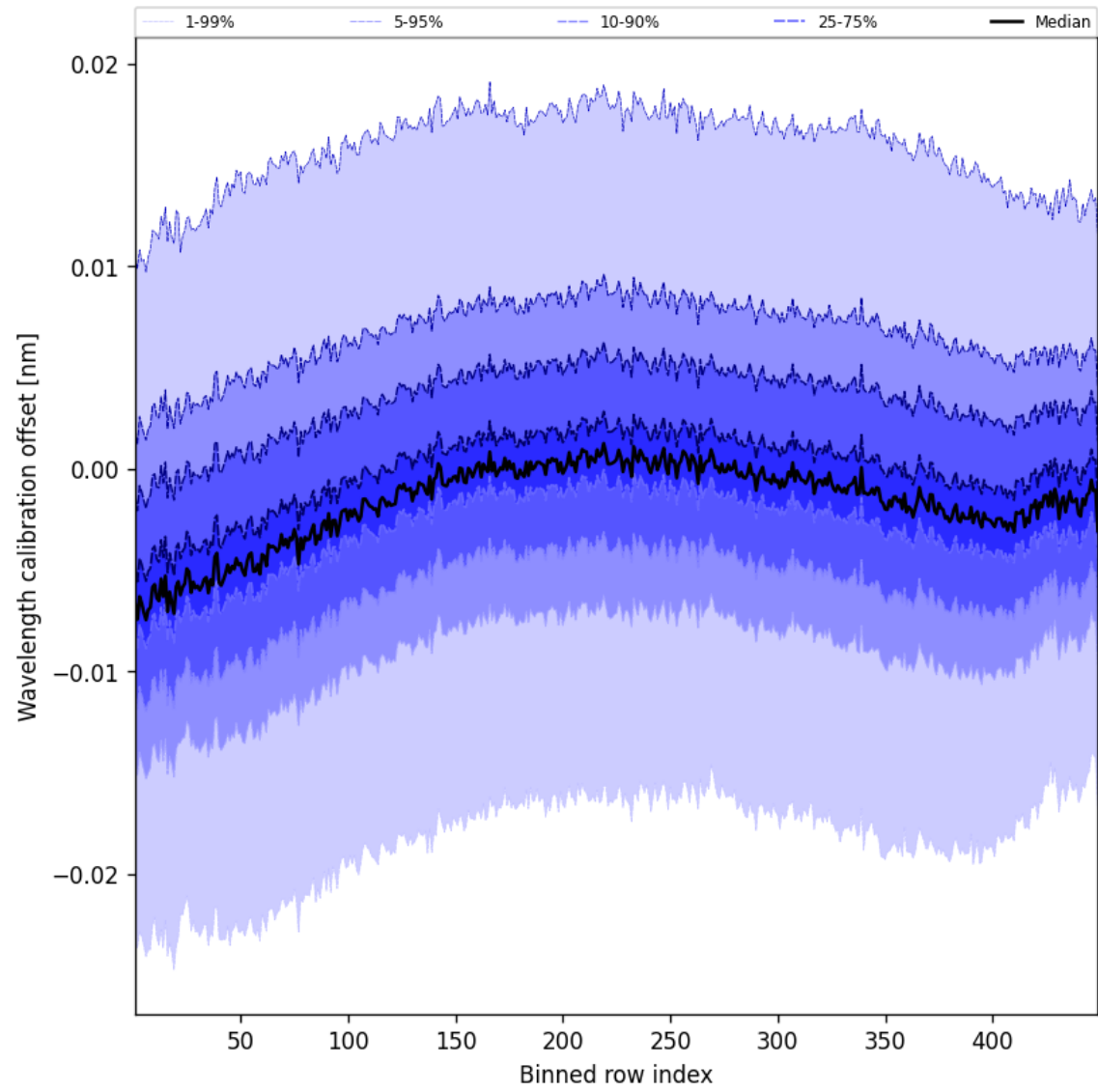
Figure 52: Along track statistics of “Wavelength calibration offset” for 2025-11-24 to 2025-11-26
