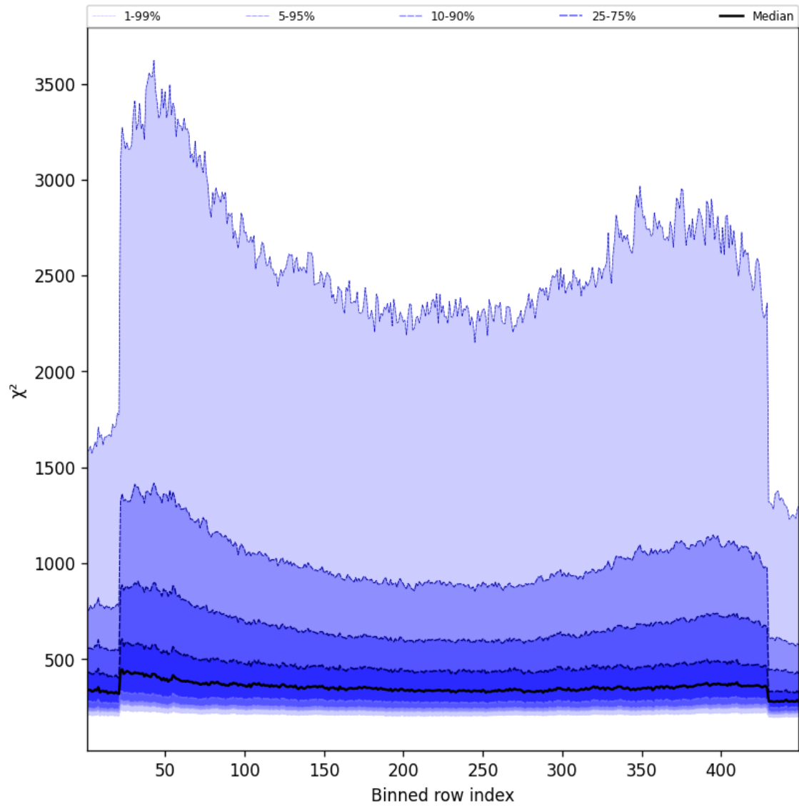
Figure 59: Along track statistics of “ \chi^2 ” for 2025-11-24 to 2025-11-26
