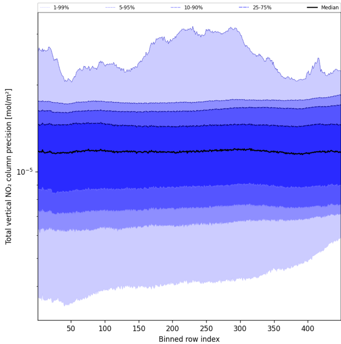
Figure 56: Along track statistics of “Total vertical NO 2 column precision” for 2025-11-24 to 2025-11-26
