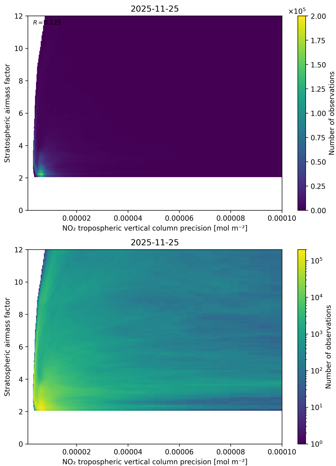
Figure 131: Scatter density plot of “NO 2 tropospheric vertical column precision” against “Stratospheric airmass factor” for 2025-11-24 to 2025-11-26.
