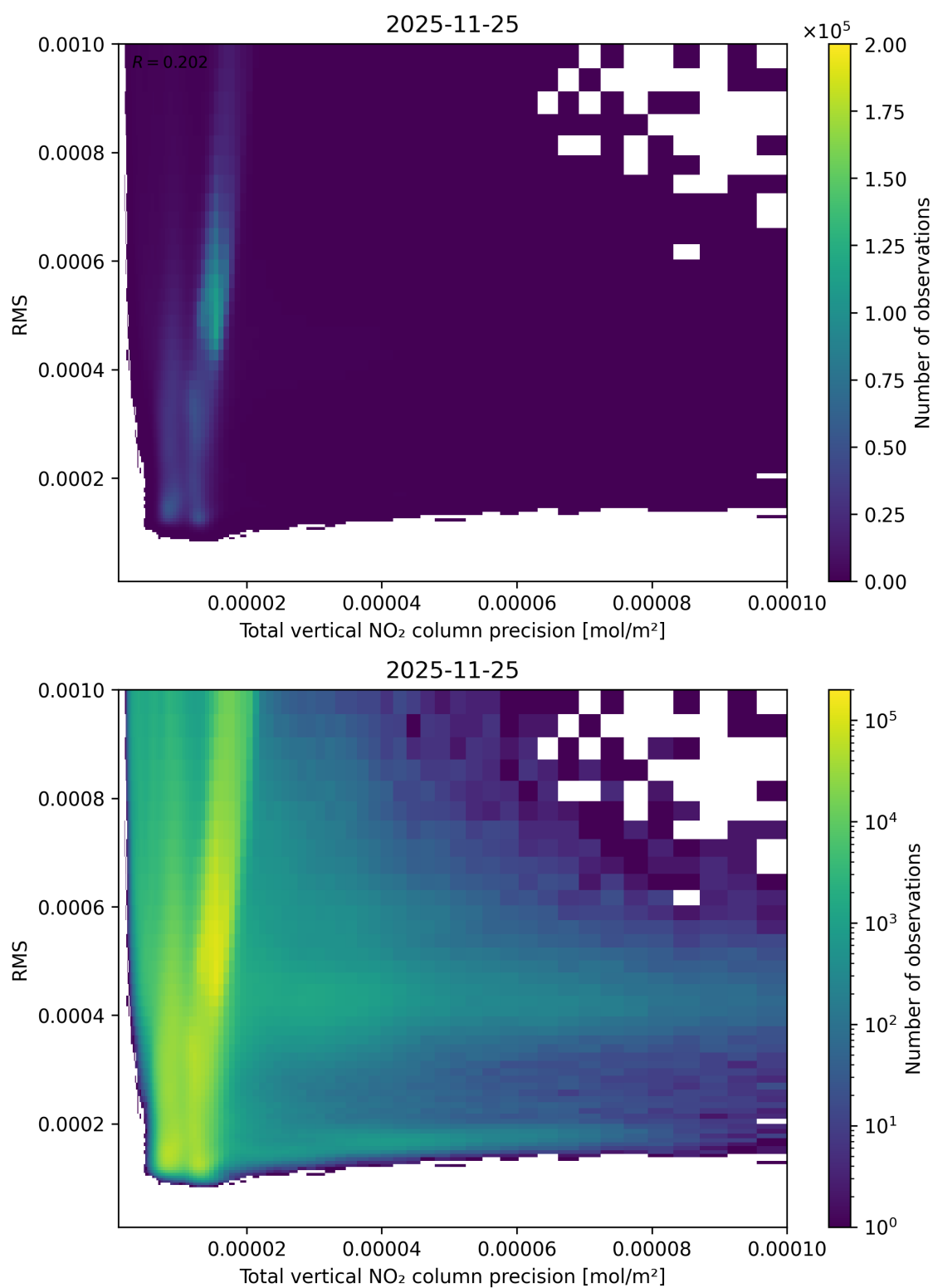
Figure 119: Scatter density plot of “Total vertical NO 2 column precision” against “RMS” for 2025-11-24 to 2025-11-26.
