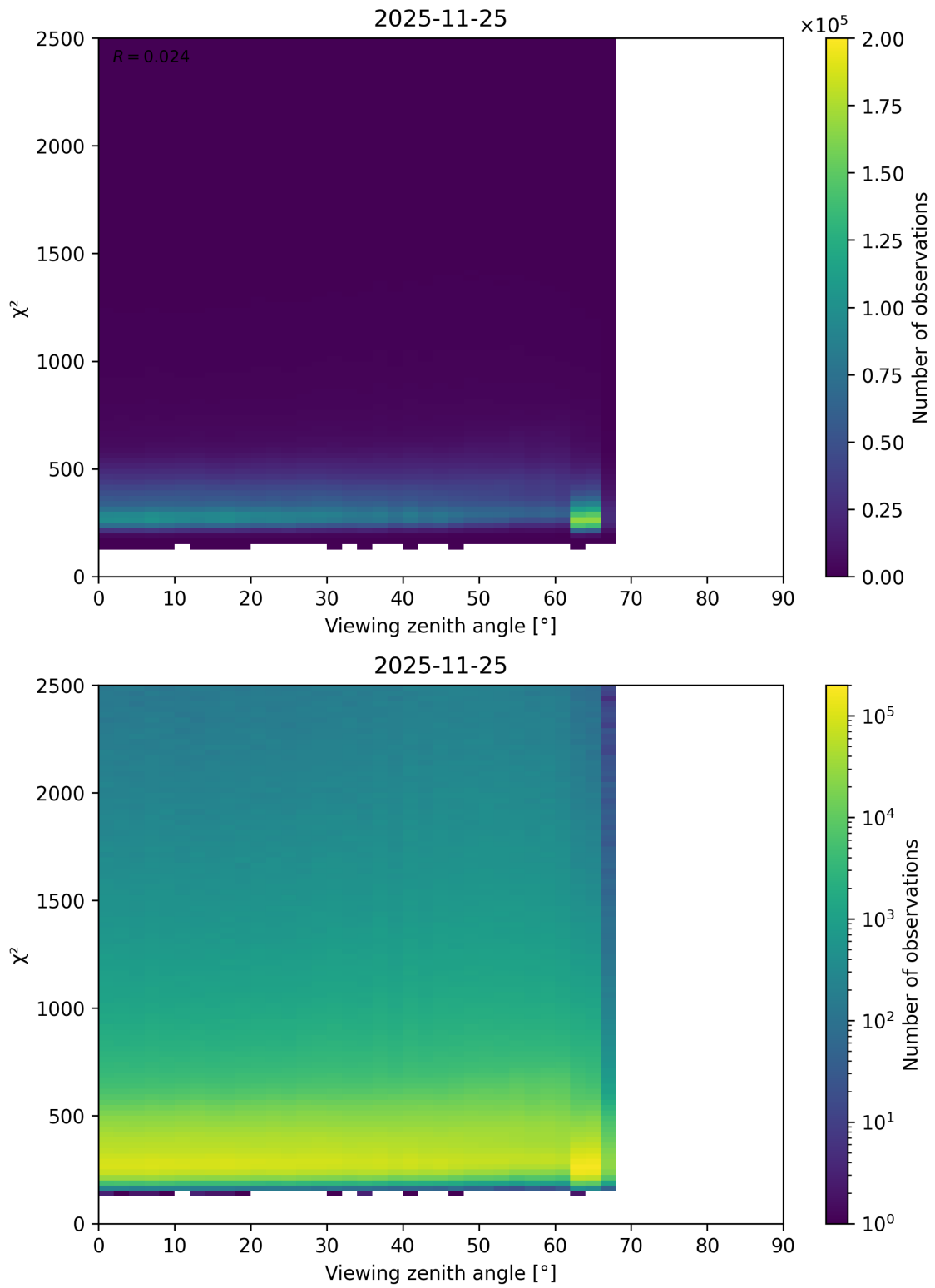
Figure 162: Scatter density plot of “Viewing zenith angle” against “ \chi^2 ” for 2025-11-24 to 2025-11-26.
