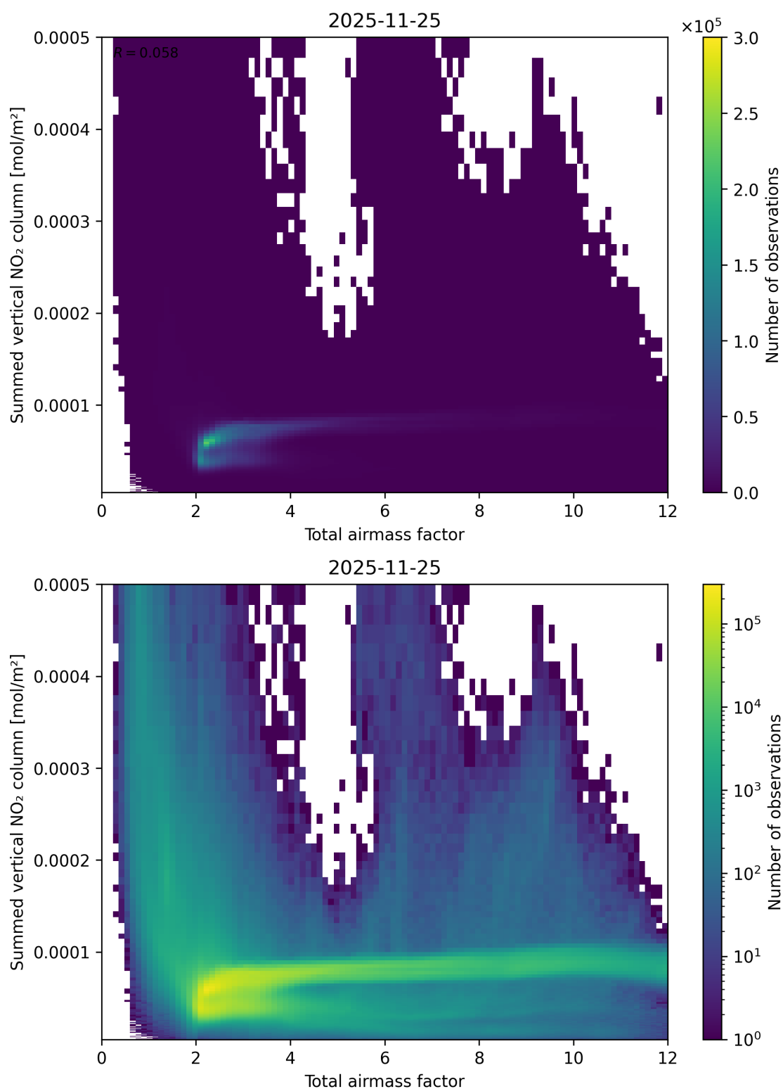
Figure 65: Scatter density plot of “Total airmass factor” against “Summed vertical NO 2 column” for 2025-11-24 to 2025-11-26.
