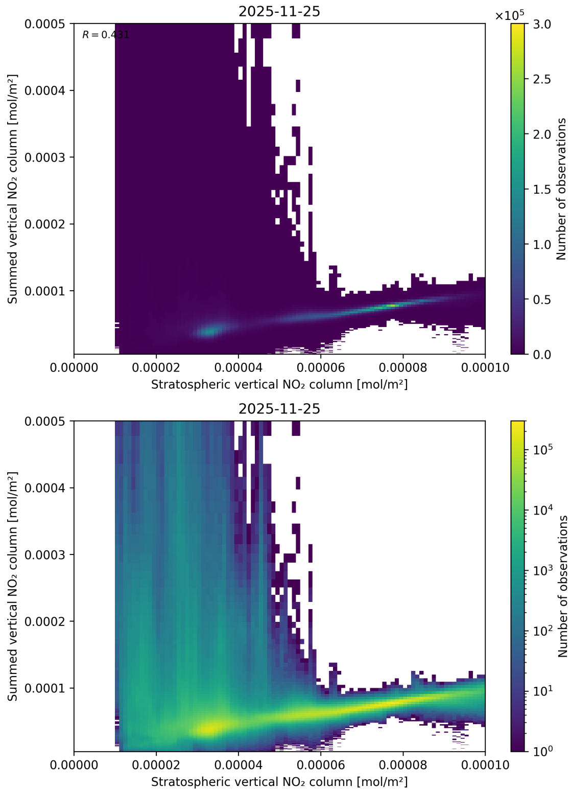
Figure 98: Scatter density plot of “Stratospheric vertical NO 2 column” against “Summed vertical NO 2 column” for 2025-11-24 to 2025-11-26.
