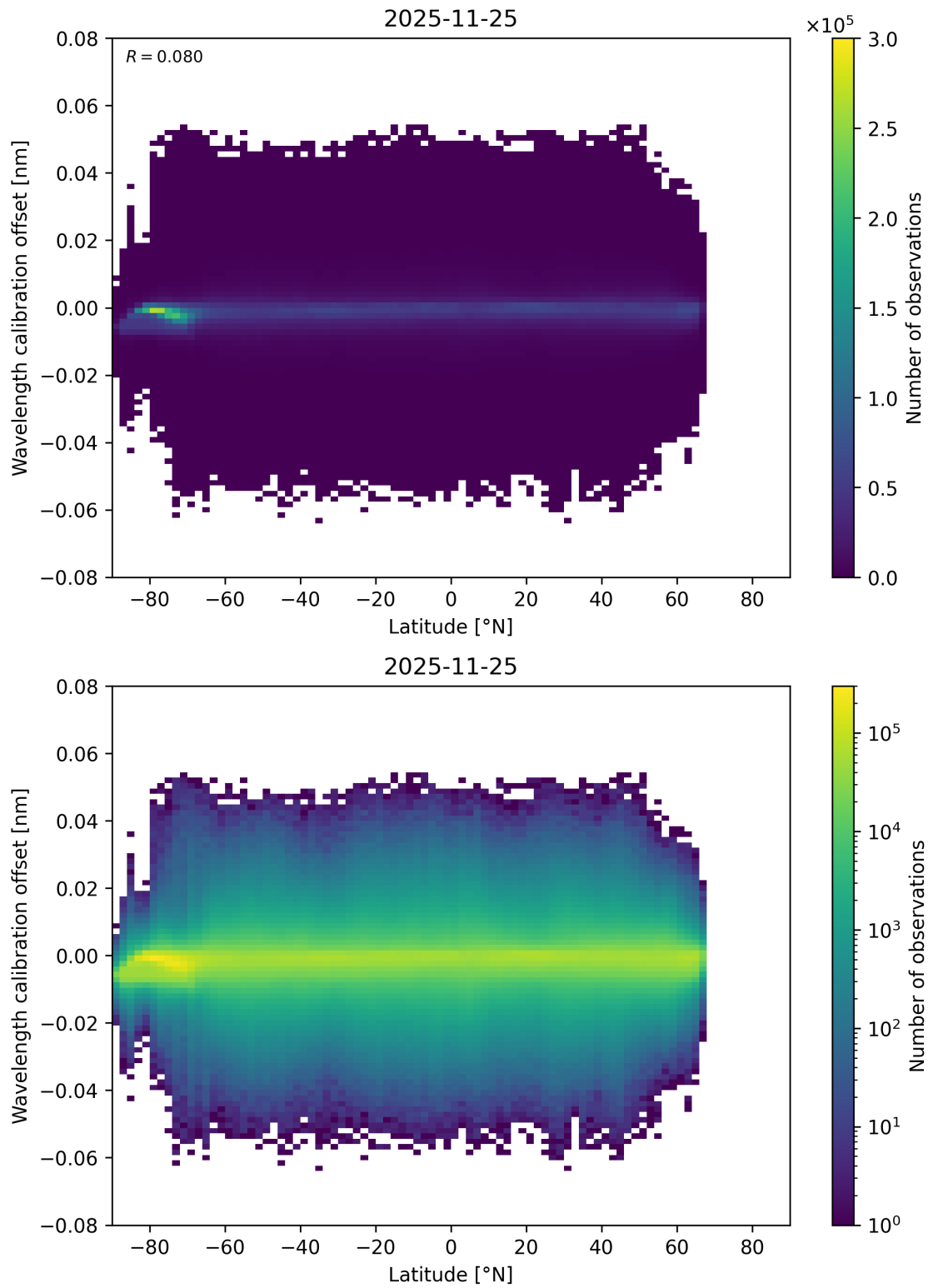
Figure 95: Scatter density plot of “Latitude” against “Wavelength calibration offset” for 2025-11-24 to 2025-11-26.
