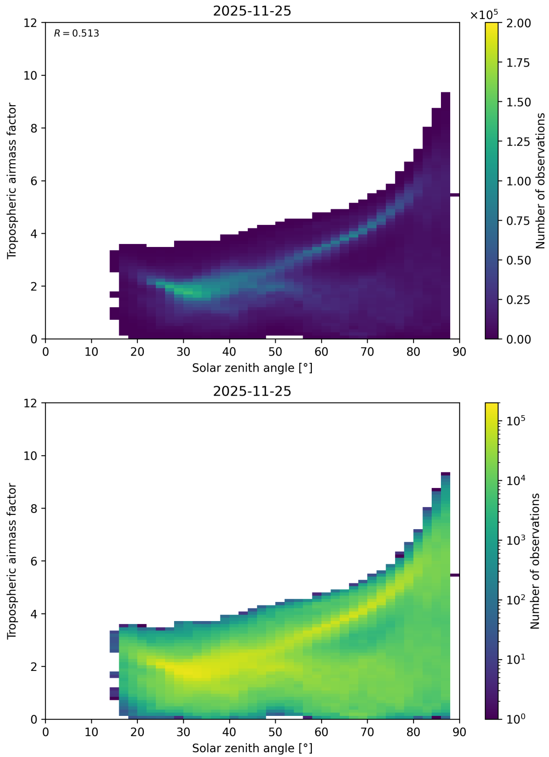
Figure 147: Scatter density plot of “Solar zenith angle” against “Tropospheric airmass factor” for 2025-11-24 to 2025-11-26.
