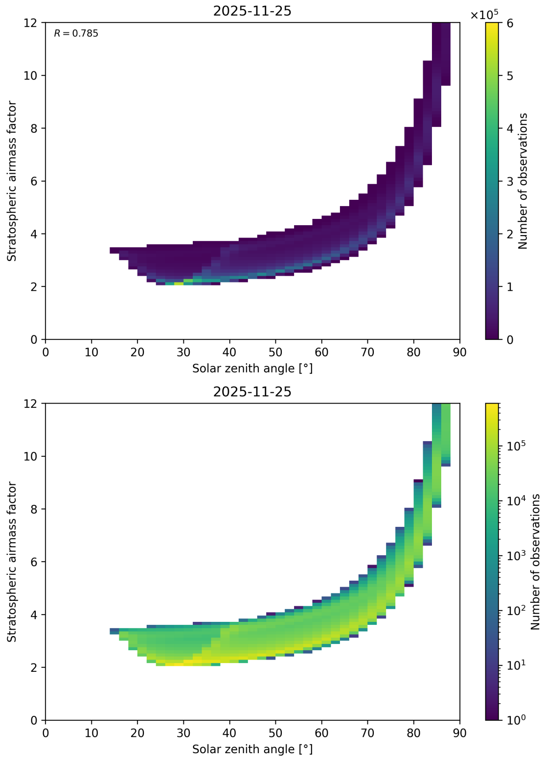
Figure 145: Scatter density plot of “Solar zenith angle” against “Stratospheric airmass factor” for 2025-11-24 to 2025-11-26.
