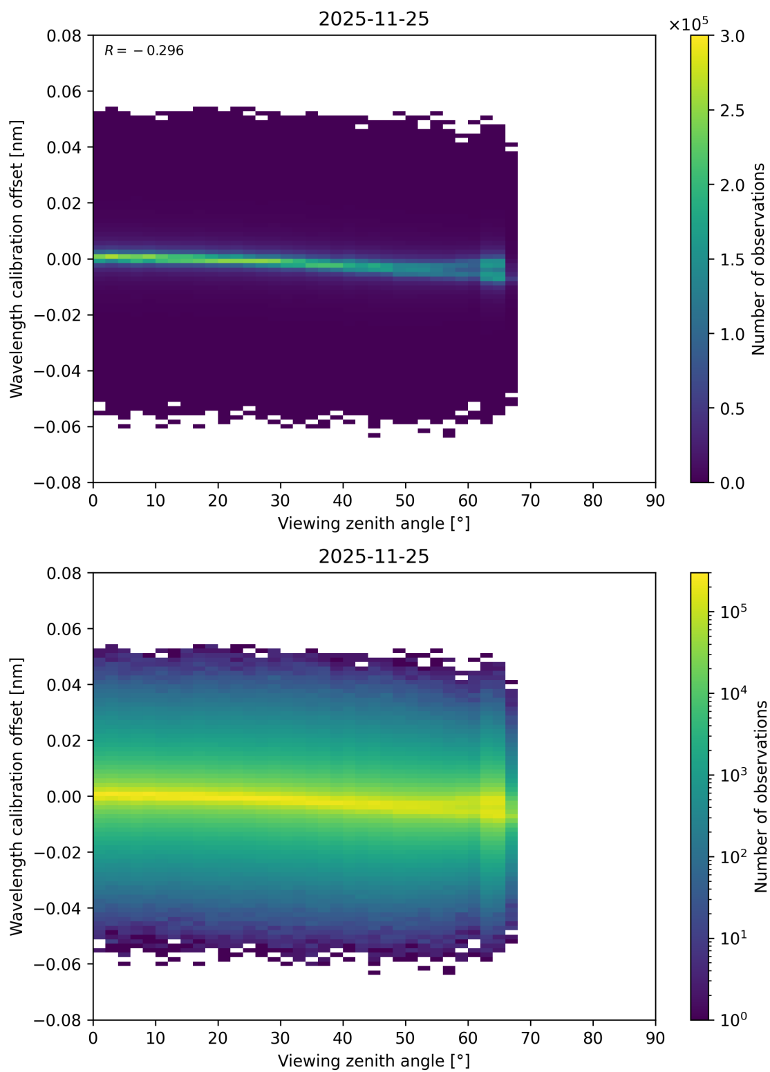
Figure 173: Scatter density plot of “Viewing zenith angle” against “Wavelength calibration offset” for 2025-11-24 to 2025-11-26.
