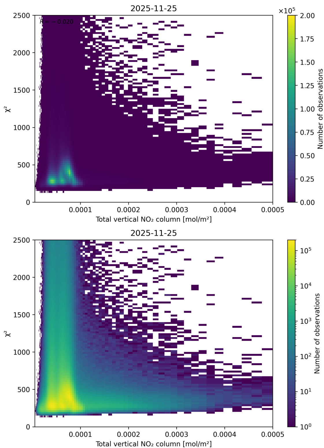
Figure 111: Scatter density plot of “Total vertical NO 2 column” against “ \chi^2 ” for 2025-11-24 to 2025-11-26.
