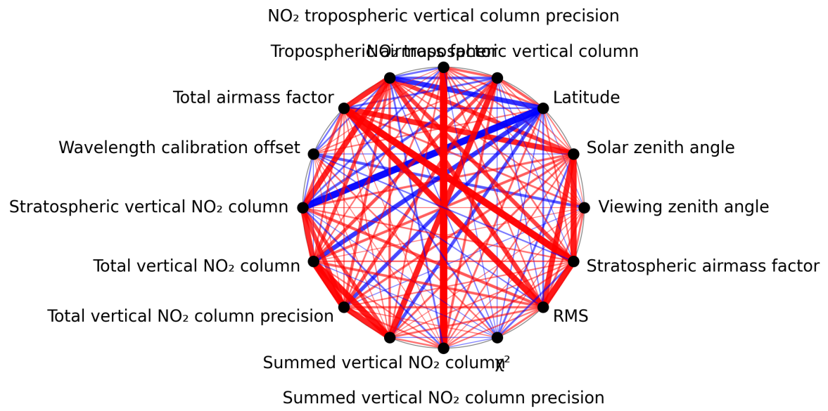
Figure 1: Map of correlation graph for 2025-11-24 to 2025-11-26.
