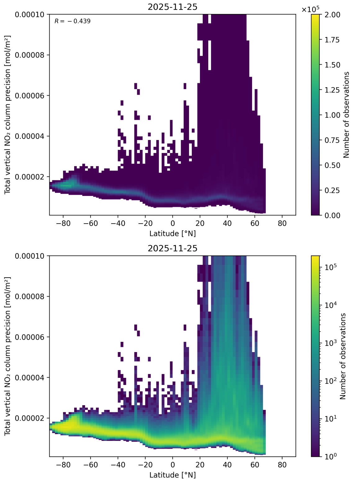
Figure 91: Scatter density plot of “Latitude” against “Total vertical NO 2 column precision” for 2025-11-24 to 2025-11-26.
