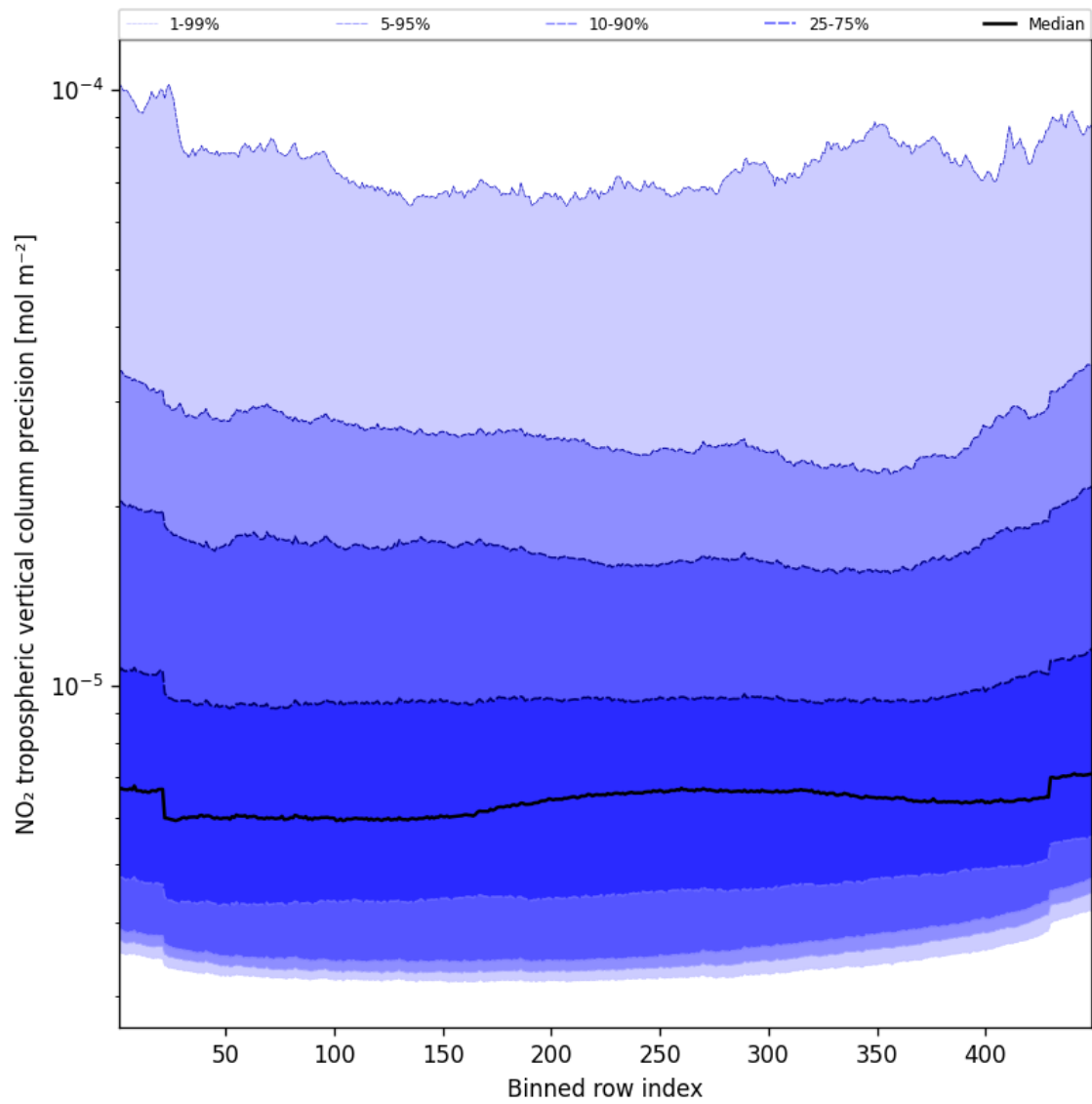
Figure 47: Along track statistics of “NO 2 tropospheric vertical column precision” for 2025-11-24 to 2025-11-26
