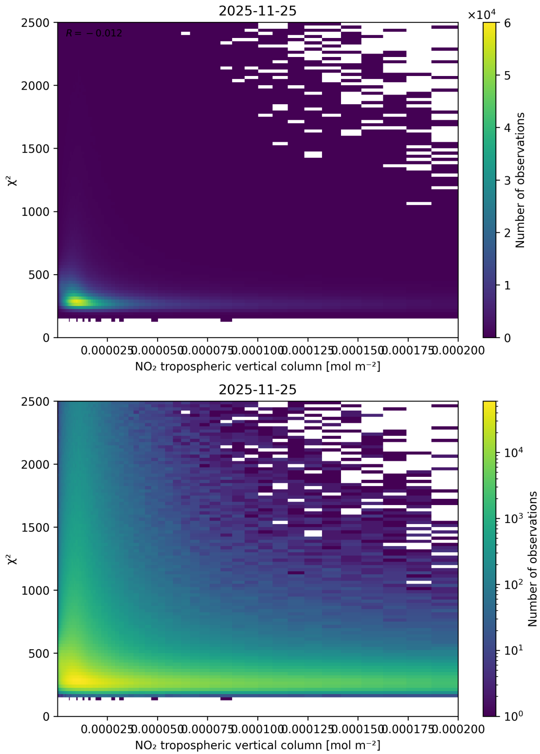
Figure 124: Scatter density plot of “NO 2 tropospheric vertical column” against “ \chi^2 ” for 2025-11-24 to 2025-11-26.
