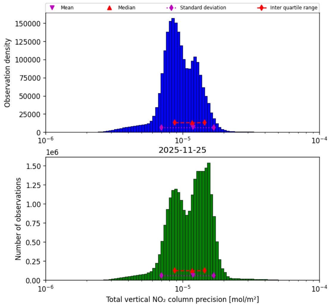
Figure 39: Histogram of “Total vertical NO 2 column precision” for 2025-11-24 to 2025-11-26
