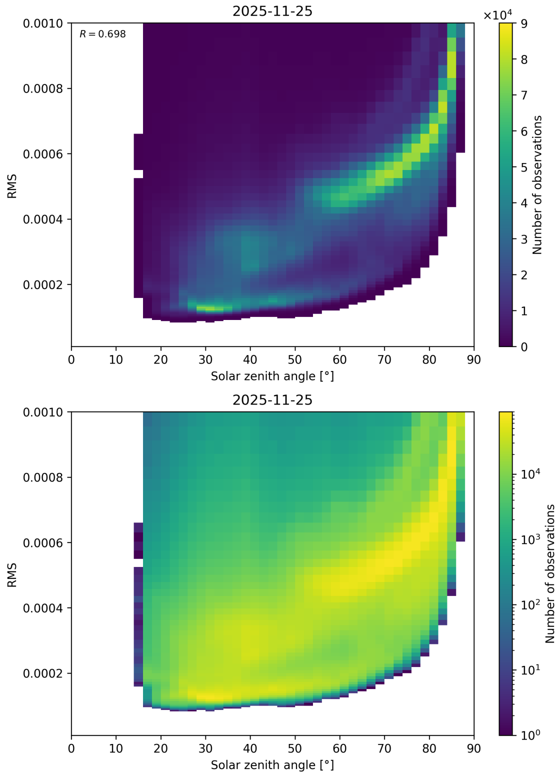
Figure 157: Scatter density plot of “Solar zenith angle” against “RMS” for 2025-11-24 to 2025-11-26.
