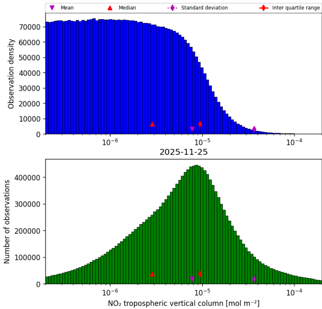
Figure 29: Histogram of “NO 2 tropospheric vertical column” for 2025-11-24 to 2025-11-26
