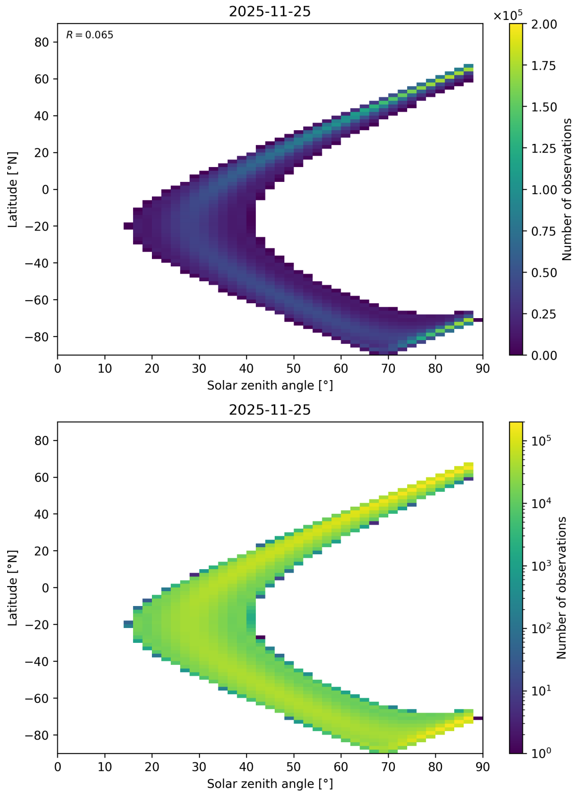
Figure 149: Scatter density plot of “Solar zenith angle” against “Latitude” for 2025-11-24 to 2025-11-26.
