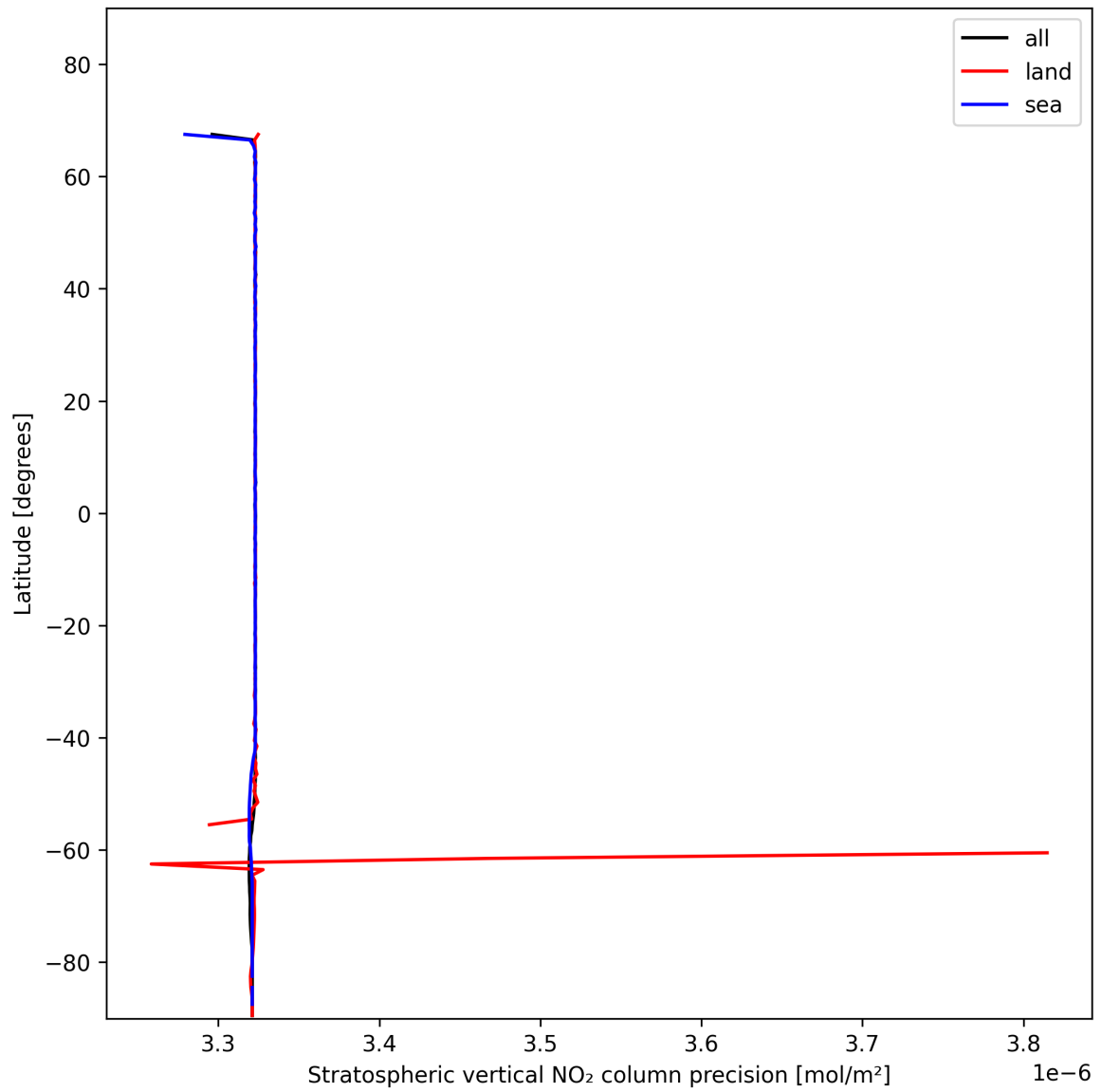
Figure 20: Zonal average of “Stratospheric vertical NO 2 column precision” for 2025-11-24 to 2025-11-26.
