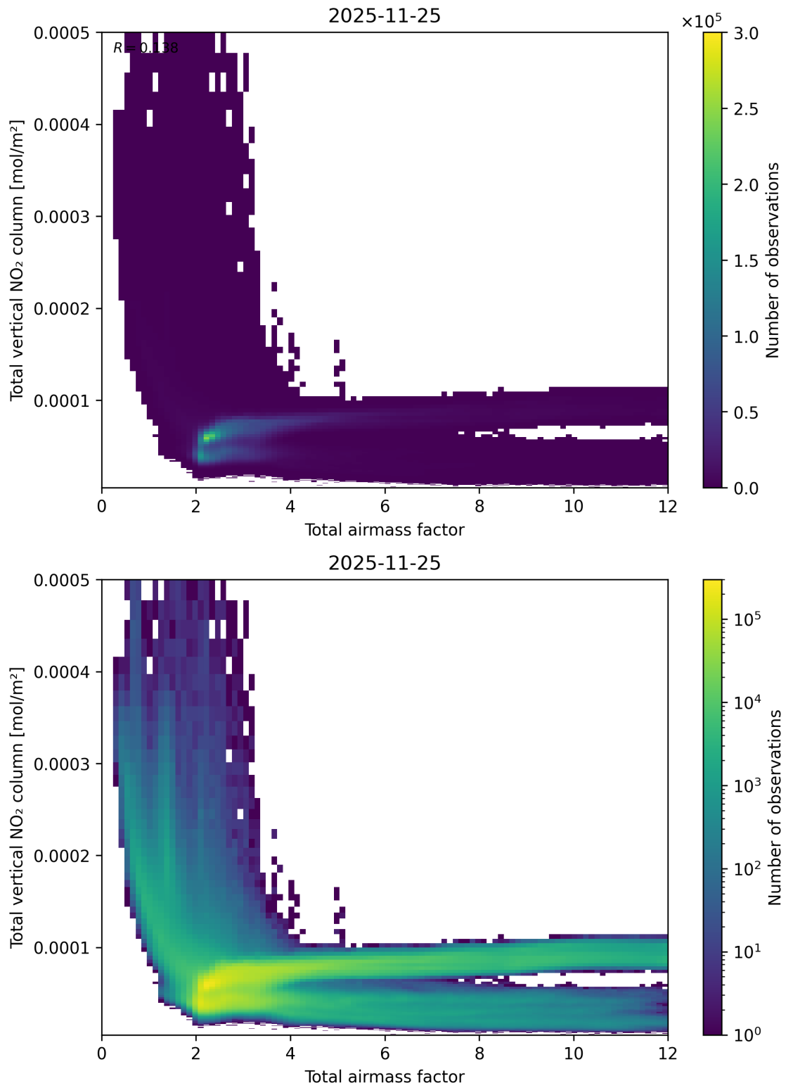
Figure 67: Scatter density plot of “Total airmass factor” against “Total vertical NO 2 column” for 2025-11-24 to 2025-11-26.
