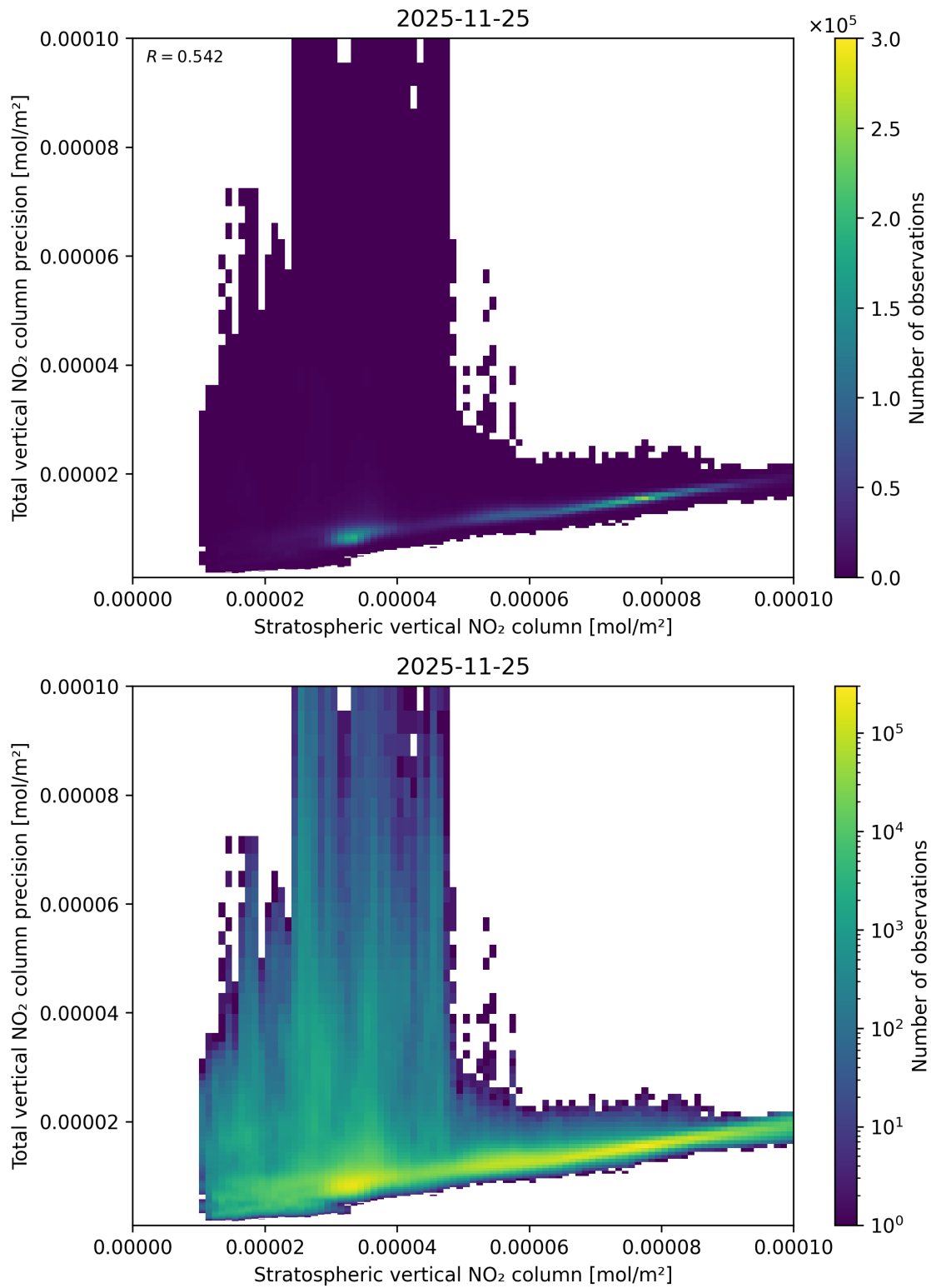
Figure 101: Scatter density plot of “Stratospheric vertical NO 2 column” against “Total vertical NO 2 column precision” for 2025-11-24 to 2025-11-26.
