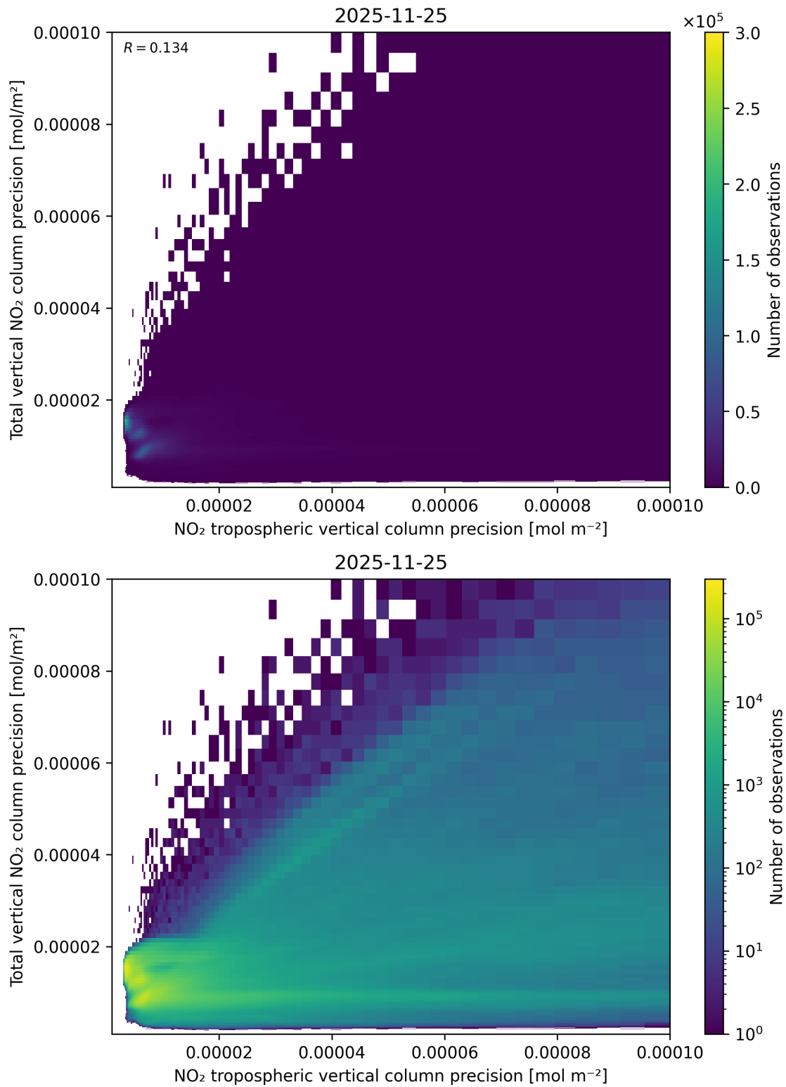
Figure 139: Scatter density plot of “NO 2 tropospheric vertical column precision” against “Total vertical NO 2 column precision” for 2025-11-24 to 2025-11-26.
