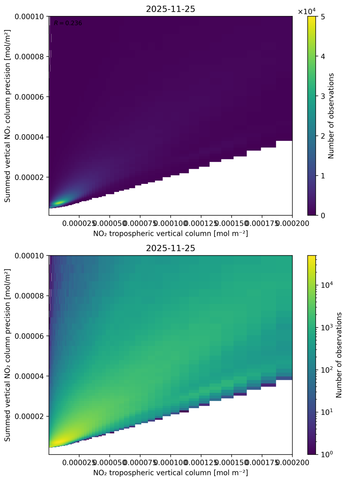
Figure 127: Scatter density plot of “NO 2 tropospheric vertical column” against “Summed vertical NO 2 column precision” for 2025-11-24 to 2025-11-26.
