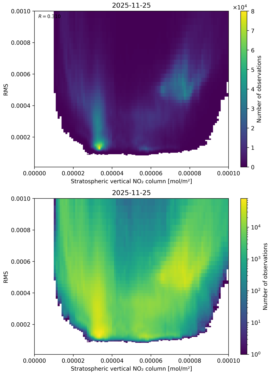
Figure 102: Scatter density plot of “Stratospheric vertical NO 2 column” against “RMS” for 2025-11-24 to 2025-11-26.
