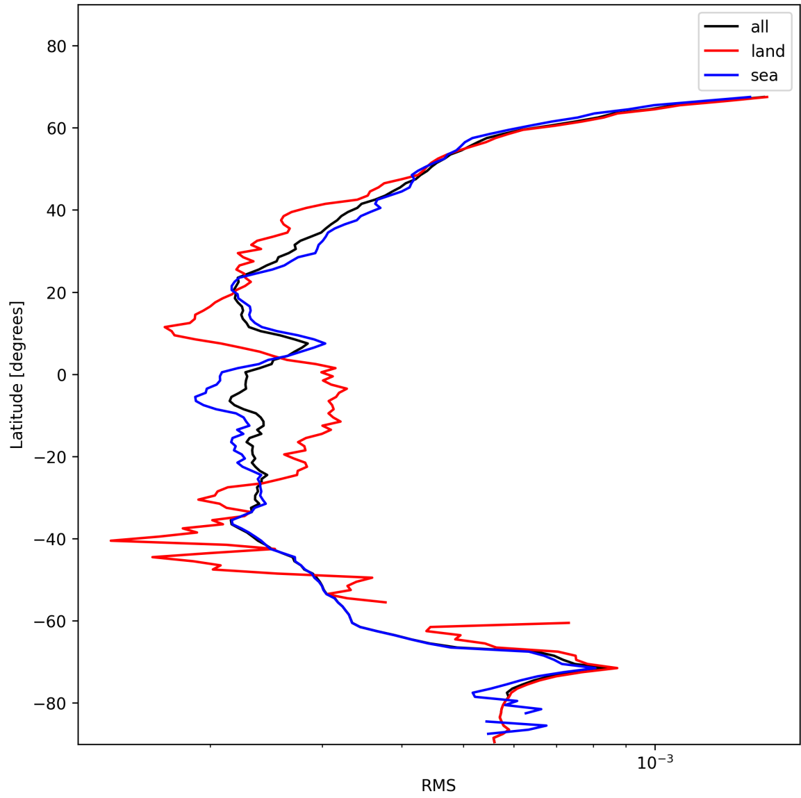
Figure 26: Zonal average of “RMS” for 2025-11-24 to 2025-11-26.
