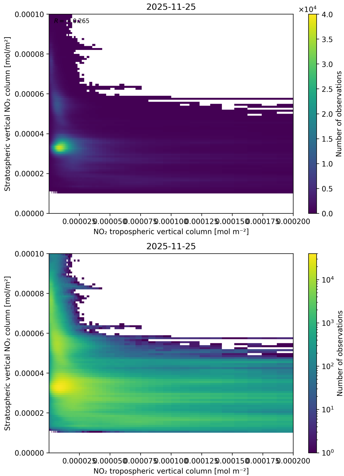
Figure 125: Scatter density plot of “NO 2 tropospheric vertical column” against “Stratospheric vertical NO 2 column” for 2025-11-24 to 2025-11-26.
