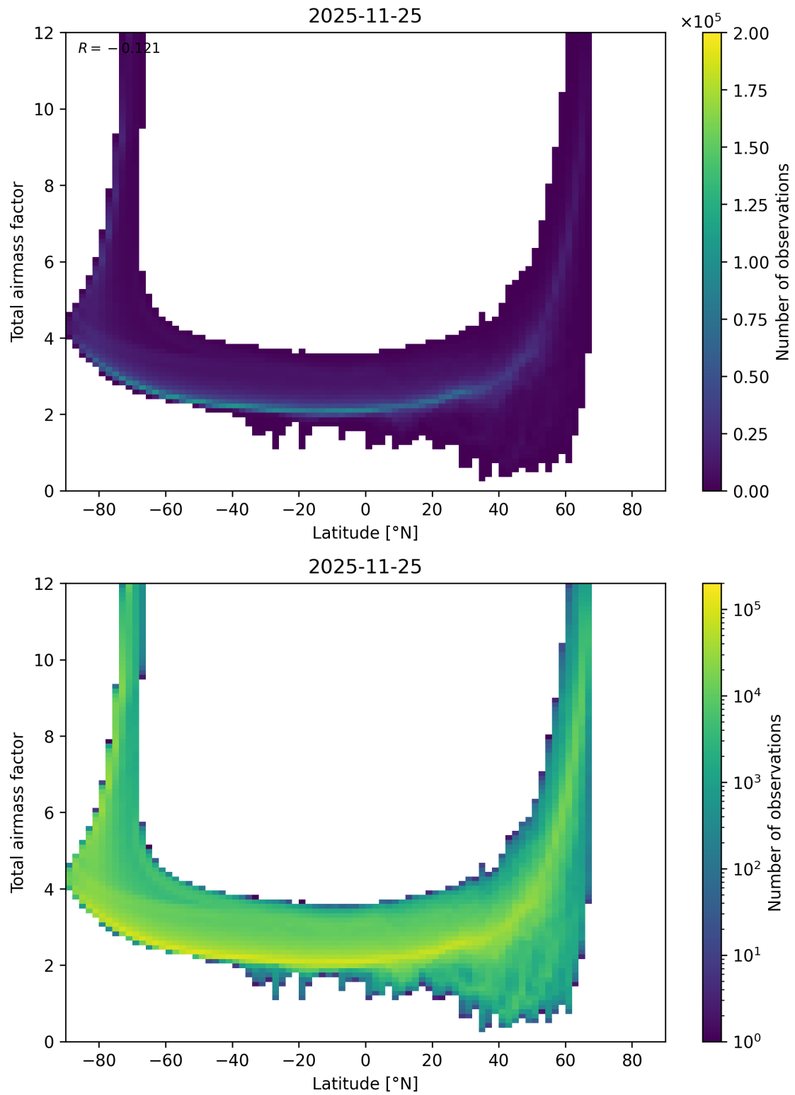
Figure 84: Scatter density plot of “Latitude” against “Total airmass factor” for 2025-11-24 to 2025-11-26.
