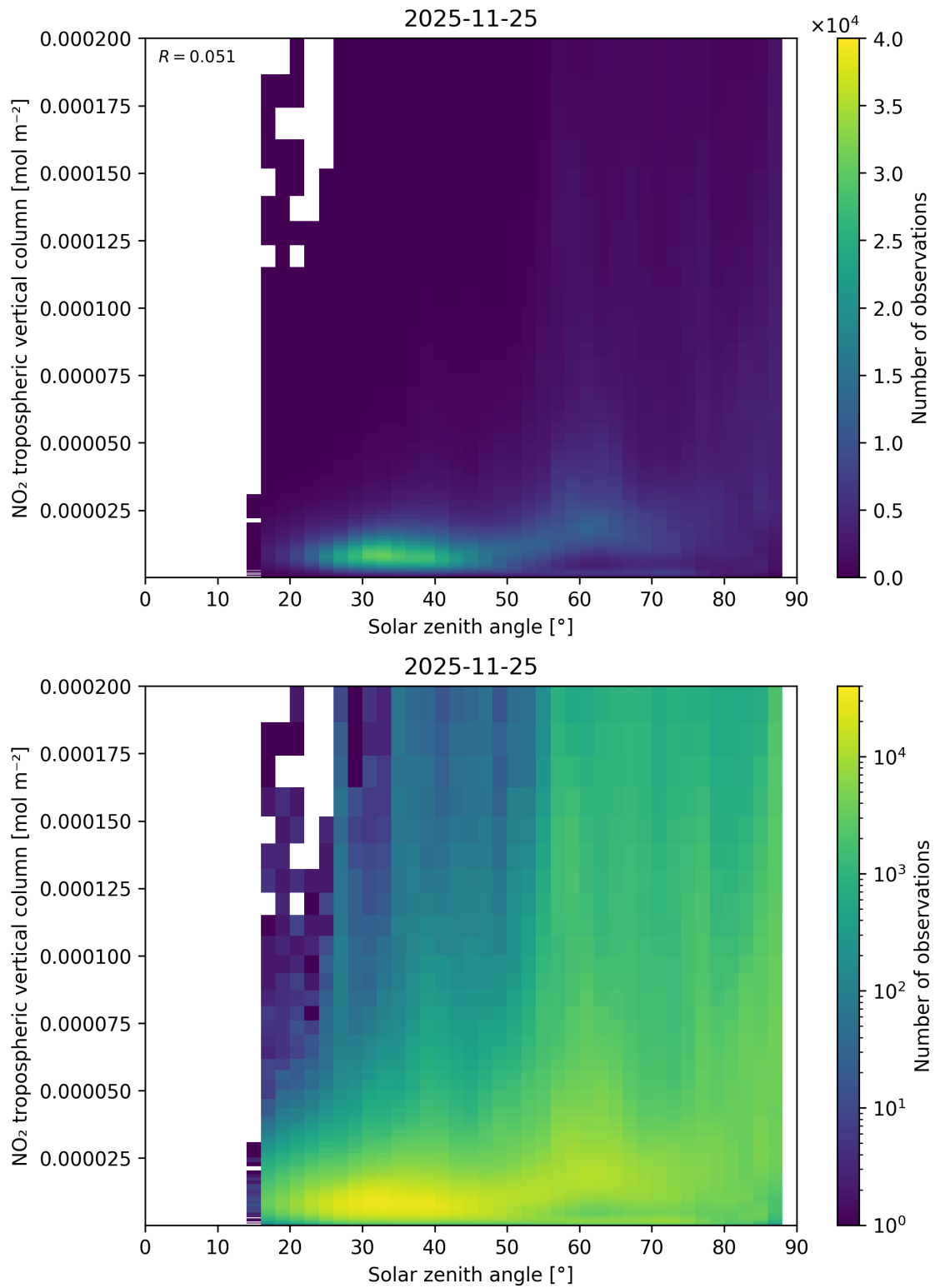
Figure 155: Scatter density plot of “Solar zenith angle” against “NO 2 tropospheric vertical column” for 2025-11-24 to 2025-11-26.
