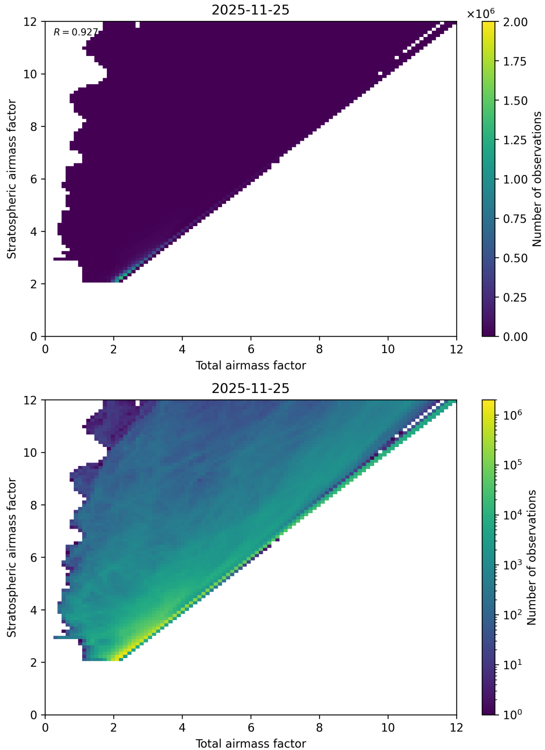
Figure 62: Scatter density plot of “Total airmass factor” against “Stratospheric airmass factor” for 2025-11-24 to 2025-11-26.
