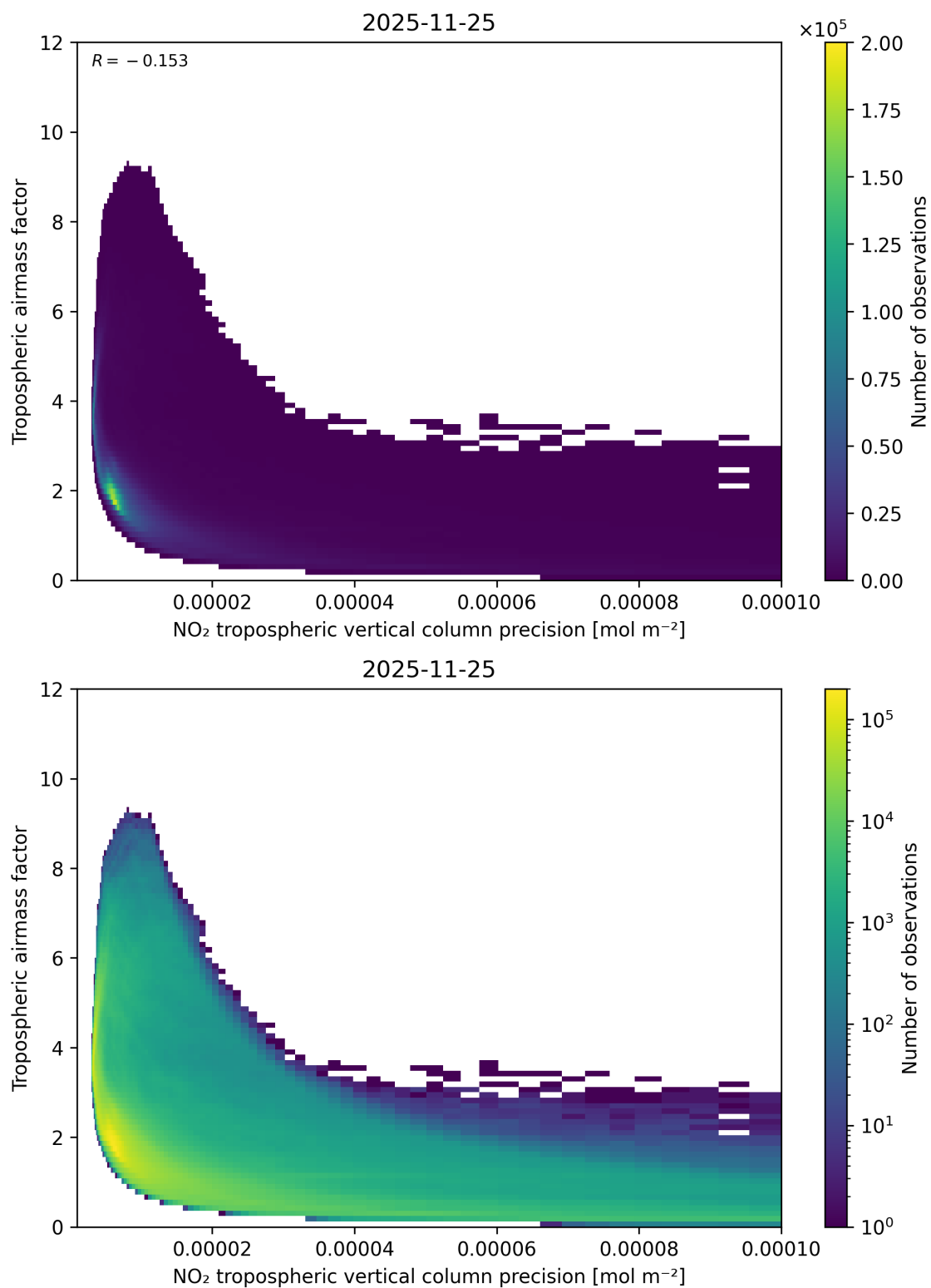
Figure 133: Scatter density plot of “NO 2 tropospheric vertical column precision” against “Tropospheric airmass factor” for 2025-11-24 to 2025-11-26.
