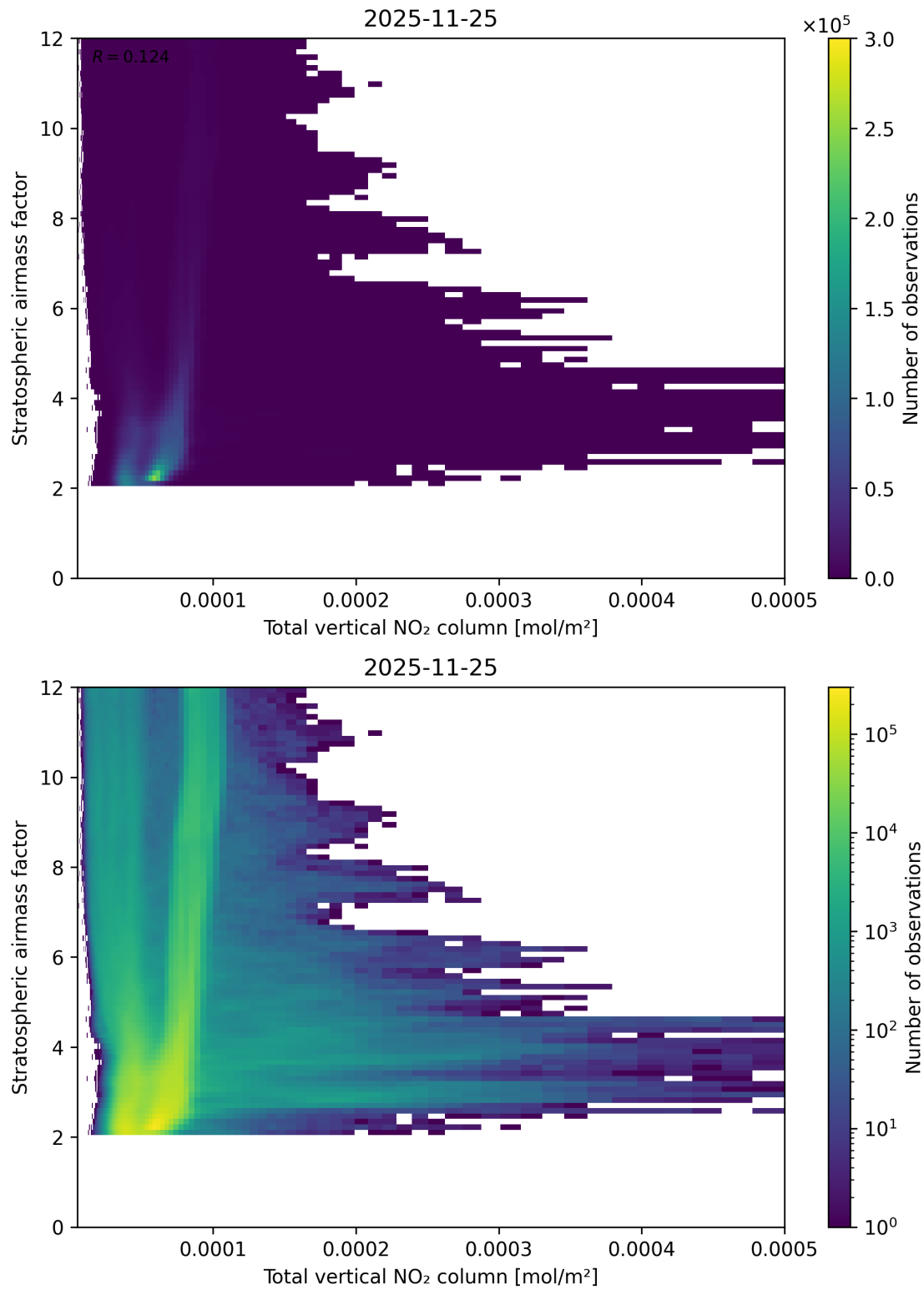
Figure 110: Scatter density plot of “Total vertical NO 2 column” against “Stratospheric air mass factor” for 2025-11-24 to 2025-11-26.
