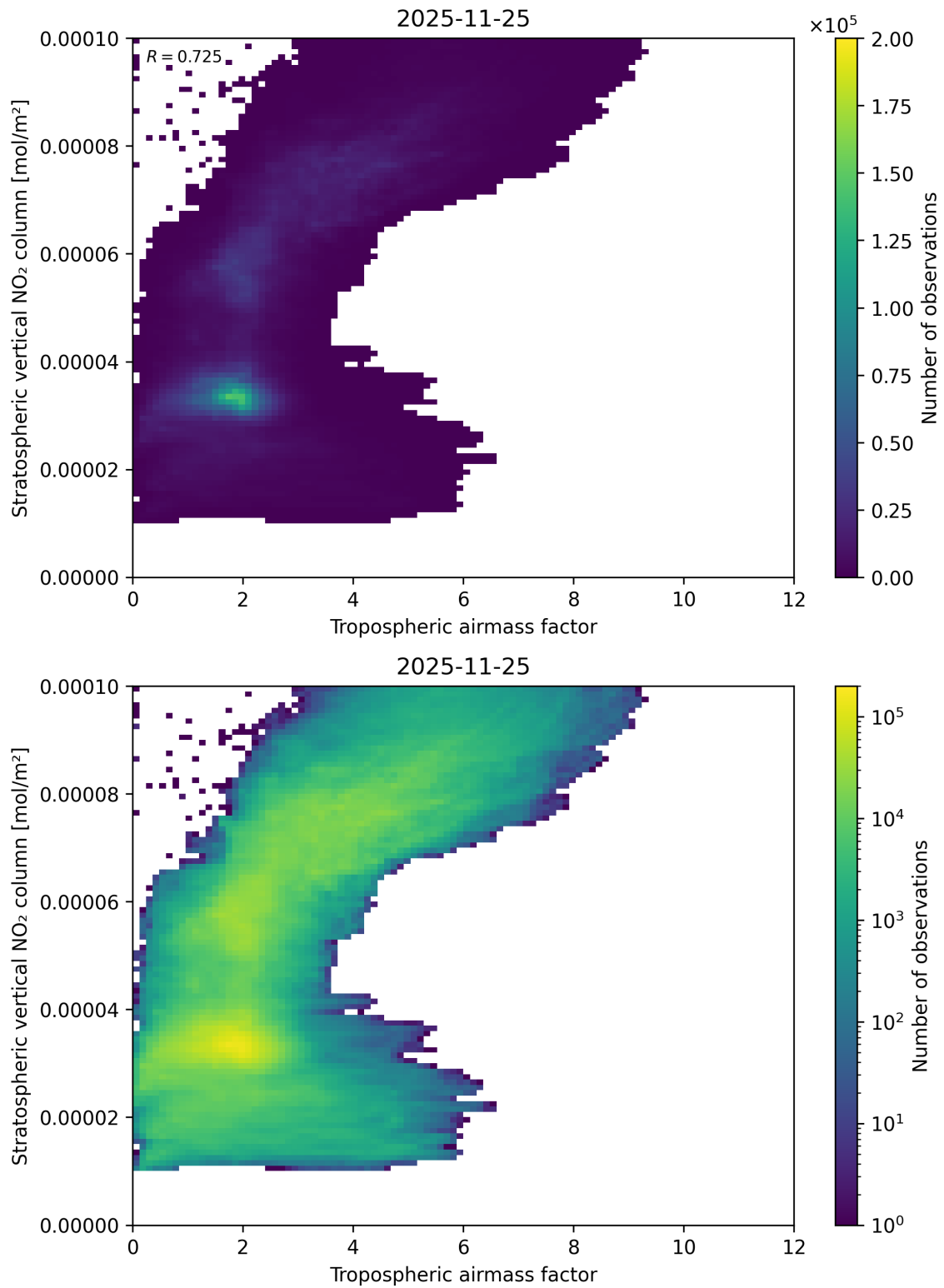
Figure 74: Scatter density plot of “Tropospheric air mass factor” against “Stratospheric vertical NO 2 column” for 2025-11-24 to 2025-11-26.
