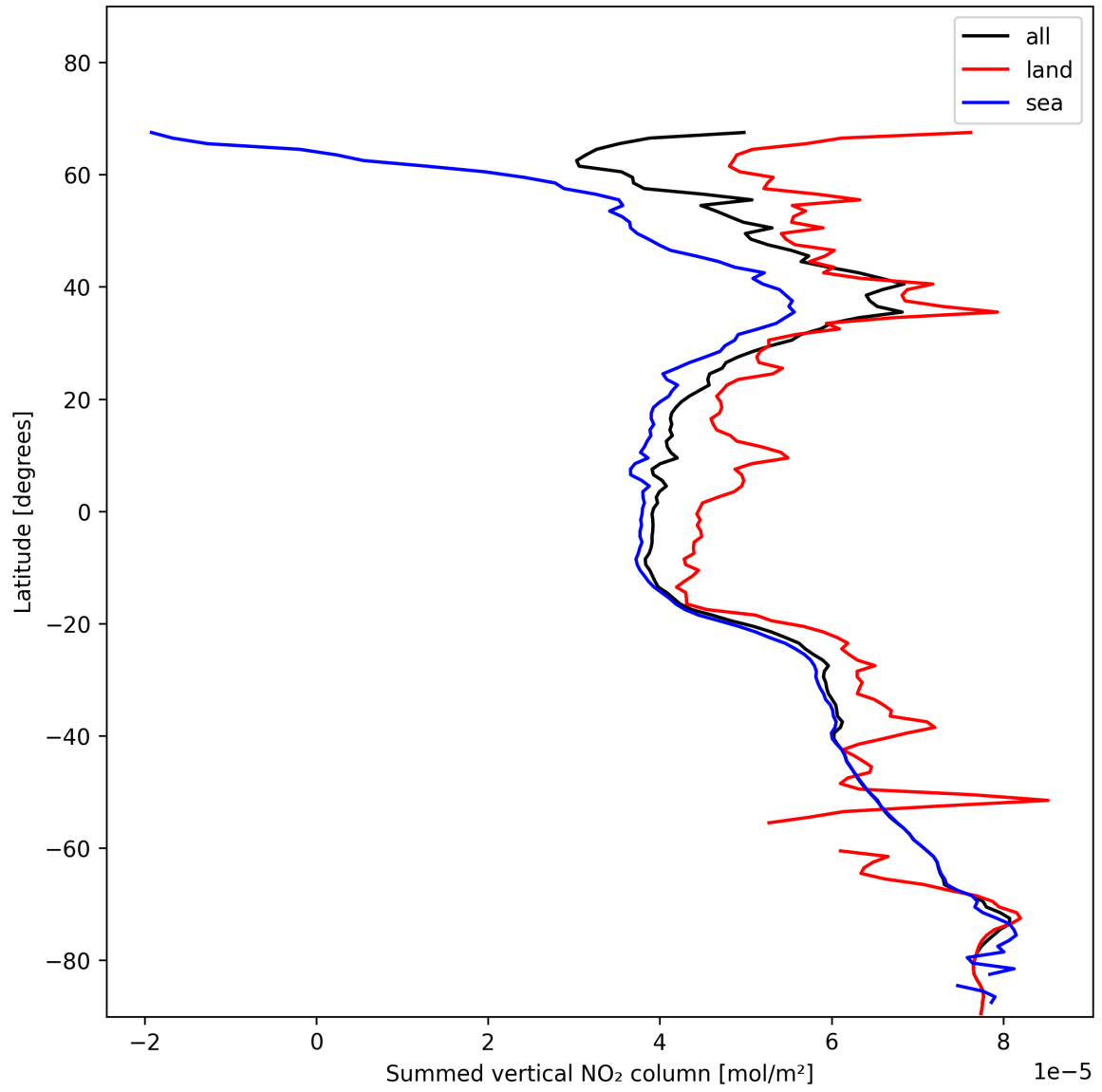
Figure 23: Zonal average of “Summed vertical NO 2 column” for 2025-11-24 to 2025-11-26.
