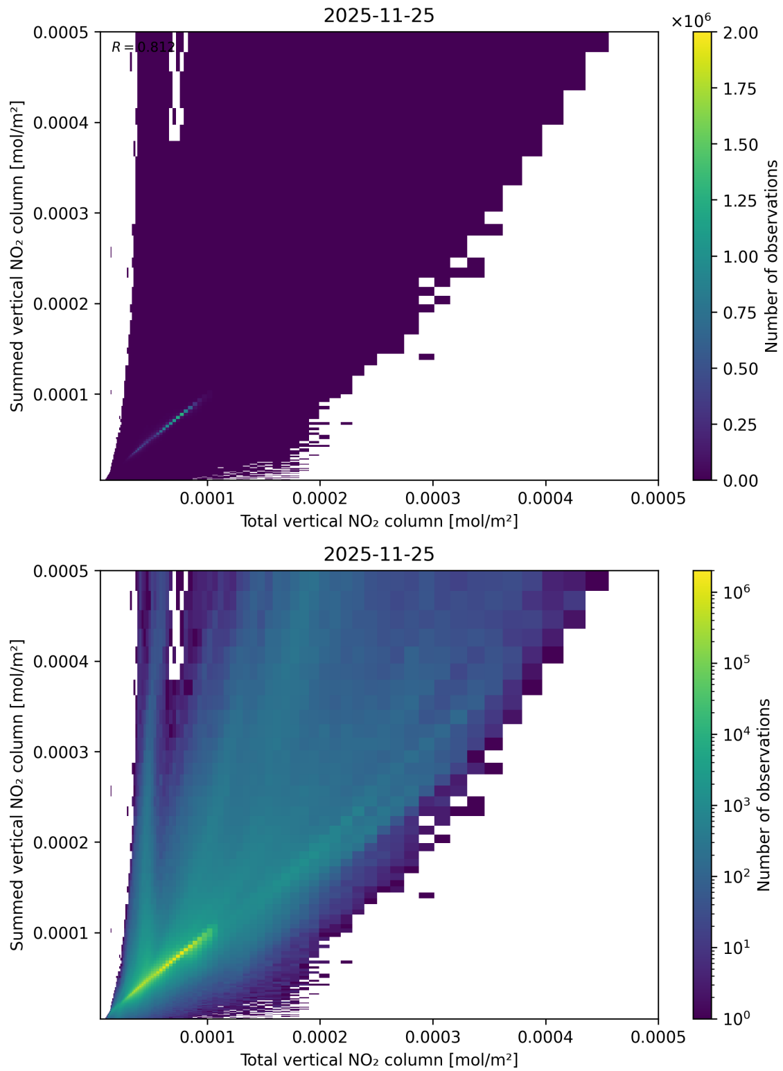
Figure 112: Scatter density plot of “Total vertical NO 2 column” against “Summed vertical NO 2 column” for 2025-11-24 to 2025-11-26.
