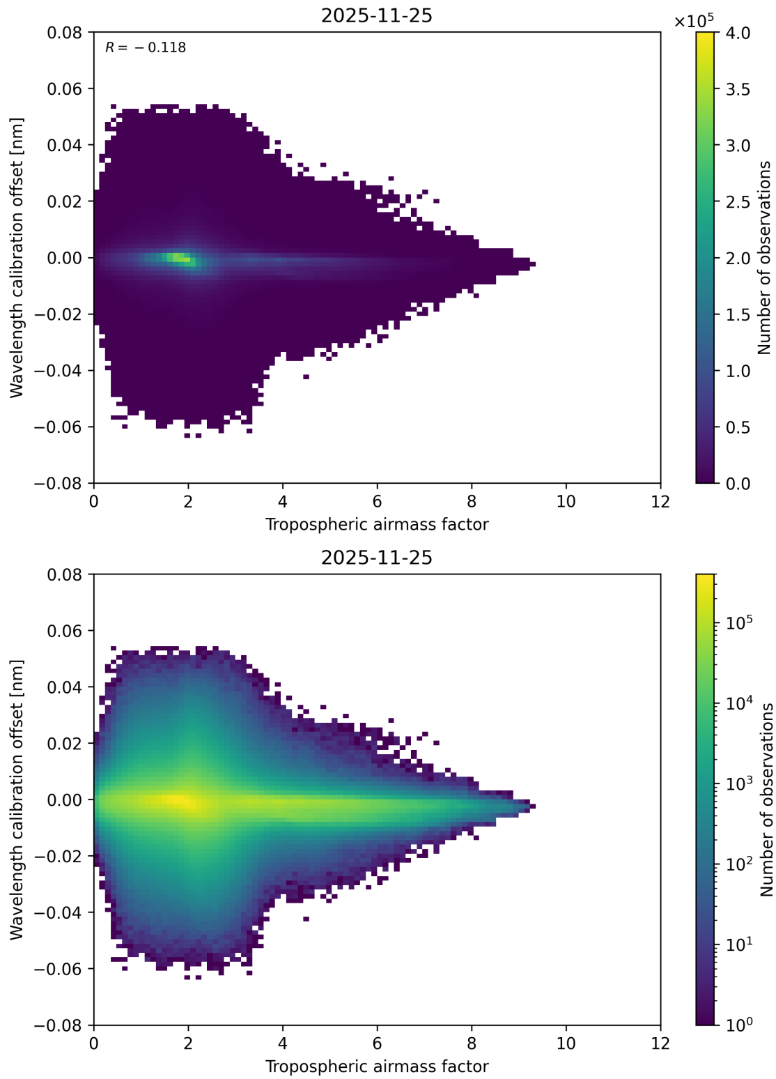
Figure 80: Scatter density plot of “Tropospheric airmass factor” against “Wavelength calibration offset” for 2025-11-24 to 2025-11-26.
