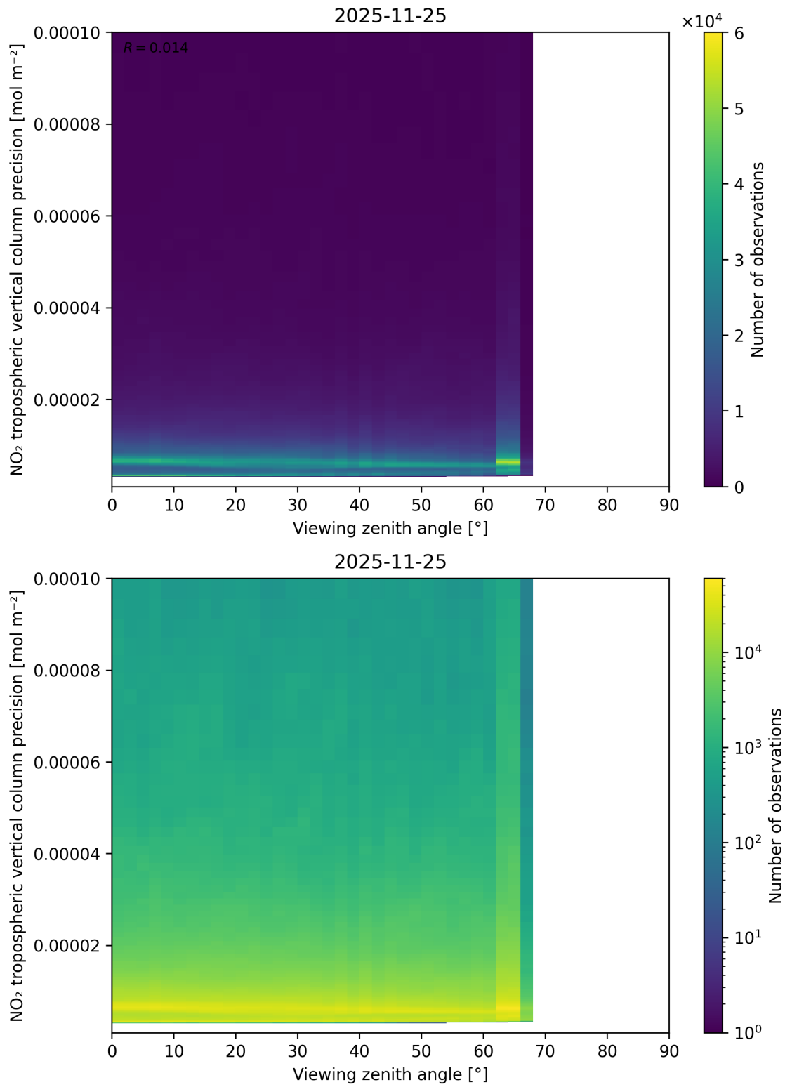
Figure 170: Scatter density plot of “Viewing zenith angle” against “NO 2 tropospheric vertical column precision” for 2025-11-24 to 2025-11-26.
