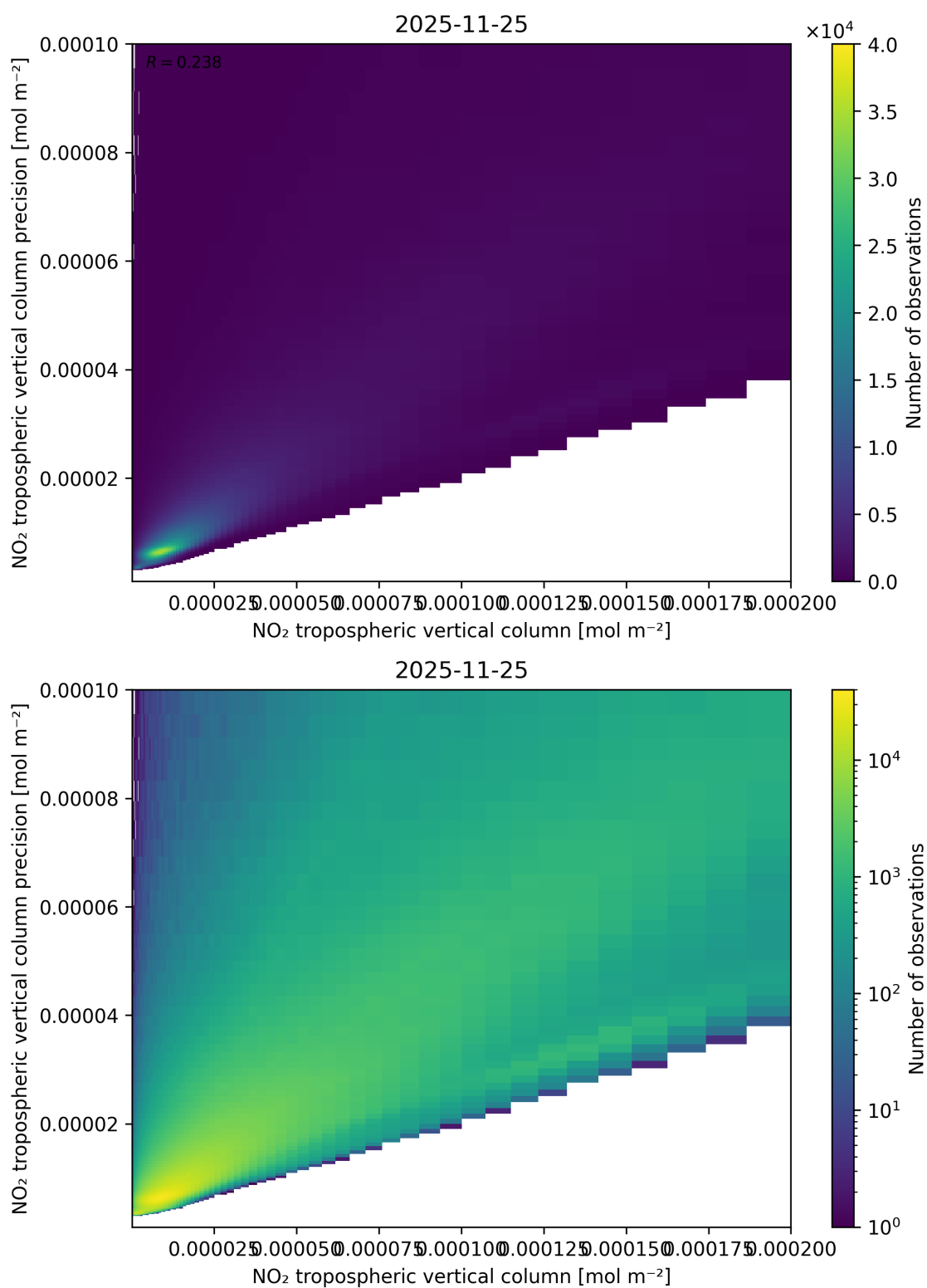
Figure 130: Scatter density plot of “NO 2 tropospheric vertical column” against “NO 2 tropospheric vertical column precision” for 2025-11-24 to 2025-11-26.
