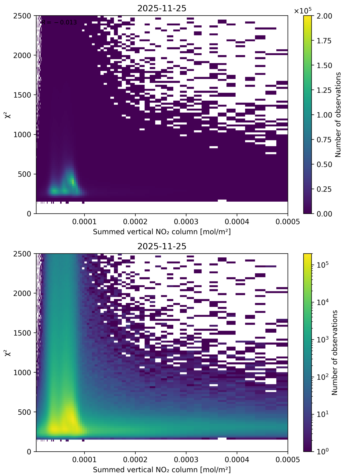
Figure 104: Scatter density plot of “Summed vertical NO 2 column” against “ \chi^2 ” for 2025-11-24 to 2025-11-26.
