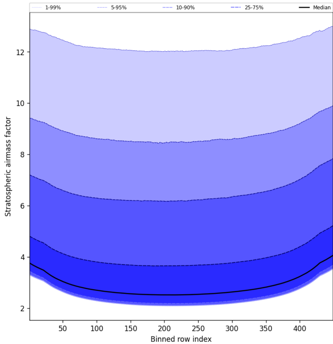
Figure 61: Along track statistics of “Stratospheric air mass factor” for 2025-11-24 to 2025-11-26
