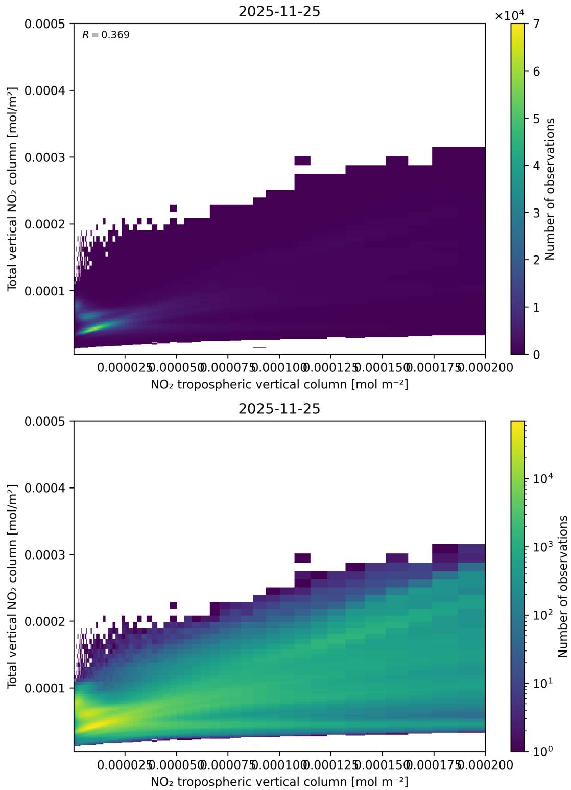
Figure 128: Scatter density plot of “NO 2 tropospheric vertical column” against “Total vertical NO 2 column” for 2025-11-24 to 2025-11-26.
