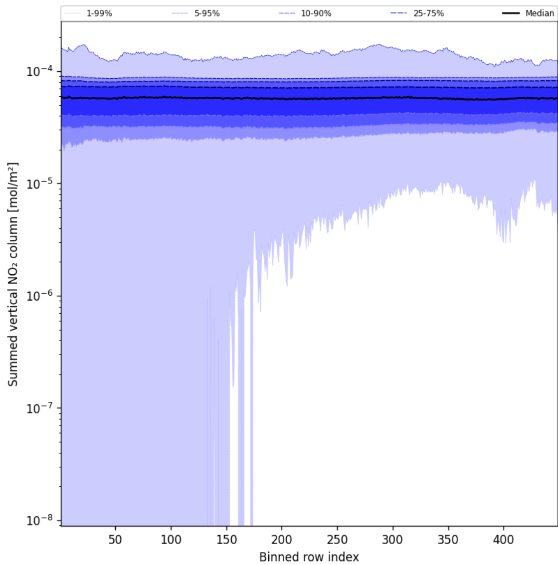
Figure 57: Along track statistics of “Summed vertical NO 2 column” for 2025-11-24 to 2025-11-26
