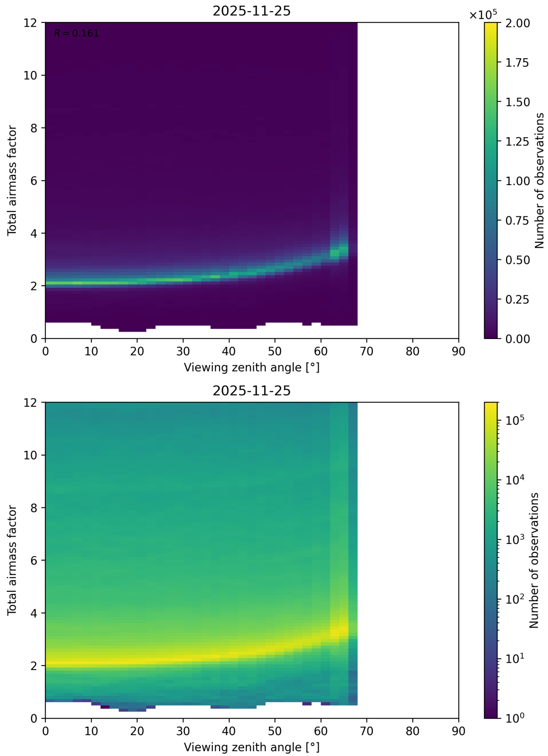
Figure 160: Scatter density plot of “Viewing zenith angle” against “Total airmass factor” for 2025-11-24 to 2025-11-26.
