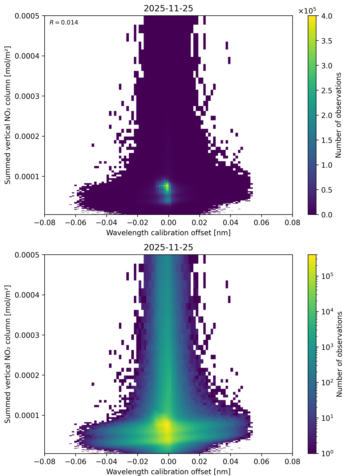
Figure 177: Scatter density plot of “Wavelength calibration offset” against “Summed vertical NO 2 column” for 2025-11-24 to 2025-11-26.
