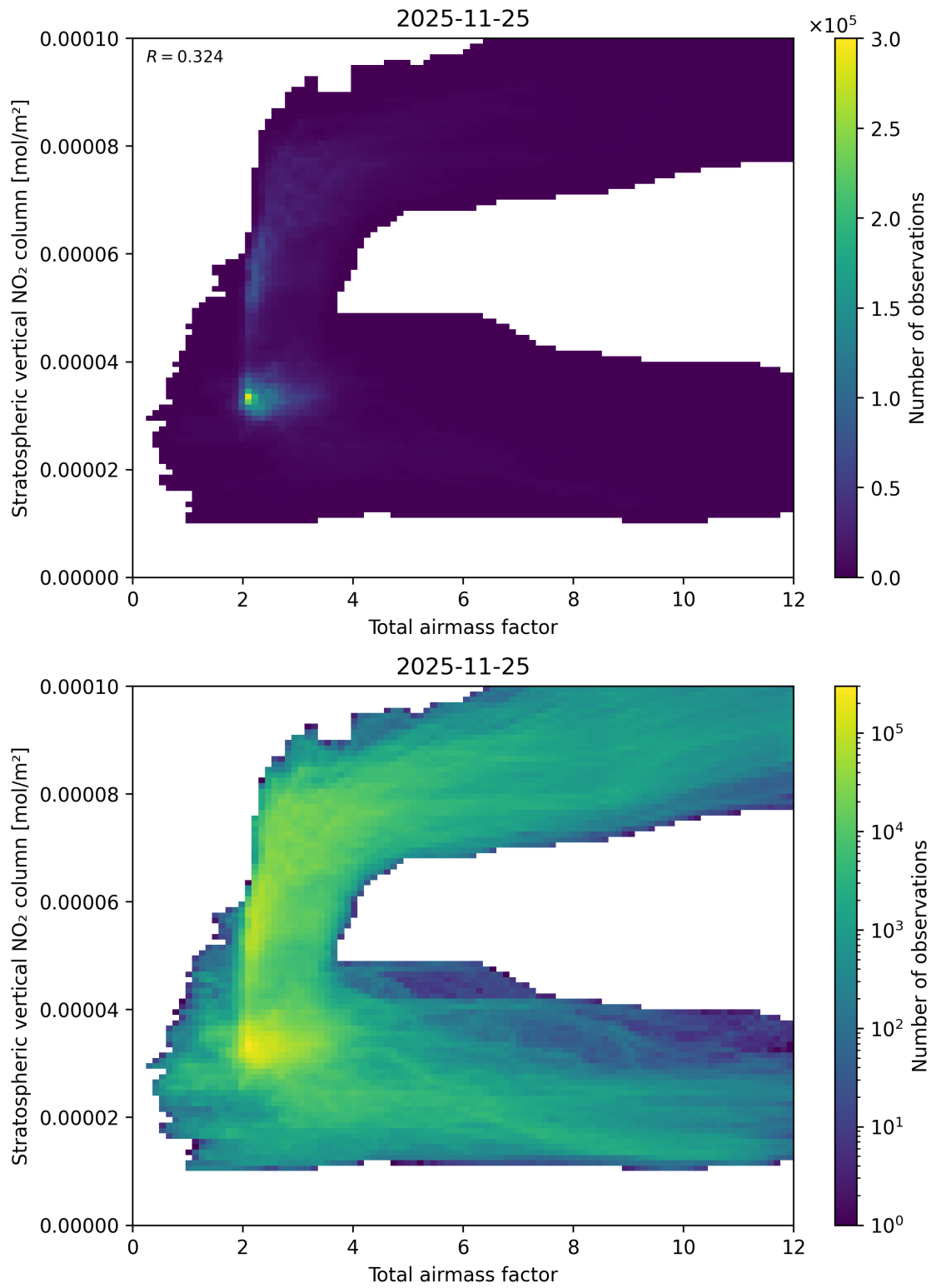
Figure 64: Scatter density plot of “Total airmass factor” against “Stratospheric vertical NO 2 column” for 2025-11-24 to 2025-11-26.
