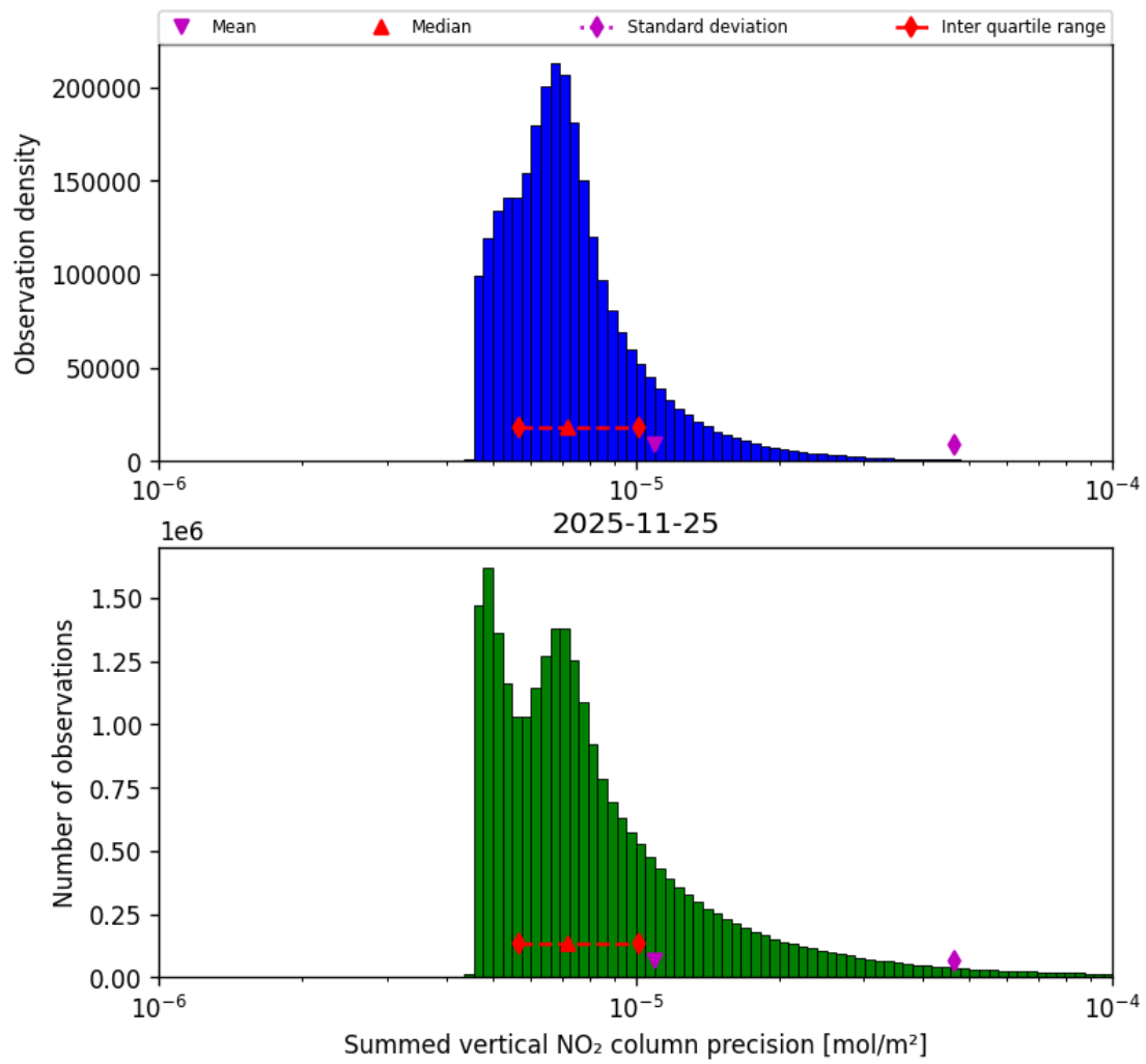
Figure 41: Histogram of “Summed vertical NO 2 column precision” for 2025-11-24 to 2025-11-26
