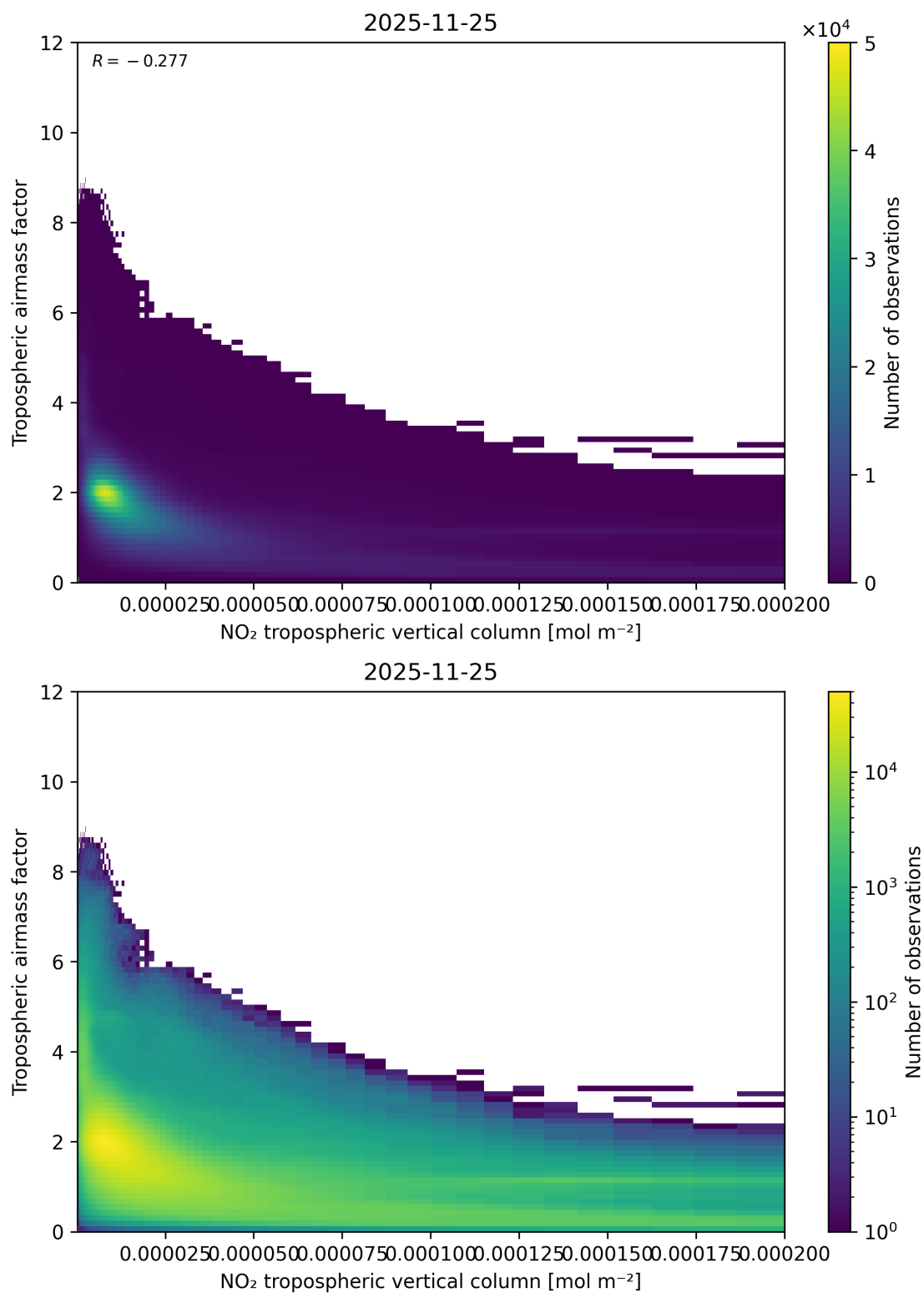
Figure 123: Scatter density plot of “NO 2 tropospheric vertical column” against “Tropospheric air mass factor” for 2025-11-24 to 2025-11-26.
