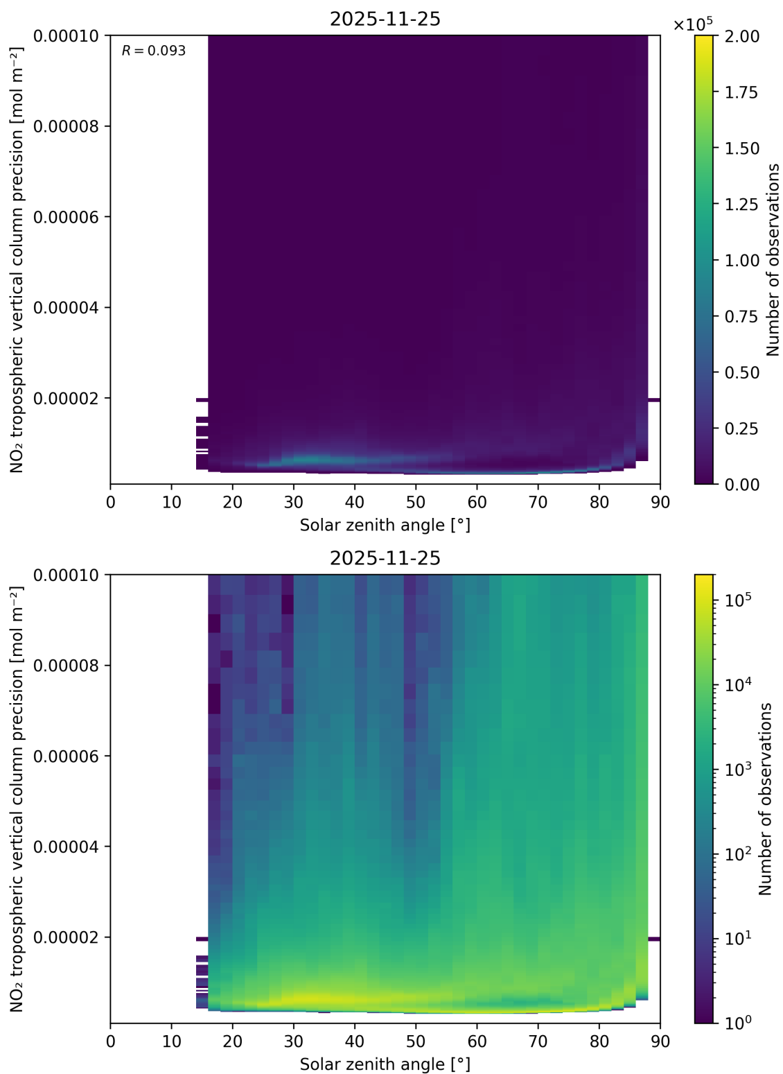
Figure 156: Scatter density plot of “Solar zenith angle” against “NO 2 tropospheric vertical column precision” for 2025-11-24 to 2025-11-26.
