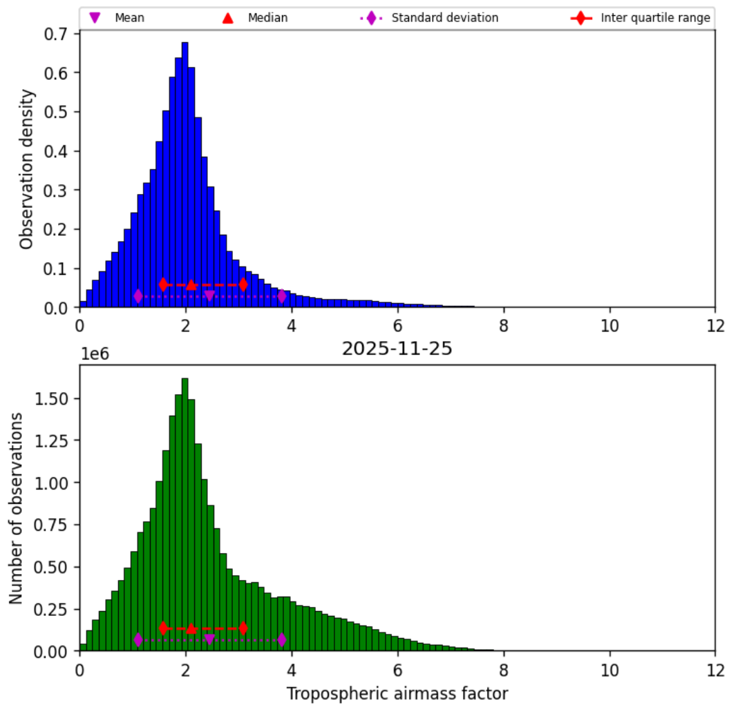
Figure 31: Histogram of “Tropospheric airmass factor” for 2025-11-24 to 2025-11-26
