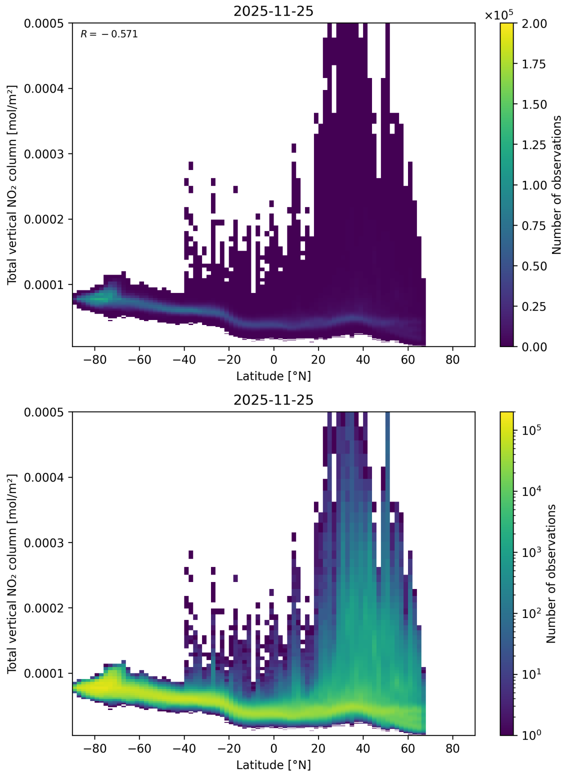
Figure 90: Scatter density plot of “Latitude” against “Total vertical NO 2 column” for 2025-11-24 to 2025-11-26.
