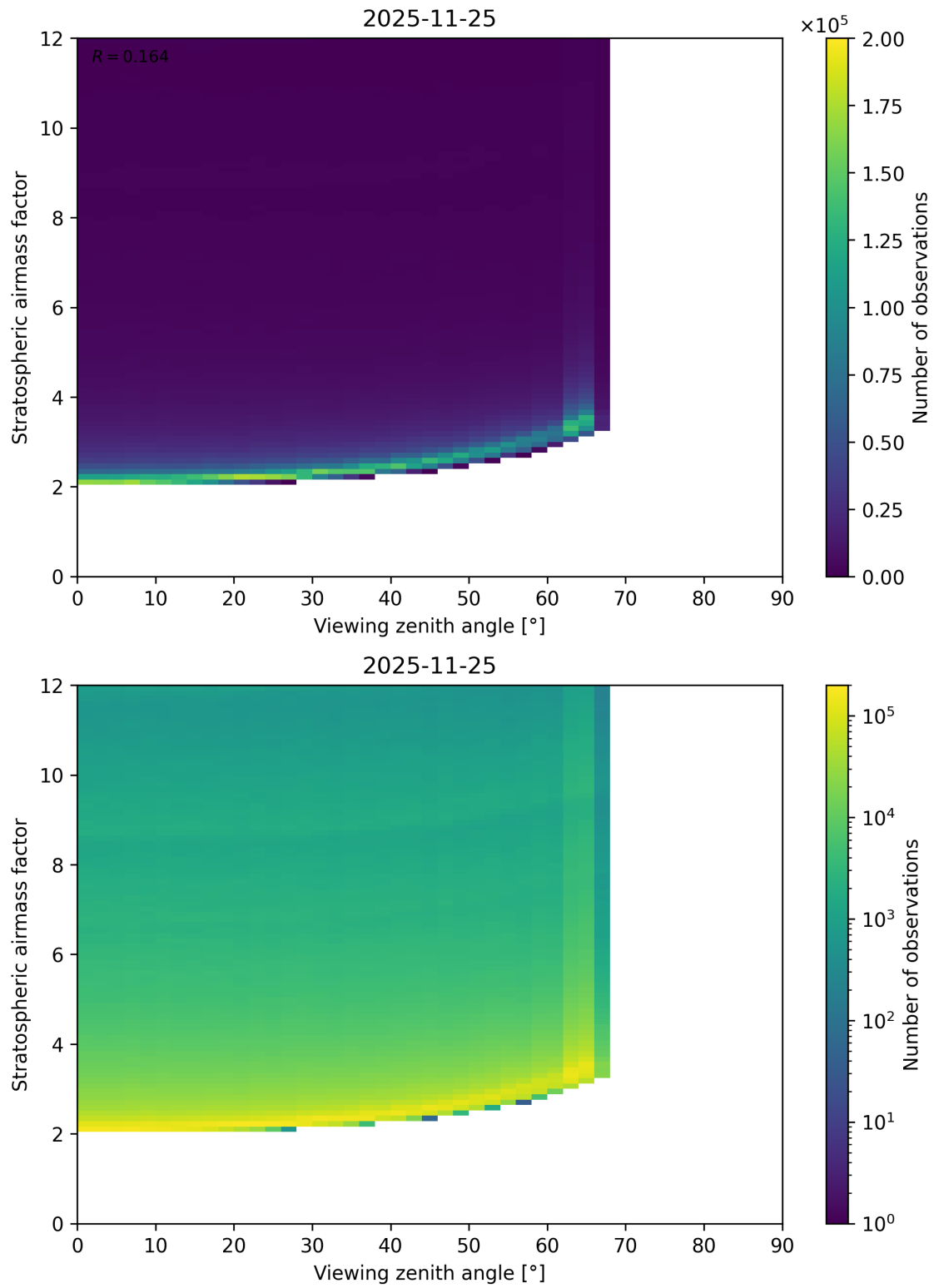
Figure 159: Scatter density plot of “Viewing zenith angle” against “Stratospheric airmass factor” for 2025-11-24 to 2025-11-26.
