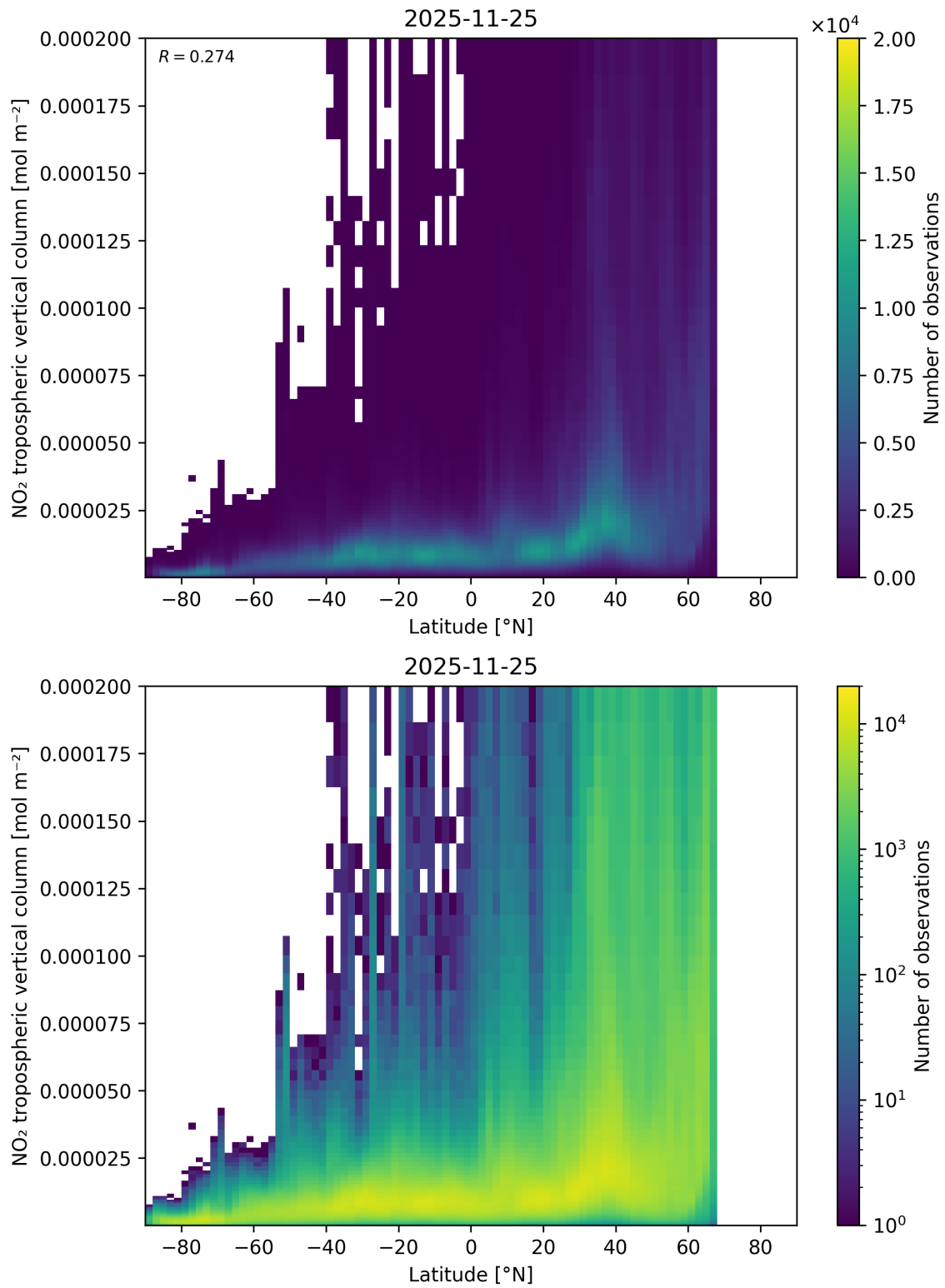
Figure 92: Scatter density plot of “Latitude” against “NO 2 tropospheric vertical column” for 2025-11-24 to 2025-11-26.
