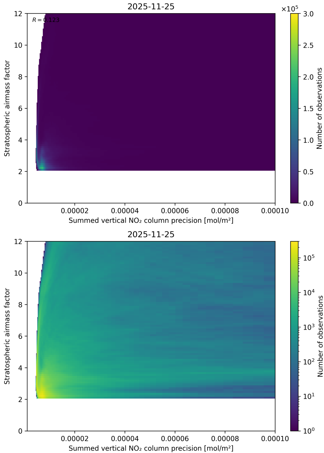
Figure 106: Scatter density plot of “Summed vertical NO 2 column precision” against “Stratospheric airmass factor” for 2025-11-24 to 2025-11-26.
