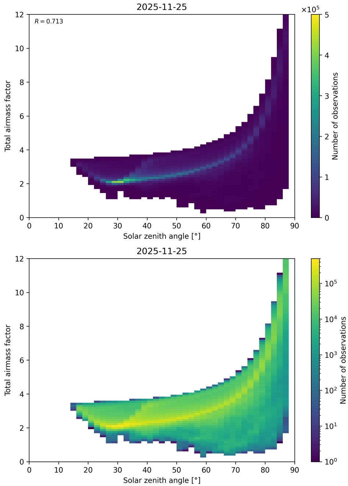
Figure 146: Scatter density plot of “Solar zenith angle” against “Total air mass factor” for 2025-11-24 to 2025-11-26.
