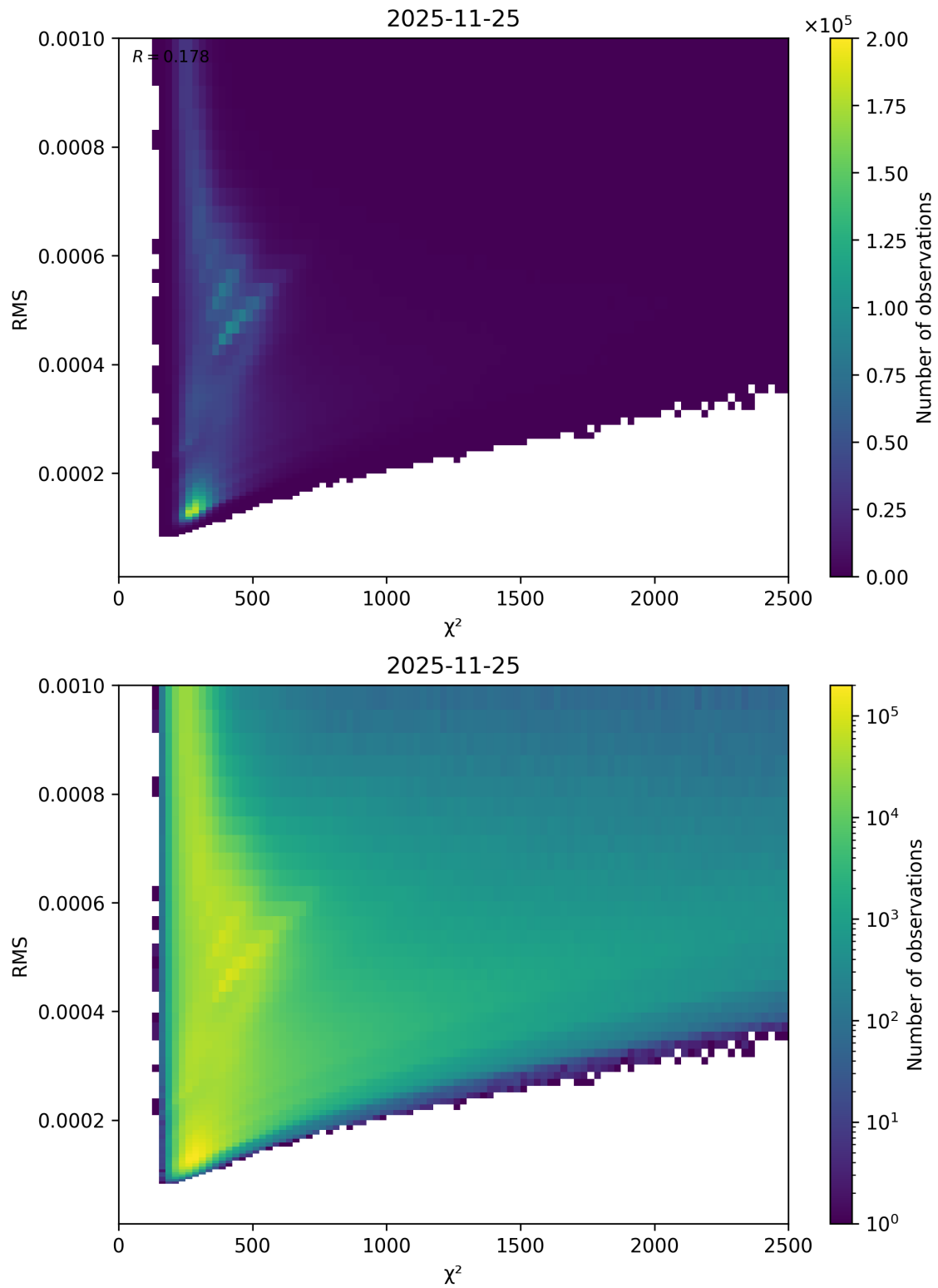
Figure 82: Scatter density plot of “ \chi^2 ” against “RMS” for 2025-11-24 to 2025-11-26.
