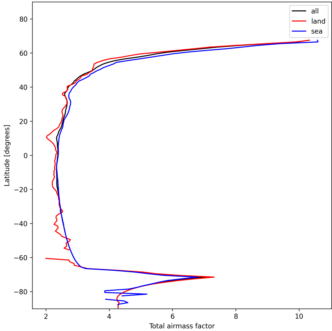
Figure 15: Zonal average of “Total airmass factor” for 2025-11-24 to 2025-11-26.
