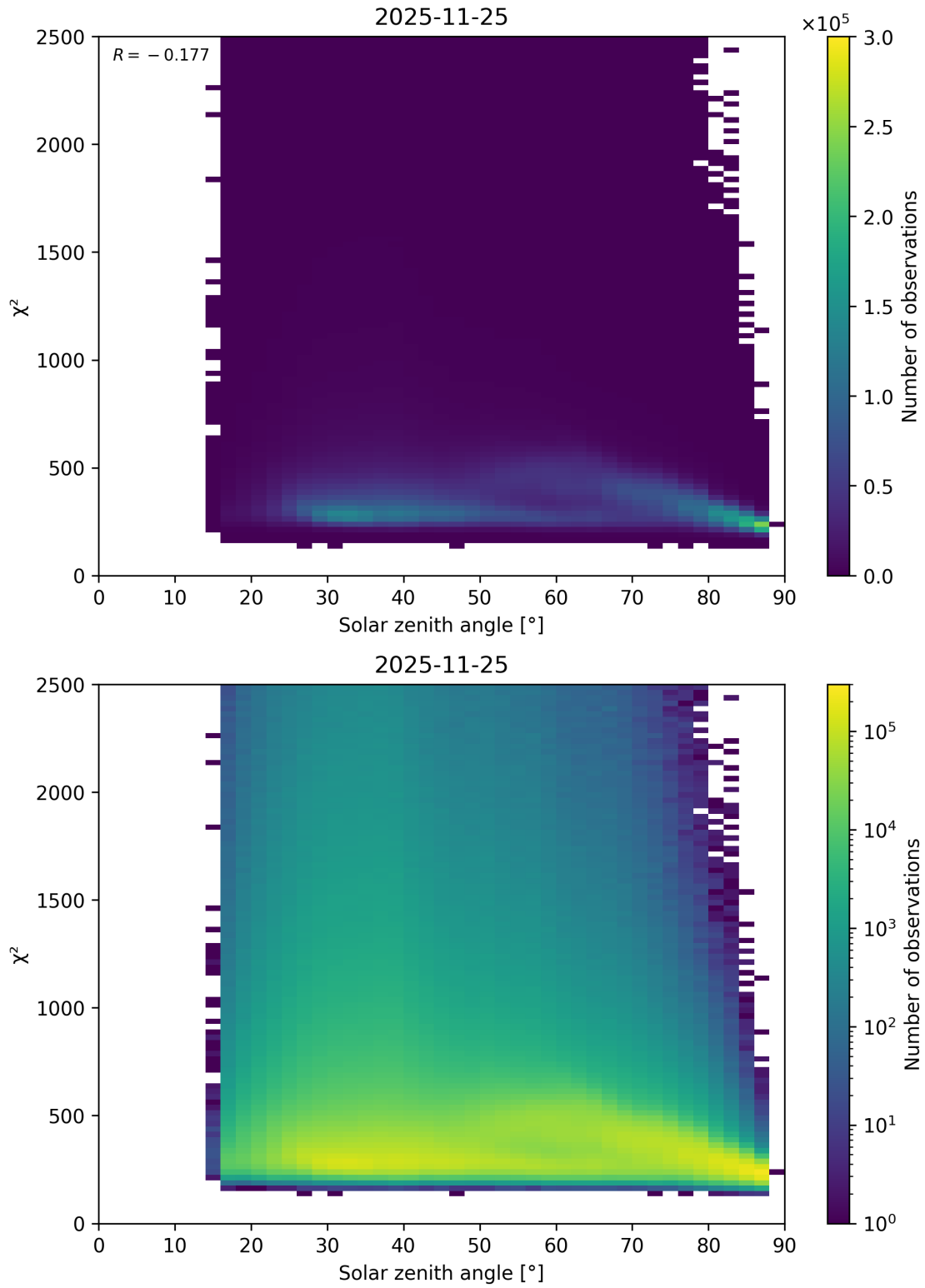
Figure 148: Scatter density plot of “Solar zenith angle” against “ \chi^2 ” for 2025-11-24 to 2025-11-26.
