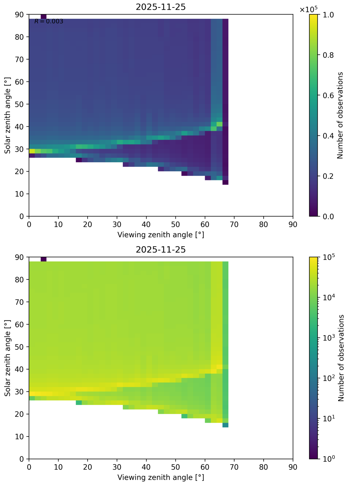
Figure 172: Scatter density plot of “Viewing zenith angle” against “Solar zenith angle” for 2025-11-24 to 2025-11-26.
