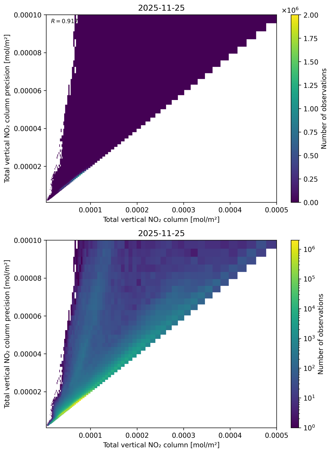
Figure 114: Scatter density plot of “Total vertical NO 2 column” against “Total vertical NO 2 column precision” for 2025-11-24 to 2025-11-26.
