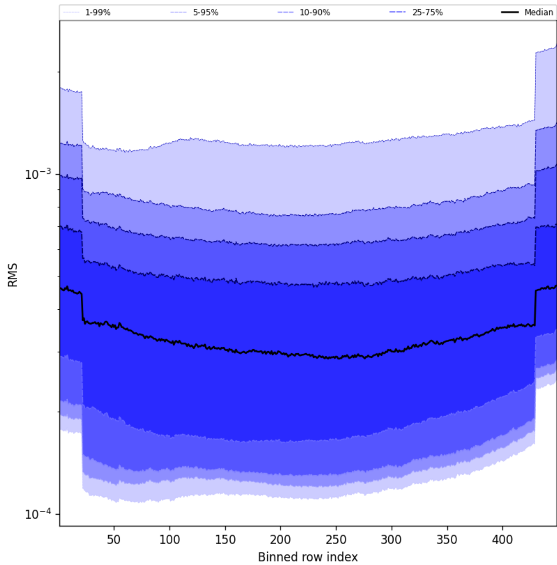
Figure 60: Along track statistics of “RMS” for 2025-11-24 to 2025-11-26
