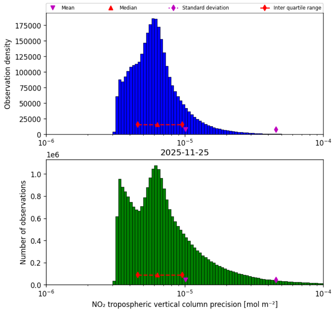
Figure 30: Histogram of “NO 2 tropospheric vertical column precision” for 2025-11-24 to 2025-11-26
