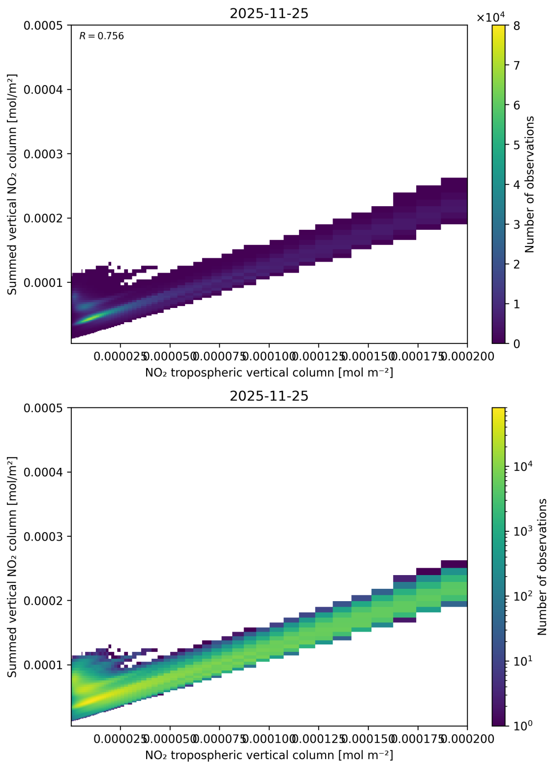
Figure 126: Scatter density plot of “NO 2 tropospheric vertical column” against “Summed vertical NO 2 column” for 2025-11-24 to 2025-11-26.
