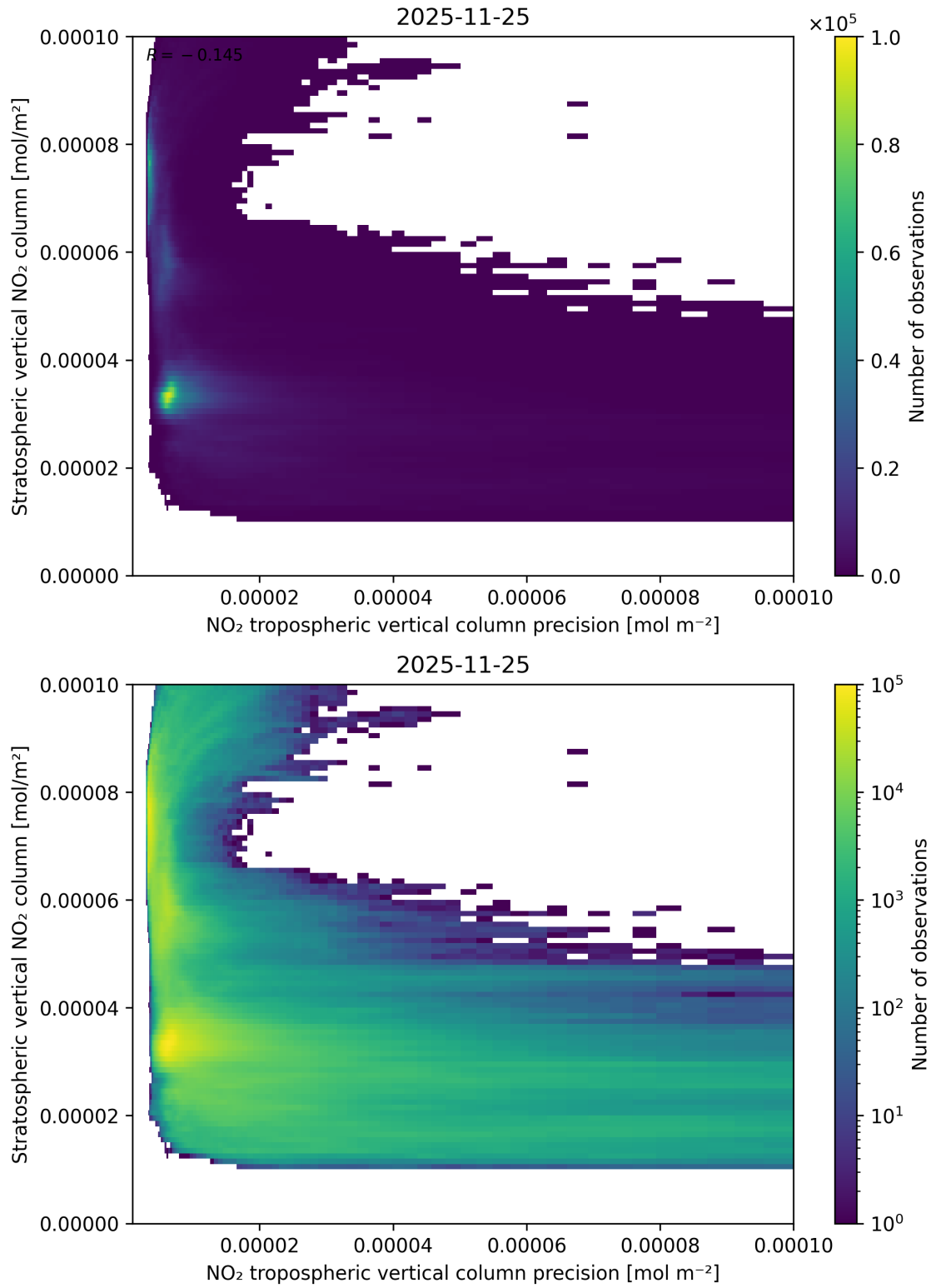
Figure 135: Scatter density plot of “NO 2 tropospheric vertical column precision” against “Stratospheric vertical NO 2 column” for 2025-11-24 to 2025-11-26.
