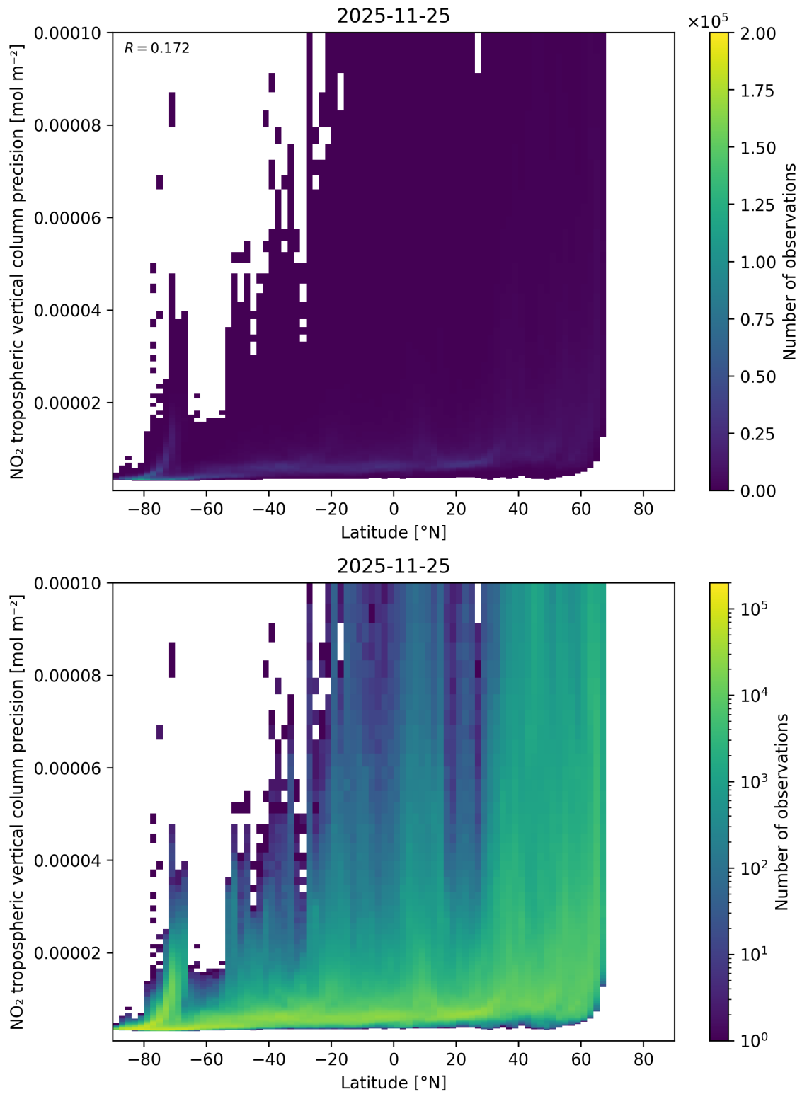
Figure 93: Scatter density plot of “Latitude” against “NO 2 tropospheric vertical column precision” for 2025-11-24 to 2025-11-26.
