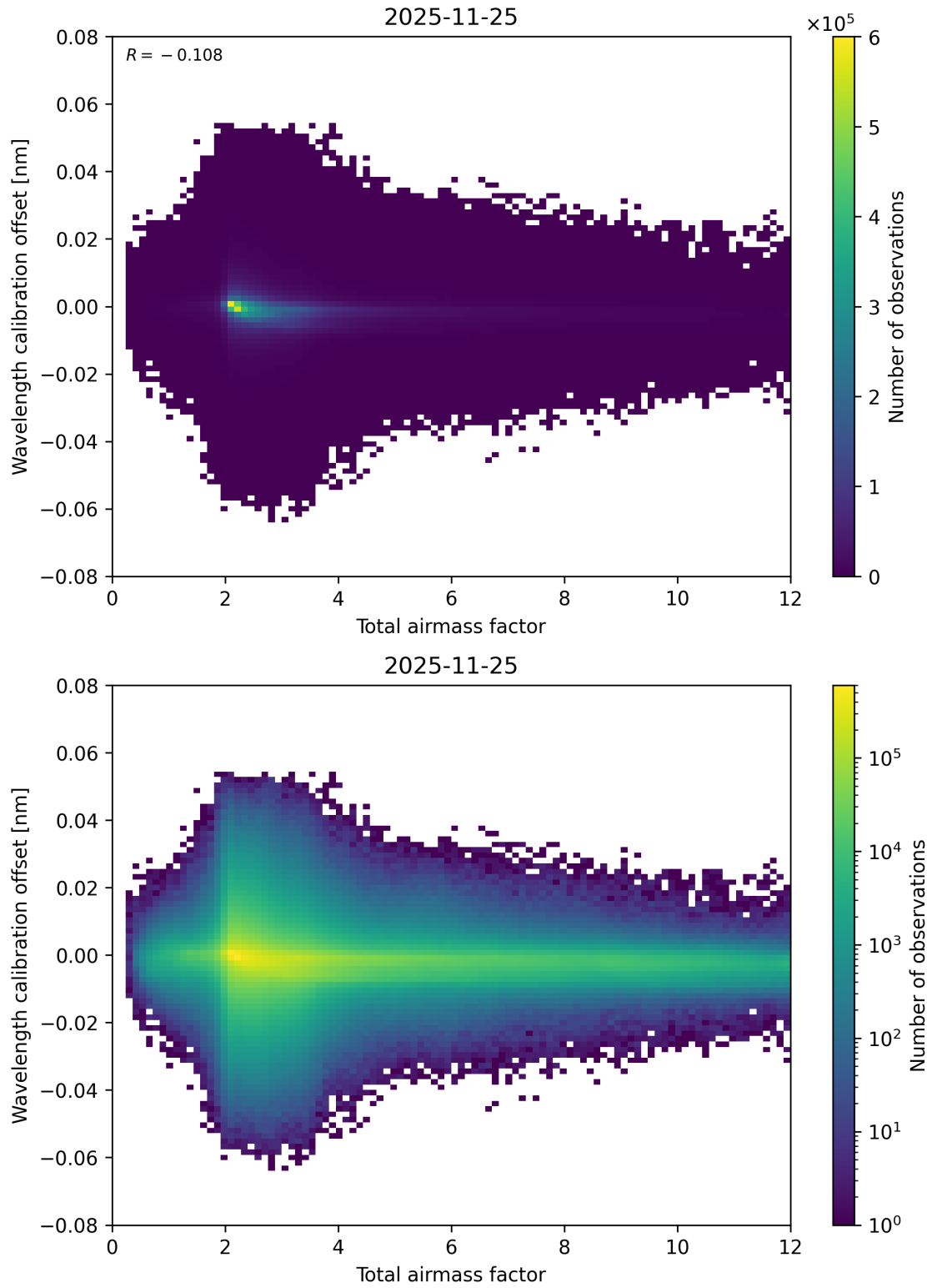
Figure 70: Scatter density plot of “Total airmass factor” against “Wavelength calibration offset” for 2025-11-24 to 2025-11-26.
