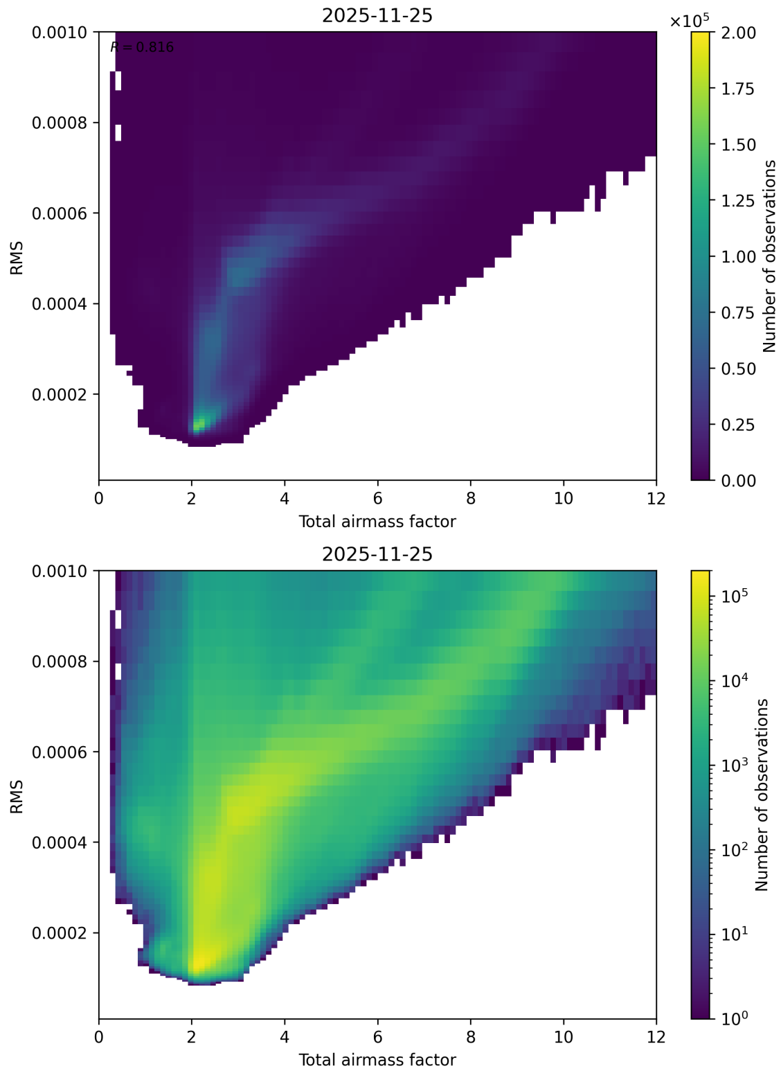
Figure 69: Scatter density plot of “Total airmass factor” against “RMS” for 2025-11-24 to 2025-11-26.
