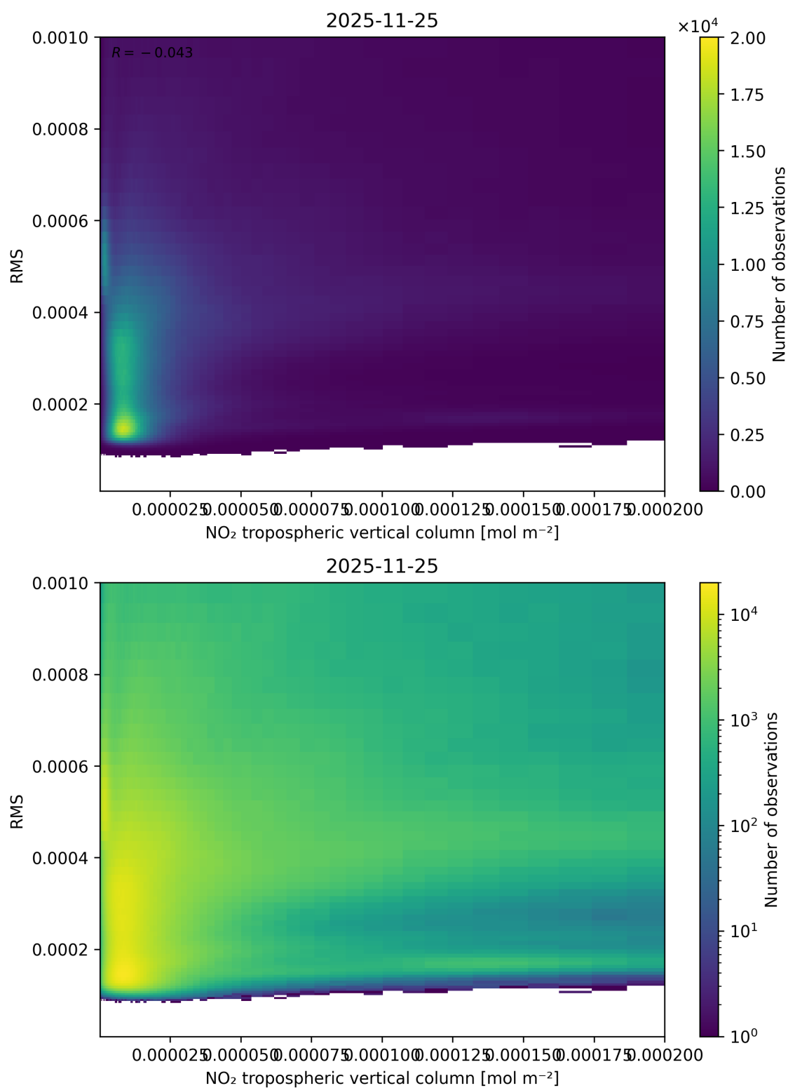
Figure 142: Scatter density plot of “NO 2 tropospheric vertical column” against “RMS” for 2025-11-24 to 2025-11-26.
