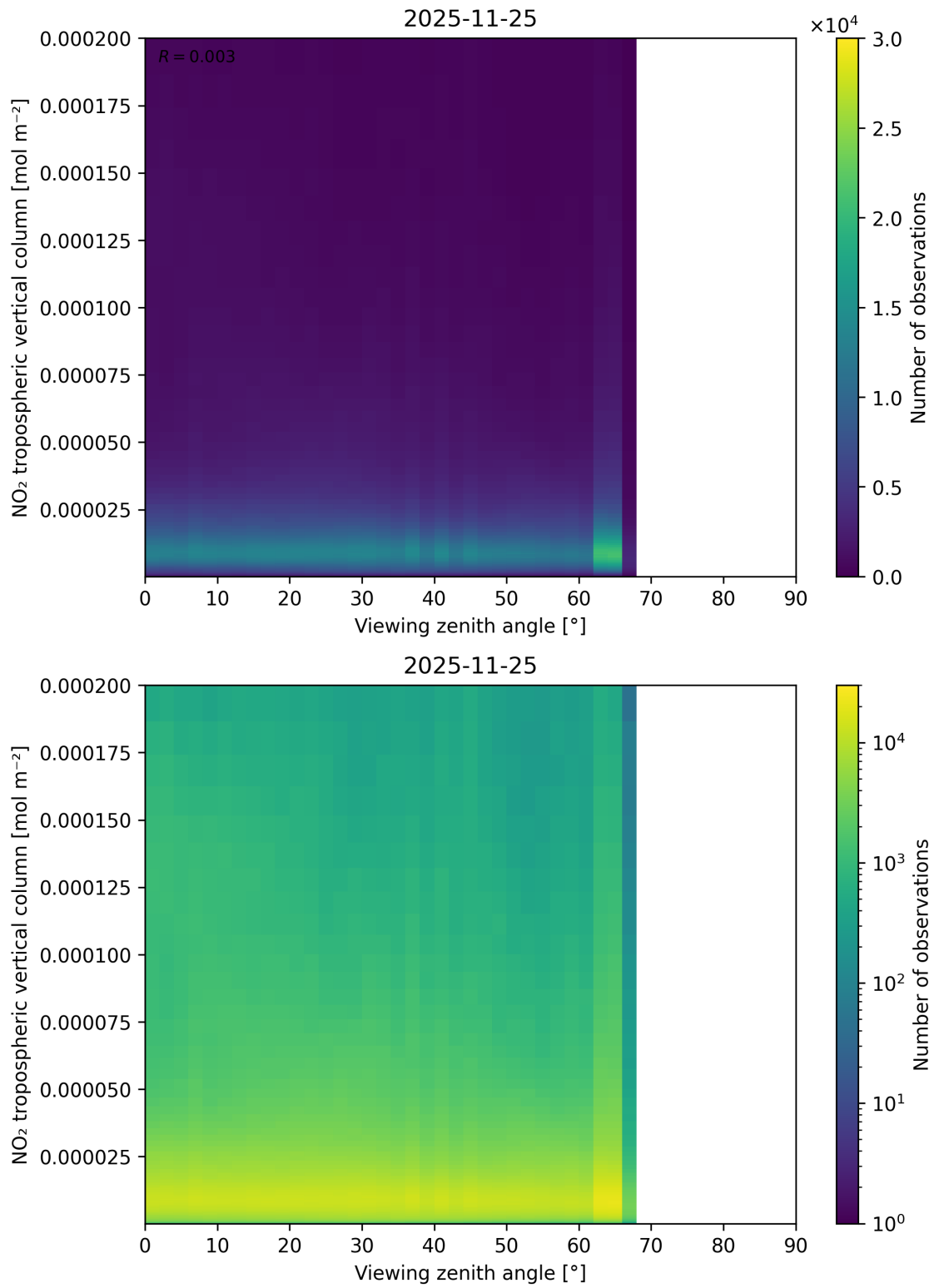
Figure 169: Scatter density plot of “Viewing zenith angle” against “NO 2 tropospheric vertical column” for 2025-11-24 to 2025-11-26.
