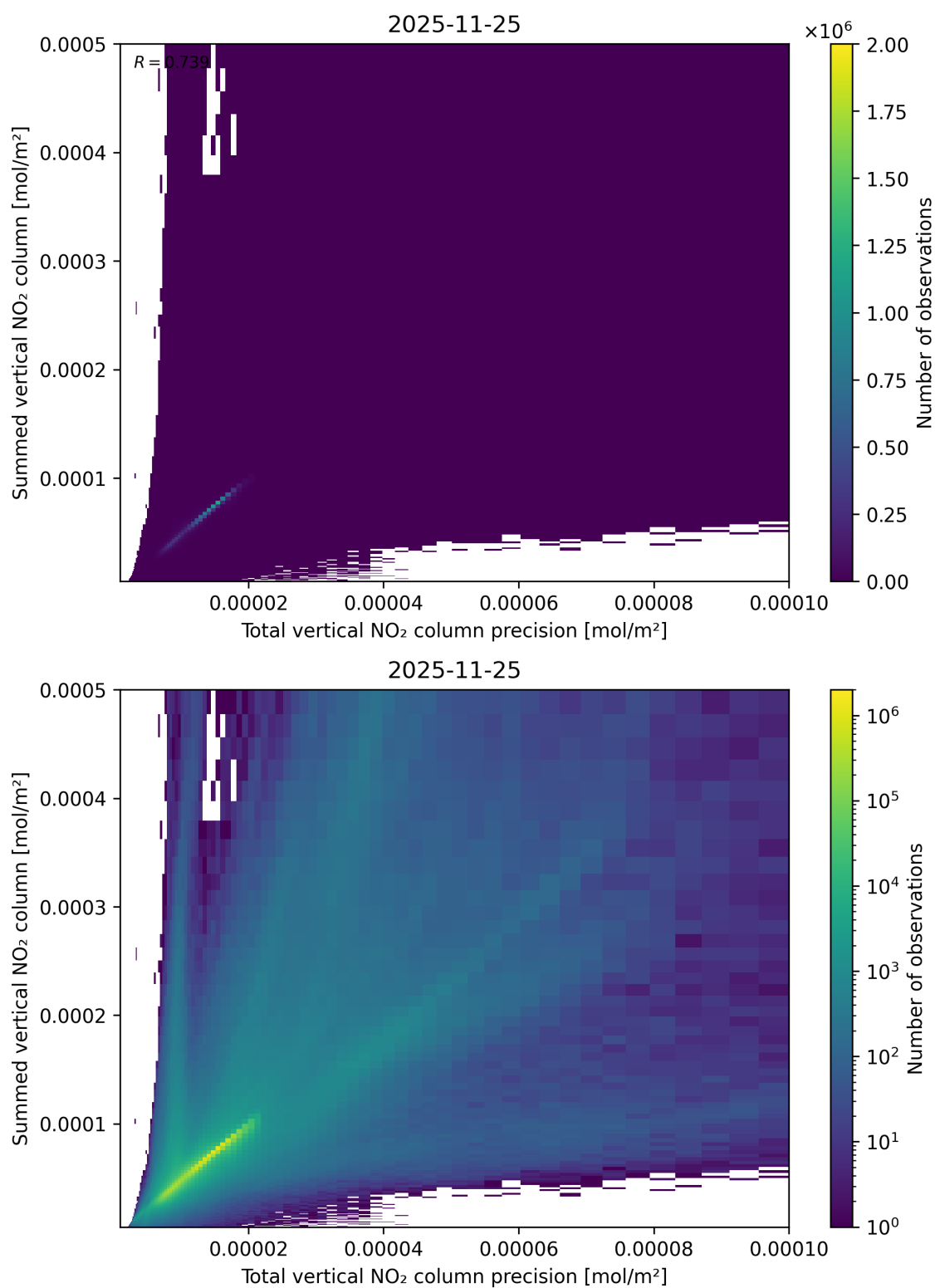
Figure 117: Scatter density plot of “Total vertical NO 2 column precision” against “Summed vertical NO 2 column” for 2025-11-24 to 2025-11-26.
