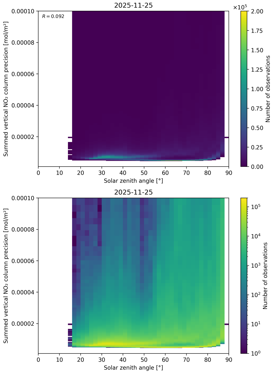
Figure 152: Scatter density plot of “Solar zenith angle” against “Summed vertical NO 2 column precision” for 2025-11-24 to 2025-11-26.
