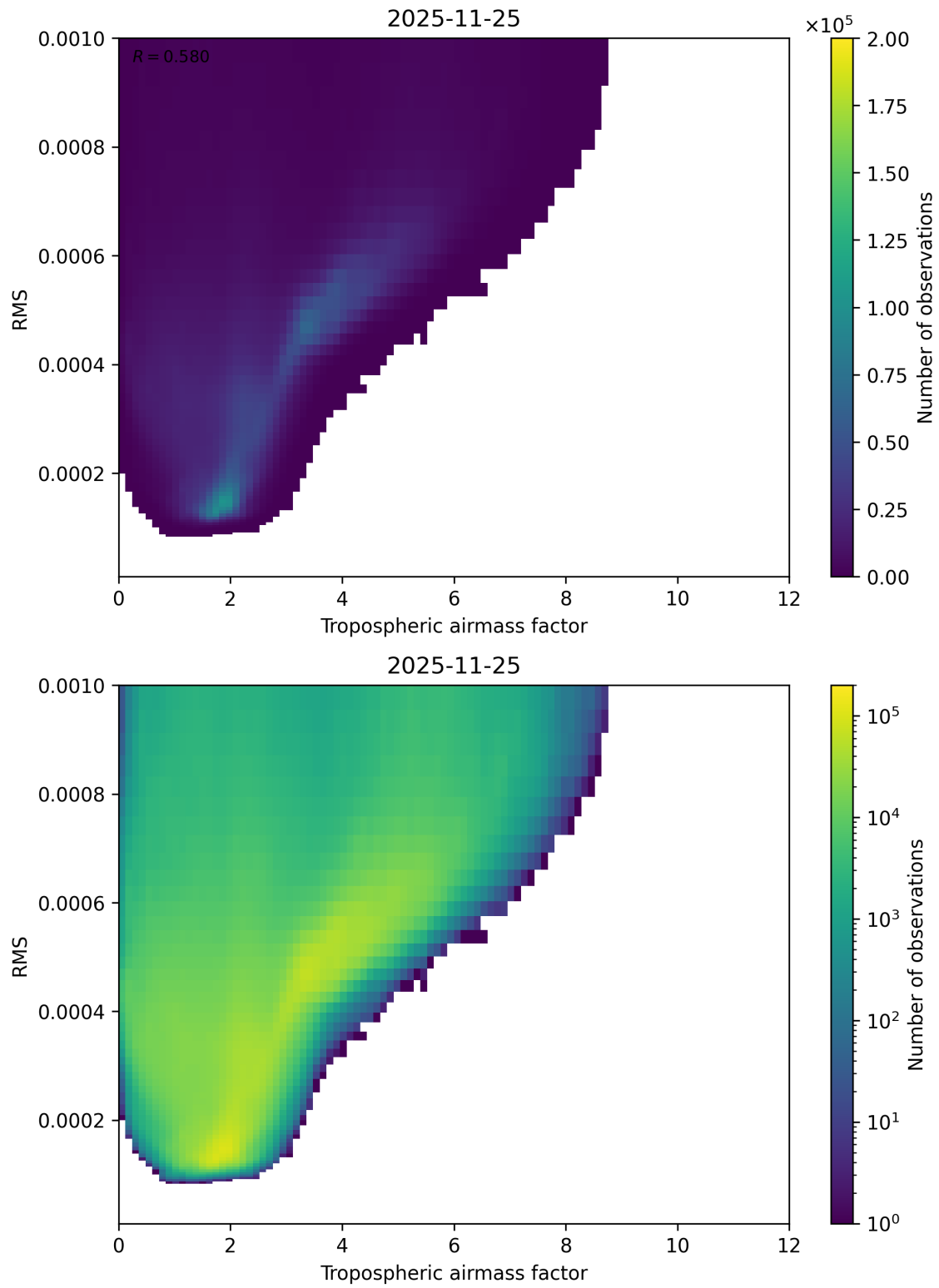
Figure 79: Scatter density plot of “Tropospheric airmass factor” against “RMS” for 2025-11-24 to 2025-11-26.
