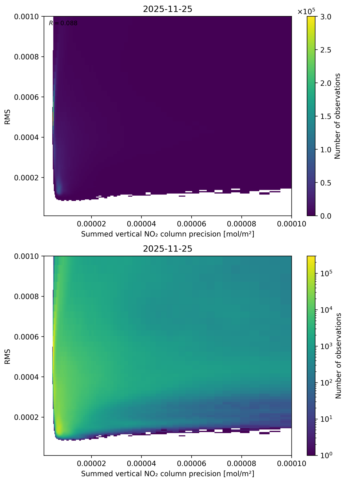
Figure 108: Scatter density plot of “Summed vertical NO 2 column precision” against “RMS” for 2025-11-24 to 2025-11-26.
