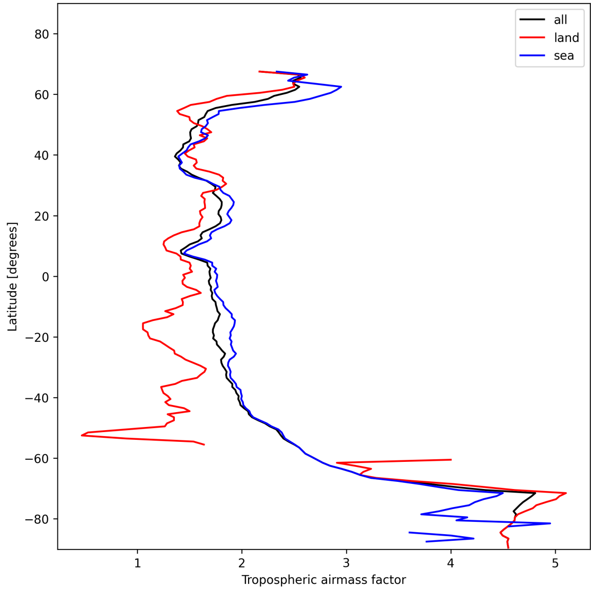
Figure 14: Zonal average of “Tropospheric air mass factor” for 2025-11-24 to 2025-11-26.
