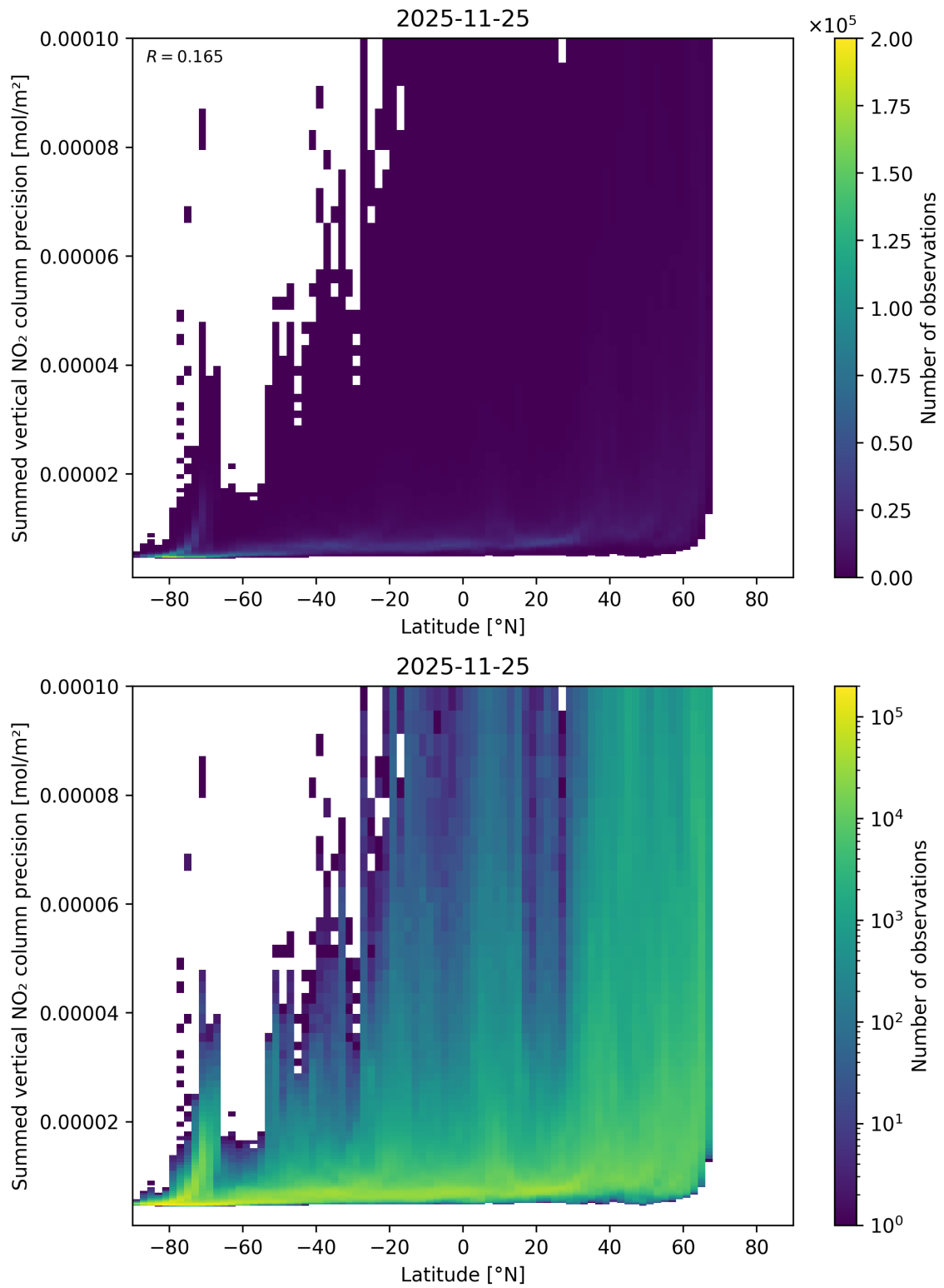
Figure 89: Scatter density plot of “Latitude” against “Summed vertical NO 2 column precision” for 2025-11-24 to 2025-11-26.
