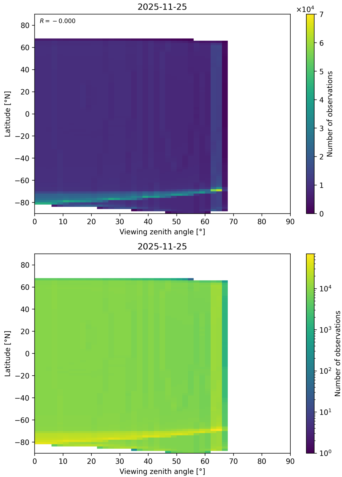
Figure 163: Scatter density plot of “Viewing zenith angle” against “Latitude” for 2025-11-24 to 2025-11-26.
