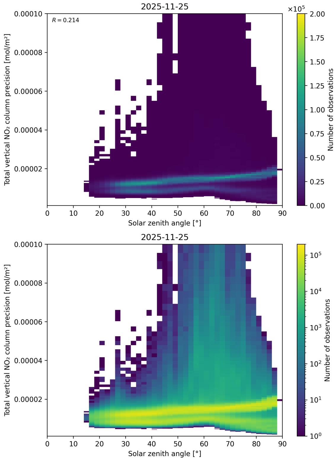
Figure 154: Scatter density plot of “Solar zenith angle” against “Total vertical NO 2 column precision” for 2025-11-24 to 2025-11-26.
