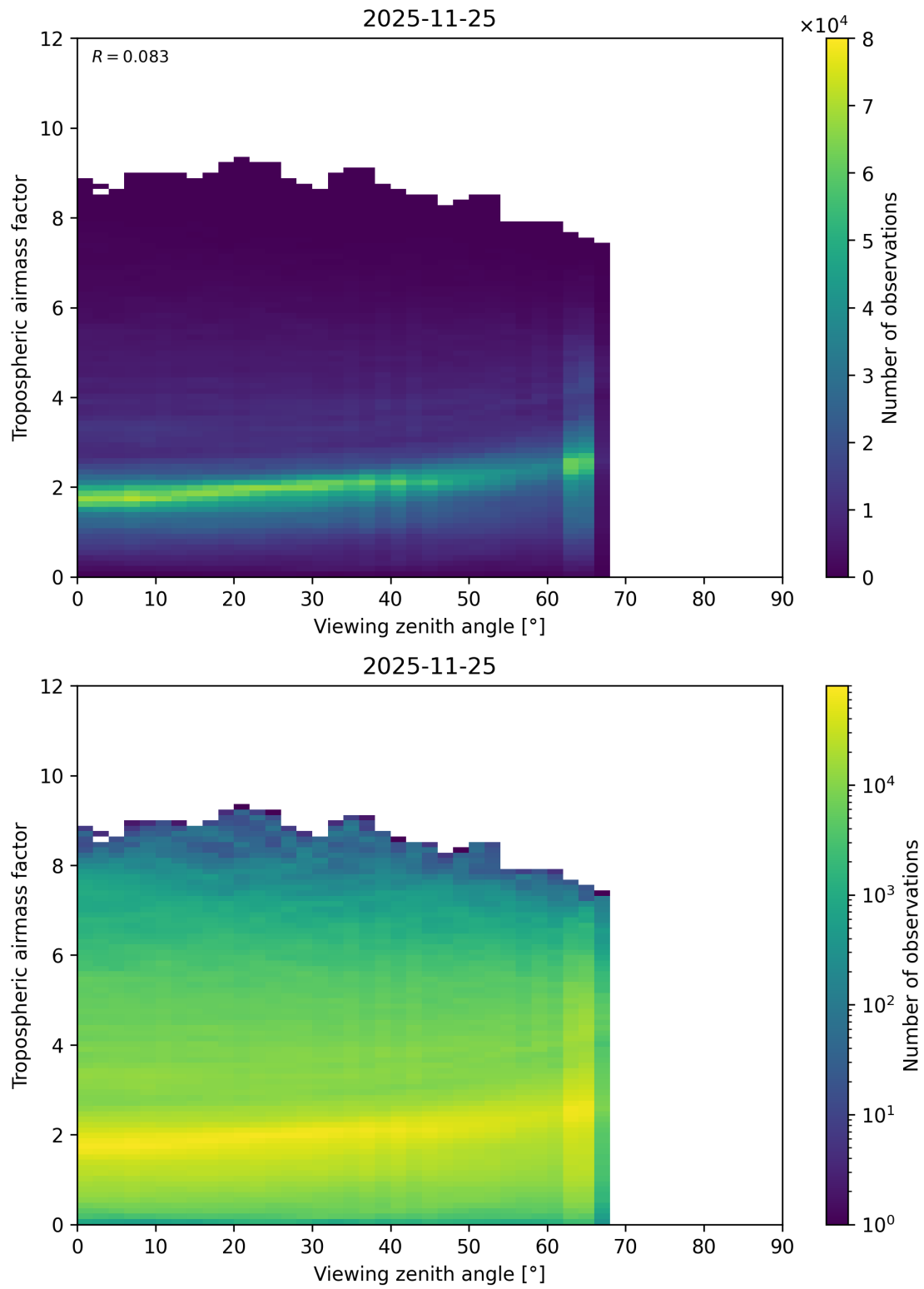
Figure 161: Scatter density plot of “Viewing zenith angle” against “Tropospheric airmass factor” for 2025-11-24 to 2025-11-26.
