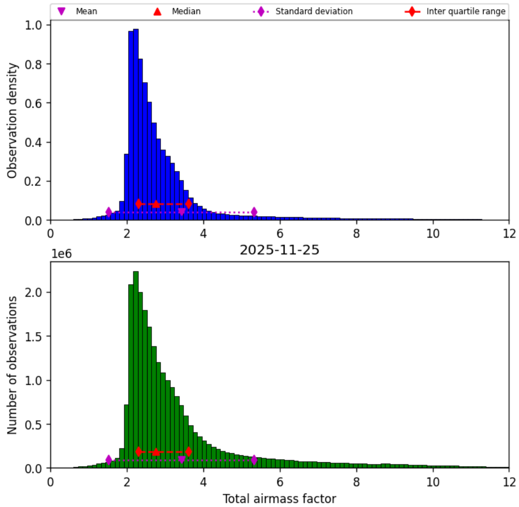
Figure 32: Histogram of “Total airmass factor” for 2025-11-24 to 2025-11-26
