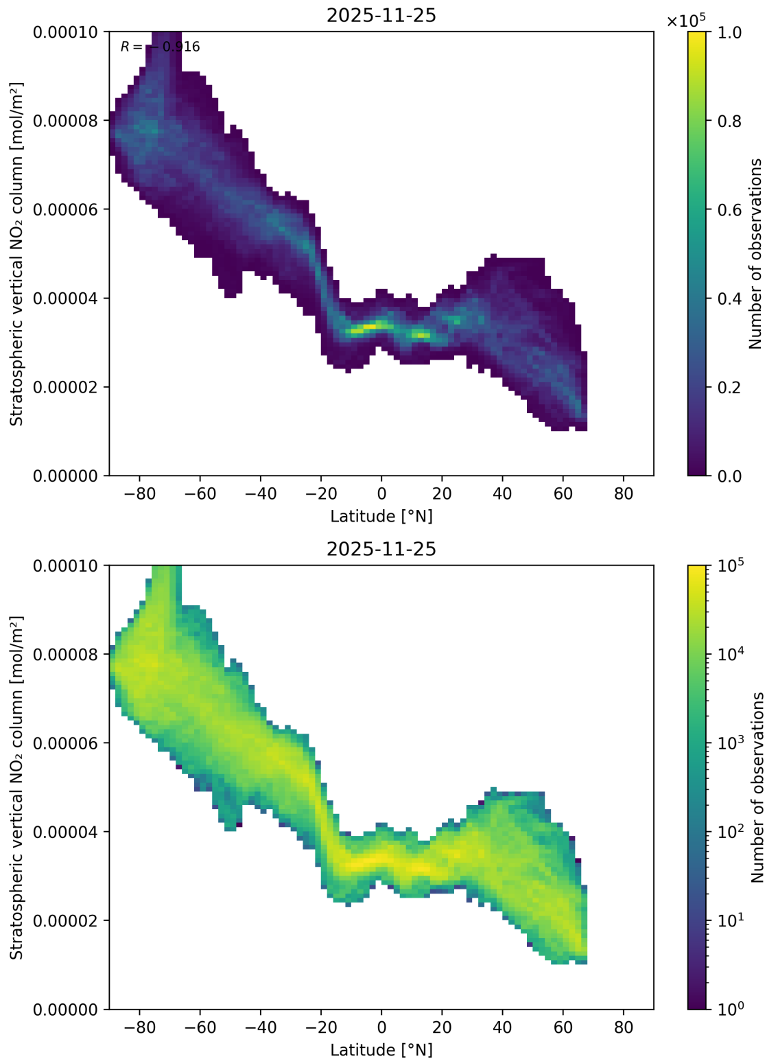
Figure 87: Scatter density plot of “Latitude” against “Stratospheric vertical NO 2 column” for 2025-11-24 to 2025-11-26.
