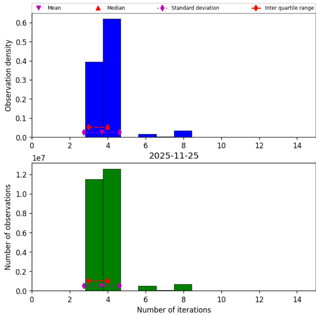
Figure 34: Histogram of “Number of iterations” for 2025-11-24 to 2025-11-26
