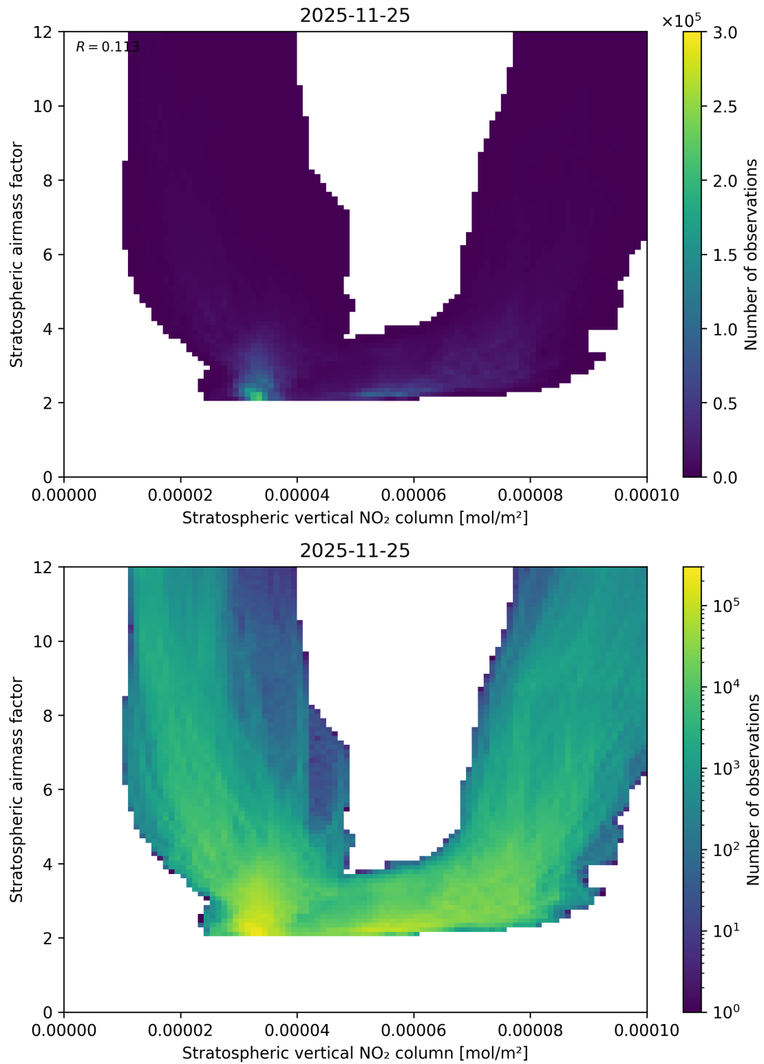
Figure 96: Scatter density plot of “Stratospheric vertical NO 2 column” against “Stratospheric airmass factor” for 2025-11-24 to 2025-11-26.
