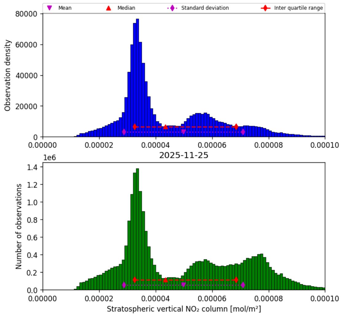
Figure 36: Histogram of “Stratospheric vertical NO 2 column” for 2025-11-24 to 2025-11-26
