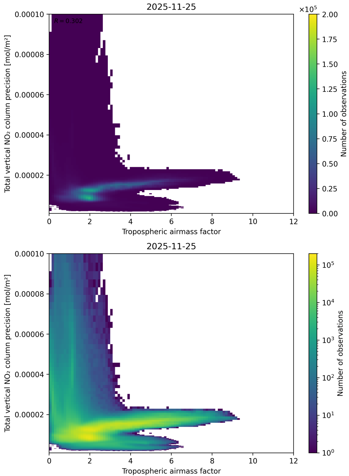
Figure 78: Scatter density plot of “Tropospheric air mass factor” against “Total vertical NO 2 column precision” for 2025-11-24 to 2025-11-26.
