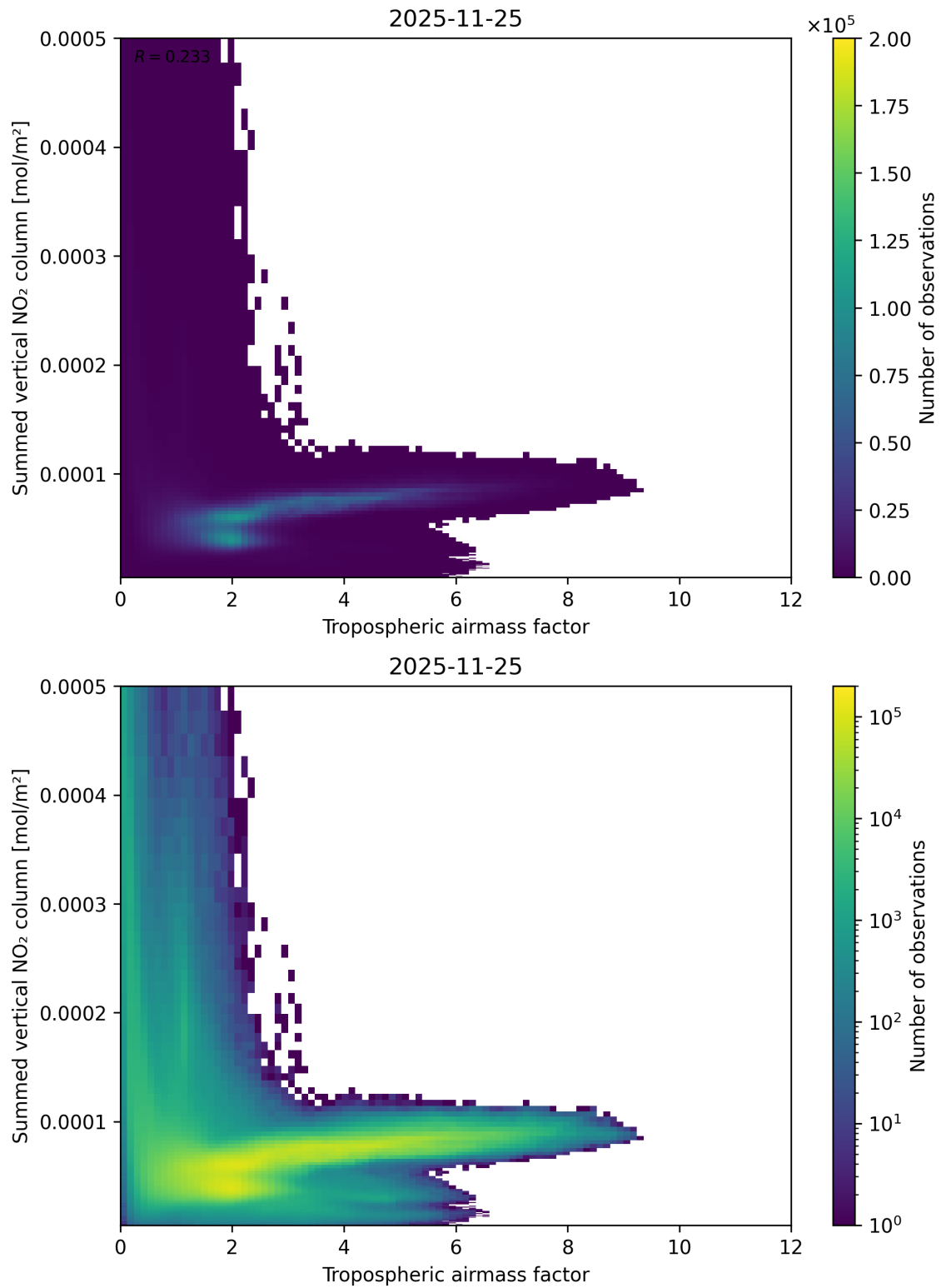
Figure 75: Scatter density plot of “Tropospheric air mass factor” against “Summed vertical NO 2 column” for 2025-11-24 to 2025-11-26.
