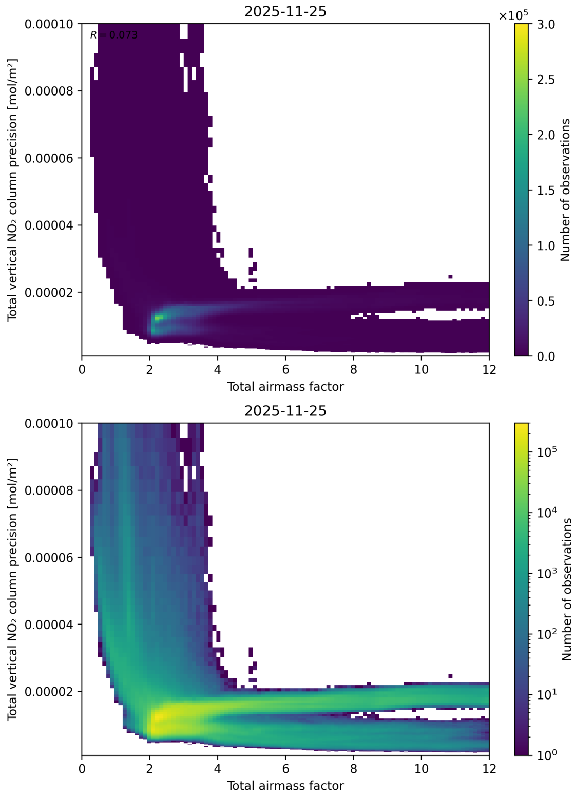
Figure 68: Scatter density plot of “Total airmass factor” against “Total vertical NO 2 column precision” for 2025-11-24 to 2025-11-26.
