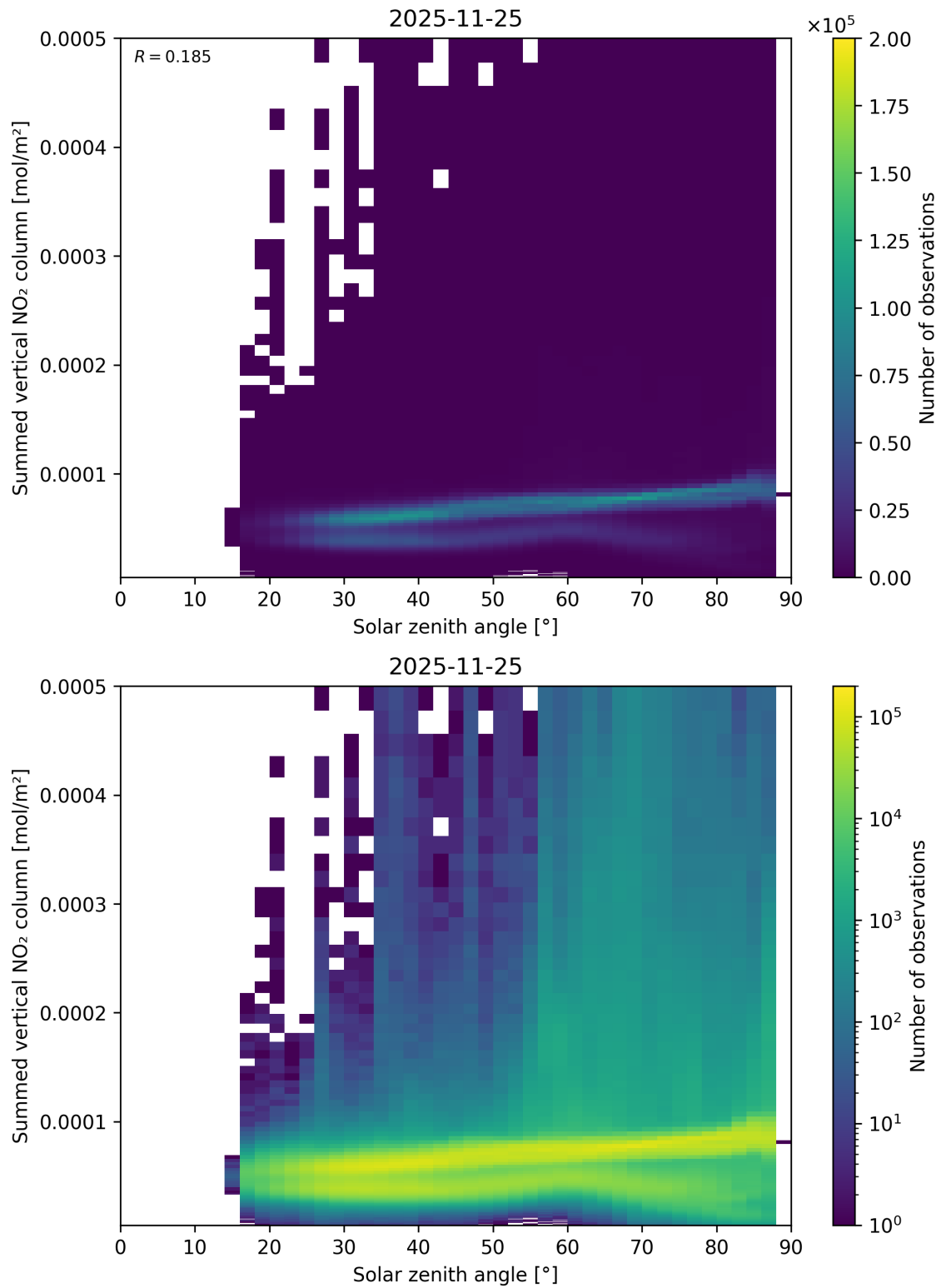
Figure 151: Scatter density plot of “Solar zenith angle” against “Summed vertical NO 2 column” for 2025-11-24 to 2025-11-26.
