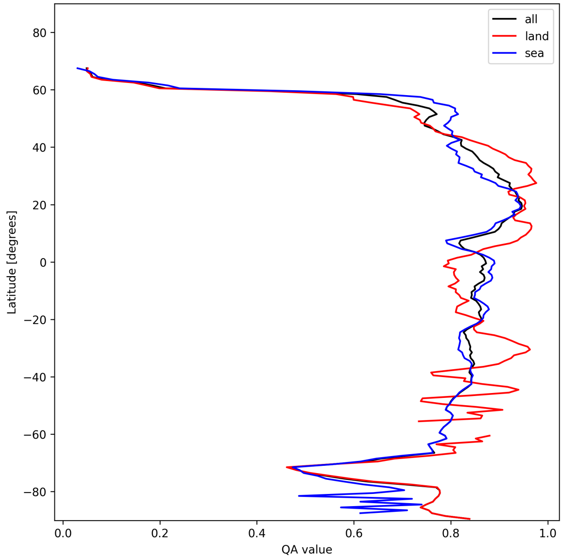
Figure 11: Zonal average of “QA value” for 2025-11-25 to 2025-11-27.
