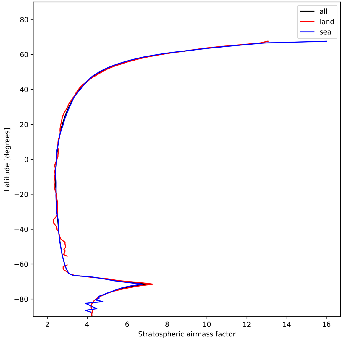
Figure 27: Zonal average of “Stratospheric airmass factor” for 2025-11-25 to 2025-11-27.
