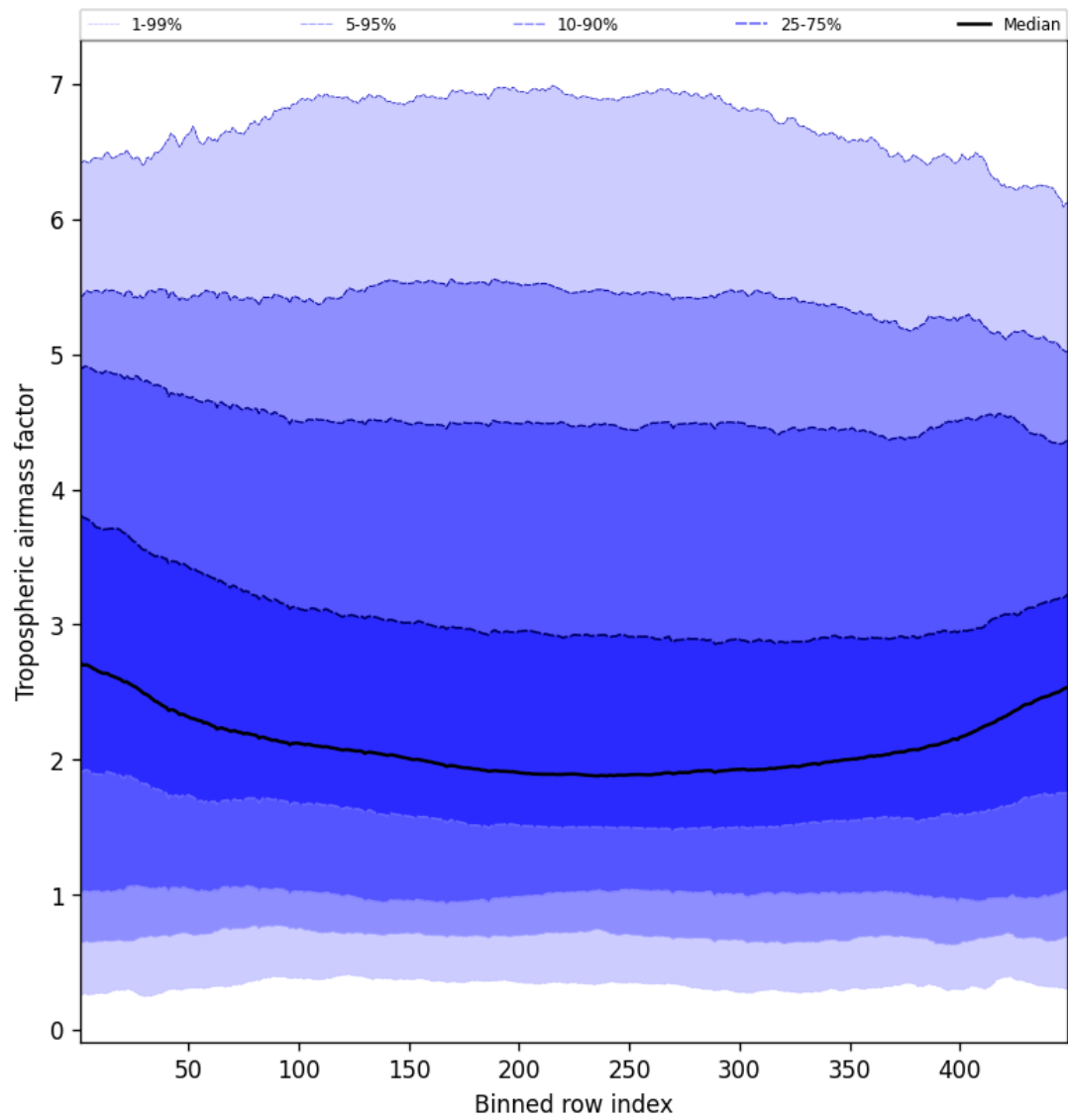
Figure 48: Along track statistics of “Tropospheric airmass factor” for 2025-11-25 to 2025-11-27
