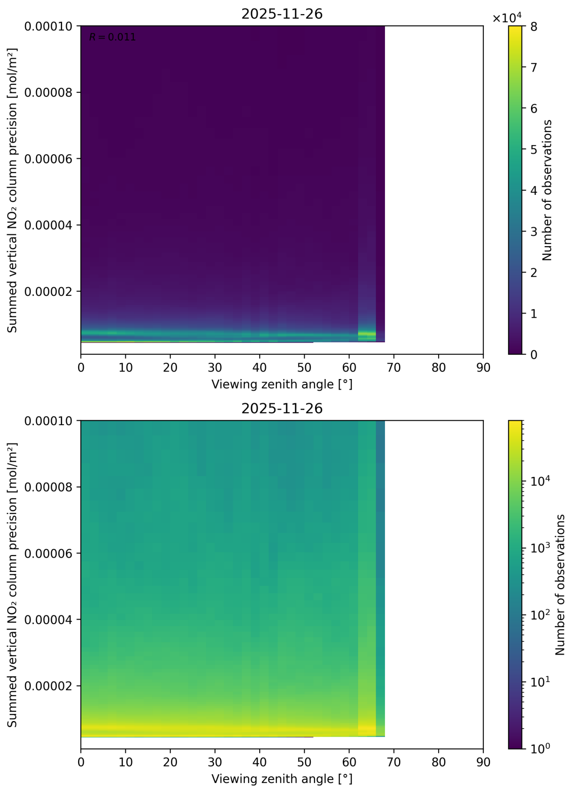
Figure 166: Scatter density plot of “Viewing zenith angle” against “Summed vertical NO 2 column precision” for 2025-11-25 to 2025-11-27.
