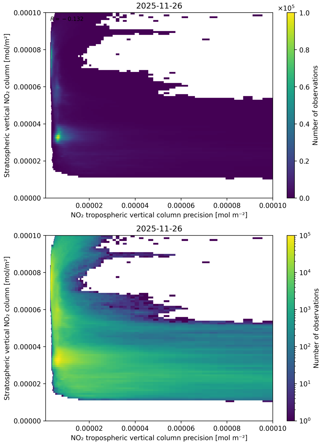
Figure 135: Scatter density plot of “NO 2 tropospheric vertical column precision” against “Stratospheric vertical NO 2 column” for 2025-11-25 to 2025-11-27.
