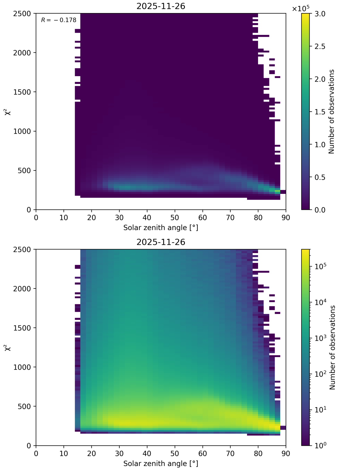
Figure 148: Scatter density plot of “Solar zenith angle” against “ \chi^2 ” for 2025-11-25 to 2025-11-27.
