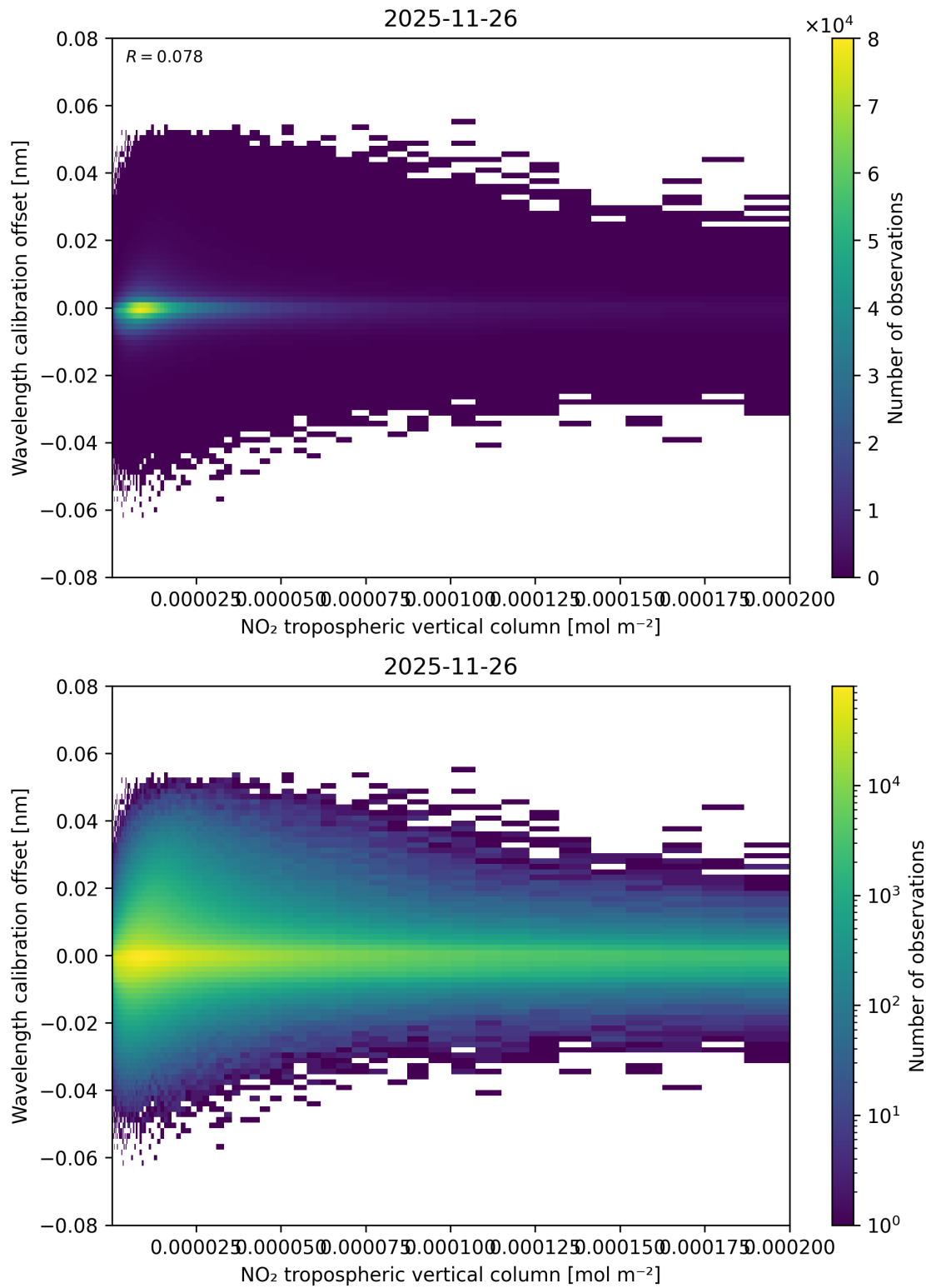
Figure 143: Scatter density plot of “NO 2 tropospheric vertical column” against “Wavelength calibration offset” for 2025-11-25 to 2025-11-27.
