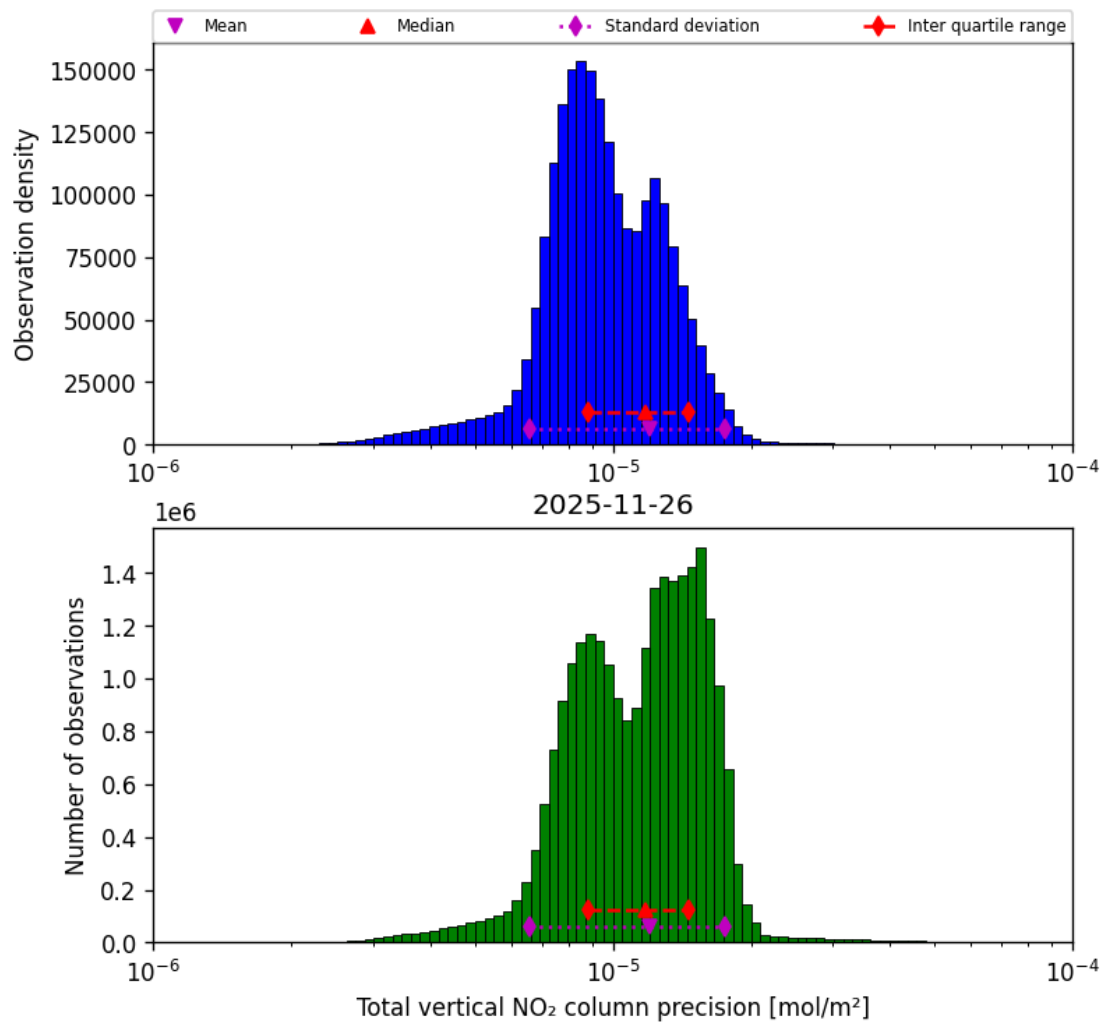
Figure 39: Histogram of “Total vertical NO 2 column precision” for 2025-11-25 to 2025-11-27
