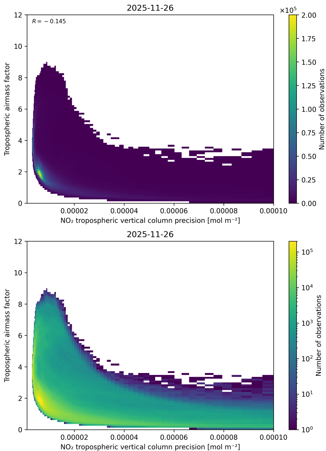
Figure 133: Scatter density plot of “NO 2 tropospheric vertical column precision” against “Tropospheric air mass factor” for 2025-11-25 to 2025-11-27.
