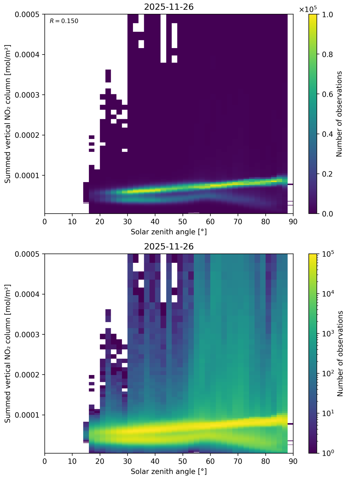
Figure 151: Scatter density plot of “Solar zenith angle” against “Summed vertical NO 2 column” for 2025-11-25 to 2025-11-27.
