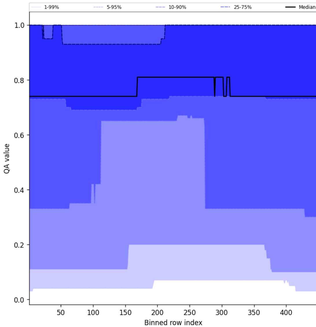
Figure 45: Along track statistics of “QA value” for 2025-11-25 to 2025-11-27
