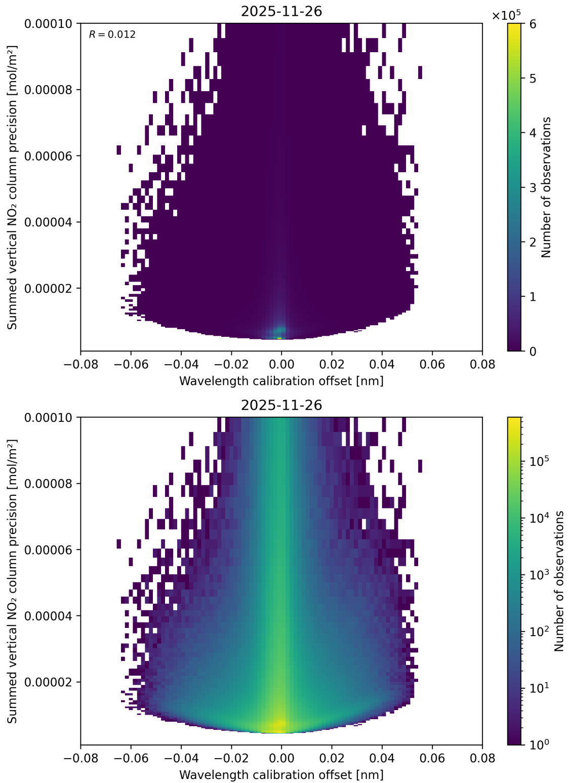
Figure 178: Scatter density plot of “Wavelength calibration offset” against “Summed vertical NO 2 column precision” for 2025-11-25 to 2025-11-27.
