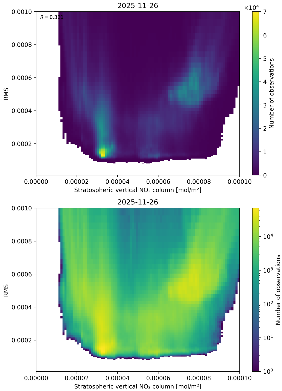
Figure 102: Scatter density plot of “Stratospheric vertical NO 2 column” against “RMS” for 2025-11-25 to 2025-11-27.
