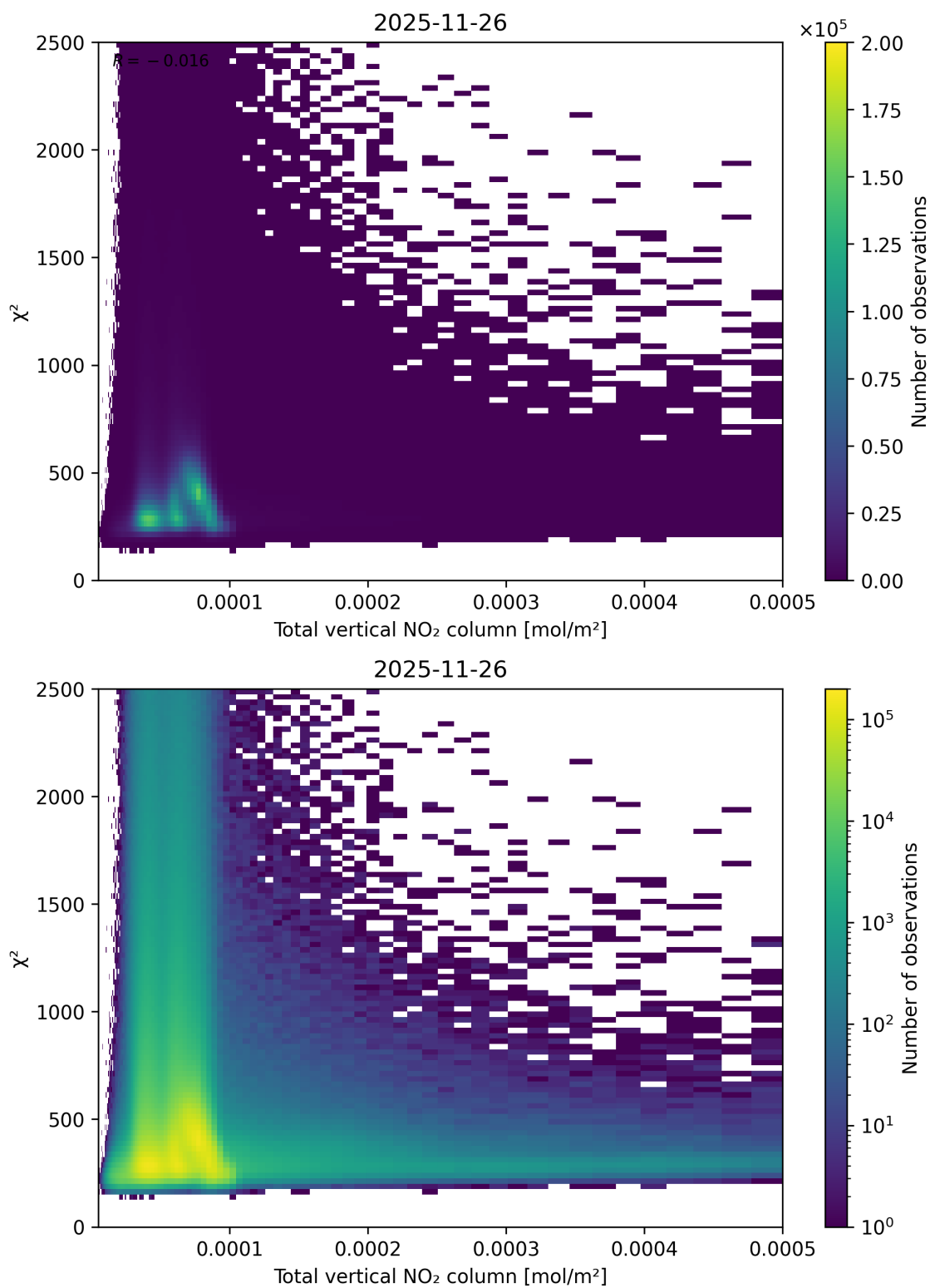
Figure 111: Scatter density plot of “Total vertical NO 2 column” against “ \chi^2 ” for 2025-11-25 to 2025-11-27.
