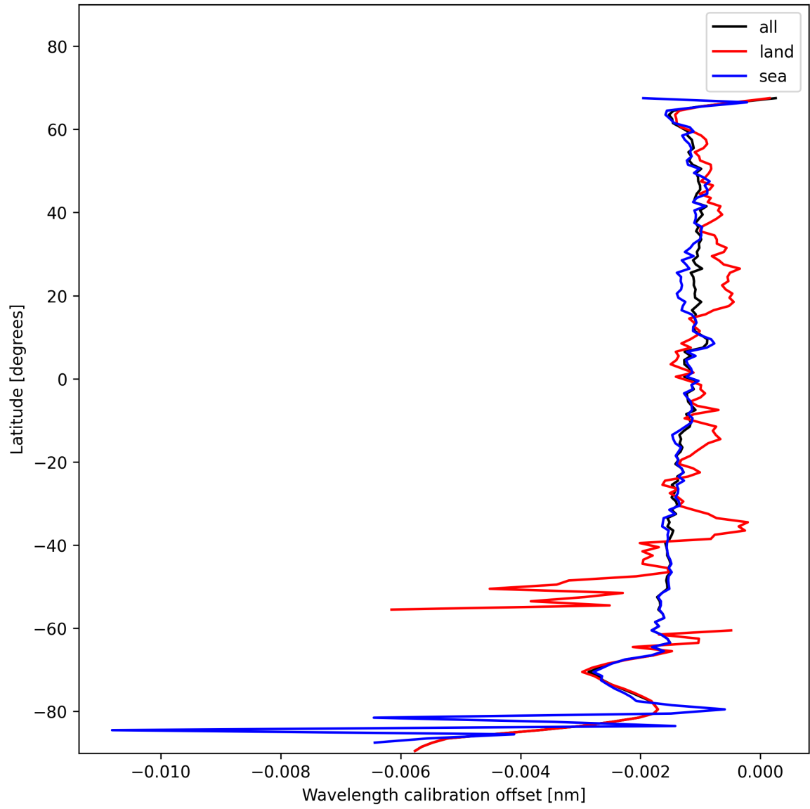
Figure 18: Zonal average of “Wavelength calibration offset” for 2025-11-25 to 2025-11-27.
