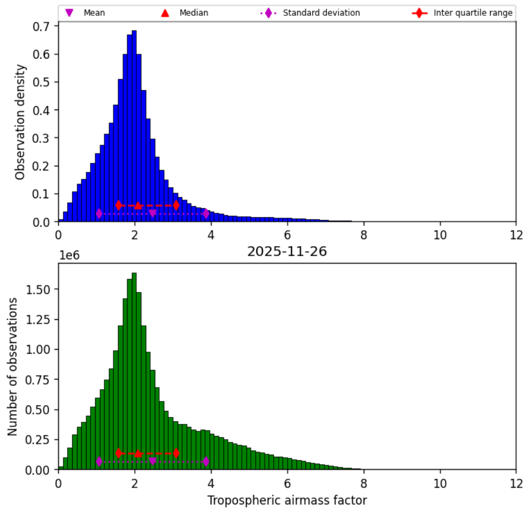
Figure 31: Histogram of “Tropospheric airmass factor” for 2025-11-25 to 2025-11-27
