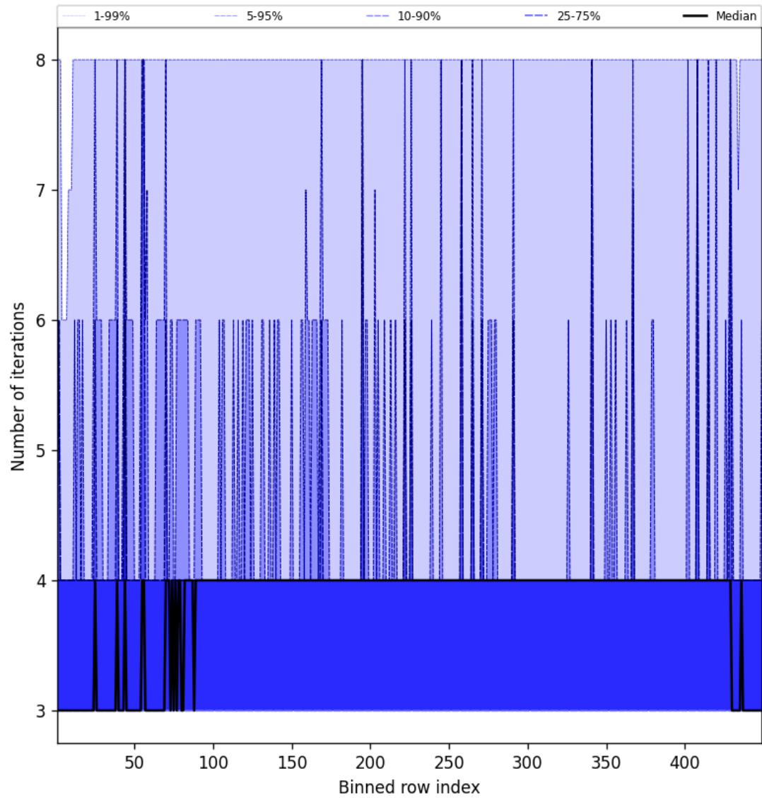
Figure 51: Along track statistics of “Number of iterations” for 2025-11-25 to 2025-11-27
