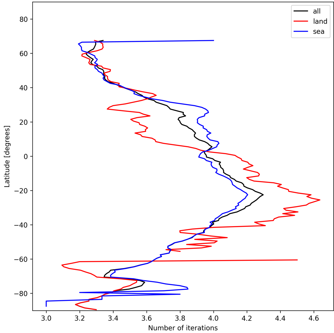
Figure 17: Zonal average of “Number of iterations” for 2025-11-25 to 2025-11-27.
