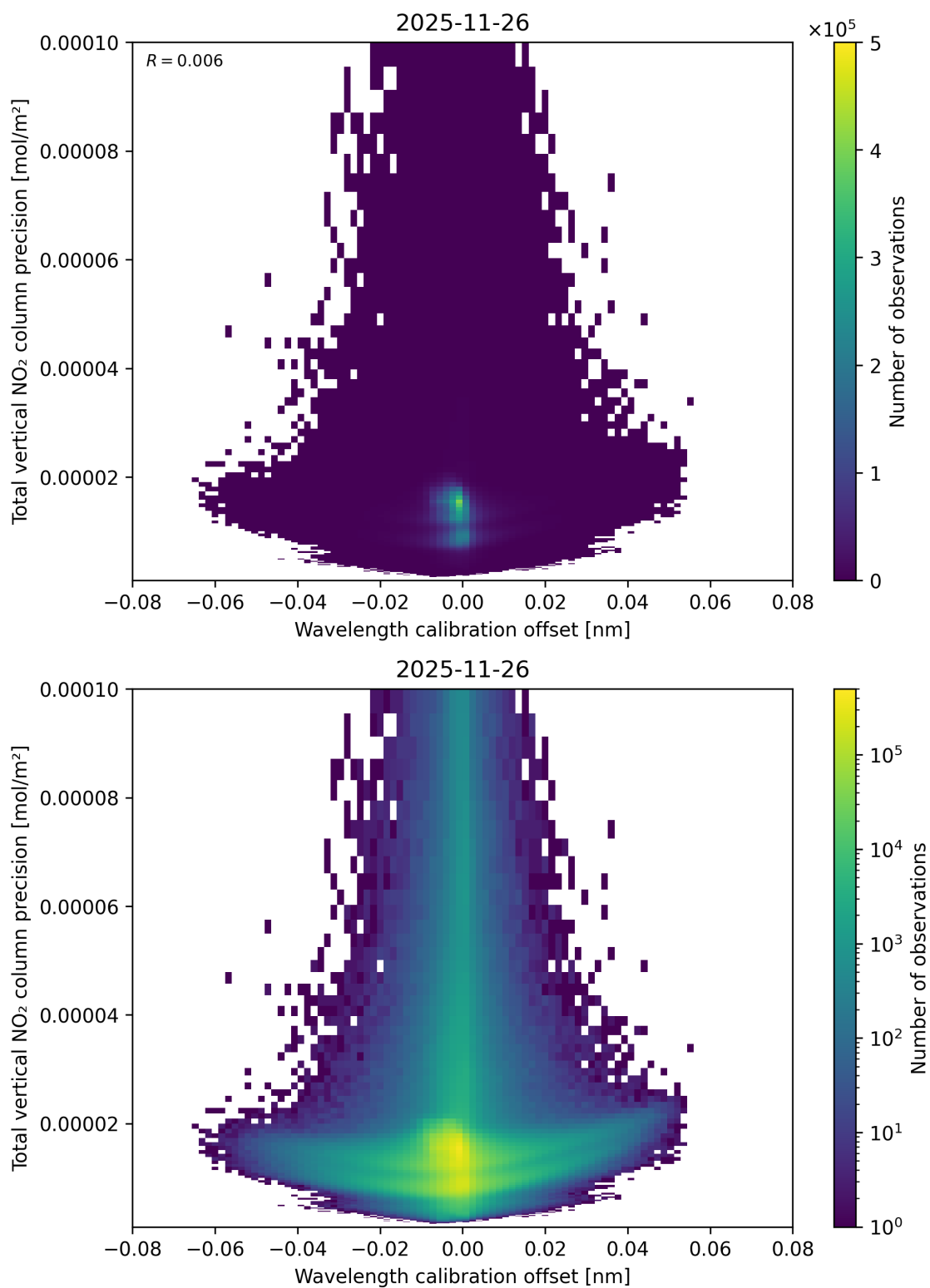
Figure 180: Scatter density plot of “Wavelength calibration offset” against “Total vertical NO 2 column precision” for 2025-11-25 to 2025-11-27.
