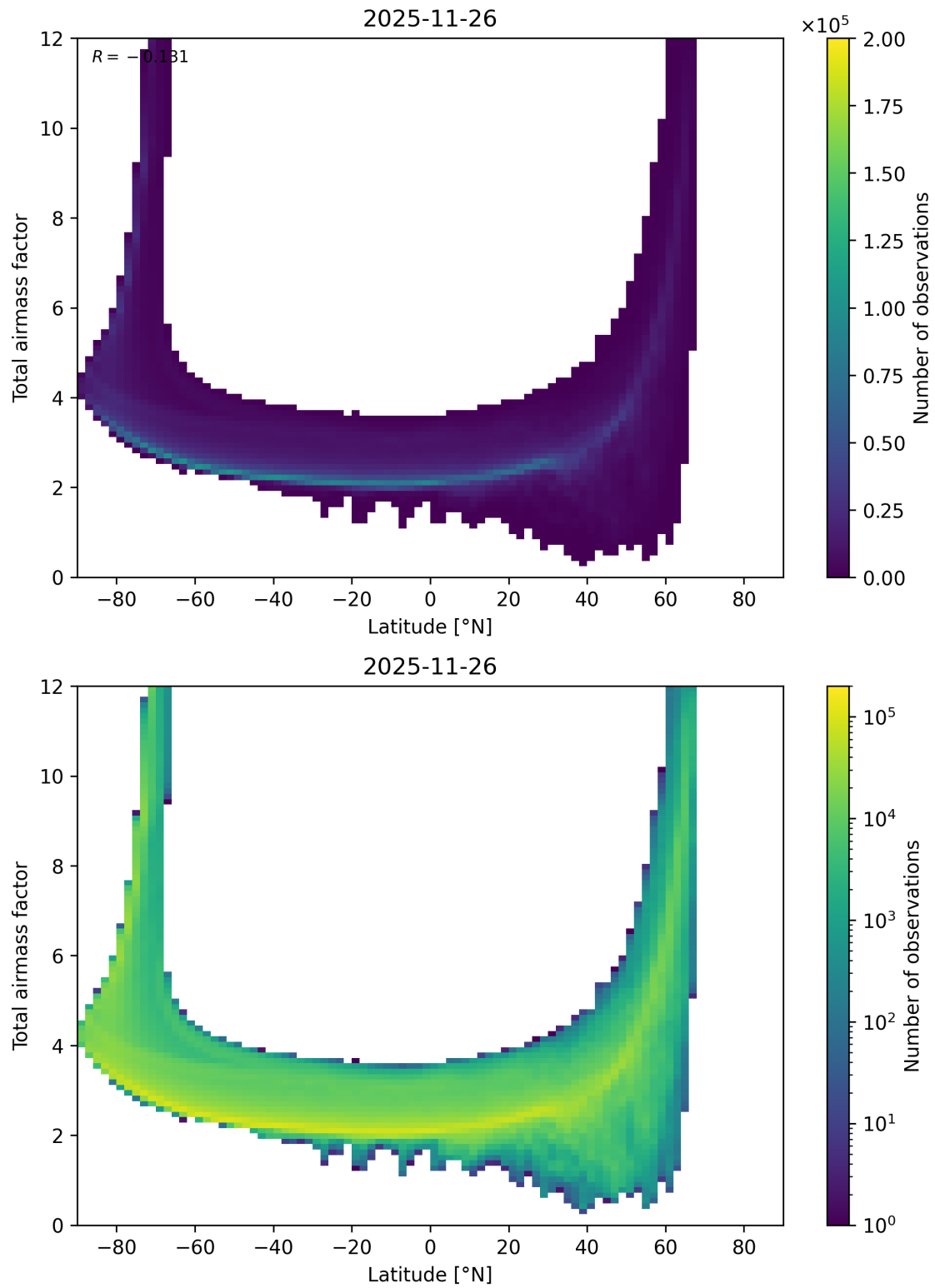
Figure 84: Scatter density plot of “Latitude” against “Total airmass factor” for 2025-11-25 to 2025-11-27.
