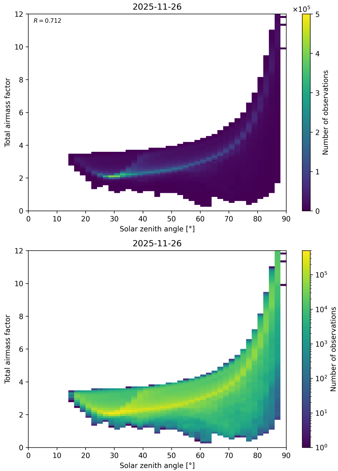
Figure 146: Scatter density plot of “Solar zenith angle” against “Total air mass factor” for 2025-11-25 to 2025-11-27.
