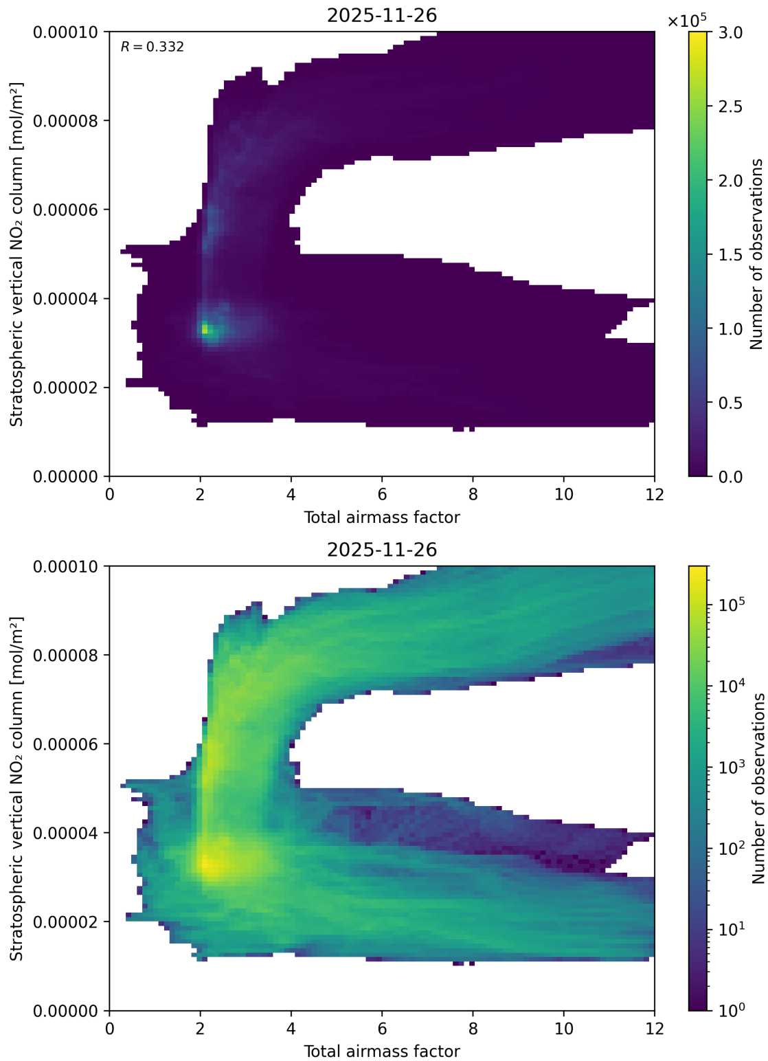
Figure 64: Scatter density plot of “Total airmass factor” against “Stratospheric vertical \text{NO}_2 column” for 2025-11-25 to 2025-11-27.
