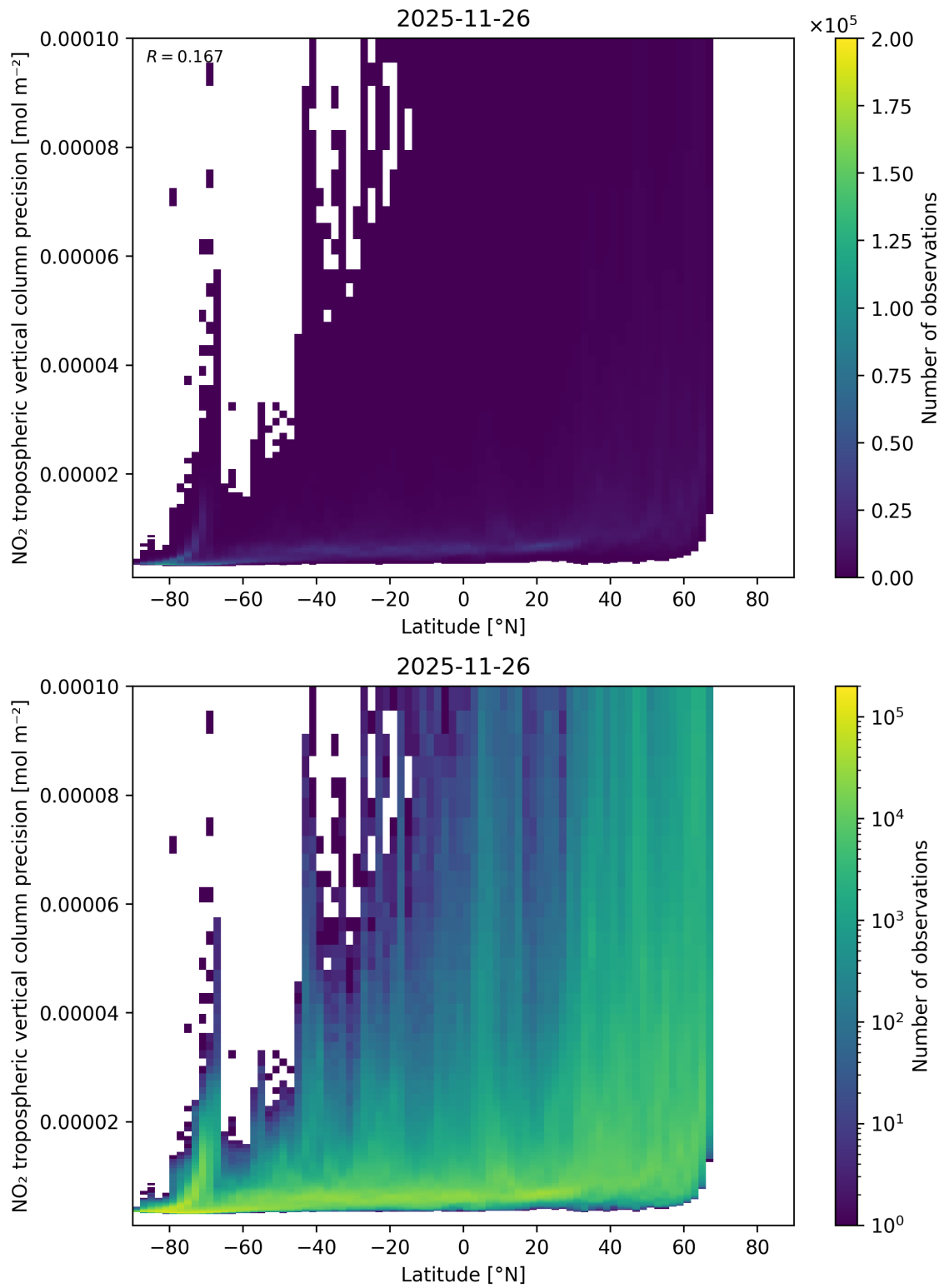
Figure 93: Scatter density plot of “Latitude” against “NO 2 tropospheric vertical column precision” for 2025-11-25 to 2025-11-27.
