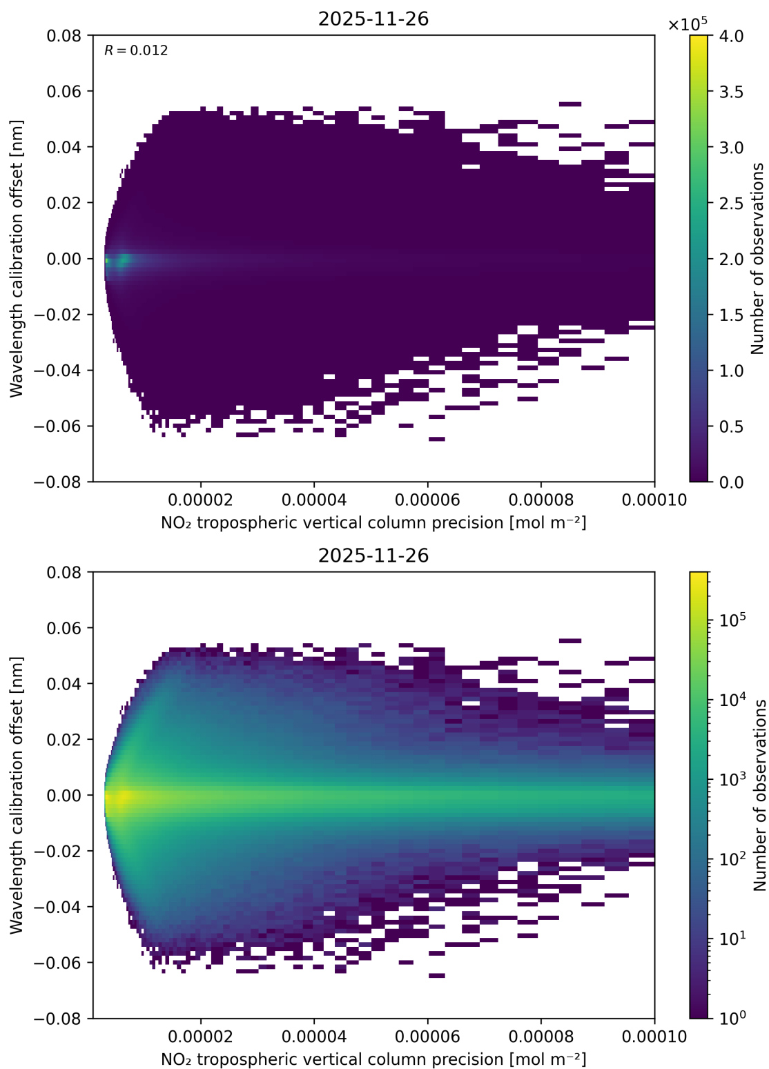
Figure 141: Scatter density plot of “NO 2 tropospheric vertical column precision” against “Wavelength calibration offset” for 2025-11-25 to 2025-11-27.
