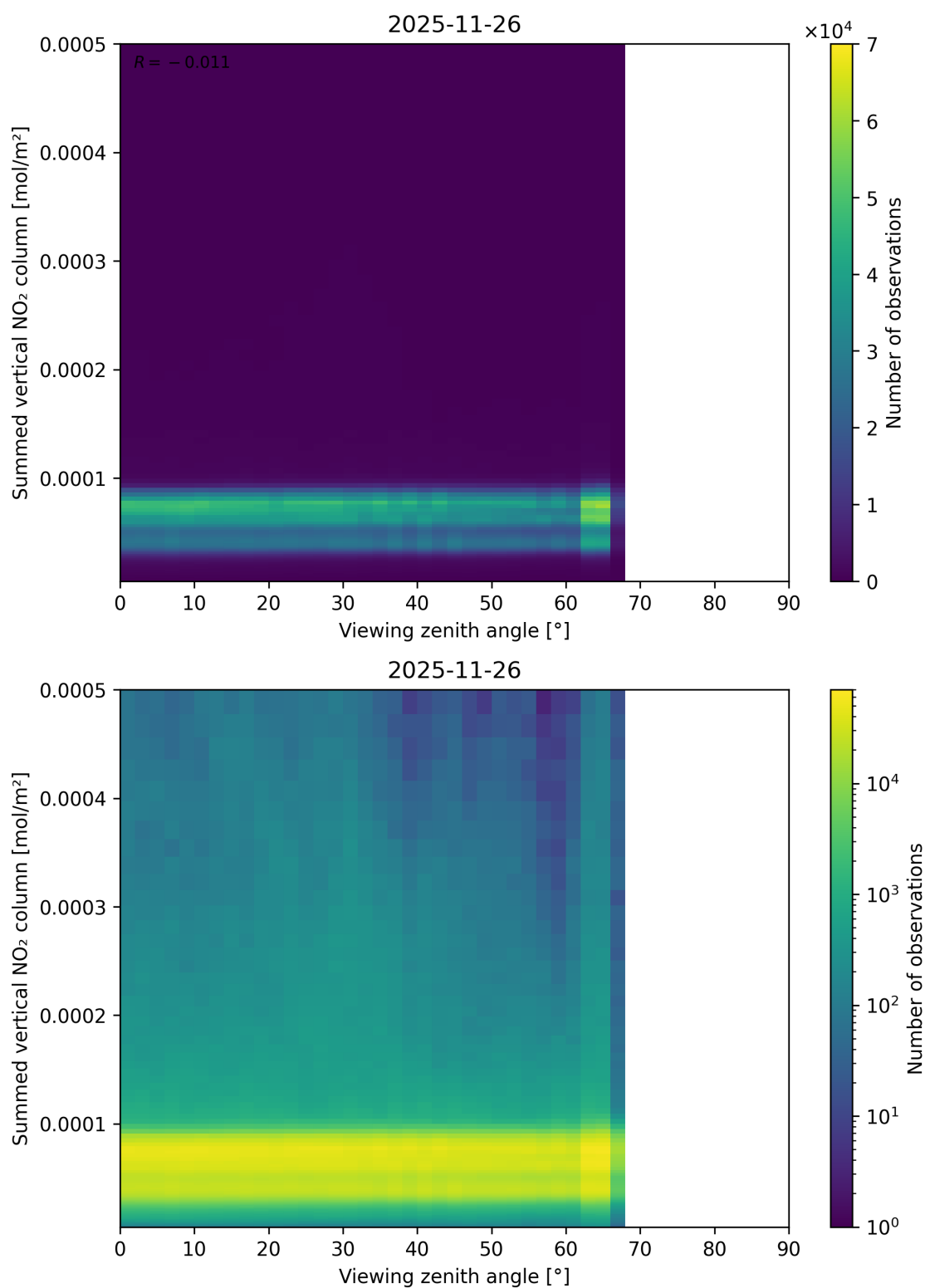
Figure 165: Scatter density plot of “Viewing zenith angle” against “Summed vertical NO 2 column” for 2025-11-25 to 2025-11-27.
