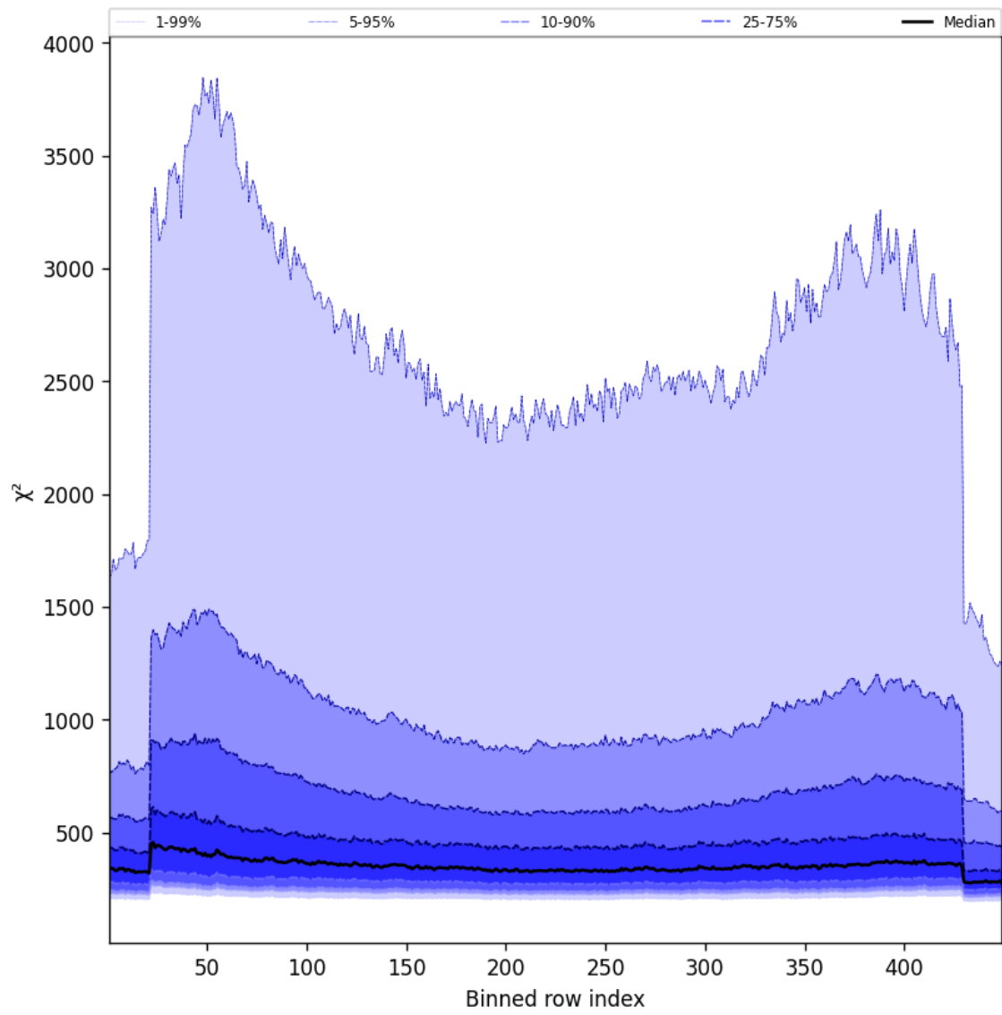
Figure 59: Along track statistics of “ \chi^2 ” for 2025-11-25 to 2025-11-27
