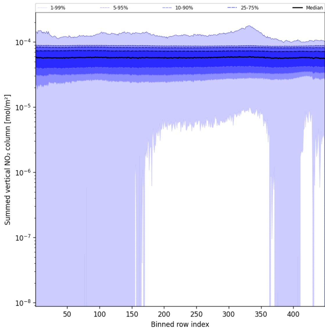
Figure 57: Along track statistics of “Summed vertical NO 2 column” for 2025-11-25 to 2025-11-27
