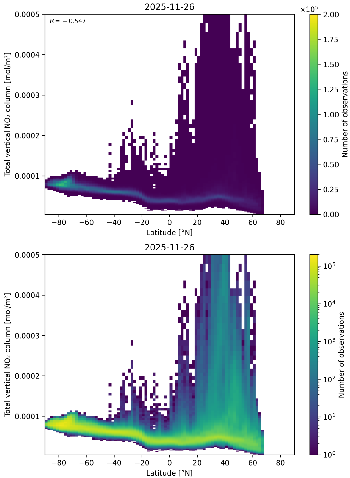
Figure 90: Scatter density plot of “Latitude” against “Total vertical NO 2 column” for 2025-11-25 to 2025-11-27.
