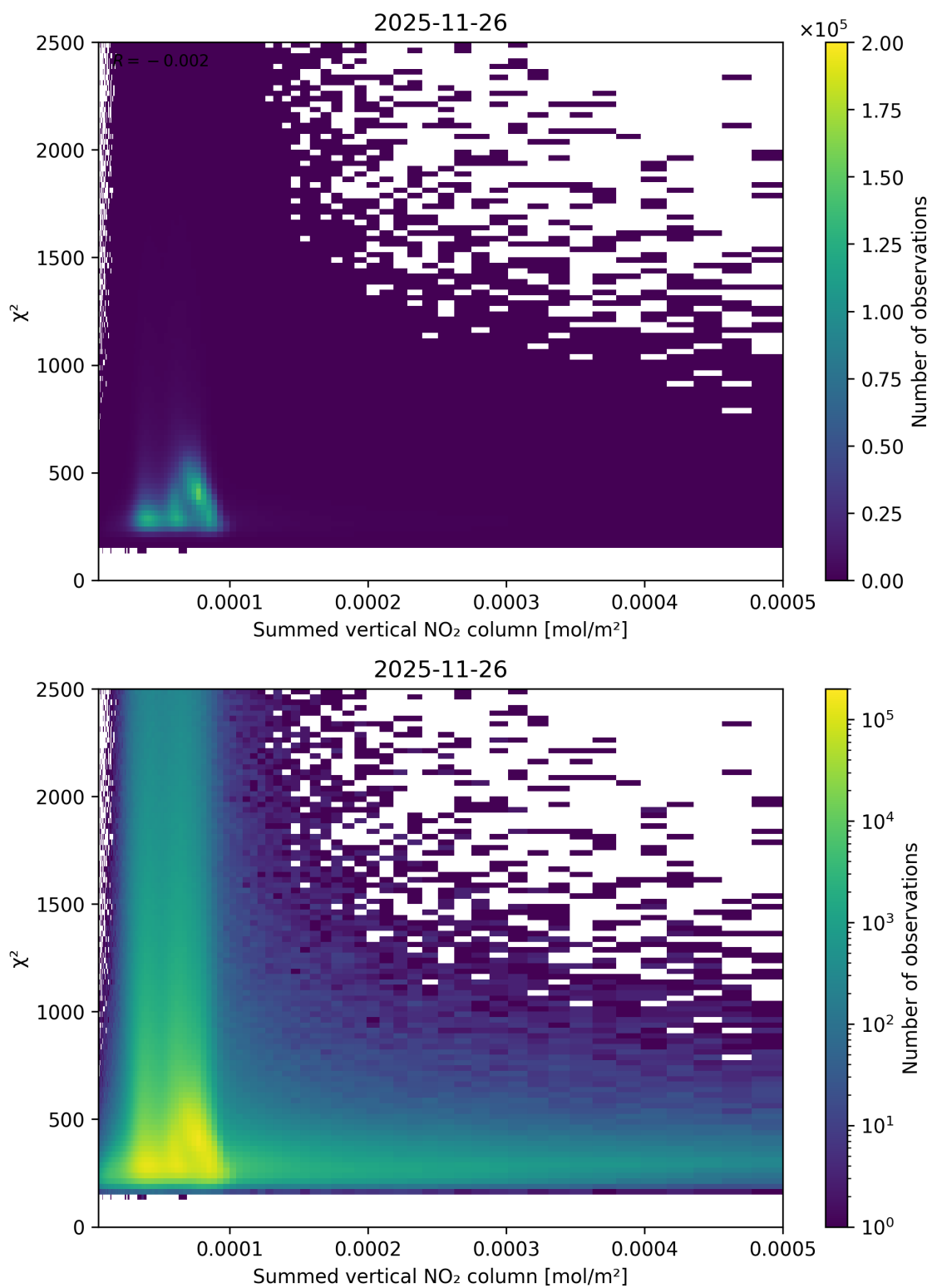
Figure 104: Scatter density plot of “Summed vertical NO 2 column” against “ \chi^2 ” for 2025-11-25 to 2025-11-27.
