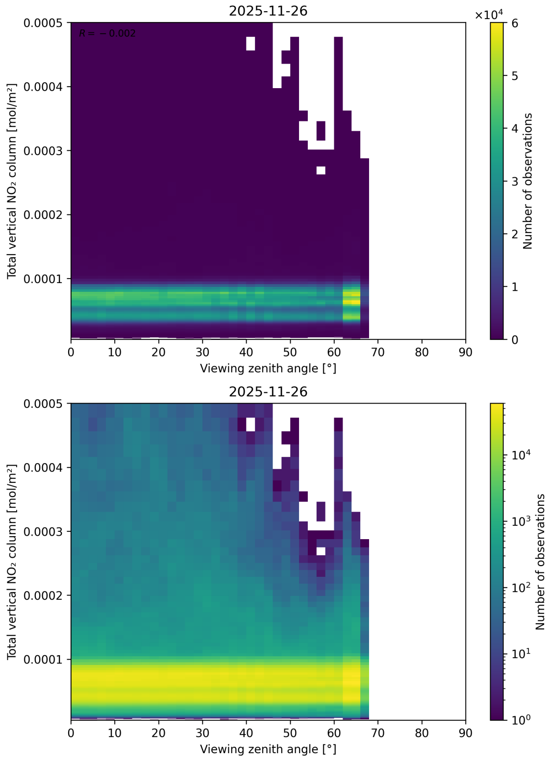
Figure 167: Scatter density plot of “Viewing zenith angle” against “Total vertical NO 2 column” for 2025-11-25 to 2025-11-27.
