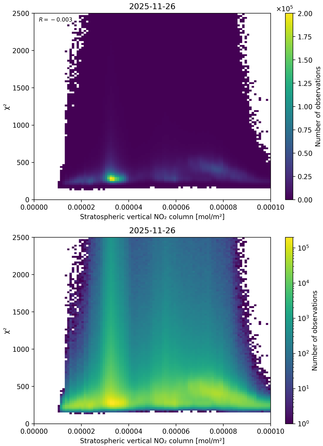
Figure 97: Scatter density plot of “Stratospheric vertical NO 2 column” against “ \chi^2 ” for 2025-11-25 to 2025-11-27.
