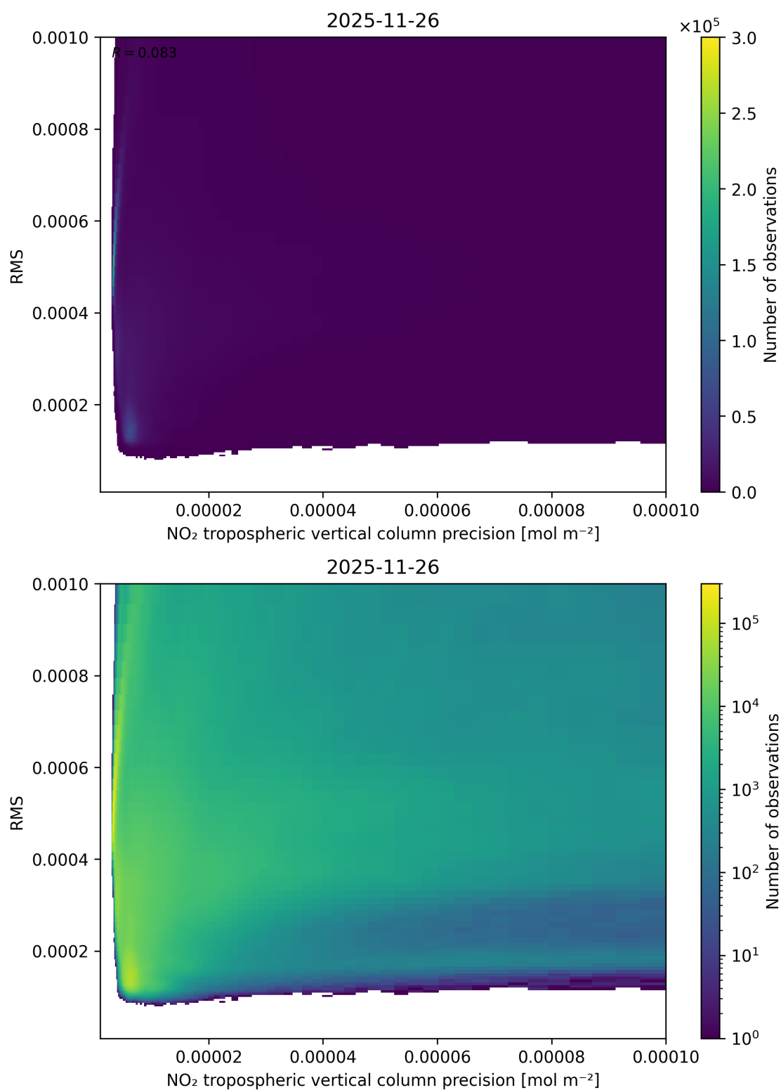
Figure 140: Scatter density plot of “NO 2 tropospheric vertical column precision” against “RMS” for 2025-11-25 to 2025-11-27.
