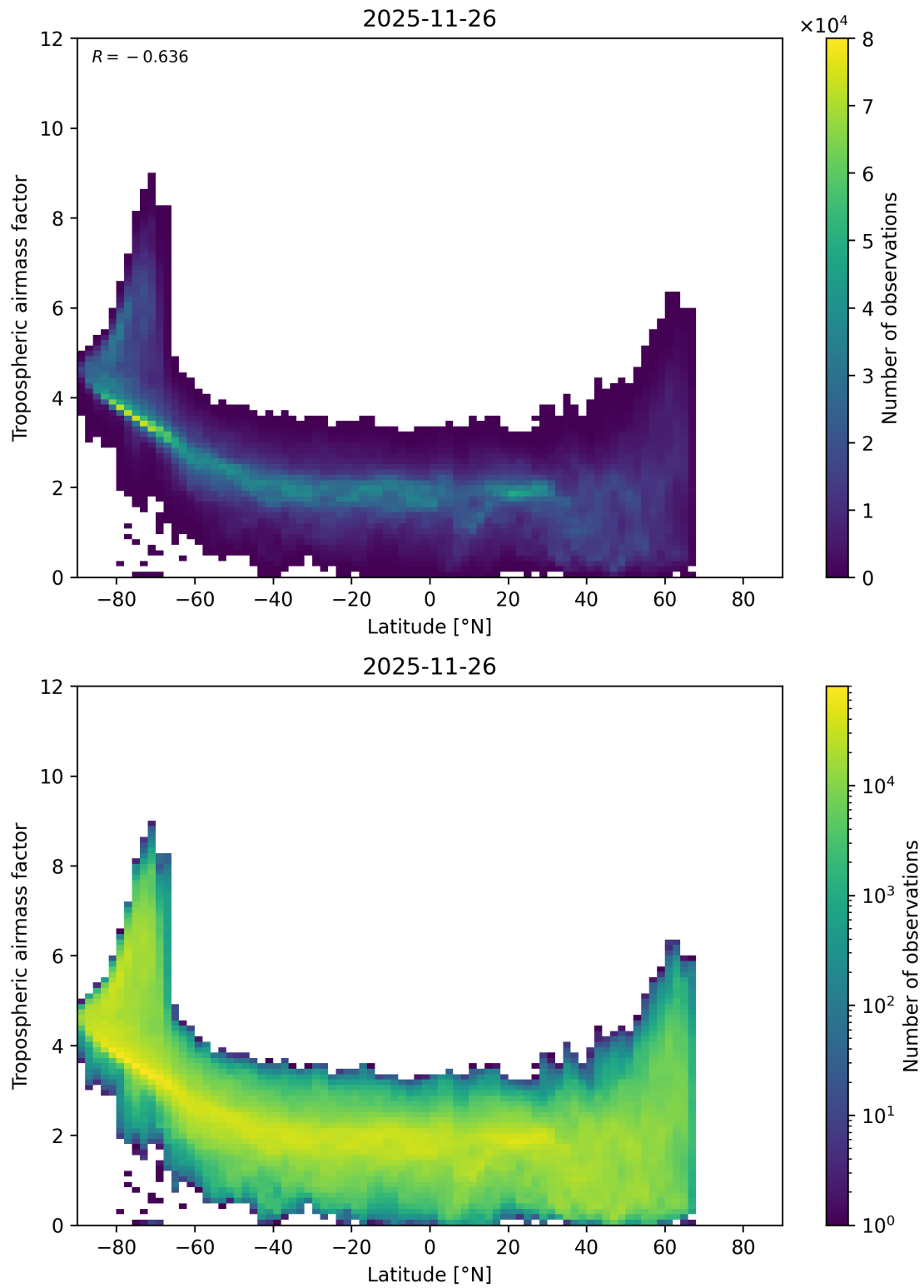
Figure 85: Scatter density plot of “Latitude” against “Tropospheric airmass factor” for 2025-11-25 to 2025-11-27.
