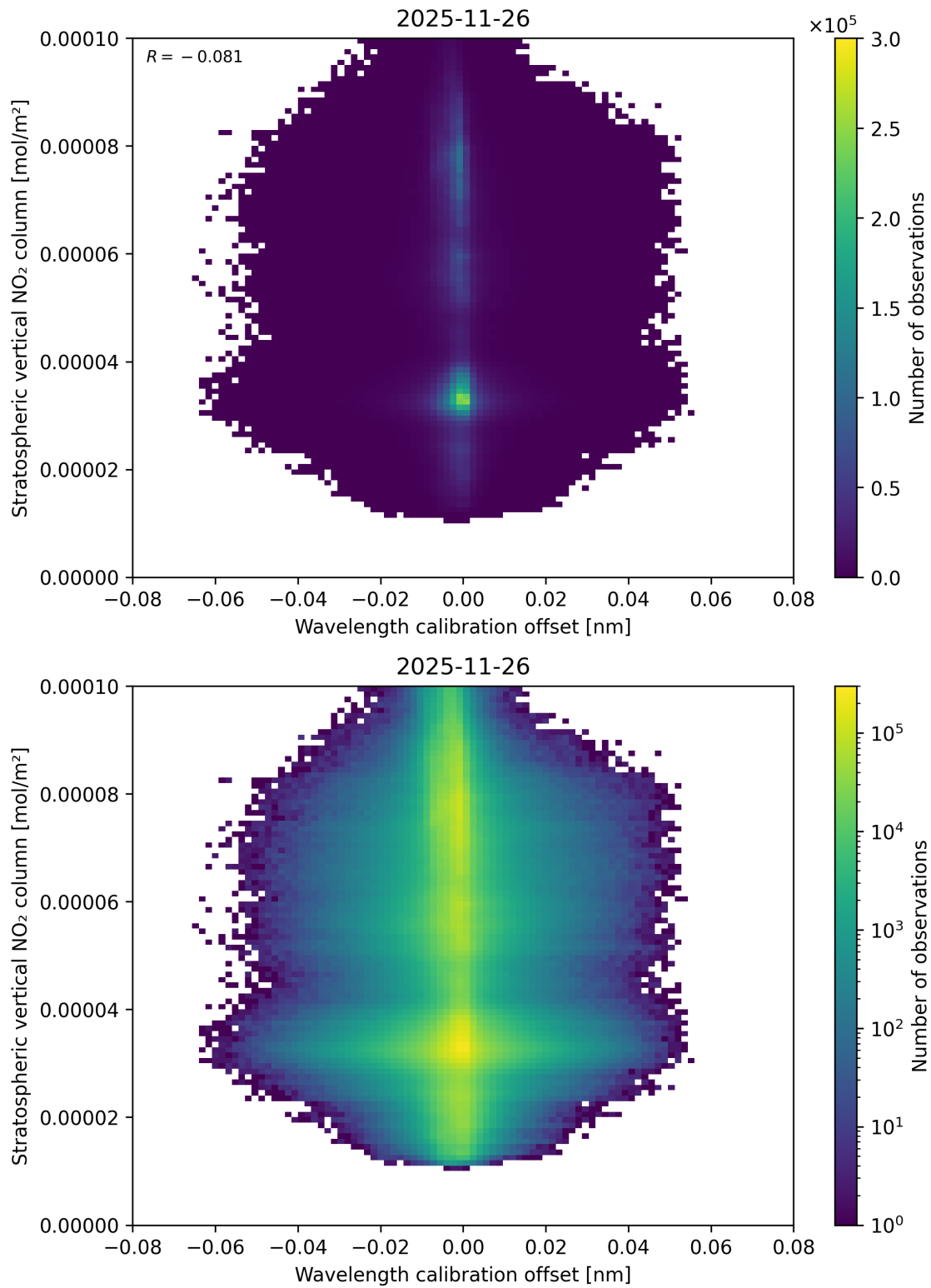
Figure 176: Scatter density plot of “Wavelength calibration offset” against “Stratospheric vertical NO 2 column” for 2025-11-25 to 2025-11-27.
