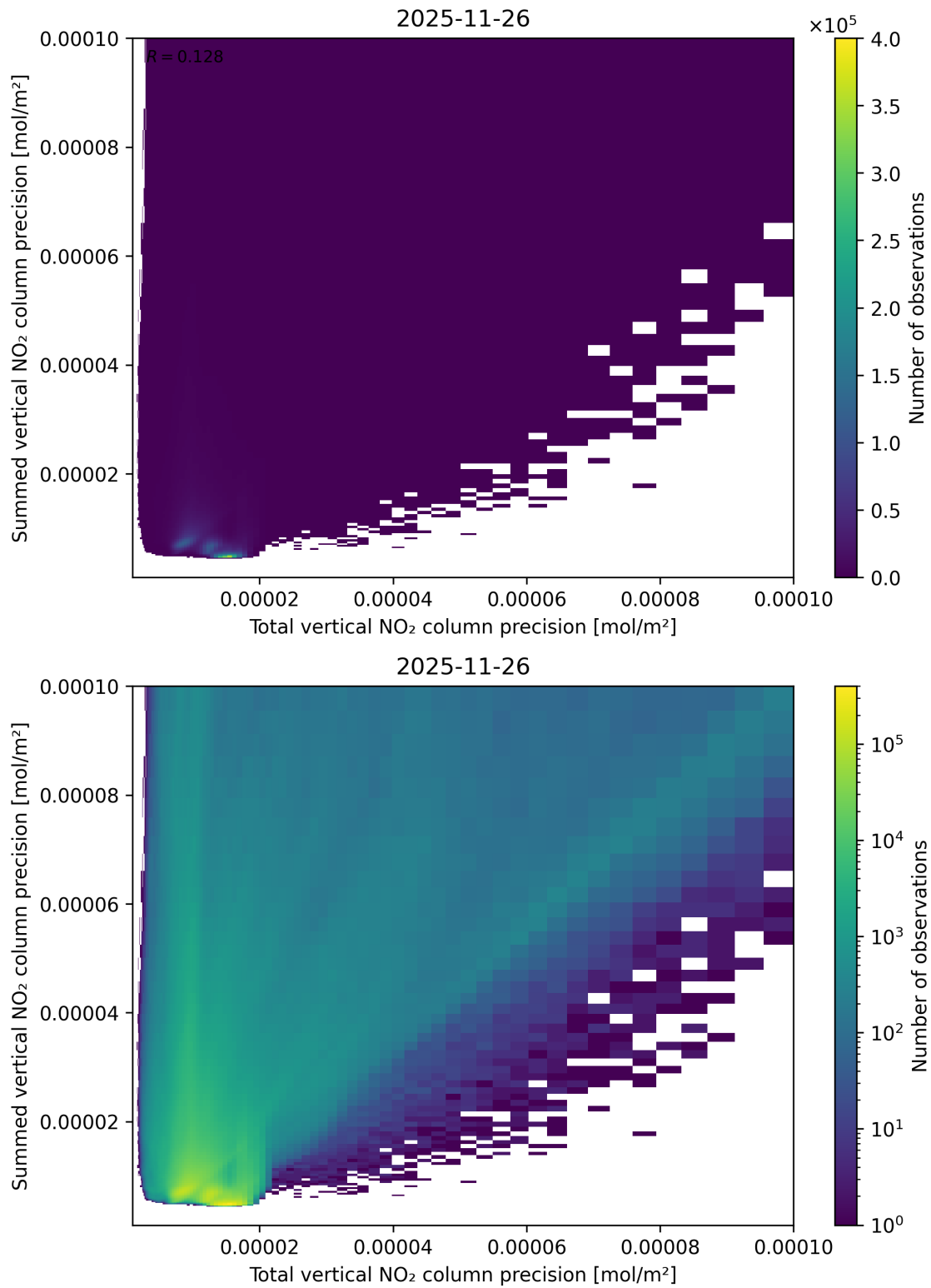
Figure 118: Scatter density plot of “Total vertical NO 2 column precision” against “Summed vertical NO 2 column precision” for 2025-11-25 to 2025-11-27.
