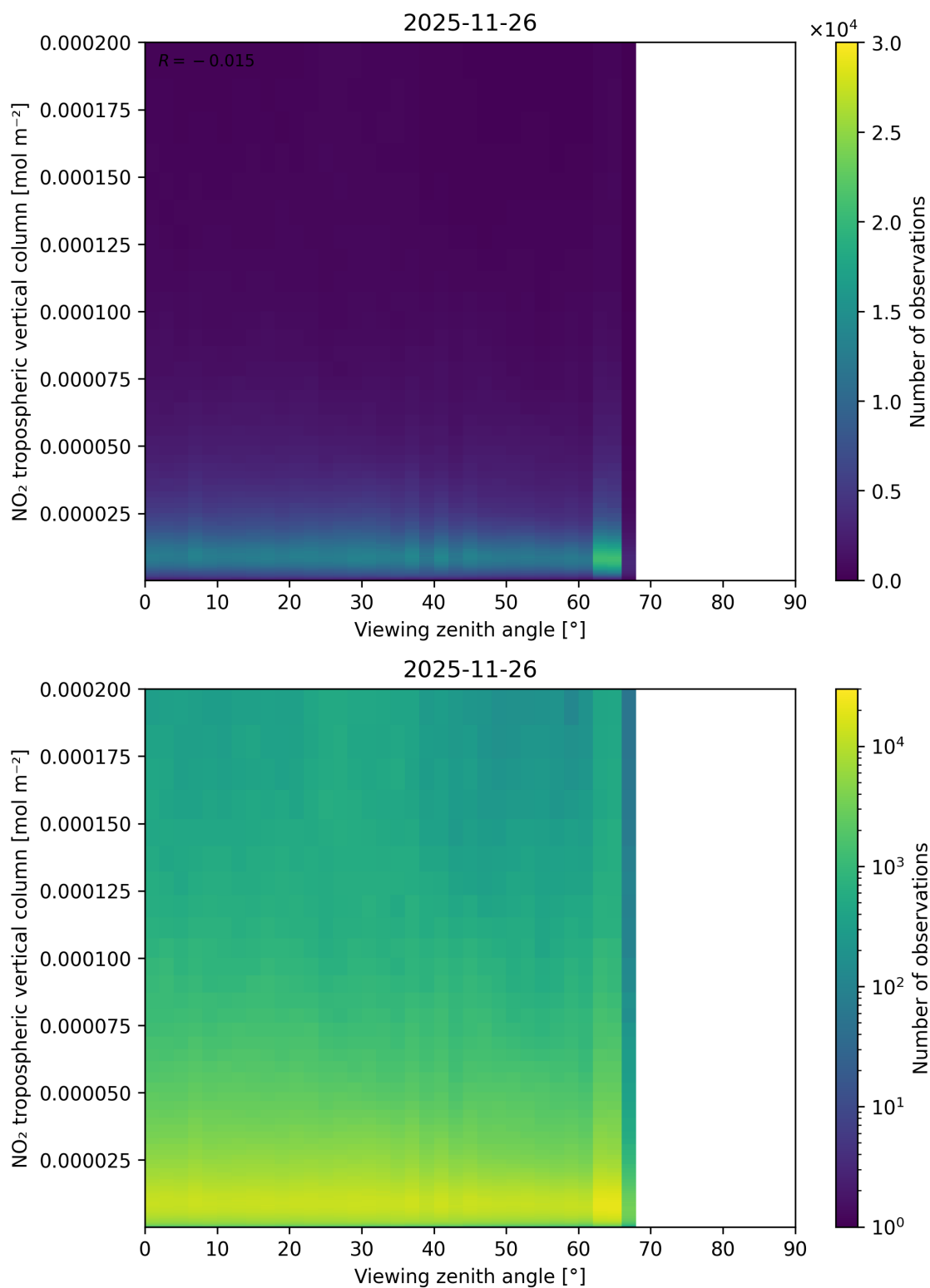
Figure 169: Scatter density plot of “Viewing zenith angle” against “NO 2 tropospheric vertical column” for 2025-11-25 to 2025-11-27.
