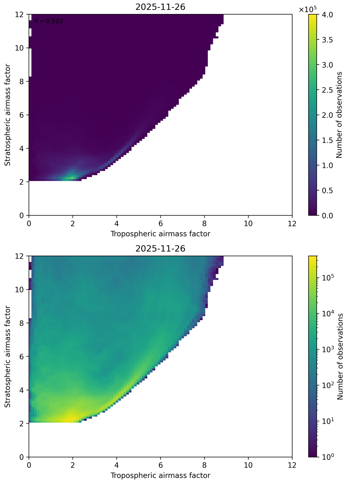
Figure 71: Scatter density plot of “Tropospheric airmass factor” against “Stratospheric airmass factor” for 2025-11-25 to 2025-11-27.
