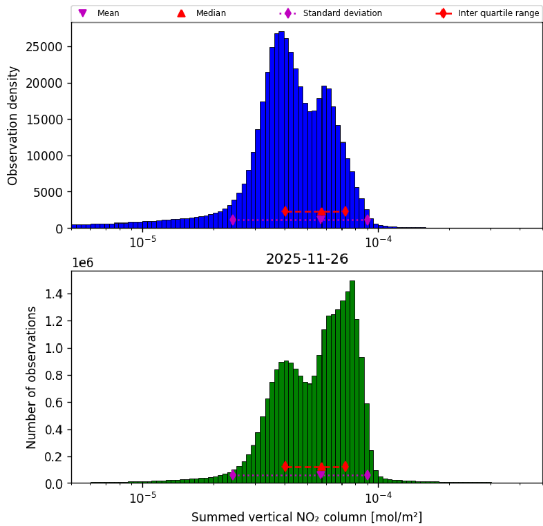
Figure 40: Histogram of “Summed vertical NO 2 column” for 2025-11-25 to 2025-11-27
