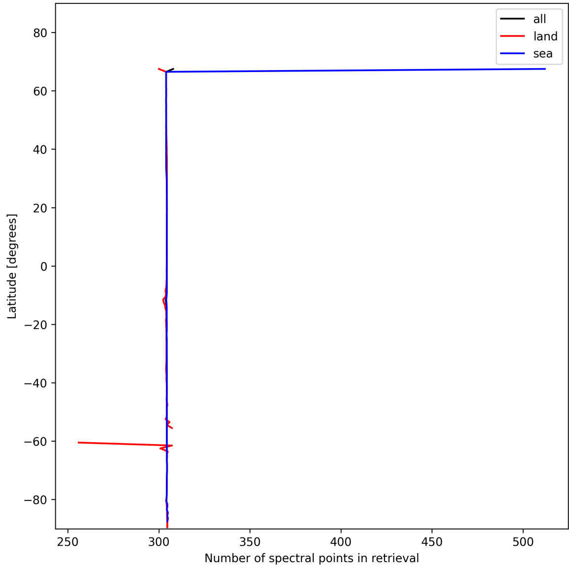
Figure 16: Zonal average of “Number of spectral points in retrieval” for 2025-11-25 to 2025-11-27.
