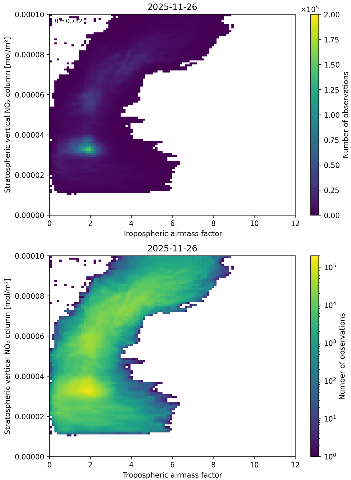
Figure 74: Scatter density plot of “Tropospheric air mass factor” against “Stratospheric vertical NO 2 column” for 2025-11-25 to 2025-11-27.
