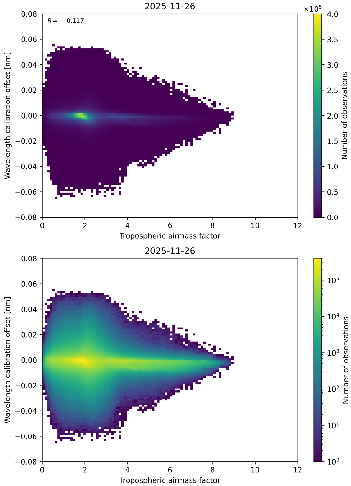
Figure 80: Scatter density plot of “Tropospheric airmass factor” against “Wavelength calibration offset” for 2025-11-25 to 2025-11-27.
