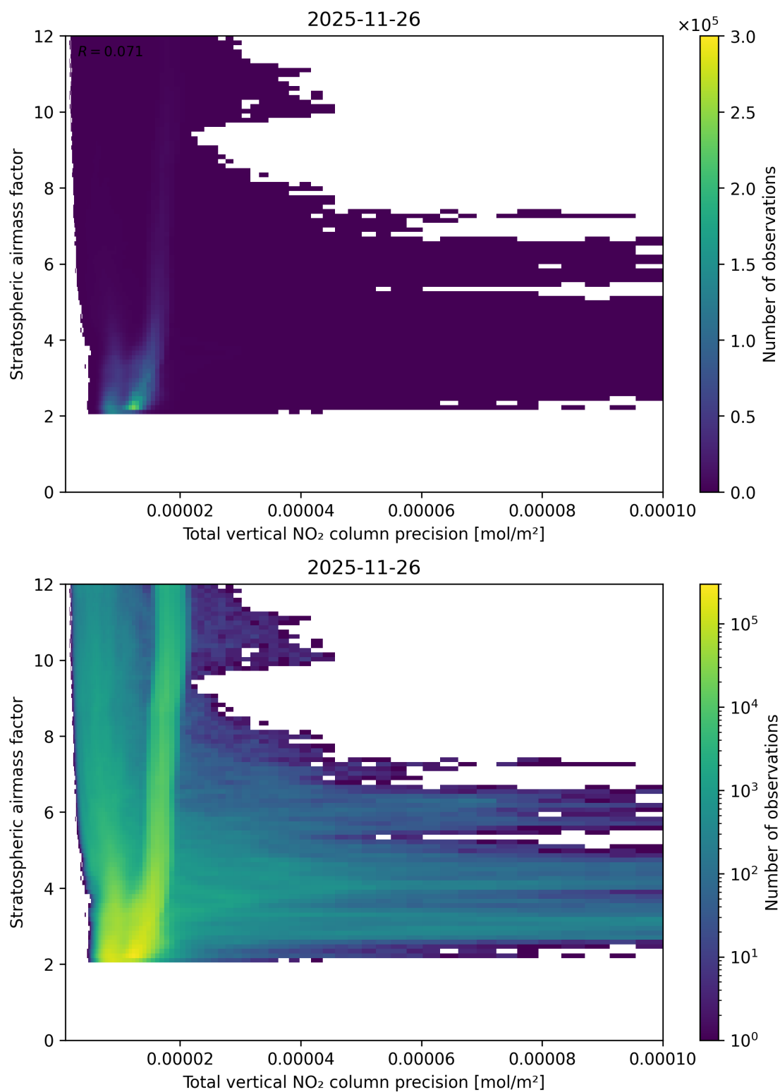
Figure 115: Scatter density plot of “Total vertical NO 2 column precision” against “Stratospheric air mass factor” for 2025-11-25 to 2025-11-27.
