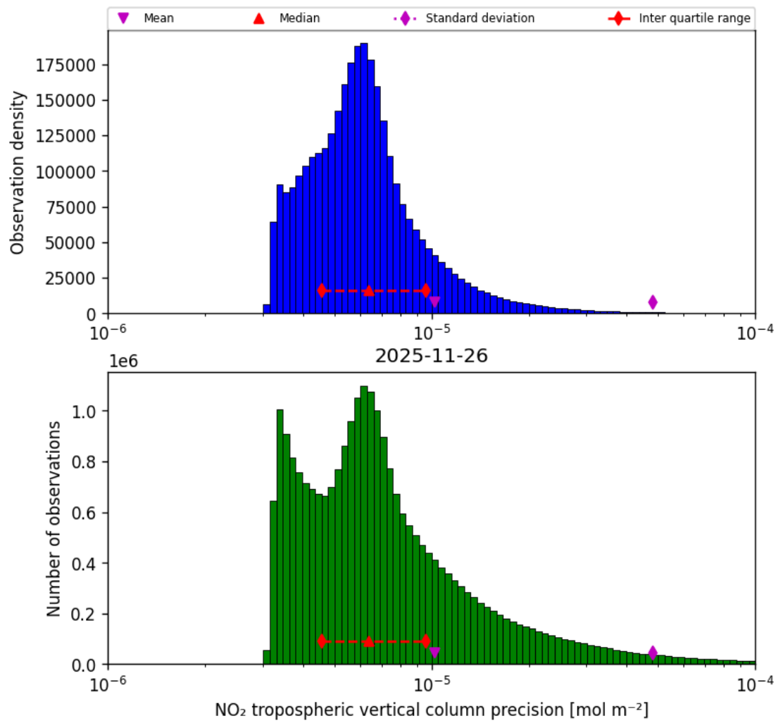
Figure 30: Histogram of “NO 2 tropospheric vertical column precision” for 2025-11-25 to 2025-11-27
