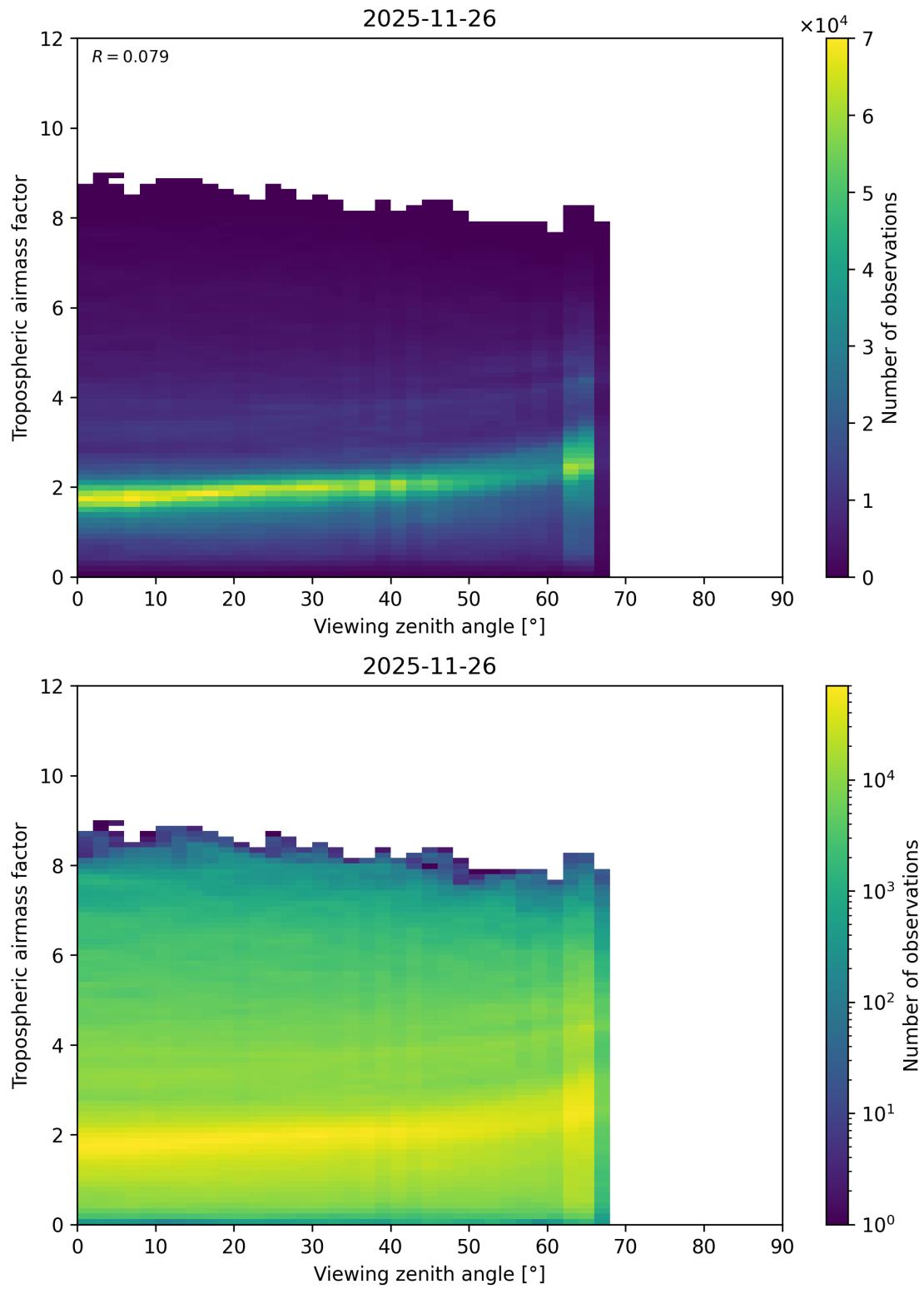
Figure 161: Scatter density plot of “Viewing zenith angle” against “Tropospheric airmass factor” for 2025-11-25 to 2025-11-27.
