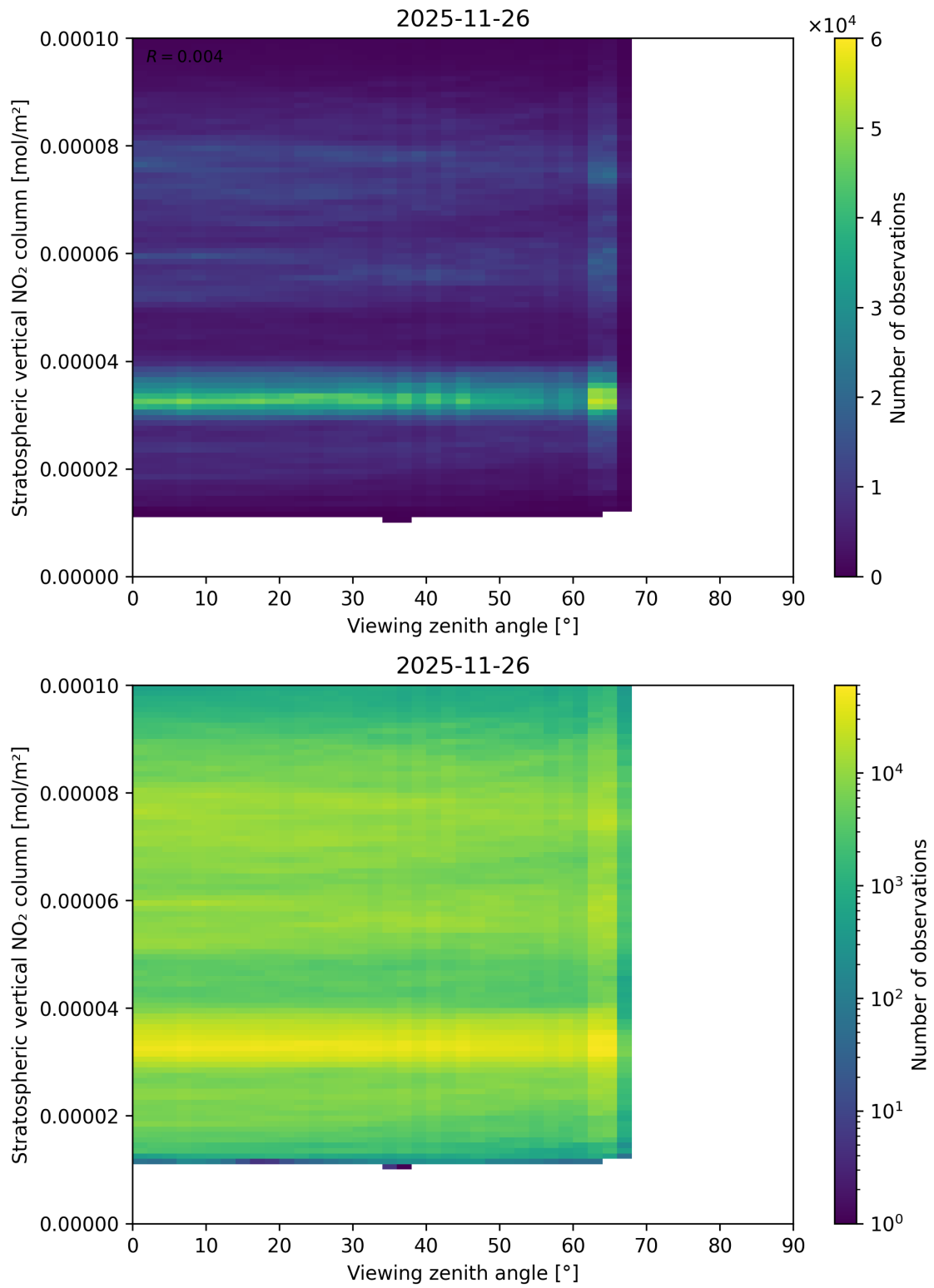
Figure 164: Scatter density plot of “Viewing zenith angle” against “Stratospheric vertical NO 2 column” for 2025-11-25 to 2025-11-27.
