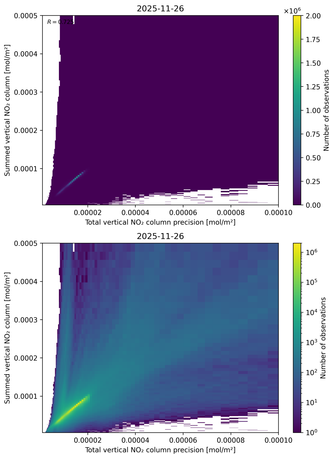
Figure 117: Scatter density plot of “Total vertical NO 2 column precision” against “Summed vertical NO 2 column” for 2025-11-25 to 2025-11-27.
