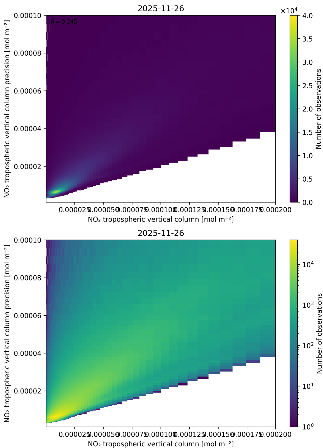
Figure 130: Scatter density plot of “NO 2 tropospheric vertical column” against “NO 2 tropospheric vertical column precision” for 2025-11-25 to 2025-11-27.
