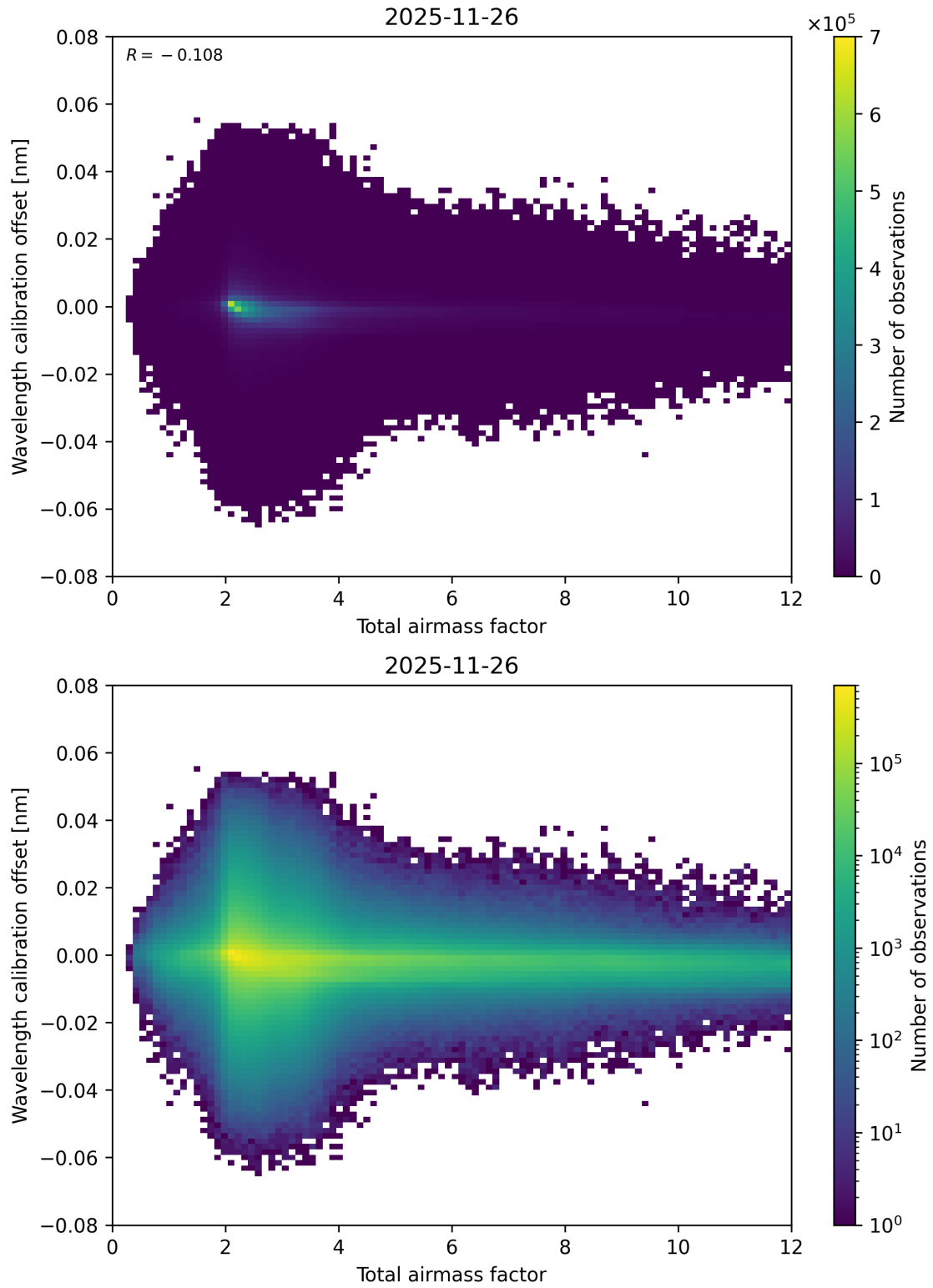
Figure 70: Scatter density plot of “Total airmass factor” against “Wavelength calibration offset” for 2025-11-25 to 2025-11-27.
