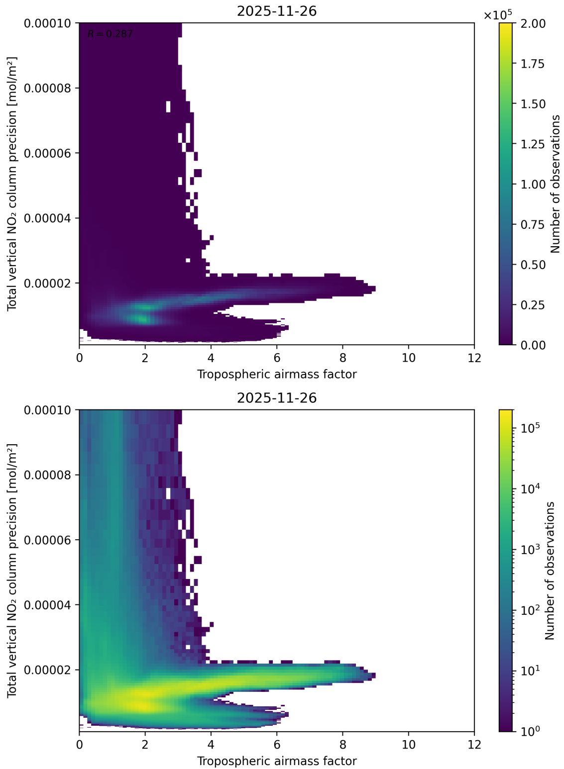
Figure 78: Scatter density plot of “Tropospheric airmass factor” against “Total vertical NO 2 column precision” for 2025-11-25 to 2025-11-27.
