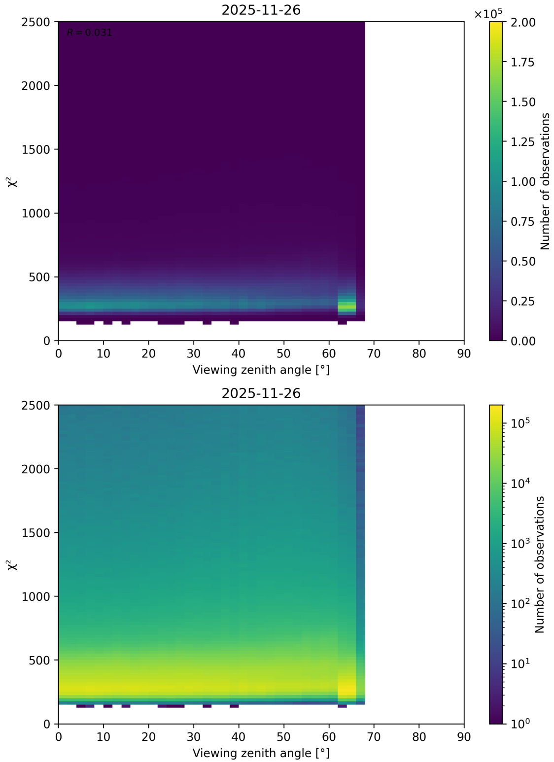
Figure 162: Scatter density plot of “Viewing zenith angle” against “ \chi^2 ” for 2025-11-25 to 2025-11-27.
