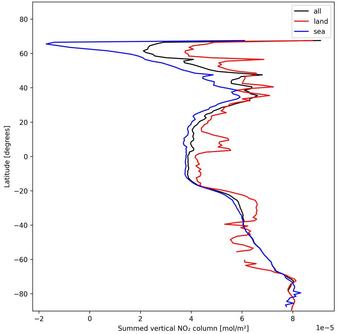
Figure 23: Zonal average of “Summed vertical NO 2 column” for 2025-11-25 to 2025-11-27.
