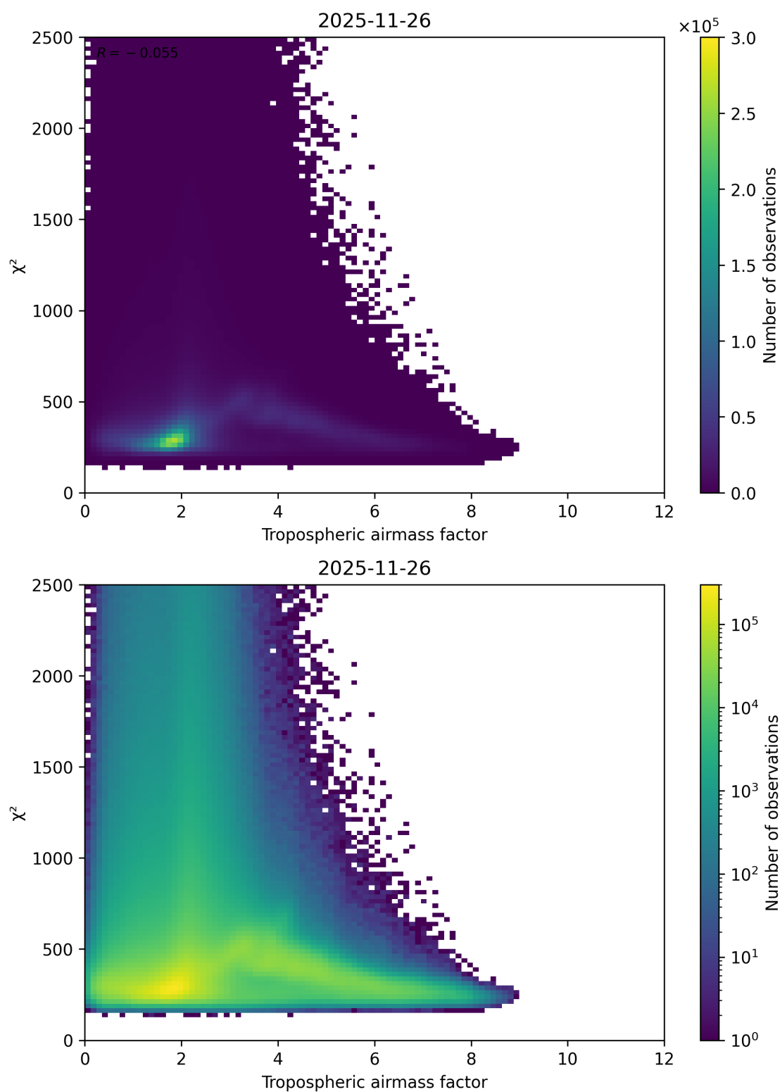
Figure 73: Scatter density plot of “Tropospheric airmass factor” against “ \chi^2 ” for 2025-11-25 to 2025-11-27.
