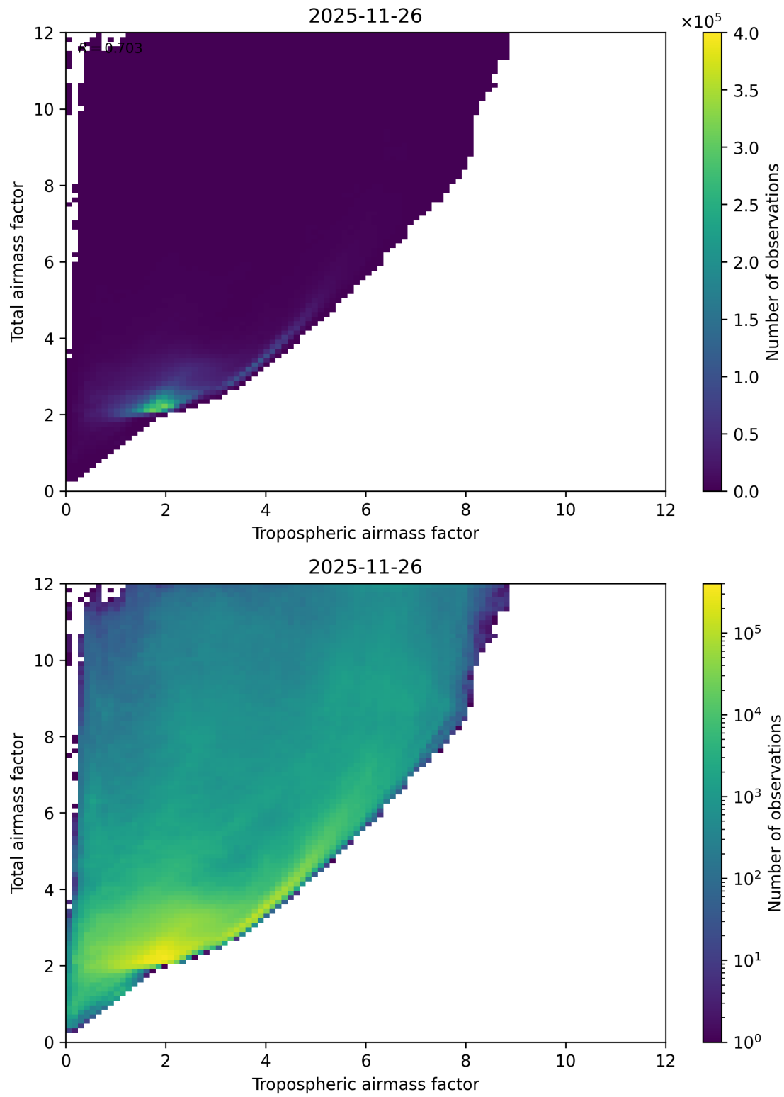
Figure 72: Scatter density plot of “Tropospheric airmass factor” against “Total airmass factor” for 2025-11-25 to 2025-11-27.
