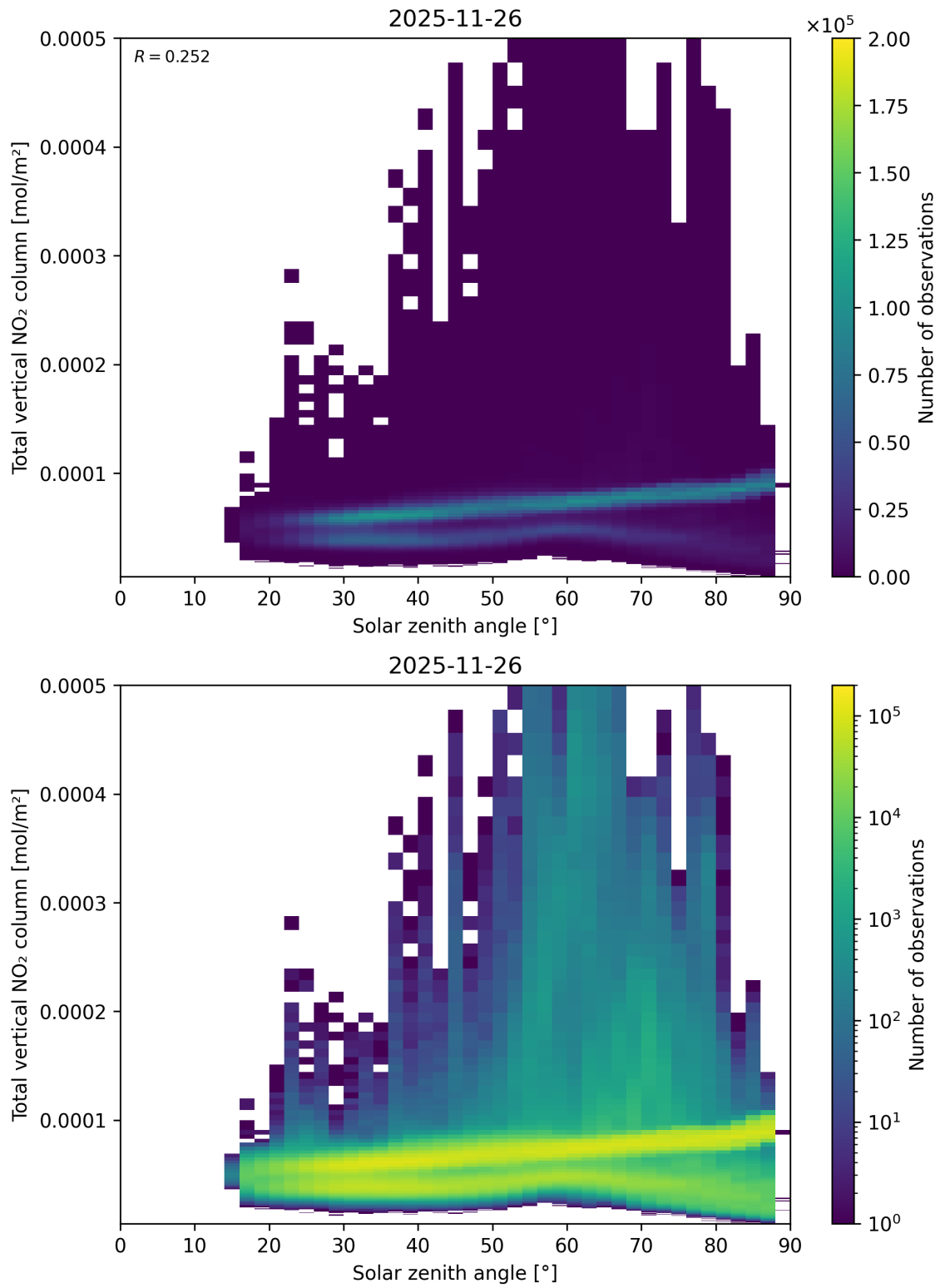
Figure 153: Scatter density plot of “Solar zenith angle” against “Total vertical \text{NO}_2 column” for 2025-11-25 to 2025-11-27.
