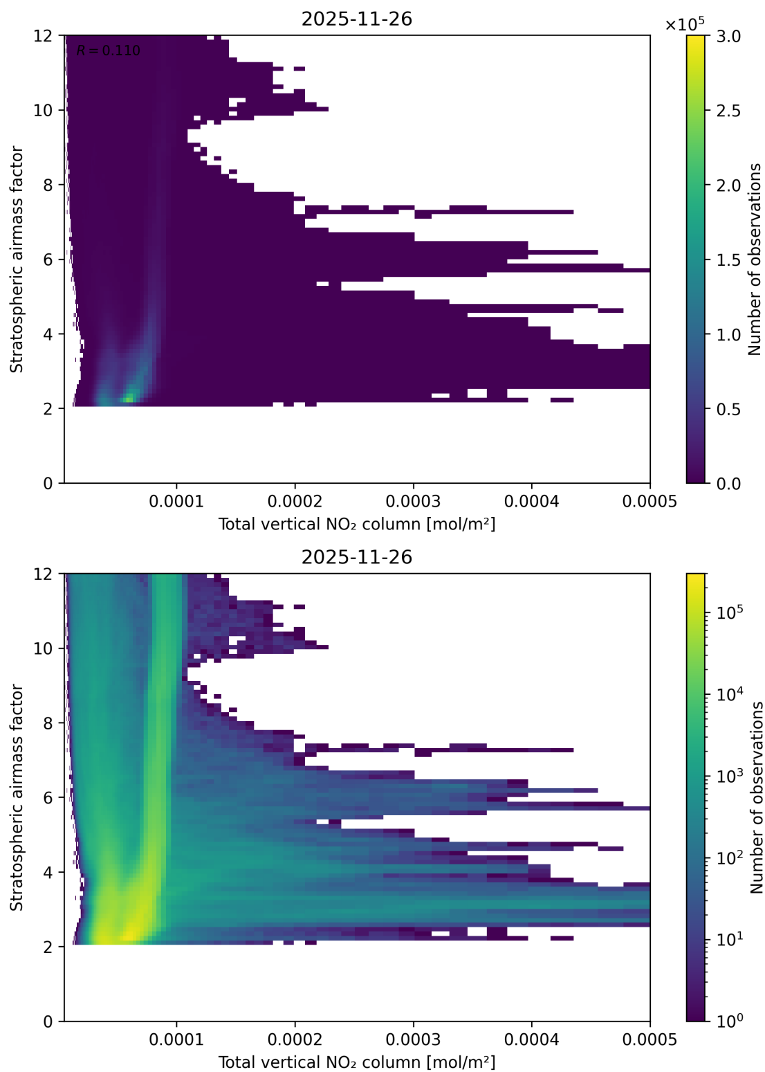
Figure 110: Scatter density plot of “Total vertical NO 2 column” against “Stratospheric airmass factor” for 2025-11-25 to 2025-11-27.
