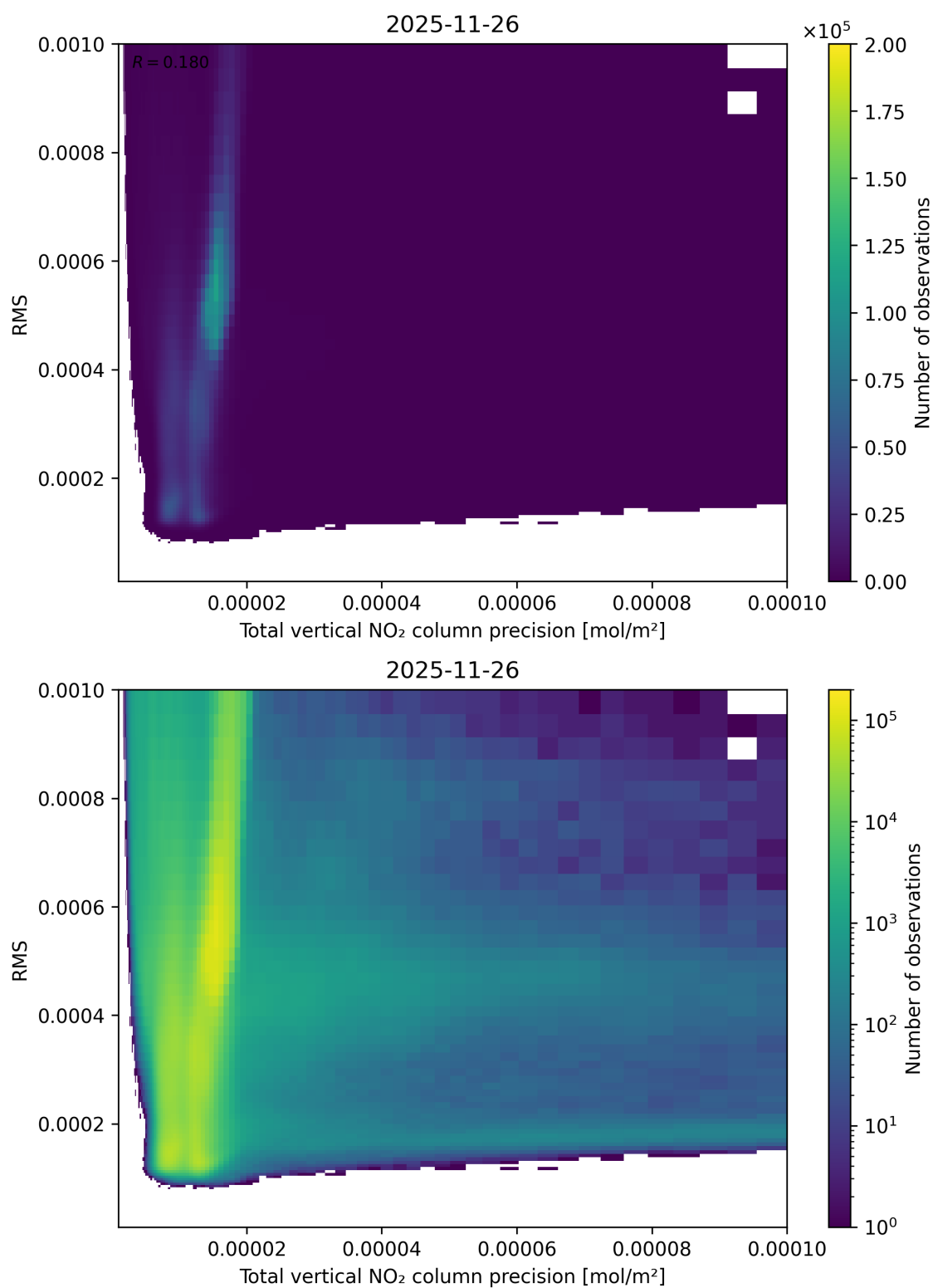
Figure 119: Scatter density plot of “Total vertical NO 2 column precision” against “RMS” for 2025-11-25 to 2025-11-27.
