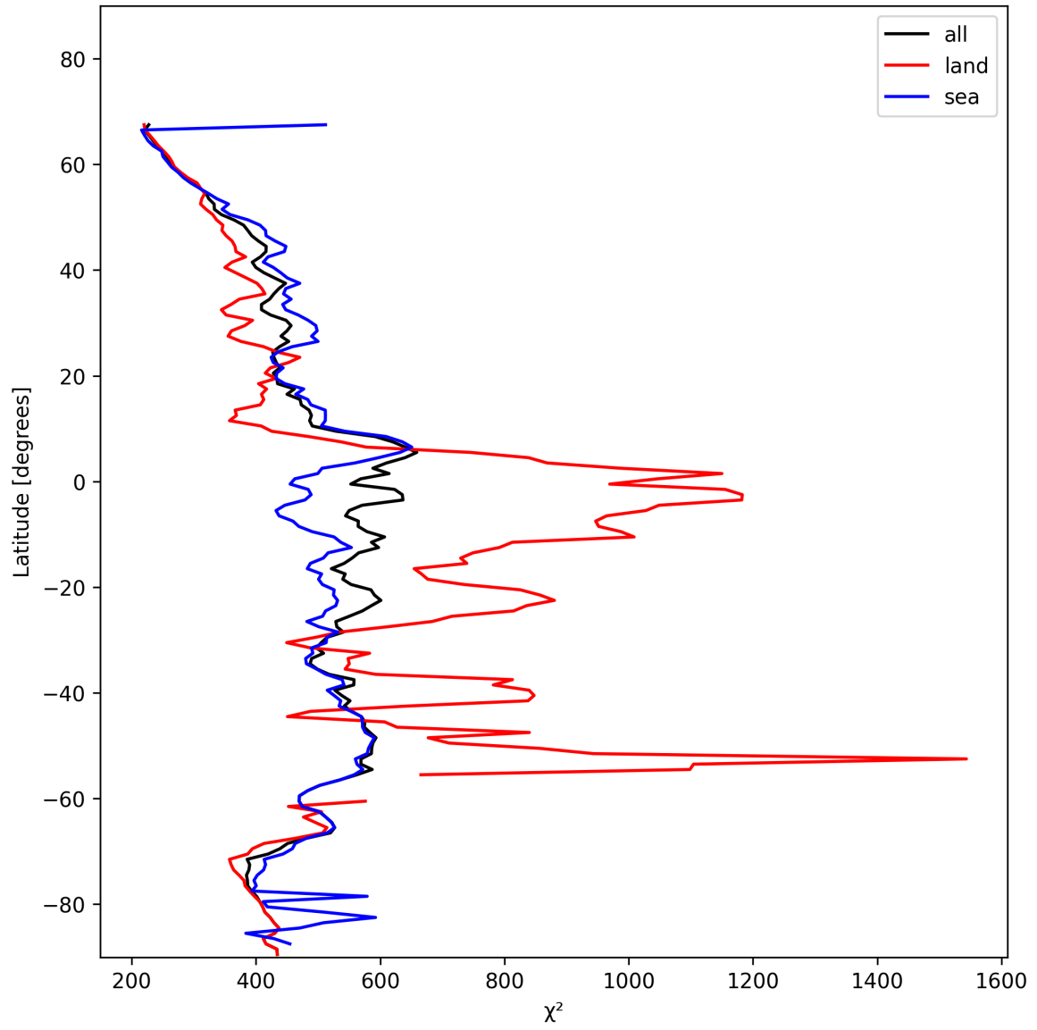
Figure 25: Zonal average of “ \chi^2 ” for 2025-11-25 to 2025-11-27.
