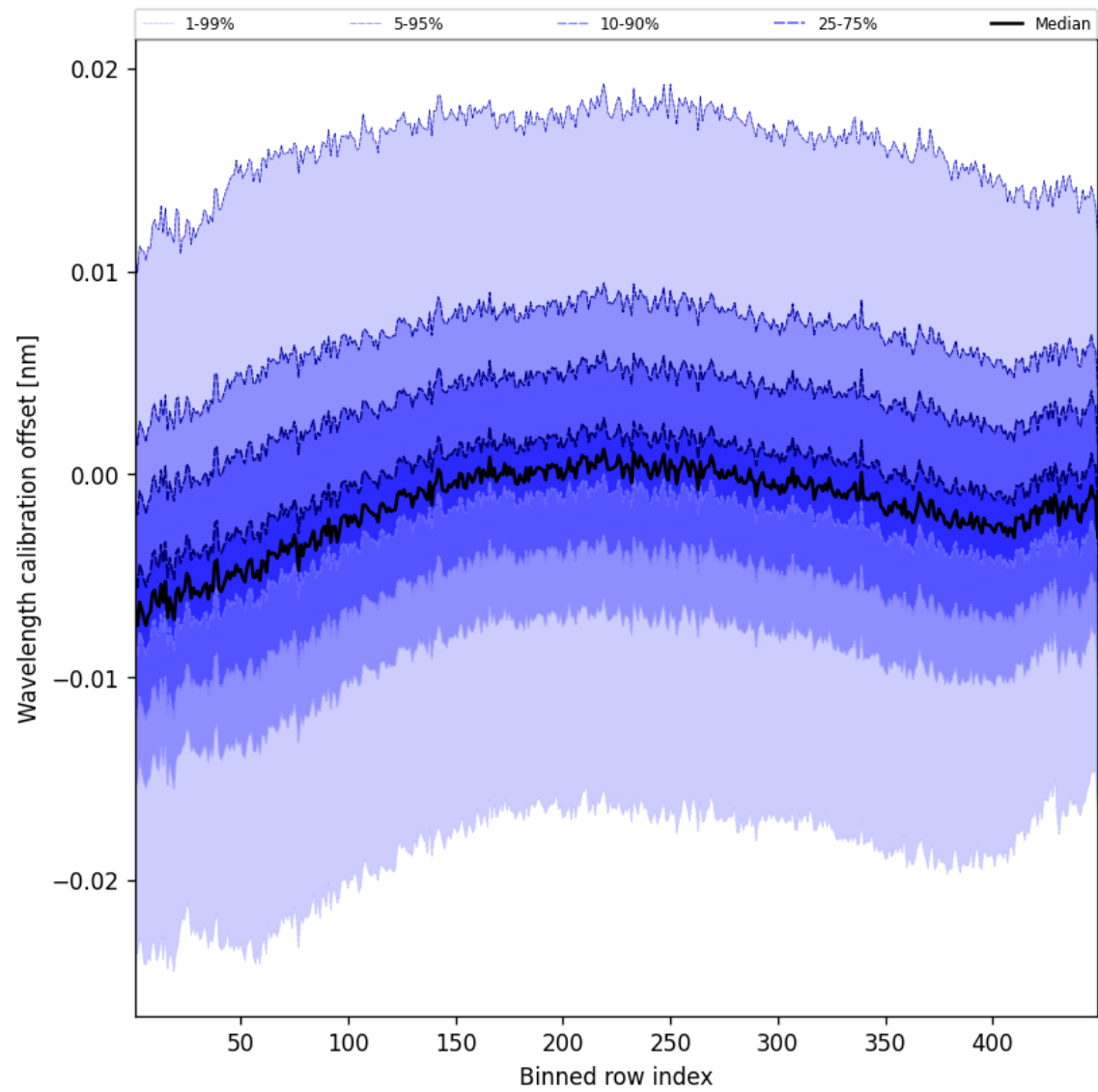
Figure 52: Along track statistics of “Wavelength calibration offset” for 2025-11-25 to 2025-11-27
