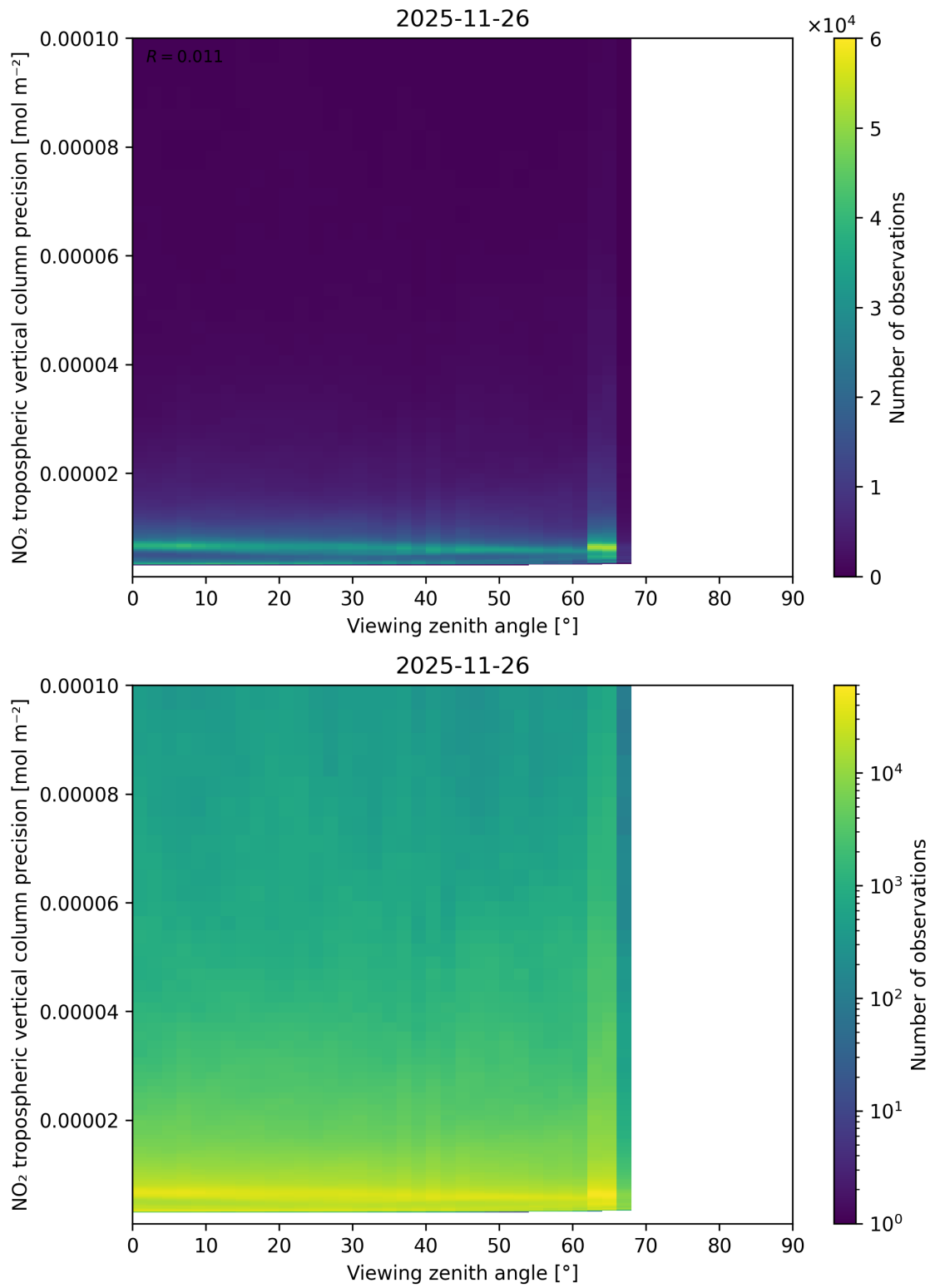
Figure 170: Scatter density plot of “Viewing zenith angle” against “NO 2 tropospheric vertical column precision” for 2025-11-25 to 2025-11-27.
