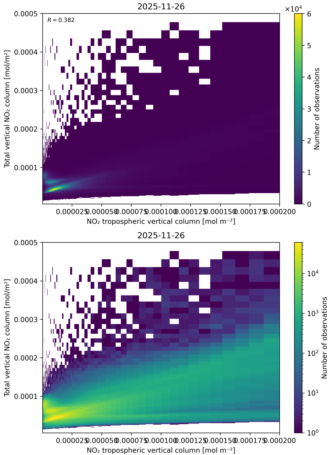
Figure 128: Scatter density plot of “NO 2 tropospheric vertical column” against “Total vertical NO 2 column” for 2025-11-25 to 2025-11-27.
