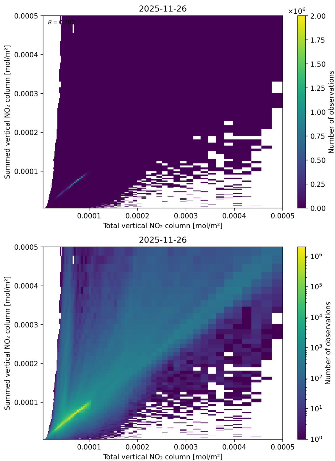
Figure 112: Scatter density plot of “Total vertical NO 2 column” against “Summed vertical NO 2 column” for 2025-11-25 to 2025-11-27.
