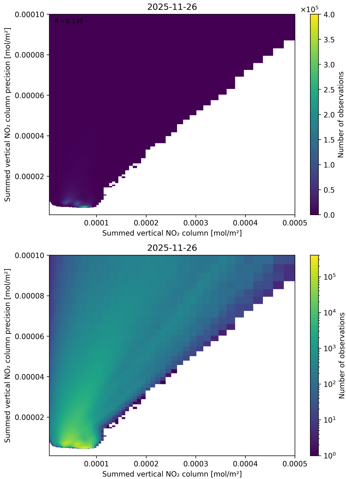
Figure 105: Scatter density plot of “Summed vertical NO 2 column” against “Summed vertical NO 2 column precision” for 2025-11-25 to 2025-11-27.
