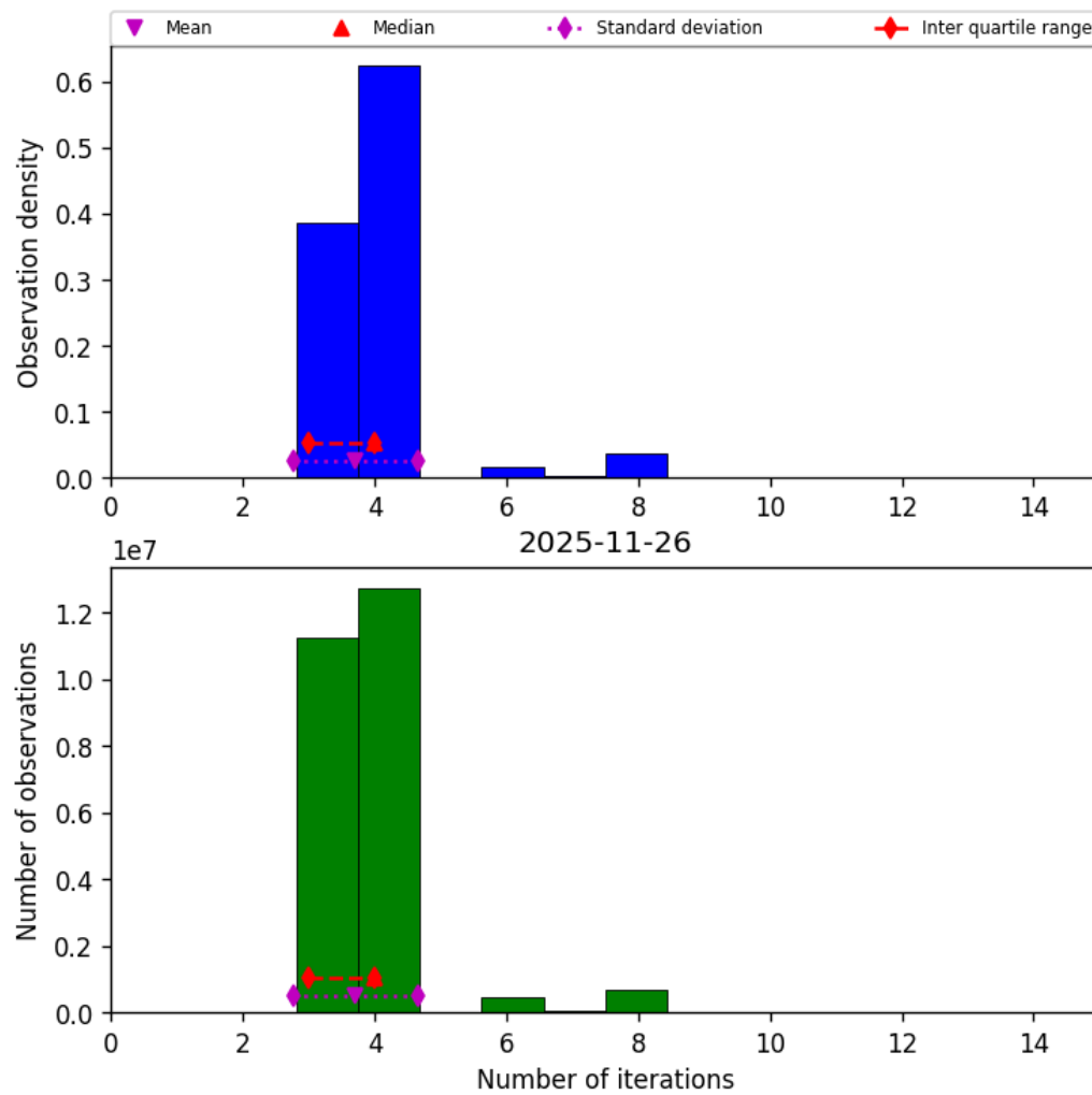
Figure 34: Histogram of “Number of iterations” for 2025-11-25 to 2025-11-27
