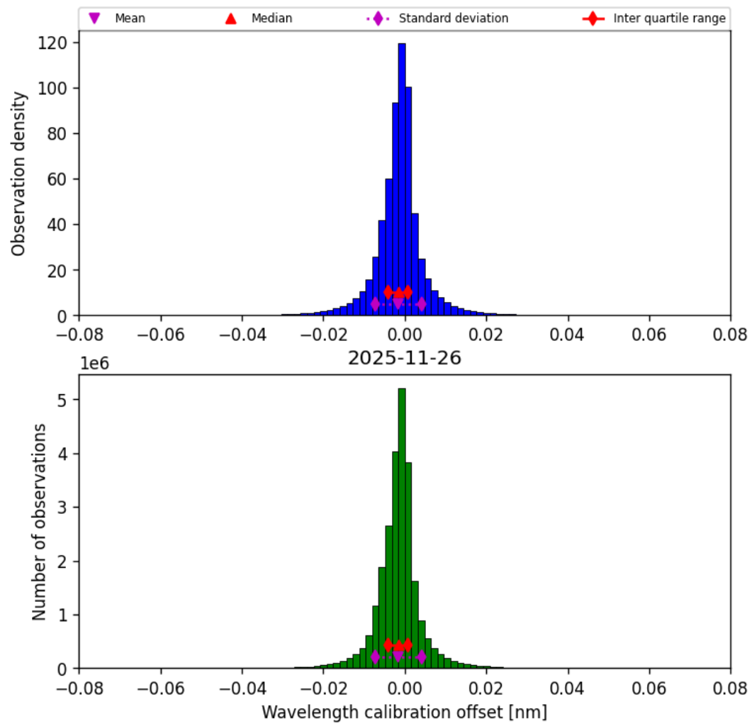
Figure 35: Histogram of “Wavelength calibration offset” for 2025-11-25 to 2025-11-27
