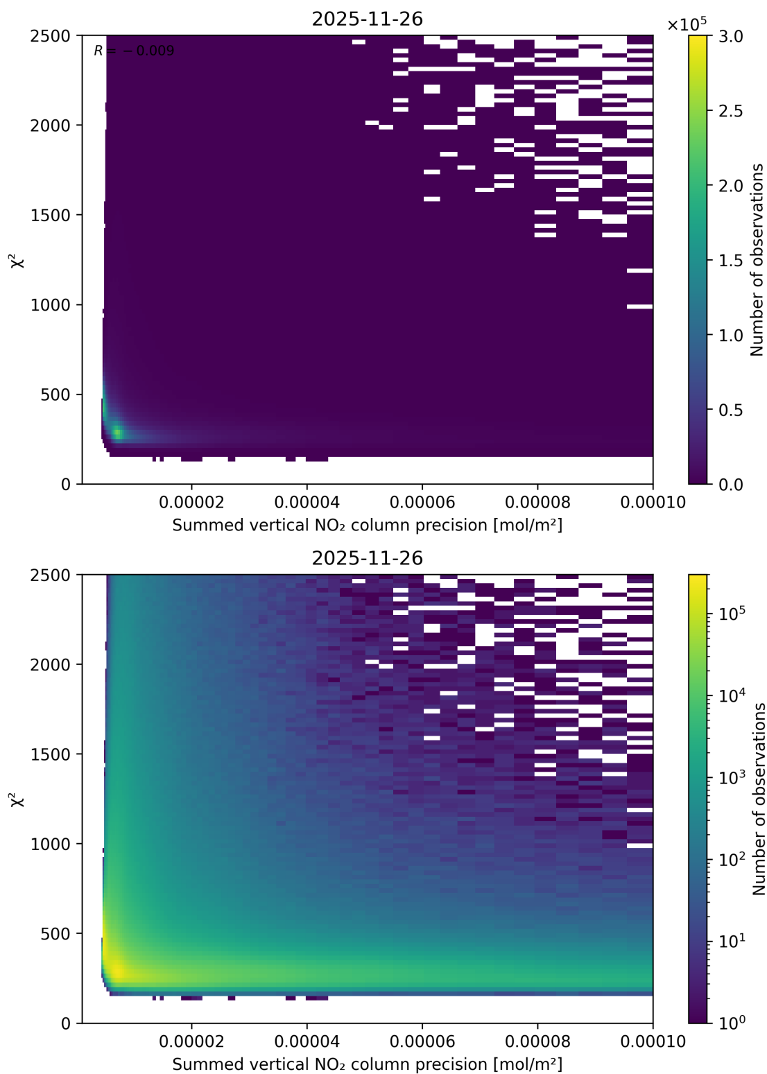
Figure 107: Scatter density plot of “Summed vertical NO 2 column precision” against “ \chi^2 ” for 2025-11-25 to 2025-11-27.
