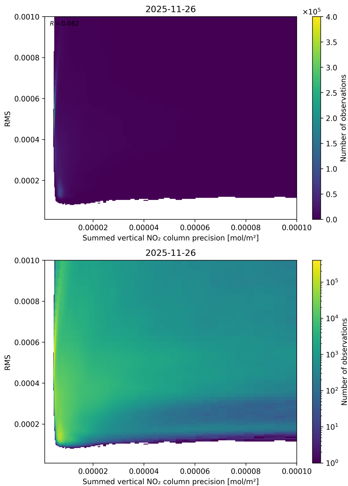
Figure 108: Scatter density plot of “Summed vertical NO 2 column precision” against “RMS” for 2025-11-25 to 2025-11-27.
