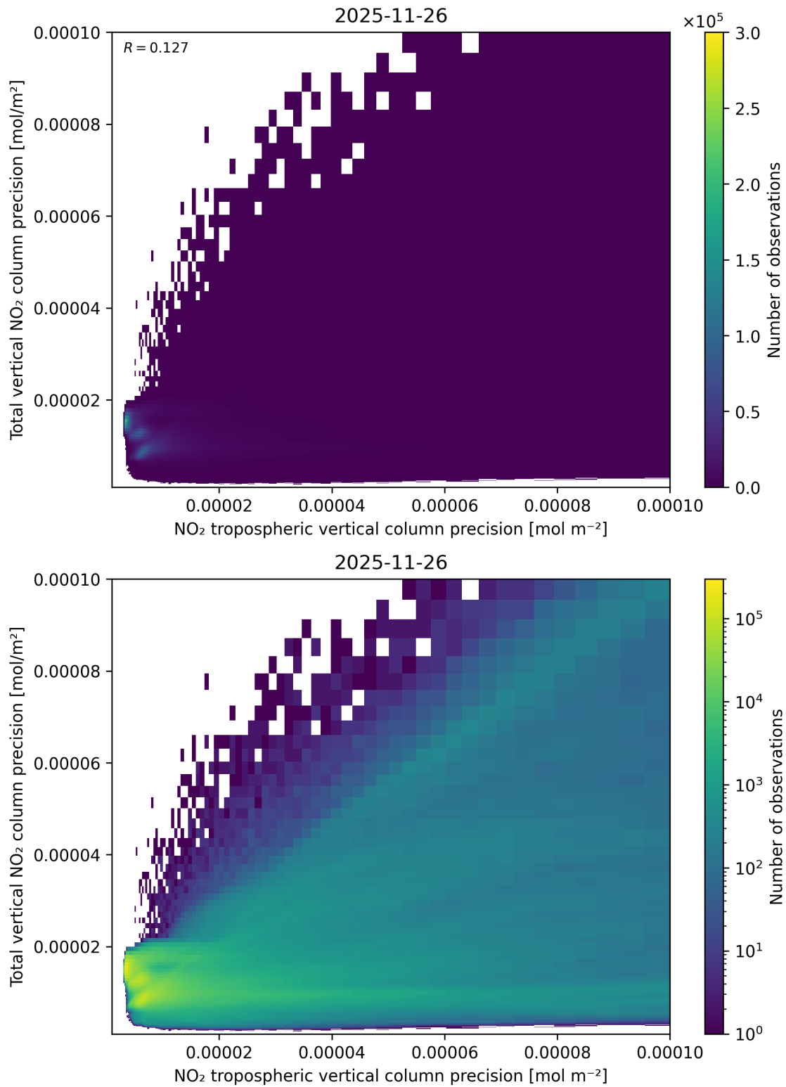
Figure 139: Scatter density plot of “NO 2 tropospheric vertical column precision” against “Total vertical NO 2 column precision” for 2025-11-25 to 2025-11-27.
