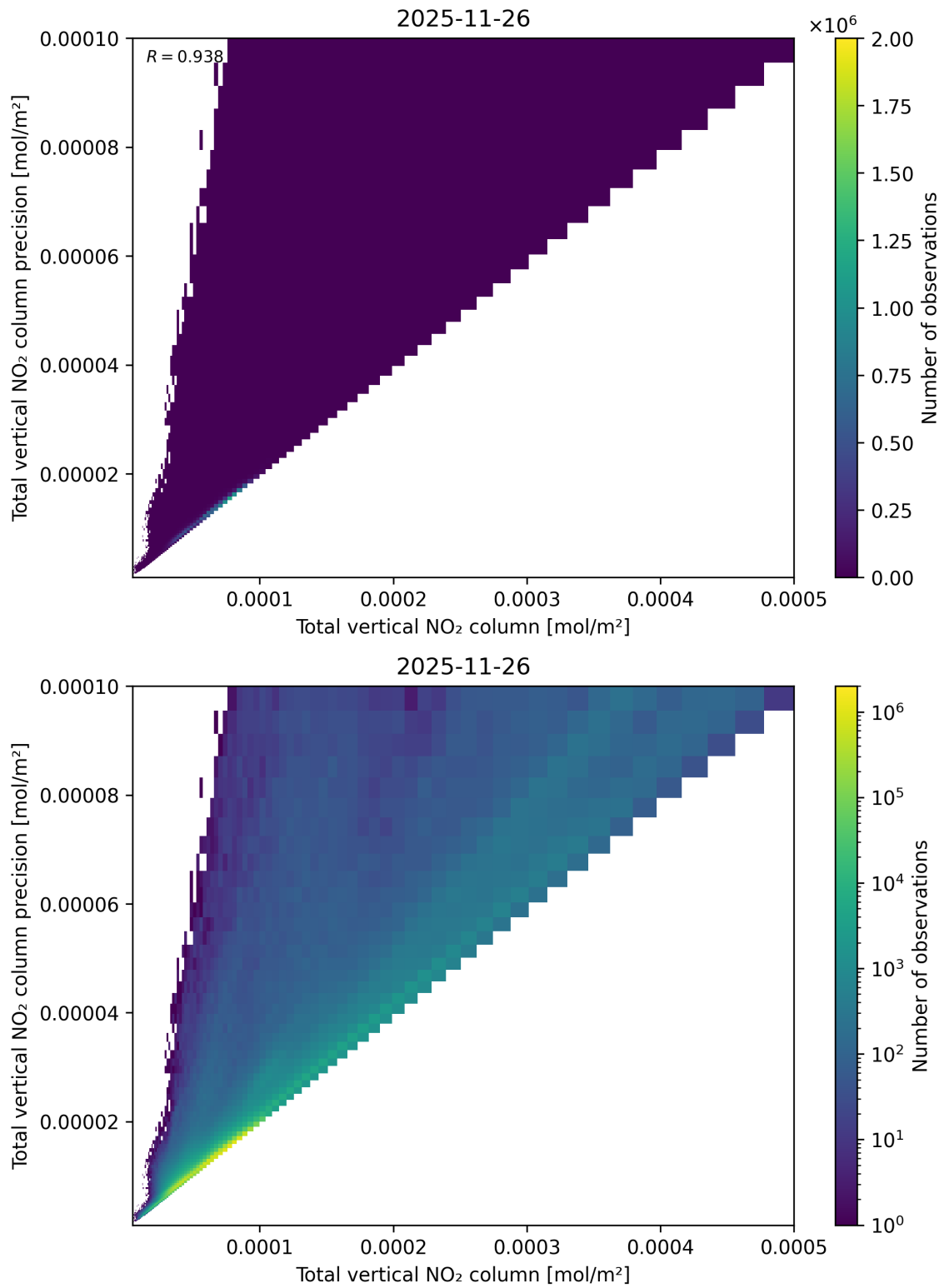
Figure 114: Scatter density plot of “Total vertical NO 2 column” against “Total vertical NO 2 column precision” for 2025-11-25 to 2025-11-27.
