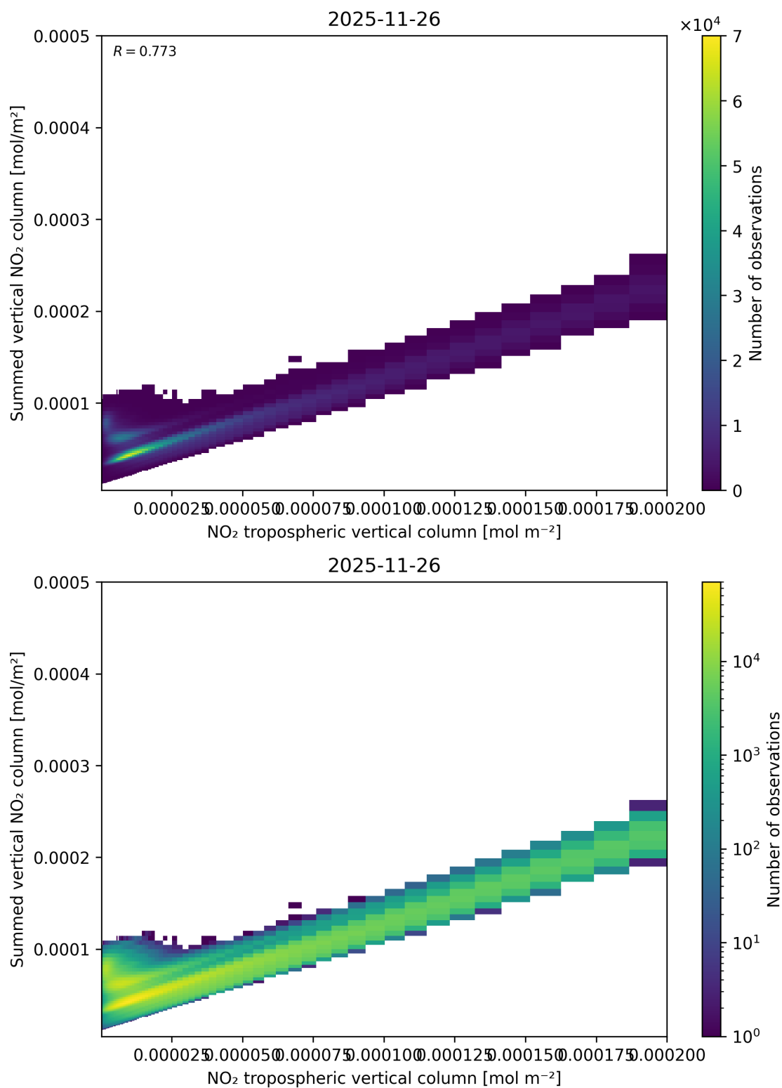
Figure 126: Scatter density plot of “NO 2 tropospheric vertical column” against “Summed vertical NO 2 column” for 2025-11-25 to 2025-11-27.
