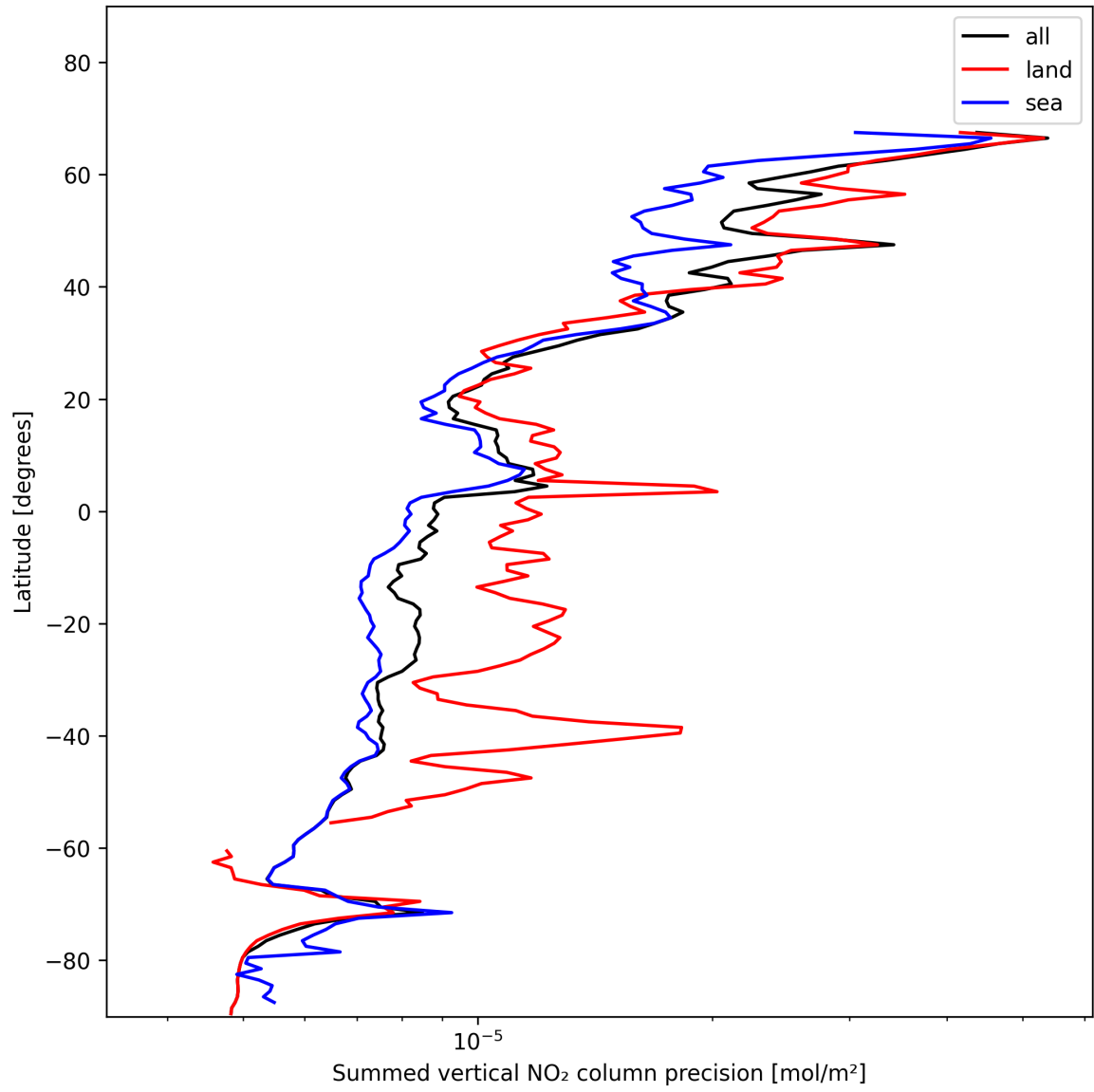
Figure 24: Zonal average of “Summed vertical NO 2 column precision” for 2025-11-25 to 2025-11-27.
