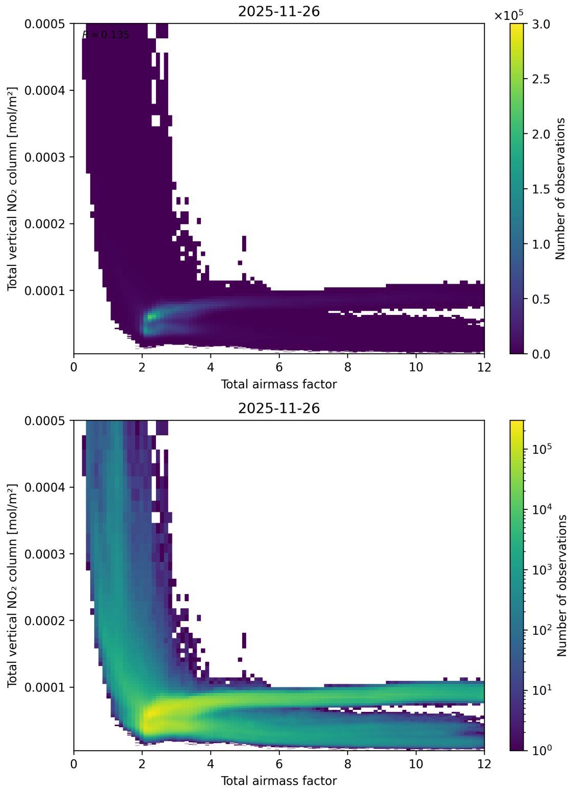
Figure 67: Scatter density plot of “Total airmass factor” against “Total vertical NO 2 column” for 2025-11-25 to 2025-11-27.
