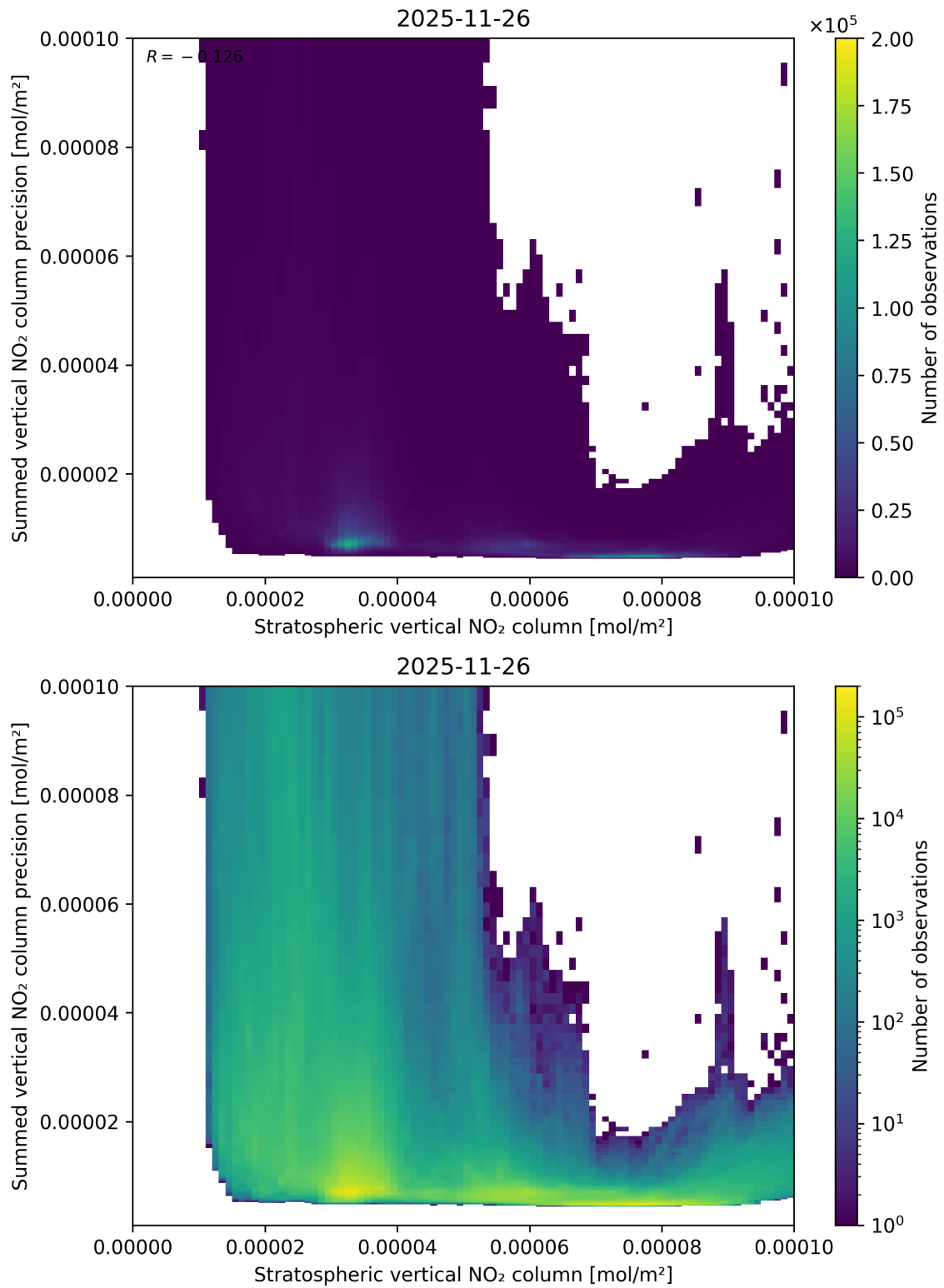
Figure 99: Scatter density plot of “Stratospheric vertical NO 2 column” against “Summed vertical NO 2 column precision” for 2025-11-25 to 2025-11-27.
