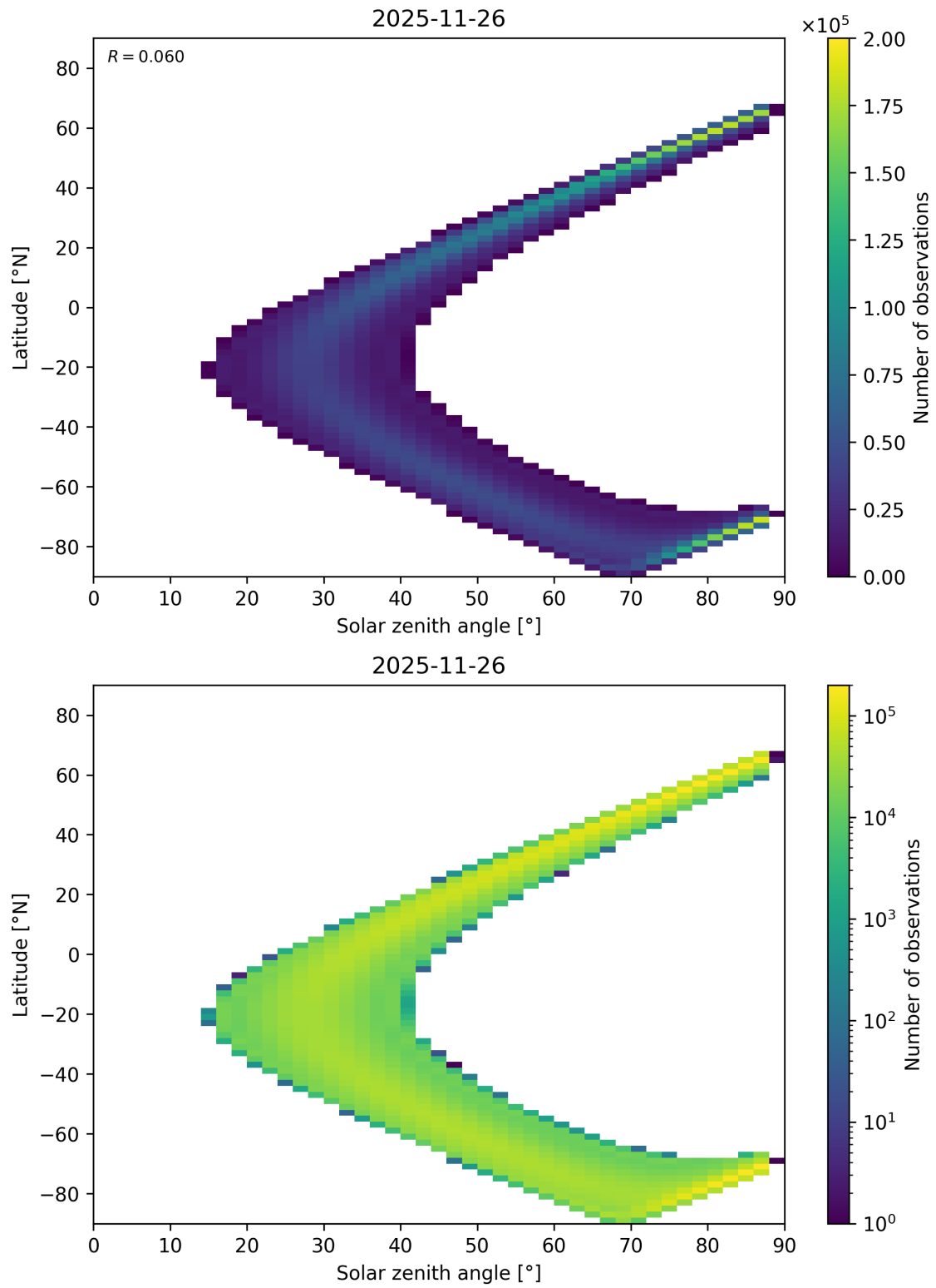
Figure 149: Scatter density plot of “Solar zenith angle” against “Latitude” for 2025-11-25 to 2025-11-27.
