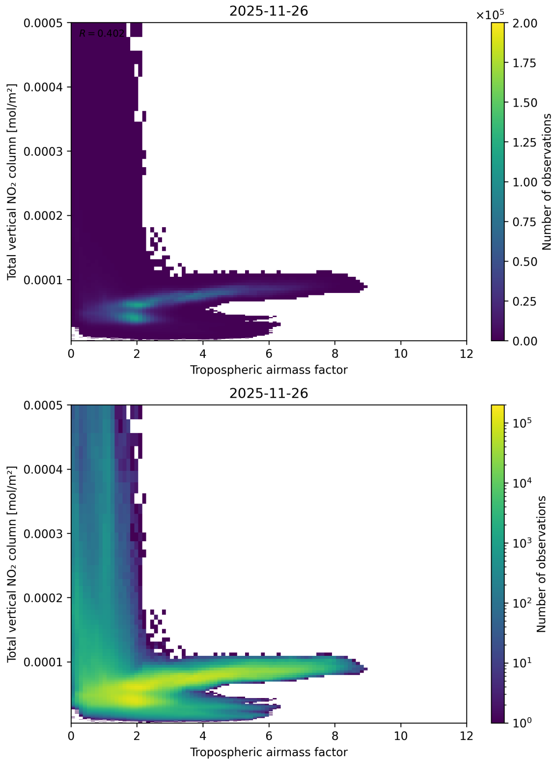
Figure 77: Scatter density plot of “Tropospheric airmass factor” against “Total vertical NO 2 column” for 2025-11-25 to 2025-11-27.
