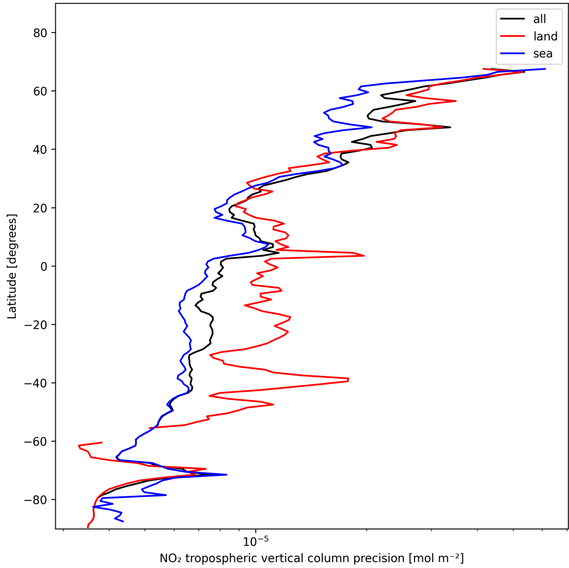
Figure 13: Zonal average of “NO 2 tropospheric vertical column precision” for 2025-11-25 to 2025-11-27.
