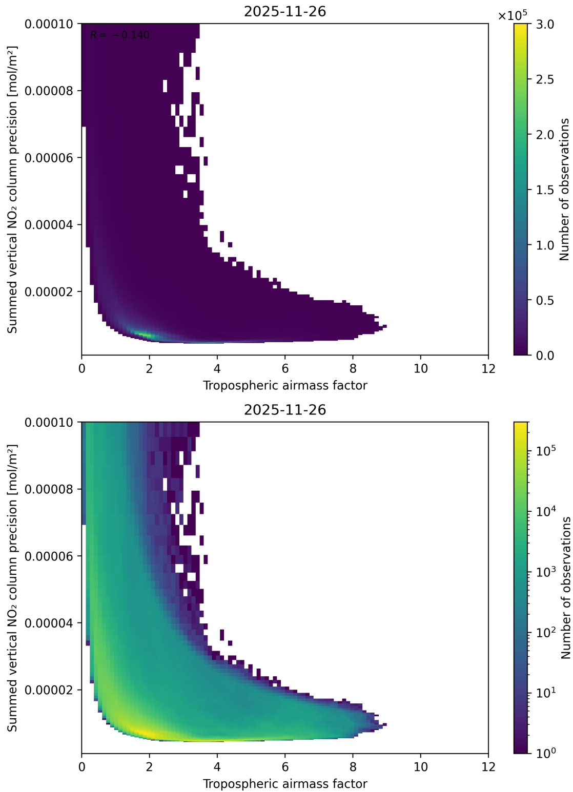
Figure 76: Scatter density plot of “Tropospheric air mass factor” against “Summed vertical NO 2 column precision” for 2025-11-25 to 2025-11-27.
