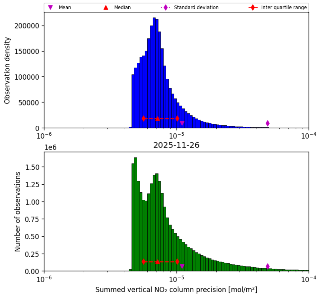
Figure 41: Histogram of “Summed vertical NO 2 column precision” for 2025-11-25 to 2025-11-27
