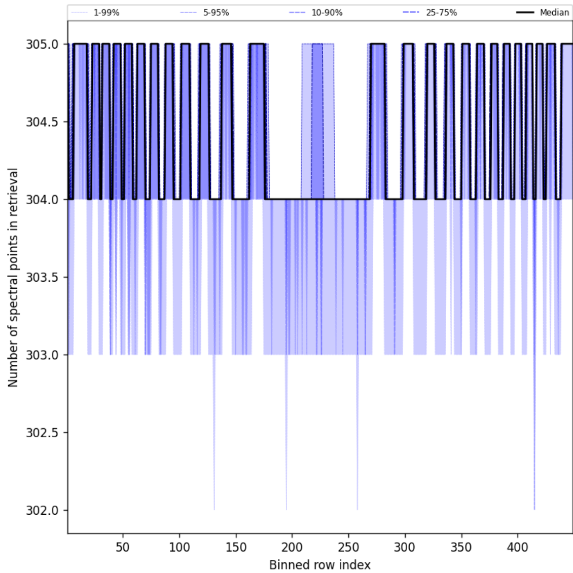
Figure 50: Along track statistics of “Number of spectral points in retrieval” for 2025-11-25 to 2025-11-27
