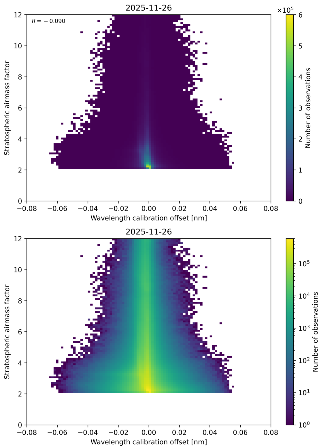
Figure 174: Scatter density plot of “Wavelength calibration offset” against “Stratospheric airmass factor” for 2025-11-25 to 2025-11-27.
