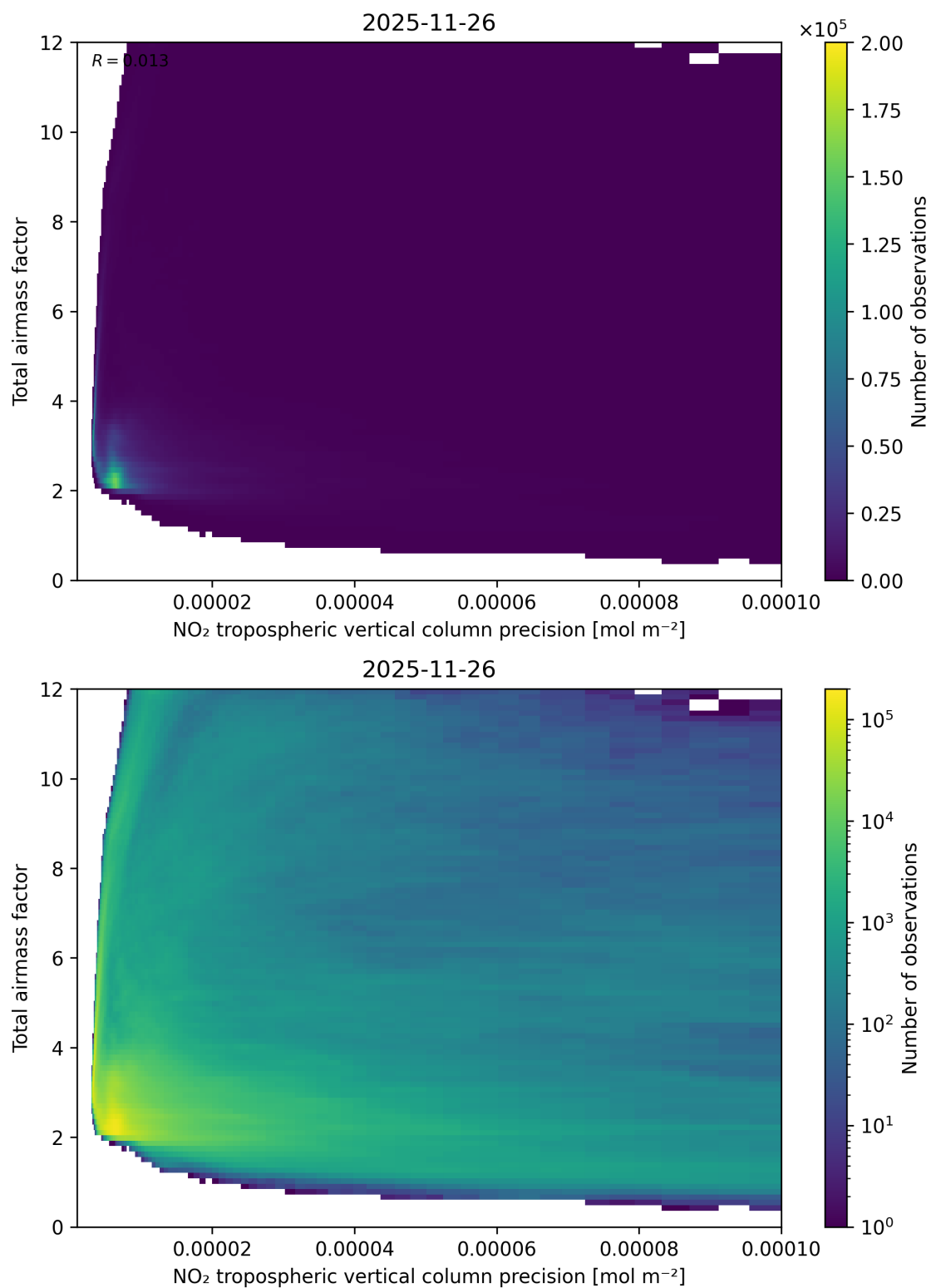
Figure 132: Scatter density plot of “NO 2 tropospheric vertical column precision” against “Total air mass factor” for 2025-11-25 to 2025-11-27.
