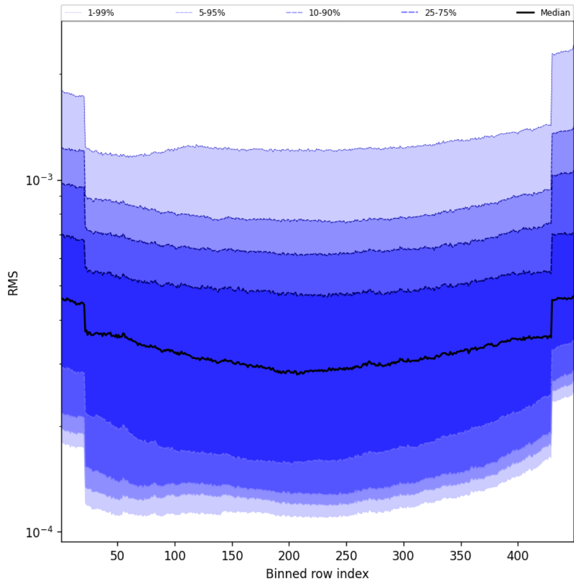
Figure 60: Along track statistics of “RMS” for 2025-11-25 to 2025-11-27
