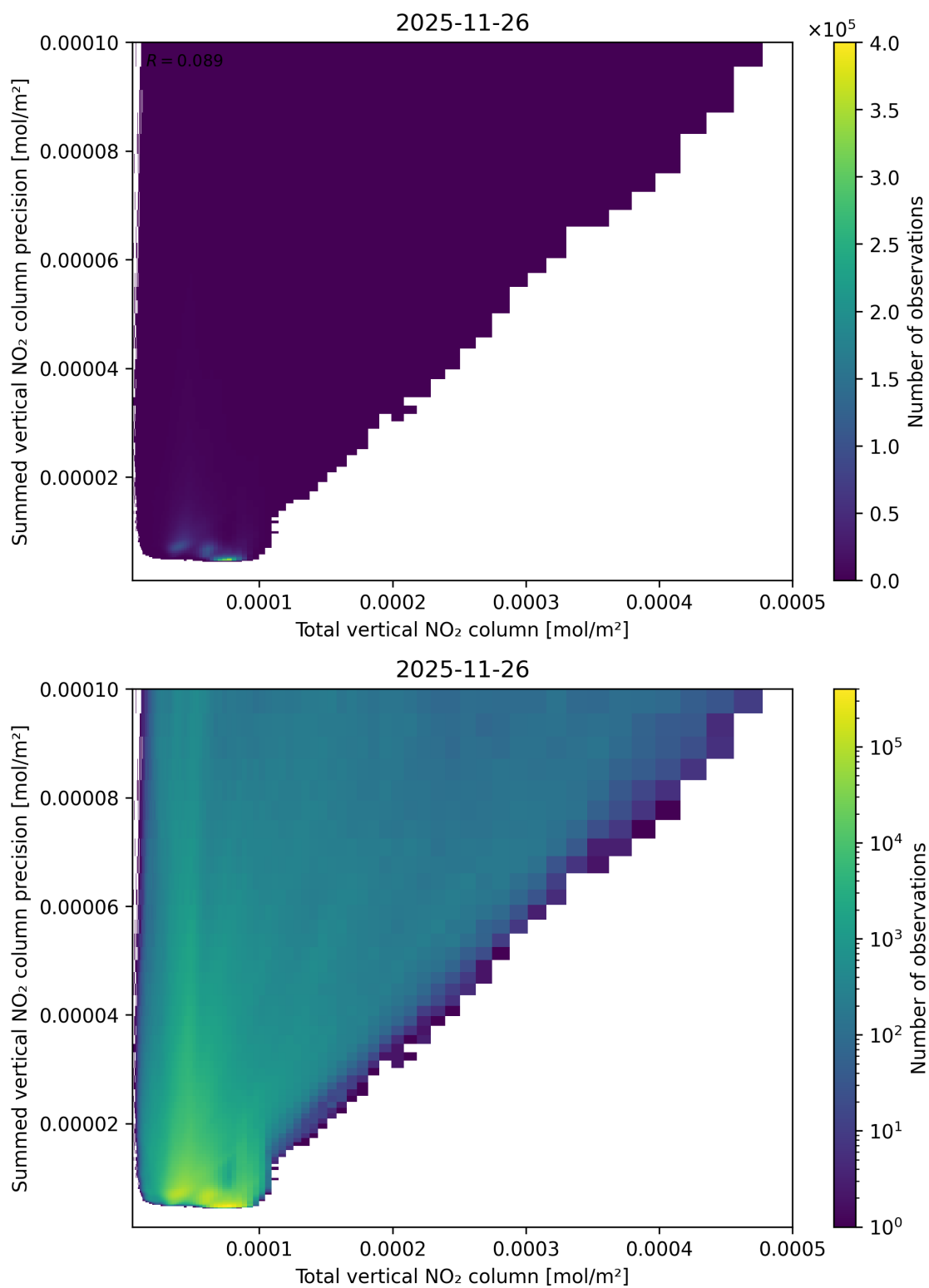
Figure 113: Scatter density plot of “Total vertical NO 2 column” against “Summed vertical NO 2 column precision” for 2025-11-25 to 2025-11-27.
