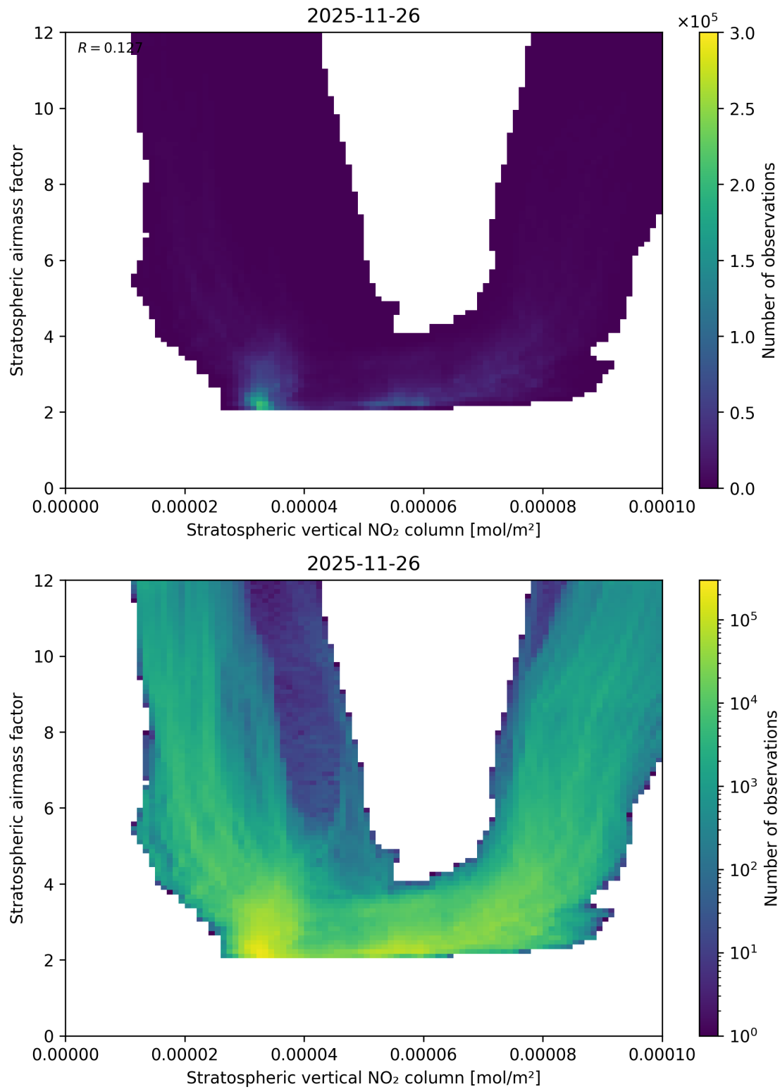
Figure 96: Scatter density plot of “Stratospheric vertical NO 2 column” against “Stratospheric airmass factor” for 2025-11-25 to 2025-11-27.
