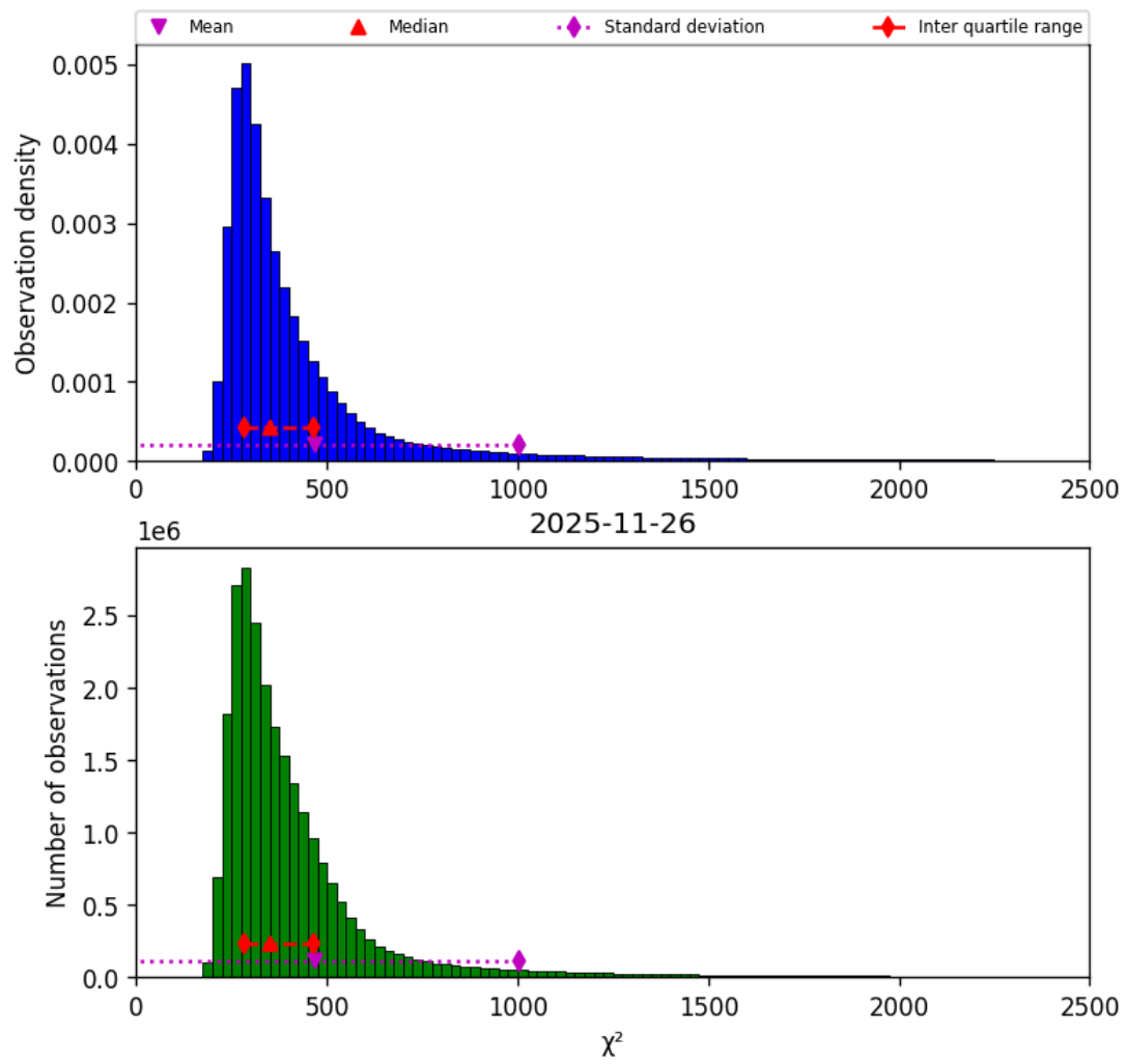
Figure 42: Histogram of “ \chi^2 ” for 2025-11-25 to 2025-11-27
