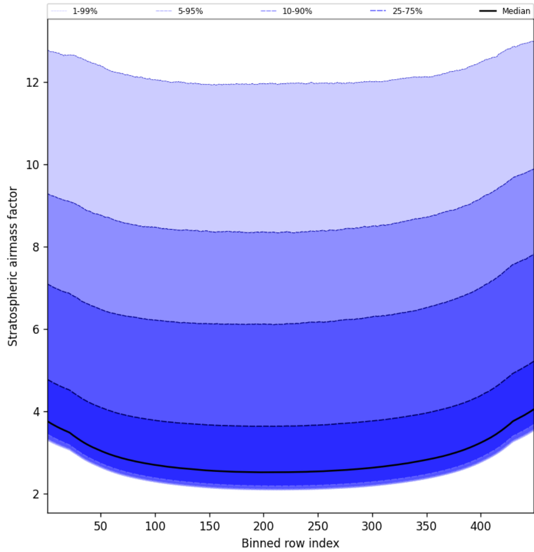
Figure 61: Along track statistics of “Stratospheric air mass factor” for 2025-11-25 to 2025-11-27
