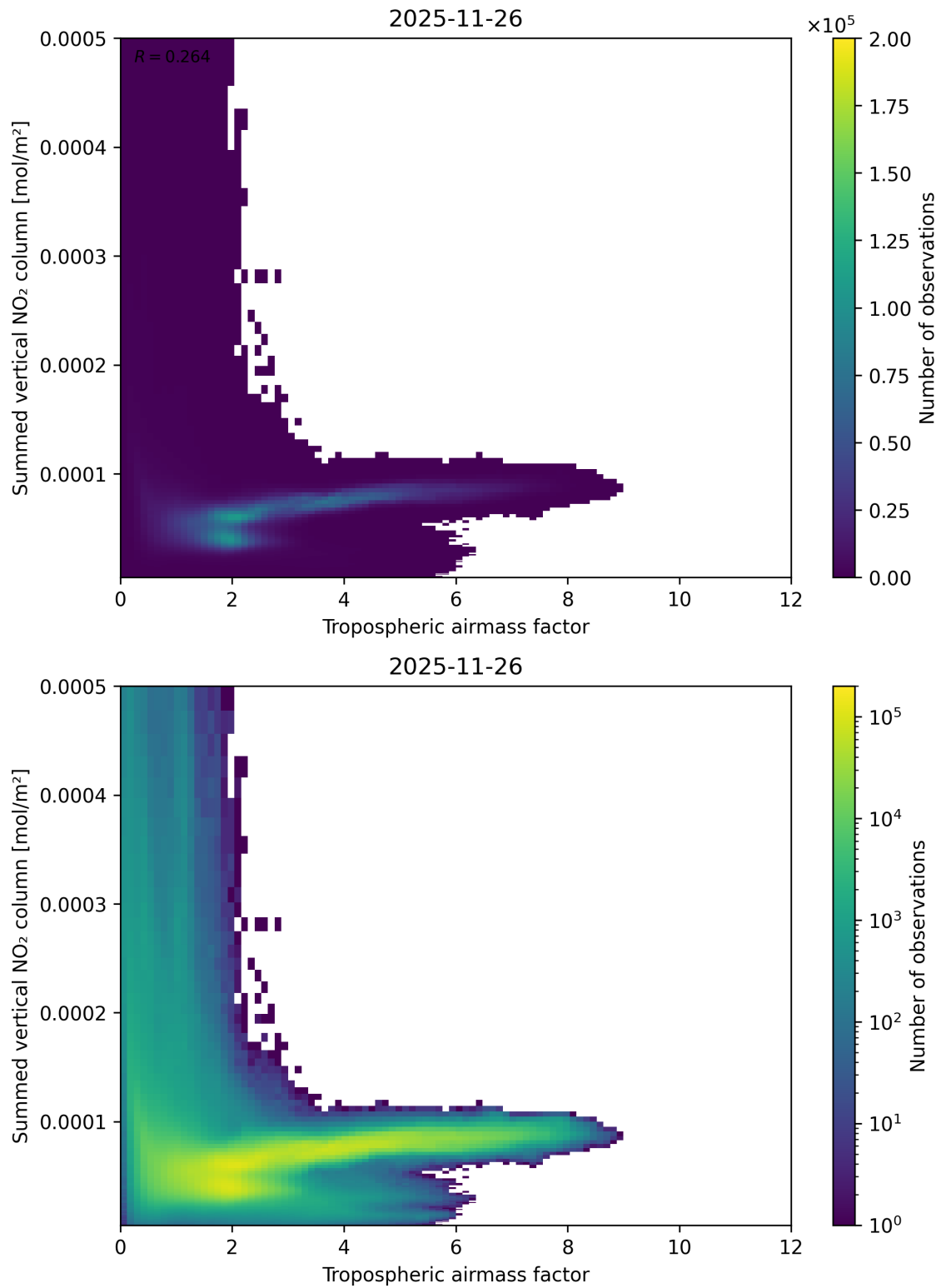
Figure 75: Scatter density plot of “Tropospheric air mass factor” against “Summed vertical NO 2 column” for 2025-11-25 to 2025-11-27.
