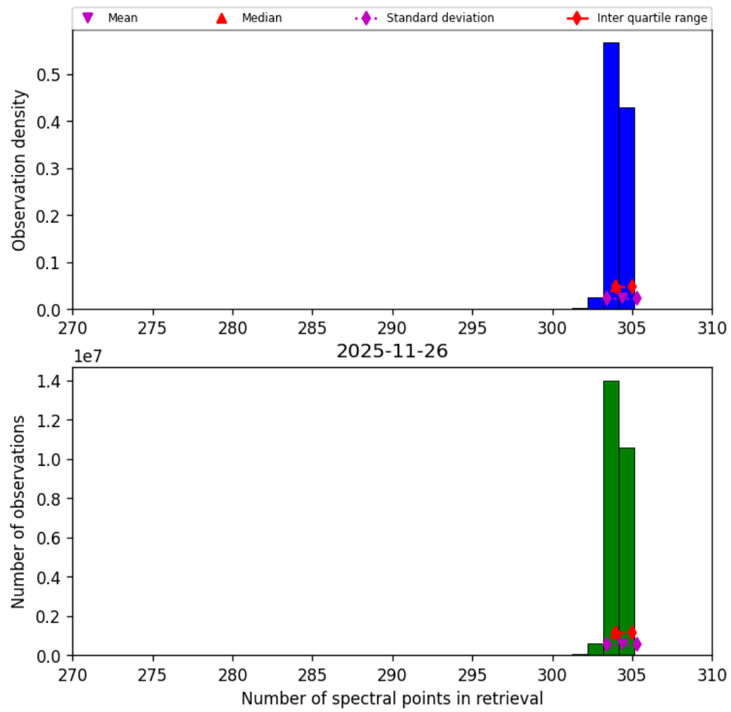
Figure 33: Histogram of “Number of spectral points in retrieval” for 2025-11-25 to 2025-11-27
