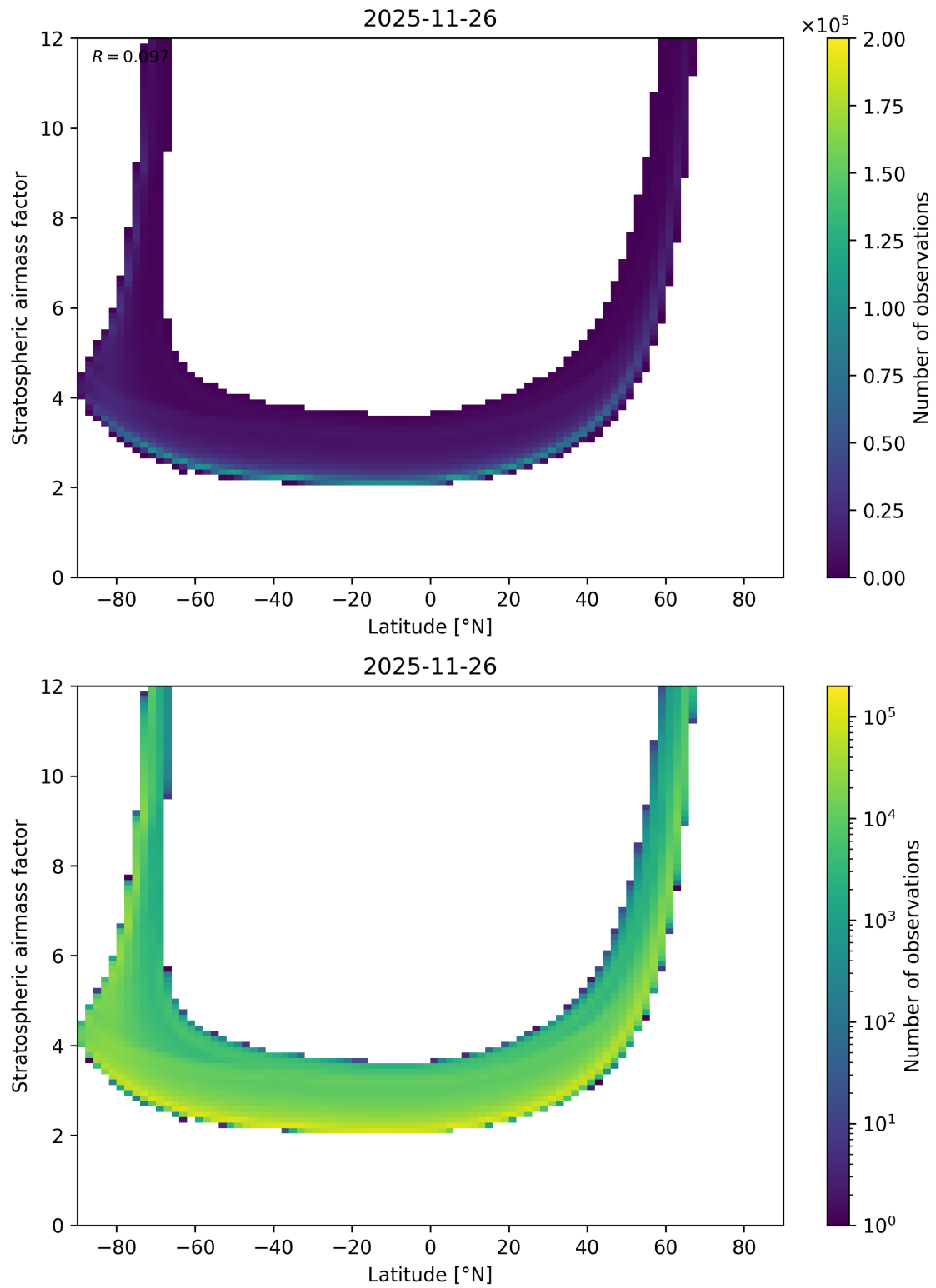
Figure 83: Scatter density plot of “Latitude” against “Stratospheric air mass factor” for 2025-11-25 to 2025-11-27.
