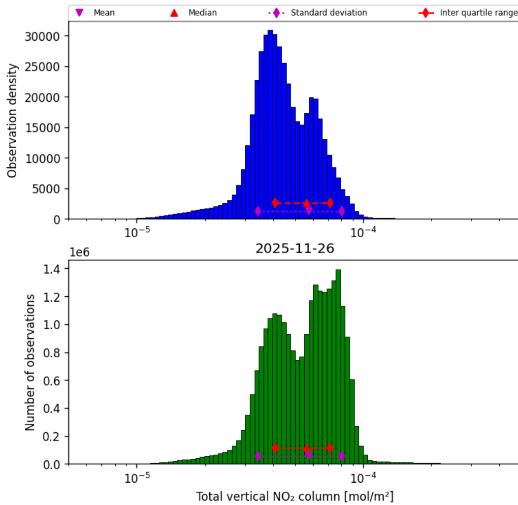
Figure 38: Histogram of “Total vertical NO 2 column” for 2025-11-25 to 2025-11-27
