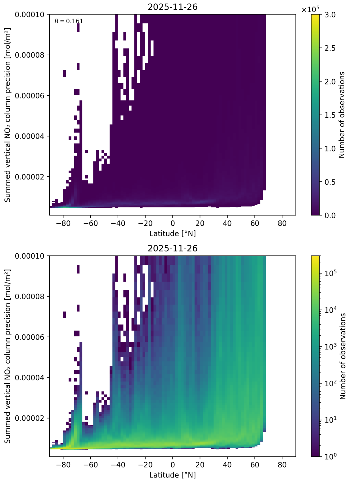
Figure 89: Scatter density plot of “Latitude” against “Summed vertical NO 2 column precision” for 2025-11-25 to 2025-11-27.
