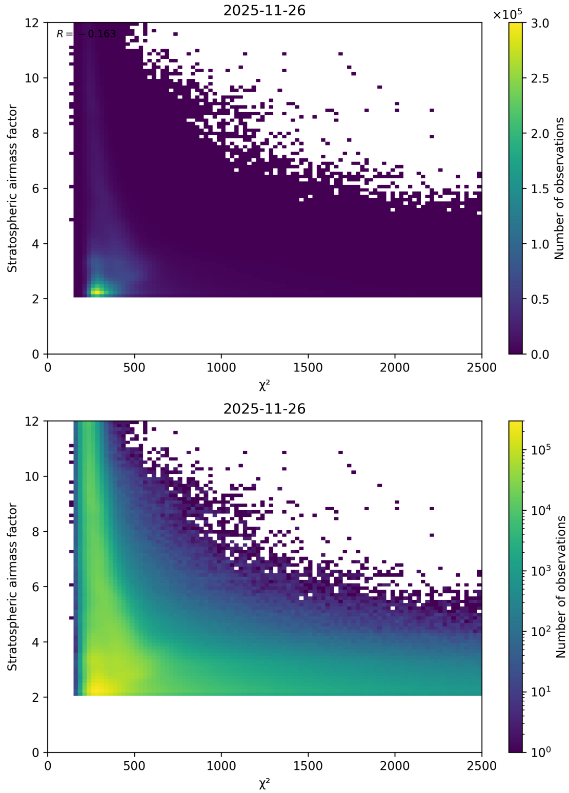
Figure 81: Scatter density plot of “ \chi^2 ” against “Stratospheric airmass factor” for 2025-11-25 to 2025-11-27.
