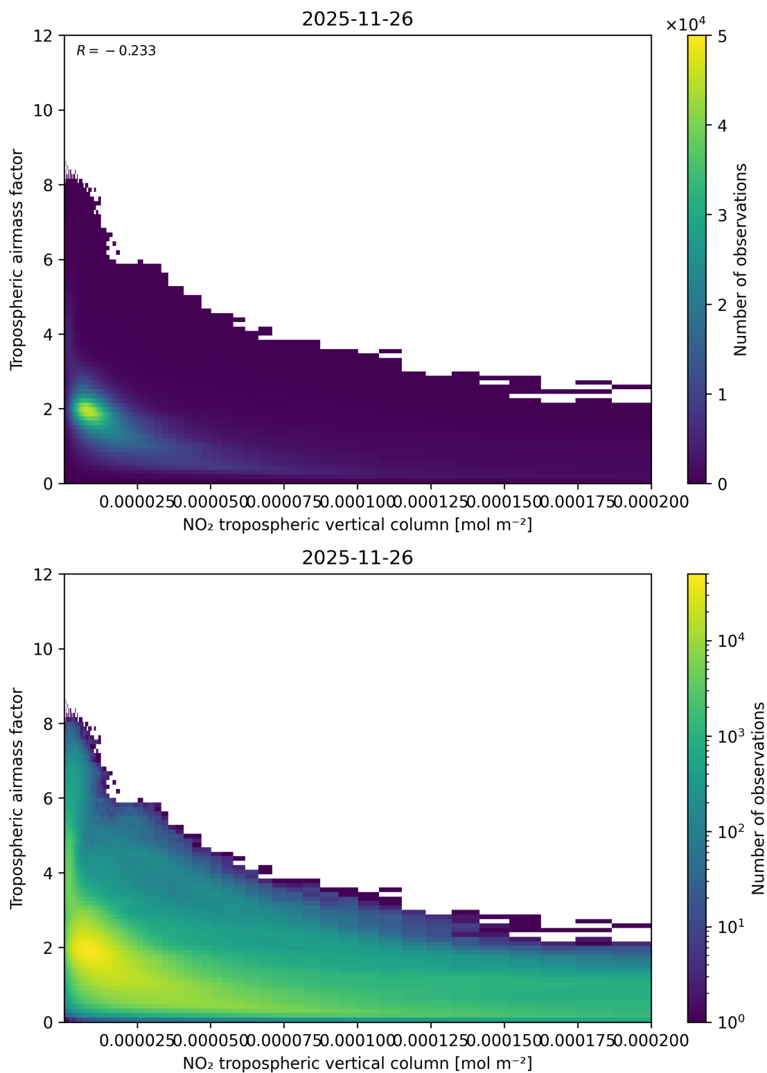
Figure 123: Scatter density plot of “NO 2 tropospheric vertical column” against “Tropospheric air mass factor” for 2025-11-25 to 2025-11-27.
