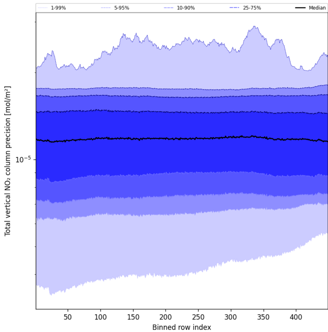
Figure 56: Along track statistics of “Total vertical NO 2 column precision” for 2025-11-25 to 2025-11-27
