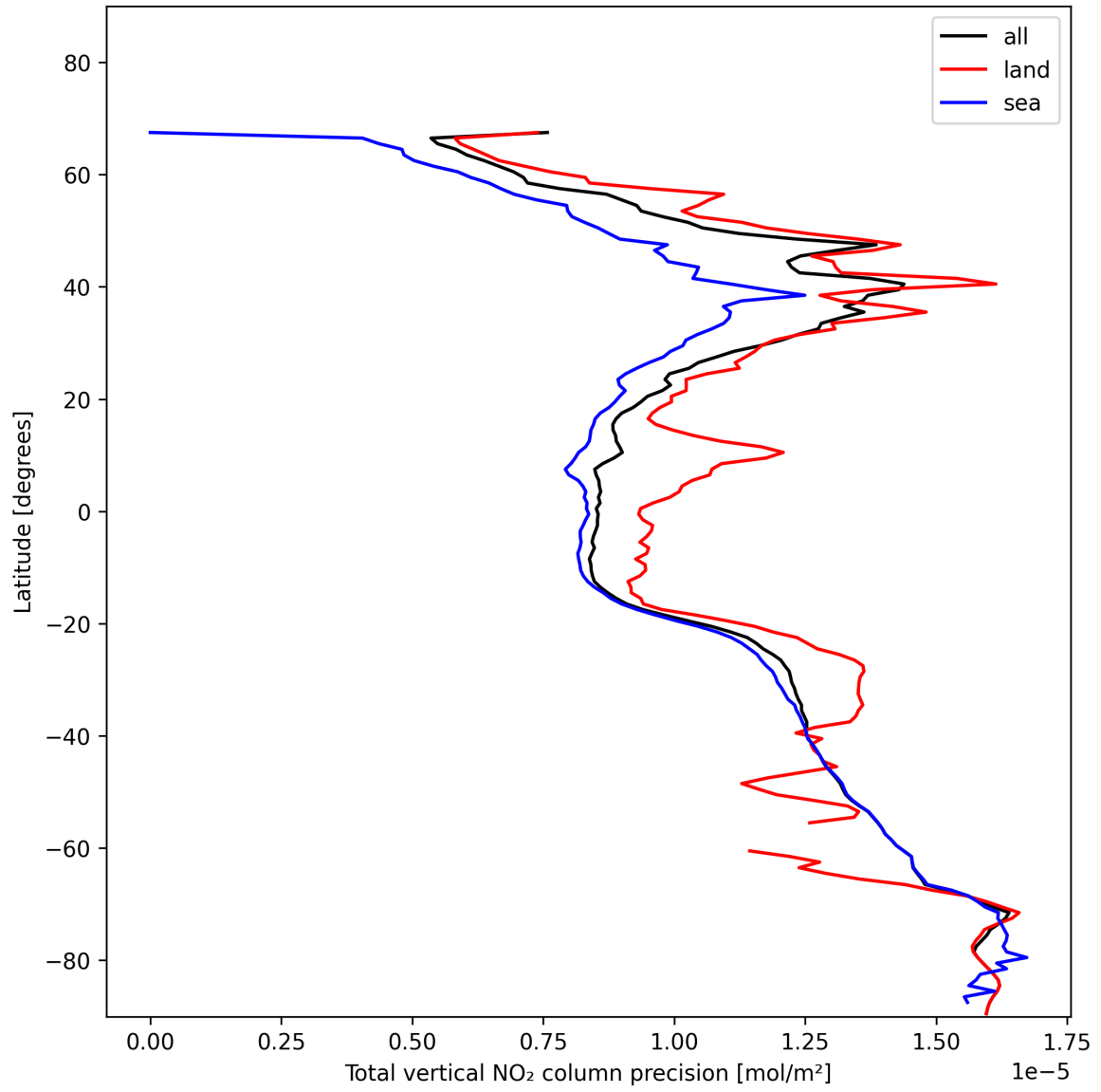
Figure 22: Zonal average of “Total vertical NO 2 column precision” for 2025-11-25 to 2025-11-27.
