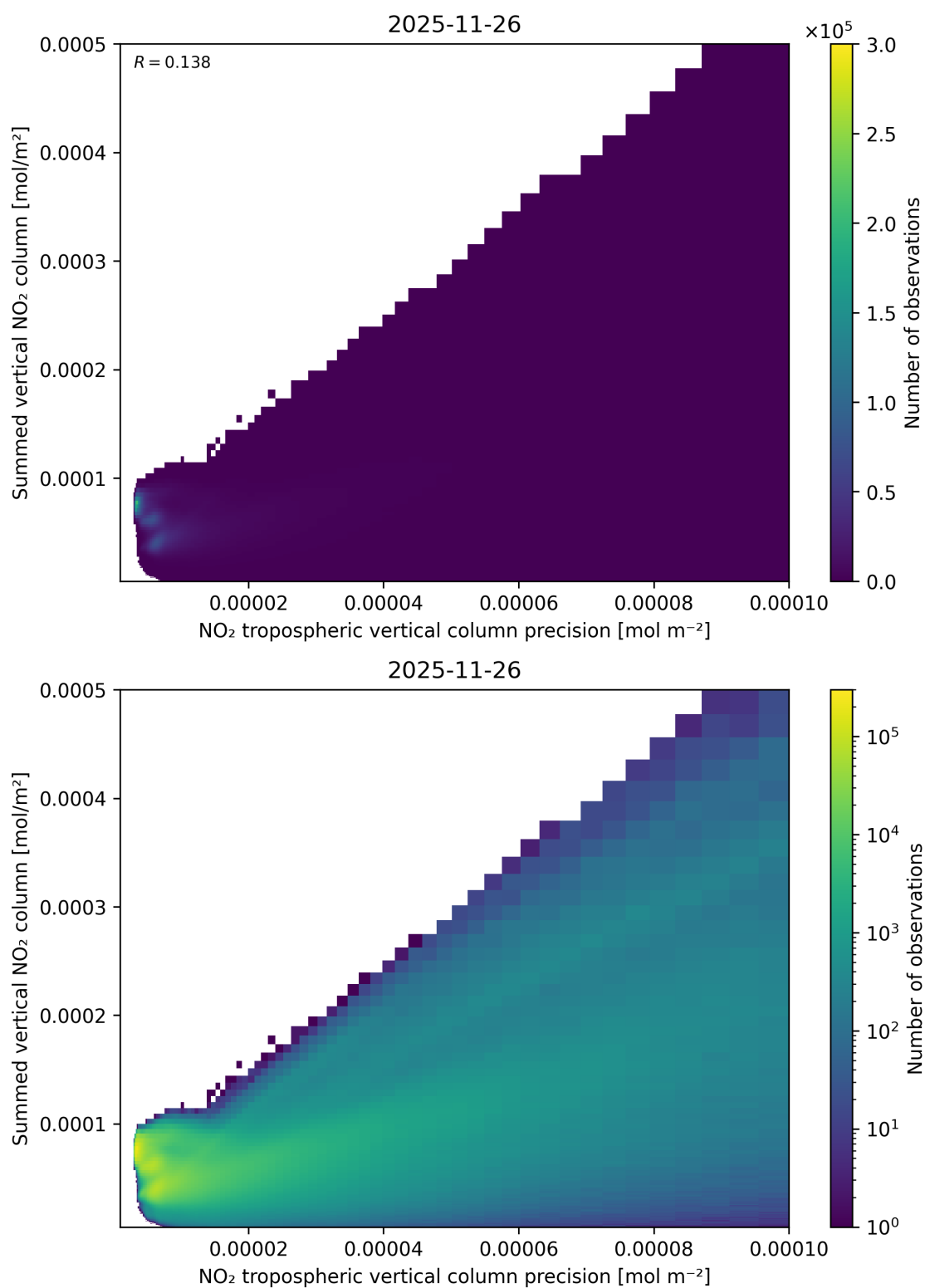
Figure 136: Scatter density plot of “NO 2 tropospheric vertical column precision” against “Summed vertical NO 2 column” for 2025-11-25 to 2025-11-27.
