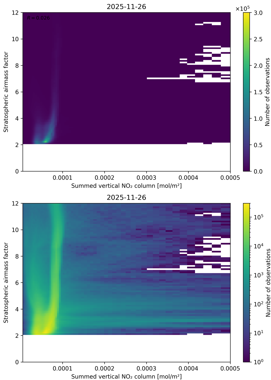
Figure 103: Scatter density plot of “Summed vertical NO 2 column” against “Stratospheric airmass factor” for 2025-11-25 to 2025-11-27.
