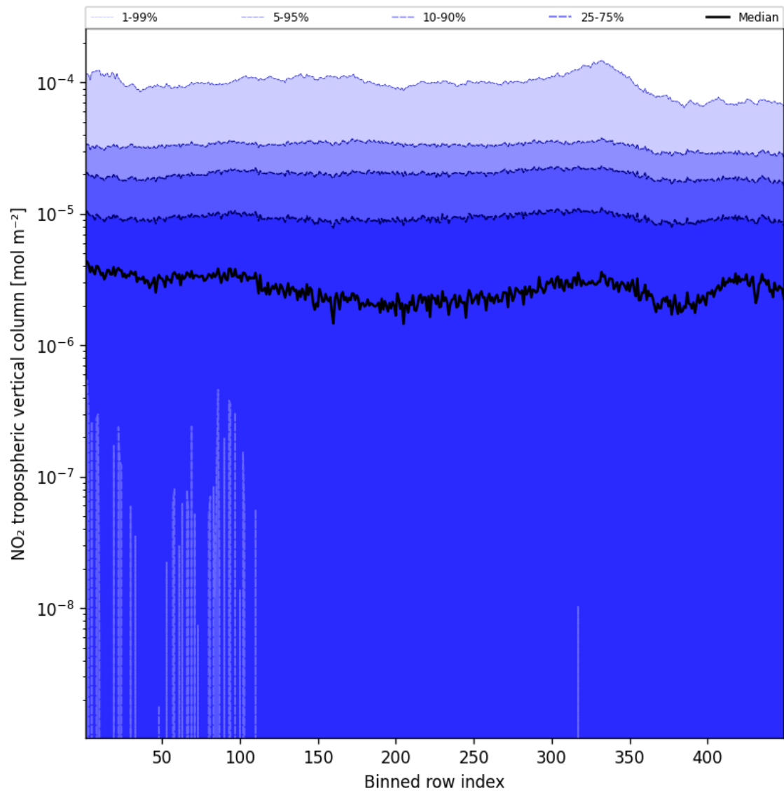
Figure 46: Along track statistics of “NO 2 tropospheric vertical column” for 2025-11-25 to 2025-11-27
