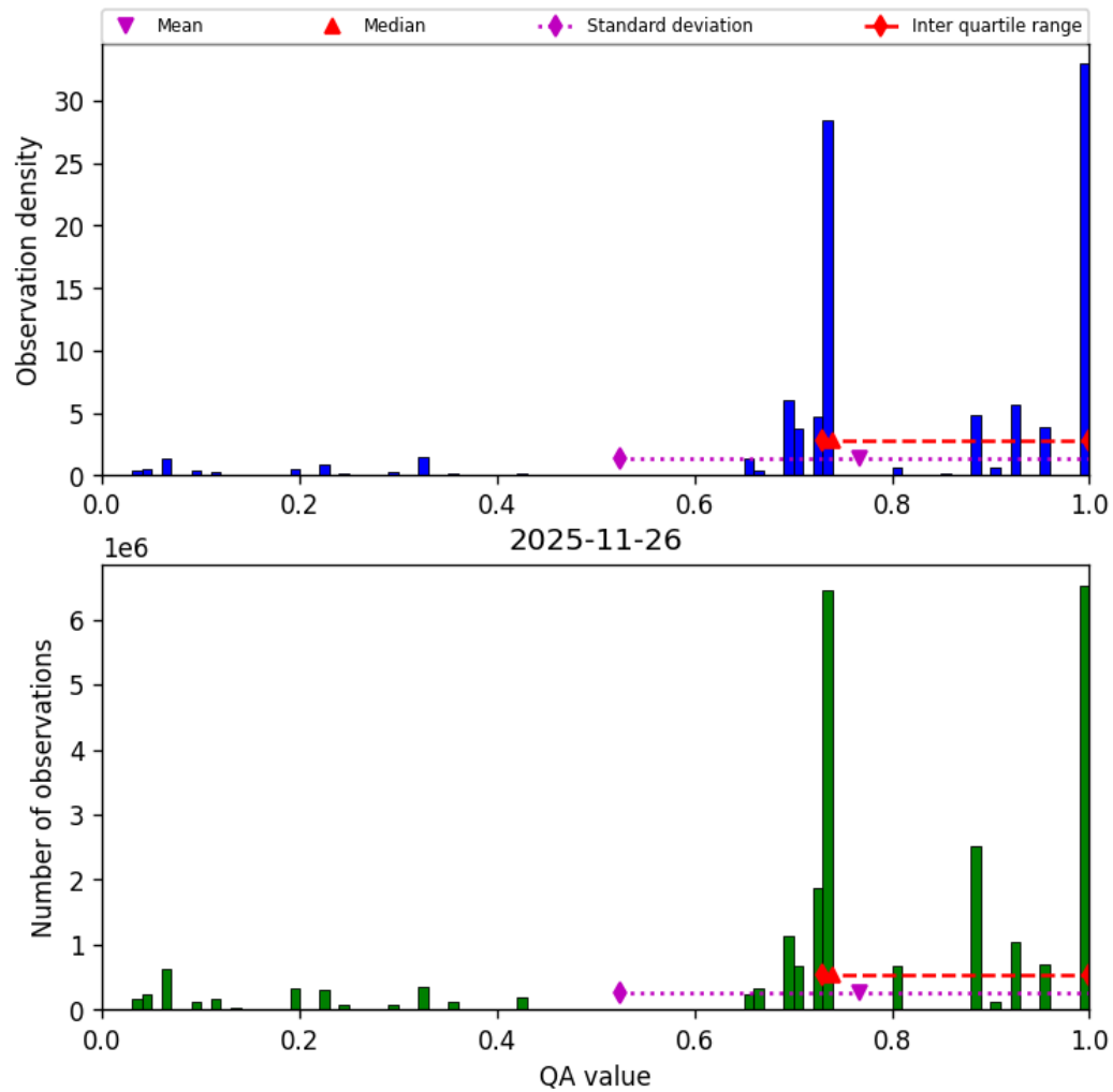
Figure 28: Histogram of “QA value” for 2025-11-25 to 2025-11-27
