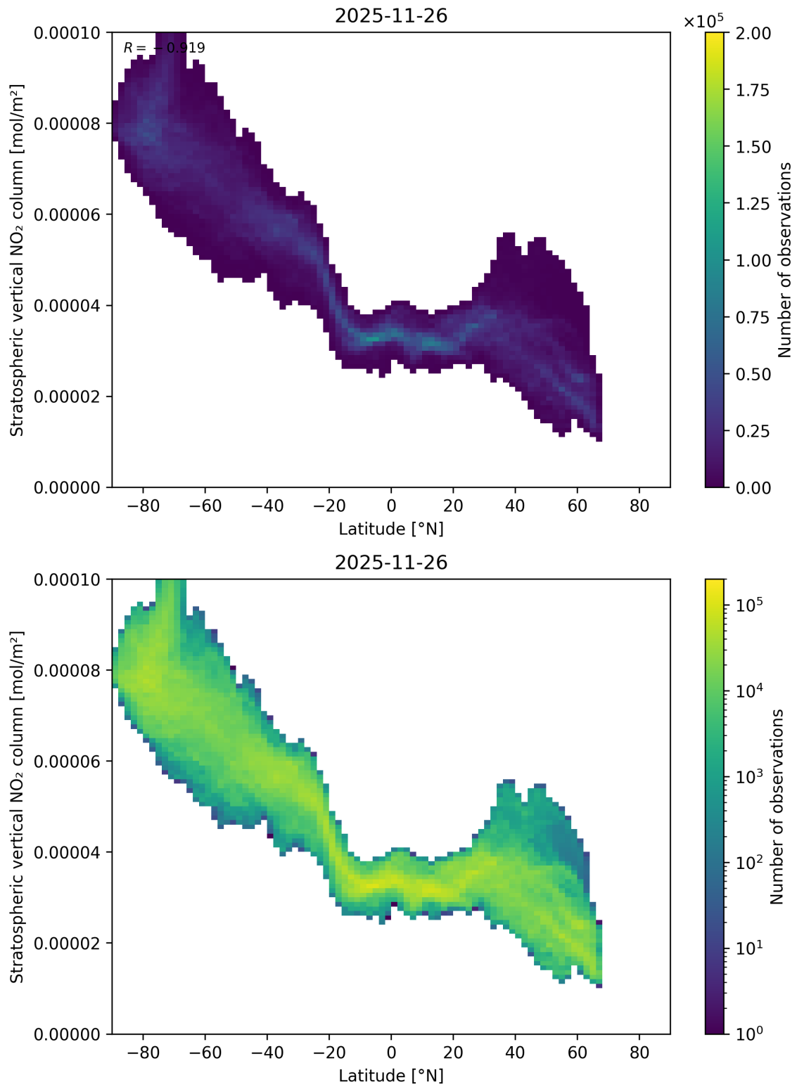
Figure 87: Scatter density plot of “Latitude” against “Stratospheric vertical NO 2 column” for 2025-11-25 to 2025-11-27.
