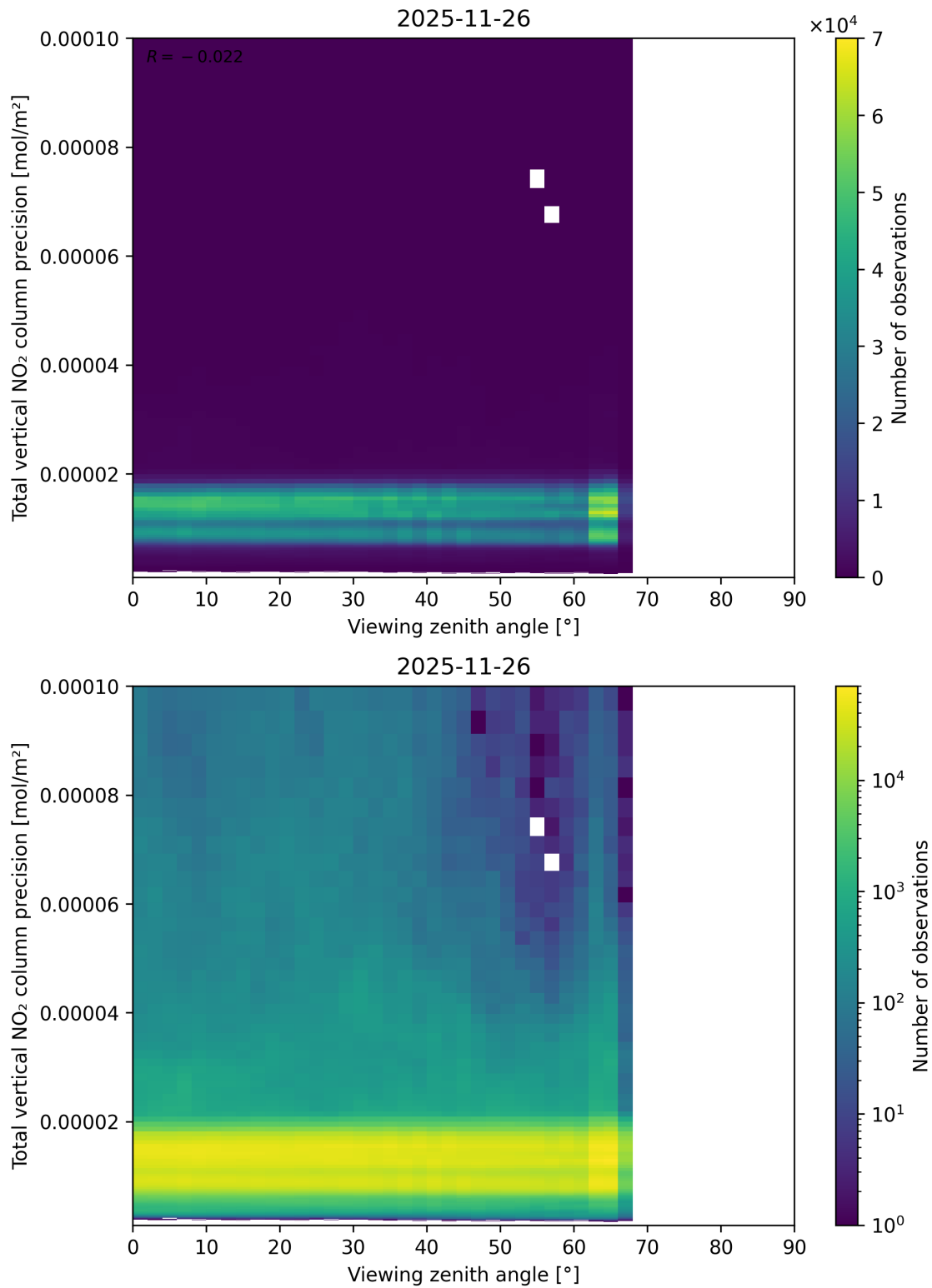
Figure 168: Scatter density plot of “Viewing zenith angle” against “Total vertical NO 2 column precision” for 2025-11-25 to 2025-11-27.
