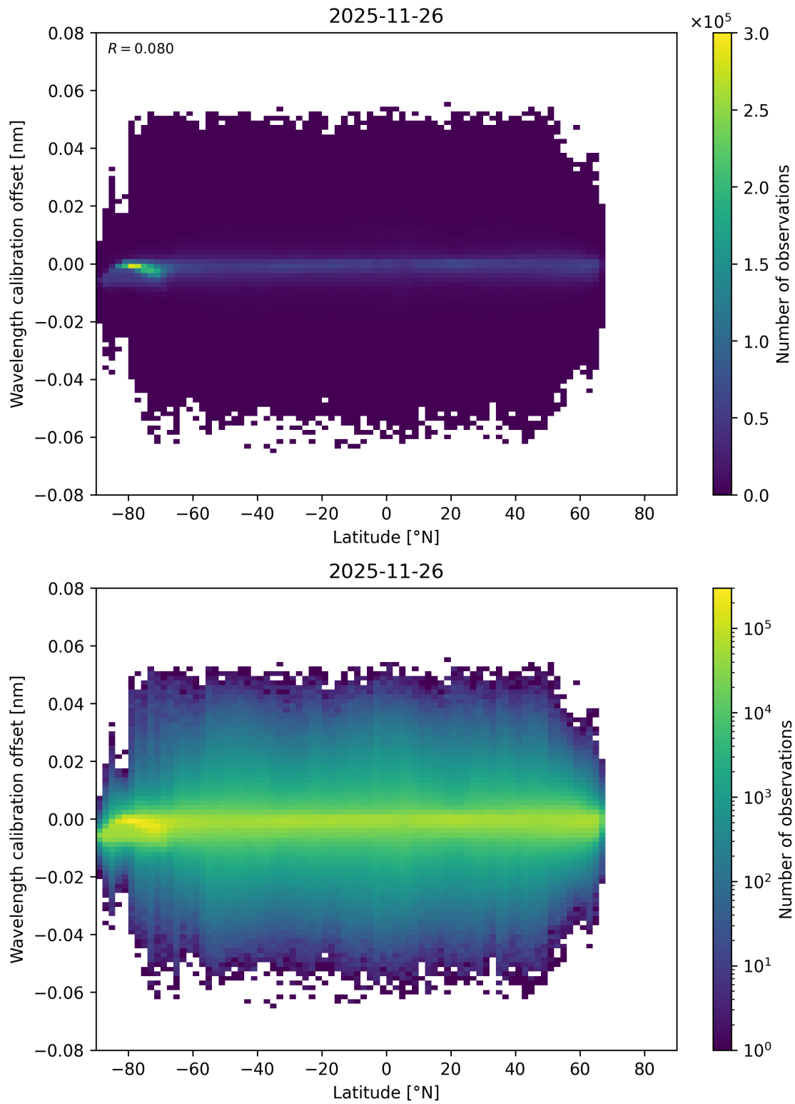
Figure 95: Scatter density plot of “Latitude” against “Wavelength calibration offset” for 2025-11-25 to 2025-11-27.
