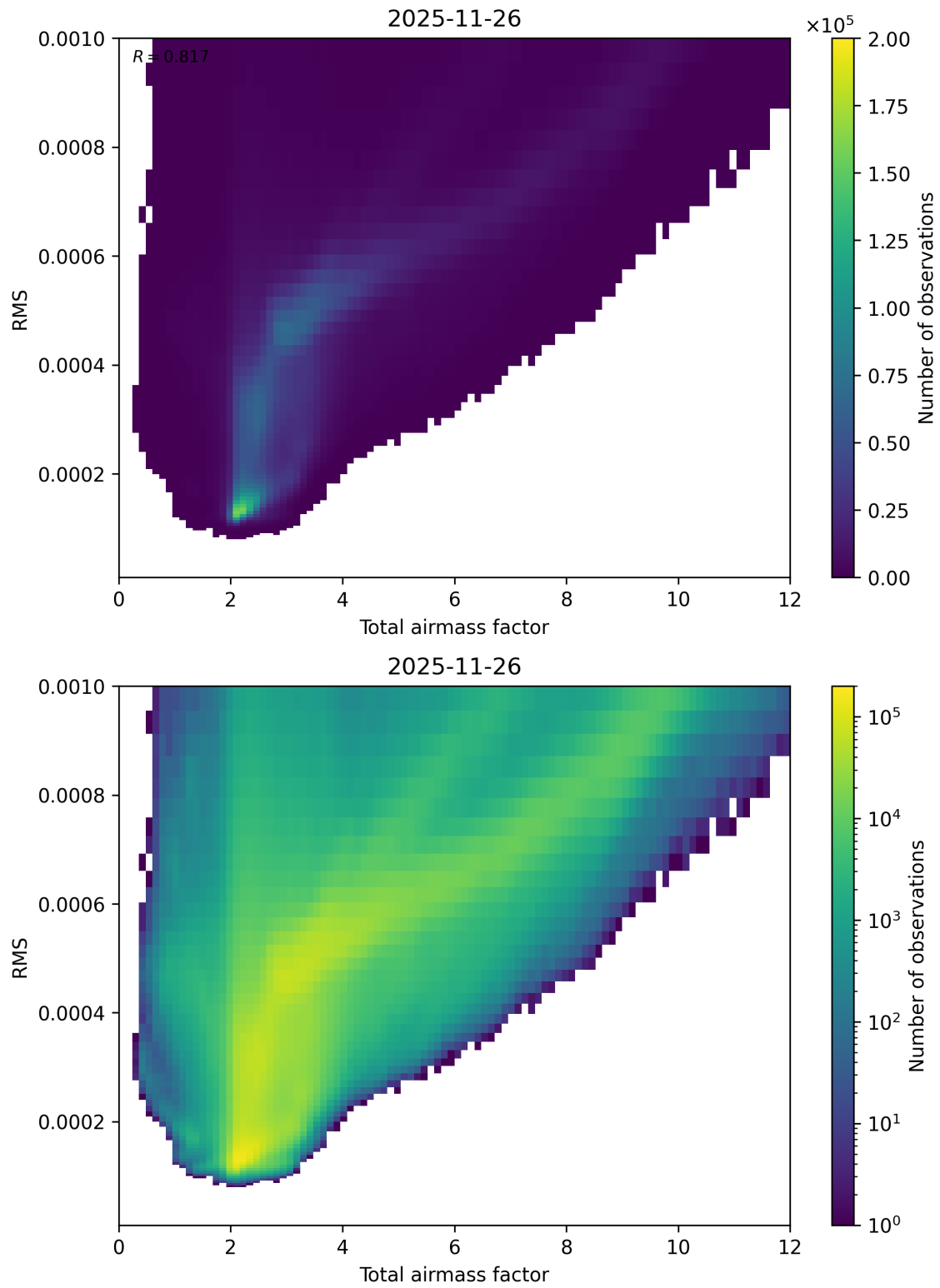
Figure 69: Scatter density plot of “Total airmass factor” against “RMS” for 2025-11-25 to 2025-11-27.
