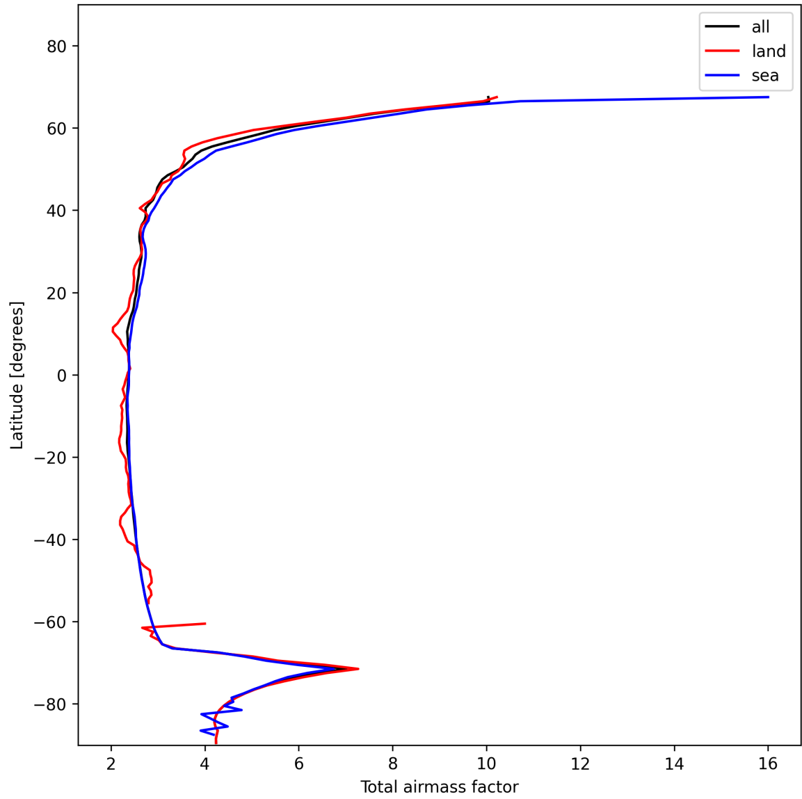
Figure 15: Zonal average of “Total airmass factor” for 2025-11-25 to 2025-11-27.
