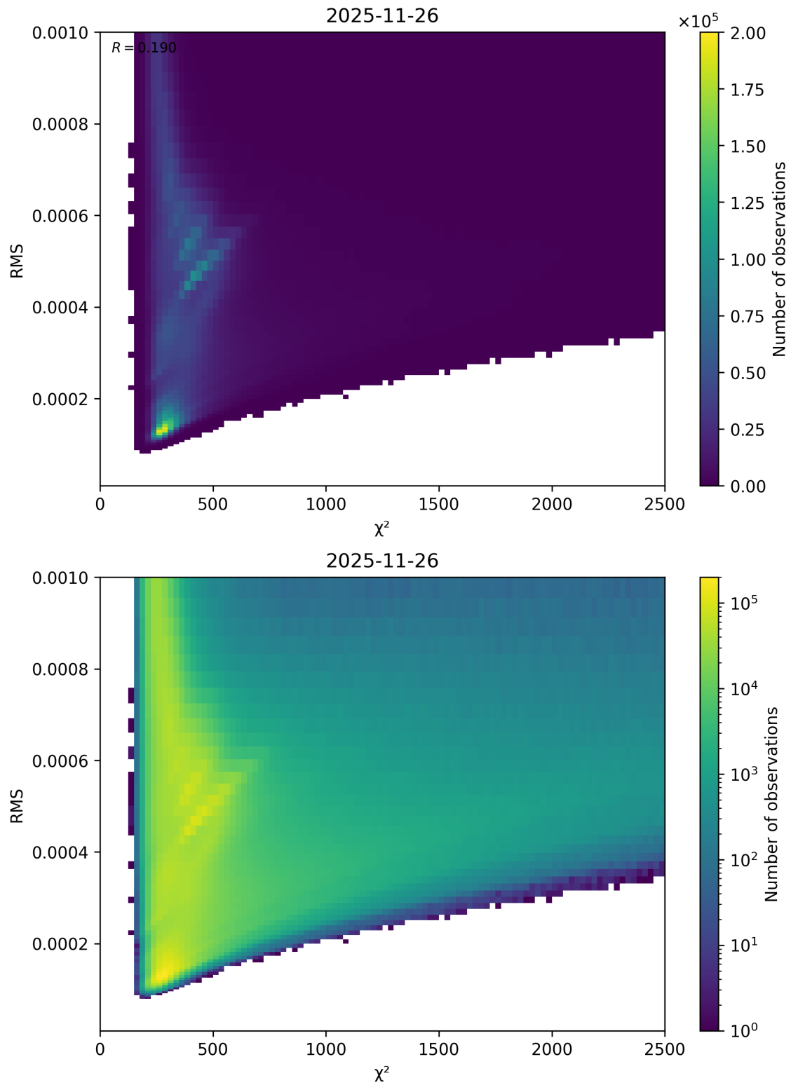
Figure 82: Scatter density plot of “ \chi^2 ” against “RMS” for 2025-11-25 to 2025-11-27.
