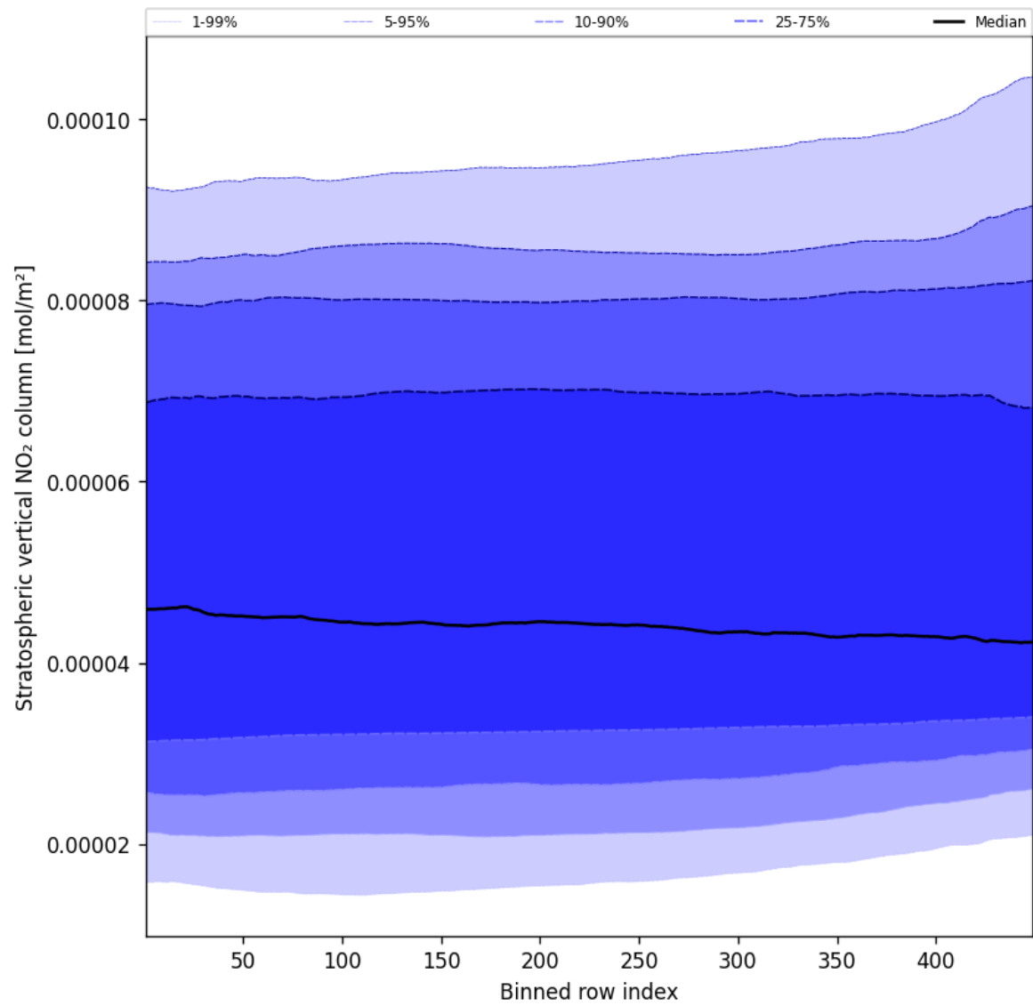
Figure 53: Along track statistics of “Stratospheric vertical NO 2 column” for 2025-11-25 to 2025-11-27
