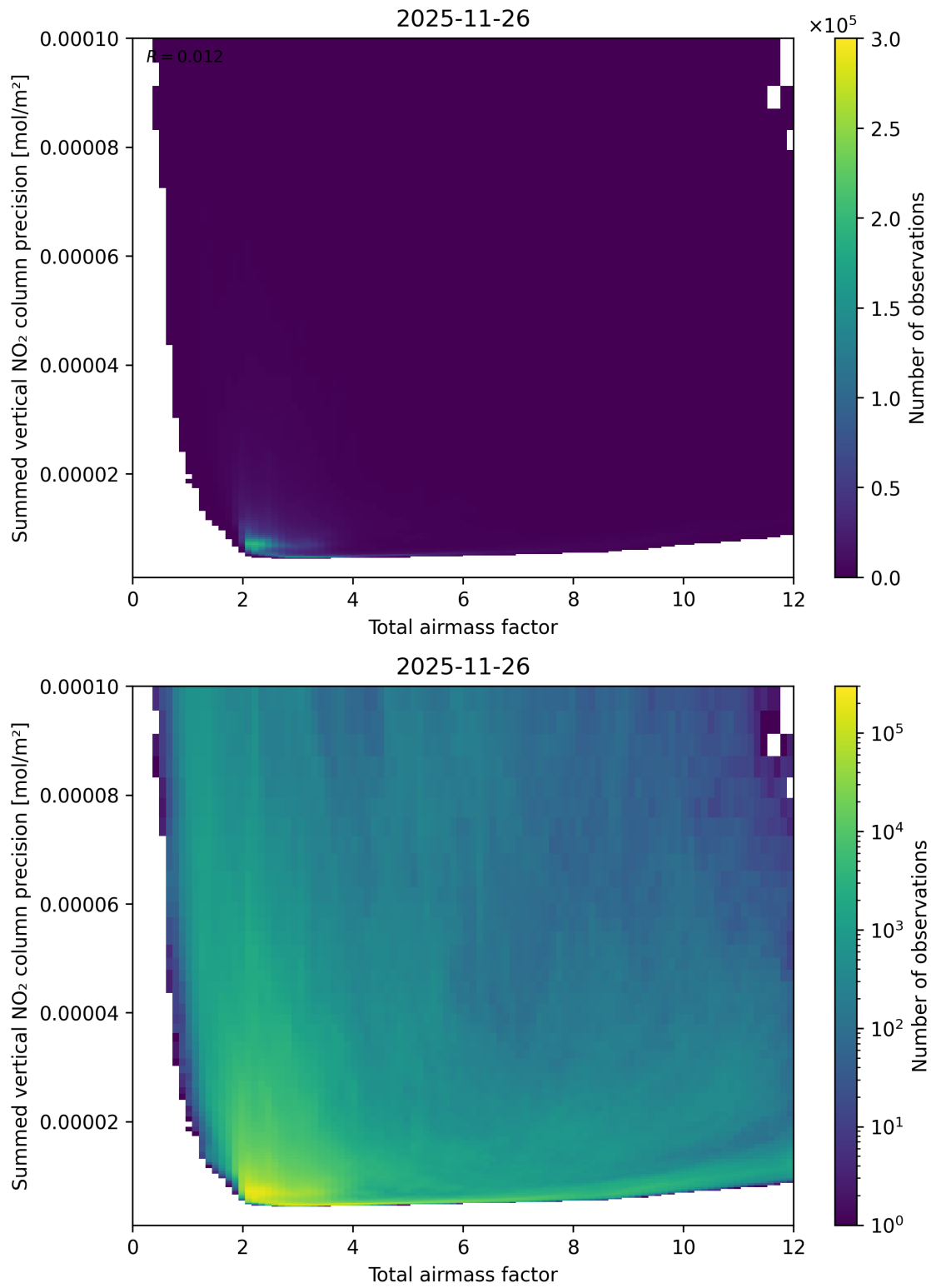
Figure 66: Scatter density plot of “Total airmass factor” against “Summed vertical NO 2 column precision” for 2025-11-25 to 2025-11-27.
