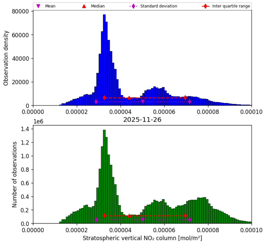
Figure 36: Histogram of “Stratospheric vertical NO 2 column” for 2025-11-25 to 2025-11-27
