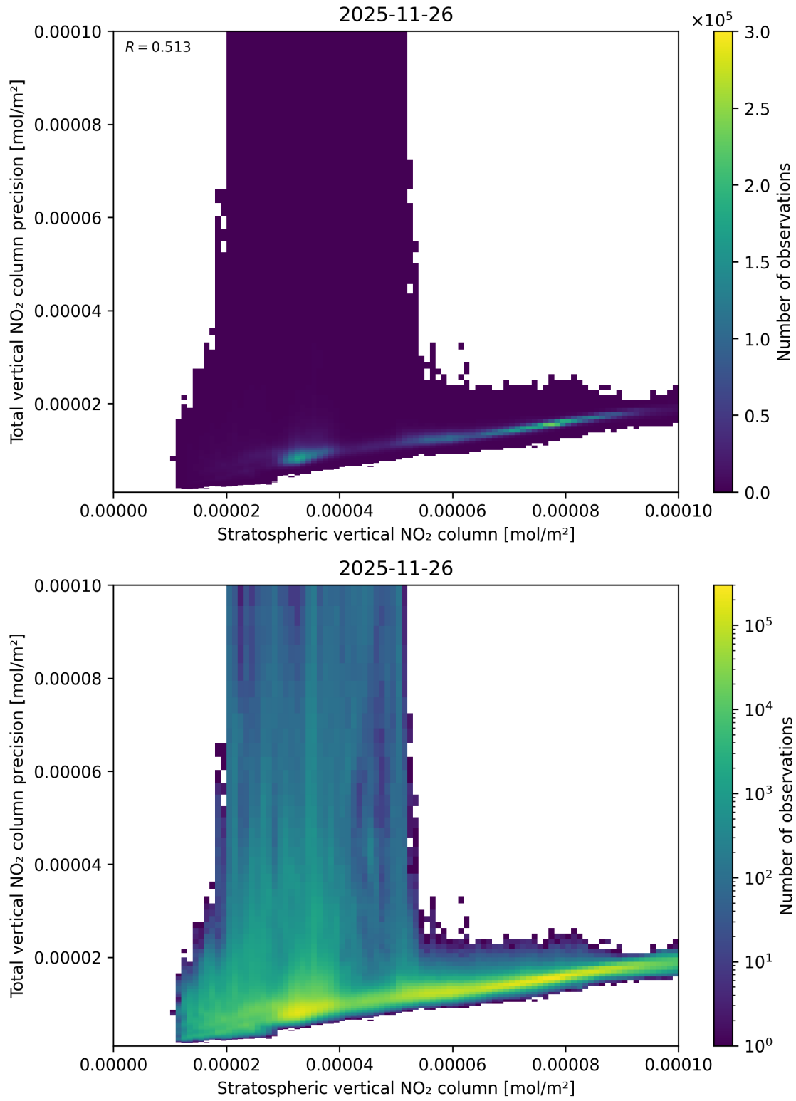
Figure 101: Scatter density plot of “Stratospheric vertical NO 2 column” against “Total vertical NO 2 column precision” for 2025-11-25 to 2025-11-27.
