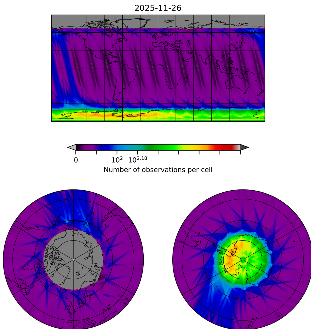
Figure 10: Map of the number of observations for 2025-11-25 to 2025-11-27
