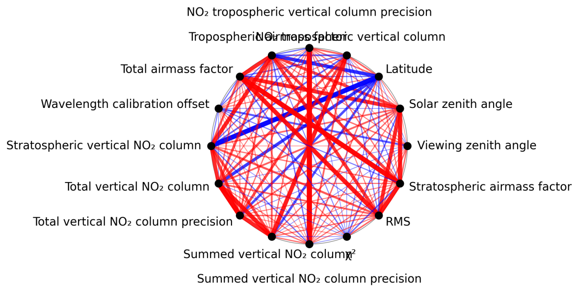
Figure 1: Map of correlation graph for 2025-11-25 to 2025-11-27.
