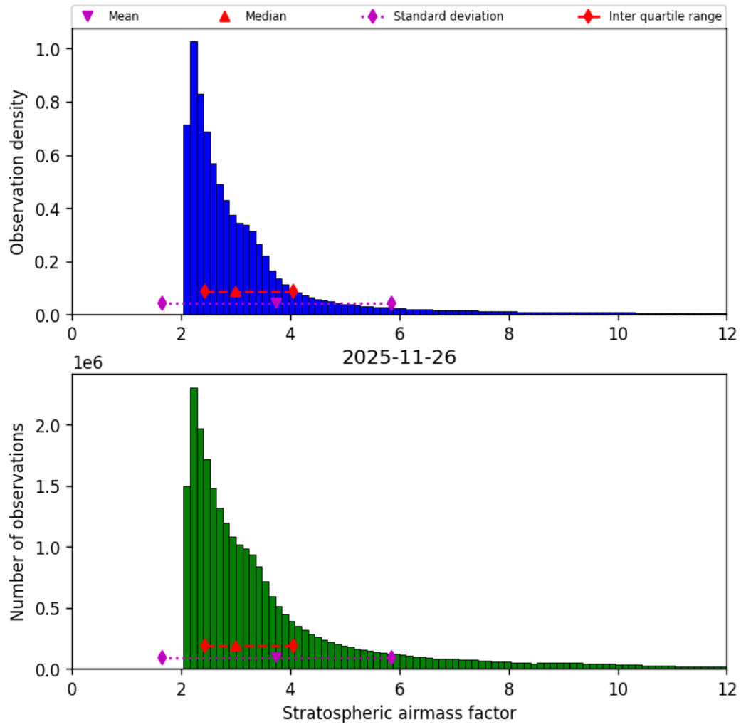
Figure 44: Histogram of “Stratospheric airmass factor” for 2025-11-25 to 2025-11-27
