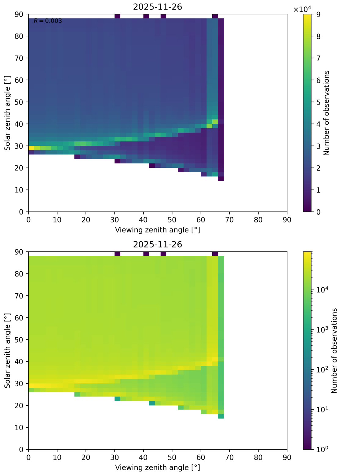
Figure 172: Scatter density plot of “Viewing zenith angle” against “Solar zenith angle” for 2025-11-25 to 2025-11-27.
