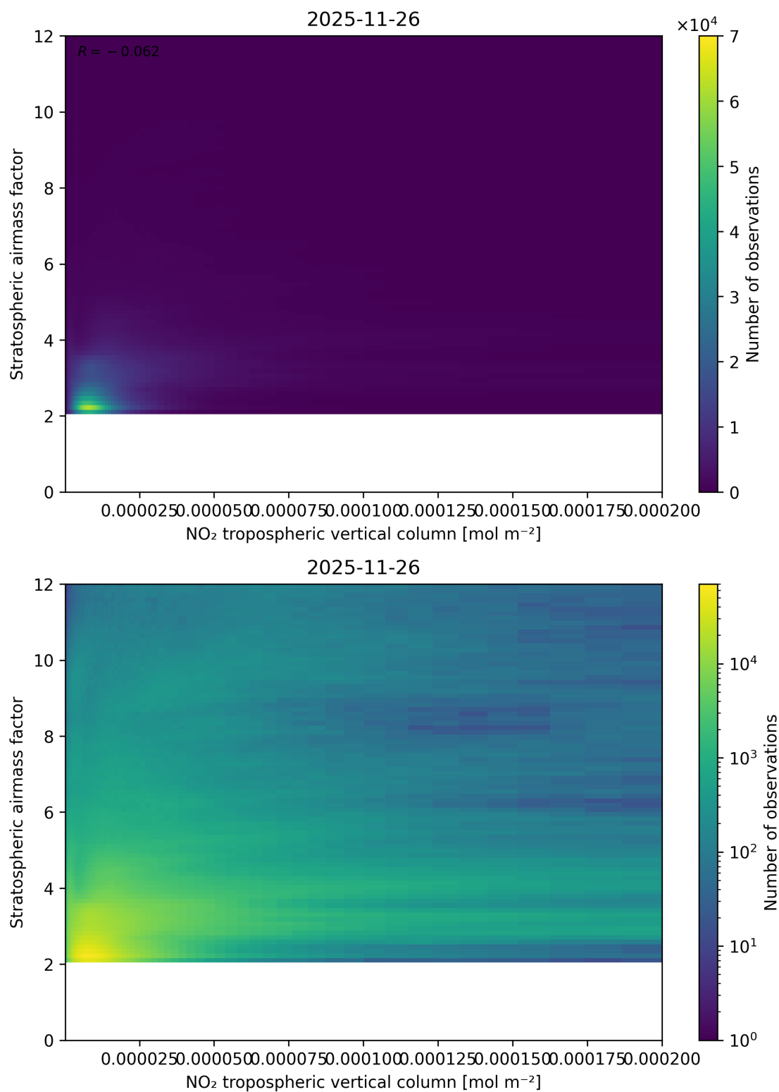
Figure 121: Scatter density plot of “NO 2 tropospheric vertical column” against “Stratospheric airmass factor” for 2025-11-25 to 2025-11-27.
