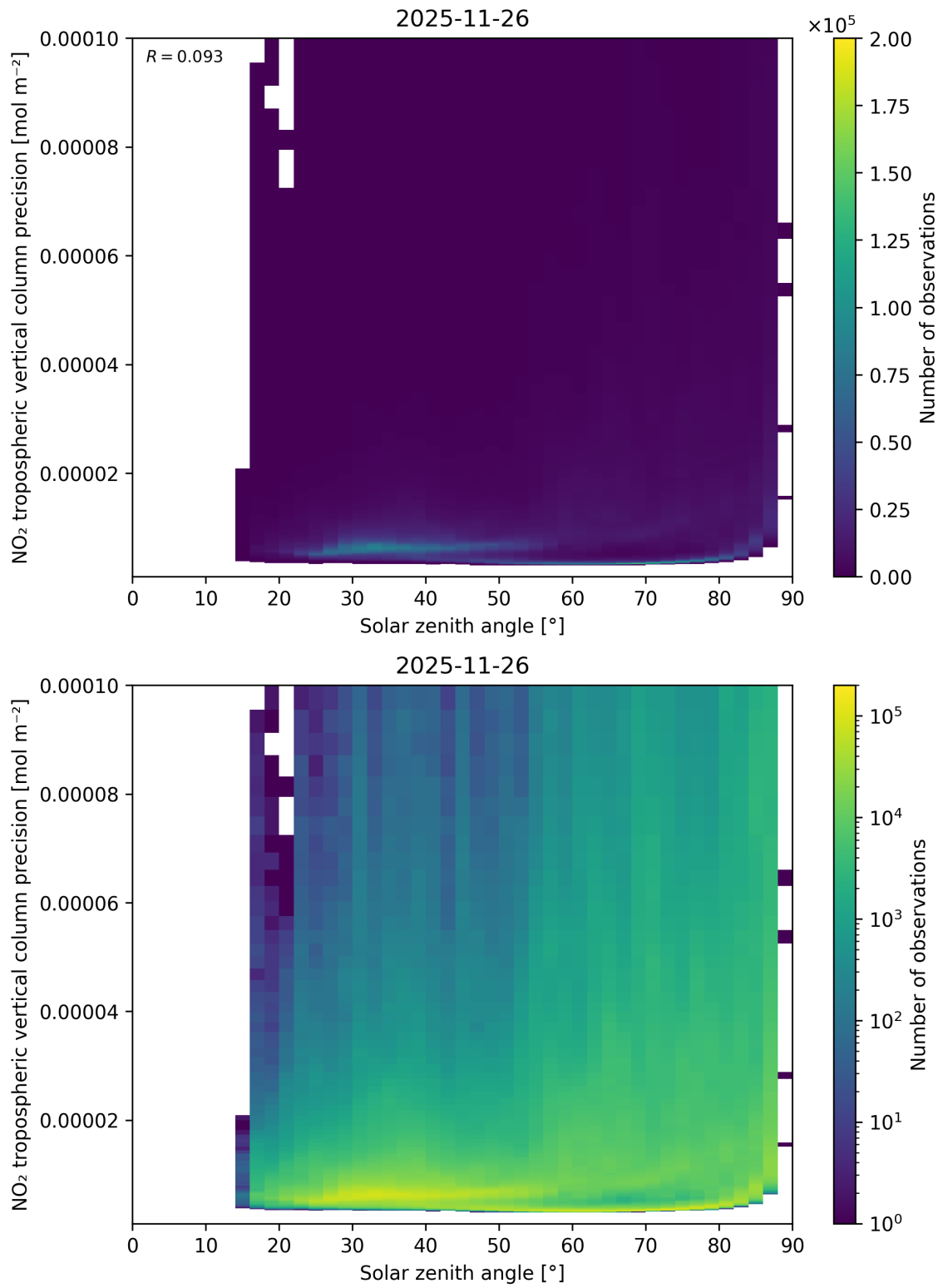
Figure 156: Scatter density plot of “Solar zenith angle” against “NO 2 tropospheric vertical column precision” for 2025-11-25 to 2025-11-27.
