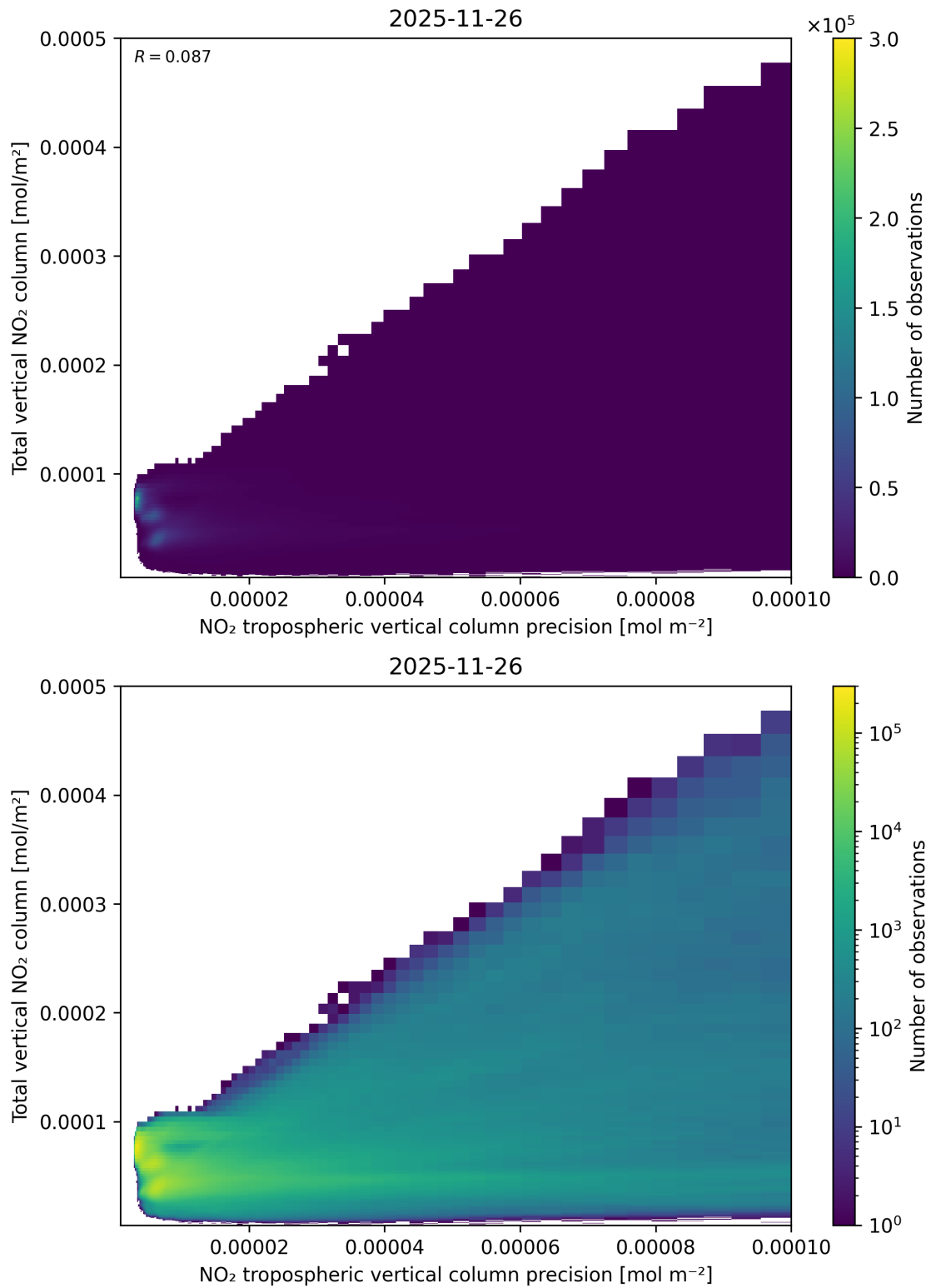
Figure 138: Scatter density plot of “NO 2 tropospheric vertical column precision” against “Total vertical NO 2 column” for 2025-11-25 to 2025-11-27.
