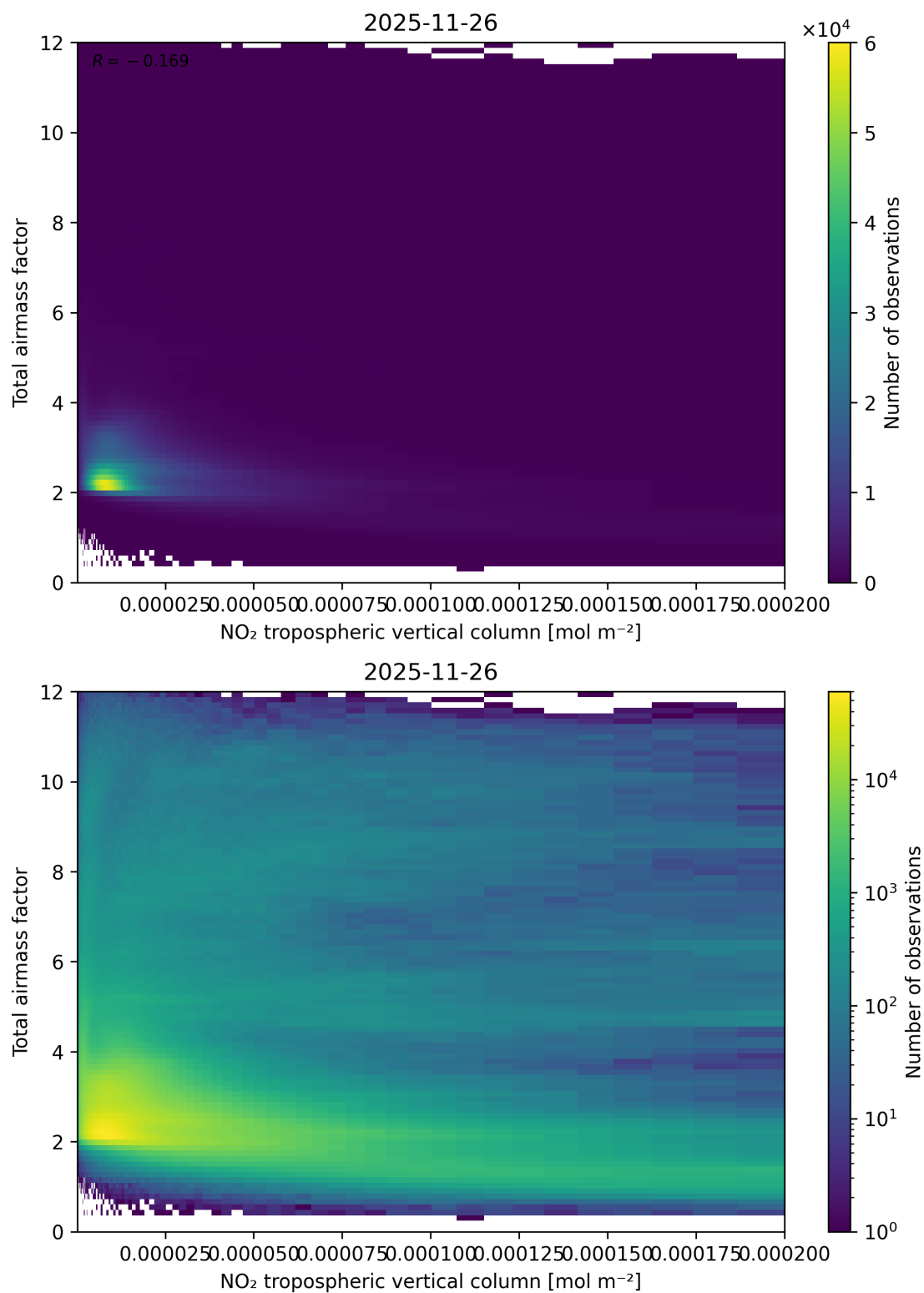
Figure 122: Scatter density plot of “NO 2 tropospheric vertical column” against “Total air mass factor” for 2025-11-25 to 2025-11-27.
