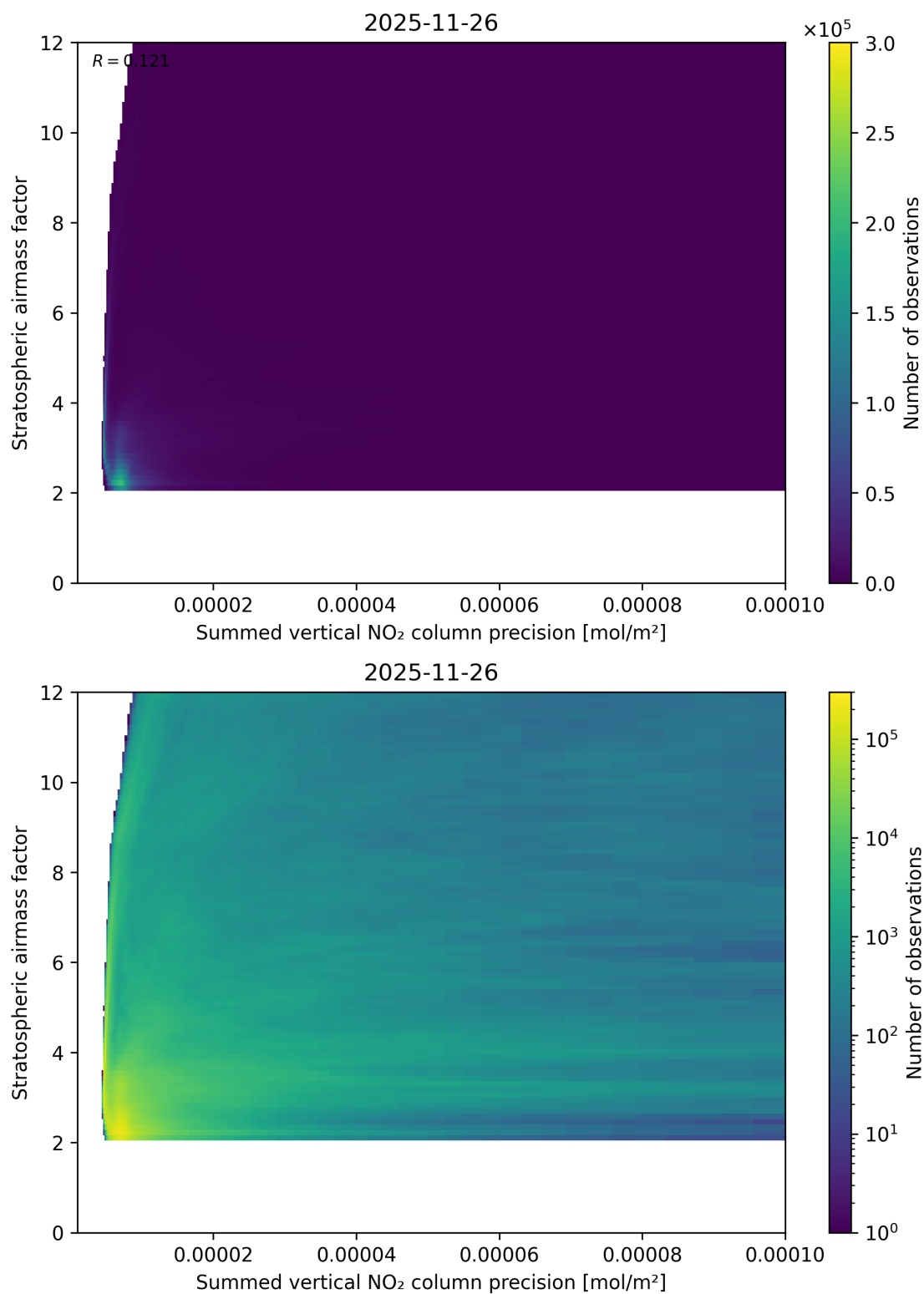
Figure 106: Scatter density plot of “Summed vertical NO 2 column precision” against “Stratospheric airmass factor” for 2025-11-25 to 2025-11-27.
