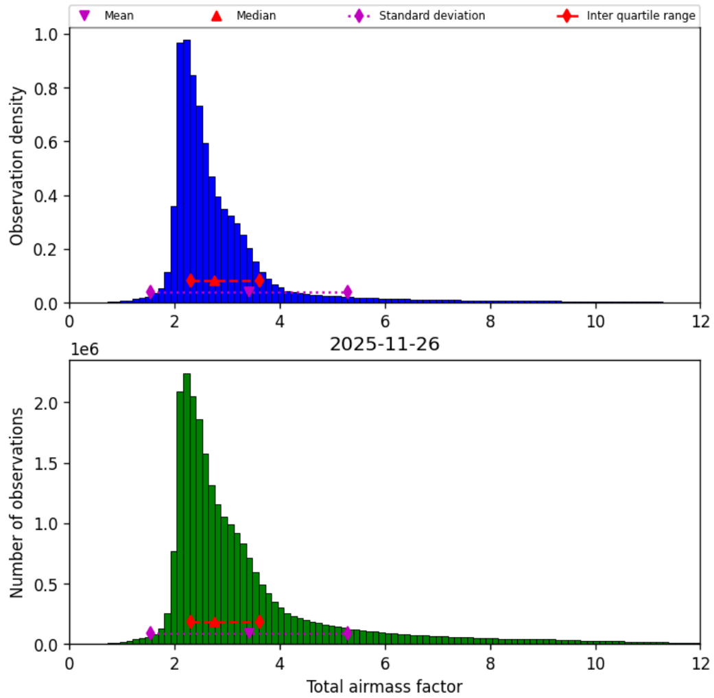
Figure 32: Histogram of “Total airmass factor” for 2025-11-25 to 2025-11-27
