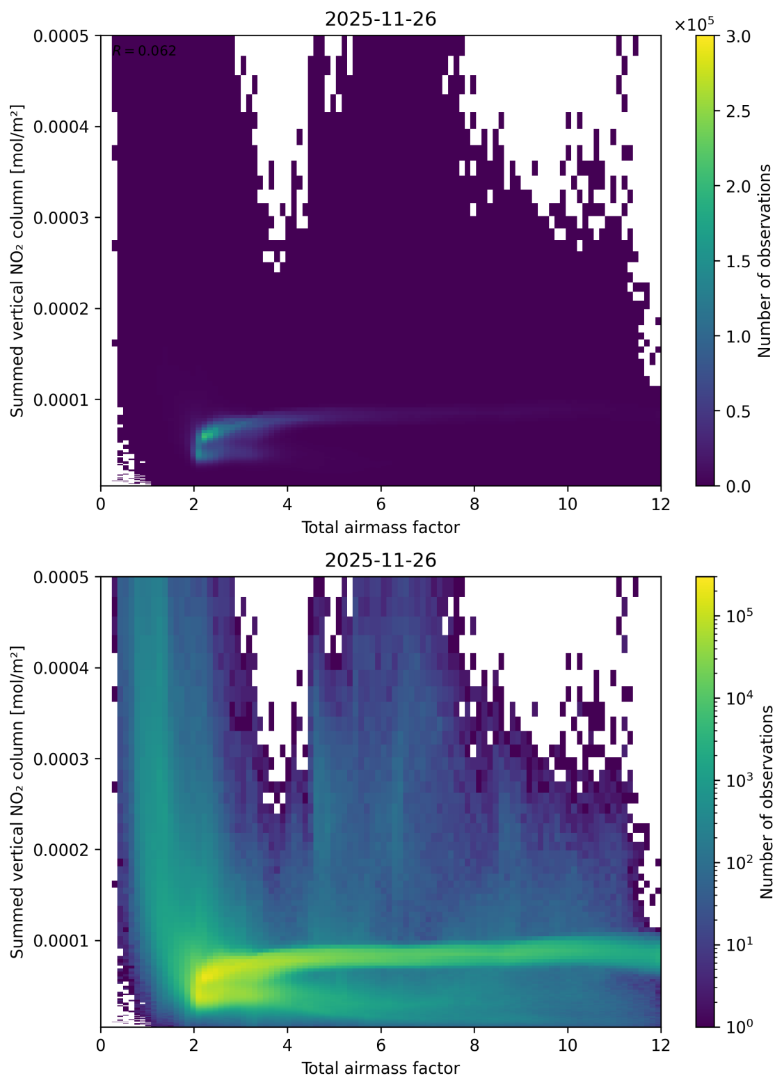
Figure 65: Scatter density plot of “Total airmass factor” against “Summed vertical NO 2 column” for 2025-11-25 to 2025-11-27.
