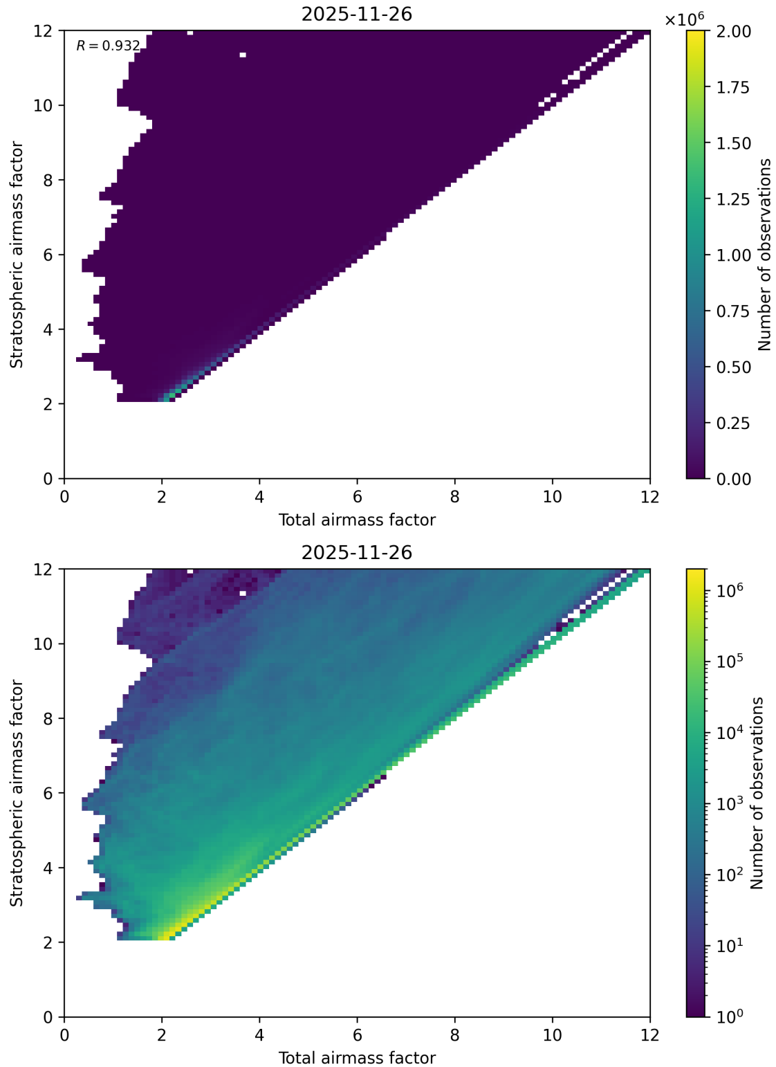
Figure 62: Scatter density plot of “Total airmass factor” against “Stratospheric airmass factor” for 2025-11-25 to 2025-11-27.
