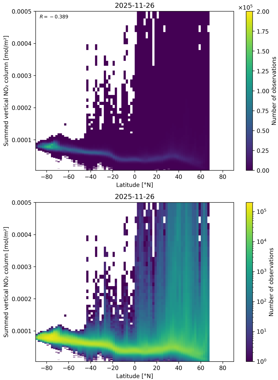
Figure 88: Scatter density plot of “Latitude” against “Summed vertical NO 2 column” for 2025-11-25 to 2025-11-27.
