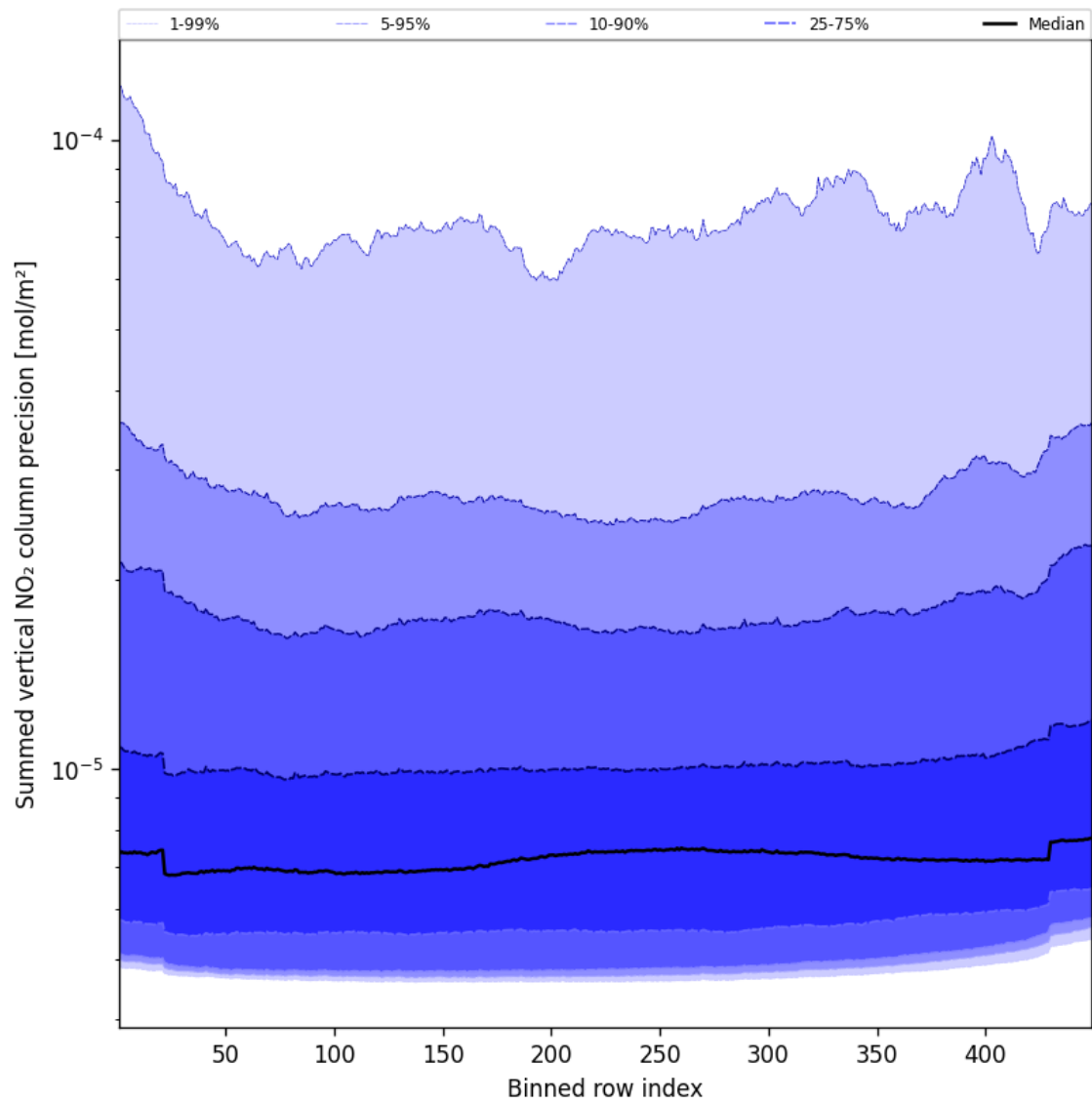
Figure 58: Along track statistics of “Summed vertical NO 2 column precision” for 2025-11-25 to 2025-11-27
