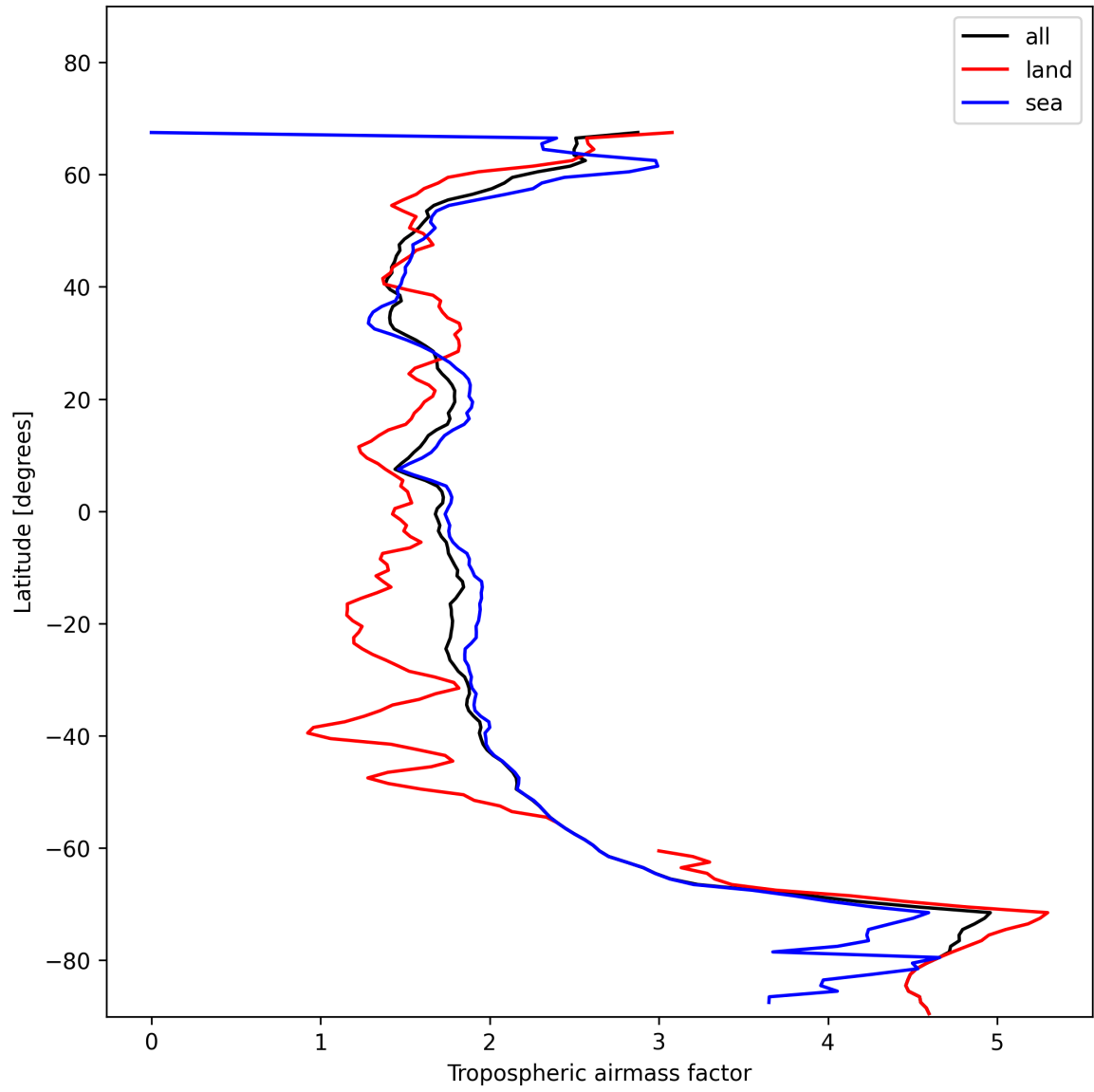
Figure 14: Zonal average of “Tropospheric airmass factor” for 2025-11-25 to 2025-11-27.
