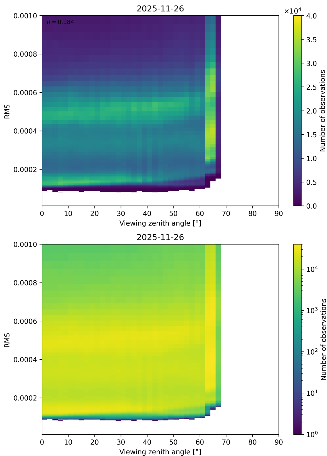
Figure 171: Scatter density plot of “Viewing zenith angle” against “RMS” for 2025-11-25 to 2025-11-27.
