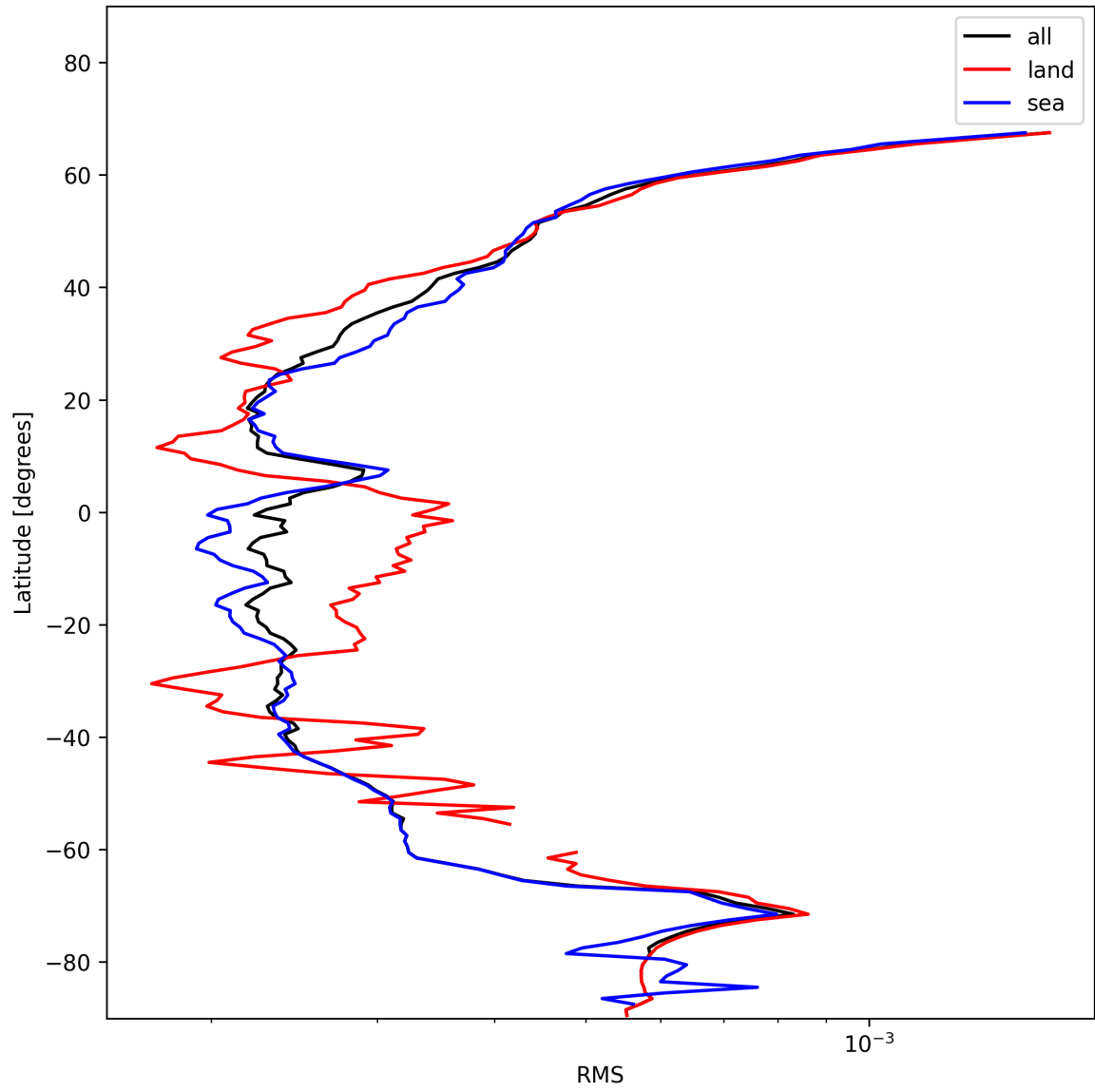
Figure 26: Zonal average of “RMS” for 2025-11-25 to 2025-11-27.
