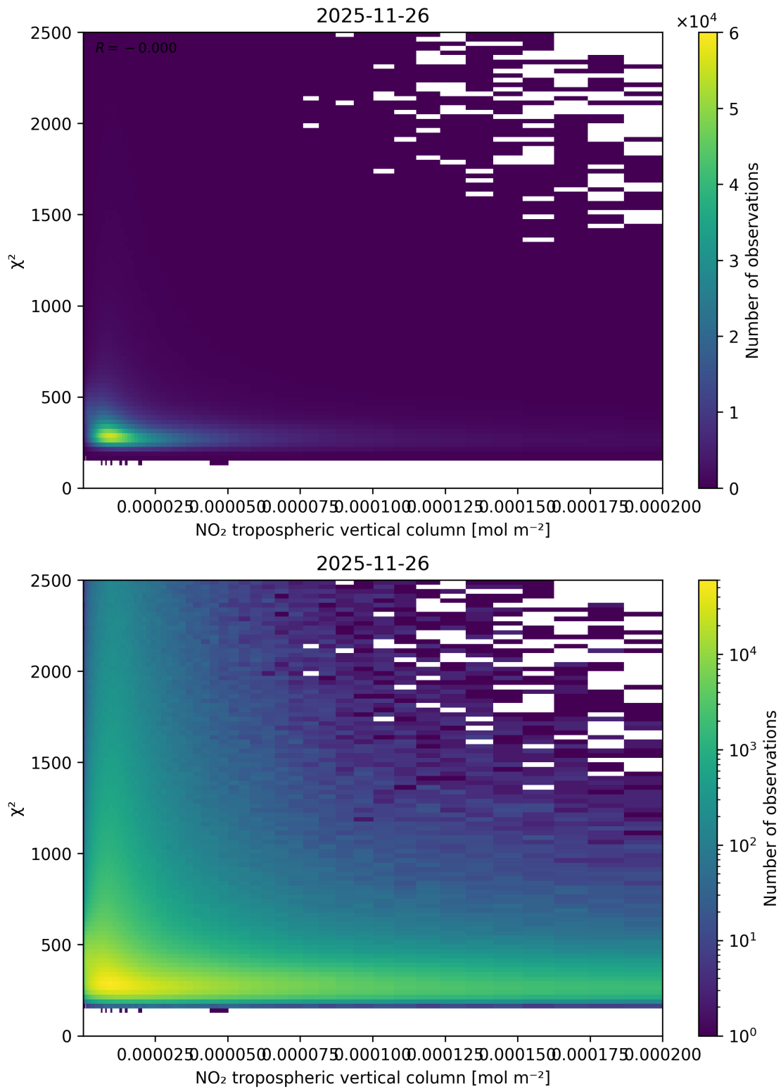
Figure 124: Scatter density plot of “NO 2 tropospheric vertical column” against “ \chi^2 ” for 2025-11-25 to 2025-11-27.
