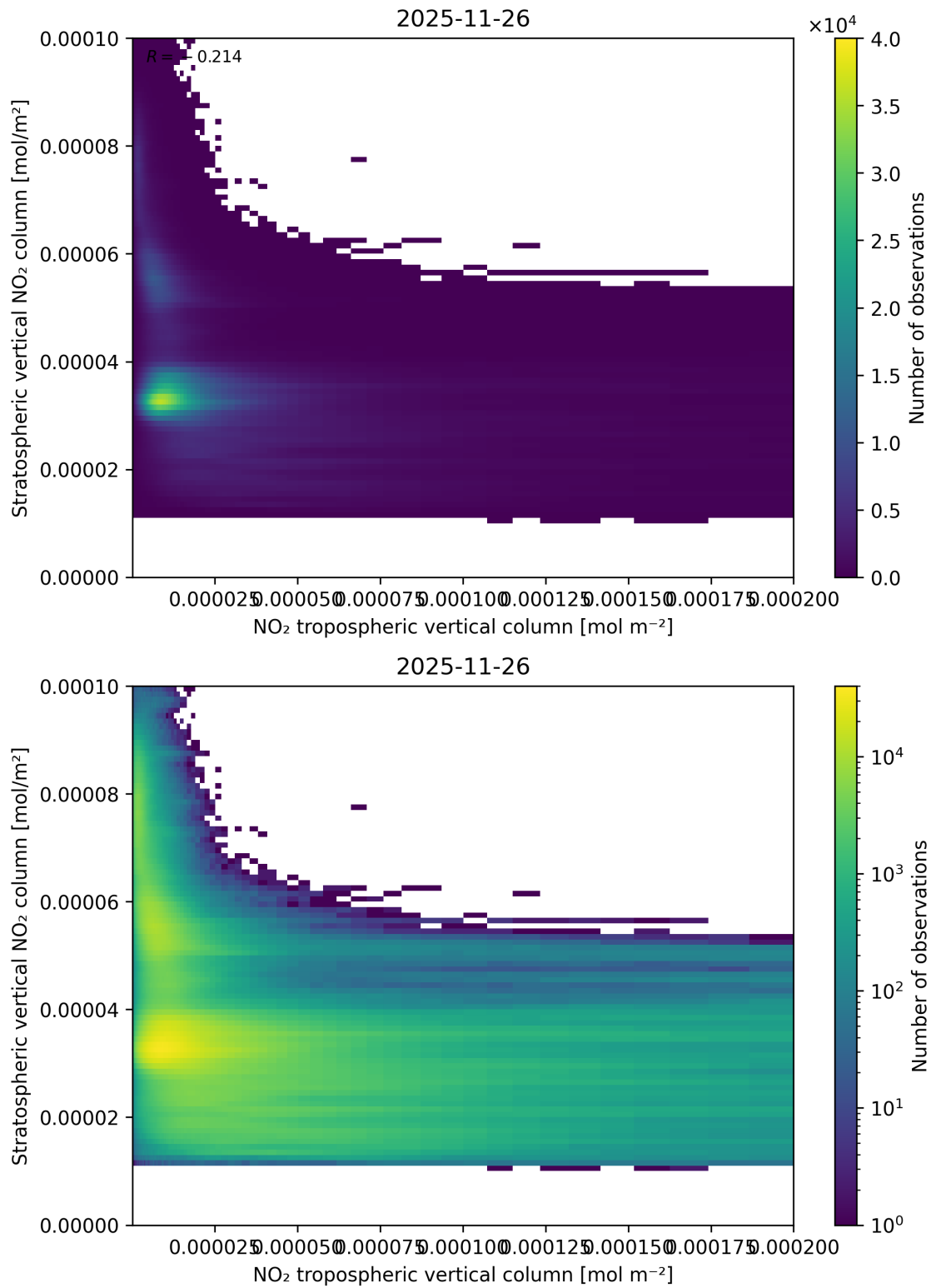
Figure 125: Scatter density plot of “NO 2 tropospheric vertical column” against “Stratospheric vertical NO 2 column” for 2025-11-25 to 2025-11-27.
