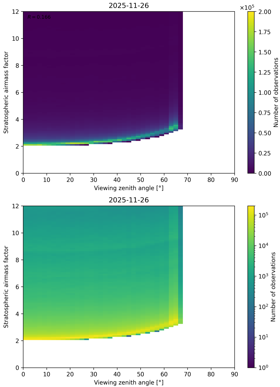
Figure 159: Scatter density plot of “Viewing zenith angle” against “Stratospheric airmass factor” for 2025-11-25 to 2025-11-27.
