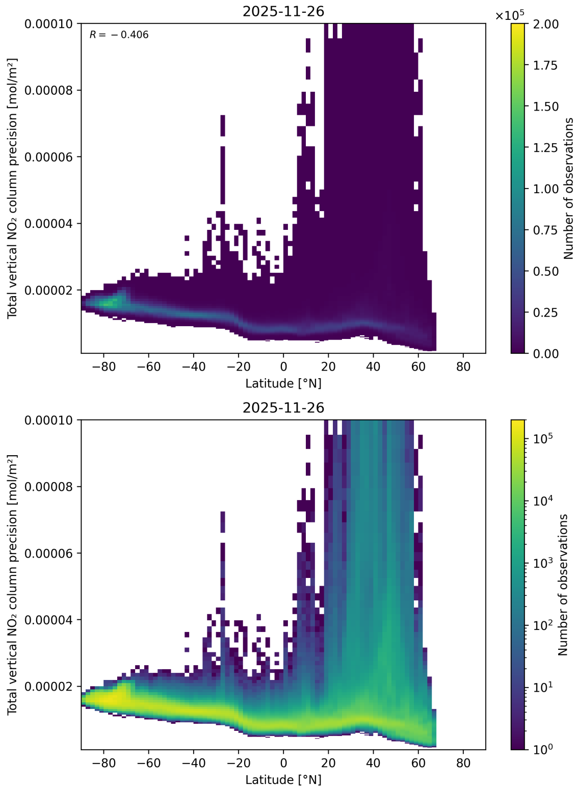
Figure 91: Scatter density plot of “Latitude” against “Total vertical NO 2 column precision” for 2025-11-25 to 2025-11-27.
