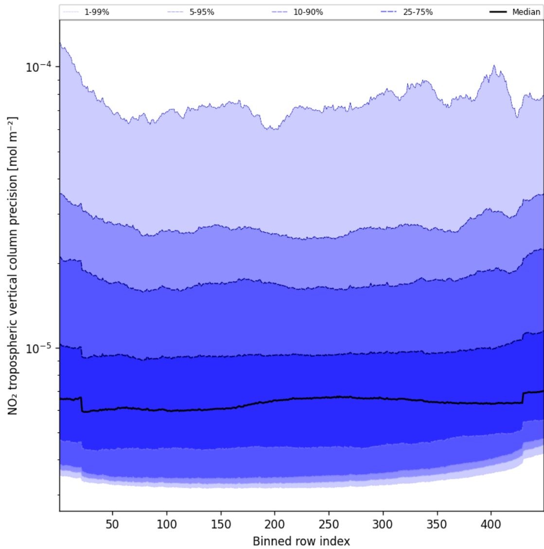
Figure 47: Along track statistics of “NO 2 tropospheric vertical column precision” for 2025-11-25 to 2025-11-27
