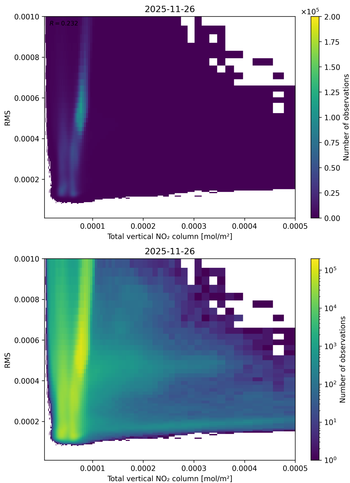
Figure 120: Scatter density plot of “Total vertical NO 2 column” against “RMS” for 2025-11-25 to 2025-11-27.
