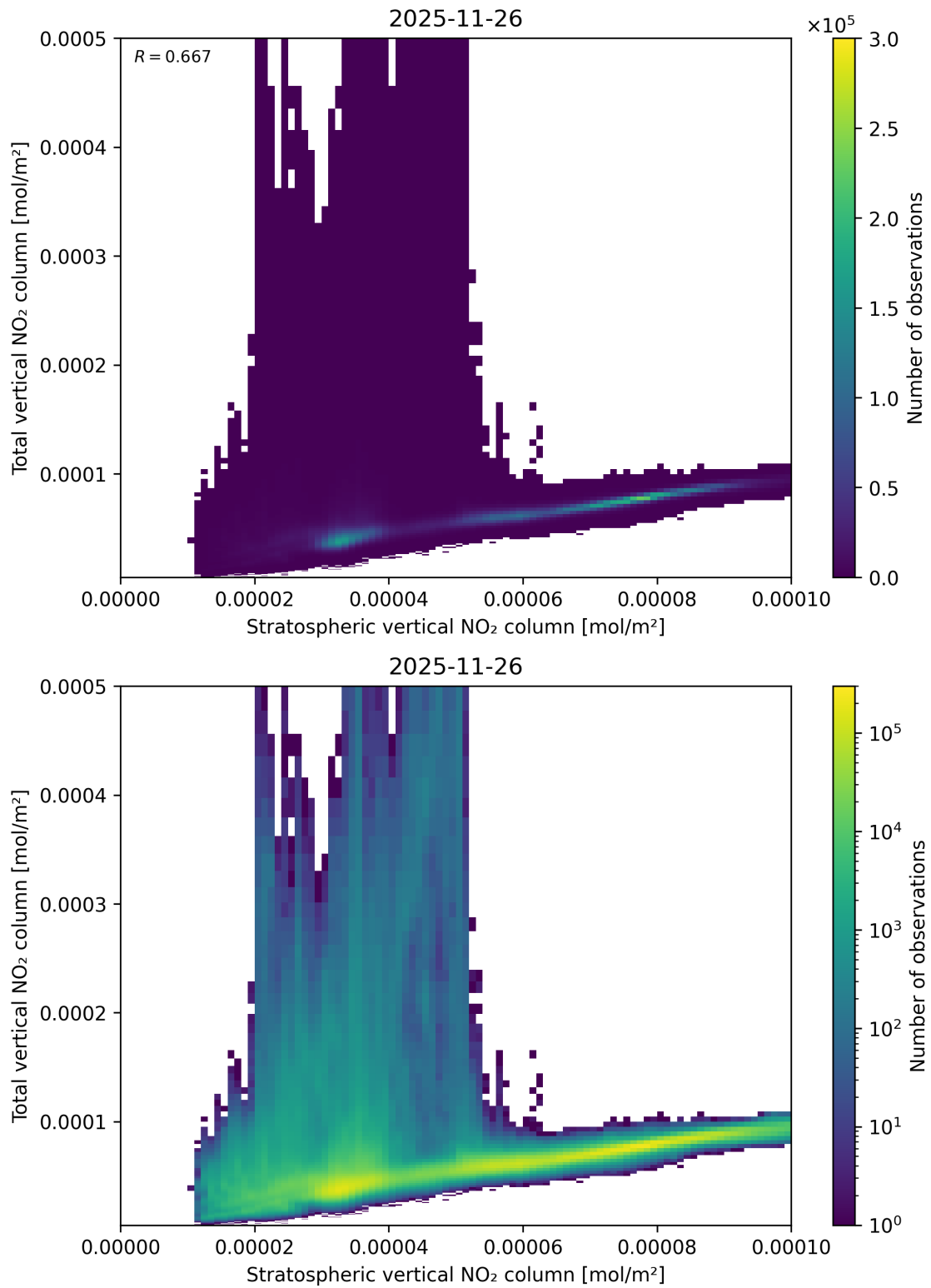
Figure 100: Scatter density plot of “Stratospheric vertical NO 2 column” against “Total vertical NO 2 column” for 2025-11-25 to 2025-11-27.
