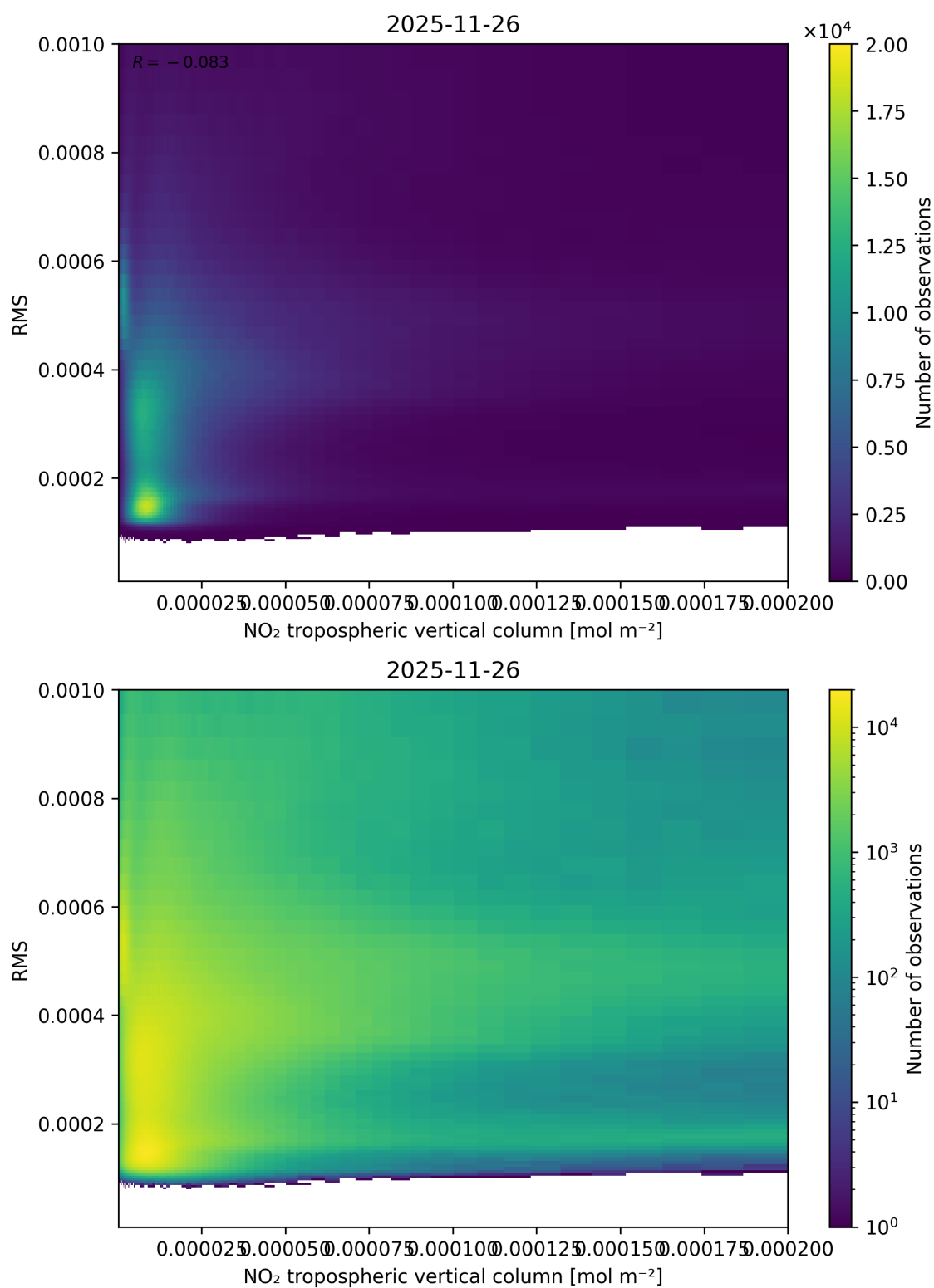
Figure 142: Scatter density plot of “NO 2 tropospheric vertical column” against “RMS” for 2025-11-25 to 2025-11-27.
