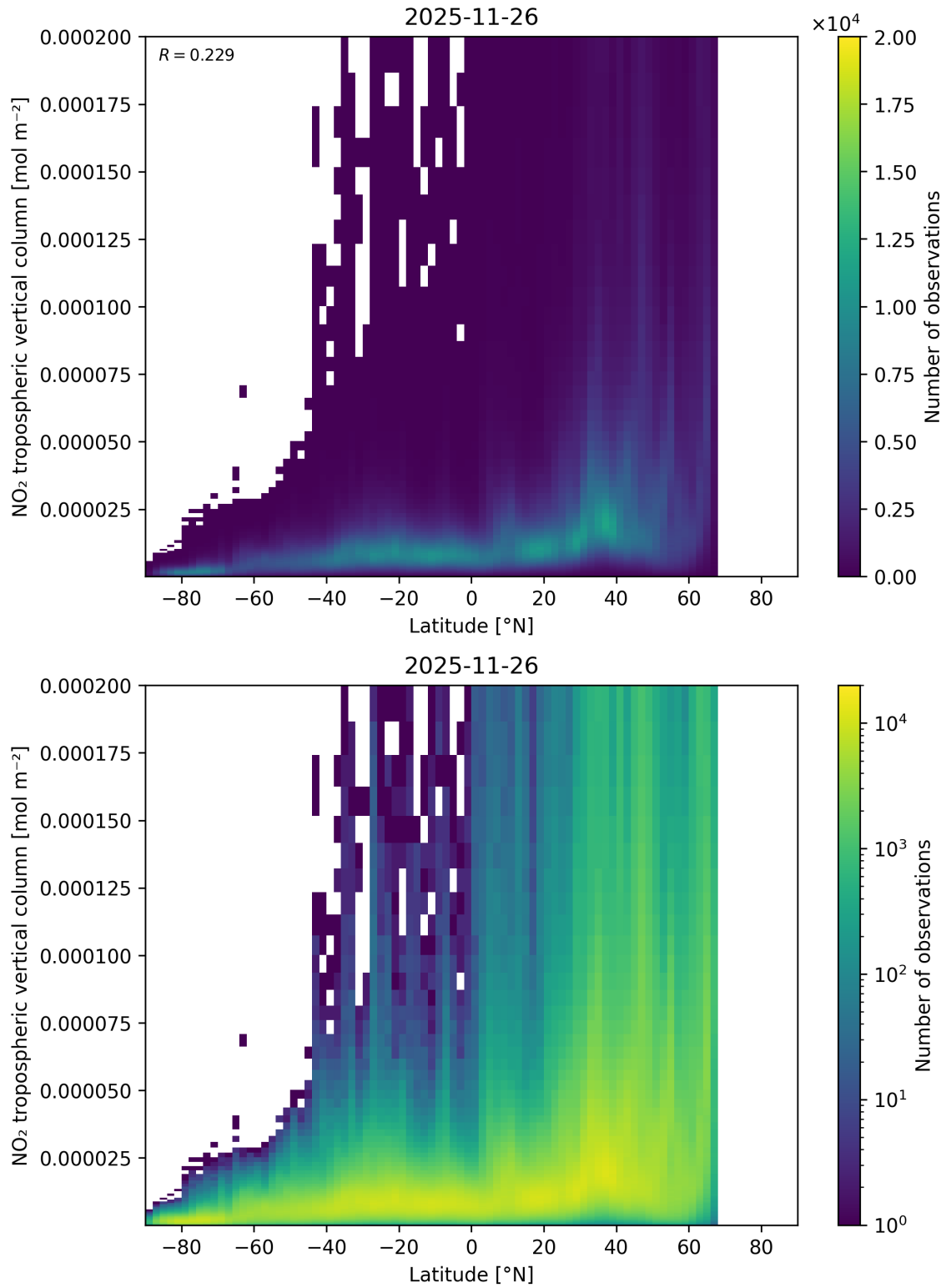
Figure 92: Scatter density plot of “Latitude” against “NO 2 tropospheric vertical column” for 2025-11-25 to 2025-11-27.
