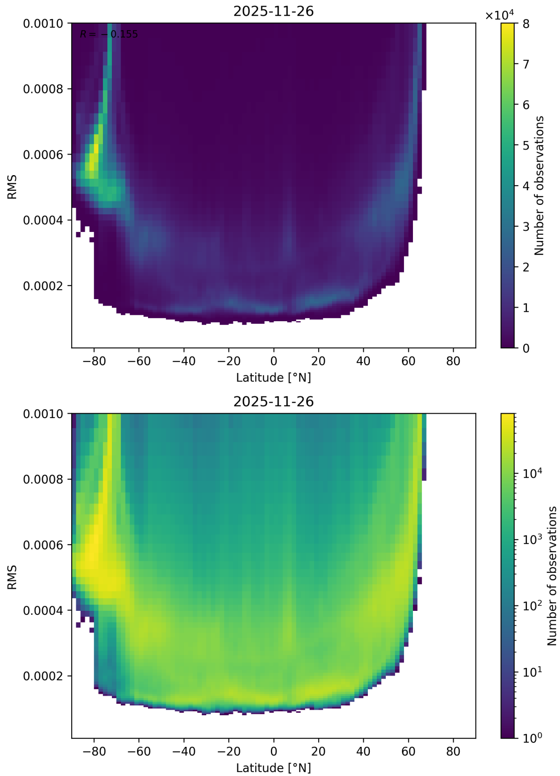
Figure 94: Scatter density plot of “Latitude” against “RMS” for 2025-11-25 to 2025-11-27.
