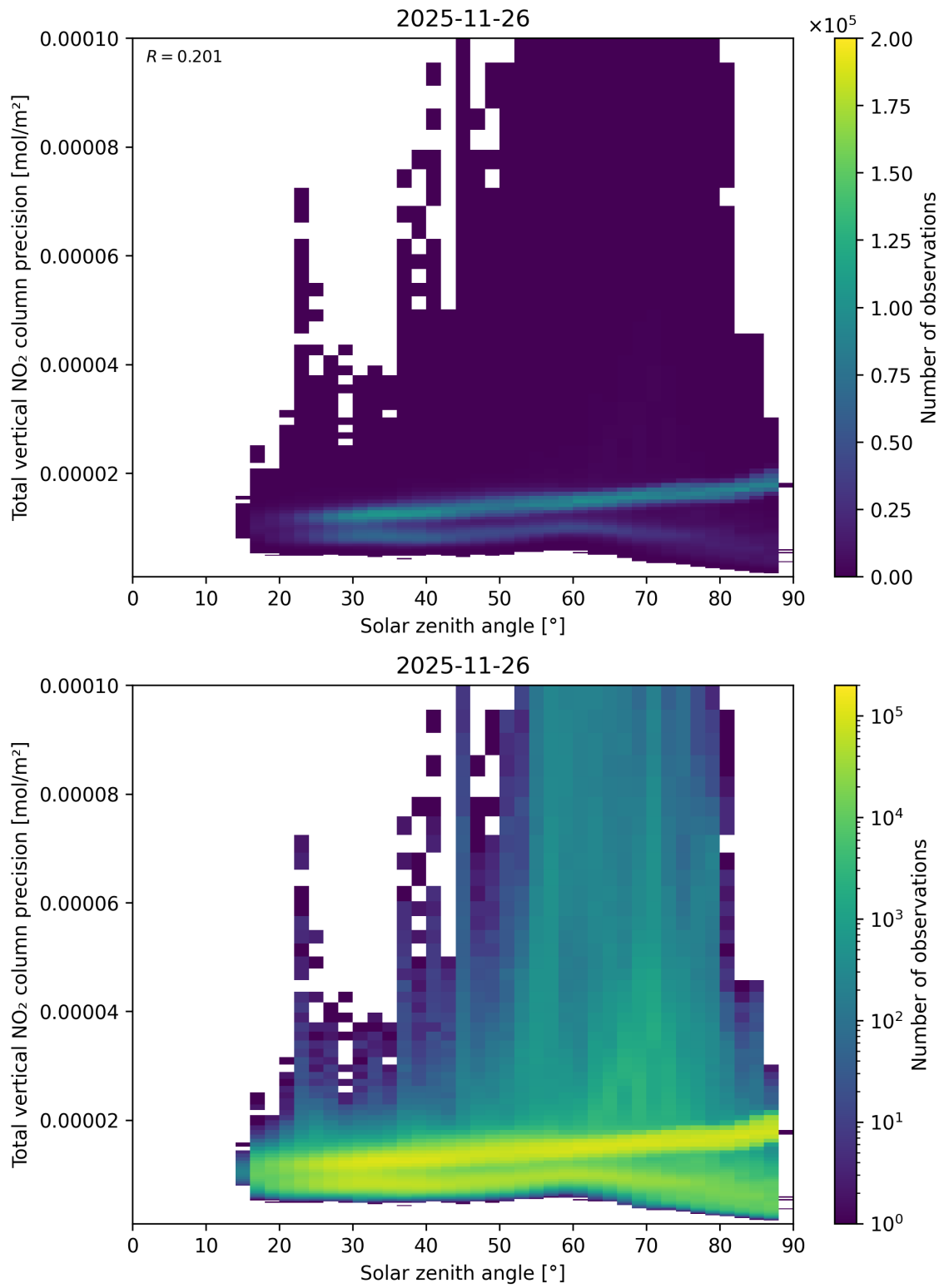
Figure 154: Scatter density plot of “Solar zenith angle” against “Total vertical NO 2 column precision” for 2025-11-25 to 2025-11-27.
