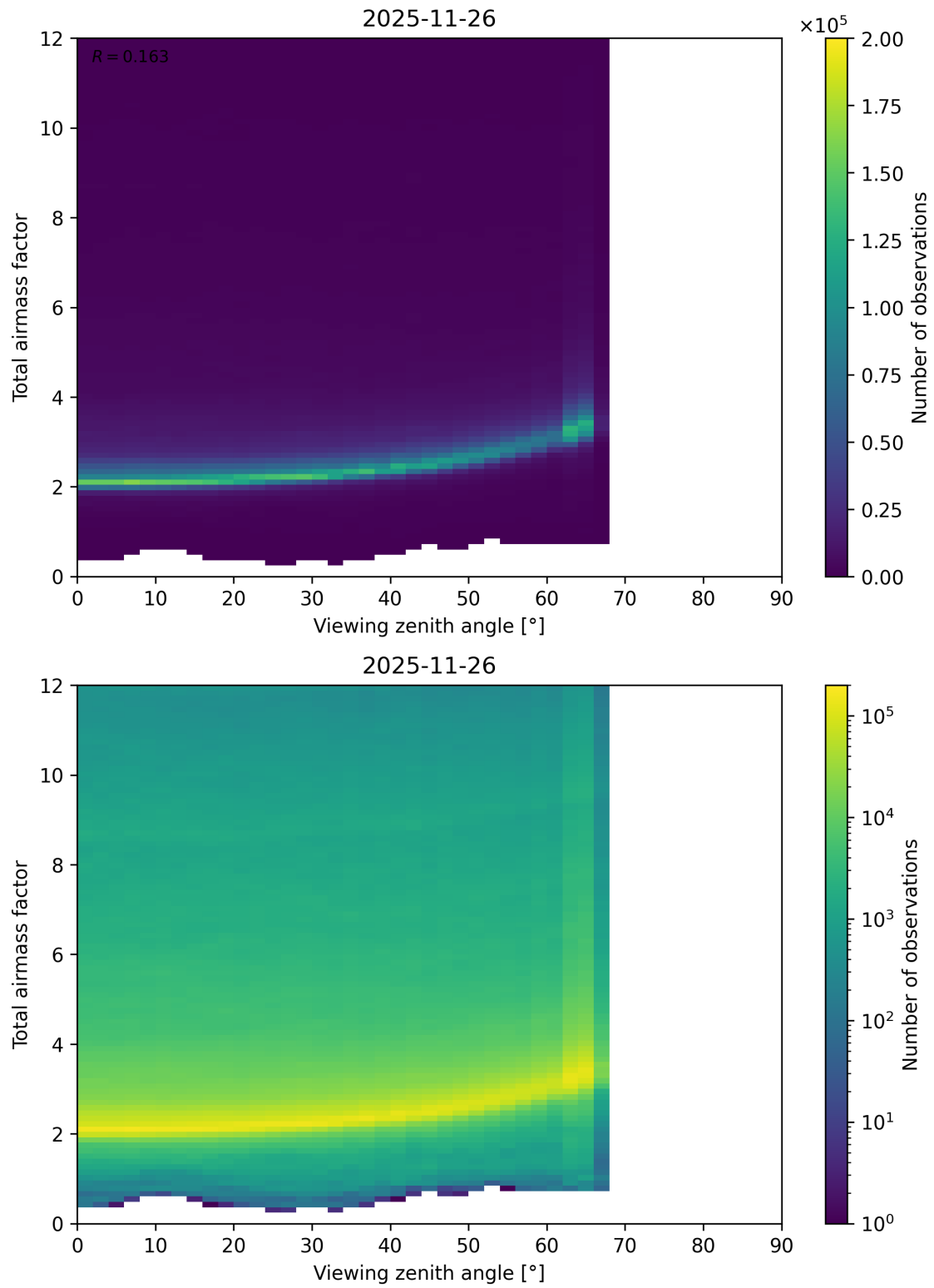
Figure 160: Scatter density plot of “Viewing zenith angle” against “Total airmass factor” for 2025-11-25 to 2025-11-27.
