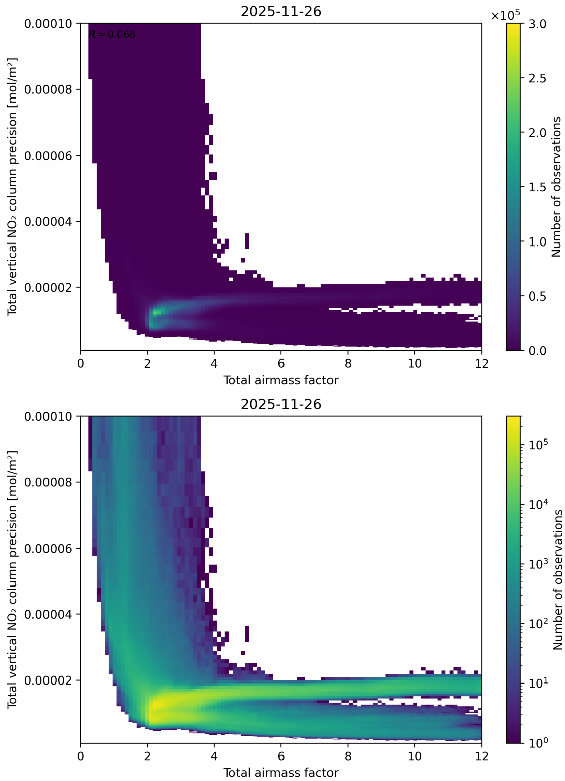
Figure 68: Scatter density plot of “Total airmass factor” against “Total vertical NO 2 column precision” for 2025-11-25 to 2025-11-27.
