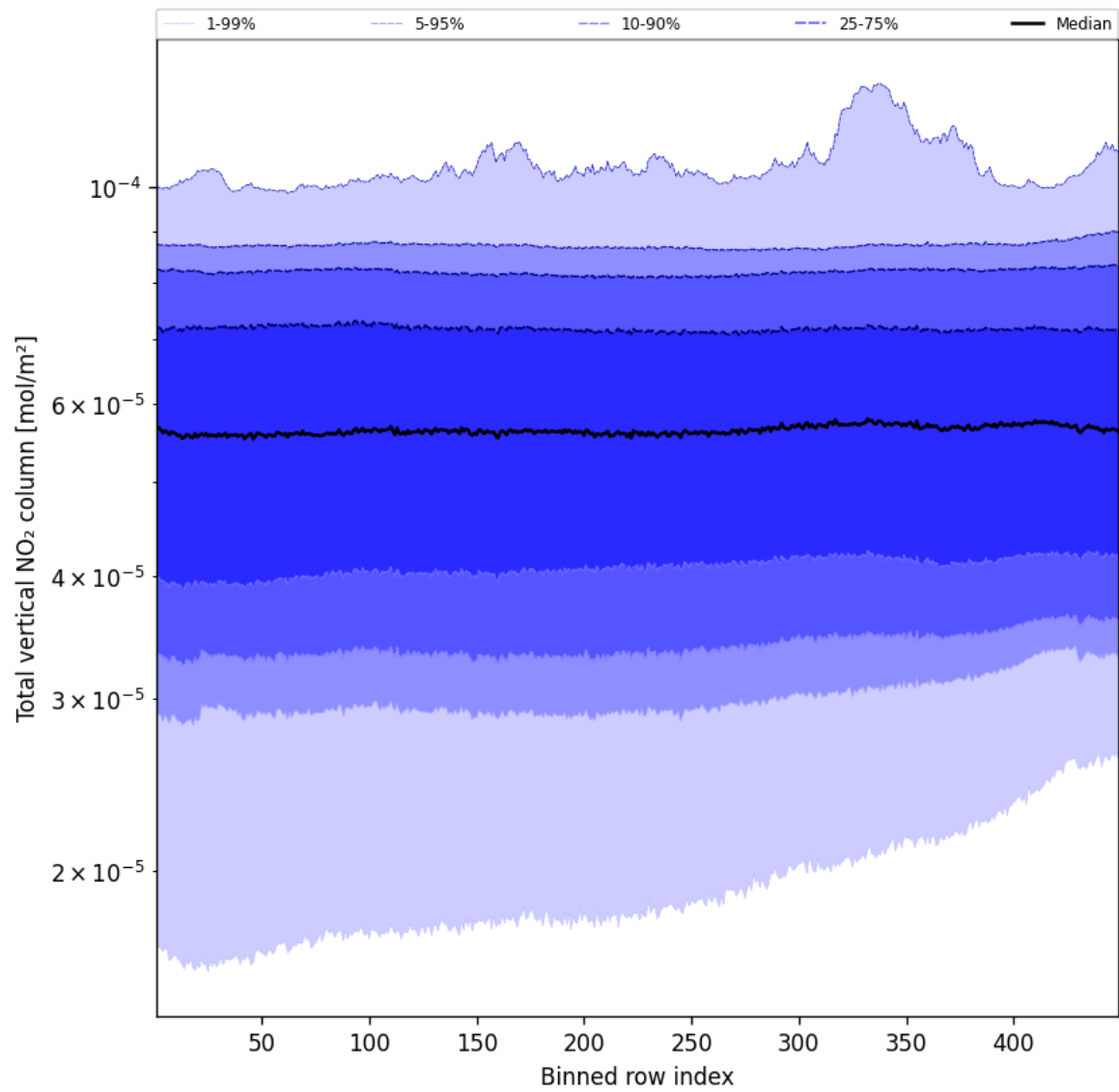
Figure 55: Along track statistics of “Total vertical NO 2 column” for 2025-11-25 to 2025-11-27
