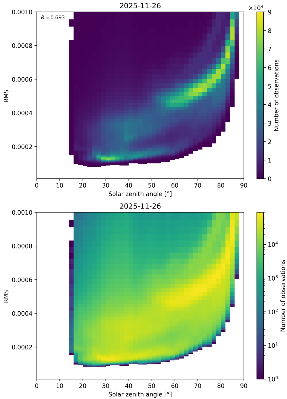
Figure 157: Scatter density plot of “Solar zenith angle” against “RMS” for 2025-11-25 to 2025-11-27.
