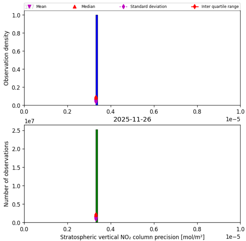
Figure 37: Histogram of “Stratospheric vertical NO 2 column precision” for 2025-11-25 to 2025-11-27
