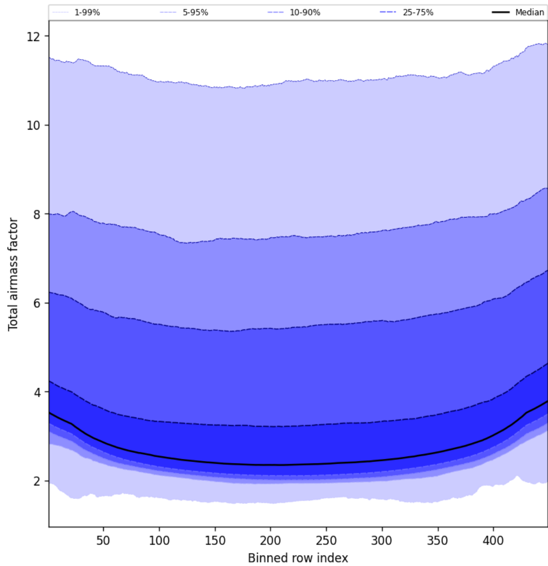
Figure 49: Along track statistics of “Total airmass factor” for 2025-11-25 to 2025-11-27
