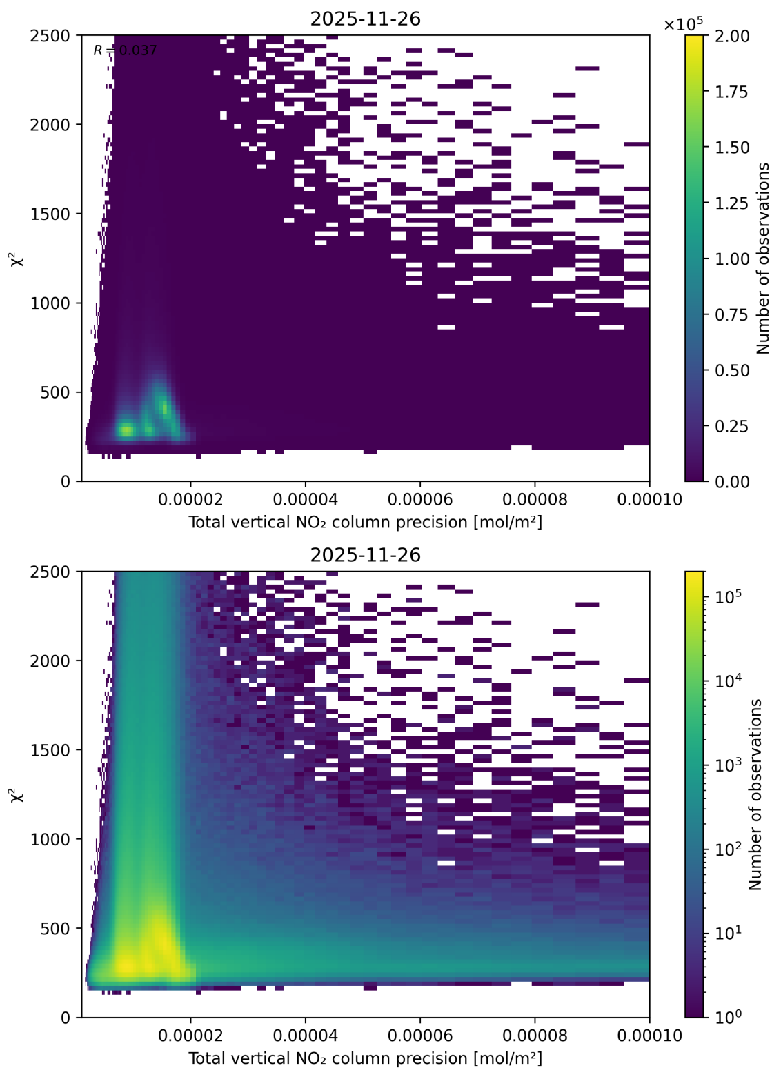
Figure 116: Scatter density plot of “Total vertical NO 2 column precision” against “ \chi^2 ” for 2025-11-25 to 2025-11-27.
