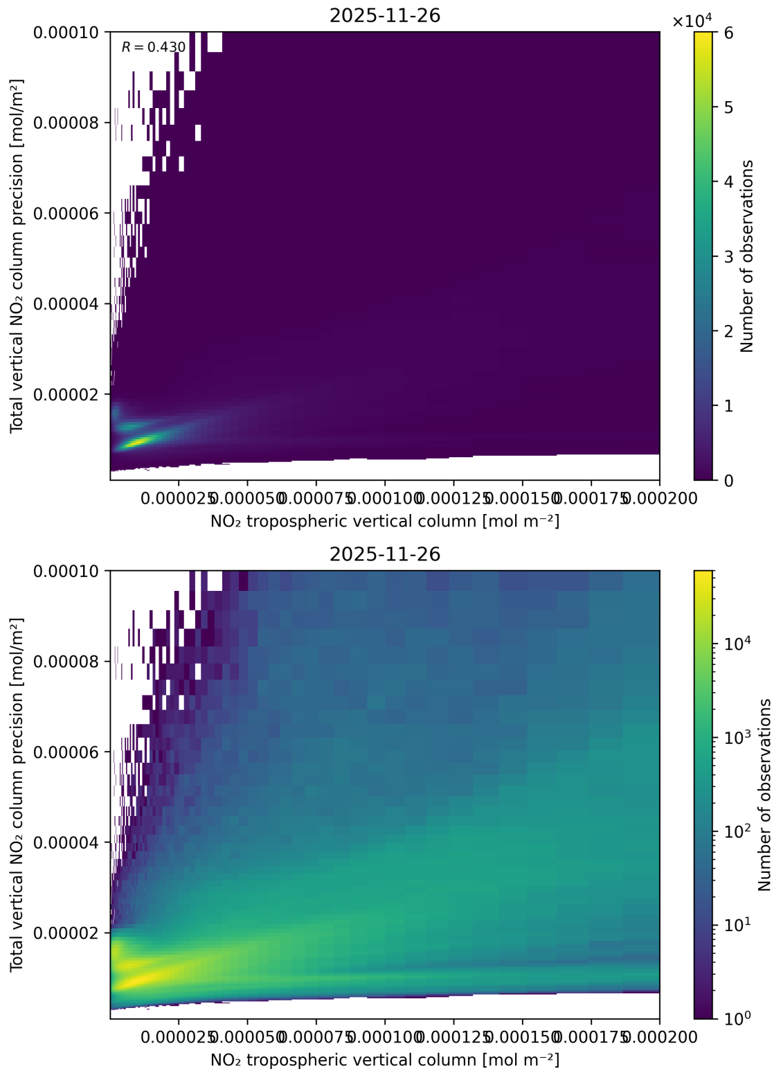
Figure 129: Scatter density plot of “NO 2 tropospheric vertical column” against “Total vertical NO 2 column precision” for 2025-11-25 to 2025-11-27.
