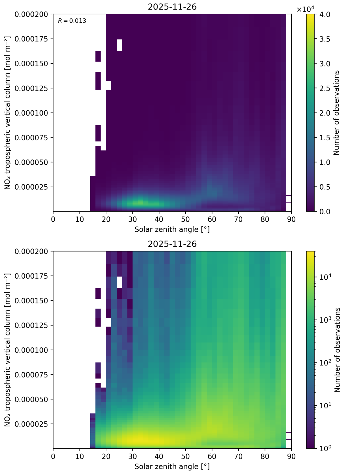
Figure 155: Scatter density plot of “Solar zenith angle” against “NO 2 tropospheric vertical column” for 2025-11-25 to 2025-11-27.
