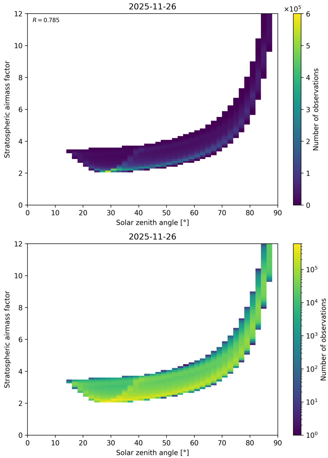
Figure 145: Scatter density plot of “Solar zenith angle” against “Stratospheric airmass factor” for 2025-11-25 to 2025-11-27.
