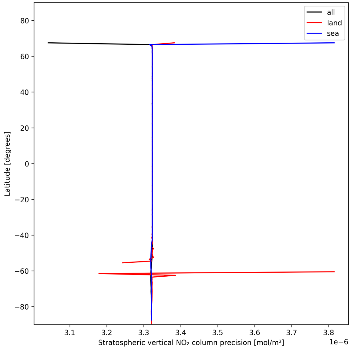
Figure 20: Zonal average of “Stratospheric vertical NO 2 column precision” for 2025-11-25 to 2025-11-27.
