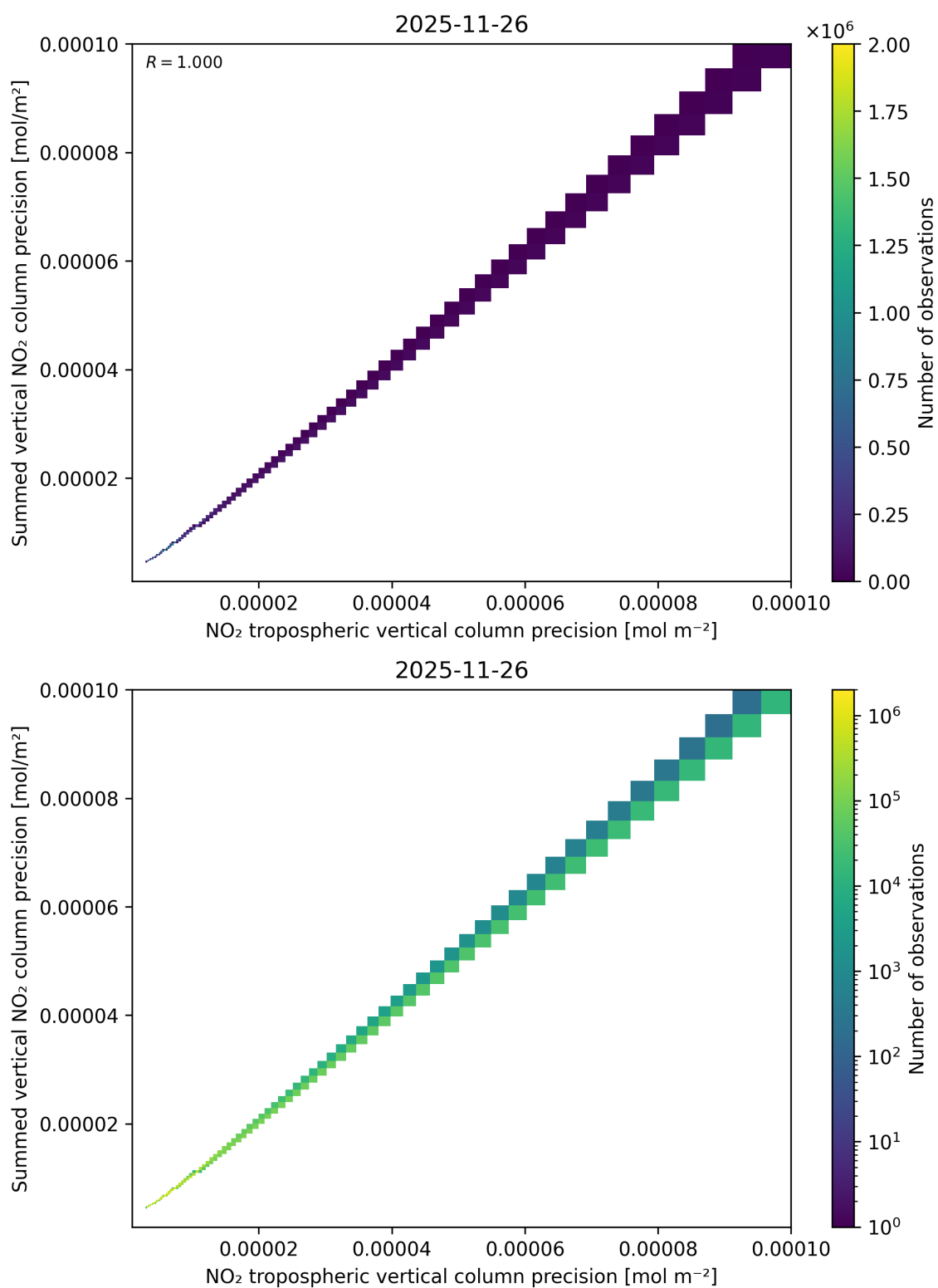
Figure 137: Scatter density plot of “NO 2 tropospheric vertical column precision” against “Summed vertical NO 2 column precision” for 2025-11-25 to 2025-11-27.
