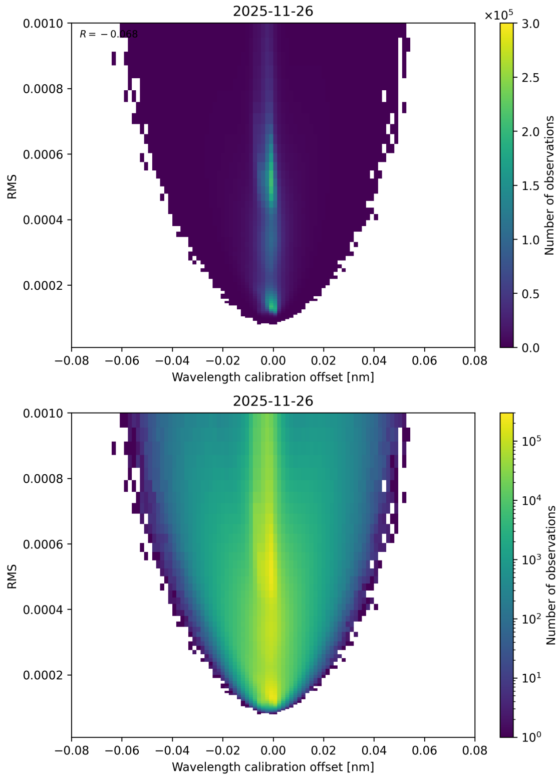
Figure 181: Scatter density plot of “Wavelength calibration offset” against “RMS” for 2025-11-25 to 2025-11-27.
