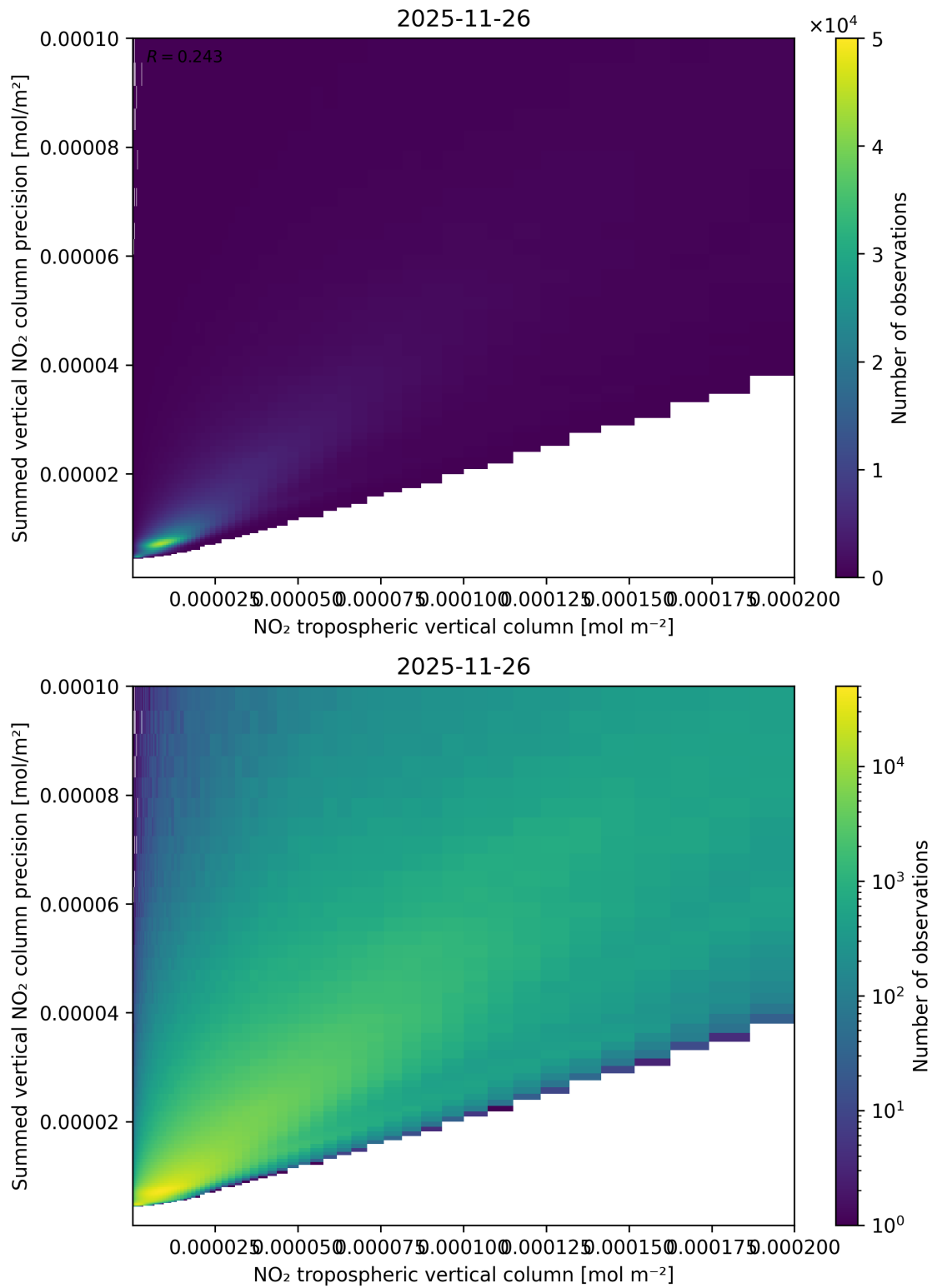
Figure 127: Scatter density plot of “NO 2 tropospheric vertical column” against “Summed vertical NO 2 column precision” for 2025-11-25 to 2025-11-27.
