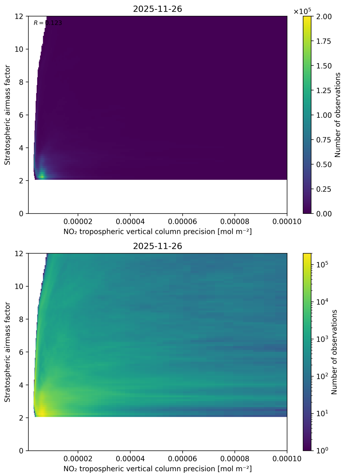
Figure 131: Scatter density plot of “NO 2 tropospheric vertical column precision” against “Stratospheric airmass factor” for 2025-11-25 to 2025-11-27.
