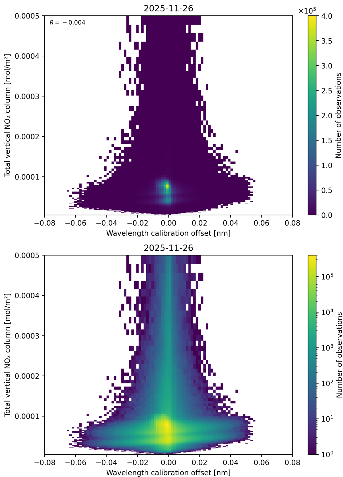
Figure 179: Scatter density plot of “Wavelength calibration offset” against “Total vertical NO 2 column” for 2025-11-25 to 2025-11-27.
