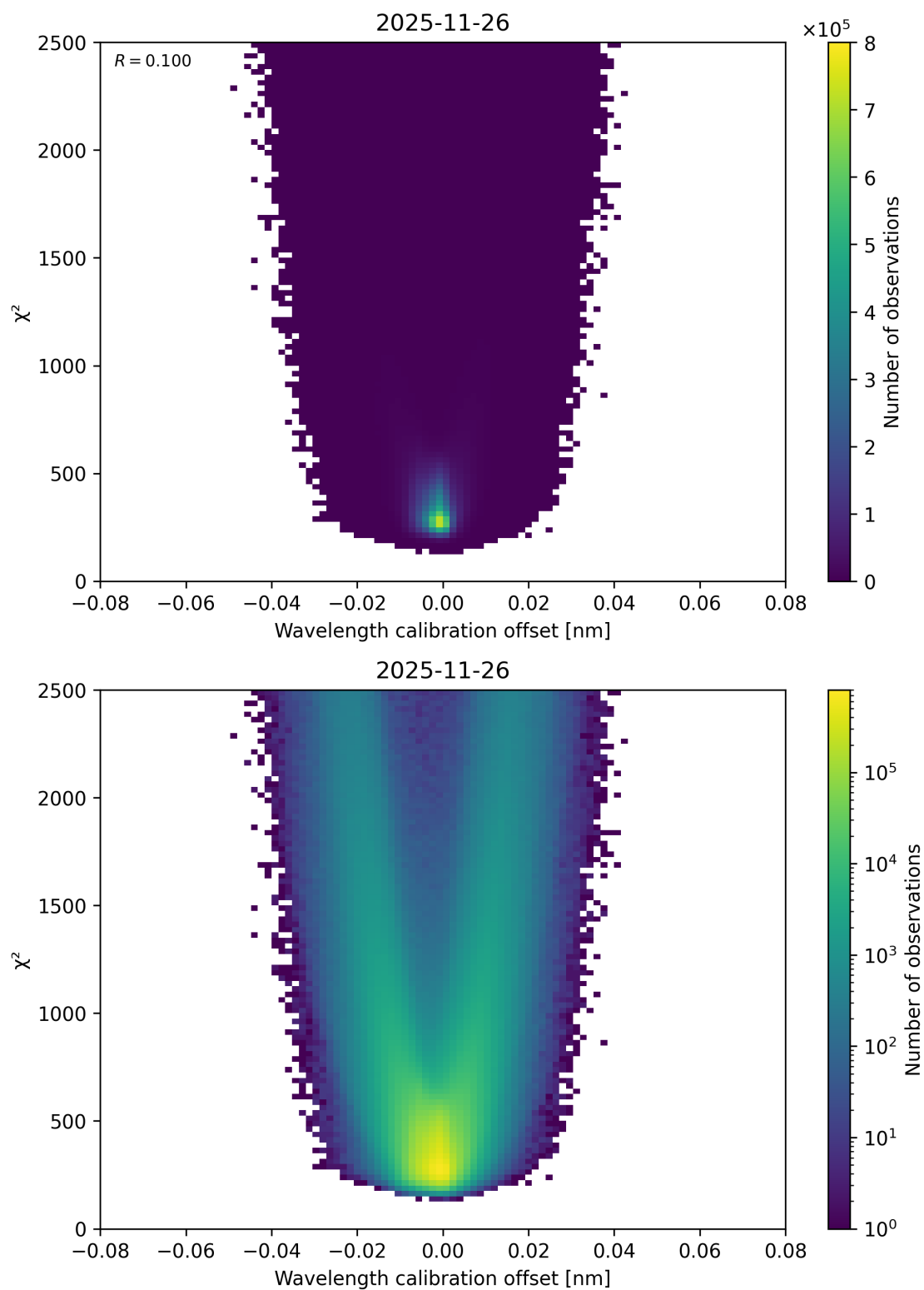
Figure 175: Scatter density plot of “Wavelength calibration offset” against “ \chi^2 ” for 2025-11-25 to 2025-11-27.
