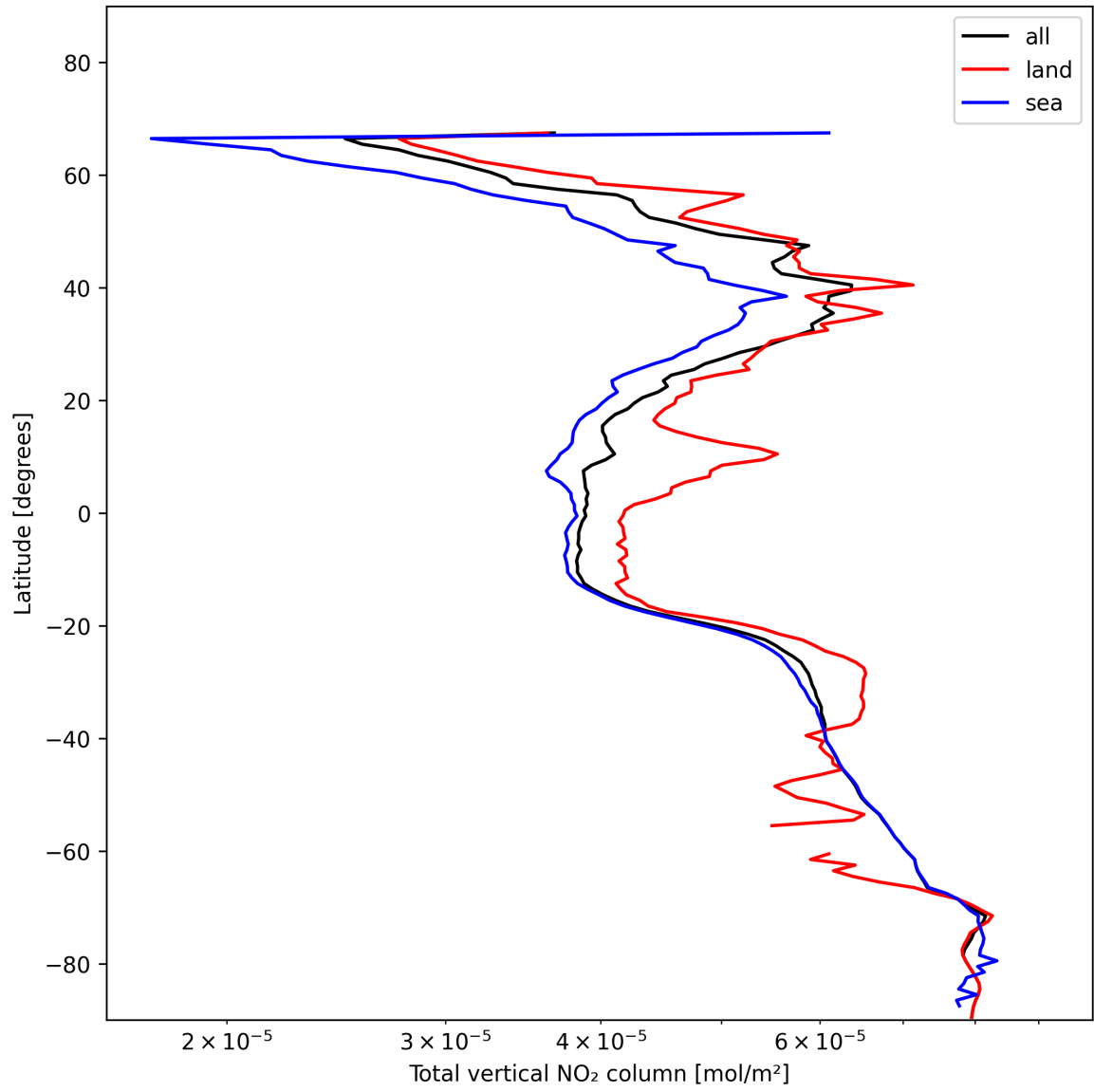
Figure 21: Zonal average of “Total vertical NO 2 column” for 2025-11-25 to 2025-11-27.
