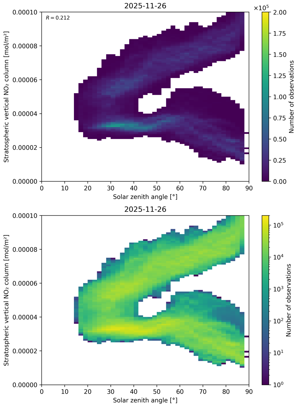
Figure 150: Scatter density plot of “Solar zenith angle” against “Stratospheric vertical NO 2 column” for 2025-11-25 to 2025-11-27.
