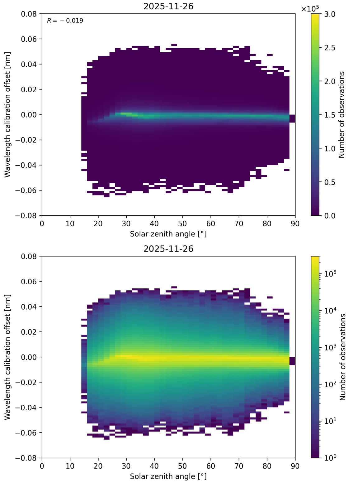
Figure 158: Scatter density plot of “Solar zenith angle” against “Wavelength calibration offset” for 2025-11-25 to 2025-11-27.
