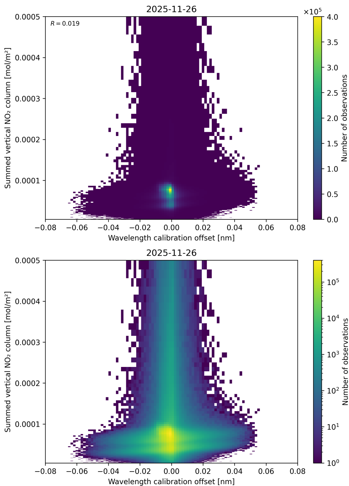
Figure 177: Scatter density plot of “Wavelength calibration offset” against “Summed vertical NO 2 column” for 2025-11-25 to 2025-11-27.
