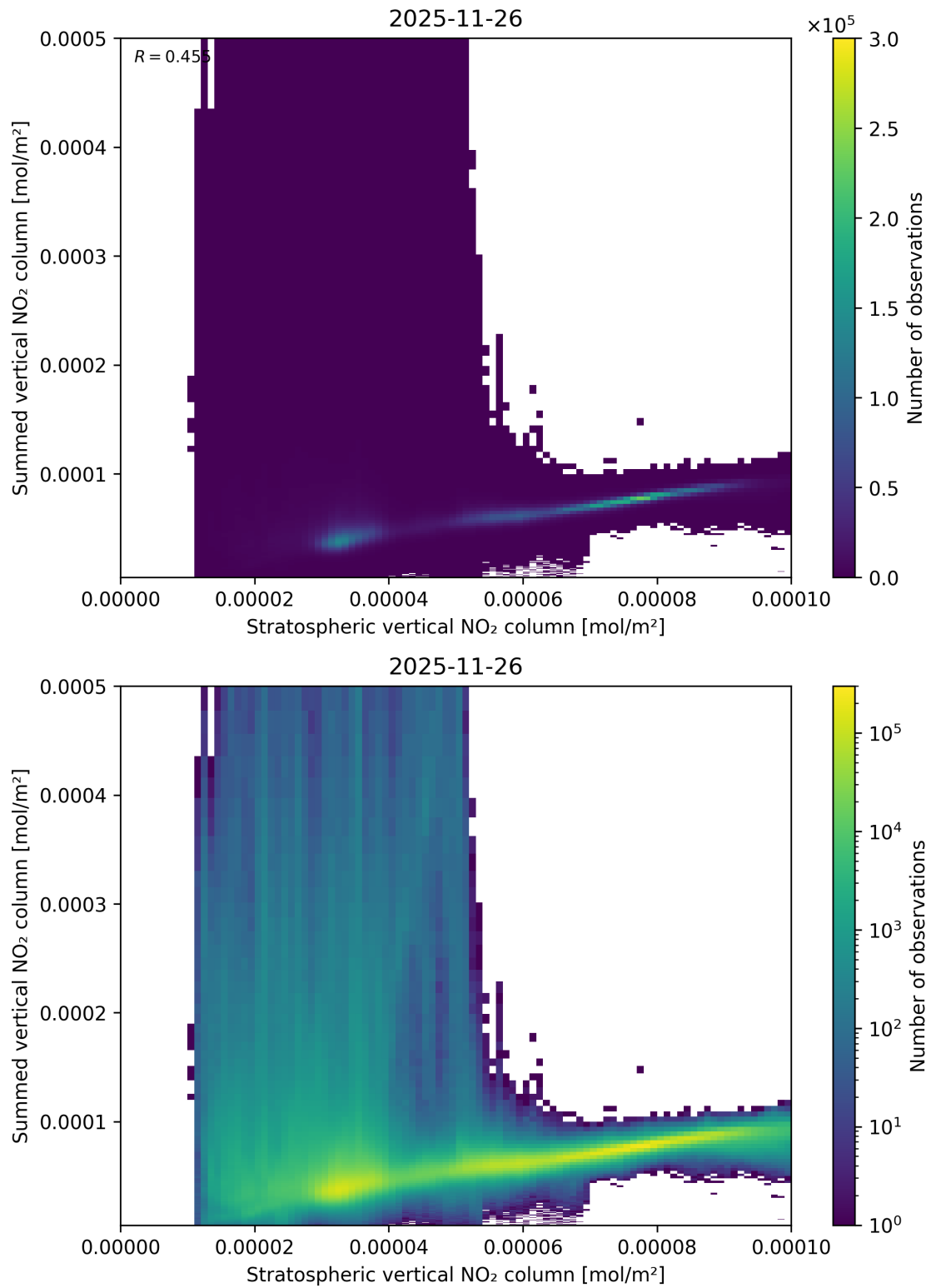
Figure 98: Scatter density plot of “Stratospheric vertical NO 2 column” against “Summed vertical NO 2 column” for 2025-11-25 to 2025-11-27.
