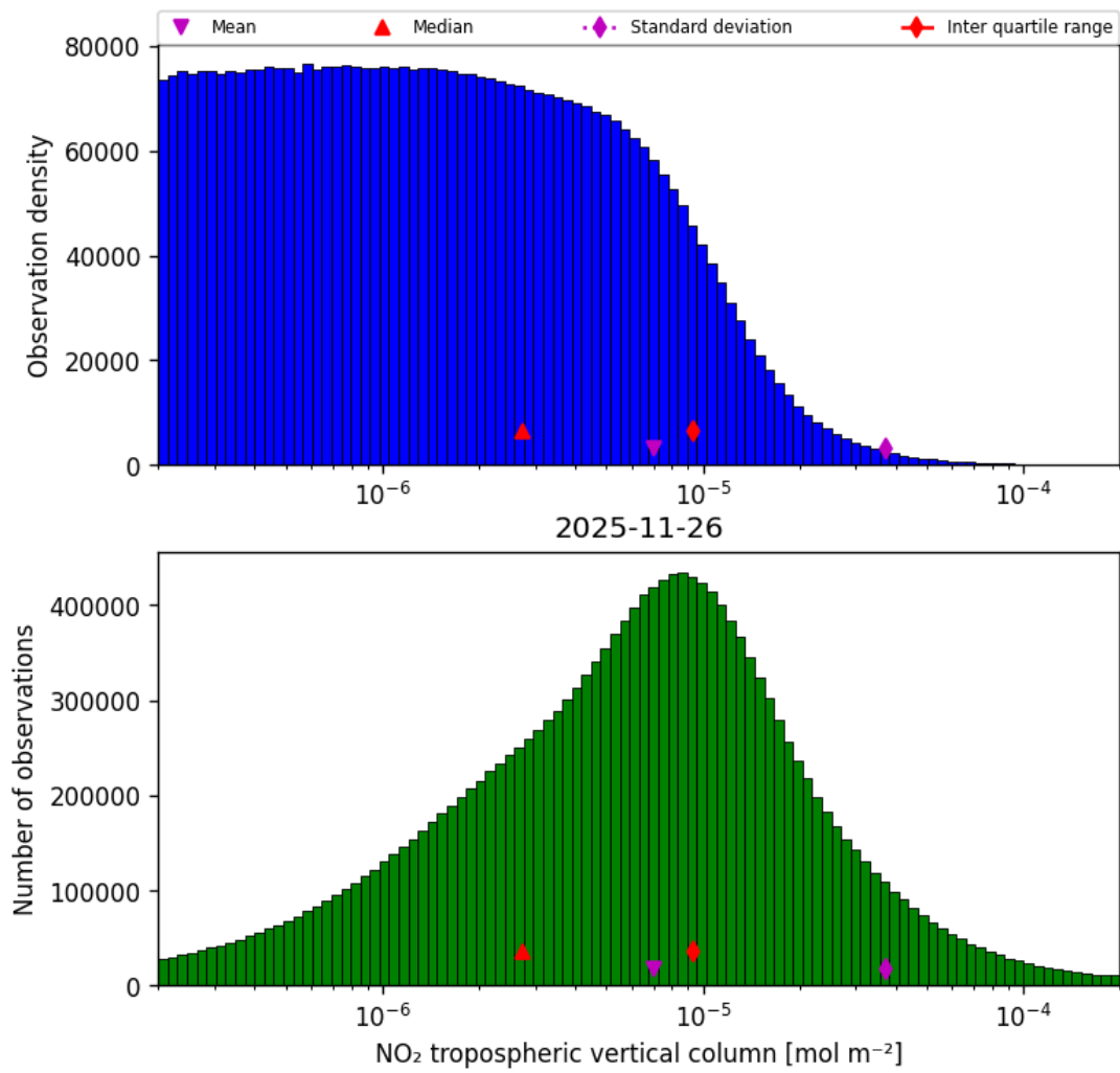
Figure 29: Histogram of “NO 2 tropospheric vertical column” for 2025-11-25 to 2025-11-27
