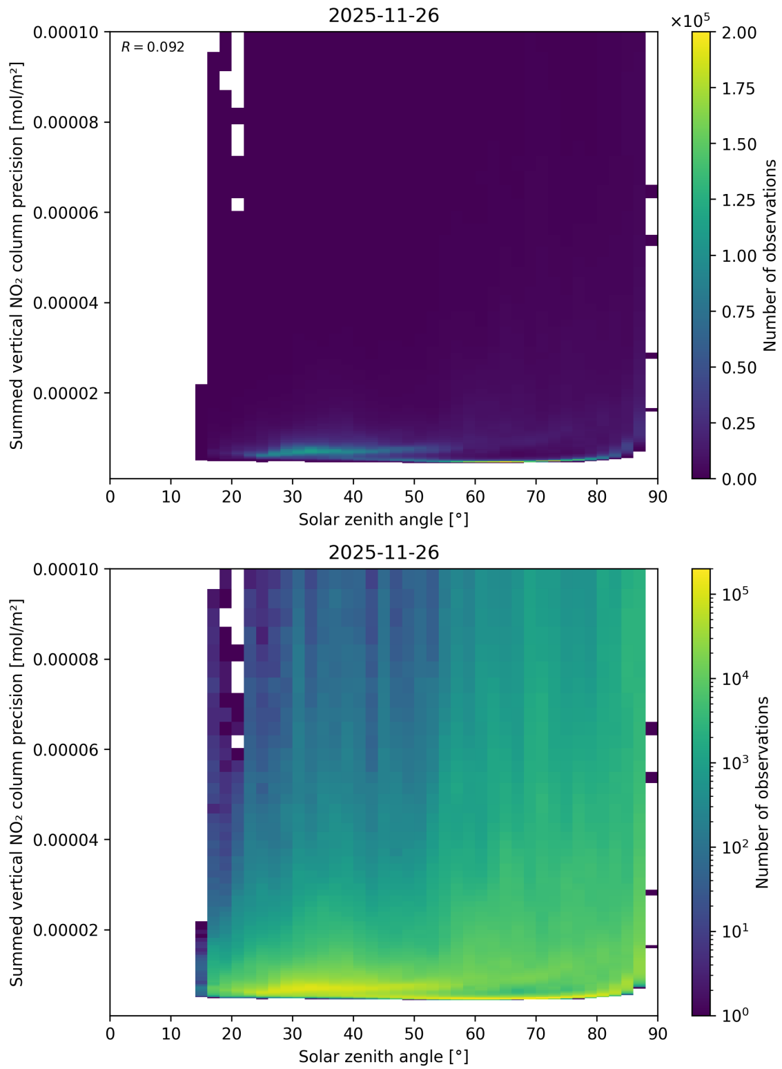
Figure 152: Scatter density plot of “Solar zenith angle” against “Summed vertical NO 2 column precision” for 2025-11-25 to 2025-11-27.
