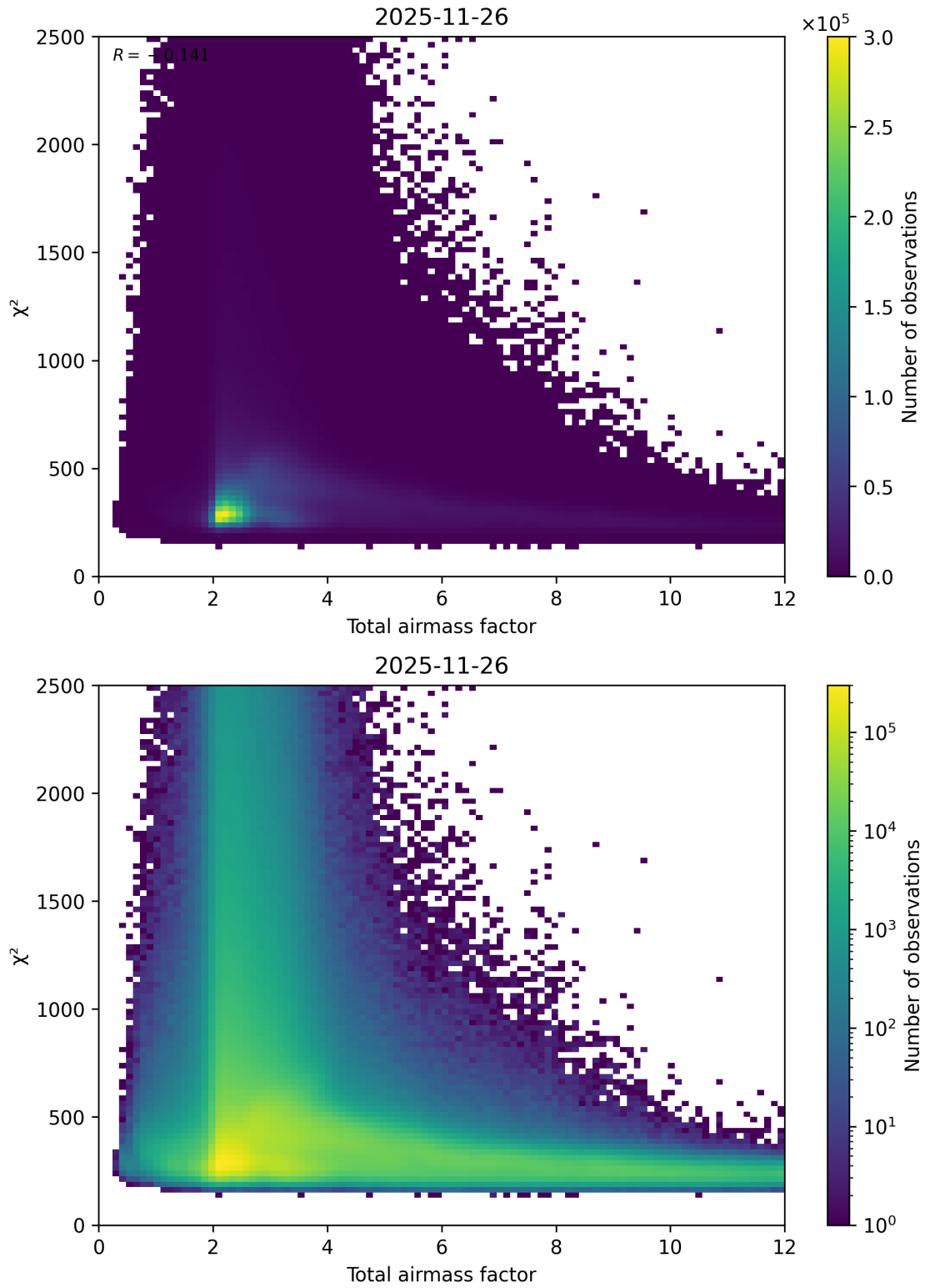
Figure 63: Scatter density plot of “Total airmass factor” against “ \chi^2 ” for 2025-11-25 to 2025-11-27.
