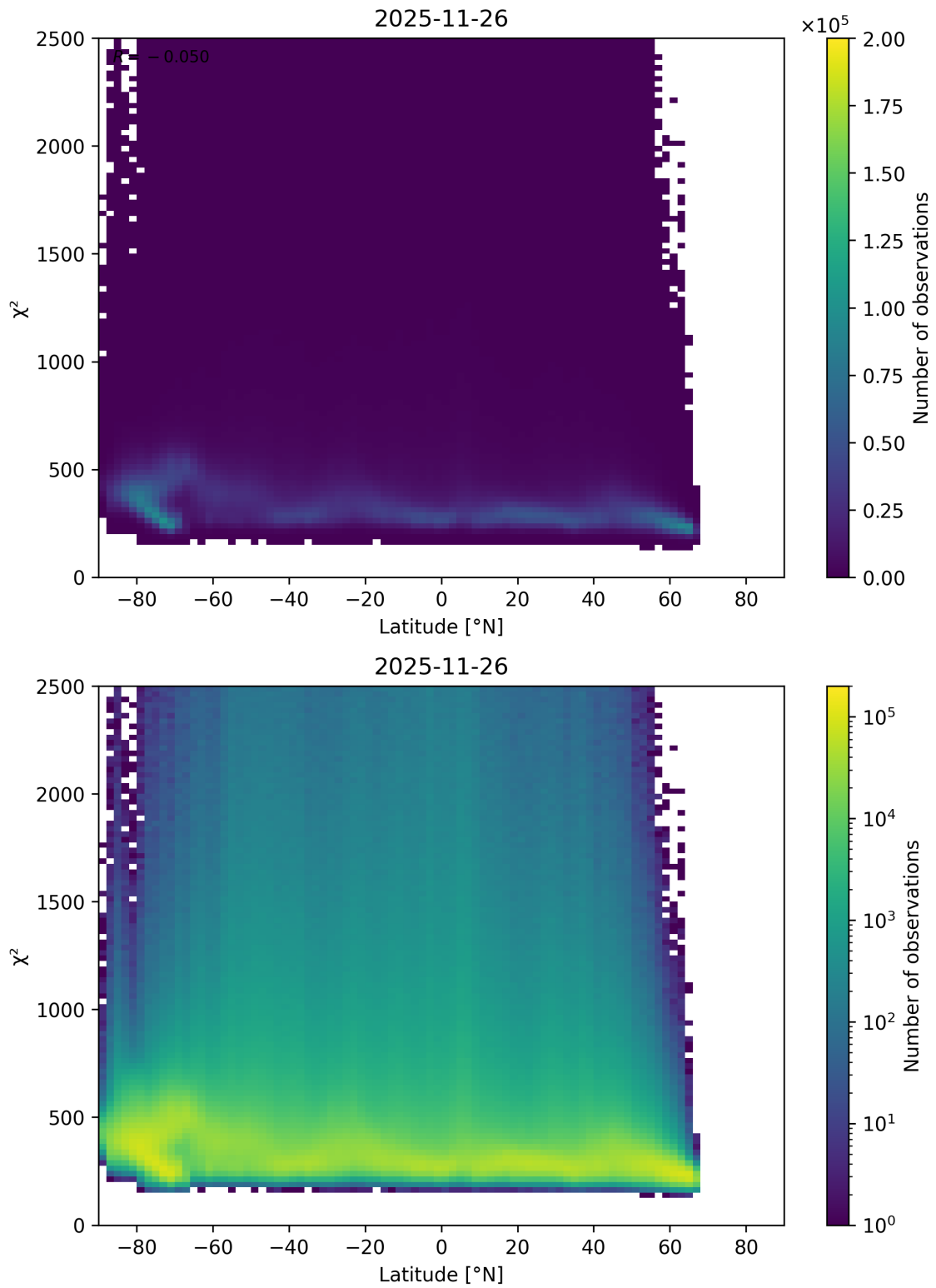
Figure 86: Scatter density plot of “Latitude” against “ \chi^2 ” for 2025-11-25 to 2025-11-27.
