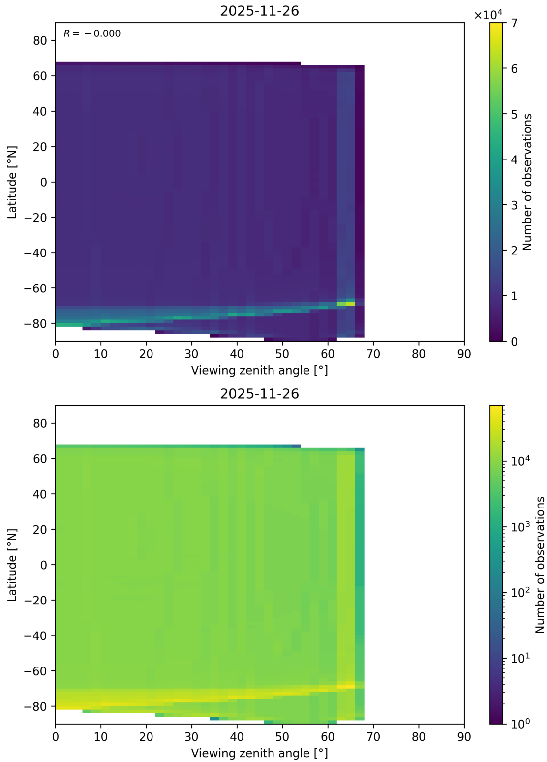
Figure 163: Scatter density plot of “Viewing zenith angle” against “Latitude” for 2025-11-25 to 2025-11-27.
