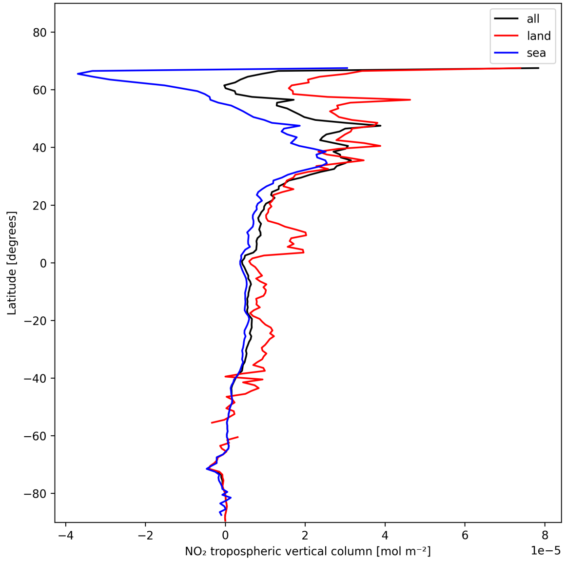
Figure 12: Zonal average of “NO 2 tropospheric vertical column” for 2025-11-25 to 2025-11-27.
