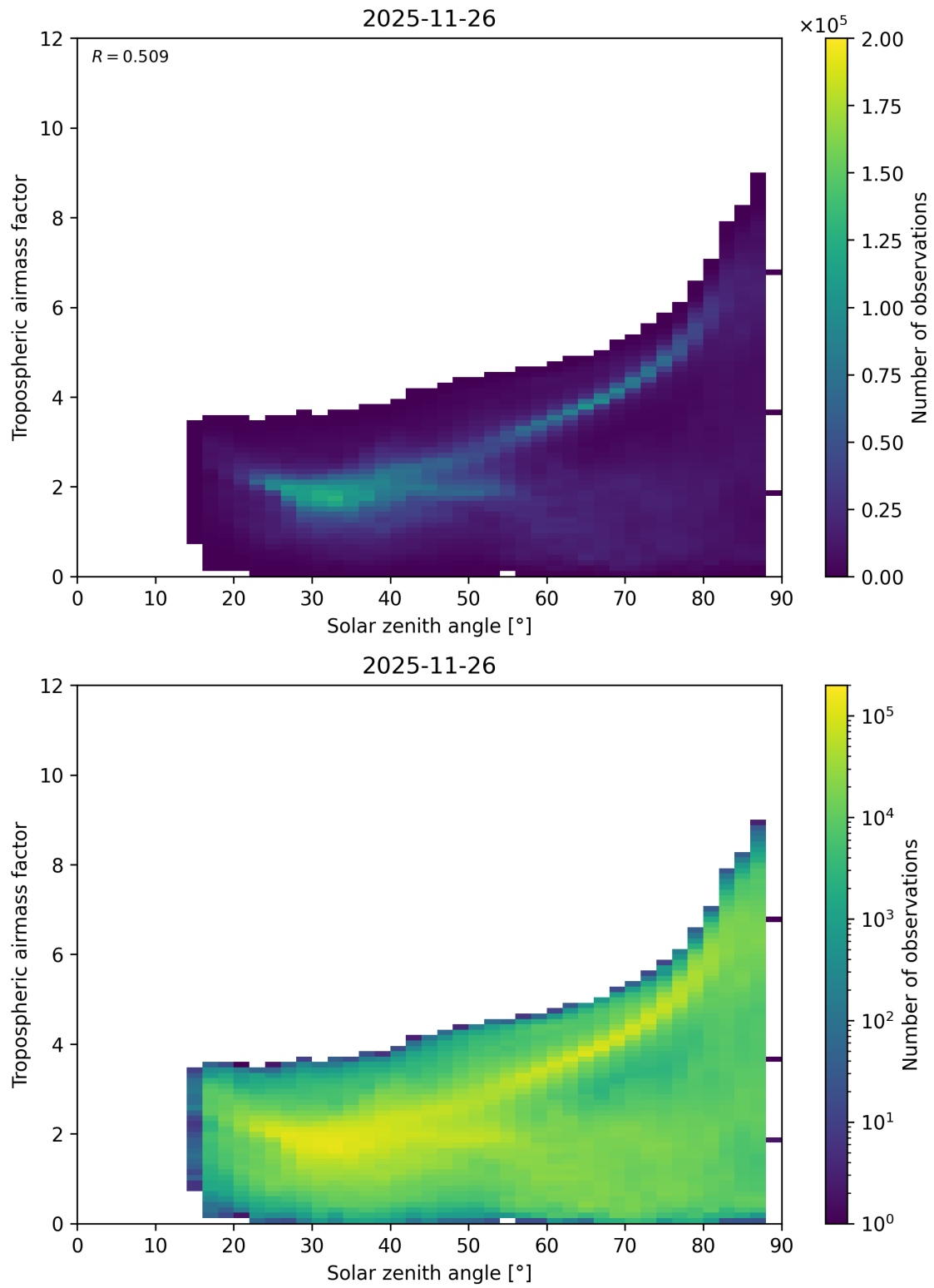
Figure 147: Scatter density plot of “Solar zenith angle” against “Tropospheric airmass factor” for 2025-11-25 to 2025-11-27.
