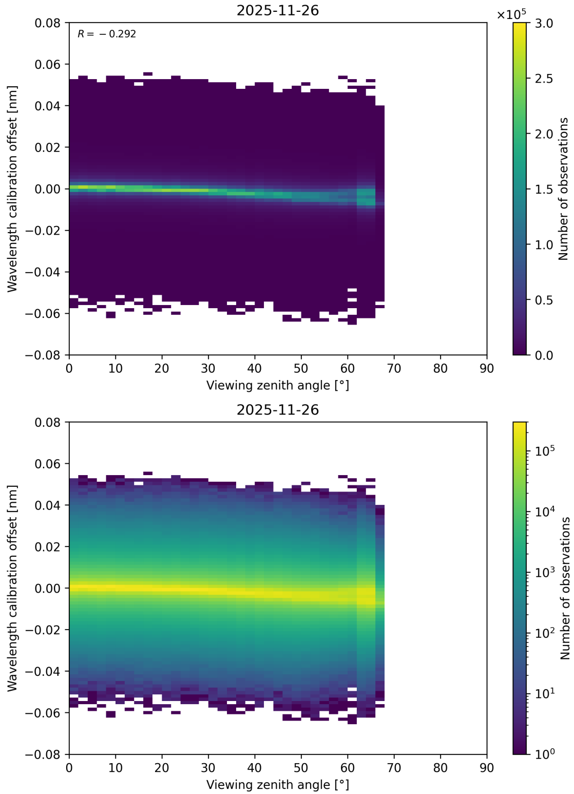
Figure 173: Scatter density plot of “Viewing zenith angle” against “Wavelength calibration offset” for 2025-11-25 to 2025-11-27.
