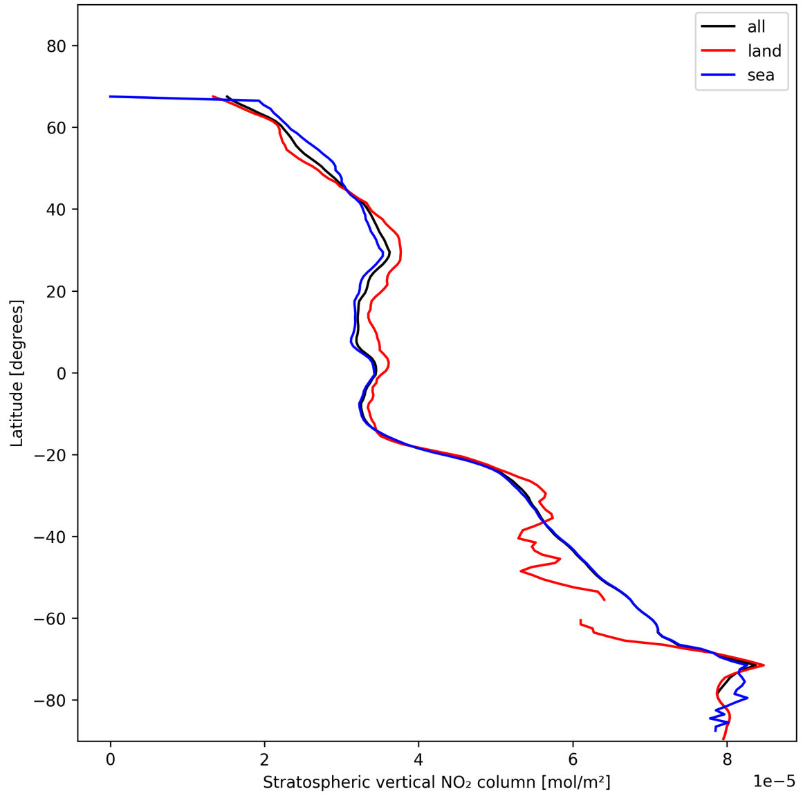
Figure 19: Zonal average of “Stratospheric vertical NO 2 column” for 2025-11-25 to 2025-11-27.
