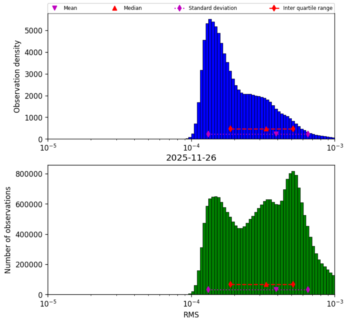
Figure 43: Histogram of “RMS” for 2025-11-25 to 2025-11-27
