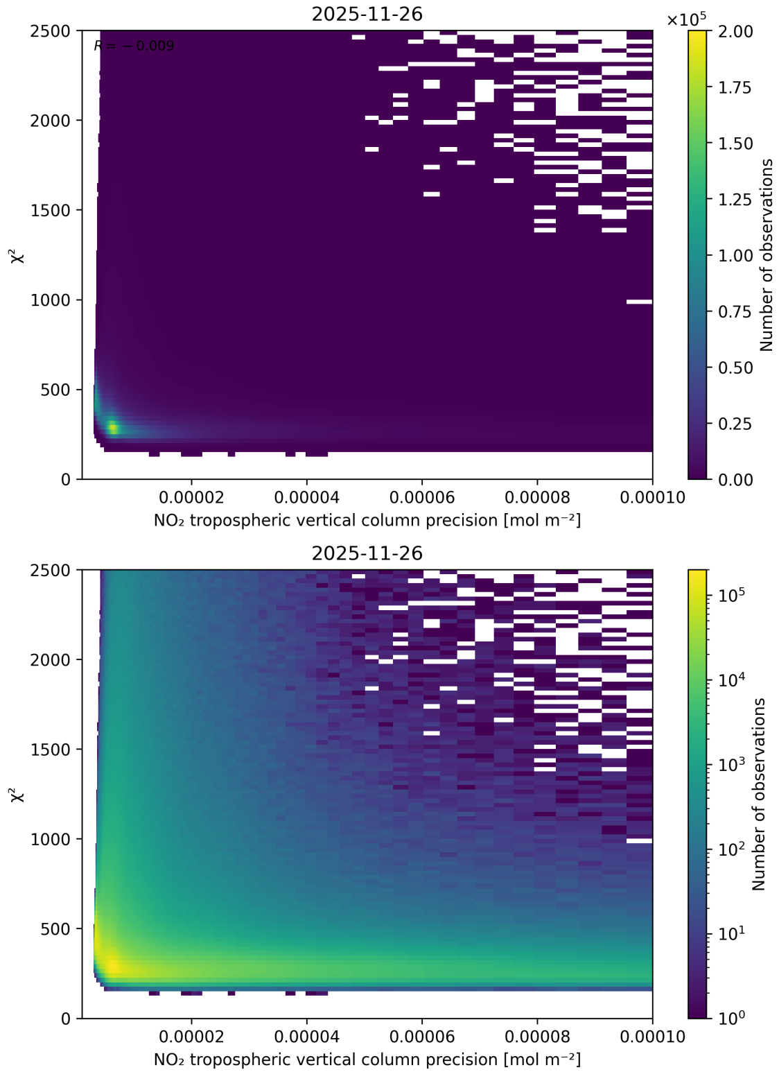
Figure 134: Scatter density plot of “NO 2 tropospheric vertical column precision” against “ \chi^2 ” for 2025-11-25 to 2025-11-27.
