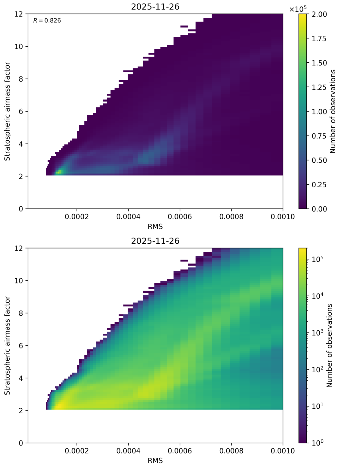
Figure 144: Scatter density plot of “RMS” against “Stratospheric airmass factor” for 2025-11-25 to 2025-11-27.
