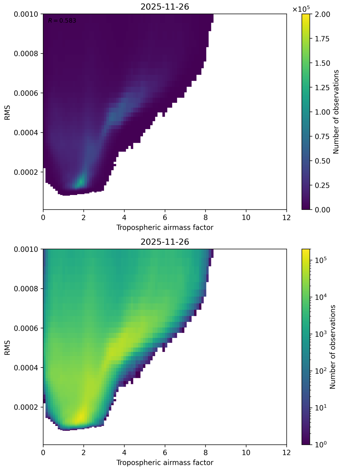
Figure 79: Scatter density plot of “Tropospheric airmass factor” against “RMS” for 2025-11-25 to 2025-11-27.
