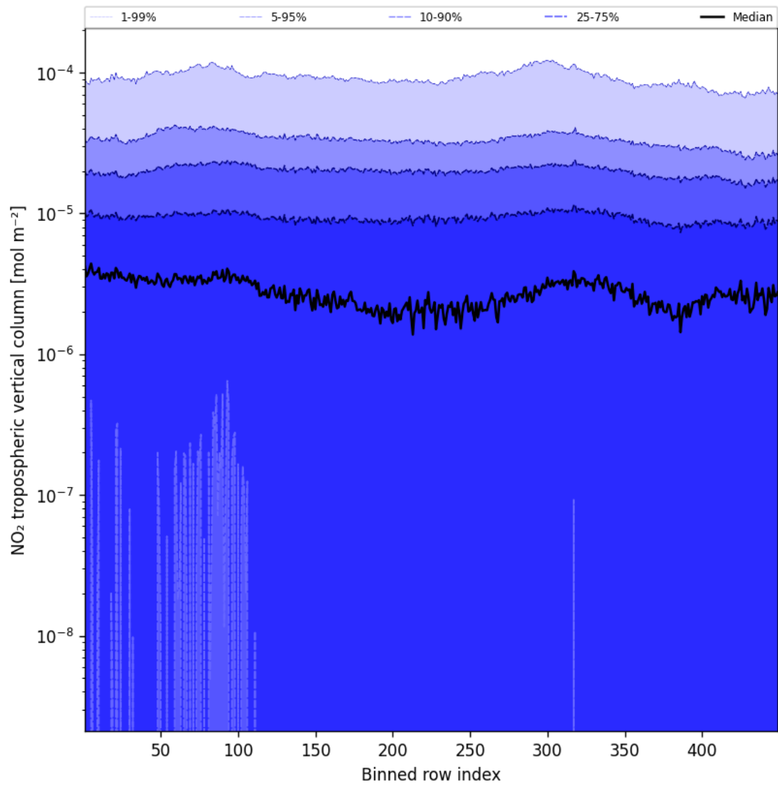
Figure 46: Along track statistics of “NO 2 tropospheric vertical column” for 2025-11-26 to 2025-11-28
