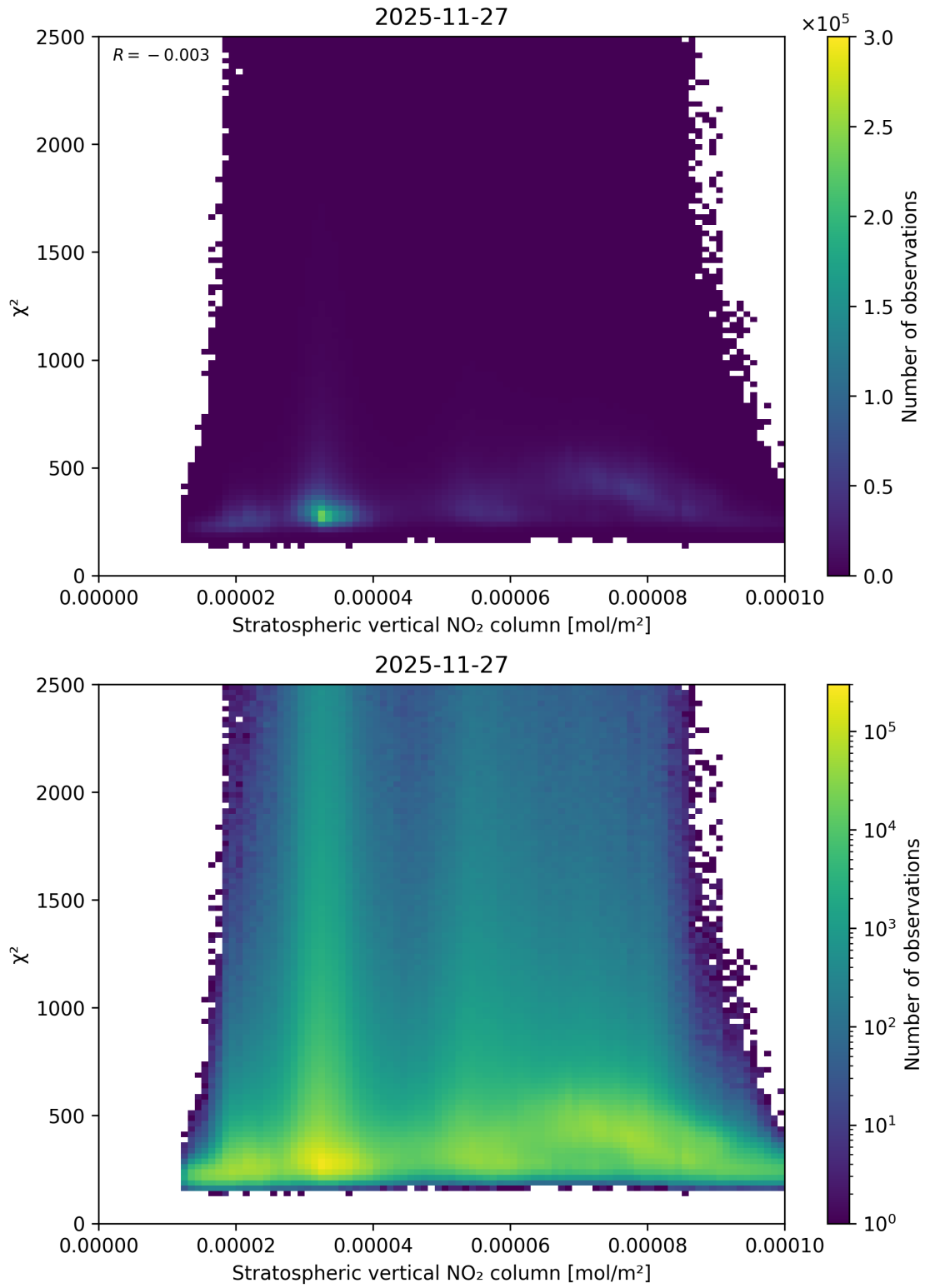
Figure 97: Scatter density plot of “Stratospheric vertical NO 2 column” against “ \chi^2 ” for 2025-11-26 to 2025-11-28.
