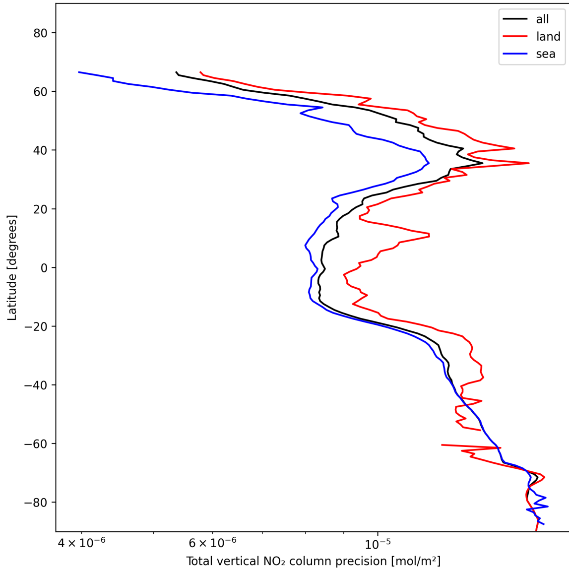
Figure 22: Zonal average of “Total vertical NO 2 column precision” for 2025-11-26 to 2025-11-28.
