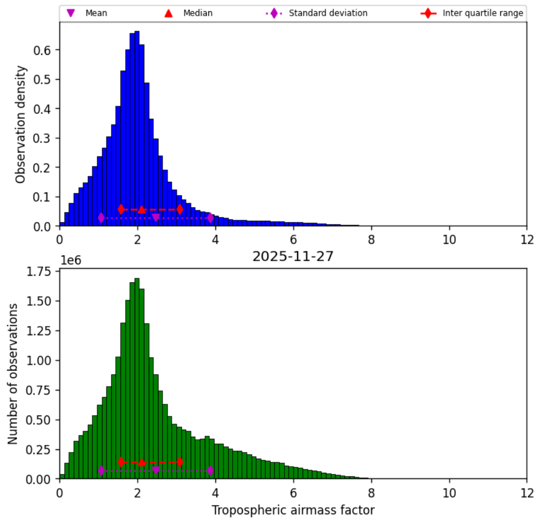
Figure 31: Histogram of “Tropospheric airmass factor” for 2025-11-26 to 2025-11-28
