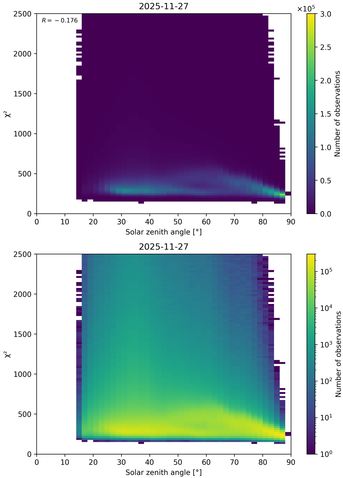
Figure 148: Scatter density plot of “Solar zenith angle” against “ \chi^2 ” for 2025-11-26 to 2025-11-28.
