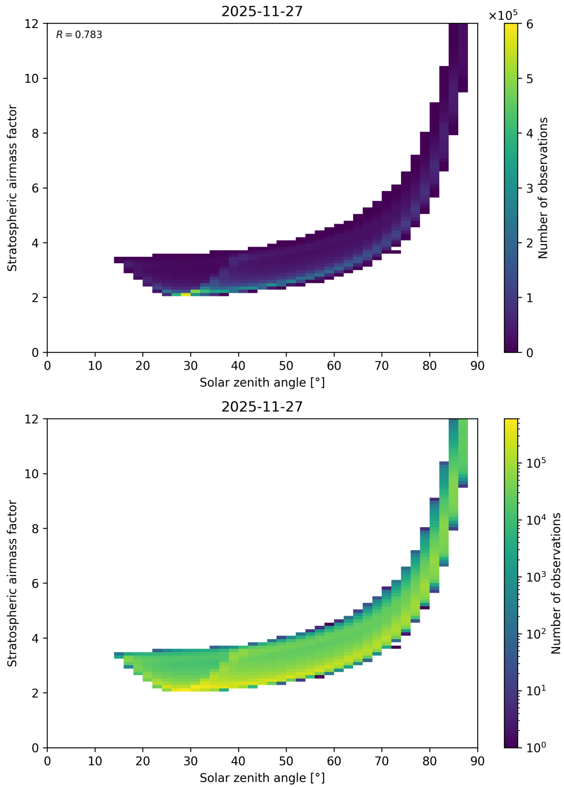
Figure 145: Scatter density plot of “Solar zenith angle” against “Stratospheric airmass factor” for 2025-11-26 to 2025-11-28.
