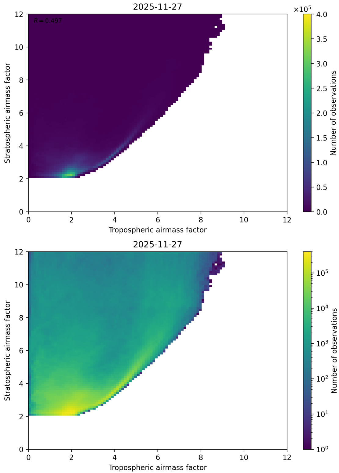
Figure 71: Scatter density plot of “Tropospheric airmass factor” against “Stratospheric airmass factor” for 2025-11-26 to 2025-11-28.
