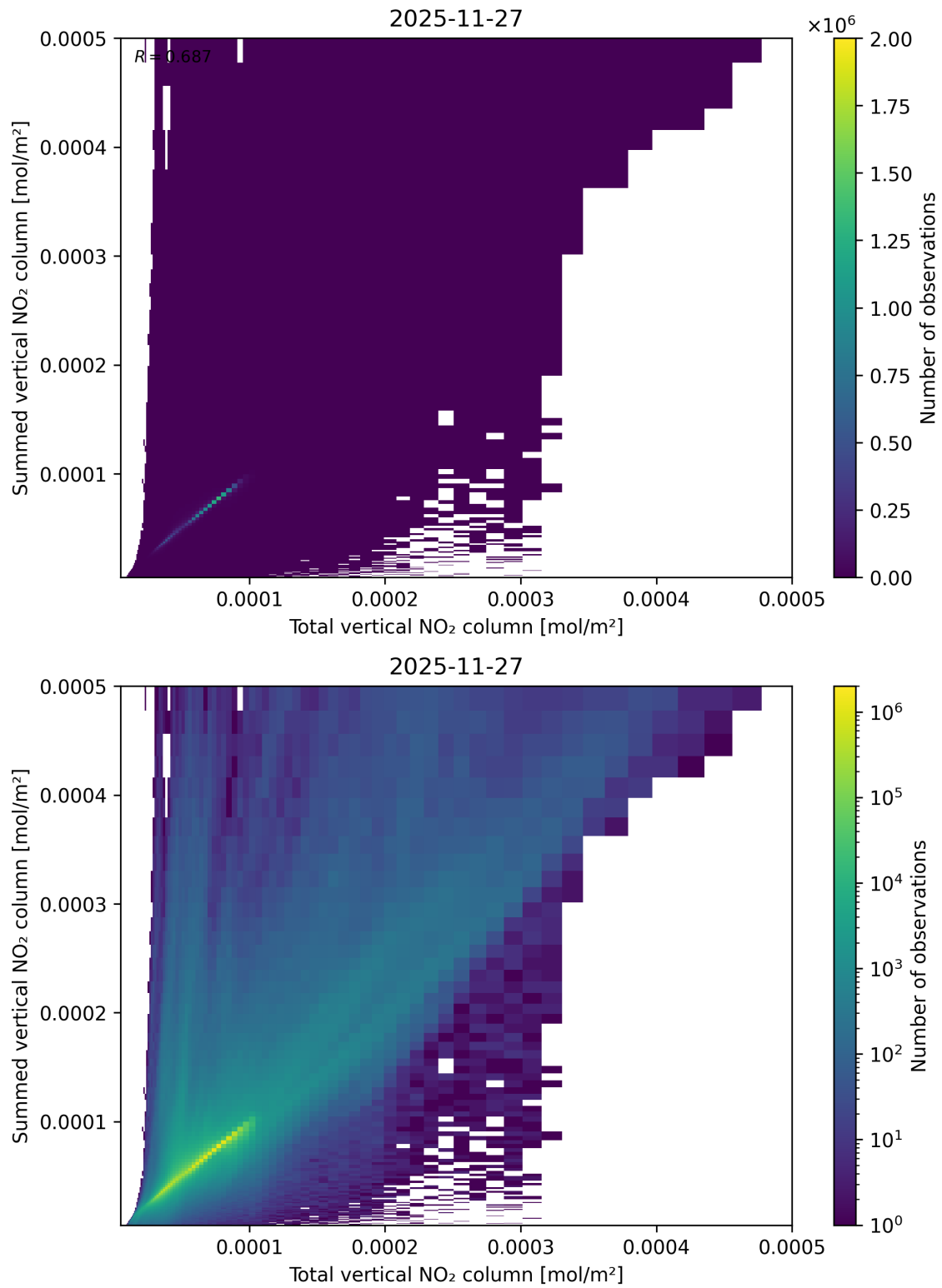
Figure 112: Scatter density plot of “Total vertical NO 2 column” against “Summed vertical NO 2 column” for 2025-11-26 to 2025-11-28.
