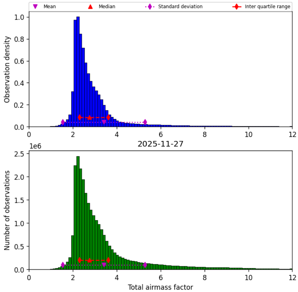
Figure 32: Histogram of “Total airmass factor” for 2025-11-26 to 2025-11-28
