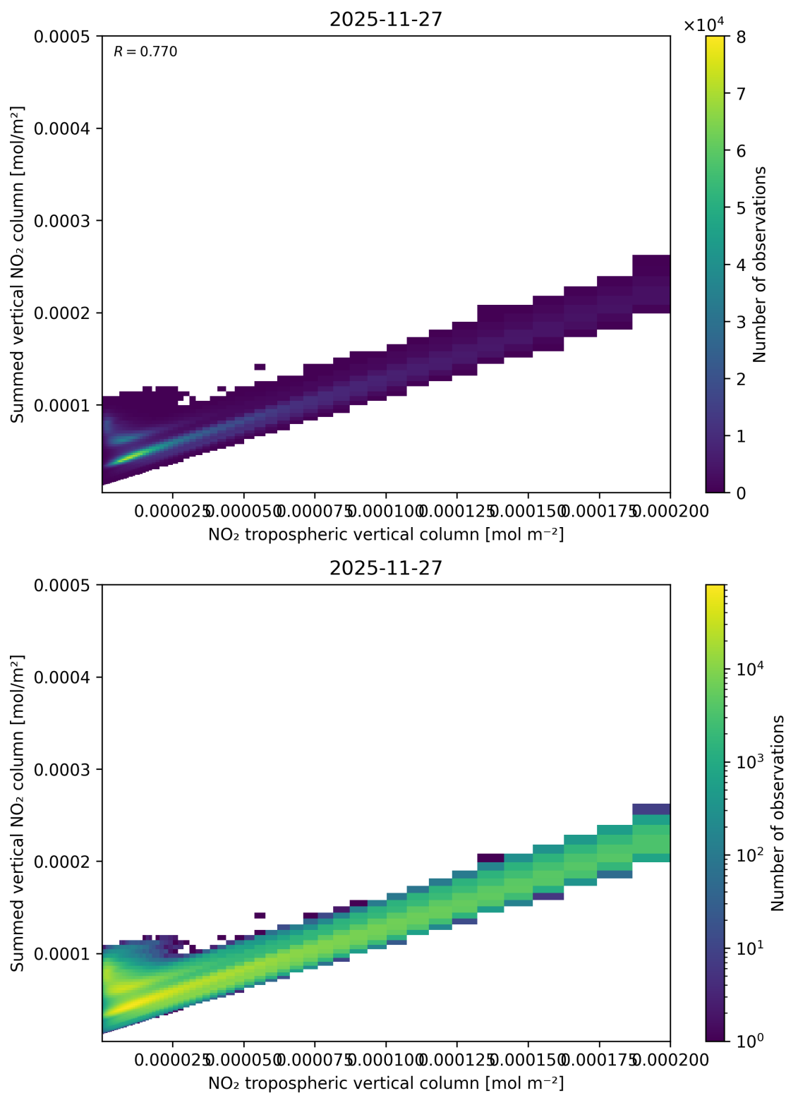
Figure 126: Scatter density plot of “NO 2 tropospheric vertical column” against “Summed vertical NO 2 column” for 2025-11-26 to 2025-11-28.
