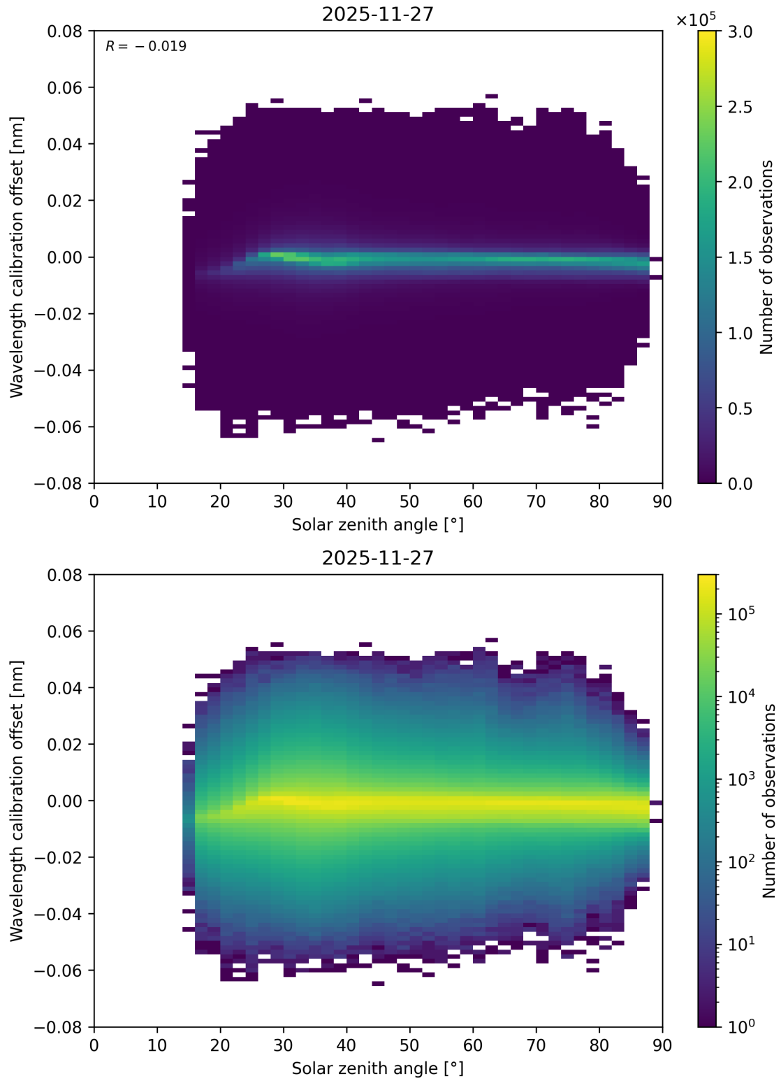
Figure 158: Scatter density plot of “Solar zenith angle” against “Wavelength calibration offset” for 2025-11-26 to 2025-11-28.
