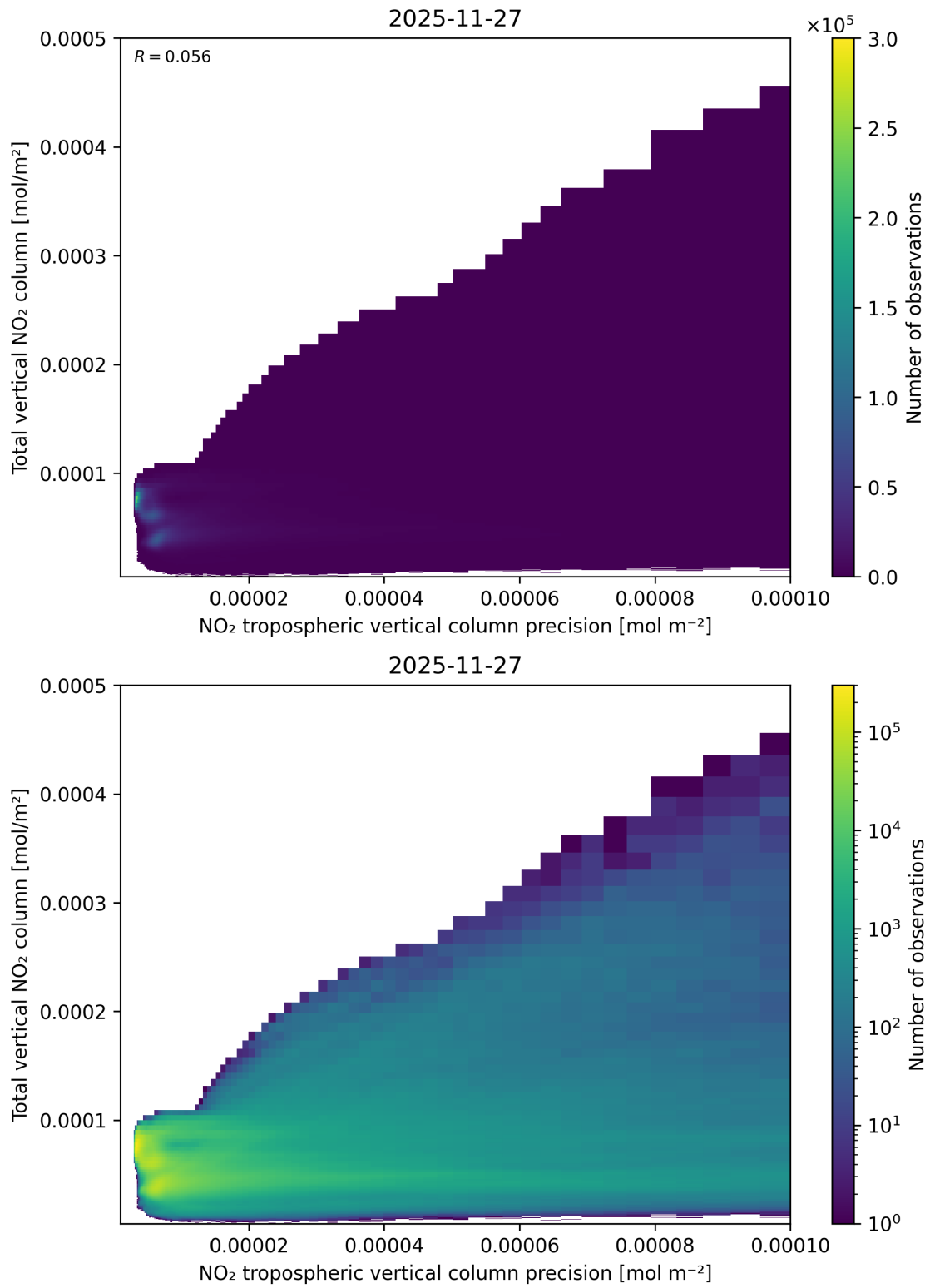
Figure 138: Scatter density plot of “NO 2 tropospheric vertical column precision” against “Total vertical NO 2 column” for 2025-11-26 to 2025-11-28.
