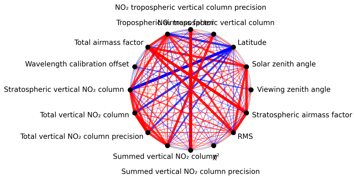
Figure 1: Map of correlation graph for 2025-11-26 to 2025-11-28.
