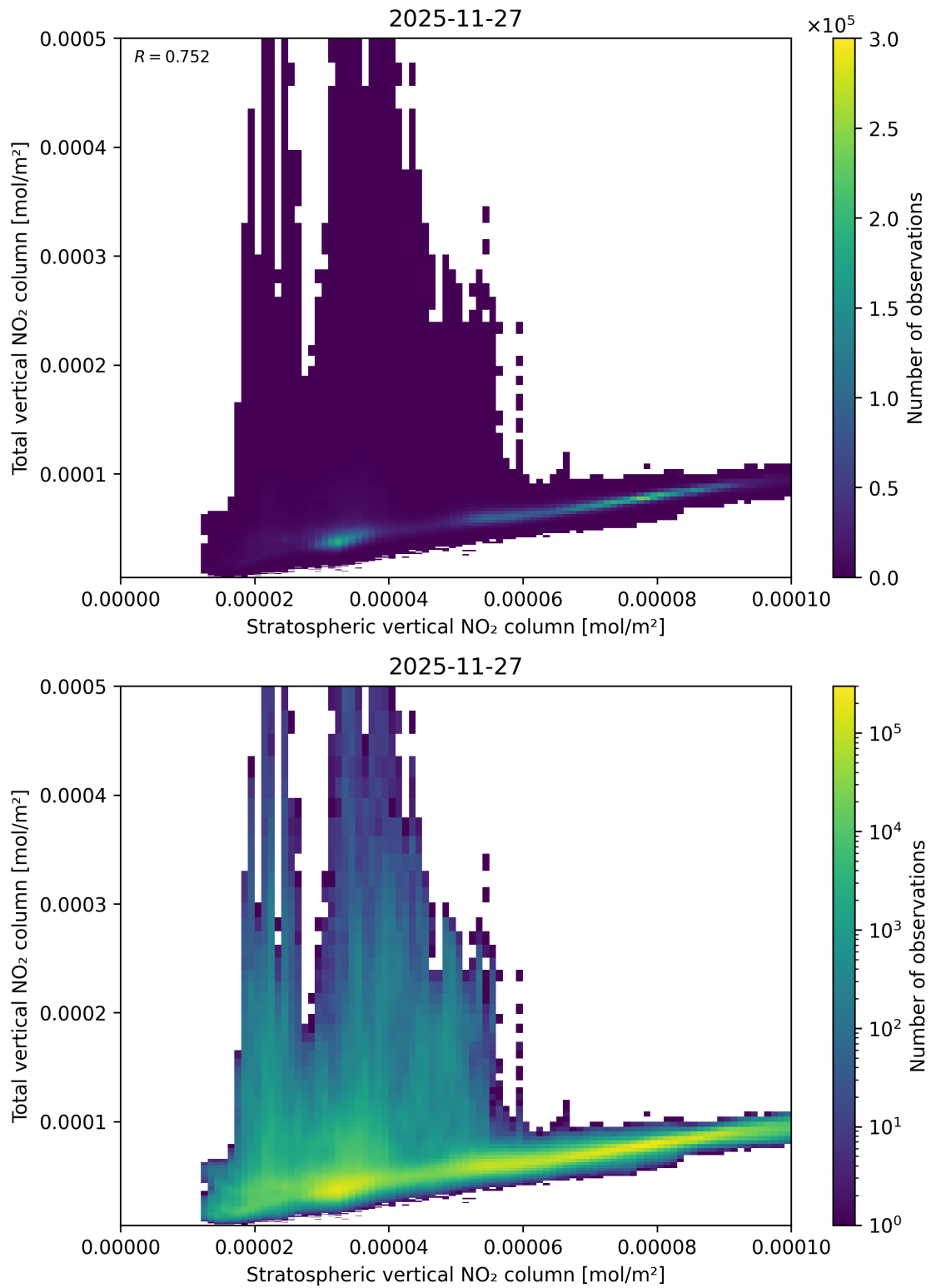
Figure 100: Scatter density plot of “Stratospheric vertical NO 2 column” against “Total vertical NO 2 column” for 2025-11-26 to 2025-11-28.
