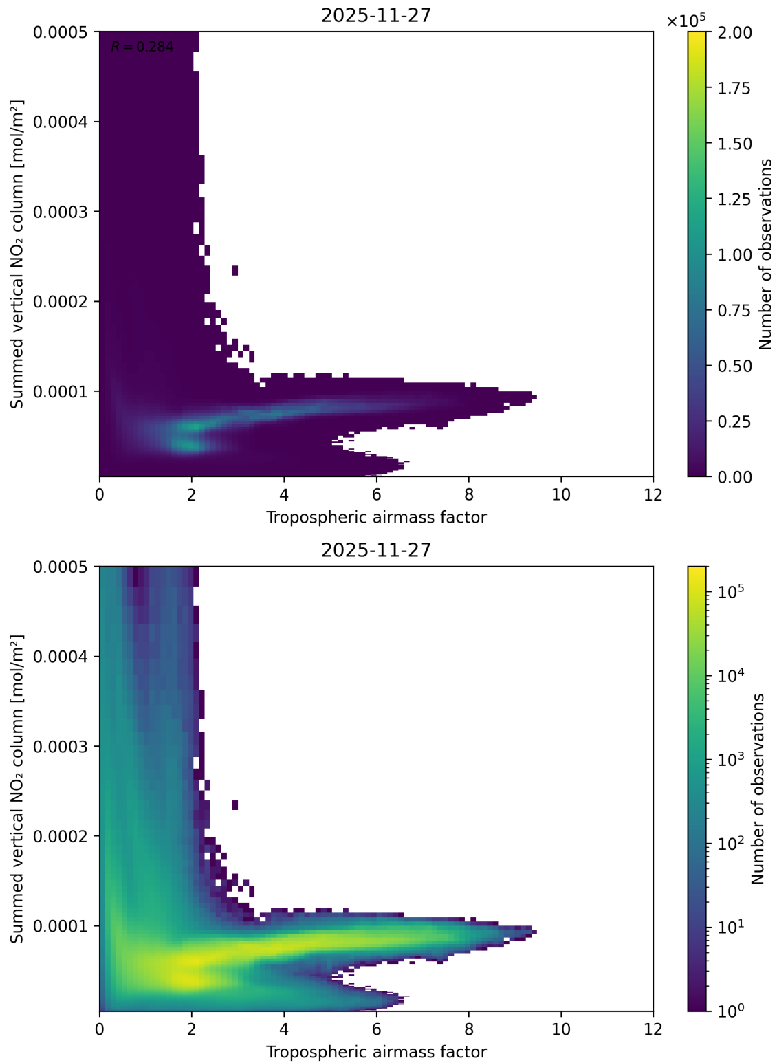
Figure 75: Scatter density plot of “Tropospheric air mass factor” against “Summed vertical NO 2 column” for 2025-11-26 to 2025-11-28.
