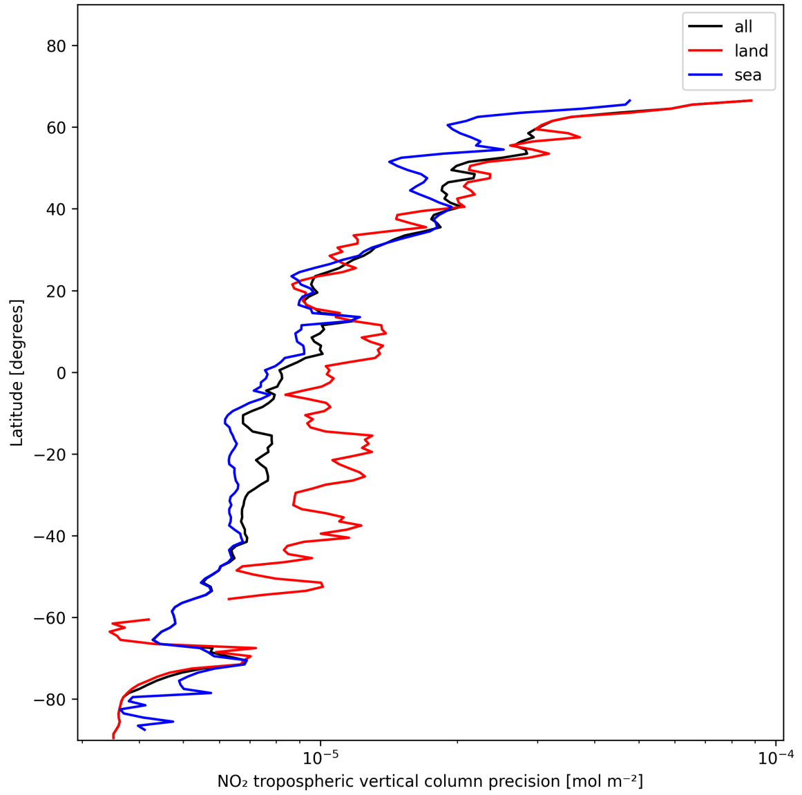
Figure 13: Zonal average of “NO 2 tropospheric vertical column precision” for 2025-11-26 to 2025-11-28.
