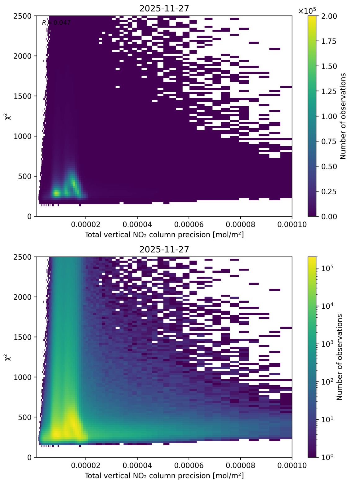
Figure 116: Scatter density plot of “Total vertical NO 2 column precision” against “ \chi^2 ” for 2025-11-26 to 2025-11-28.
