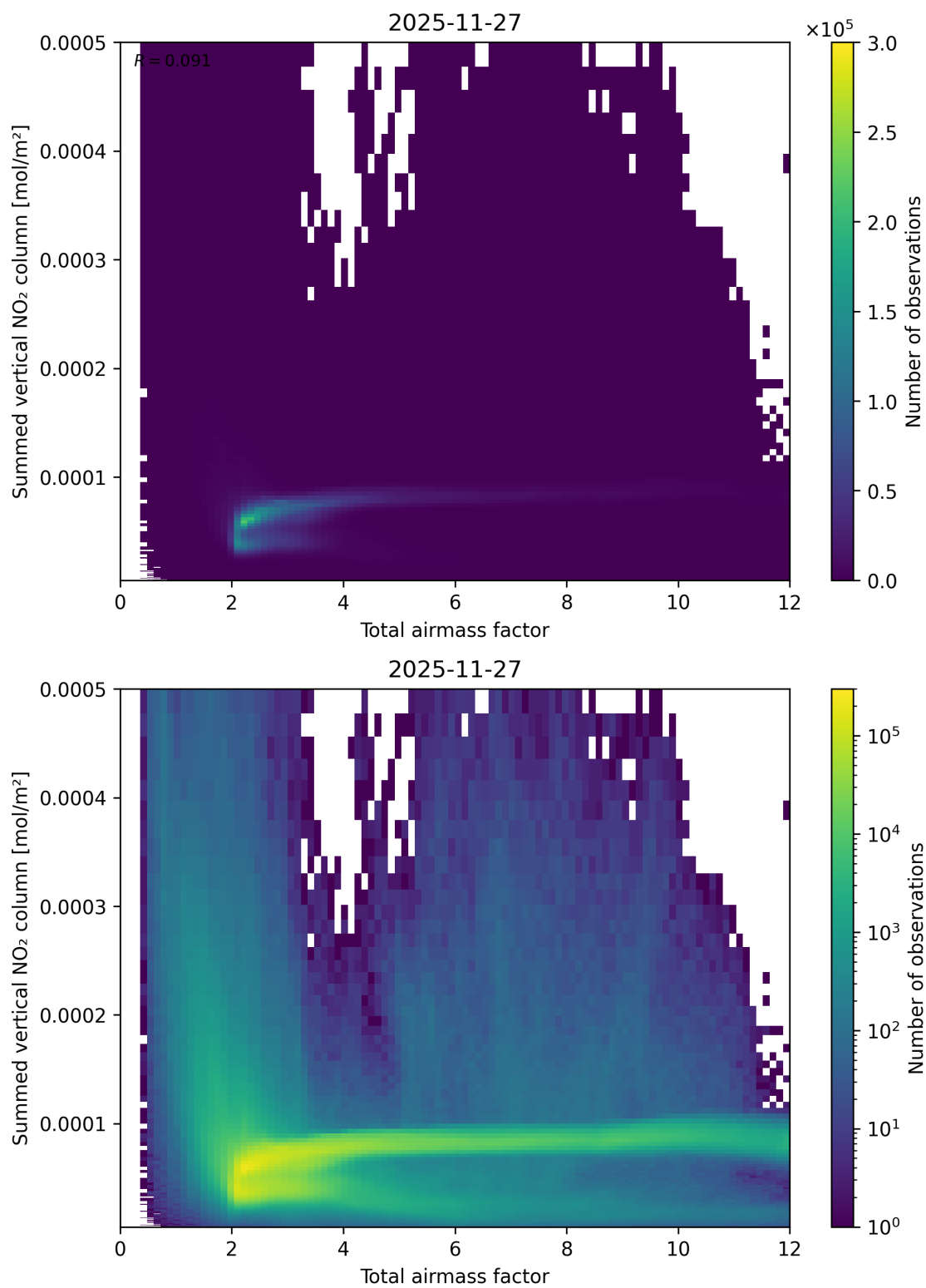
Figure 65: Scatter density plot of “Total airmass factor” against “Summed vertical NO 2 column” for 2025-11-26 to 2025-11-28.
