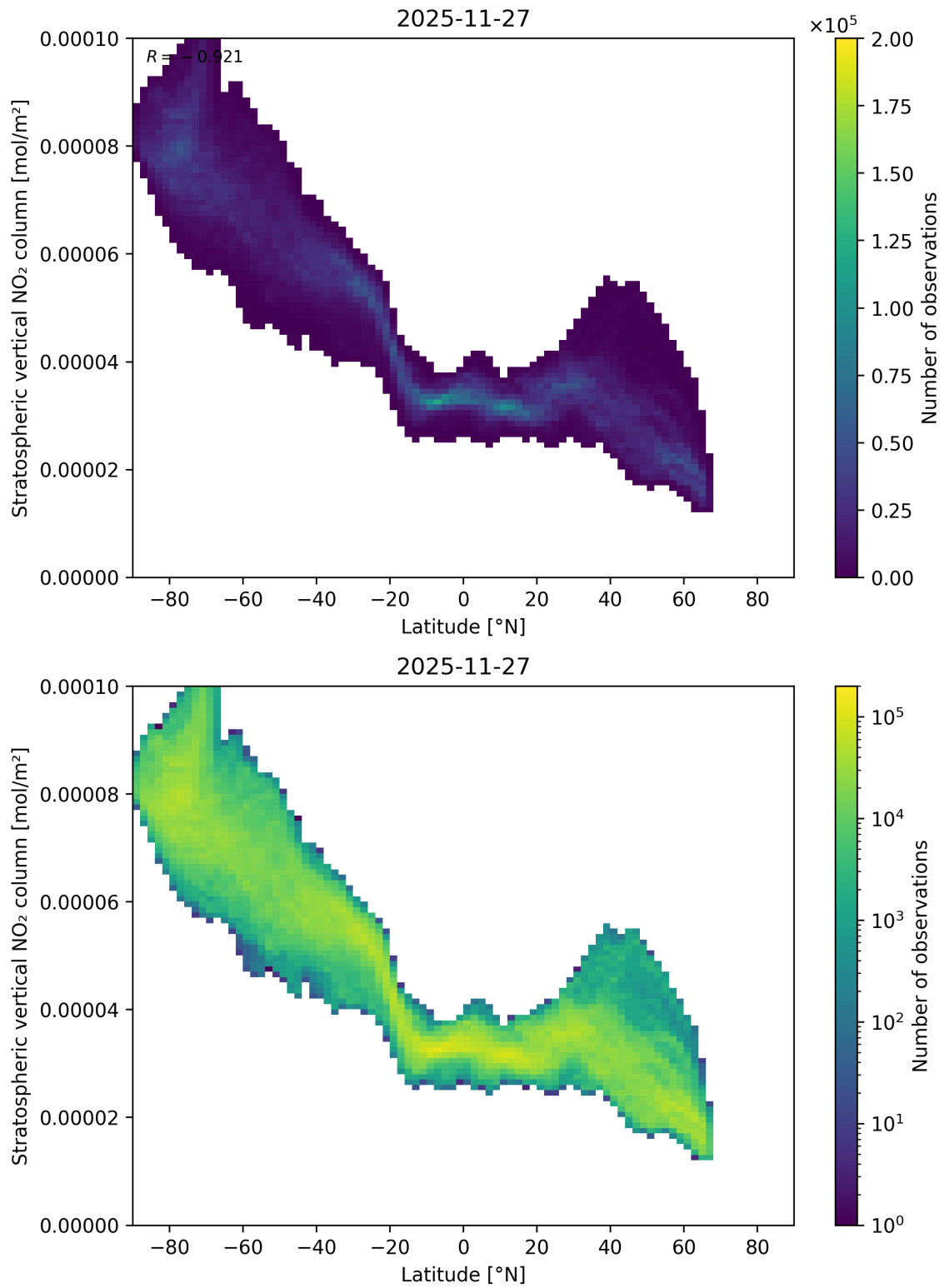
Figure 87: Scatter density plot of “Latitude” against “Stratospheric vertical NO 2 column” for 2025-11-26 to 2025-11-28.
