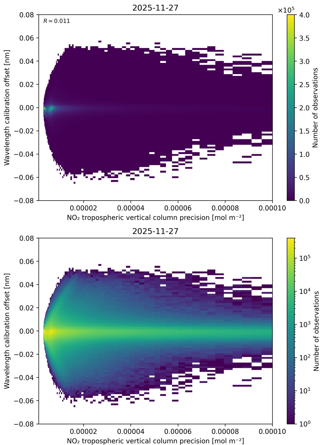
Figure 141: Scatter density plot of “NO 2 tropospheric vertical column precision” against “Wavelength calibration offset” for 2025-11-26 to 2025-11-28.
