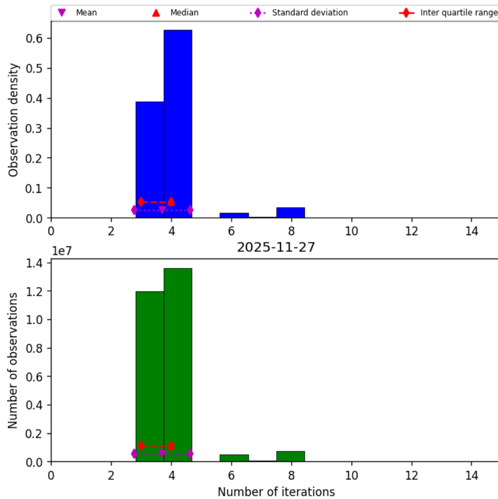
Figure 34: Histogram of “Number of iterations” for 2025-11-26 to 2025-11-28
