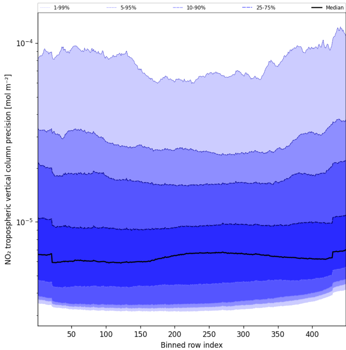
Figure 47: Along track statistics of “NO 2 tropospheric vertical column precision” for 2025-11-26 to 2025-11-28
