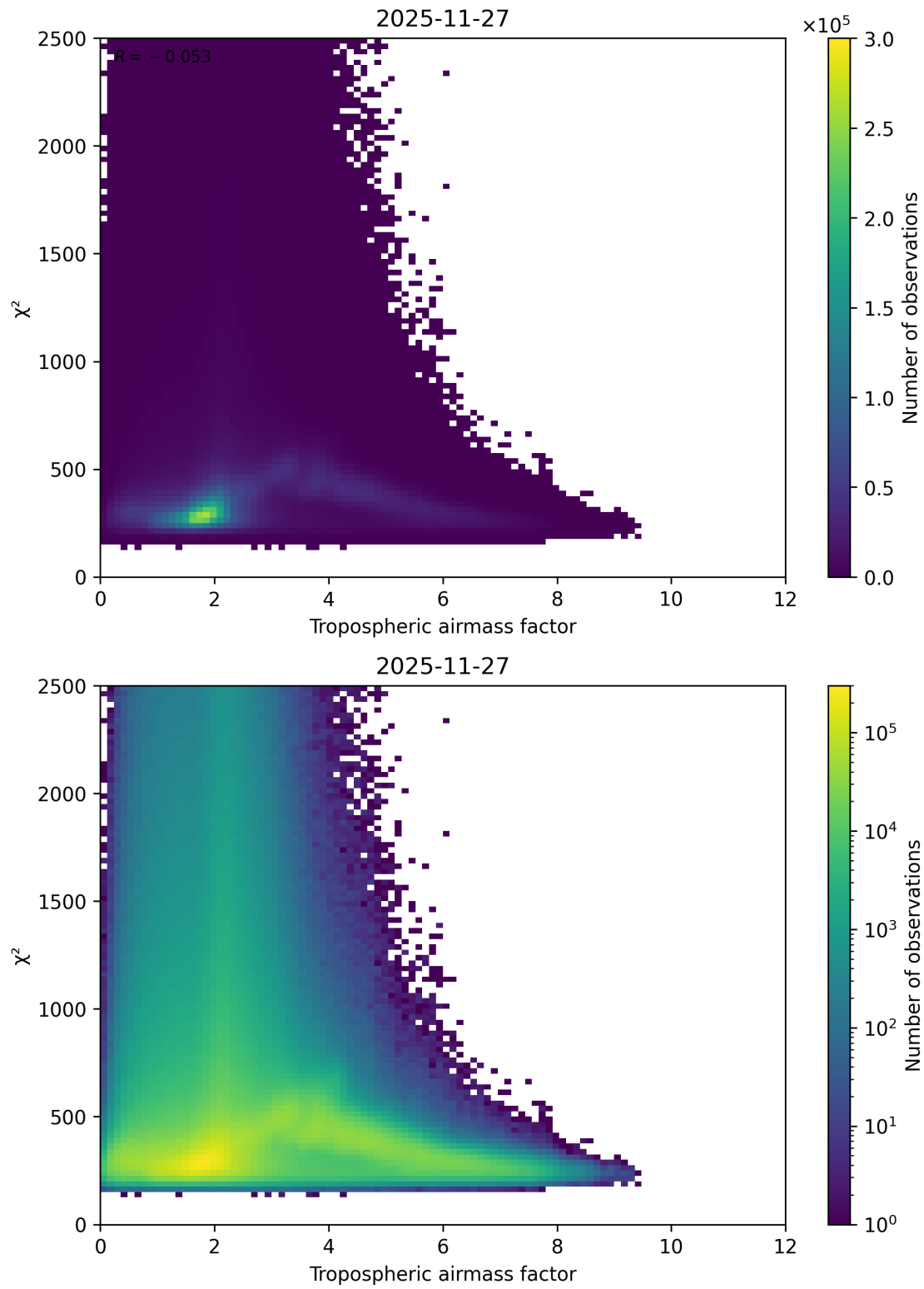
Figure 73: Scatter density plot of “Tropospheric airmass factor” against “ \chi^2 ” for 2025-11-26 to 2025-11-28.
