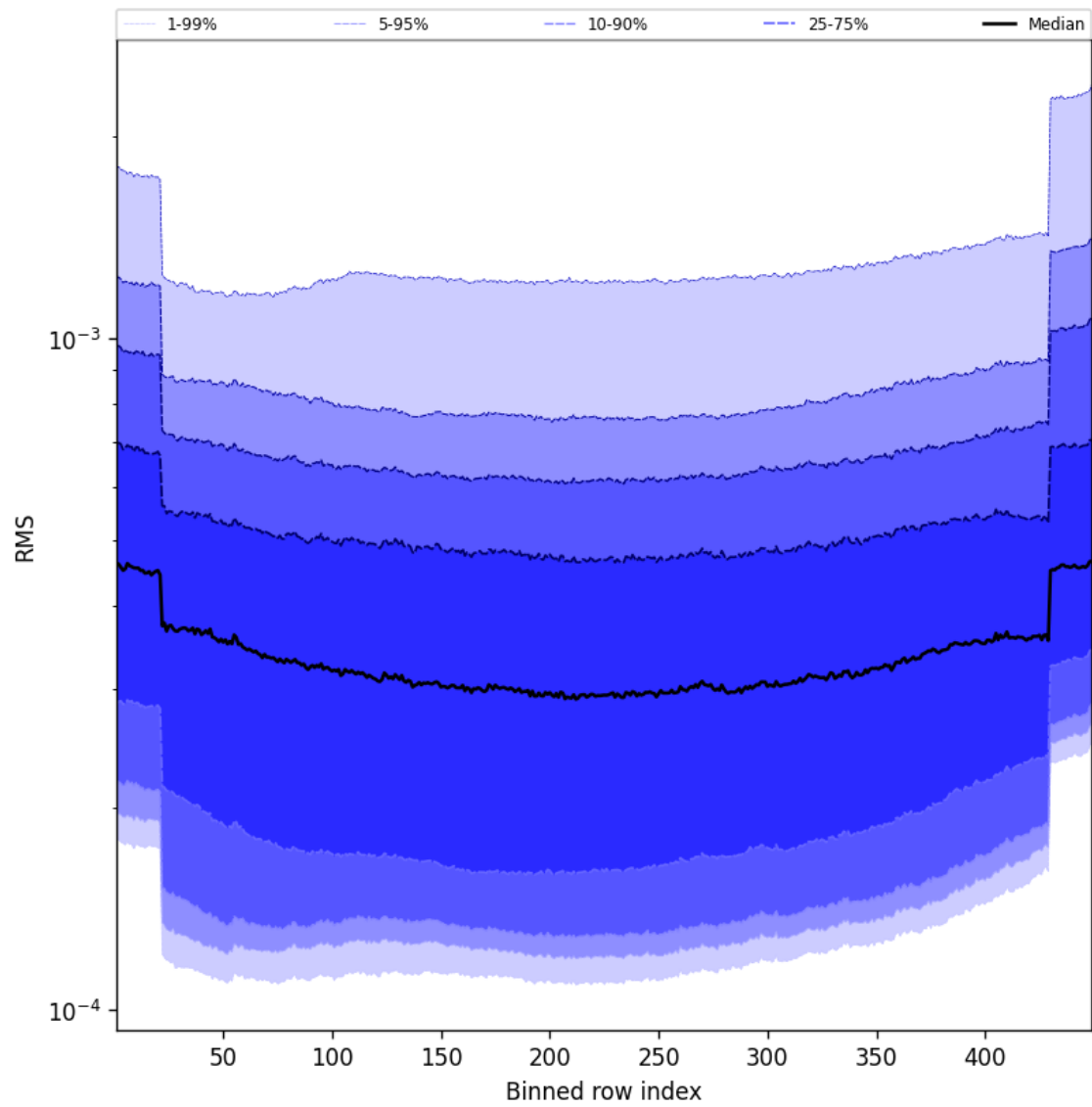
Figure 60: Along track statistics of “RMS” for 2025-11-26 to 2025-11-28
