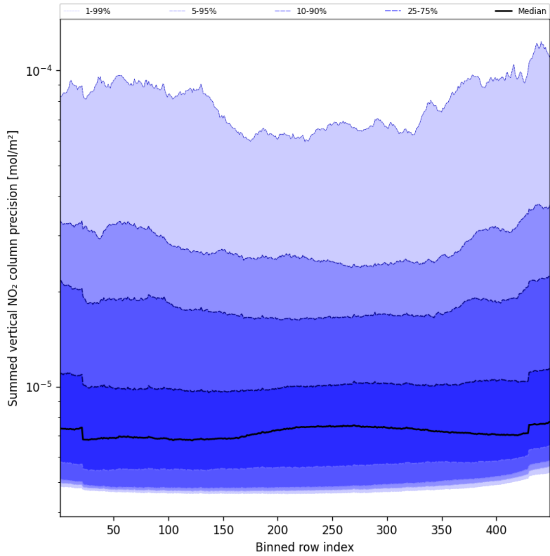
Figure 58: Along track statistics of “Summed vertical NO 2 column precision” for 2025-11-26 to 2025-11-28
