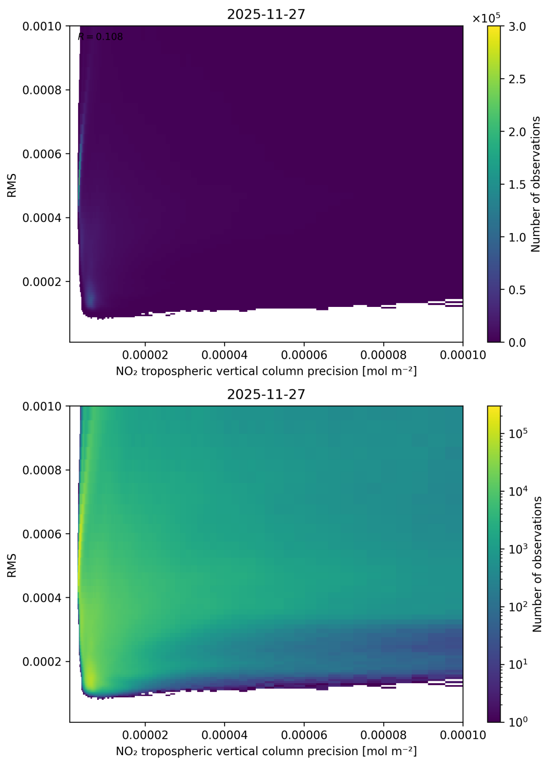
Figure 140: Scatter density plot of “NO 2 tropospheric vertical column precision” against “RMS” for 2025-11-26 to 2025-11-28.
