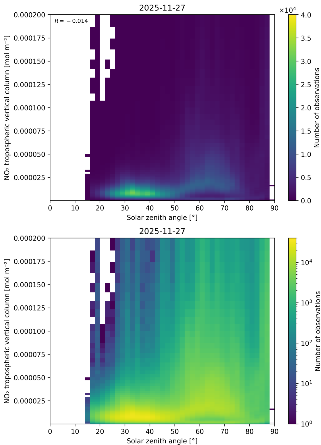
Figure 155: Scatter density plot of “Solar zenith angle” against “NO 2 tropospheric vertical column” for 2025-11-26 to 2025-11-28.
