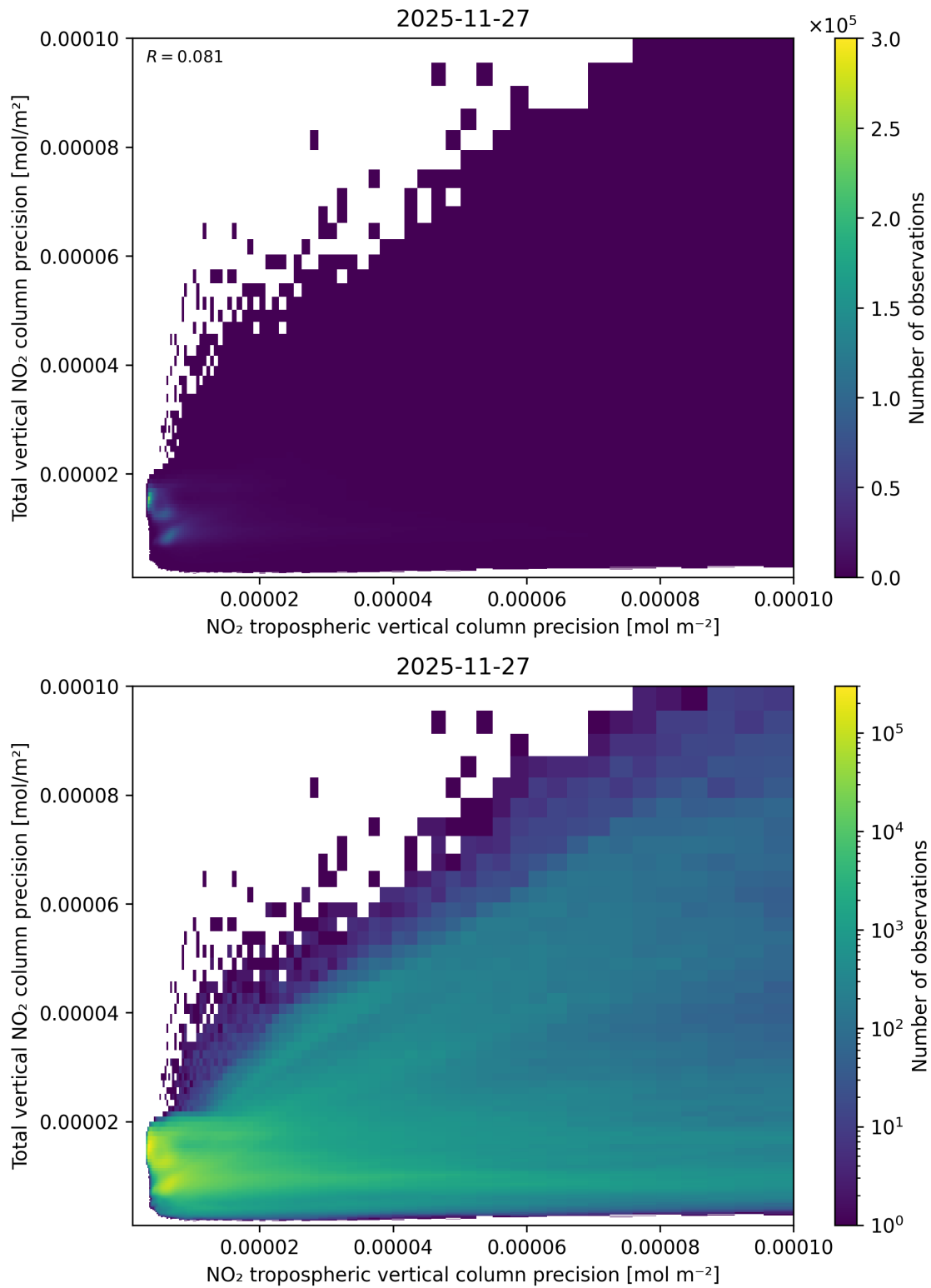
Figure 139: Scatter density plot of “NO 2 tropospheric vertical column precision” against “Total vertical NO 2 column precision” for 2025-11-26 to 2025-11-28.
