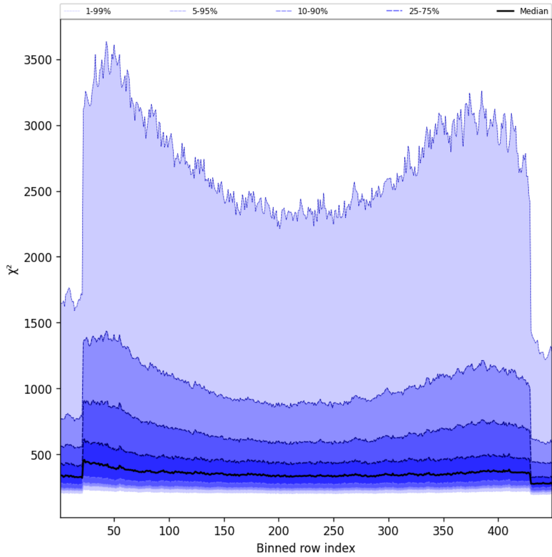
Figure 59: Along track statistics of “ \chi^2 ” for 2025-11-26 to 2025-11-28
