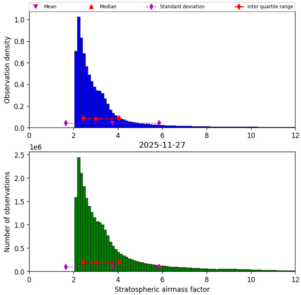
Figure 44: Histogram of “Stratospheric airmass factor” for 2025-11-26 to 2025-11-28
