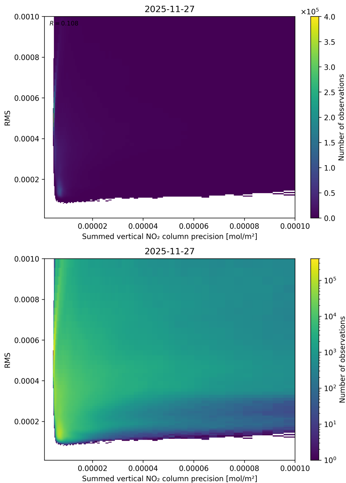
Figure 108: Scatter density plot of “Summed vertical NO 2 column precision” against “RMS” for 2025-11-26 to 2025-11-28.
