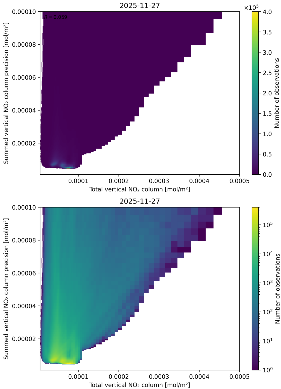
Figure 113: Scatter density plot of “Total vertical NO 2 column” against “Summed vertical NO 2 column precision” for 2025-11-26 to 2025-11-28.
