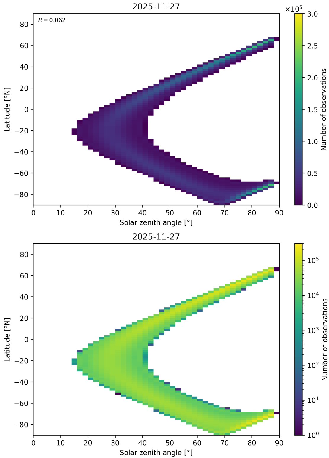
Figure 149: Scatter density plot of “Solar zenith angle” against “Latitude” for 2025-11-26 to 2025-11-28.
