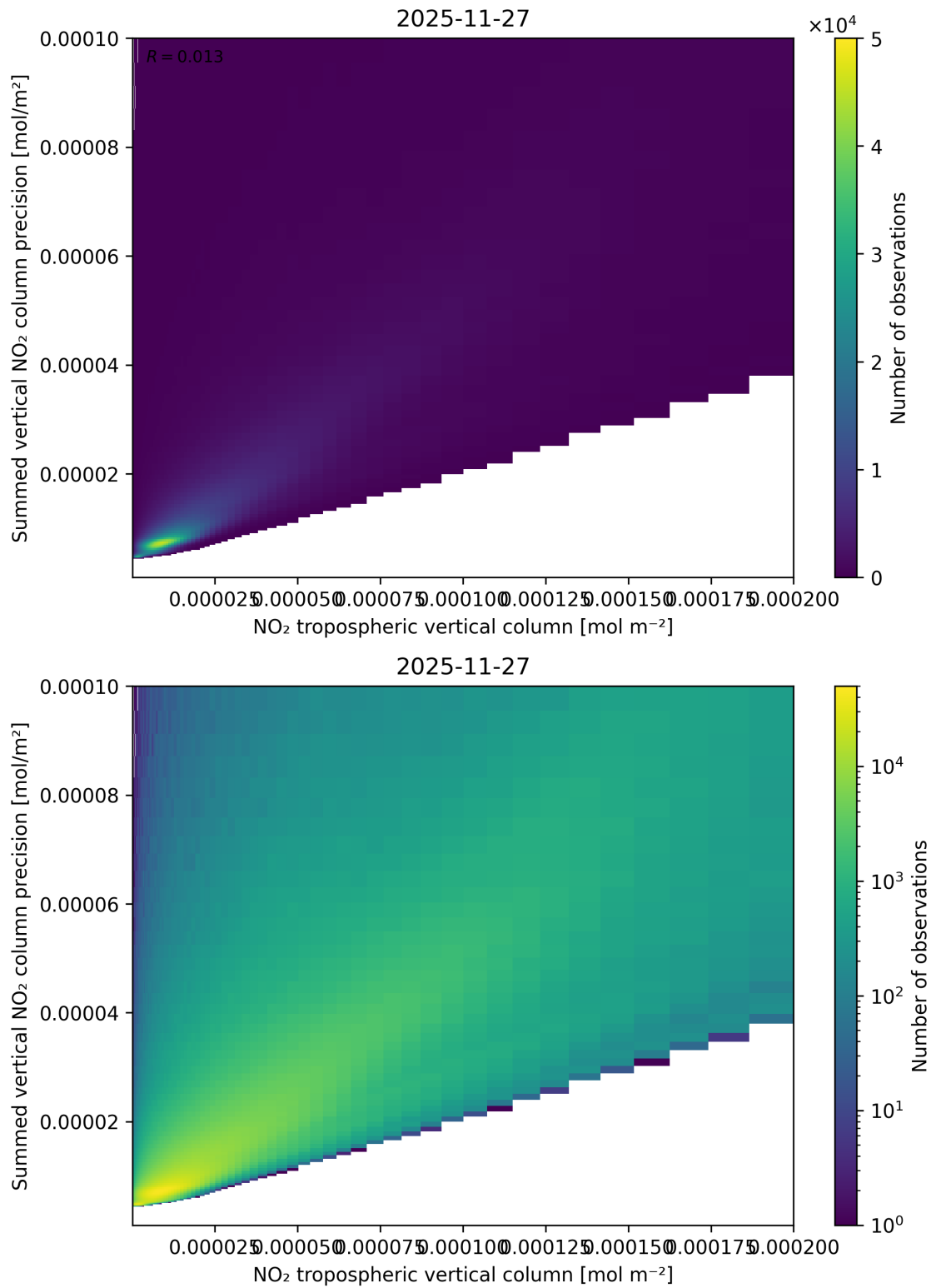
Figure 127: Scatter density plot of “NO 2 tropospheric vertical column” against “Summed vertical NO 2 column precision” for 2025-11-26 to 2025-11-28.
