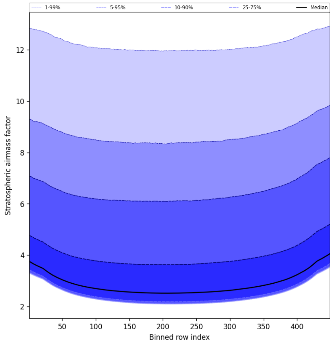
Figure 61: Along track statistics of “Stratospheric airmass factor” for 2025-11-26 to 2025-11-28
