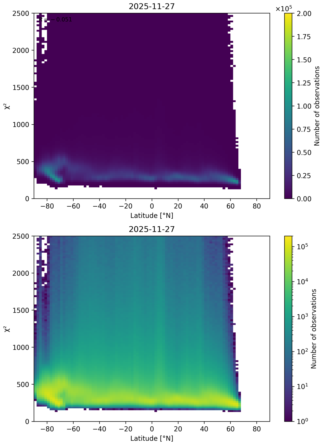
Figure 86: Scatter density plot of “Latitude” against “ \chi^2 ” for 2025-11-26 to 2025-11-28.
