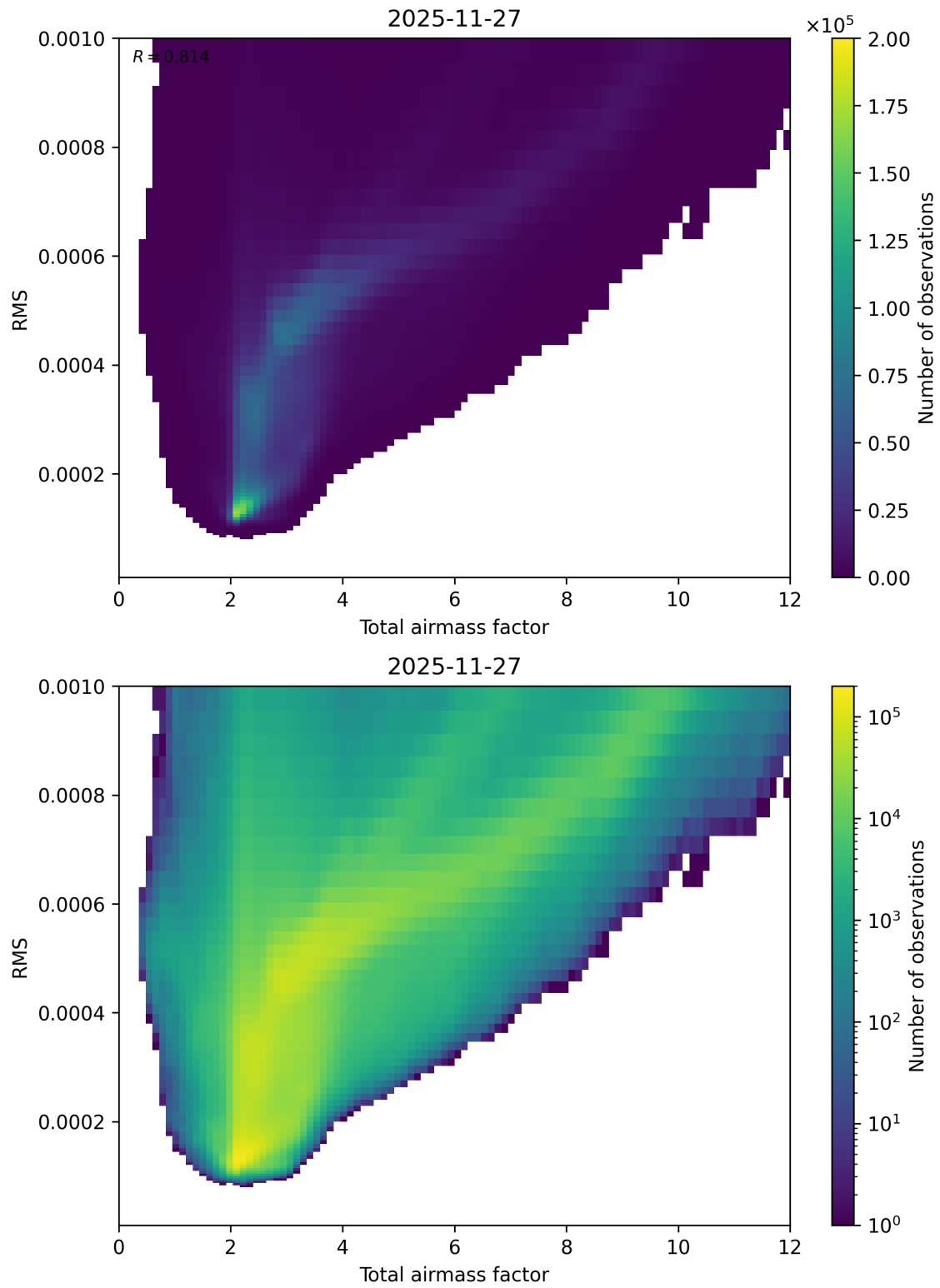
Figure 69: Scatter density plot of “Total airmass factor” against “RMS” for 2025-11-26 to 2025-11-28.
