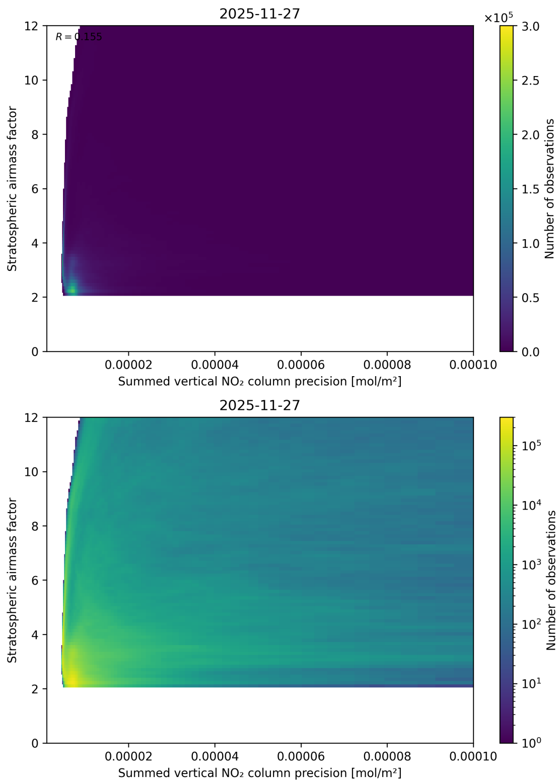
Figure 106: Scatter density plot of “Summed vertical NO 2 column precision” against “Stratospheric airmass factor” for 2025-11-26 to 2025-11-28.
