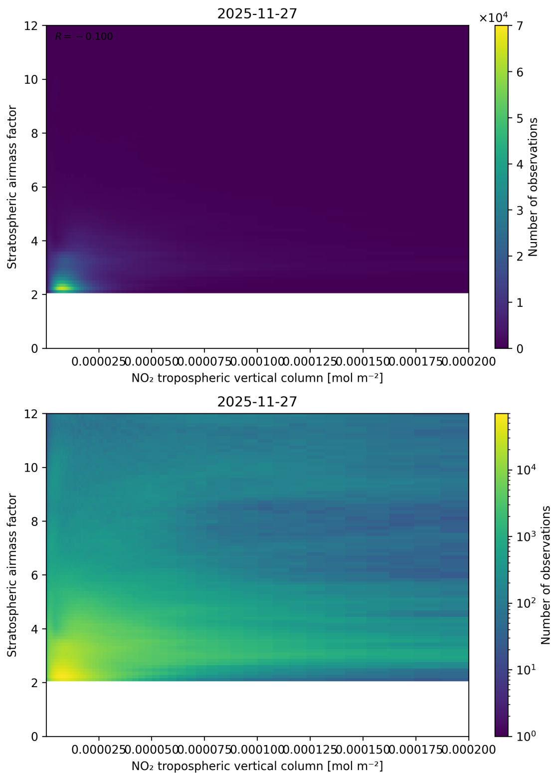
Figure 121: Scatter density plot of “NO 2 tropospheric vertical column” against “Stratospheric airmass factor” for 2025-11-26 to 2025-11-28.
