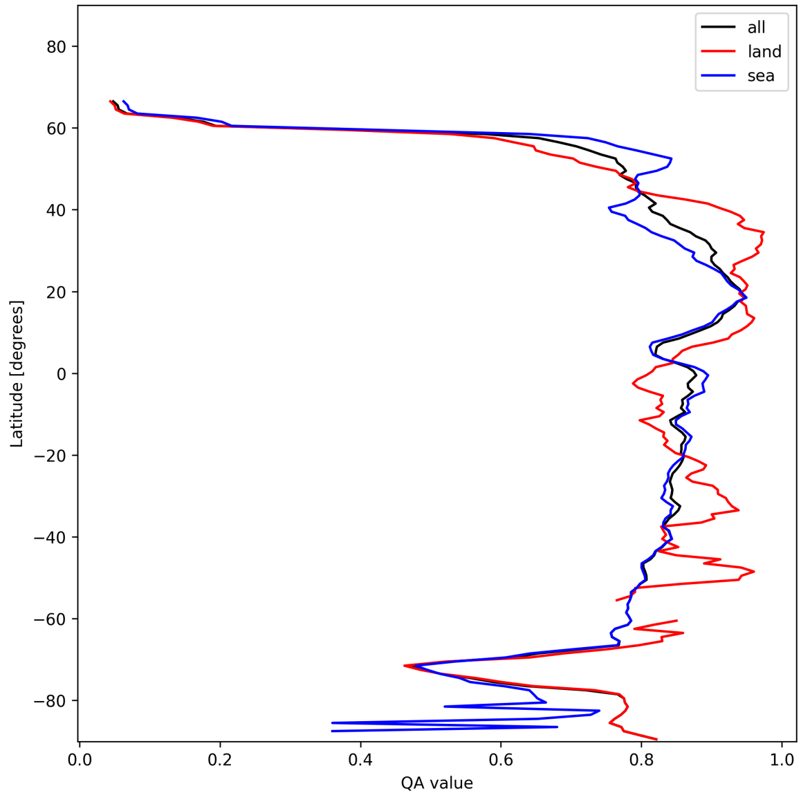
Figure 11: Zonal average of “QA value” for 2025-11-26 to 2025-11-28.
