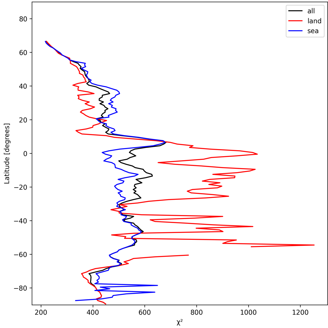
Figure 25: Zonal average of “ \chi^2 ” for 2025-11-26 to 2025-11-28.
