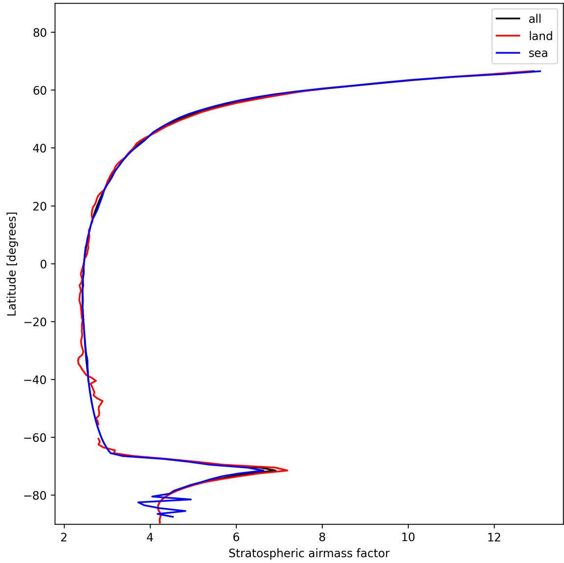
Figure 27: Zonal average of “Stratospheric air mass factor” for 2025-11-26 to 2025-11-28.
