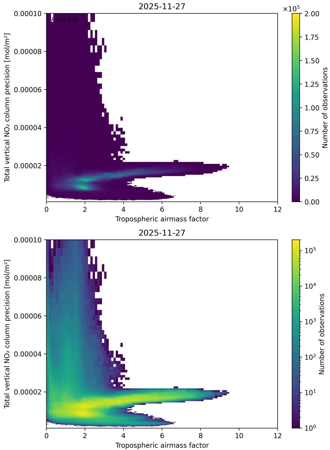
Figure 78: Scatter density plot of “Tropospheric air mass factor” against “Total vertical NO 2 column precision” for 2025-11-26 to 2025-11-28.
