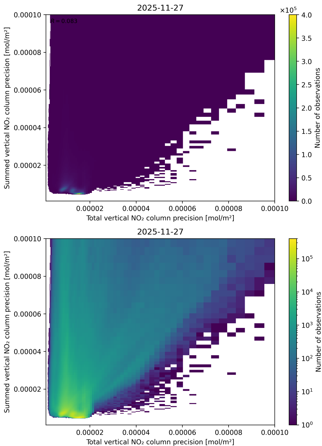
Figure 118: Scatter density plot of “Total vertical NO 2 column precision” against “Summed vertical NO 2 column precision” for 2025-11-26 to 2025-11-28.
