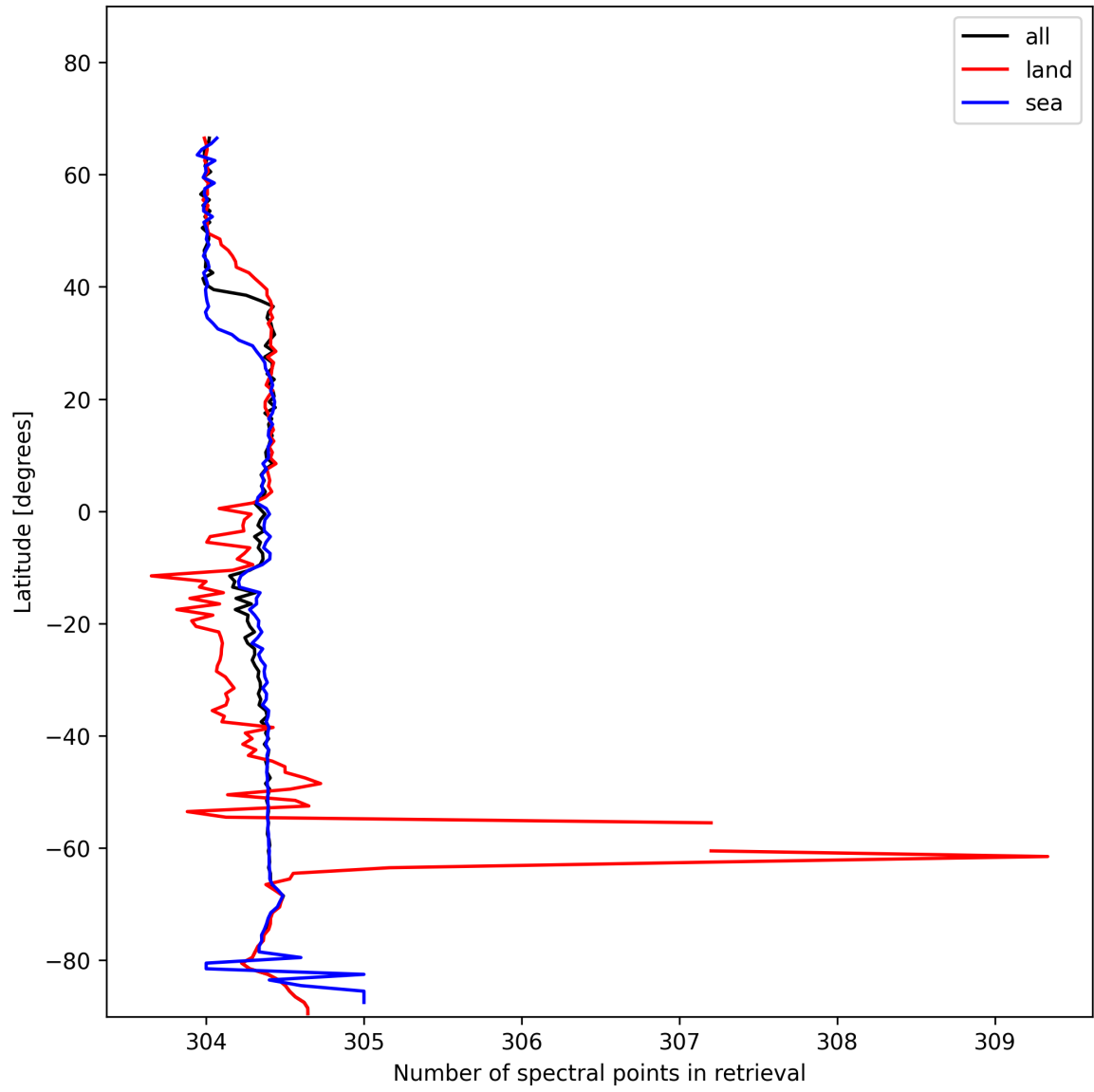
Figure 16: Zonal average of “Number of spectral points in retrieval” for 2025-11-26 to 2025-11-28.
