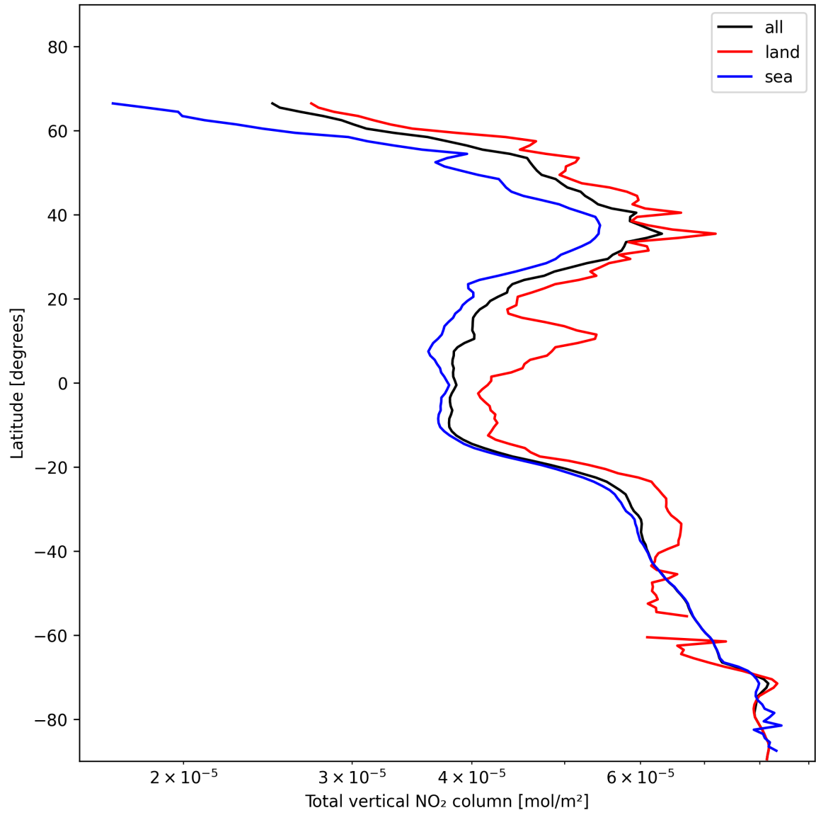
Figure 21: Zonal average of “Total vertical NO 2 column” for 2025-11-26 to 2025-11-28.
