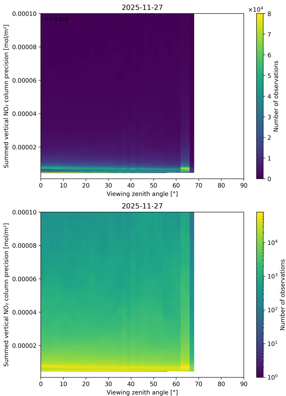
Figure 166: Scatter density plot of “Viewing zenith angle” against “Summed vertical NO 2 column precision” for 2025-11-26 to 2025-11-28.
