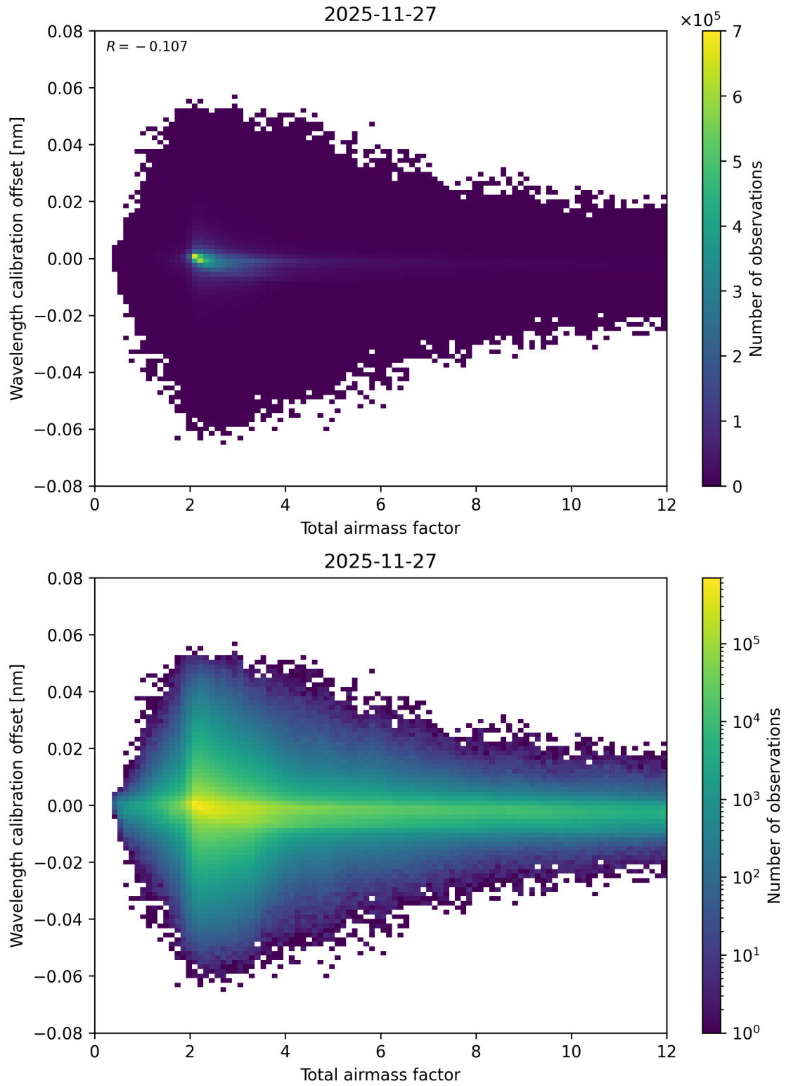
Figure 70: Scatter density plot of “Total airmass factor” against “Wavelength calibration offset” for 2025-11-26 to 2025-11-28.
