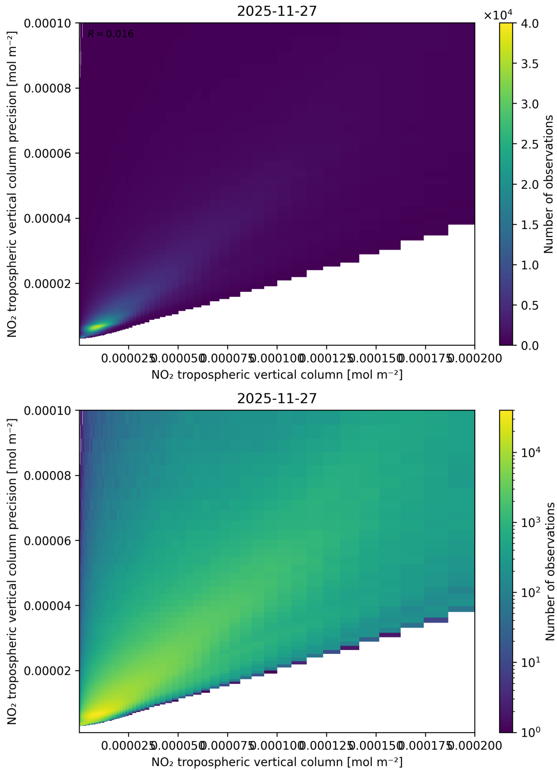
Figure 130: Scatter density plot of “NO 2 tropospheric vertical column” against “NO 2 tropospheric vertical column precision” for 2025-11-26 to 2025-11-28.
