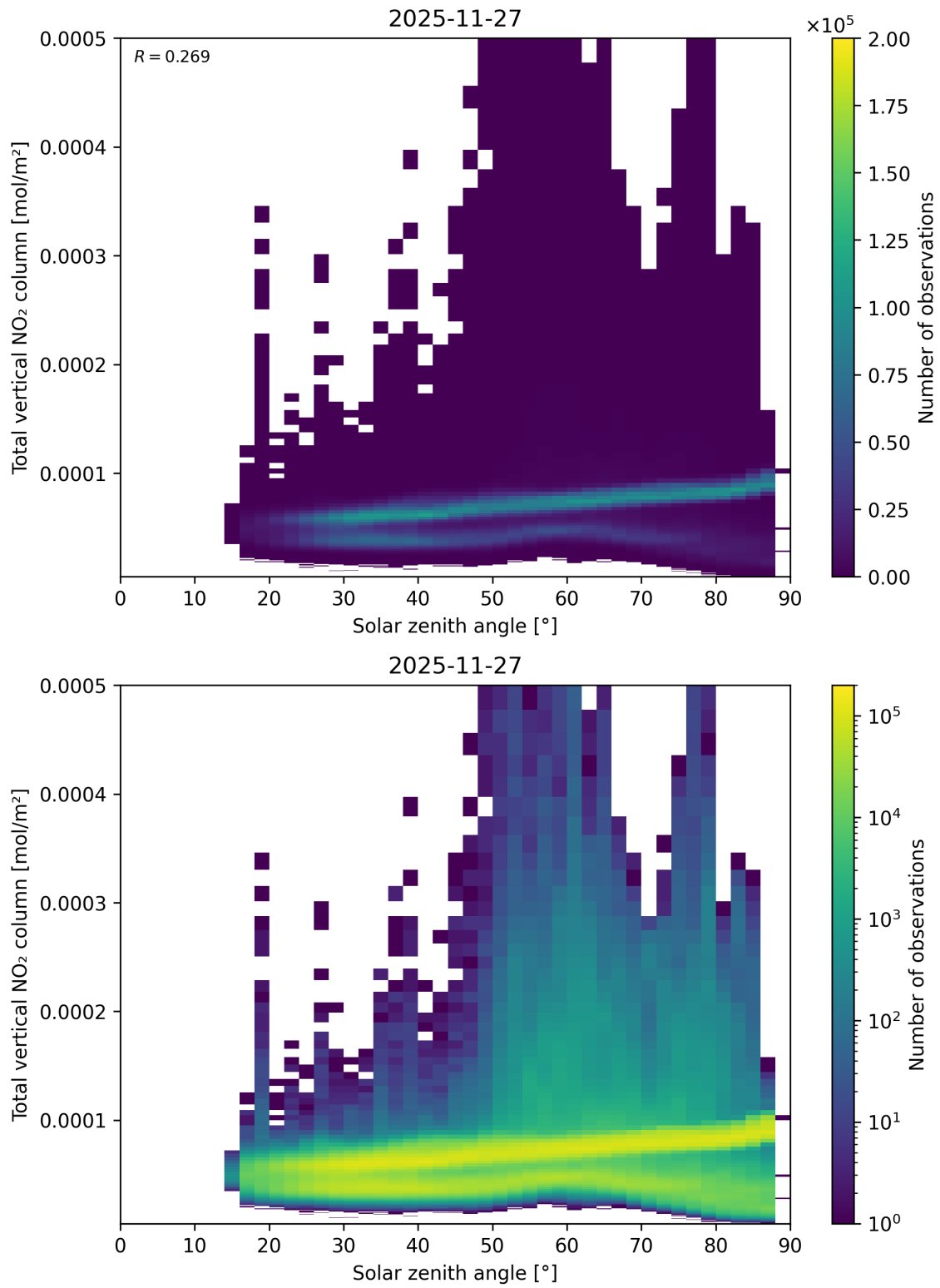
Figure 153: Scatter density plot of “Solar zenith angle” against “Total vertical NO 2 column” for 2025-11-26 to 2025-11-28.
