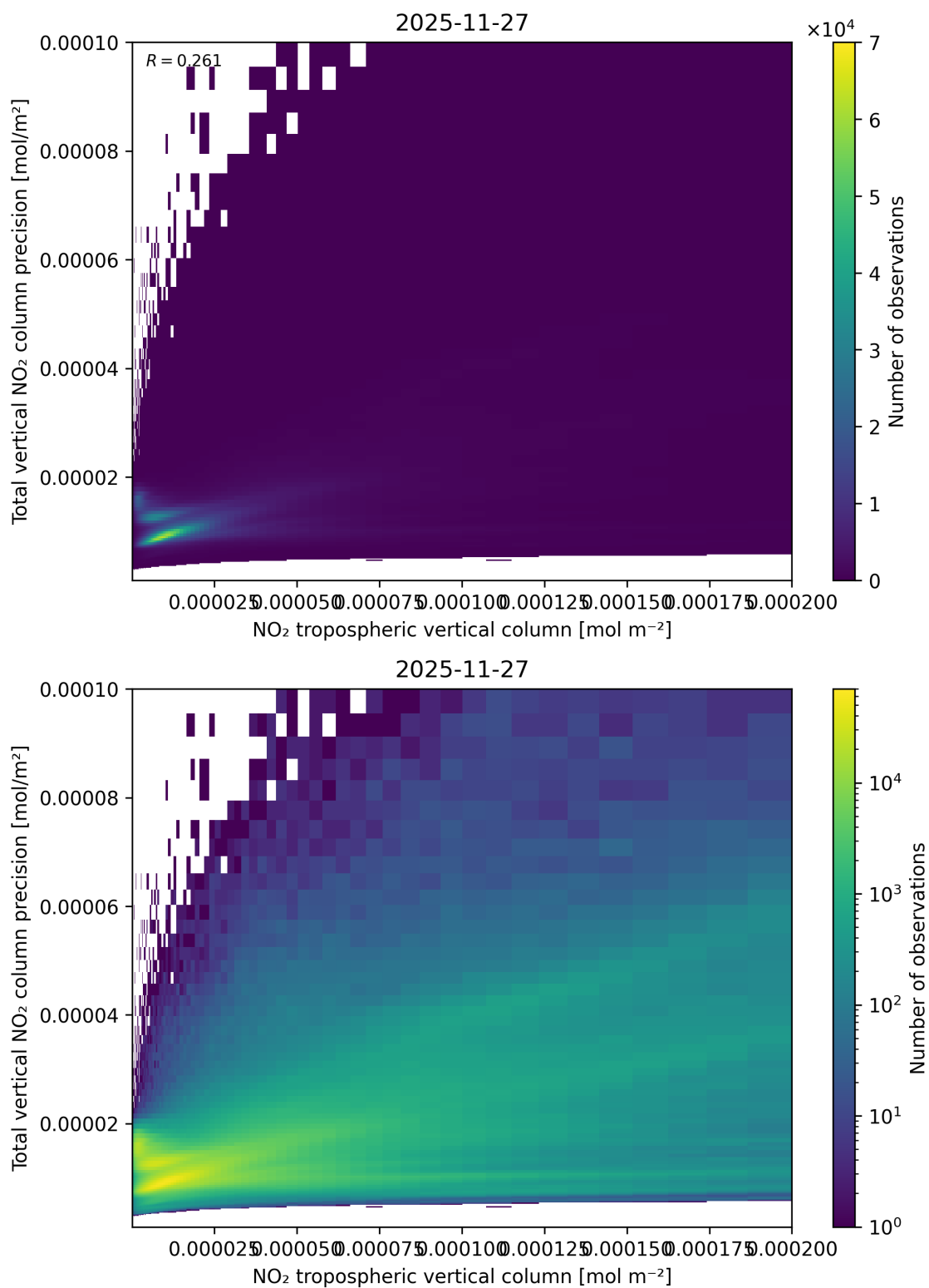
Figure 129: Scatter density plot of “NO 2 tropospheric vertical column” against “Total vertical NO 2 column precision” for 2025-11-26 to 2025-11-28.
