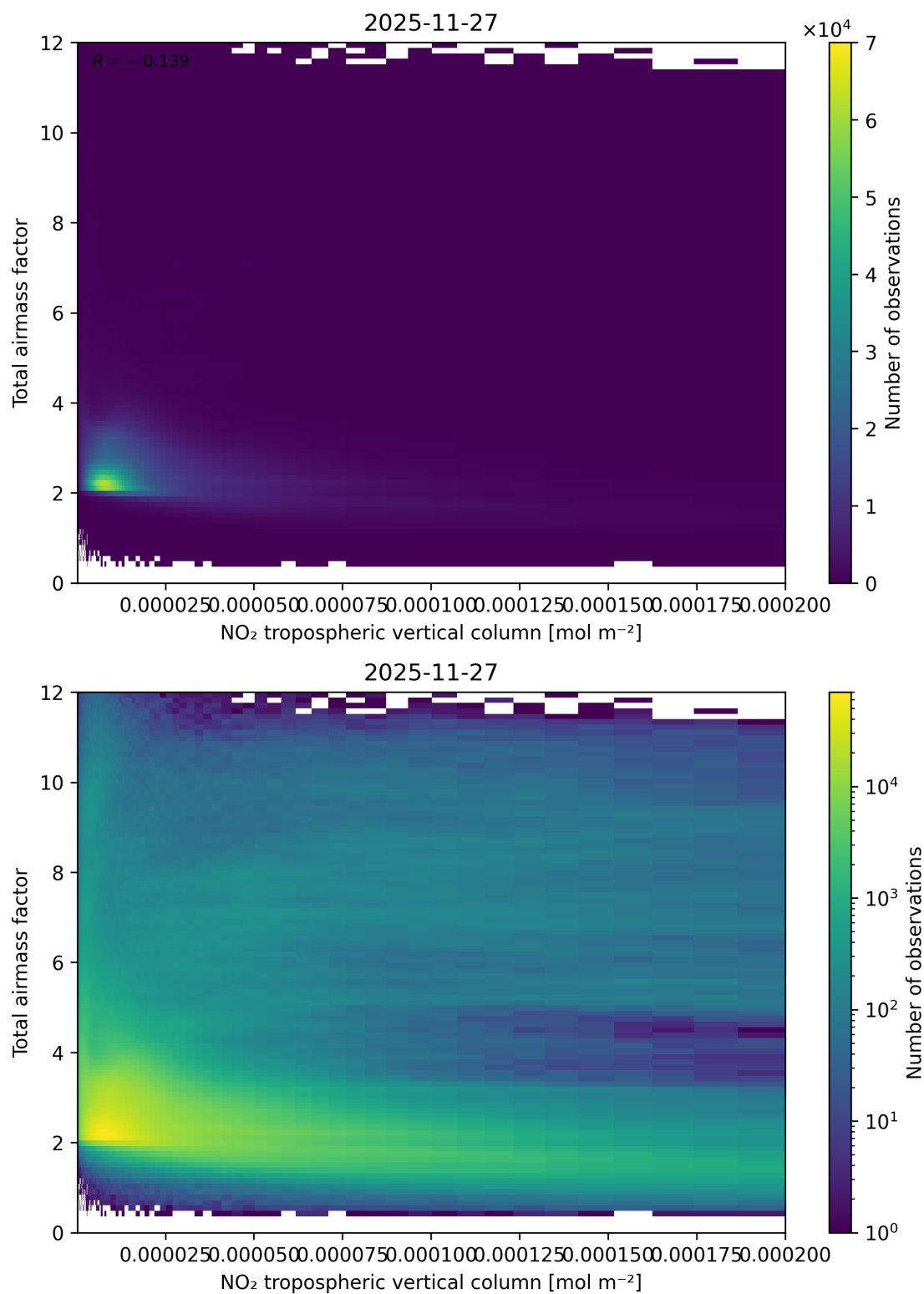
Figure 122: Scatter density plot of “NO 2 tropospheric vertical column” against “Total air mass factor” for 2025-11-26 to 2025-11-28.
