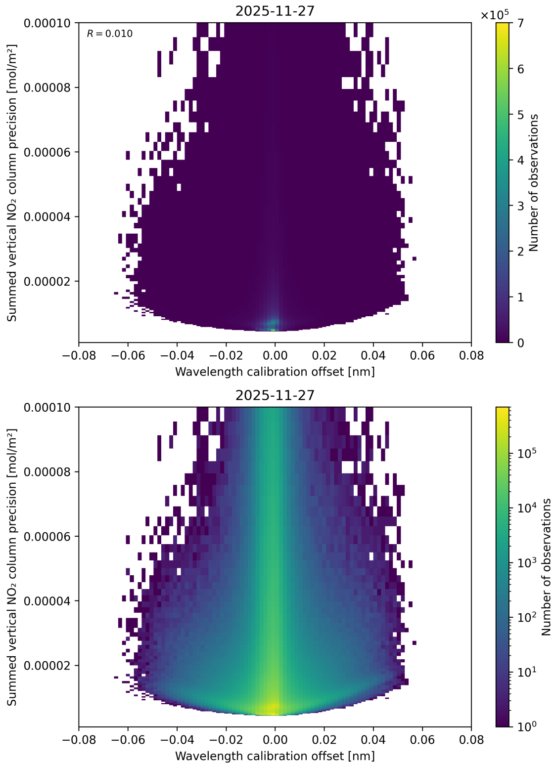
Figure 178: Scatter density plot of “Wavelength calibration offset” against “Summed vertical NO 2 column precision” for 2025-11-26 to 2025-11-28.
