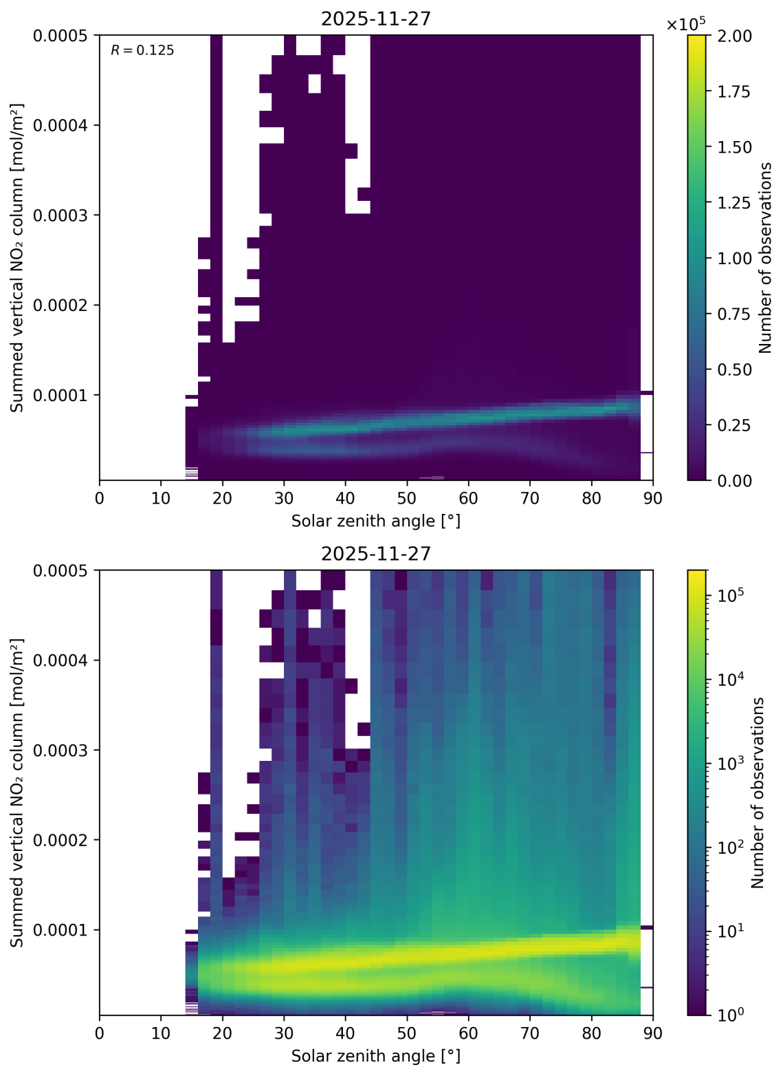
Figure 151: Scatter density plot of “Solar zenith angle” against “Summed vertical NO 2 column” for 2025-11-26 to 2025-11-28.
