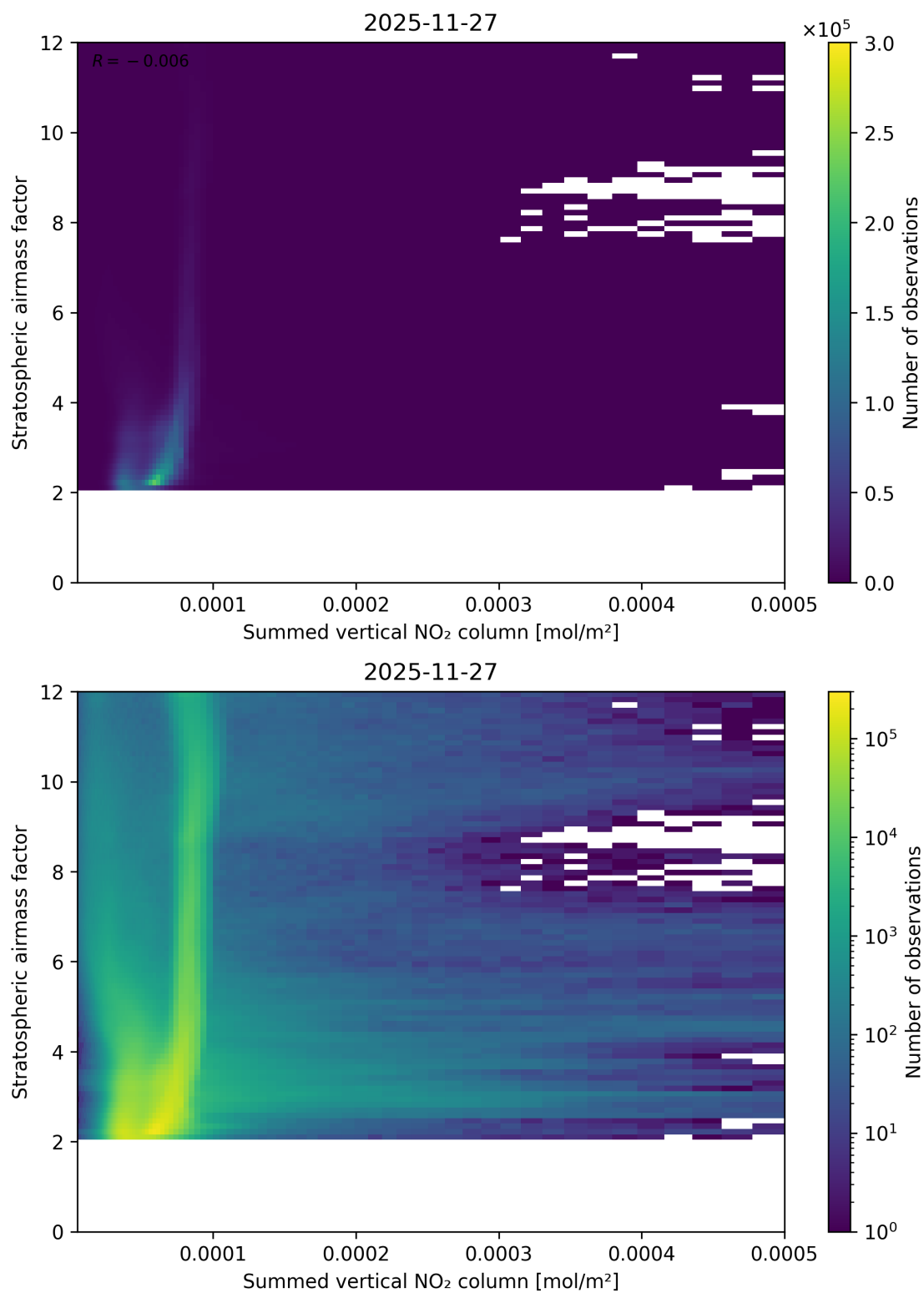
Figure 103: Scatter density plot of “Summed vertical NO 2 column” against “Stratospheric airmass factor” for 2025-11-26 to 2025-11-28.
