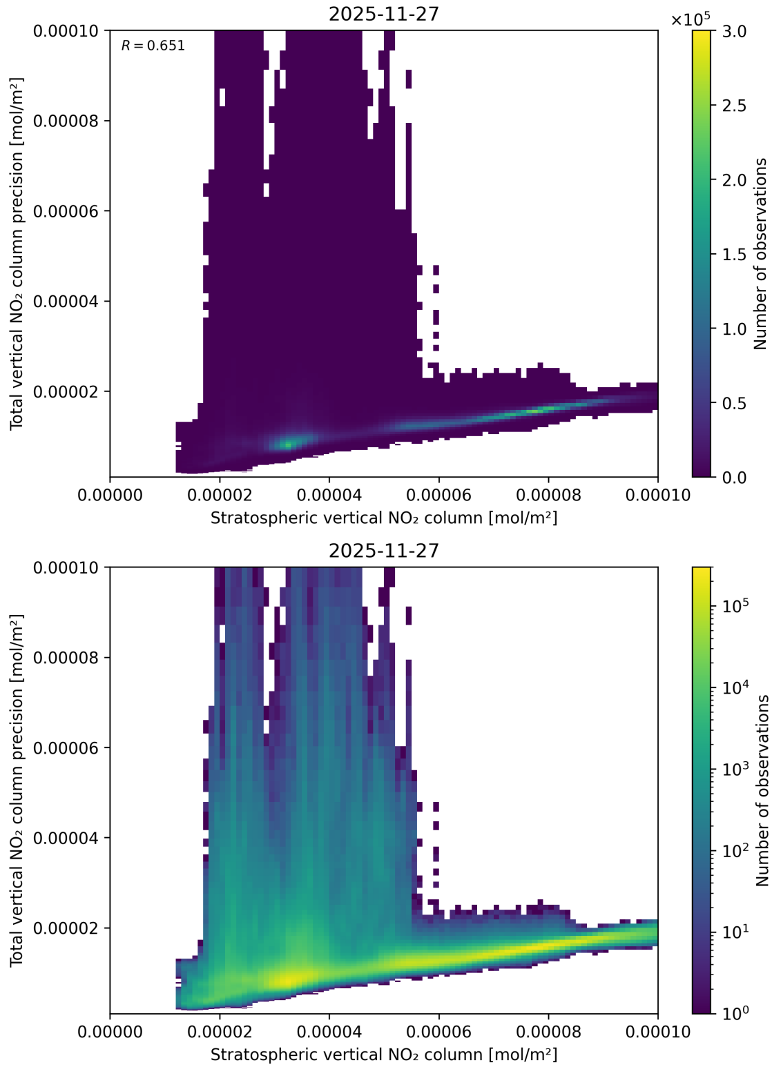
Figure 101: Scatter density plot of “Stratospheric vertical NO 2 column” against “Total vertical NO 2 column precision” for 2025-11-26 to 2025-11-28.
