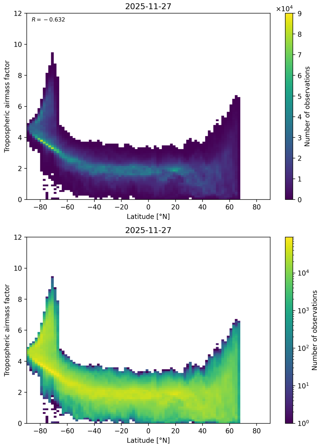
Figure 85: Scatter density plot of “Latitude” against “Tropospheric air mass factor” for 2025-11-26 to 2025-11-28.
