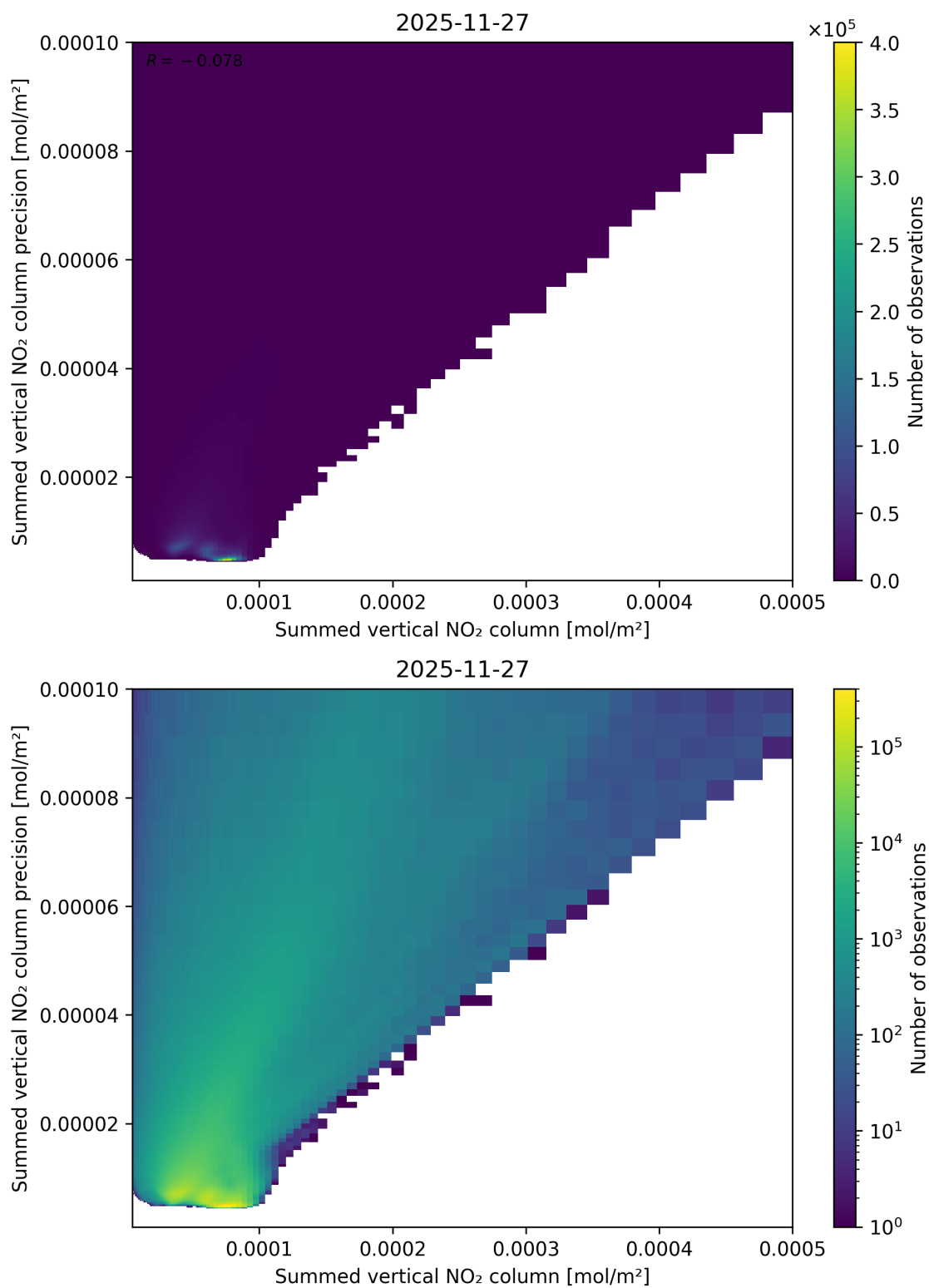
Figure 105: Scatter density plot of “Summed vertical NO 2 column” against “Summed vertical NO 2 column precision” for 2025-11-26 to 2025-11-28.
