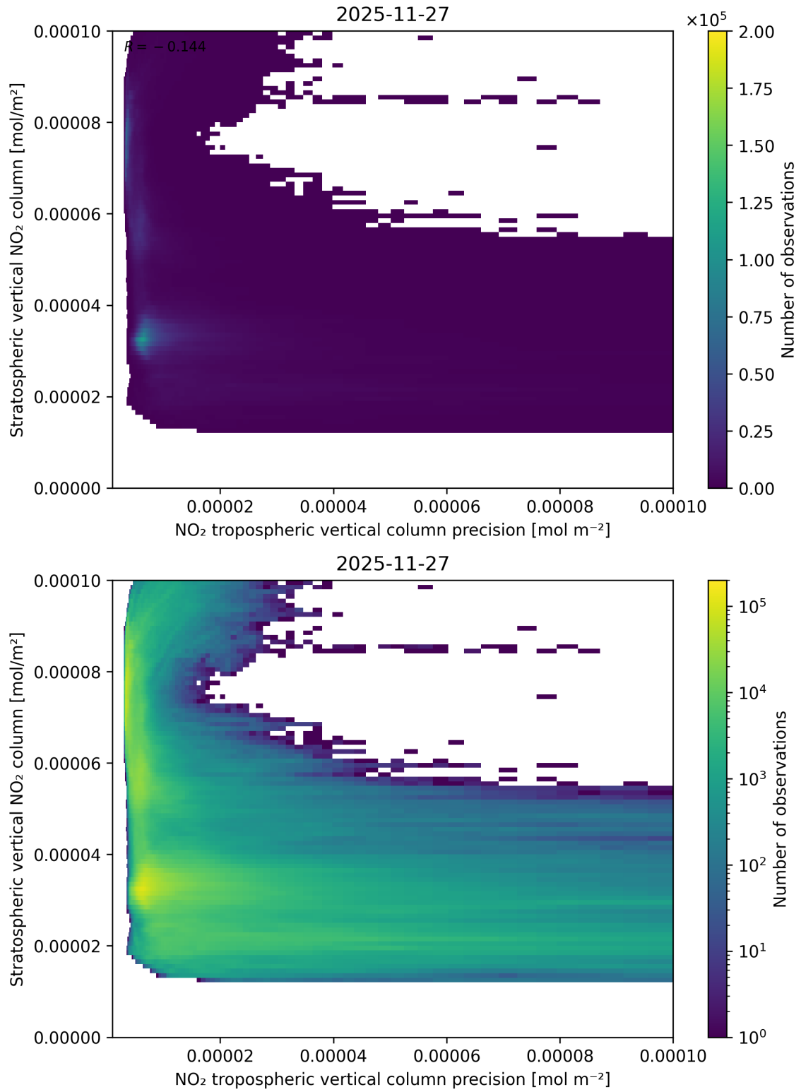
Figure 135: Scatter density plot of “NO 2 tropospheric vertical column precision” against “Stratospheric vertical NO 2 column” for 2025-11-26 to 2025-11-28.
