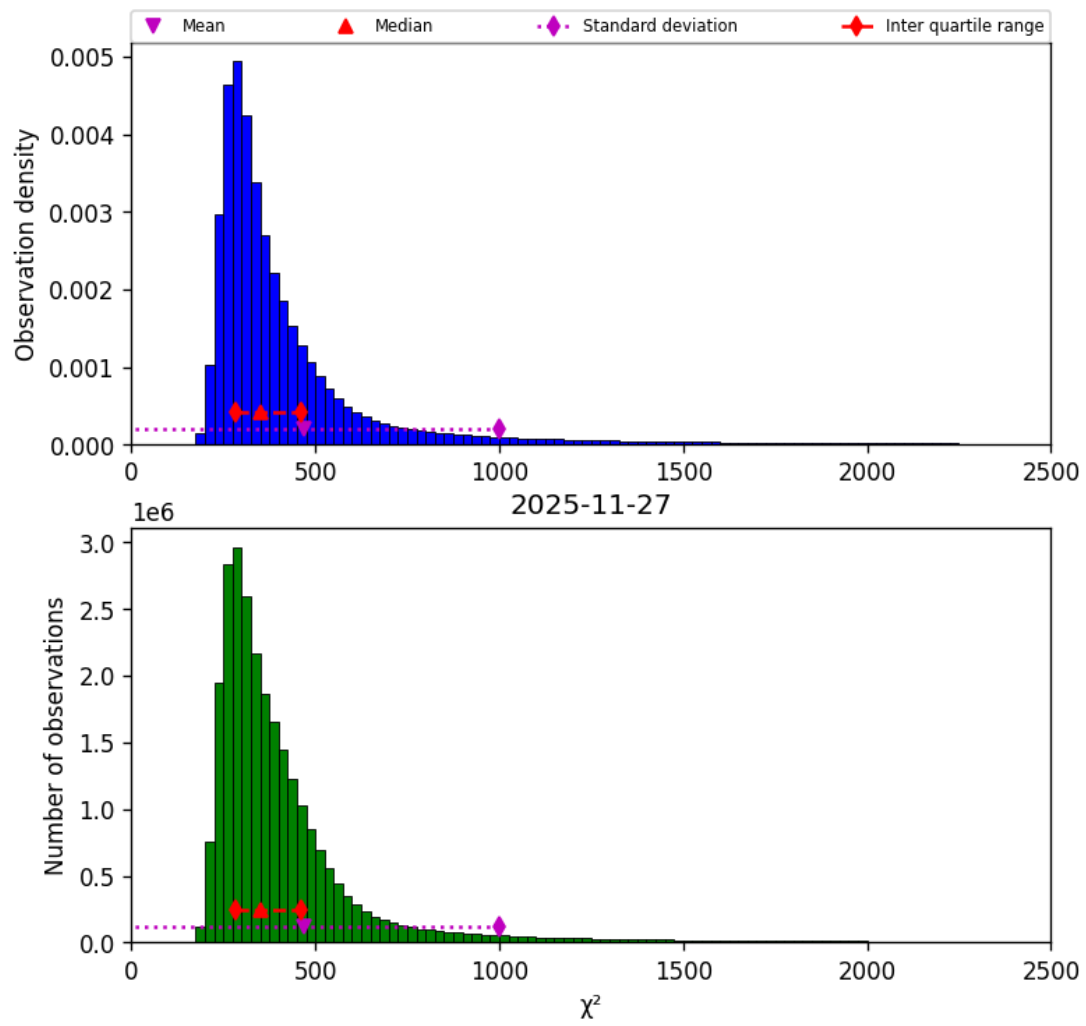
Figure 42: Histogram of “ \chi^2 ” for 2025-11-26 to 2025-11-28
