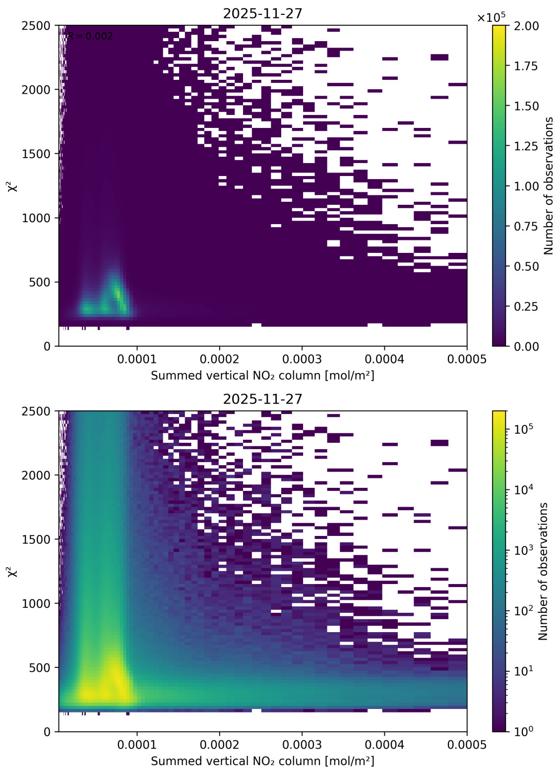
Figure 104: Scatter density plot of “Summed vertical NO 2 column” against “ \chi^2 ” for 2025-11-26 to 2025-11-28.
