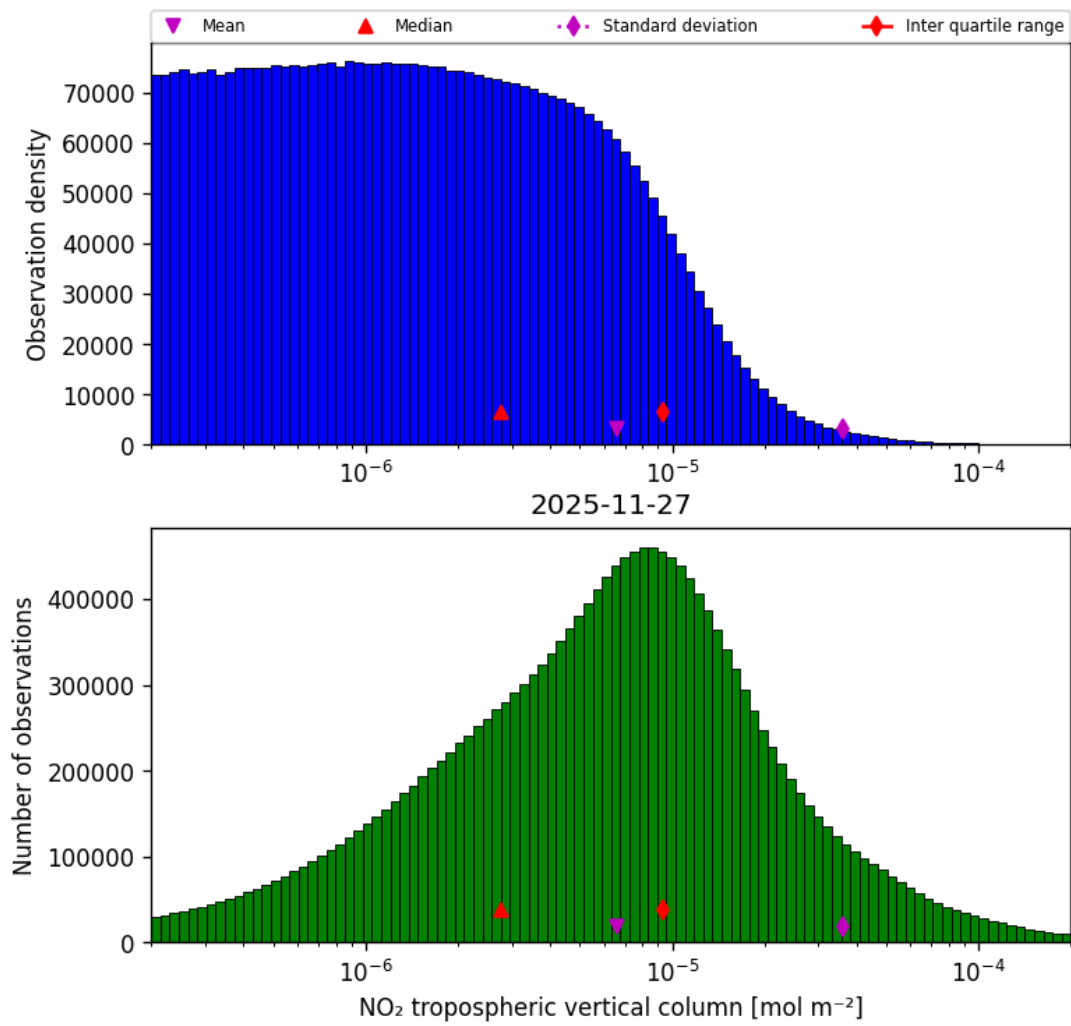
Figure 29: Histogram of “NO 2 tropospheric vertical column” for 2025-11-26 to 2025-11-28
