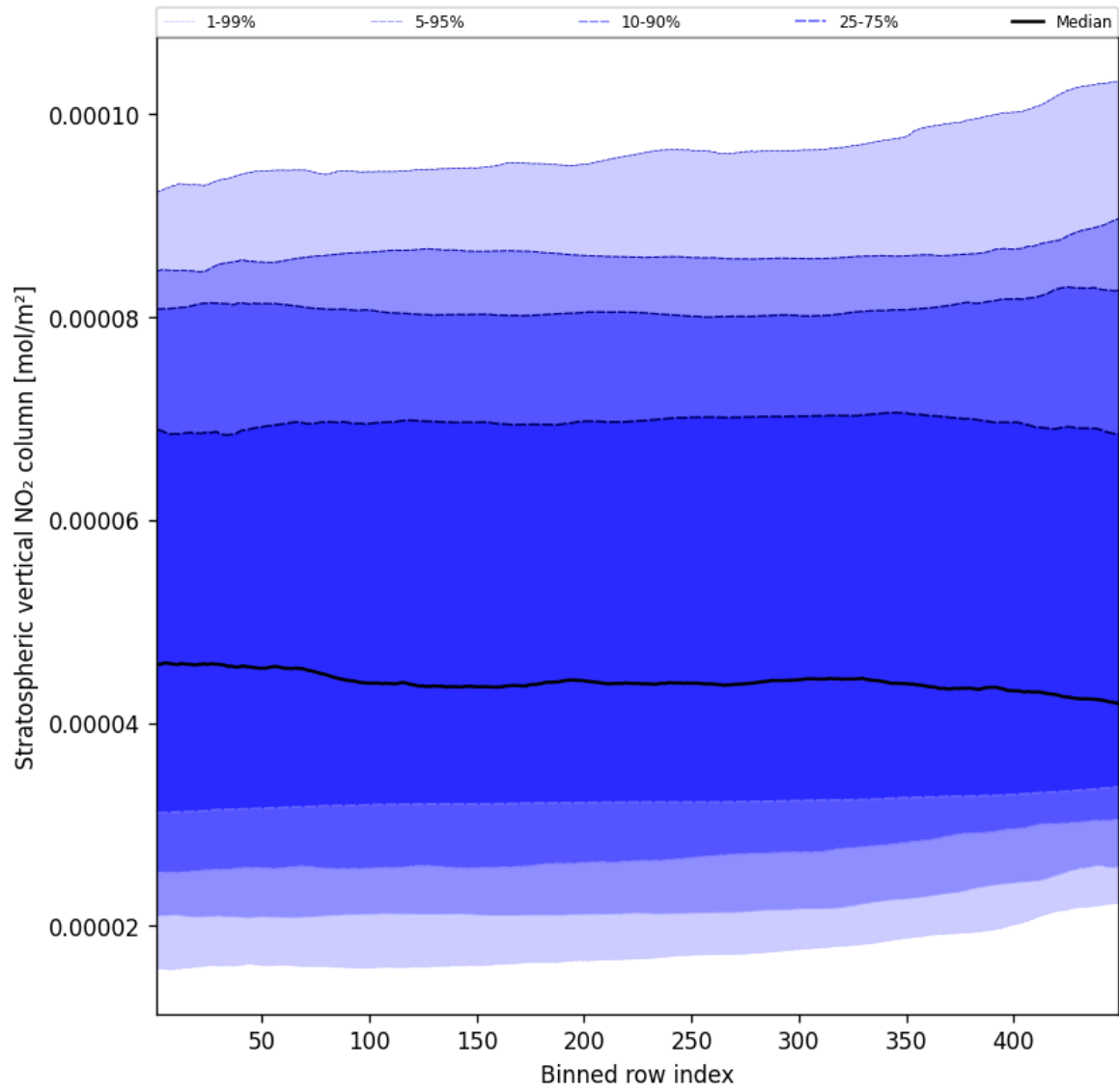
Figure 53: Along track statistics of “Stratospheric vertical NO 2 column” for 2025-11-26 to 2025-11-28
