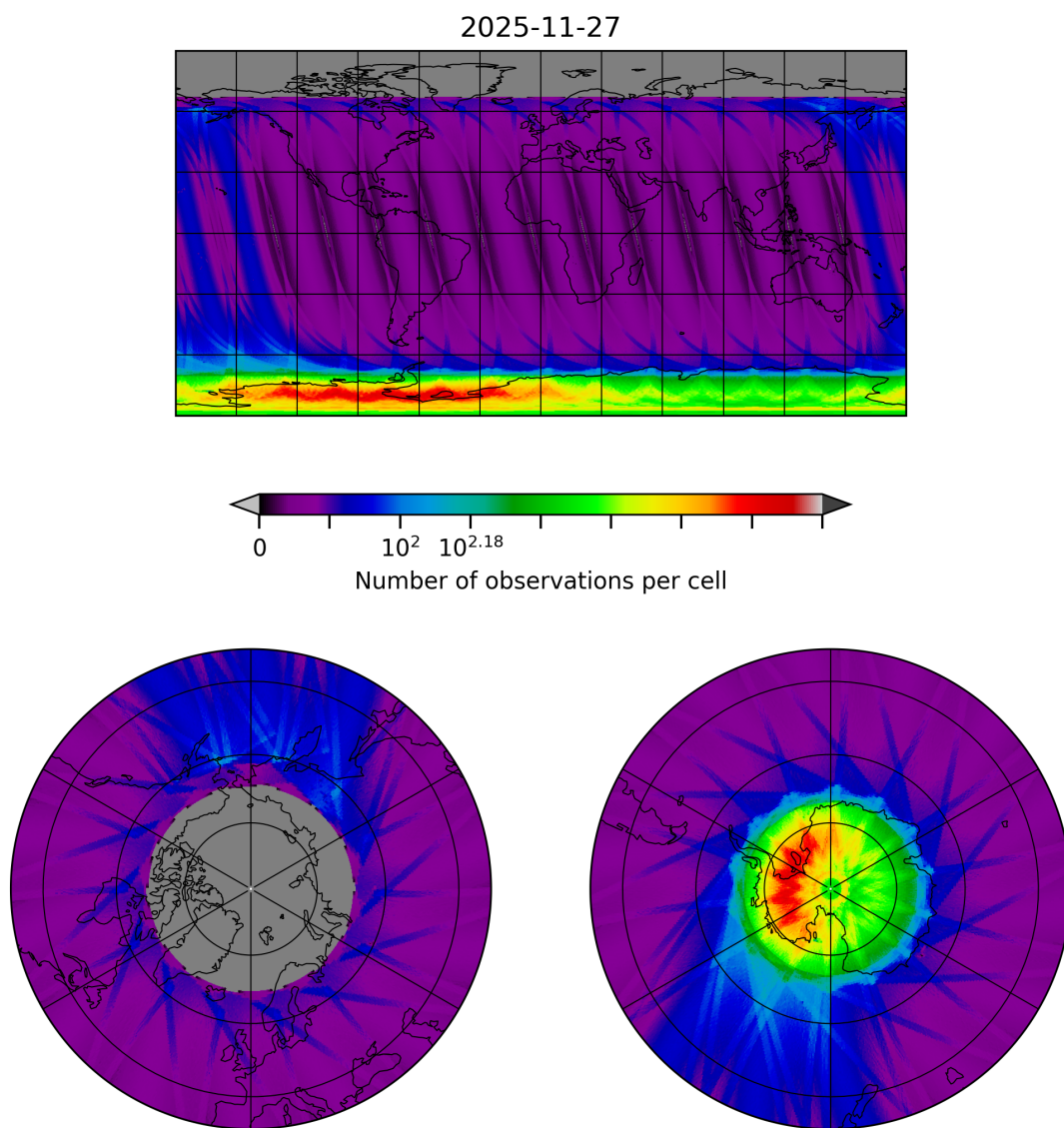
Figure 10: Map of the number of observations for 2025-11-26 to 2025-11-28
