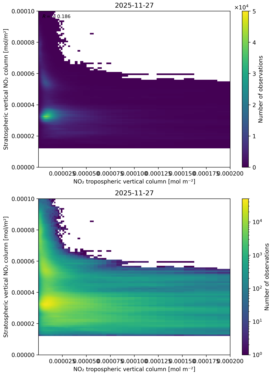
Figure 125: Scatter density plot of “NO 2 tropospheric vertical column” against “Stratospheric vertical NO 2 column” for 2025-11-26 to 2025-11-28.
