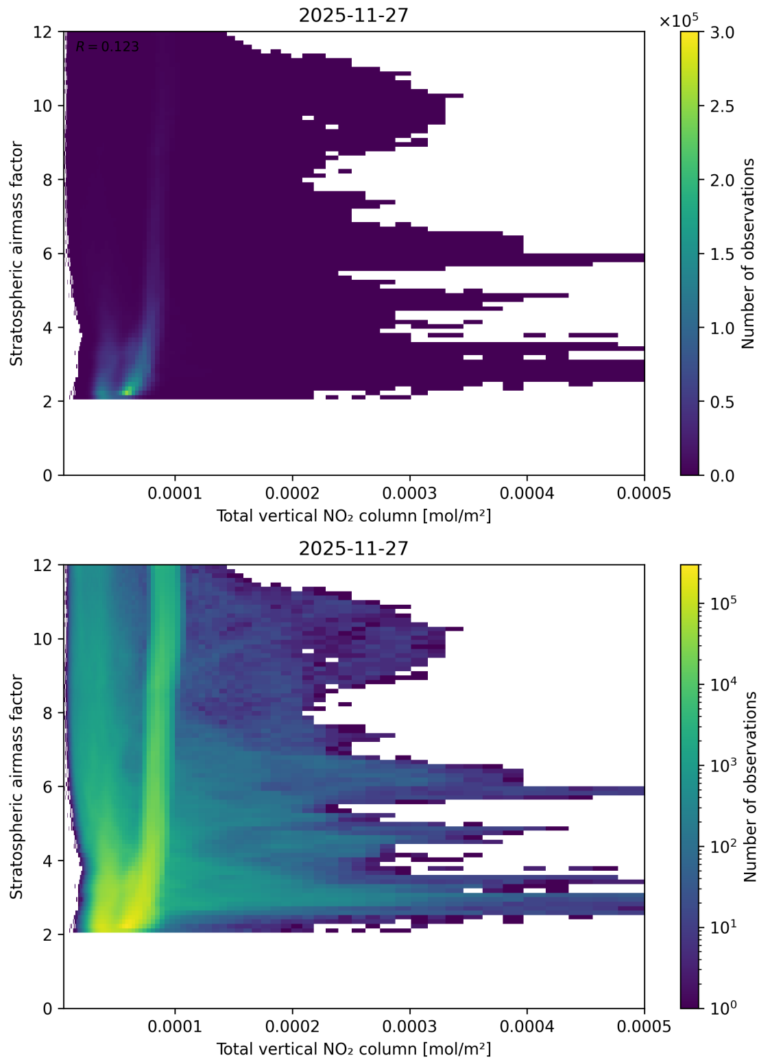
Figure 110: Scatter density plot of “Total vertical NO 2 column” against “Stratospheric airmass factor” for 2025-11-26 to 2025-11-28.
