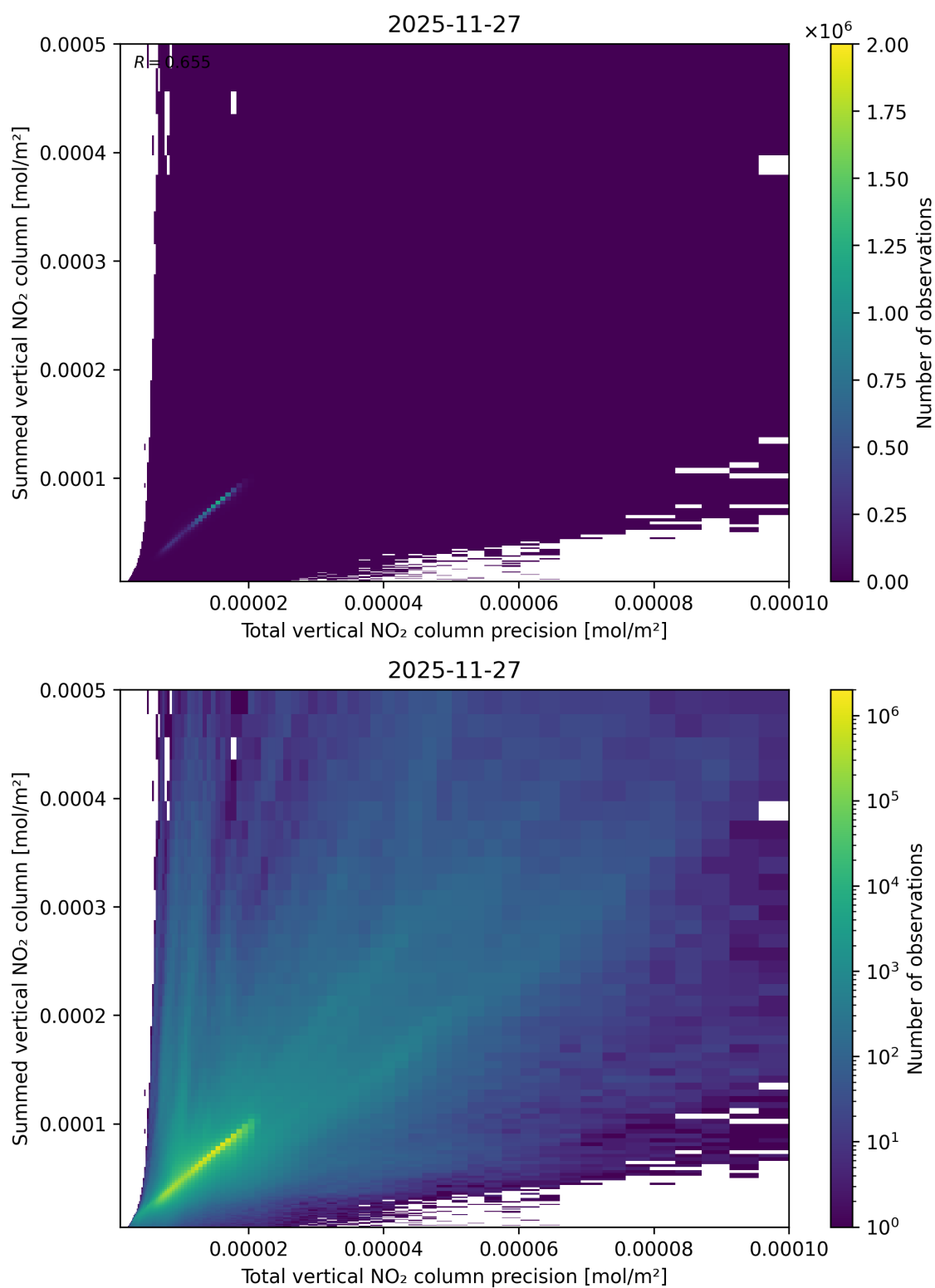
Figure 117: Scatter density plot of “Total vertical NO 2 column precision” against “Summed vertical NO 2 column” for 2025-11-26 to 2025-11-28.
