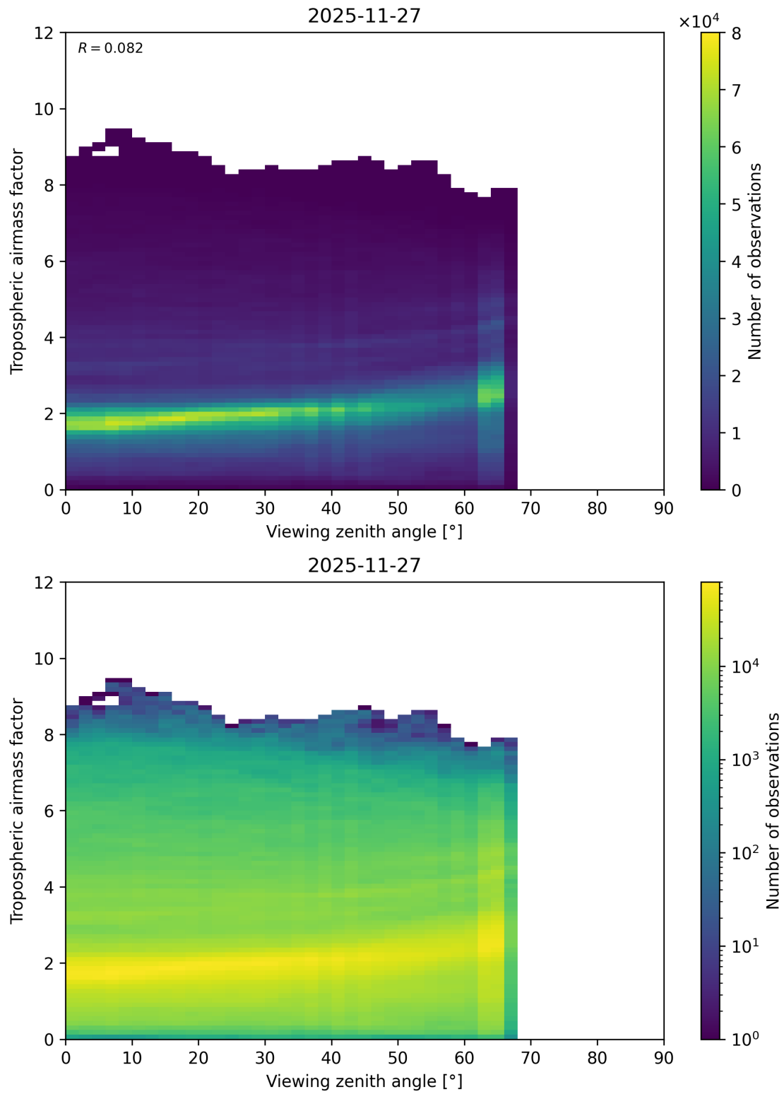
Figure 161: Scatter density plot of “Viewing zenith angle” against “Tropospheric airmass factor” for 2025-11-26 to 2025-11-28.
