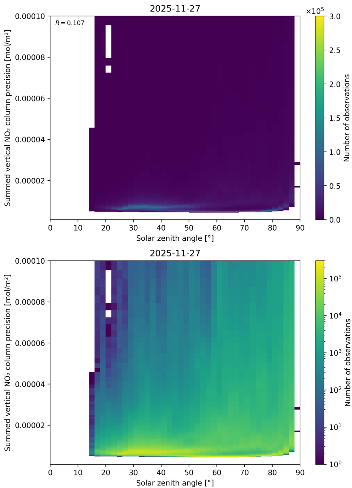
Figure 152: Scatter density plot of “Solar zenith angle” against “Summed vertical NO 2 column precision” for 2025-11-26 to 2025-11-28.
