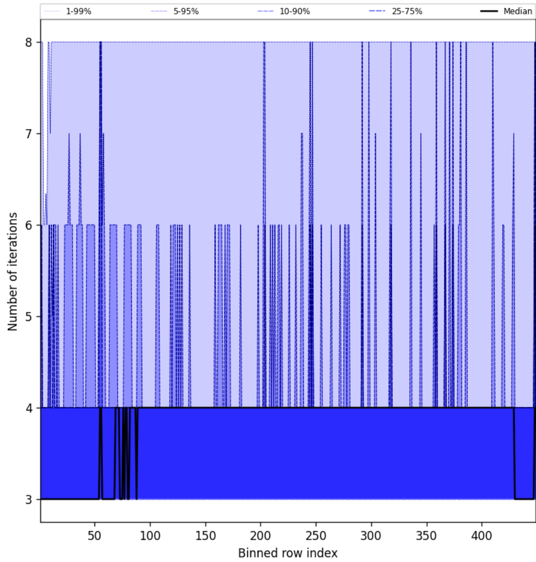
Figure 51: Along track statistics of “Number of iterations” for 2025-11-26 to 2025-11-28
