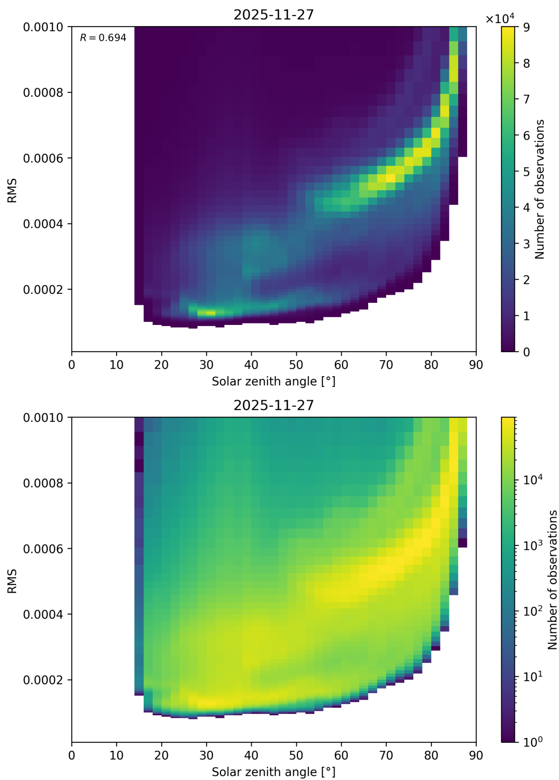
Figure 157: Scatter density plot of “Solar zenith angle” against “RMS” for 2025-11-26 to 2025-11-28.
