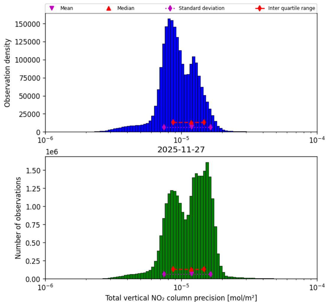
Figure 39: Histogram of “Total vertical NO 2 column precision” for 2025-11-26 to 2025-11-28
