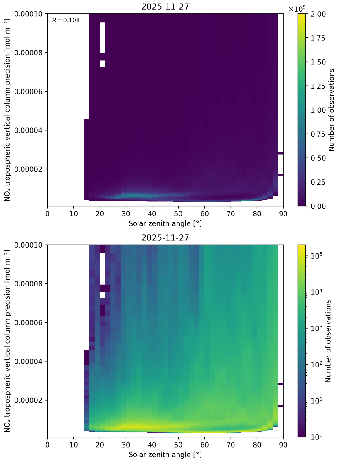
Figure 156: Scatter density plot of “Solar zenith angle” against “NO 2 tropospheric vertical column precision” for 2025-11-26 to 2025-11-28.
