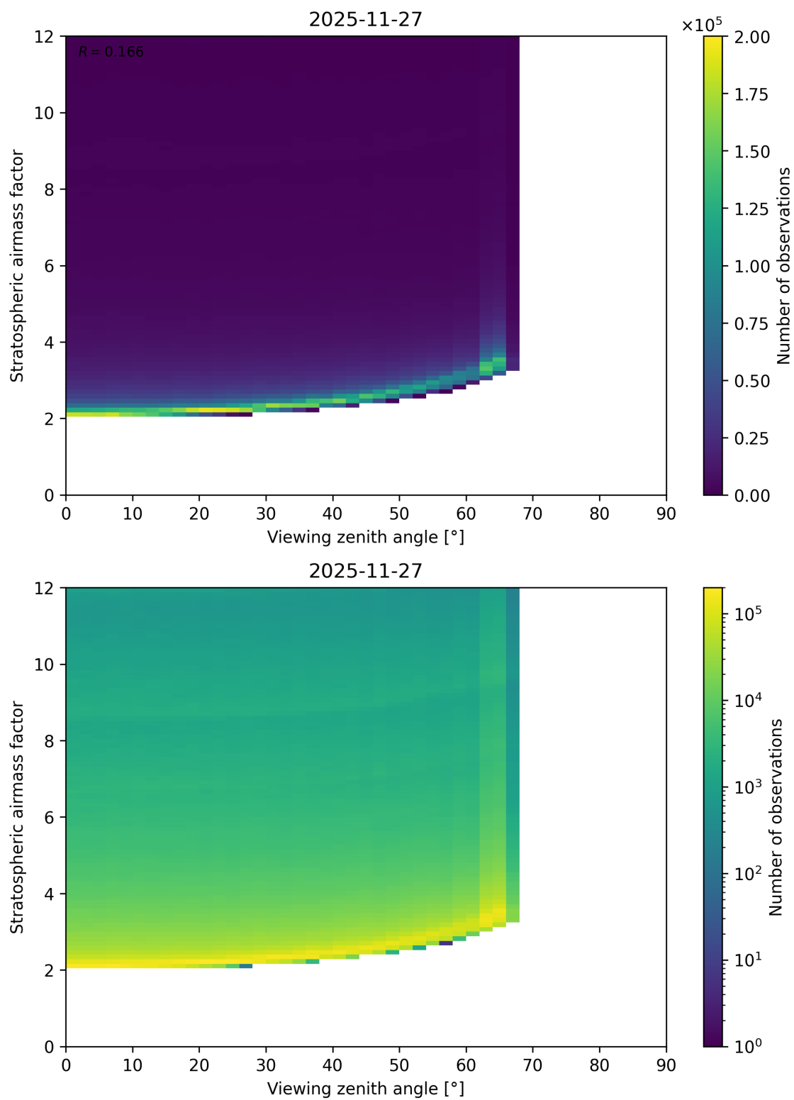
Figure 159: Scatter density plot of “Viewing zenith angle” against “Stratospheric airmass factor” for 2025-11-26 to 2025-11-28.
