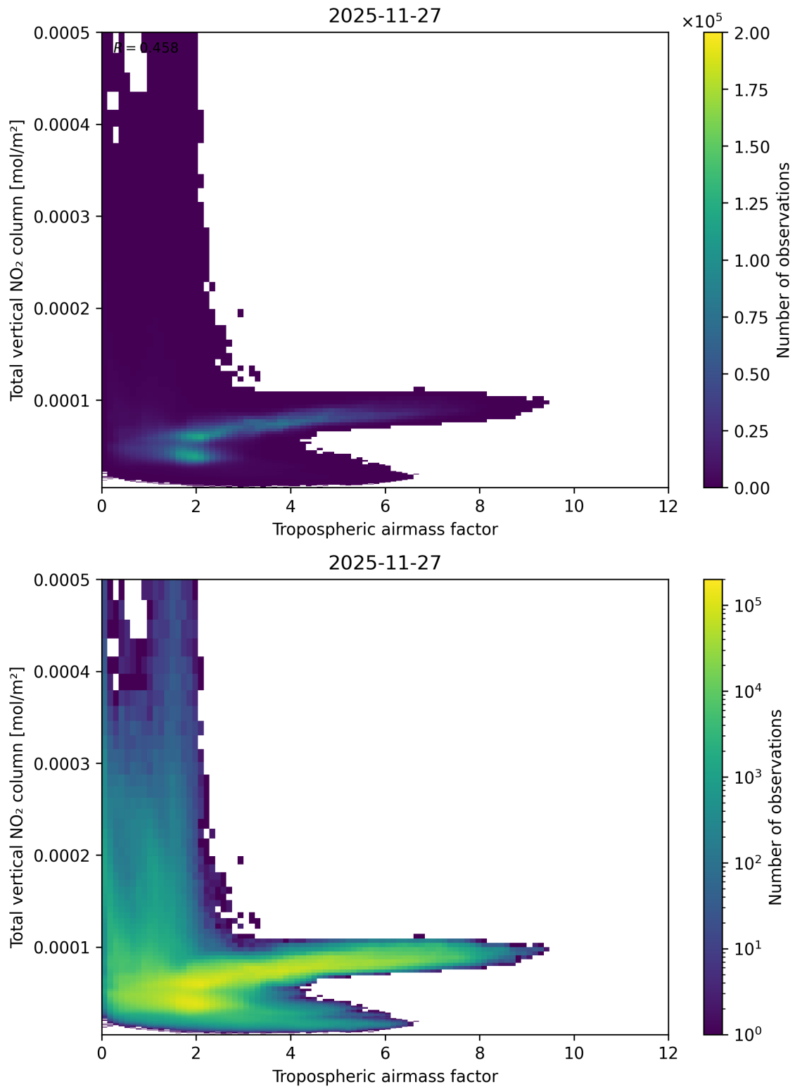
Figure 77: Scatter density plot of “Tropospheric airmass factor” against “Total vertical NO 2 column” for 2025-11-26 to 2025-11-28.
