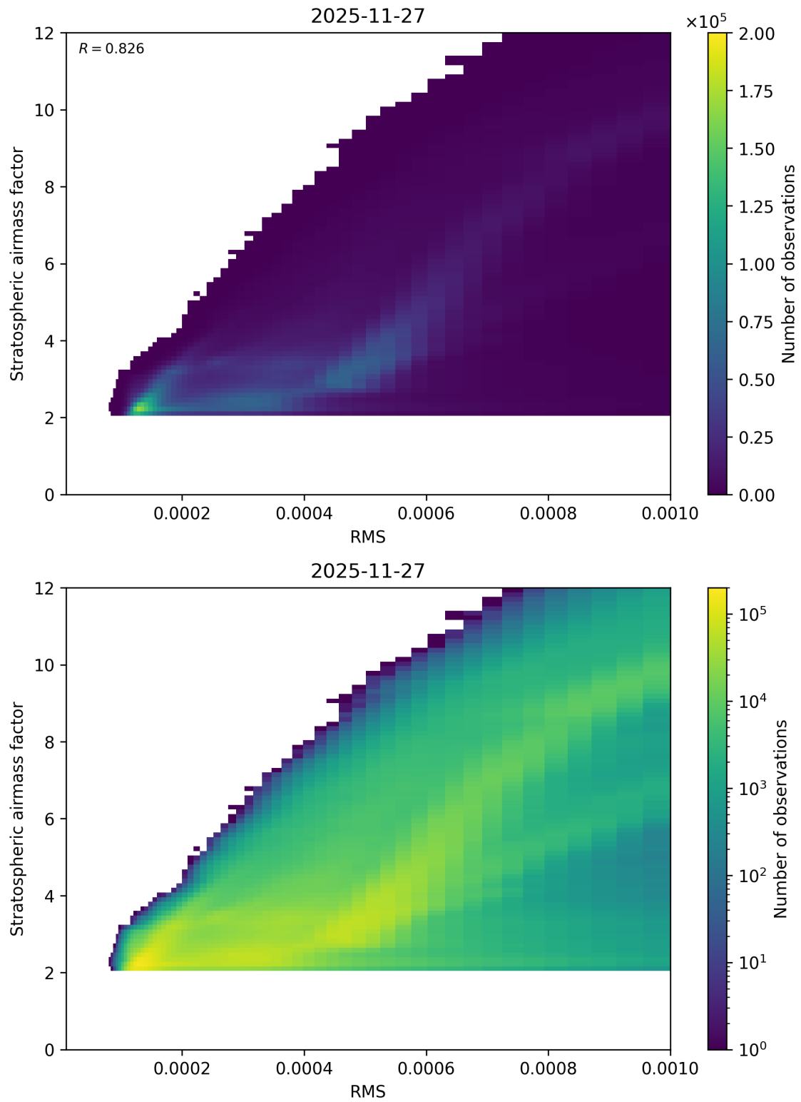
Figure 144: Scatter density plot of “RMS” against “Stratospheric airmass factor” for 2025-11-26 to 2025-11-28.
