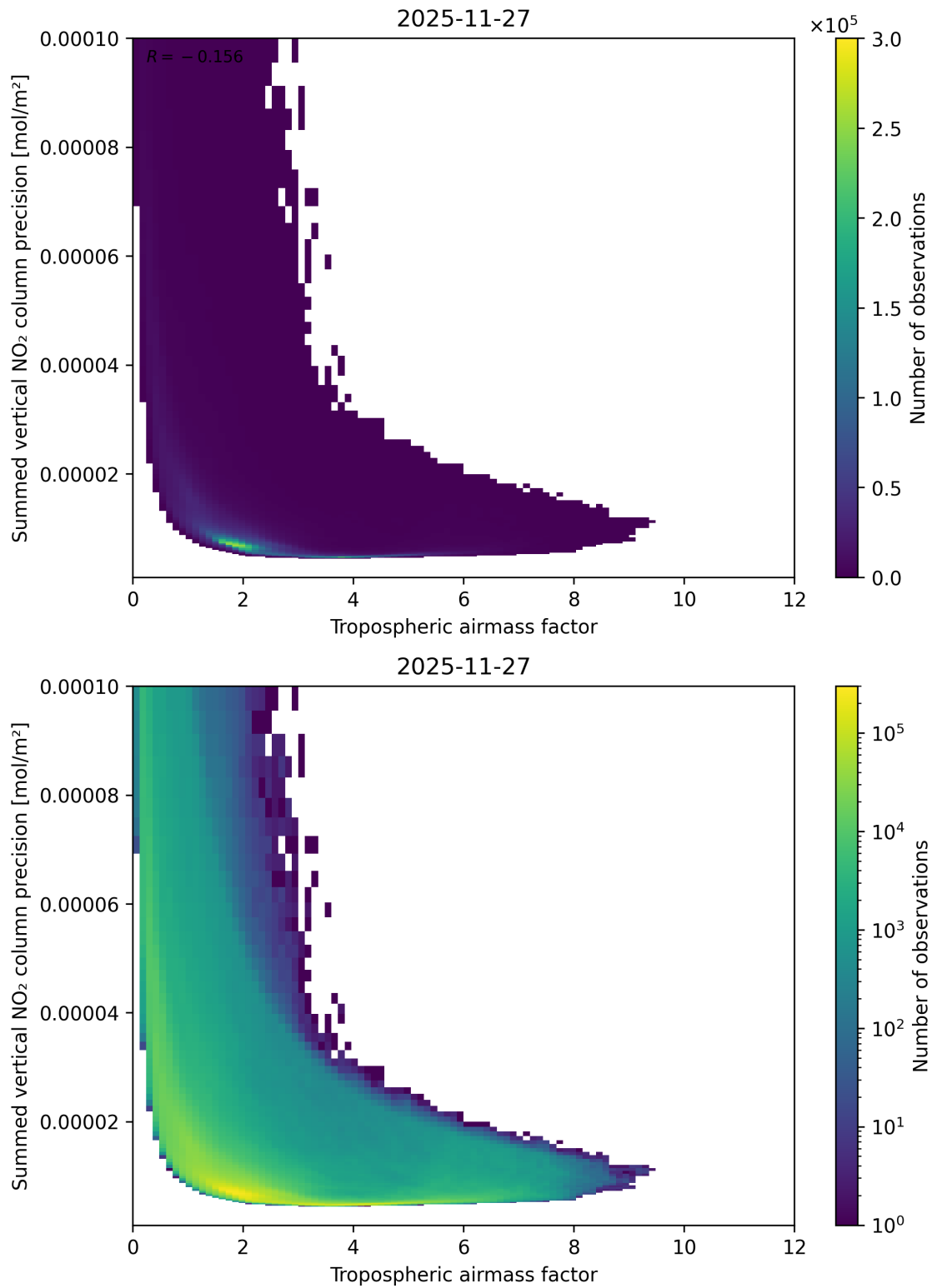
Figure 76: Scatter density plot of “Tropospheric air mass factor” against “Summed vertical NO 2 column precision” for 2025-11-26 to 2025-11-28.
