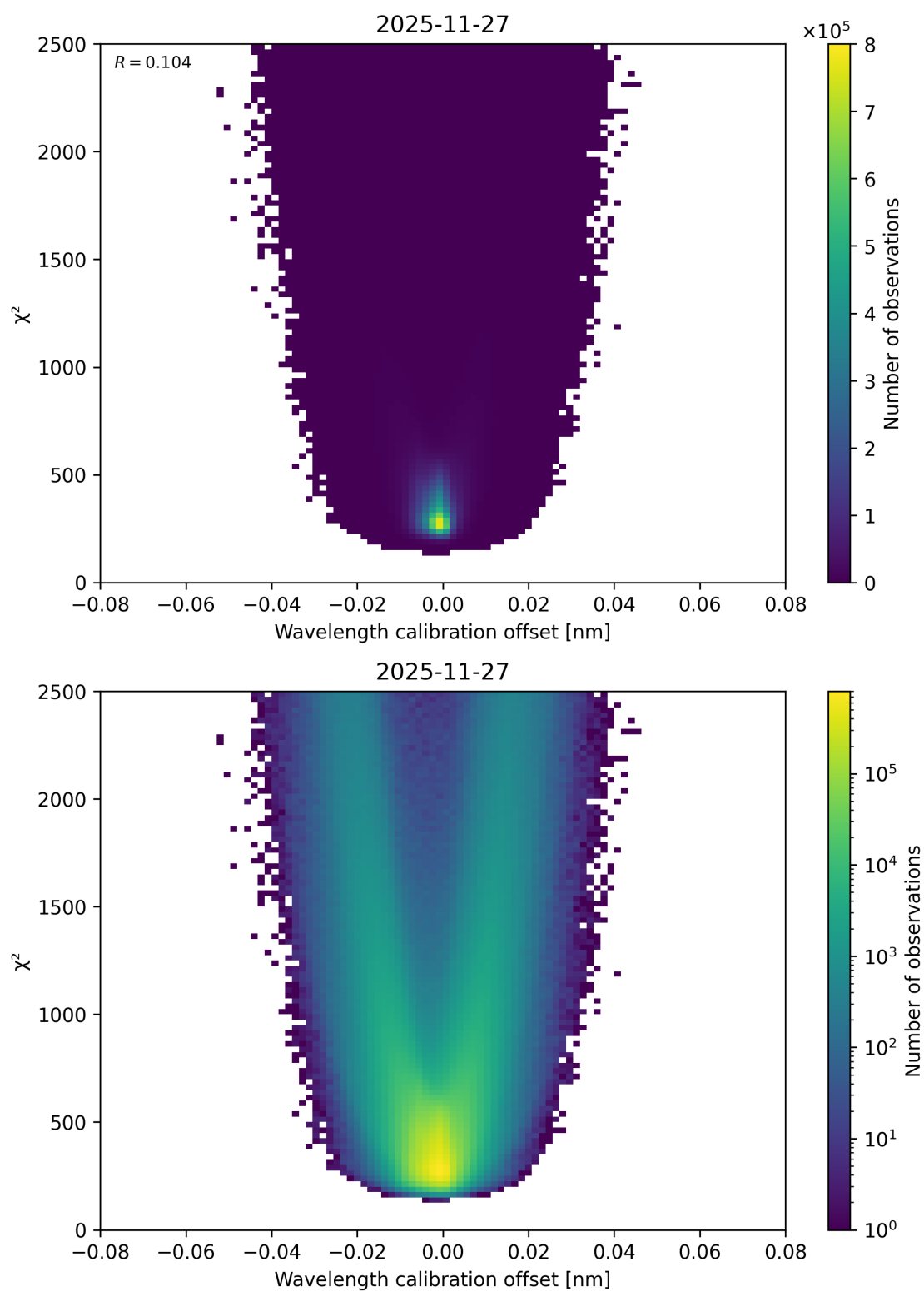
Figure 175: Scatter density plot of “Wavelength calibration offset” against “ \chi^2 ” for 2025-11-26 to 2025-11-28.
