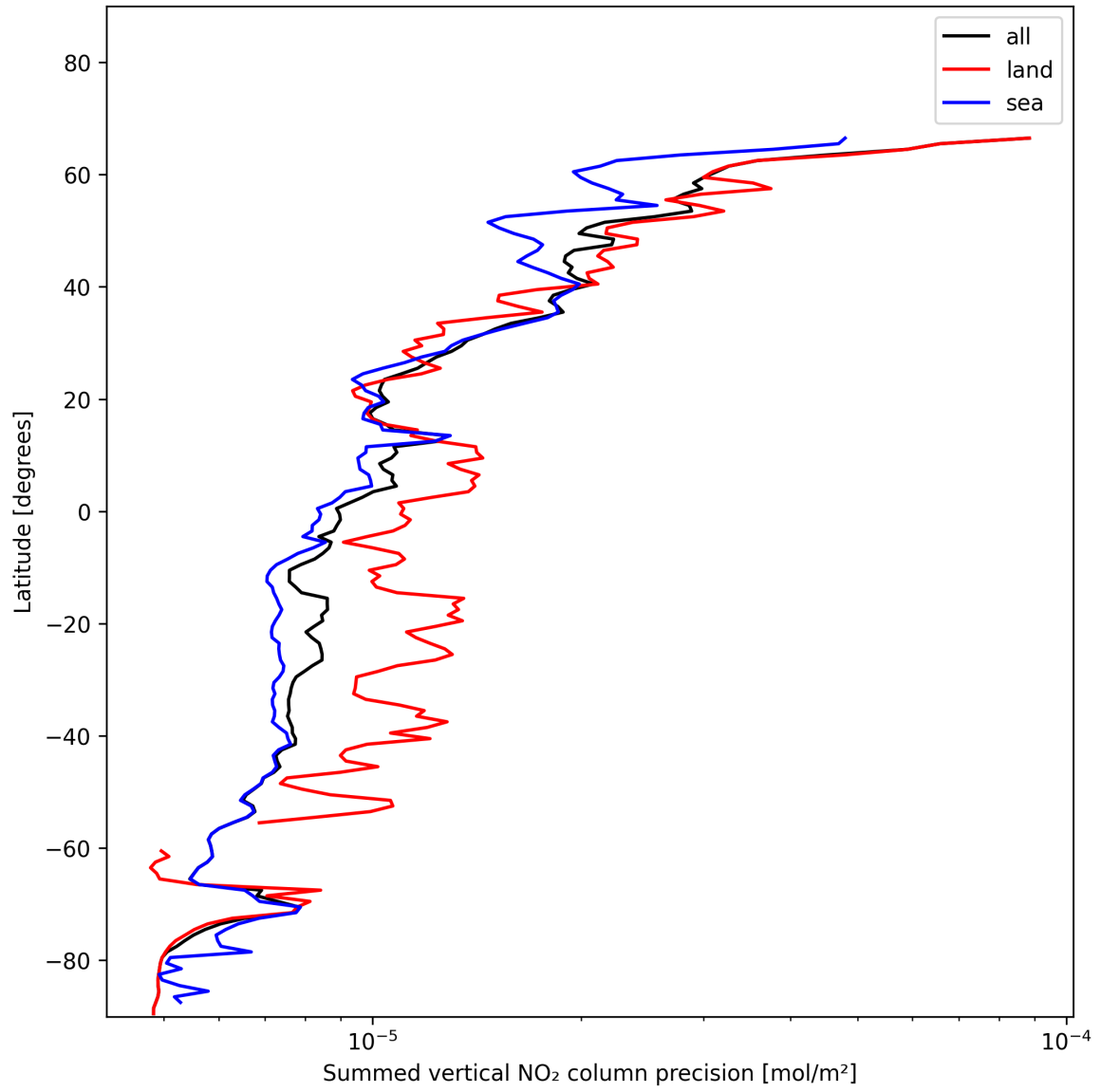
Figure 24: Zonal average of “Summed vertical NO 2 column precision” for 2025-11-26 to 2025-11-28.
