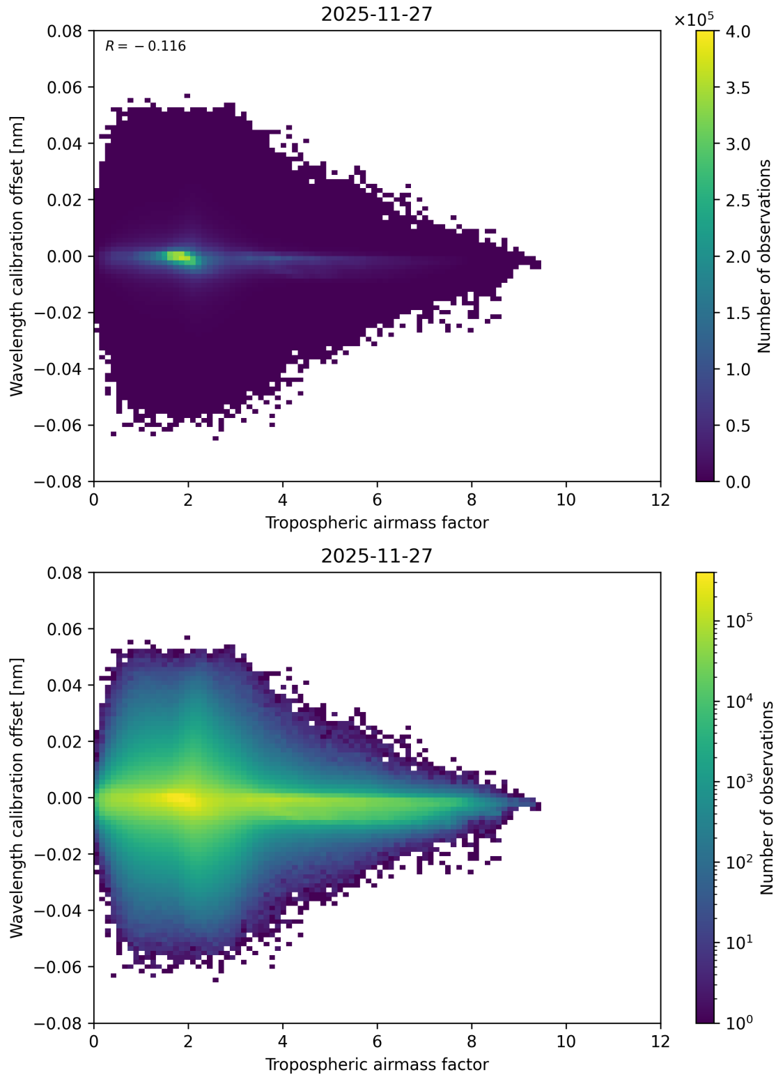
Figure 80: Scatter density plot of “Tropospheric airmass factor” against “Wavelength calibration offset” for 2025-11-26 to 2025-11-28.
