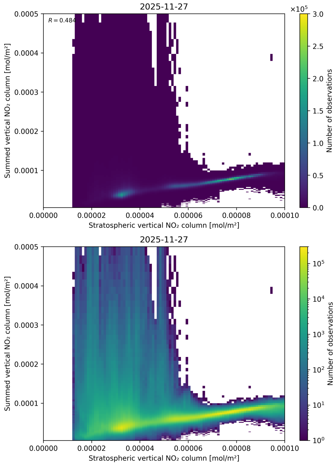
Figure 98: Scatter density plot of “Stratospheric vertical NO 2 column” against “Summed vertical NO 2 column” for 2025-11-26 to 2025-11-28.
