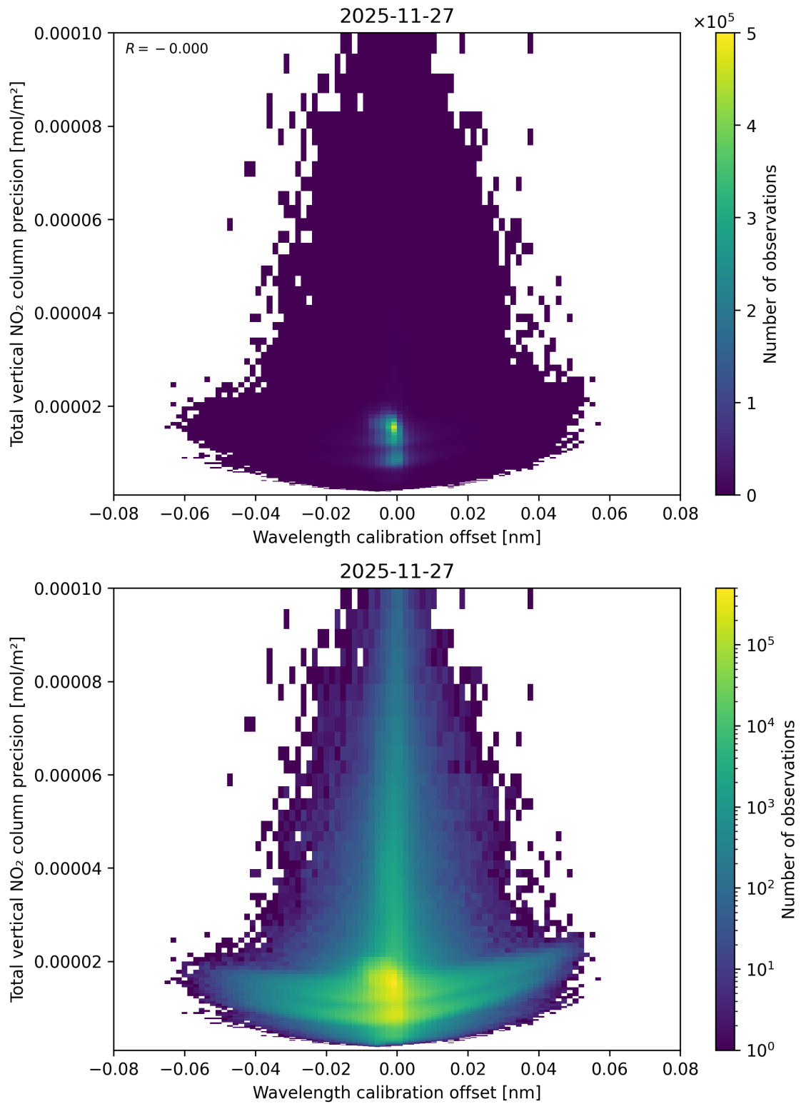
Figure 180: Scatter density plot of “Wavelength calibration offset” against “Total vertical NO 2 column precision” for 2025-11-26 to 2025-11-28.
