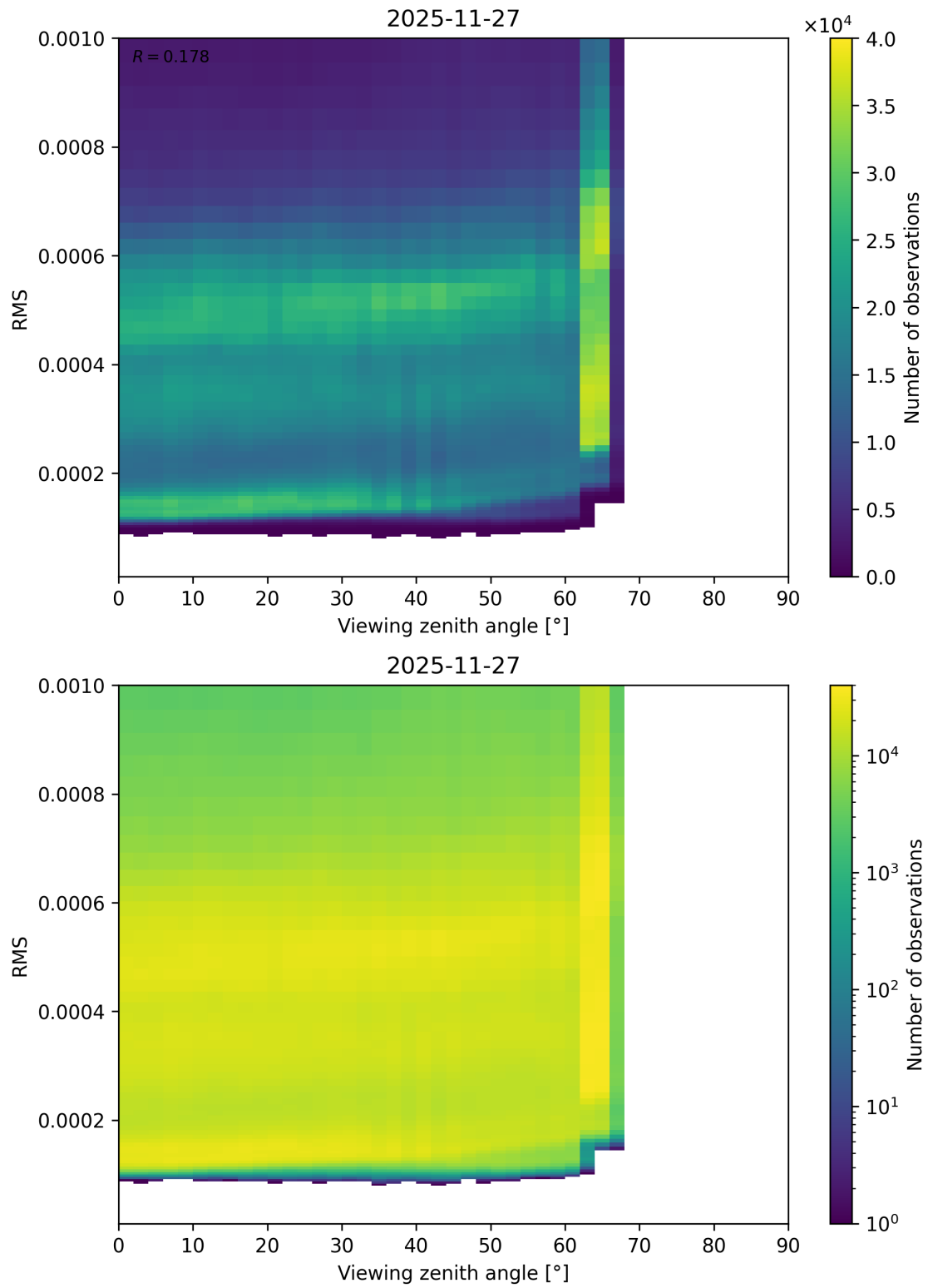
Figure 171: Scatter density plot of “Viewing zenith angle” against “RMS” for 2025-11-26 to 2025-11-28.
