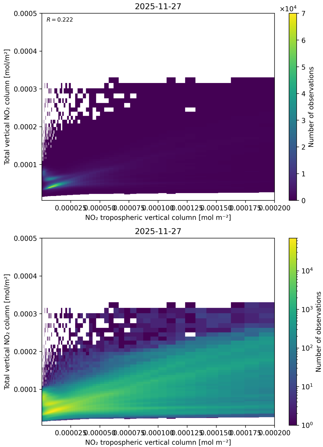
Figure 128: Scatter density plot of “NO 2 tropospheric vertical column” against “Total vertical NO 2 column” for 2025-11-26 to 2025-11-28.
