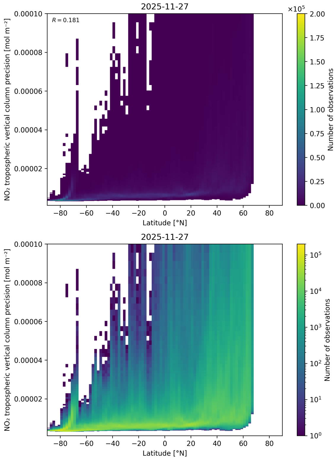
Figure 93: Scatter density plot of “Latitude” against “NO 2 tropospheric vertical column precision” for 2025-11-26 to 2025-11-28.
