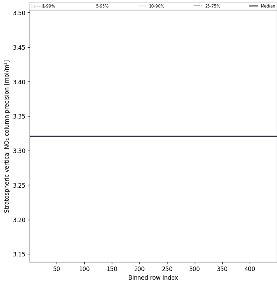
Figure 54: Along track statistics of “Stratospheric vertical NO 2 column precision” for 2025-11-26 to 2025-11-28
