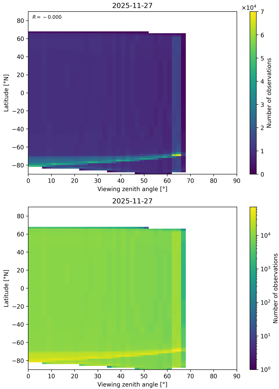
Figure 163: Scatter density plot of “Viewing zenith angle” against “Latitude” for 2025-11-26 to 2025-11-28.
