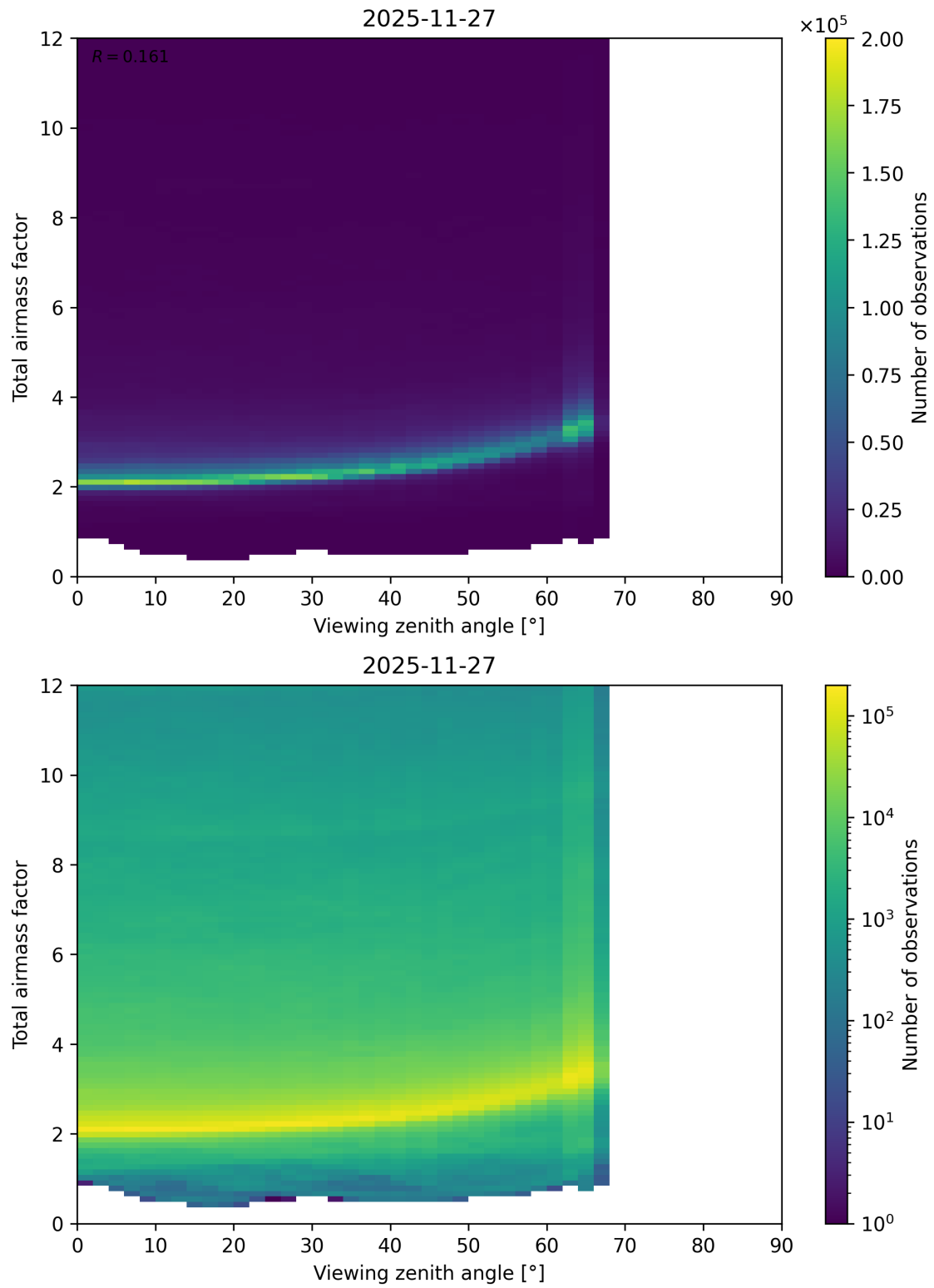
Figure 160: Scatter density plot of “Viewing zenith angle” against “Total airmass factor” for 2025-11-26 to 2025-11-28.
