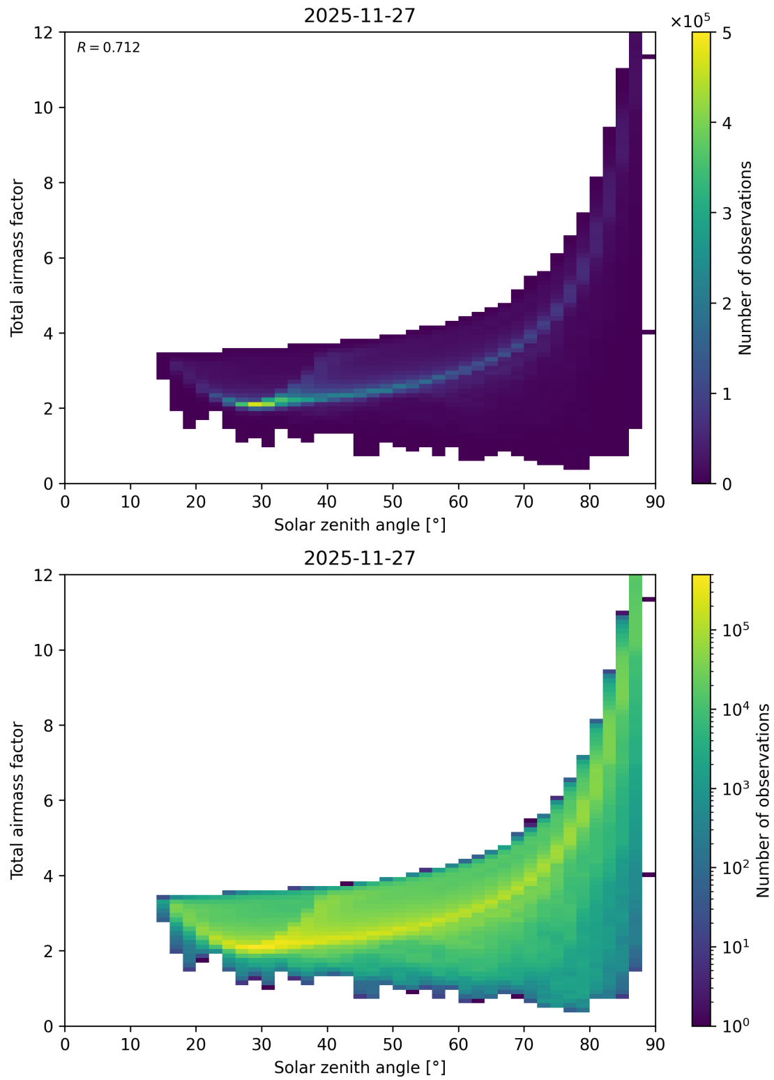
Figure 146: Scatter density plot of “Solar zenith angle” against “Total airmass factor” for 2025-11-26 to 2025-11-28.
