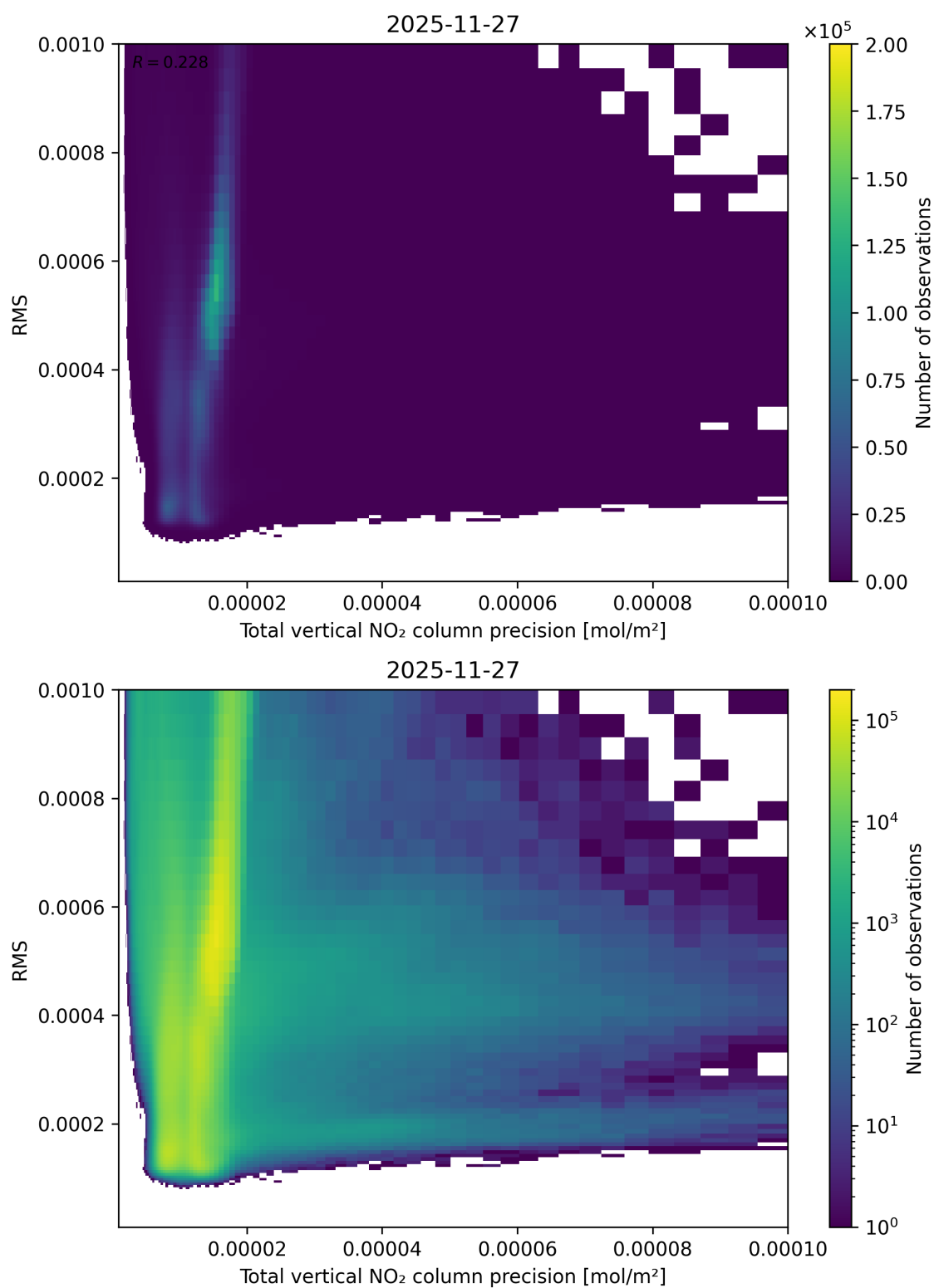
Figure 119: Scatter density plot of “Total vertical NO 2 column precision” against “RMS” for 2025-11-26 to 2025-11-28.
