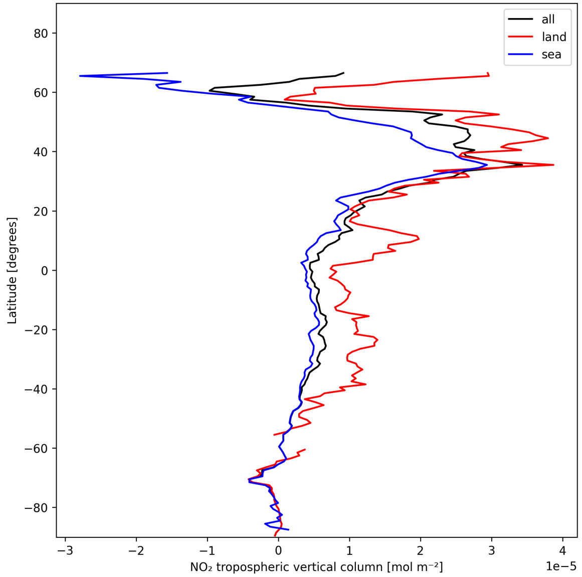
Figure 12: Zonal average of “NO 2 tropospheric vertical column” for 2025-11-26 to 2025-11-28.
