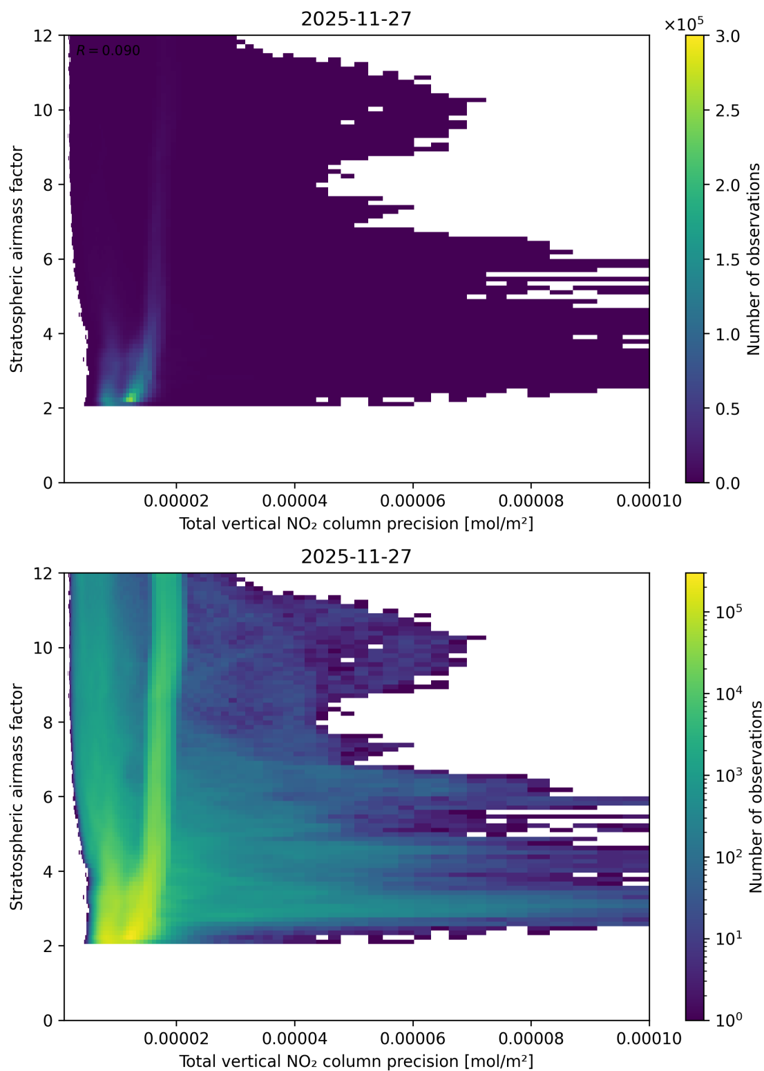
Figure 115: Scatter density plot of “Total vertical NO 2 column precision” against “Stratospheric air mass factor” for 2025-11-26 to 2025-11-28.
