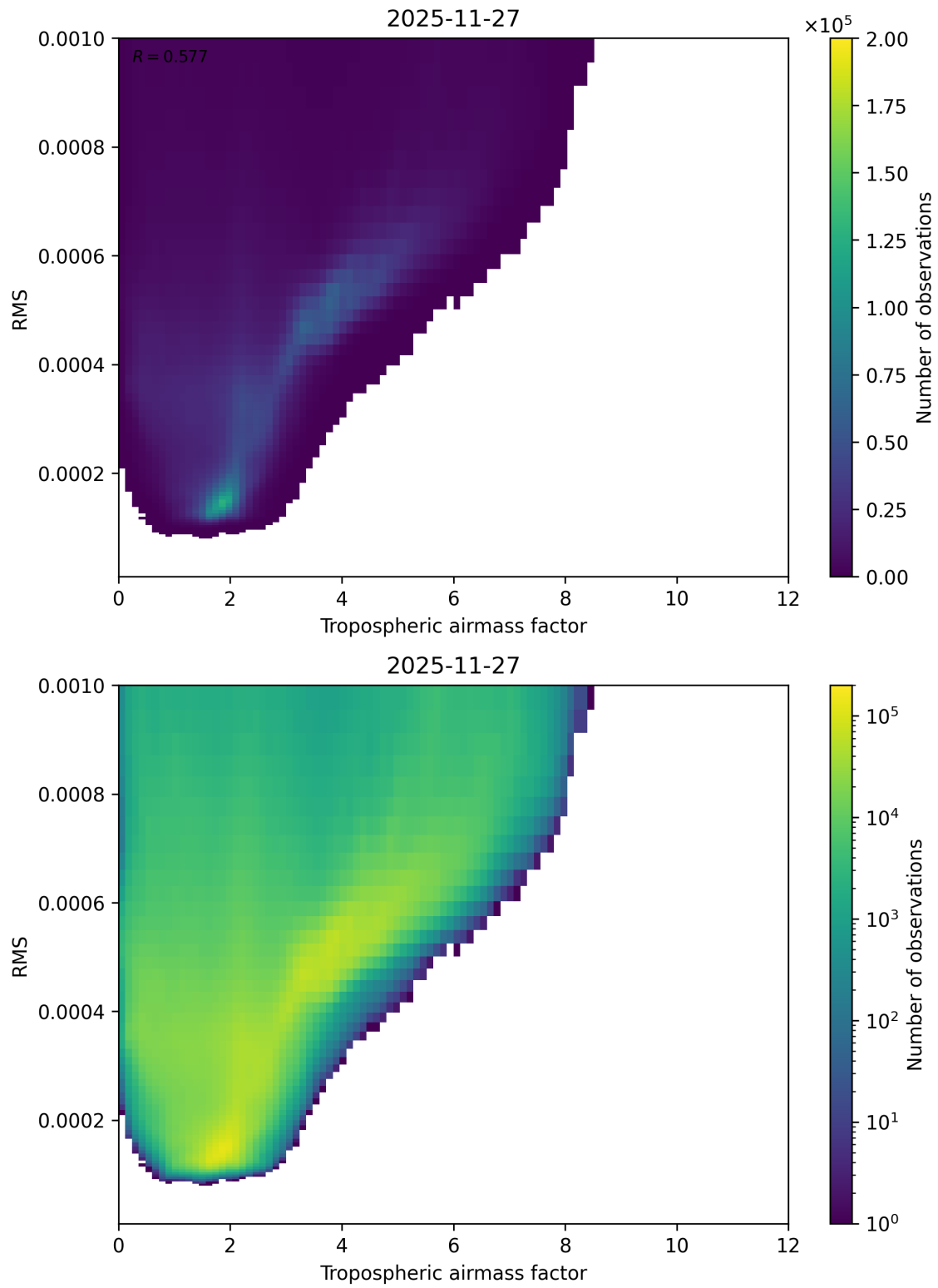
Figure 79: Scatter density plot of “Tropospheric airmass factor” against “RMS” for 2025-11-26 to 2025-11-28.
