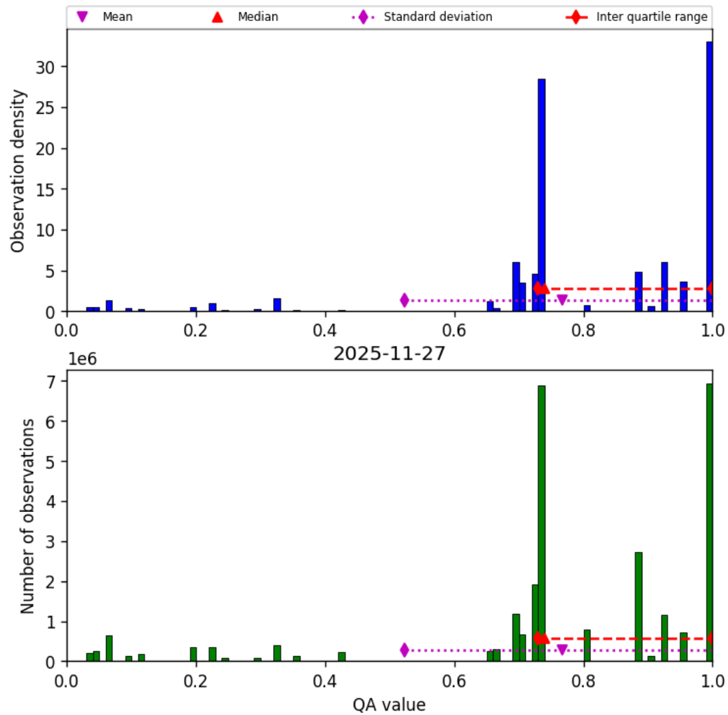
Figure 28: Histogram of “QA value” for 2025-11-26 to 2025-11-28
