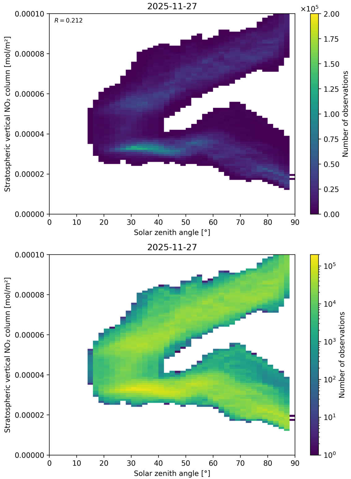
Figure 150: Scatter density plot of “Solar zenith angle” against “Stratospheric vertical NO 2 column” for 2025-11-26 to 2025-11-28.
