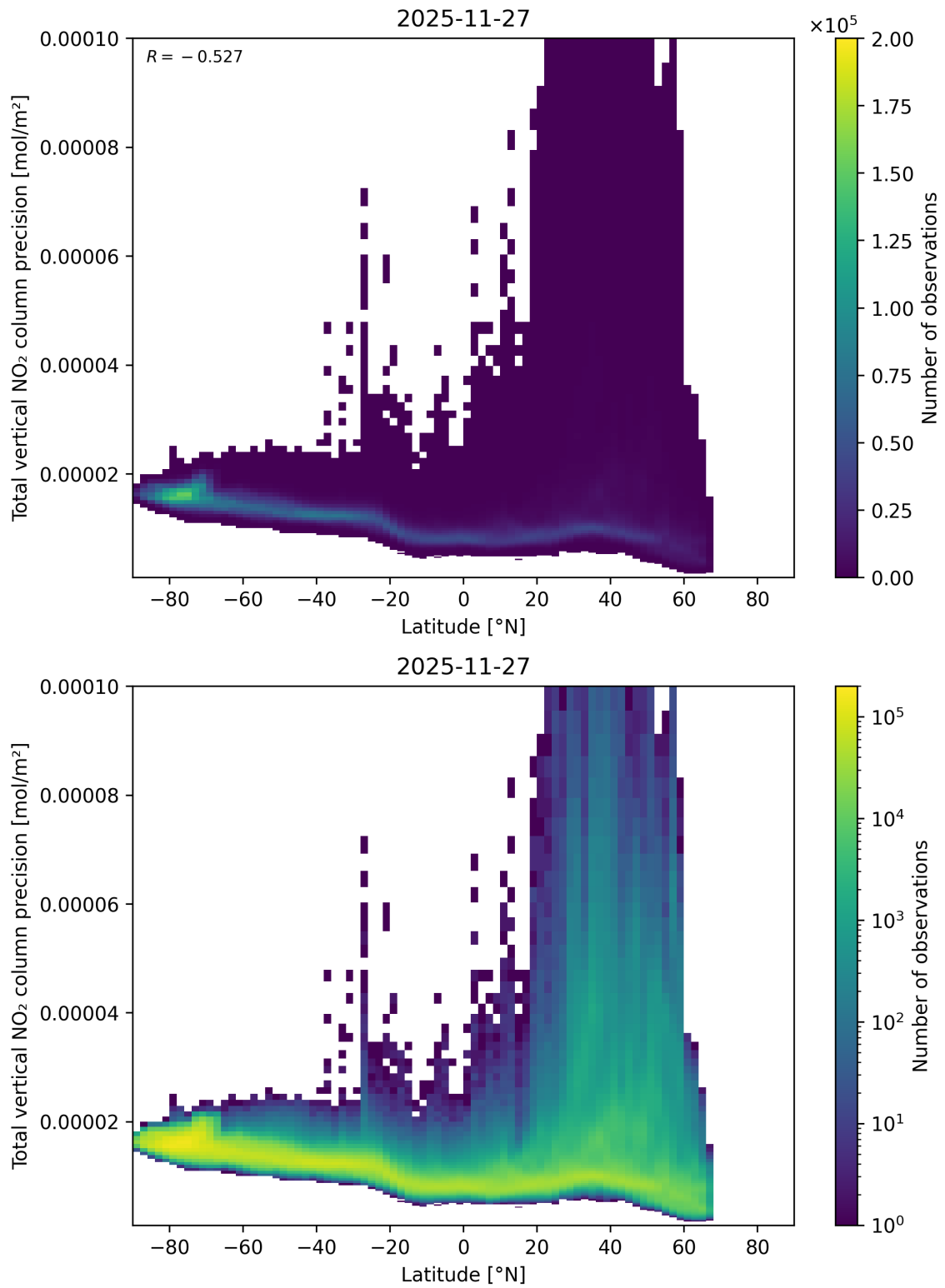
Figure 91: Scatter density plot of “Latitude” against “Total vertical NO 2 column precision” for 2025-11-26 to 2025-11-28.
