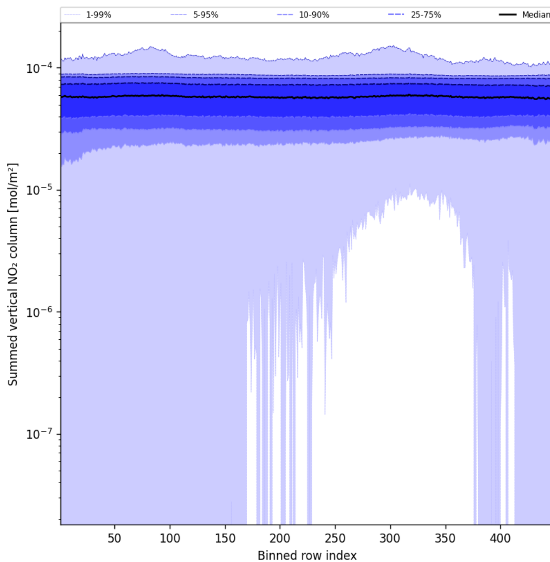
Figure 57: Along track statistics of “Summed vertical NO 2 column” for 2025-11-26 to 2025-11-28
