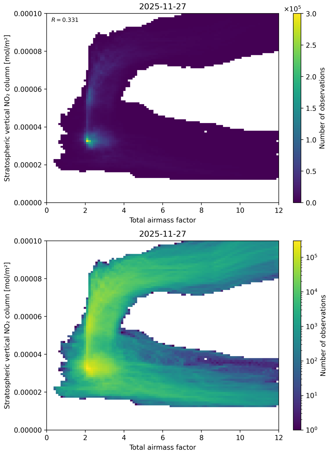
Figure 64: Scatter density plot of “Total airmass factor” against “Stratospheric vertical \text{NO}_2 column” for 2025-11-26 to 2025-11-28.
