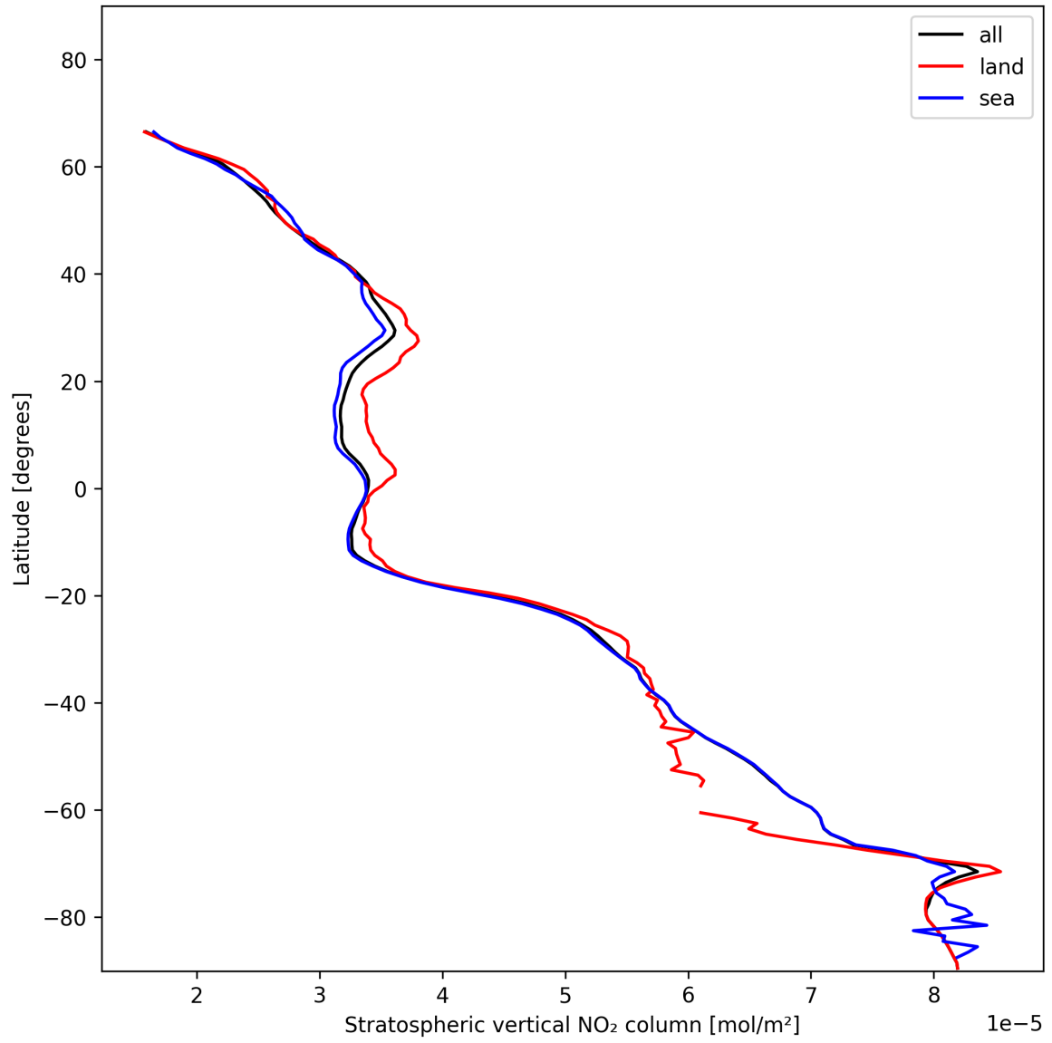
Figure 19: Zonal average of “Stratospheric vertical NO 2 column” for 2025-11-26 to 2025-11-28.
