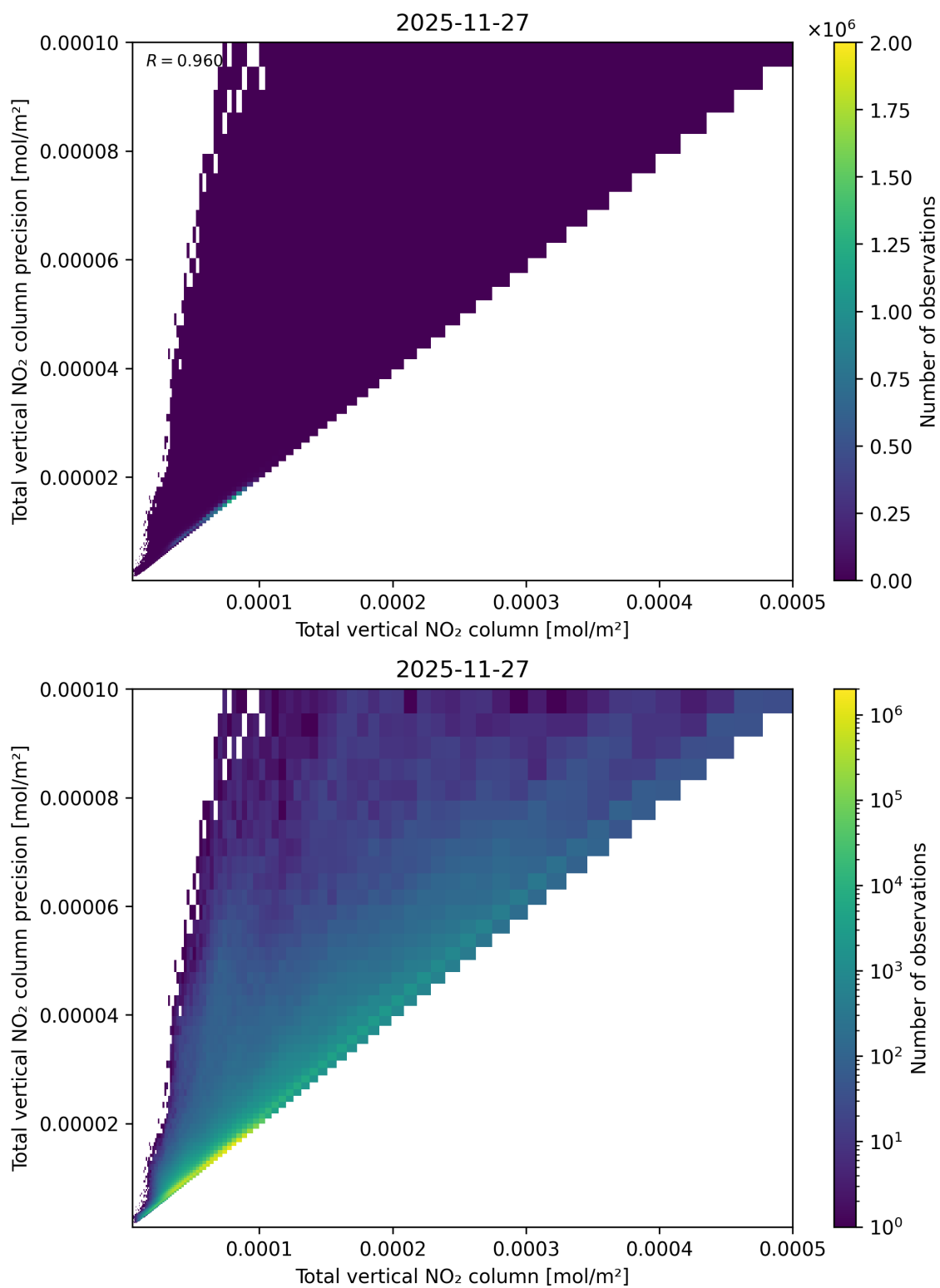
Figure 114: Scatter density plot of “Total vertical NO 2 column” against “Total vertical NO 2 column precision” for 2025-11-26 to 2025-11-28.
