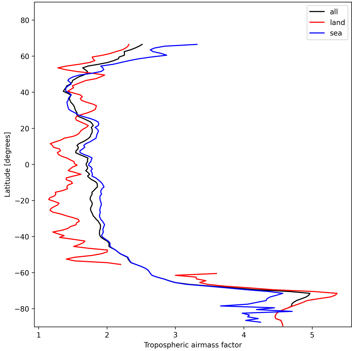
Figure 14: Zonal average of “Tropospheric air mass factor” for 2025-11-26 to 2025-11-28.
