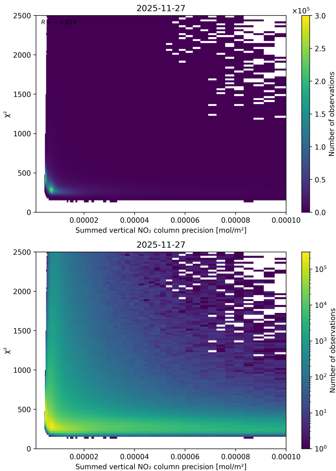
Figure 107: Scatter density plot of “Summed vertical NO 2 column precision” against “ \chi^2 ” for 2025-11-26 to 2025-11-28.
