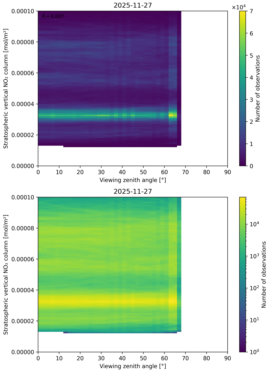
Figure 164: Scatter density plot of “Viewing zenith angle” against “Stratospheric vertical NO 2 column” for 2025-11-26 to 2025-11-28.
