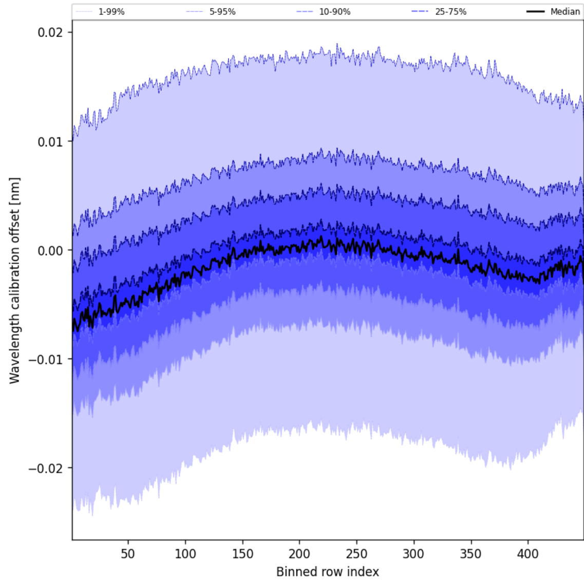
Figure 52: Along track statistics of “Wavelength calibration offset” for 2025-11-26 to 2025-11-28
