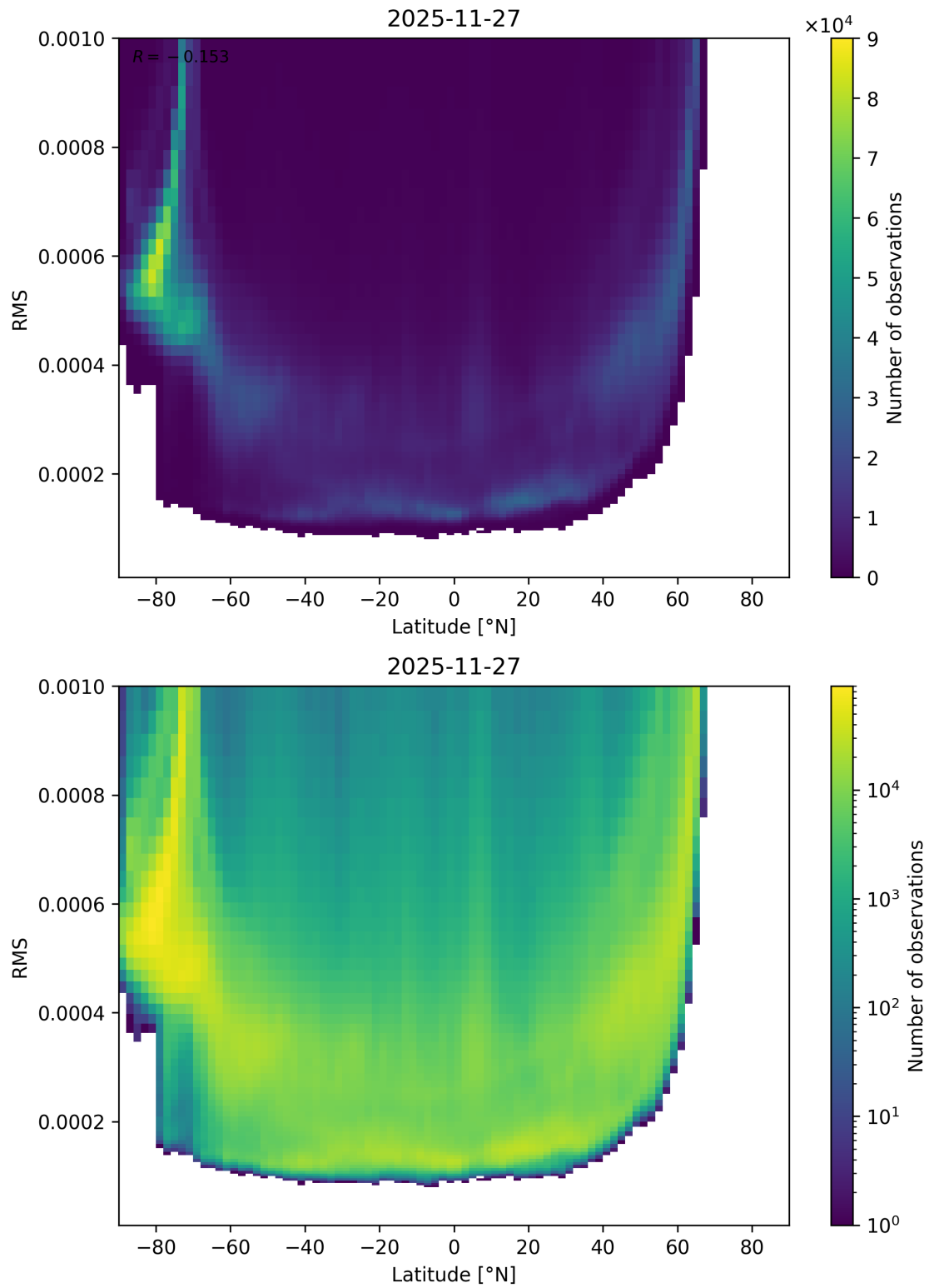
Figure 94: Scatter density plot of “Latitude” against “RMS” for 2025-11-26 to 2025-11-28.
