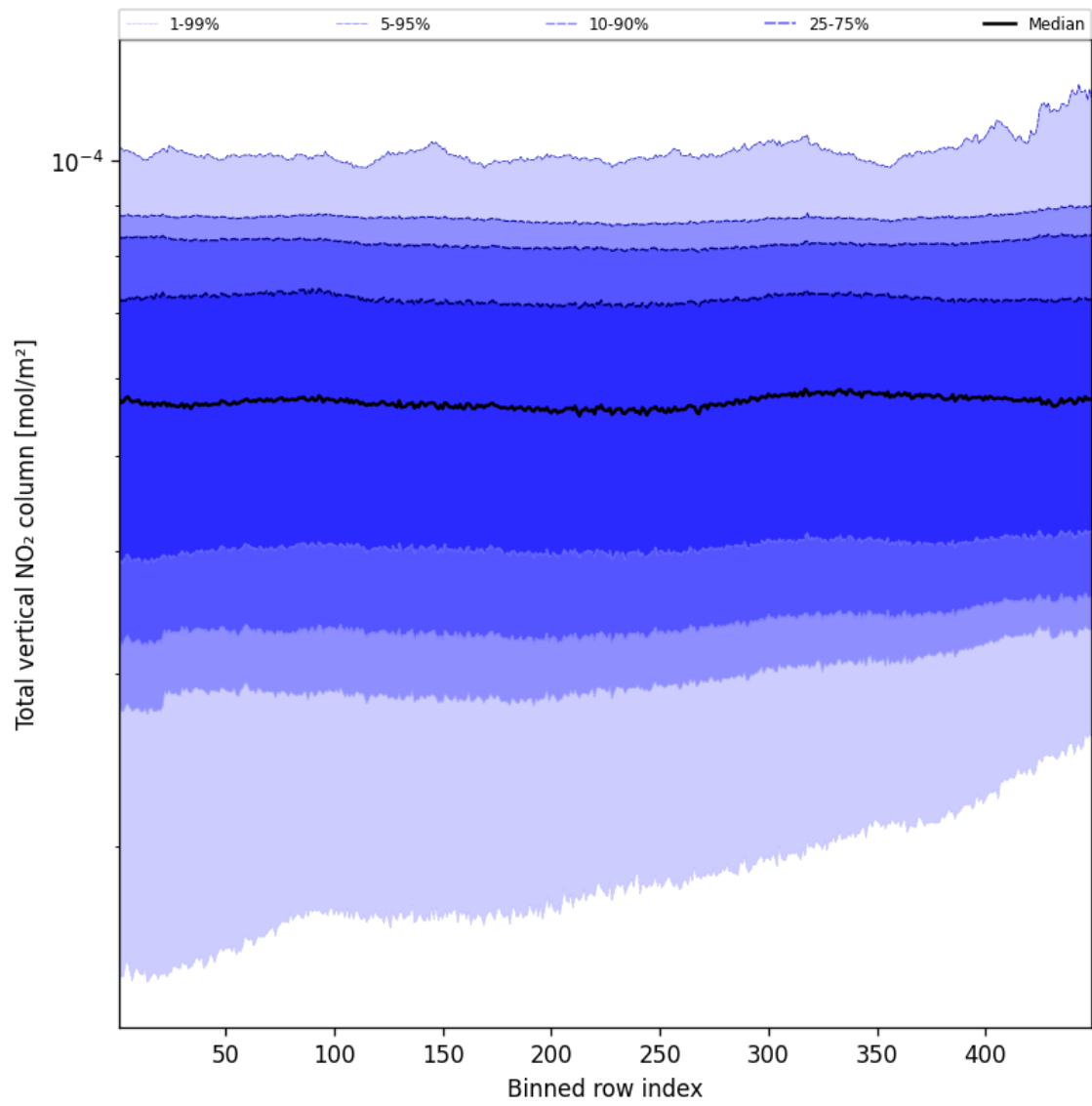
Figure 55: Along track statistics of “Total vertical NO 2 column” for 2025-11-26 to 2025-11-28
