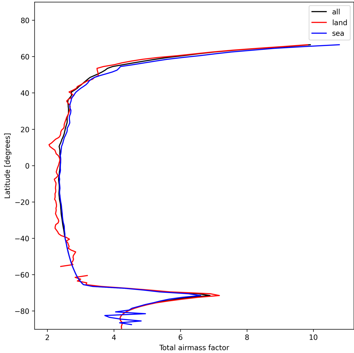
Figure 15: Zonal average of “Total airmass factor” for 2025-11-26 to 2025-11-28.
