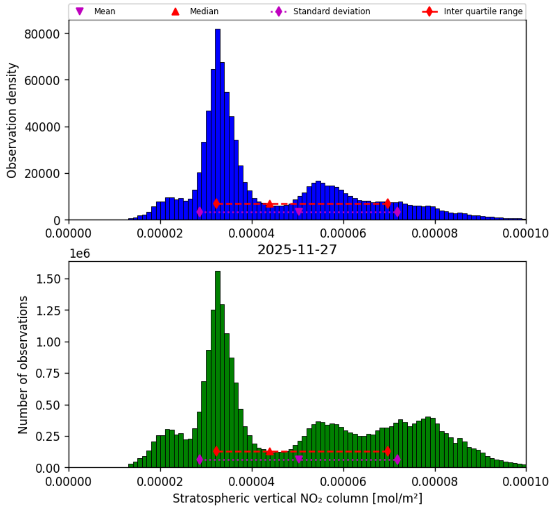
Figure 36: Histogram of “Stratospheric vertical NO 2 column” for 2025-11-26 to 2025-11-28
