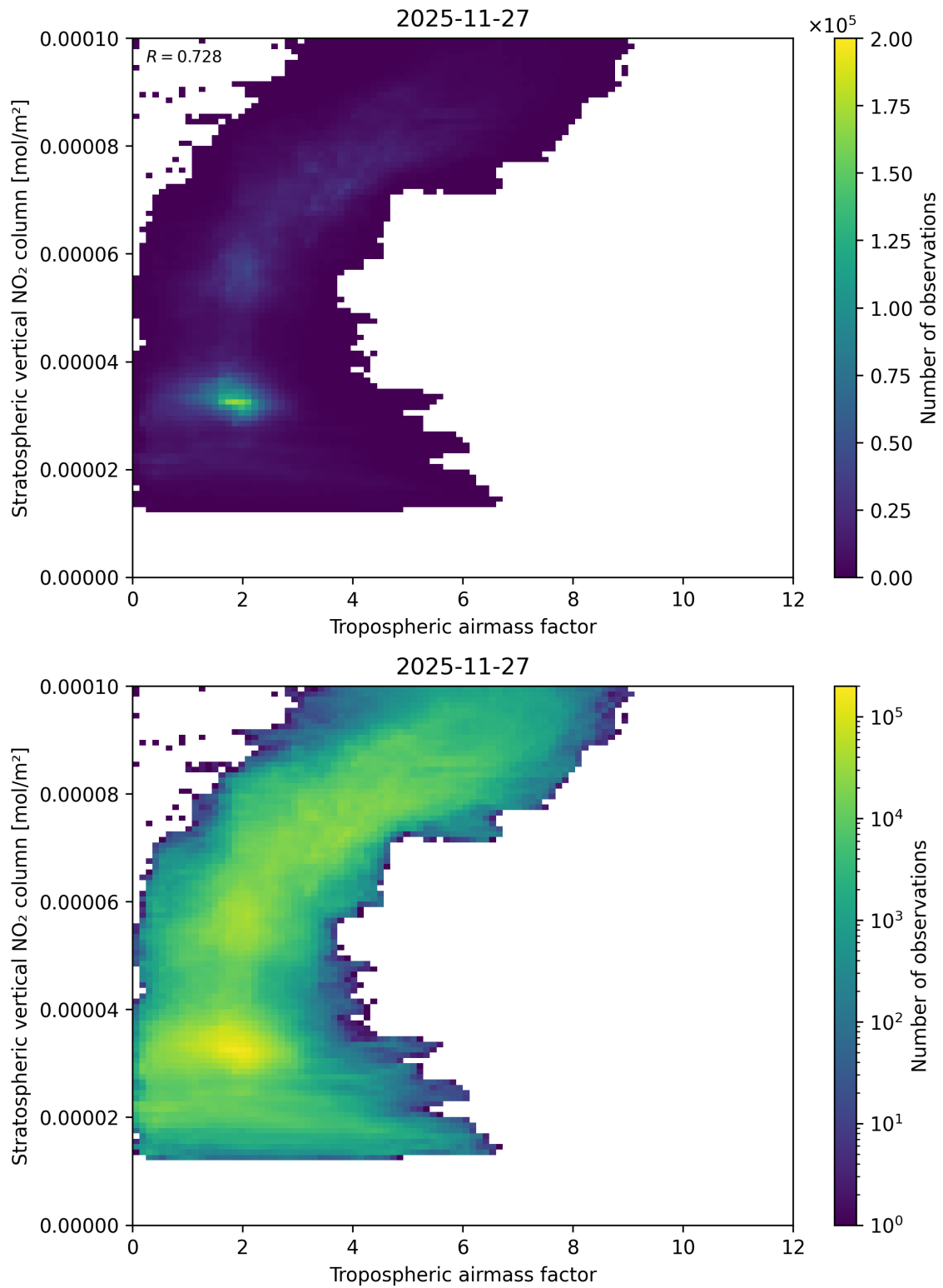
Figure 74: Scatter density plot of “Tropospheric air mass factor” against “Stratospheric vertical NO 2 column” for 2025-11-26 to 2025-11-28.
