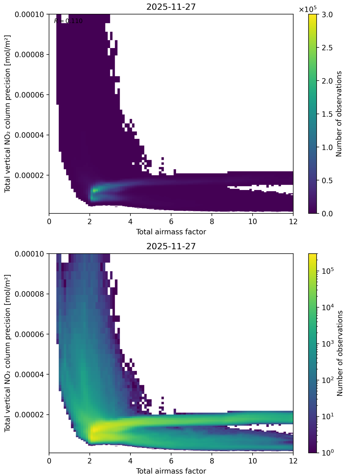
Figure 68: Scatter density plot of “Total airmass factor” against “Total vertical NO 2 column precision” for 2025-11-26 to 2025-11-28.
