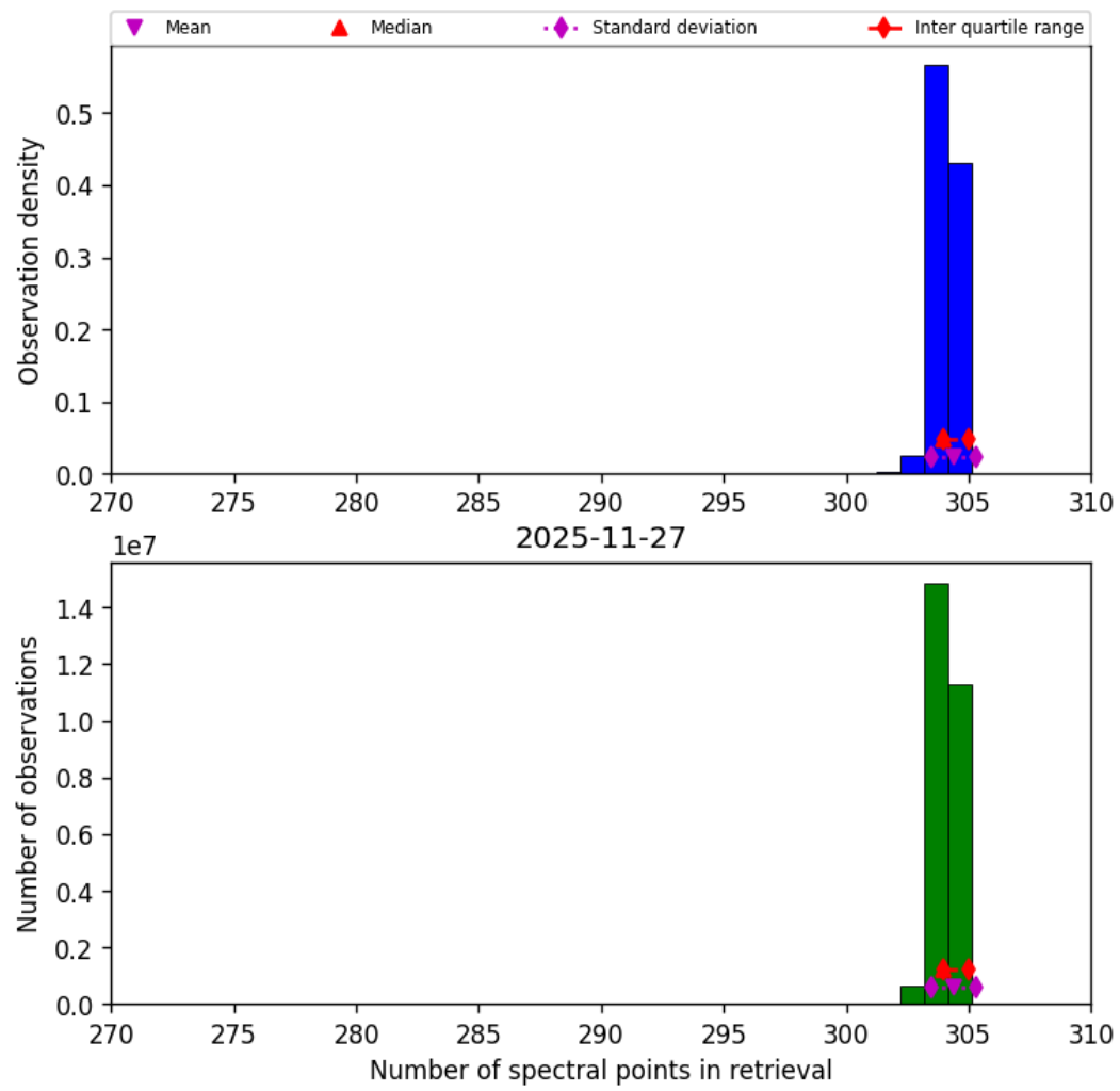
Figure 33: Histogram of “Number of spectral points in retrieval” for 2025-11-26 to 2025-11-28
