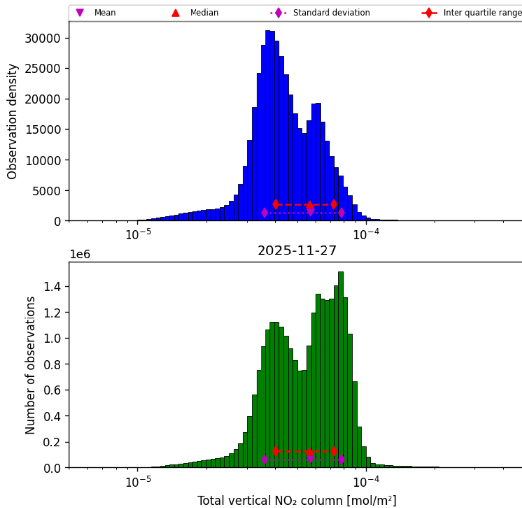
Figure 38: Histogram of “Total vertical NO 2 column” for 2025-11-26 to 2025-11-28
