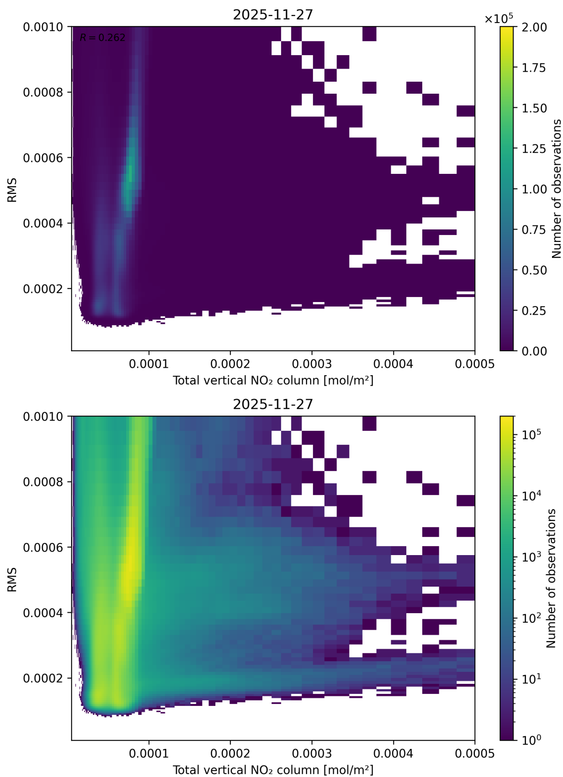
Figure 120: Scatter density plot of “Total vertical NO 2 column” against “RMS” for 2025-11-26 to 2025-11-28.
