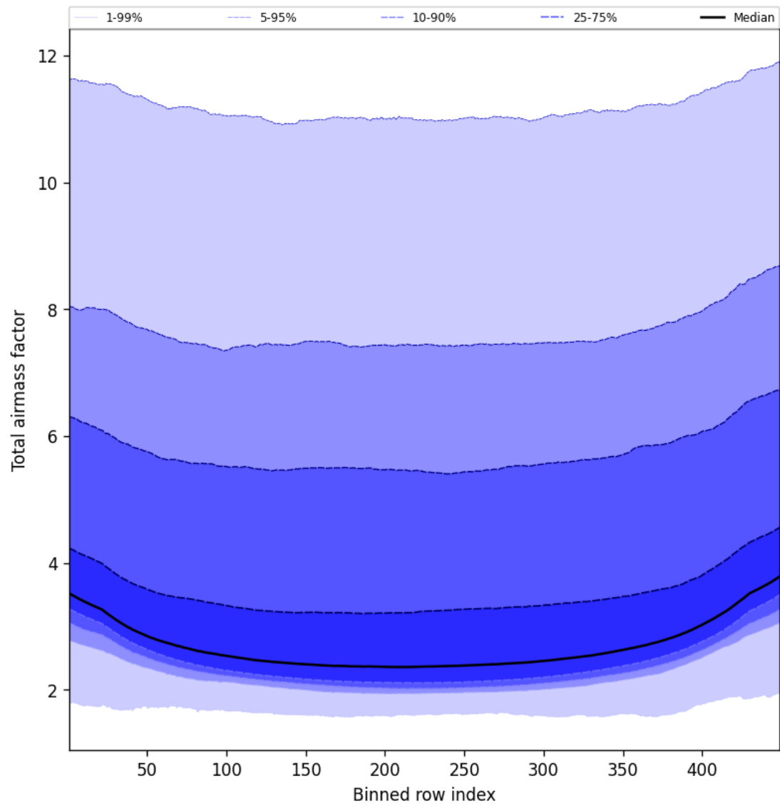
Figure 49: Along track statistics of “Total airmass factor” for 2025-11-26 to 2025-11-28
