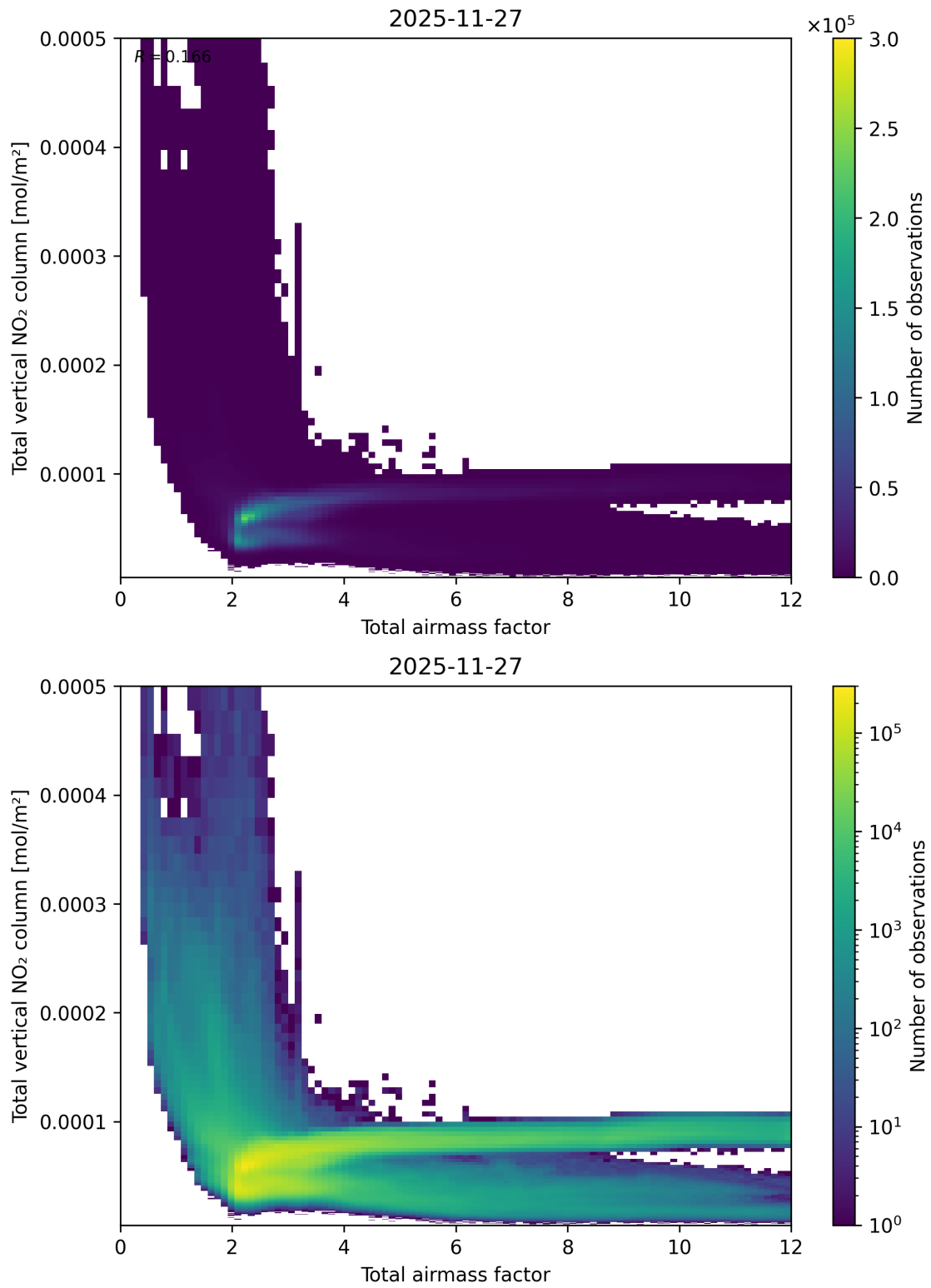
Figure 67: Scatter density plot of “Total airmass factor” against “Total vertical NO 2 column” for 2025-11-26 to 2025-11-28.
