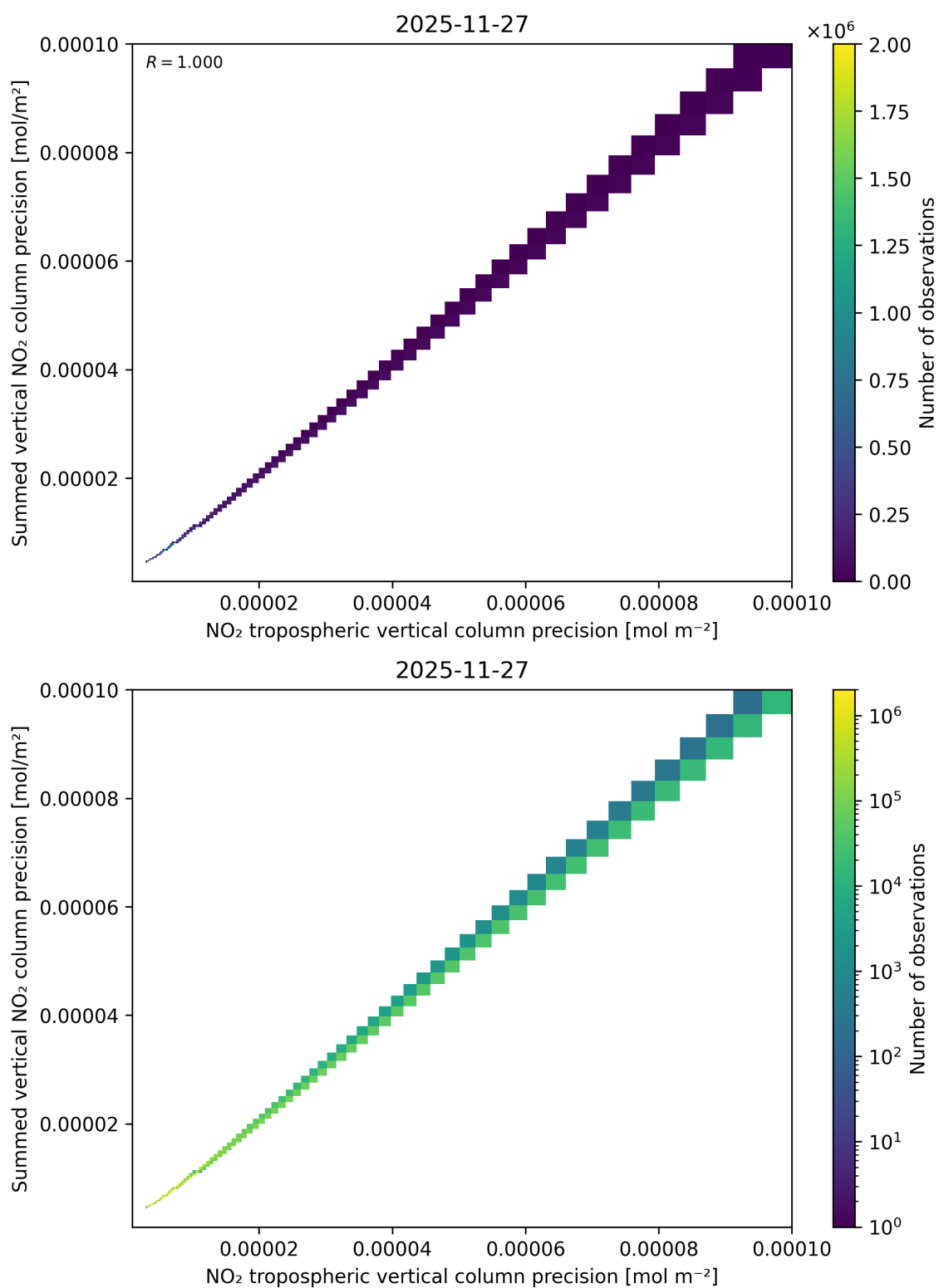
Figure 137: Scatter density plot of “NO 2 tropospheric vertical column precision” against “Summed vertical NO 2 column precision” for 2025-11-26 to 2025-11-28.
