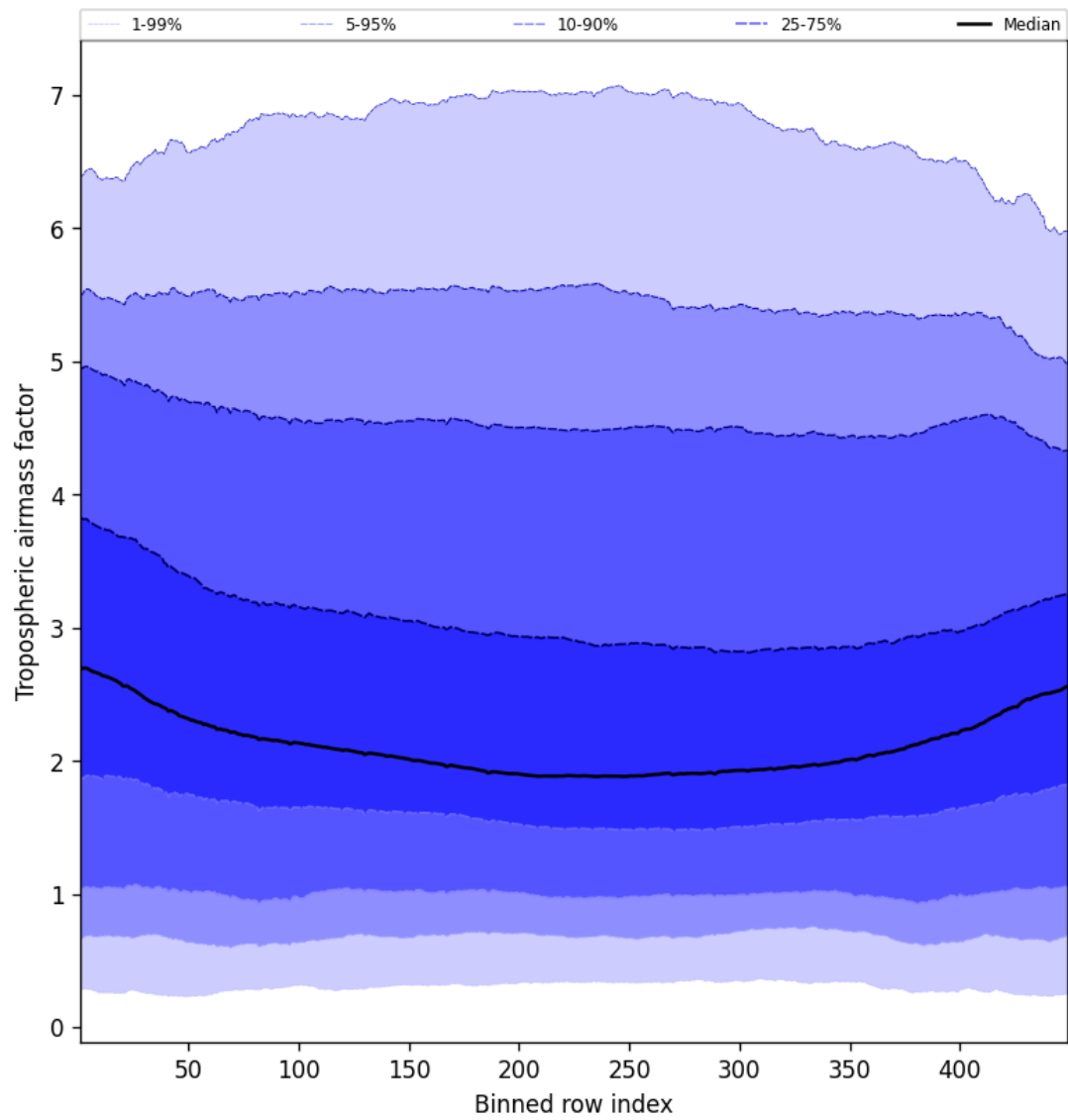
Figure 48: Along track statistics of “Tropospheric airmass factor” for 2025-11-26 to 2025-11-28
