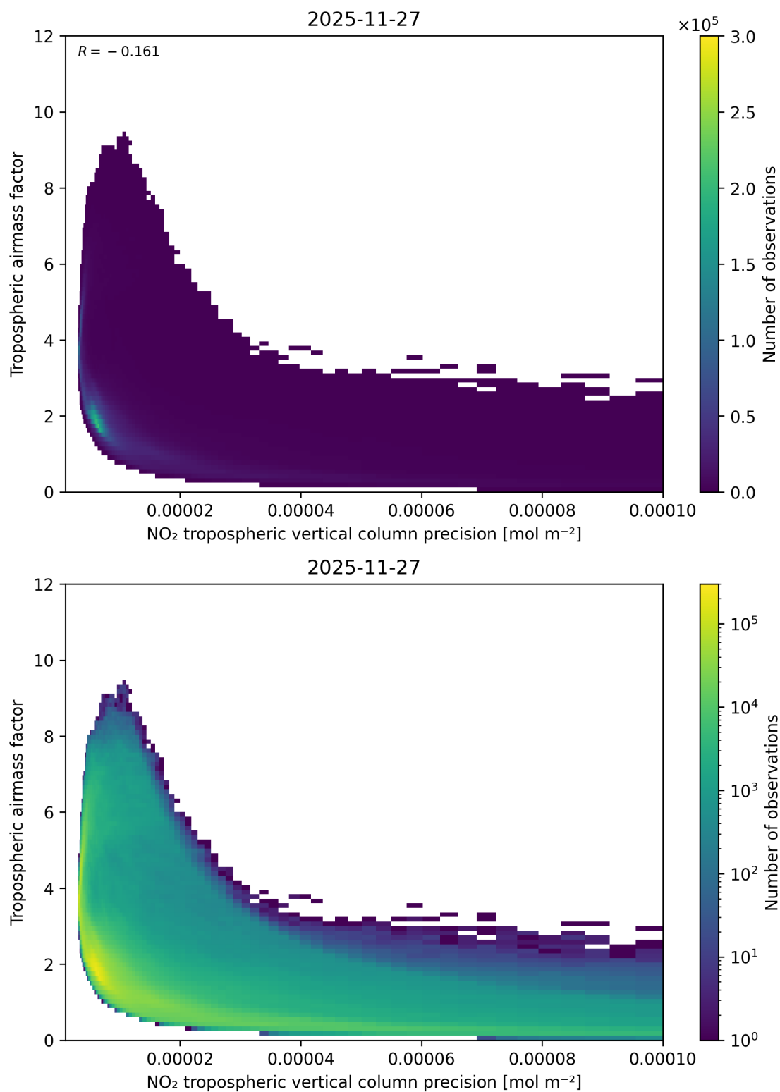
Figure 133: Scatter density plot of “NO 2 tropospheric vertical column precision” against “Tropospheric air mass factor” for 2025-11-26 to 2025-11-28.
