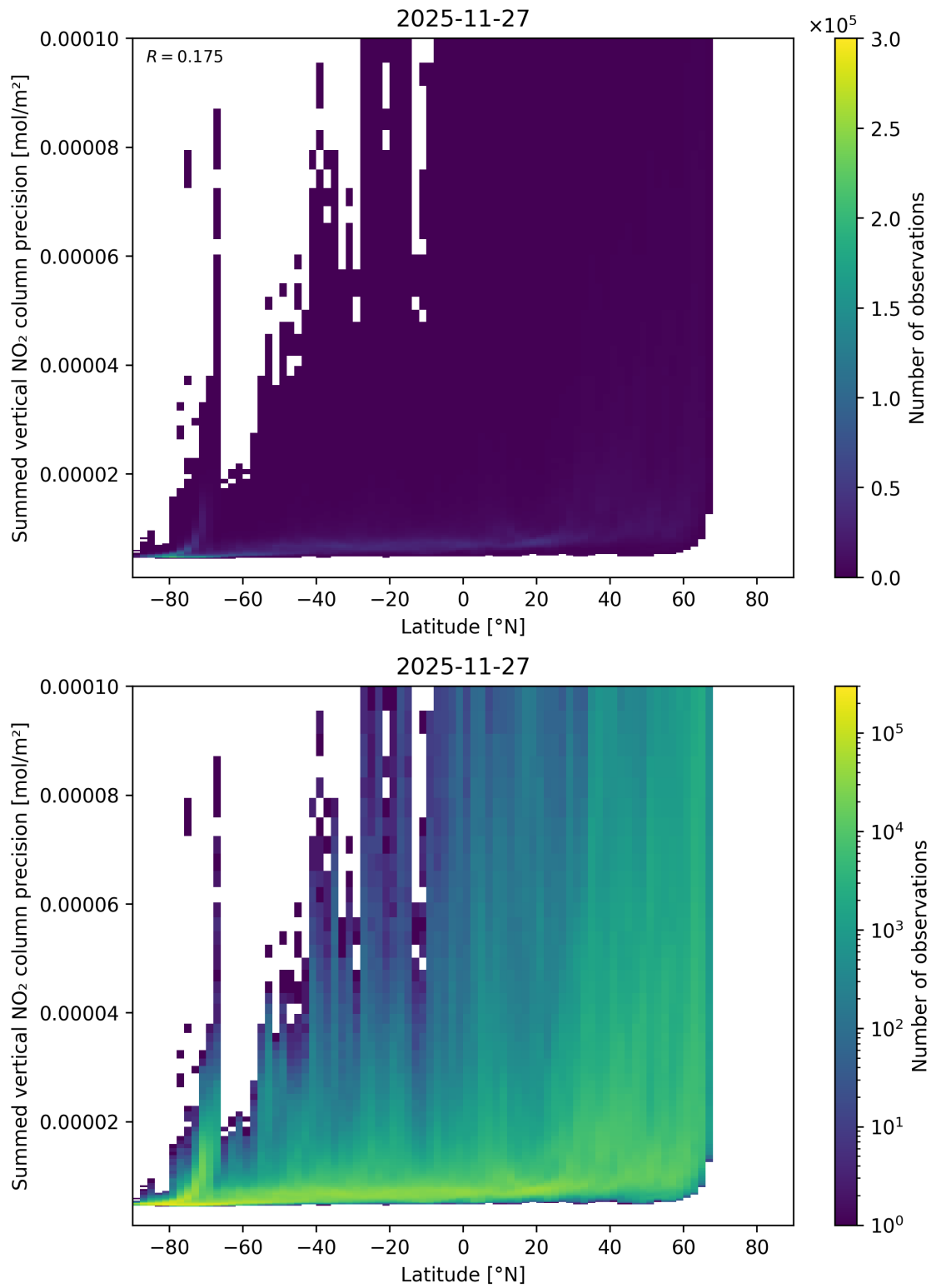
Figure 89: Scatter density plot of “Latitude” against “Summed vertical NO 2 column precision” for 2025-11-26 to 2025-11-28.
