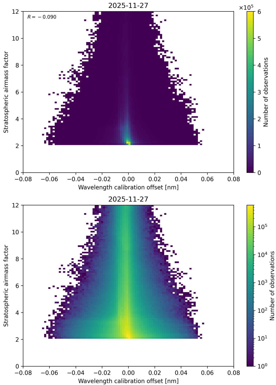
Figure 174: Scatter density plot of “Wavelength calibration offset” against “Stratospheric air mass factor” for 2025-11-26 to 2025-11-28.
