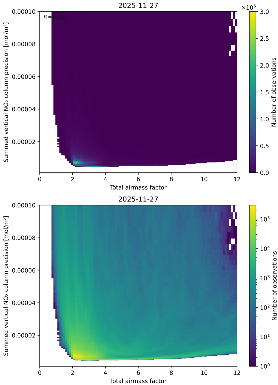
Figure 66: Scatter density plot of “Total airmass factor” against “Summed vertical NO 2 column precision” for 2025-11-26 to 2025-11-28.
