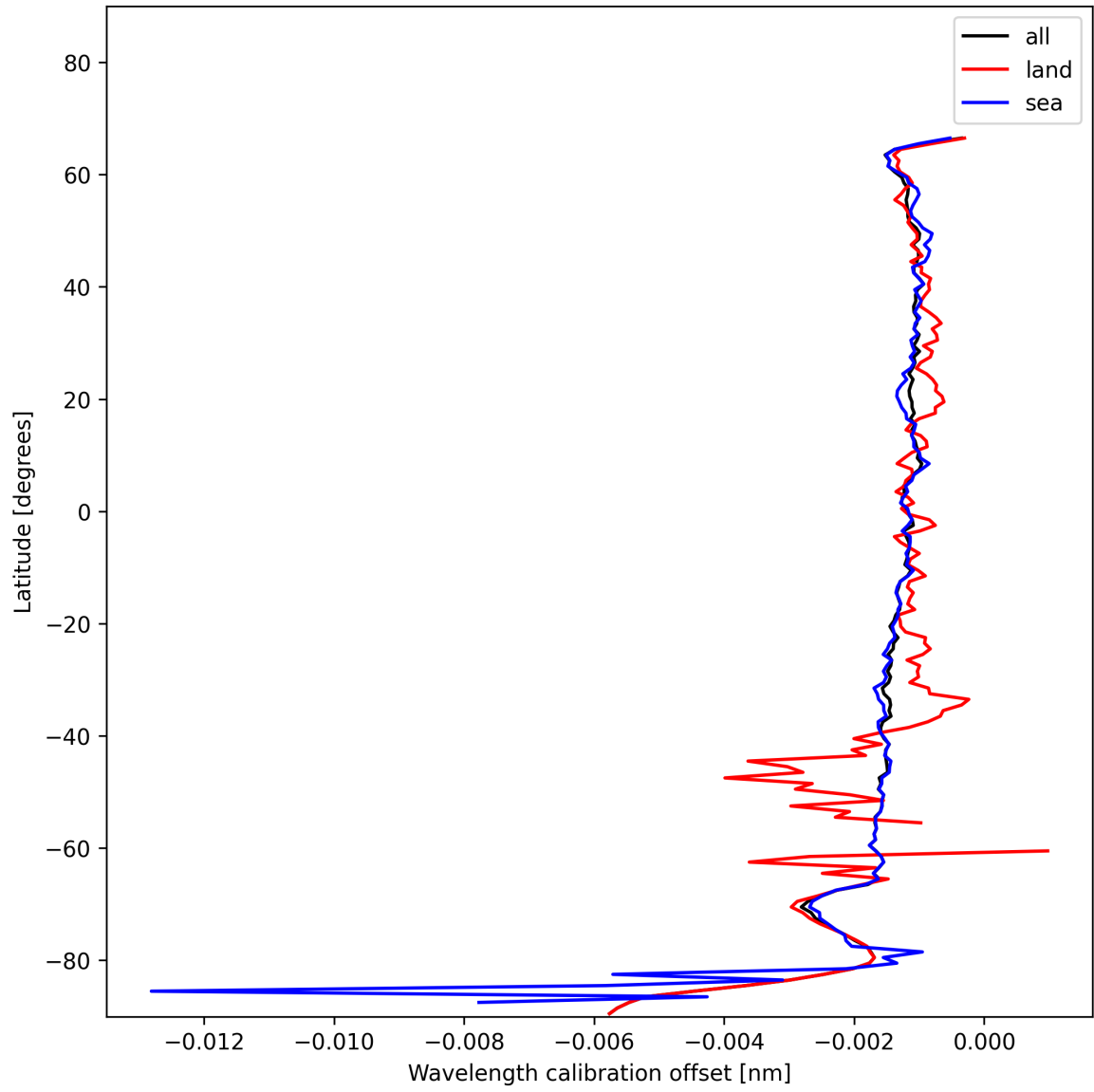
Figure 18: Zonal average of “Wavelength calibration offset” for 2025-11-26 to 2025-11-28.
