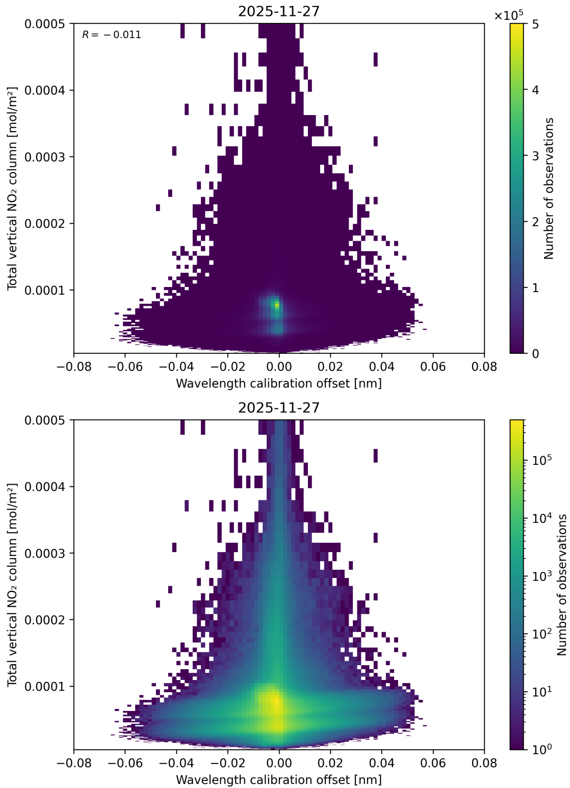
Figure 179: Scatter density plot of “Wavelength calibration offset” against “Total vertical NO 2 column” for 2025-11-26 to 2025-11-28.
