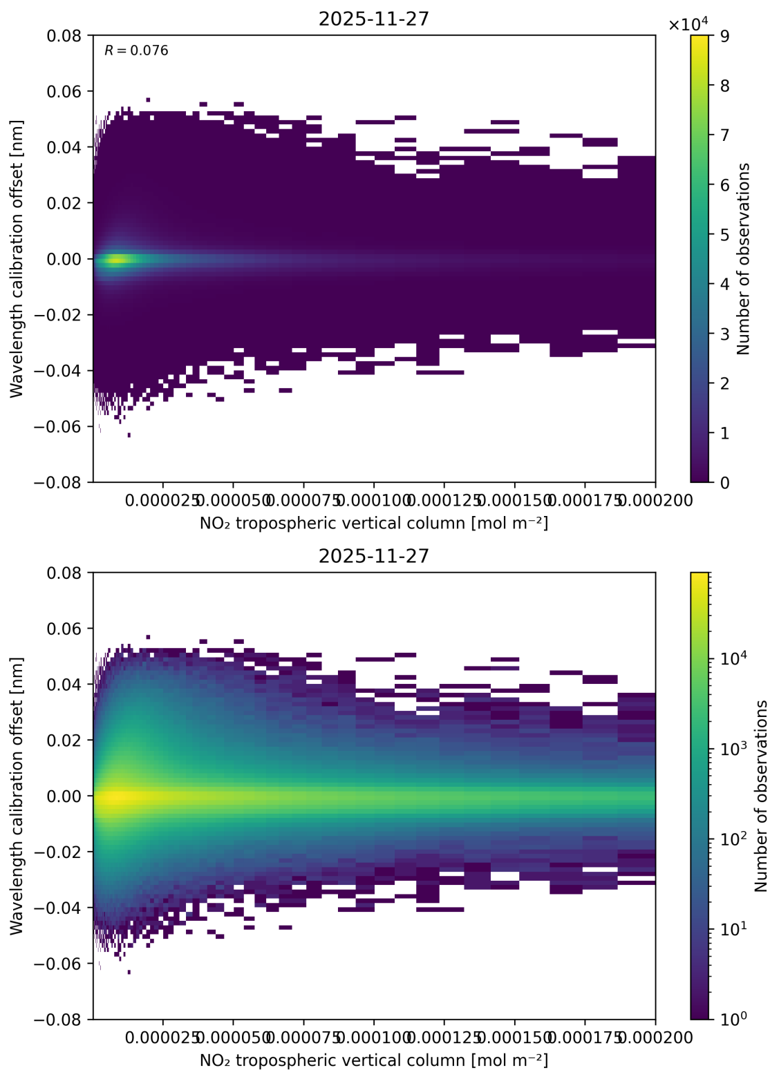
Figure 143: Scatter density plot of “NO 2 tropospheric vertical column” against “Wavelength calibration offset” for 2025-11-26 to 2025-11-28.
