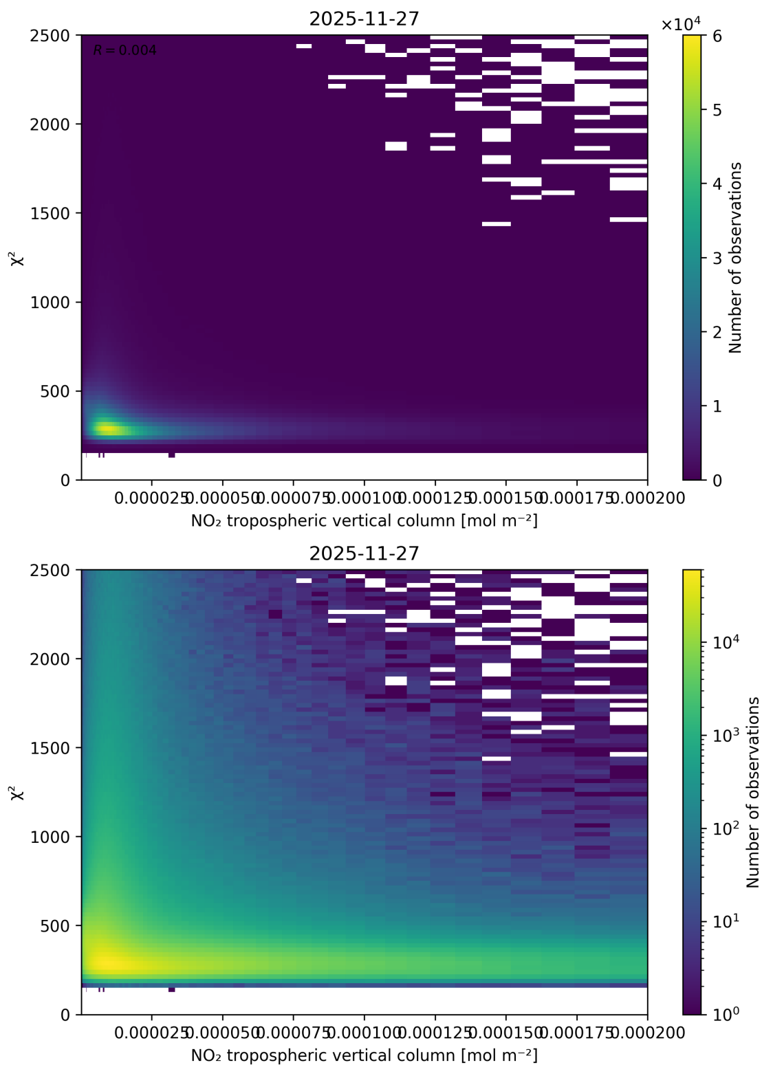
Figure 124: Scatter density plot of “NO 2 tropospheric vertical column” against “ \chi^2 ” for 2025-11-26 to 2025-11-28.
