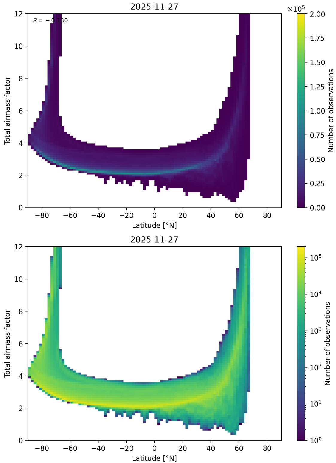
Figure 84: Scatter density plot of “Latitude” against “Total airmass factor” for 2025-11-26 to 2025-11-28.
