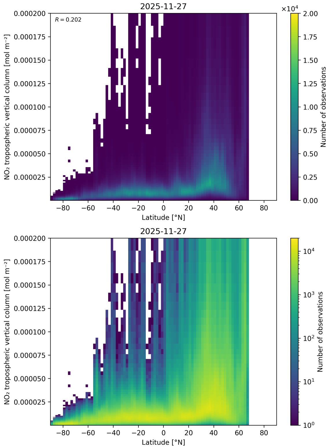
Figure 92: Scatter density plot of “Latitude” against “NO 2 tropospheric vertical column” for 2025-11-26 to 2025-11-28.
