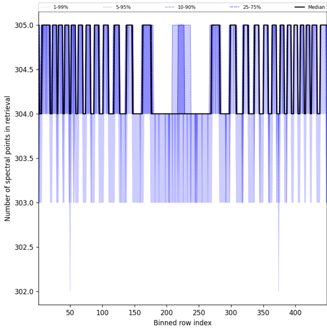
Figure 50: Along track statistics of “Number of spectral points in retrieval” for 2025-11-26 to 2025-11-28
