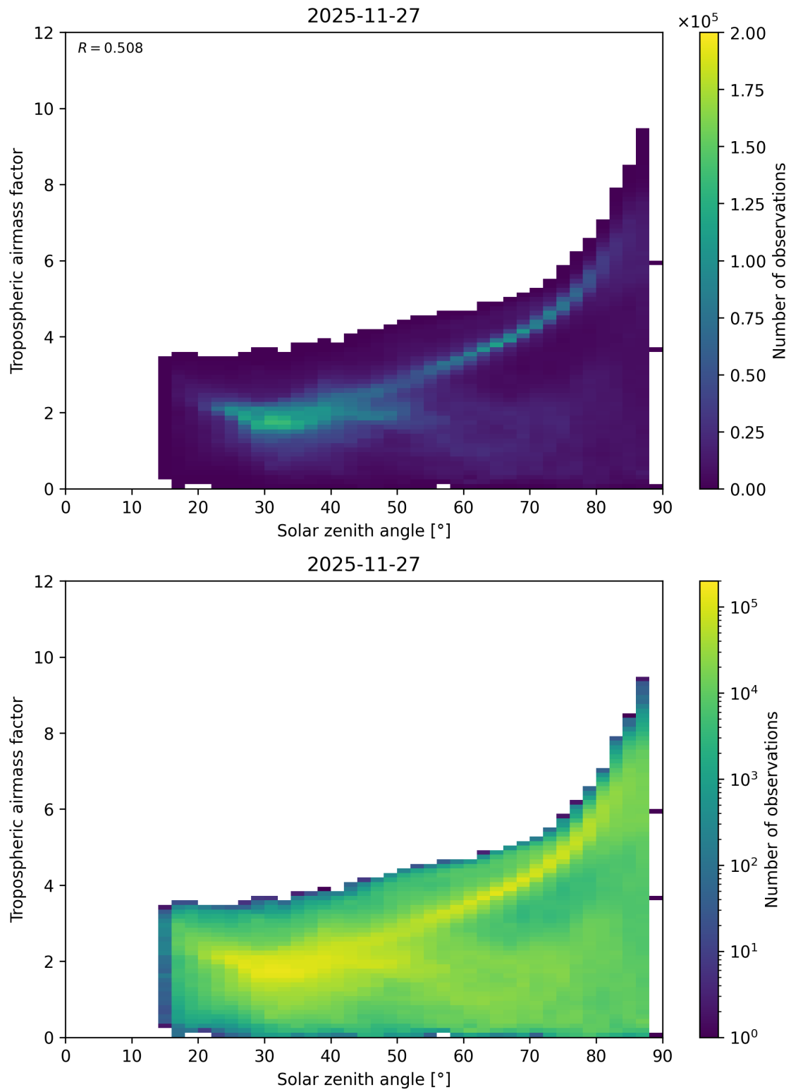
Figure 147: Scatter density plot of “Solar zenith angle” against “Tropospheric airmass factor” for 2025-11-26 to 2025-11-28.
