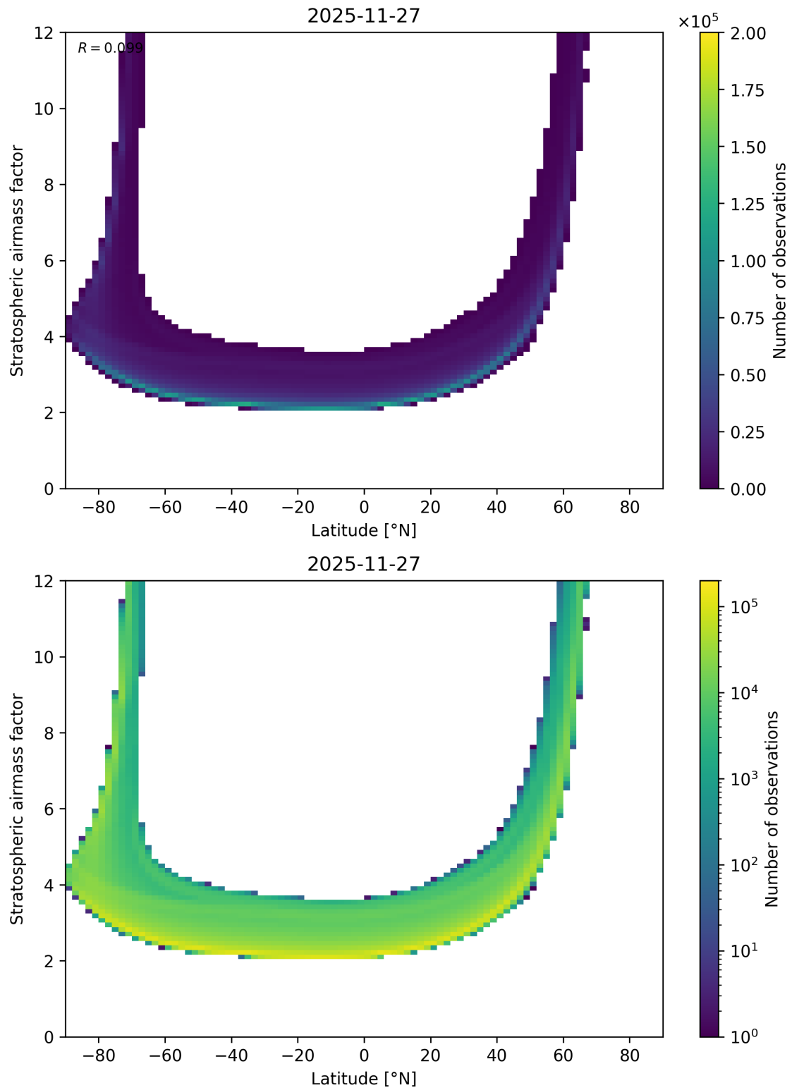
Figure 83: Scatter density plot of “Latitude” against “Stratospheric air mass factor” for 2025-11-26 to 2025-11-28.
