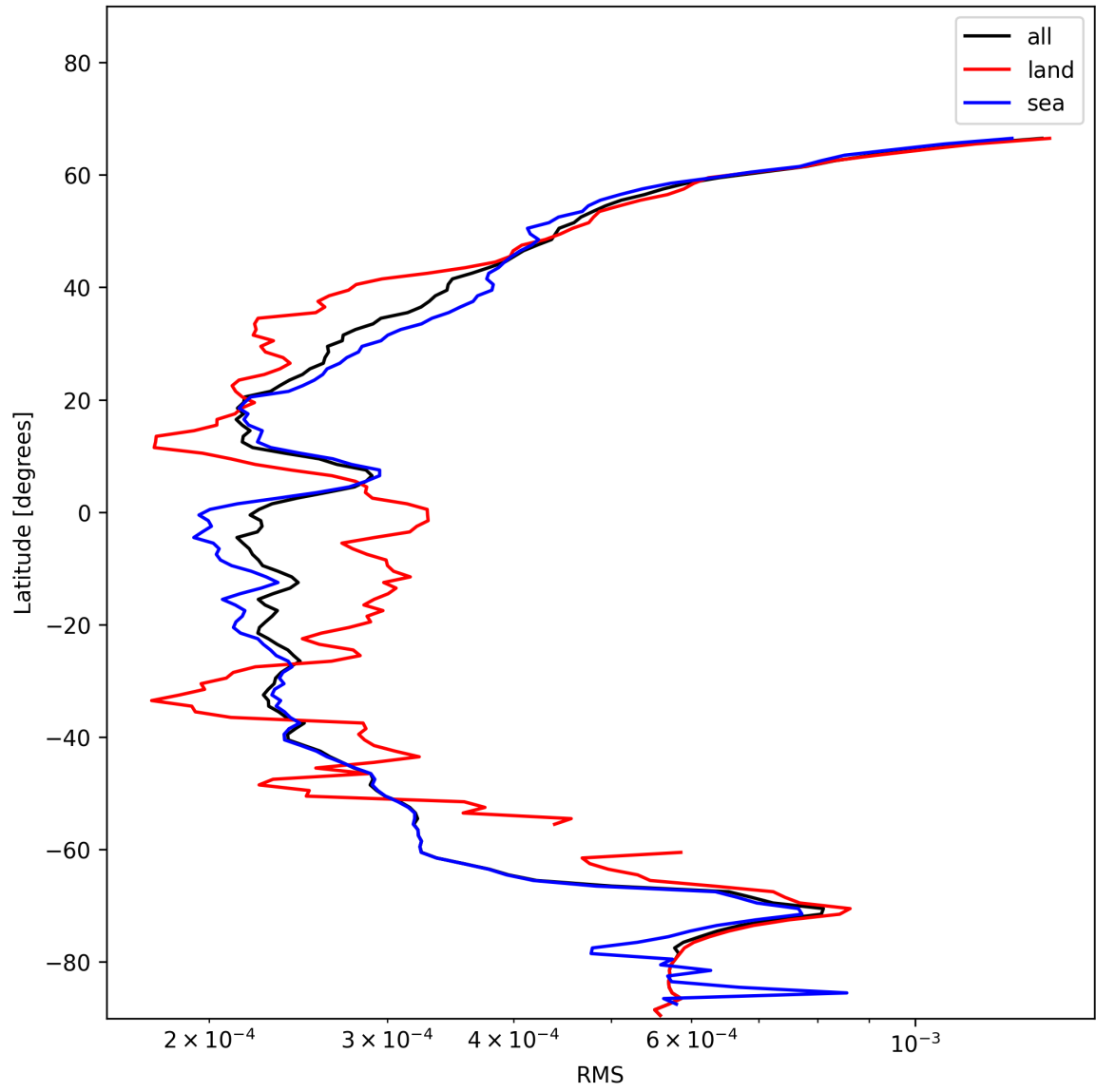
Figure 26: Zonal average of “RMS” for 2025-11-26 to 2025-11-28.
