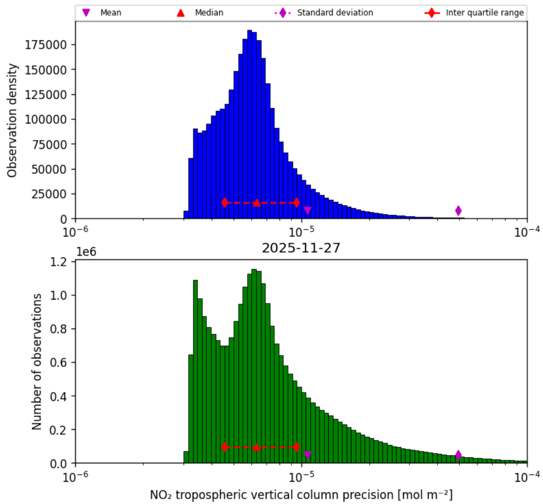
Figure 30: Histogram of “NO 2 tropospheric vertical column precision” for 2025-11-26 to 2025-11-28
