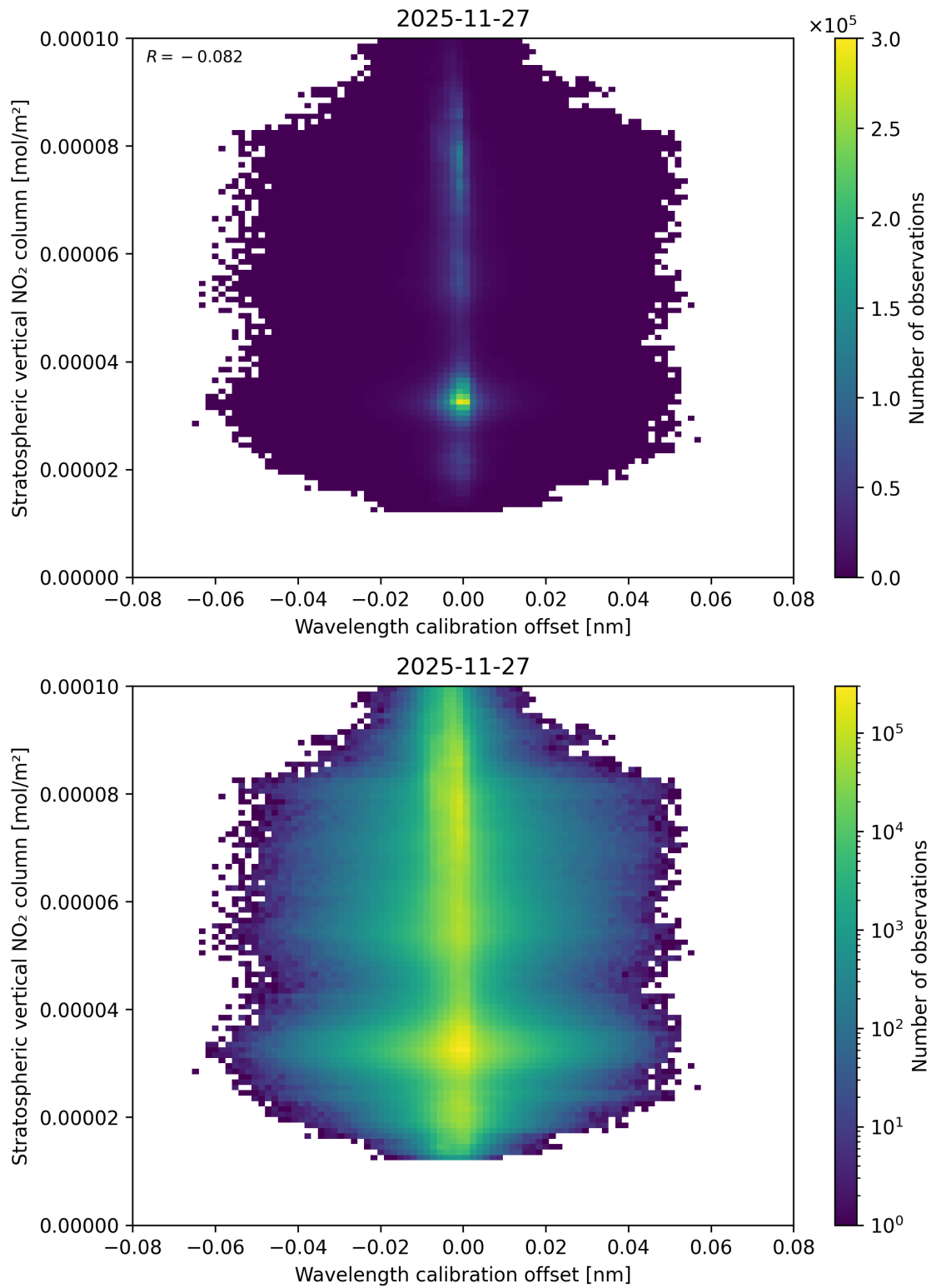
Figure 176: Scatter density plot of “Wavelength calibration offset” against “Stratospheric vertical NO 2 column” for 2025-11-26 to 2025-11-28.
