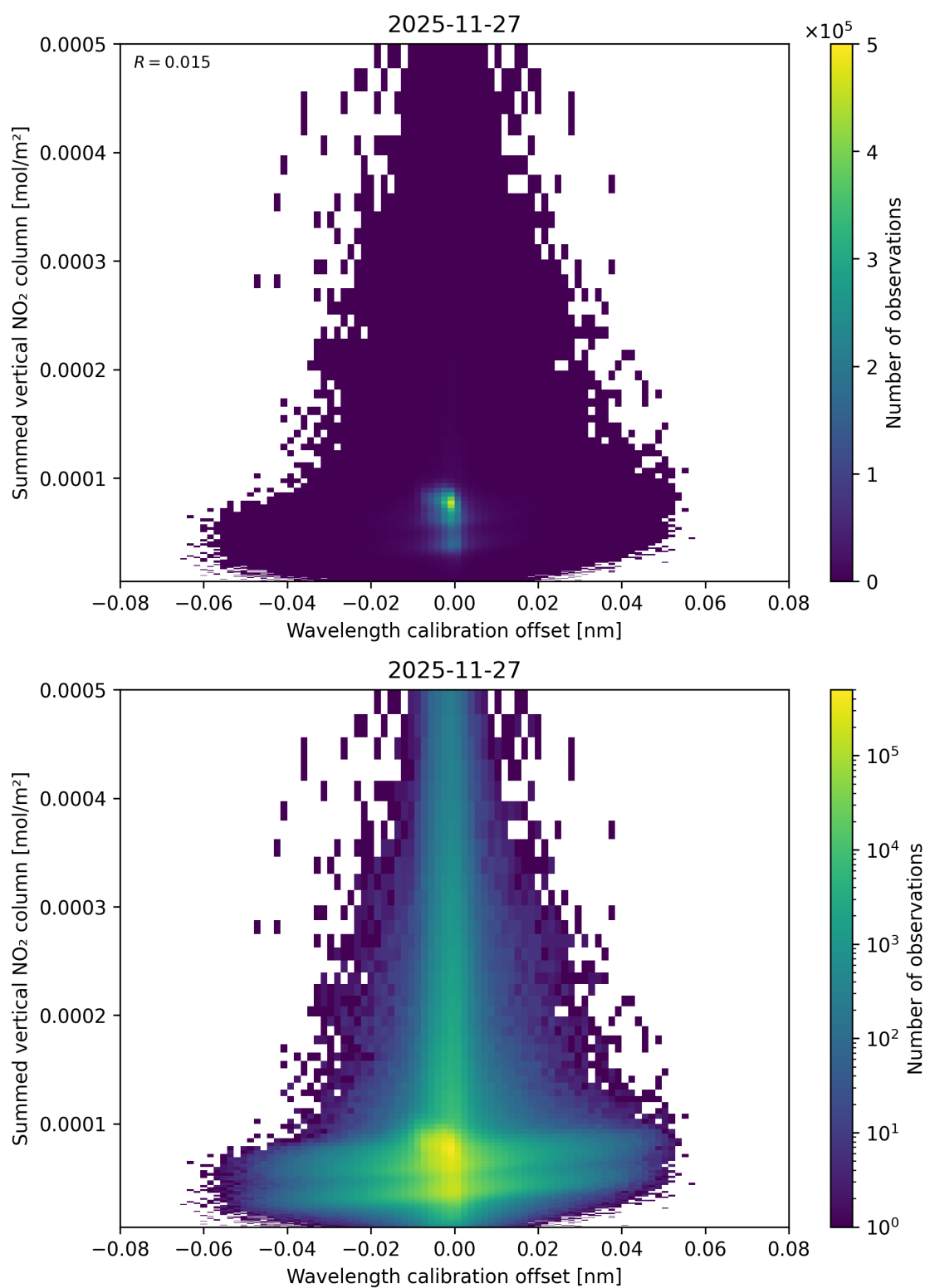
Figure 177: Scatter density plot of “Wavelength calibration offset” against “Summed vertical NO 2 column” for 2025-11-26 to 2025-11-28.
