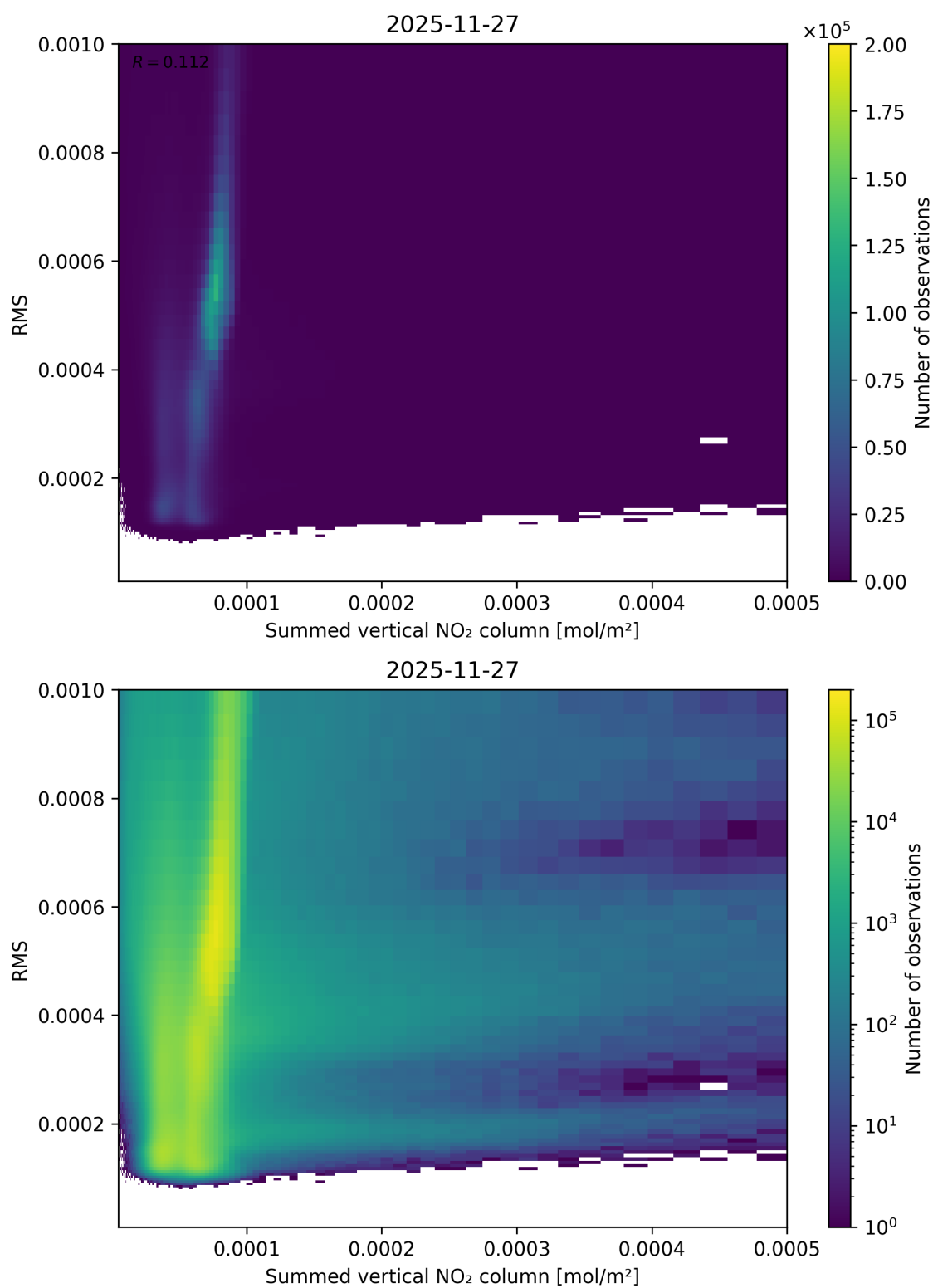
Figure 109: Scatter density plot of “Summed vertical NO 2 column” against “RMS” for 2025-11-26 to 2025-11-28.
