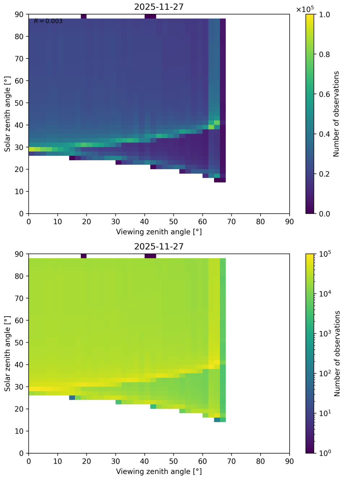
Figure 172: Scatter density plot of “Viewing zenith angle” against “Solar zenith angle” for 2025-11-26 to 2025-11-28.
