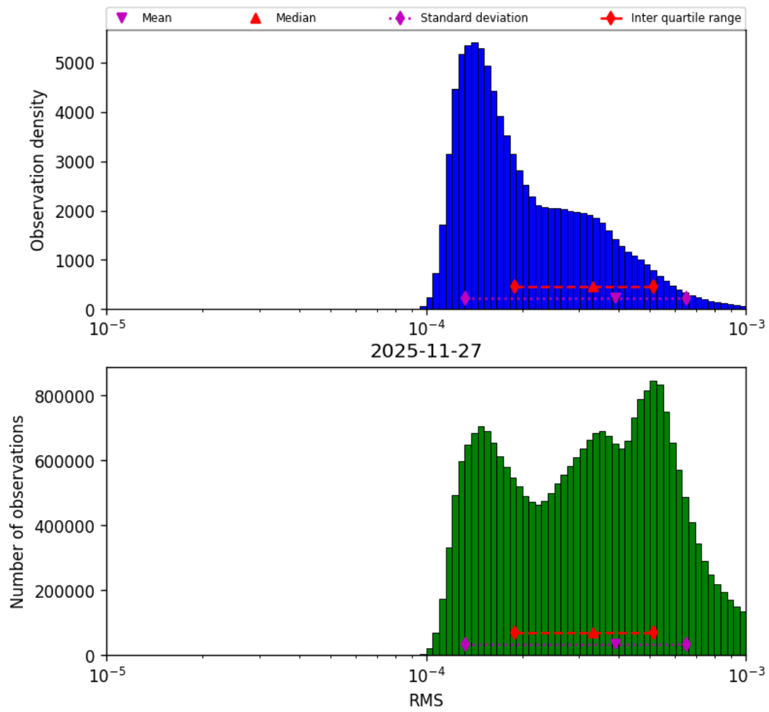
Figure 43: Histogram of “RMS” for 2025-11-26 to 2025-11-28
