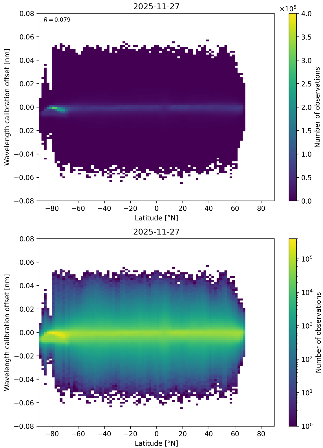
Figure 95: Scatter density plot of “Latitude” against “Wavelength calibration offset” for 2025-11-26 to 2025-11-28.
