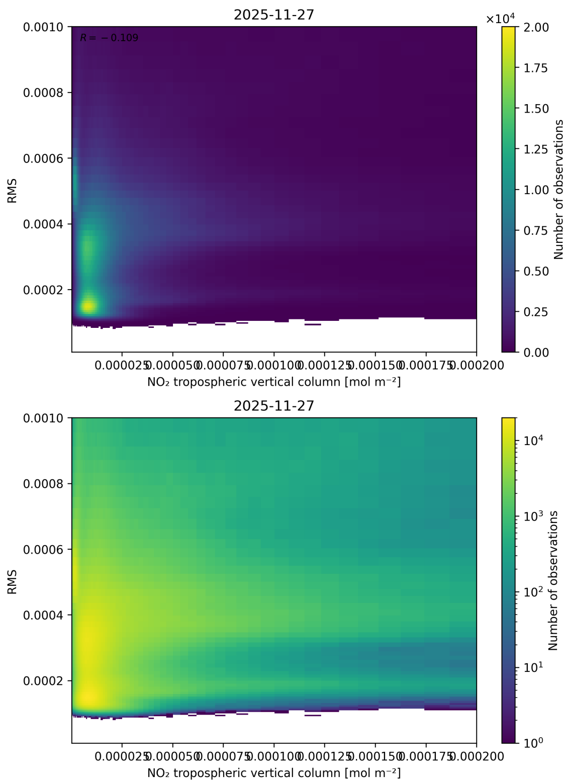
Figure 142: Scatter density plot of “NO 2 tropospheric vertical column” against “RMS” for 2025-11-26 to 2025-11-28.
