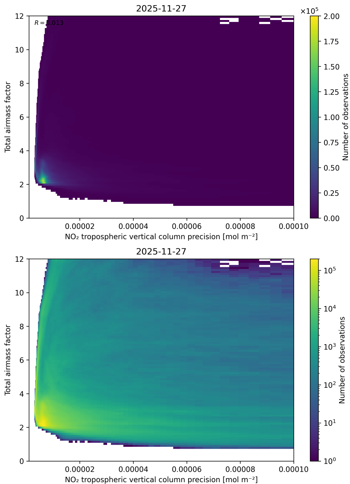
Figure 132: Scatter density plot of “NO 2 tropospheric vertical column precision” against “Total air mass factor” for 2025-11-26 to 2025-11-28.
