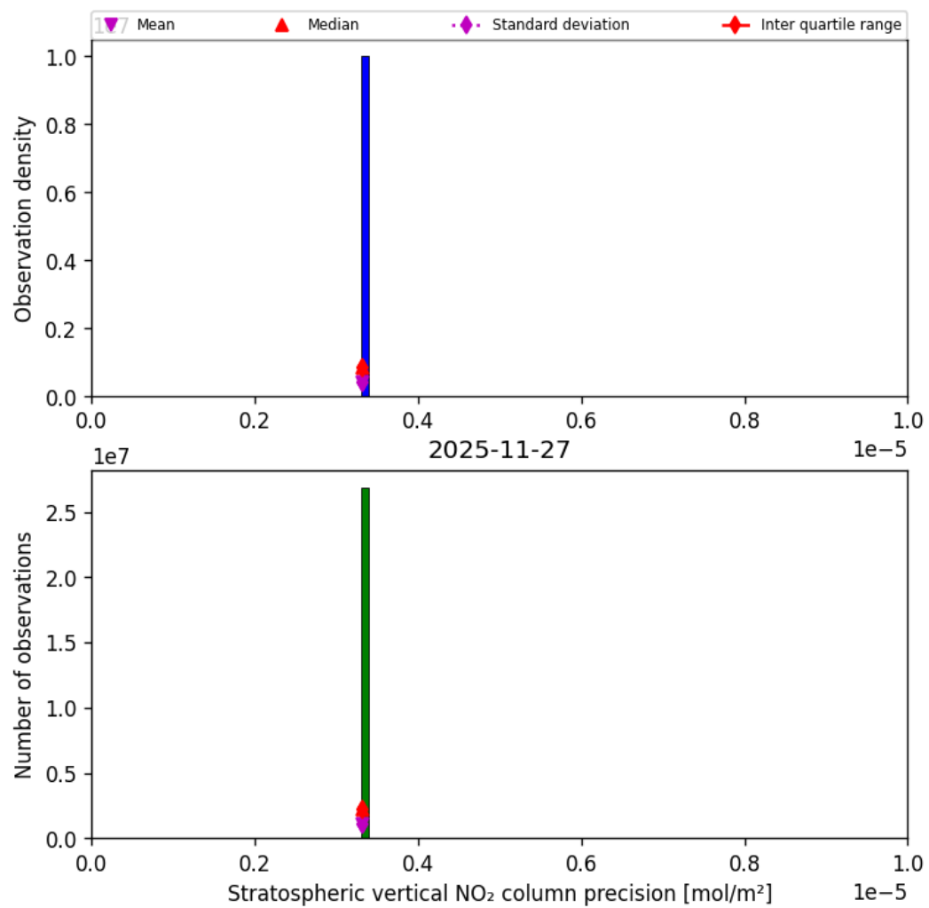
Figure 37: Histogram of “Stratospheric vertical NO 2 column precision” for 2025-11-26 to 2025-11-28
