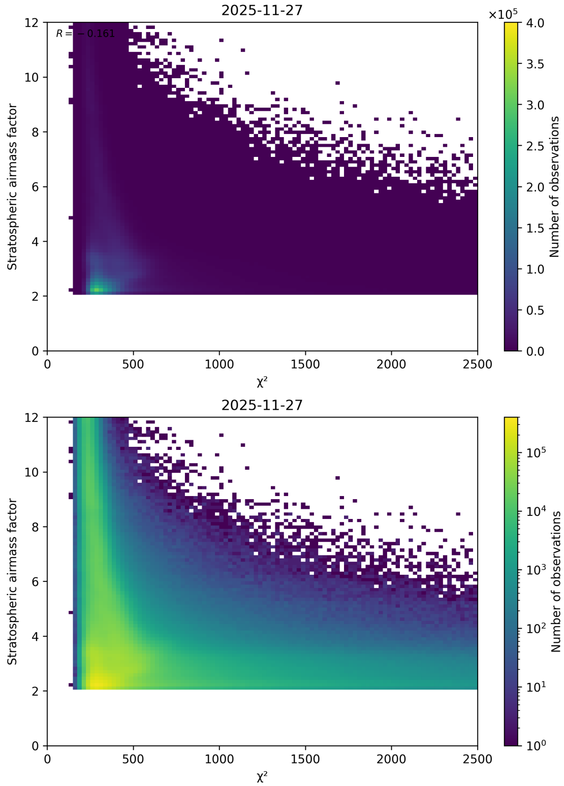
Figure 81: Scatter density plot of “ \chi^2 ” against “Stratospheric airmass factor” for 2025-11-26 to 2025-11-28.
