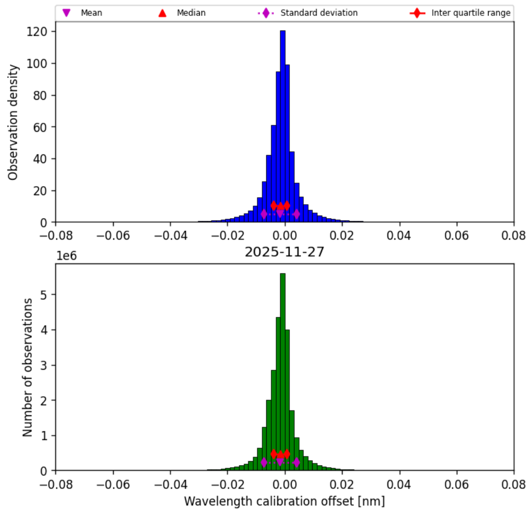
Figure 35: Histogram of “Wavelength calibration offset” for 2025-11-26 to 2025-11-28
