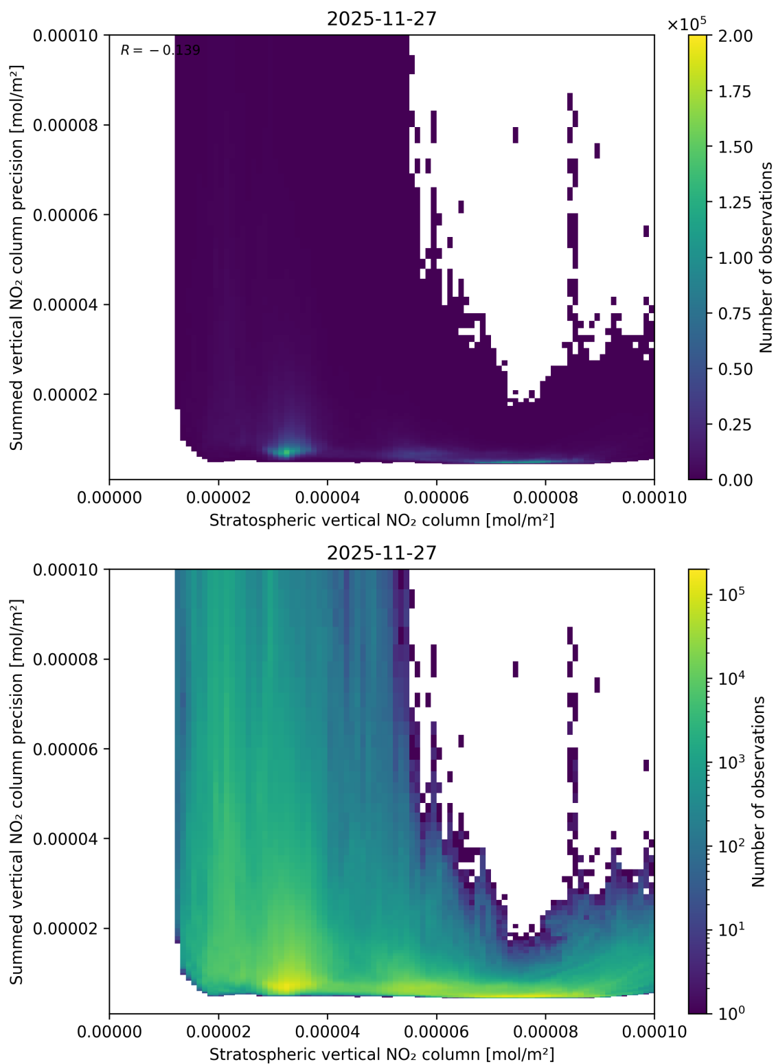
Figure 99: Scatter density plot of “Stratospheric vertical NO 2 column” against “Summed vertical NO 2 column precision” for 2025-11-26 to 2025-11-28.
