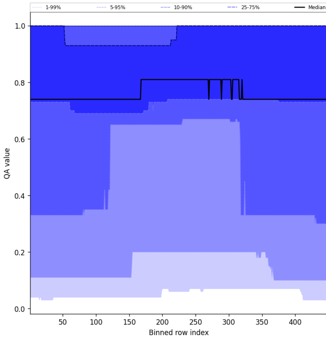
Figure 45: Along track statistics of “QA value” for 2025-11-26 to 2025-11-28
