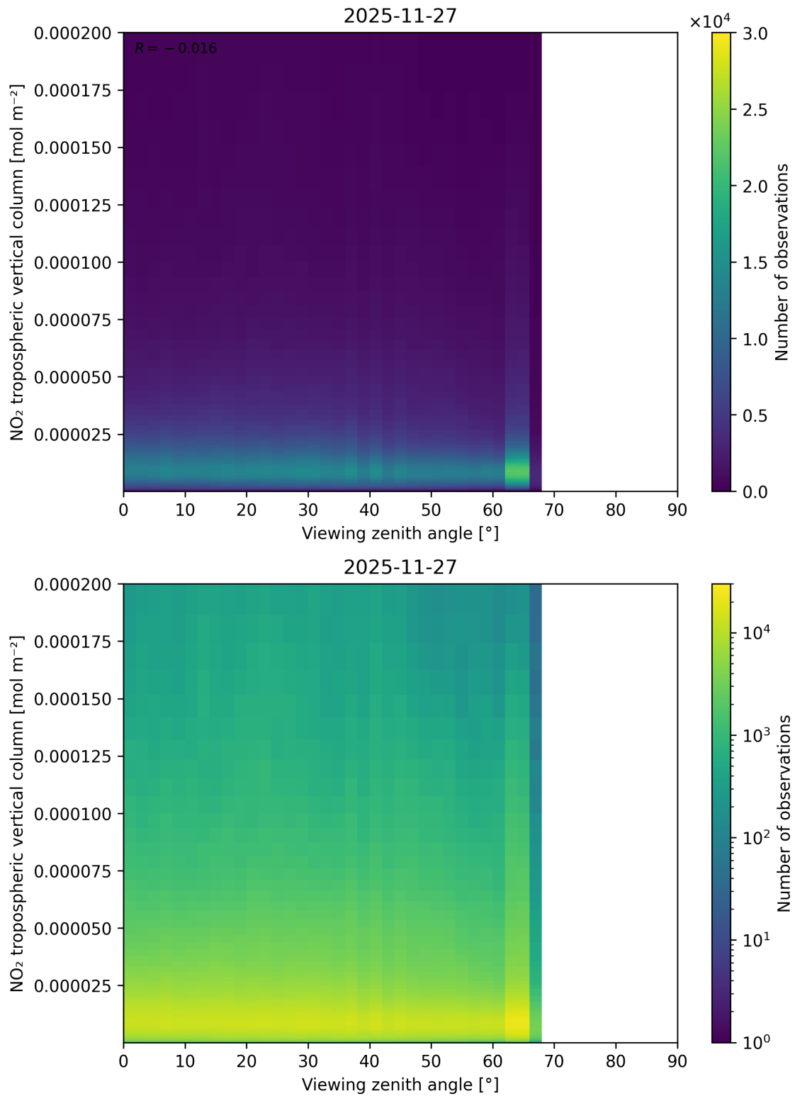
Figure 169: Scatter density plot of “Viewing zenith angle” against “NO 2 tropospheric vertical column” for 2025-11-26 to 2025-11-28.
