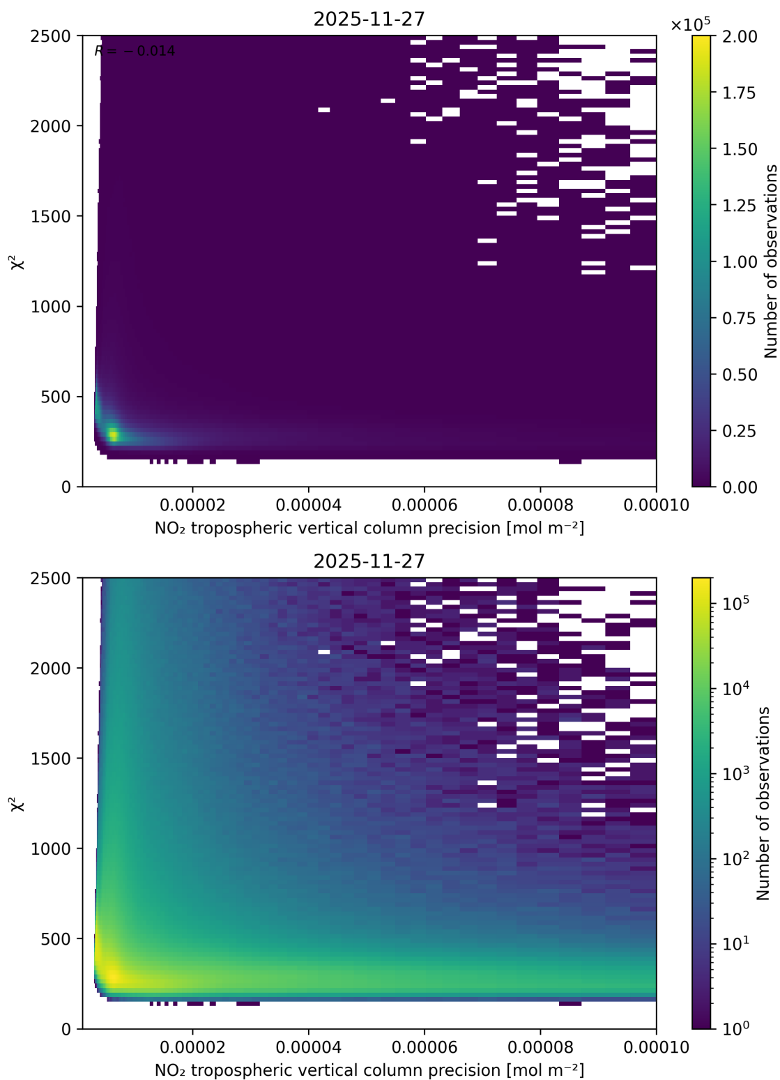
Figure 134: Scatter density plot of “NO 2 tropospheric vertical column precision” against “ \chi^2 ” for 2025-11-26 to 2025-11-28.
