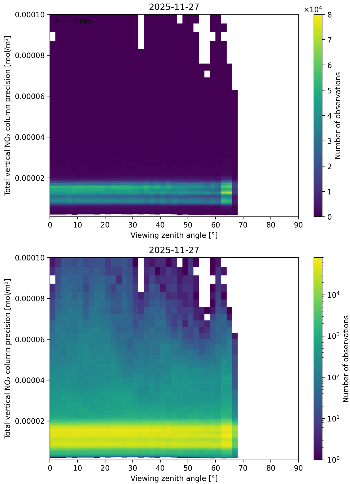
Figure 168: Scatter density plot of “Viewing zenith angle” against “Total vertical NO 2 column precision” for 2025-11-26 to 2025-11-28.
