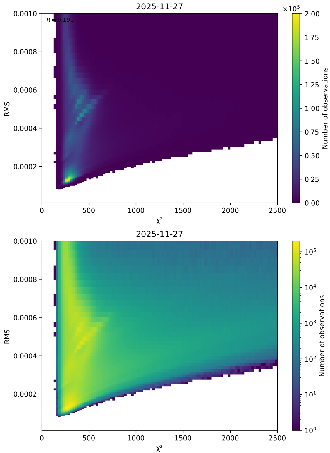
Figure 82: Scatter density plot of “ \chi^2 ” against “RMS” for 2025-11-26 to 2025-11-28.
