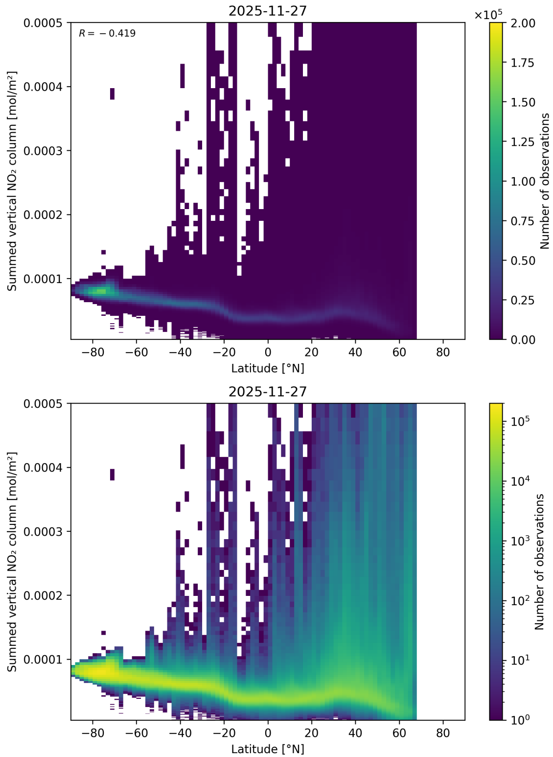
Figure 88: Scatter density plot of “Latitude” against “Summed vertical NO 2 column” for 2025-11-26 to 2025-11-28.
