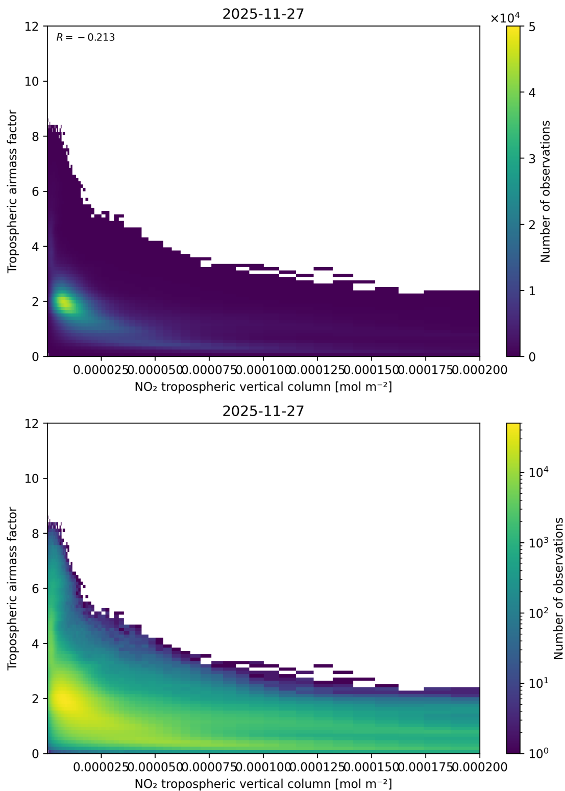
Figure 123: Scatter density plot of “NO 2 tropospheric vertical column” against “Tropospheric air mass factor” for 2025-11-26 to 2025-11-28.
