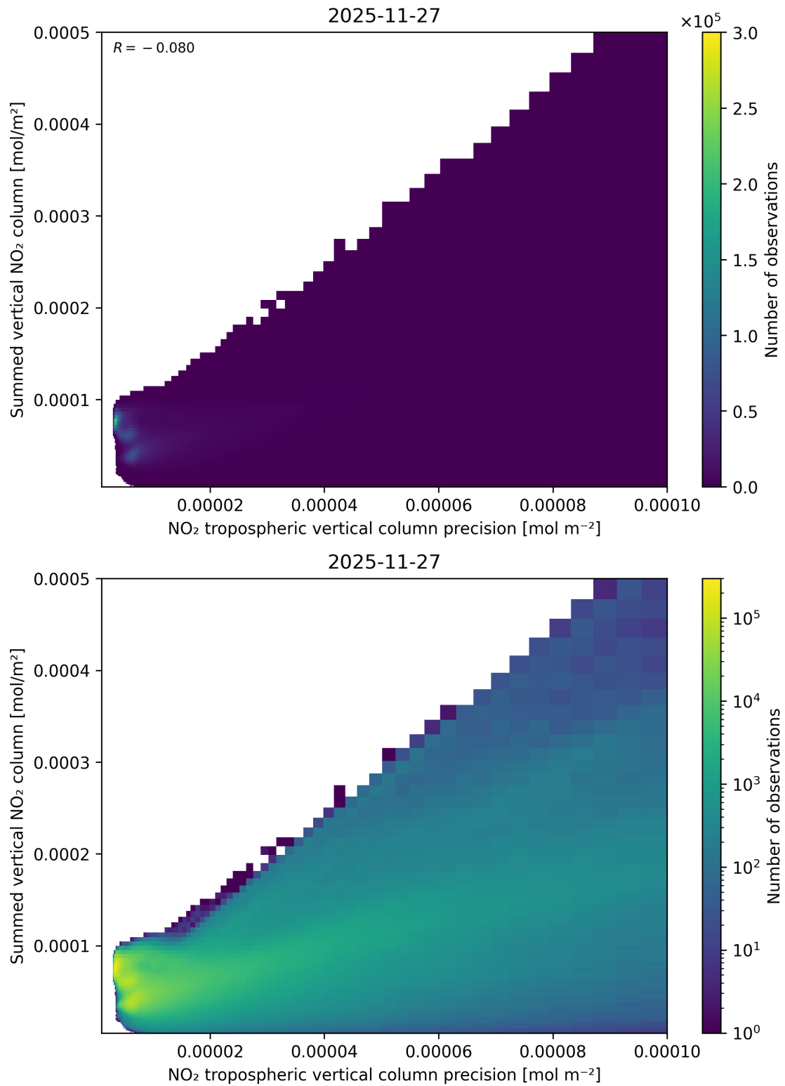
Figure 136: Scatter density plot of “NO 2 tropospheric vertical column precision” against “Summed vertical NO 2 column” for 2025-11-26 to 2025-11-28.
