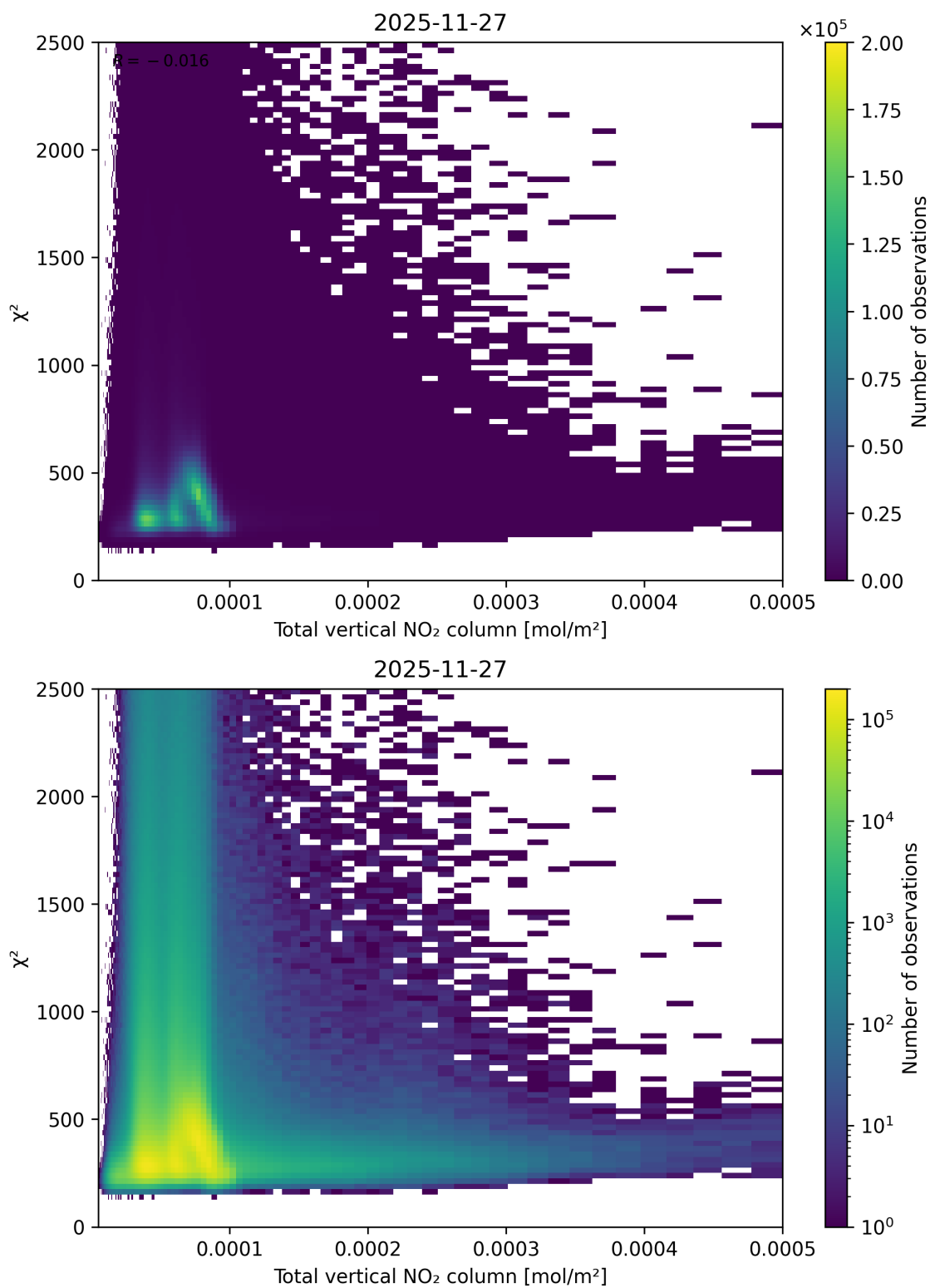
Figure 111: Scatter density plot of “Total vertical NO 2 column” against “ \chi^2 ” for 2025-11-26 to 2025-11-28.
