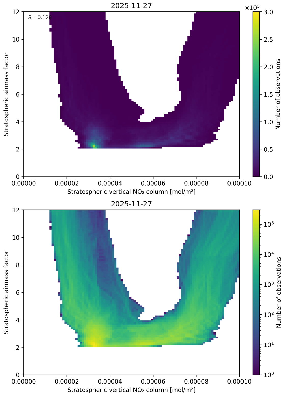
Figure 96: Scatter density plot of “Stratospheric vertical NO 2 column” against “Stratospheric airmass factor” for 2025-11-26 to 2025-11-28.
