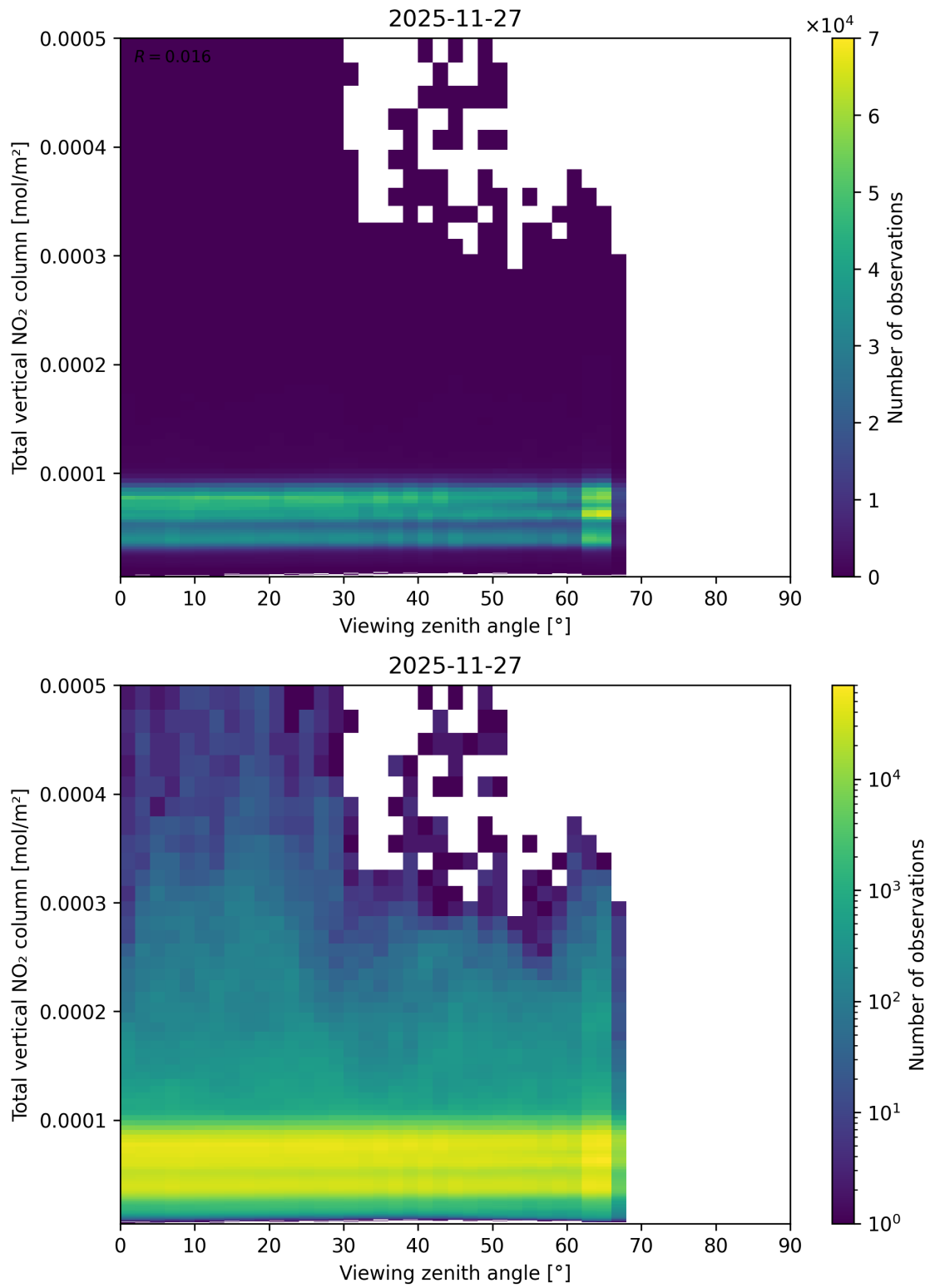
Figure 167: Scatter density plot of “Viewing zenith angle” against “Total vertical NO 2 column” for 2025-11-26 to 2025-11-28.
