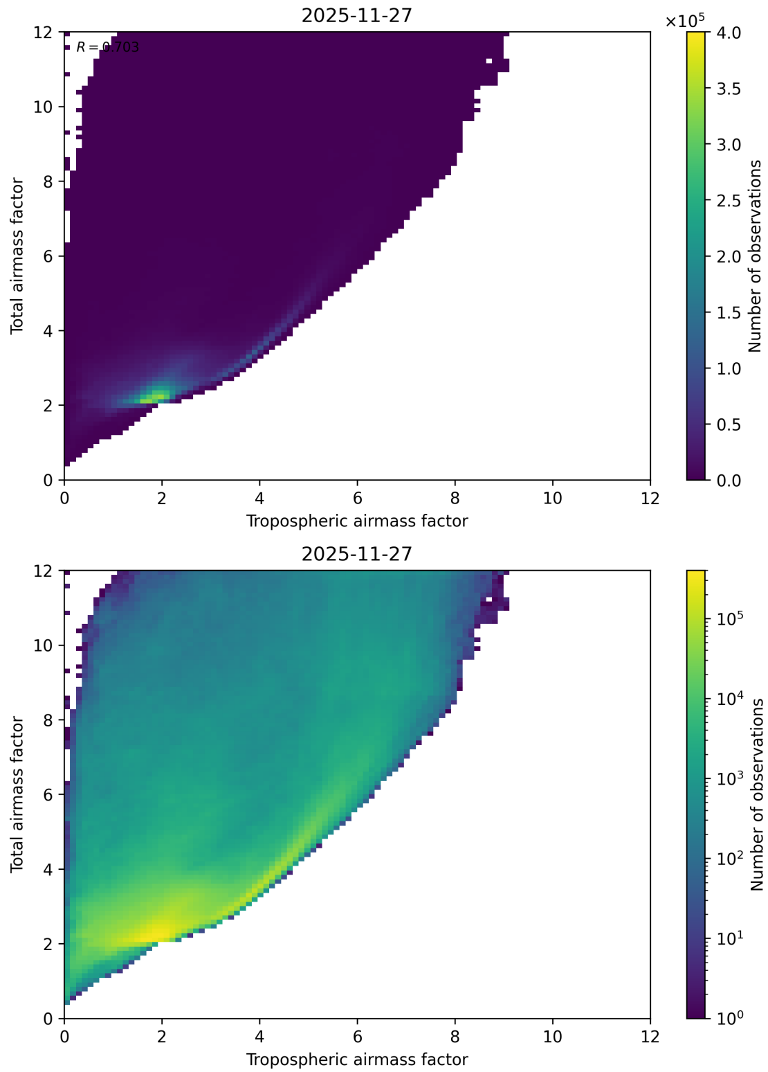
Figure 72: Scatter density plot of “Tropospheric airmass factor” against “Total airmass factor” for 2025-11-26 to 2025-11-28.
