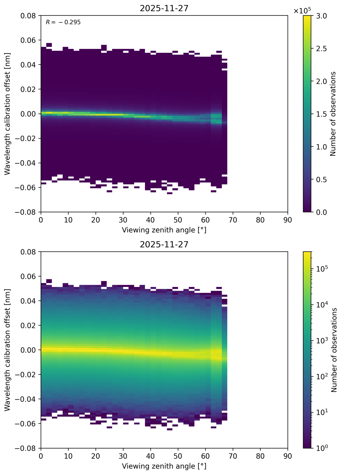
Figure 173: Scatter density plot of “Viewing zenith angle” against “Wavelength calibration offset” for 2025-11-26 to 2025-11-28.
