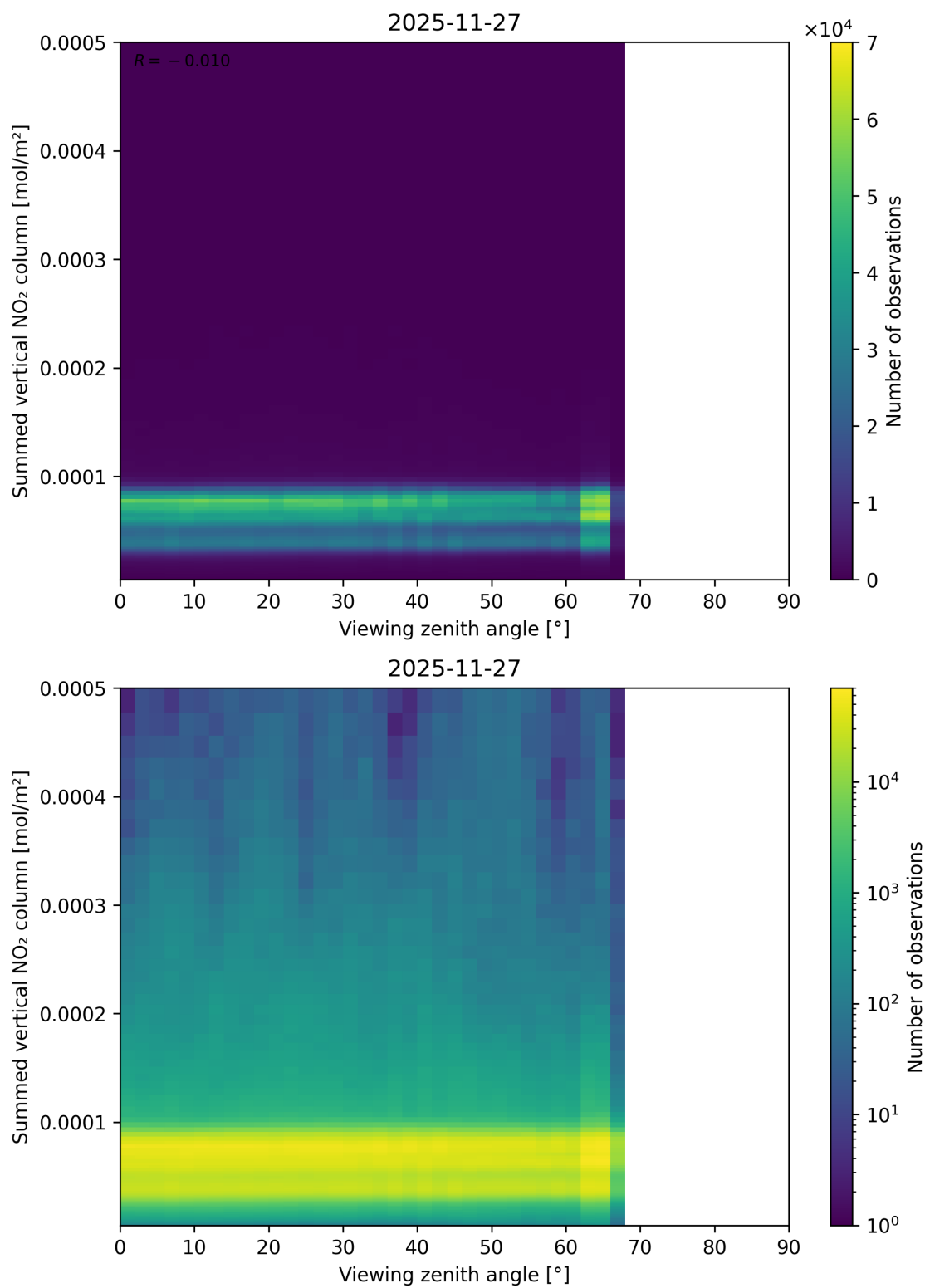
Figure 165: Scatter density plot of “Viewing zenith angle” against “Summed vertical NO 2 column” for 2025-11-26 to 2025-11-28.
