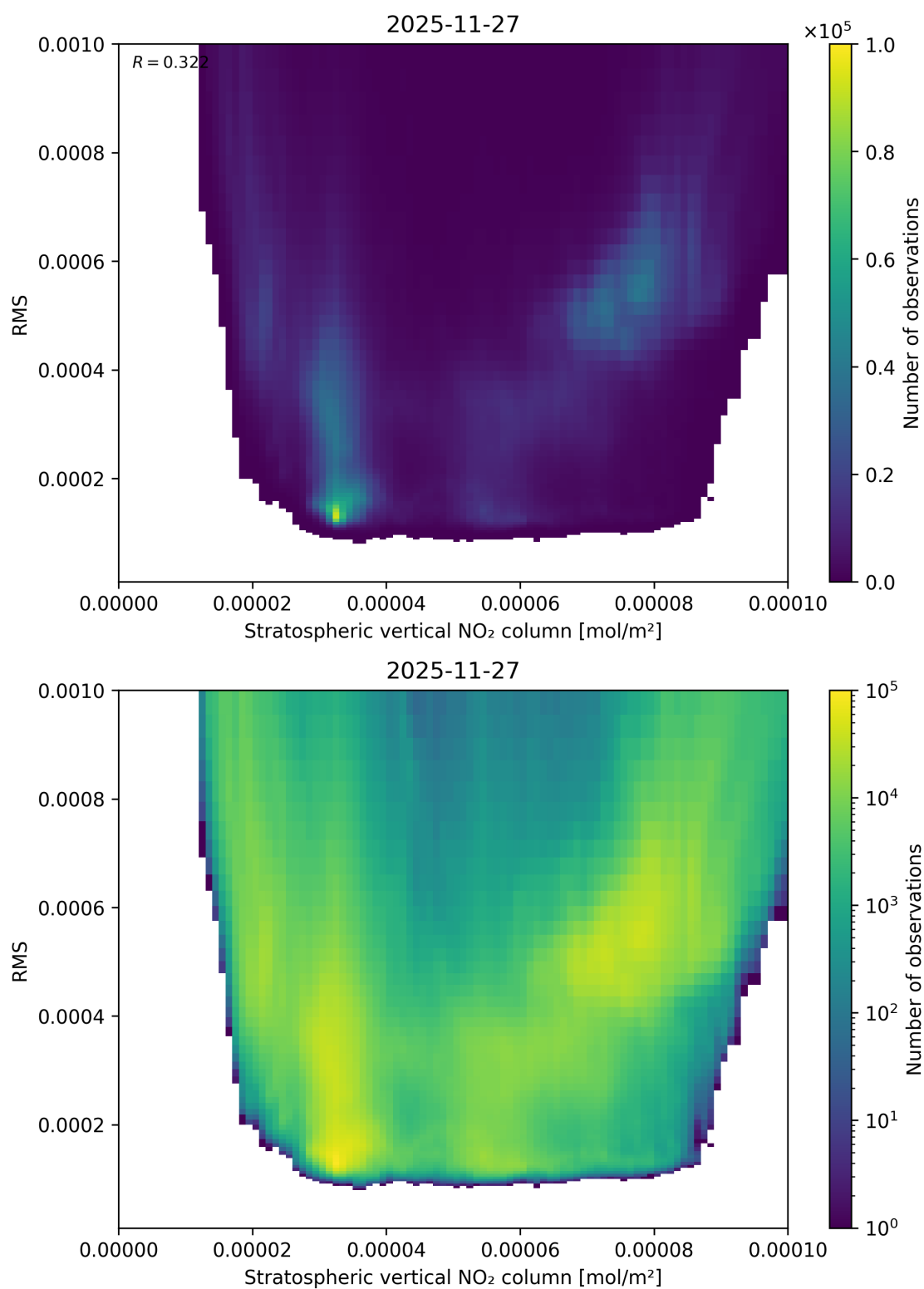
Figure 102: Scatter density plot of “Stratospheric vertical NO 2 column” against “RMS” for 2025-11-26 to 2025-11-28.
