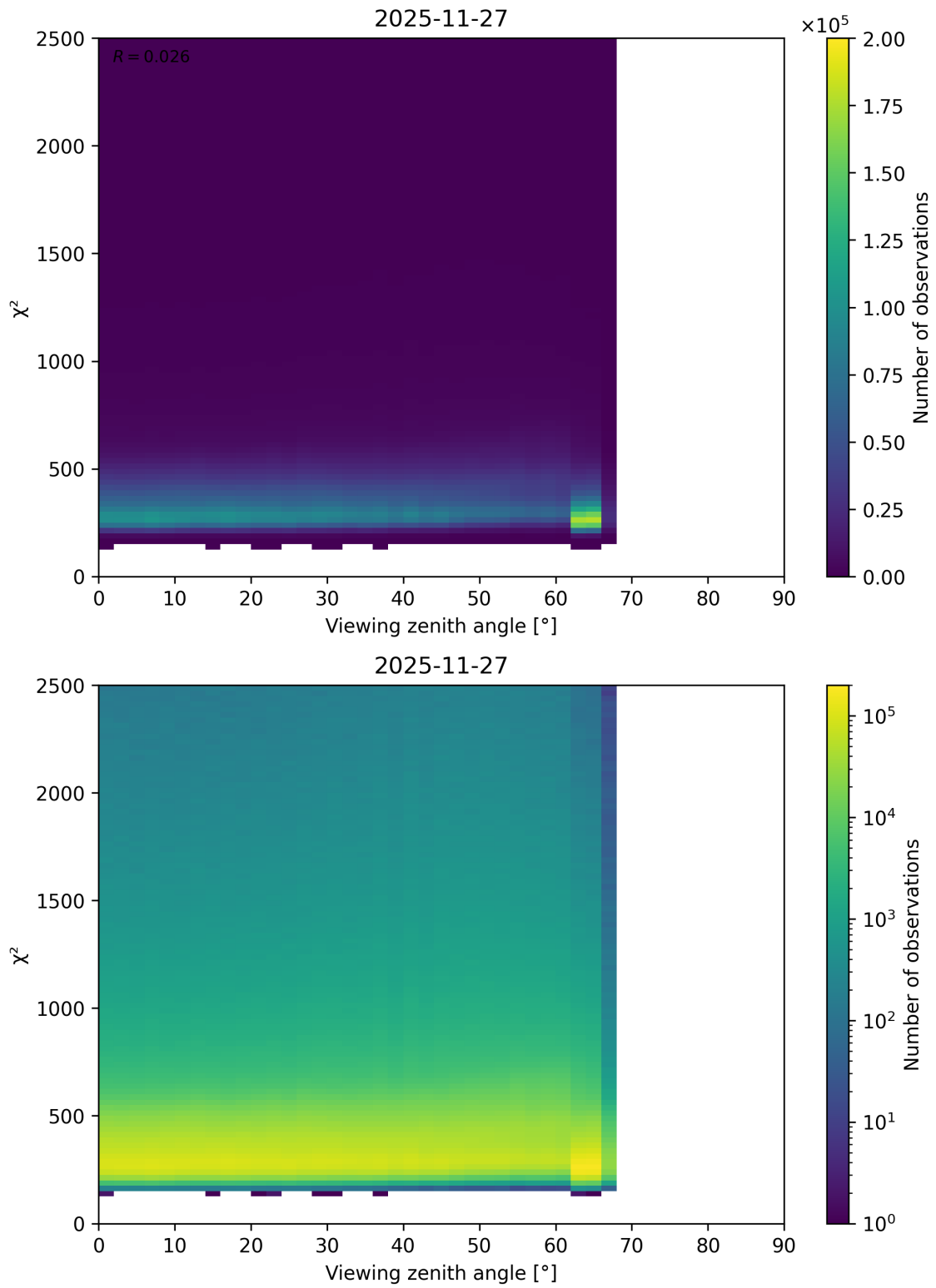
Figure 162: Scatter density plot of “Viewing zenith angle” against “ \chi^2 ” for 2025-11-26 to 2025-11-28.
