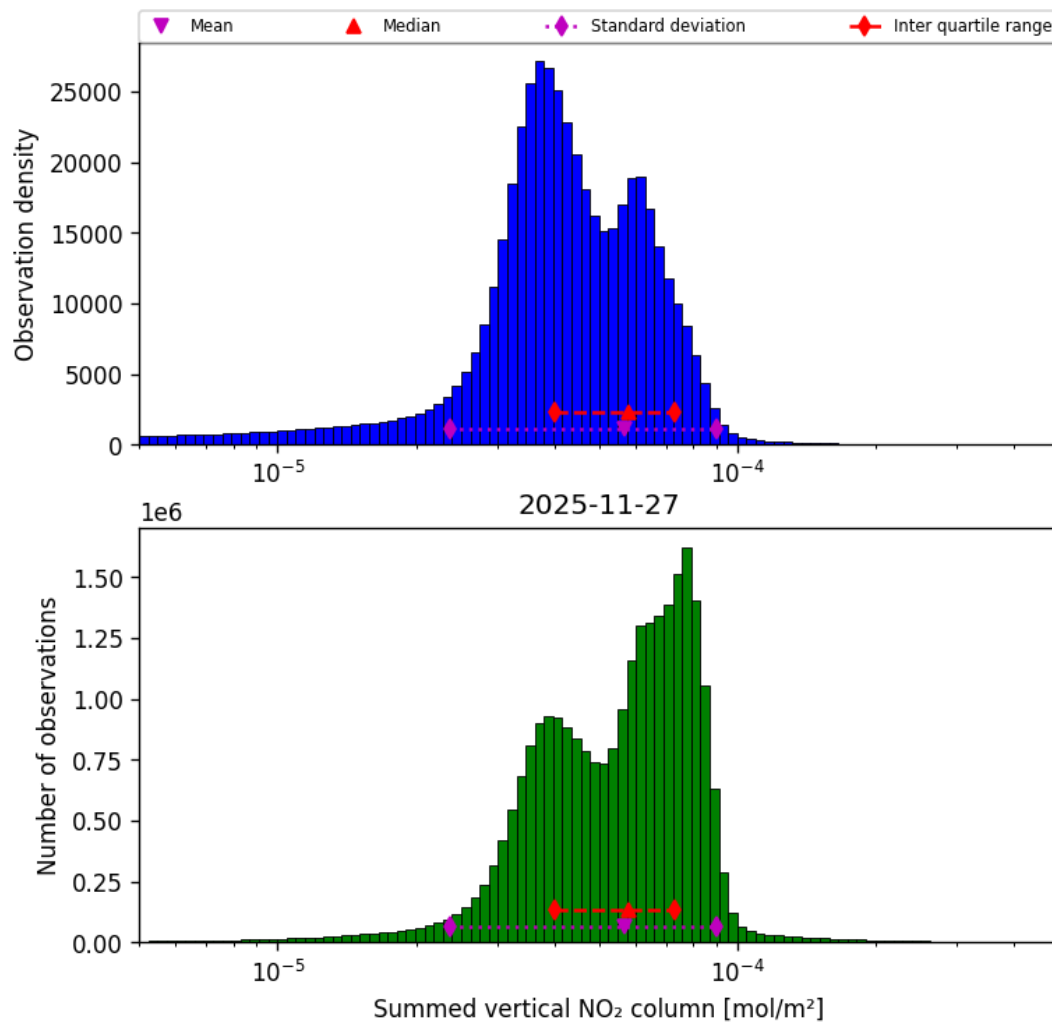
Figure 40: Histogram of “Summed vertical NO 2 column” for 2025-11-26 to 2025-11-28
