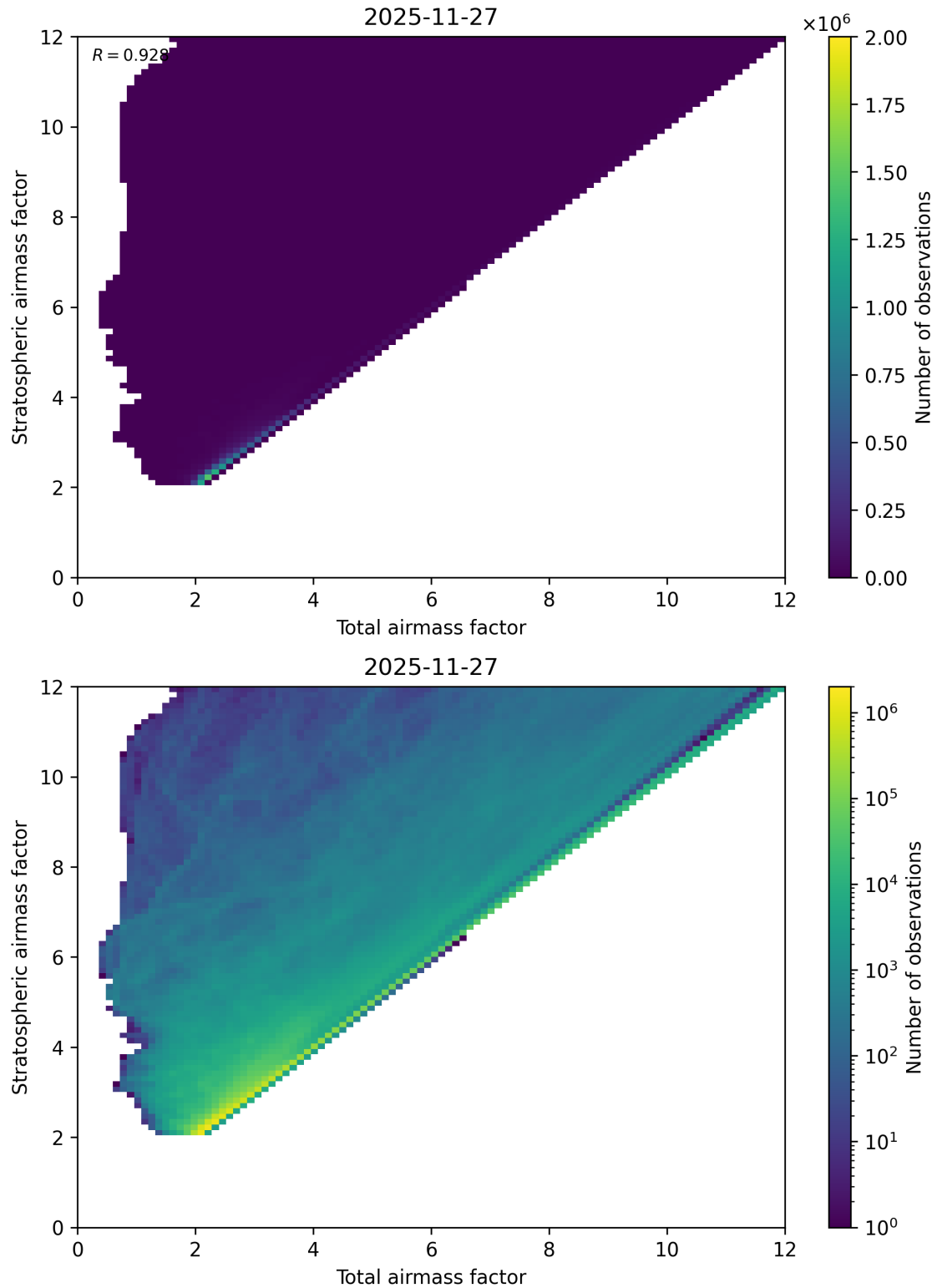
Figure 62: Scatter density plot of “Total airmass factor” against “Stratospheric airmass factor” for 2025-11-26 to 2025-11-28.
