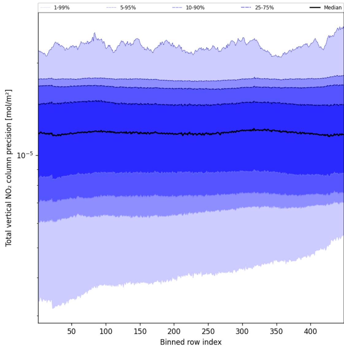
Figure 56: Along track statistics of “Total vertical NO 2 column precision” for 2025-11-26 to 2025-11-28
