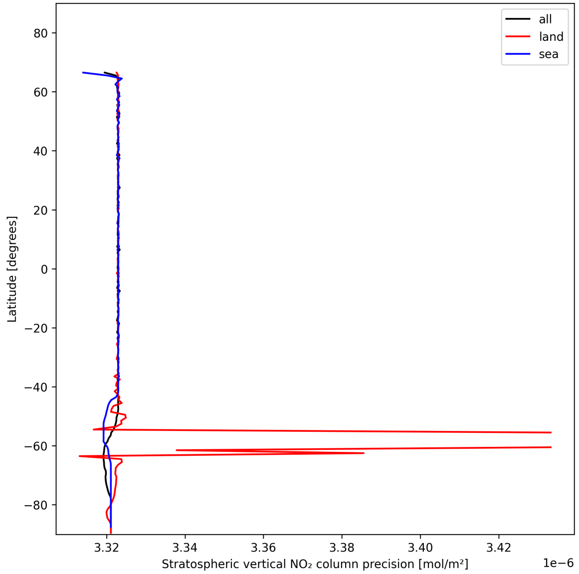
Figure 20: Zonal average of “Stratospheric vertical NO 2 column precision” for 2025-11-26 to 2025-11-28.
