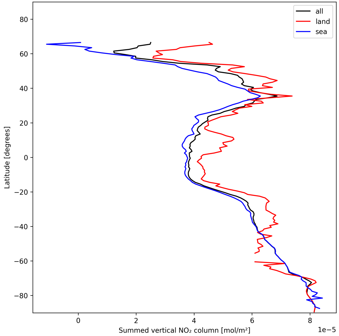
Figure 23: Zonal average of “Summed vertical NO 2 column” for 2025-11-26 to 2025-11-28.
