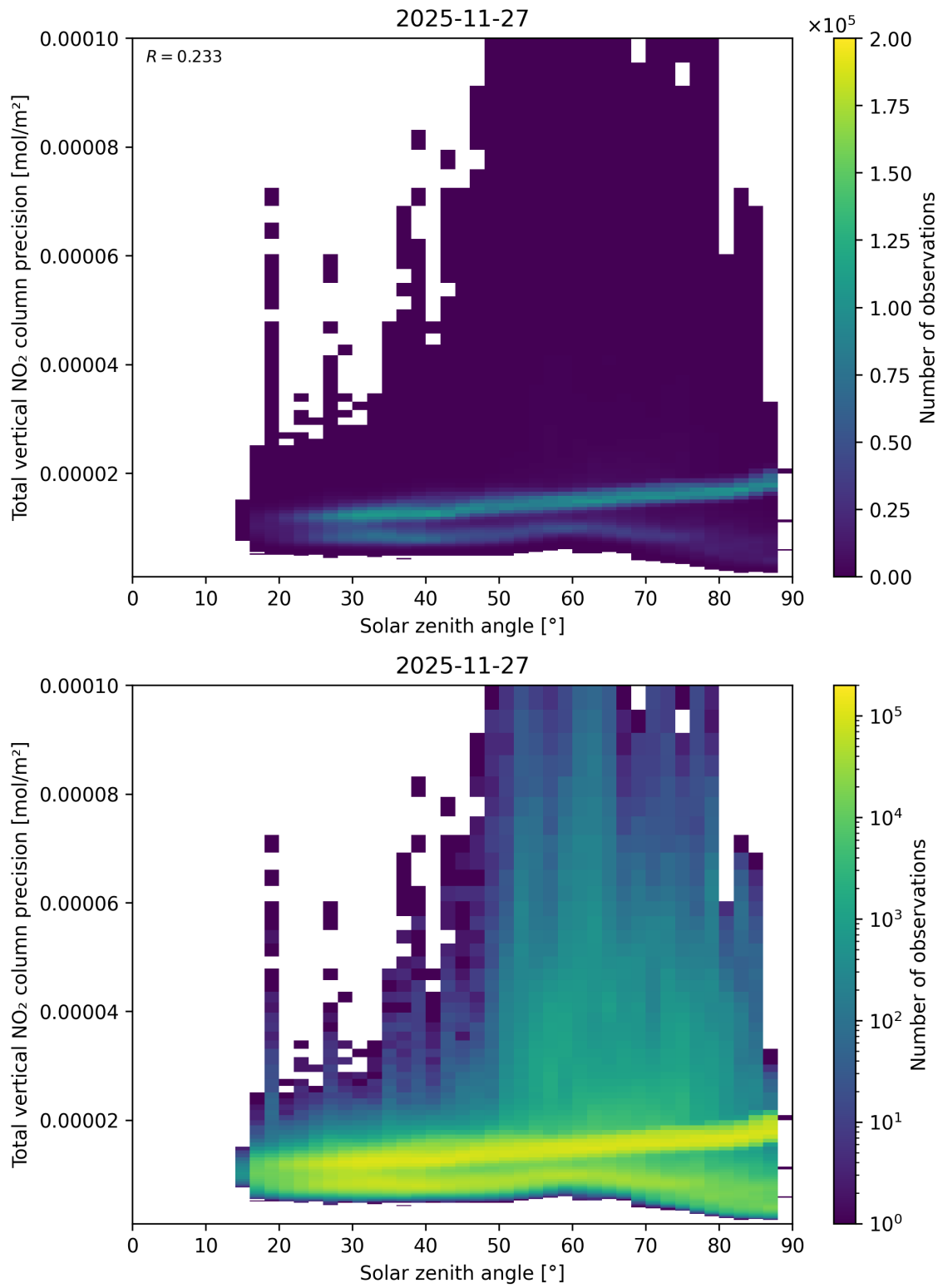
Figure 154: Scatter density plot of “Solar zenith angle” against “Total vertical NO 2 column precision” for 2025-11-26 to 2025-11-28.
