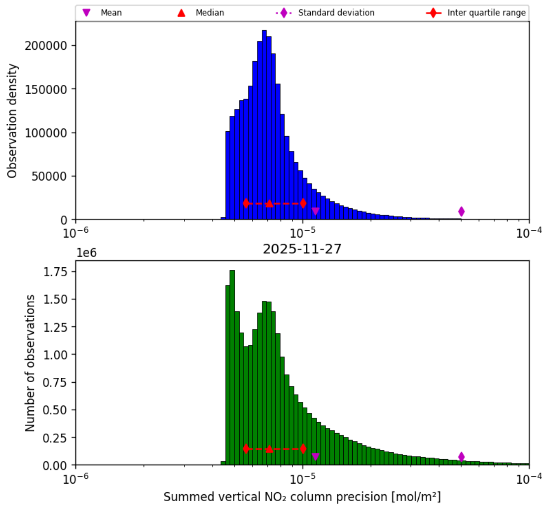
Figure 41: Histogram of "Summed vertical NO 2 column precision" for 2025-11-26 to 2025-11-28
