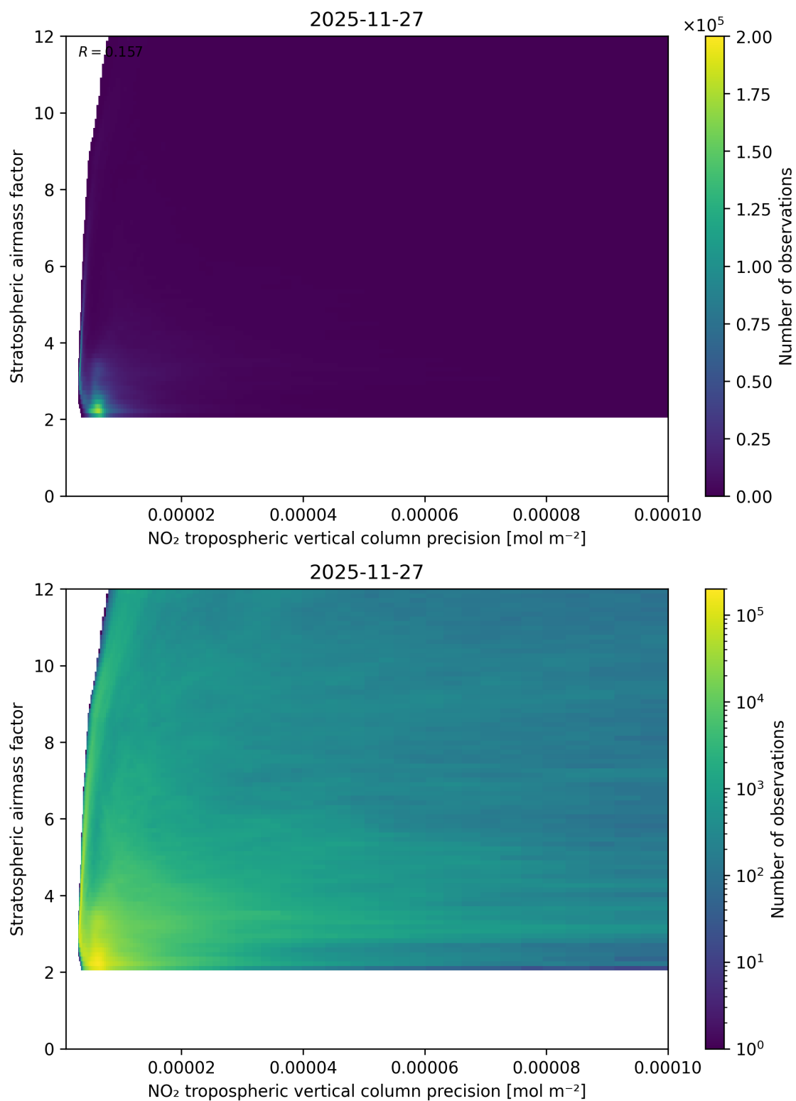
Figure 131: Scatter density plot of “NO 2 tropospheric vertical column precision” against “Stratospheric airmass factor” for 2025-11-26 to 2025-11-28.
