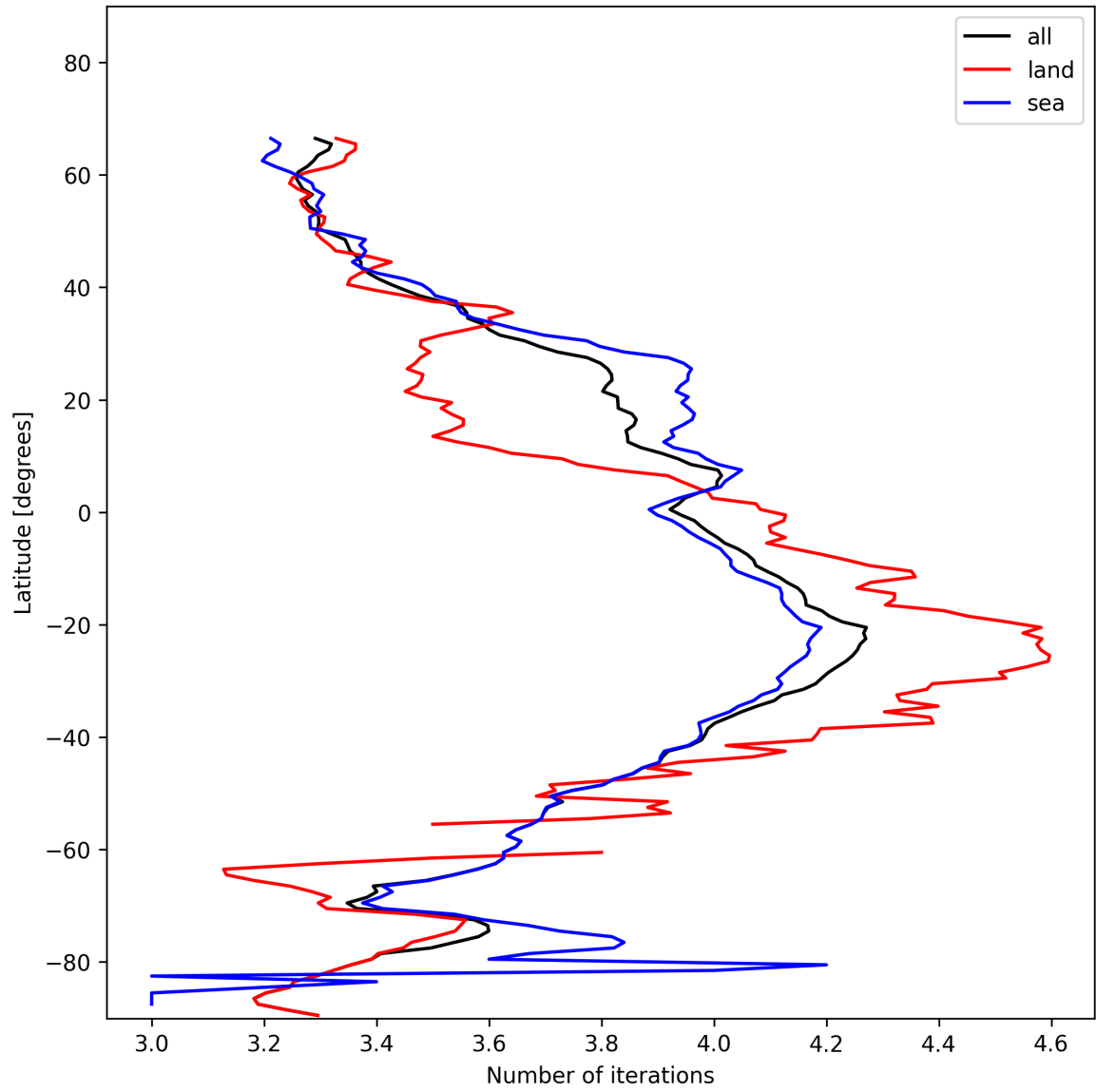
Figure 17: Zonal average of “Number of iterations” for 2025-11-26 to 2025-11-28.
