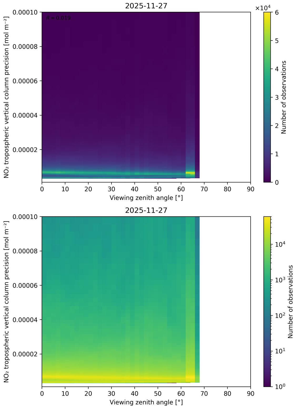
Figure 170: Scatter density plot of “Viewing zenith angle” against “NO 2 tropospheric vertical column precision” for 2025-11-26 to 2025-11-28.
