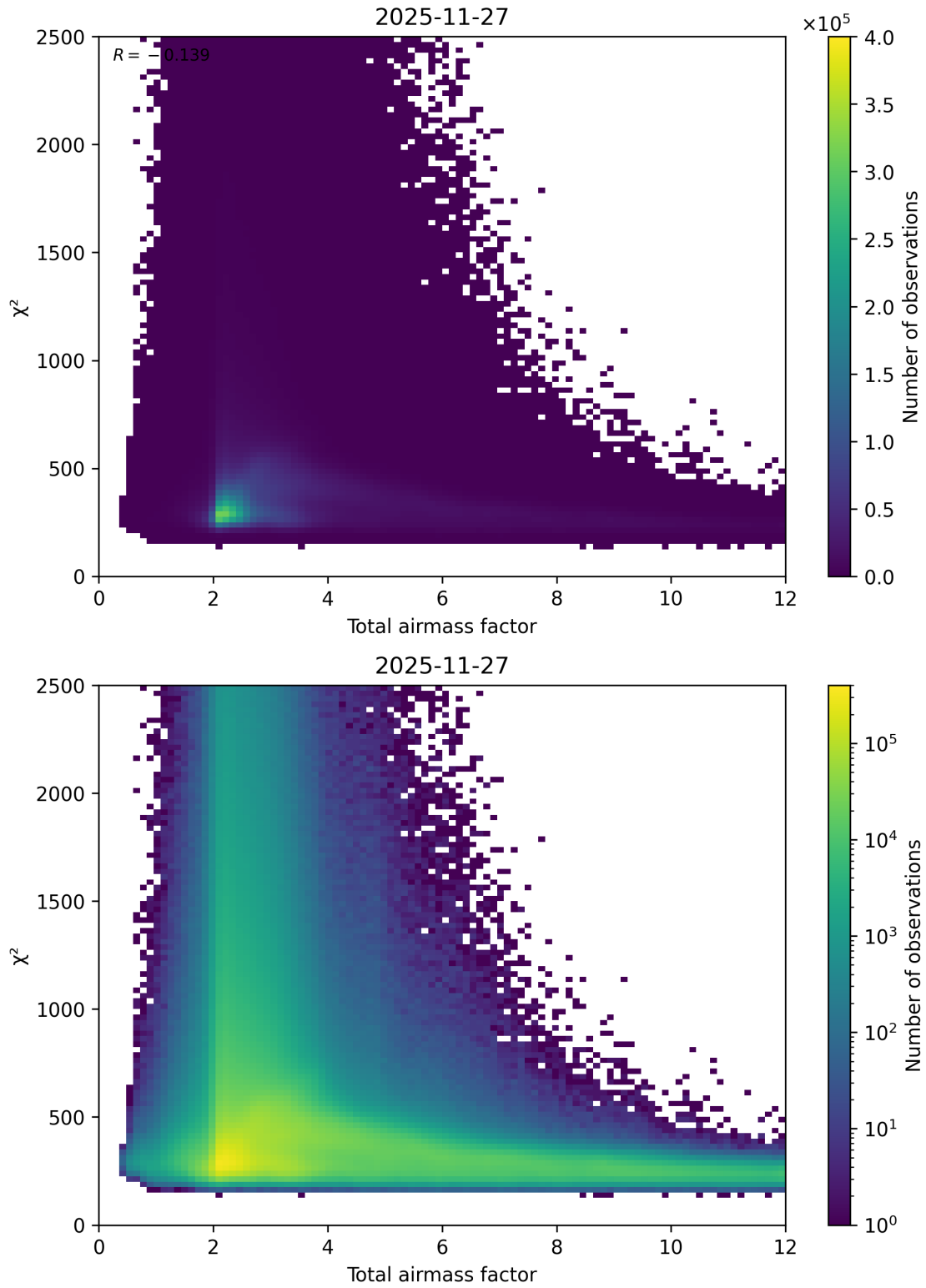
Figure 63: Scatter density plot of “Total airmass factor” against “ \chi^2 ” for 2025-11-26 to 2025-11-28.
