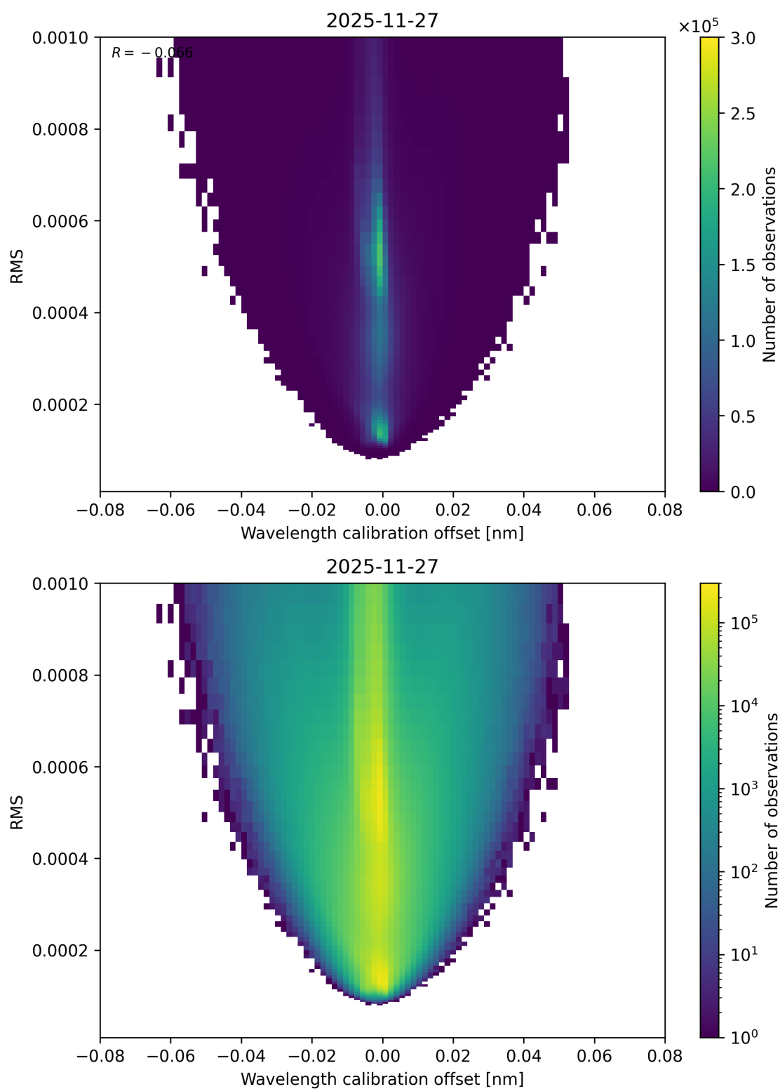
Figure 181: Scatter density plot of “Wavelength calibration offset” against “RMS” for 2025-11-26 to 2025-11-28.
