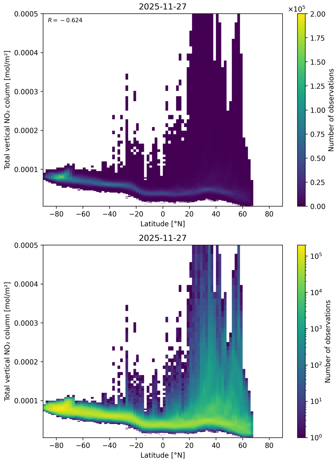
Figure 90: Scatter density plot of “Latitude” against “Total vertical NO 2 column” for 2025-11-26 to 2025-11-28.
