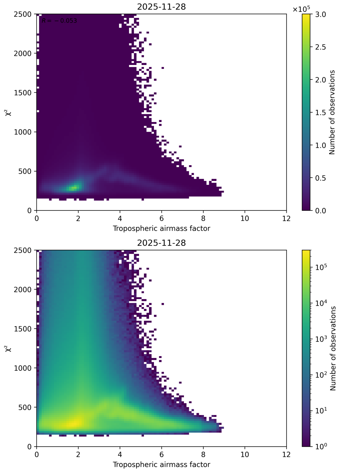
Figure 73: Scatter density plot of “Tropospheric airmass factor” against “ \chi^2 ” for 2025-11-28 to 2025-11-29.
