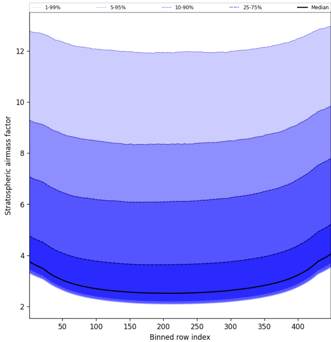
Figure 61: Along track statistics of “Stratospheric air mass factor” for 2025-11-28 to 2025-11-29
