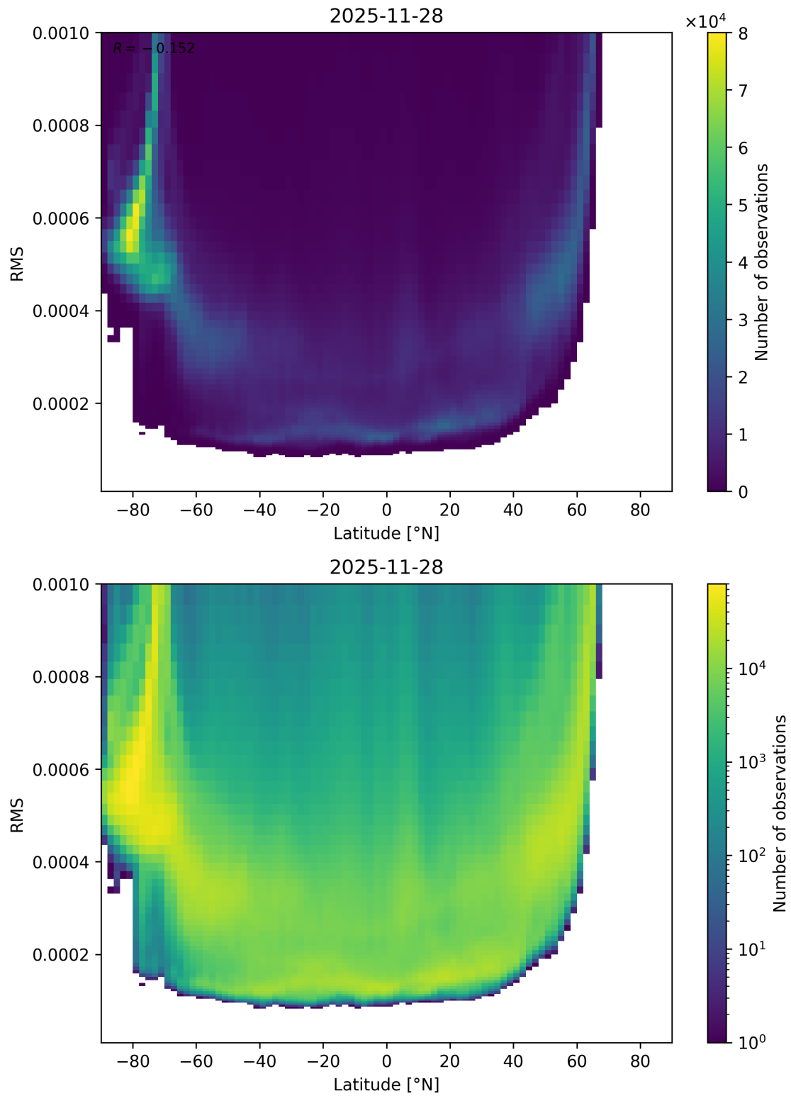
Figure 94: Scatter density plot of “Latitude” against “RMS” for 2025-11-28 to 2025-11-29.
