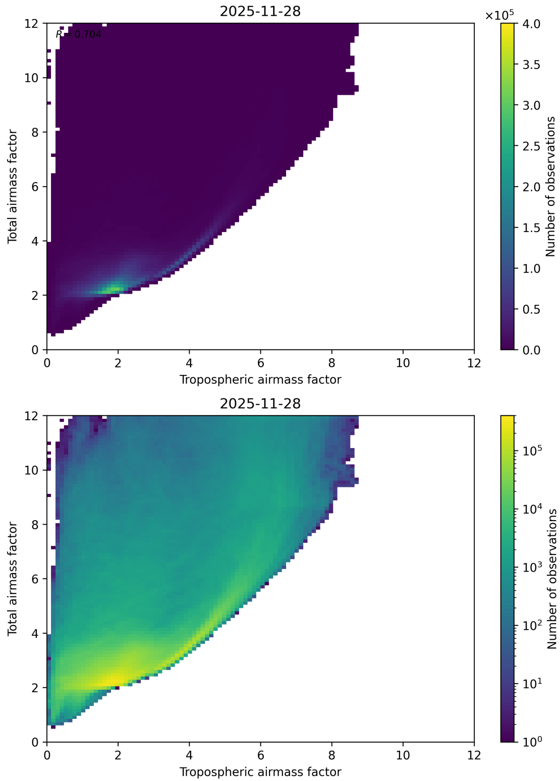
Figure 72: Scatter density plot of “Tropospheric airmass factor” against “Total airmass factor” for 2025-11-28 to 2025-11-29.
