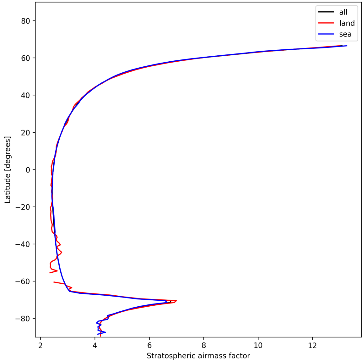
Figure 27: Zonal average of “Stratospheric air mass factor” for 2025-11-28 to 2025-11-29.
