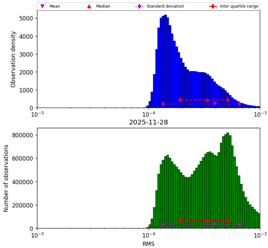
Figure 43: Histogram of “RMS” for 2025-11-28 to 2025-11-29
