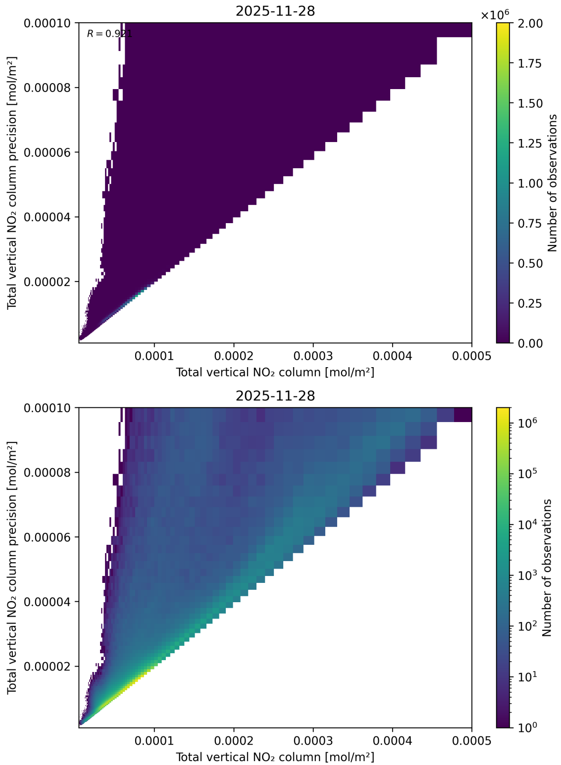
Figure 114: Scatter density plot of “Total vertical NO 2 column” against “Total vertical NO 2 column precision” for 2025-11-28 to 2025-11-29.
