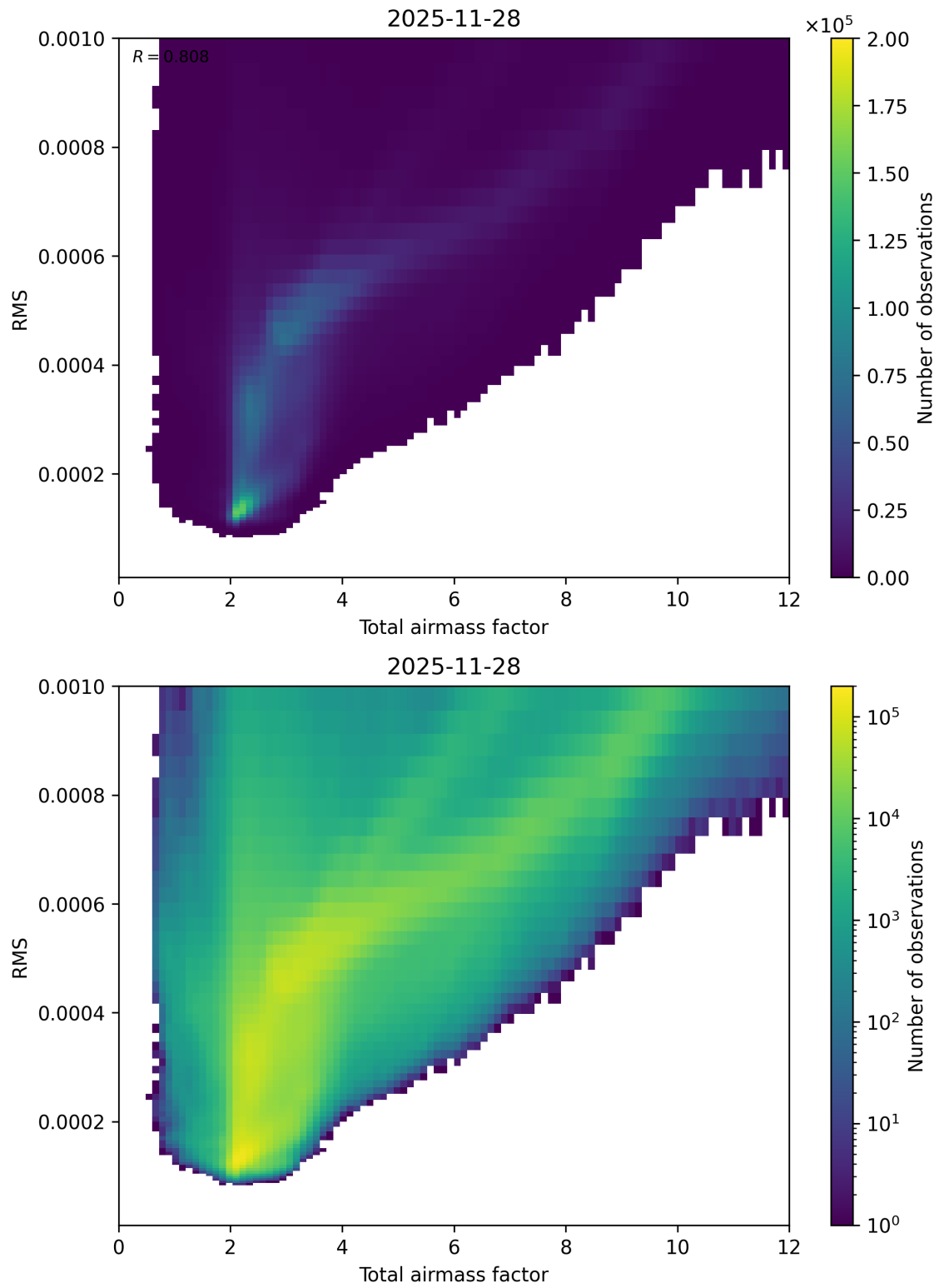
Figure 69: Scatter density plot of “Total airmass factor” against “RMS” for 2025-11-28 to 2025-11-29.
