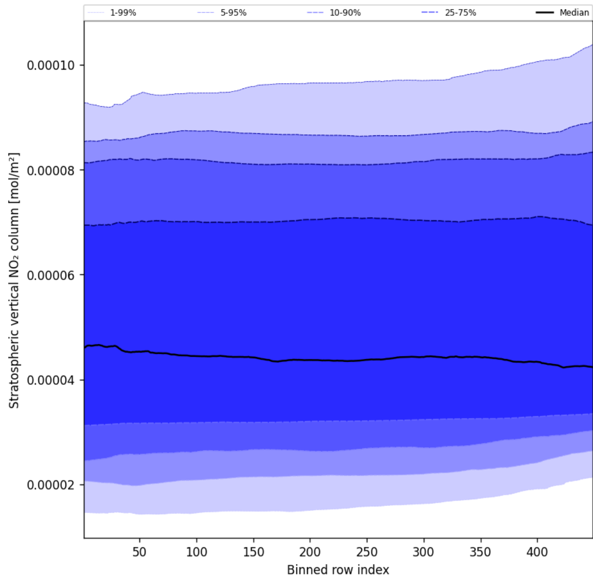
Figure 53: Along track statistics of “Stratospheric vertical NO 2 column” for 2025-11-28 to 2025-11-29
