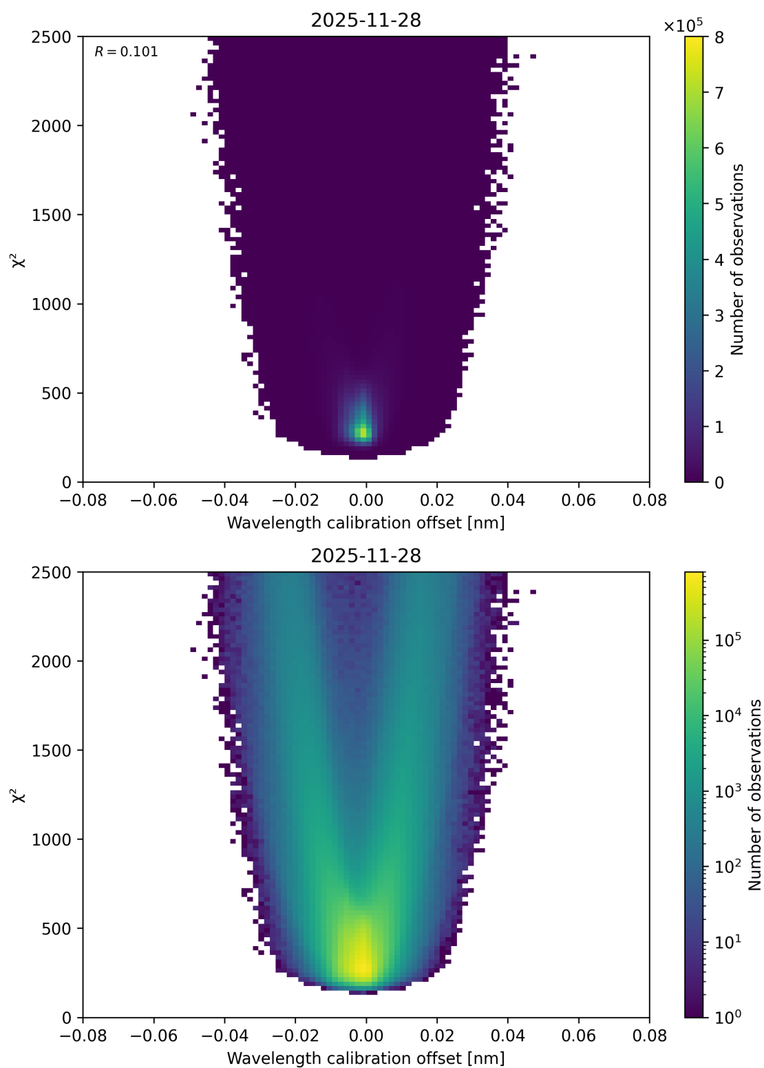
Figure 175: Scatter density plot of “Wavelength calibration offset” against “ \chi^2 ” for 2025-11-28 to 2025-11-29.
