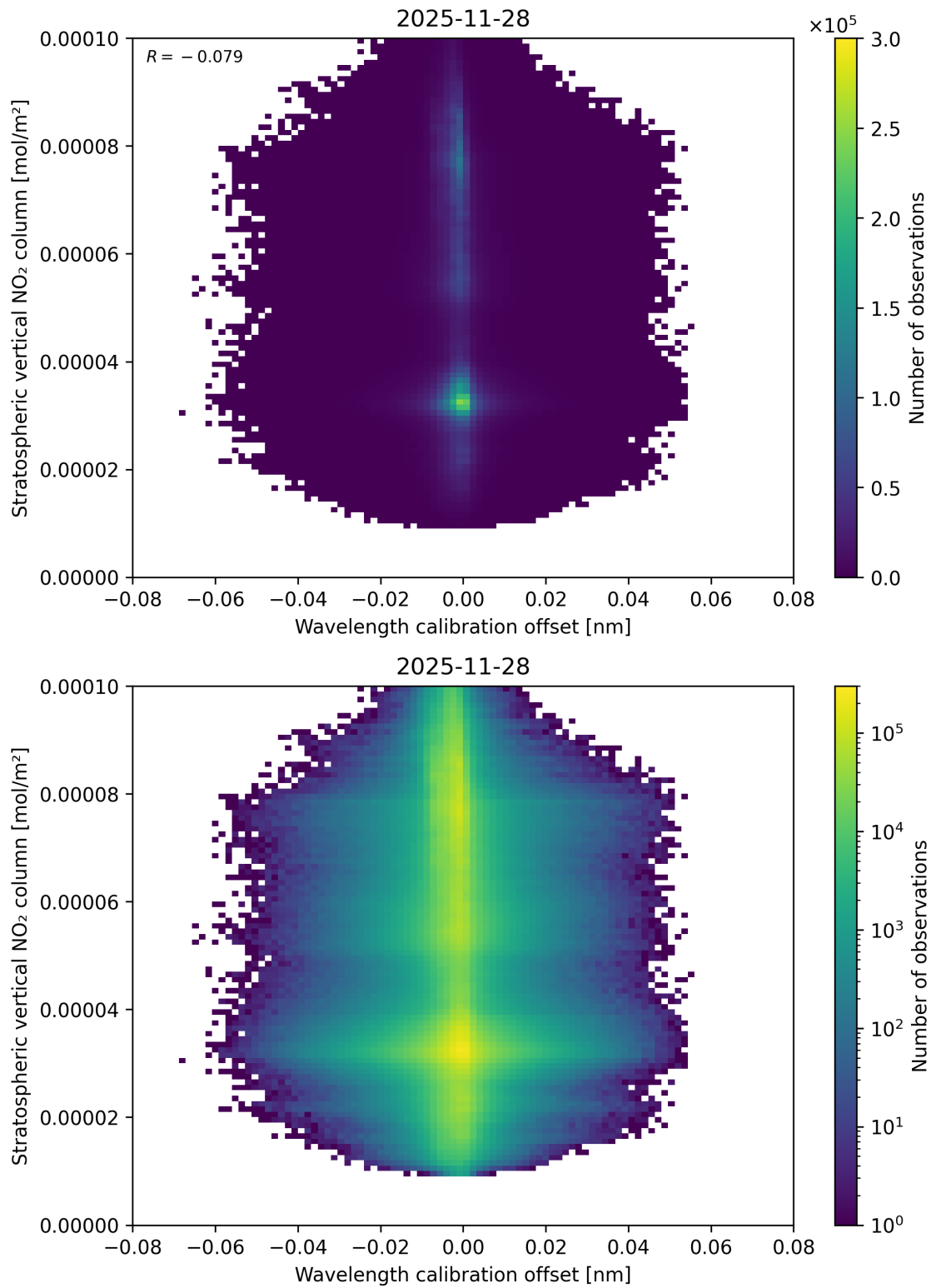
Figure 176: Scatter density plot of “Wavelength calibration offset” against “Stratospheric vertical NO 2 column” for 2025-11-28 to 2025-11-29.
