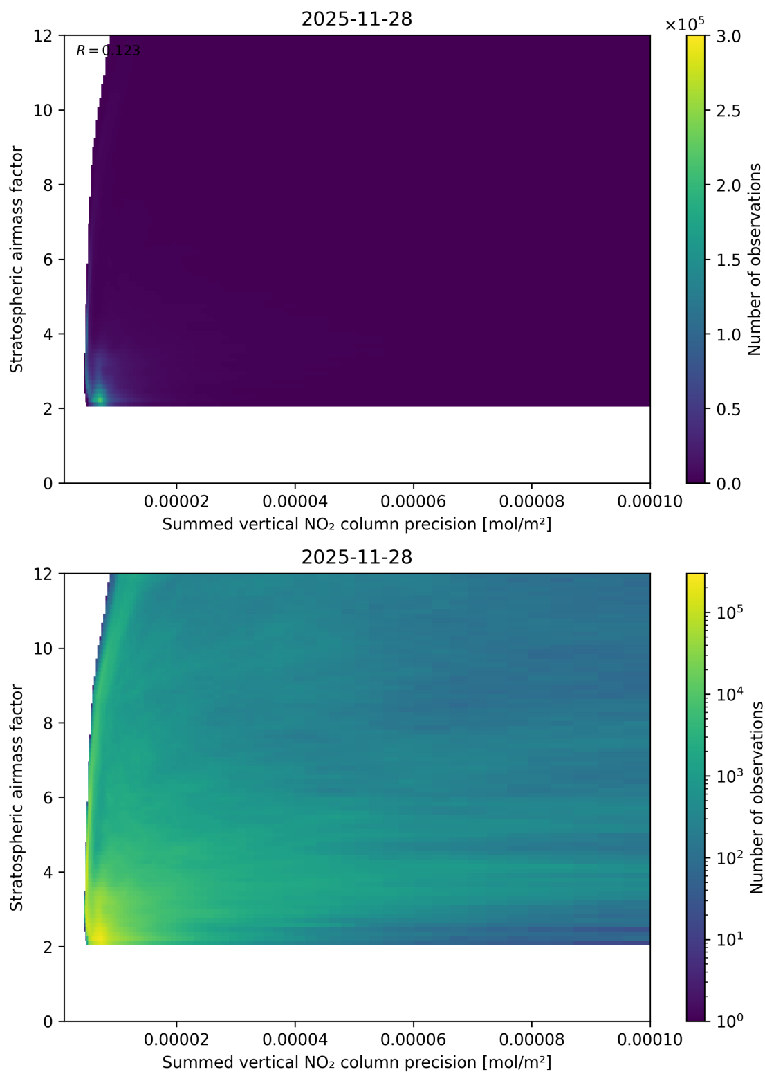
Figure 106: Scatter density plot of “Summed vertical NO 2 column precision” against “Stratospheric airmass factor” for 2025-11-28 to 2025-11-29.
