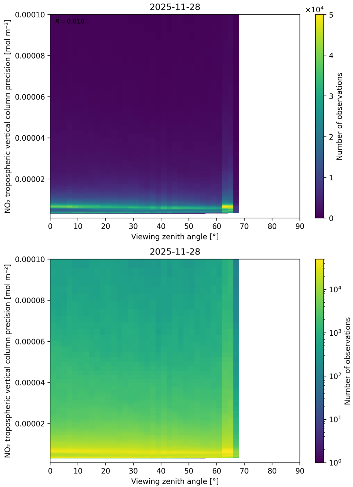
Figure 170: Scatter density plot of “Viewing zenith angle” against “NO 2 tropospheric vertical column precision” for 2025-11-28 to 2025-11-29.
