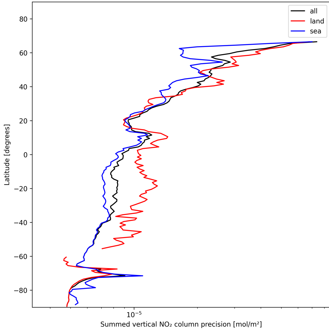
Figure 24: Zonal average of “Summed vertical NO 2 column precision” for 2025-11-28 to 2025-11-29.
