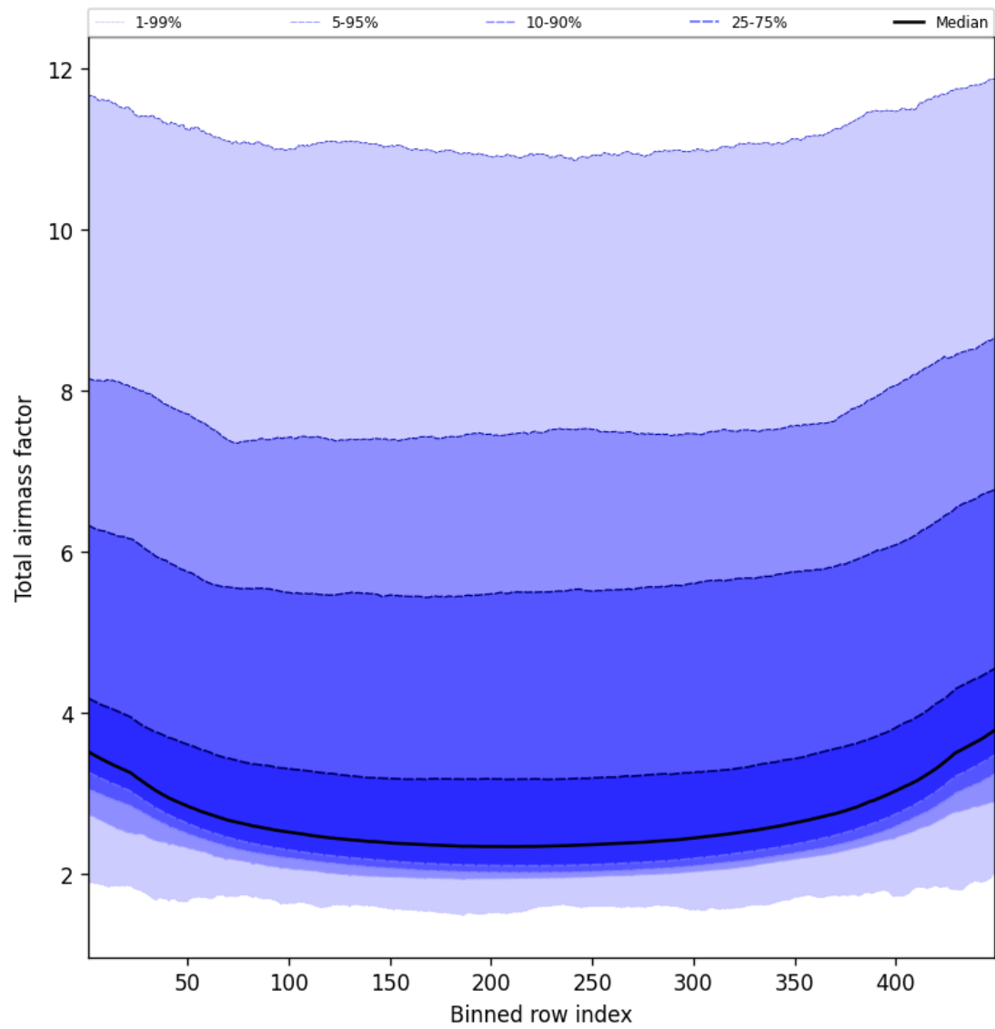
Figure 49: Along track statistics of “Total airmass factor” for 2025-11-28 to 2025-11-29
