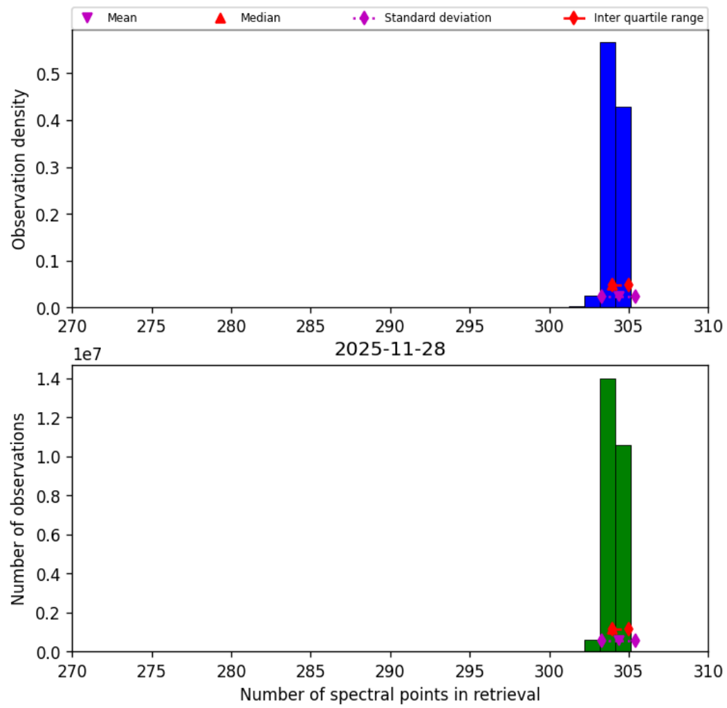
Figure 33: Histogram of “Number of spectral points in retrieval” for 2025-11-28 to 2025-11-29
