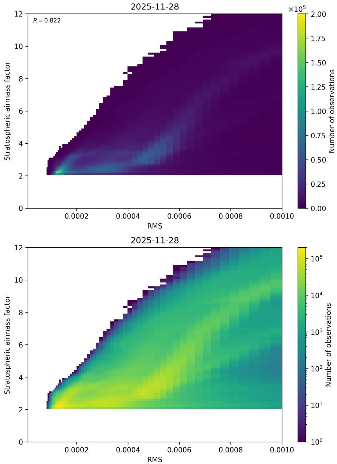
Figure 144: Scatter density plot of “RMS” against “Stratospheric airmass factor” for 2025-11-28 to 2025-11-29.
