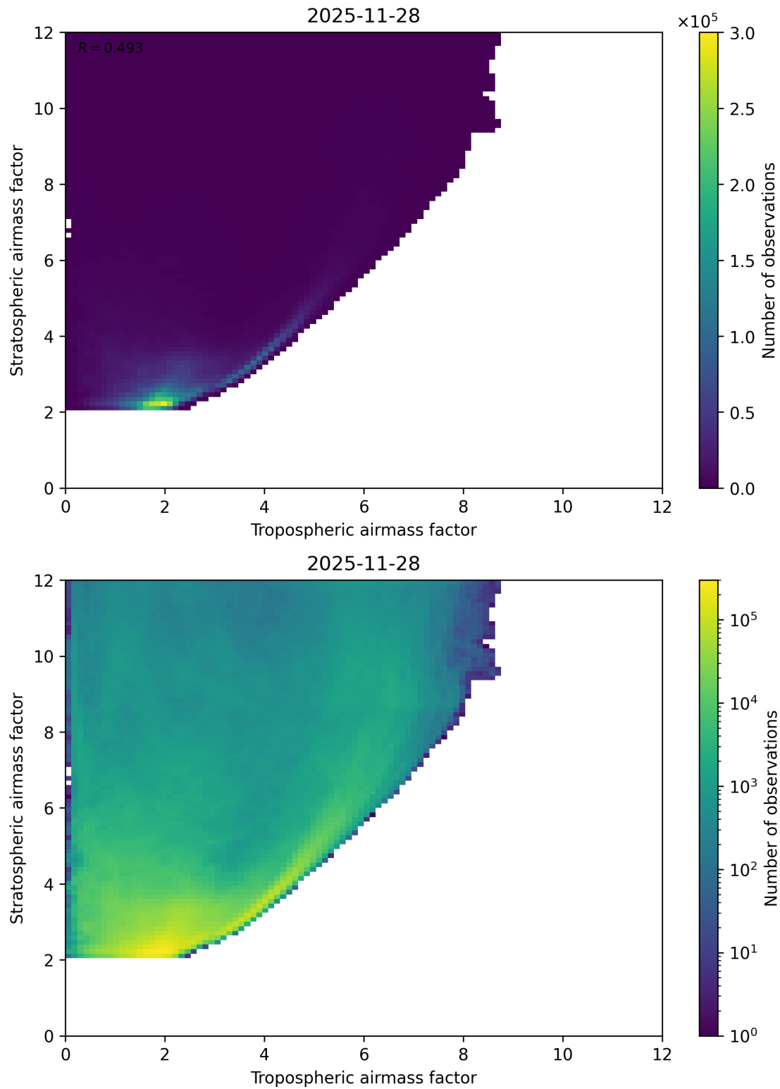
Figure 71: Scatter density plot of “Tropospheric airmass factor” against “Stratospheric airmass factor” for 2025-11-28 to 2025-11-29.
