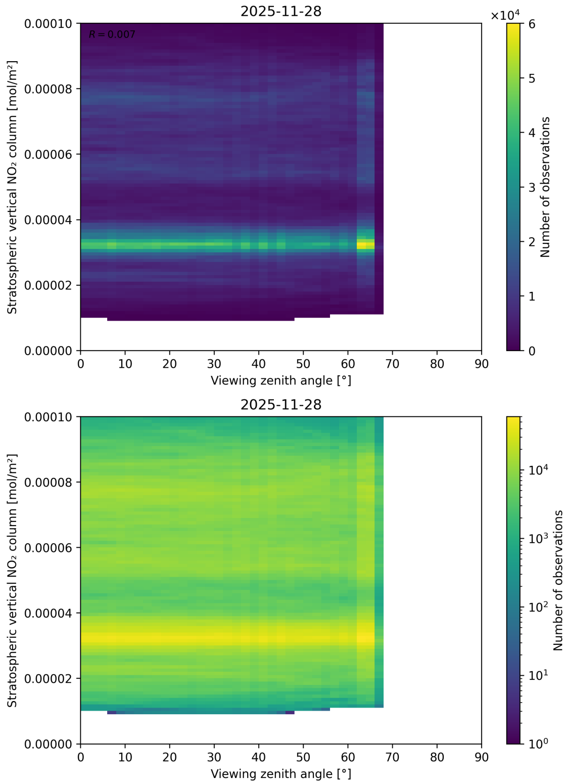
Figure 164: Scatter density plot of “Viewing zenith angle” against “Stratospheric vertical NO 2 column” for 2025-11-28 to 2025-11-29.
