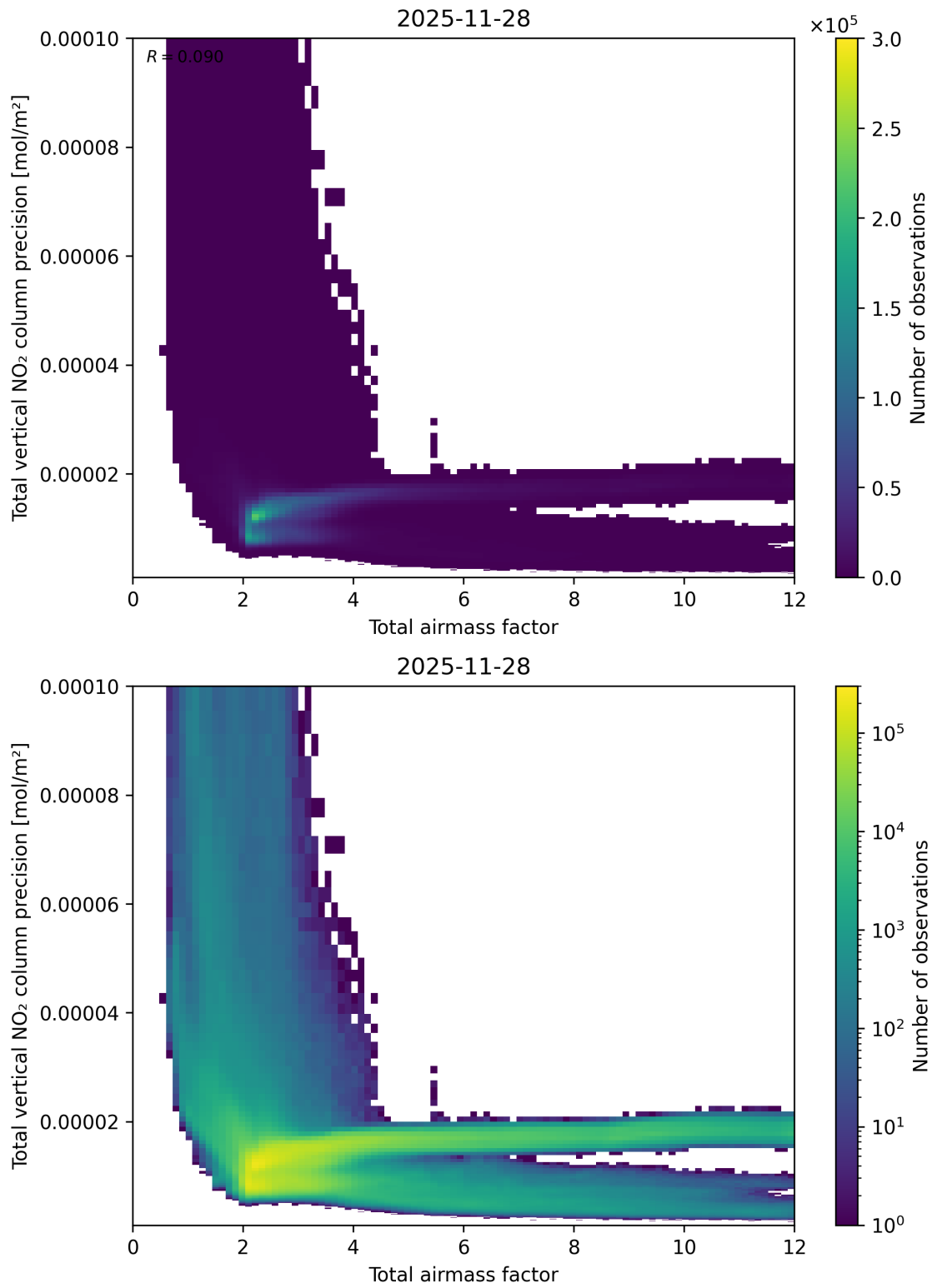
Figure 68: Scatter density plot of “Total airmass factor” against “Total vertical NO 2 column precision” for 2025-11-28 to 2025-11-29.
