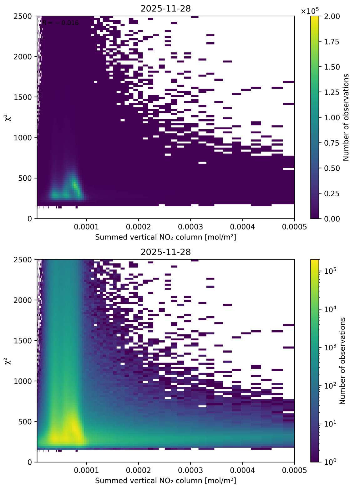
Figure 104: Scatter density plot of “Summed vertical NO 2 column” against “ \chi^2 ” for 2025-11-28 to 2025-11-29.
