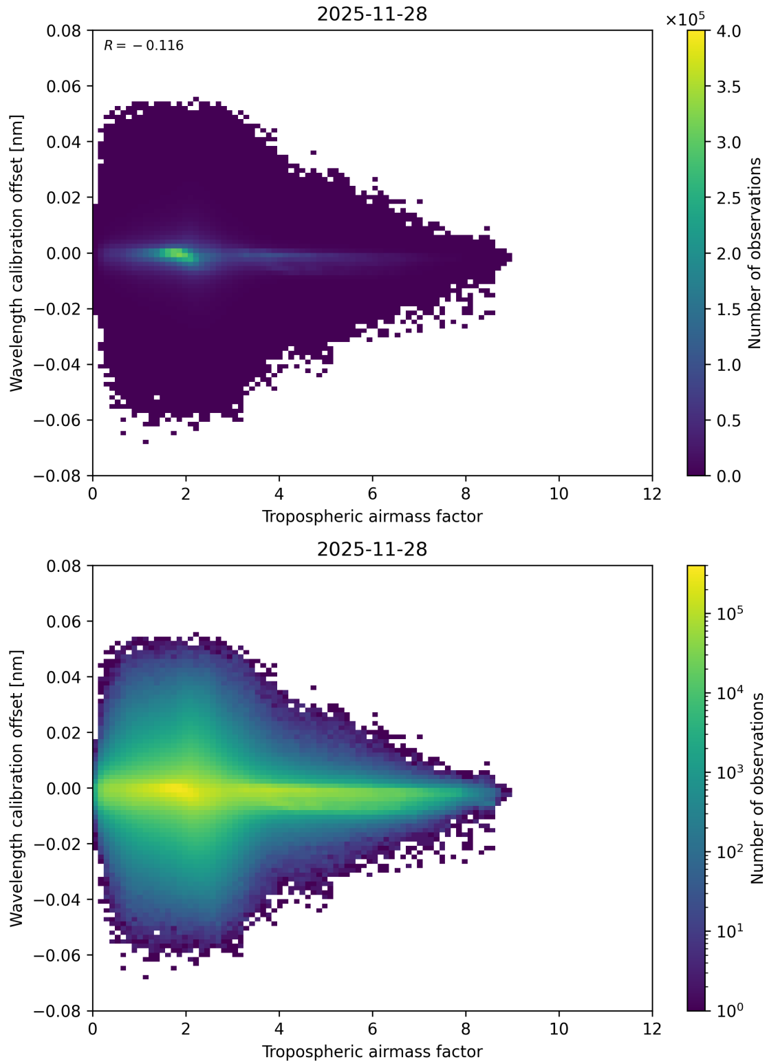
Figure 80: Scatter density plot of “Tropospheric airmass factor” against “Wavelength calibration offset” for 2025-11-28 to 2025-11-29.
