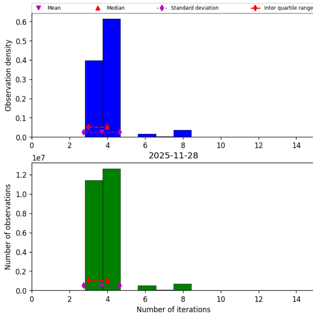
Figure 34: Histogram of “Number of iterations” for 2025-11-28 to 2025-11-29
