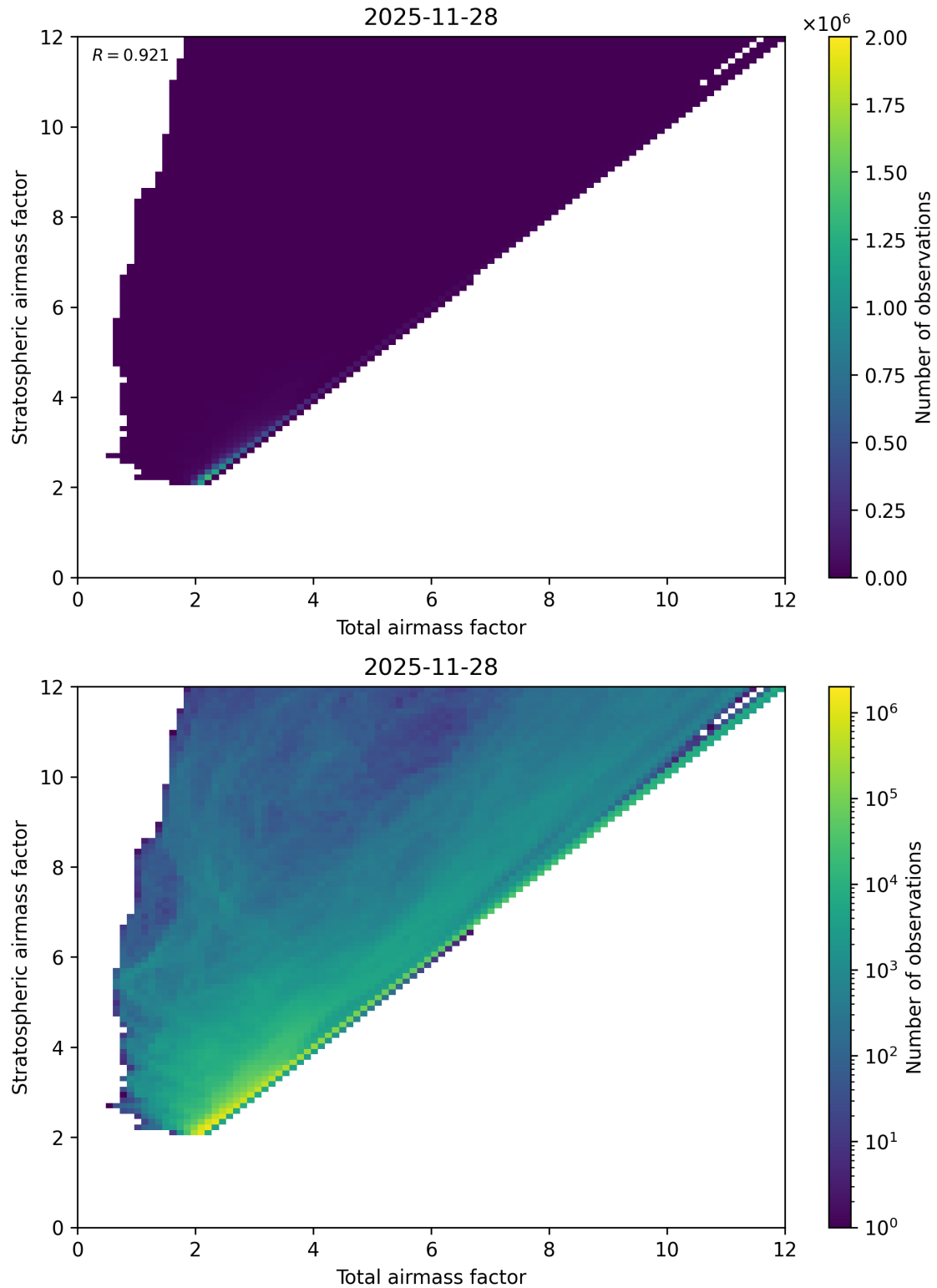
Figure 62: Scatter density plot of “Total airmass factor” against “Stratospheric airmass factor” for 2025-11-28 to 2025-11-29.
