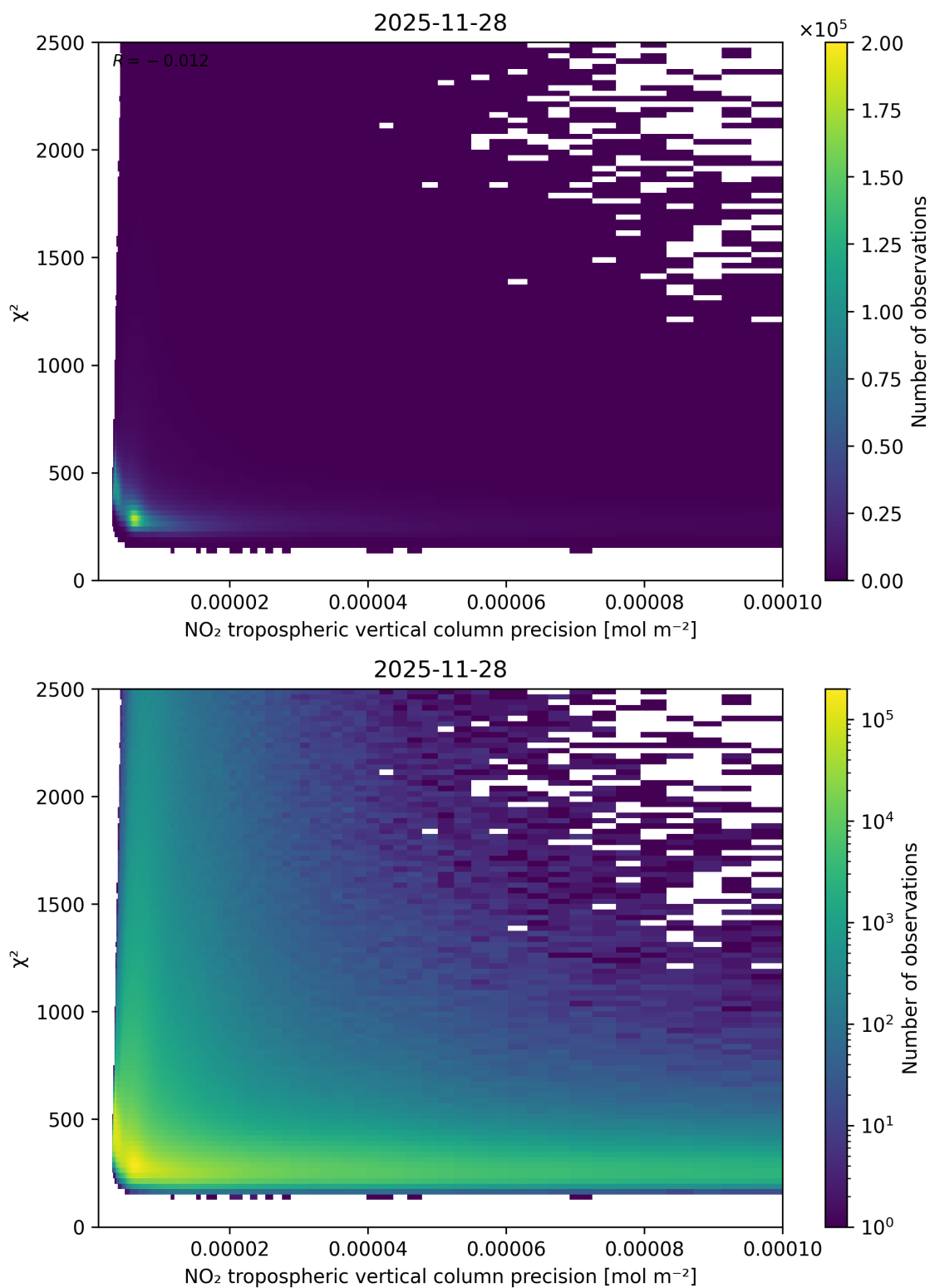
Figure 134: Scatter density plot of “NO 2 tropospheric vertical column precision” against “ \chi^2 ” for 2025-11-28 to 2025-11-29.
