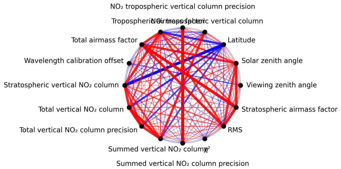
Figure 1: Map of correlation graph for 2025-11-28 to 2025-11-29.
