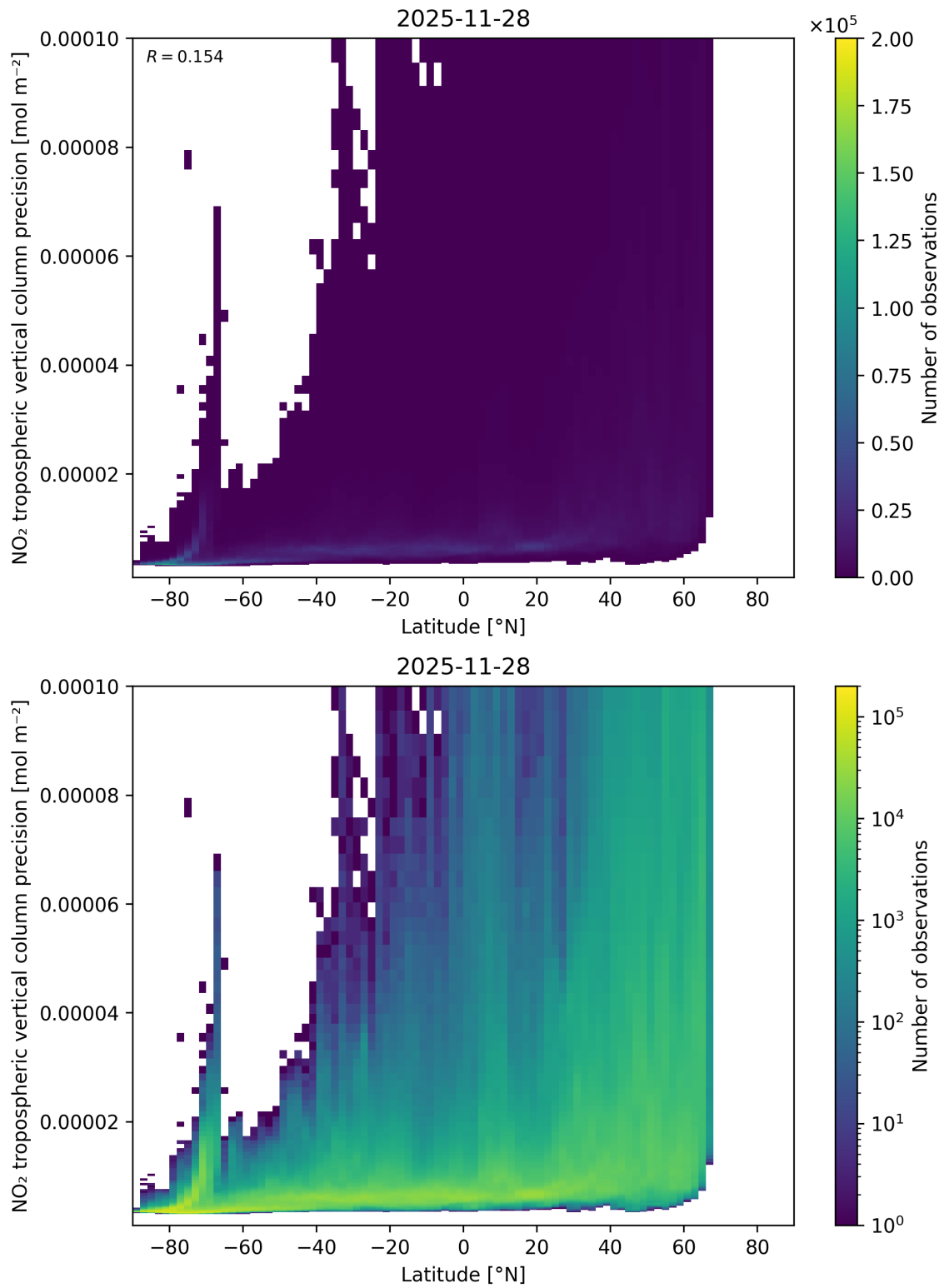
Figure 93: Scatter density plot of “Latitude” against “NO 2 tropospheric vertical column precision” for 2025-11-28 to 2025-11-29.
