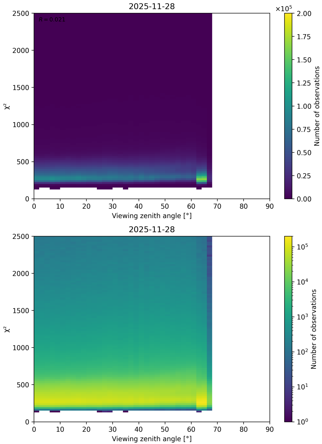
Figure 162: Scatter density plot of “Viewing zenith angle” against “ \chi^2 ” for 2025-11-28 to 2025-11-29.
