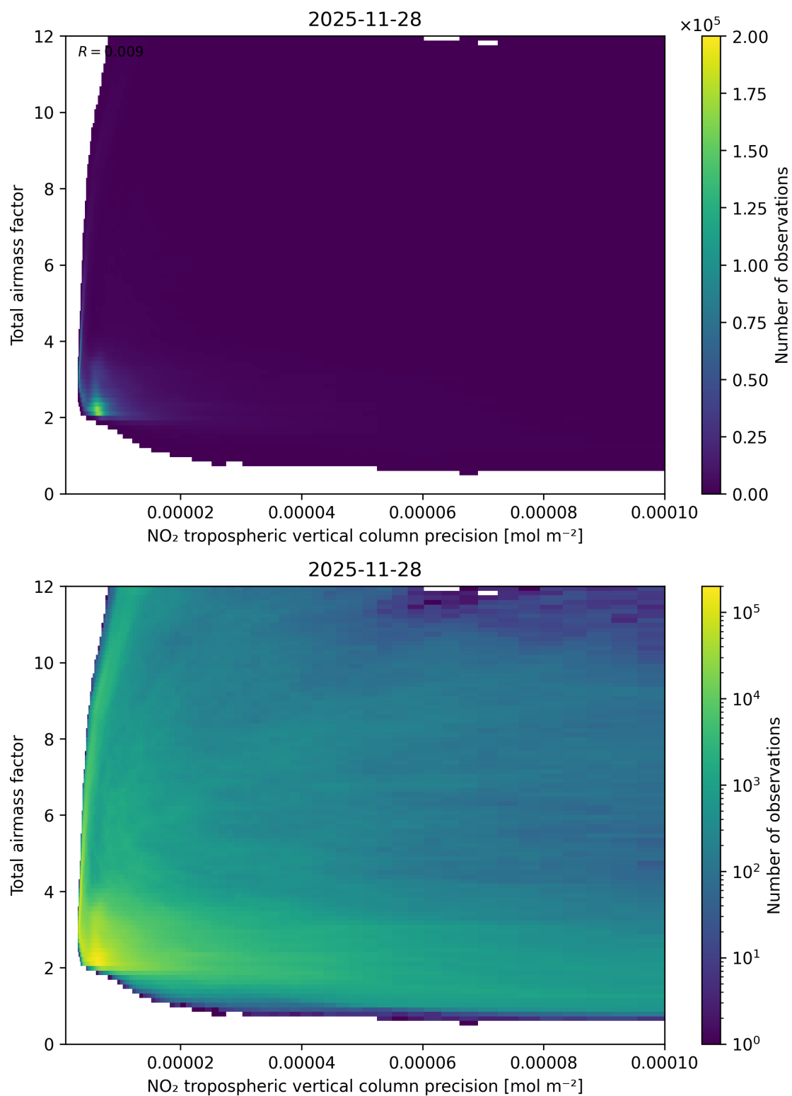
Figure 132: Scatter density plot of “NO 2 tropospheric vertical column precision” against “Total air mass factor” for 2025-11-28 to 2025-11-29.
