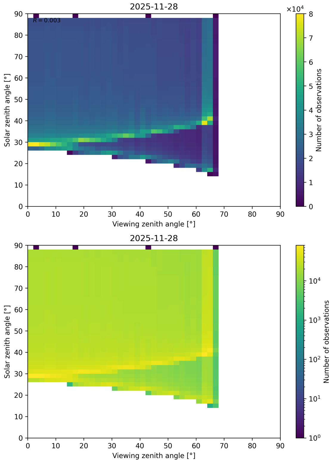
Figure 172: Scatter density plot of “Viewing zenith angle” against “Solar zenith angle” for 2025-11-28 to 2025-11-29.
