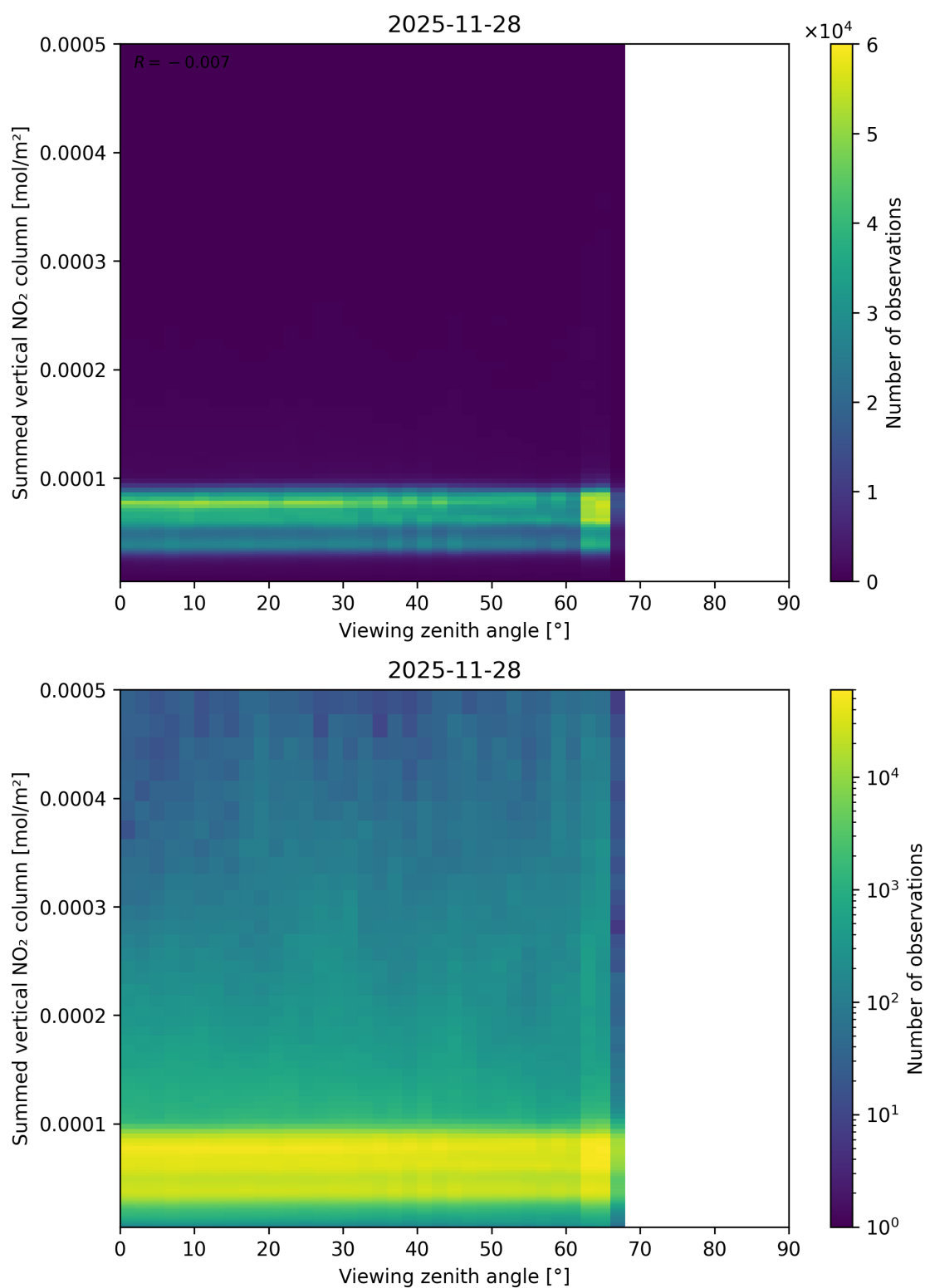
Figure 165: Scatter density plot of “Viewing zenith angle” against “Summed vertical NO 2 column” for 2025-11-28 to 2025-11-29.
