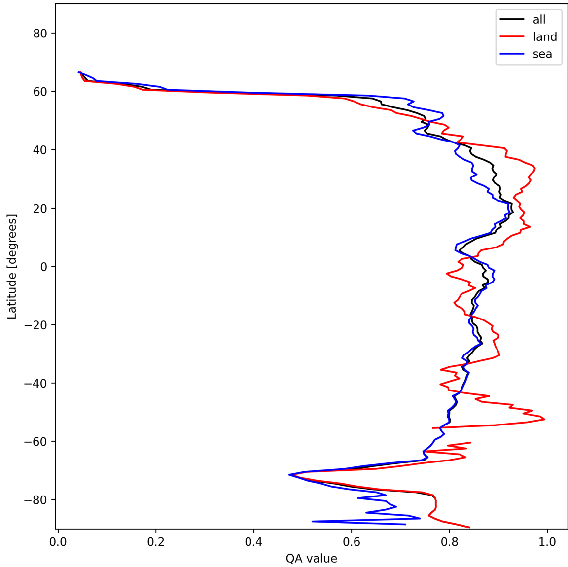
Figure 11: Zonal average of “QA value” for 2025-11-28 to 2025-11-29.
