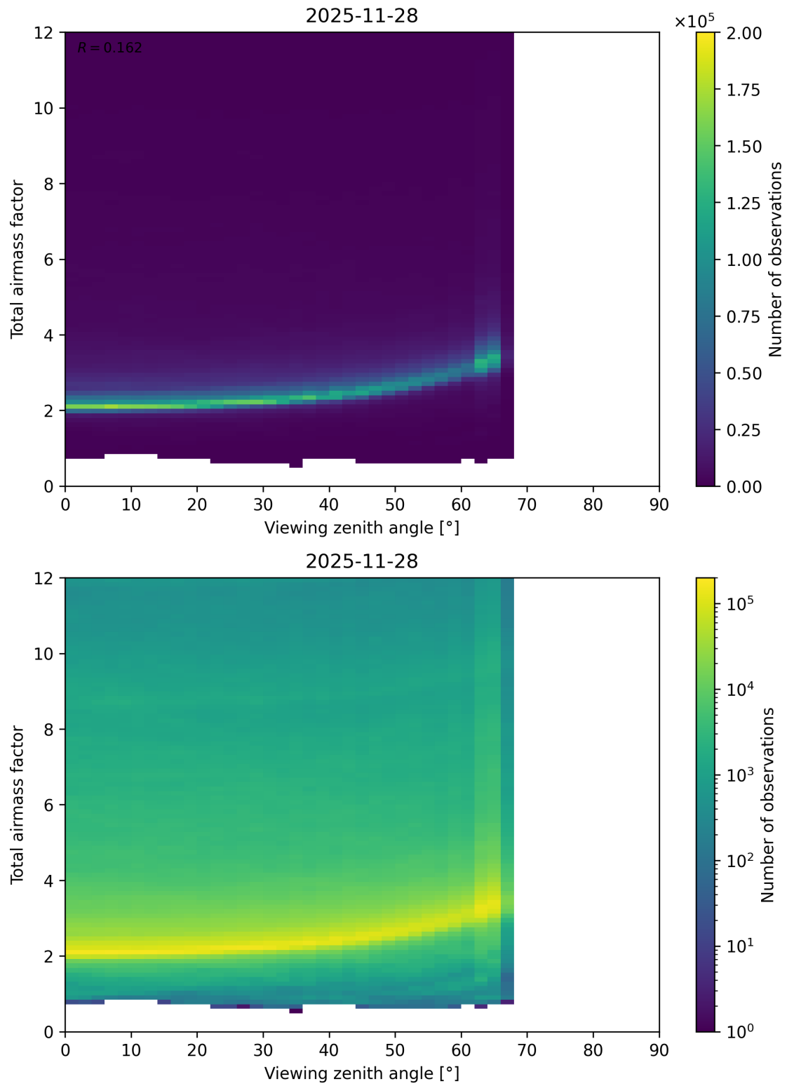
Figure 160: Scatter density plot of “Viewing zenith angle” against “Total airmass factor” for 2025-11-28 to 2025-11-29.
