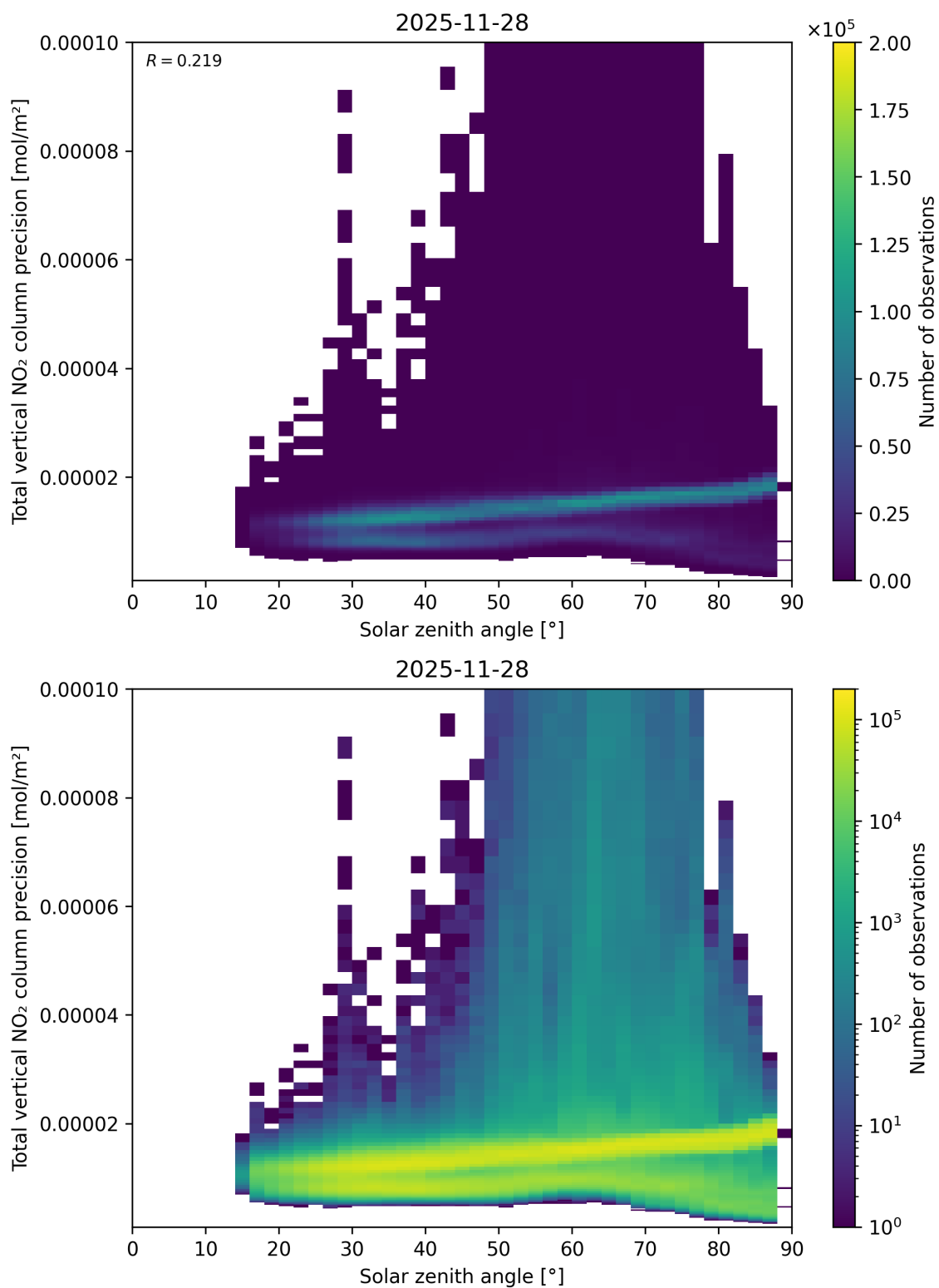
Figure 154: Scatter density plot of “Solar zenith angle” against “Total vertical NO 2 column precision” for 2025-11-28 to 2025-11-29.
