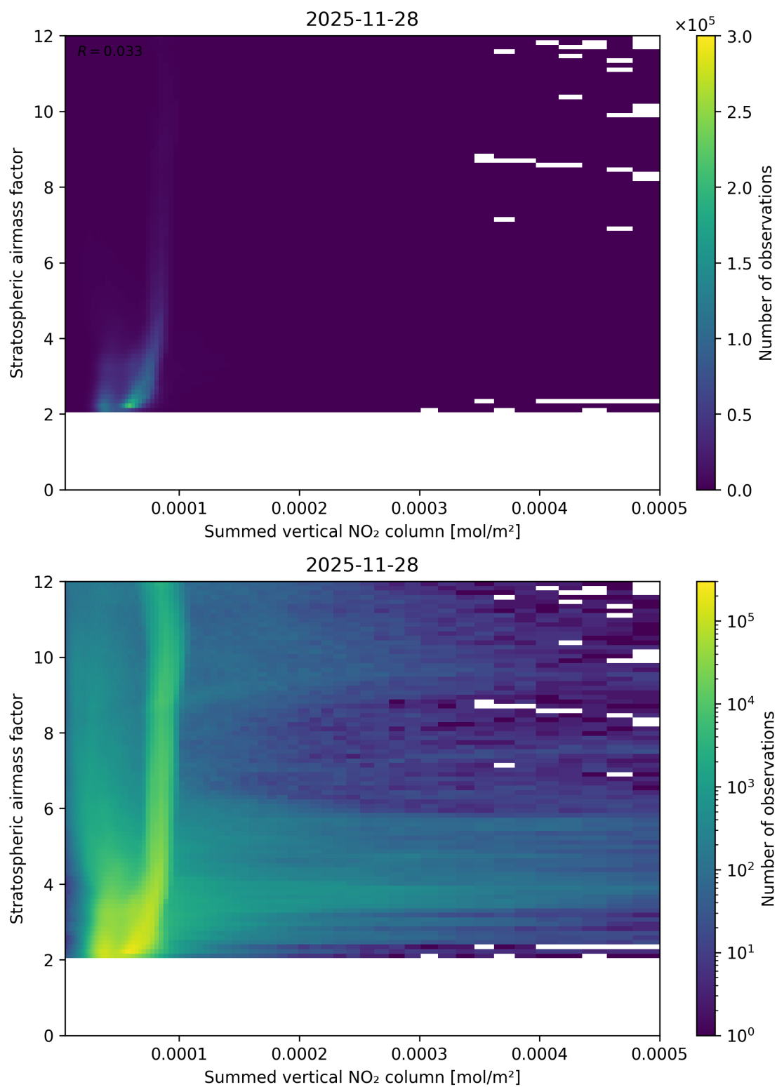
Figure 103: Scatter density plot of “Summed vertical NO 2 column” against “Stratospheric airmass factor” for 2025-11-28 to 2025-11-29.
