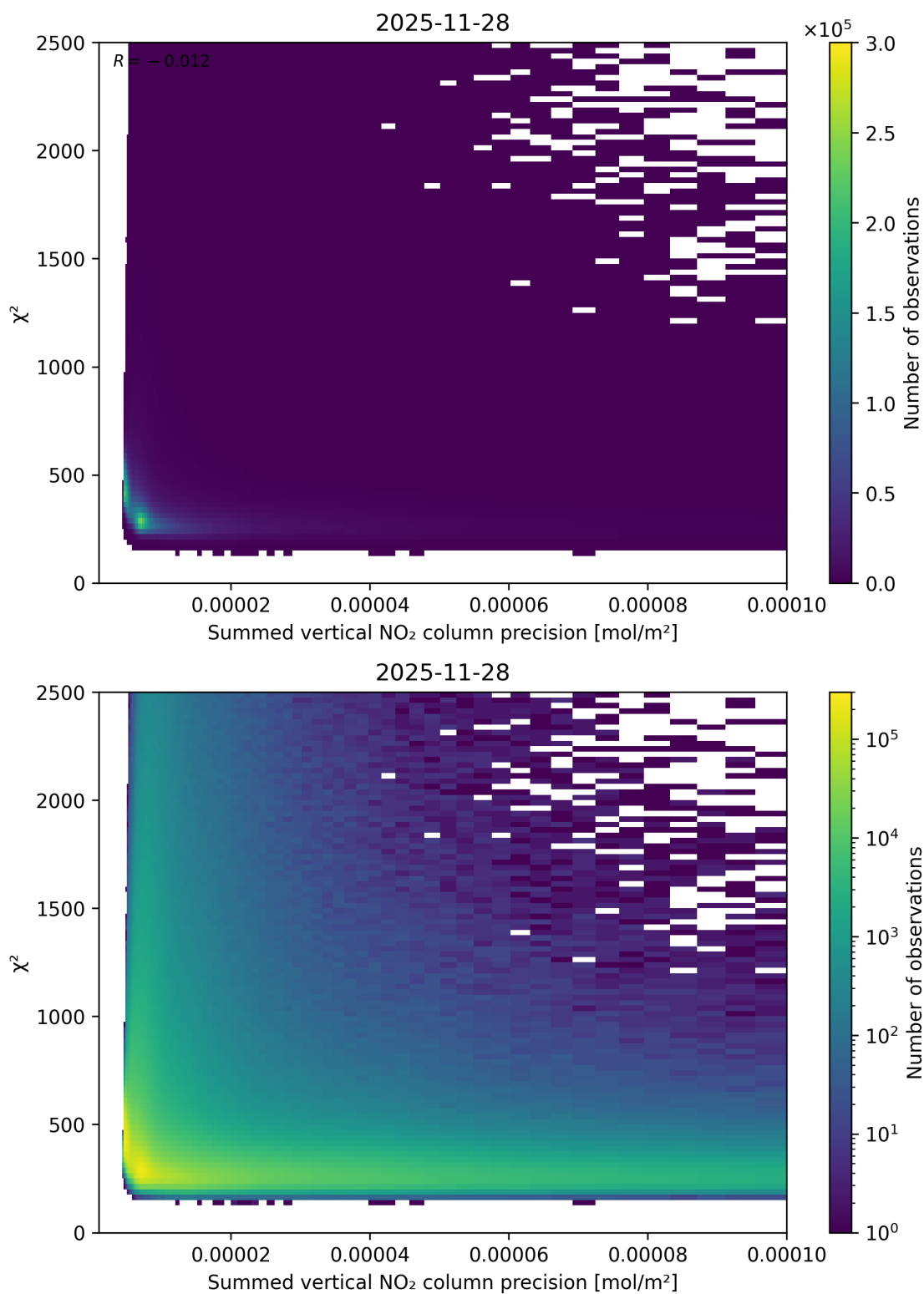
Figure 107: Scatter density plot of “Summed vertical NO 2 column precision” against “ \chi^2 ” for 2025-11-28 to 2025-11-29.
