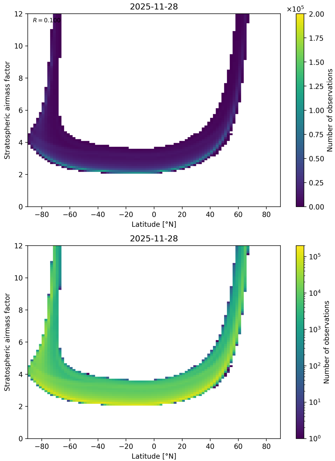
Figure 83: Scatter density plot of “Latitude” against “Stratospheric airmass factor” for 2025-11-28 to 2025-11-29.
