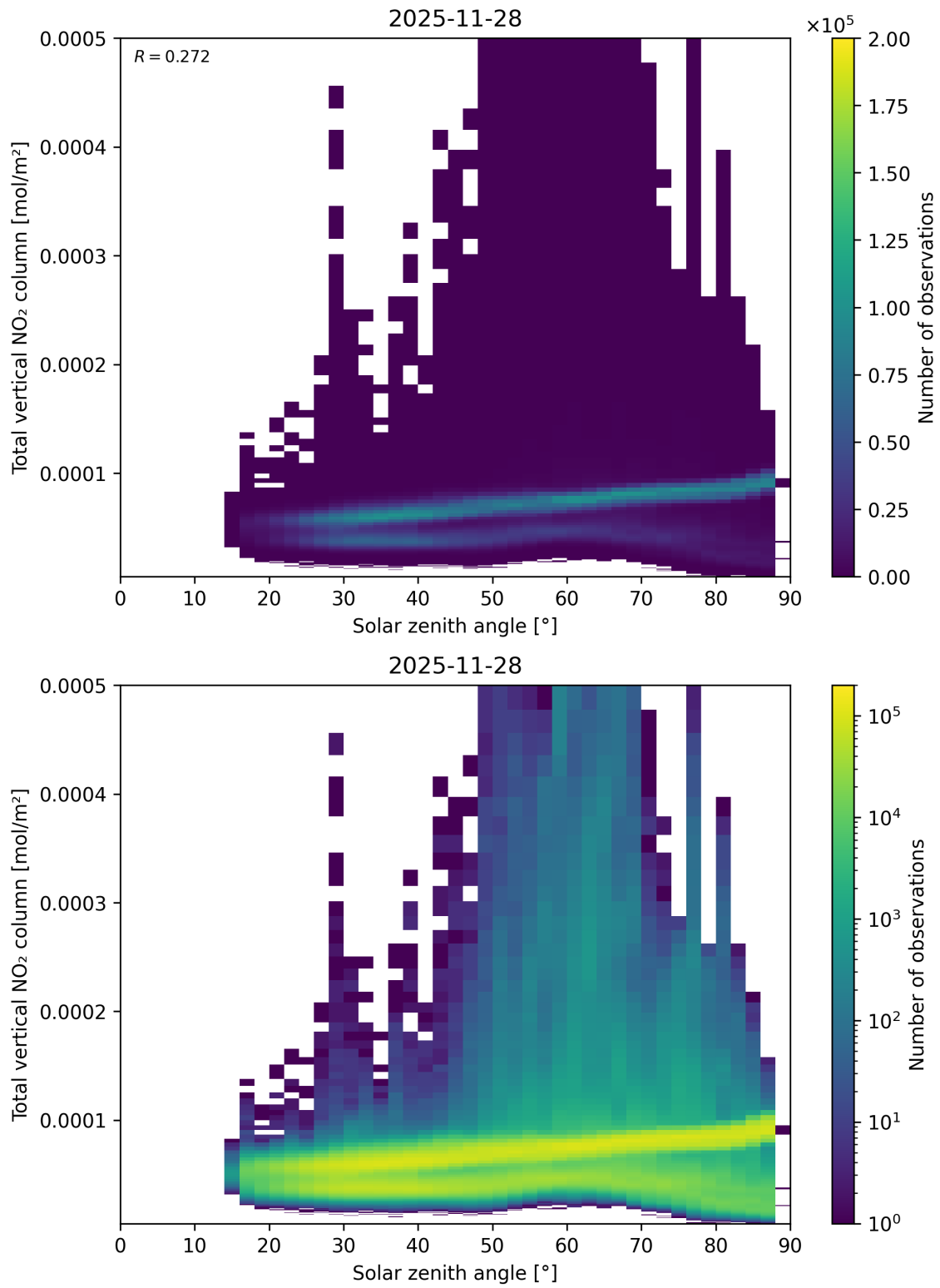
Figure 153: Scatter density plot of “Solar zenith angle” against “Total vertical NO 2 column” for 2025-11-28 to 2025-11-29.
