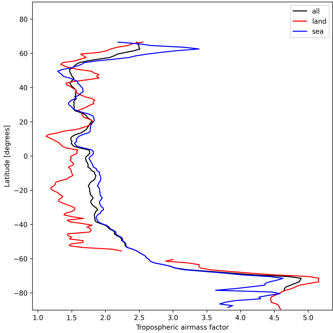
Figure 14: Zonal average of “Tropospheric airmass factor” for 2025-11-28 to 2025-11-29.
