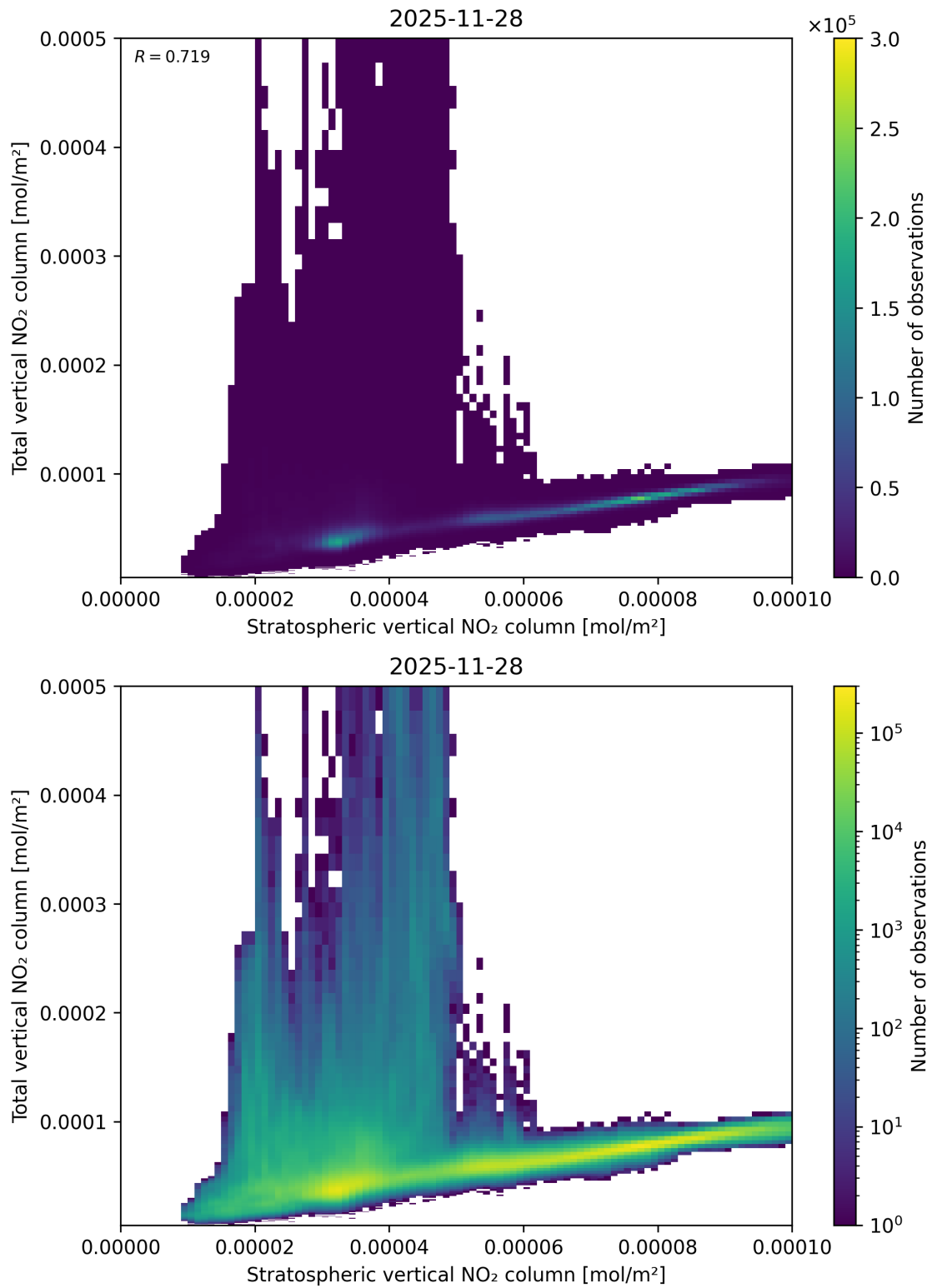
Figure 100: Scatter density plot of “Stratospheric vertical NO 2 column” against “Total vertical NO 2 column” for 2025-11-28 to 2025-11-29.
