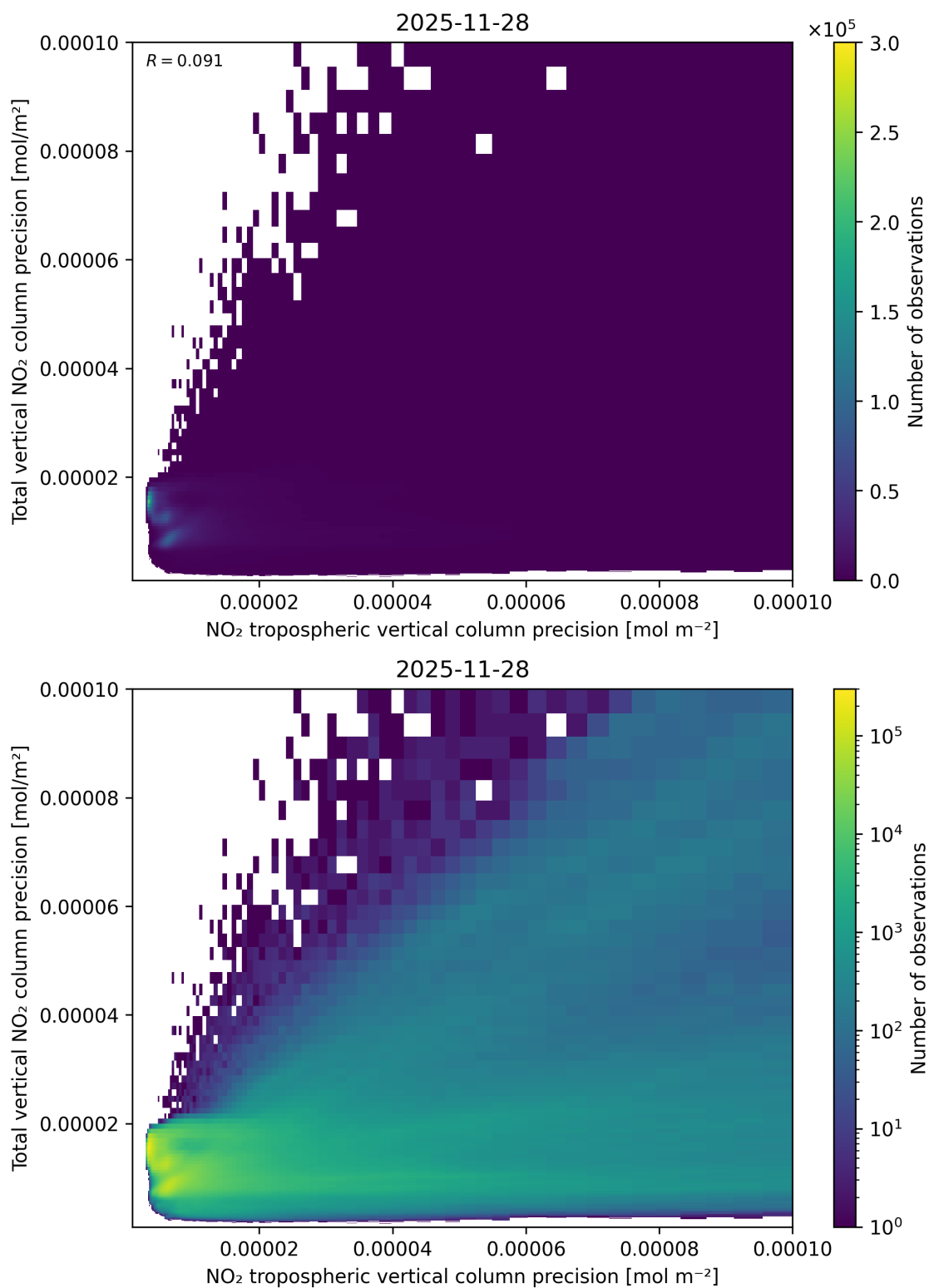
Figure 139: Scatter density plot of “NO 2 tropospheric vertical column precision” against “Total vertical NO 2 column precision” for 2025-11-28 to 2025-11-29.
