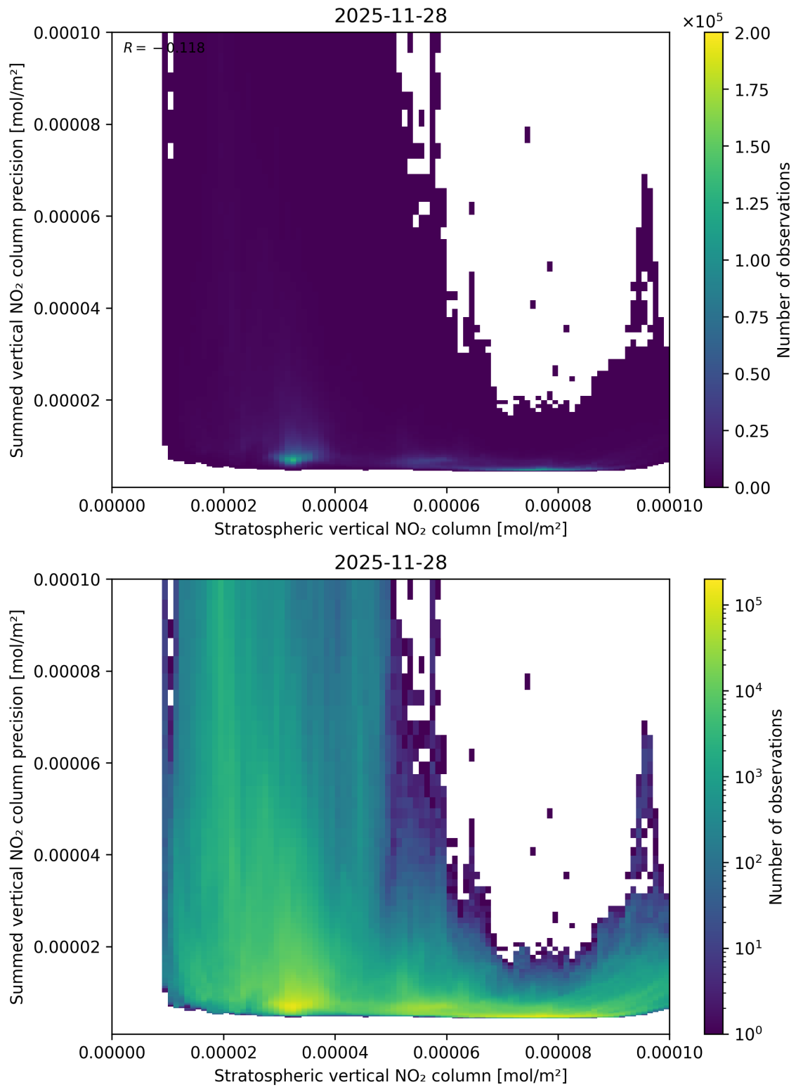
Figure 99: Scatter density plot of “Stratospheric vertical NO 2 column” against “Summed vertical NO 2 column precision” for 2025-11-28 to 2025-11-29.
