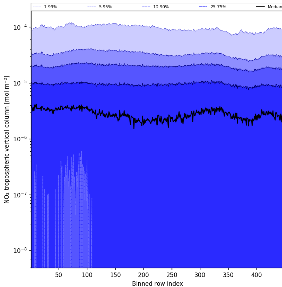
Figure 46: Along track statistics of “NO 2 tropospheric vertical column” for 2025-11-28 to 2025-11-29
