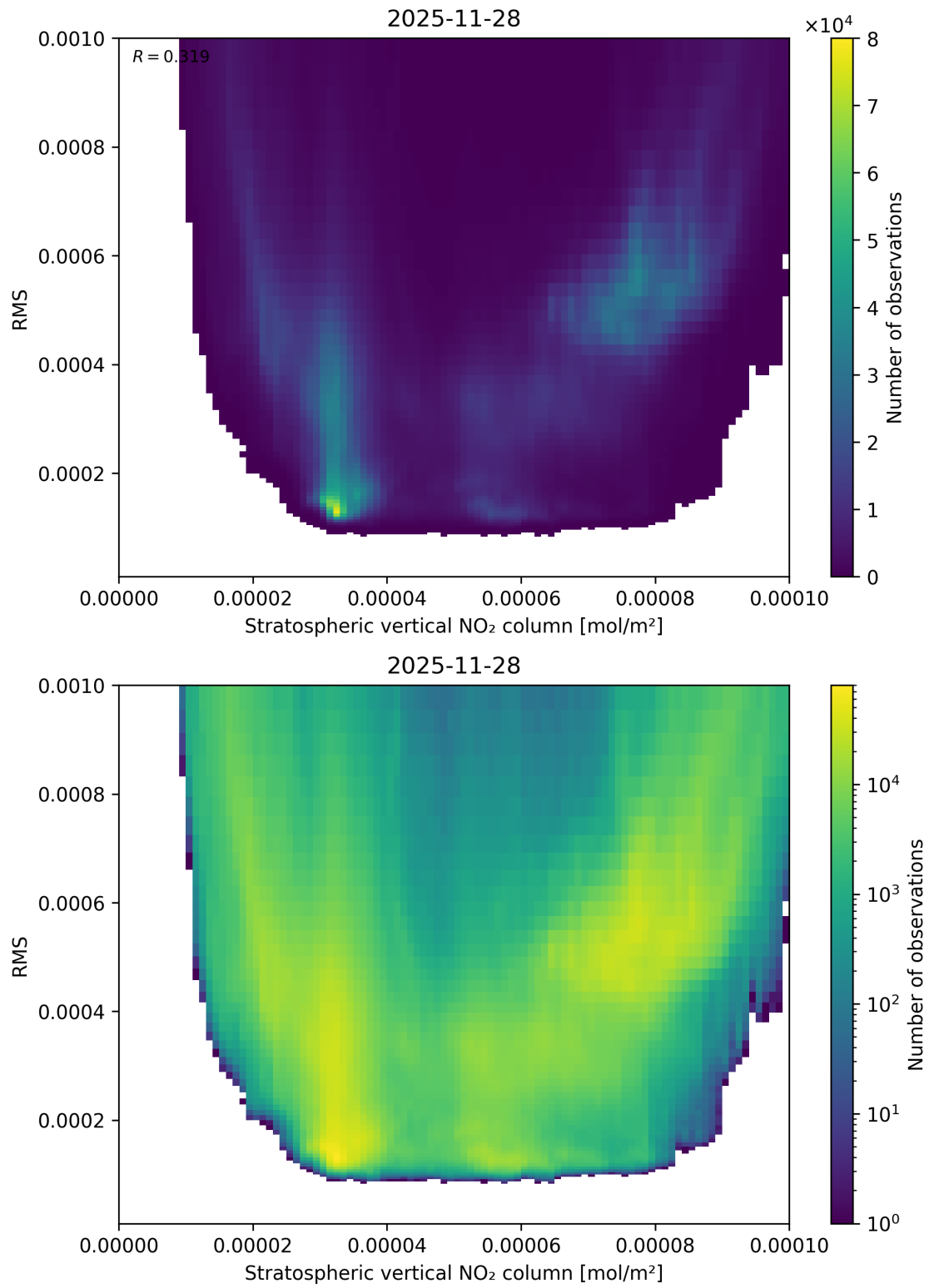
Figure 102: Scatter density plot of “Stratospheric vertical NO 2 column” against “RMS” for 2025-11-28 to 2025-11-29.
