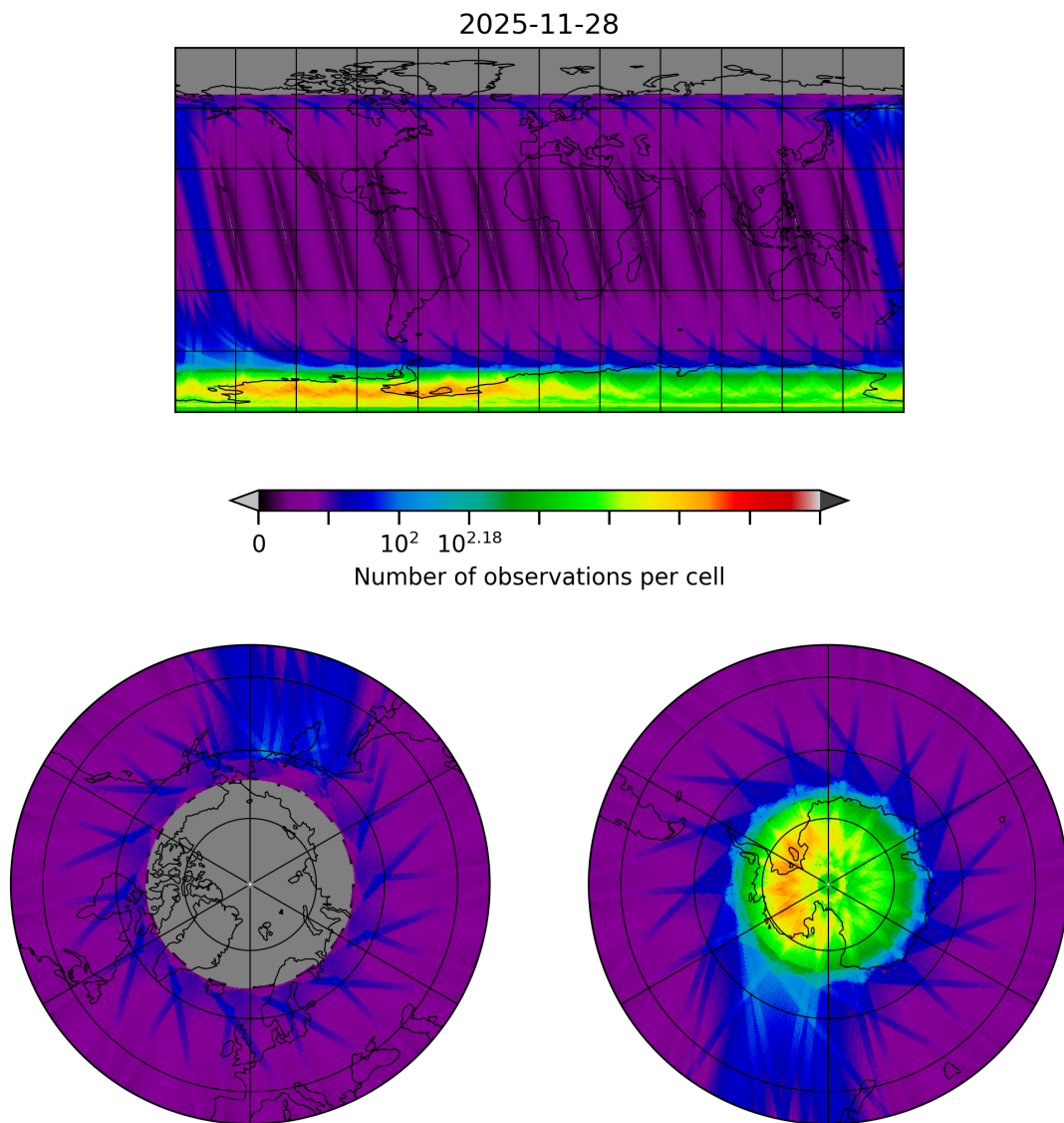
Figure 10: Map of the number of observations for 2025-11-28 to 2025-11-29
