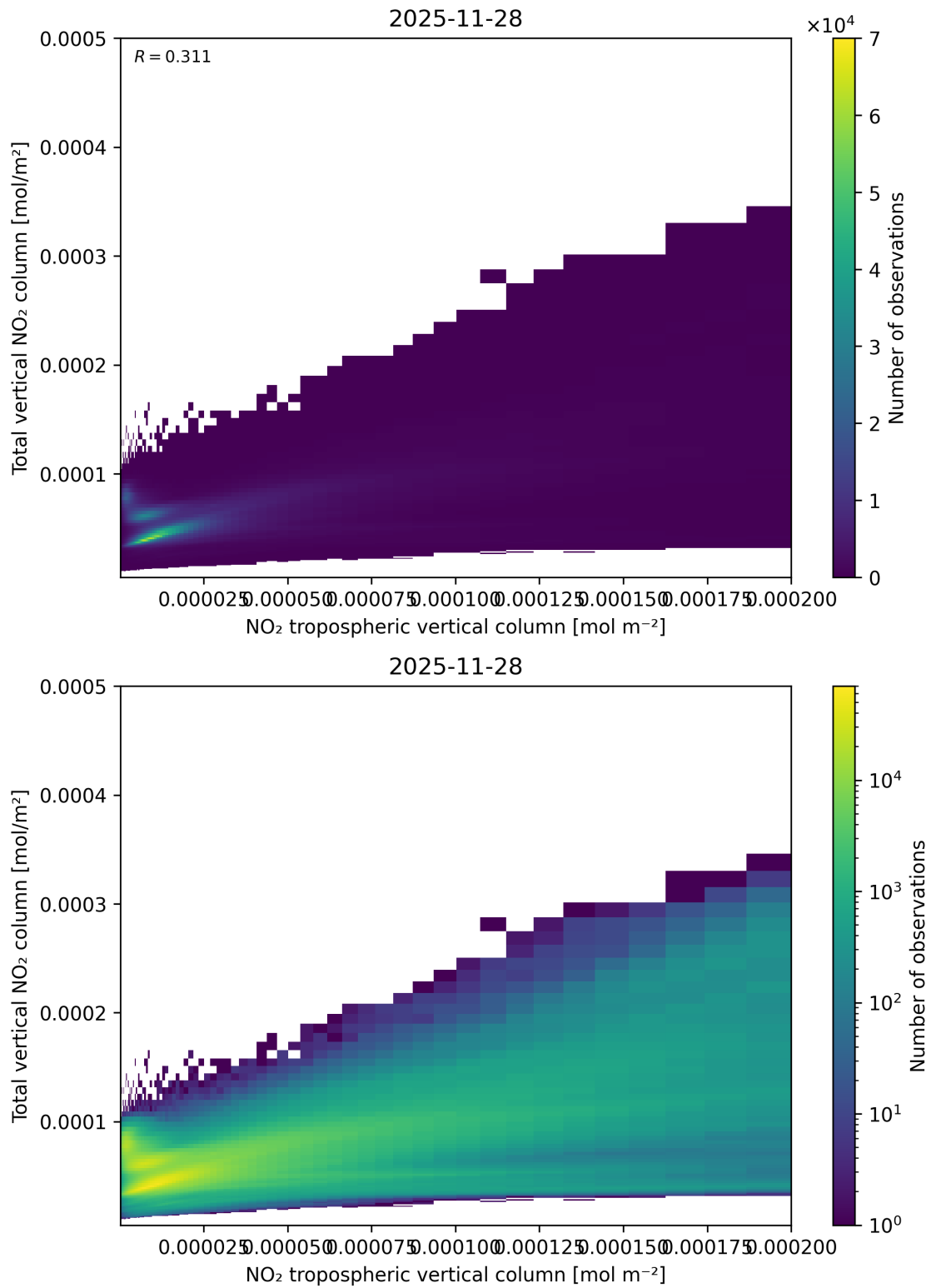
Figure 128: Scatter density plot of “NO 2 tropospheric vertical column” against “Total vertical NO 2 column” for 2025-11-28 to 2025-11-29.
