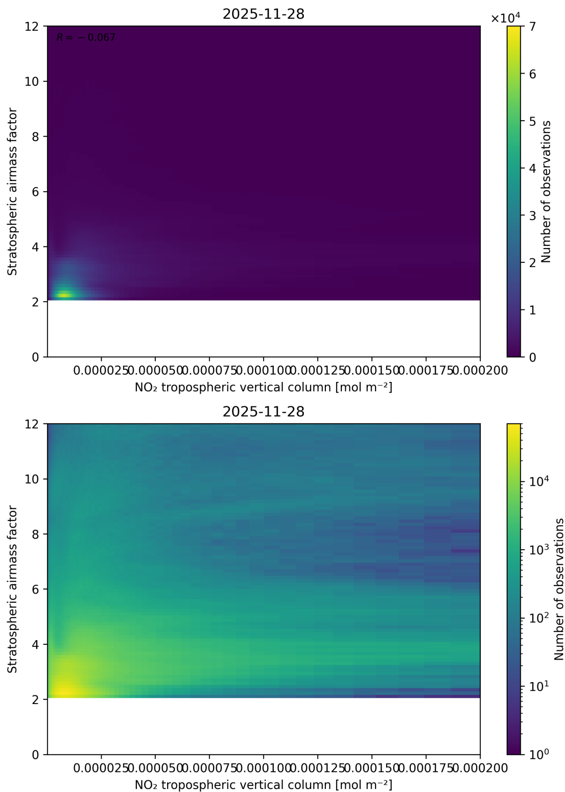
Figure 121: Scatter density plot of “NO 2 tropospheric vertical column” against “Stratospheric airmass factor” for 2025-11-28 to 2025-11-29.
