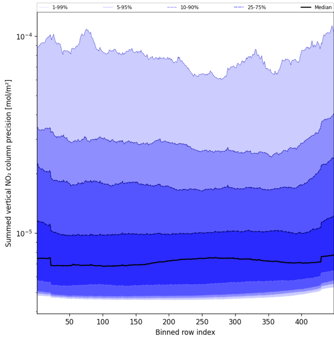
Figure 58: Along track statistics of “Summed vertical NO 2 column precision” for 2025-11-28 to 2025-11-29
