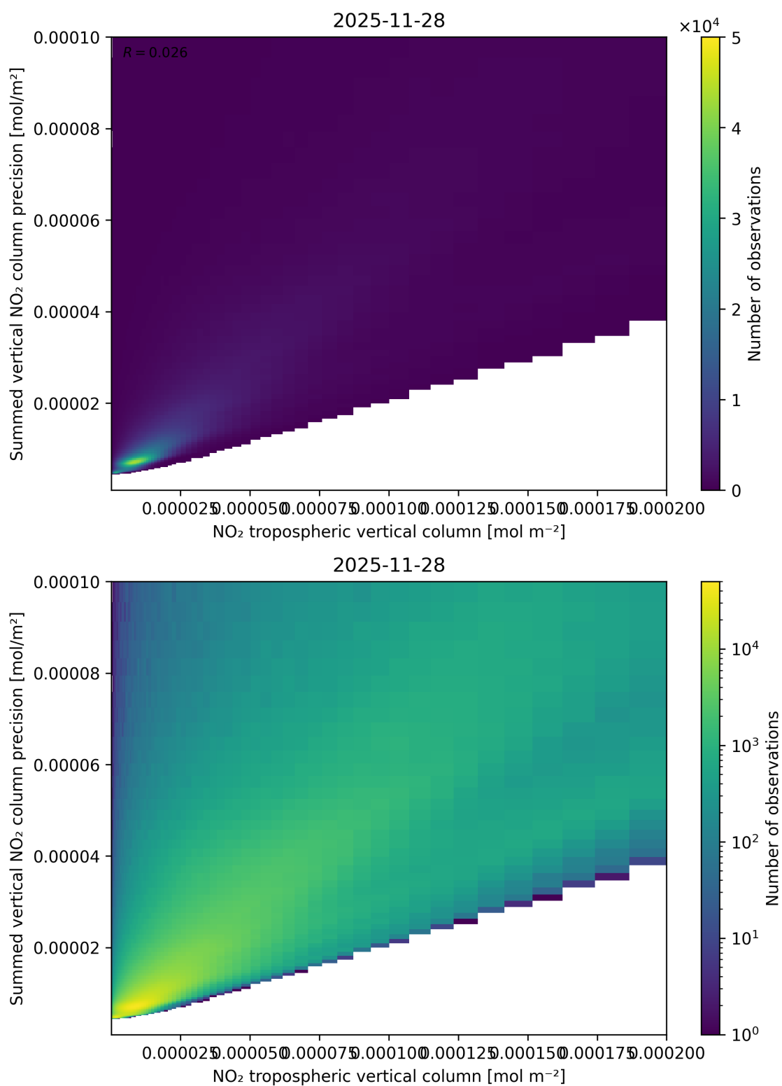
Figure 127: Scatter density plot of “NO 2 tropospheric vertical column” against “Summed vertical NO 2 column precision” for 2025-11-28 to 2025-11-29.
