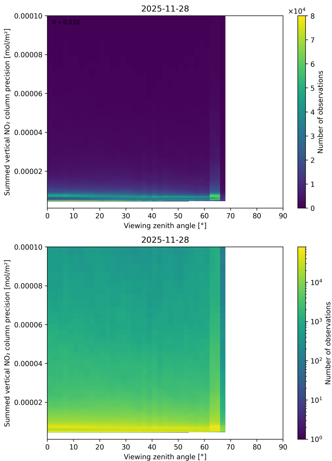
Figure 166: Scatter density plot of “Viewing zenith angle” against “Summed vertical NO 2 column precision” for 2025-11-28 to 2025-11-29.
