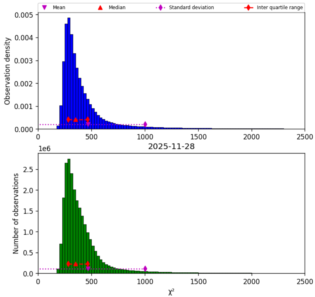
Figure 42: Histogram of “ \chi^2 ” for 2025-11-28 to 2025-11-29
