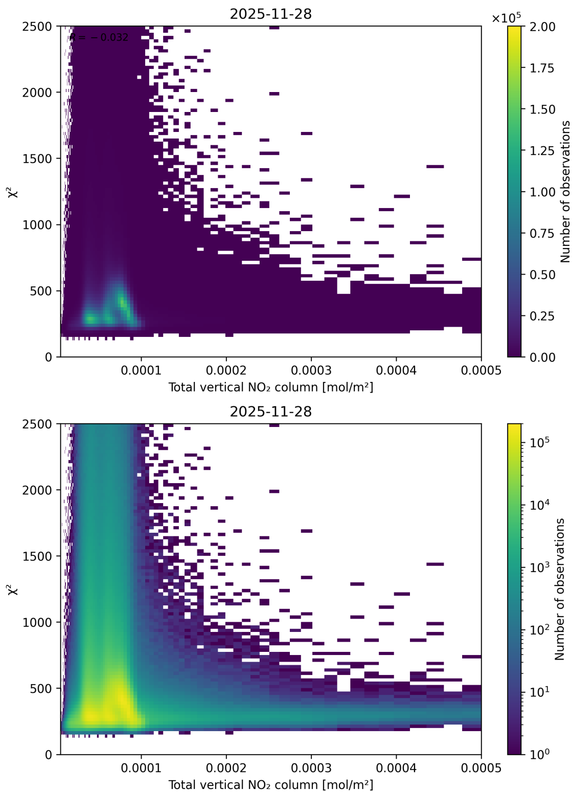
Figure 111: Scatter density plot of “Total vertical NO 2 column” against “ \chi^2 ” for 2025-11-28 to 2025-11-29.
