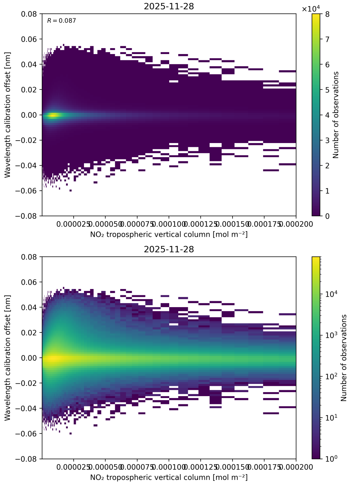
Figure 143: Scatter density plot of “NO 2 tropospheric vertical column” against “Wavelength calibration offset” for 2025-11-28 to 2025-11-29.
