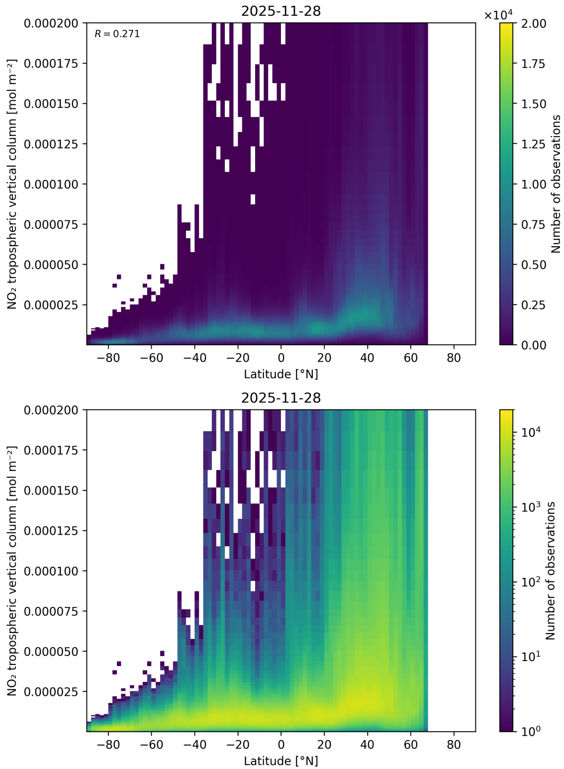
Figure 92: Scatter density plot of “Latitude” against “NO 2 tropospheric vertical column” for 2025-11-28 to 2025-11-29.
