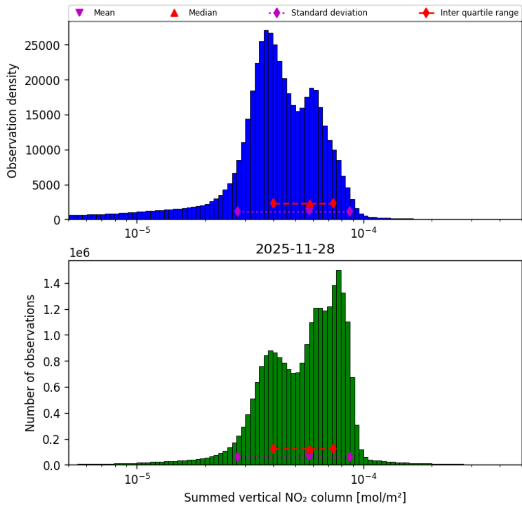
Figure 40: Histogram of “Summed vertical NO 2 column” for 2025-11-28 to 2025-11-29
