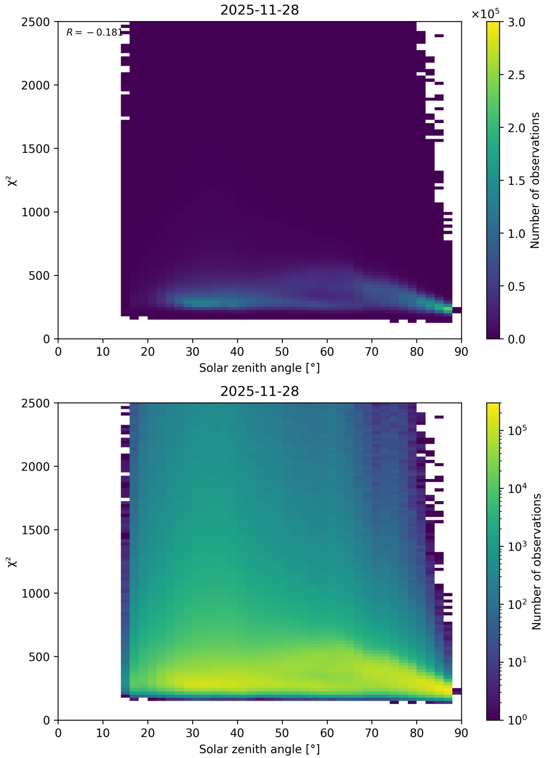
Figure 148: Scatter density plot of “Solar zenith angle” against “ \chi^2 ” for 2025-11-28 to 2025-11-29.
