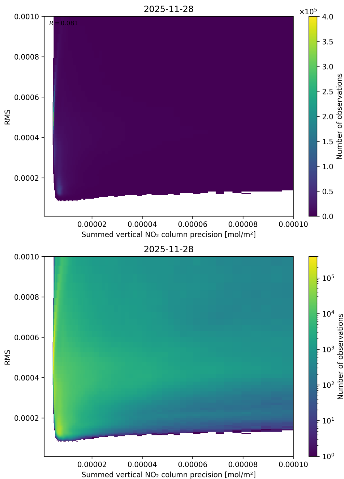
Figure 108: Scatter density plot of “Summed vertical NO 2 column precision” against “RMS” for 2025-11-28 to 2025-11-29.
