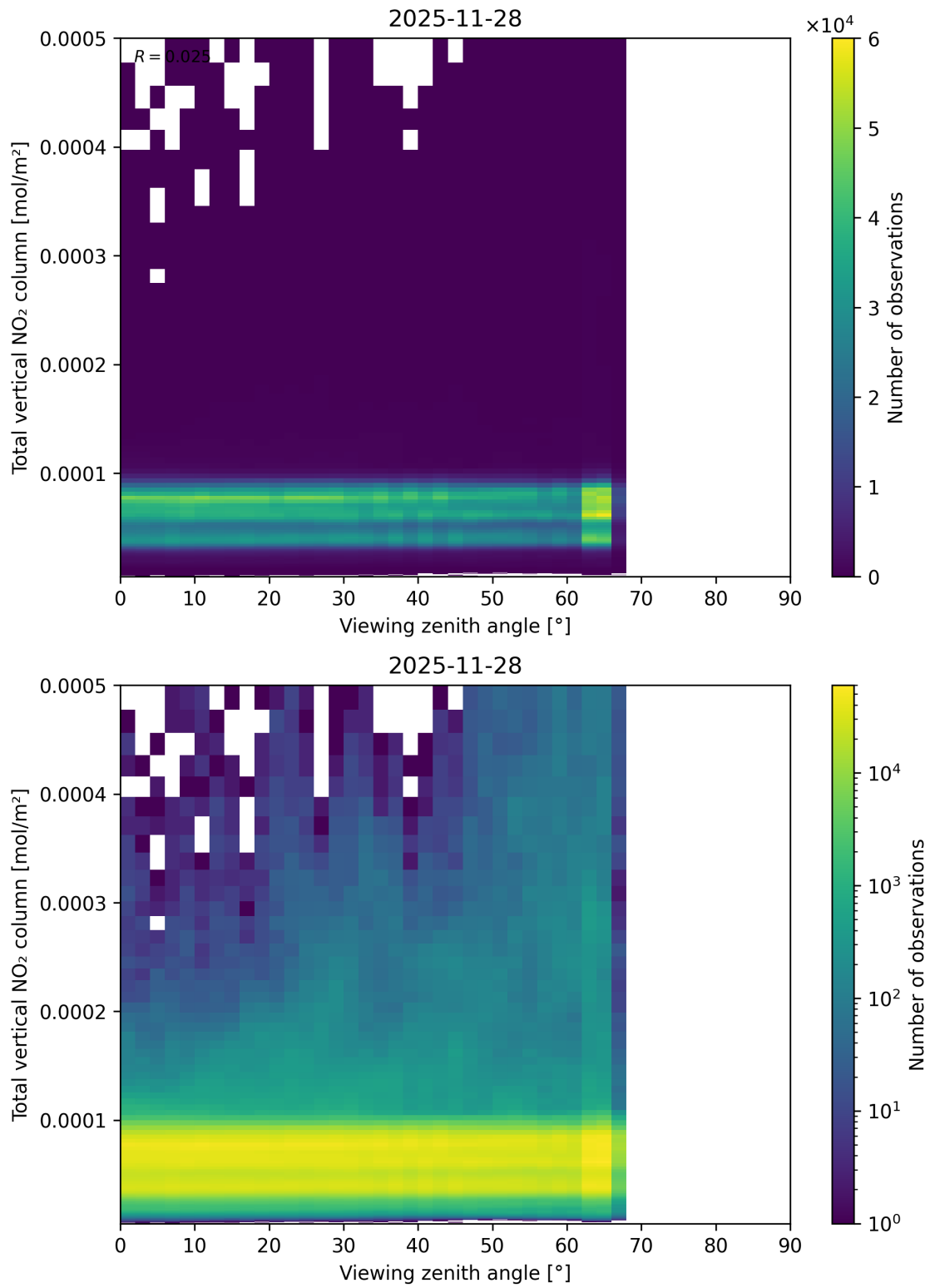
Figure 167: Scatter density plot of “Viewing zenith angle” against “Total vertical NO 2 column” for 2025-11-28 to 2025-11-29.
