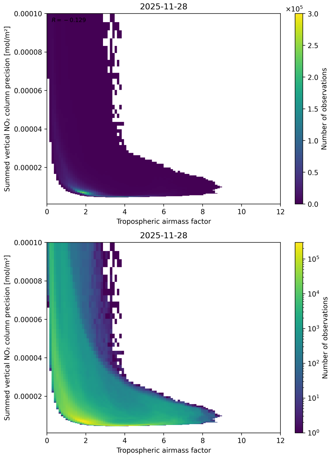
Figure 76: Scatter density plot of “Tropospheric airmass factor” against “Summed vertical NO 2 column precision” for 2025-11-28 to 2025-11-29.
