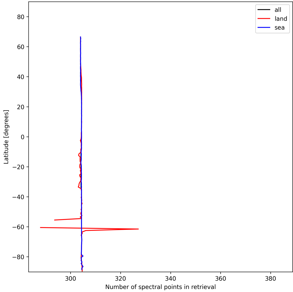
Figure 16: Zonal average of “Number of spectral points in retrieval” for 2025-11-28 to 2025-11-29.
