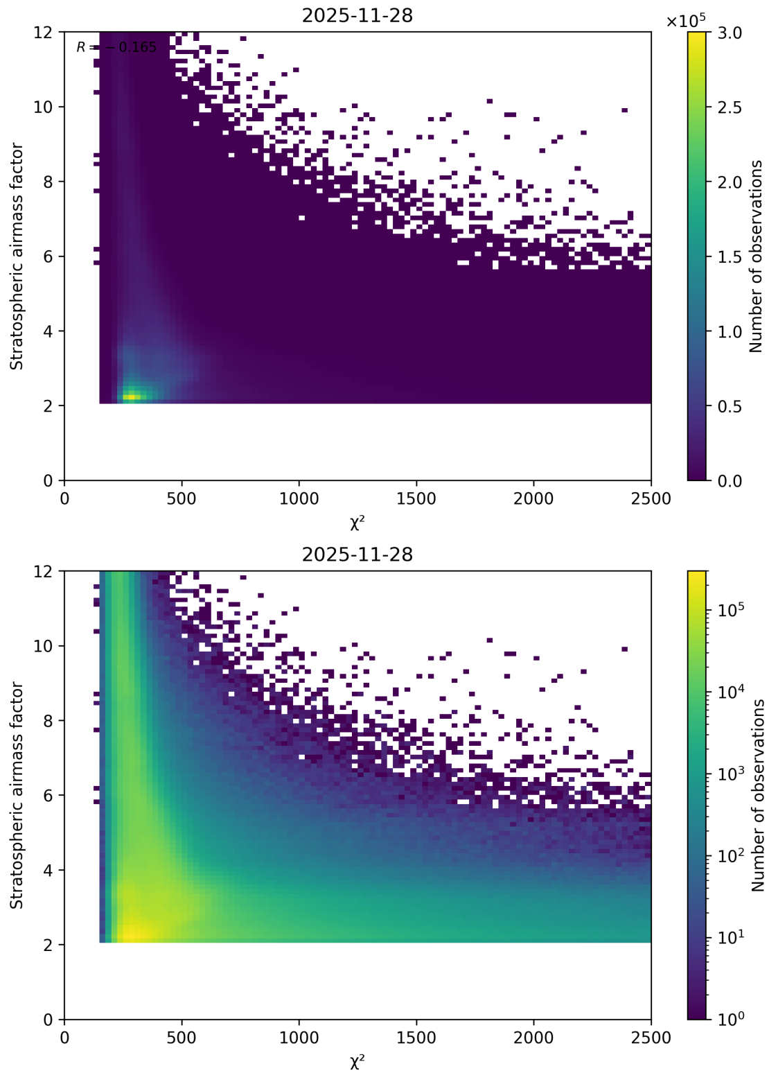
Figure 81: Scatter density plot of “ \chi^2 ” against “Stratospheric airmass factor” for 2025-11-28 to 2025-11-29.
