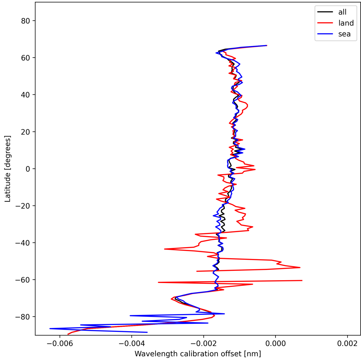
Figure 18: Zonal average of “Wavelength calibration offset” for 2025-11-28 to 2025-11-29.
