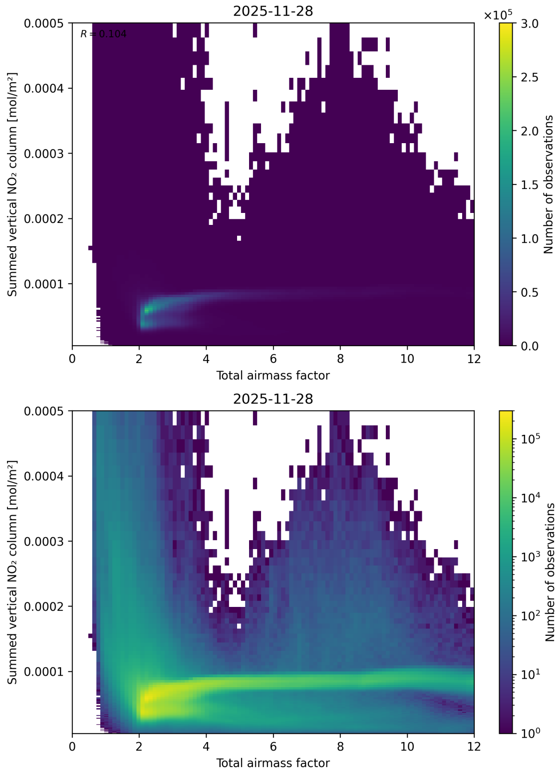
Figure 65: Scatter density plot of “Total airmass factor” against “Summed vertical NO 2 column” for 2025-11-28 to 2025-11-29.
