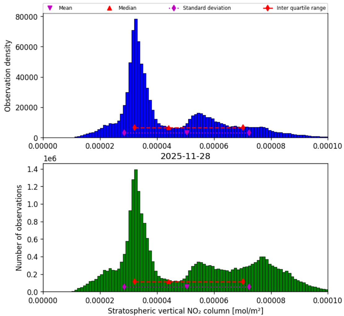
Figure 36: Histogram of “Stratospheric vertical NO 2 column” for 2025-11-28 to 2025-11-29
