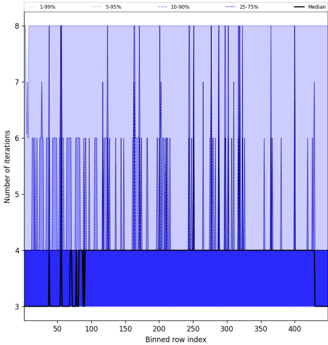
Figure 51: Along track statistics of “Number of iterations” for 2025-11-28 to 2025-11-29
