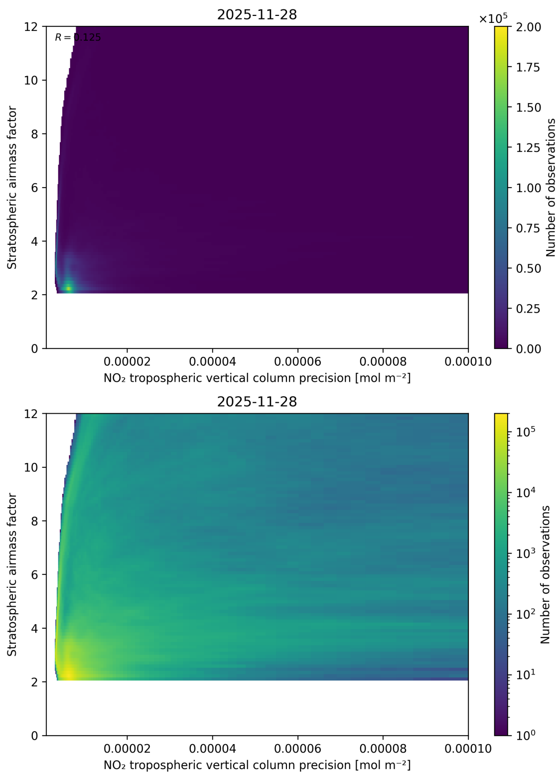
Figure 131: Scatter density plot of “NO 2 tropospheric vertical column precision” against “Stratospheric airmass factor” for 2025-11-28 to 2025-11-29.
