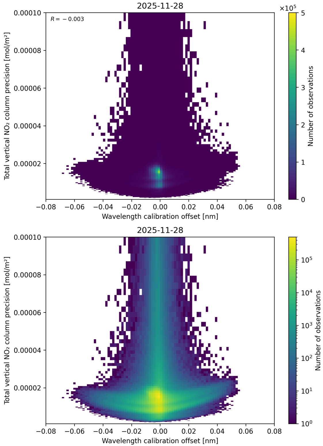
Figure 180: Scatter density plot of “Wavelength calibration offset” against “Total vertical NO 2 column precision” for 2025-11-28 to 2025-11-29.
