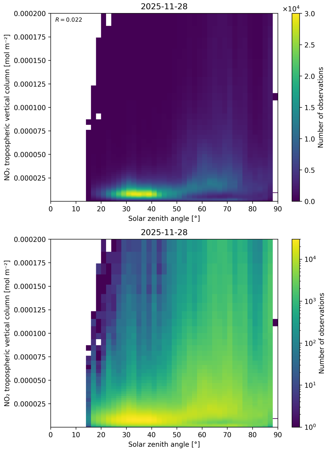
Figure 155: Scatter density plot of “Solar zenith angle” against “NO 2 tropospheric vertical column” for 2025-11-28 to 2025-11-29.
