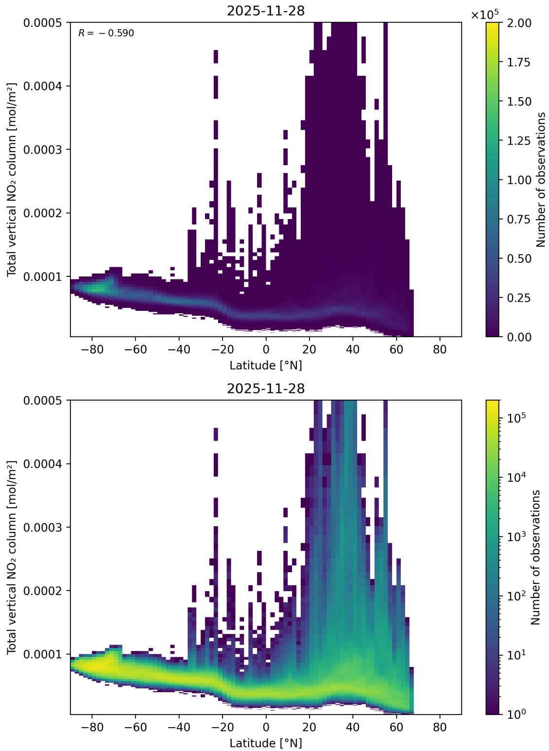
Figure 90: Scatter density plot of “Latitude” against “Total vertical NO 2 column” for 2025-11-28 to 2025-11-29.
