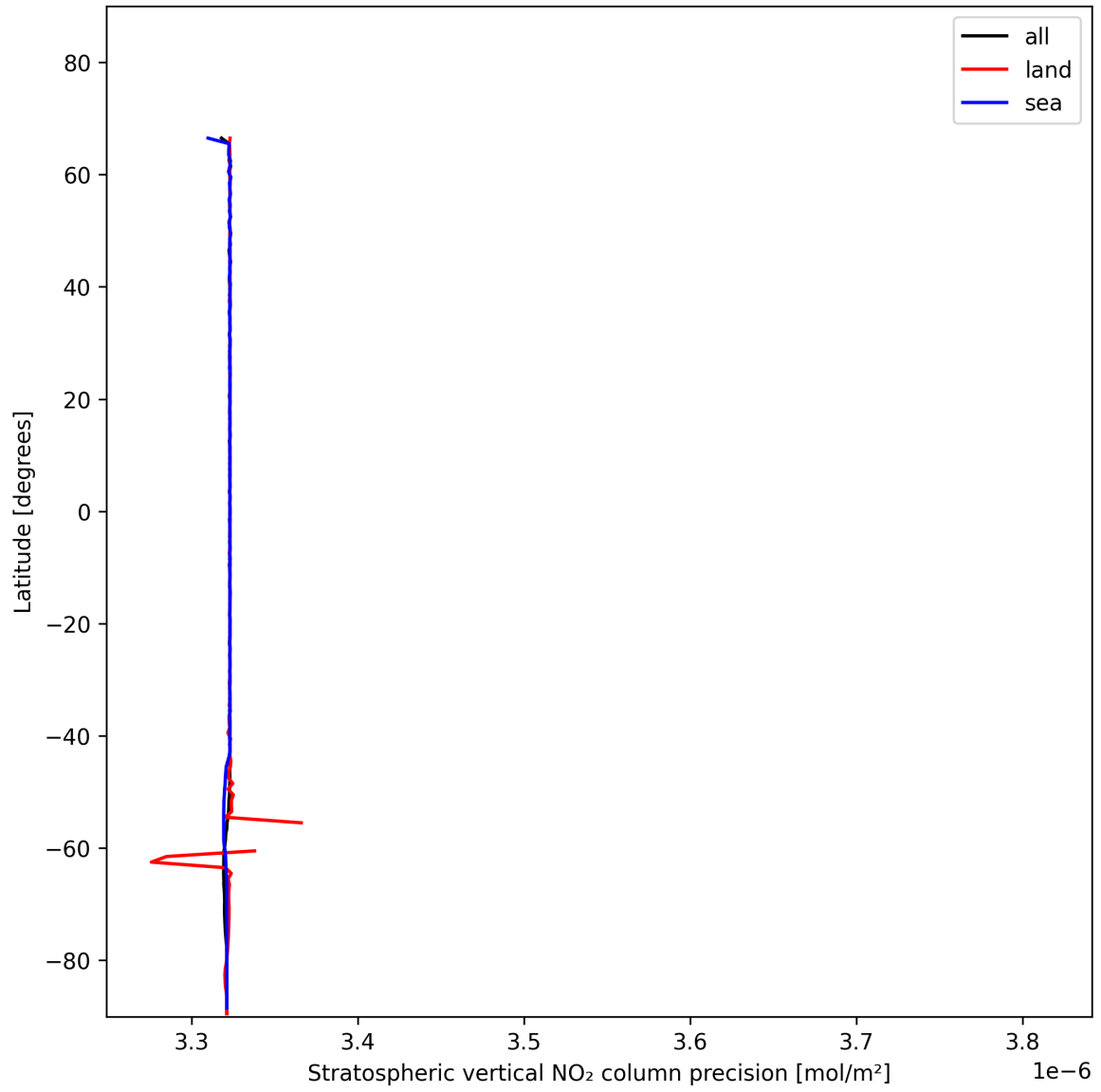
Figure 20: Zonal average of "Stratospheric vertical NO 2 column precision" for 2025-11-28 to 2025-11-29.
