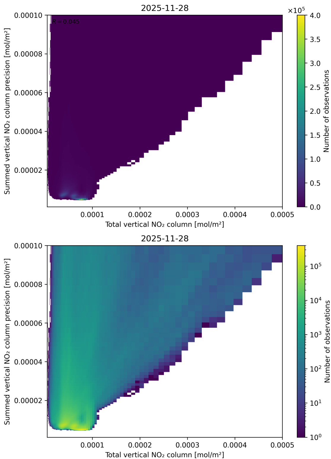
Figure 113: Scatter density plot of “Total vertical NO 2 column” against “Summed vertical NO 2 column precision” for 2025-11-28 to 2025-11-29.
