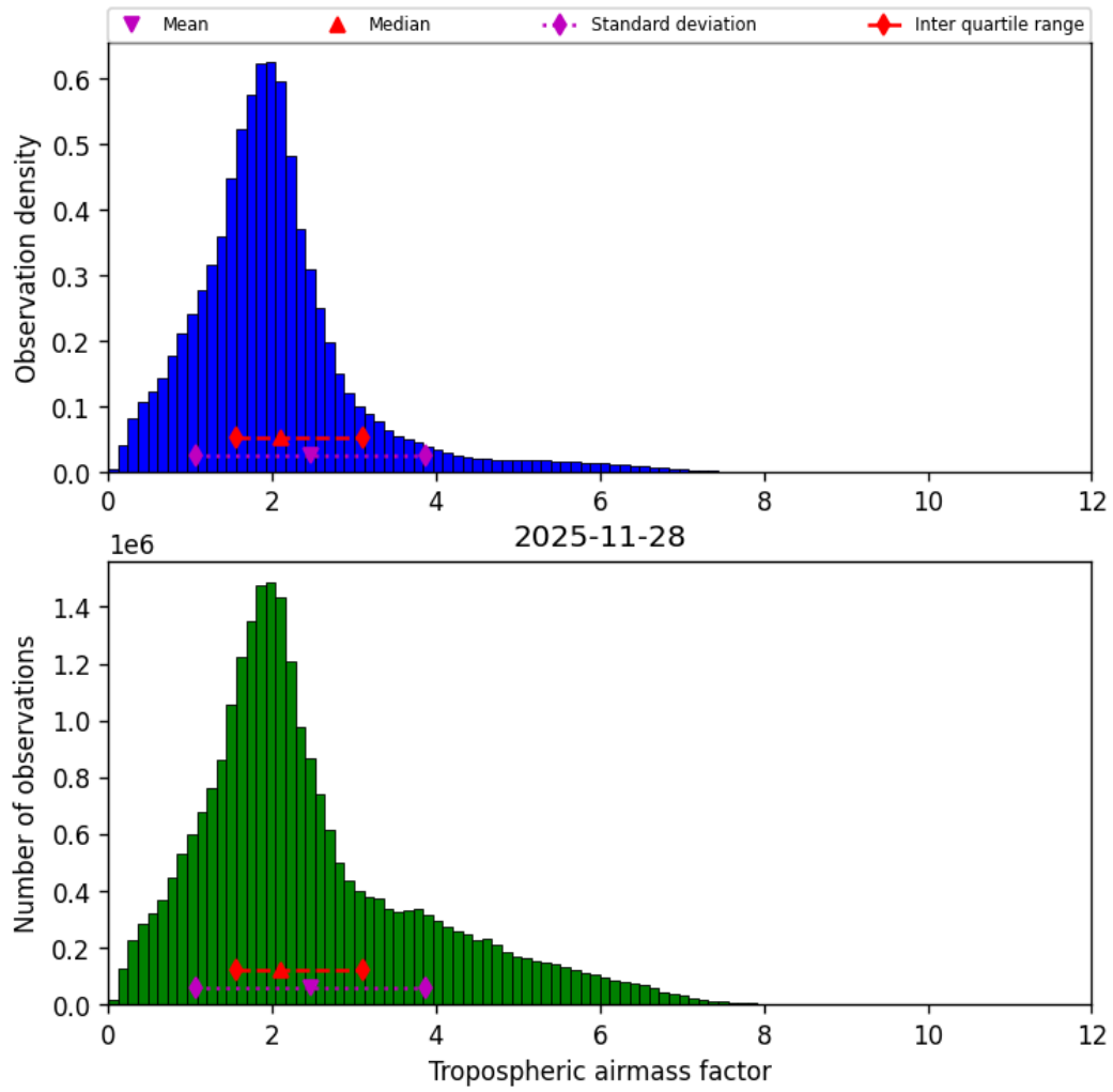
Figure 31: Histogram of “Tropospheric airmass factor” for 2025-11-28 to 2025-11-29
