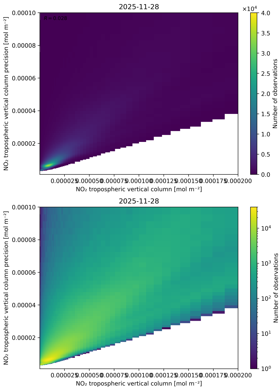
Figure 130: Scatter density plot of “NO 2 tropospheric vertical column” against “NO 2 tropospheric vertical column precision” for 2025-11-28 to 2025-11-29.
