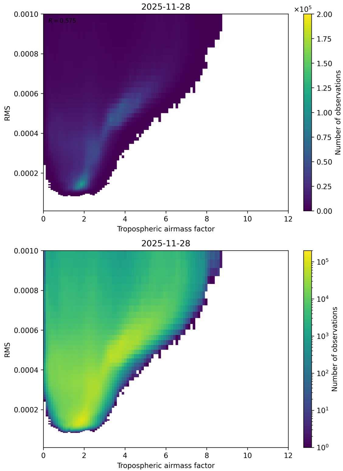
Figure 79: Scatter density plot of “Tropospheric airmass factor” against “RMS” for 2025-11-28 to 2025-11-29.
