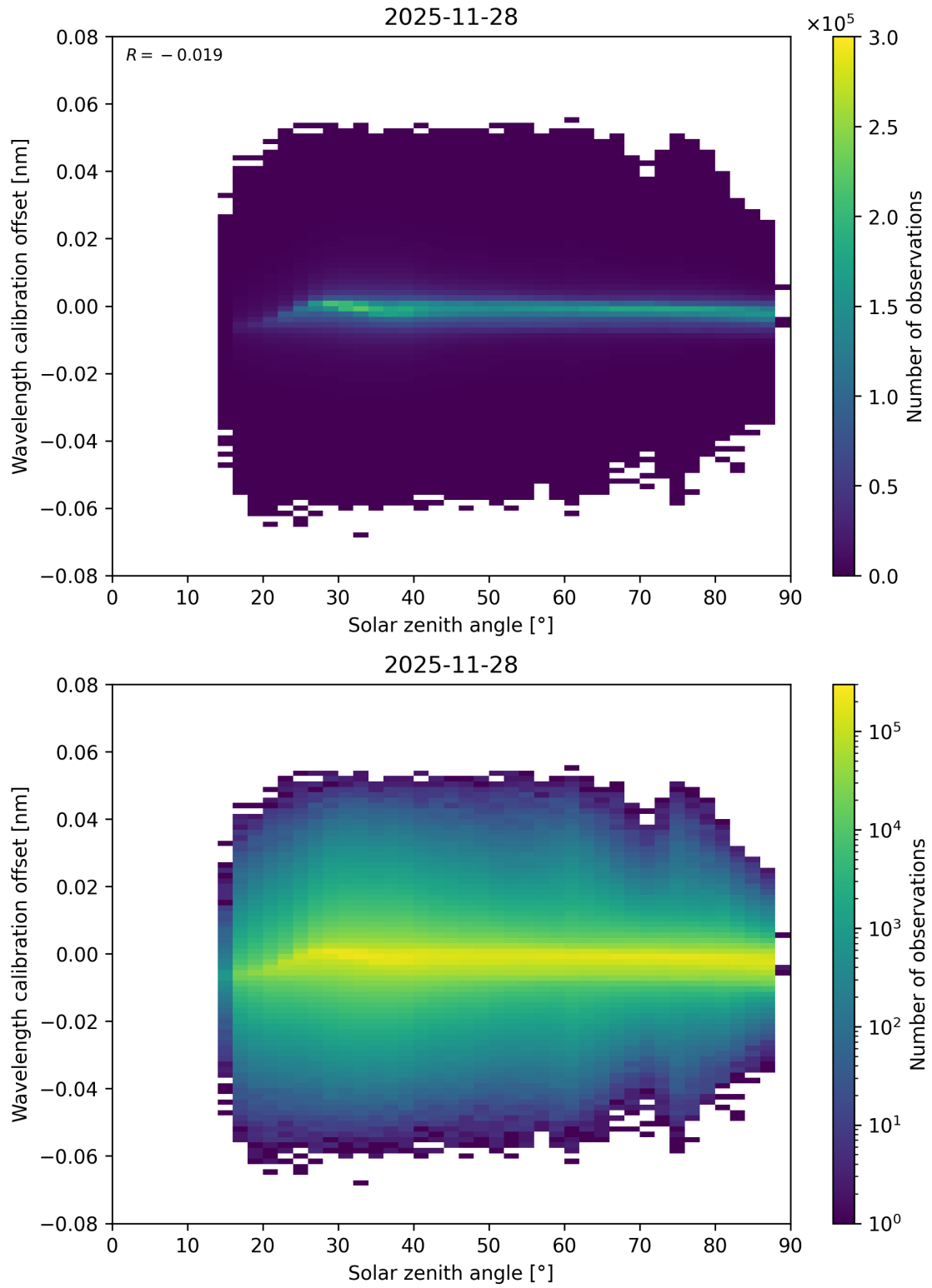
Figure 158: Scatter density plot of “Solar zenith angle” against “Wavelength calibration offset” for 2025-11-28 to 2025-11-29.
