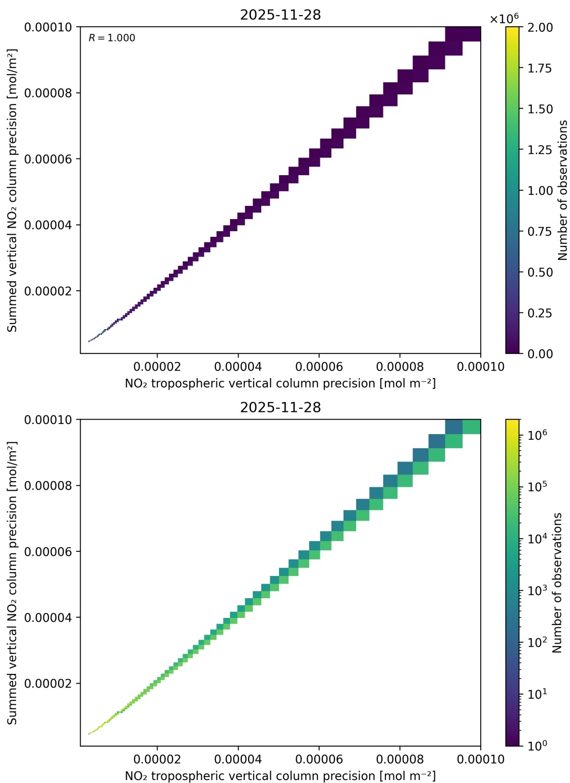
Figure 137: Scatter density plot of “NO 2 tropospheric vertical column precision” against “Summed vertical NO 2 column precision” for 2025-11-28 to 2025-11-29.
