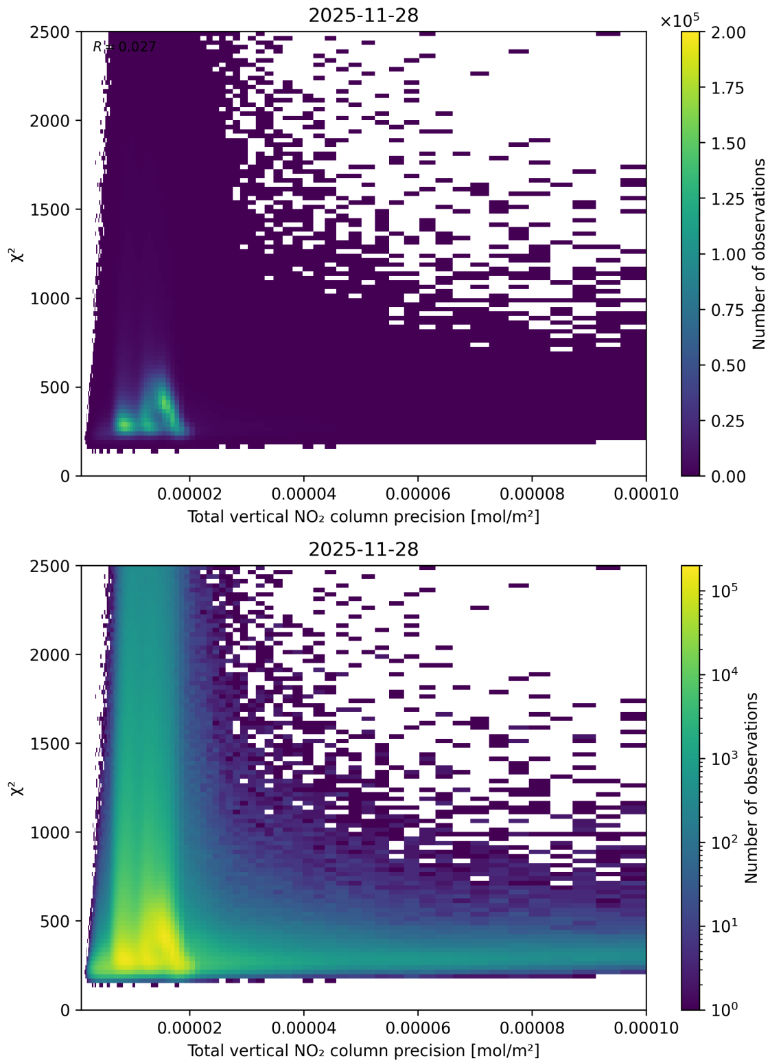
Figure 116: Scatter density plot of “Total vertical NO 2 column precision” against “ \chi^2 ” for 2025-11-28 to 2025-11-29.
