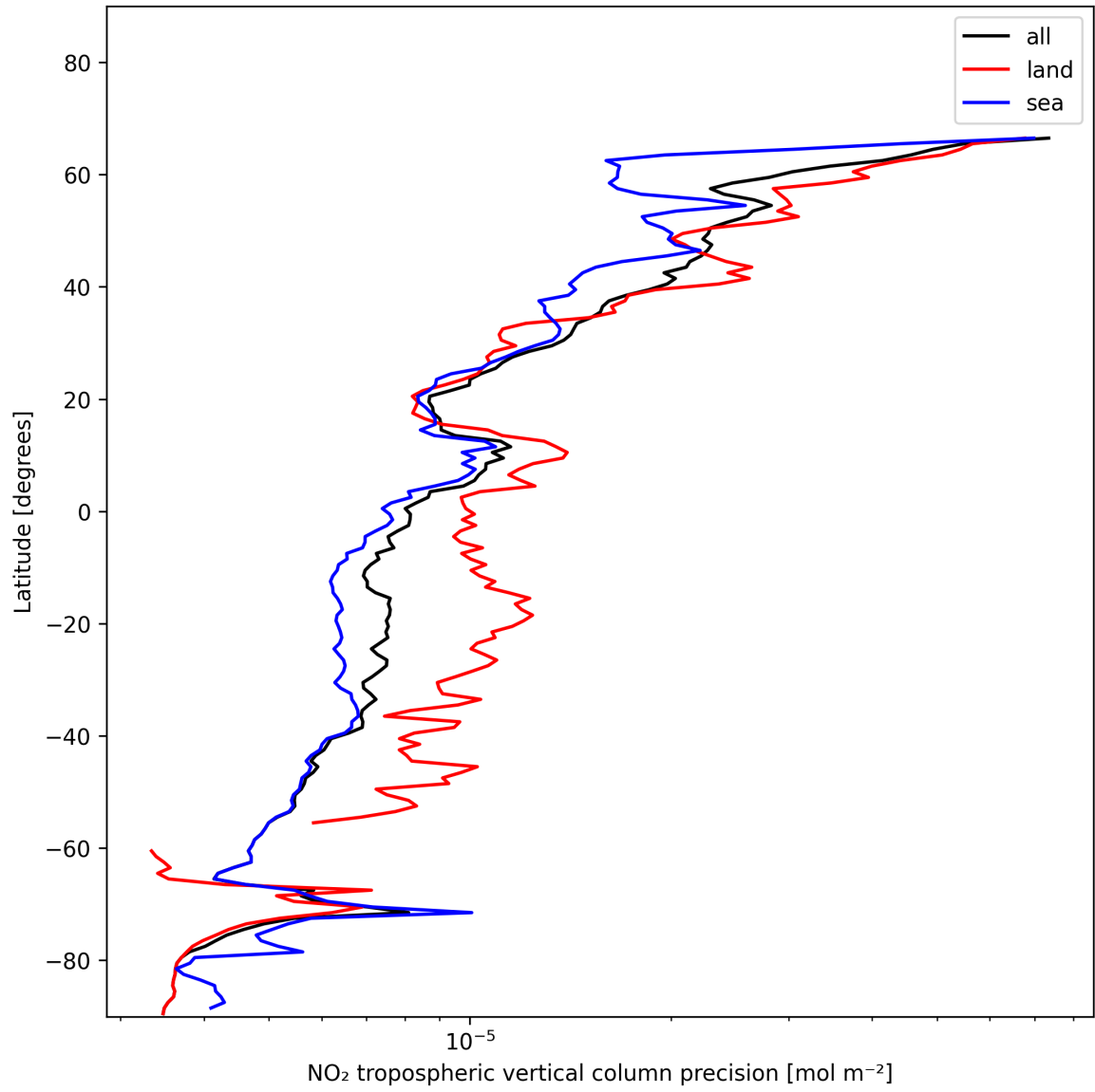
Figure 13: Zonal average of “NO 2 tropospheric vertical column precision” for 2025-11-28 to 2025-11-29.
