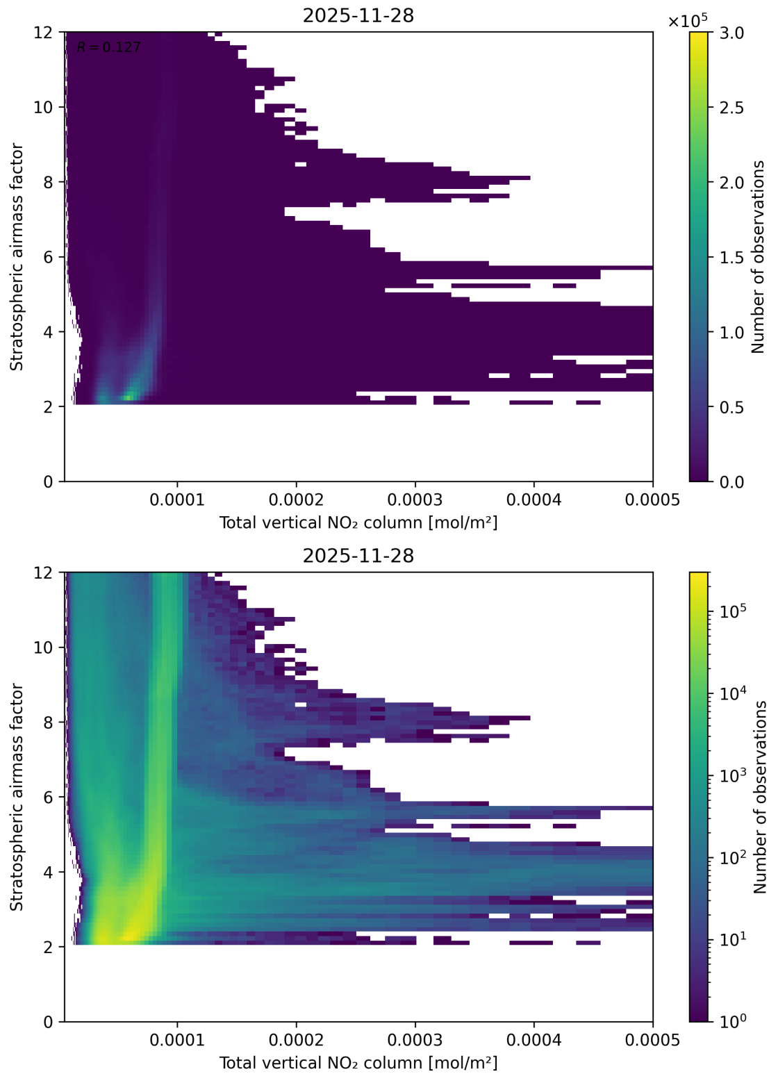
Figure 110: Scatter density plot of “Total vertical NO 2 column” against “Stratospheric airmass factor” for 2025-11-28 to 2025-11-29.
