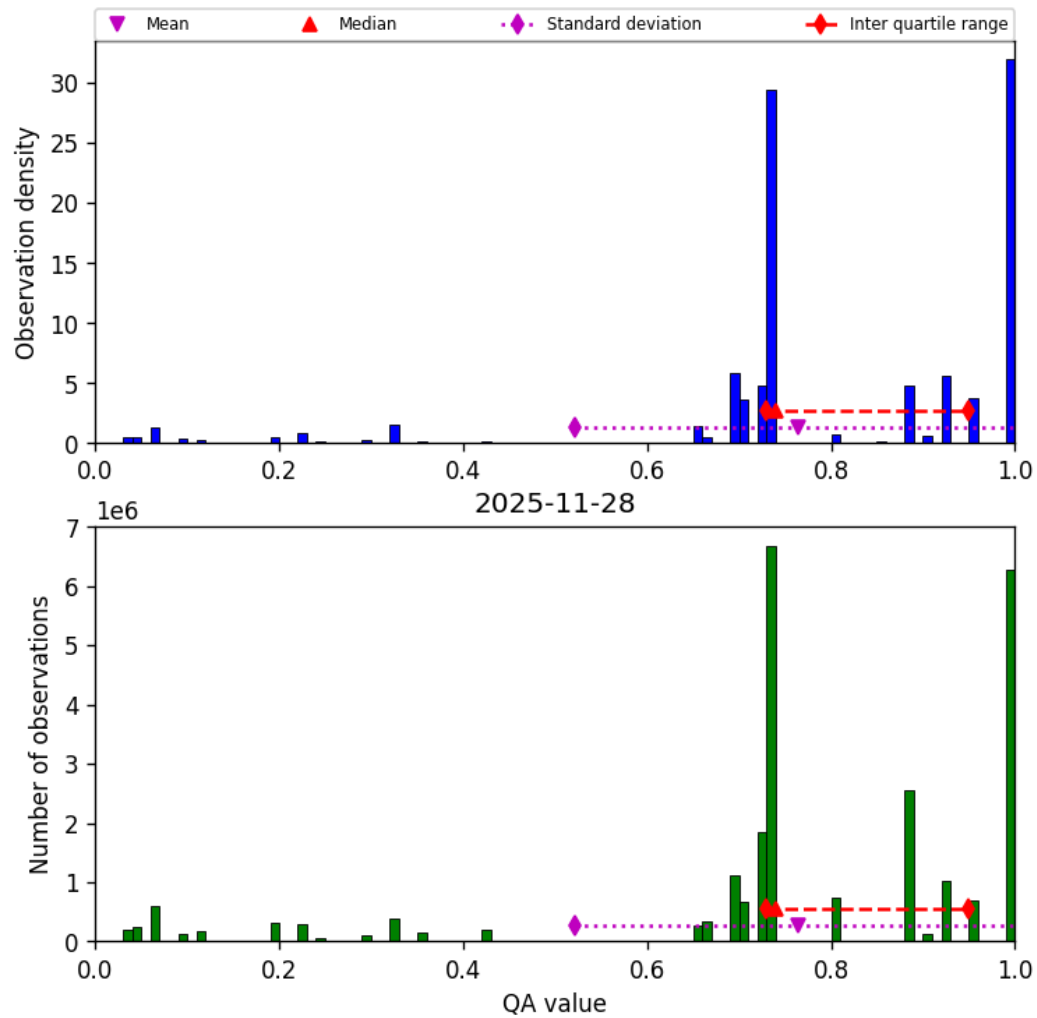
Figure 28: Histogram of “QA value” for 2025-11-28 to 2025-11-29
