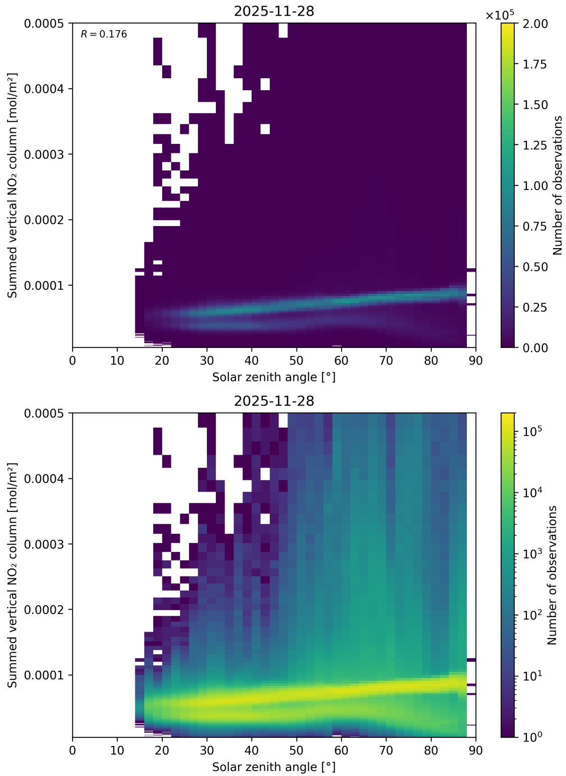
Figure 151: Scatter density plot of “Solar zenith angle” against “Summed vertical NO 2 column” for 2025-11-28 to 2025-11-29.
