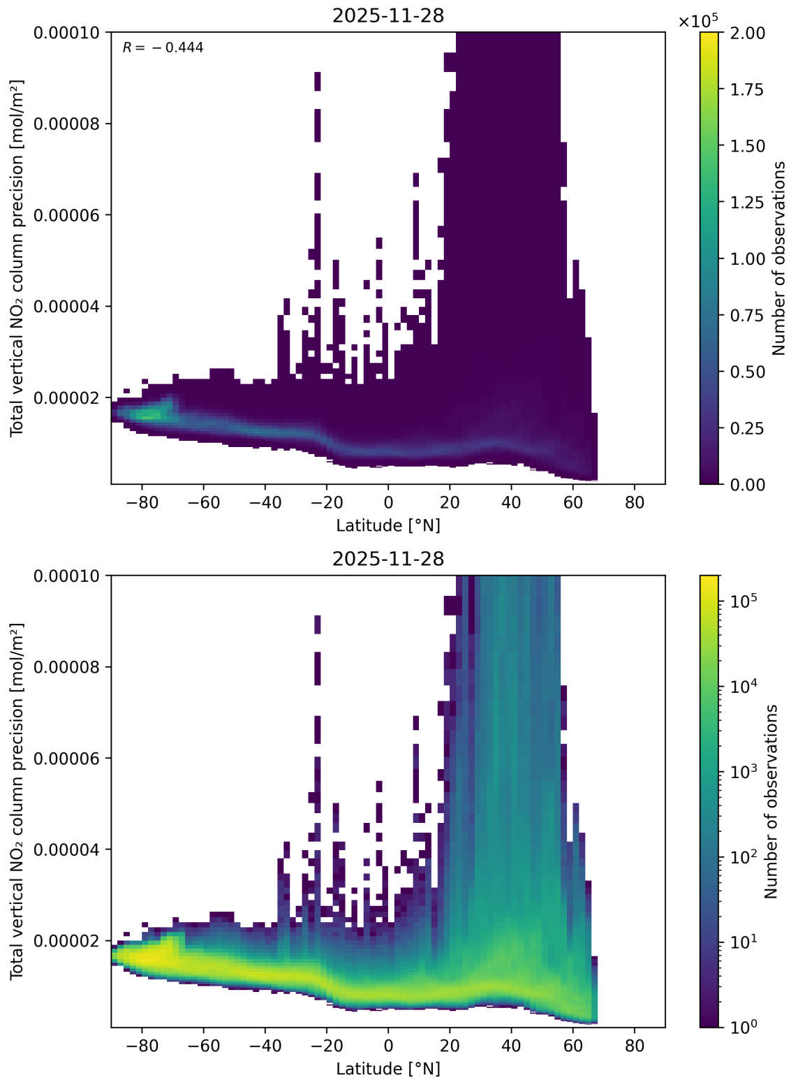
Figure 91: Scatter density plot of “Latitude” against “Total vertical NO 2 column precision” for 2025-11-28 to 2025-11-29.
