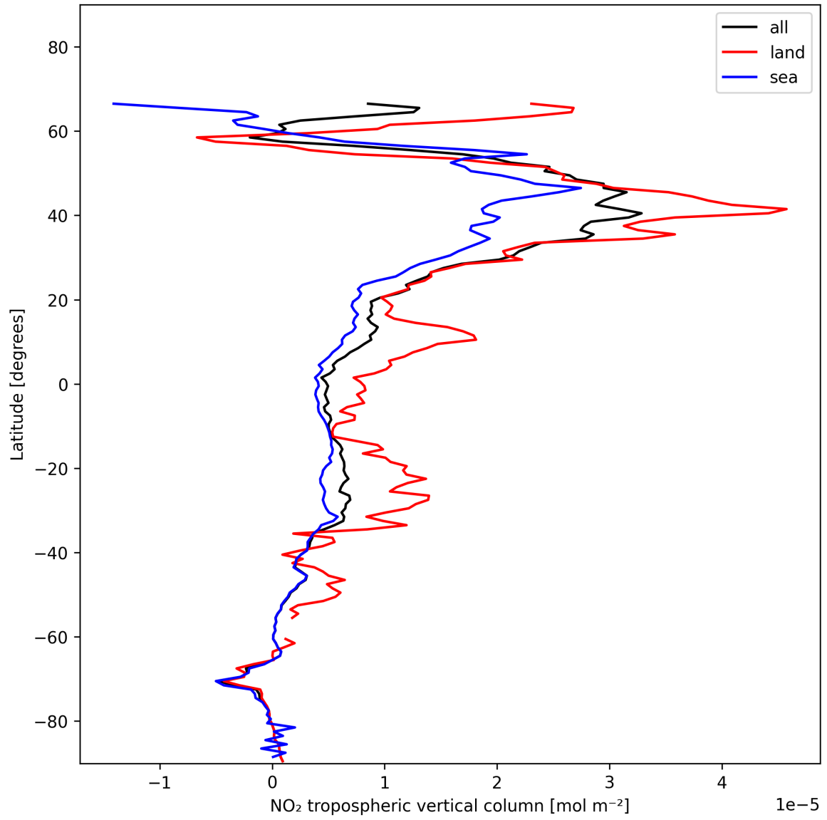
Figure 12: Zonal average of “NO 2 tropospheric vertical column” for 2025-11-28 to 2025-11-29.
