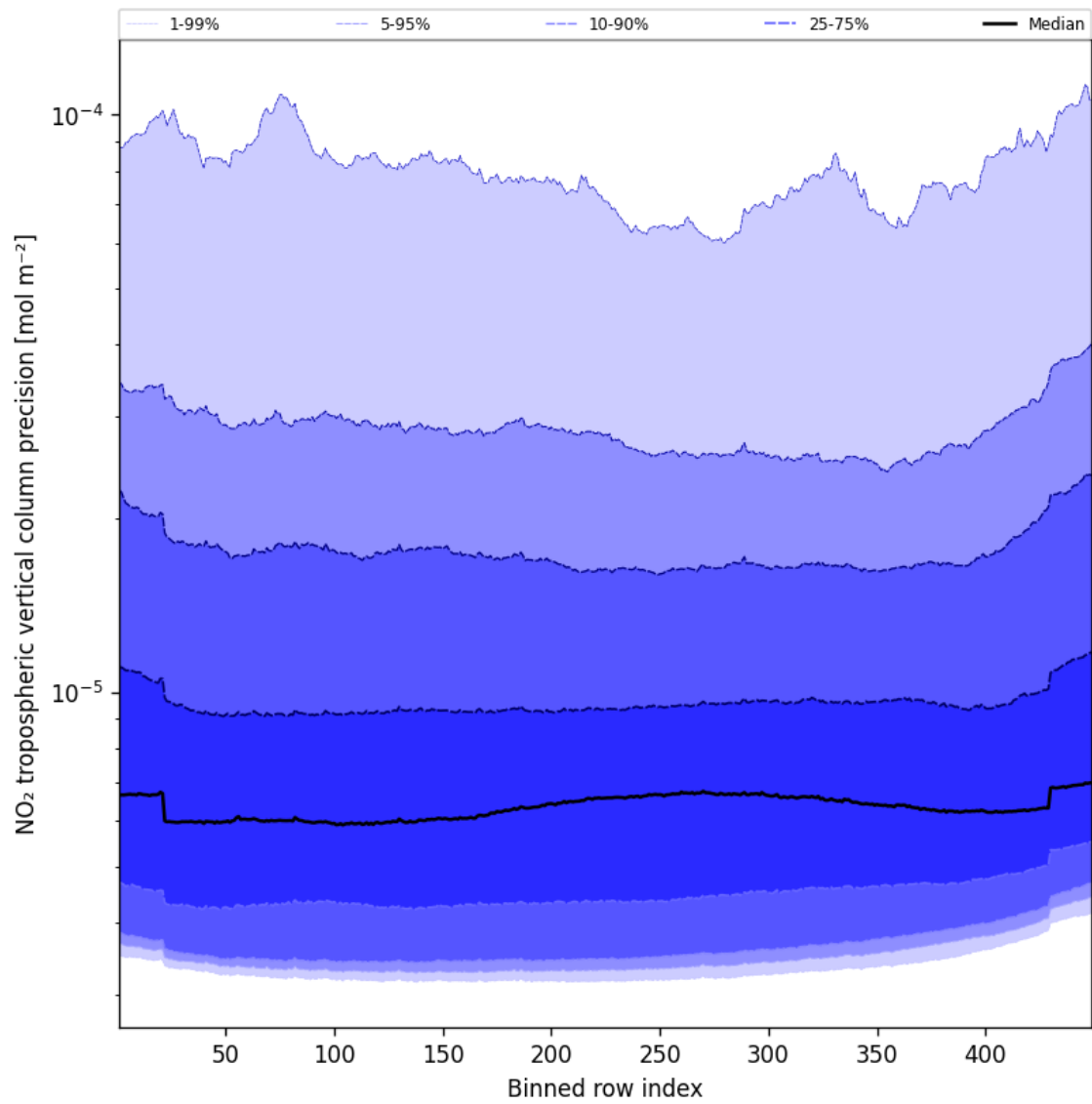
Figure 47: Along track statistics of “NO 2 tropospheric vertical column precision” for 2025-11-28 to 2025-11-29
