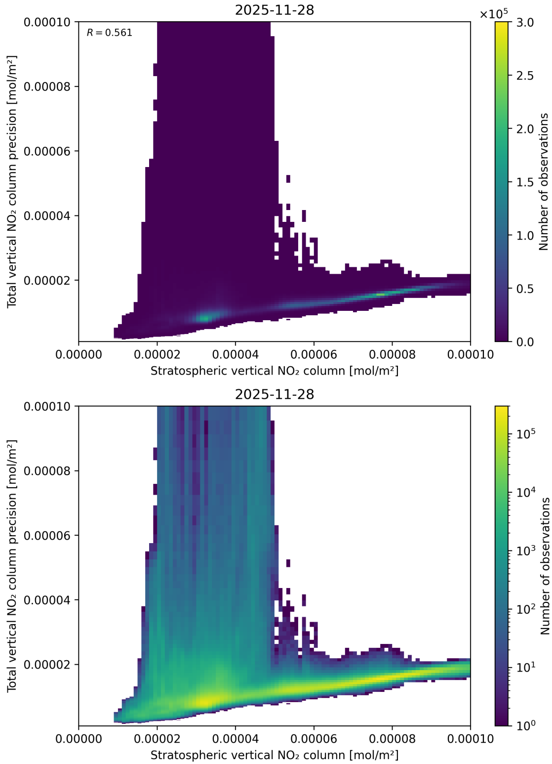
Figure 101: Scatter density plot of “Stratospheric vertical NO 2 column” against “Total vertical NO 2 column precision” for 2025-11-28 to 2025-11-29.
