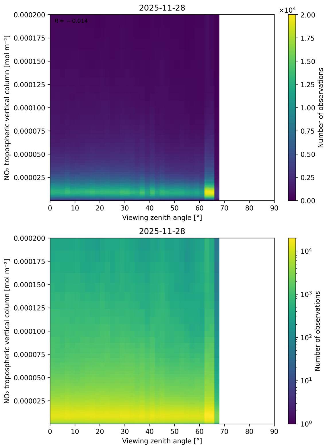
Figure 169: Scatter density plot of “Viewing zenith angle” against “NO 2 tropospheric vertical column” for 2025-11-28 to 2025-11-29.
