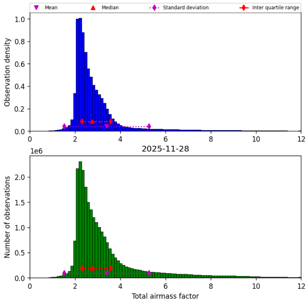
Figure 32: Histogram of “Total airmass factor” for 2025-11-28 to 2025-11-29
