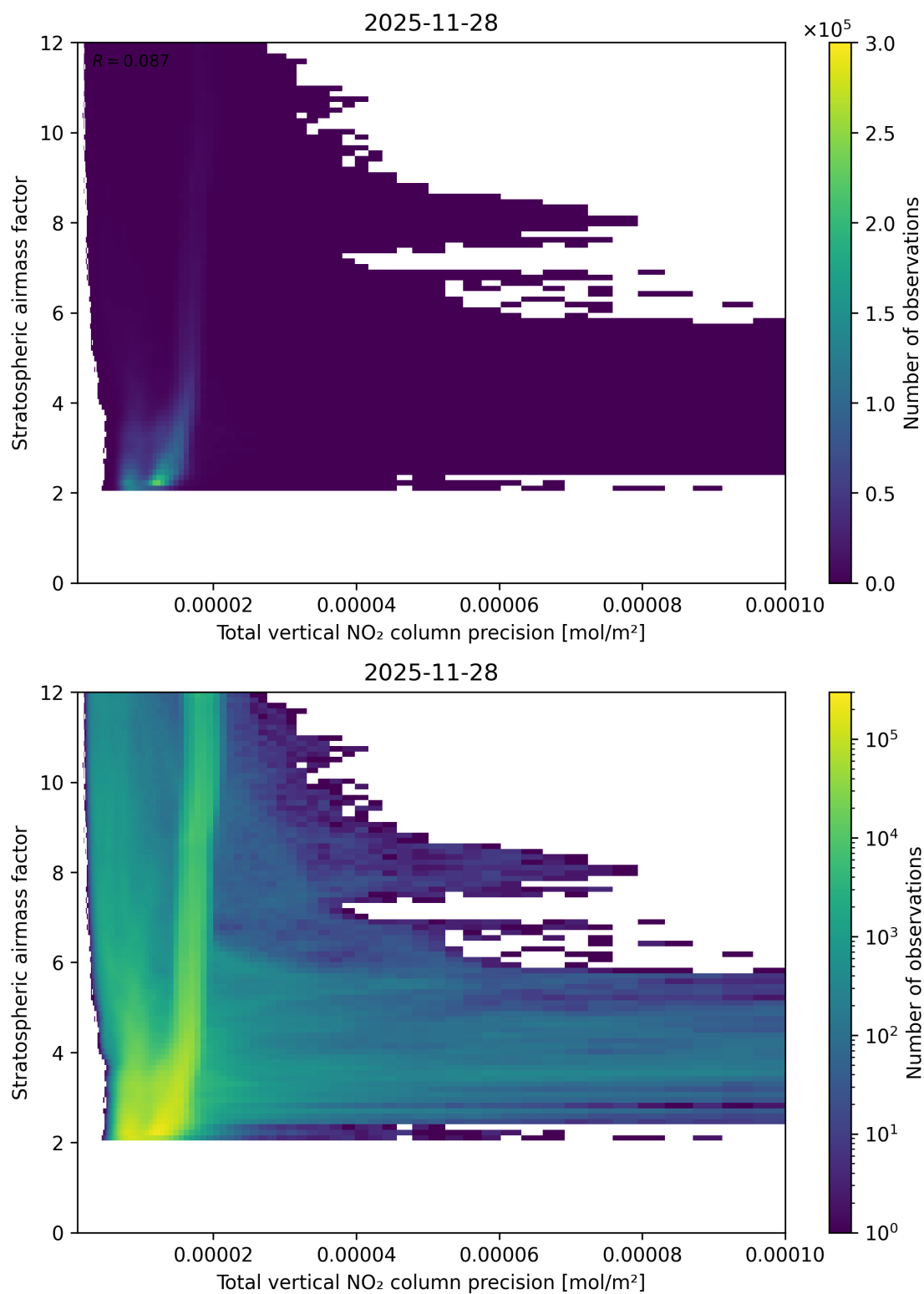
Figure 115: Scatter density plot of “Total vertical NO 2 column precision” against “Stratospheric air mass factor” for 2025-11-28 to 2025-11-29.
