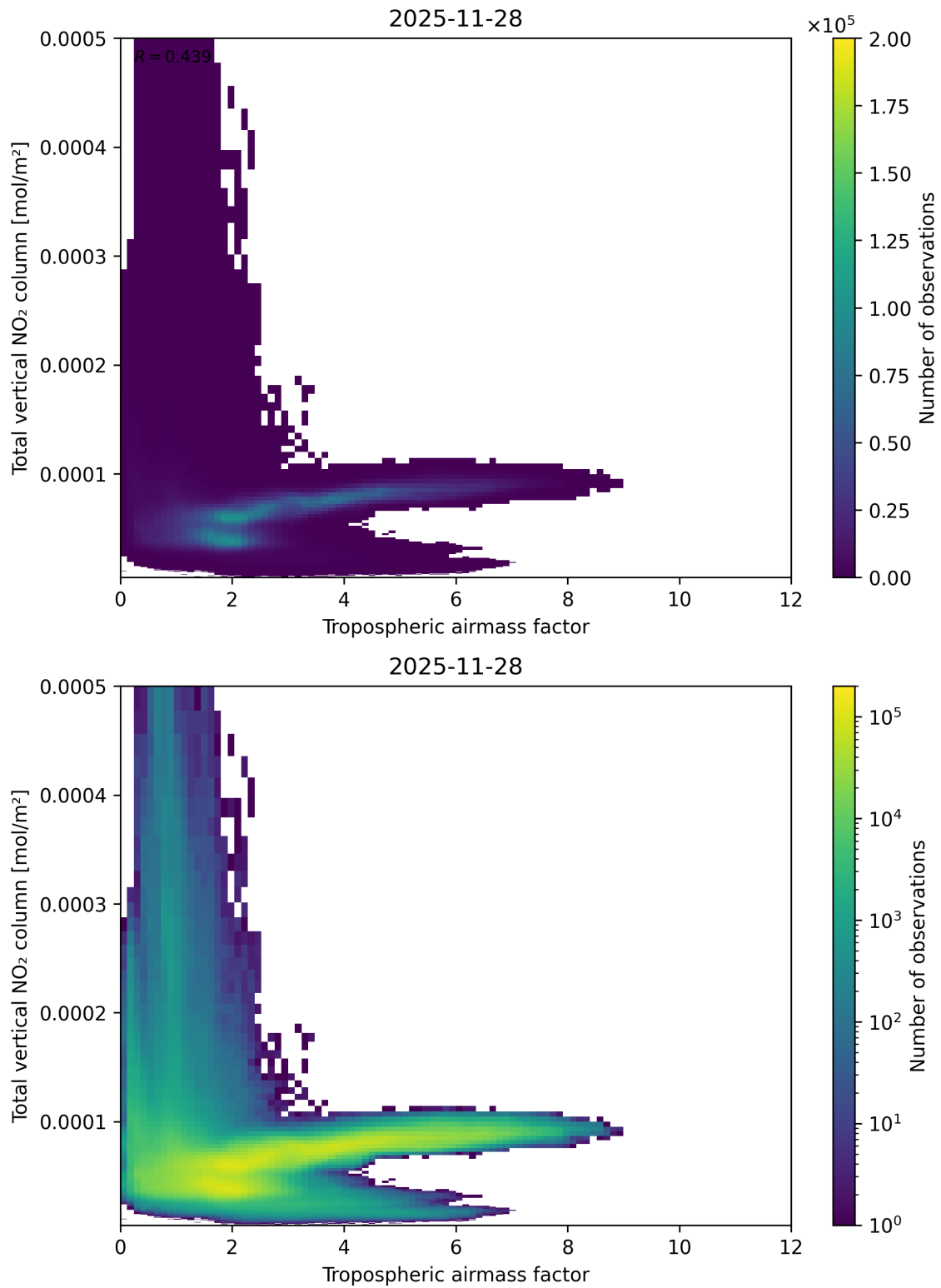
Figure 77: Scatter density plot of “Tropospheric airmass factor” against “Total vertical \text{NO}_2 column” for 2025-11-28 to 2025-11-29.
