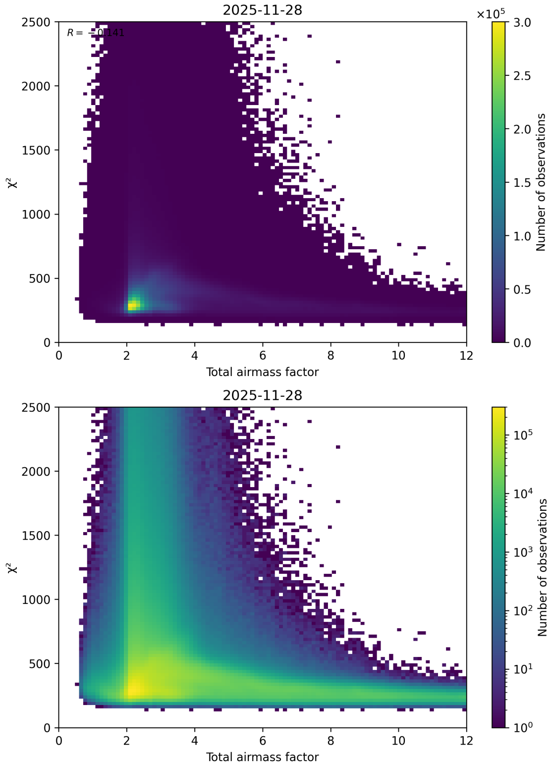
Figure 63: Scatter density plot of “Total airmass factor” against “ \chi^2 ” for 2025-11-28 to 2025-11-29.
