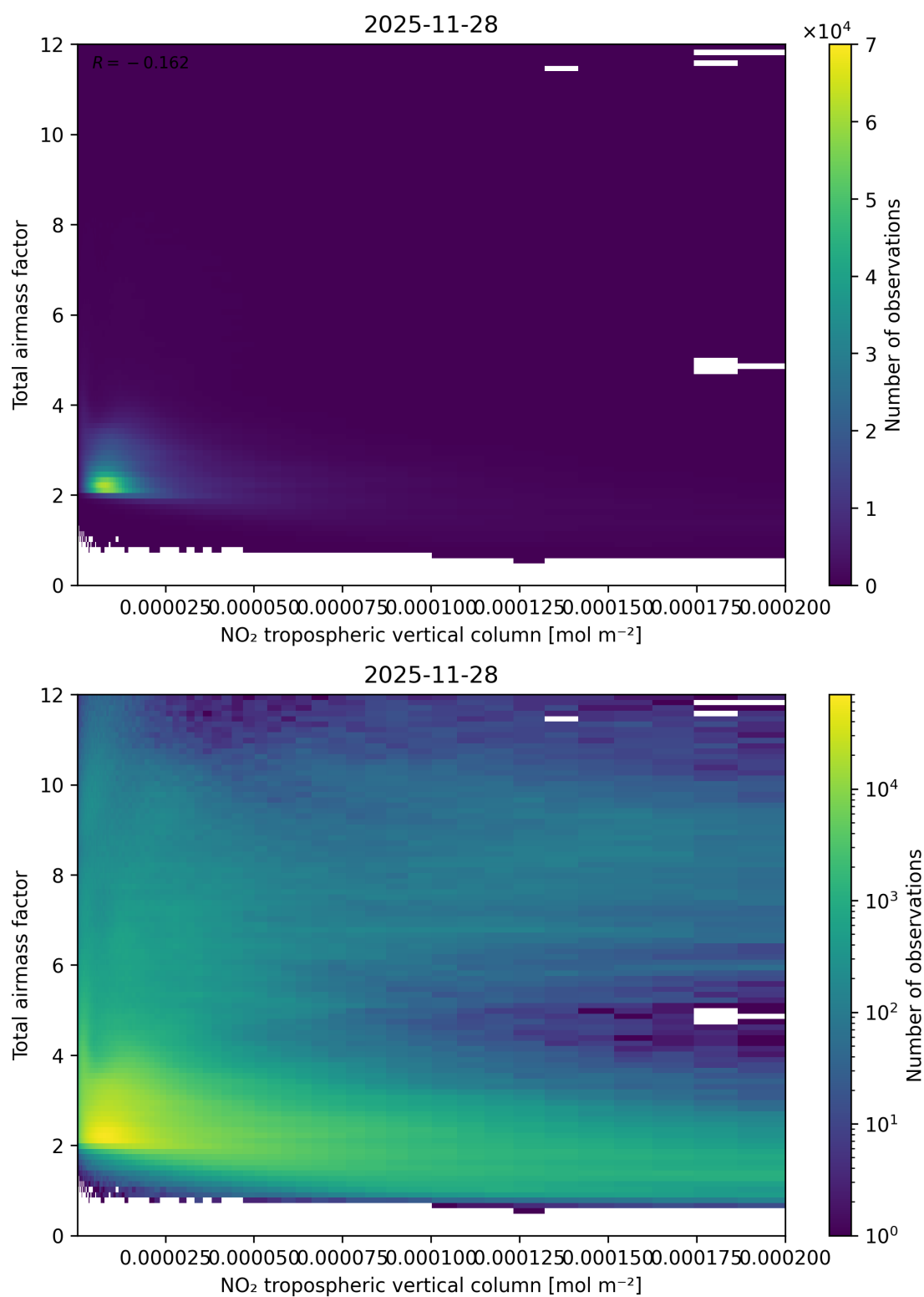
Figure 122: Scatter density plot of “NO 2 tropospheric vertical column” against “Total air mass factor” for 2025-11-28 to 2025-11-29.
