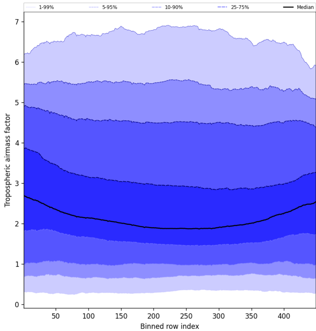
Figure 48: Along track statistics of “Tropospheric airmass factor” for 2025-11-28 to 2025-11-29
