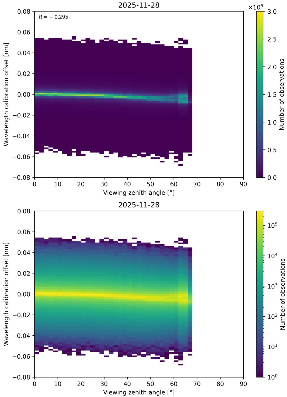
Figure 173: Scatter density plot of “Viewing zenith angle” against “Wavelength calibration offset” for 2025-11-28 to 2025-11-29.
