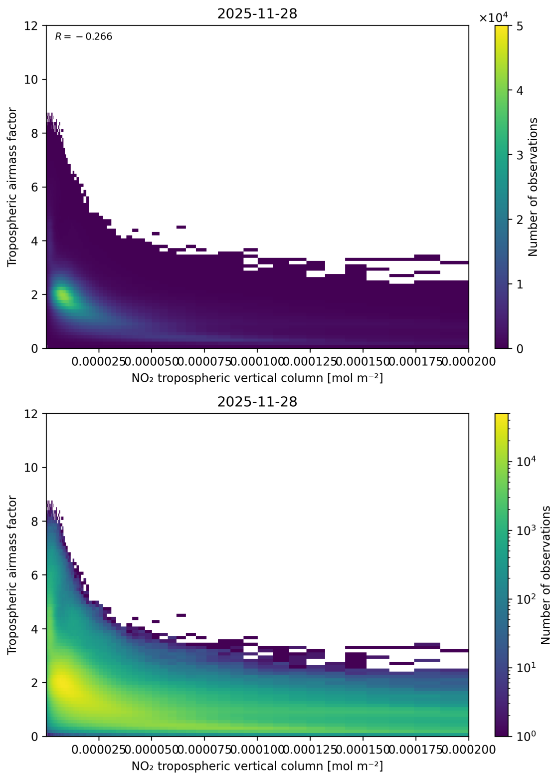
Figure 123: Scatter density plot of “NO 2 tropospheric vertical column” against “Tropospheric air mass factor” for 2025-11-28 to 2025-11-29.
