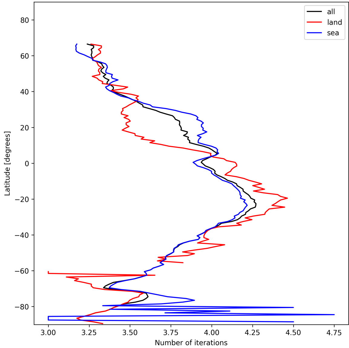
Figure 17: Zonal average of “Number of iterations” for 2025-11-28 to 2025-11-29.
