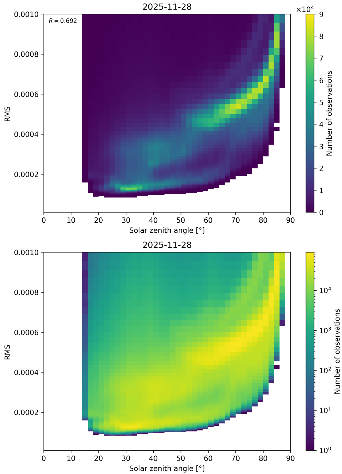
Figure 157: Scatter density plot of “Solar zenith angle” against “RMS” for 2025-11-28 to 2025-11-29.
