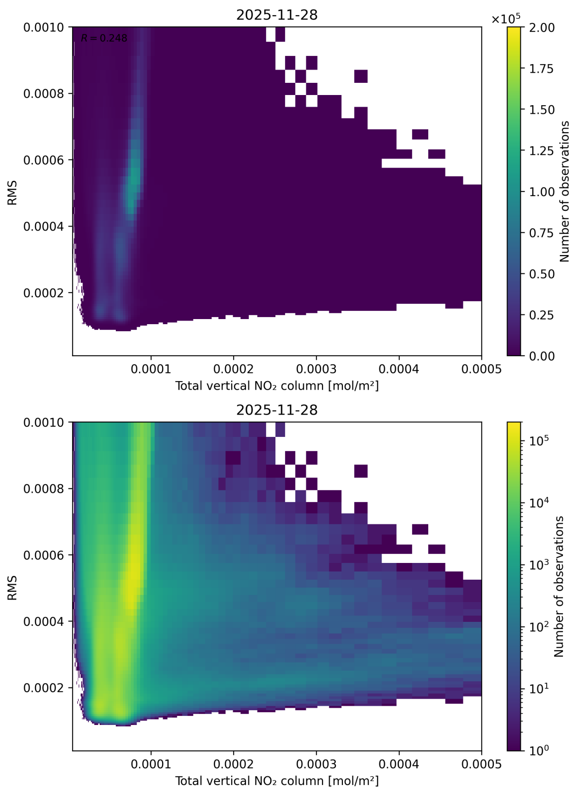
Figure 120: Scatter density plot of “Total vertical NO 2 column” against “RMS” for 2025-11-28 to 2025-11-29.
