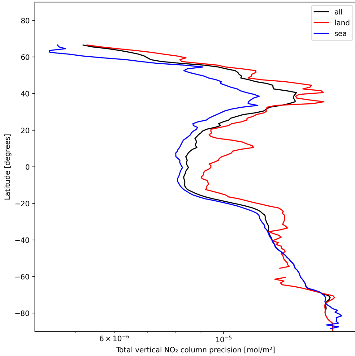
Figure 22: Zonal average of “Total vertical NO 2 column precision” for 2025-11-28 to 2025-11-29.
