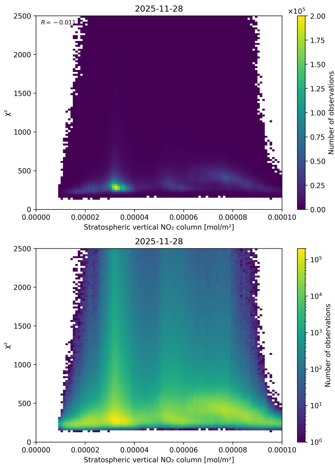
Figure 97: Scatter density plot of “Stratospheric vertical NO 2 column” against “ \chi^2 ” for 2025-11-28 to 2025-11-29.
