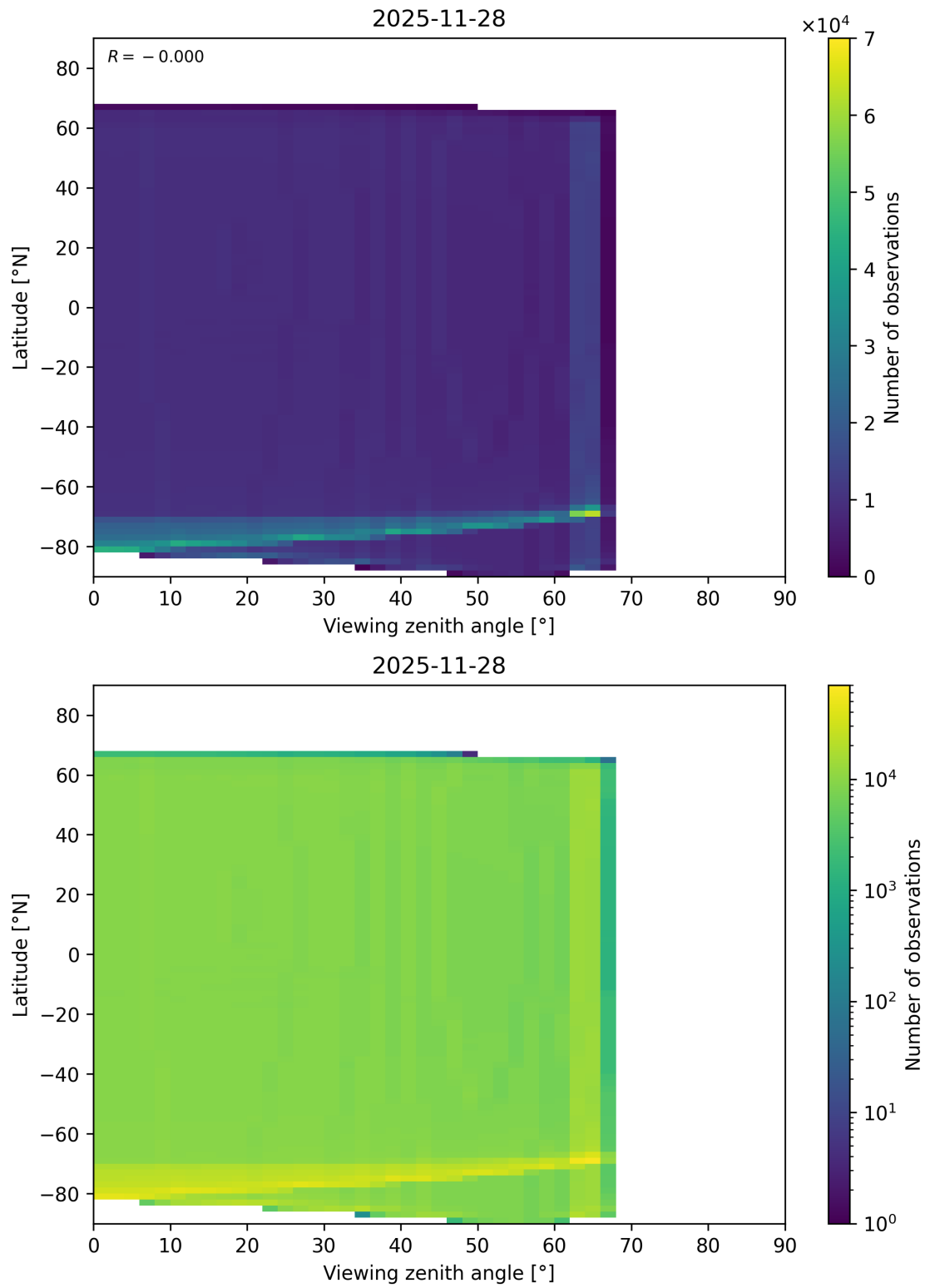
Figure 163: Scatter density plot of “Viewing zenith angle” against “Latitude” for 2025-11-28 to 2025-11-29.
