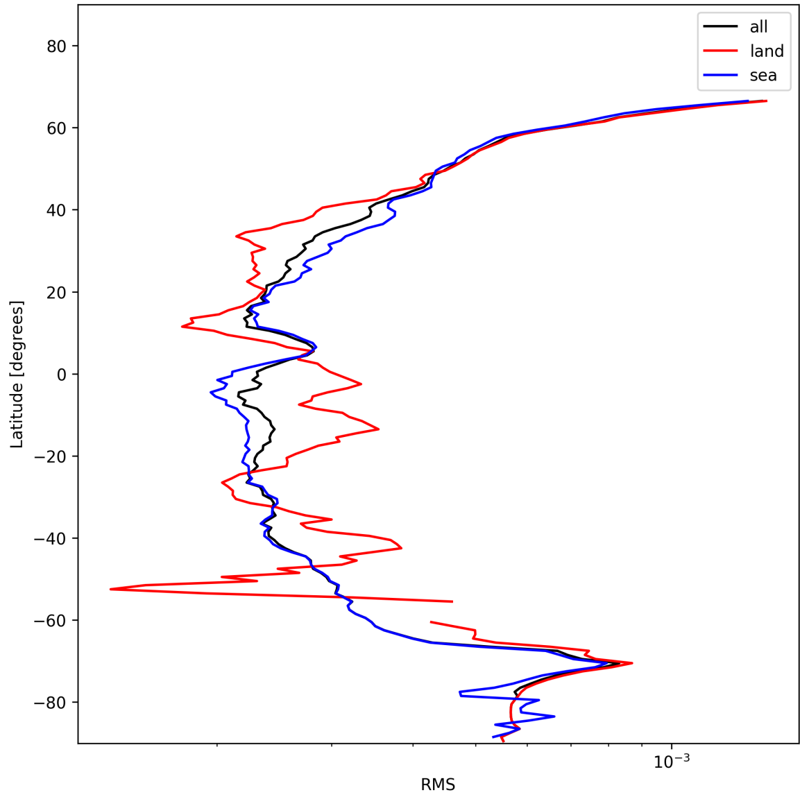
Figure 26: Zonal average of “RMS” for 2025-11-28 to 2025-11-29.
