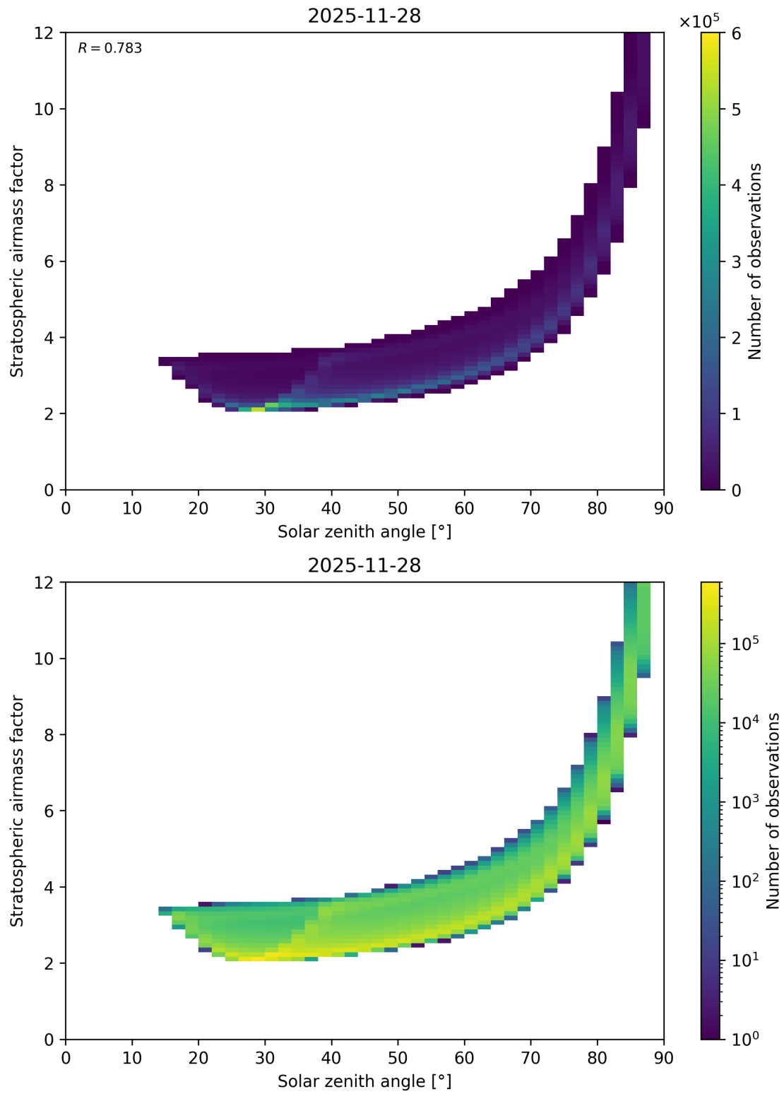
Figure 145: Scatter density plot of “Solar zenith angle” against “Stratospheric airmass factor” for 2025-11-28 to 2025-11-29.
