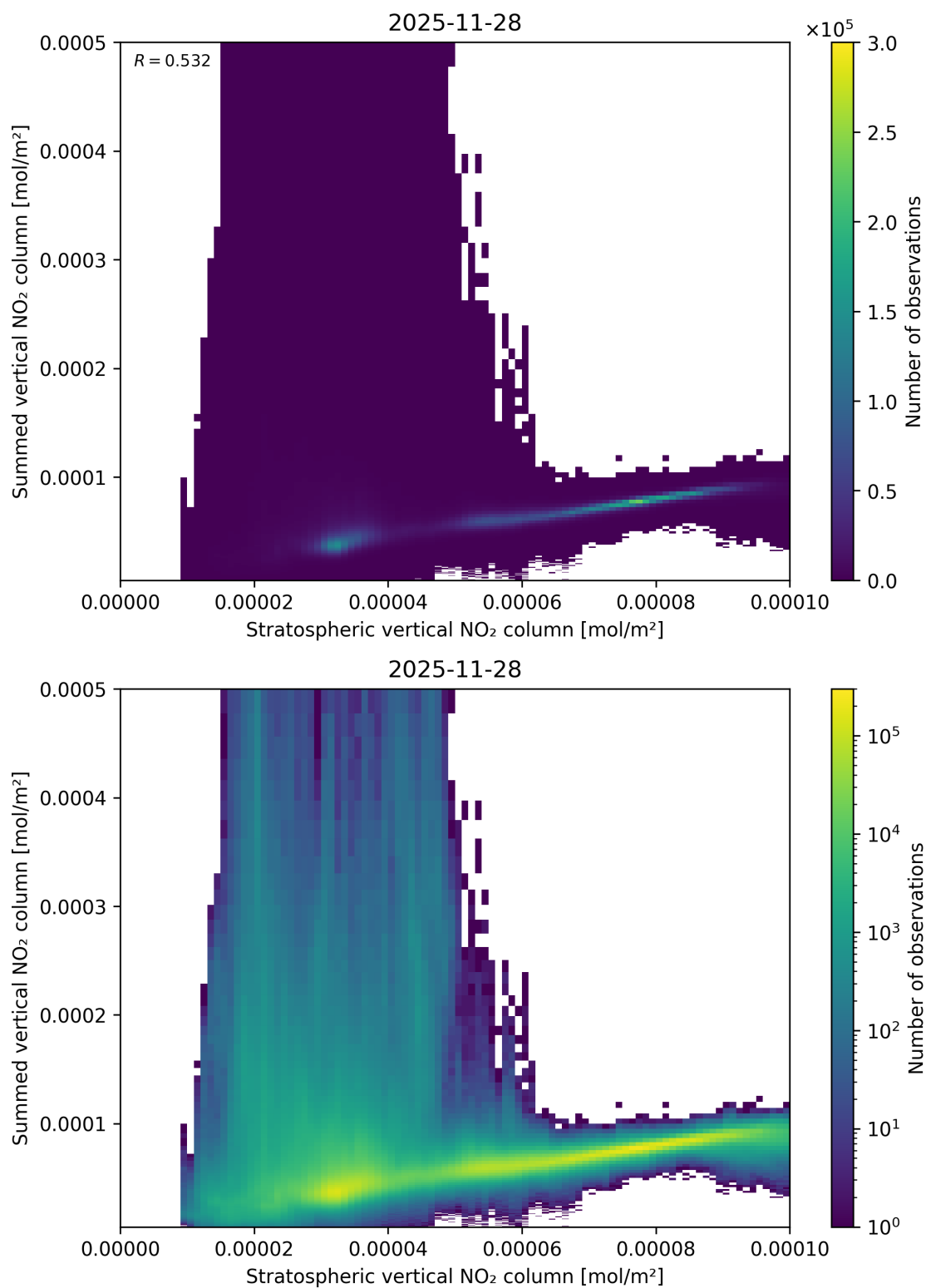
Figure 98: Scatter density plot of “Stratospheric vertical NO 2 column” against “Summed vertical NO 2 column” for 2025-11-28 to 2025-11-29.
