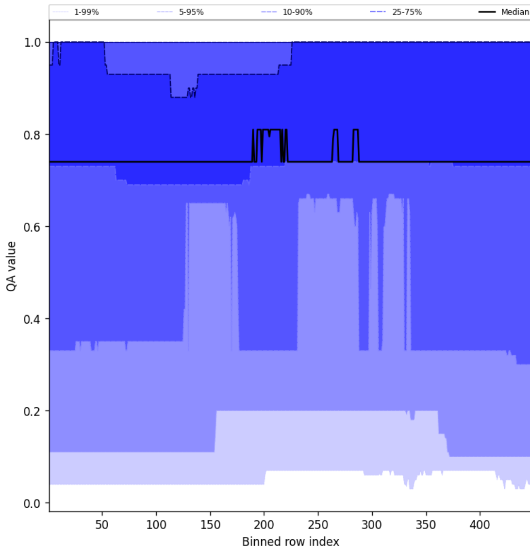
Figure 45: Along track statistics of “QA value” for 2025-11-28 to 2025-11-29
