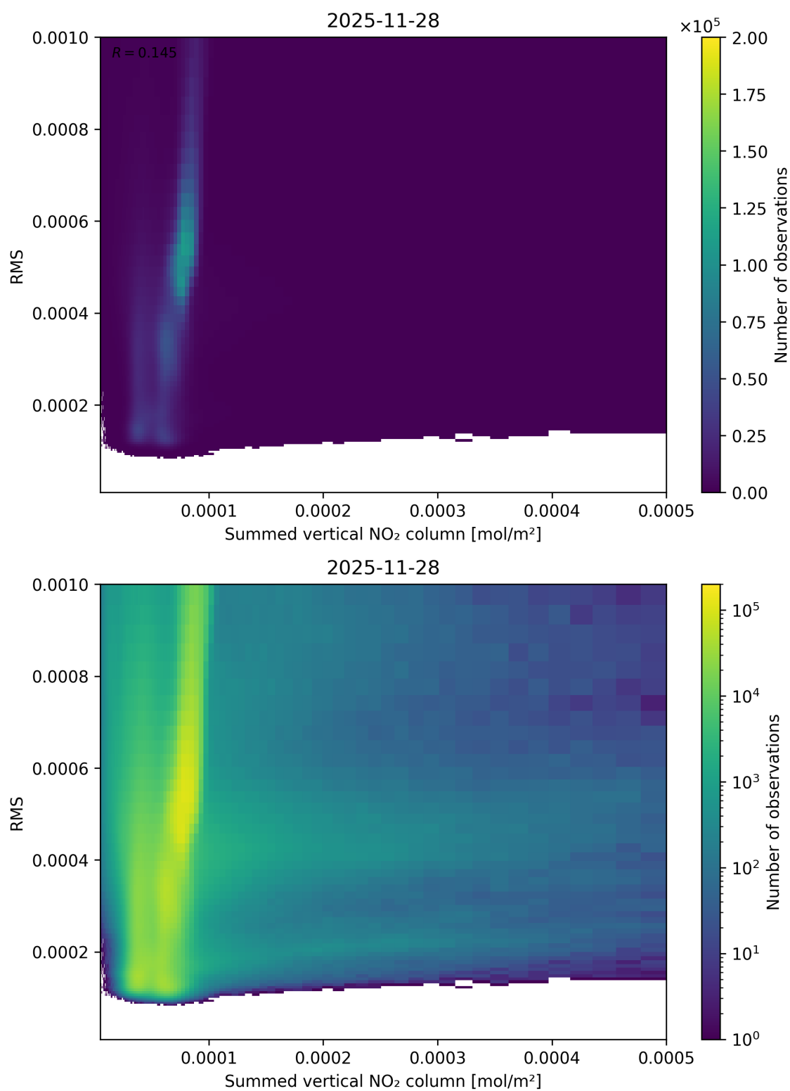
Figure 109: Scatter density plot of “Summed vertical NO 2 column” against “RMS” for 2025-11-28 to 2025-11-29.
