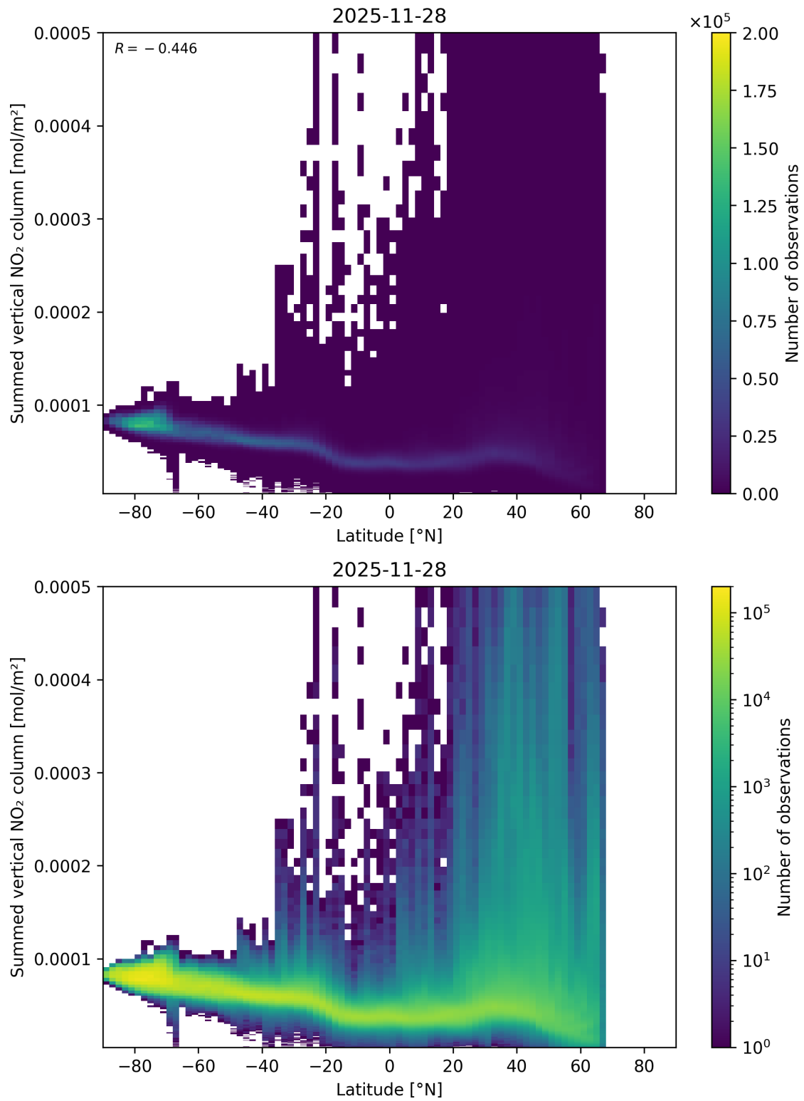
Figure 88: Scatter density plot of “Latitude” against “Summed vertical NO 2 column” for 2025-11-28 to 2025-11-29.
