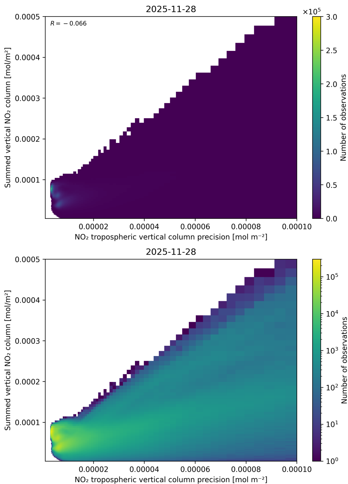
Figure 136: Scatter density plot of “NO 2 tropospheric vertical column precision” against “Summed vertical NO 2 column” for 2025-11-28 to 2025-11-29.
