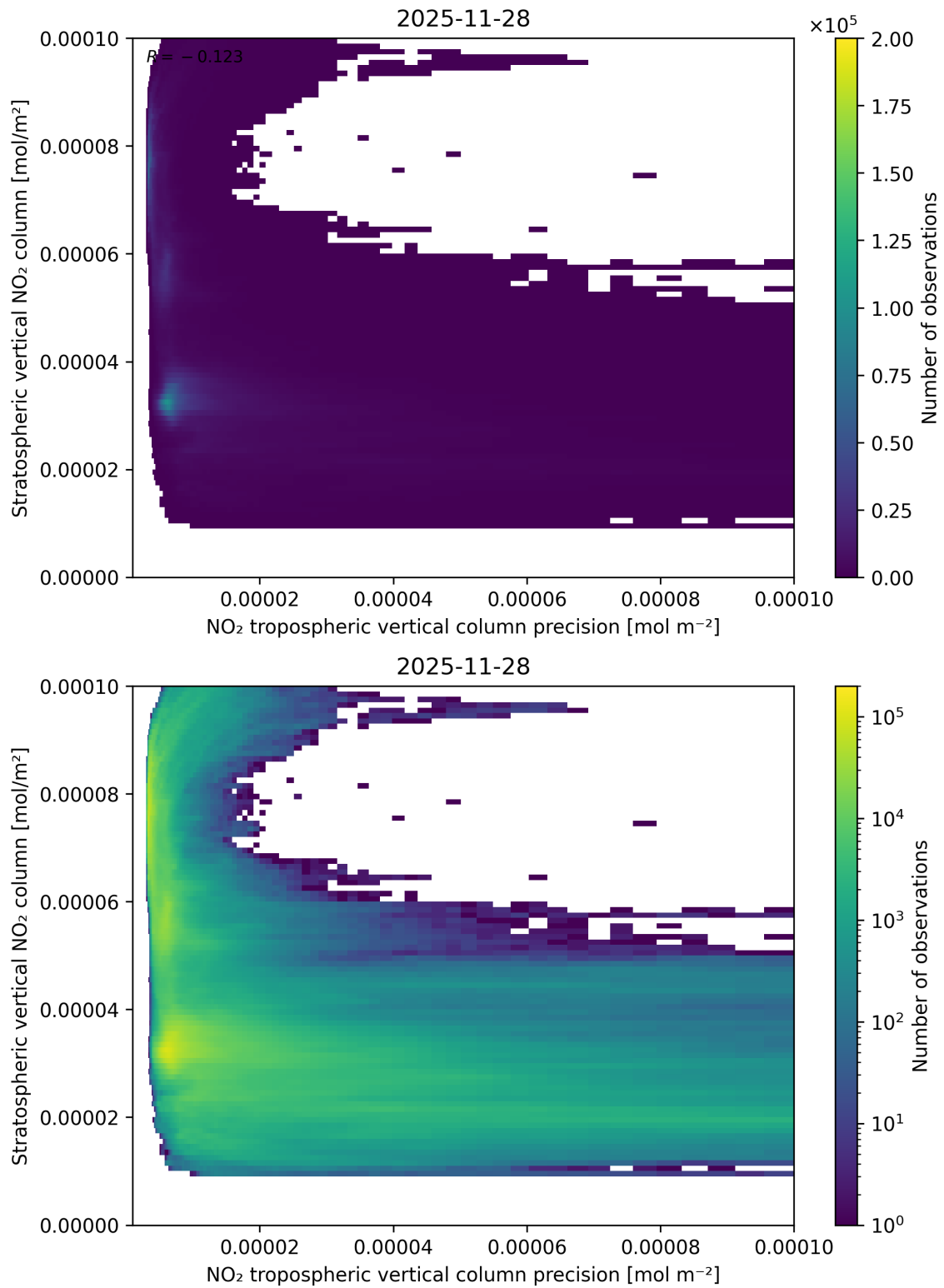
Figure 135: Scatter density plot of “NO 2 tropospheric vertical column precision” against “Stratospheric vertical NO 2 column” for 2025-11-28 to 2025-11-29.
