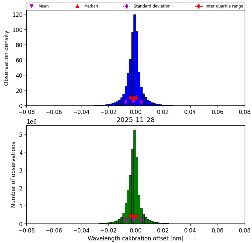
Figure 35: Histogram of “Wavelength calibration offset” for 2025-11-28 to 2025-11-29
