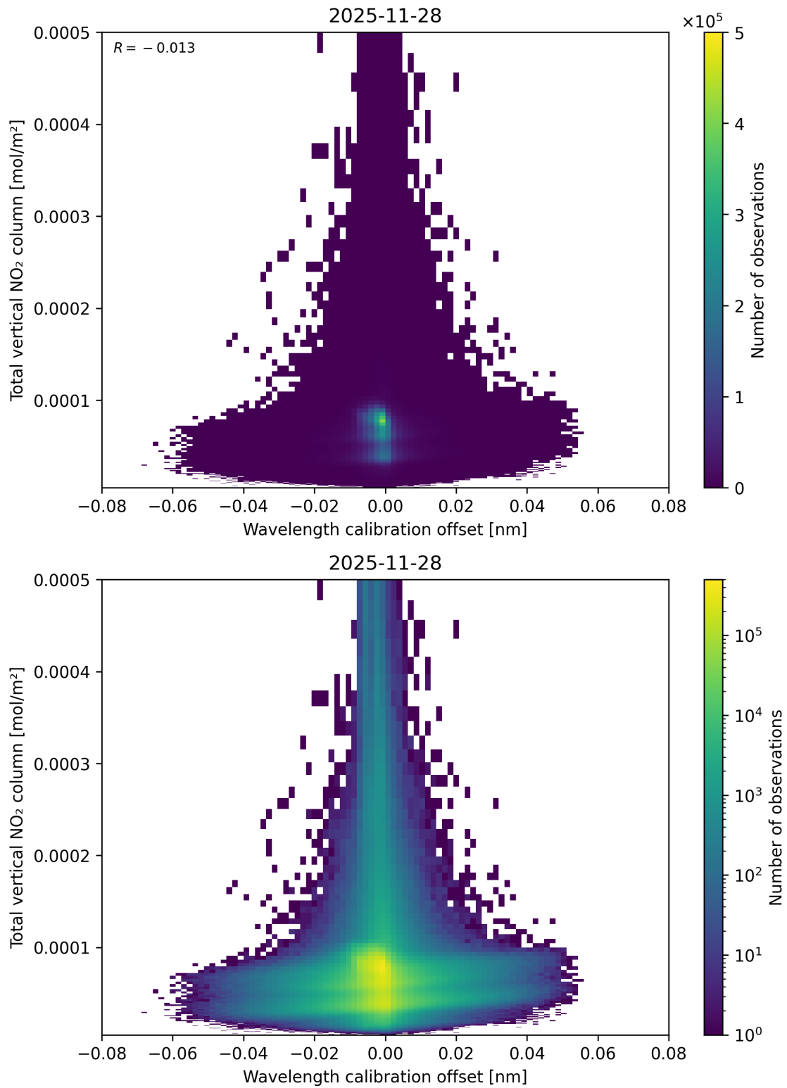
Figure 179: Scatter density plot of “Wavelength calibration offset” against “Total vertical NO 2 column” for 2025-11-28 to 2025-11-29.
