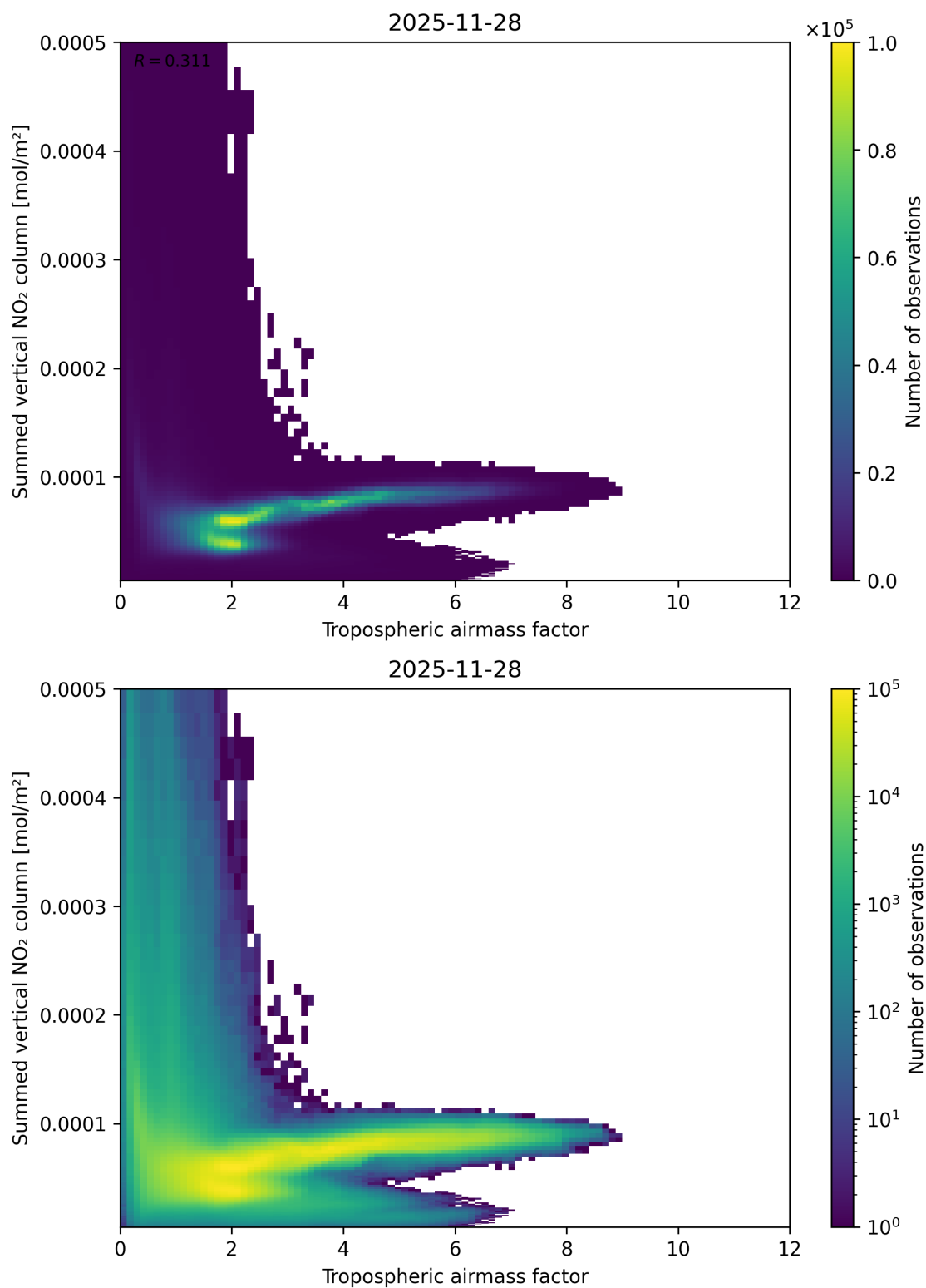
Figure 75: Scatter density plot of “Tropospheric air mass factor” against “Summed vertical NO 2 column” for 2025-11-28 to 2025-11-29.
