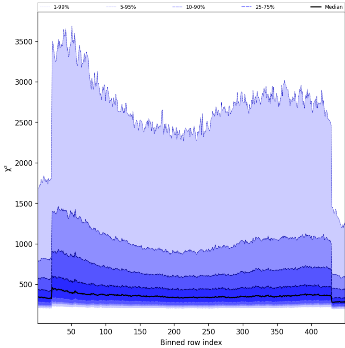
Figure 59: Along track statistics of “ \chi^2 ” for 2025-11-28 to 2025-11-29
