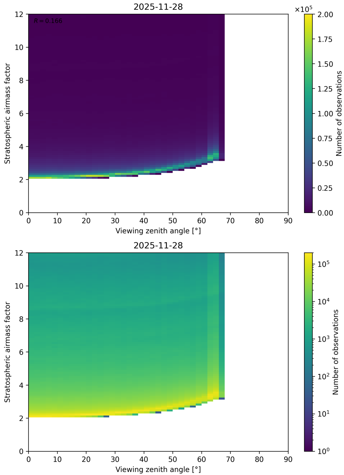
Figure 159: Scatter density plot of “Viewing zenith angle” against “Stratospheric airmass factor” for 2025-11-28 to 2025-11-29.
