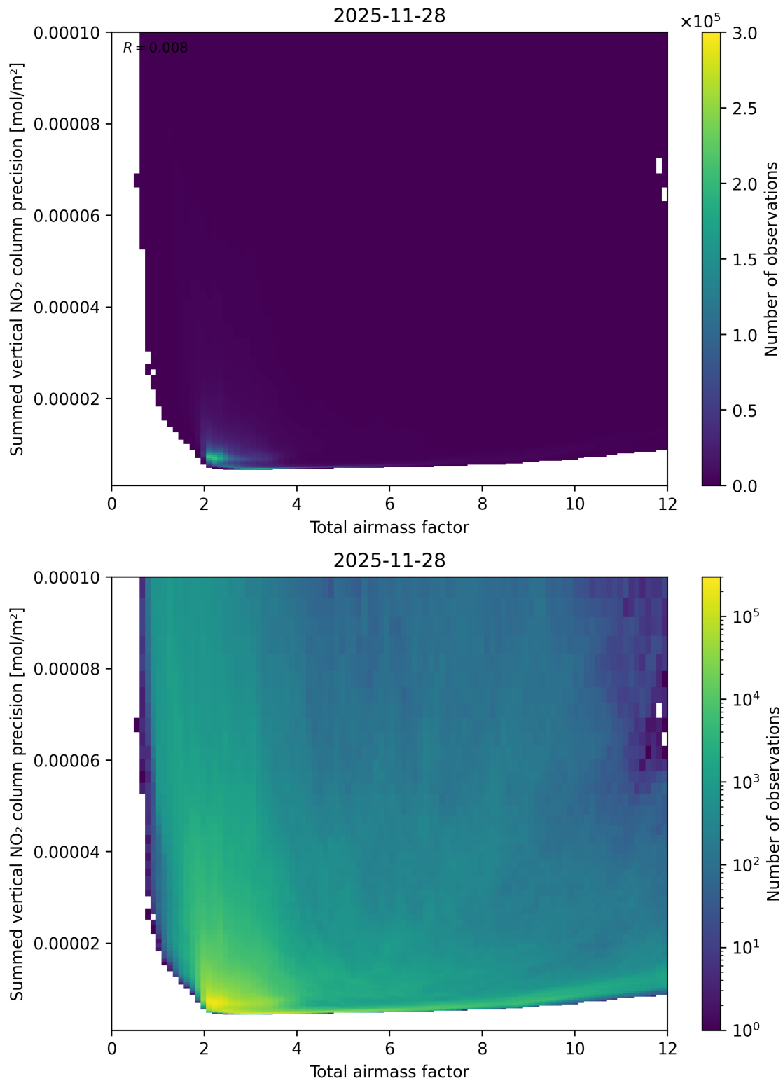
Figure 66: Scatter density plot of “Total airmass factor” against “Summed vertical NO 2 column precision” for 2025-11-28 to 2025-11-29.
