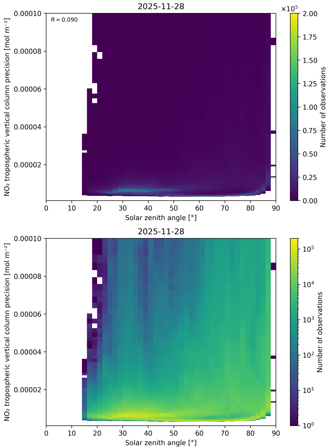
Figure 156: Scatter density plot of “Solar zenith angle” against “NO 2 tropospheric vertical column precision” for 2025-11-28 to 2025-11-29.
