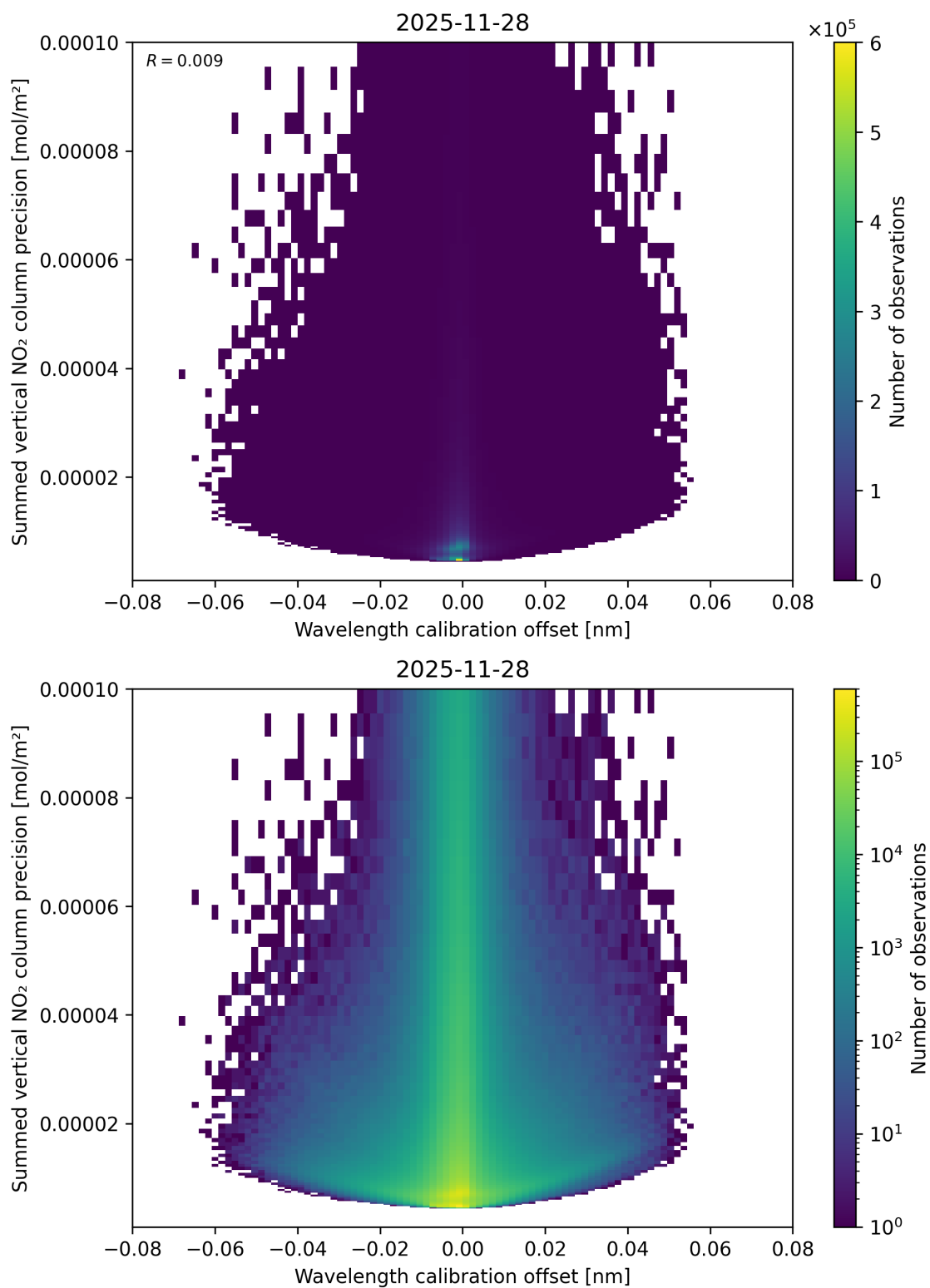
Figure 178: Scatter density plot of “Wavelength calibration offset” against “Summed vertical NO 2 column precision” for 2025-11-28 to 2025-11-29.
