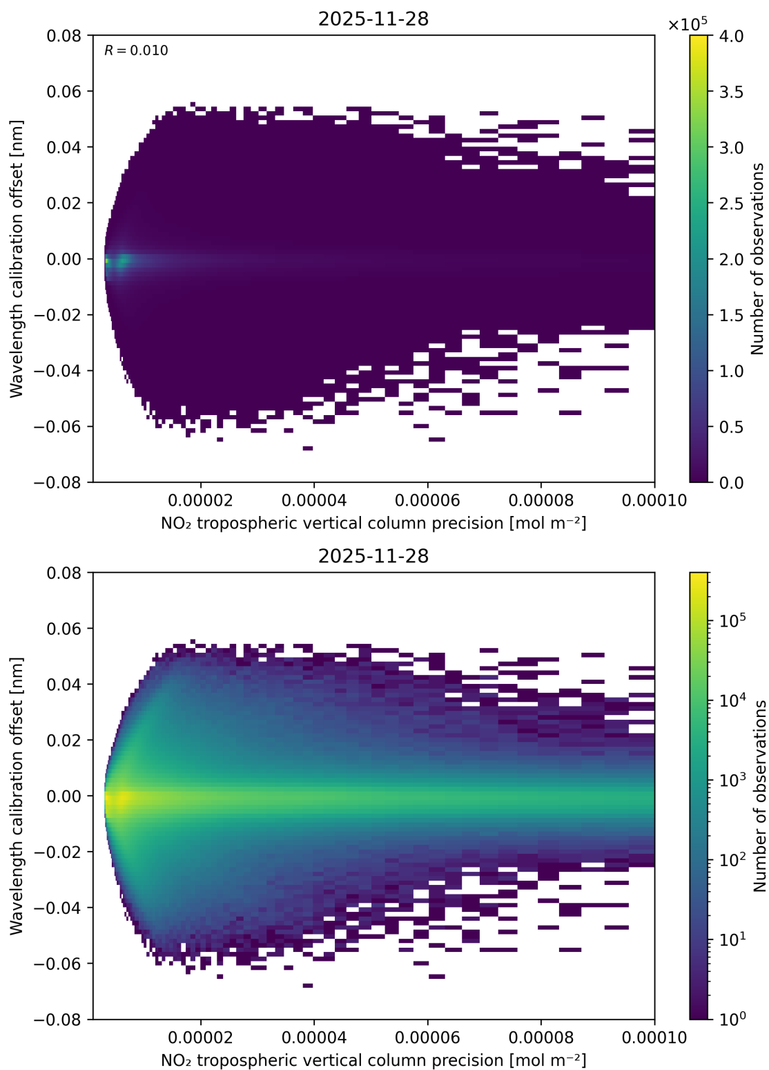
Figure 141: Scatter density plot of “NO 2 tropospheric vertical column precision” against “Wavelength calibration offset” for 2025-11-28 to 2025-11-29.
