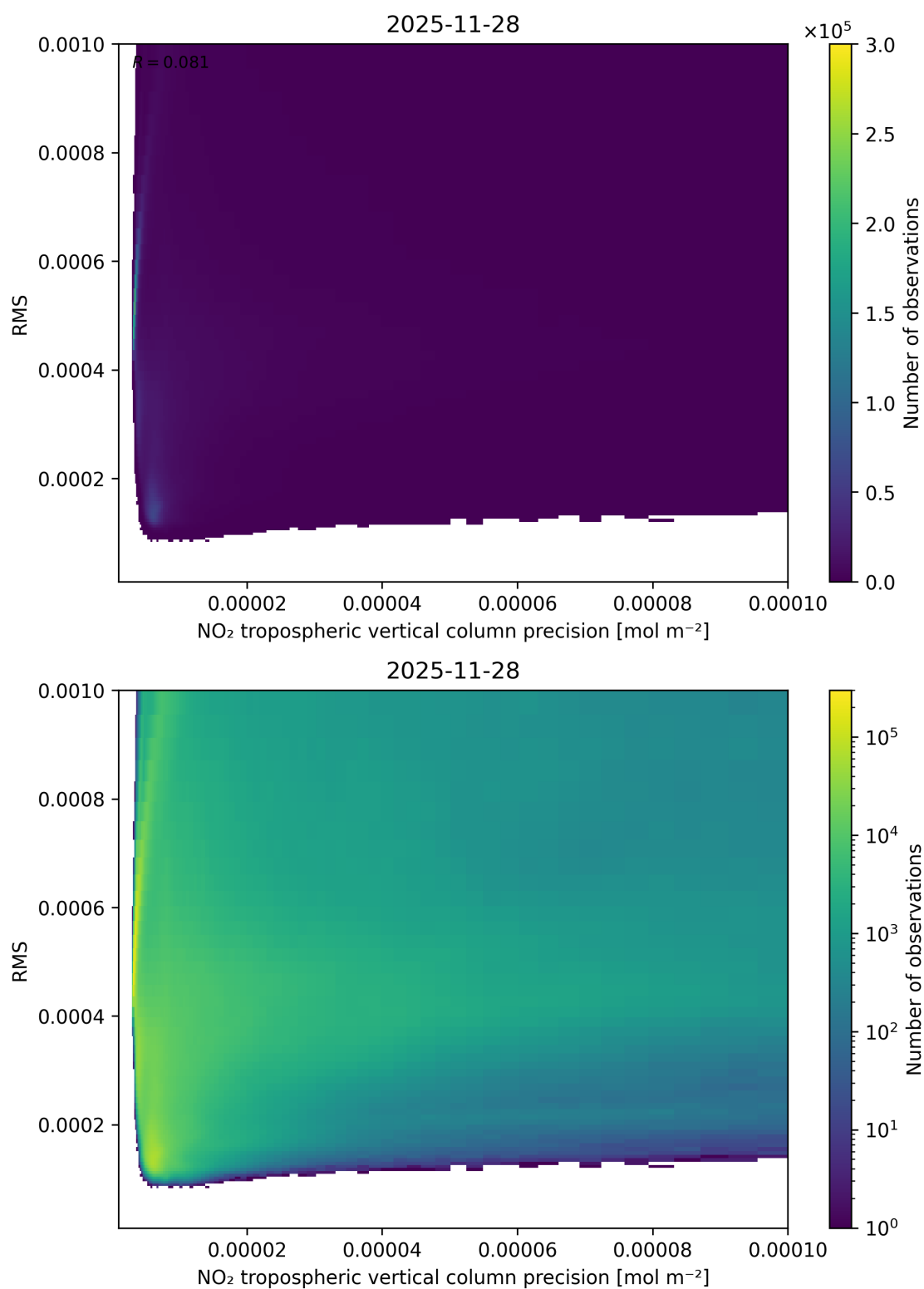
Figure 140: Scatter density plot of “NO 2 tropospheric vertical column precision” against “RMS” for 2025-11-28 to 2025-11-29.
