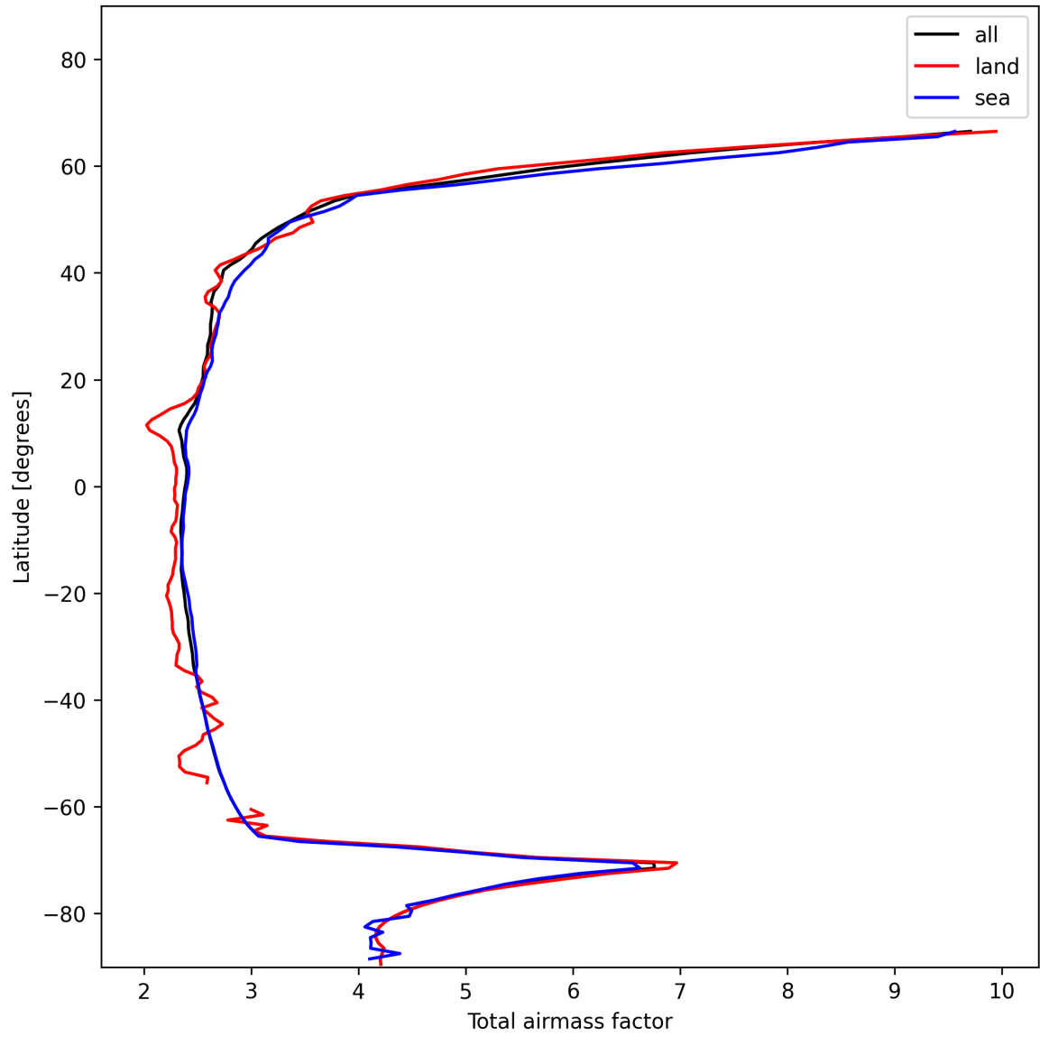
Figure 15: Zonal average of “Total airmass factor” for 2025-11-28 to 2025-11-29.
