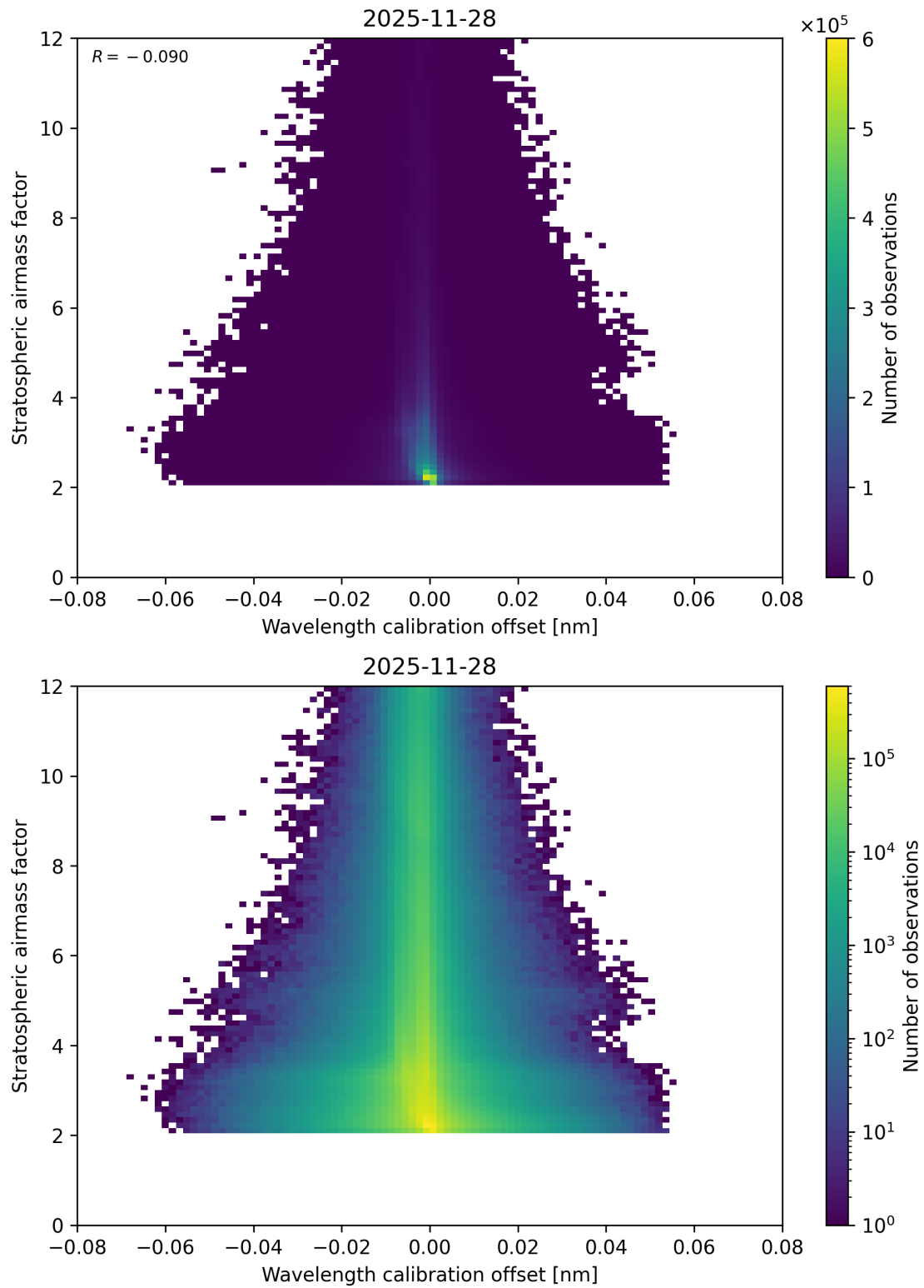
Figure 174: Scatter density plot of “Wavelength calibration offset” against “Stratospheric airmass factor” for 2025-11-28 to 2025-11-29.
