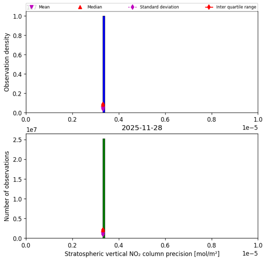
Figure 37: Histogram of “Stratospheric vertical NO 2 column precision” for 2025-11-28 to 2025-11-29
