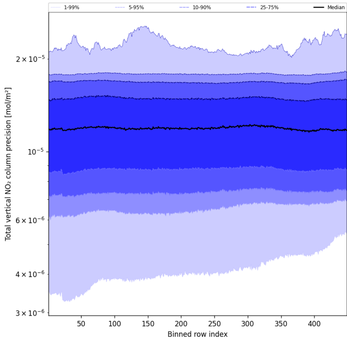
Figure 56: Along track statistics of “Total vertical NO 2 column precision” for 2025-11-28 to 2025-11-29
