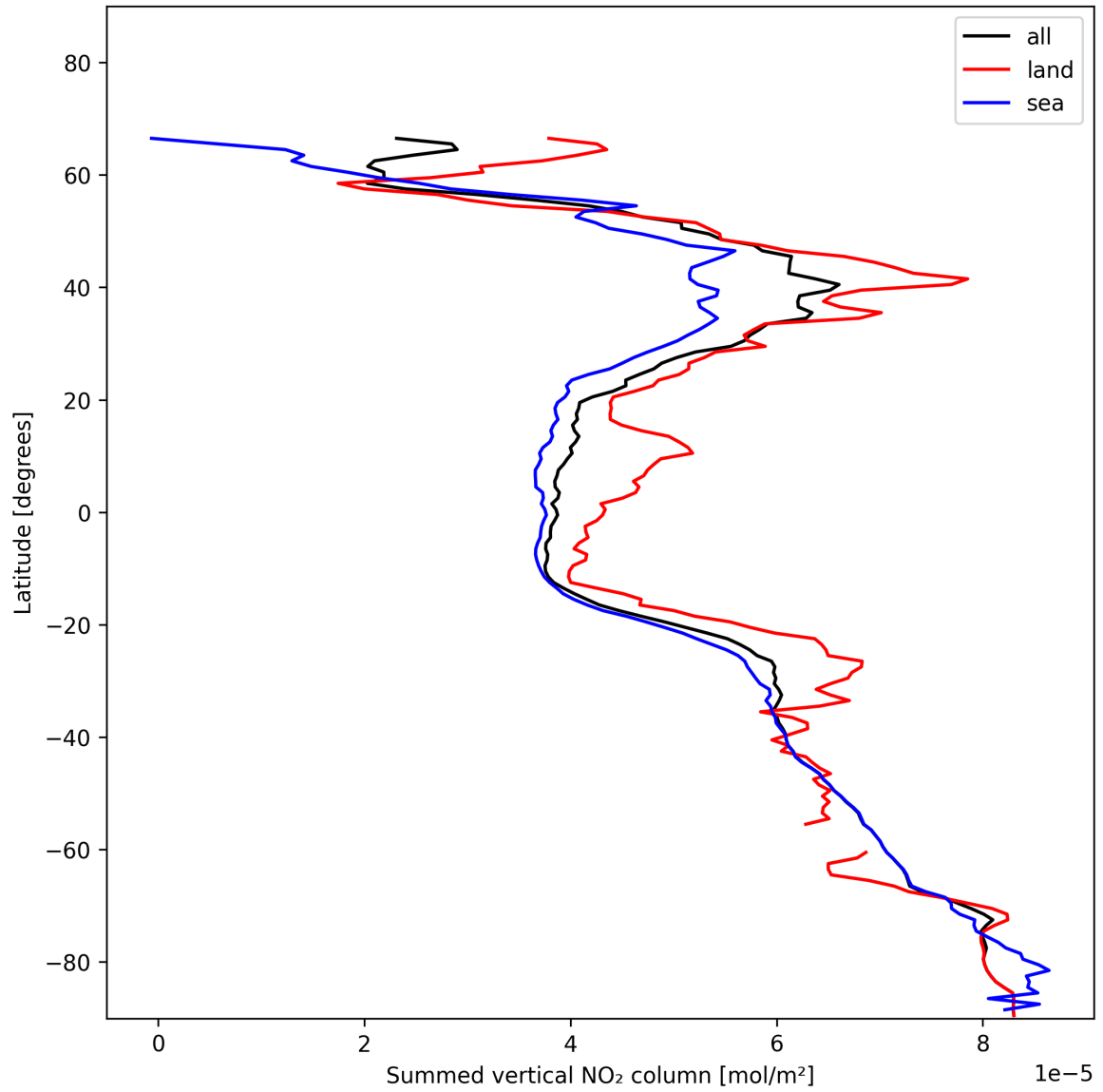
Figure 23: Zonal average of “Summed vertical NO 2 column” for 2025-11-28 to 2025-11-29.
