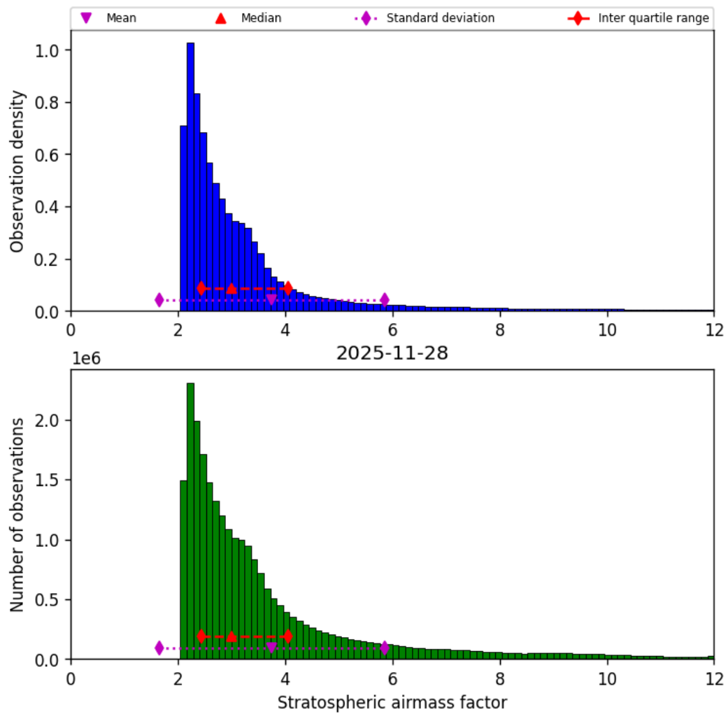
Figure 44: Histogram of “Stratospheric airmass factor” for 2025-11-28 to 2025-11-29
