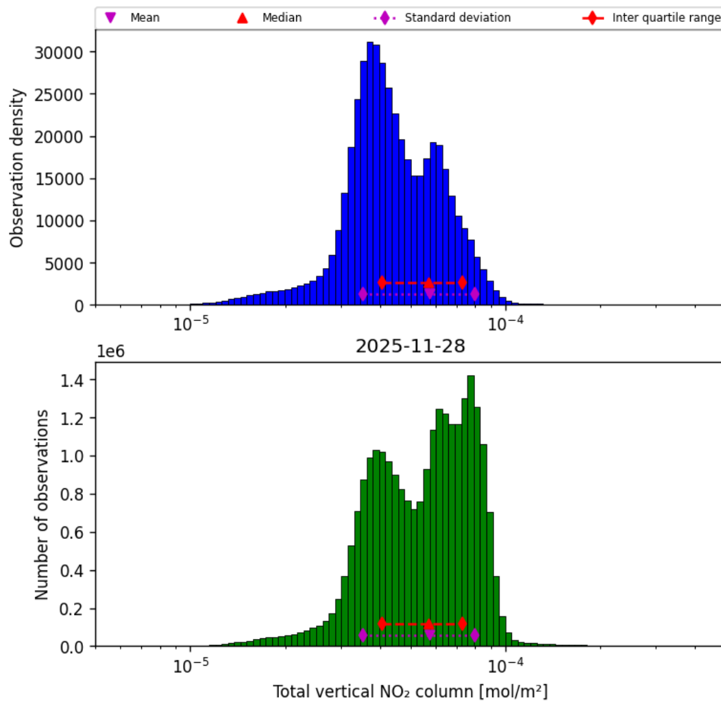
Figure 38: Histogram of “Total vertical NO 2 column” for 2025-11-28 to 2025-11-29
