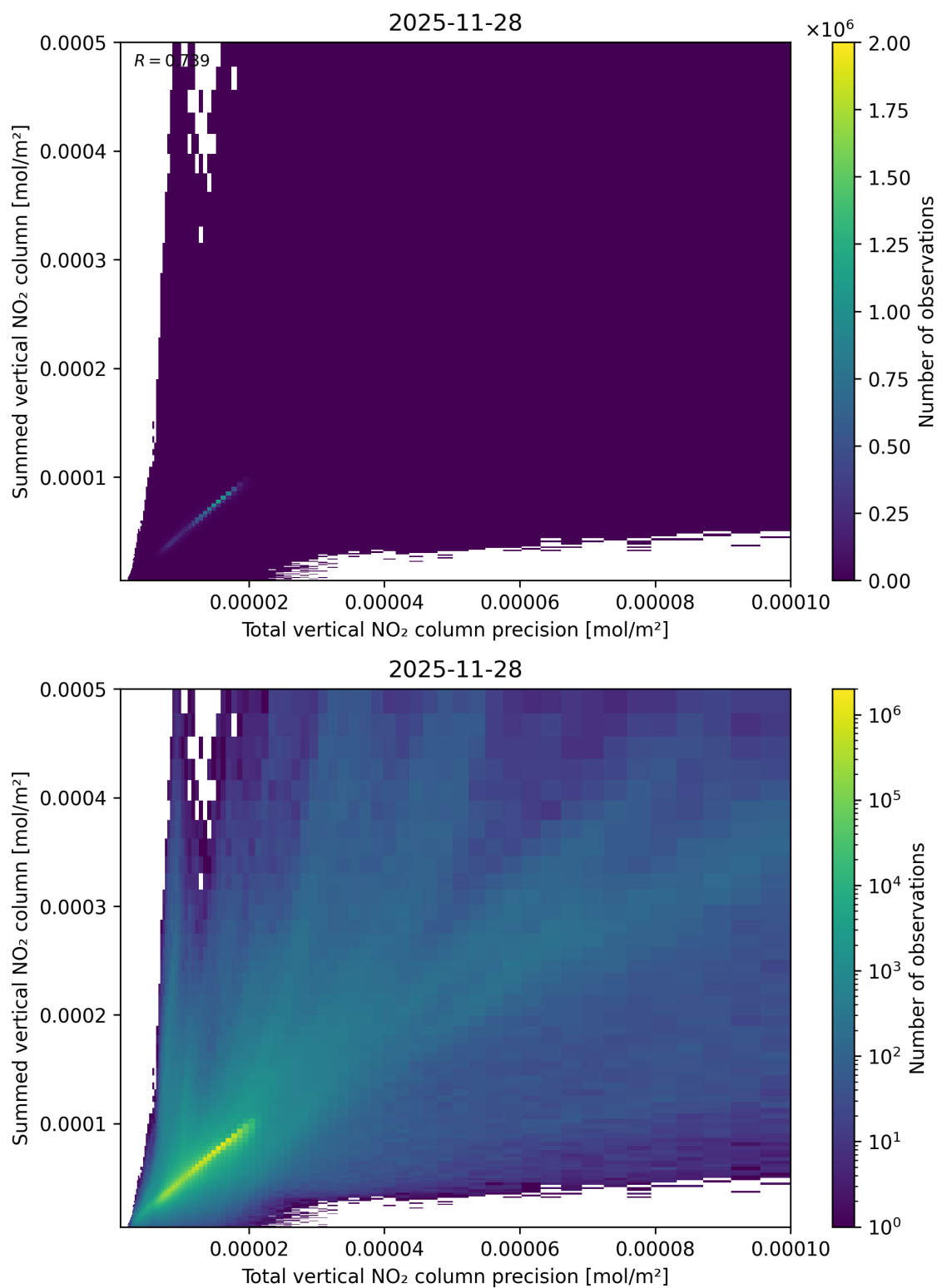
Figure 117: Scatter density plot of “Total vertical NO 2 column precision” against “Summed vertical NO 2 column” for 2025-11-28 to 2025-11-29.
