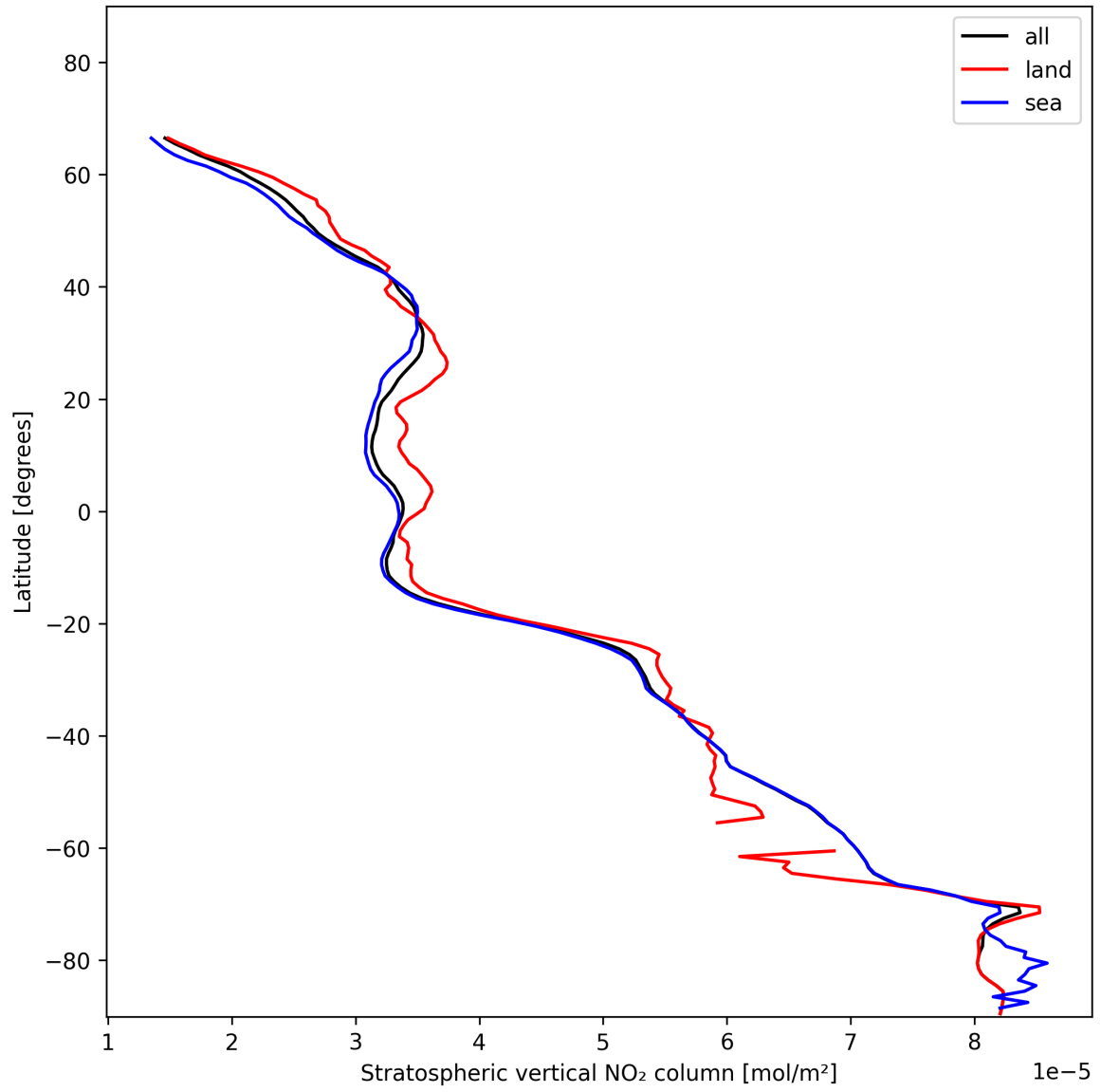
Figure 19: Zonal average of “Stratospheric vertical NO 2 column” for 2025-11-28 to 2025-11-29.
