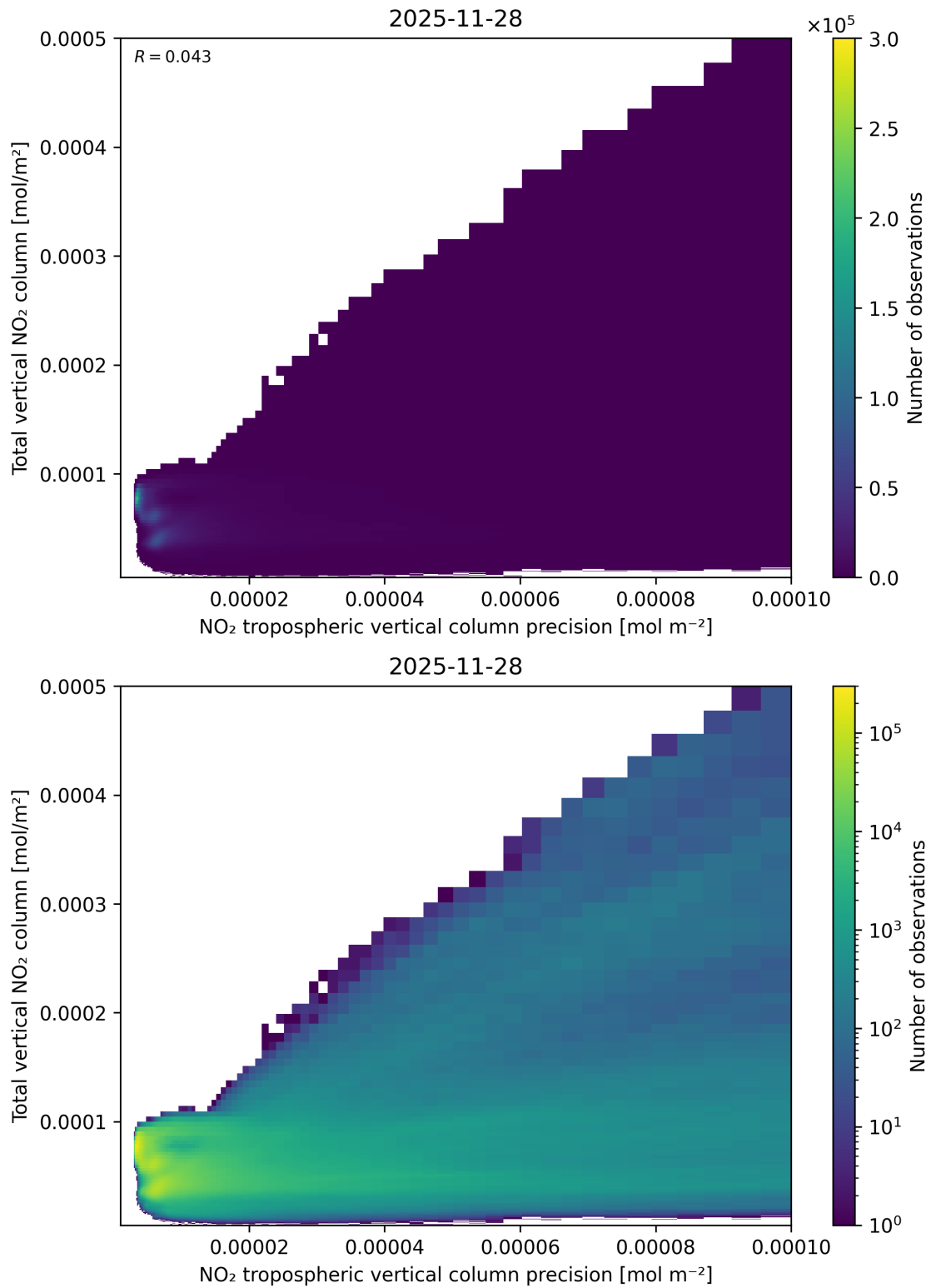
Figure 138: Scatter density plot of “NO 2 tropospheric vertical column precision” against “Total vertical NO 2 column” for 2025-11-28 to 2025-11-29.
