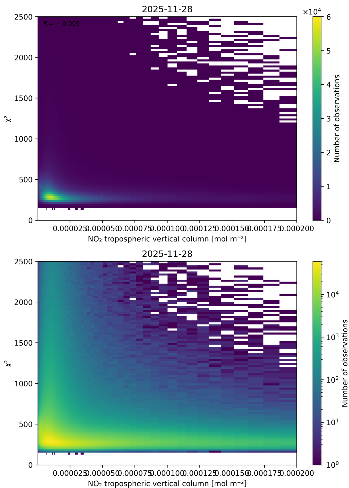
Figure 124: Scatter density plot of “NO 2 tropospheric vertical column” against “ \chi^2 ” for 2025-11-28 to 2025-11-29.
