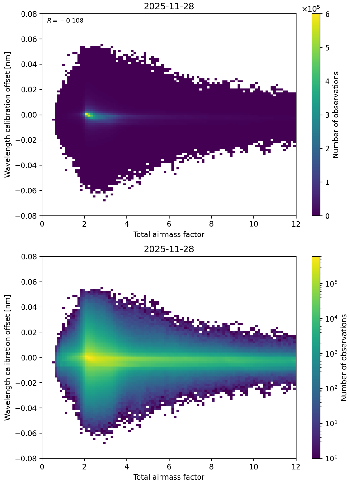
Figure 70: Scatter density plot of “Total airmass factor” against “Wavelength calibration offset” for 2025-11-28 to 2025-11-29.
