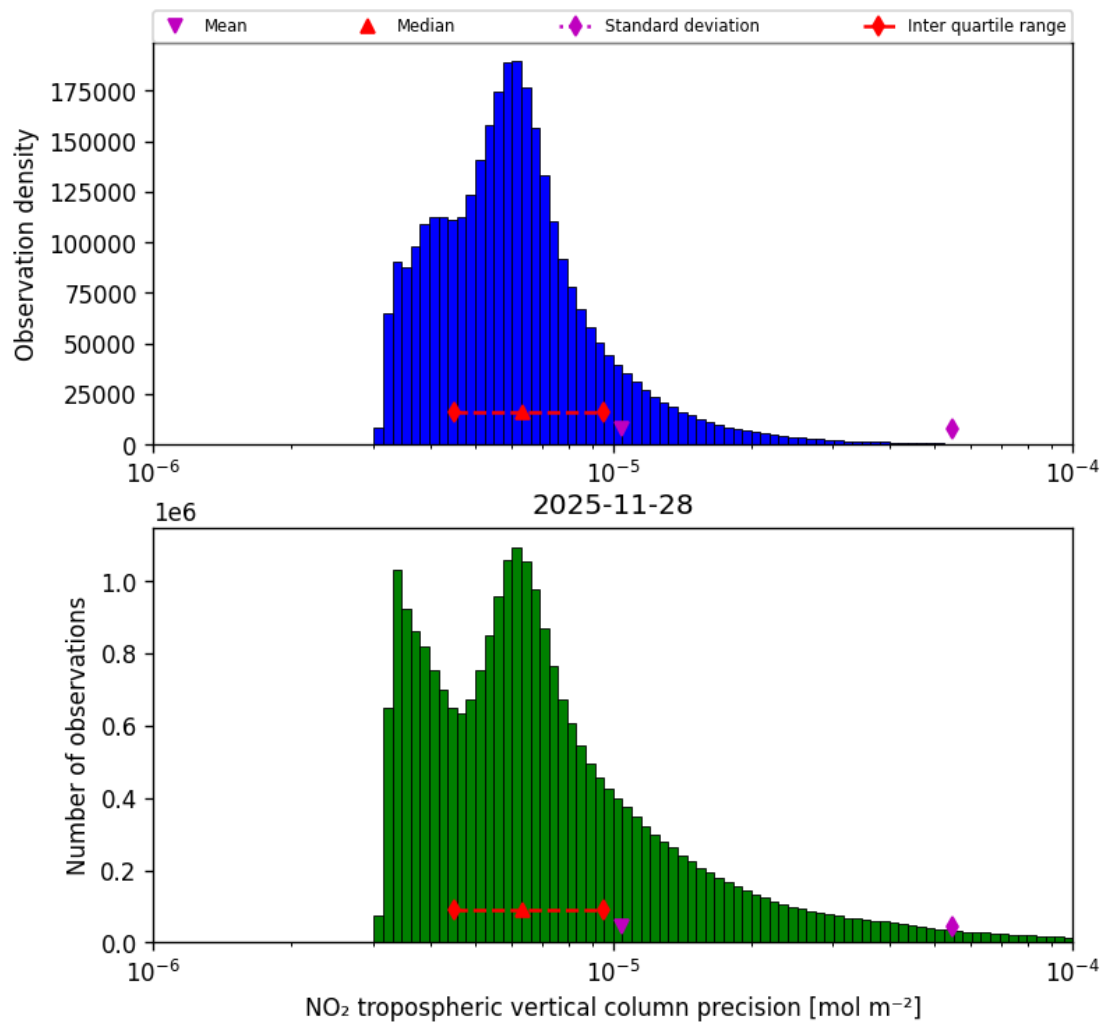
Figure 30: Histogram of “NO 2 tropospheric vertical column precision” for 2025-11-28 to 2025-11-29
