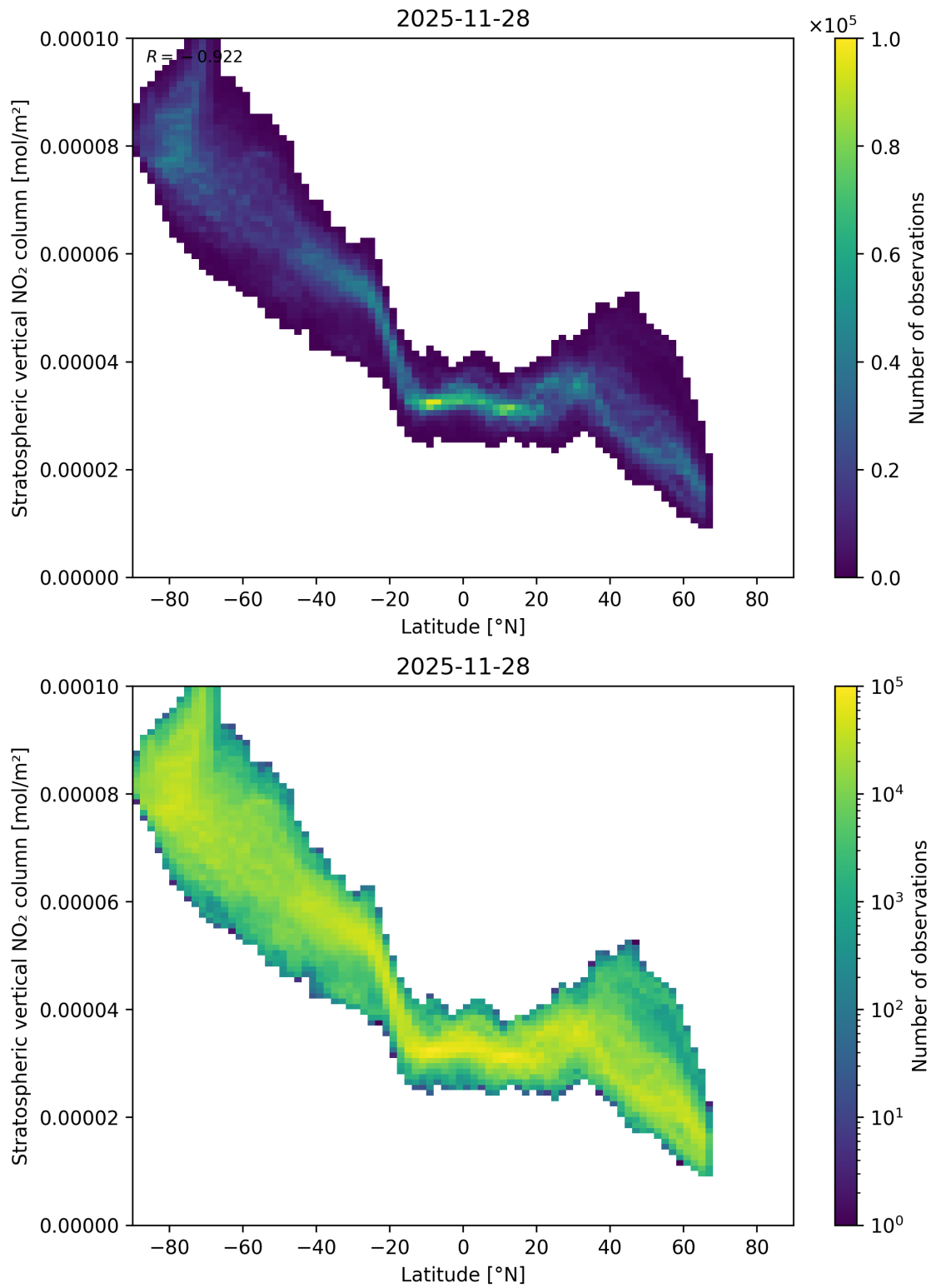
Figure 87: Scatter density plot of “Latitude” against “Stratospheric vertical NO 2 column” for 2025-11-28 to 2025-11-29.
