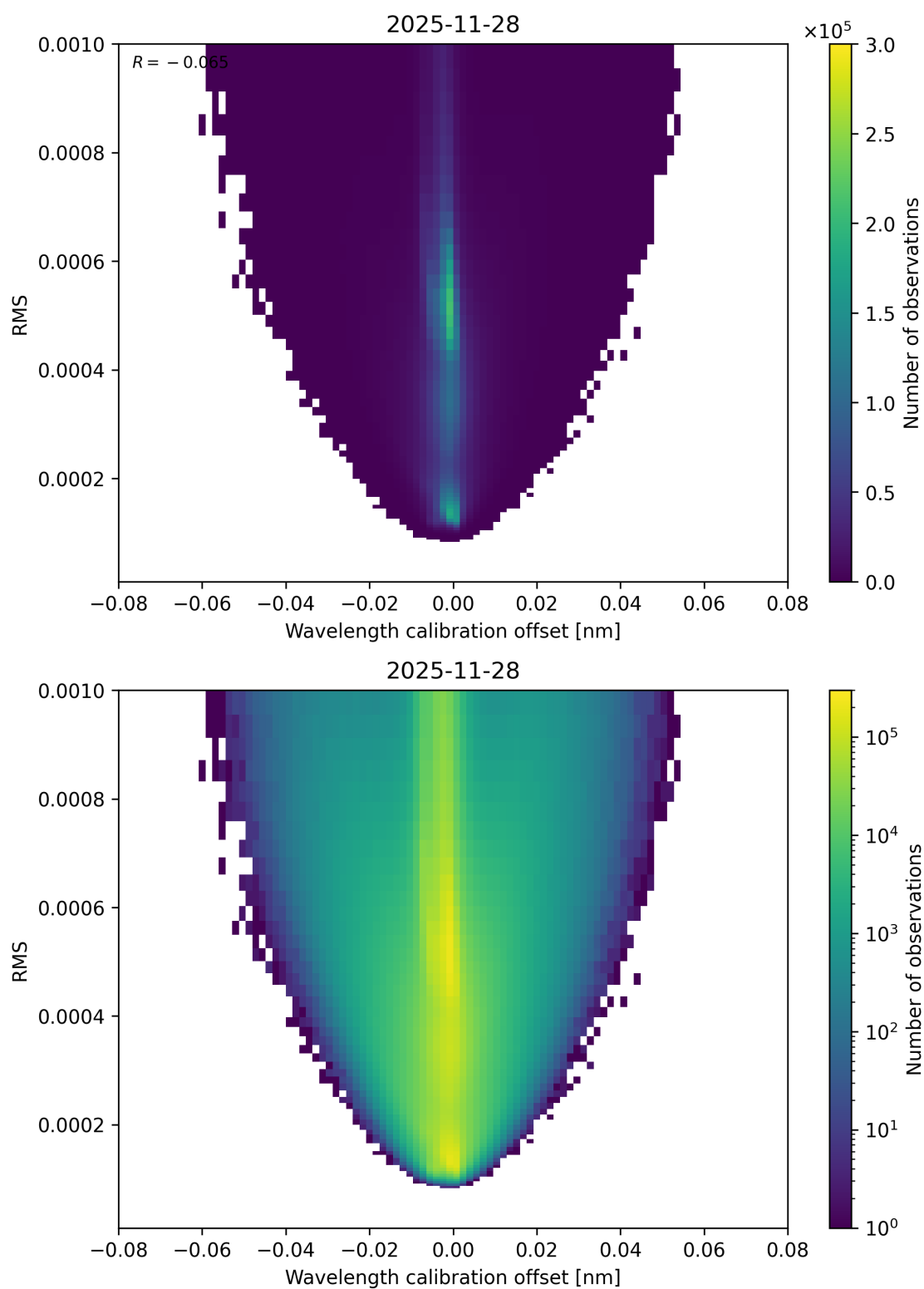
Figure 181: Scatter density plot of “Wavelength calibration offset” against “RMS” for 2025-11-28 to 2025-11-29.
