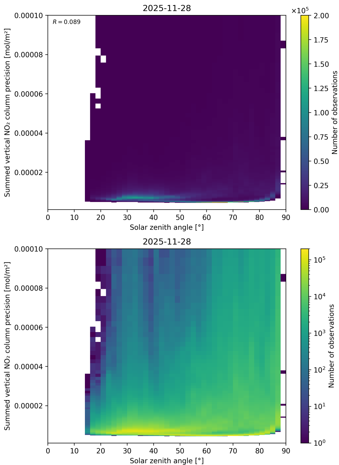
Figure 152: Scatter density plot of “Solar zenith angle” against “Summed vertical NO 2 column precision” for 2025-11-28 to 2025-11-29.
