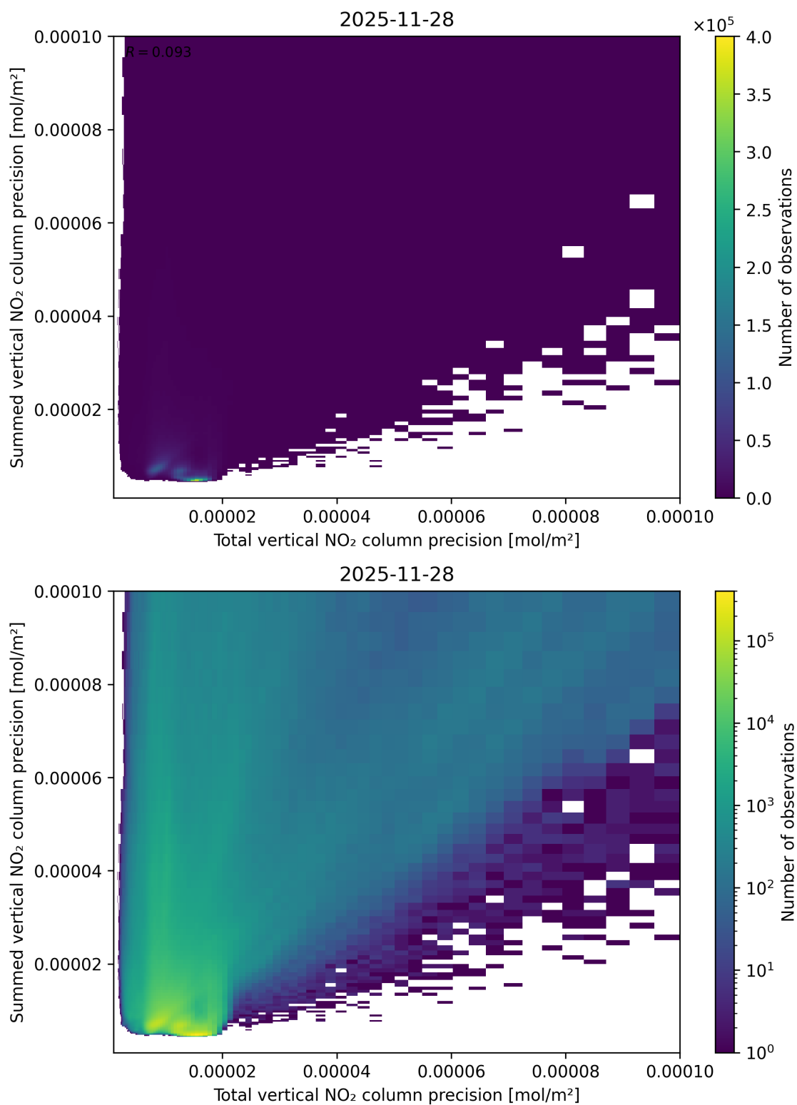
Figure 118: Scatter density plot of “Total vertical NO 2 column precision” against “Summed vertical NO 2 column precision” for 2025-11-28 to 2025-11-29.
