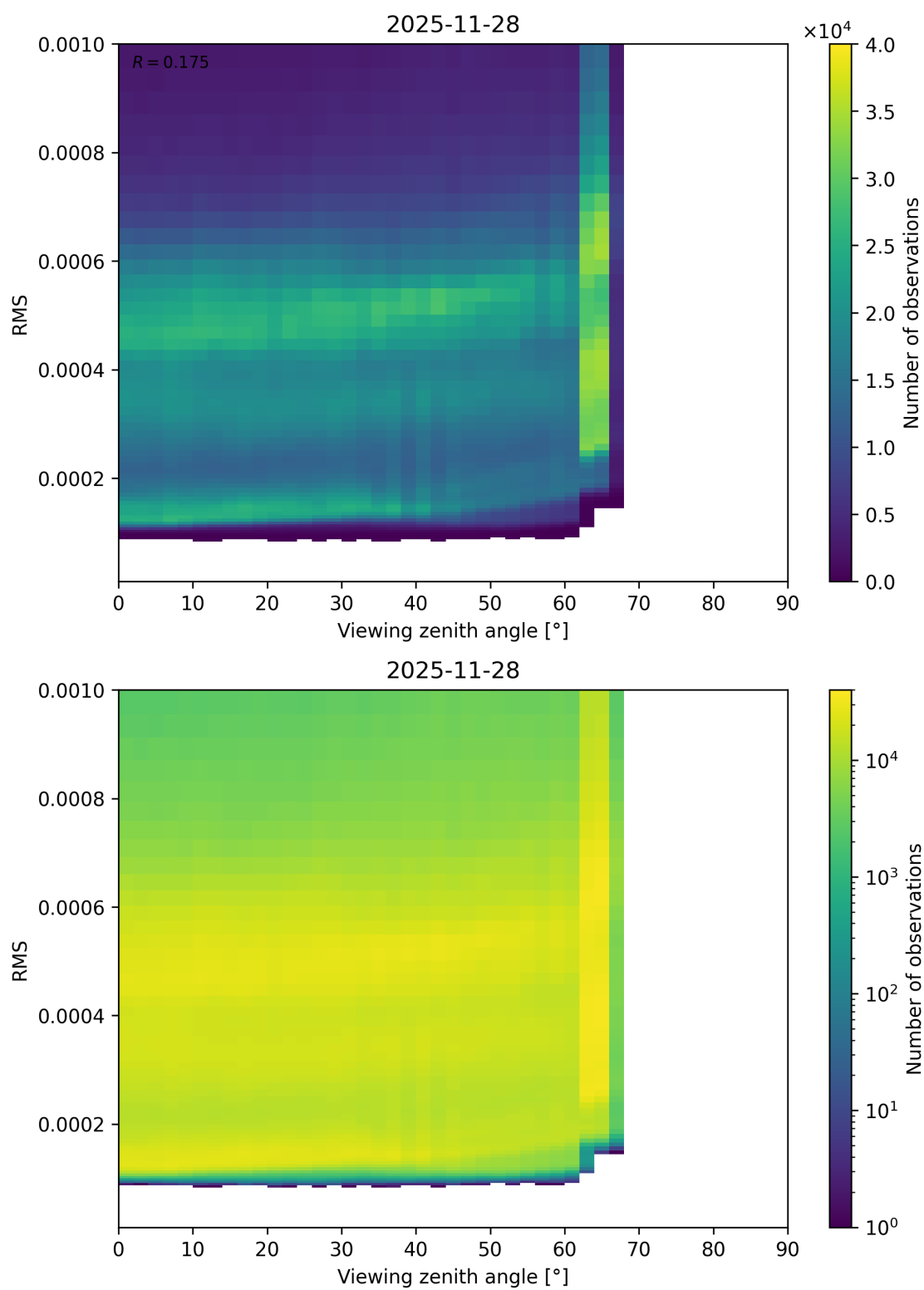
Figure 171: Scatter density plot of “Viewing zenith angle” against “RMS” for 2025-11-28 to 2025-11-29.
