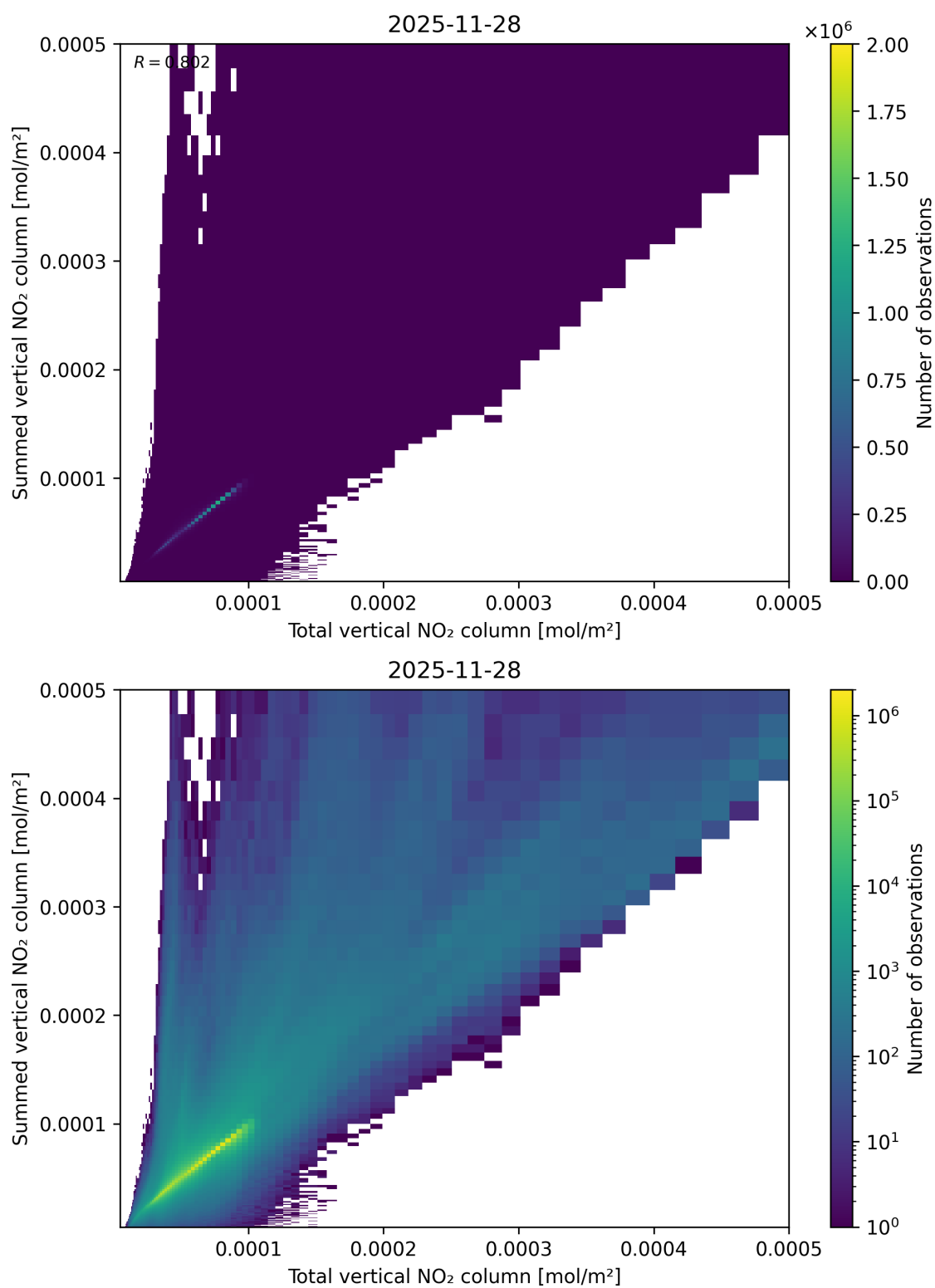
Figure 112: Scatter density plot of “Total vertical NO 2 column” against “Summed vertical NO 2 column” for 2025-11-28 to 2025-11-29.
