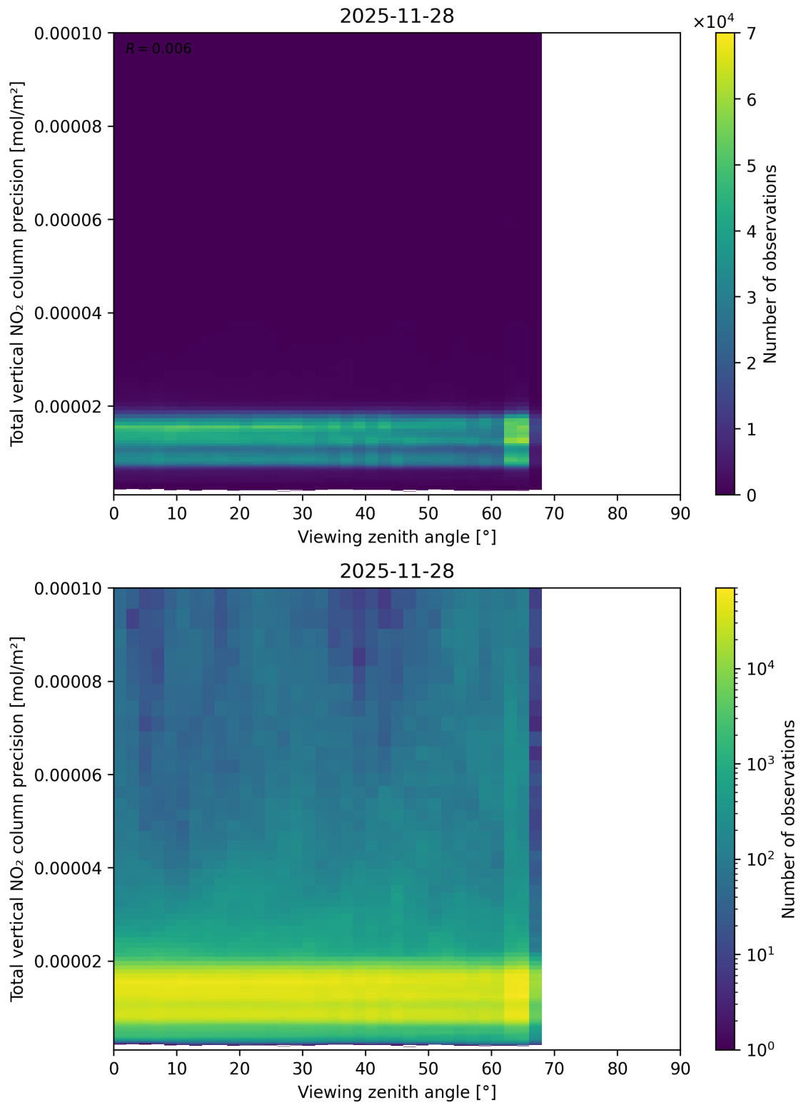
Figure 168: Scatter density plot of “Viewing zenith angle” against “Total vertical NO 2 column precision” for 2025-11-28 to 2025-11-29.
