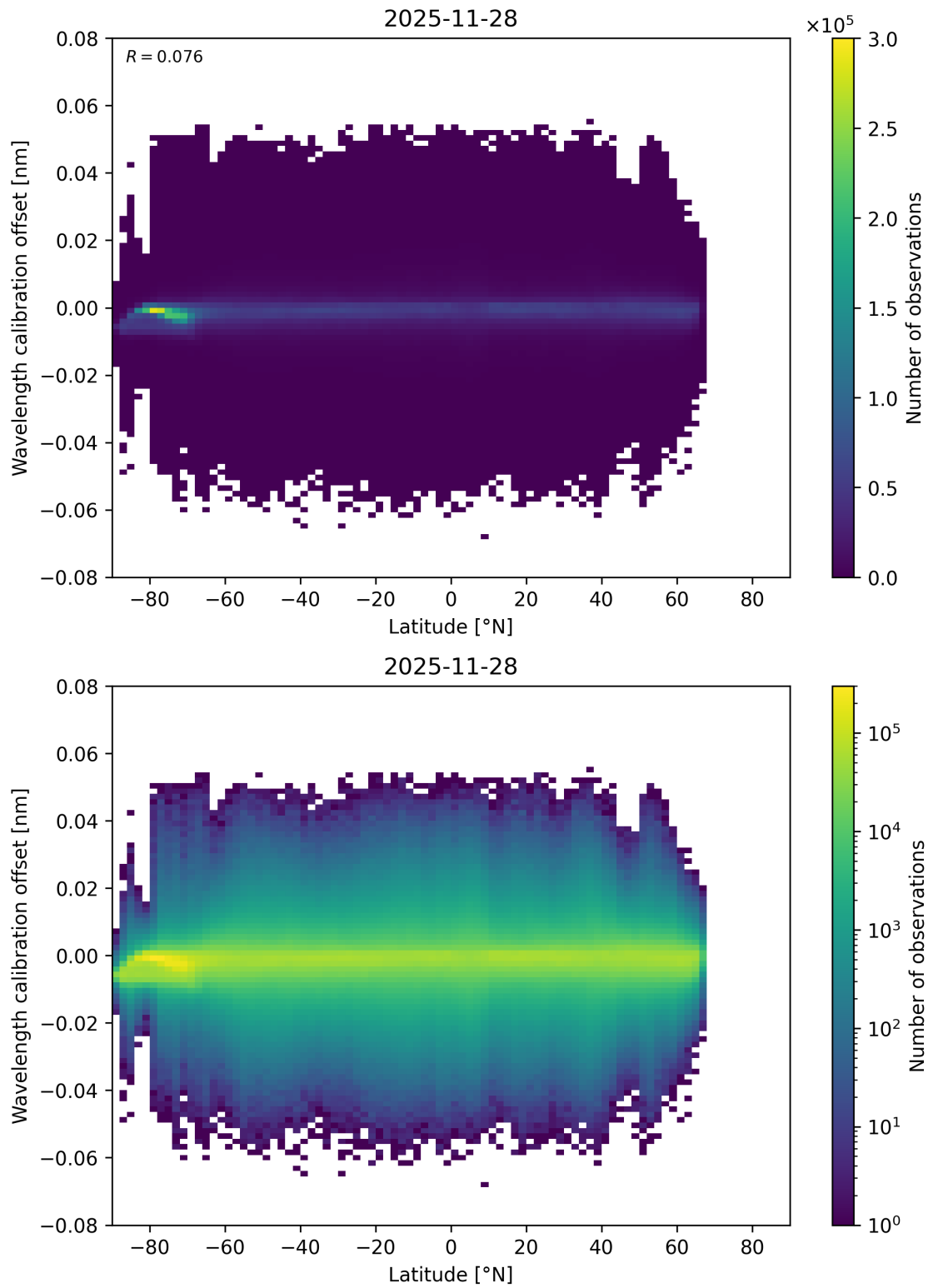
Figure 95: Scatter density plot of “Latitude” against “Wavelength calibration offset” for 2025-11-28 to 2025-11-29.
