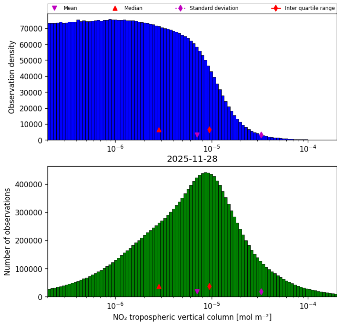
Figure 29: Histogram of “NO 2 tropospheric vertical column” for 2025-11-28 to 2025-11-29
