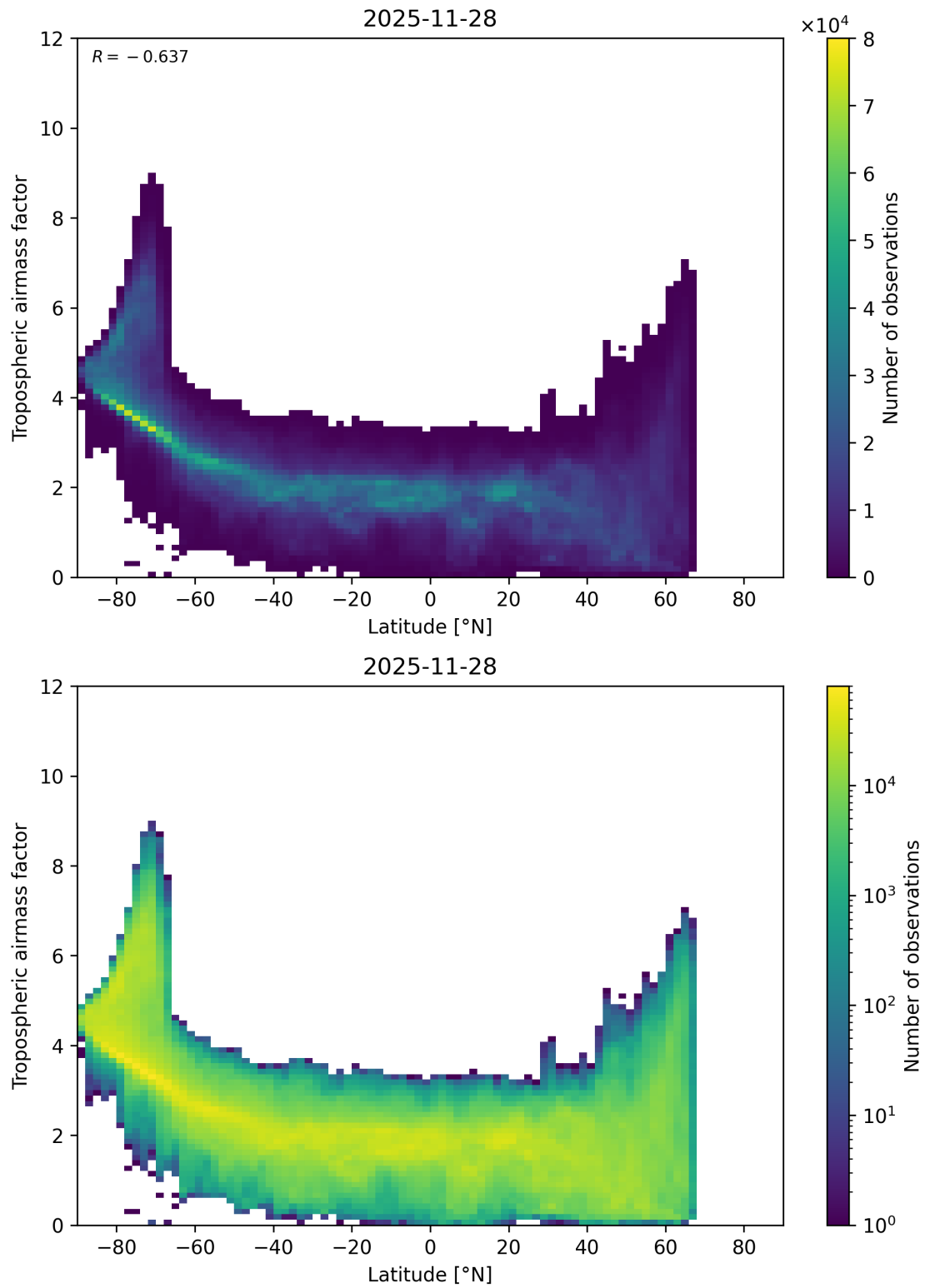
Figure 85: Scatter density plot of “Latitude” against “Tropospheric airmass factor” for 2025-11-28 to 2025-11-29.
