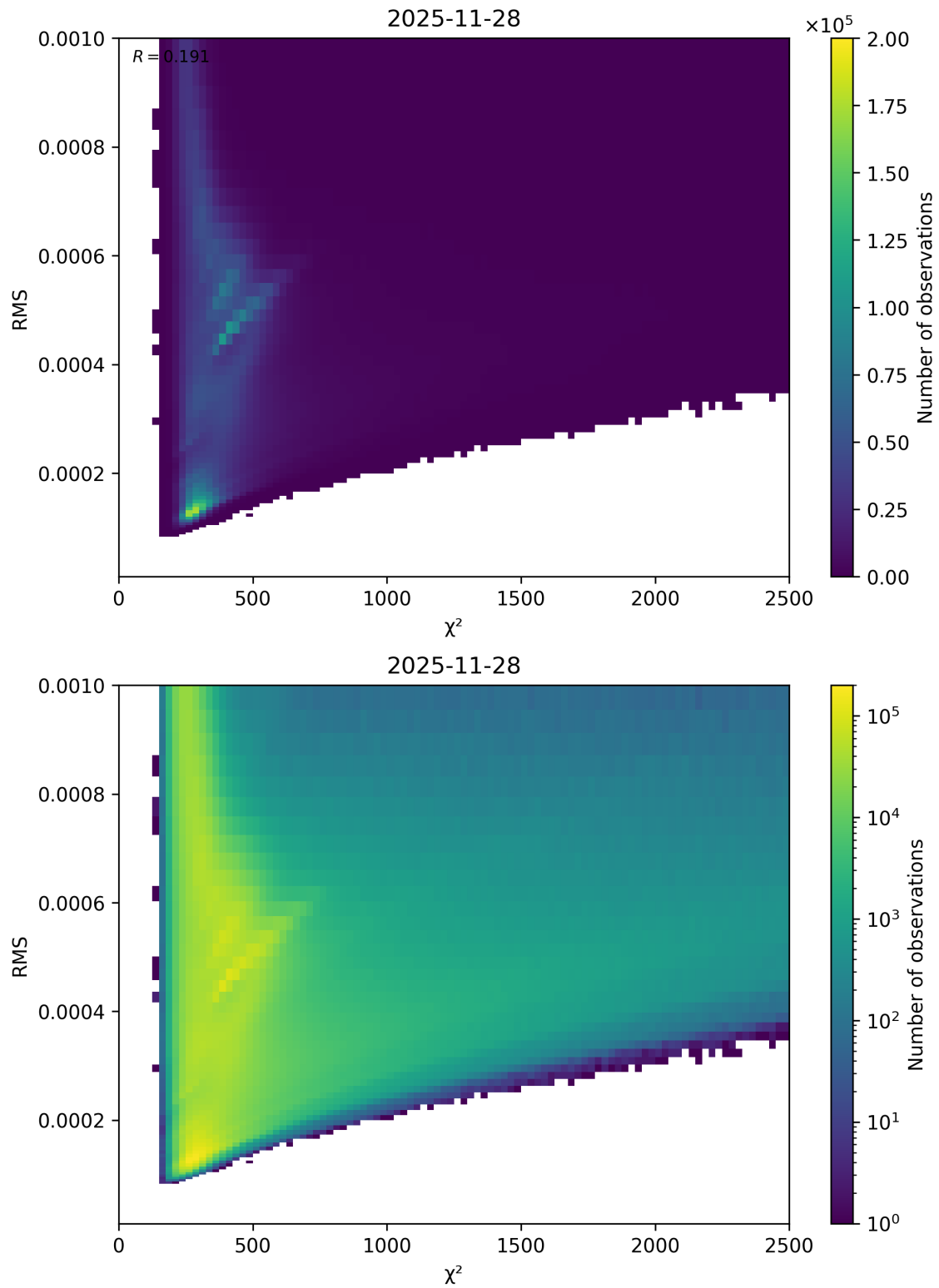
Figure 82: Scatter density plot of “ \chi^2 ” against “RMS” for 2025-11-28 to 2025-11-29.
