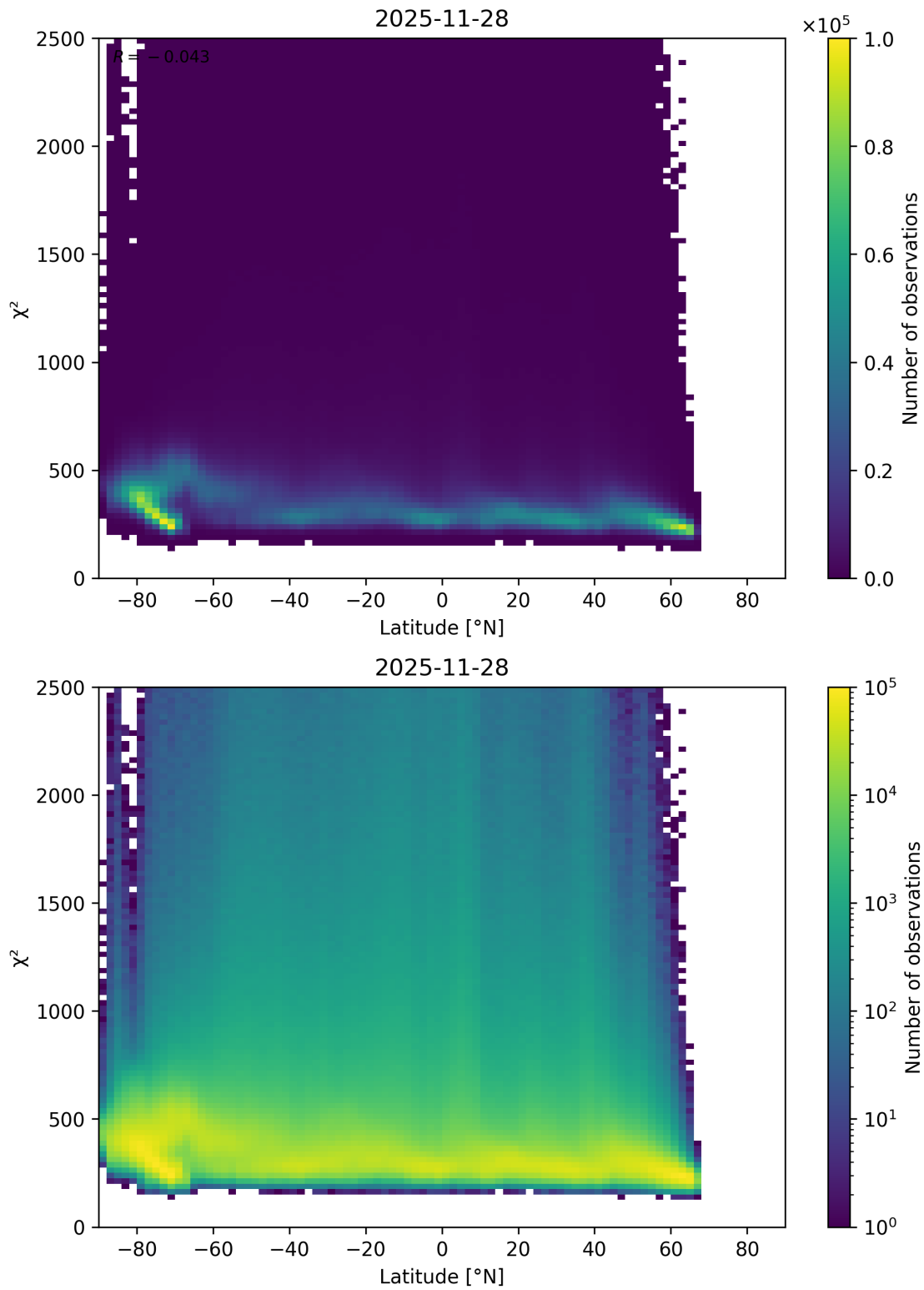
Figure 86: Scatter density plot of “Latitude” against “ \chi^2 ” for 2025-11-28 to 2025-11-29.
