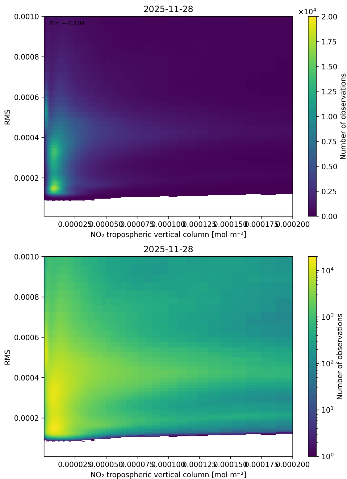
Figure 142: Scatter density plot of “NO 2 tropospheric vertical column” against “RMS” for 2025-11-28 to 2025-11-29.
