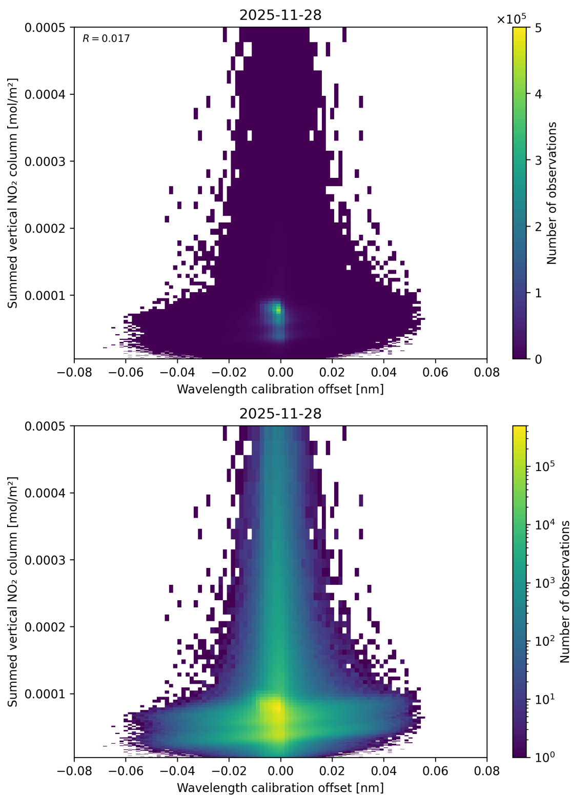
Figure 177: Scatter density plot of “Wavelength calibration offset” against “Summed vertical NO 2 column” for 2025-11-28 to 2025-11-29.
