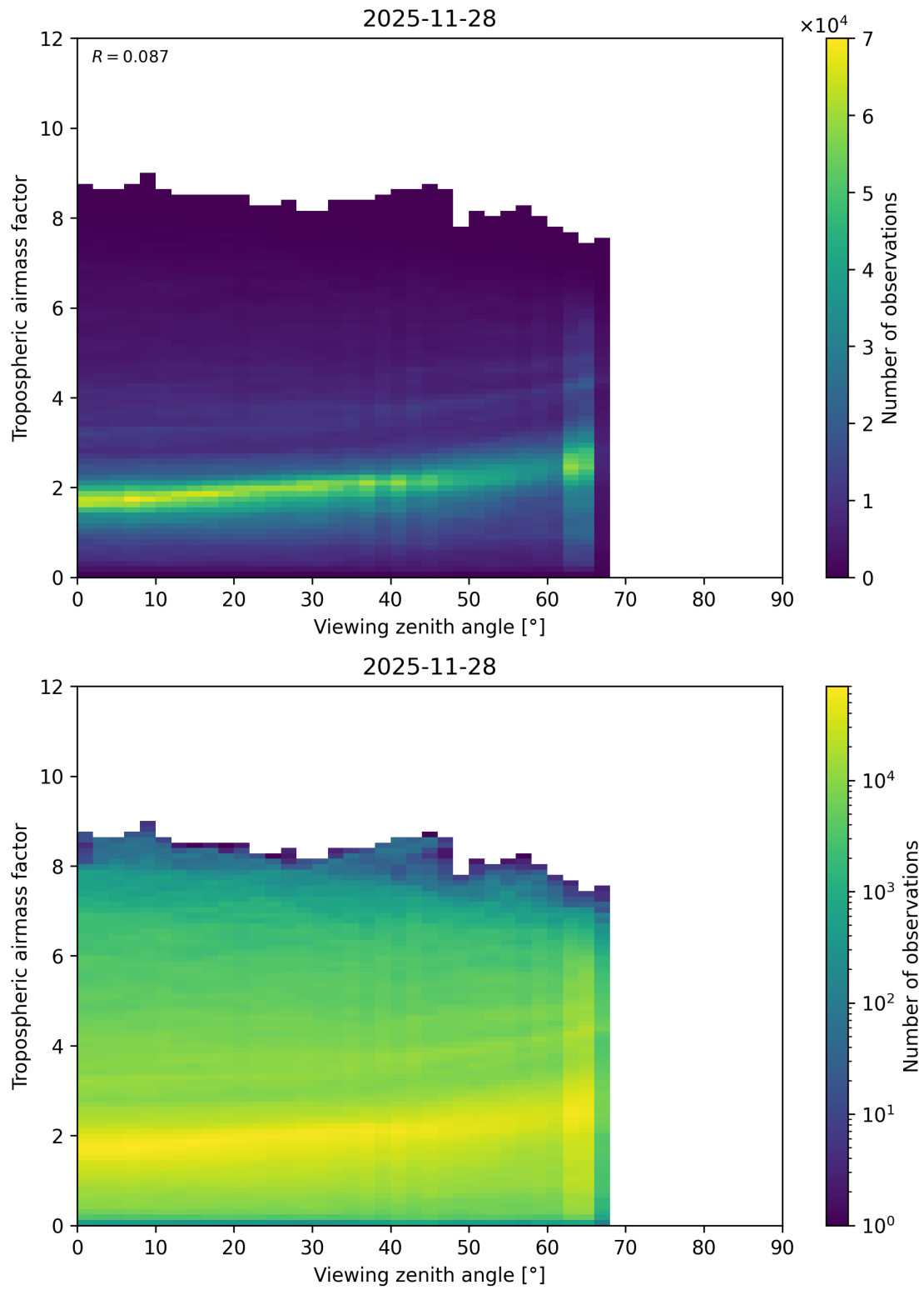
Figure 161: Scatter density plot of “Viewing zenith angle” against “Tropospheric airmass factor” for 2025-11-28 to 2025-11-29.
