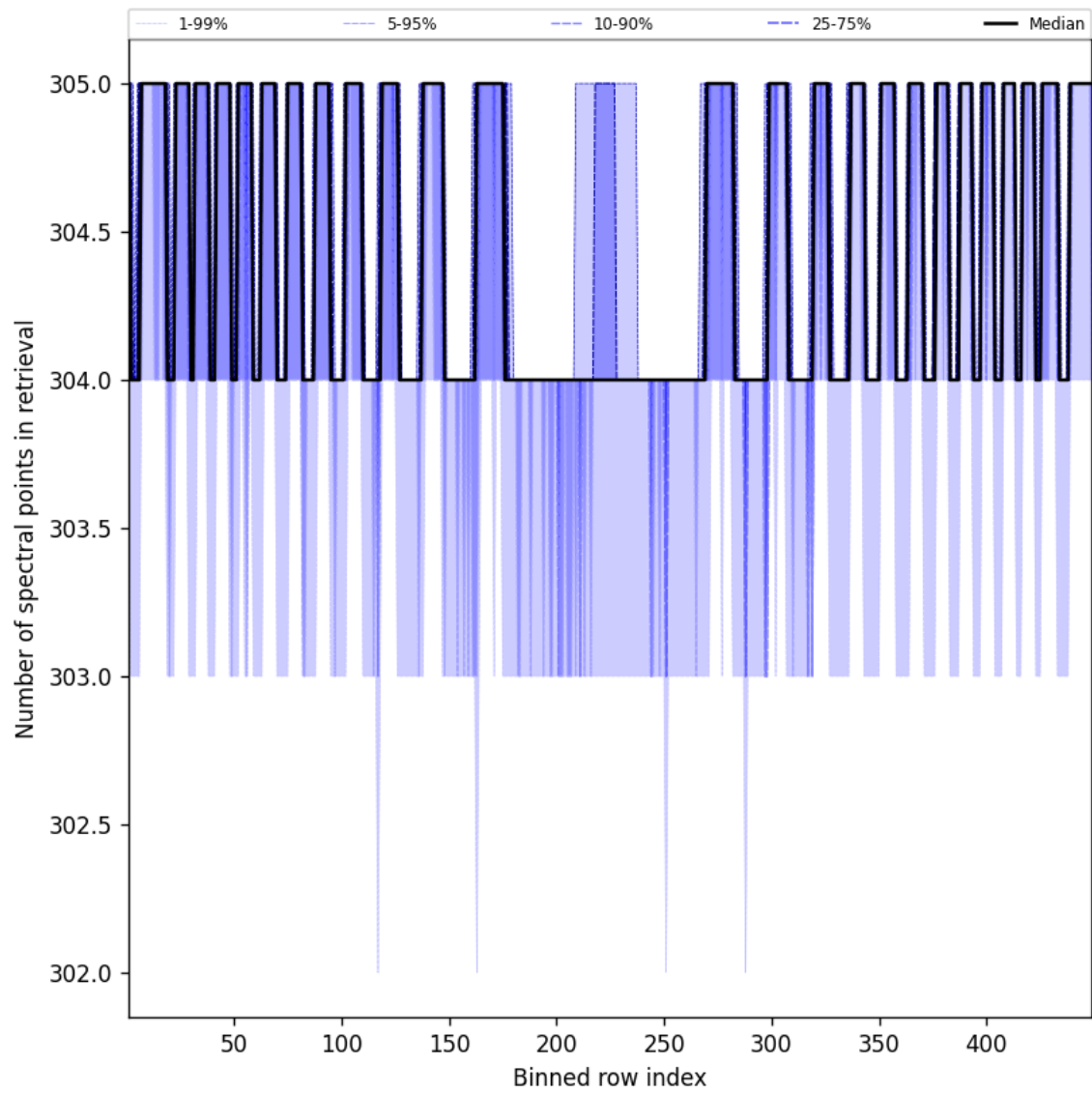
Figure 50: Along track statistics of “Number of spectral points in retrieval” for 2025-11-28 to 2025-11-29
