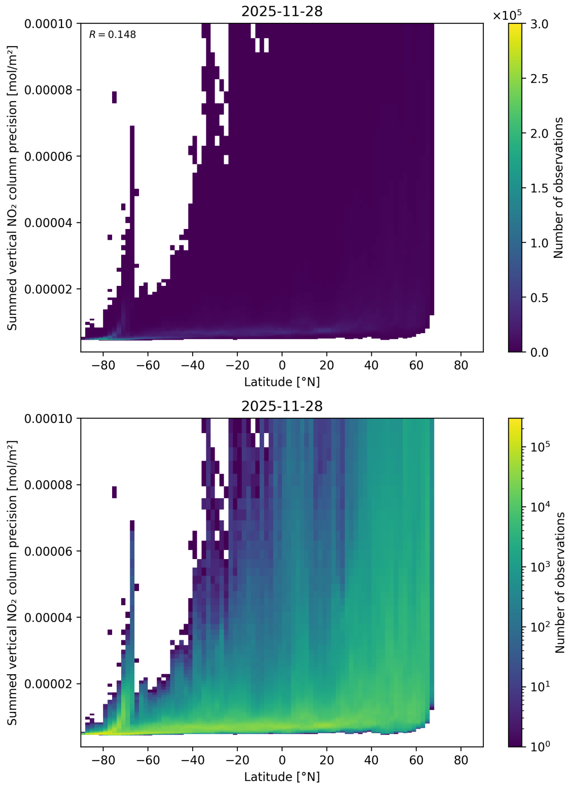
Figure 89: Scatter density plot of “Latitude” against “Summed vertical NO 2 column precision” for 2025-11-28 to 2025-11-29.
