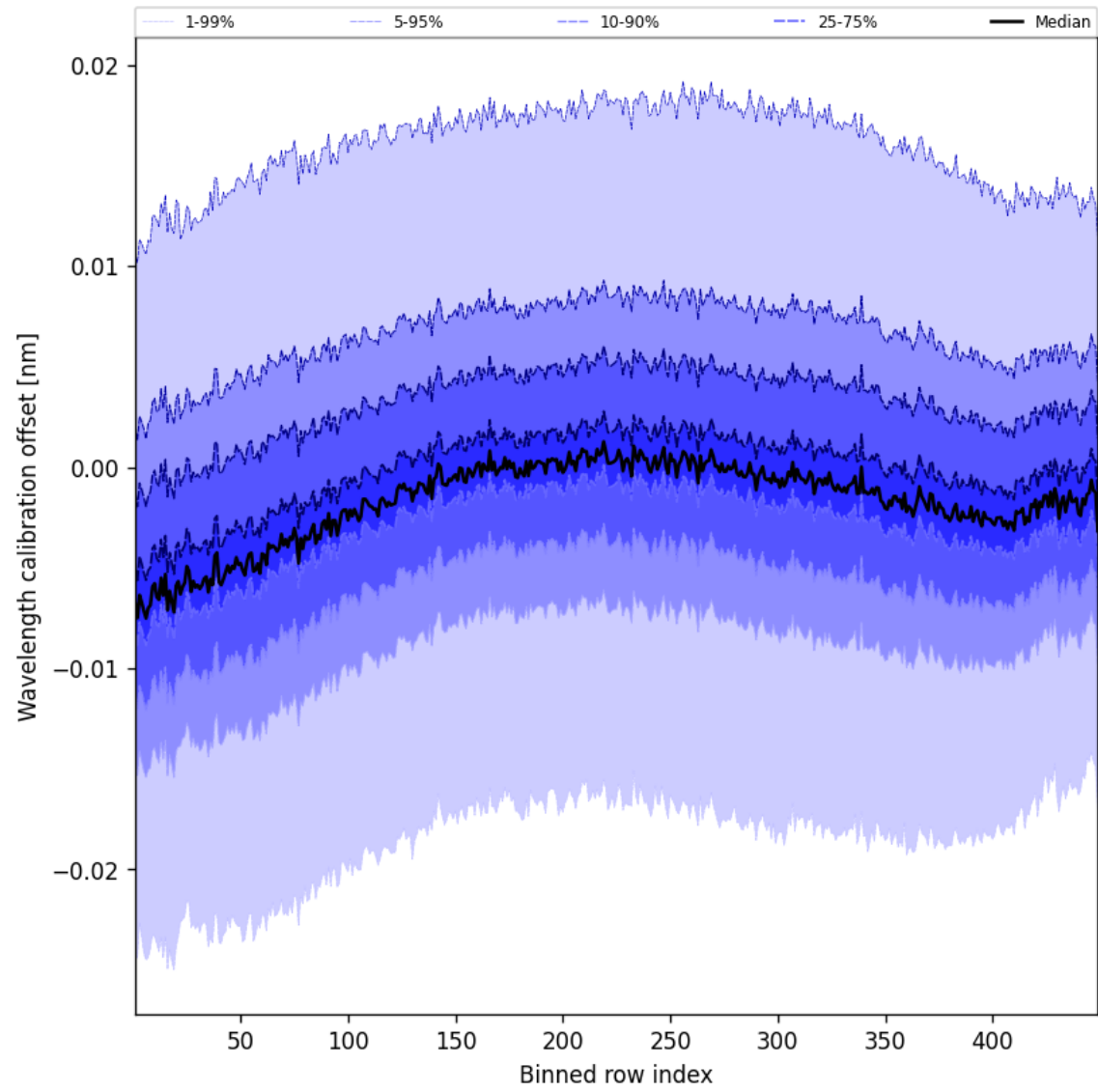
Figure 52: Along track statistics of “Wavelength calibration offset” for 2025-11-28 to 2025-11-29
