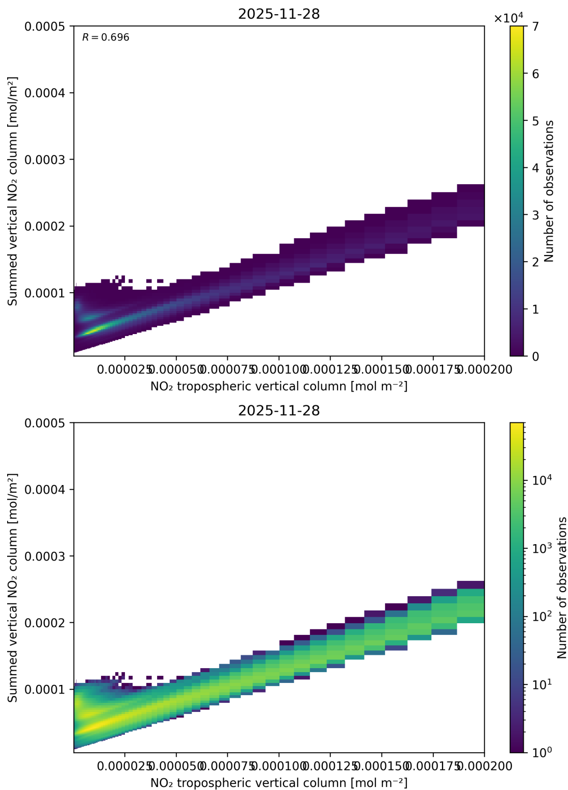
Figure 126: Scatter density plot of “NO 2 tropospheric vertical column” against “Summed vertical NO 2 column” for 2025-11-28 to 2025-11-29.
