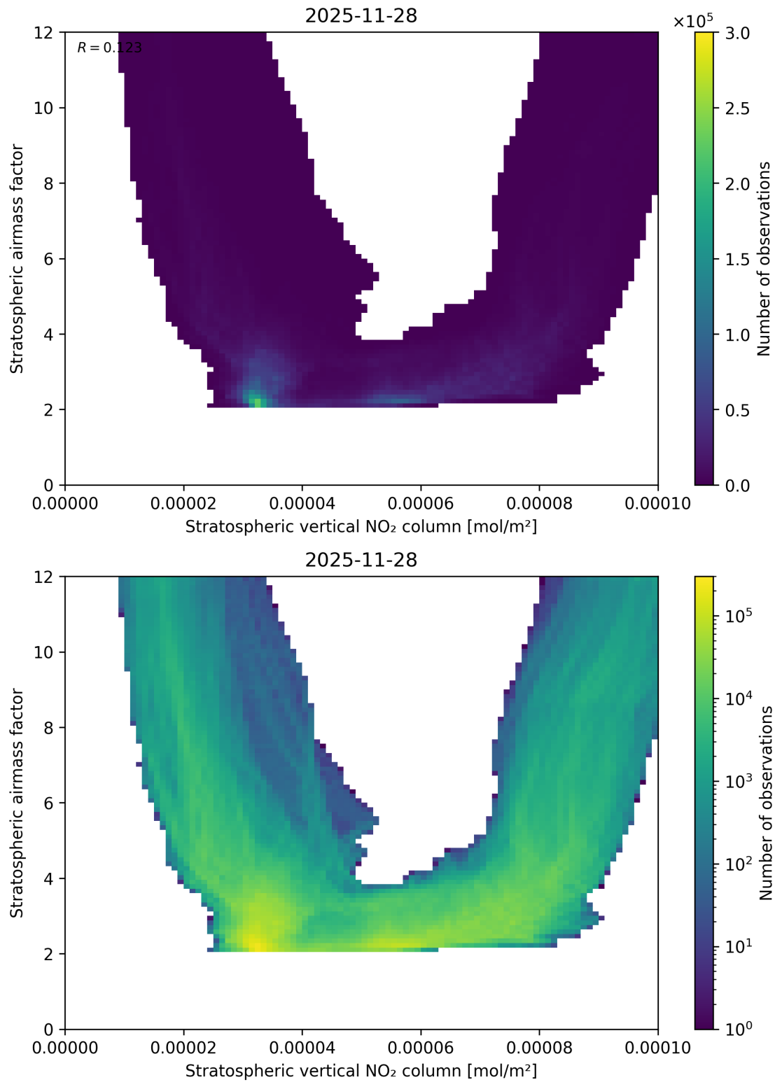
Figure 96: Scatter density plot of “Stratospheric vertical NO 2 column” against “Stratospheric airmass factor” for 2025-11-28 to 2025-11-29.
