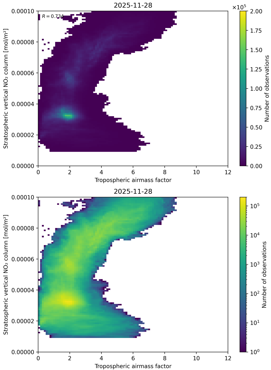
Figure 74: Scatter density plot of “Tropospheric airmass factor” against “Stratospheric vertical NO 2 column” for 2025-11-28 to 2025-11-29.
