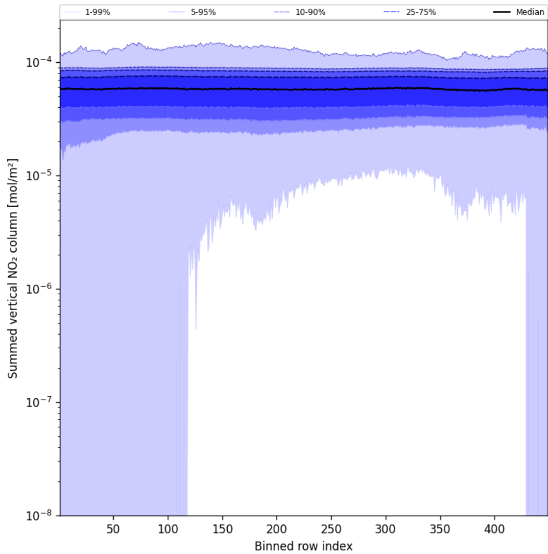
Figure 57: Along track statistics of “Summed vertical NO 2 column” for 2025-11-28 to 2025-11-29
