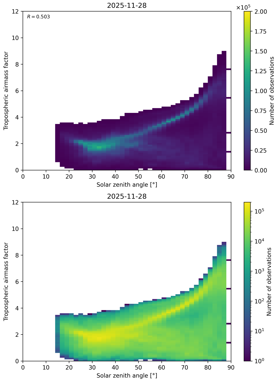
Figure 147: Scatter density plot of “Solar zenith angle” against “Tropospheric airmass factor” for 2025-11-28 to 2025-11-29.
