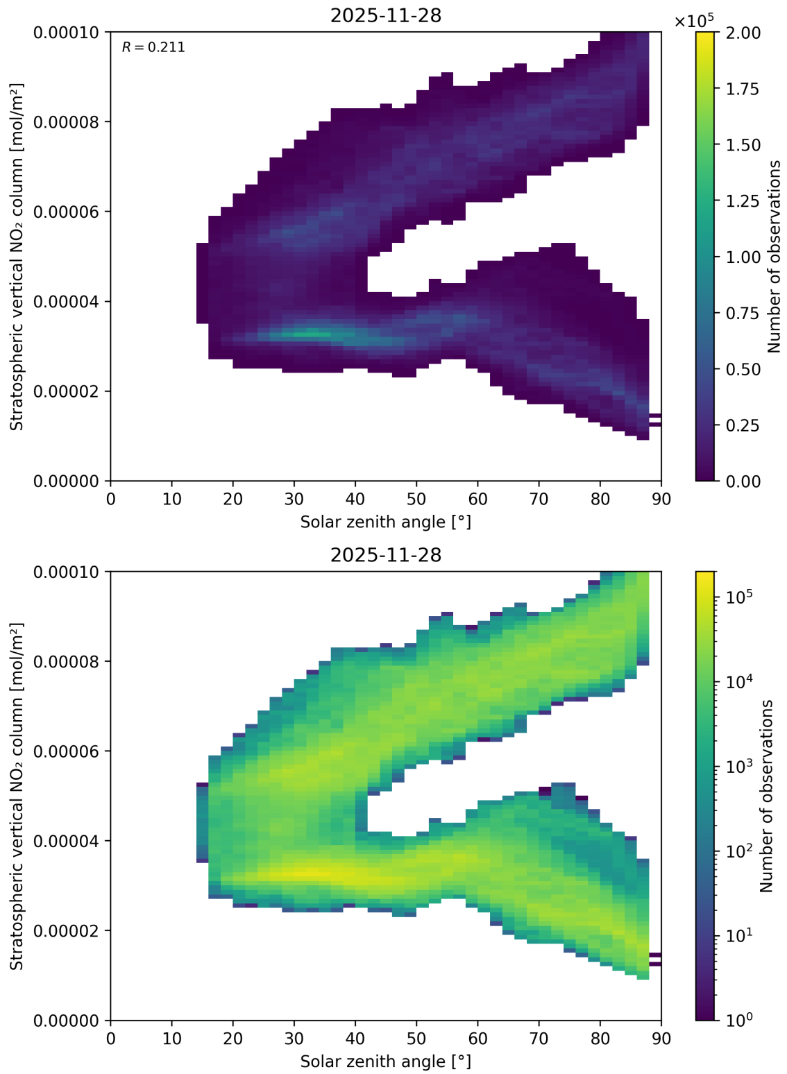
Figure 150: Scatter density plot of “Solar zenith angle” against “Stratospheric vertical NO 2 column” for 2025-11-28 to 2025-11-29.
