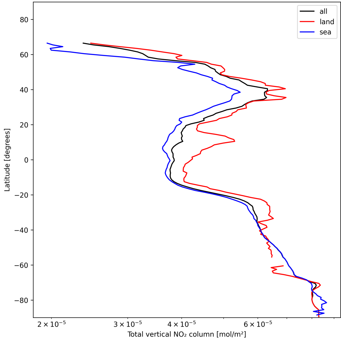
Figure 21: Zonal average of “Total vertical NO 2 column” for 2025-11-28 to 2025-11-29.
