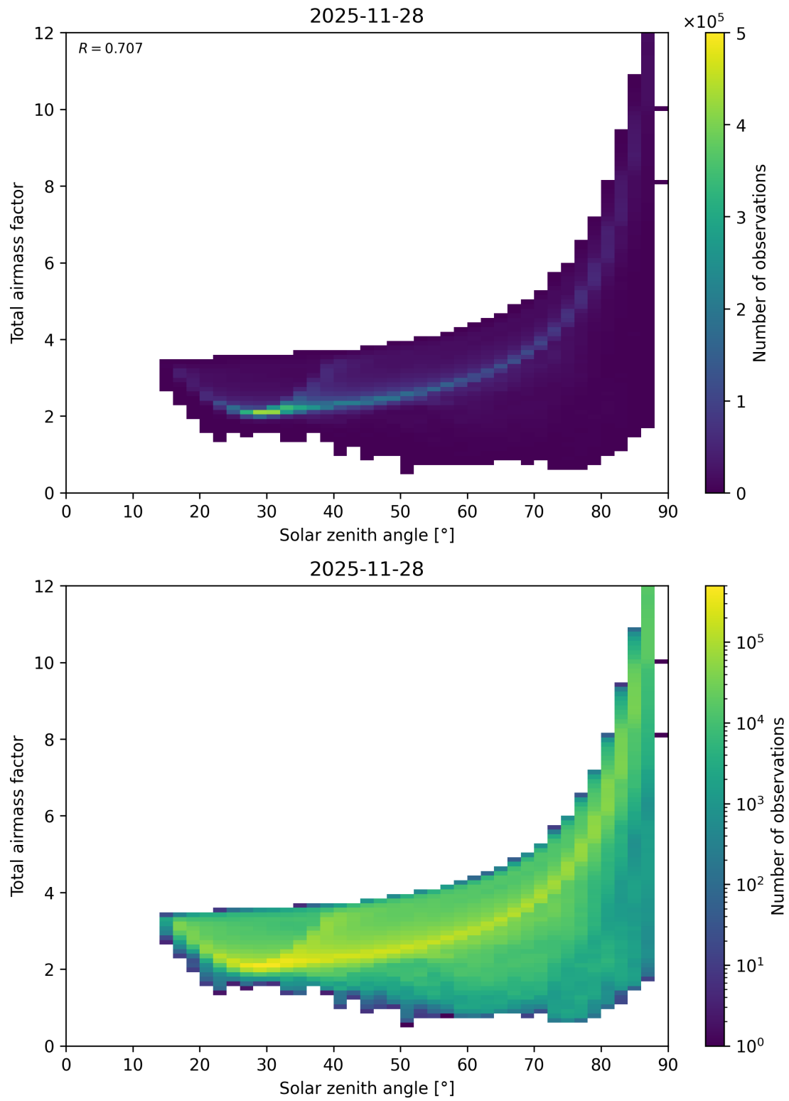
Figure 146: Scatter density plot of “Solar zenith angle” against “Total airmass factor” for 2025-11-28 to 2025-11-29.
