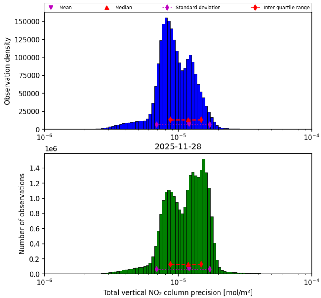
Figure 39: Histogram of “Total vertical NO 2 column precision” for 2025-11-28 to 2025-11-29
