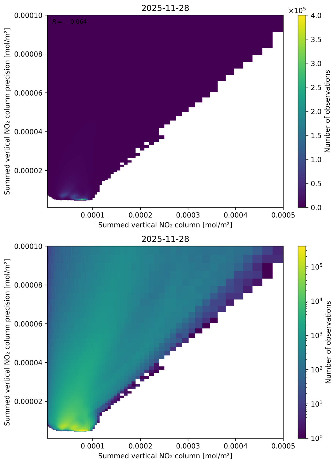
Figure 105: Scatter density plot of “Summed vertical NO 2 column” against “Summed vertical NO 2 column precision” for 2025-11-28 to 2025-11-29.
