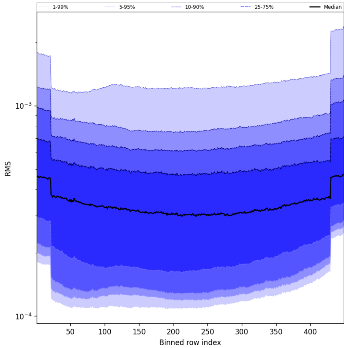
Figure 60: Along track statistics of “RMS” for 2025-11-28 to 2025-11-29
