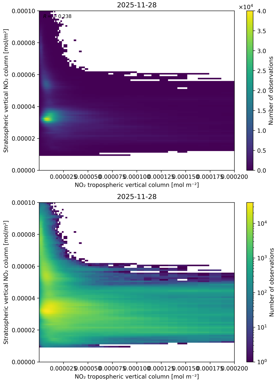
Figure 125: Scatter density plot of “NO 2 tropospheric vertical column” against “Stratospheric vertical NO 2 column” for 2025-11-28 to 2025-11-29.
