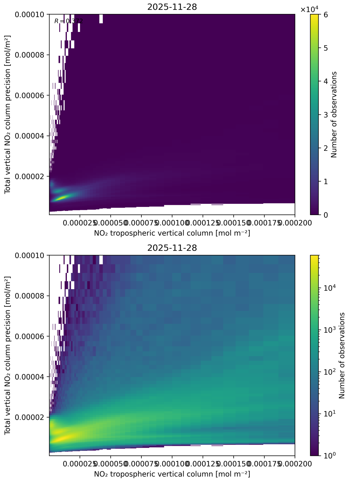
Figure 129: Scatter density plot of “NO 2 tropospheric vertical column” against “Total vertical NO 2 column precision” for 2025-11-28 to 2025-11-29.
