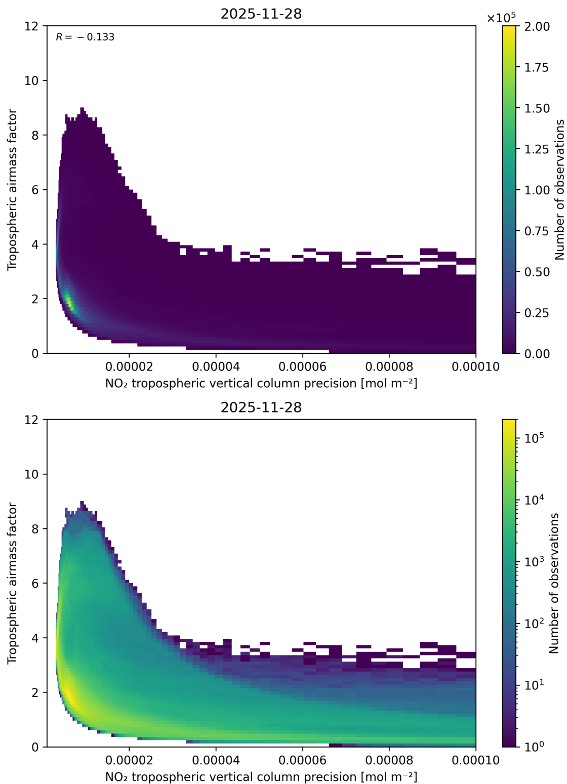
Figure 133: Scatter density plot of “NO 2 tropospheric vertical column precision” against “Tropospheric airmass factor” for 2025-11-28 to 2025-11-29.
