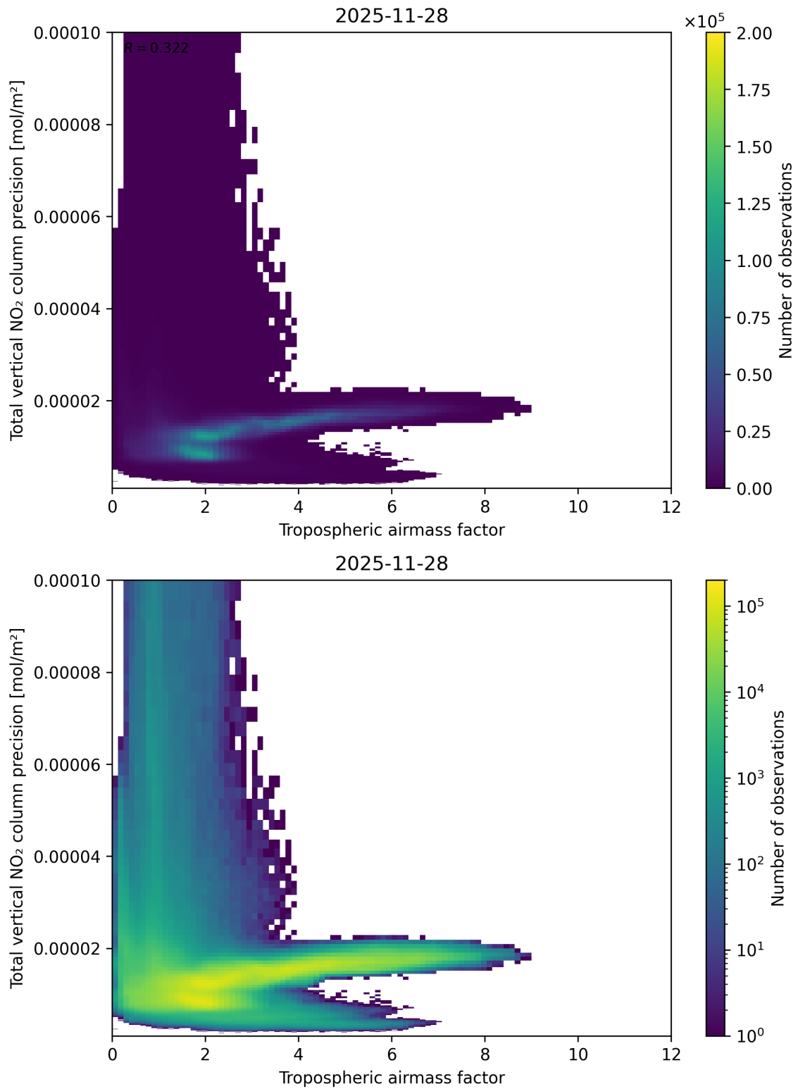
Figure 78: Scatter density plot of “Tropospheric air mass factor” against “Total vertical NO 2 column precision” for 2025-11-28 to 2025-11-29.
