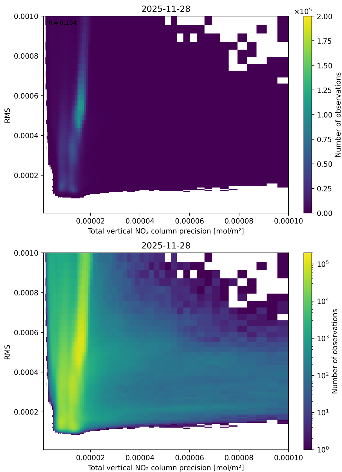
Figure 119: Scatter density plot of “Total vertical NO 2 column precision” against “RMS” for 2025-11-28 to 2025-11-29.
