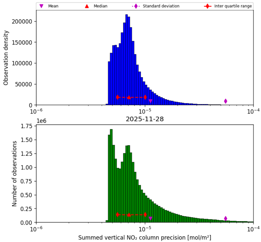
Figure 41: Histogram of “Summed vertical NO 2 column precision” for 2025-11-28 to 2025-11-29
