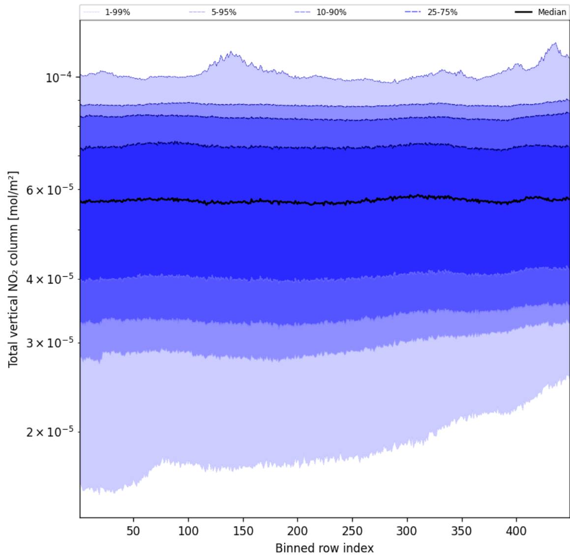
Figure 55: Along track statistics of “Total vertical NO 2 column” for 2025-11-28 to 2025-11-29
