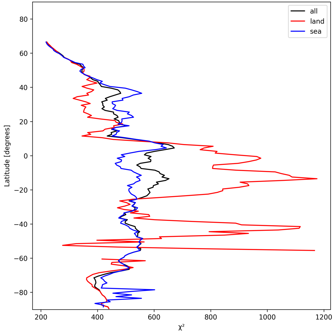
Figure 25: Zonal average of “ \chi^2 ” for 2025-11-28 to 2025-11-29.
