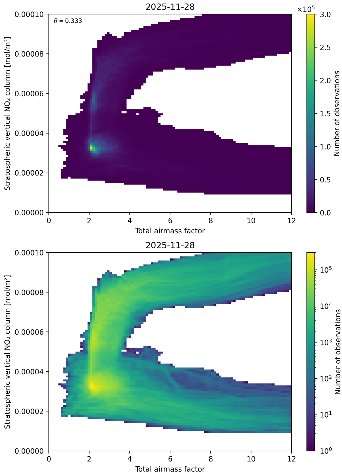
Figure 64: Scatter density plot of “Total airmass factor” against “Stratospheric vertical NO 2 column” for 2025-11-28 to 2025-11-29.
