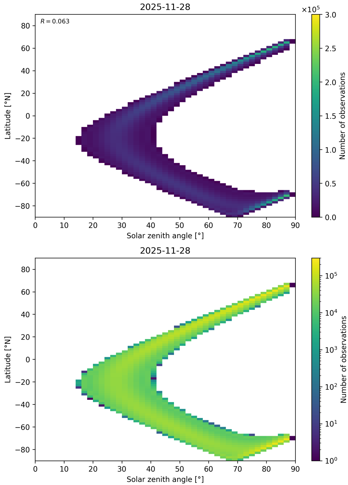
Figure 149: Scatter density plot of “Solar zenith angle” against “Latitude” for 2025-11-28 to 2025-11-29.
