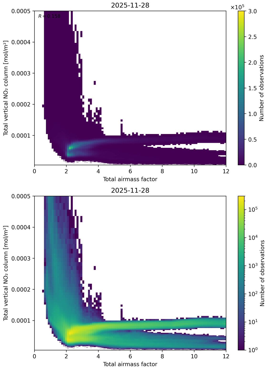
Figure 67: Scatter density plot of “Total airmass factor” against “Total vertical NO 2 column” for 2025-11-28 to 2025-11-29.
