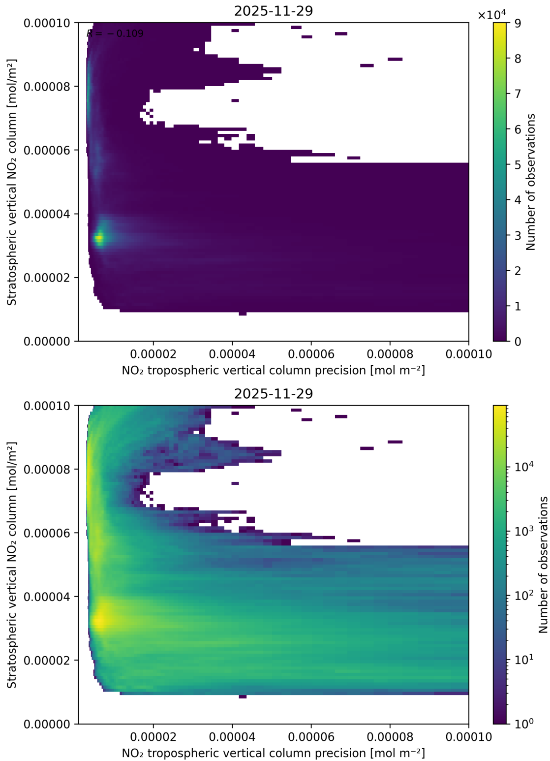
Figure 135: Scatter density plot of “NO 2 tropospheric vertical column precision” against “Stratospheric vertical NO 2 column” for 2025-11-28 to 2025-11-30.
