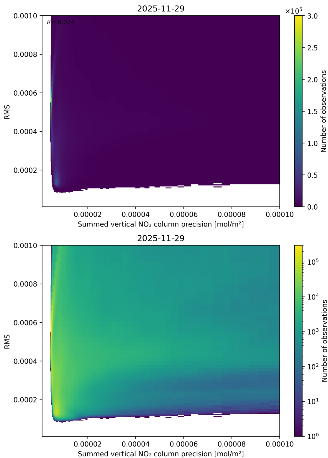
Figure 108: Scatter density plot of “Summed vertical NO 2 column precision” against “RMS” for 2025-11-28 to 2025-11-30.
