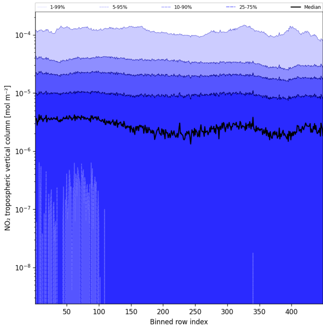
Figure 46: Along track statistics of “NO 2 tropospheric vertical column” for 2025-11-28 to 2025-11-30
