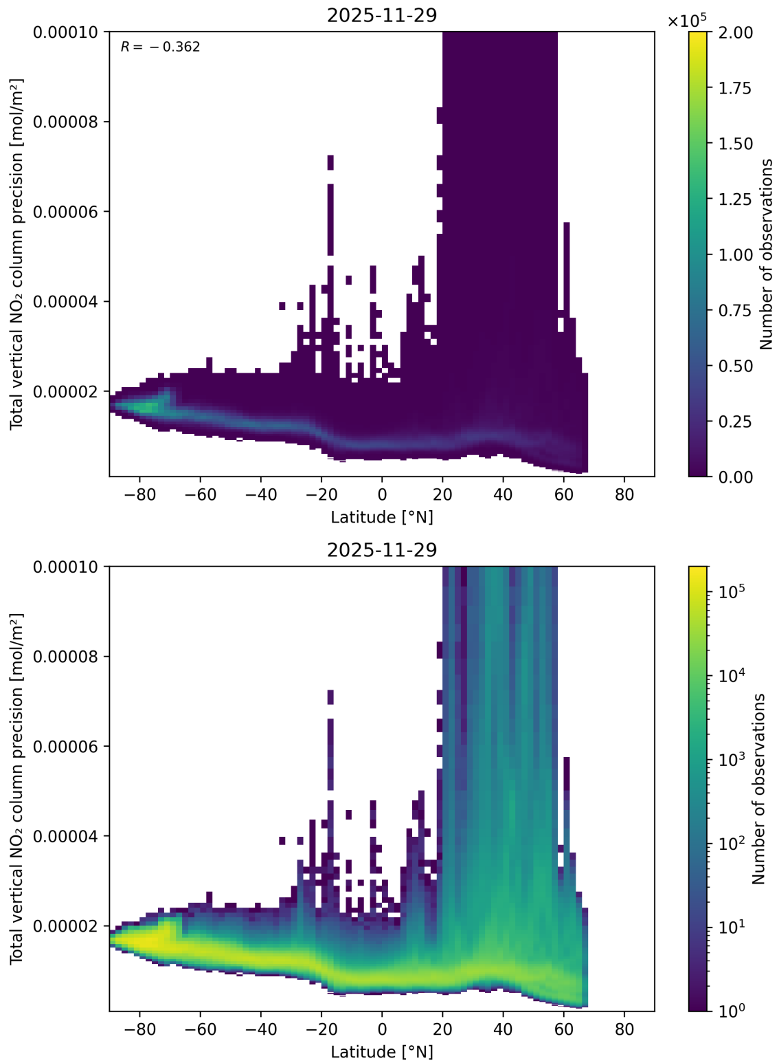
Figure 91: Scatter density plot of “Latitude” against “Total vertical NO 2 column precision” for 2025-11-28 to 2025-11-30.
