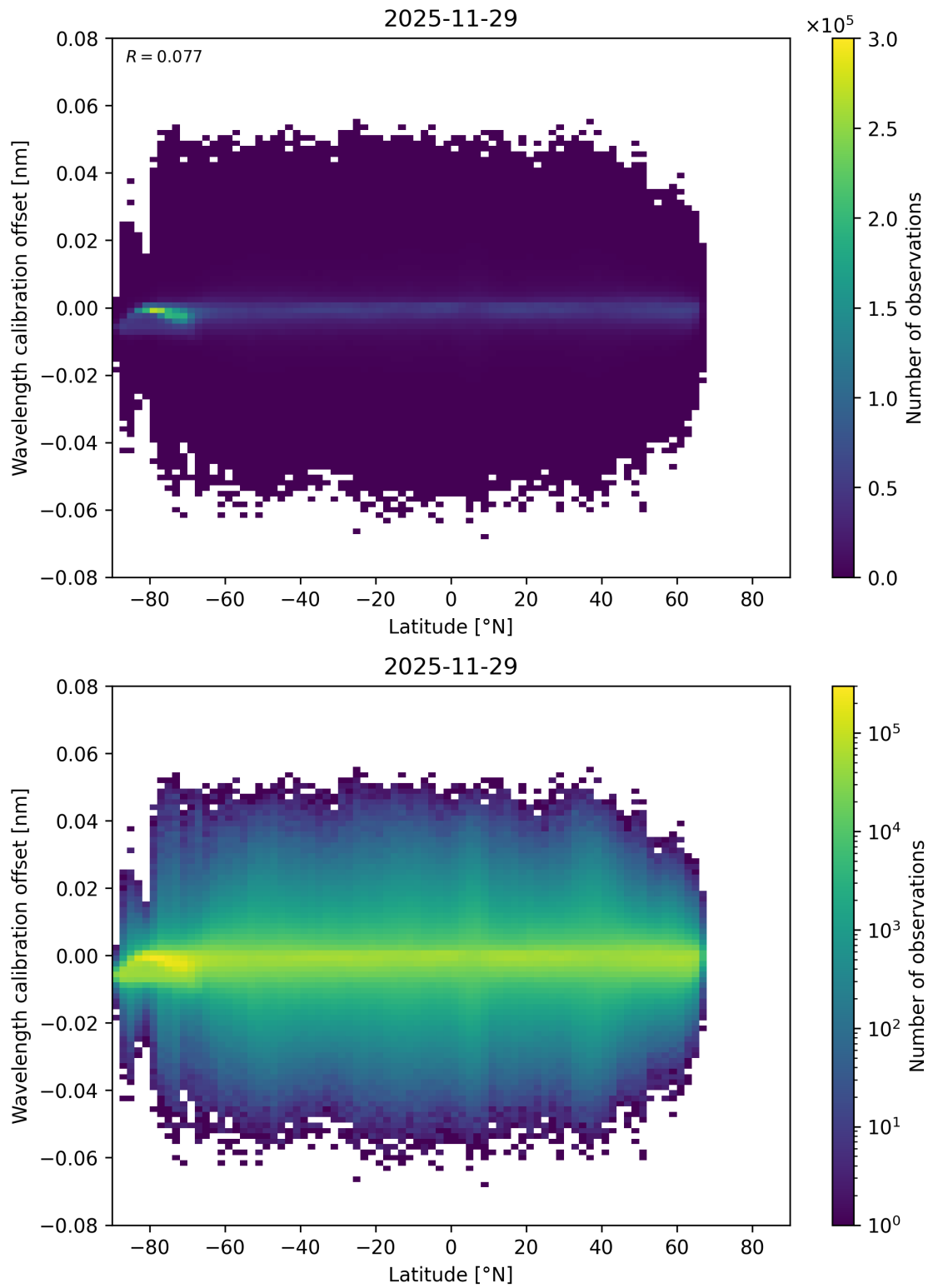
Figure 95: Scatter density plot of “Latitude” against “Wavelength calibration offset” for 2025-11-28 to 2025-11-30.
