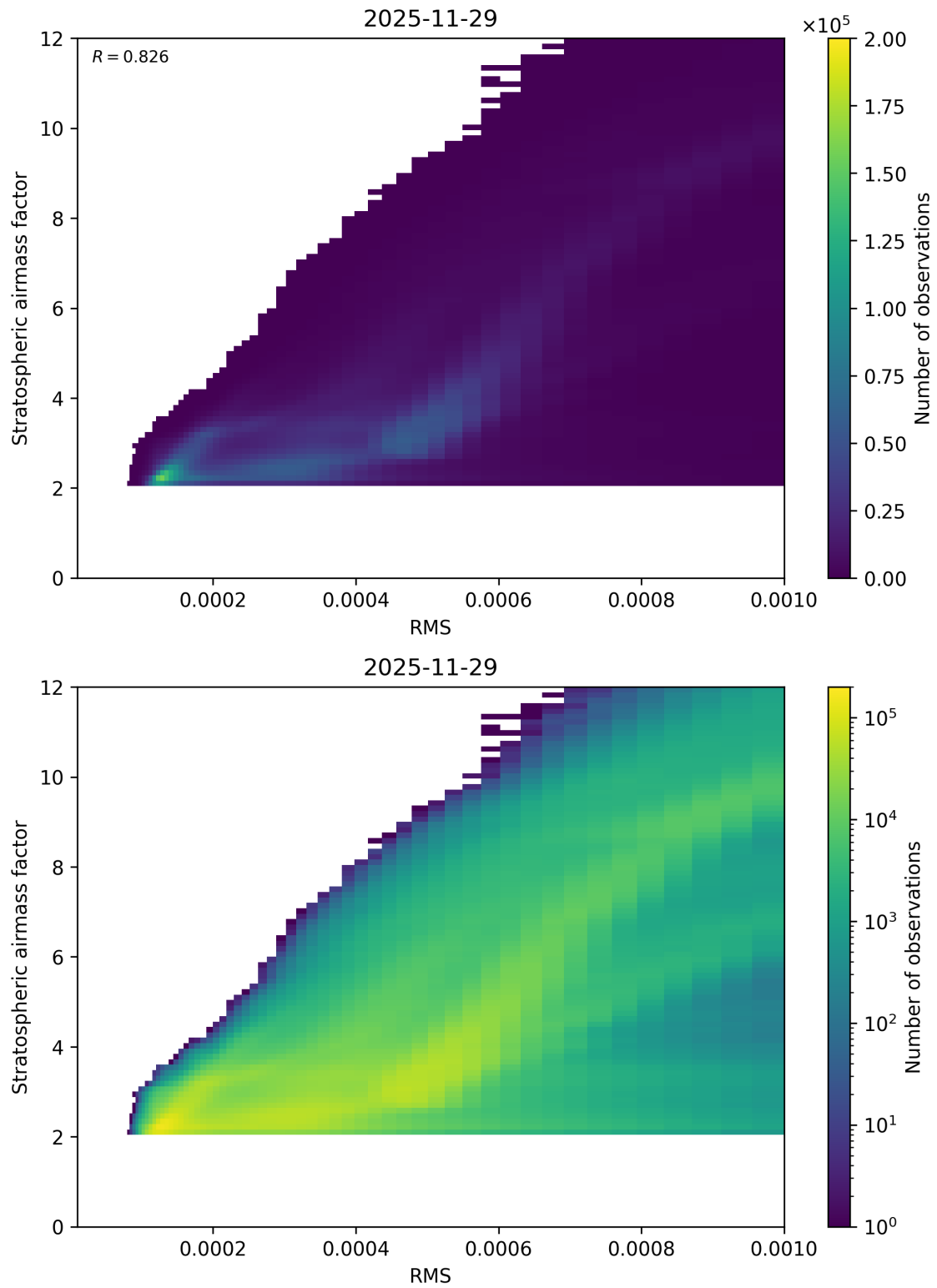
Figure 144: Scatter density plot of “RMS” against “Stratospheric airmass factor” for 2025-11-28 to 2025-11-30.
