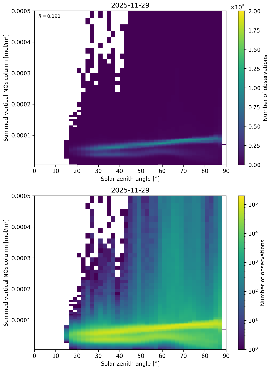
Figure 151: Scatter density plot of “Solar zenith angle” against “Summed vertical NO 2 column” for 2025-11-28 to 2025-11-30.
