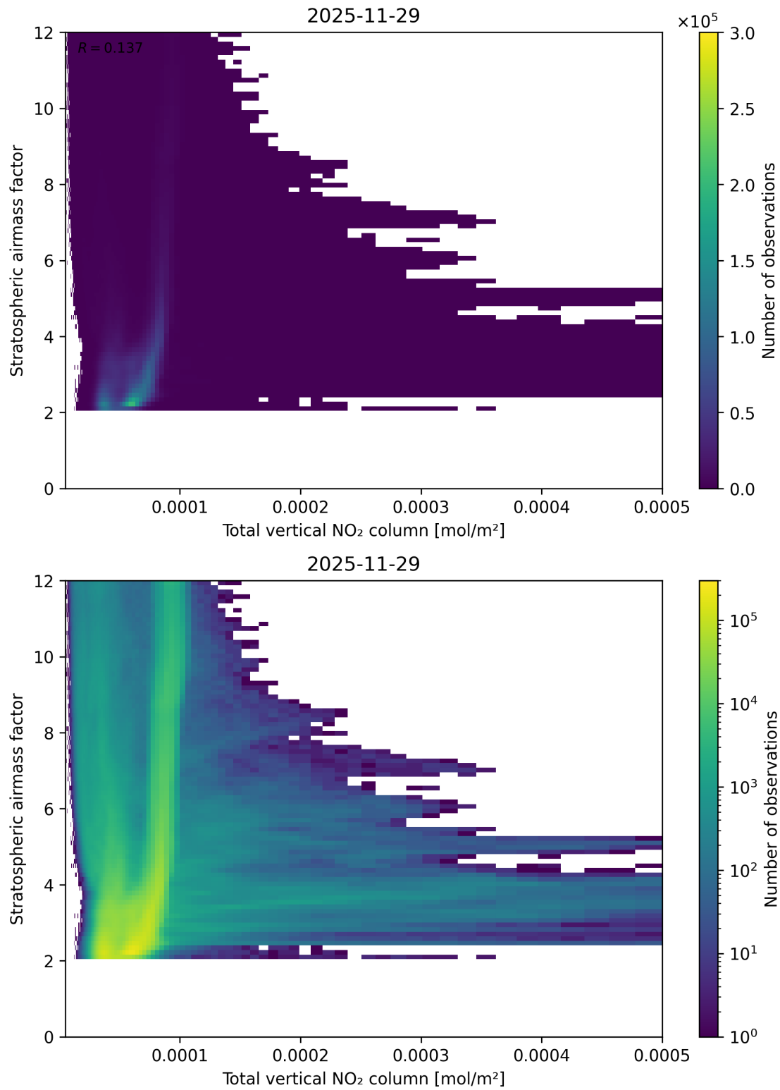
Figure 110: Scatter density plot of “Total vertical NO 2 column” against “Stratospheric airmass factor” for 2025-11-28 to 2025-11-30.
