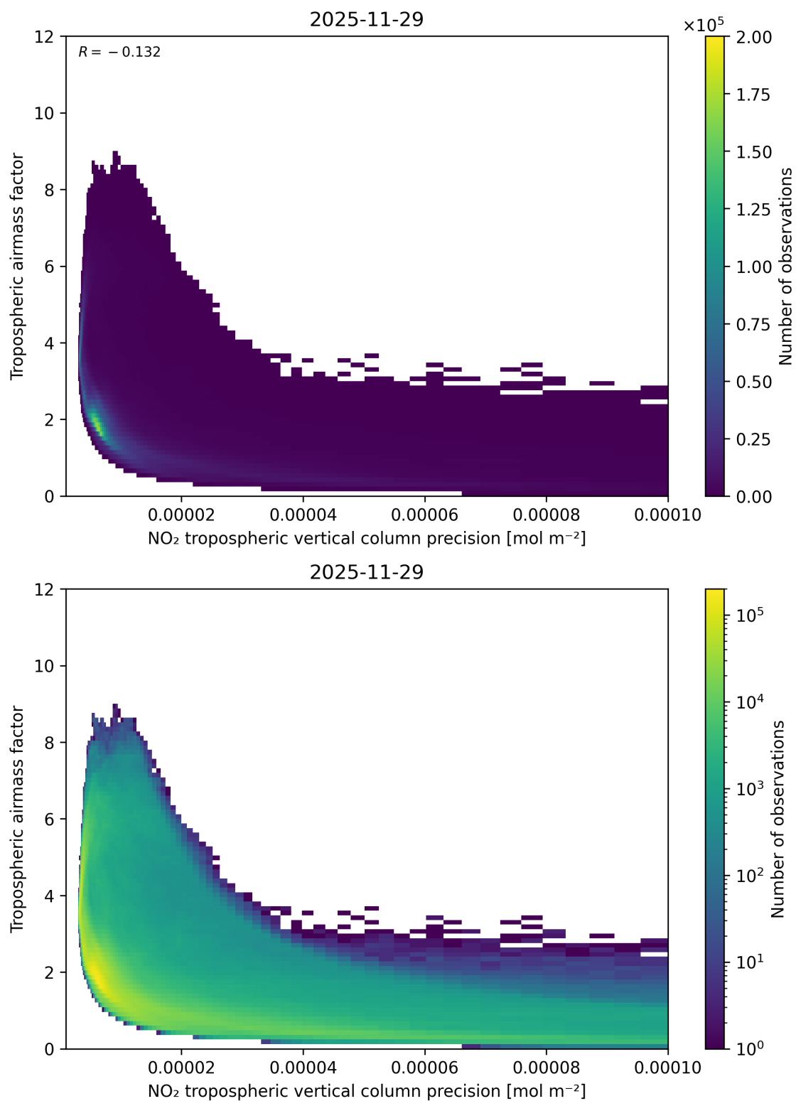
Figure 133: Scatter density plot of “NO 2 tropospheric vertical column precision” against “Tropospheric airmass factor” for 2025-11-28 to 2025-11-30.
