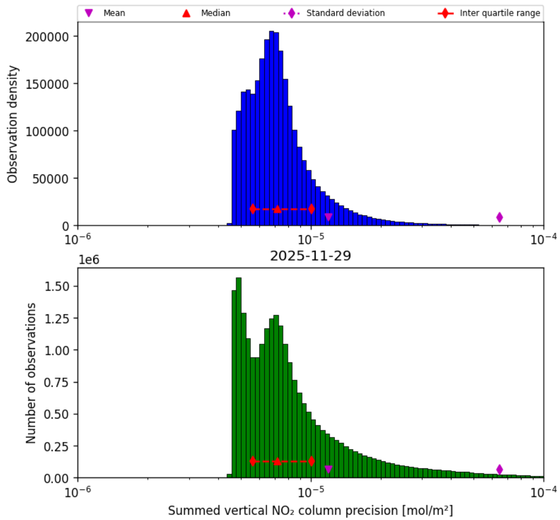
Figure 41: Histogram of "Summed vertical NO 2 column precision" for 2025-11-28 to 2025-11-30
