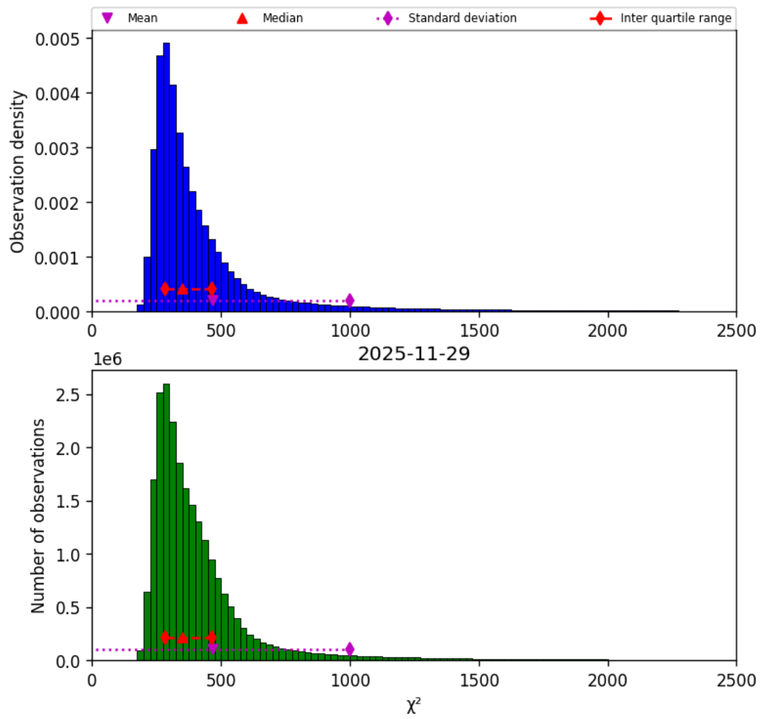
Figure 42: Histogram of “ \chi^2 ” for 2025-11-28 to 2025-11-30
