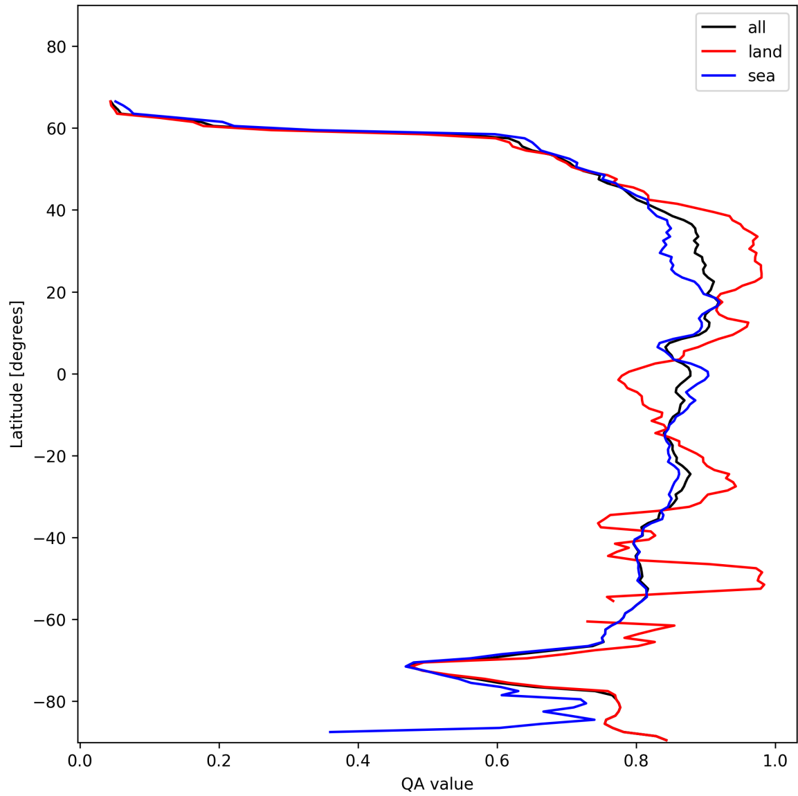
Figure 11: Zonal average of “QA value” for 2025-11-28 to 2025-11-30.
