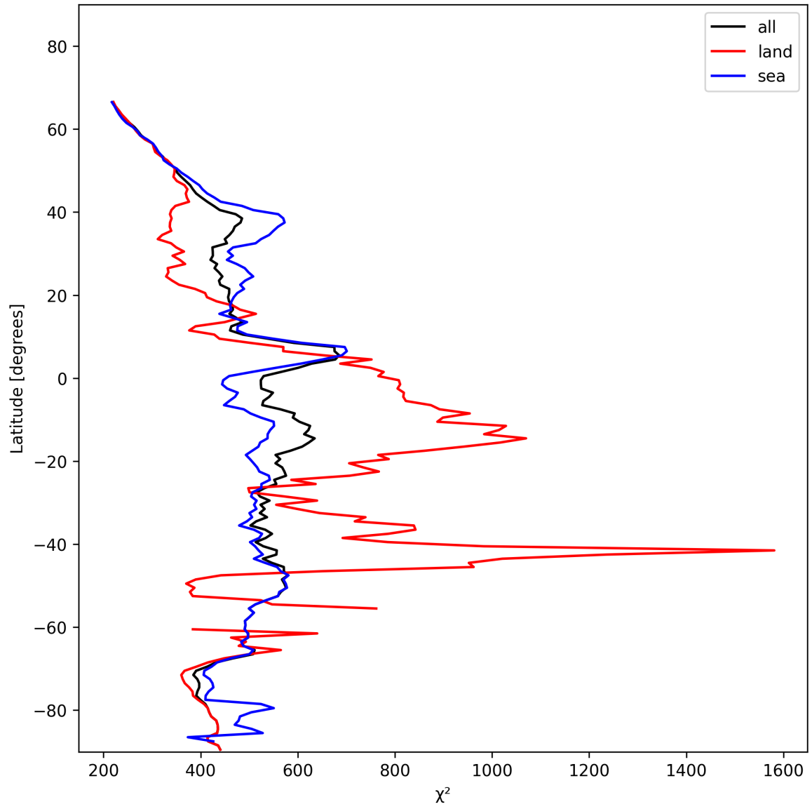
Figure 25: Zonal average of “ \chi^2 ” for 2025-11-28 to 2025-11-30.
