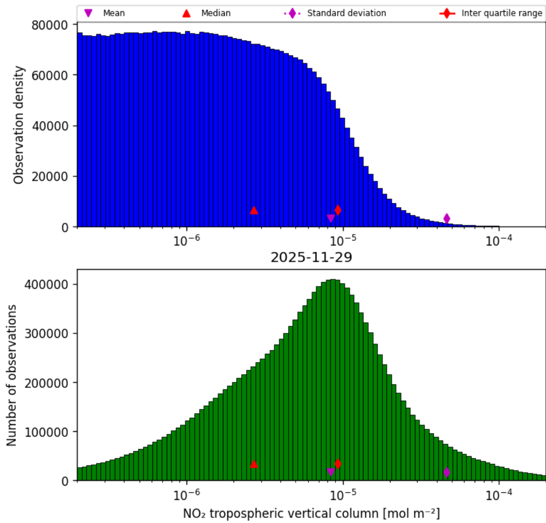
Figure 29: Histogram of “NO 2 tropospheric vertical column” for 2025-11-28 to 2025-11-30
