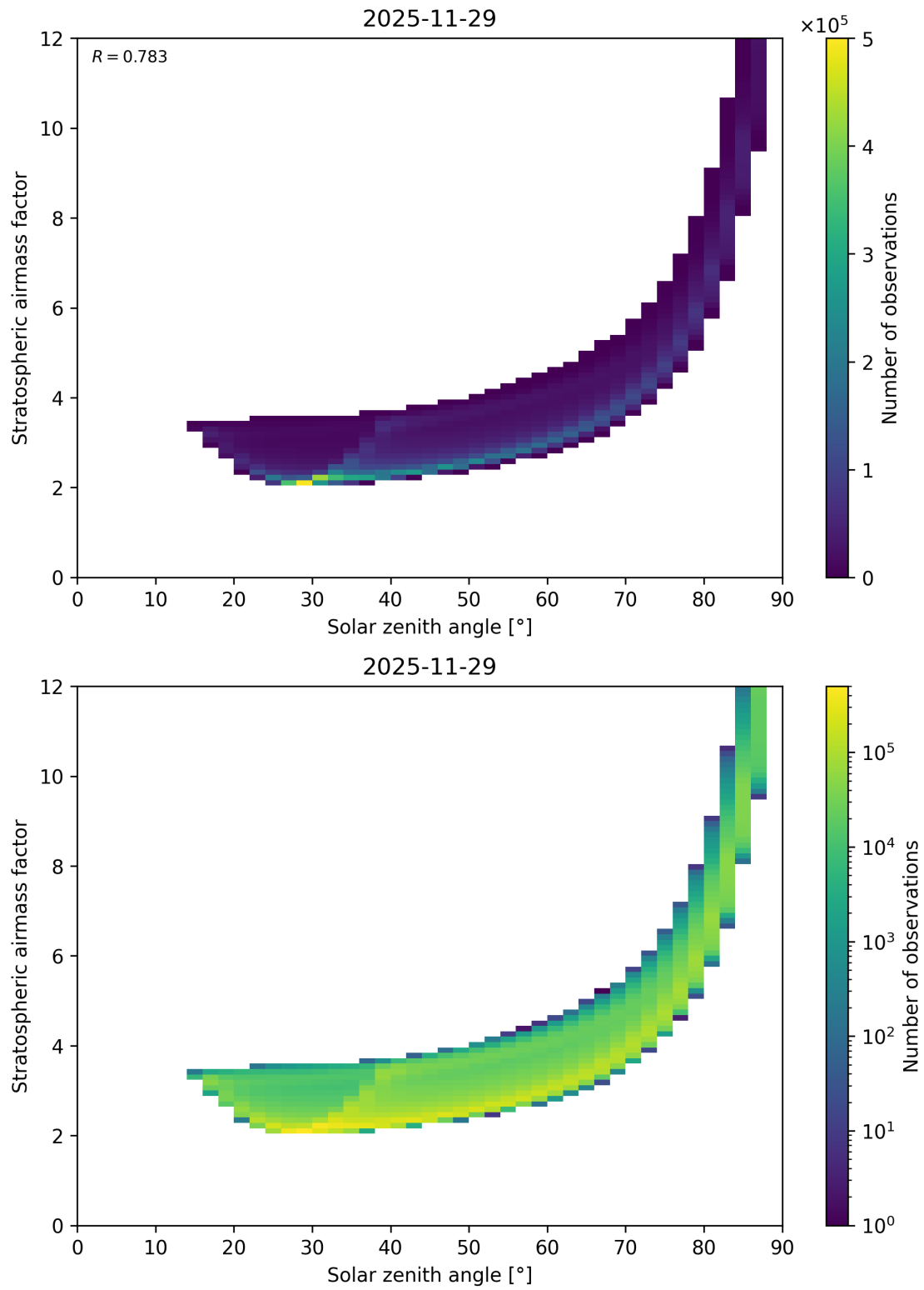
Figure 145: Scatter density plot of “Solar zenith angle” against “Stratospheric airmass factor” for 2025-11-28 to 2025-11-30.
