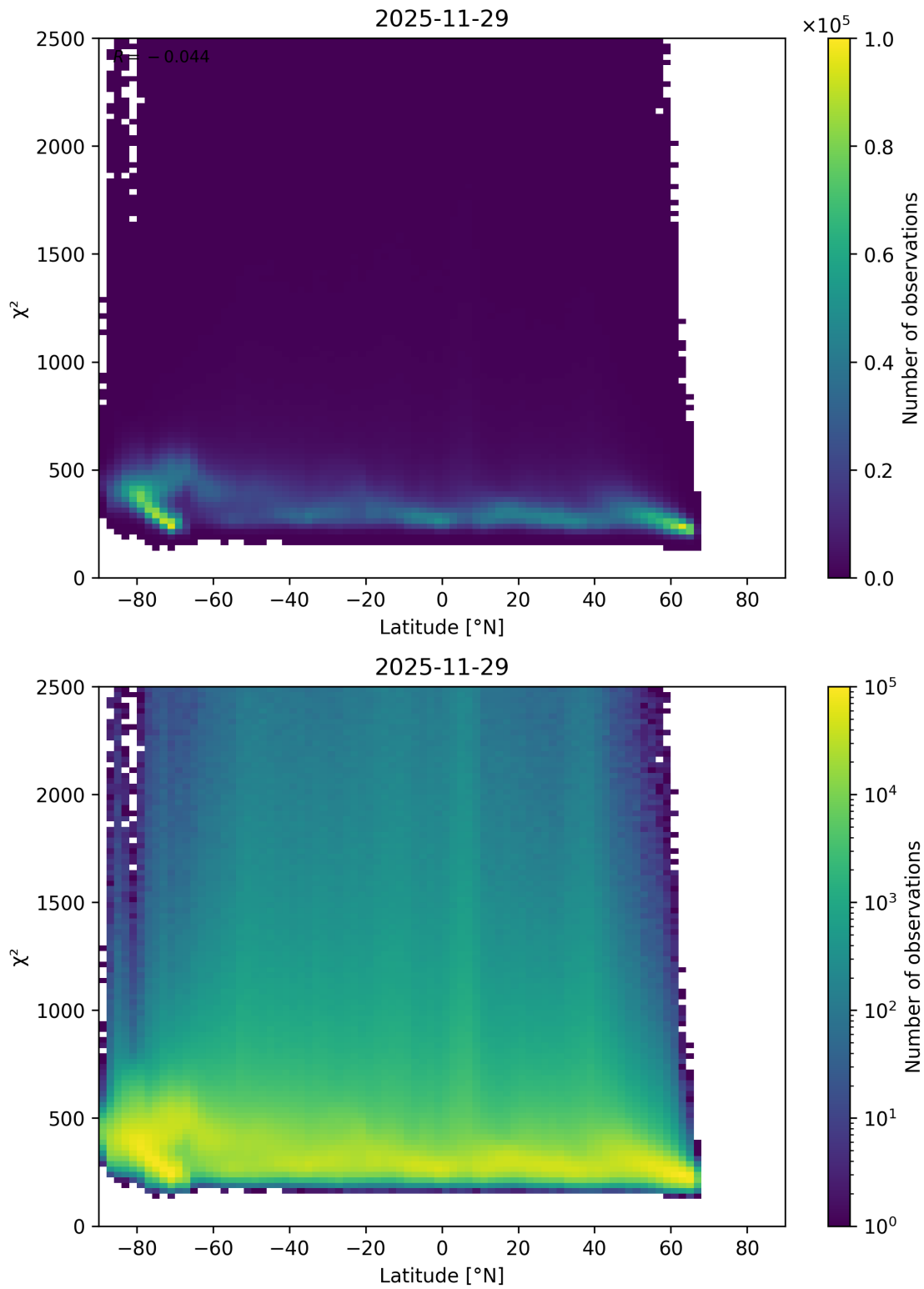
Figure 86: Scatter density plot of “Latitude” against “ \chi^2 ” for 2025-11-28 to 2025-11-30.
