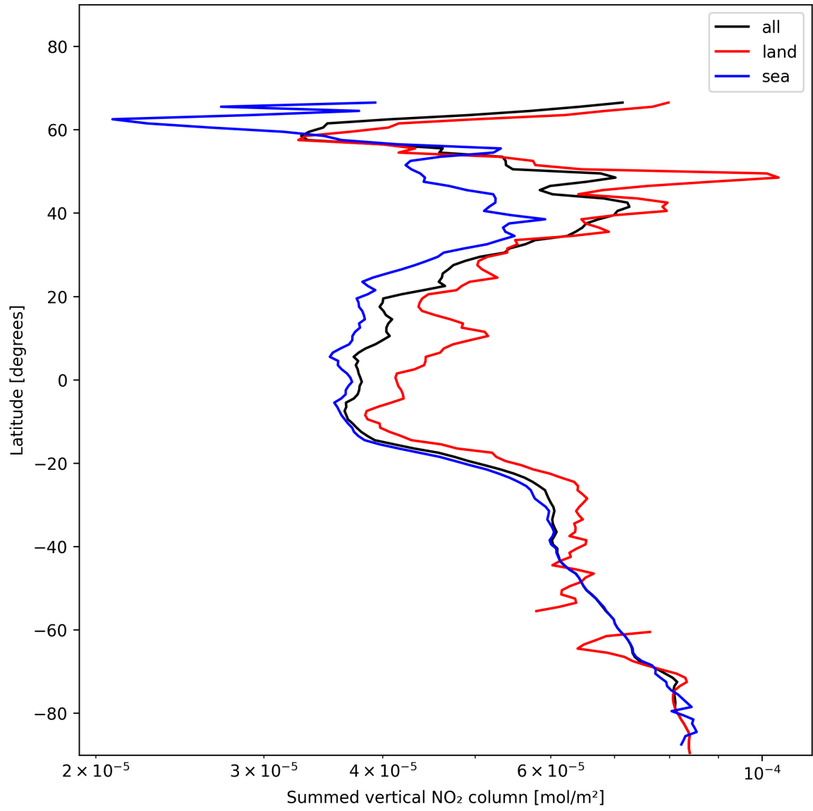
Figure 23: Zonal average of “Summed vertical NO 2 column” for 2025-11-28 to 2025-11-30.
