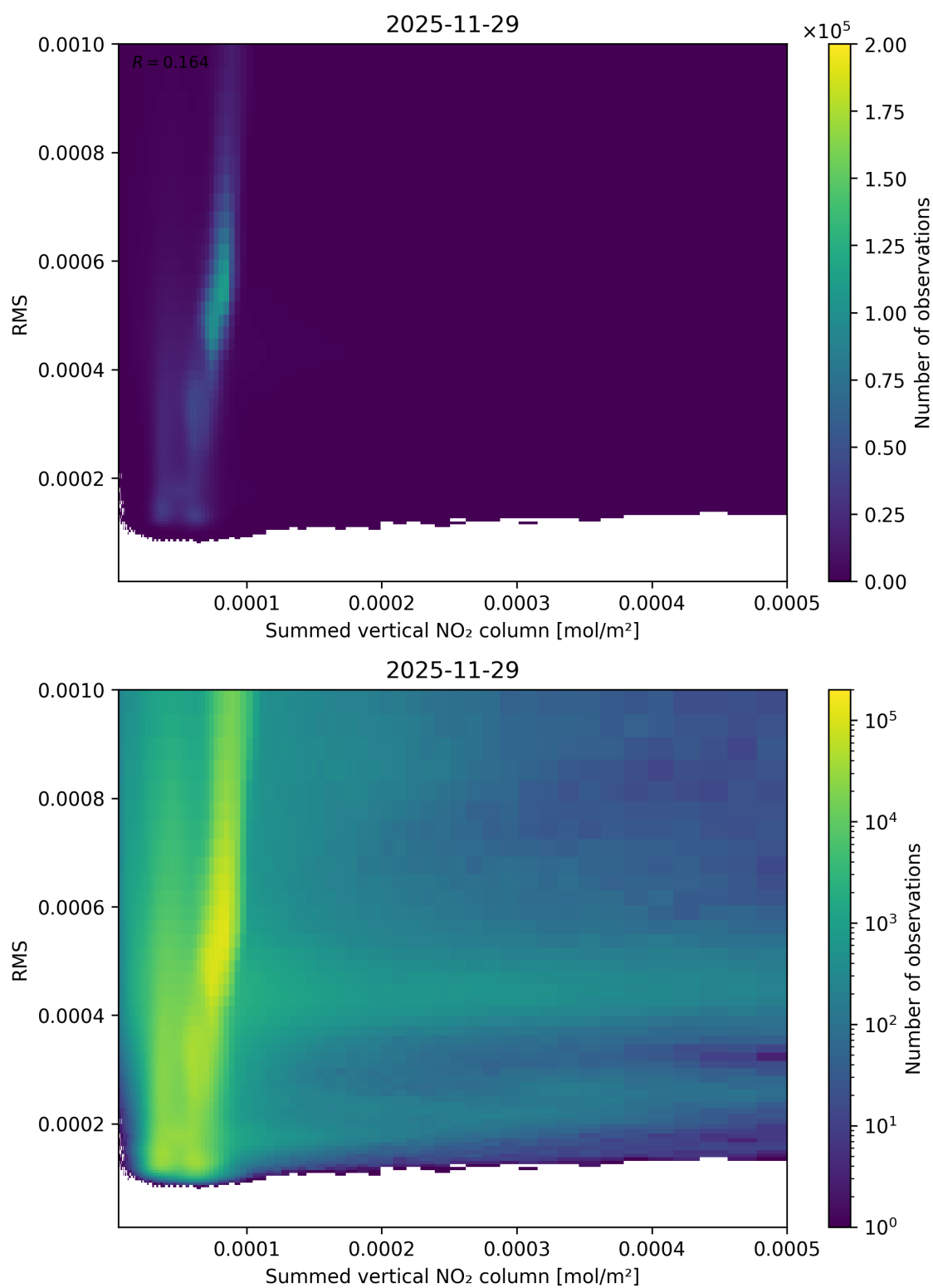
Figure 109: Scatter density plot of “Summed vertical NO 2 column” against “RMS” for 2025-11-28 to 2025-11-30.
