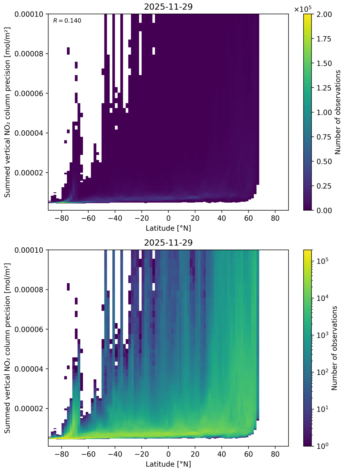
Figure 89: Scatter density plot of “Latitude” against “Summed vertical NO 2 column precision” for 2025-11-28 to 2025-11-30.
