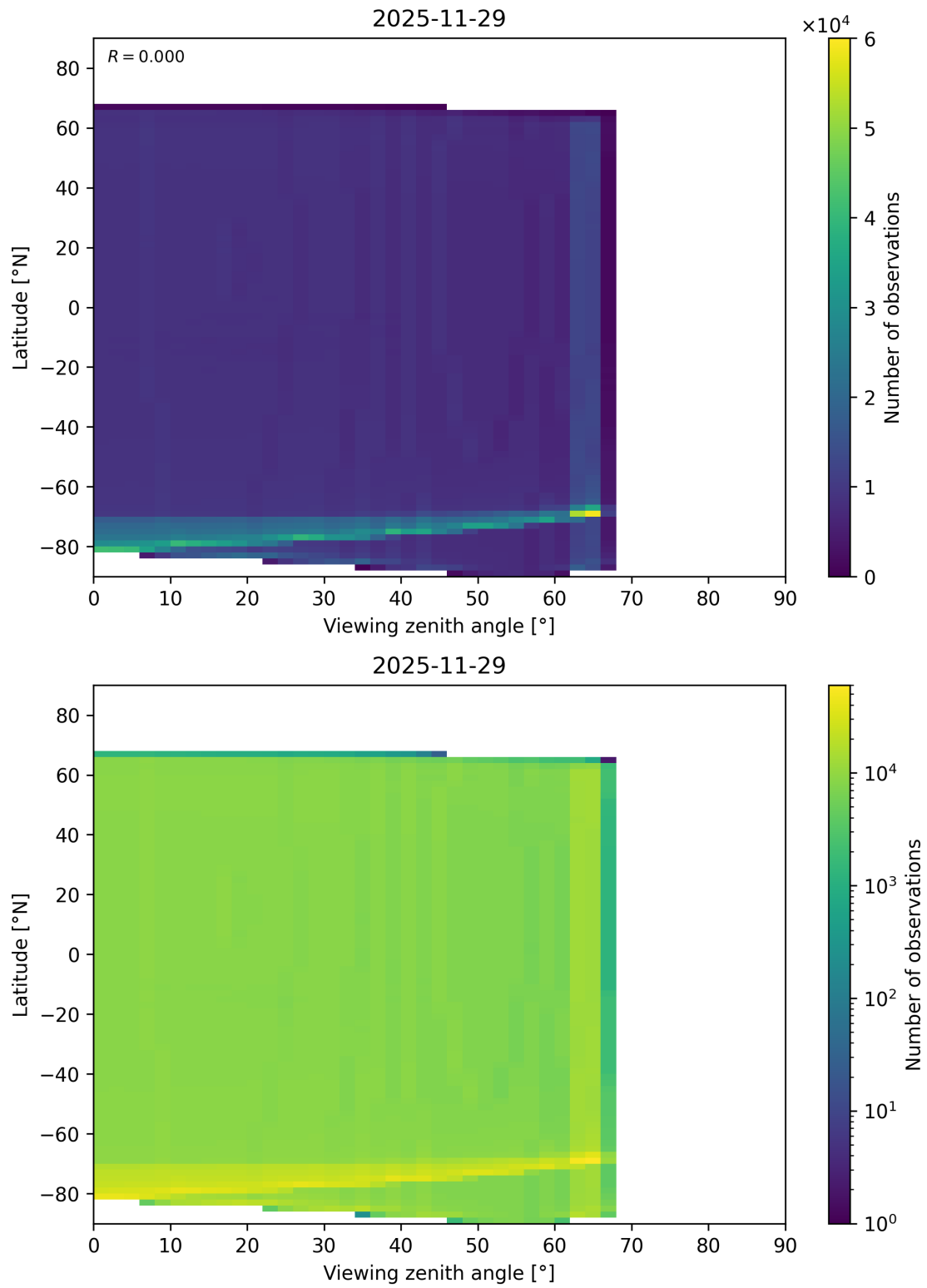
Figure 163: Scatter density plot of “Viewing zenith angle” against “Latitude” for 2025-11-28 to 2025-11-30.
