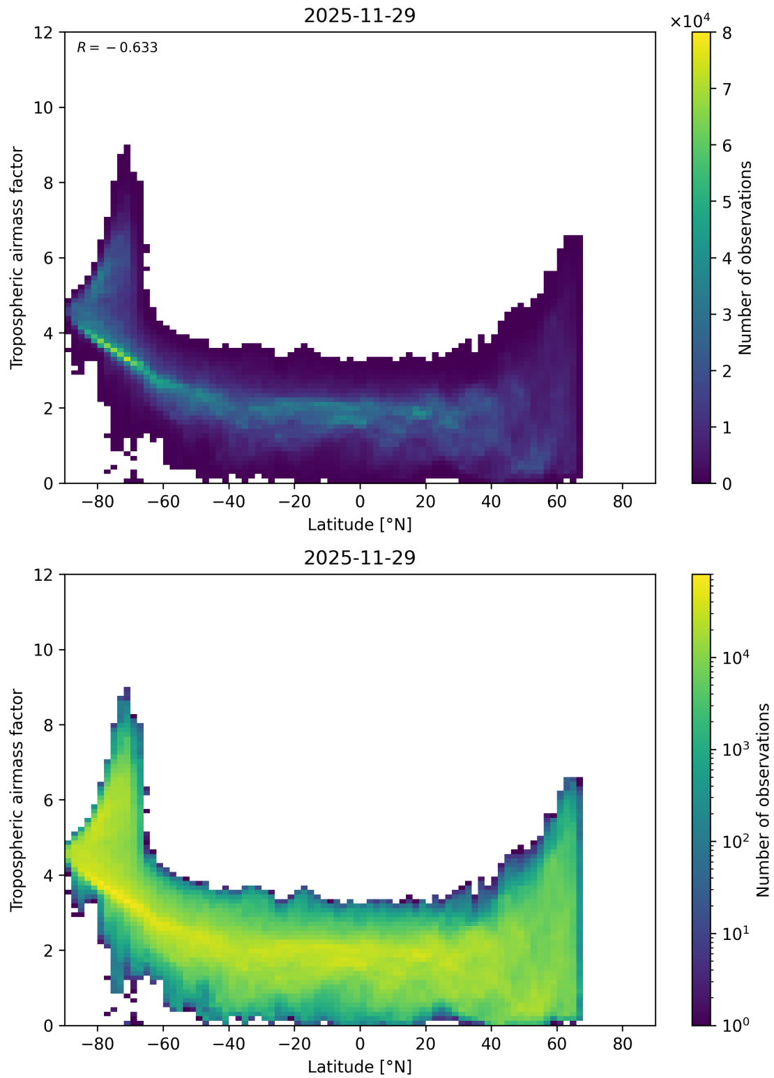
Figure 85: Scatter density plot of “Latitude” against “Tropospheric airmass factor” for 2025-11-28 to 2025-11-30.
