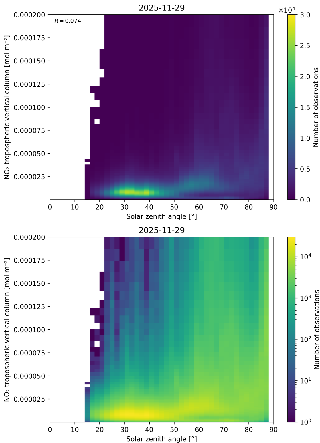
Figure 155: Scatter density plot of “Solar zenith angle” against “NO 2 tropospheric vertical column” for 2025-11-28 to 2025-11-30.
