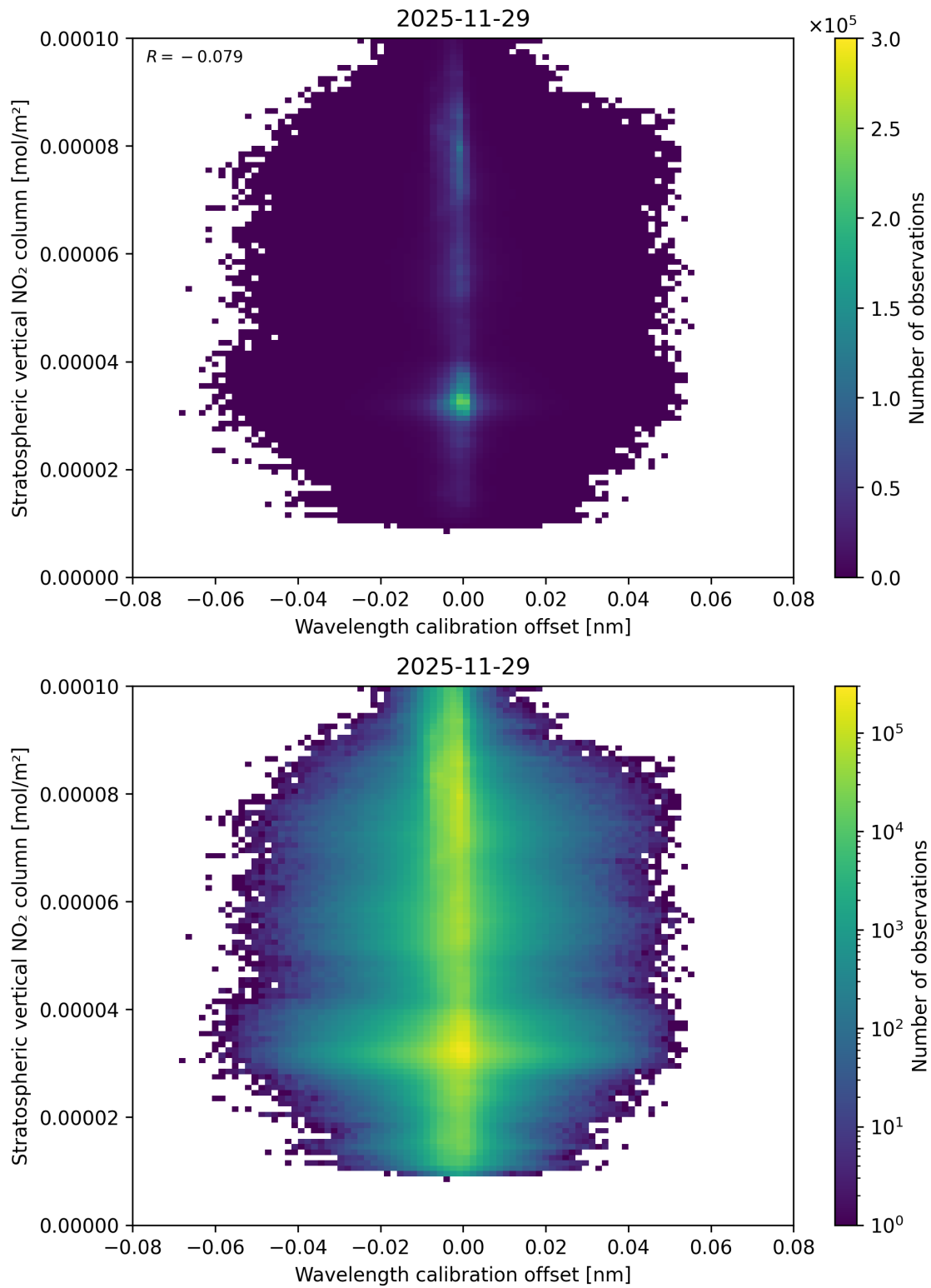
Figure 176: Scatter density plot of “Wavelength calibration offset” against “Stratospheric vertical NO 2 column” for 2025-11-28 to 2025-11-30.
