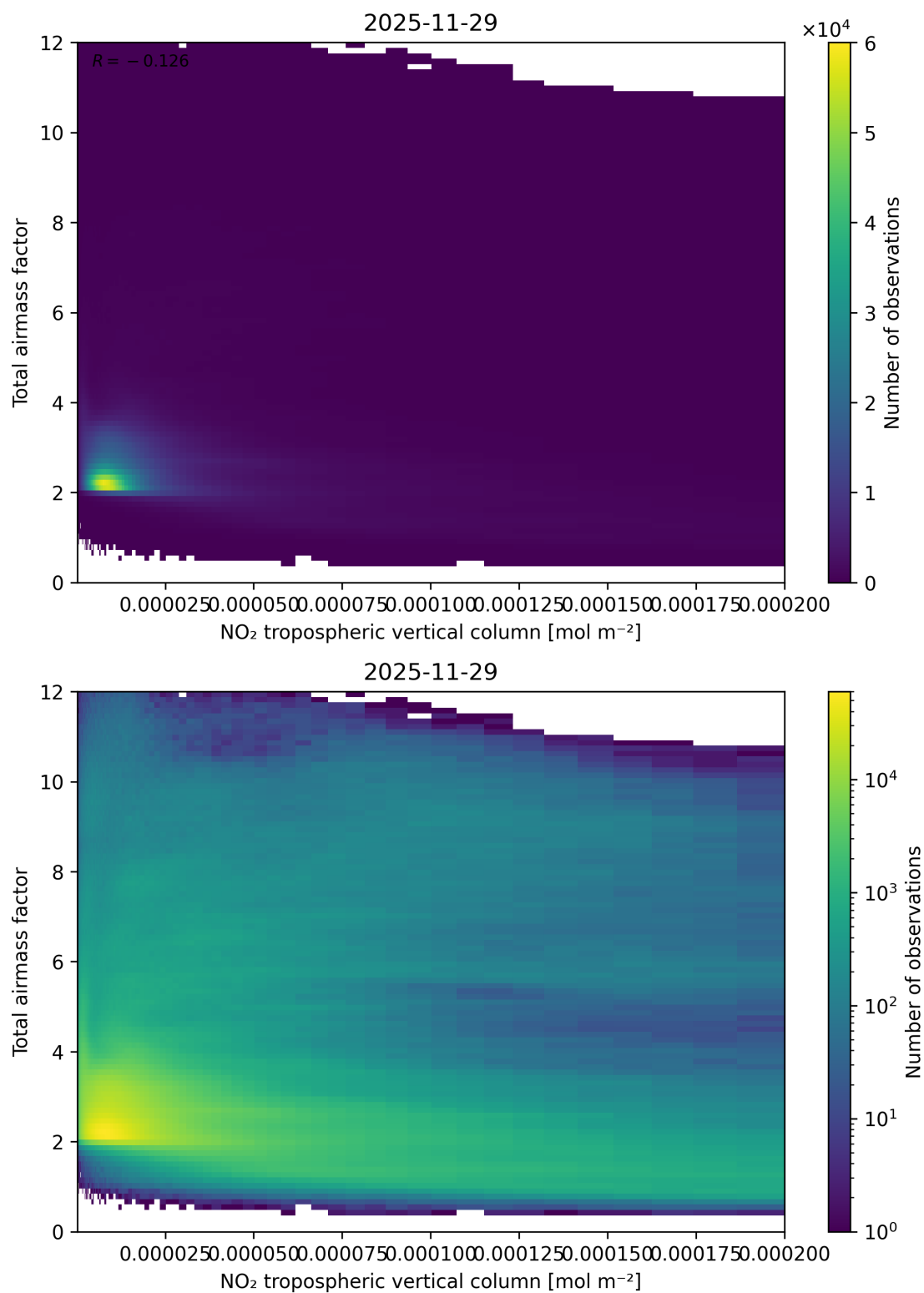
Figure 122: Scatter density plot of “NO 2 tropospheric vertical column” against “Total air mass factor” for 2025-11-28 to 2025-11-30.
