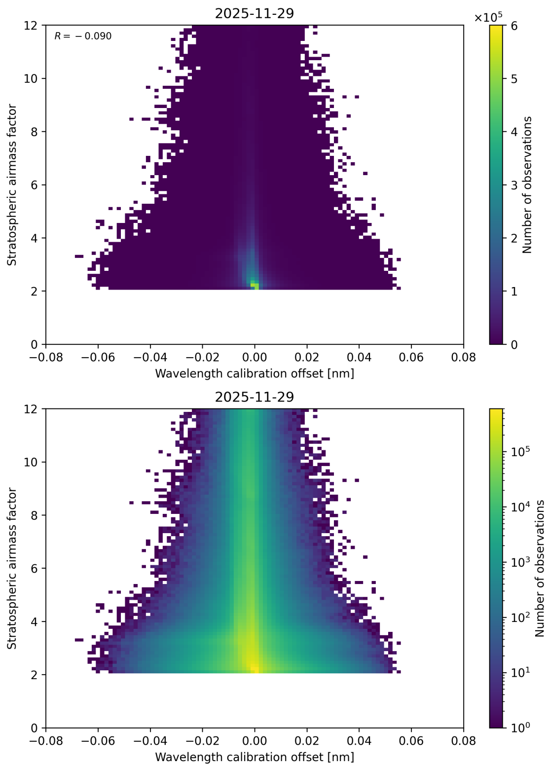
Figure 174: Scatter density plot of “Wavelength calibration offset” against “Stratospheric airmass factor” for 2025-11-28 to 2025-11-30.
