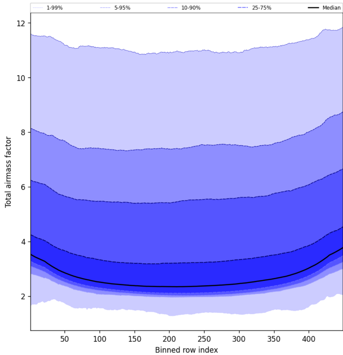
Figure 49: Along track statistics of “Total airmass factor” for 2025-11-28 to 2025-11-30
