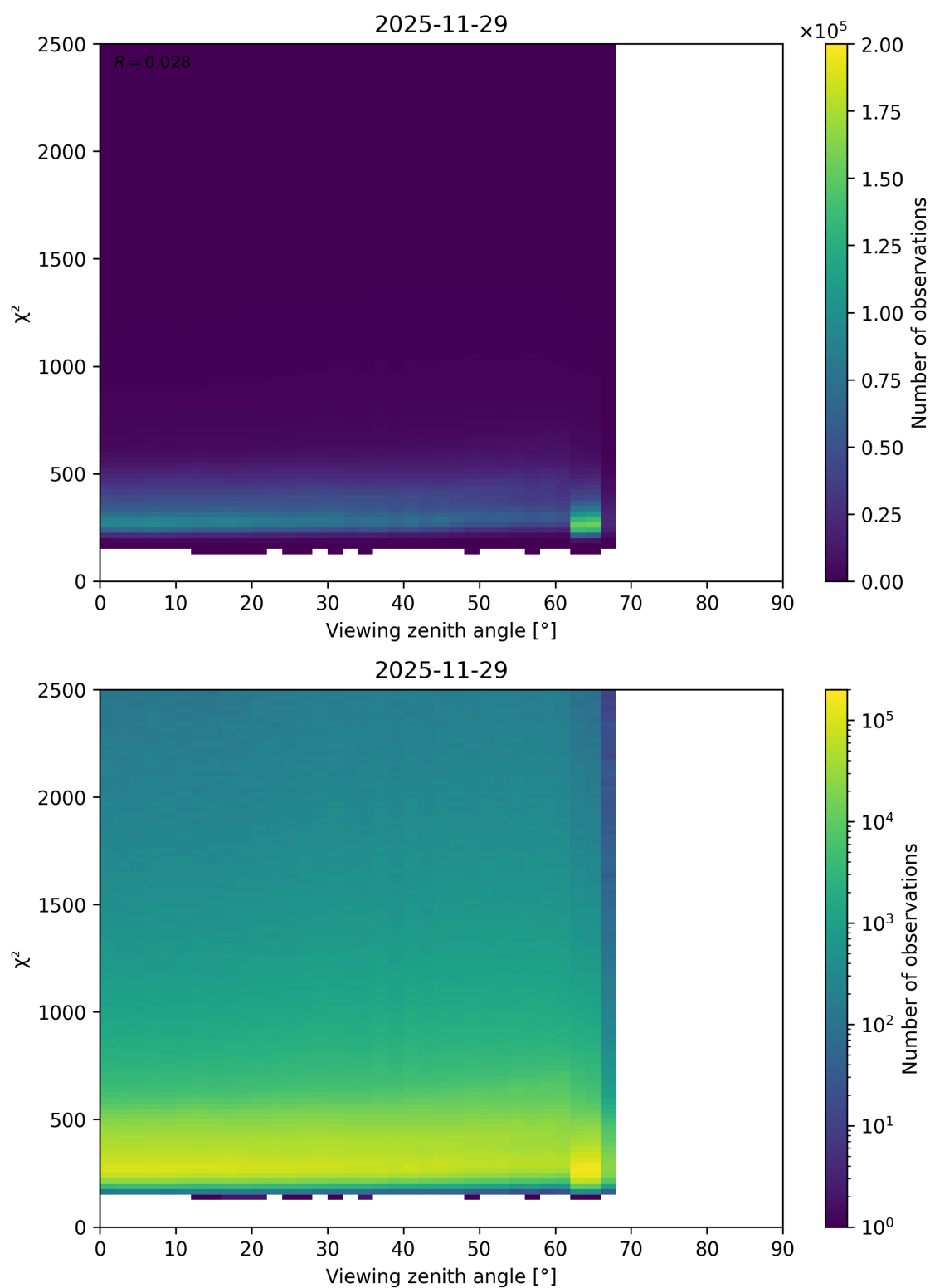
Figure 162: Scatter density plot of “Viewing zenith angle” against “ \chi^2 ” for 2025-11-28 to 2025-11-30.
