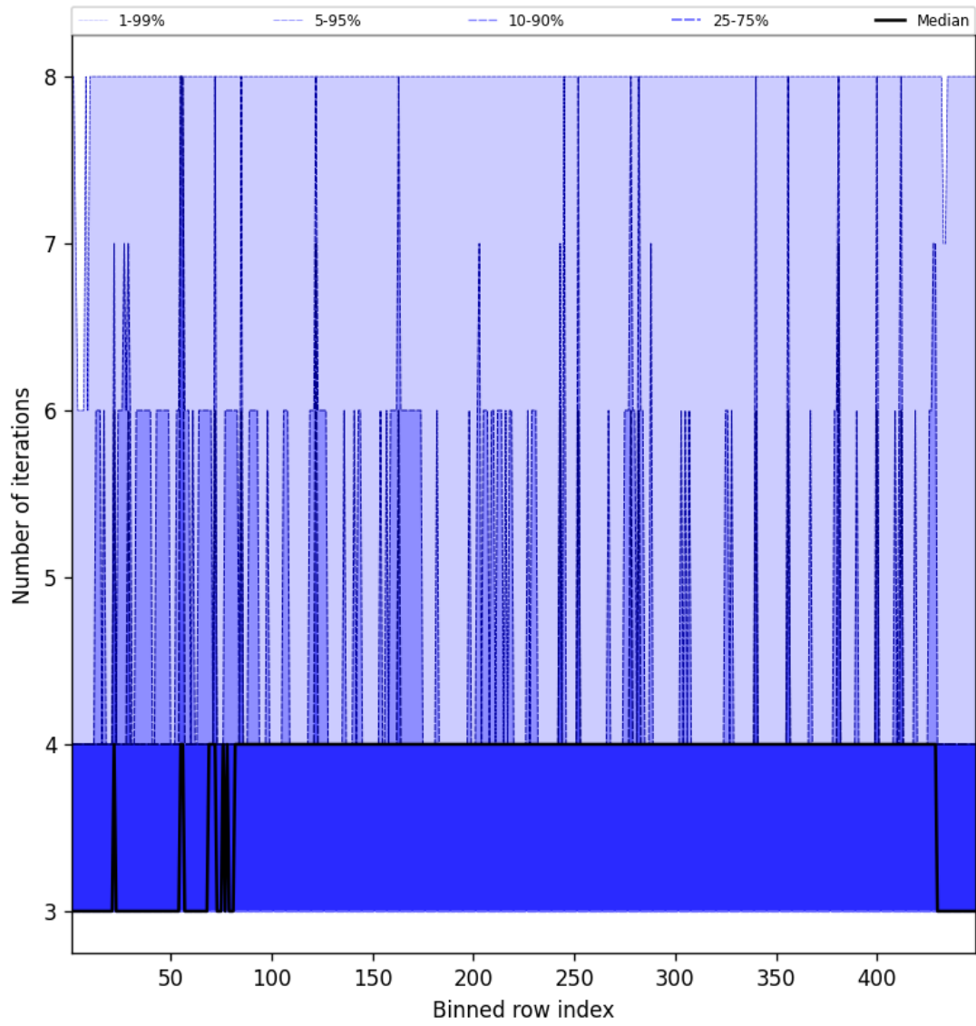
Figure 51: Along track statistics of “Number of iterations” for 2025-11-28 to 2025-11-30
