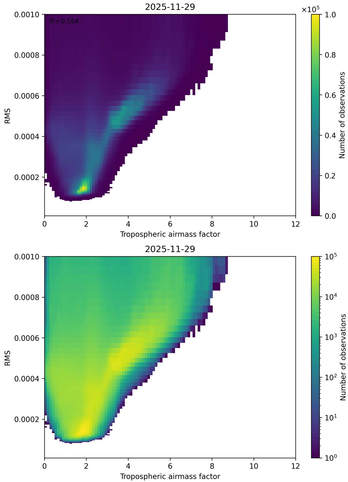
Figure 79: Scatter density plot of “Tropospheric airmass factor” against “RMS” for 2025-11-28 to 2025-11-30.
