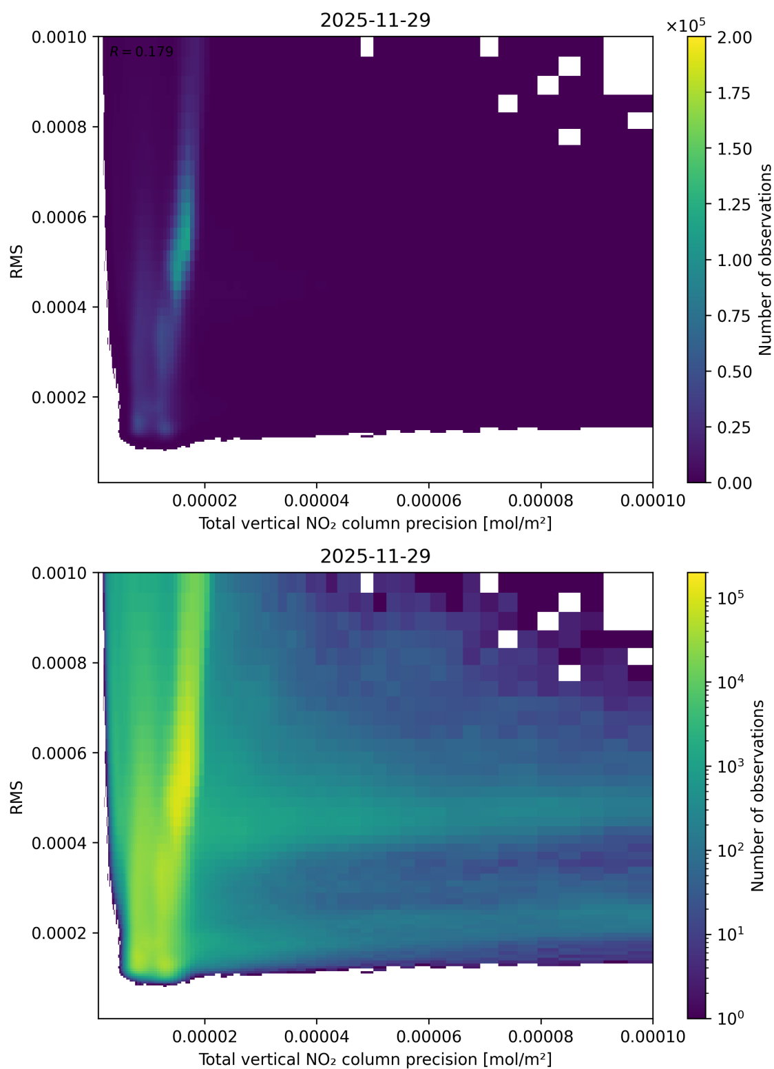
Figure 119: Scatter density plot of “Total vertical NO 2 column precision” against “RMS” for 2025-11-28 to 2025-11-30.
