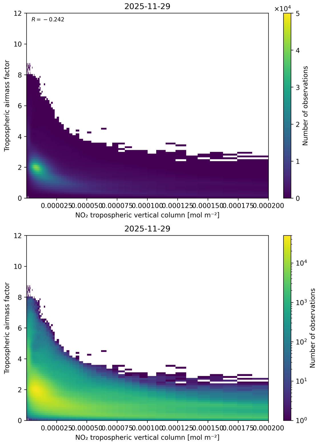
Figure 123: Scatter density plot of “NO 2 tropospheric vertical column” against “Tropospheric air mass factor” for 2025-11-28 to 2025-11-30.
