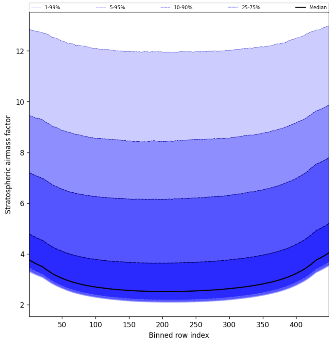
Figure 61: Along track statistics of “Stratospheric airmass factor” for 2025-11-28 to 2025-11-30
