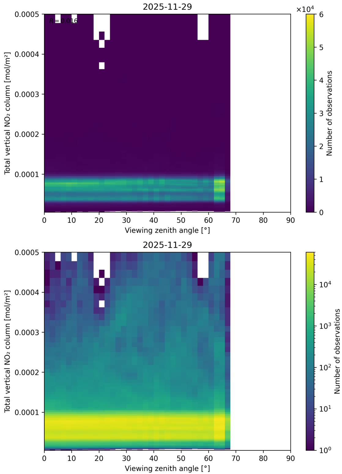
Figure 167: Scatter density plot of “Viewing zenith angle” against “Total vertical NO 2 column” for 2025-11-28 to 2025-11-30.
