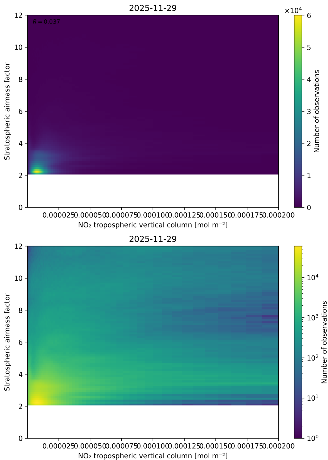
Figure 121: Scatter density plot of “NO 2 tropospheric vertical column” against “Stratospheric airmass factor” for 2025-11-28 to 2025-11-30.
