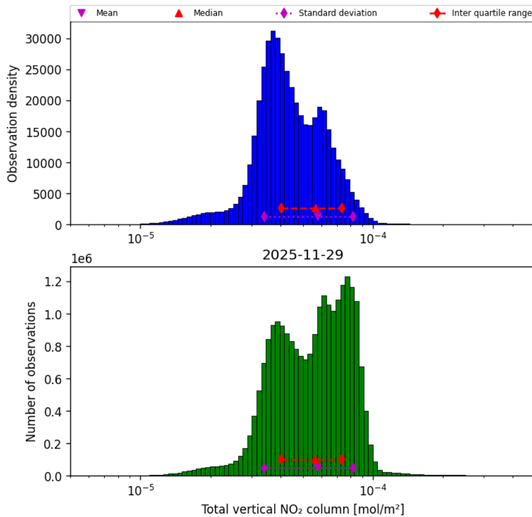
Figure 38: Histogram of “Total vertical NO 2 column” for 2025-11-28 to 2025-11-30
