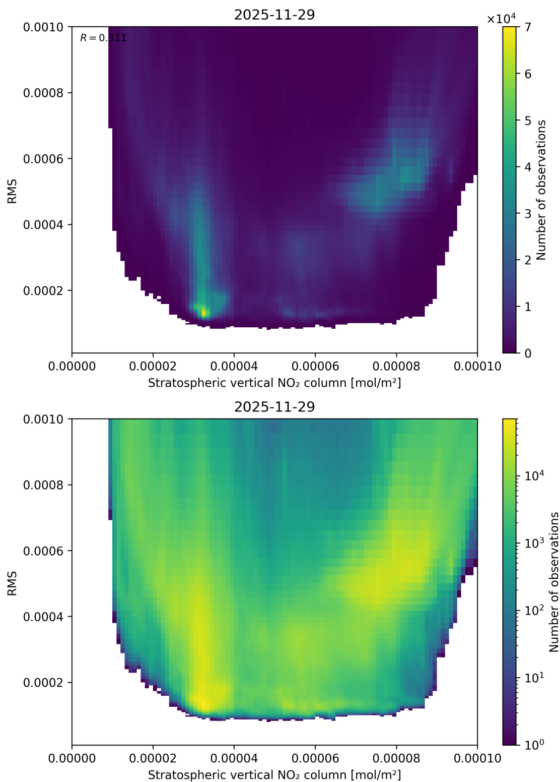
Figure 102: Scatter density plot of “Stratospheric vertical NO 2 column” against “RMS” for 2025-11-28 to 2025-11-30.
