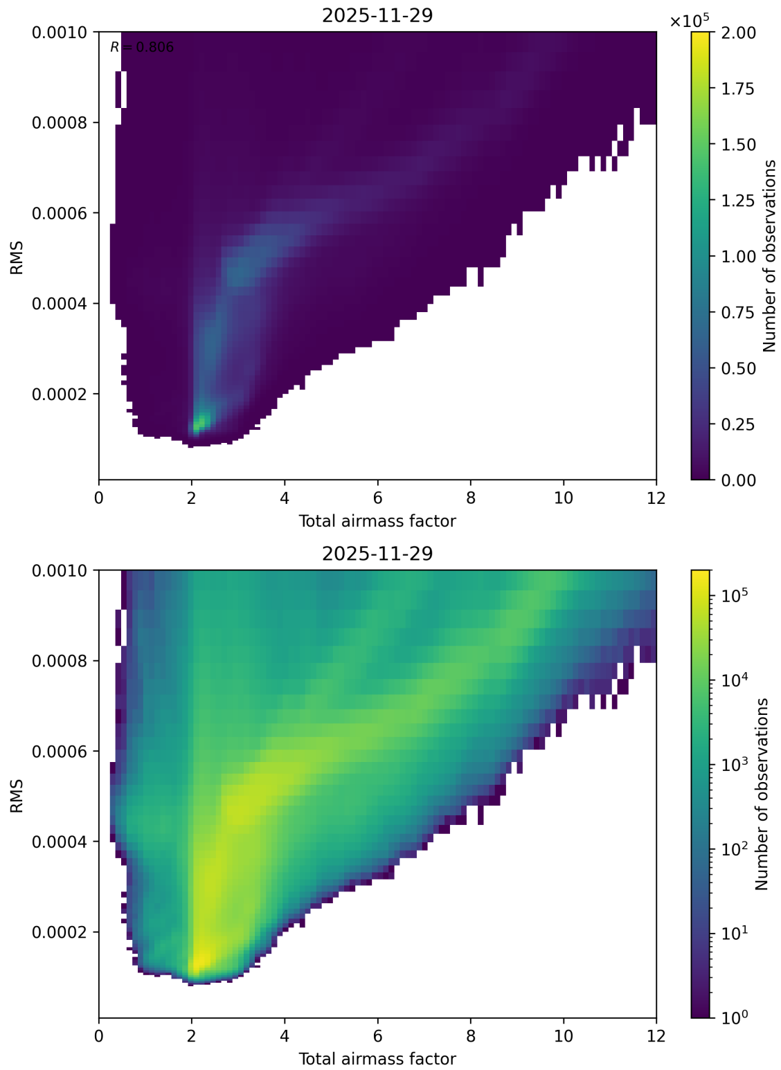
Figure 69: Scatter density plot of “Total airmass factor” against “RMS” for 2025-11-28 to 2025-11-30.
