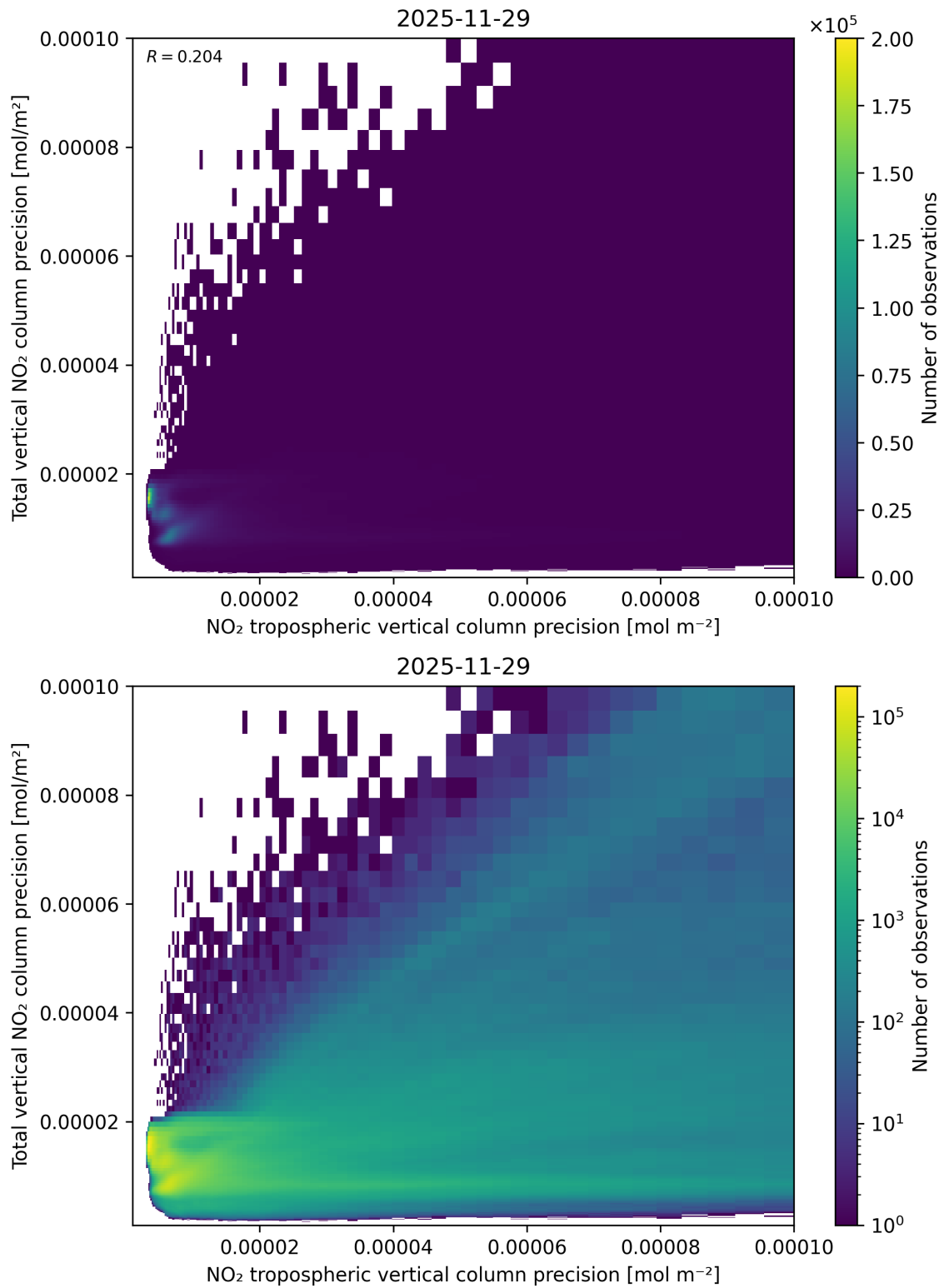
Figure 139: Scatter density plot of “NO 2 tropospheric vertical column precision” against “Total vertical NO 2 column precision” for 2025-11-28 to 2025-11-30.
