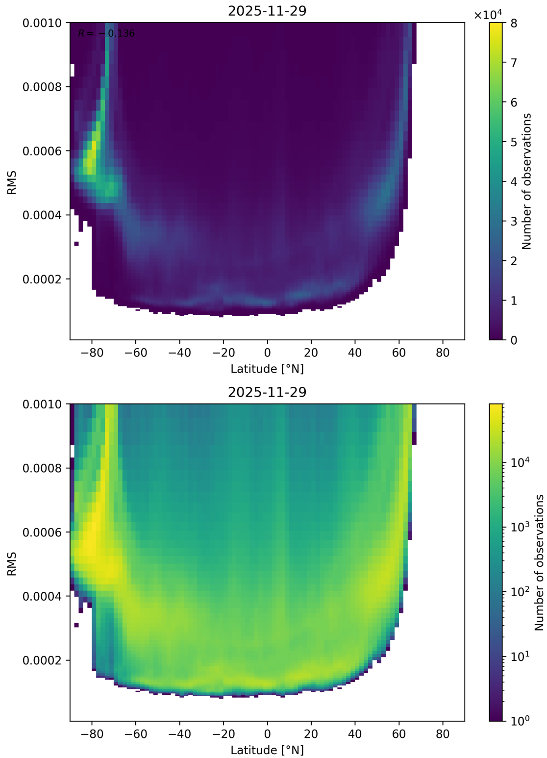
Figure 94: Scatter density plot of “Latitude” against “RMS” for 2025-11-28 to 2025-11-30.
