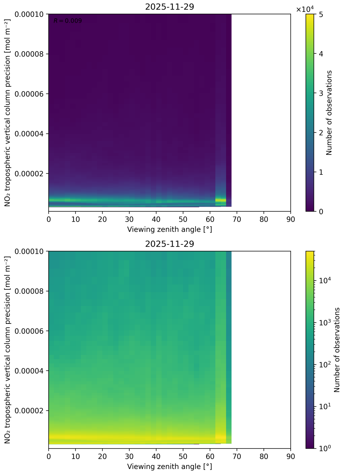
Figure 170: Scatter density plot of “Viewing zenith angle” against “NO 2 tropospheric vertical column precision” for 2025-11-28 to 2025-11-30.
