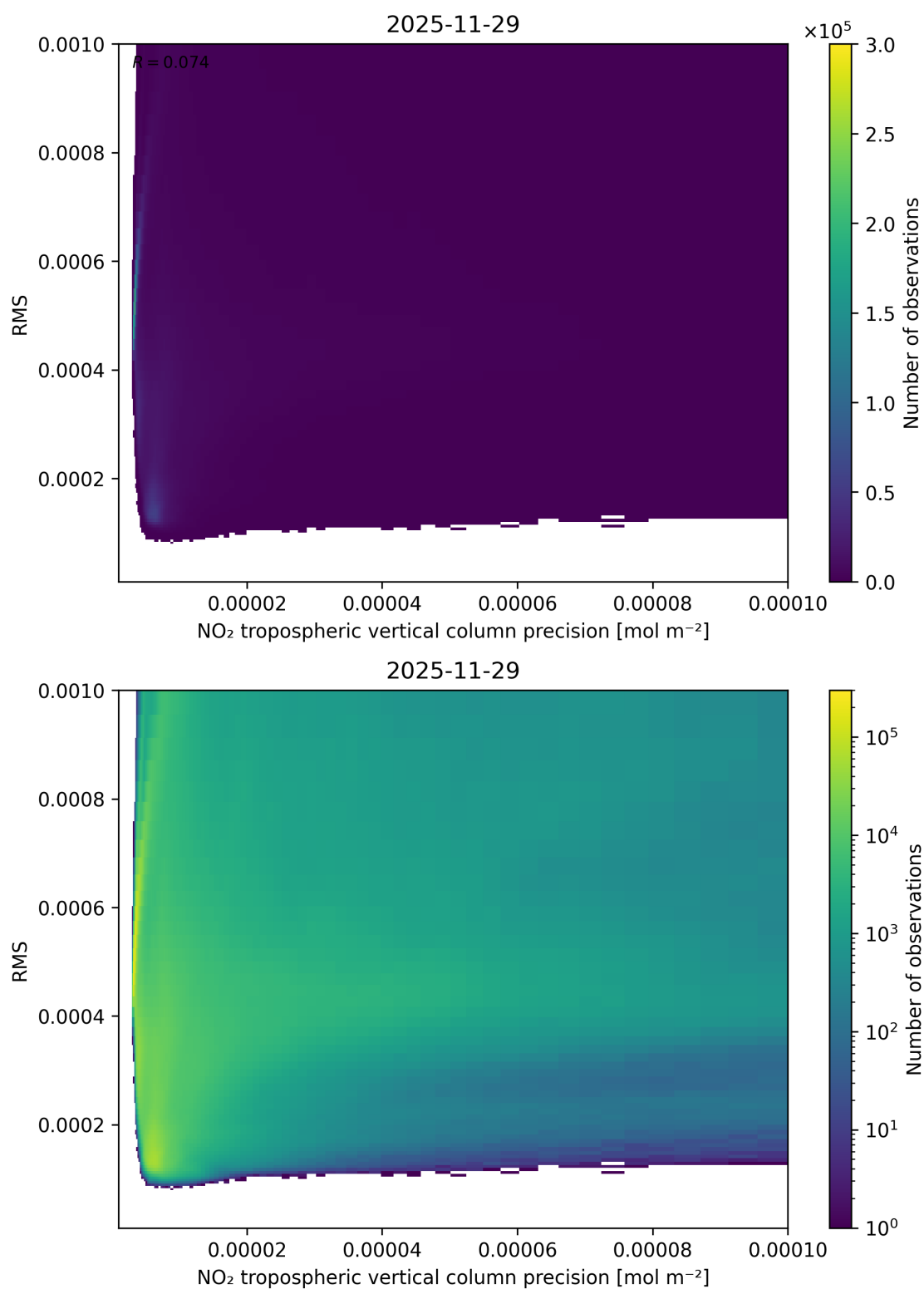
Figure 140: Scatter density plot of “NO 2 tropospheric vertical column precision” against “RMS” for 2025-11-28 to 2025-11-30.
