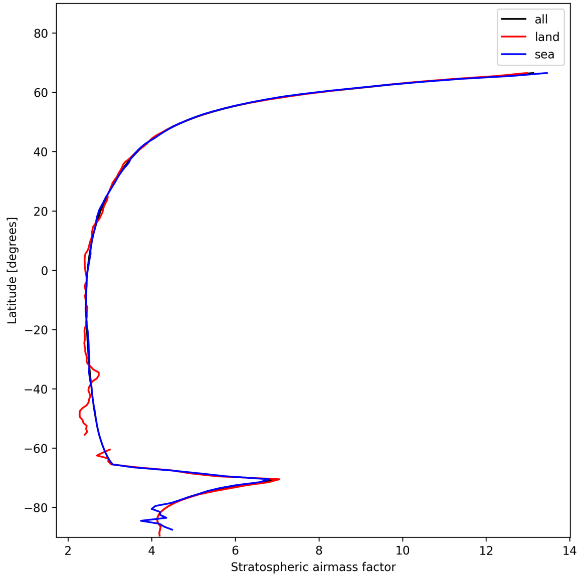
Figure 27: Zonal average of “Stratospheric airmass factor” for 2025-11-28 to 2025-11-30.
