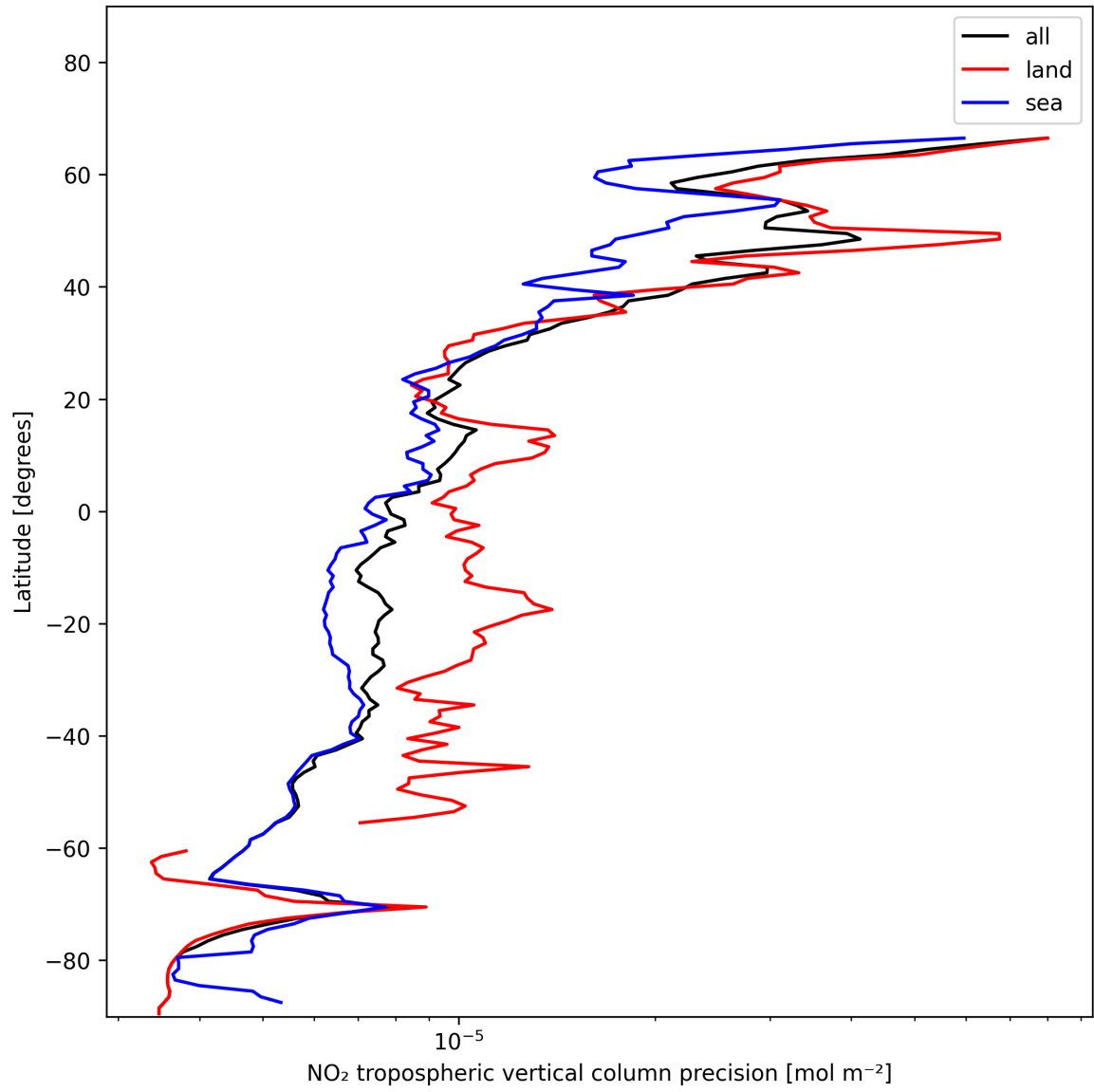
Figure 13: Zonal average of “NO 2 tropospheric vertical column precision” for 2025-11-28 to 2025-11-30.
