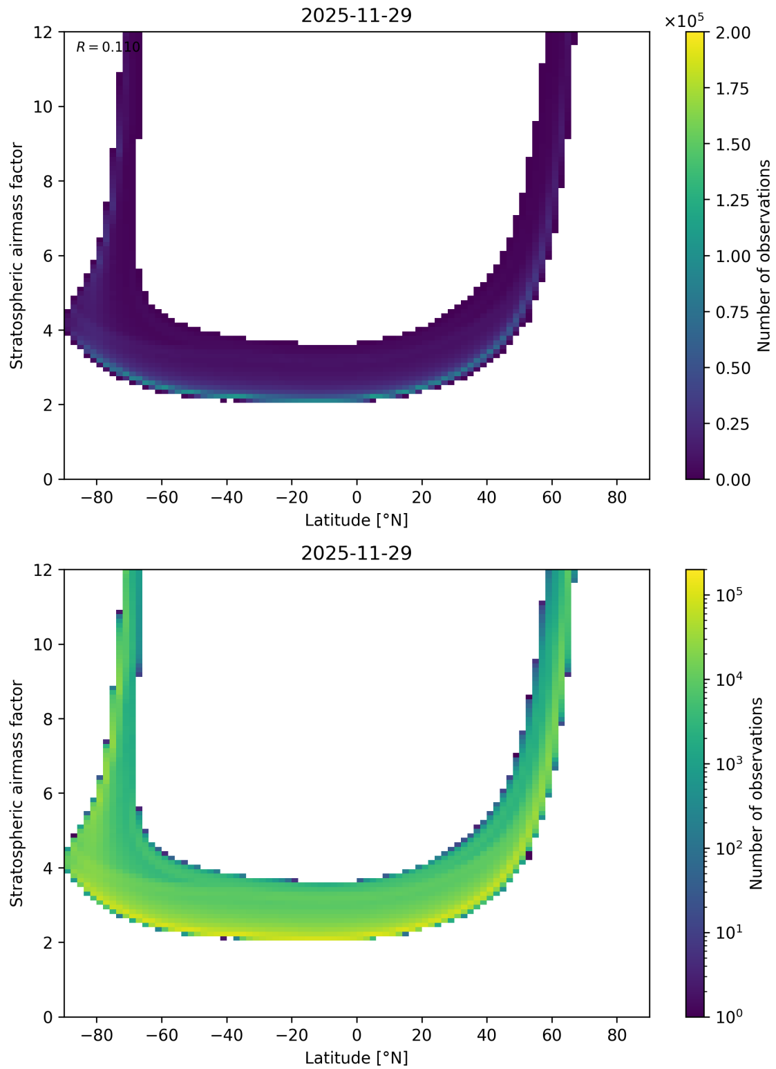
Figure 83: Scatter density plot of “Latitude” against “Stratospheric air mass factor” for 2025-11-28 to 2025-11-30.
