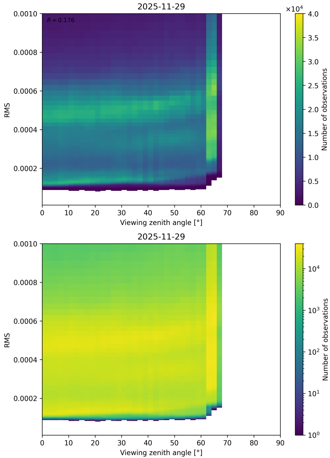
Figure 171: Scatter density plot of “Viewing zenith angle” against “RMS” for 2025-11-28 to 2025-11-30.
