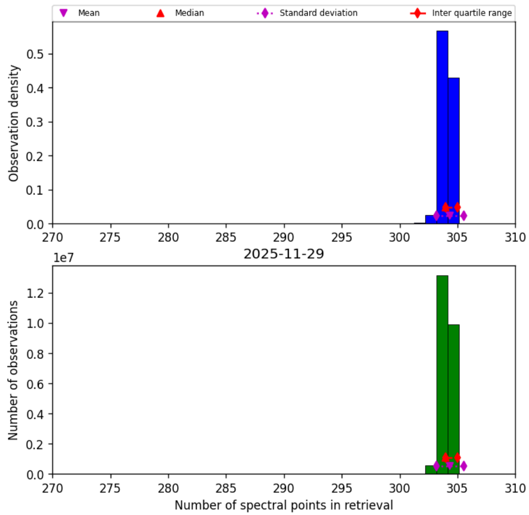
Figure 33: Histogram of “Number of spectral points in retrieval” for 2025-11-28 to 2025-11-30
