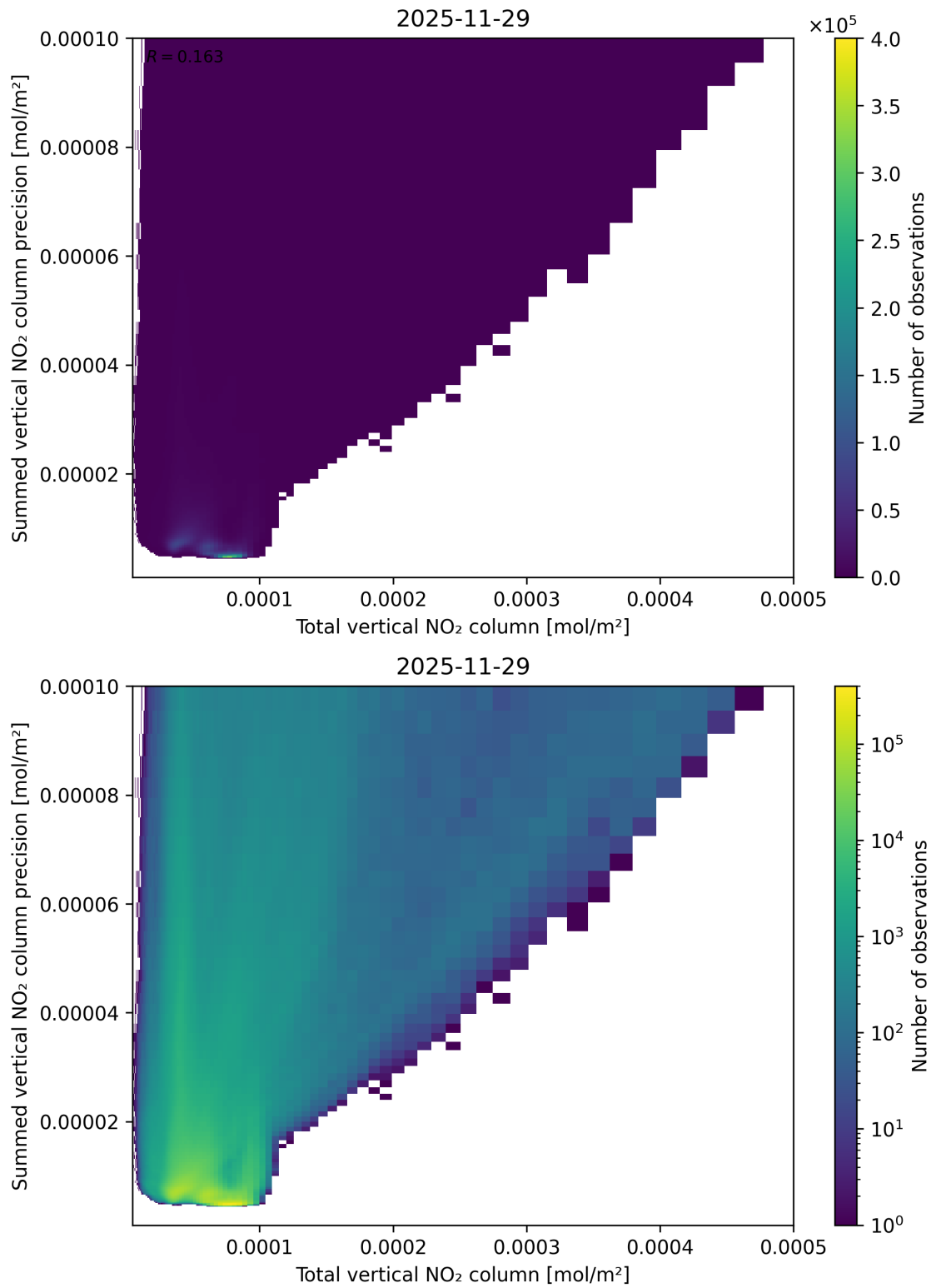
Figure 113: Scatter density plot of “Total vertical NO 2 column” against “Summed vertical NO 2 column precision” for 2025-11-28 to 2025-11-30.
