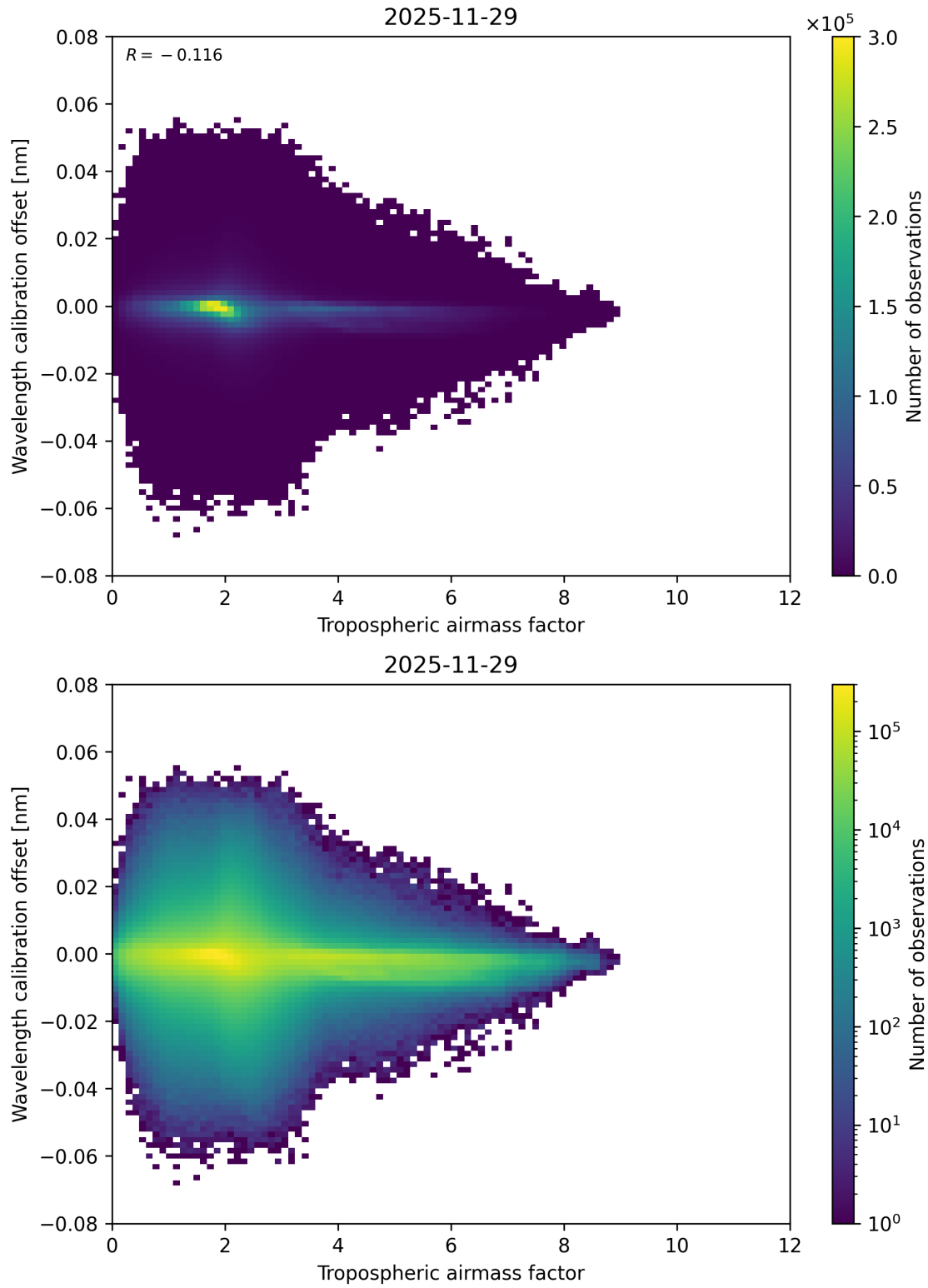
Figure 80: Scatter density plot of “Tropospheric airmass factor” against “Wavelength calibration offset” for 2025-11-28 to 2025-11-30.
