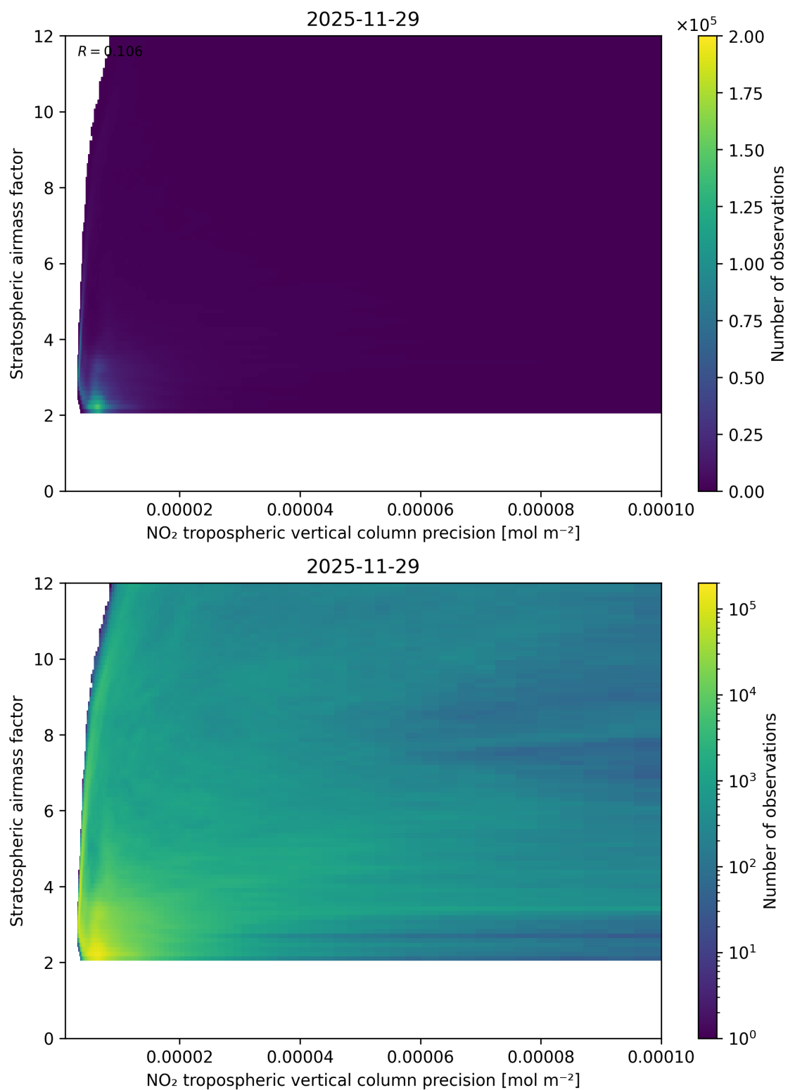
Figure 131: Scatter density plot of “NO 2 tropospheric vertical column precision” against “Stratospheric airmass factor” for 2025-11-28 to 2025-11-30.
