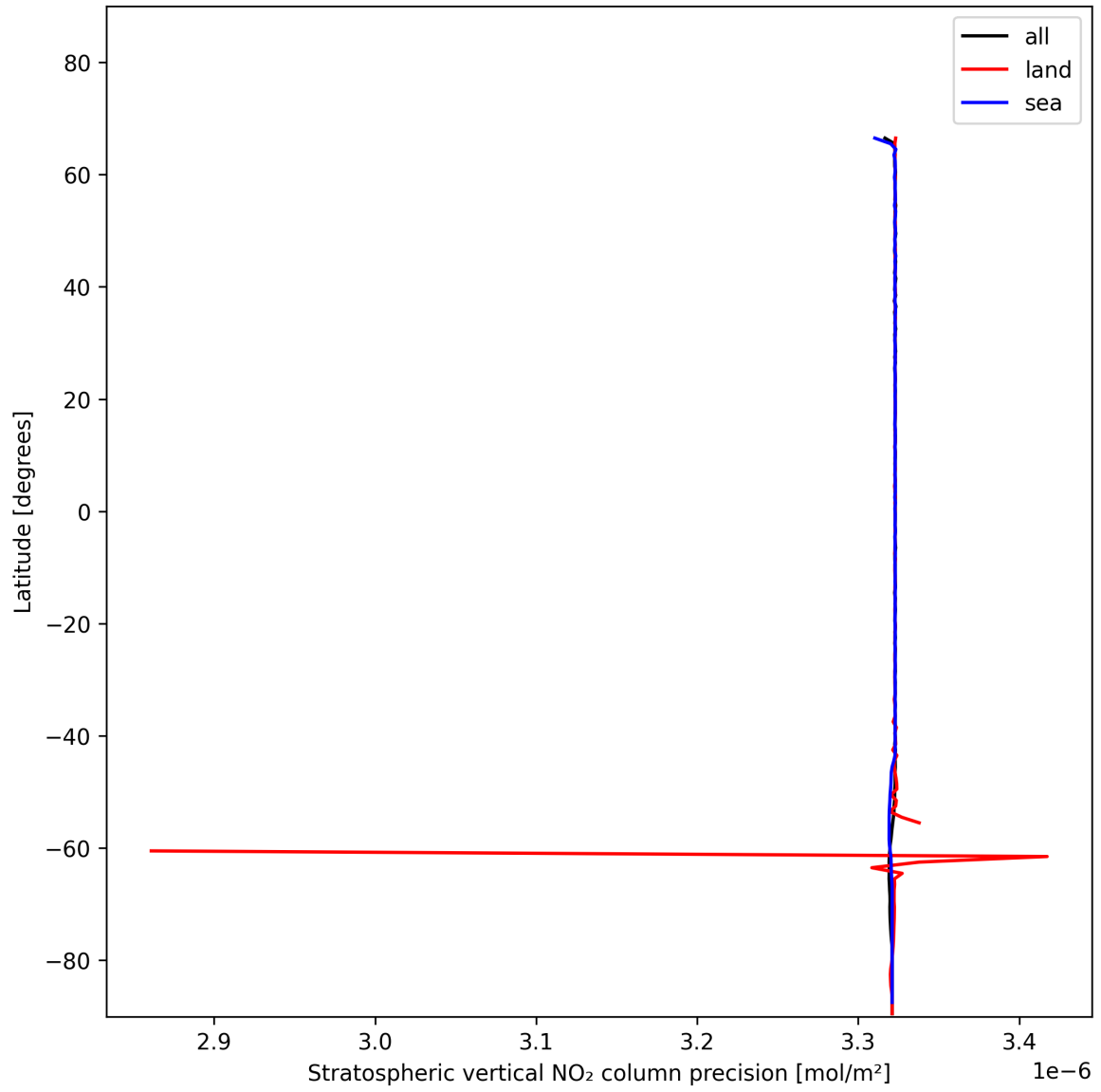
Figure 20: Zonal average of “Stratospheric vertical NO 2 column precision” for 2025-11-28 to 2025-11-30.
