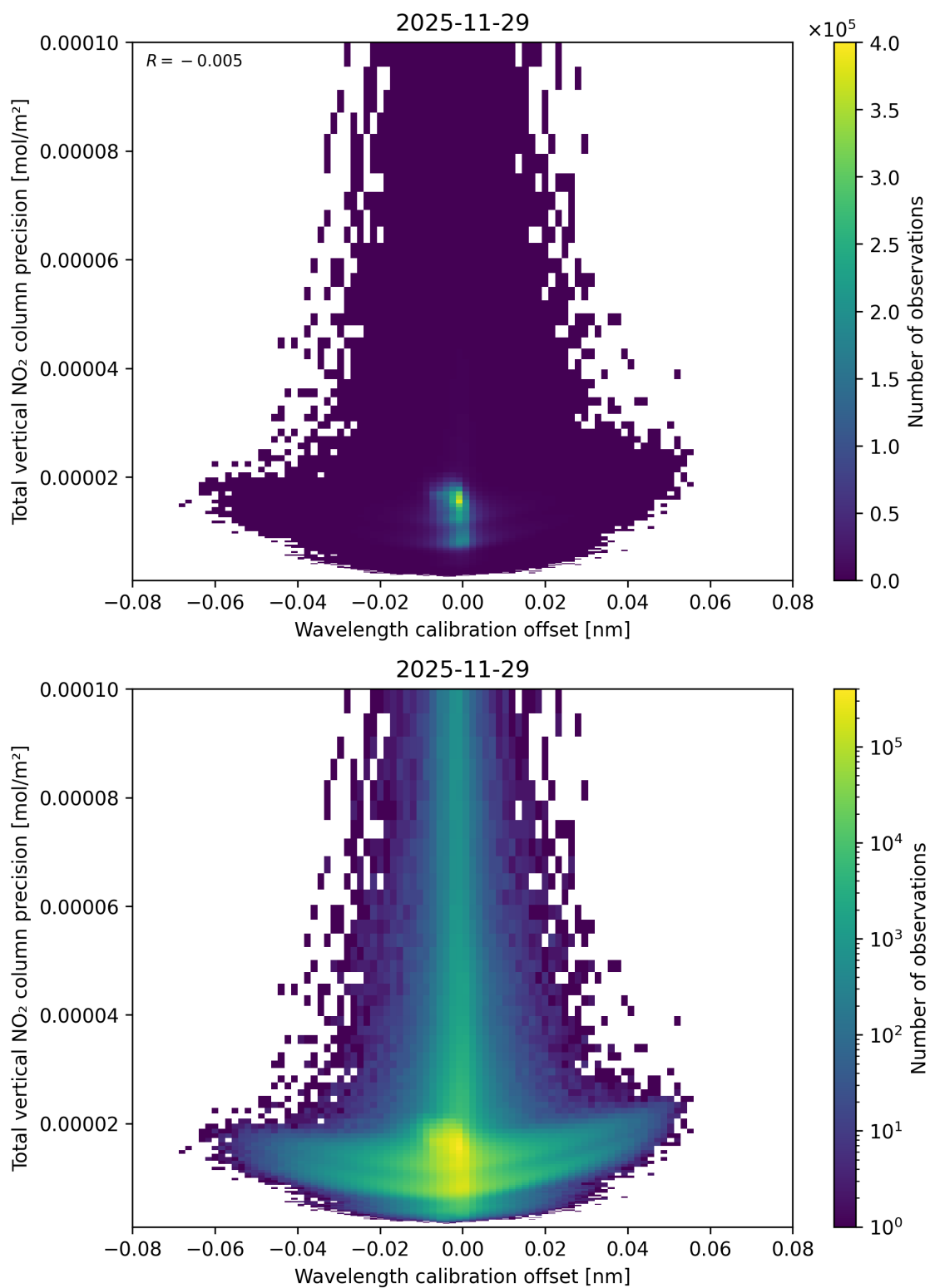
Figure 180: Scatter density plot of “Wavelength calibration offset” against “Total vertical NO 2 column precision” for 2025-11-28 to 2025-11-30.
