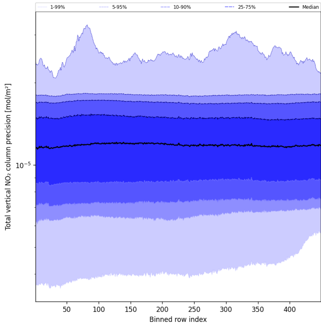
Figure 56: Along track statistics of “Total vertical NO 2 column precision” for 2025-11-28 to 2025-11-30
