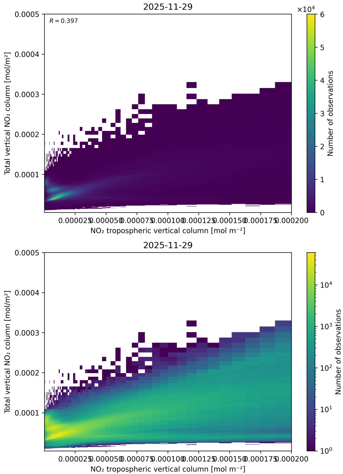
Figure 128: Scatter density plot of “NO 2 tropospheric vertical column” against “Total vertical NO 2 column” for 2025-11-28 to 2025-11-30.
