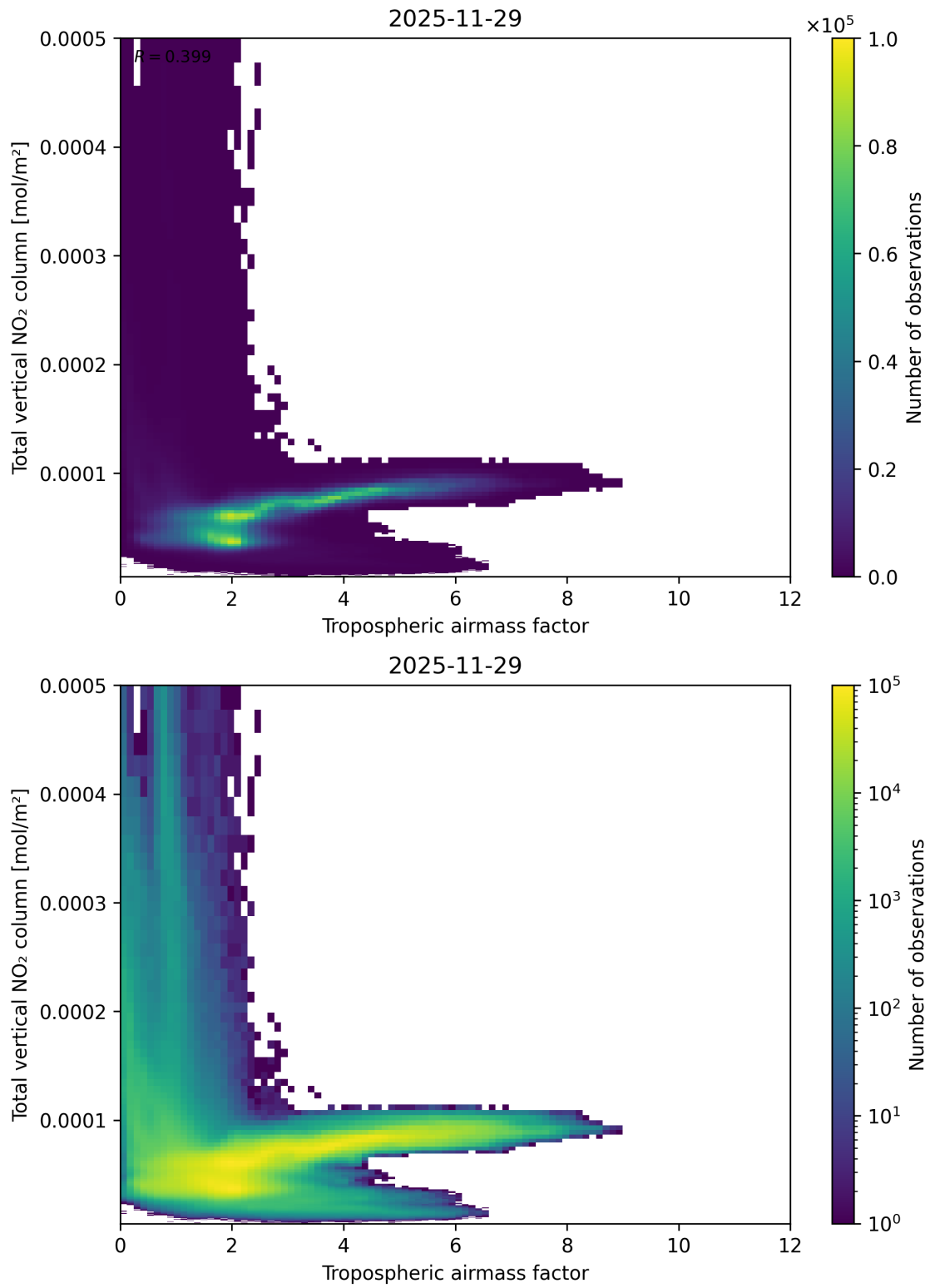
Figure 77: Scatter density plot of “Tropospheric airmass factor” against “Total vertical \text{NO}_2 column” for 2025-11-28 to 2025-11-30.
