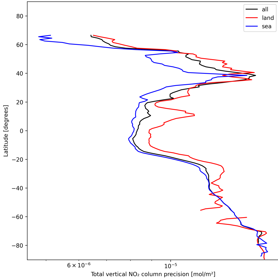
Figure 22: Zonal average of “Total vertical NO 2 column precision” for 2025-11-28 to 2025-11-30.
