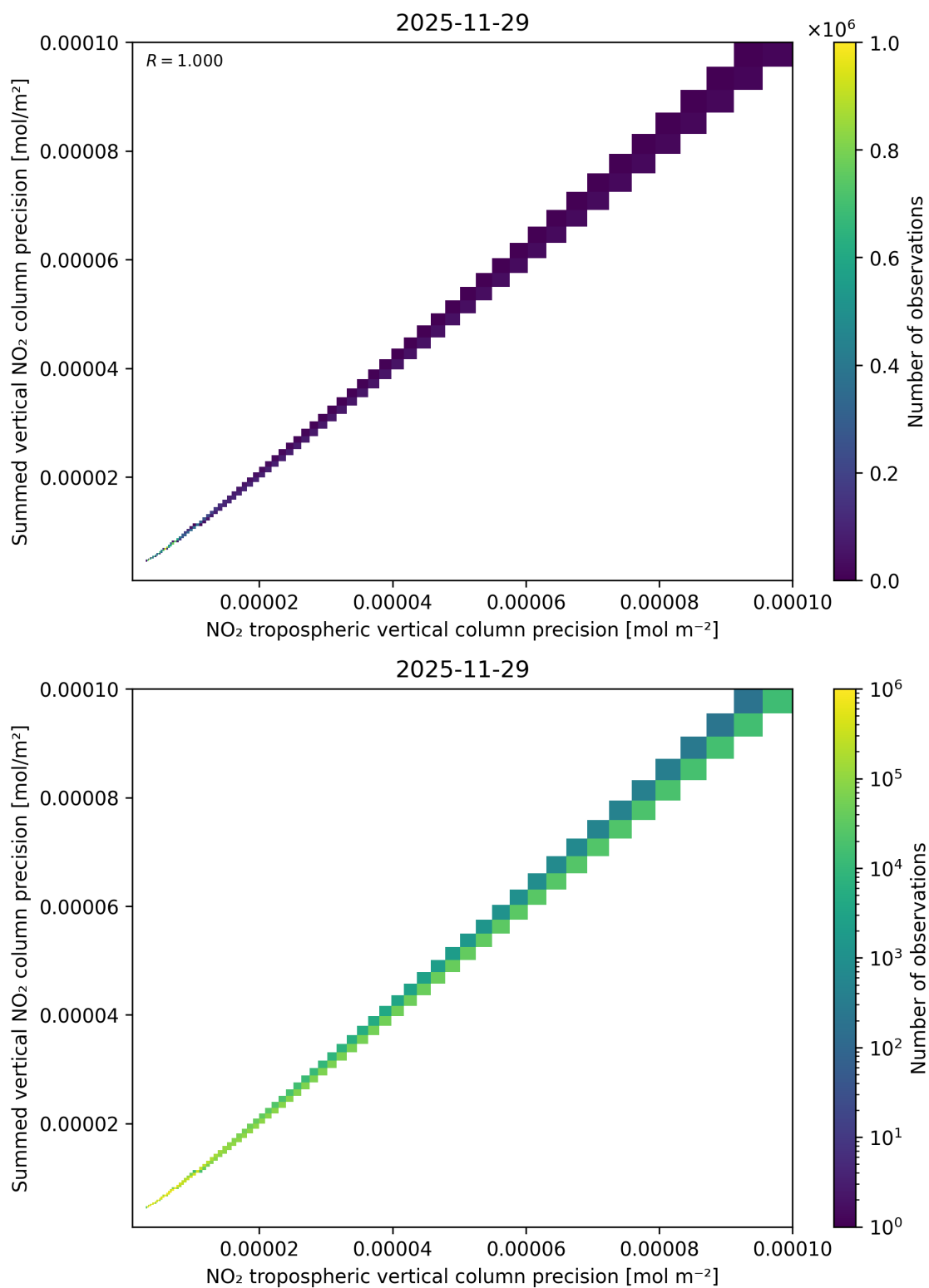
Figure 137: Scatter density plot of “NO 2 tropospheric vertical column precision” against “Summed vertical NO 2 column precision” for 2025-11-28 to 2025-11-30.
