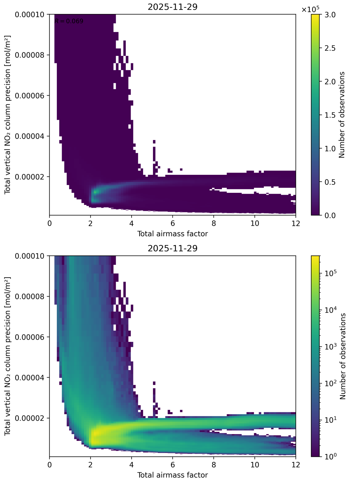
Figure 68: Scatter density plot of “Total airmass factor” against “Total vertical NO 2 column precision” for 2025-11-28 to 2025-11-30.
