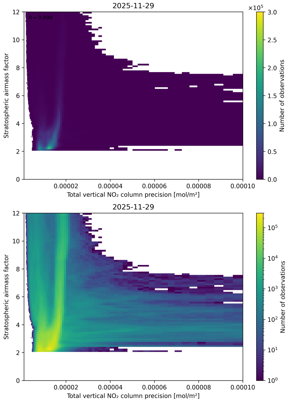
Figure 115: Scatter density plot of “Total vertical NO 2 column precision” against “Stratospheric air mass factor” for 2025-11-28 to 2025-11-30.
