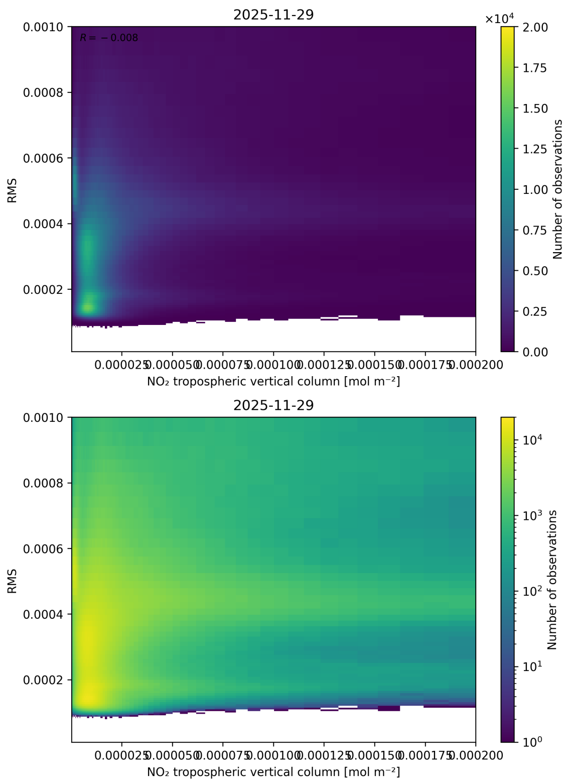
Figure 142: Scatter density plot of “NO 2 tropospheric vertical column” against “RMS” for 2025-11-28 to 2025-11-30.
