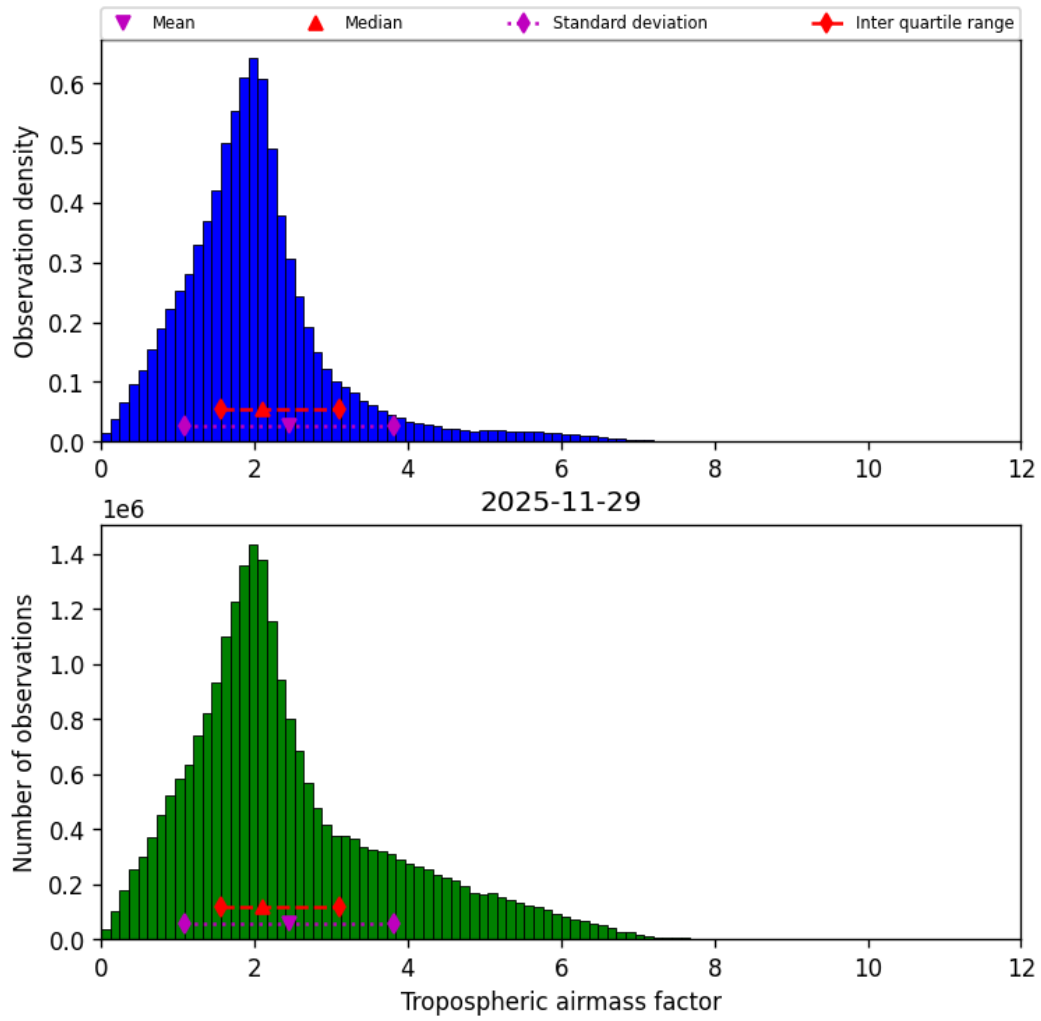
Figure 31: Histogram of “Tropospheric airmass factor” for 2025-11-28 to 2025-11-30
