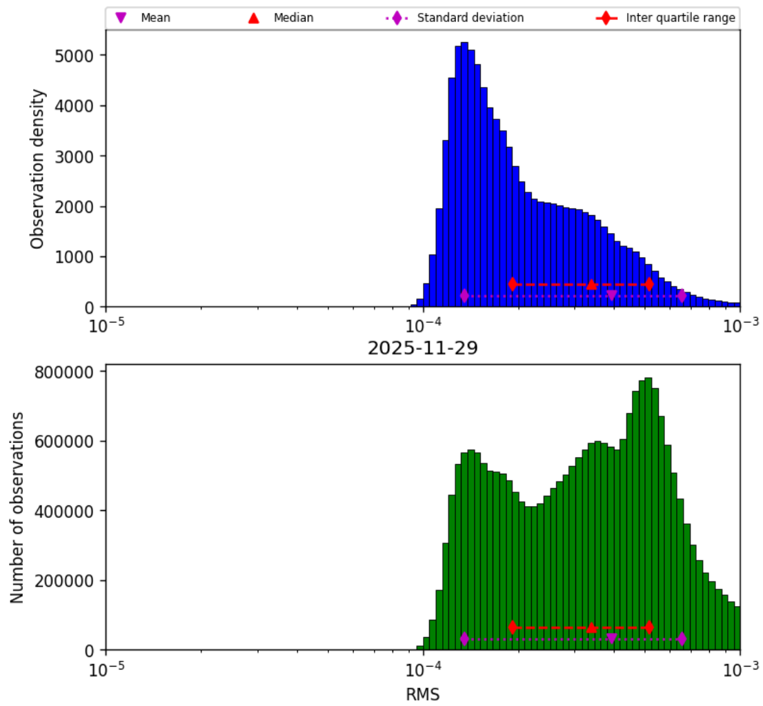
Figure 43: Histogram of “RMS” for 2025-11-28 to 2025-11-30
