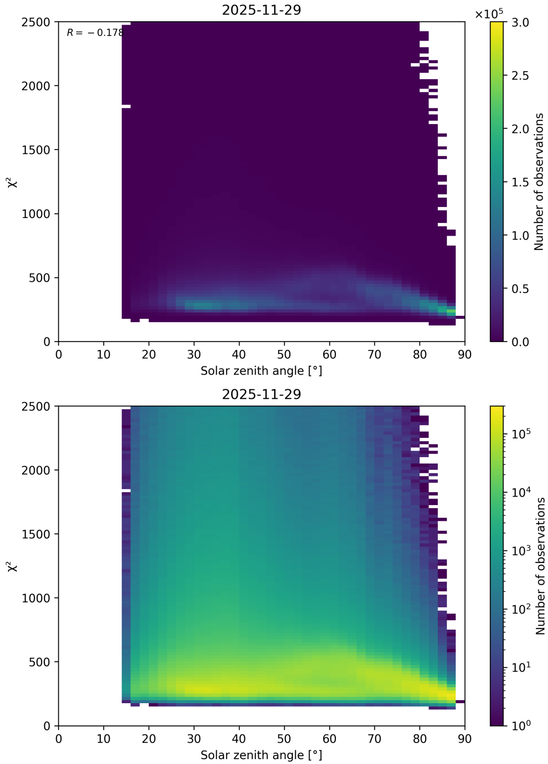
Figure 148: Scatter density plot of “Solar zenith angle” against “ \chi^2 ” for 2025-11-28 to 2025-11-30.
