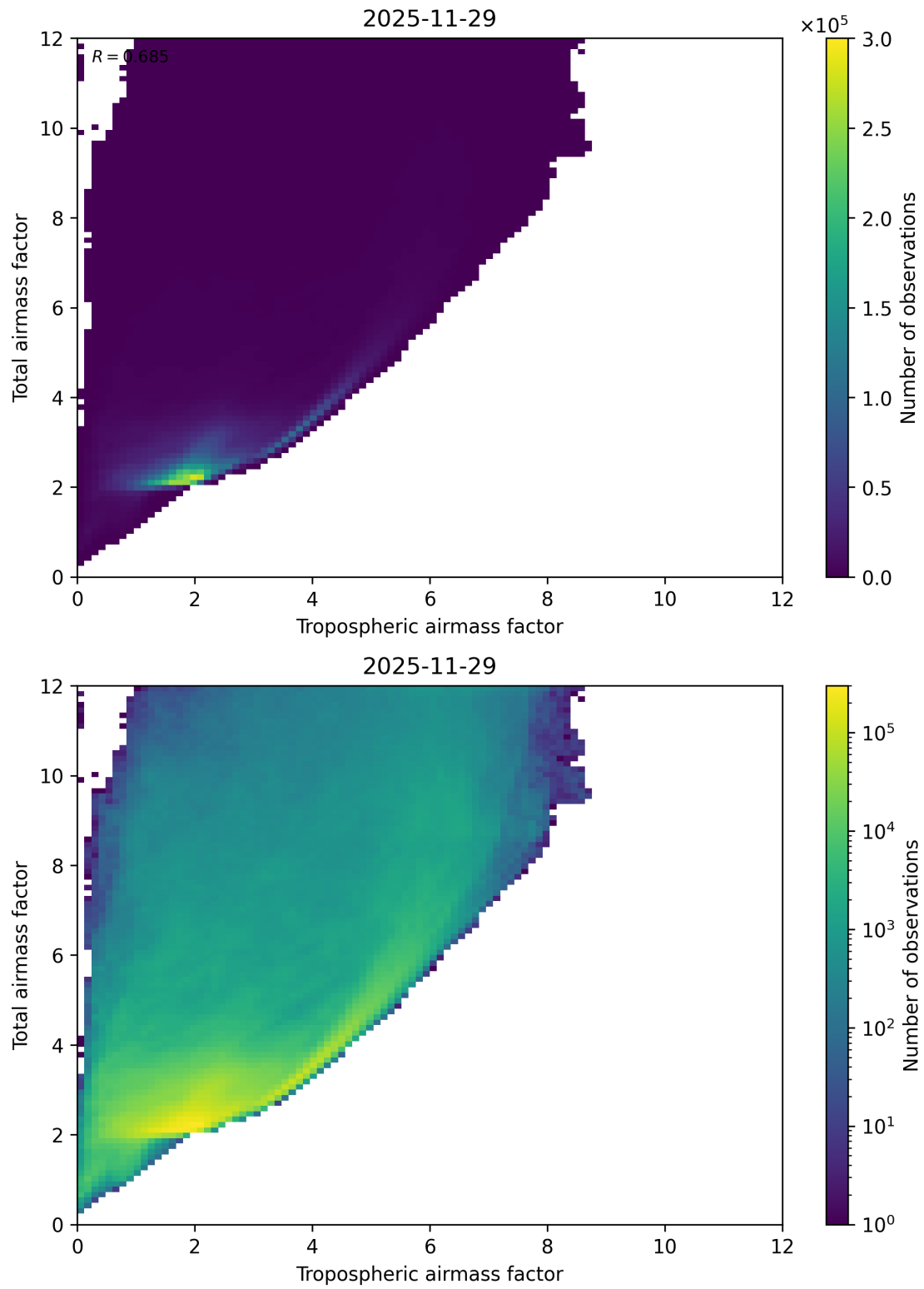
Figure 72: Scatter density plot of “Tropospheric airmass factor” against “Total airmass factor” for 2025-11-28 to 2025-11-30.
