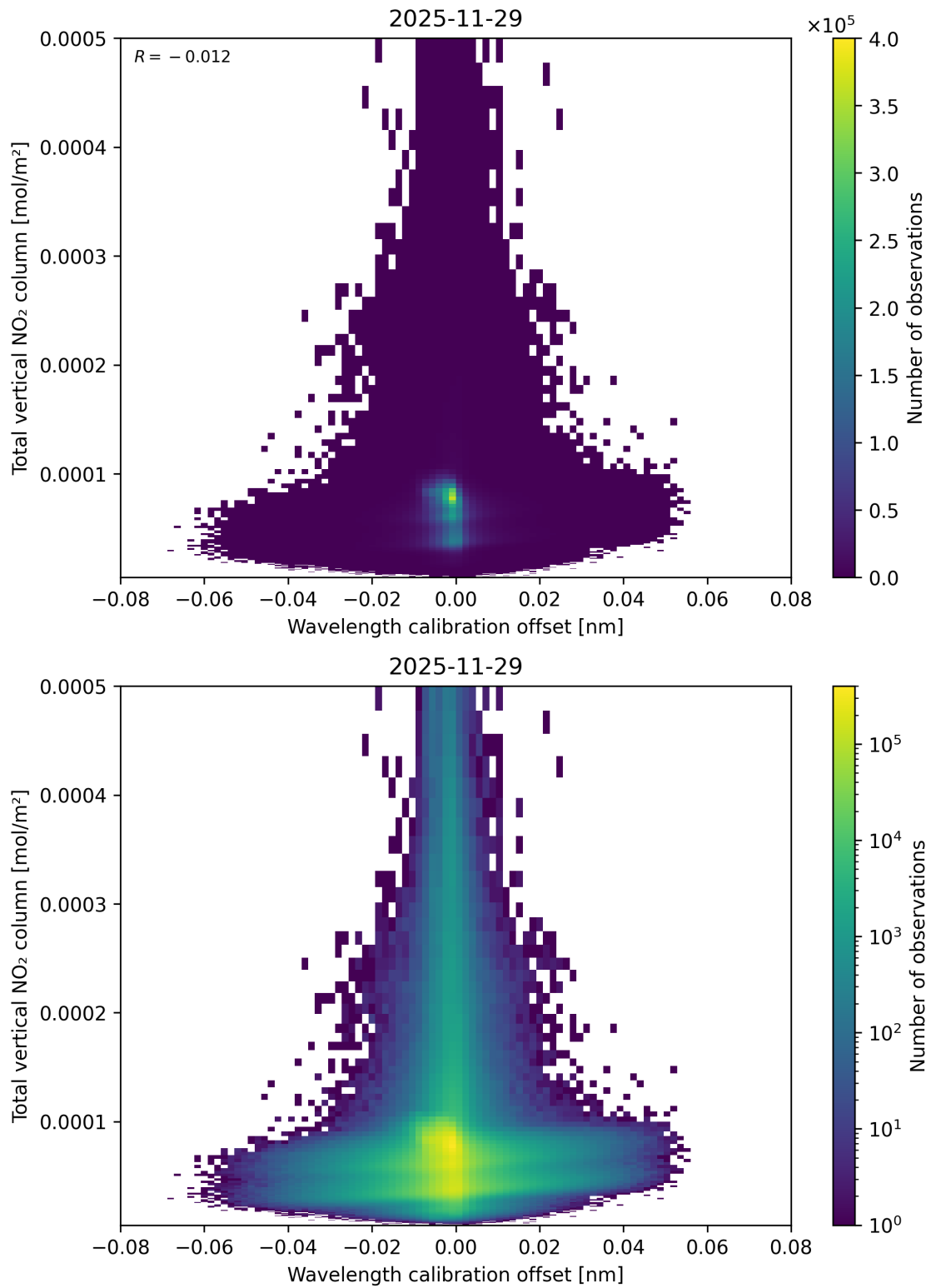
Figure 179: Scatter density plot of “Wavelength calibration offset” against “Total vertical NO 2 column” for 2025-11-28 to 2025-11-30.
