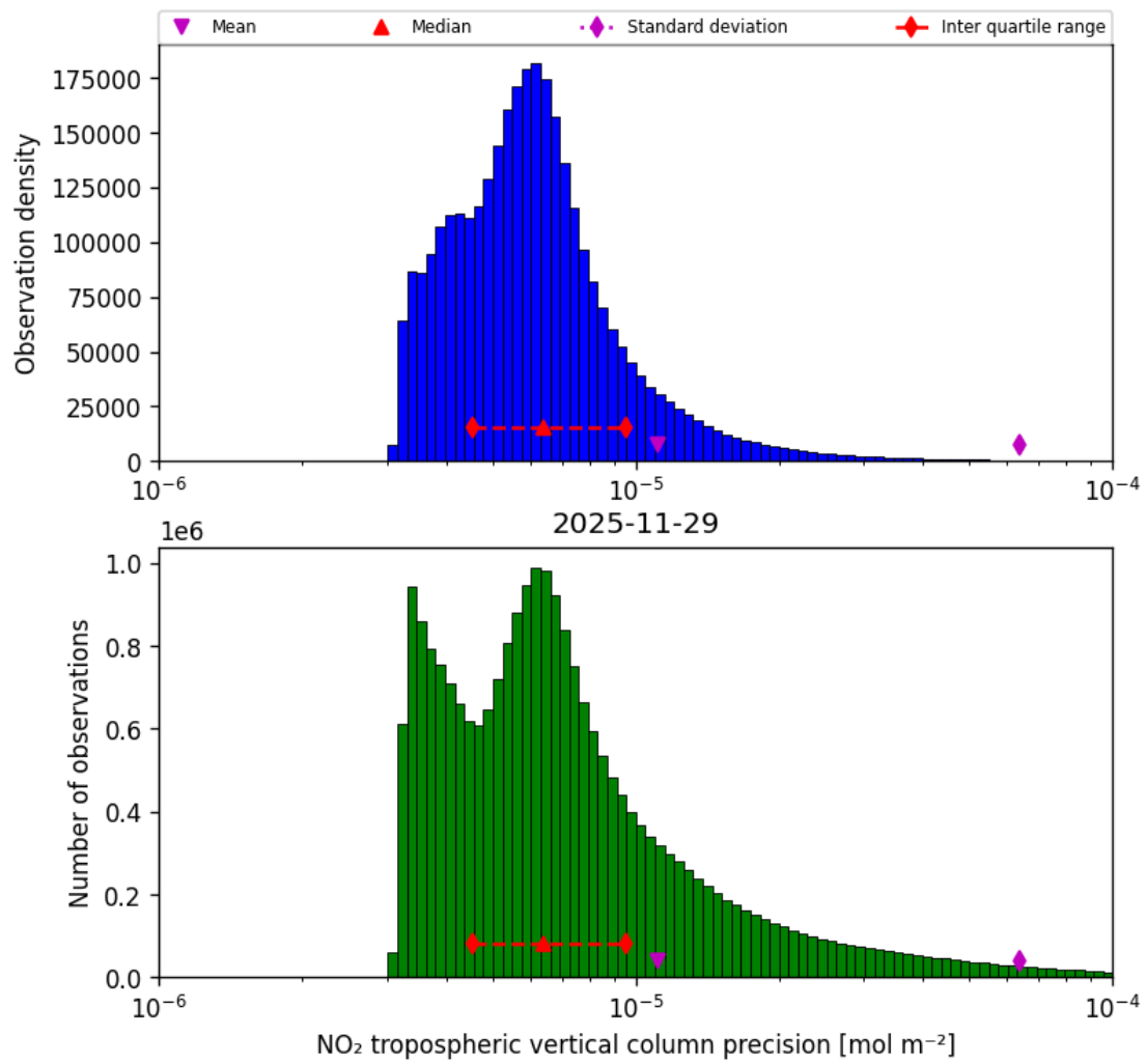
Figure 30: Histogram of “NO 2 tropospheric vertical column precision” for 2025-11-28 to 2025-11-30
