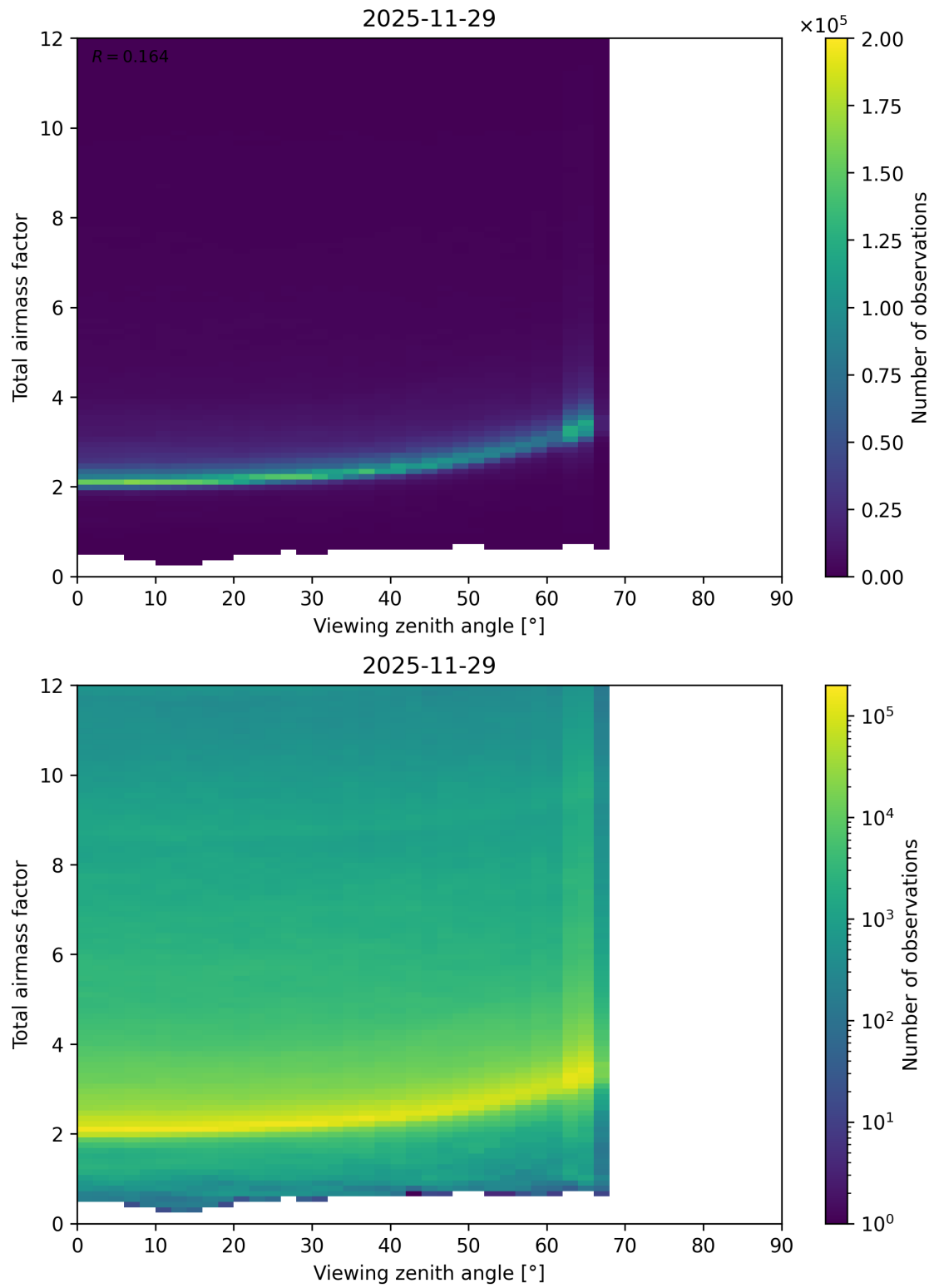
Figure 160: Scatter density plot of “Viewing zenith angle” against “Total airmass factor” for 2025-11-28 to 2025-11-30.
