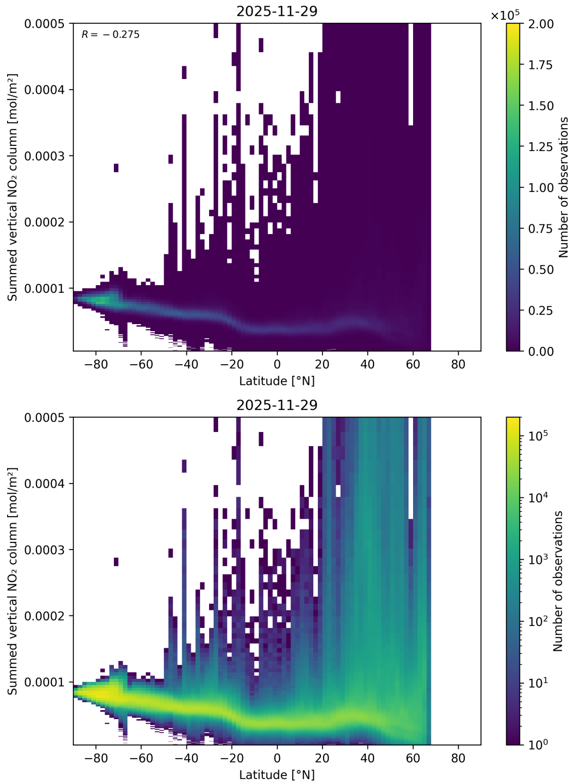
Figure 88: Scatter density plot of “Latitude” against “Summed vertical NO 2 column” for 2025-11-28 to 2025-11-30.
