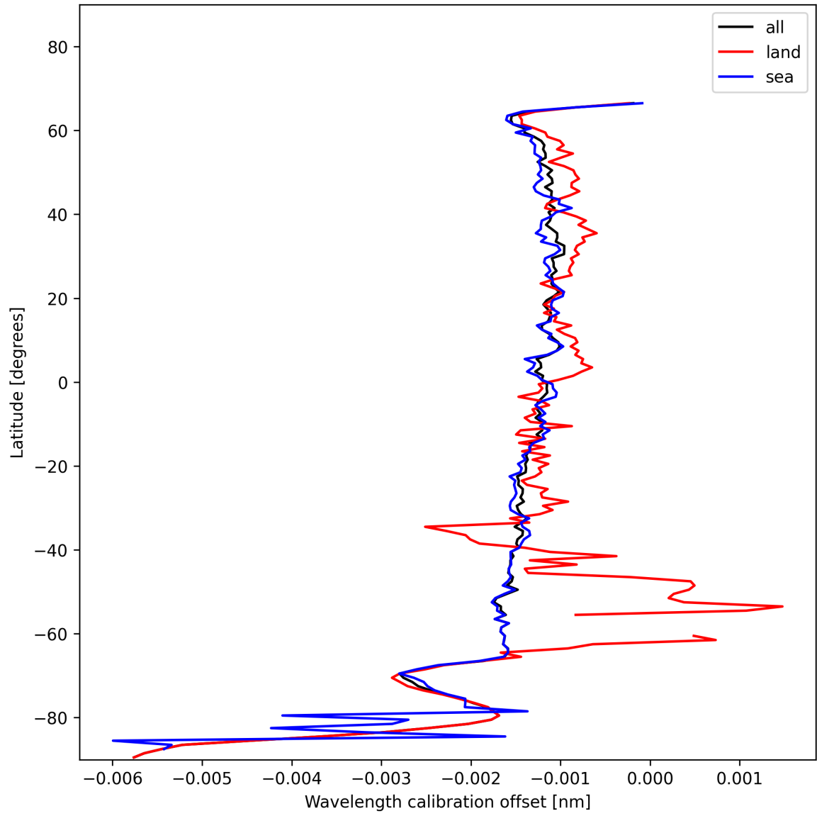
Figure 18: Zonal average of “Wavelength calibration offset” for 2025-11-28 to 2025-11-30.
