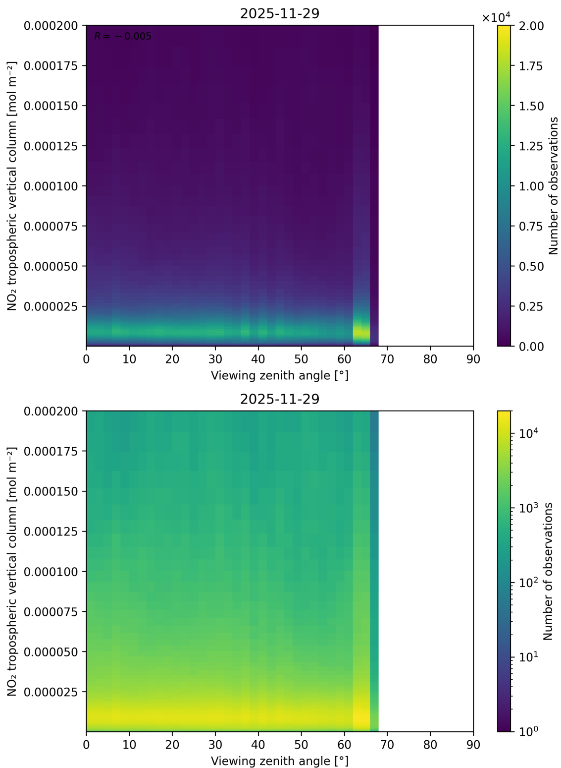
Figure 169: Scatter density plot of “Viewing zenith angle” against “NO 2 tropospheric vertical column” for 2025-11-28 to 2025-11-30.
