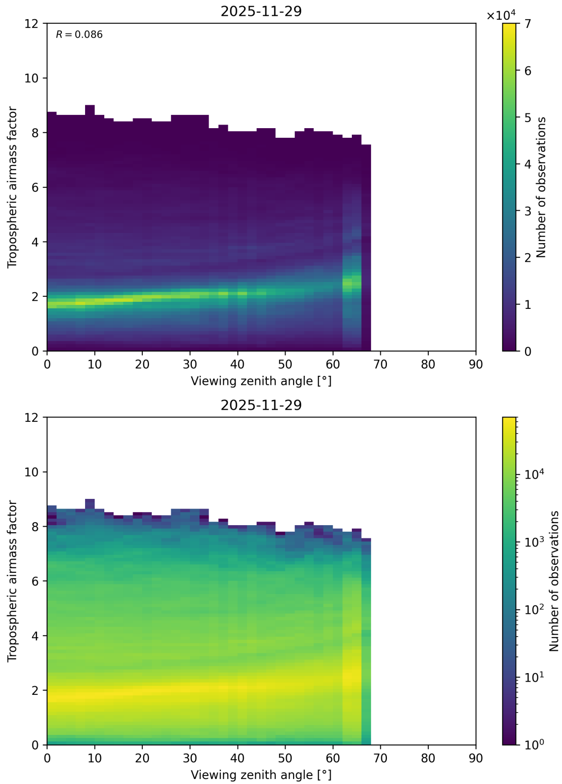
Figure 161: Scatter density plot of “Viewing zenith angle” against “Tropospheric airmass factor” for 2025-11-28 to 2025-11-30.
