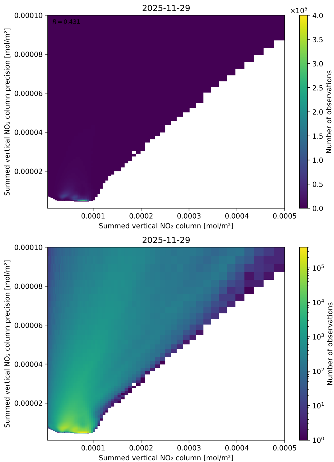
Figure 105: Scatter density plot of “Summed vertical NO 2 column” against “Summed vertical NO 2 column precision” for 2025-11-28 to 2025-11-30.
