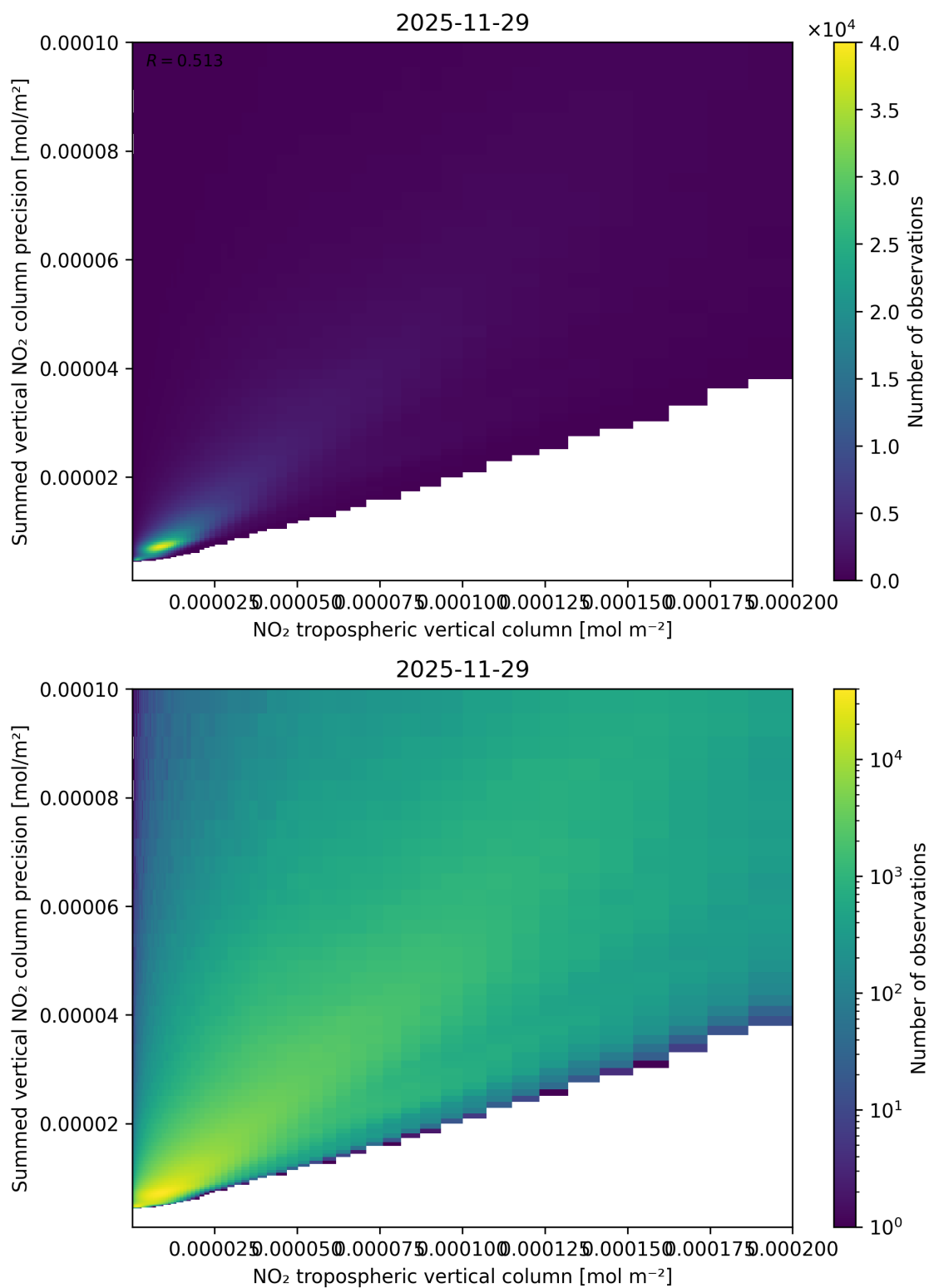
Figure 127: Scatter density plot of “NO 2 tropospheric vertical column” against “Summed vertical NO 2 column precision” for 2025-11-28 to 2025-11-30.
