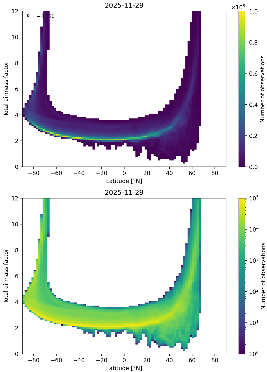
Figure 84: Scatter density plot of “Latitude” against “Total airmass factor” for 2025-11-28 to 2025-11-30.
