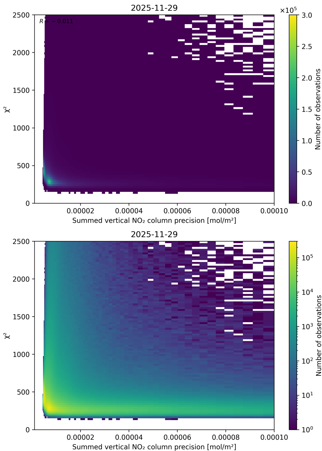
Figure 107: Scatter density plot of “Summed vertical NO 2 column precision” against “ \chi^2 ” for 2025-11-28 to 2025-11-30.
