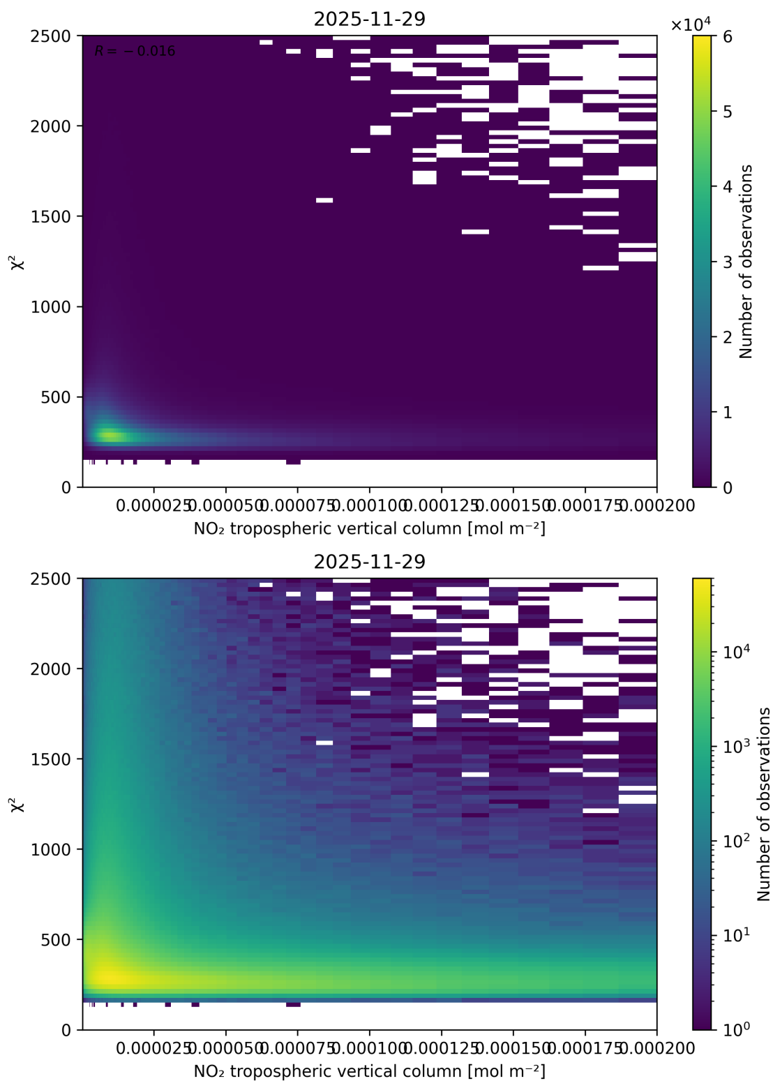
Figure 124: Scatter density plot of “NO 2 tropospheric vertical column” against “ \chi^2 ” for 2025-11-28 to 2025-11-30.
