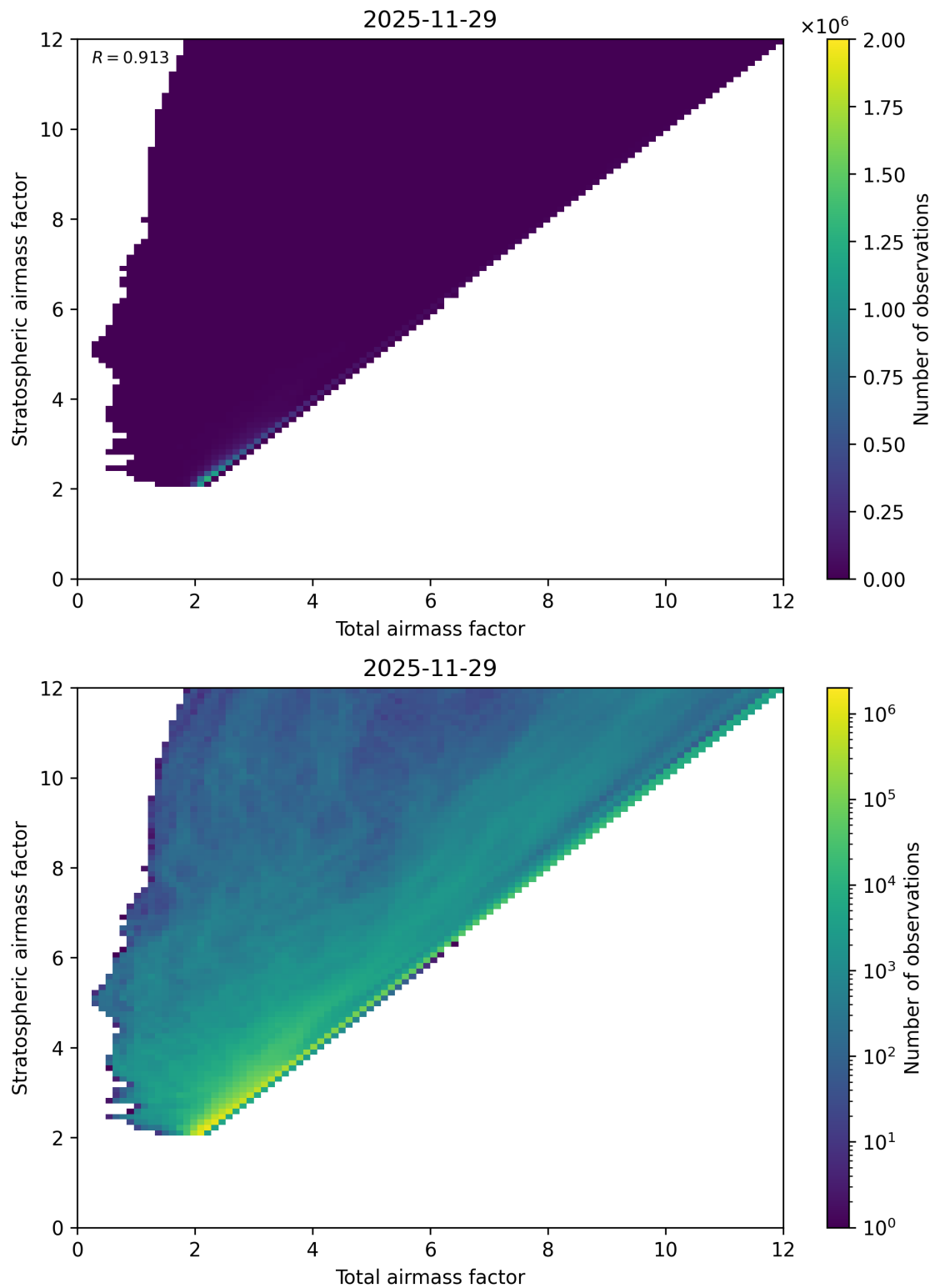
Figure 62: Scatter density plot of “Total airmass factor” against “Stratospheric airmass factor” for 2025-11-28 to 2025-11-30.
