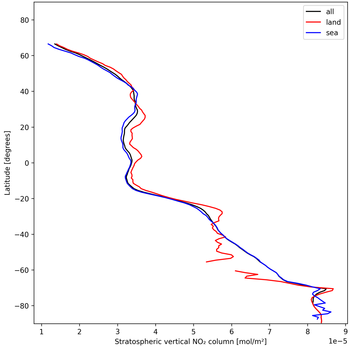
Figure 19: Zonal average of “Stratospheric vertical NO 2 column” for 2025-11-28 to 2025-11-30.
