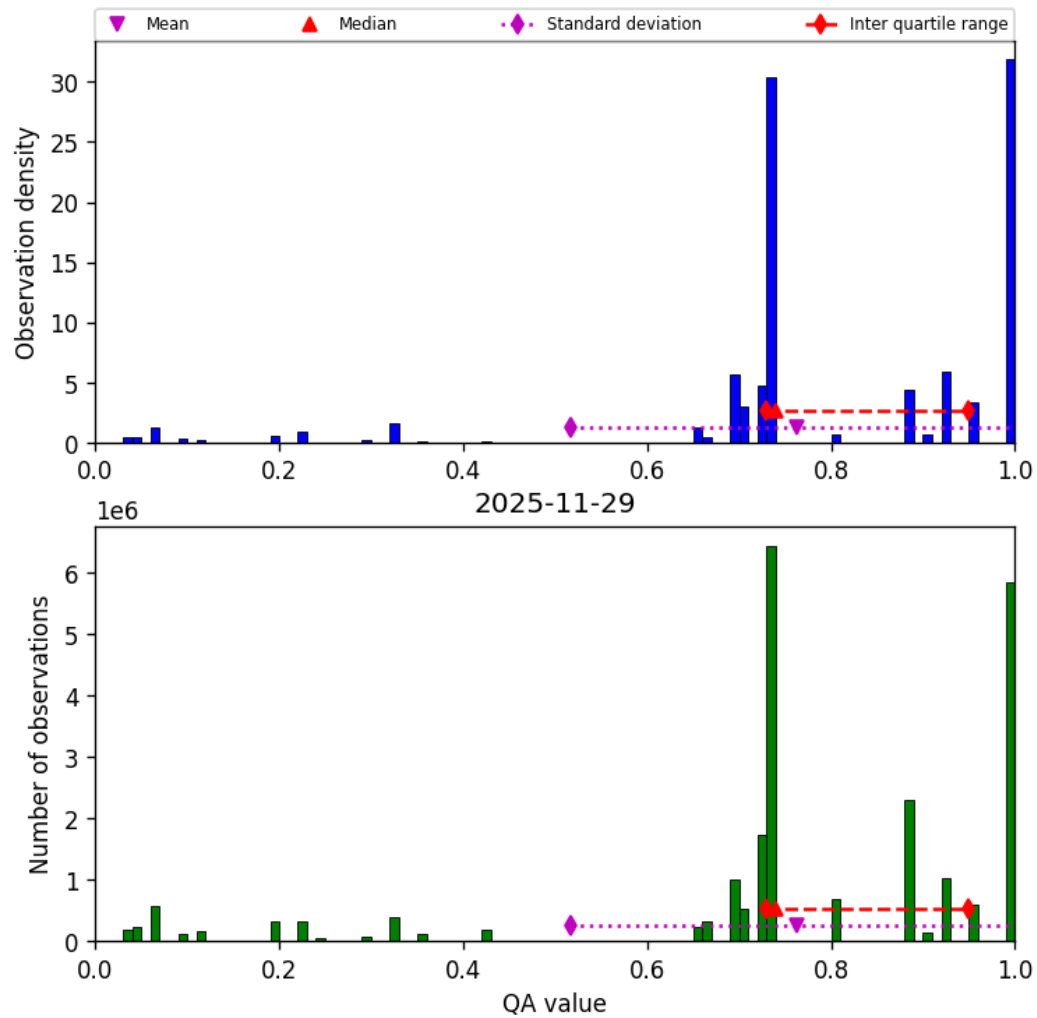
Figure 28: Histogram of “QA value” for 2025-11-28 to 2025-11-30
