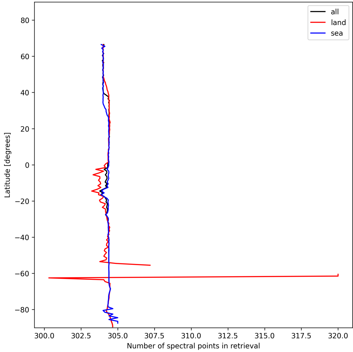
Figure 16: Zonal average of “Number of spectral points in retrieval” for 2025-11-28 to 2025-11-30.
