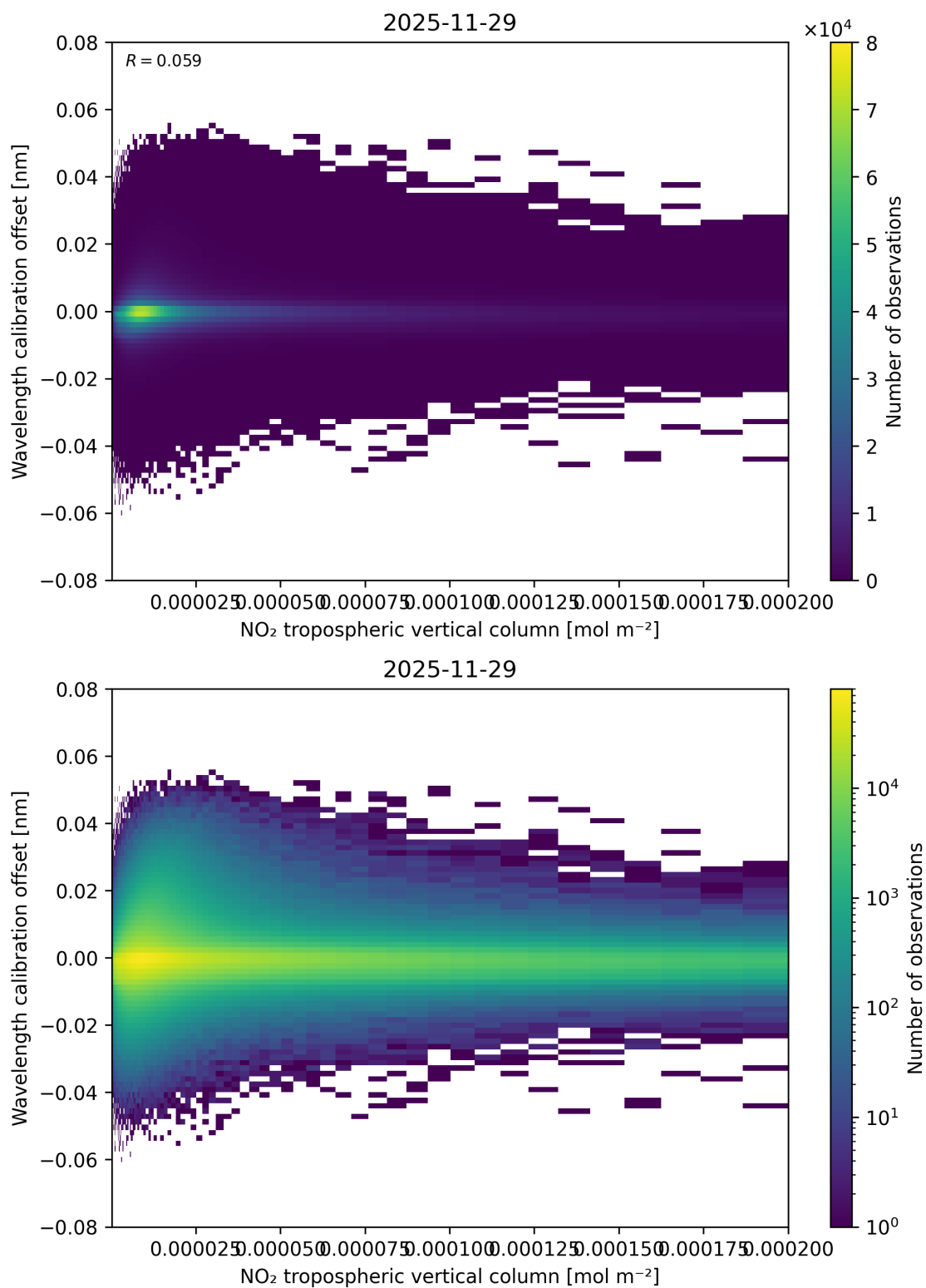
Figure 143: Scatter density plot of “NO 2 tropospheric vertical column” against “Wavelength calibration offset” for 2025-11-28 to 2025-11-30.
