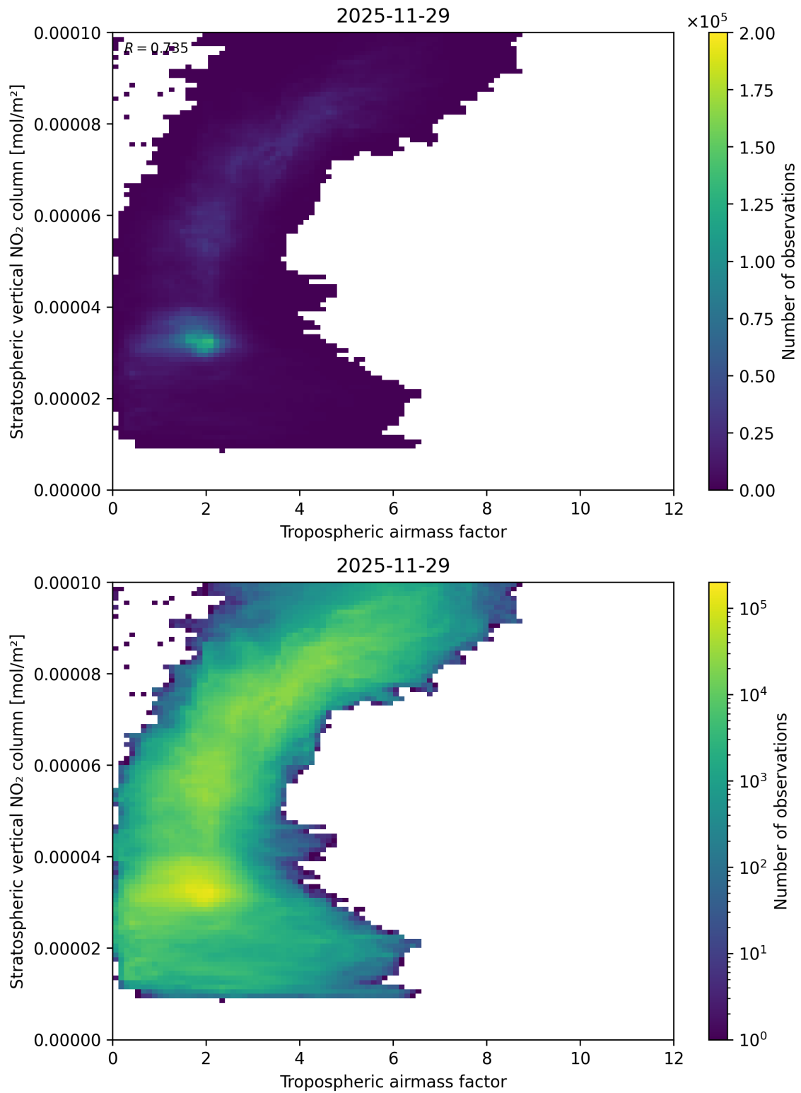
Figure 74: Scatter density plot of “Tropospheric airmass factor” against “Stratospheric vertical NO 2 column” for 2025-11-28 to 2025-11-30.
