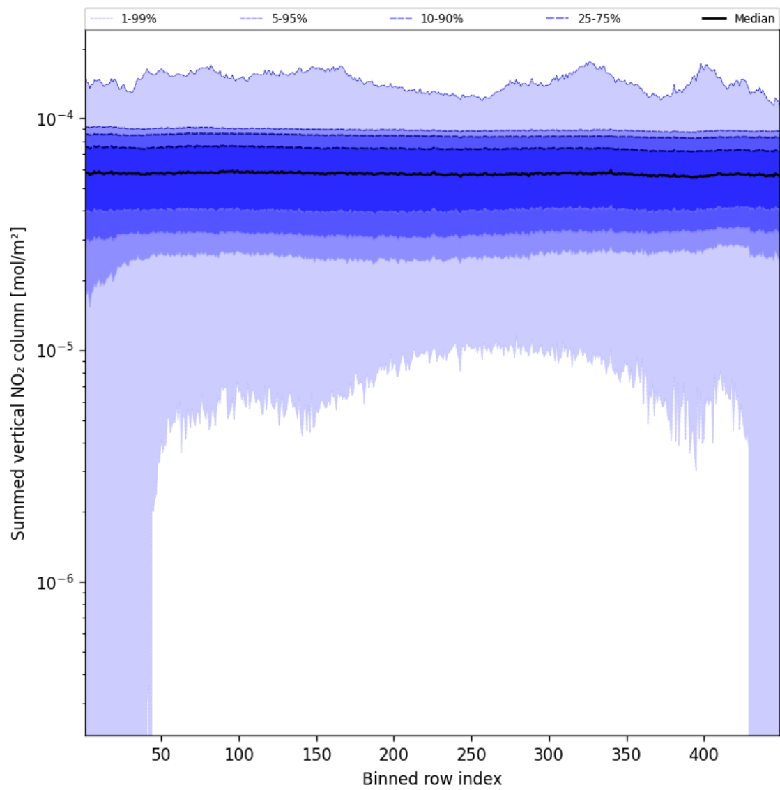
Figure 57: Along track statistics of “Summed vertical NO 2 column” for 2025-11-28 to 2025-11-30
