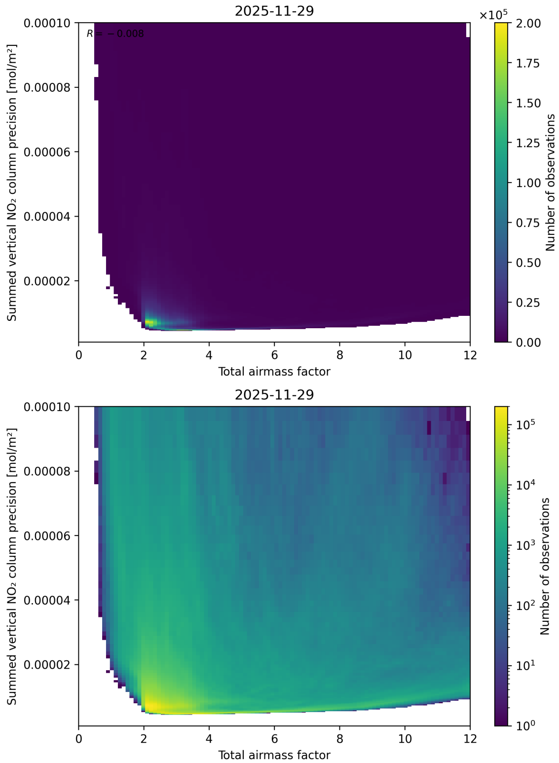
Figure 66: Scatter density plot of “Total airmass factor” against “Summed vertical NO 2 column precision” for 2025-11-28 to 2025-11-30.
