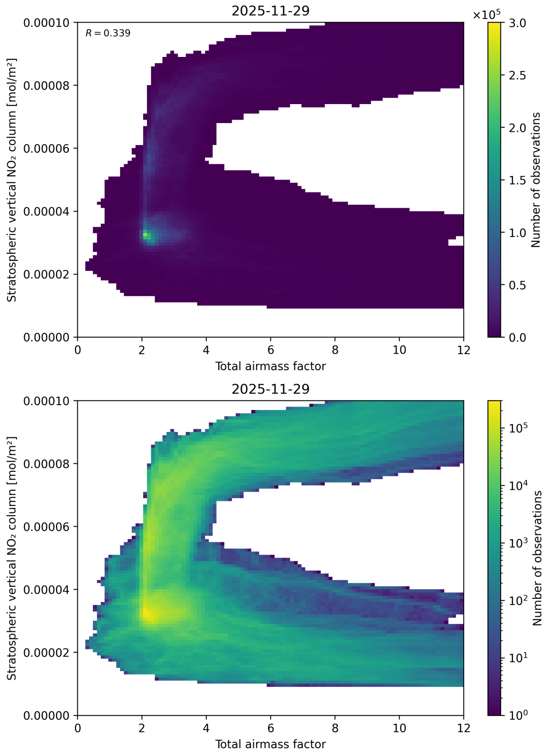
Figure 64: Scatter density plot of “Total airmass factor” against “Stratospheric vertical \text{NO}_2 column” for 2025-11-28 to 2025-11-30.
