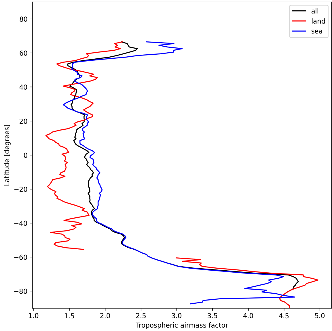
Figure 14: Zonal average of “Tropospheric air mass factor” for 2025-11-28 to 2025-11-30.
