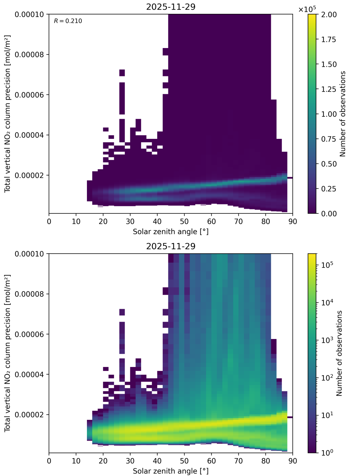
Figure 154: Scatter density plot of “Solar zenith angle” against “Total vertical NO 2 column precision” for 2025-11-28 to 2025-11-30.
