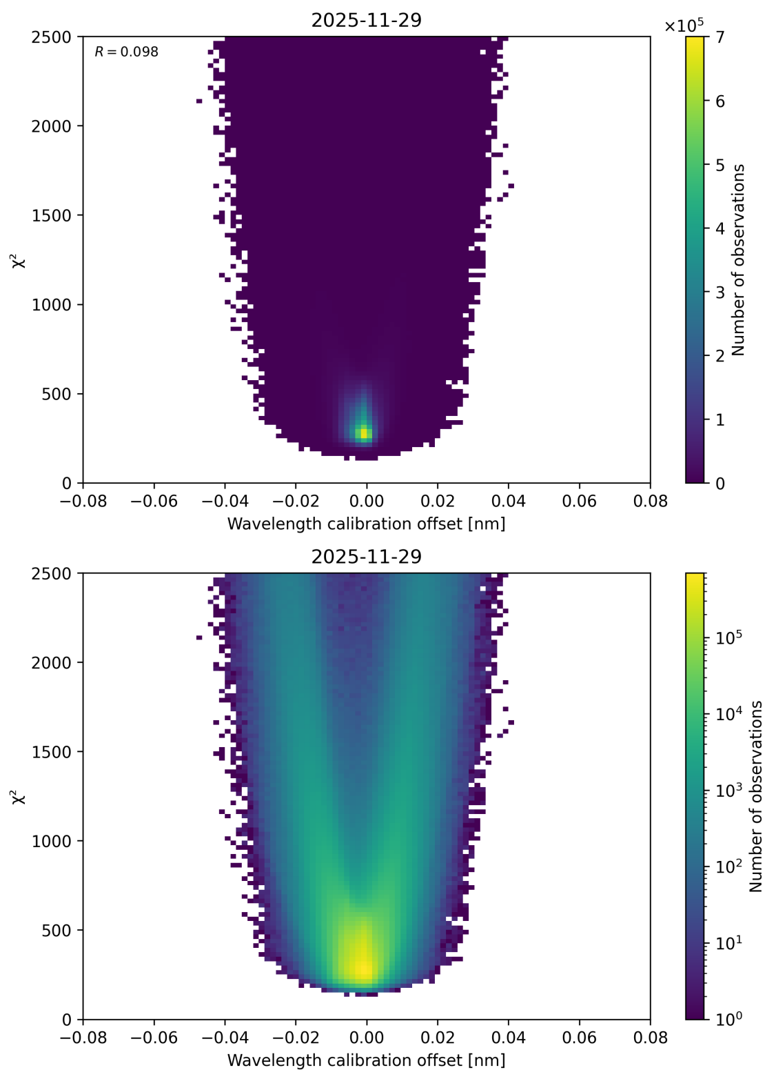
Figure 175: Scatter density plot of “Wavelength calibration offset” against “ \chi^2 ” for 2025-11-28 to 2025-11-30.
