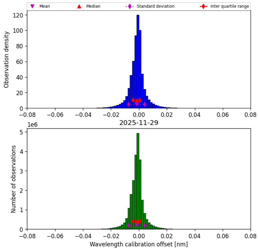
Figure 35: Histogram of “Wavelength calibration offset” for 2025-11-28 to 2025-11-30
