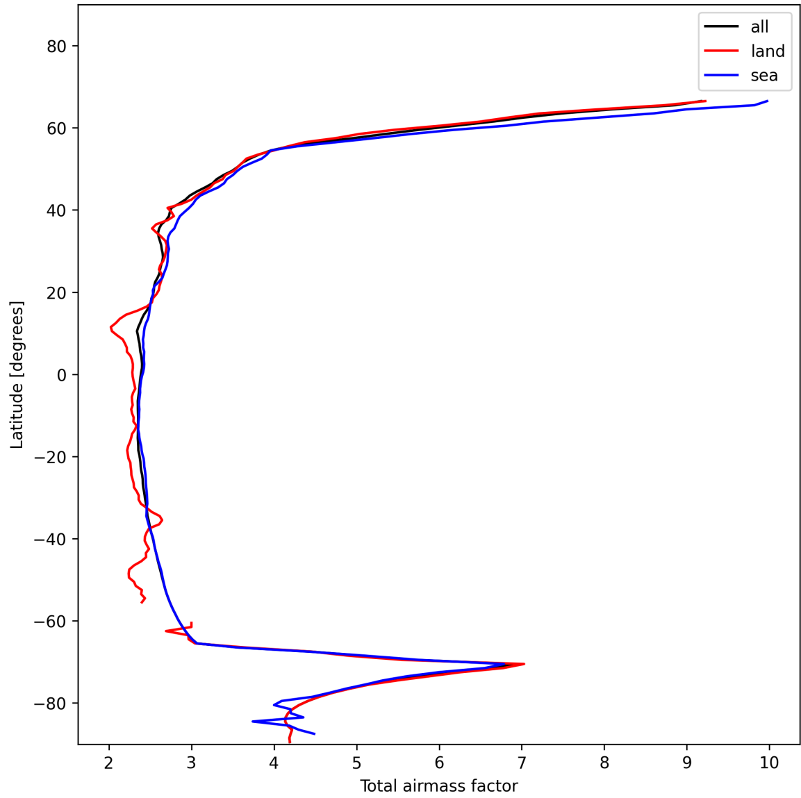
Figure 15: Zonal average of “Total airmass factor” for 2025-11-28 to 2025-11-30.
