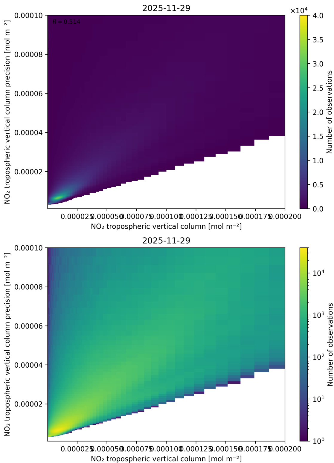
Figure 130: Scatter density plot of “NO 2 tropospheric vertical column” against “NO 2 tropospheric vertical column precision” for 2025-11-28 to 2025-11-30.
