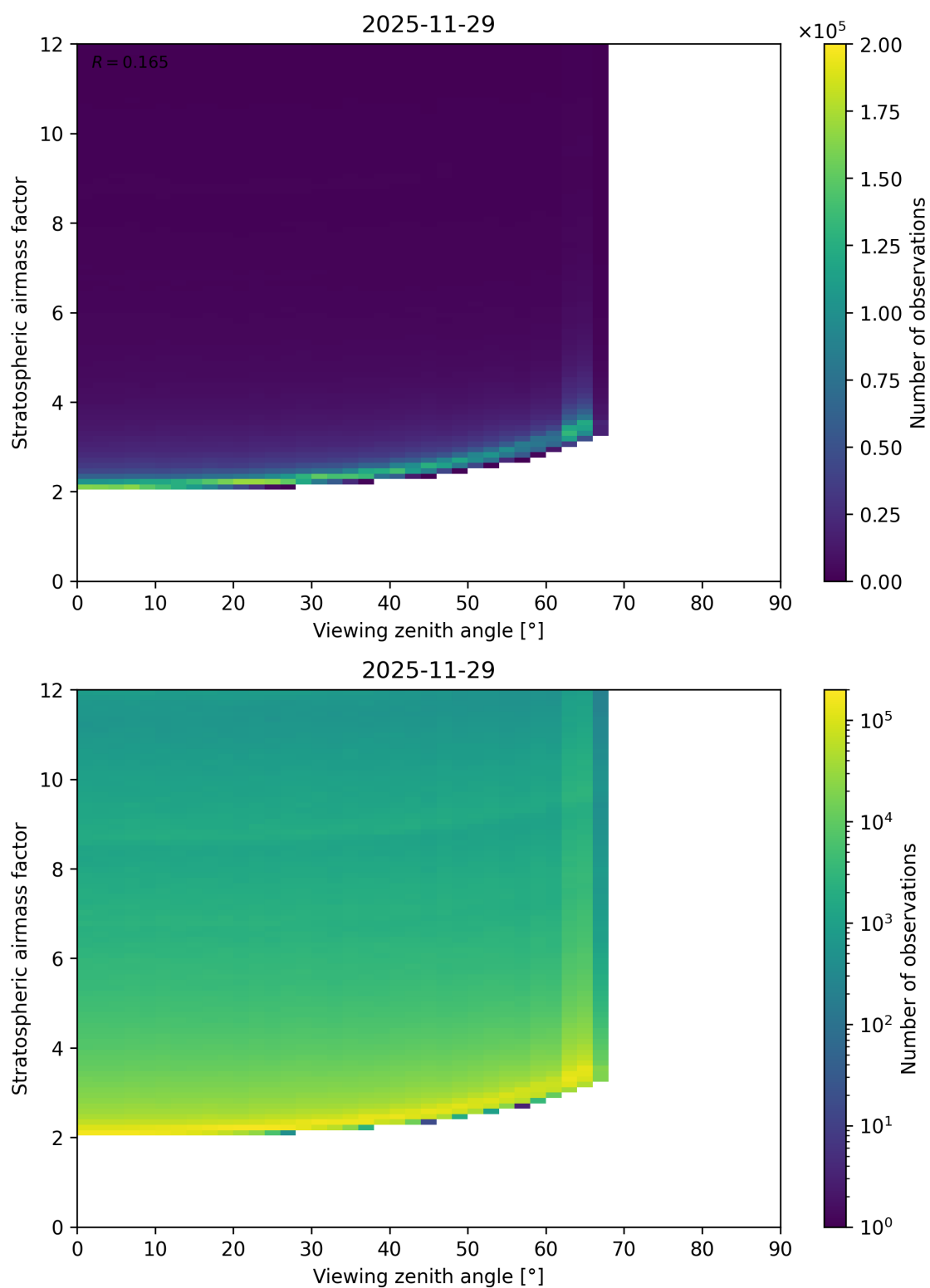
Figure 159: Scatter density plot of “Viewing zenith angle” against “Stratospheric airmass factor” for 2025-11-28 to 2025-11-30.
