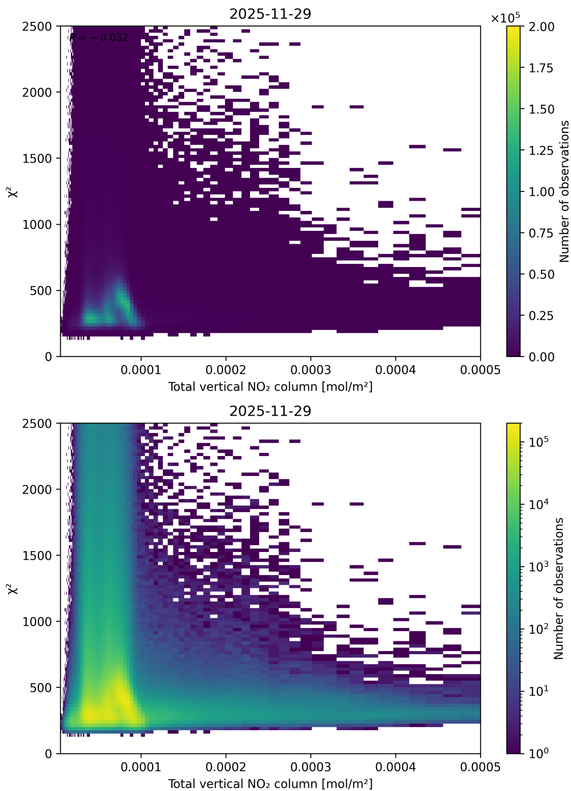
Figure 111: Scatter density plot of “Total vertical NO 2 column” against “ \chi^2 ” for 2025-11-28 to 2025-11-30.
