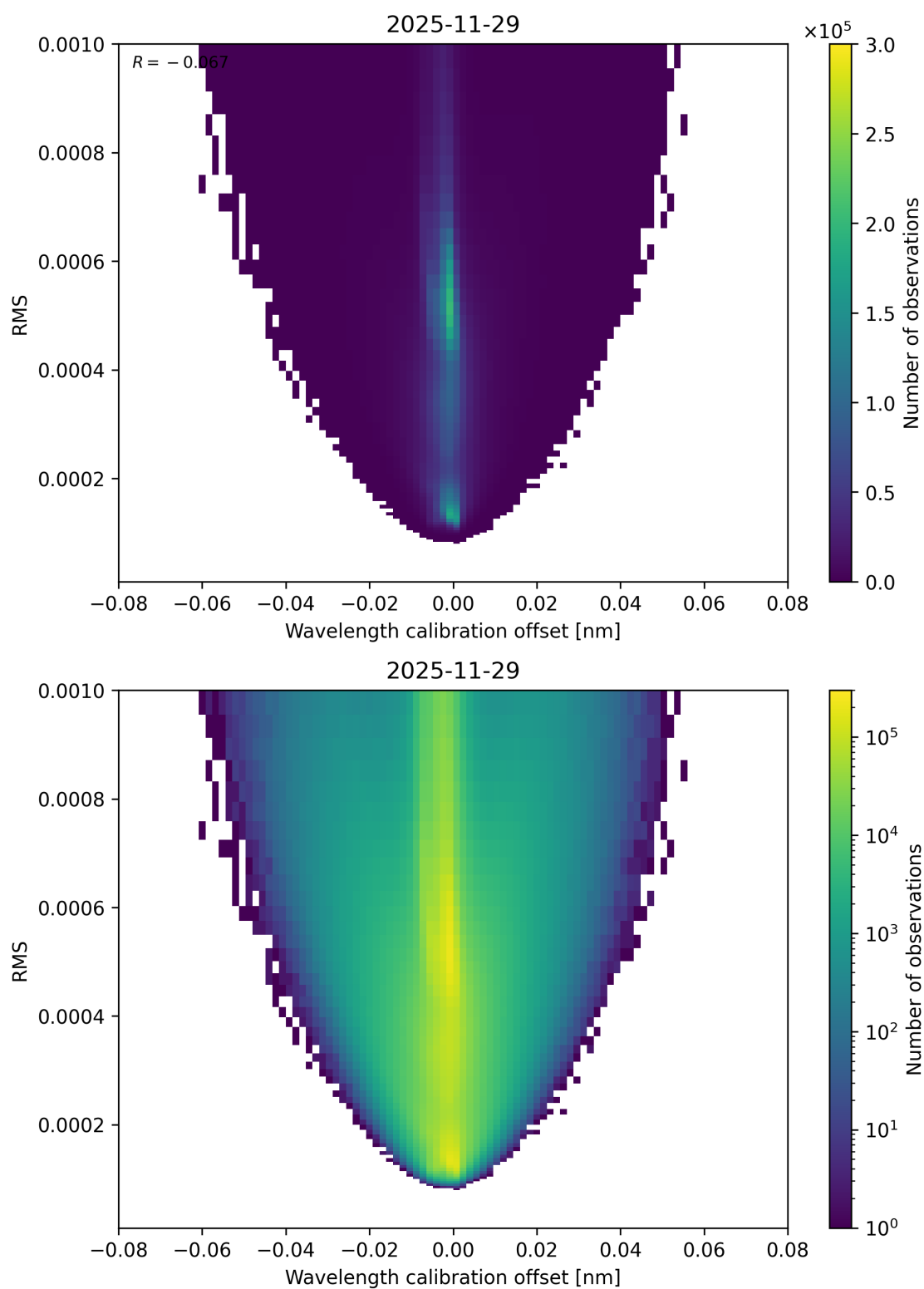
Figure 181: Scatter density plot of “Wavelength calibration offset” against “RMS” for 2025-11-28 to 2025-11-30.
