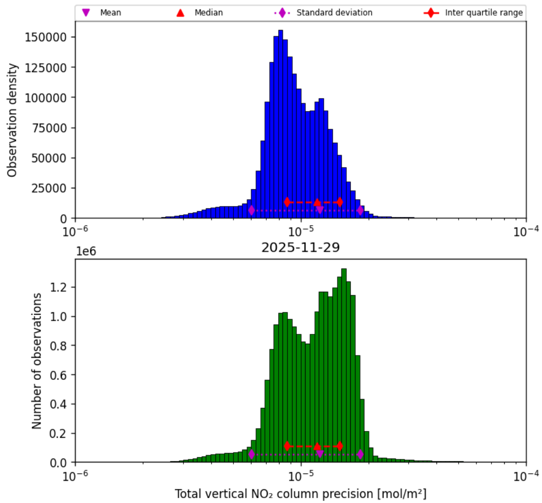
Figure 39: Histogram of “Total vertical NO 2 column precision” for 2025-11-28 to 2025-11-30
