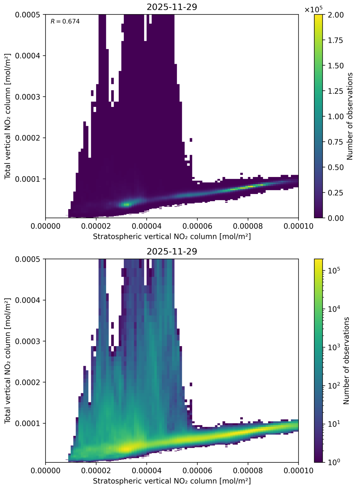
Figure 100: Scatter density plot of “Stratospheric vertical NO 2 column” against “Total vertical NO 2 column” for 2025-11-28 to 2025-11-30.
