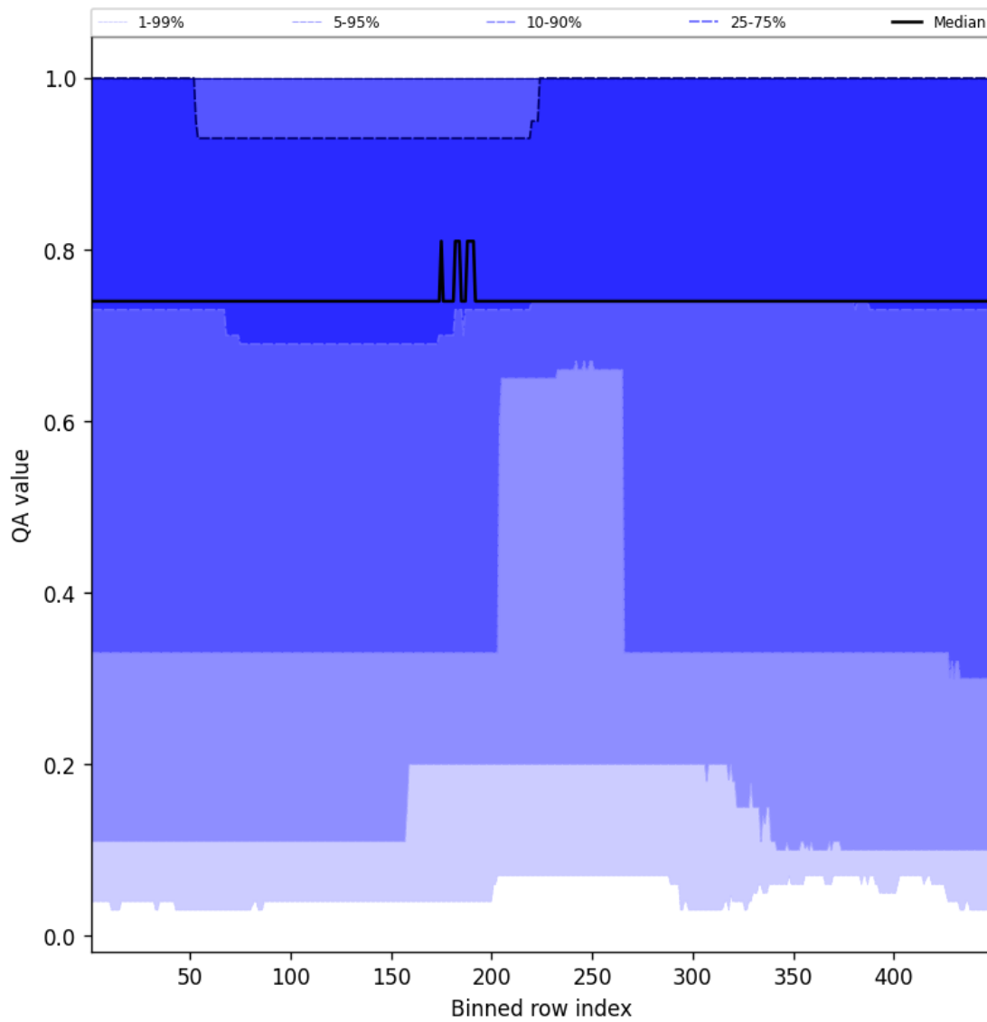
Figure 45: Along track statistics of “QA value” for 2025-11-28 to 2025-11-30
