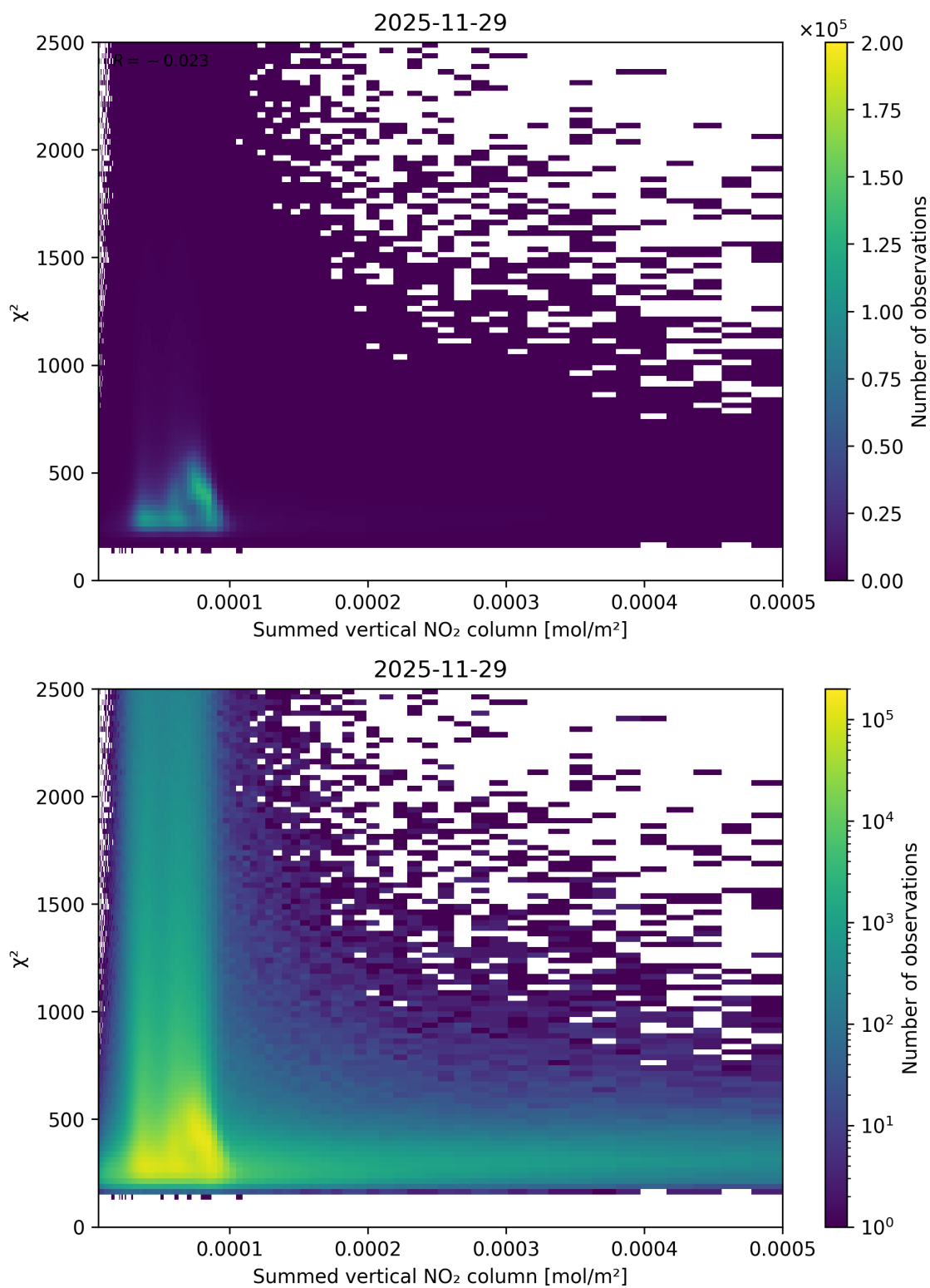
Figure 104: Scatter density plot of “Summed vertical NO 2 column” against “ \chi^2 ” for 2025-11-28 to 2025-11-30.
