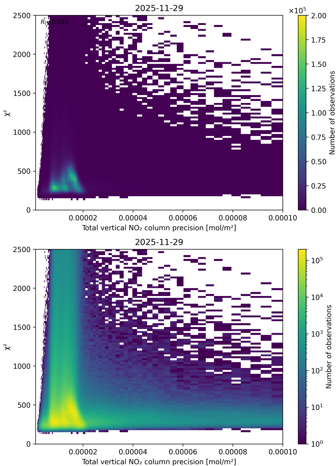
Figure 116: Scatter density plot of “Total vertical NO 2 column precision” against “ \chi^2 ” for 2025-11-28 to 2025-11-30.
