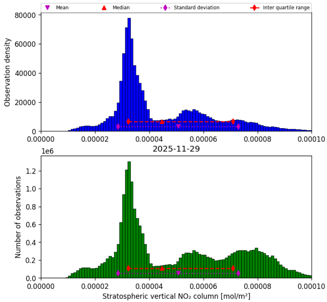
Figure 36: Histogram of “Stratospheric vertical NO 2 column” for 2025-11-28 to 2025-11-30
