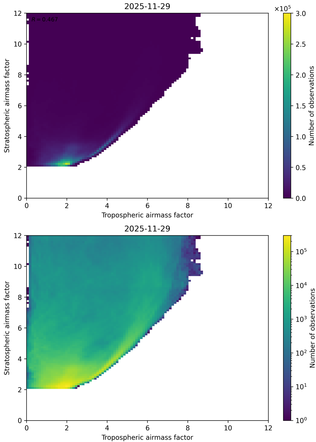
Figure 71: Scatter density plot of “Tropospheric airmass factor” against “Stratospheric airmass factor” for 2025-11-28 to 2025-11-30.
