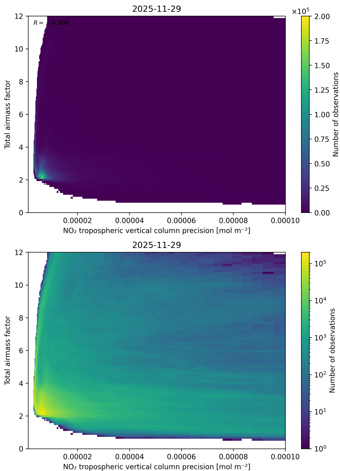
Figure 132: Scatter density plot of “NO 2 tropospheric vertical column precision” against “Total air mass factor” for 2025-11-28 to 2025-11-30.
