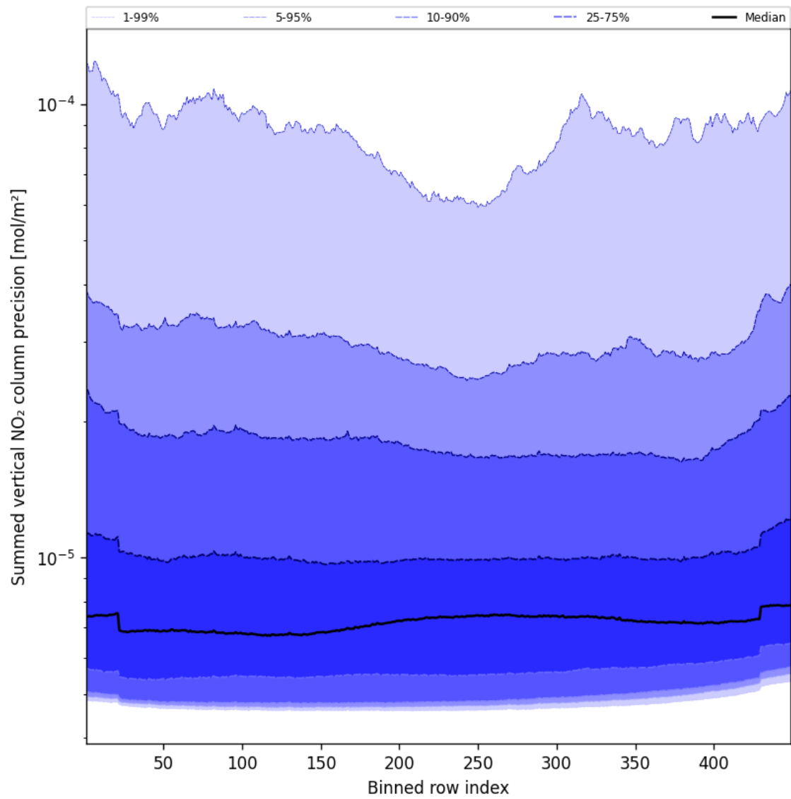
Figure 58: Along track statistics of “Summed vertical NO 2 column precision” for 2025-11-28 to 2025-11-30
