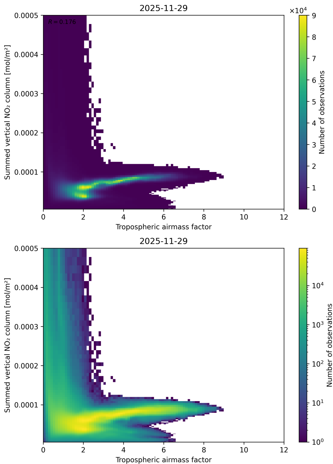
Figure 75: Scatter density plot of “Tropospheric airmass factor” against “Summed vertical NO 2 column” for 2025-11-28 to 2025-11-30.
