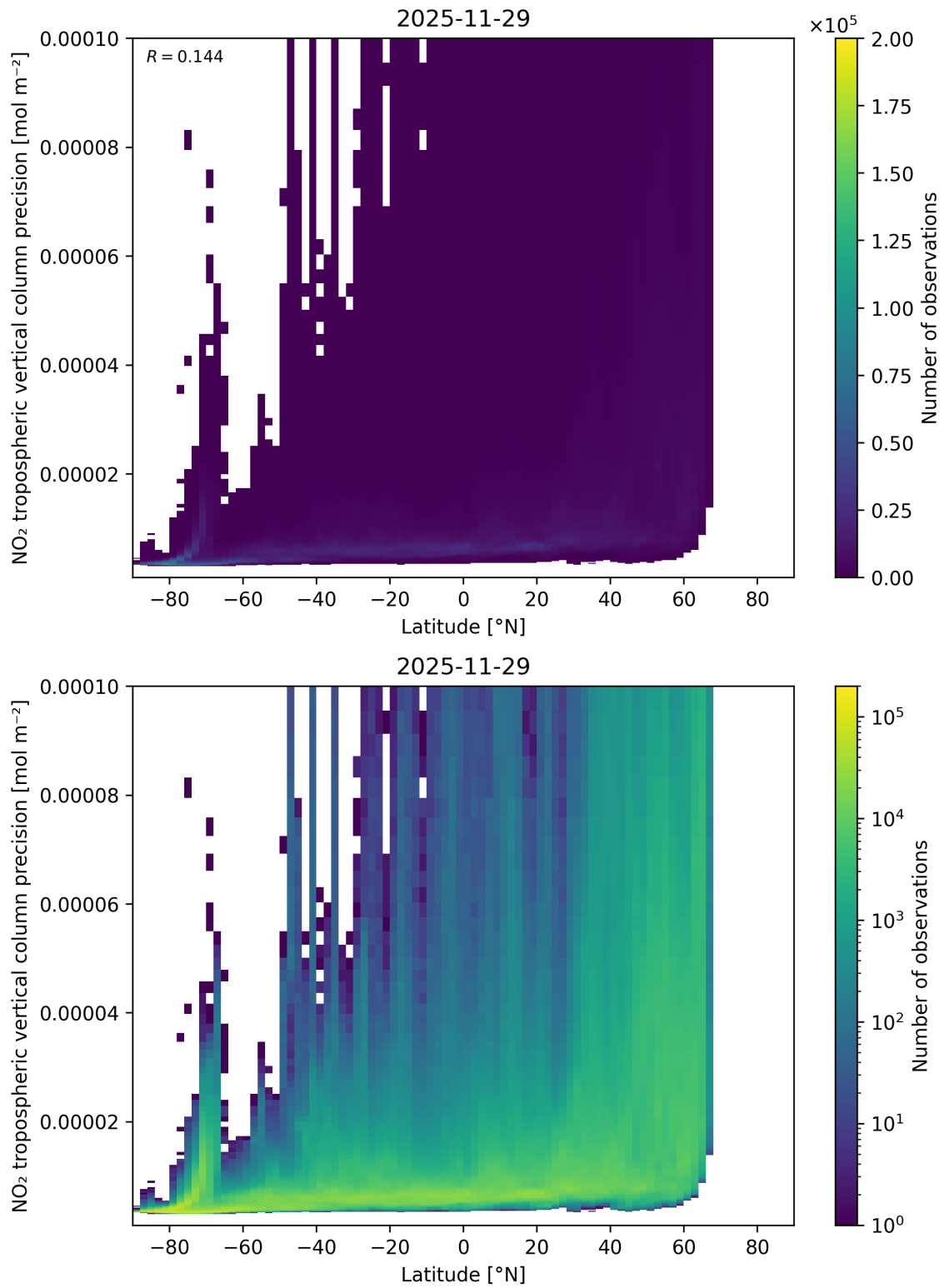
Figure 93: Scatter density plot of “Latitude” against “NO 2 tropospheric vertical column precision” for 2025-11-28 to 2025-11-30.
