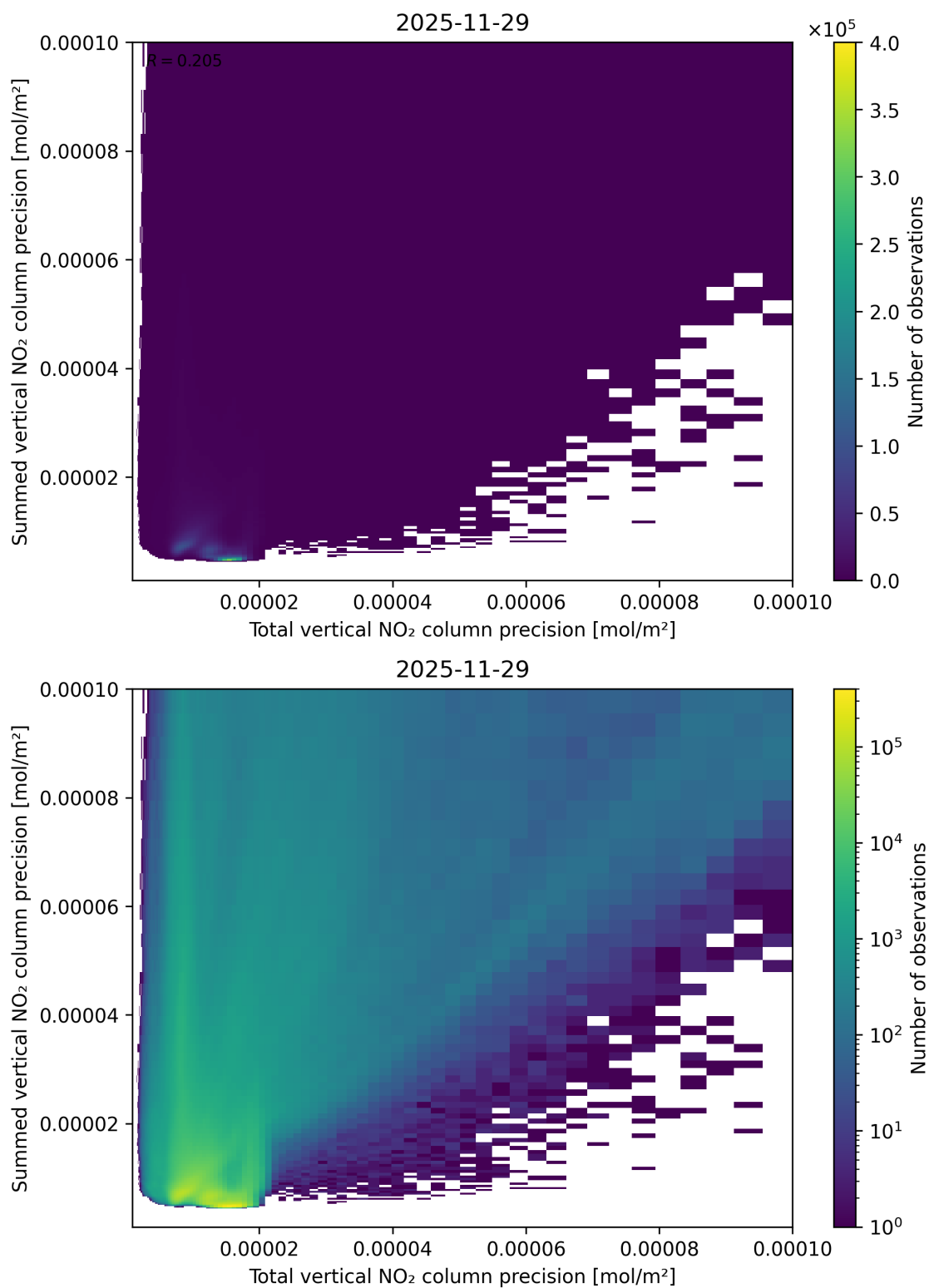
Figure 118: Scatter density plot of “Total vertical NO 2 column precision” against “Summed vertical NO 2 column precision” for 2025-11-28 to 2025-11-30.
