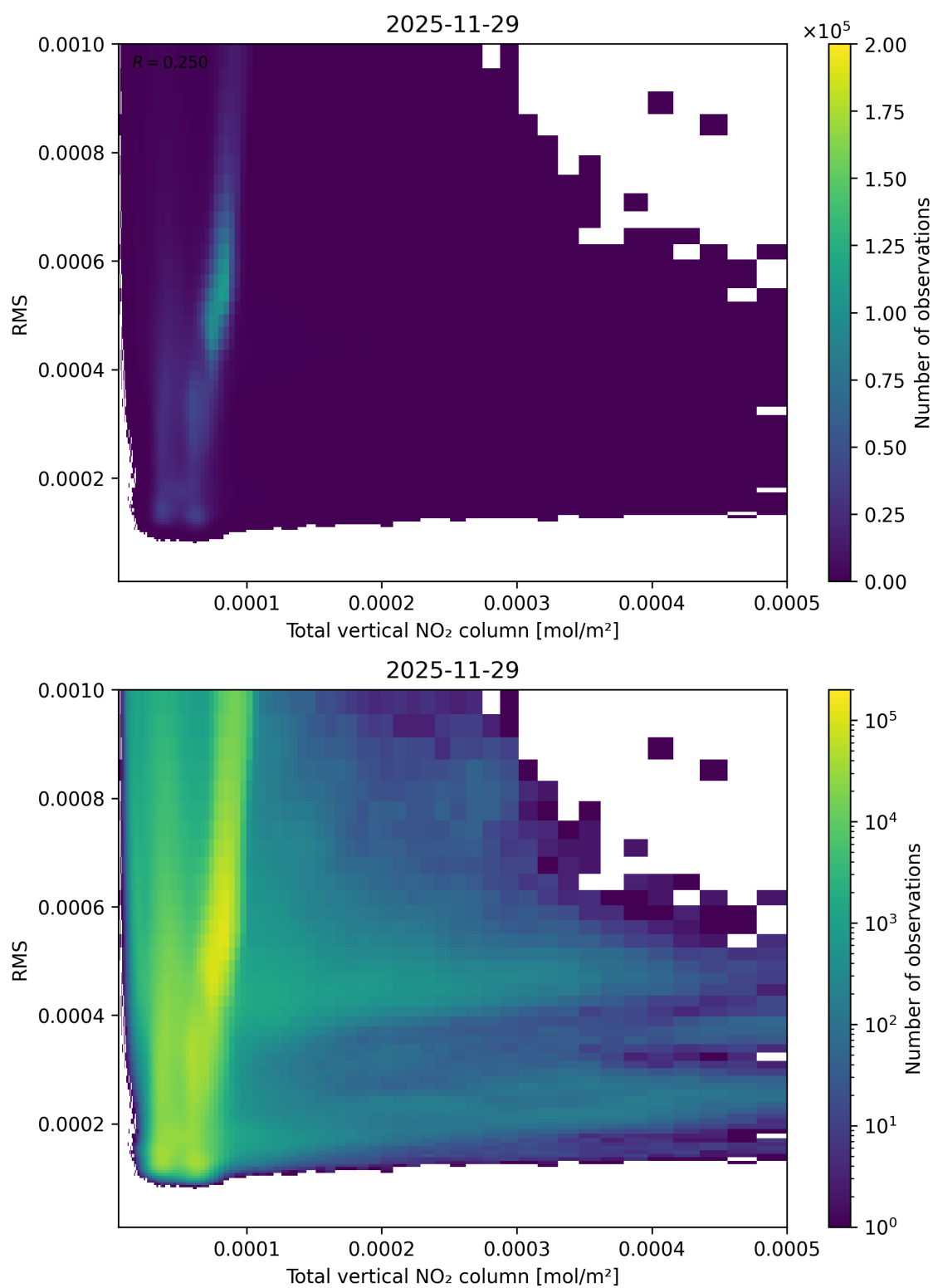
Figure 120: Scatter density plot of “Total vertical NO 2 column” against “RMS” for 2025-11-28 to 2025-11-30.
