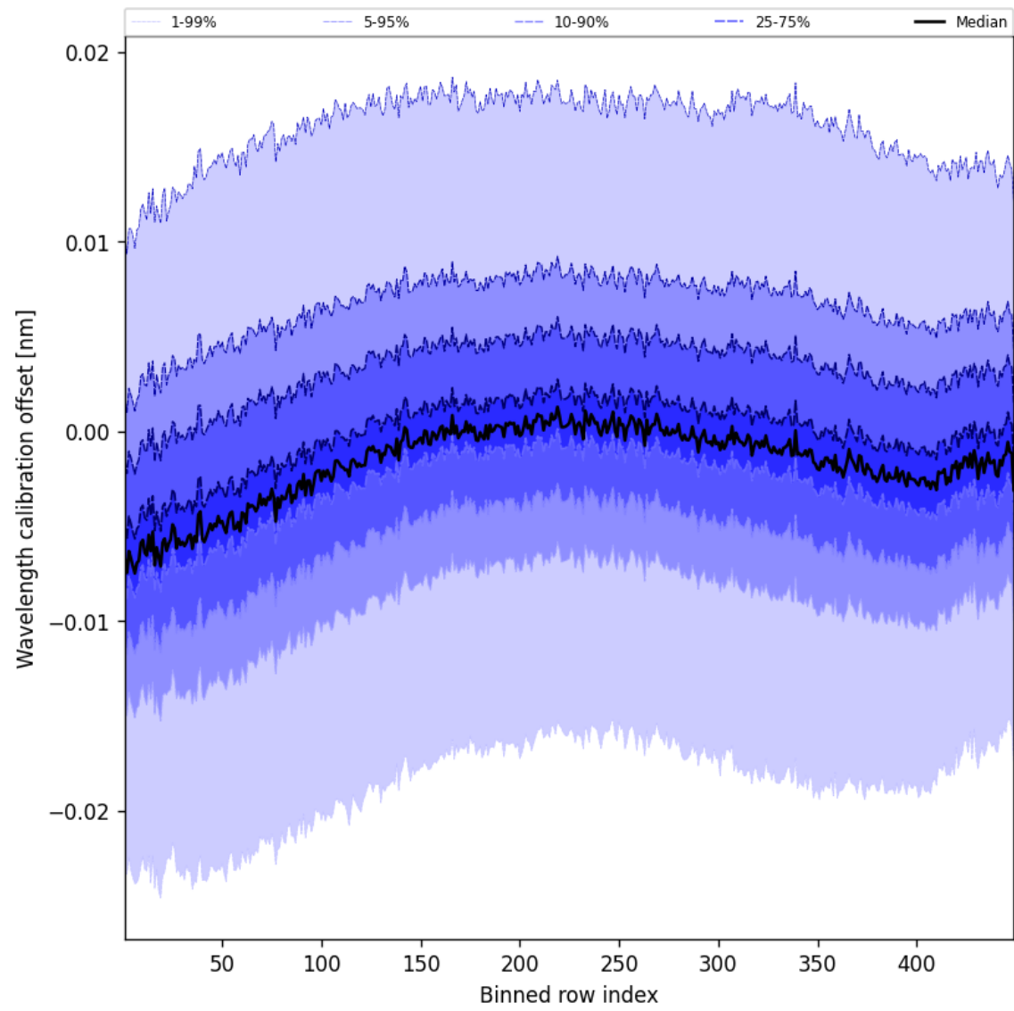
Figure 52: Along track statistics of “Wavelength calibration offset” for 2025-11-28 to 2025-11-30
