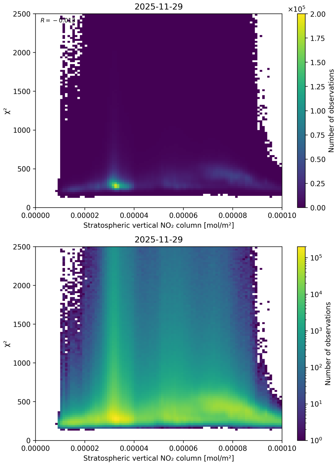
Figure 97: Scatter density plot of “Stratospheric vertical NO 2 column” against “ \chi^2 ” for 2025-11-28 to 2025-11-30.
