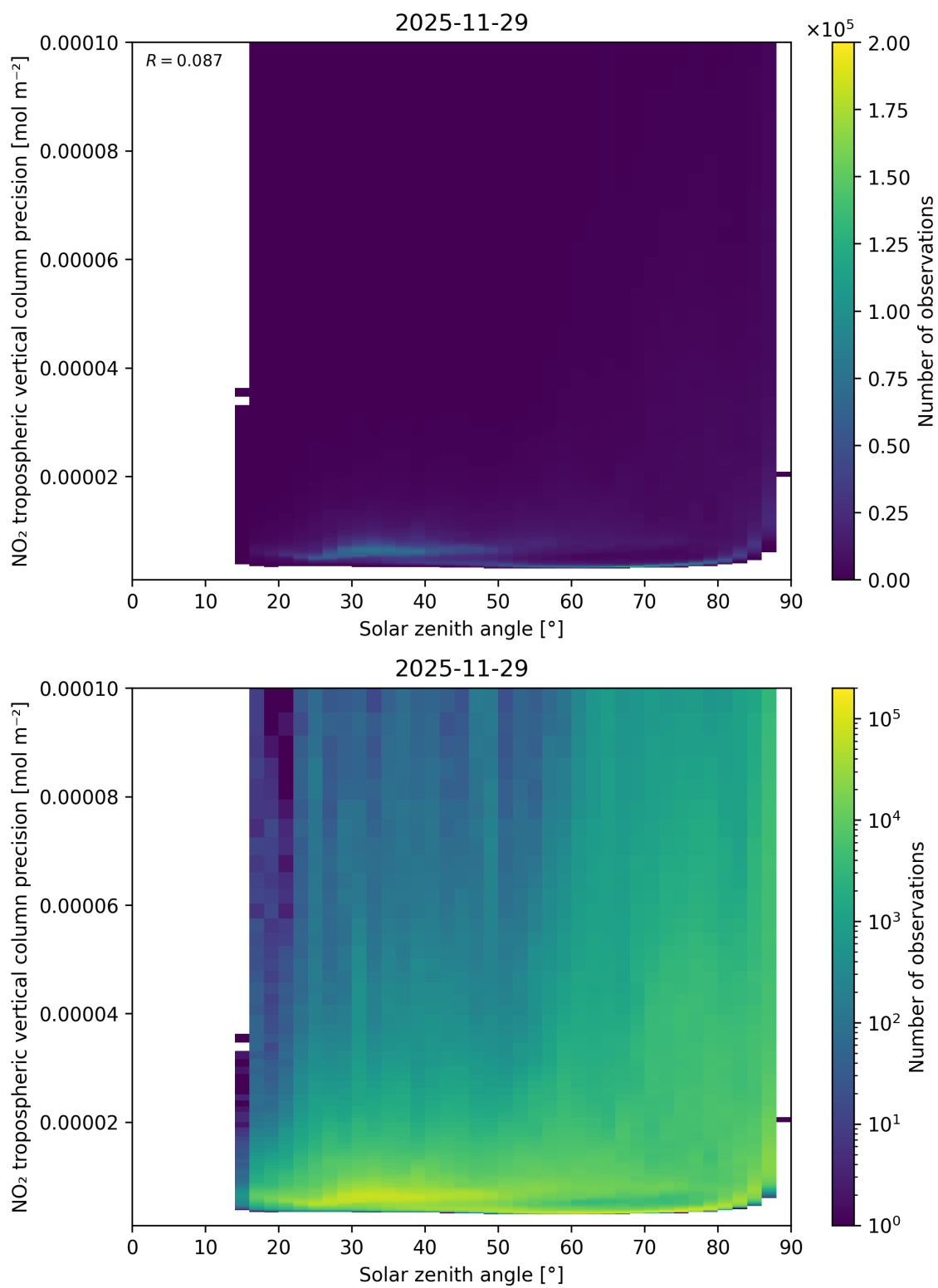
Figure 156: Scatter density plot of “Solar zenith angle” against “NO 2 tropospheric vertical column precision” for 2025-11-28 to 2025-11-30.
