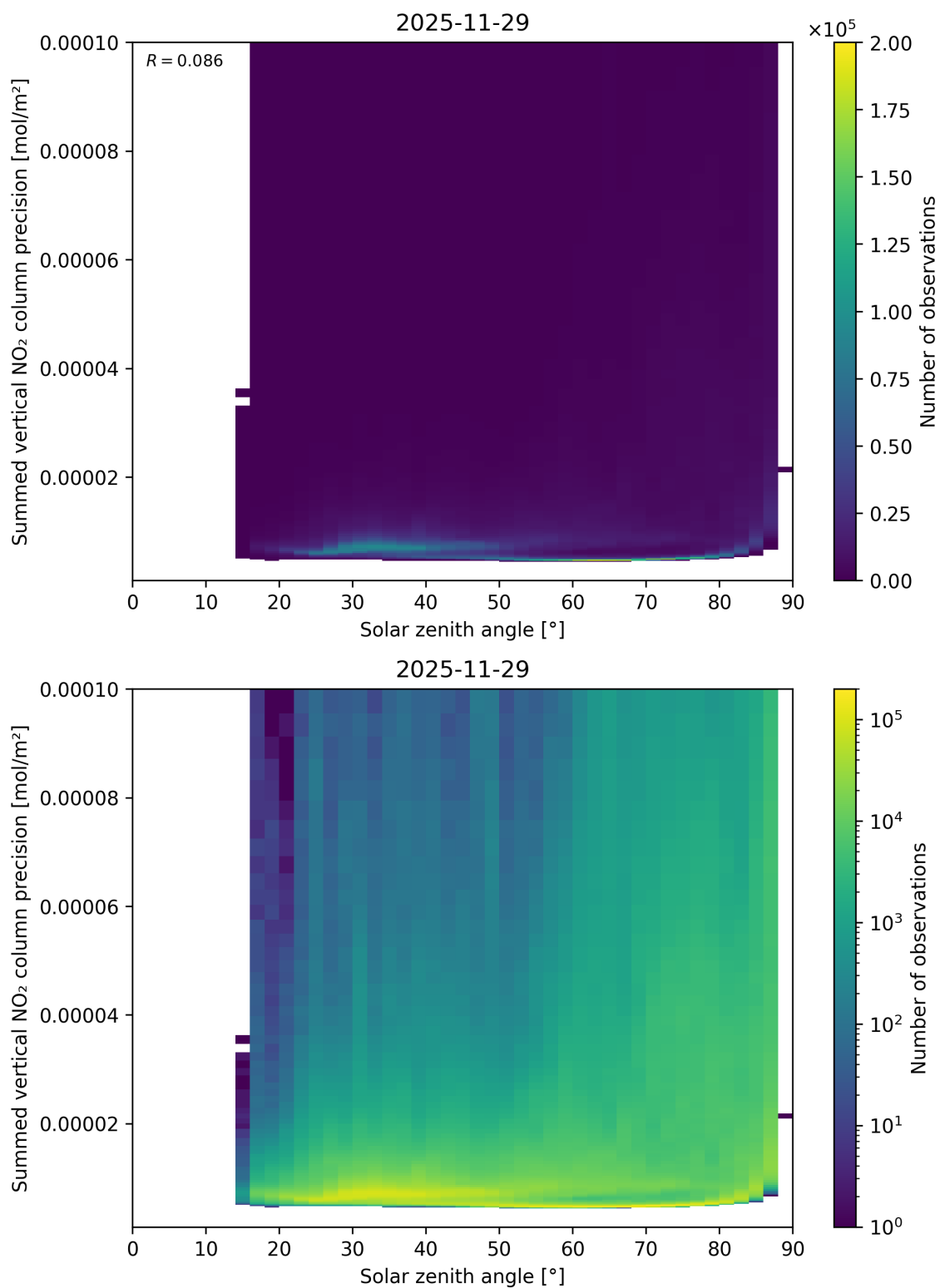
Figure 152: Scatter density plot of “Solar zenith angle” against “Summed vertical NO 2 column precision” for 2025-11-28 to 2025-11-30.
