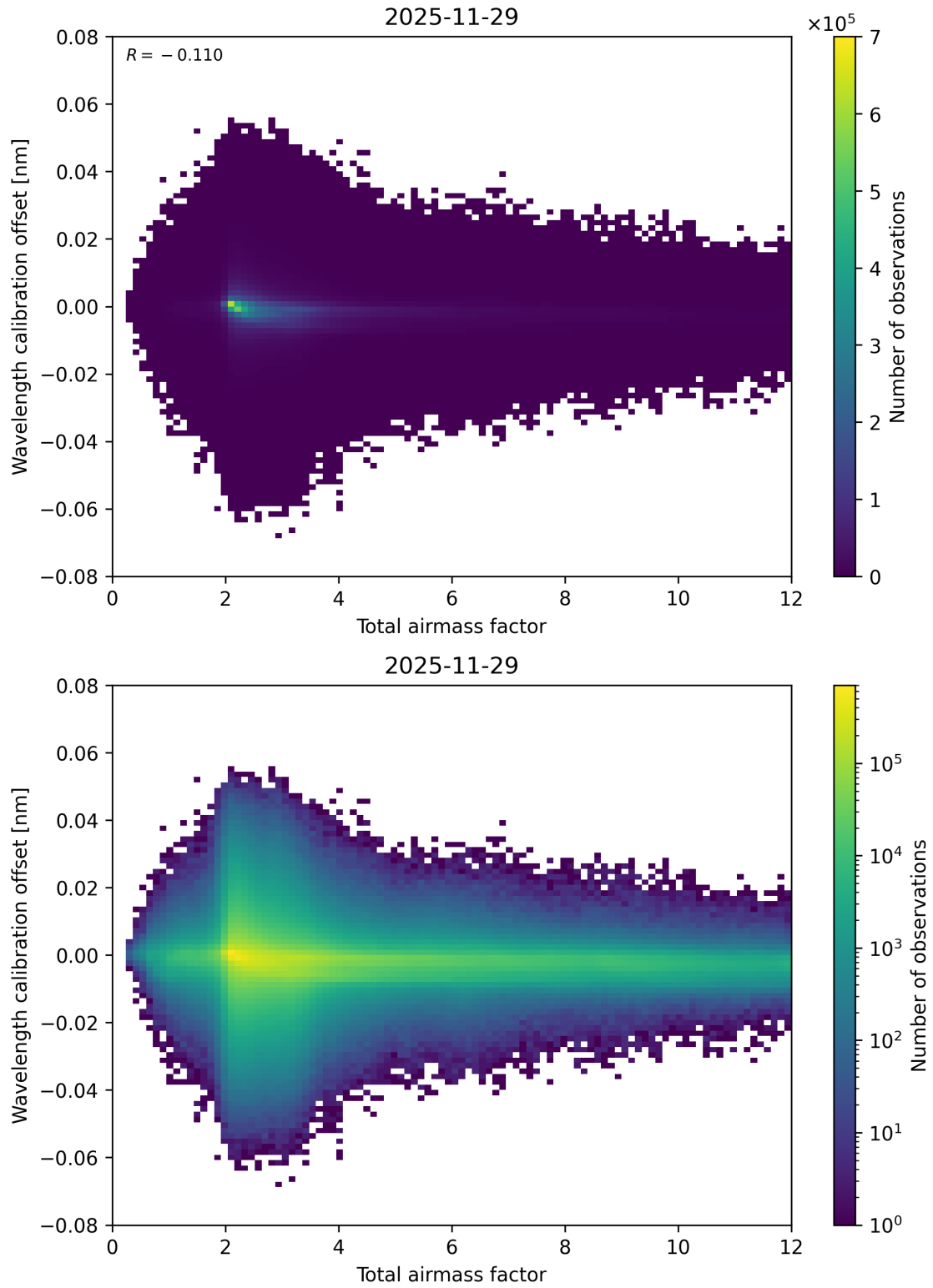
Figure 70: Scatter density plot of “Total airmass factor” against “Wavelength calibration offset” for 2025-11-28 to 2025-11-30.
