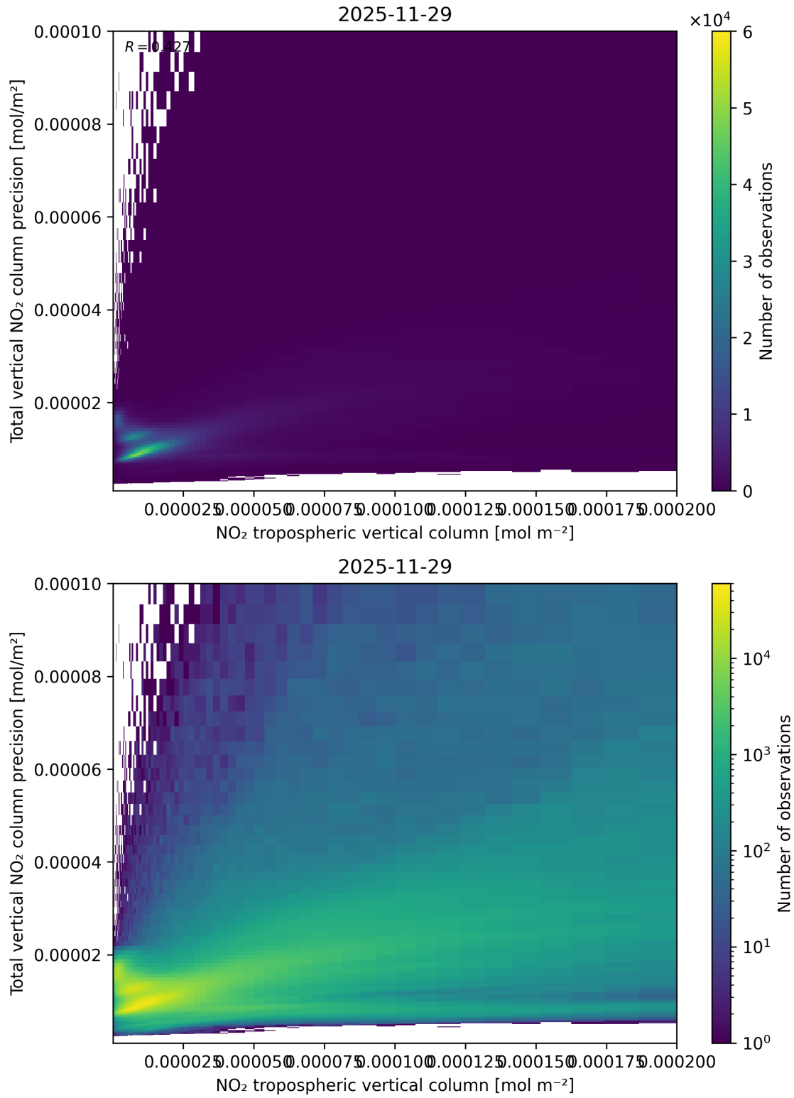
Figure 129: Scatter density plot of “NO 2 tropospheric vertical column” against “Total vertical NO 2 column precision” for 2025-11-28 to 2025-11-30.
