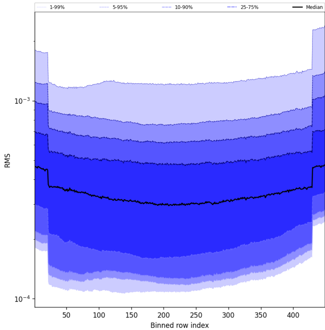
Figure 60: Along track statistics of “RMS” for 2025-11-28 to 2025-11-30
