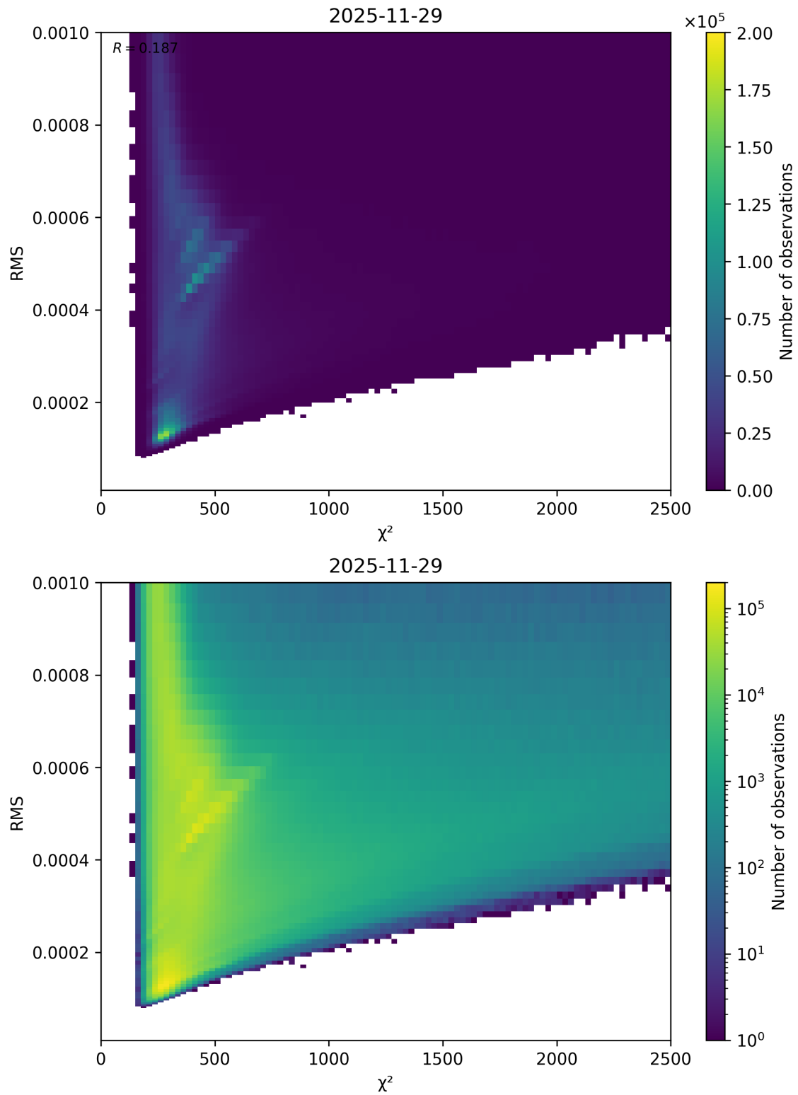
Figure 82: Scatter density plot of “ \chi^2 ” against “RMS” for 2025-11-28 to 2025-11-30.
