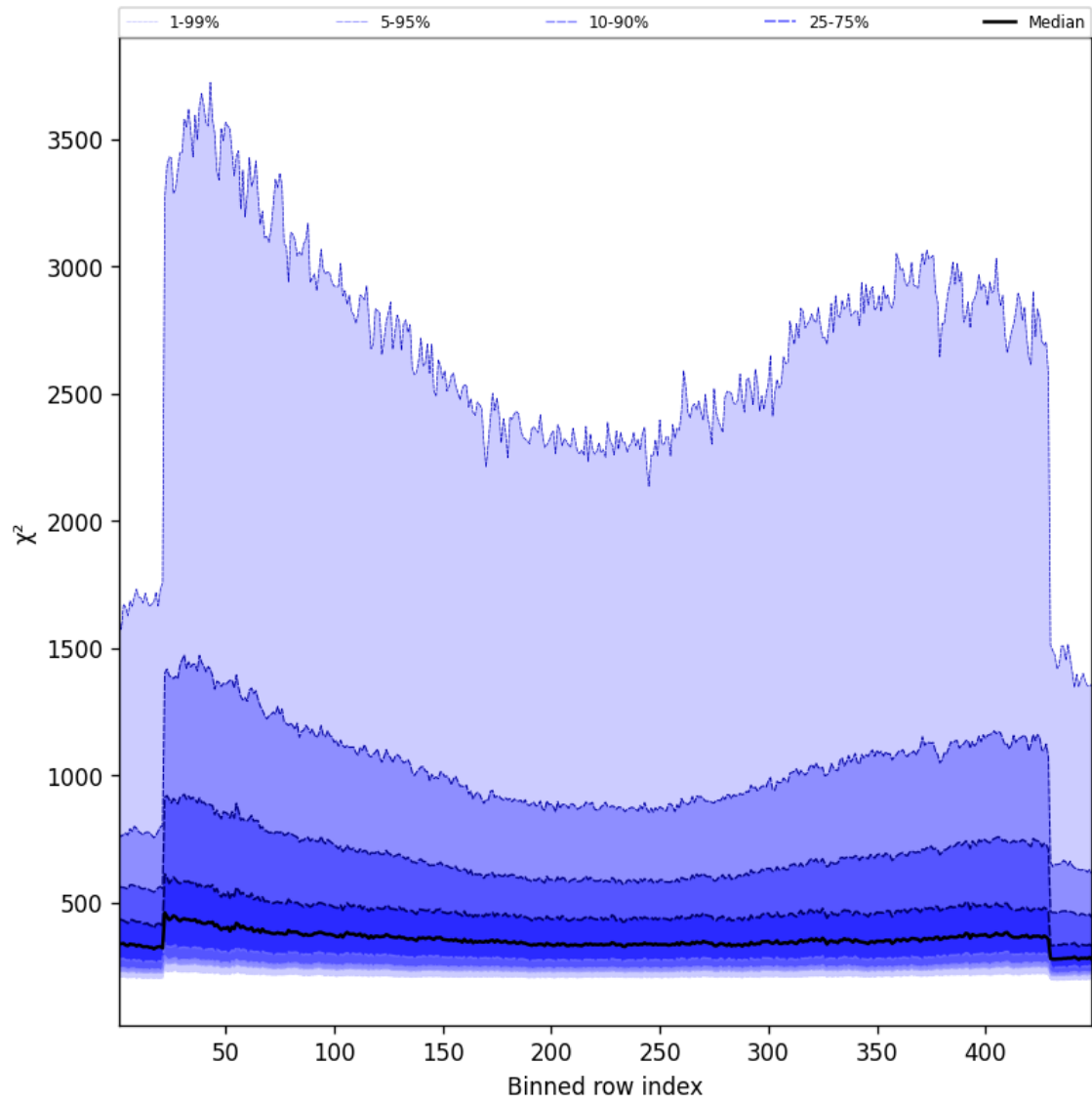
Figure 59: Along track statistics of “ \chi^2 ” for 2025-11-28 to 2025-11-30
