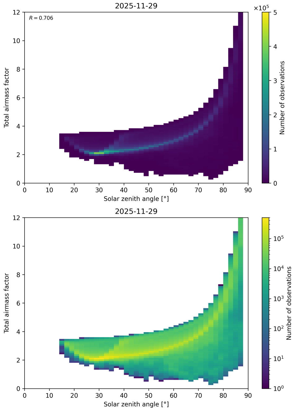
Figure 146: Scatter density plot of “Solar zenith angle” against “Total airmass factor” for 2025-11-28 to 2025-11-30.
