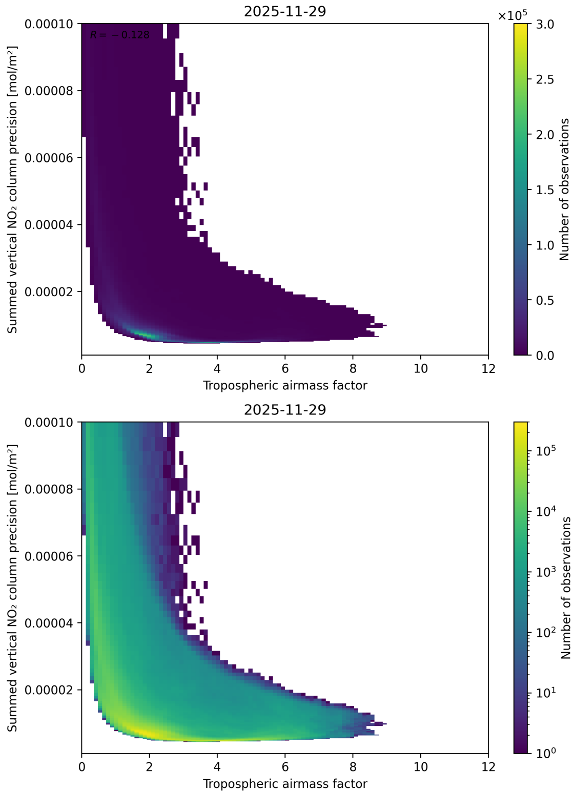
Figure 76: Scatter density plot of “Tropospheric airmass factor” against “Summed vertical NO 2 column precision” for 2025-11-28 to 2025-11-30.
