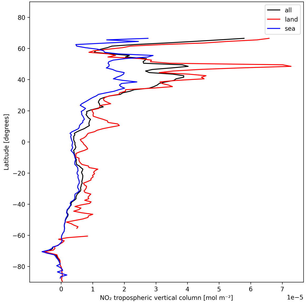
Figure 12: Zonal average of “NO 2 tropospheric vertical column” for 2025-11-28 to 2025-11-30.
