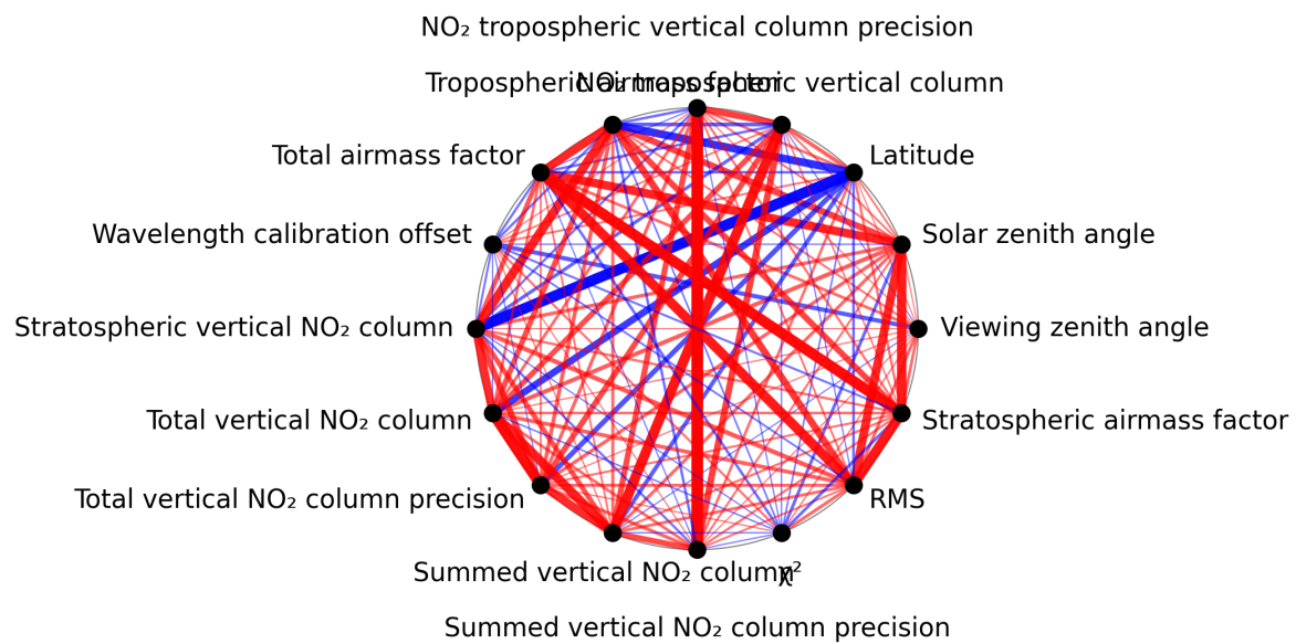
Figure 1: Map of correlation graph for 2025-11-28 to 2025-11-30.
