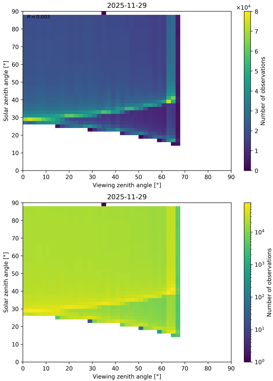
Figure 172: Scatter density plot of “Viewing zenith angle” against “Solar zenith angle” for 2025-11-28 to 2025-11-30.
