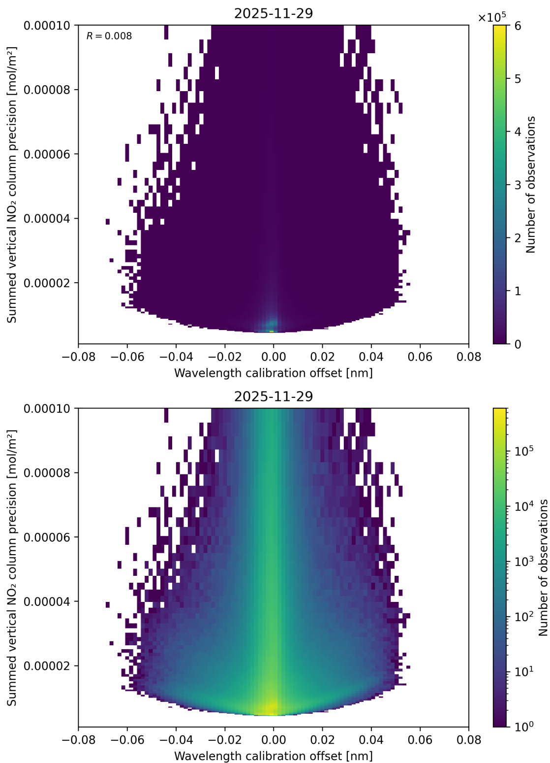
Figure 178: Scatter density plot of “Wavelength calibration offset” against “Summed vertical NO 2 column precision” for 2025-11-28 to 2025-11-30.
