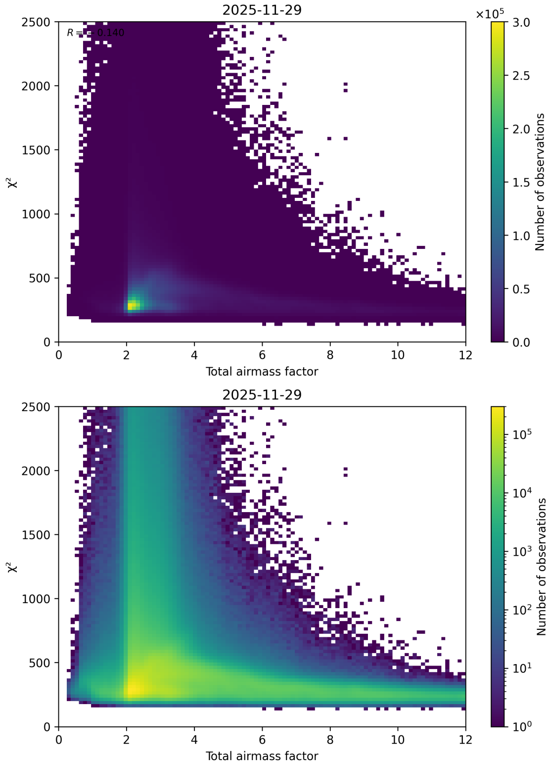
Figure 63: Scatter density plot of “Total airmass factor” against “ \chi^2 ” for 2025-11-28 to 2025-11-30.
