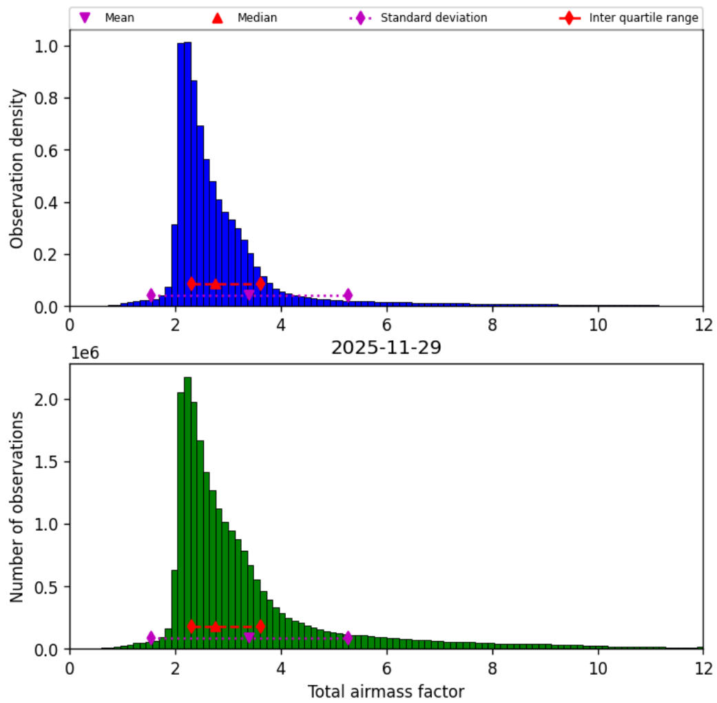
Figure 32: Histogram of “Total airmass factor” for 2025-11-28 to 2025-11-30
