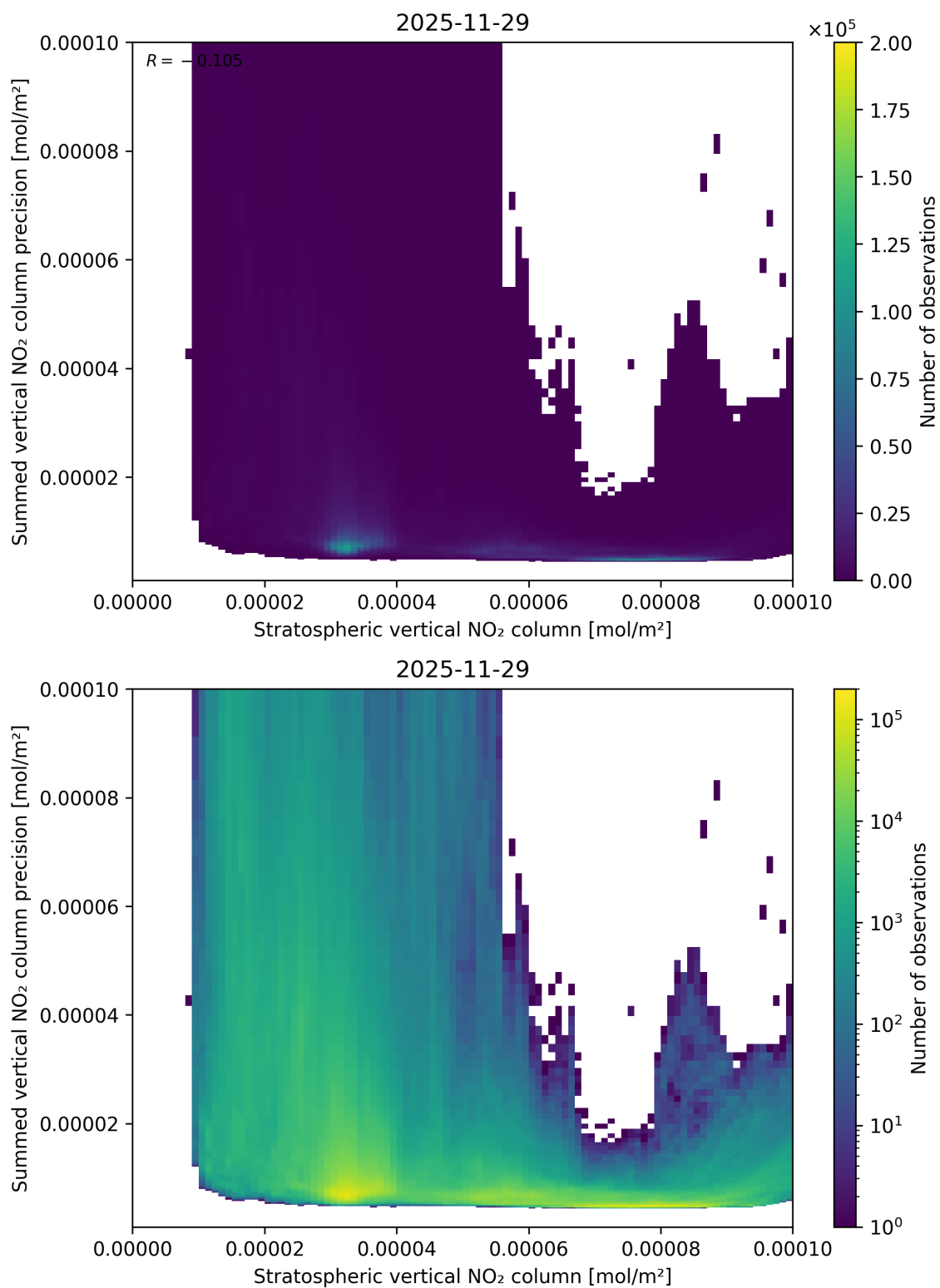
Figure 99: Scatter density plot of “Stratospheric vertical NO 2 column” against “Summed vertical NO 2 column precision” for 2025-11-28 to 2025-11-30.
