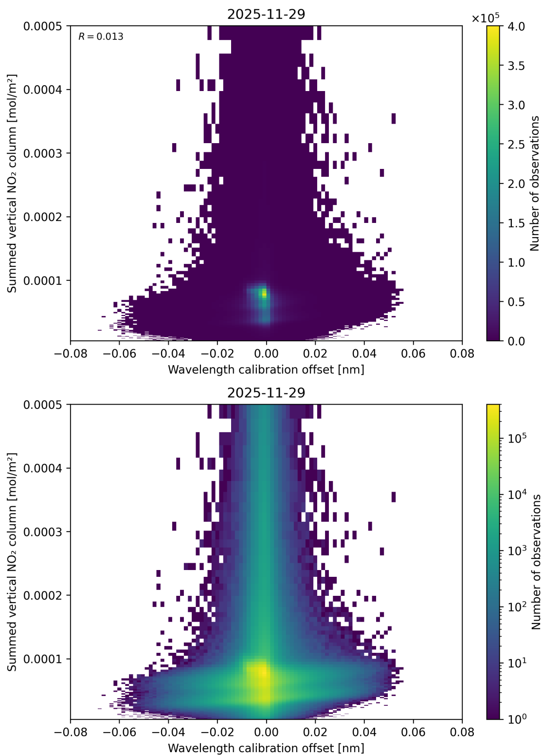
Figure 177: Scatter density plot of “Wavelength calibration offset” against “Summed vertical NO 2 column” for 2025-11-28 to 2025-11-30.
