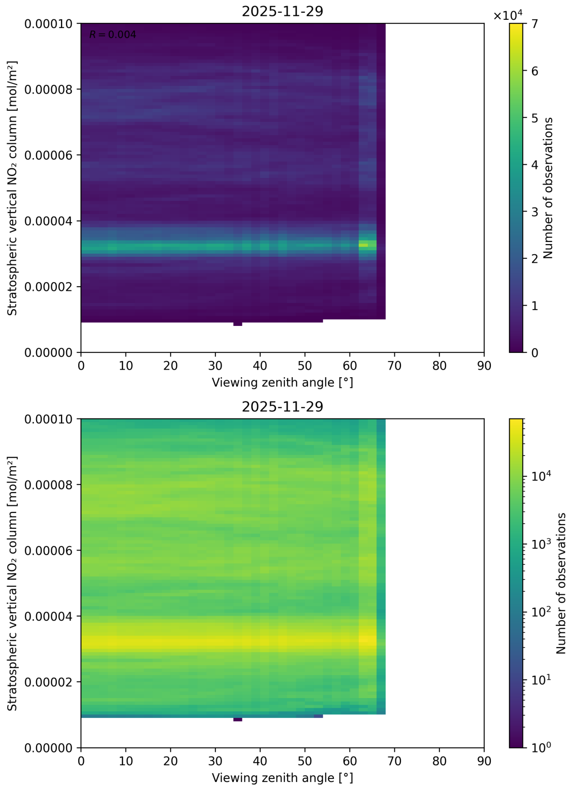
Figure 164: Scatter density plot of “Viewing zenith angle” against “Stratospheric vertical NO 2 column” for 2025-11-28 to 2025-11-30.
