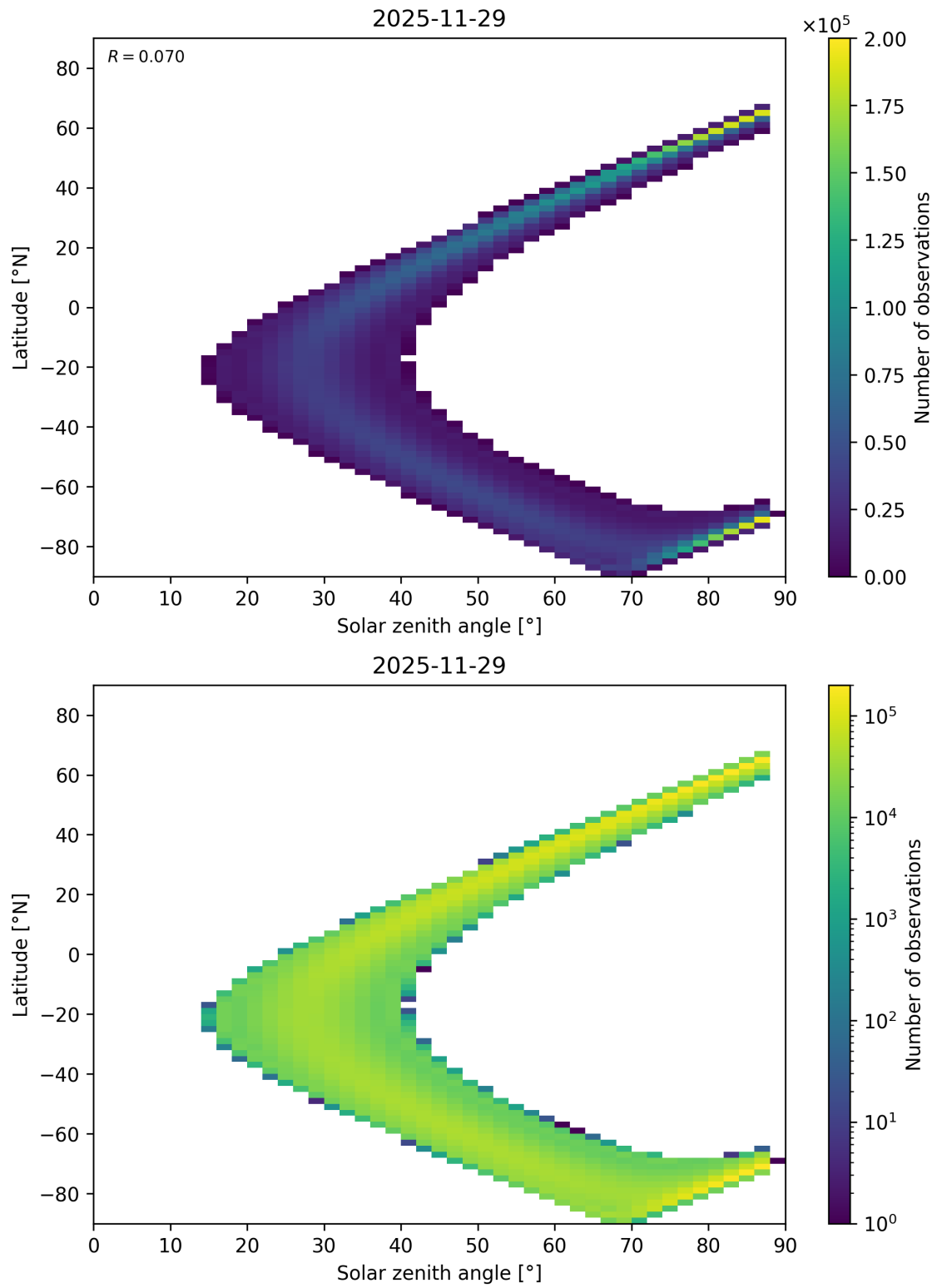
Figure 149: Scatter density plot of “Solar zenith angle” against “Latitude” for 2025-11-28 to 2025-11-30.
