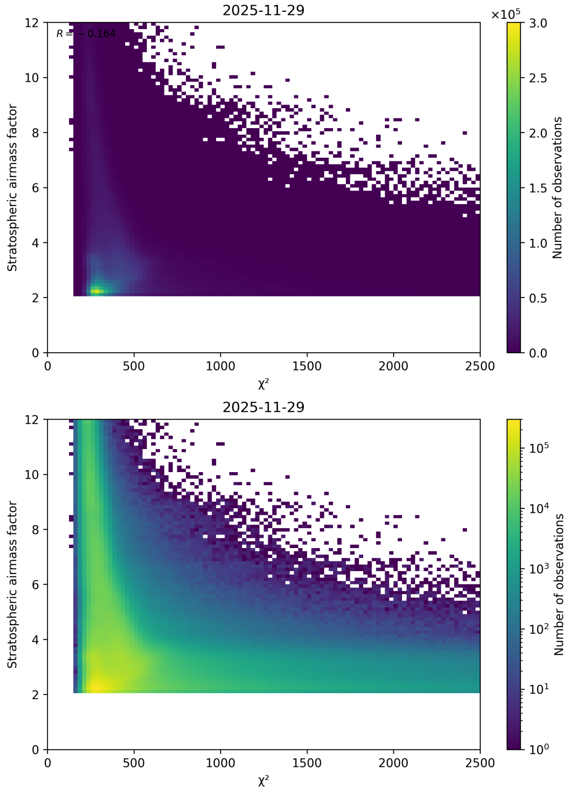
Figure 81: Scatter density plot of “ \chi^2 ” against “Stratospheric airmass factor” for 2025-11-28 to 2025-11-30.
