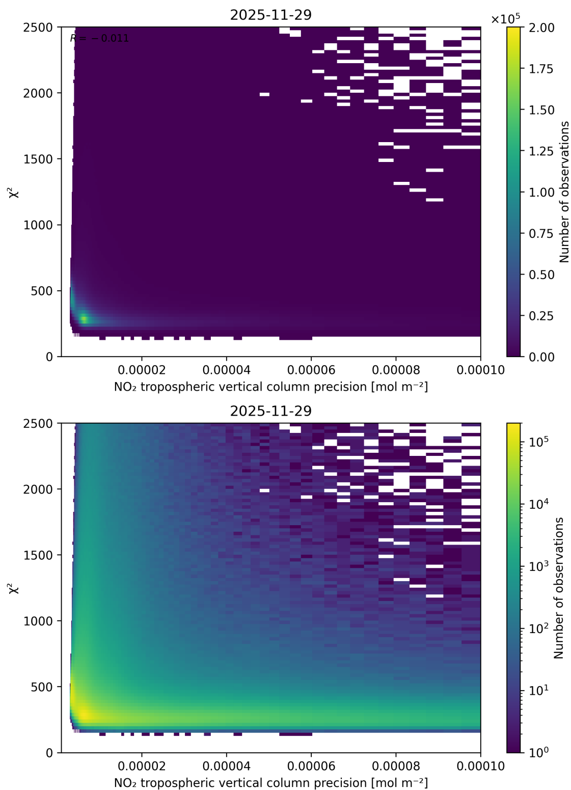
Figure 134: Scatter density plot of “NO 2 tropospheric vertical column precision” against “ \chi^2 ” for 2025-11-28 to 2025-11-30.
