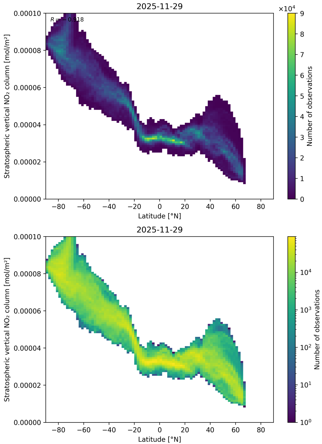
Figure 87: Scatter density plot of “Latitude” against “Stratospheric vertical NO 2 column” for 2025-11-28 to 2025-11-30.
