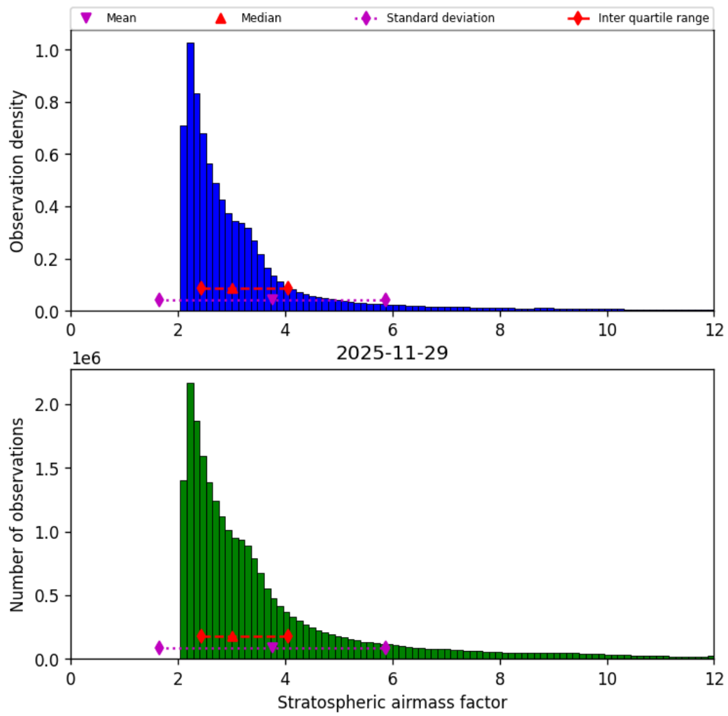
Figure 44: Histogram of “Stratospheric airmass factor” for 2025-11-28 to 2025-11-30
