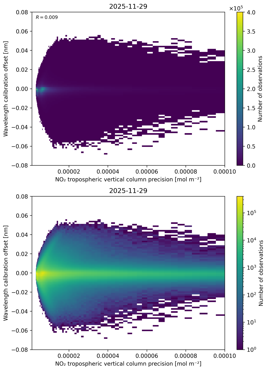
Figure 141: Scatter density plot of “NO 2 tropospheric vertical column precision” against “Wavelength calibration offset” for 2025-11-28 to 2025-11-30.
