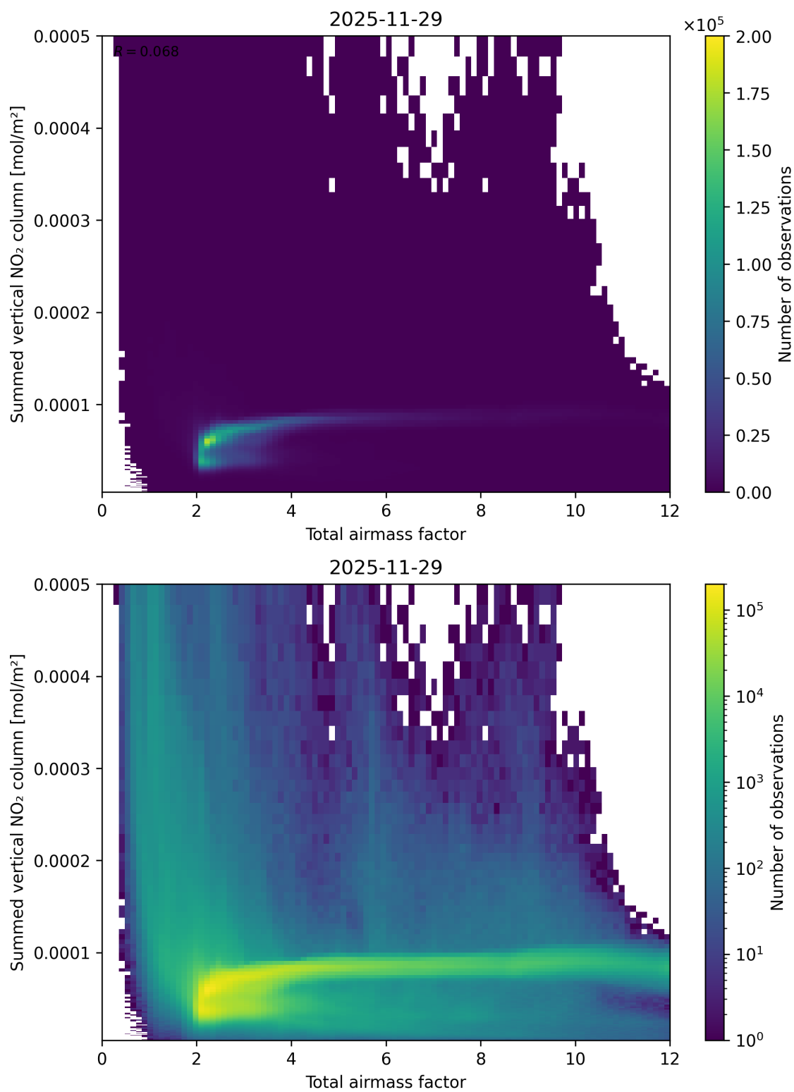
Figure 65: Scatter density plot of “Total airmass factor” against “Summed vertical NO 2 column” for 2025-11-28 to 2025-11-30.
