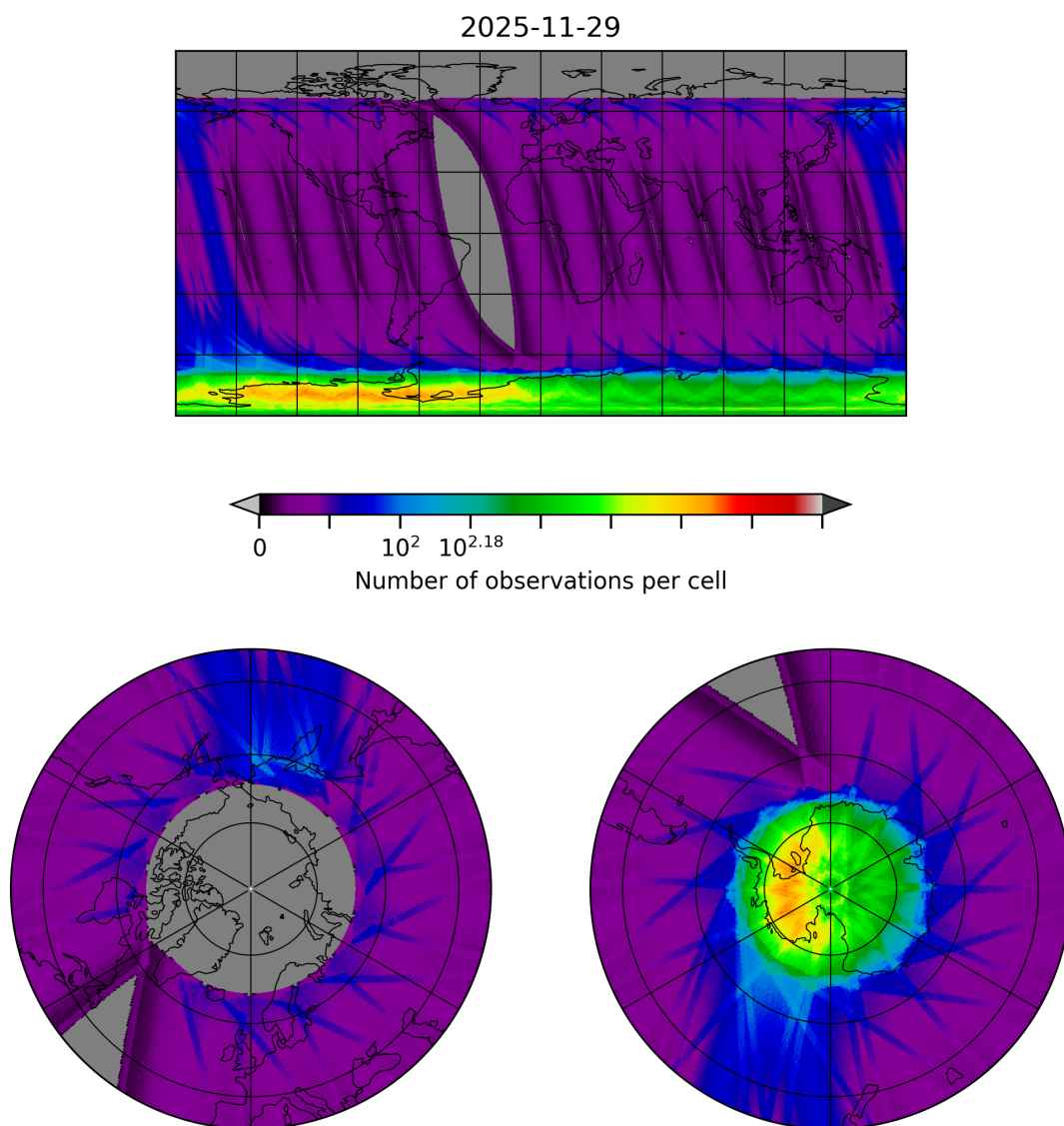
Figure 10: Map of the number of observations for 2025-11-28 to 2025-11-30
