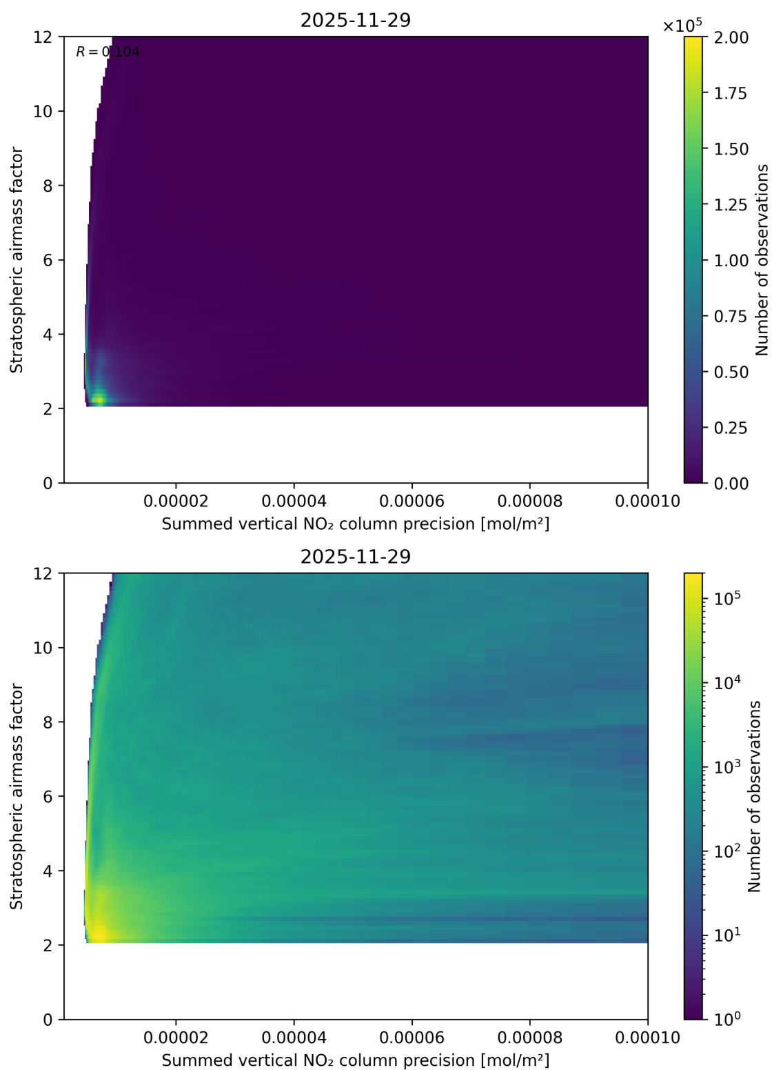
Figure 106: Scatter density plot of “Summed vertical NO 2 column precision” against “Stratospheric airmass factor” for 2025-11-28 to 2025-11-30.
