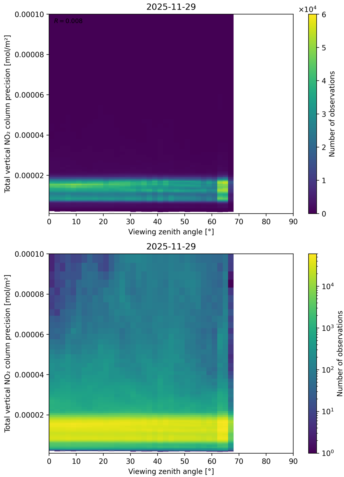
Figure 168: Scatter density plot of “Viewing zenith angle” against “Total vertical NO 2 column precision” for 2025-11-28 to 2025-11-30.
