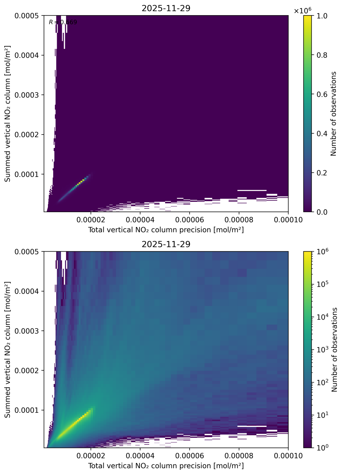
Figure 117: Scatter density plot of “Total vertical NO 2 column precision” against “Summed vertical NO 2 column” for 2025-11-28 to 2025-11-30.
