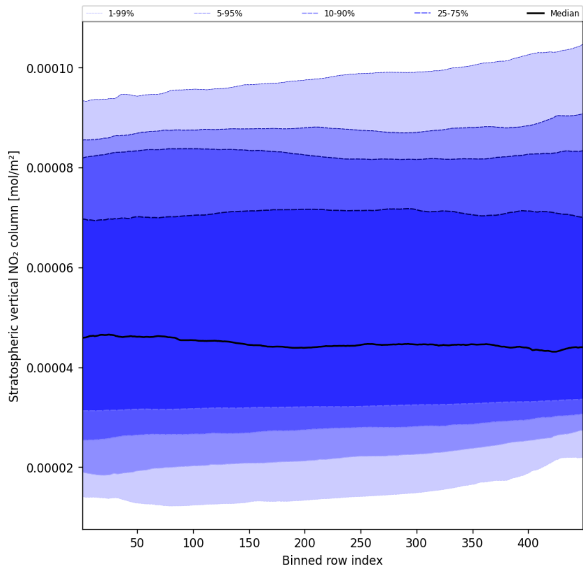
Figure 53: Along track statistics of “Stratospheric vertical NO 2 column” for 2025-11-28 to 2025-11-30
