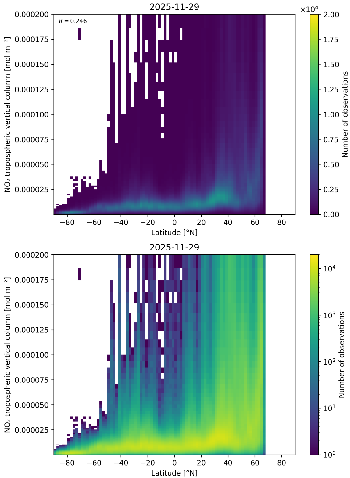
Figure 92: Scatter density plot of “Latitude” against “NO 2 tropospheric vertical column” for 2025-11-28 to 2025-11-30.
