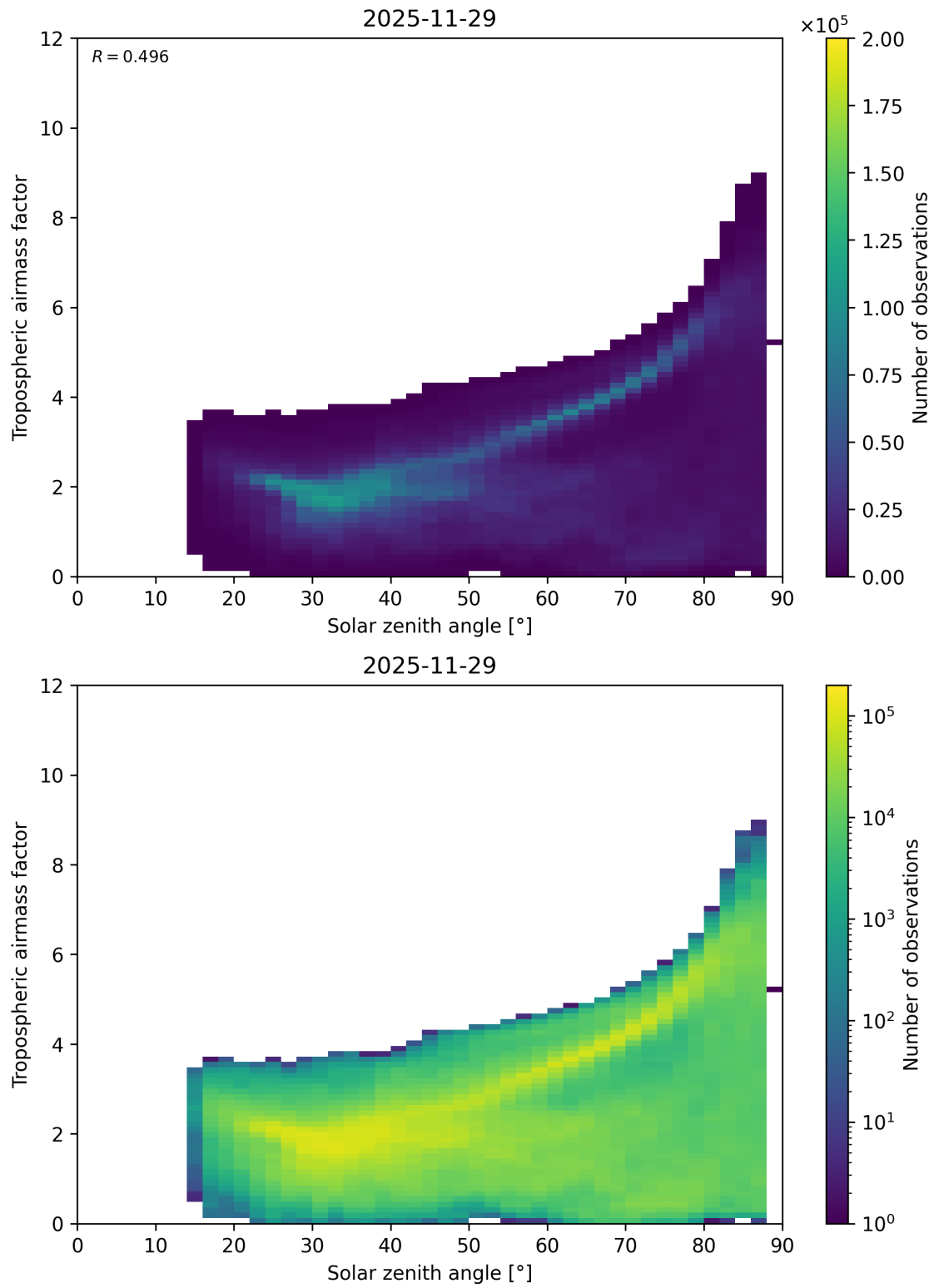
Figure 147: Scatter density plot of “Solar zenith angle” against “Tropospheric airmass factor” for 2025-11-28 to 2025-11-30.
