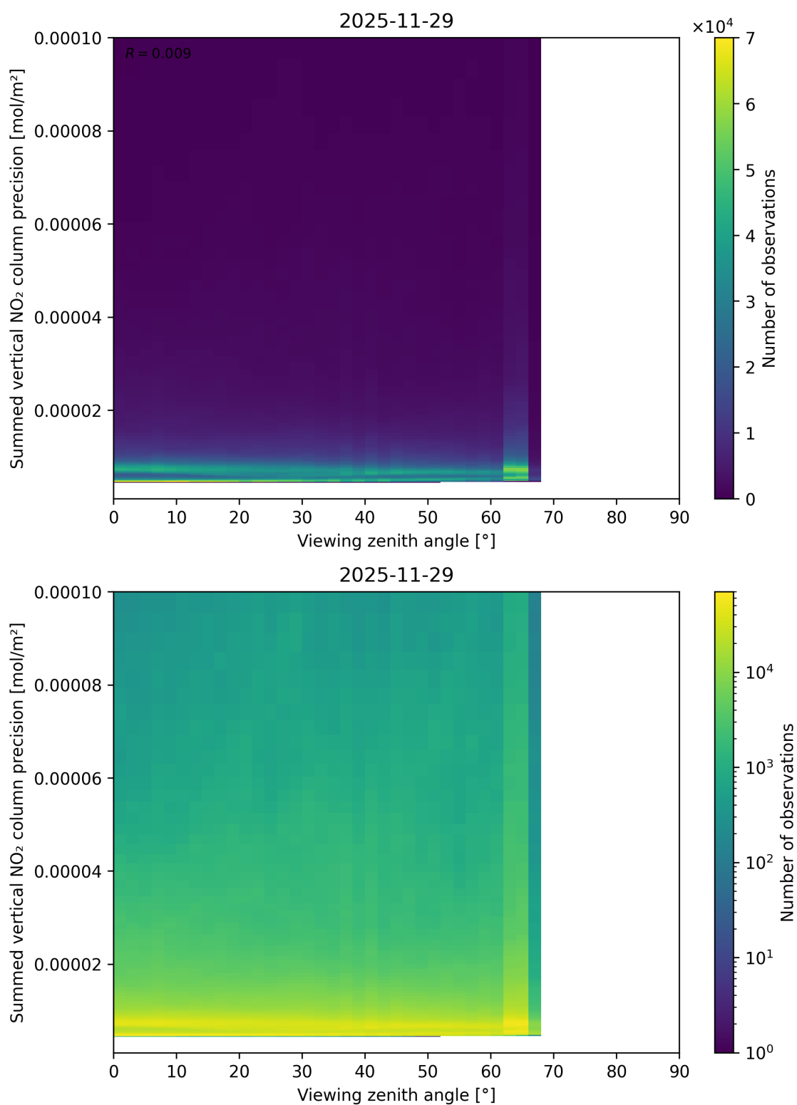
Figure 166: Scatter density plot of “Viewing zenith angle” against “Summed vertical NO 2 column precision” for 2025-11-28 to 2025-11-30.
