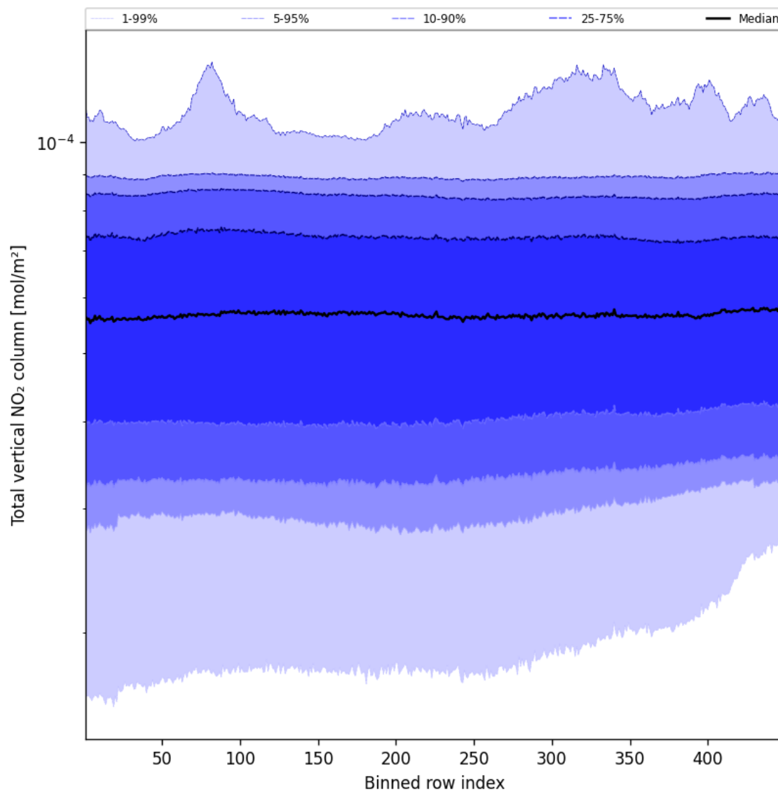
Figure 55: Along track statistics of “Total vertical NO 2 column” for 2025-11-28 to 2025-11-30
