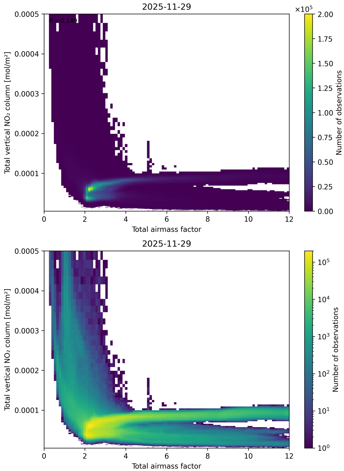
Figure 67: Scatter density plot of “Total airmass factor” against “Total vertical NO 2 column” for 2025-11-28 to 2025-11-30.
