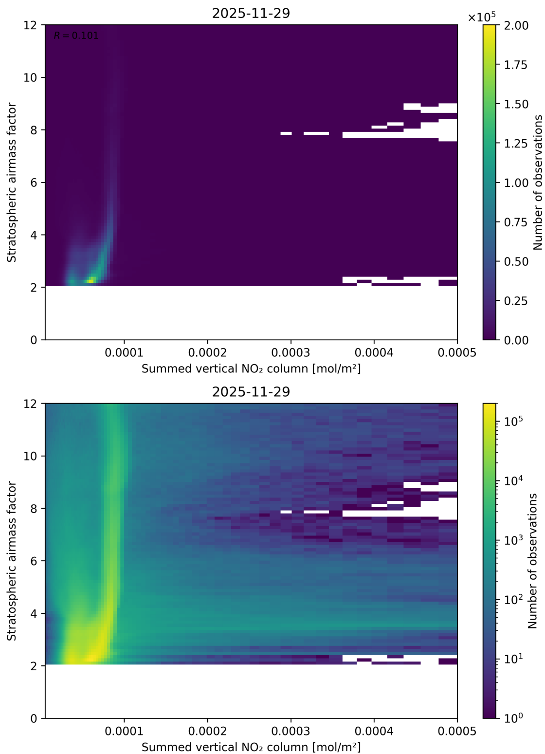
Figure 103: Scatter density plot of “Summed vertical NO 2 column” against “Stratospheric airmass factor” for 2025-11-28 to 2025-11-30.
