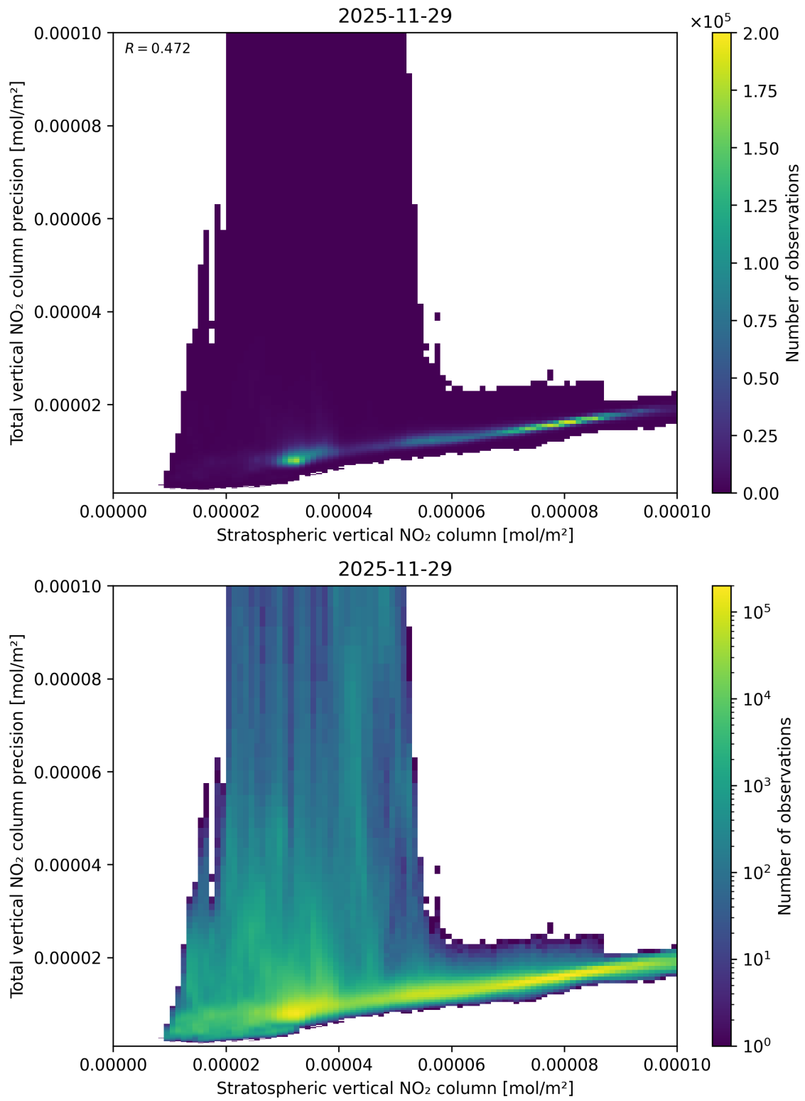
Figure 101: Scatter density plot of “Stratospheric vertical NO 2 column” against “Total vertical NO 2 column precision” for 2025-11-28 to 2025-11-30.
