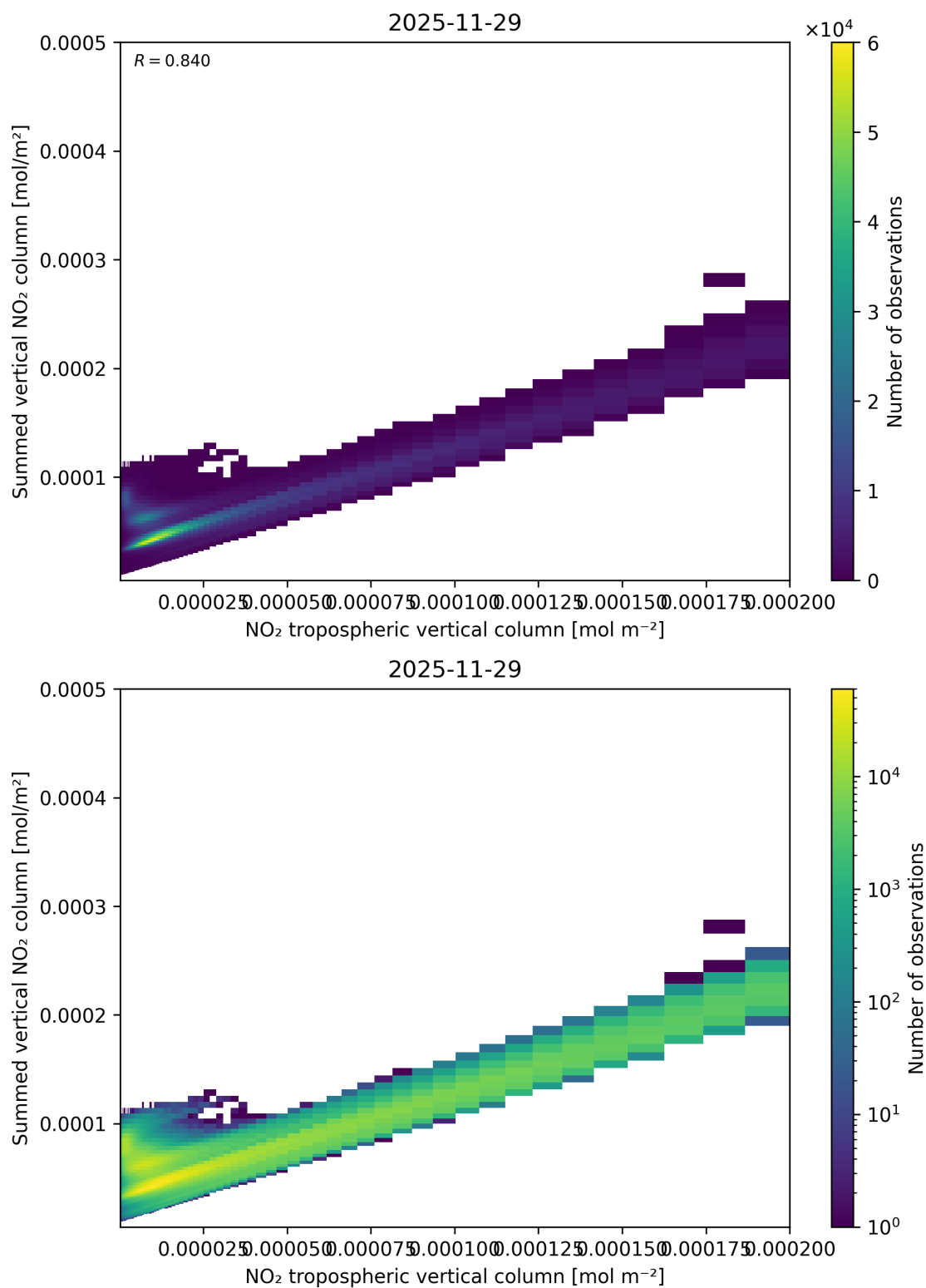
Figure 126: Scatter density plot of “NO 2 tropospheric vertical column” against “Summed vertical NO 2 column” for 2025-11-28 to 2025-11-30.
