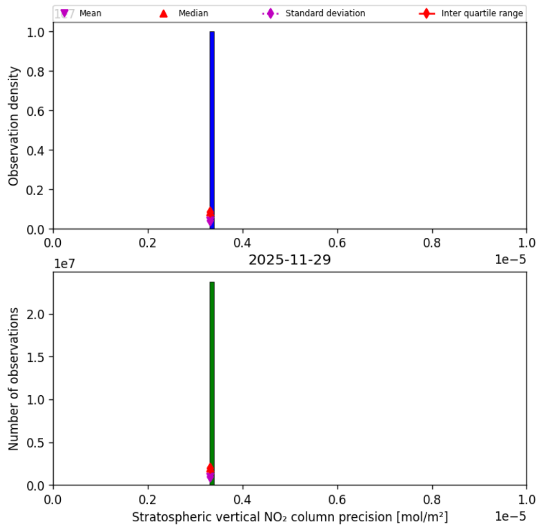
Figure 37: Histogram of “Stratospheric vertical NO 2 column precision” for 2025-11-28 to 2025-11-30
