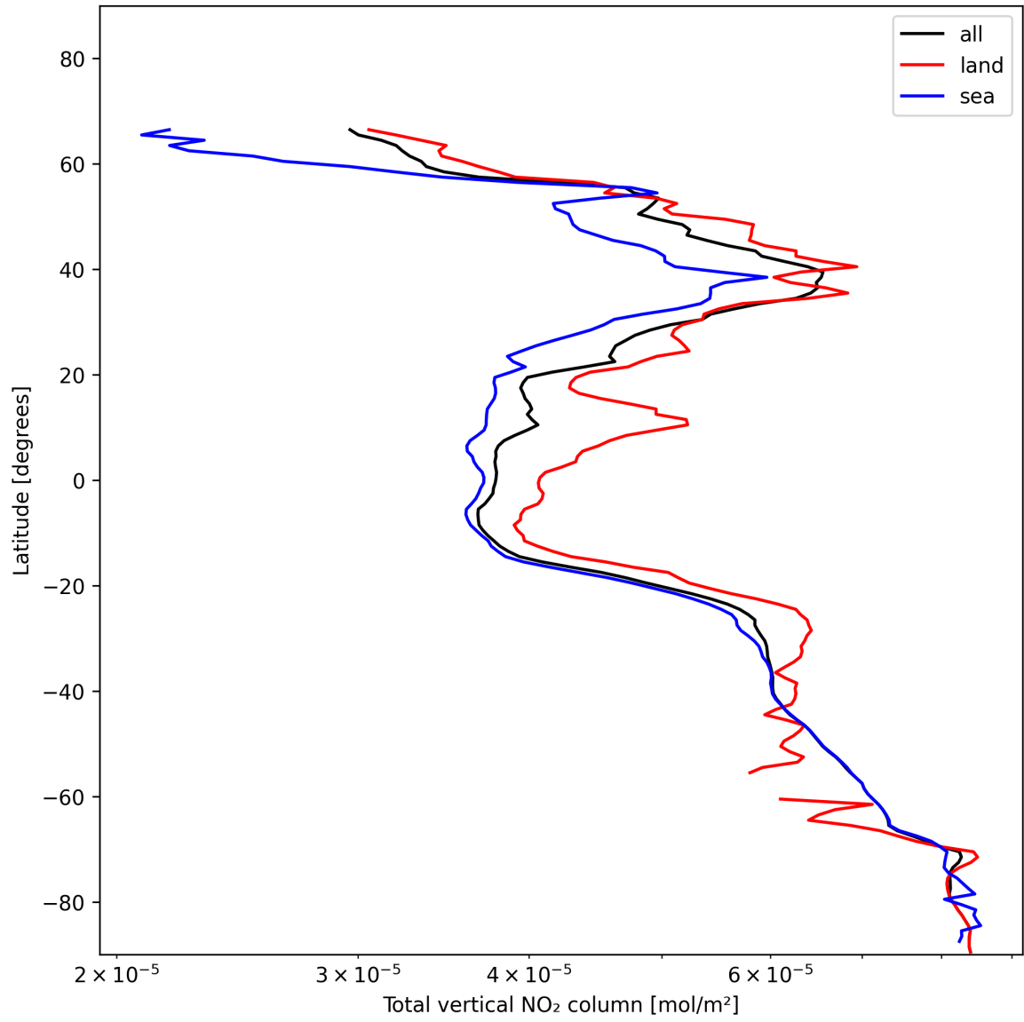
Figure 21: Zonal average of “Total vertical NO 2 column” for 2025-11-28 to 2025-11-30.
