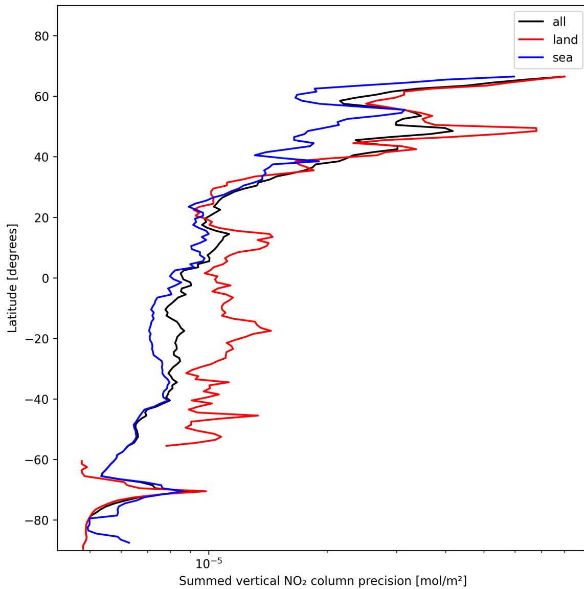
Figure 24: Zonal average of “Summed vertical NO 2 column precision” for 2025-11-28 to 2025-11-30.
