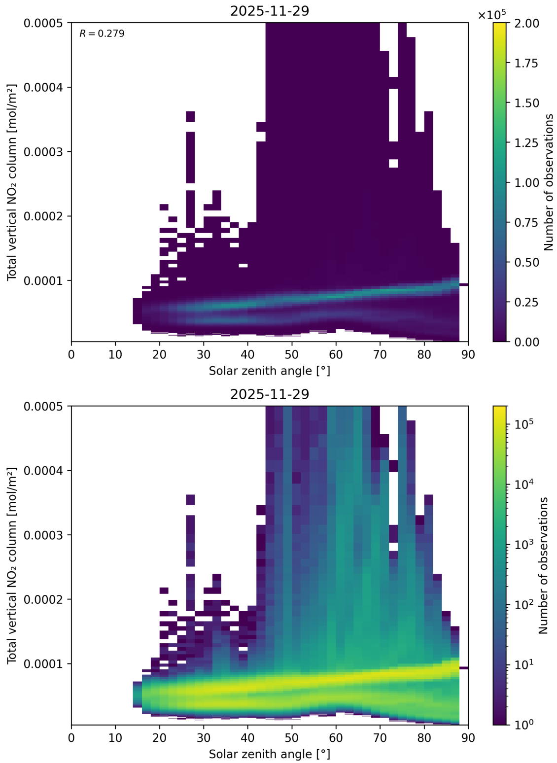
Figure 153: Scatter density plot of “Solar zenith angle” against “Total vertical NO 2 column” for 2025-11-28 to 2025-11-30.
