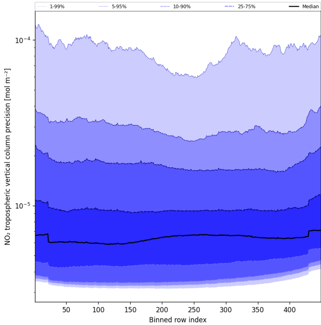
Figure 47: Along track statistics of “NO 2 tropospheric vertical column precision” for 2025-11-28 to 2025-11-30
