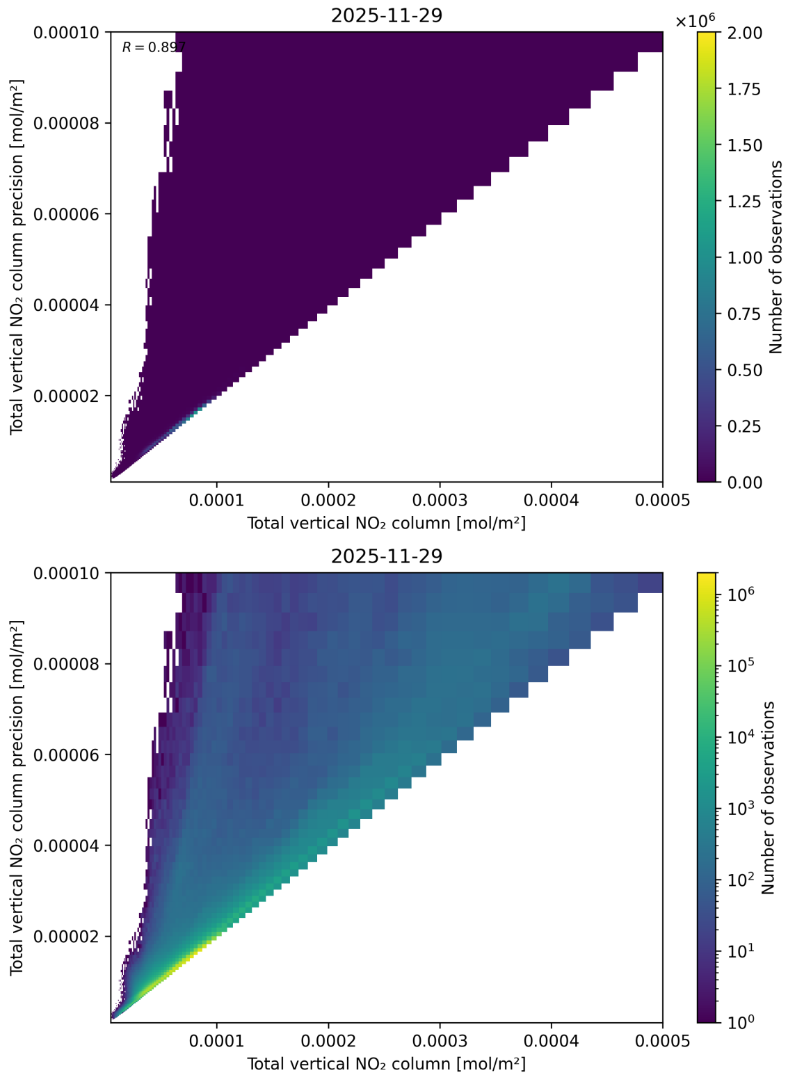
Figure 114: Scatter density plot of “Total vertical NO 2 column” against “Total vertical NO 2 column precision” for 2025-11-28 to 2025-11-30.
