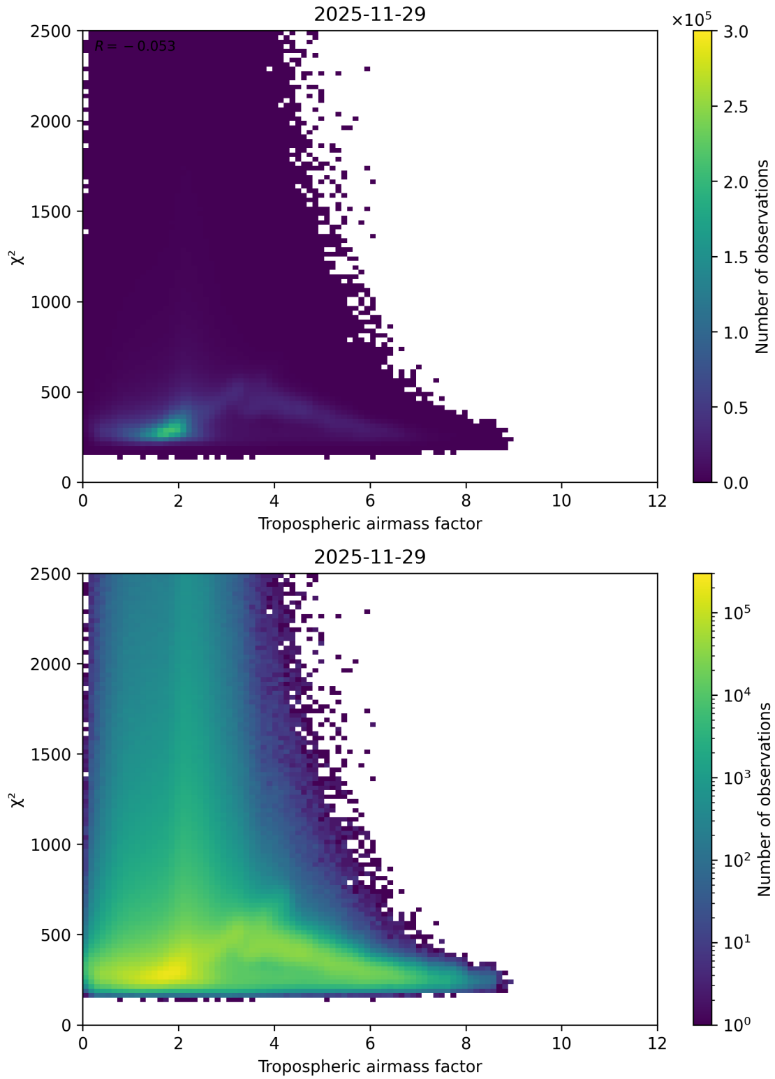
Figure 73: Scatter density plot of “Tropospheric airmass factor” against “ \chi^2 ” for 2025-11-28 to 2025-11-30.
