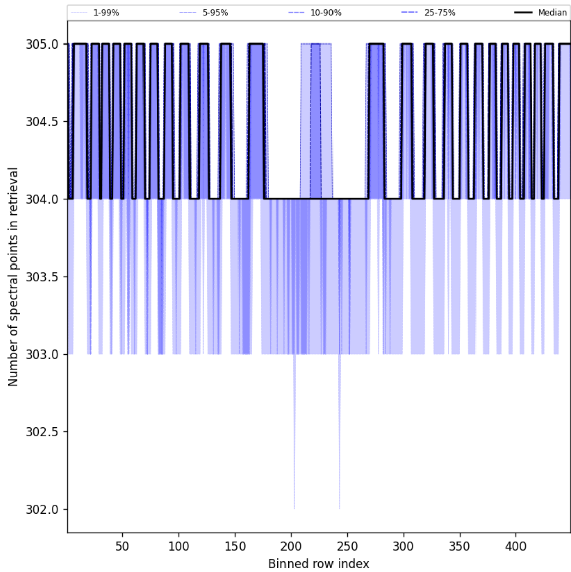
Figure 50: Along track statistics of “Number of spectral points in retrieval” for 2025-11-28 to 2025-11-30
