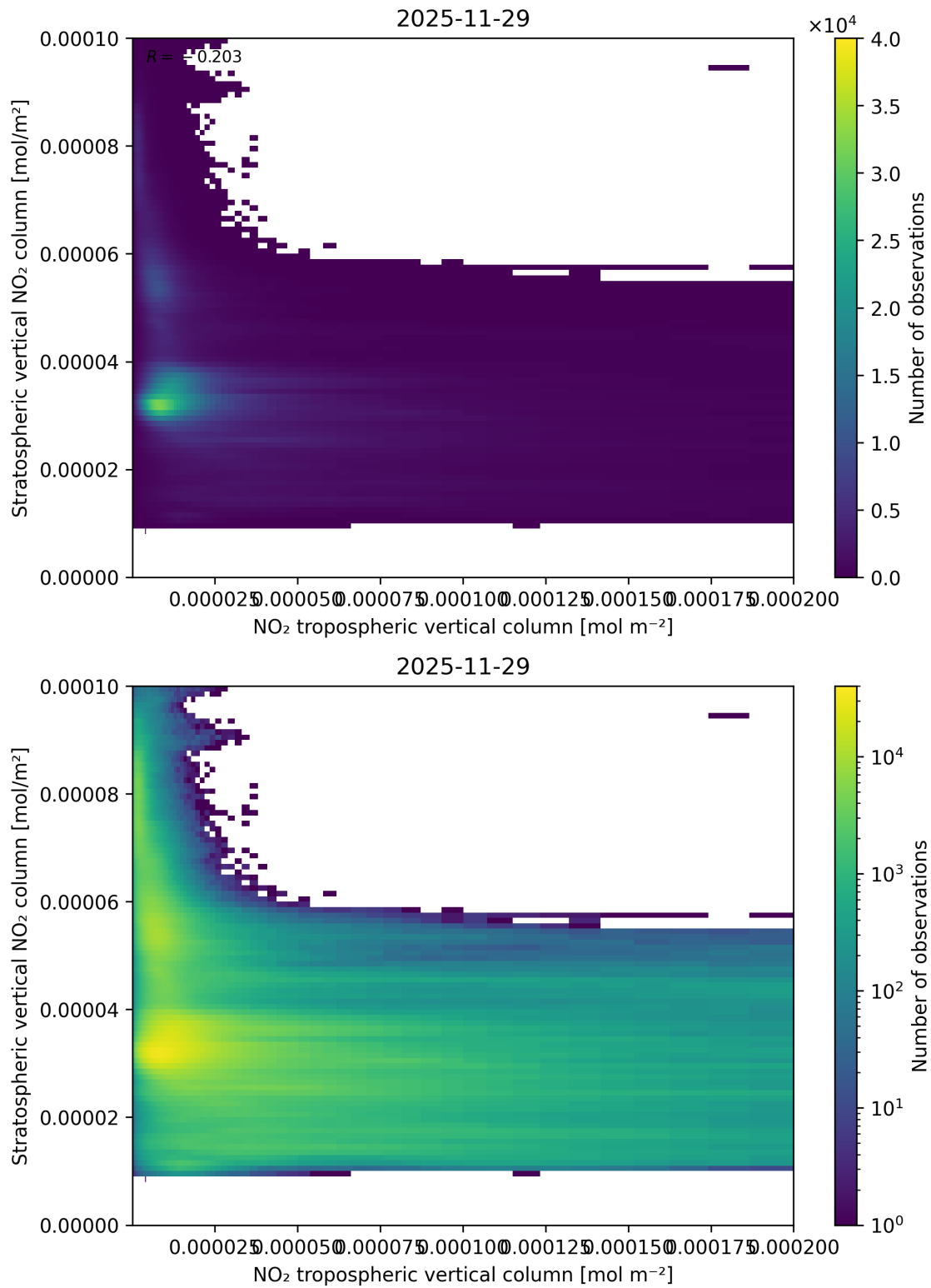
Figure 125: Scatter density plot of “NO 2 tropospheric vertical column” against “Stratospheric vertical NO 2 column” for 2025-11-28 to 2025-11-30.
