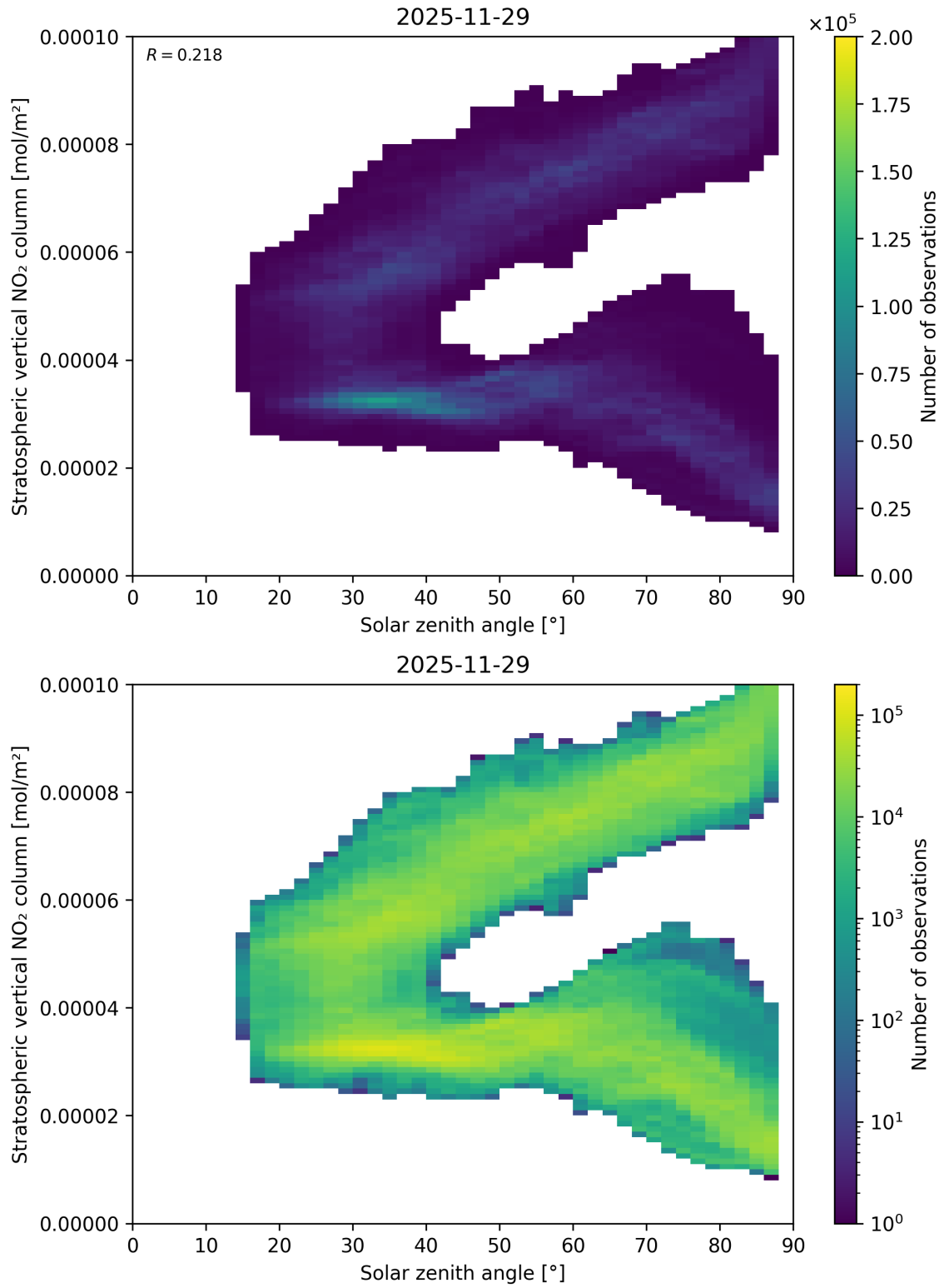
Figure 150: Scatter density plot of “Solar zenith angle” against “Stratospheric vertical NO 2 column” for 2025-11-28 to 2025-11-30.
