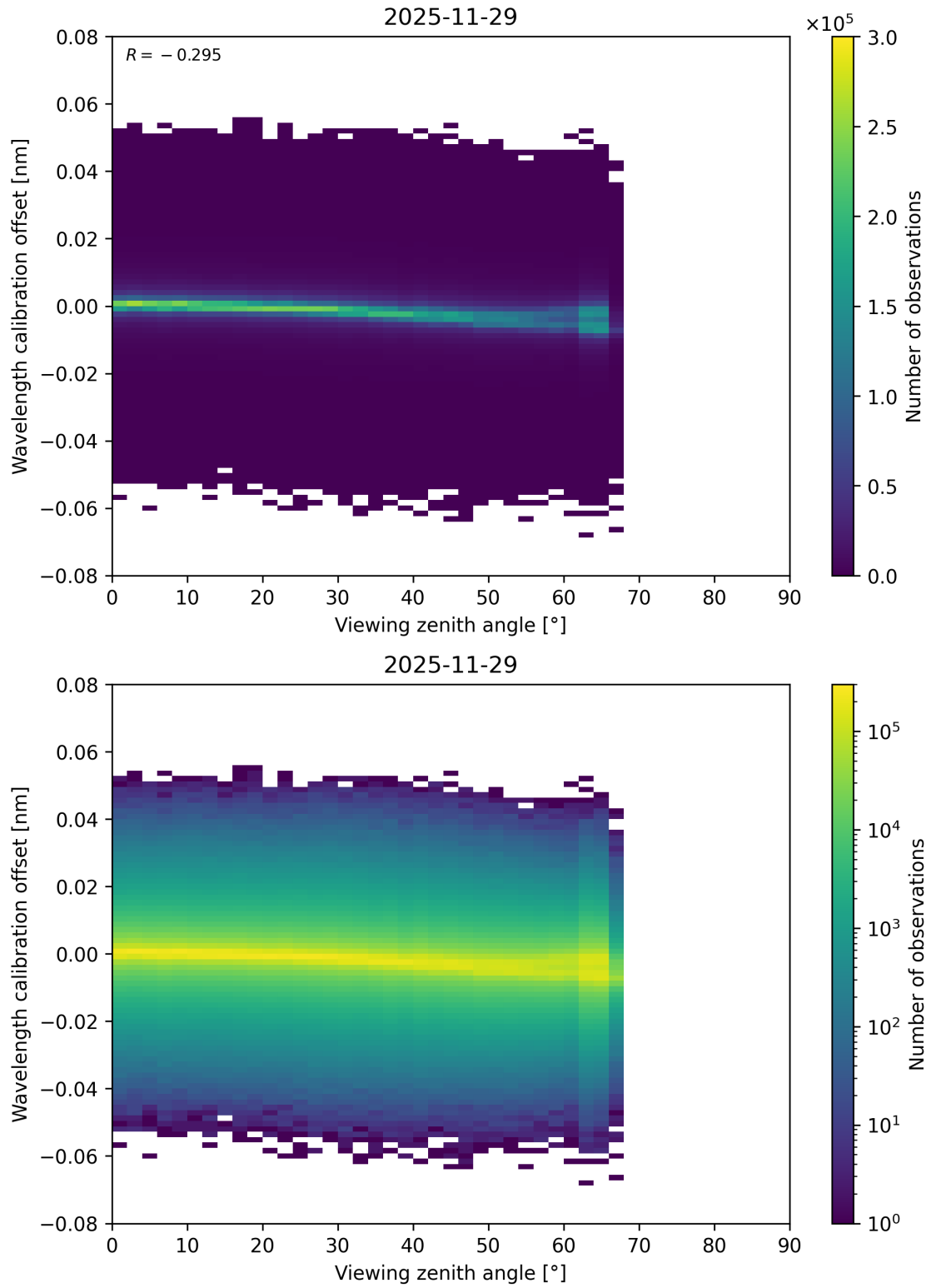
Figure 173: Scatter density plot of “Viewing zenith angle” against “Wavelength calibration offset” for 2025-11-28 to 2025-11-30.
