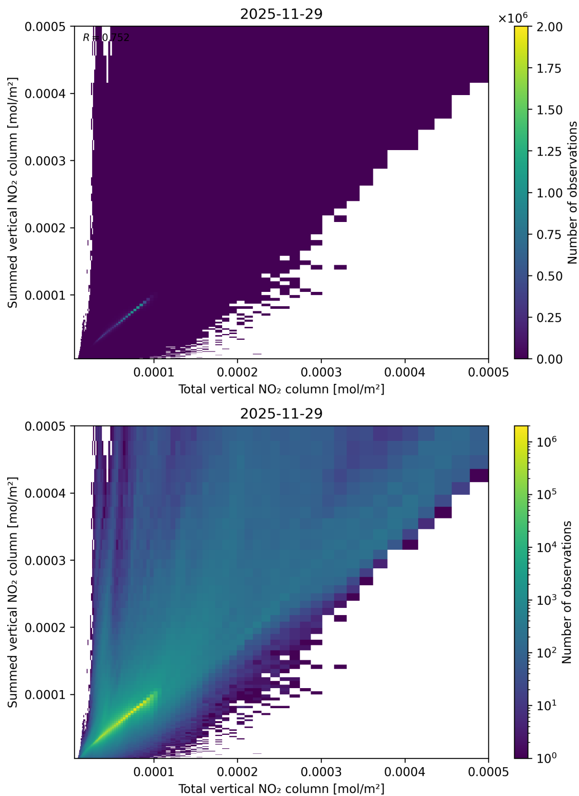
Figure 112: Scatter density plot of “Total vertical NO 2 column” against “Summed vertical NO 2 column” for 2025-11-28 to 2025-11-30.
