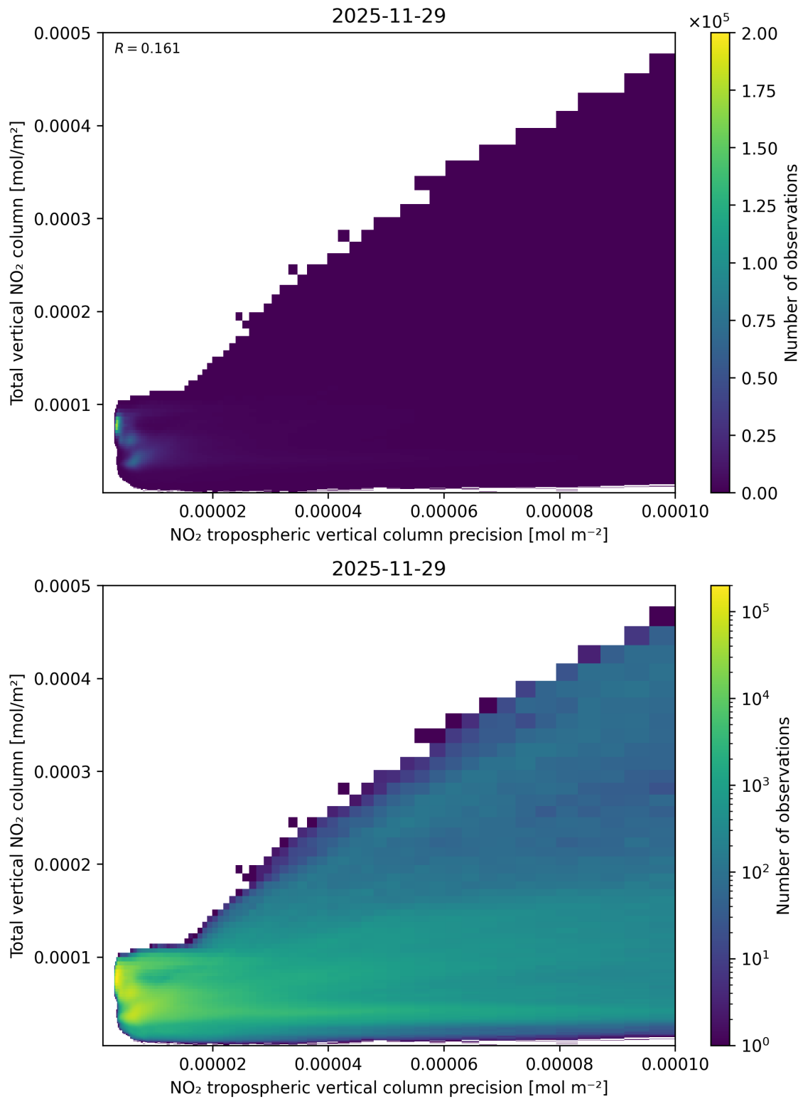
Figure 138: Scatter density plot of “NO 2 tropospheric vertical column precision” against “Total vertical NO 2 column” for 2025-11-28 to 2025-11-30.
