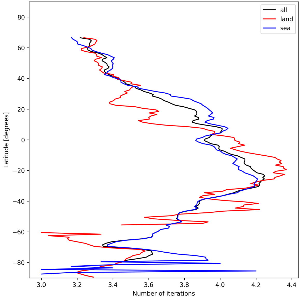
Figure 17: Zonal average of “Number of iterations” for 2025-11-28 to 2025-11-30.
