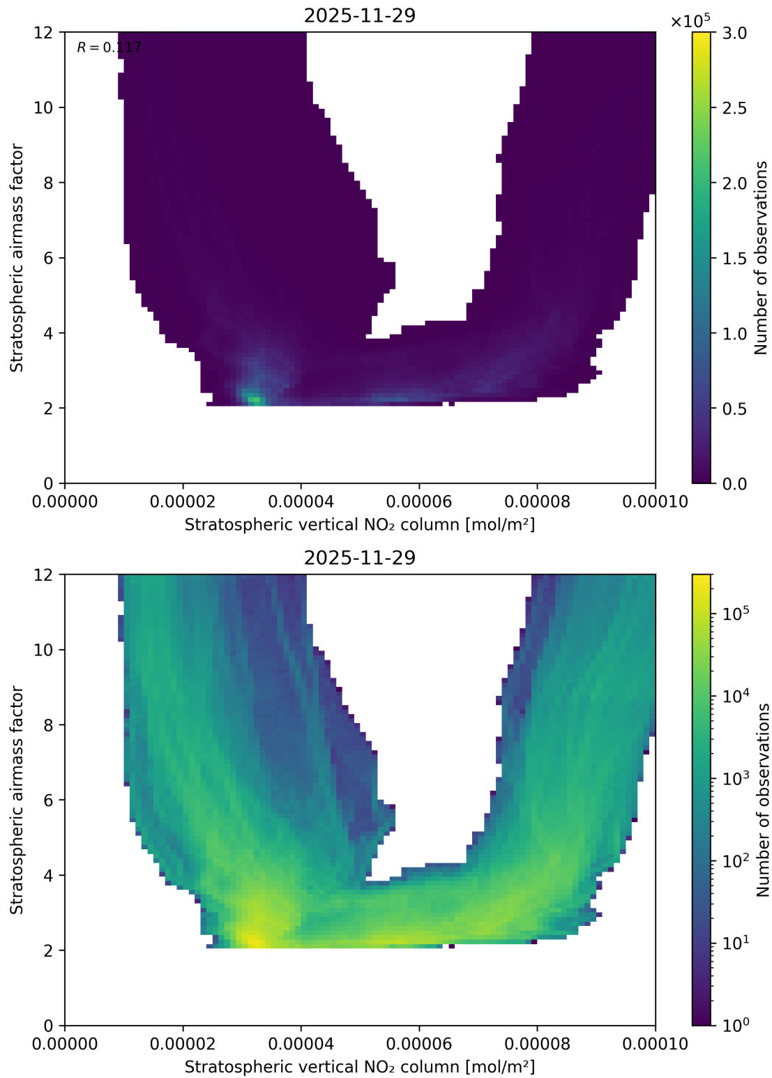
Figure 96: Scatter density plot of “Stratospheric vertical NO 2 column” against “Stratospheric airmass factor” for 2025-11-28 to 2025-11-30.
