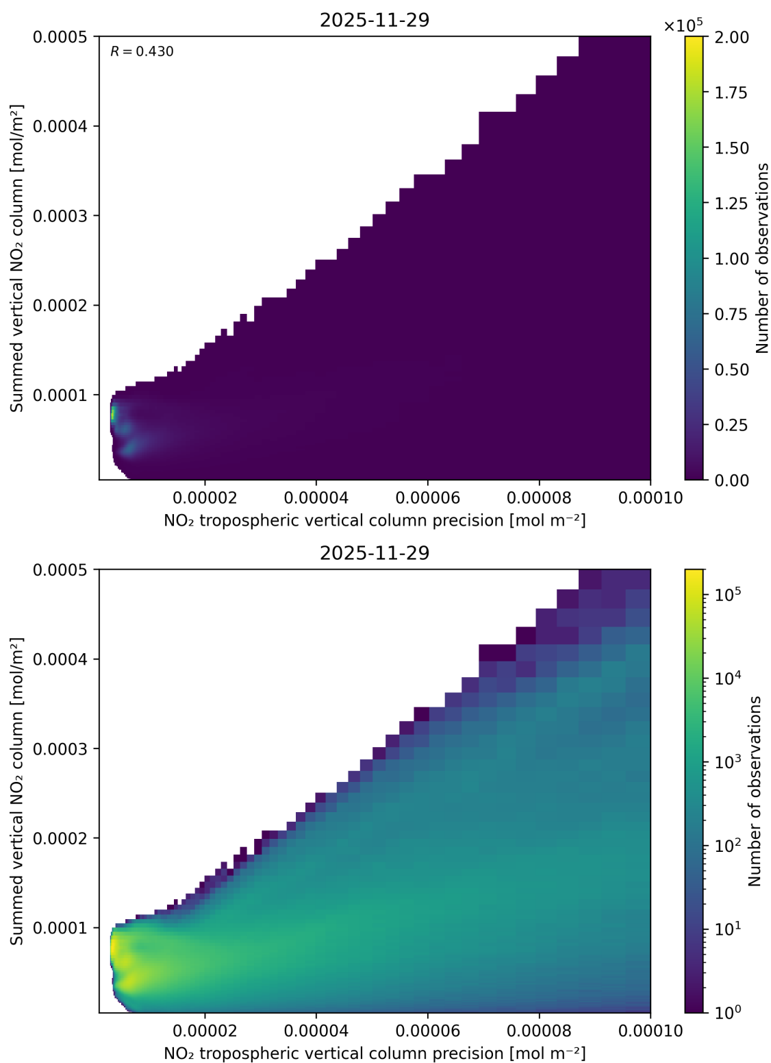
Figure 136: Scatter density plot of “NO 2 tropospheric vertical column precision” against “Summed vertical NO 2 column” for 2025-11-28 to 2025-11-30.
