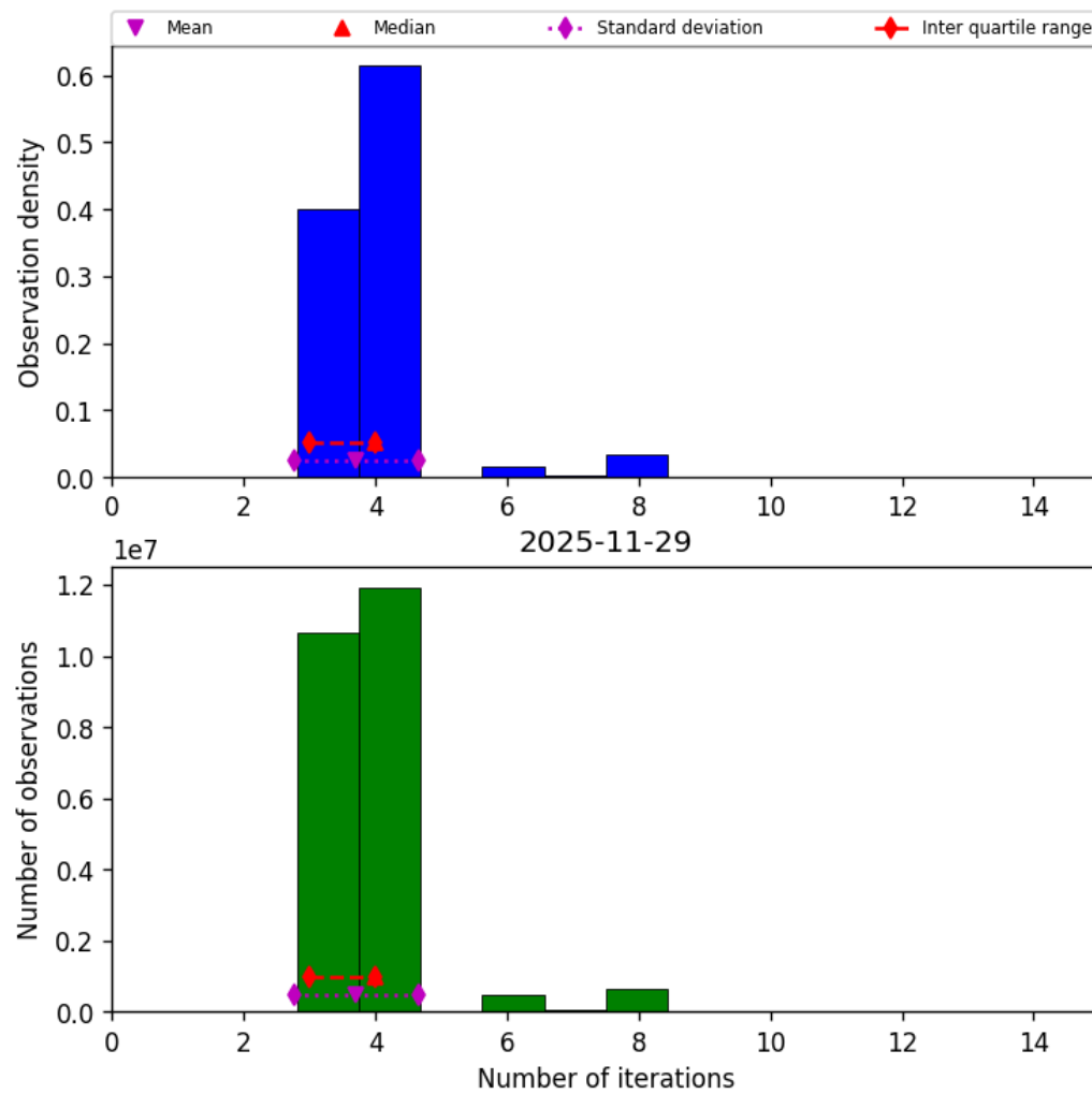
Figure 34: Histogram of “Number of iterations” for 2025-11-28 to 2025-11-30
