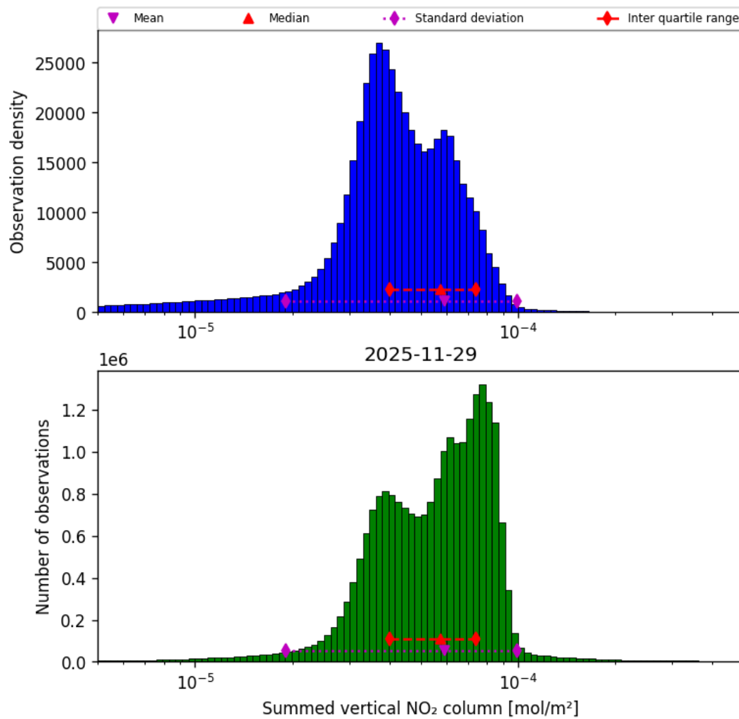
Figure 40: Histogram of “Summed vertical NO 2 column” for 2025-11-28 to 2025-11-30
