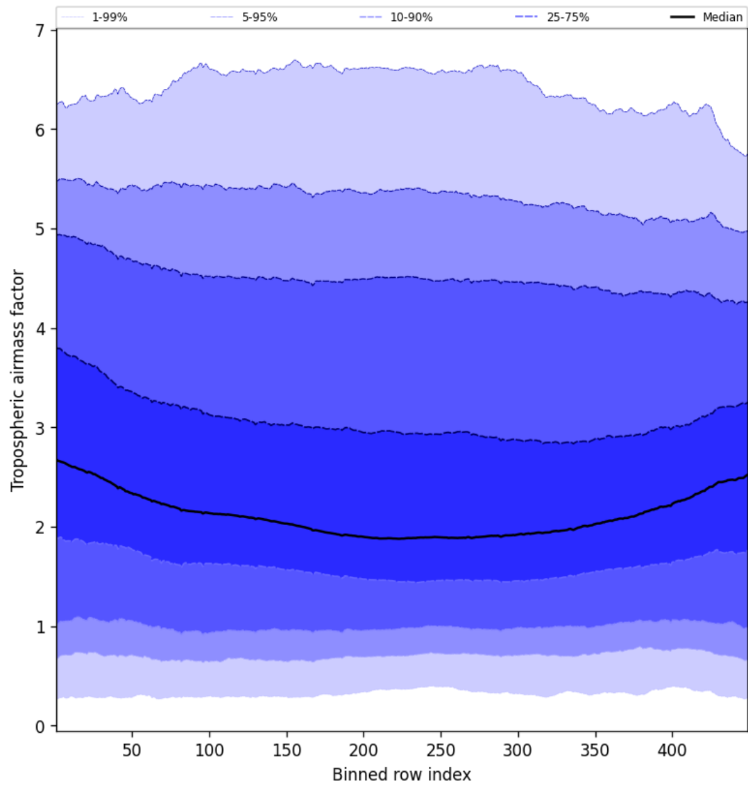
Figure 48: Along track statistics of “Tropospheric air mass factor” for 2025-11-28 to 2025-11-30
