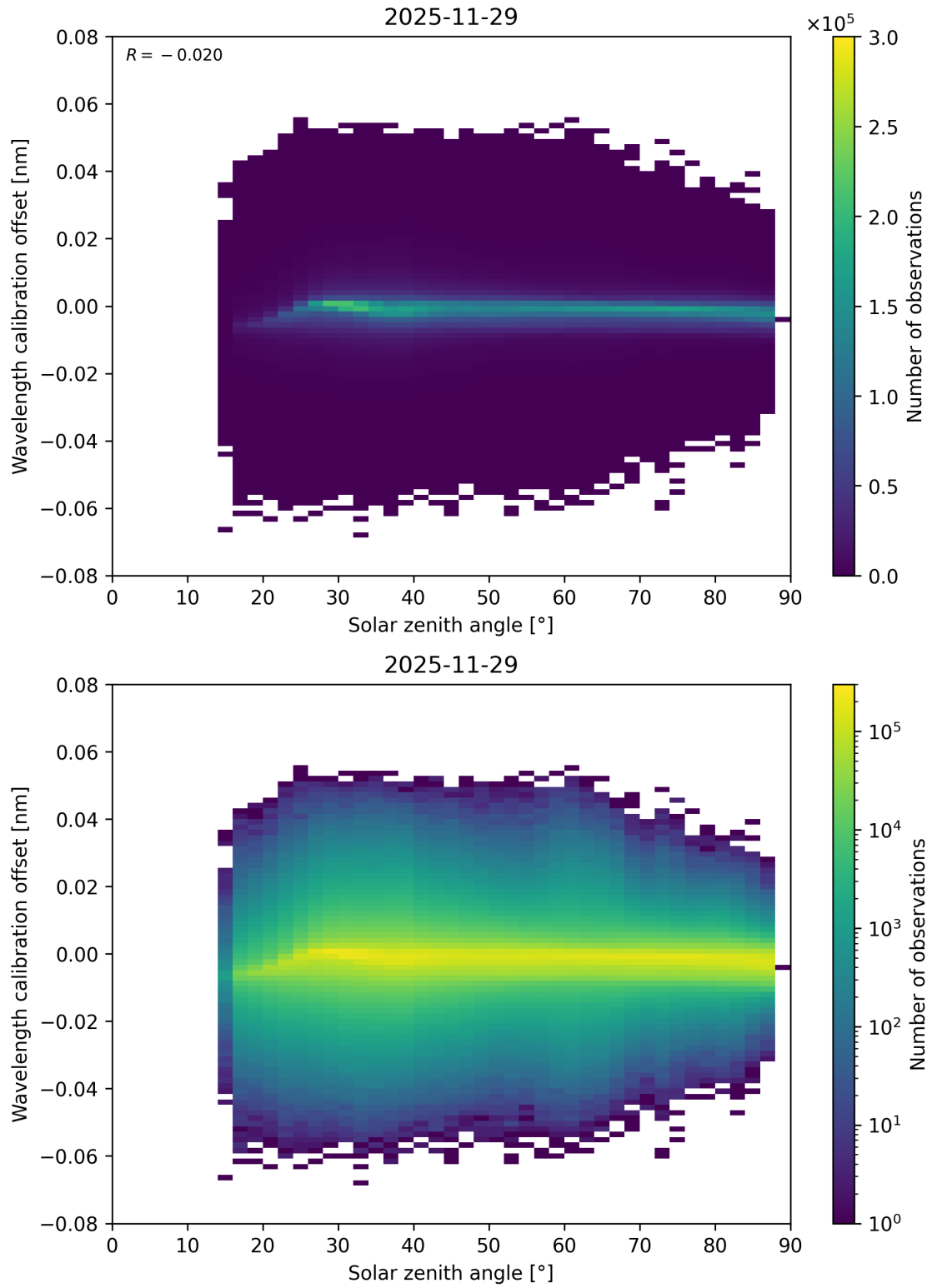
Figure 158: Scatter density plot of “Solar zenith angle” against “Wavelength calibration offset” for 2025-11-28 to 2025-11-30.
