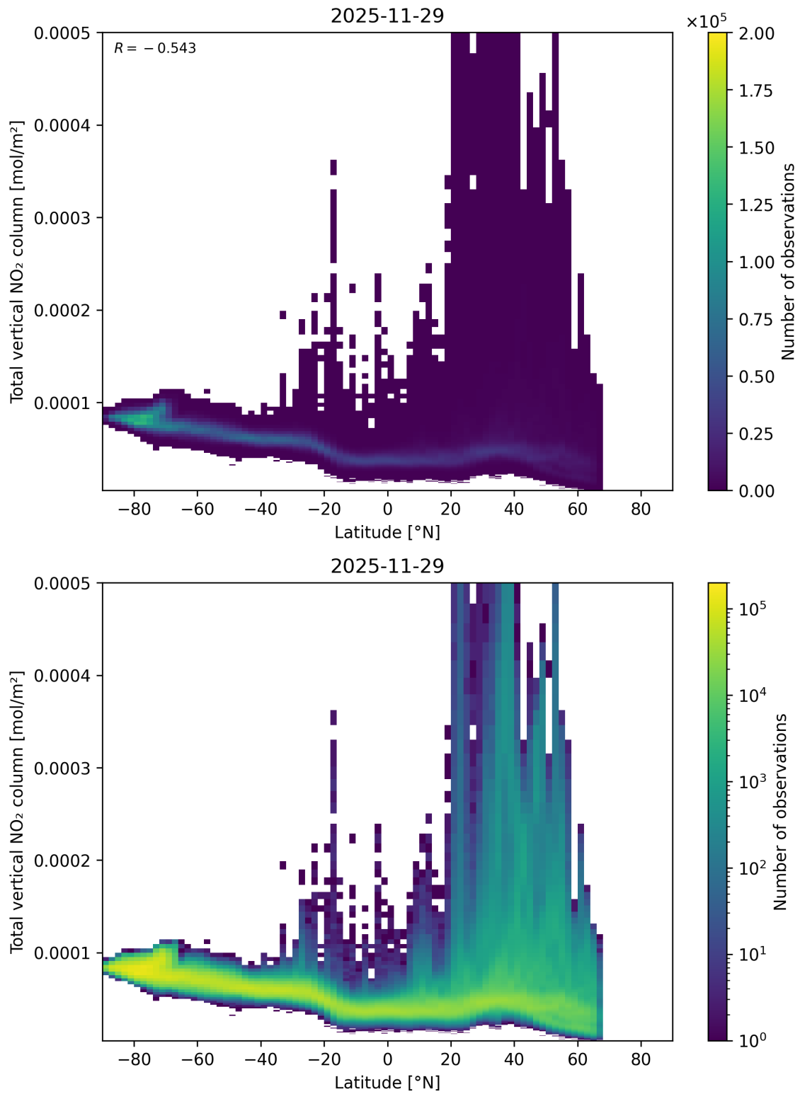
Figure 90: Scatter density plot of “Latitude” against “Total vertical NO 2 column” for 2025-11-28 to 2025-11-30.
