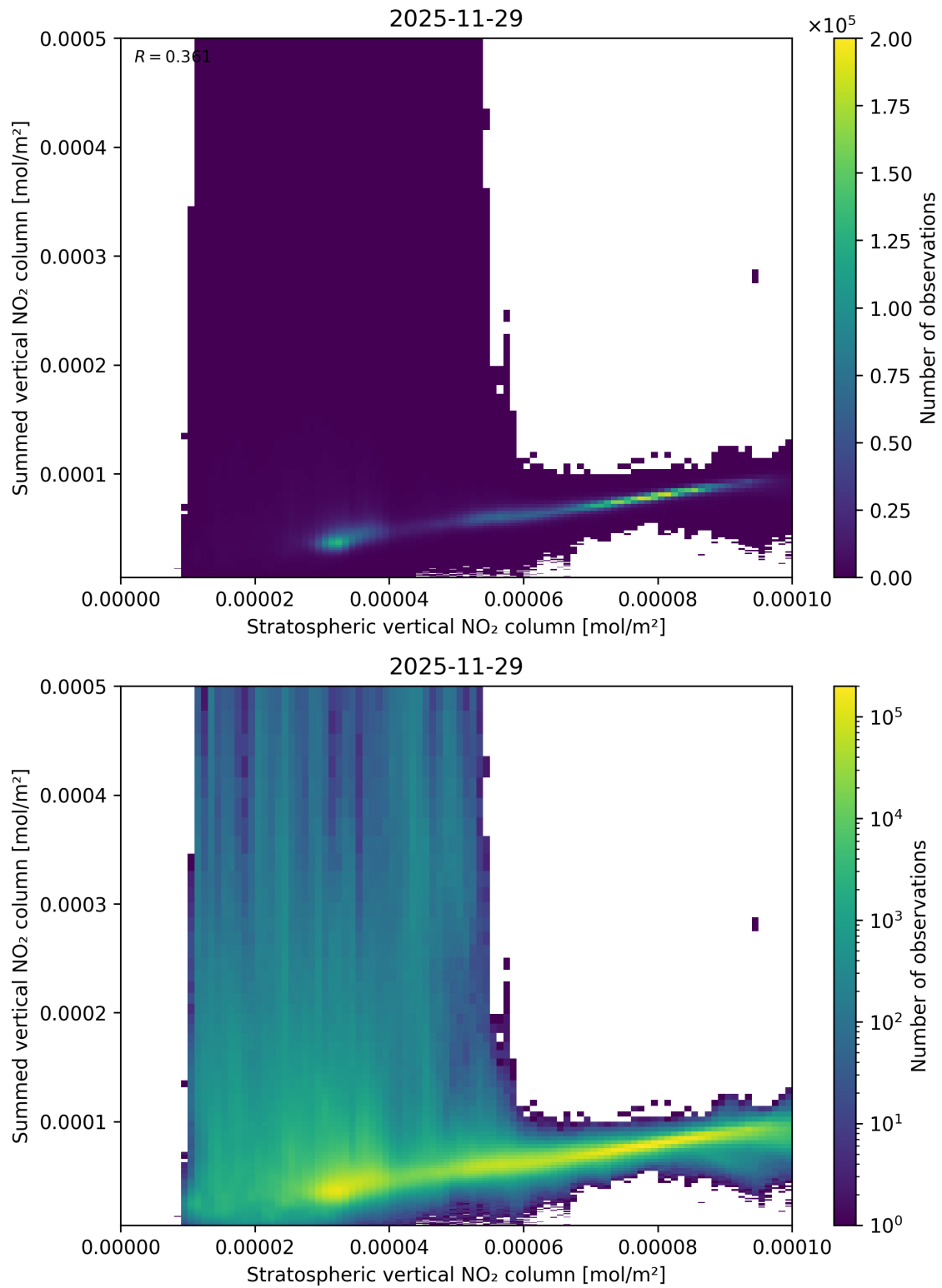
Figure 98: Scatter density plot of “Stratospheric vertical NO 2 column” against “Summed vertical NO 2 column” for 2025-11-28 to 2025-11-30.
