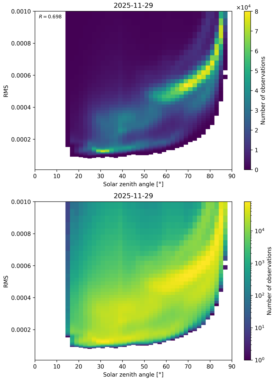
Figure 157: Scatter density plot of “Solar zenith angle” against “RMS” for 2025-11-28 to 2025-11-30.
