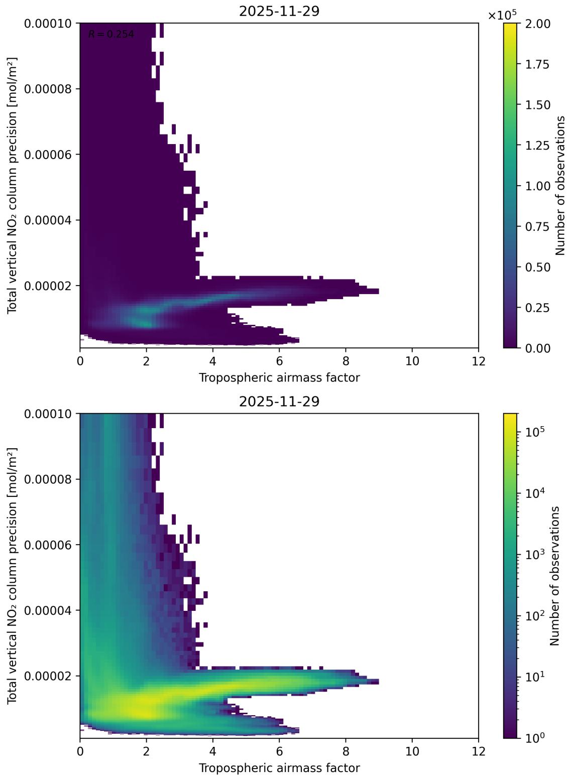
Figure 78: Scatter density plot of “Tropospheric air mass factor” against “Total vertical NO 2 column precision” for 2025-11-28 to 2025-11-30.
