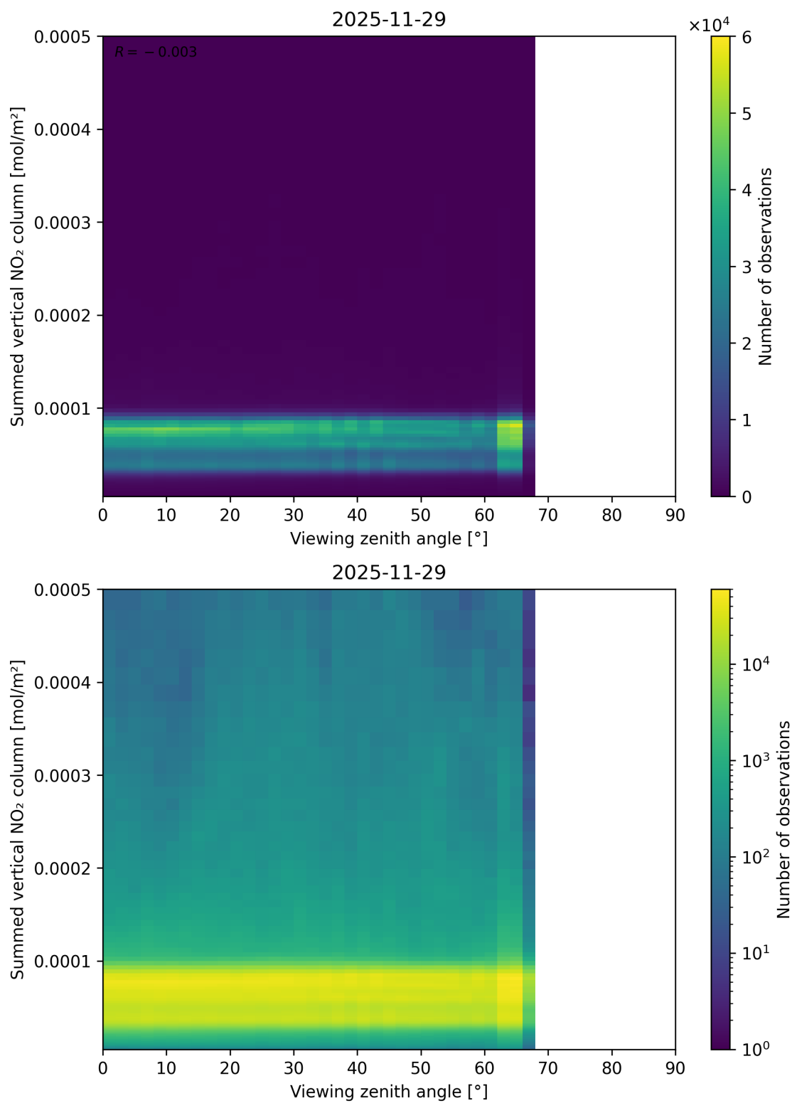
Figure 165: Scatter density plot of “Viewing zenith angle” against “Summed vertical NO 2 column” for 2025-11-28 to 2025-11-30.
