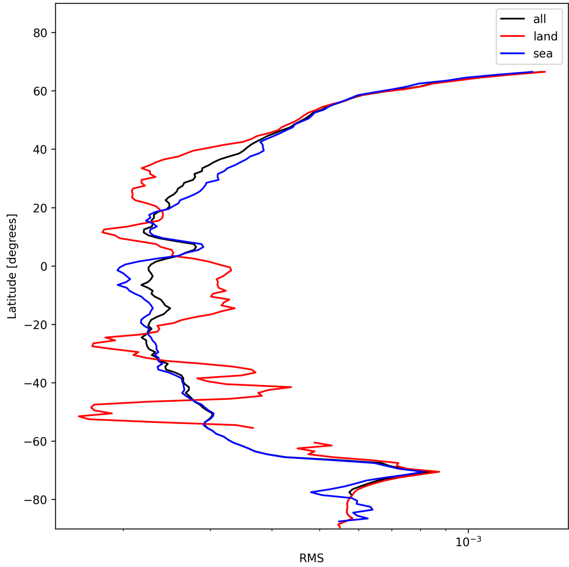
Figure 26: Zonal average of “RMS” for 2025-11-28 to 2025-11-30.
