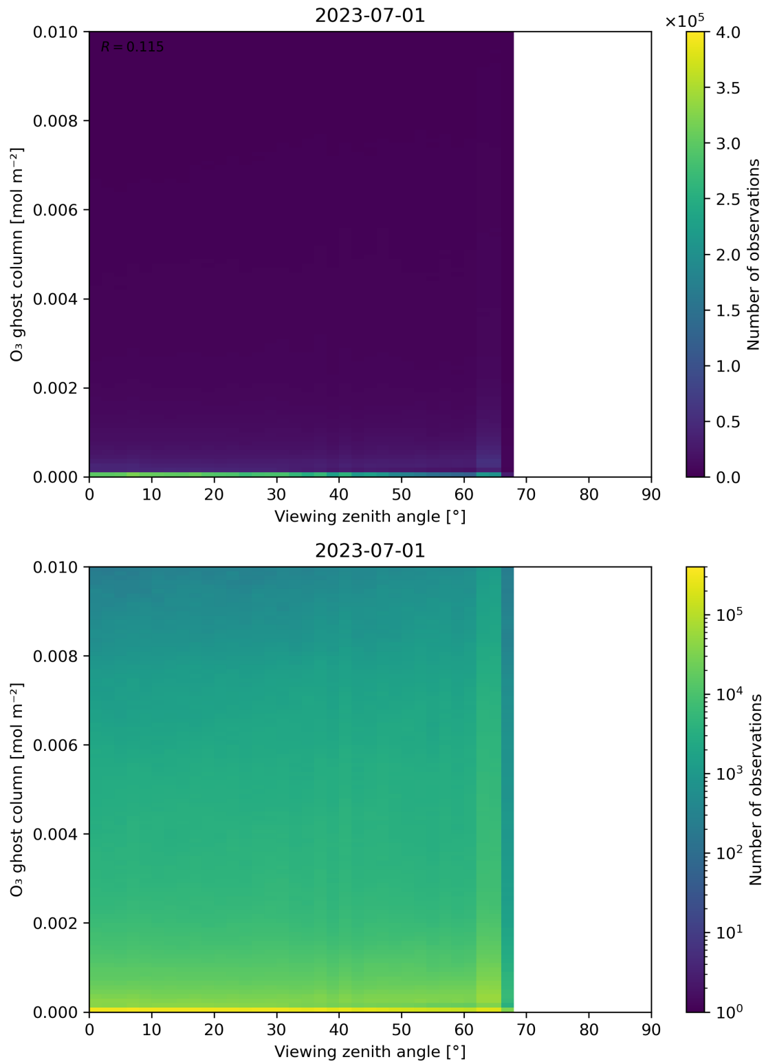
Figure 51: Scatter density plot of “Viewing zenith angle” against “O 3 ghost column” for 2023-06-30 to 2023-07-02.
