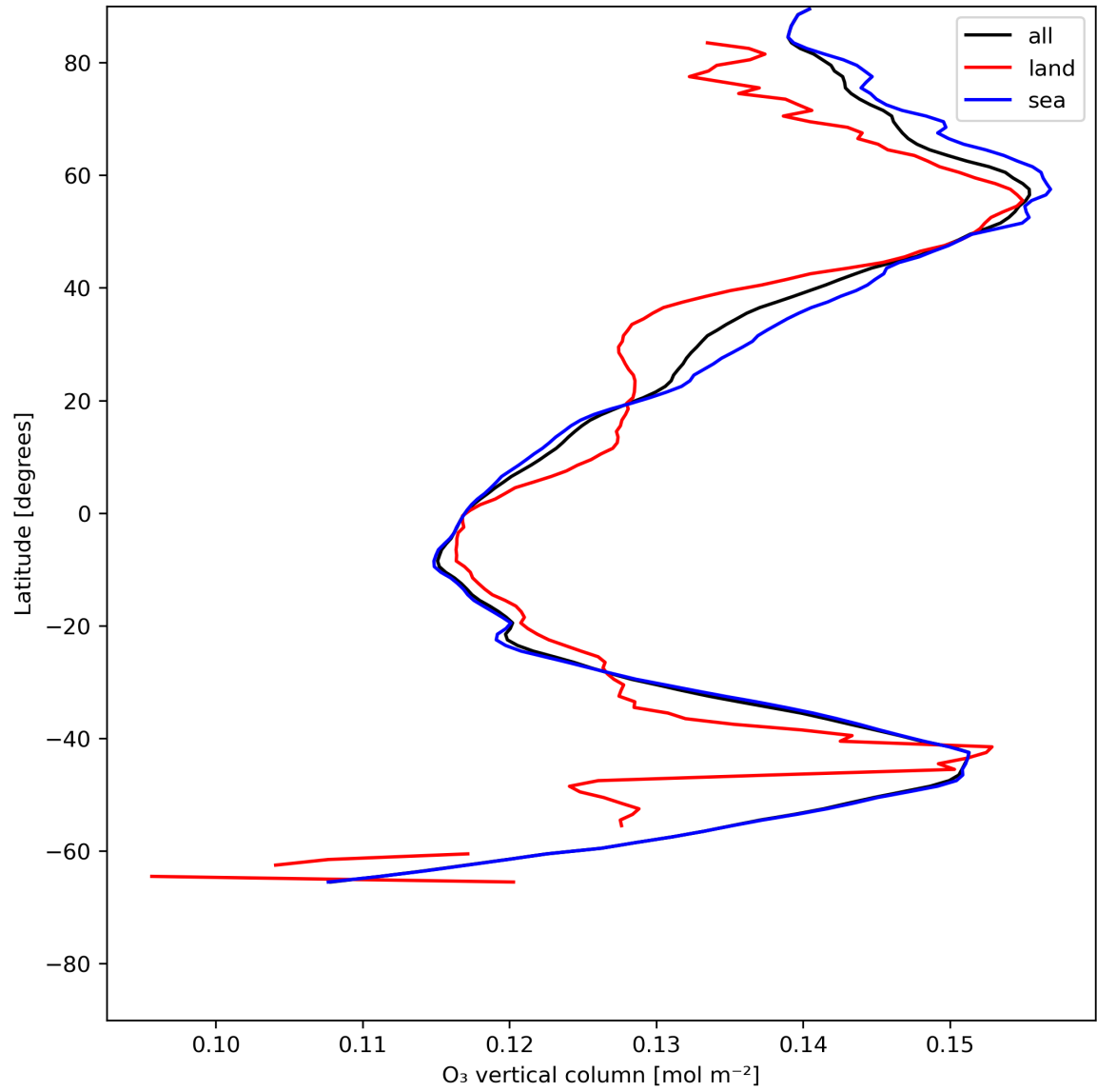
Figure 14: Zonal average of “O 3 vertical column” for 2023-06-30 to 2023-07-02.
