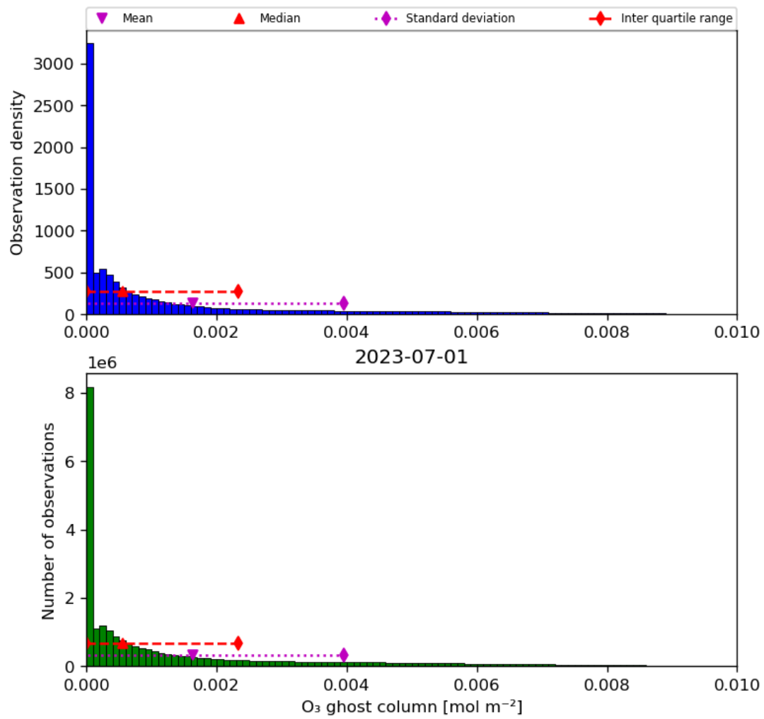
Figure 25: Histogram of “O 3 ghost column” for 2023-06-30 to 2023-07-02
