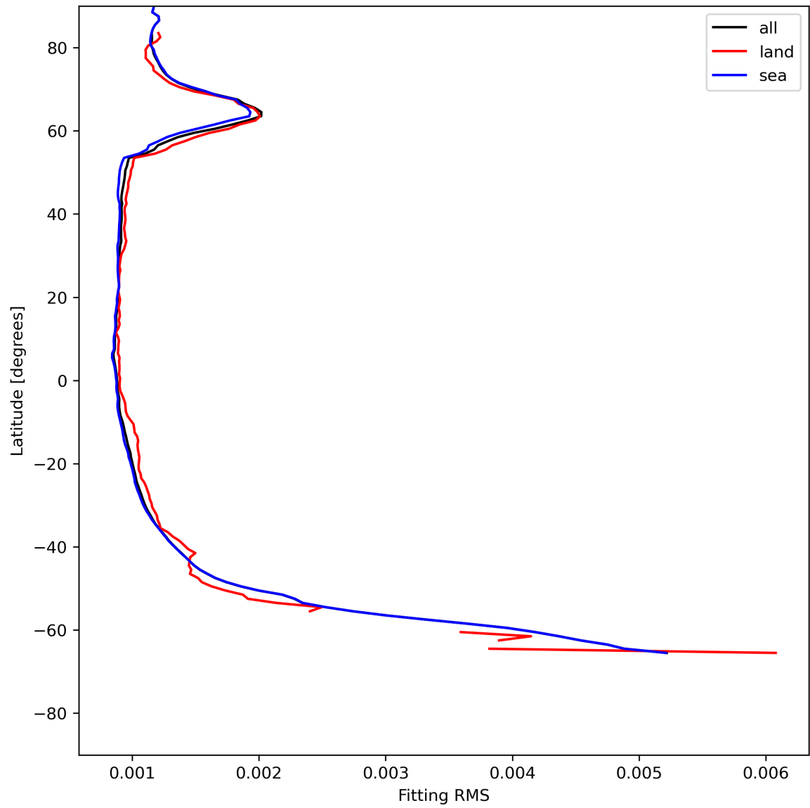
Figure 16: Zonal average of “Fitting RMS” for 2023-06-30 to 2023-07-02.
