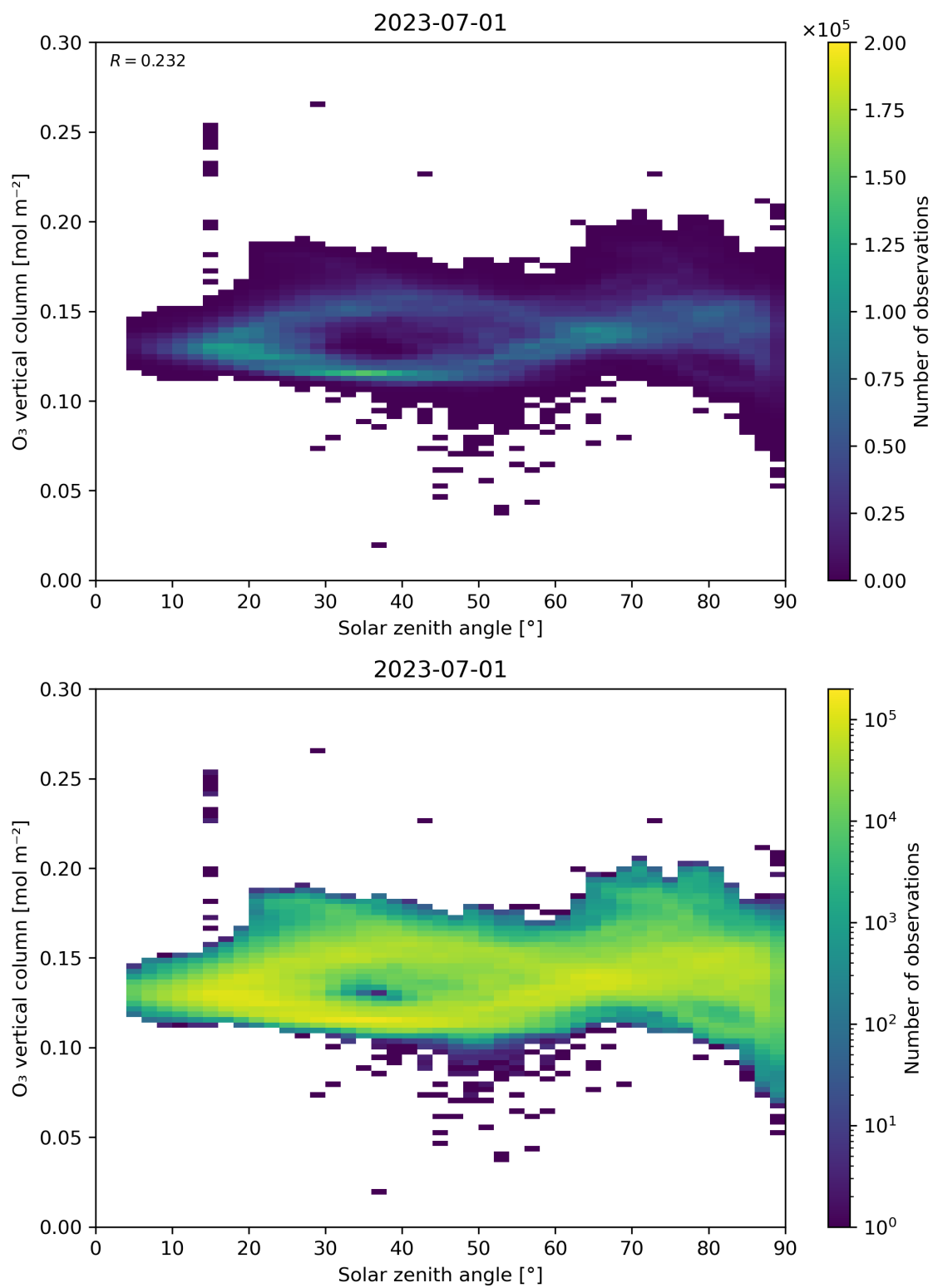
Figure 47: Scatter density plot of “Solar zenith angle” against “O 3 vertical column” for 2023-06-30 to 2023-07-02.
