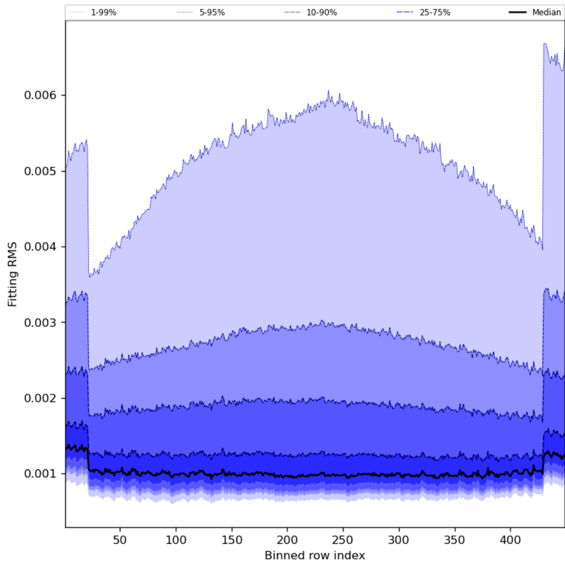
Figure 30: Along track statistics of “Fitting RMS” for 2023-06-30 to 2023-07-02
