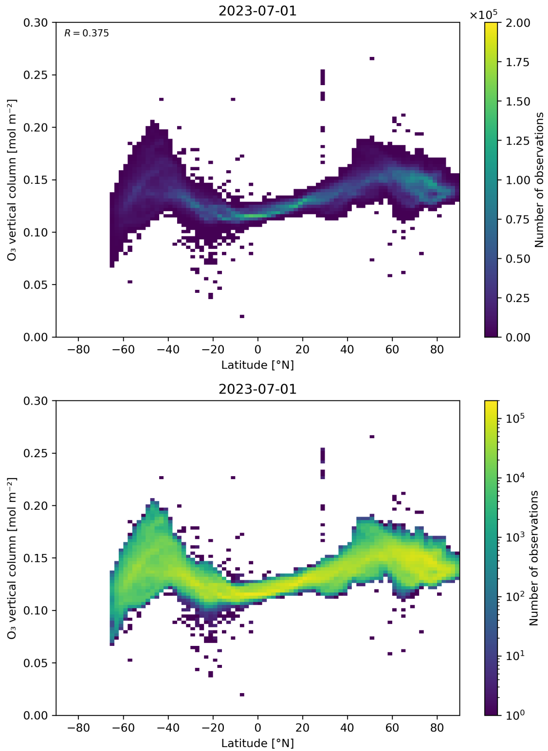
Figure 36: Scatter density plot of “Latitude” against “O 3 vertical column” for 2023-06-30 to 2023-07-02.
