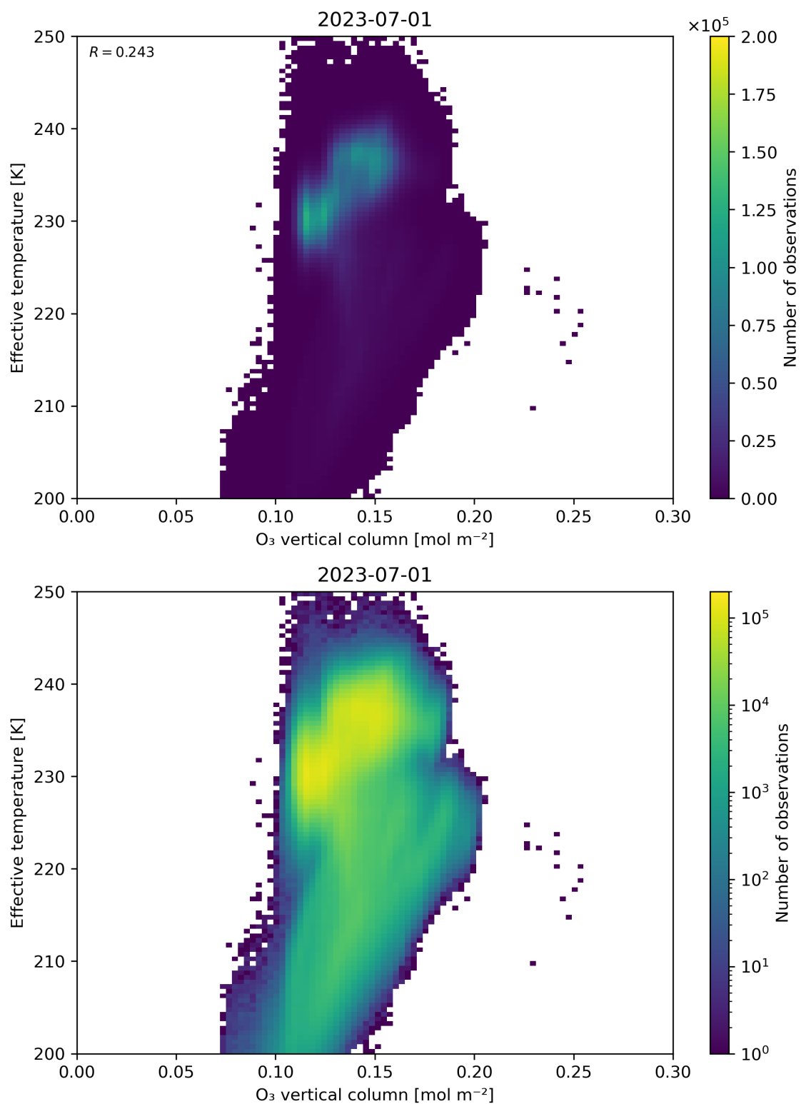
Figure 39: Scatter density plot of “O 3 vertical column” against “Effective temperature” for 2023-06-30 to 2023-07-02.
