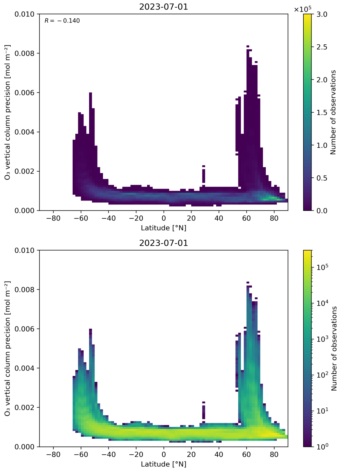
Figure 37: Scatter density plot of “Latitude” against “O 3 vertical column precision” for 2023-06-30 to 2023-07-02.
