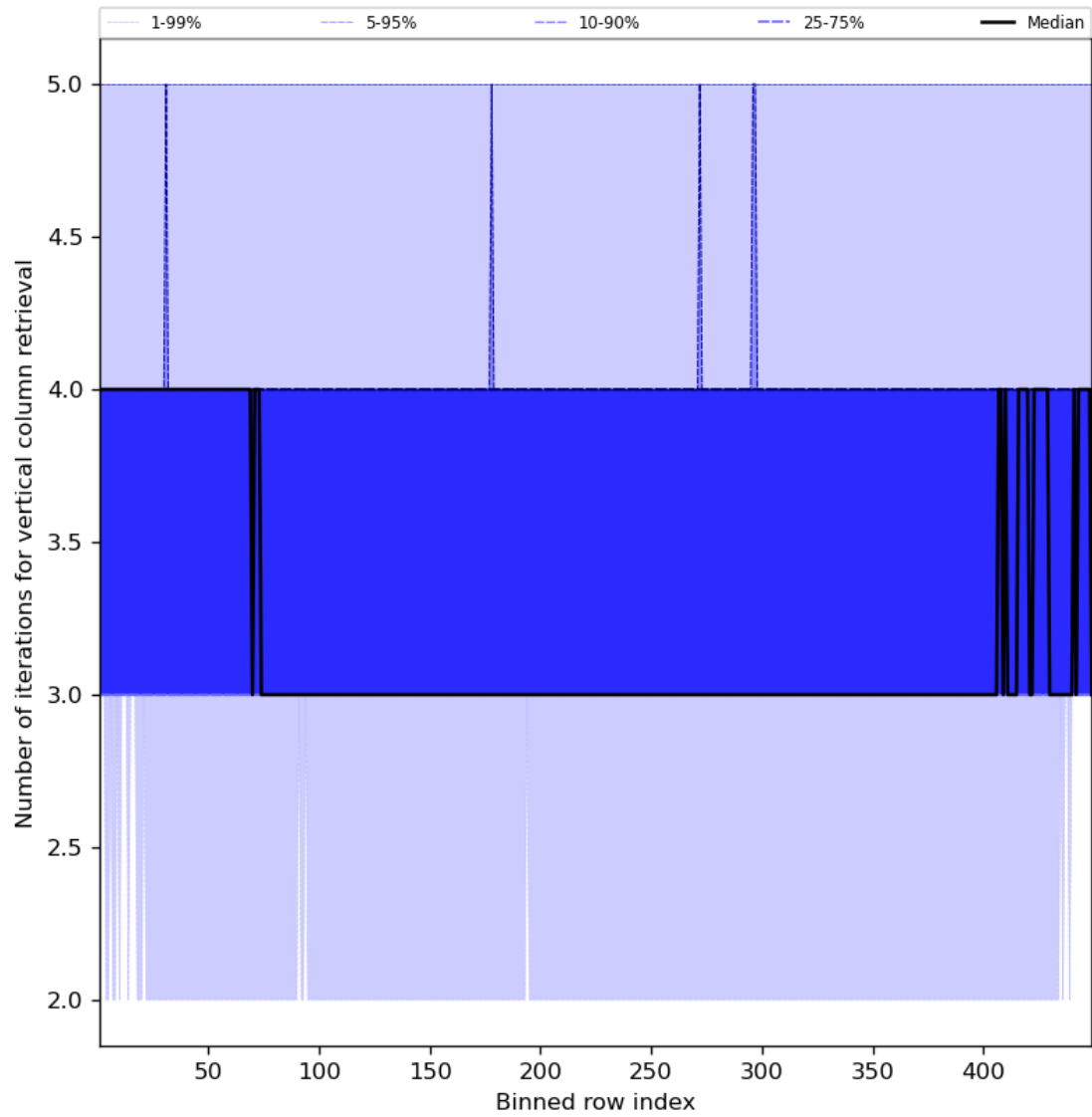
Figure 33: Along track statistics of “Number of iterations for vertical column retrieval” for 2023-06-30 to 2023-07-02
