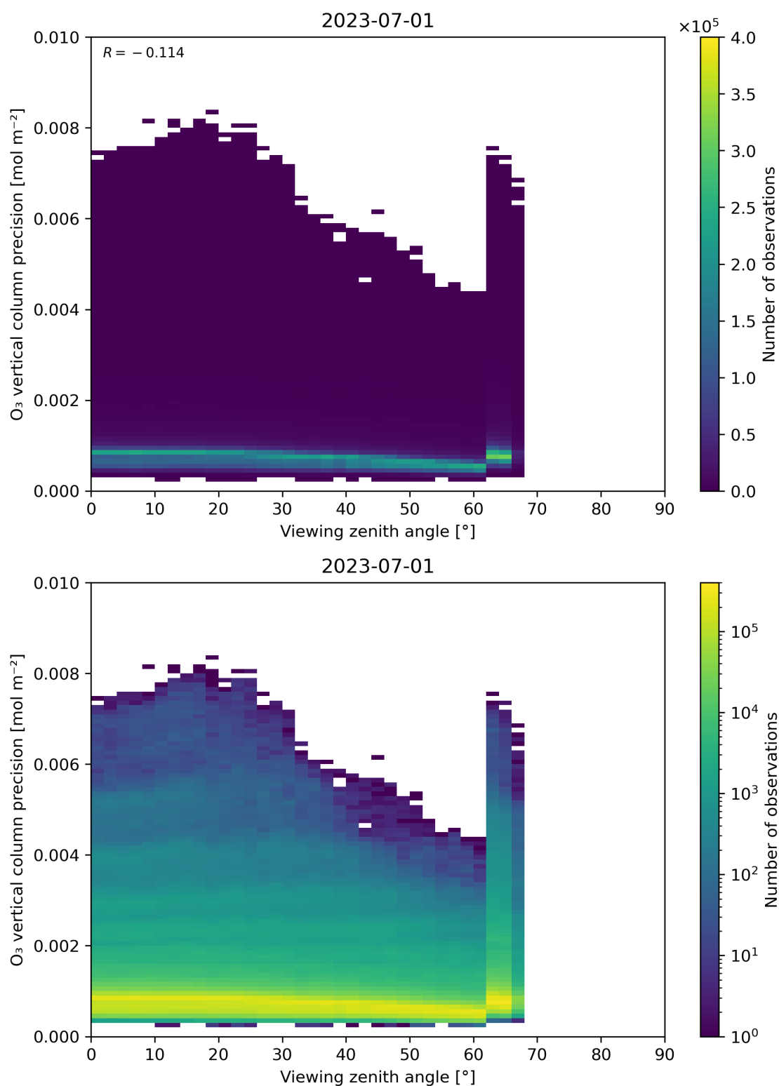
Figure 53: Scatter density plot of "Viewing zenith angle" against "O 3 vertical column precision" for 2023-06-30 to 2023-07-02.
