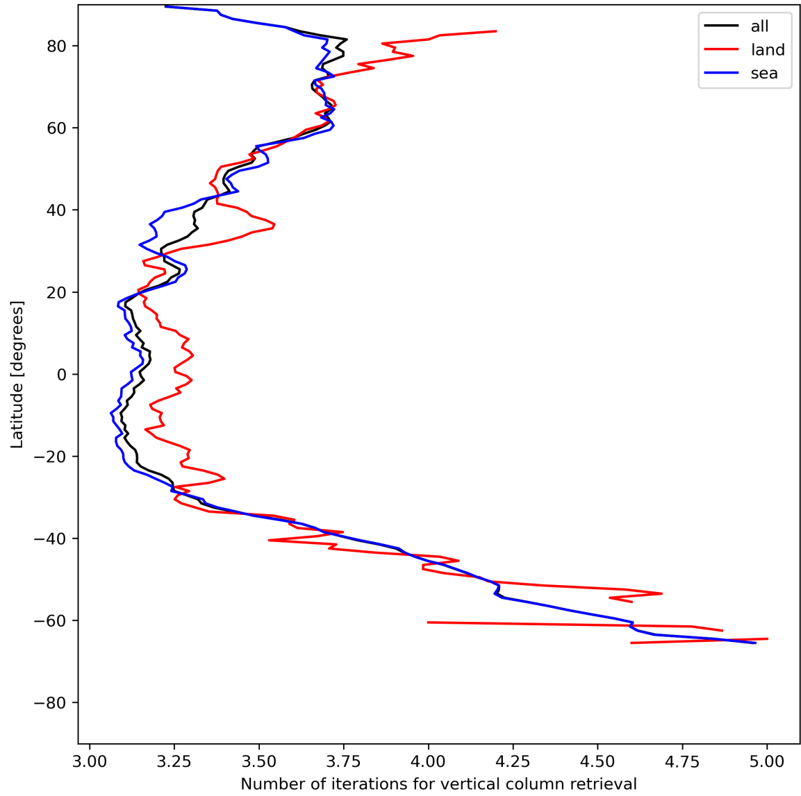
Figure 19: Zonal average of “Number of iterations for vertical column retrieval” for 2023-06-30 to 2023-07-02.
