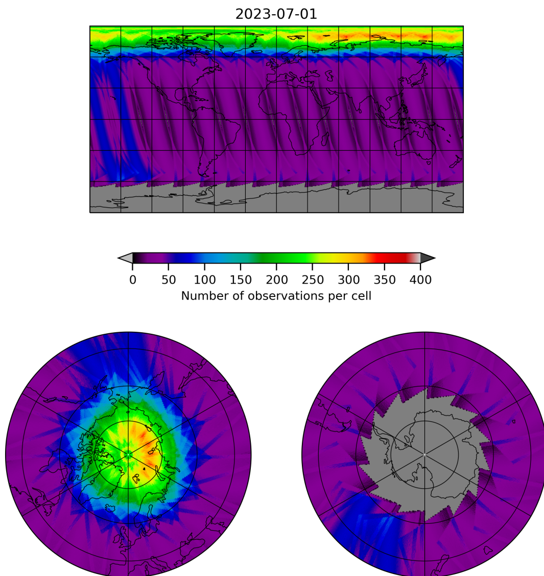
Figure 12: Map of the number of observations for 2023-06-30 to 2023-07-02
