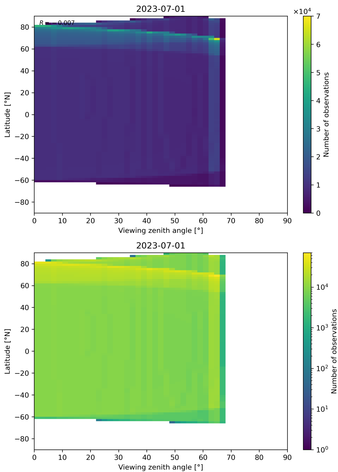
Figure 49: Scatter density plot of “Viewing zenith angle” against “Latitude” for 2023-06-30 to 2023-07-02.
