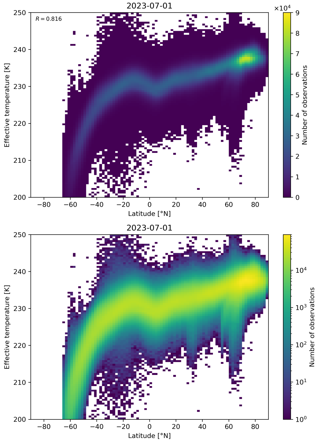
Figure 34: Scatter density plot of “Latitude” against “Effective temperature” for 2023-06-30 to 2023-07-02.
