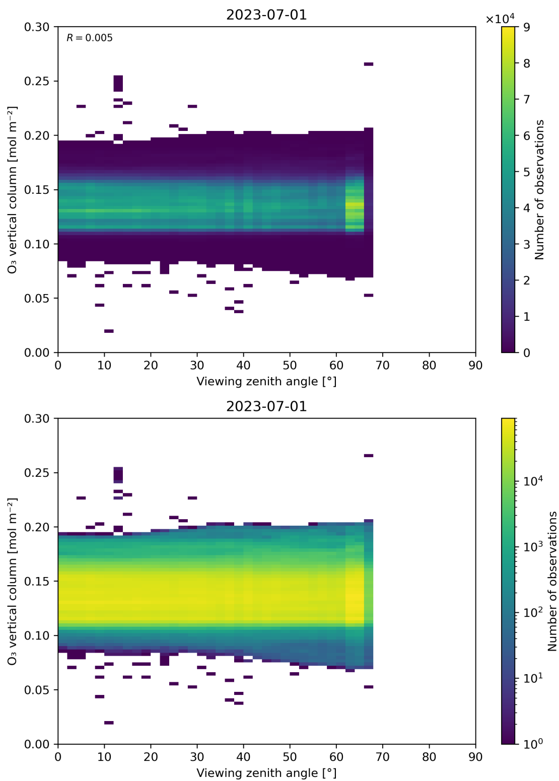
Figure 52: Scatter density plot of “Viewing zenith angle” against “O 3 vertical column” for 2023-06-30 to 2023-07-02.
