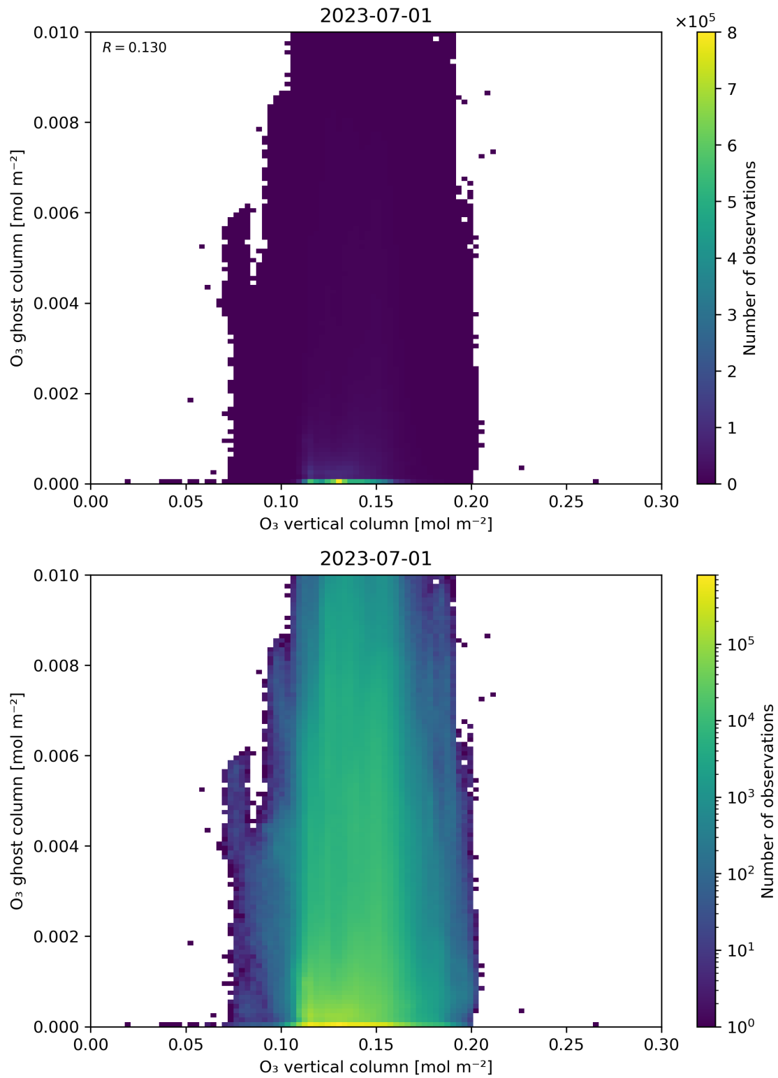
Figure 40: Scatter density plot of “O 3 vertical column” against “O 3 ghost column” for 2023-06-30 to 2023-07-02.
