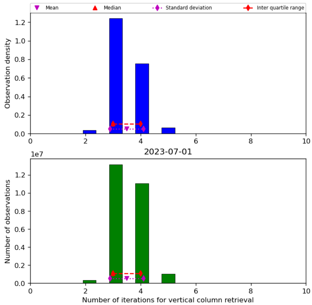
Figure 26: Histogram of “Number of iterations for vertical column retrieval” for 2023-06-30 to 2023-07-02
