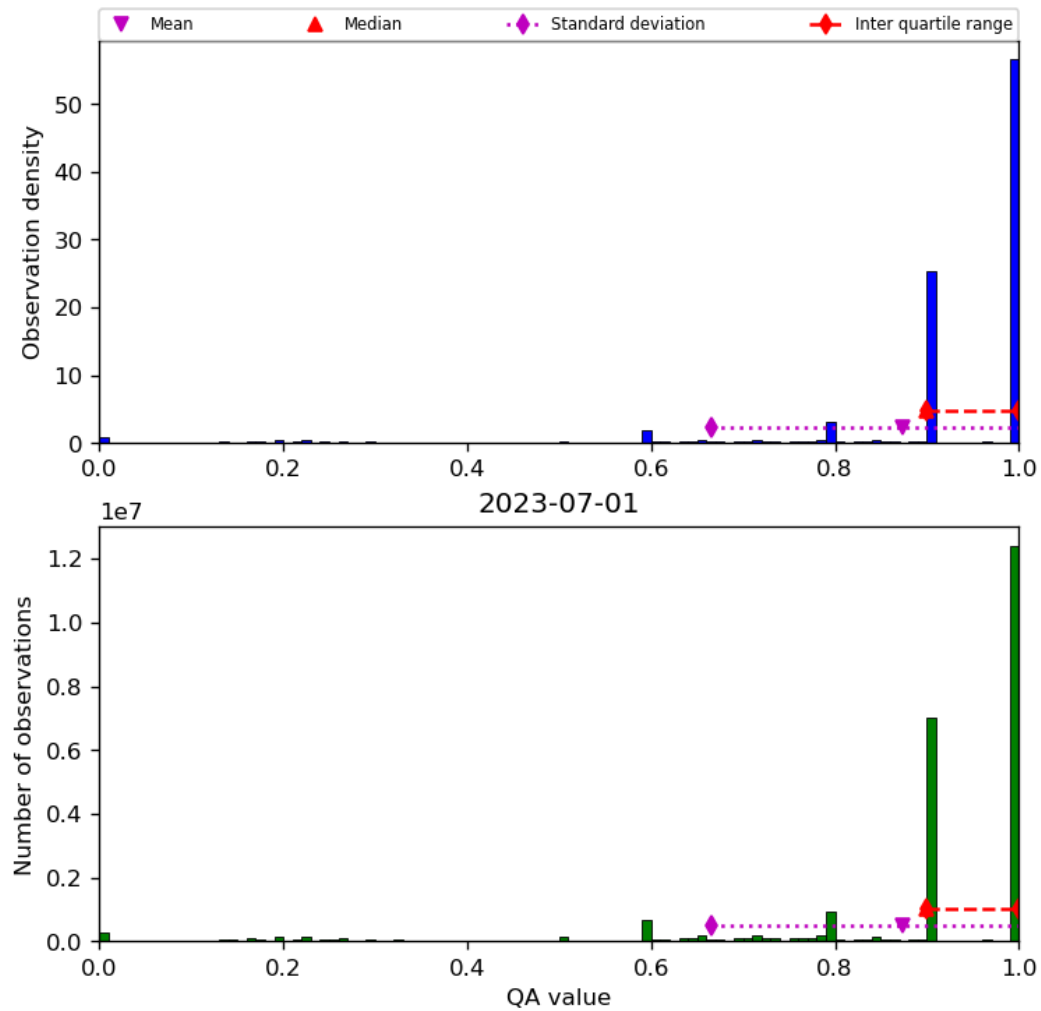
Figure 20: Histogram of “QA value” for 2023-06-30 to 2023-07-02
