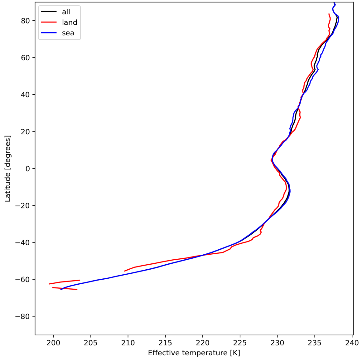
Figure 17: Zonal average of “Effective temperature” for 2023-06-30 to 2023-07-02.
