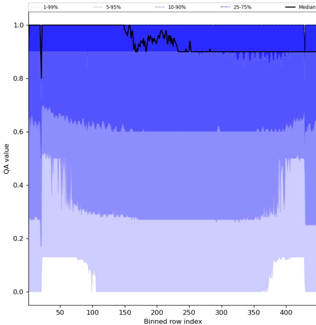
Figure 27: Along track statistics of “QA value” for 2023-06-30 to 2023-07-02
