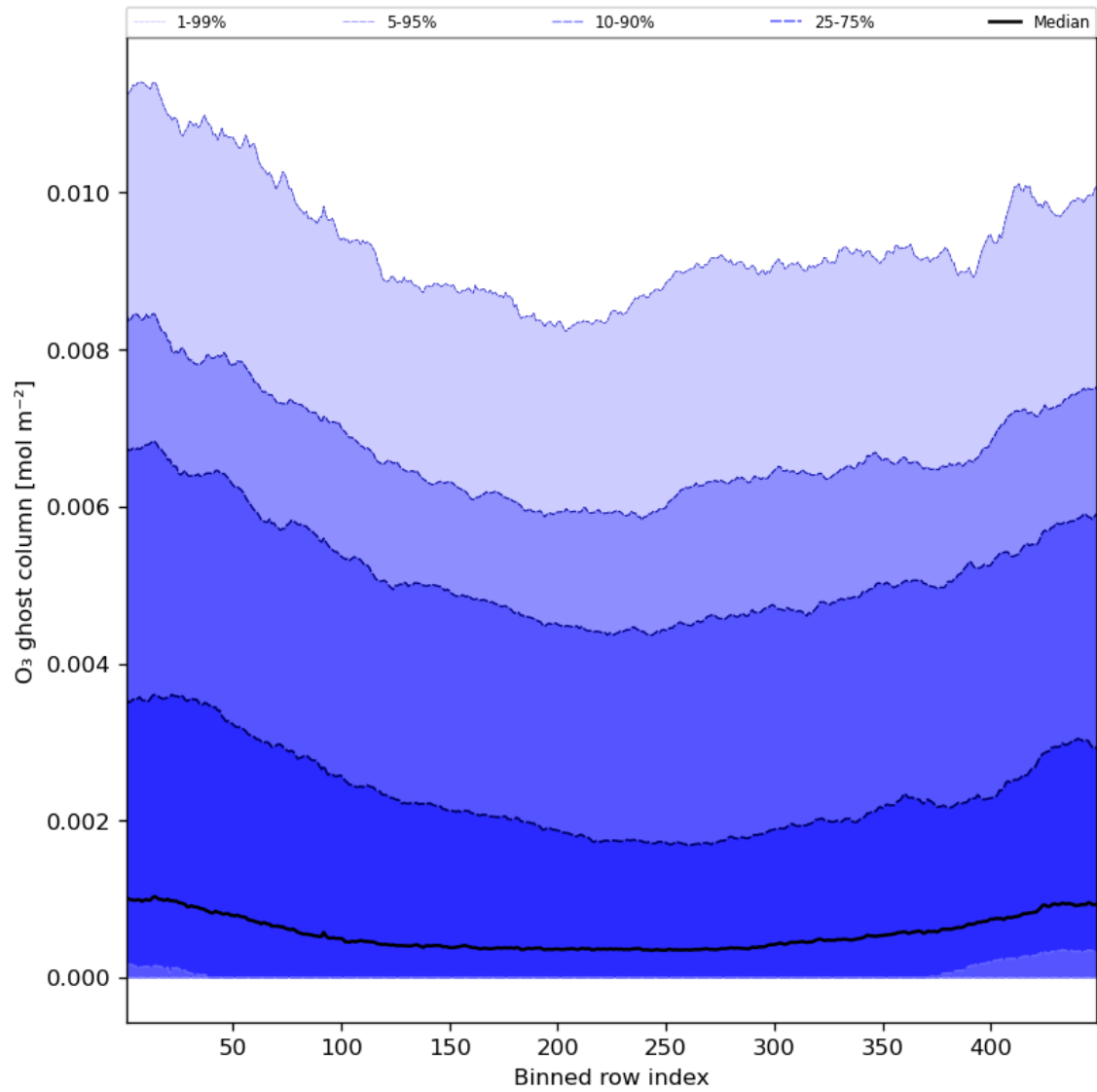
Figure 32: Along track statistics of “O 3 ghost column” for 2023-06-30 to 2023-07-02
