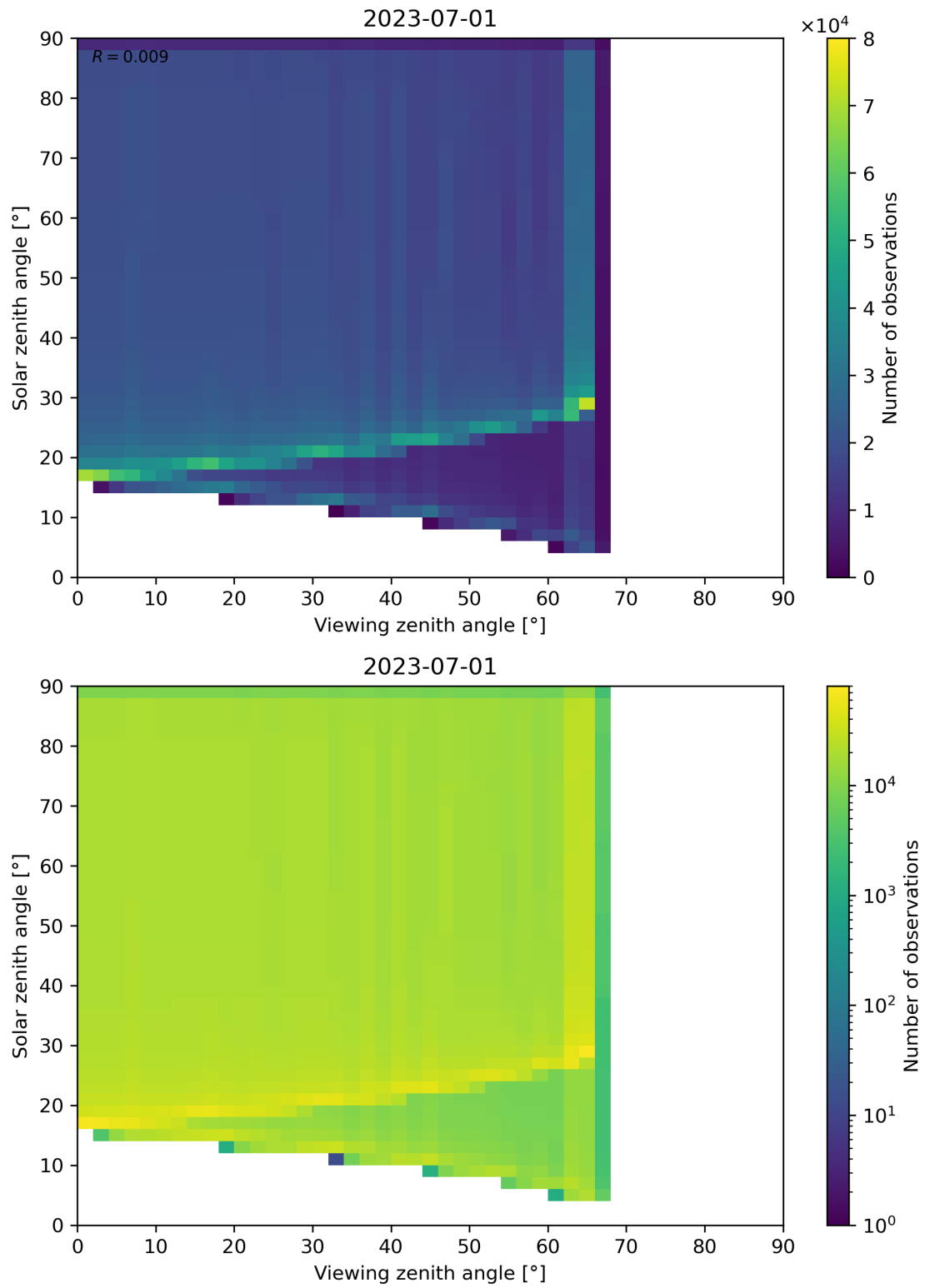
Figure 54: Scatter density plot of “Viewing zenith angle” against “Solar zenith angle” for 2023-06-30 to 2023-07-02.
