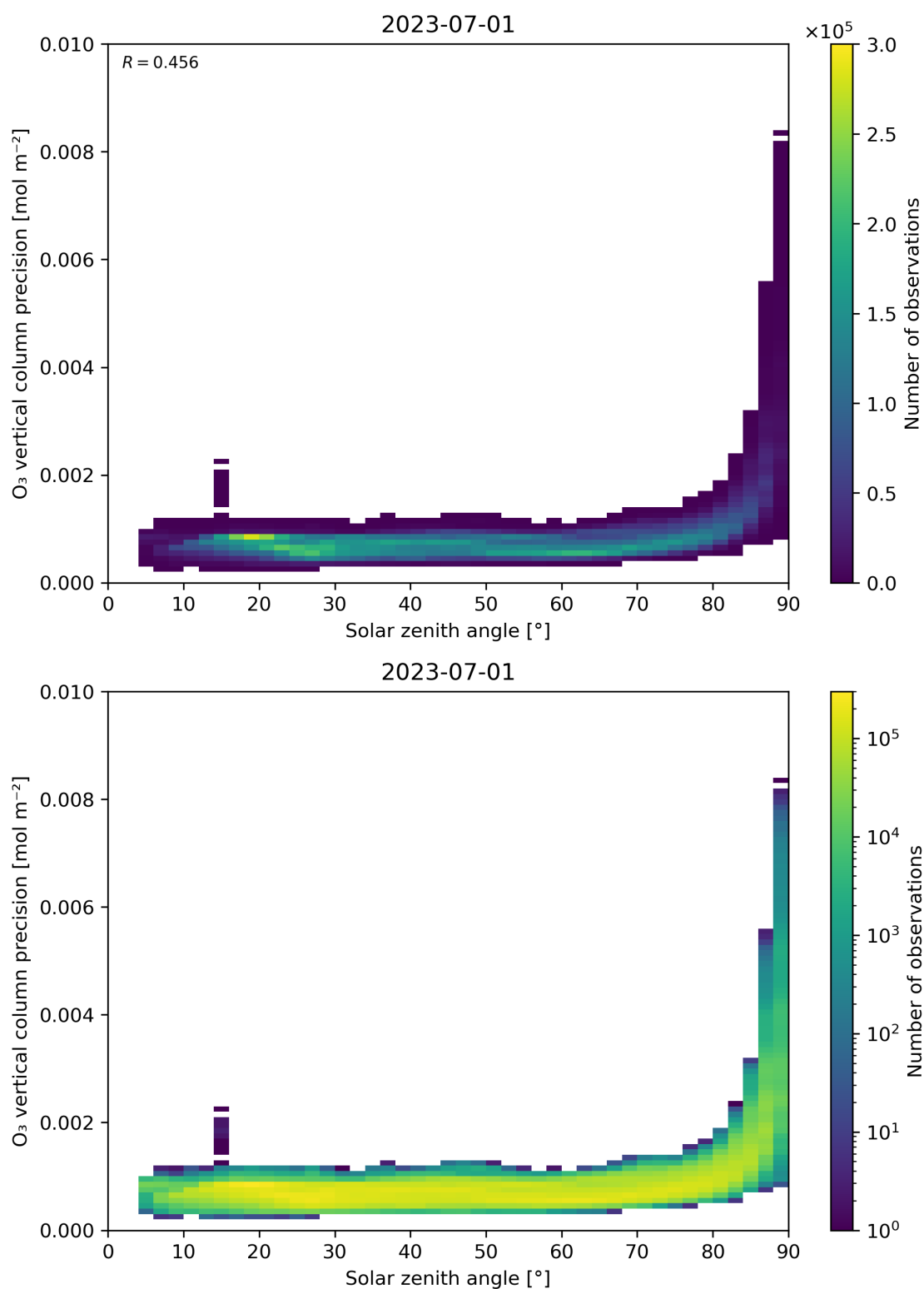
Figure 48: Scatter density plot of “Solar zenith angle” against “O 3 vertical column precision” for 2023-06-30 to 2023-07-02.
