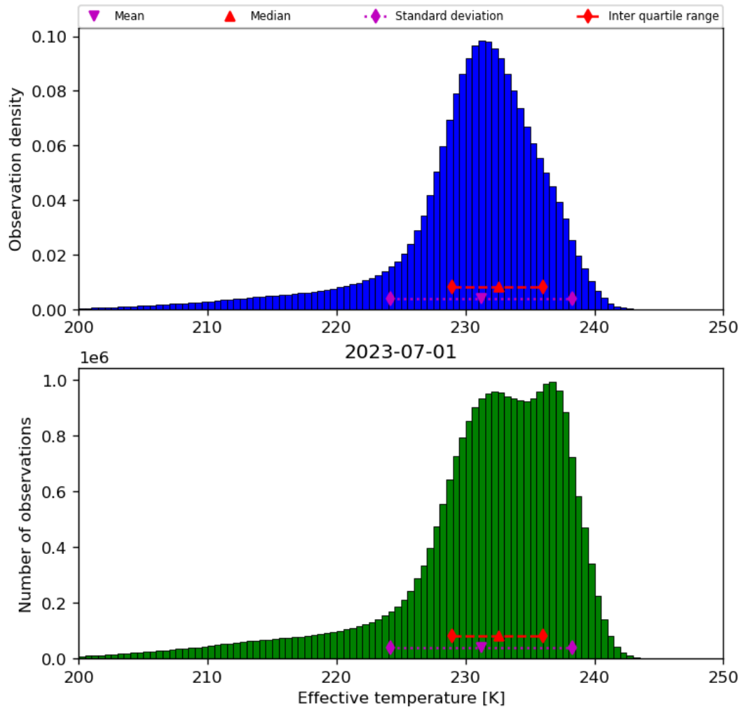
Figure 24: Histogram of “Effective temperature” for 2023-06-30 to 2023-07-02
