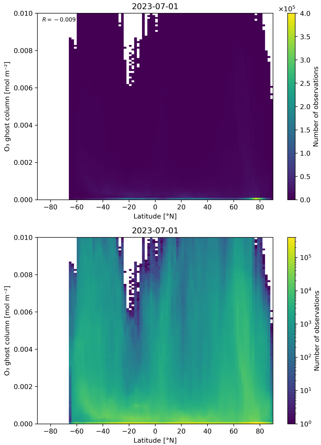
Figure 35: Scatter density plot of “Latitude” against “O 3 ghost column” for 2023-06-30 to 2023-07-02.
