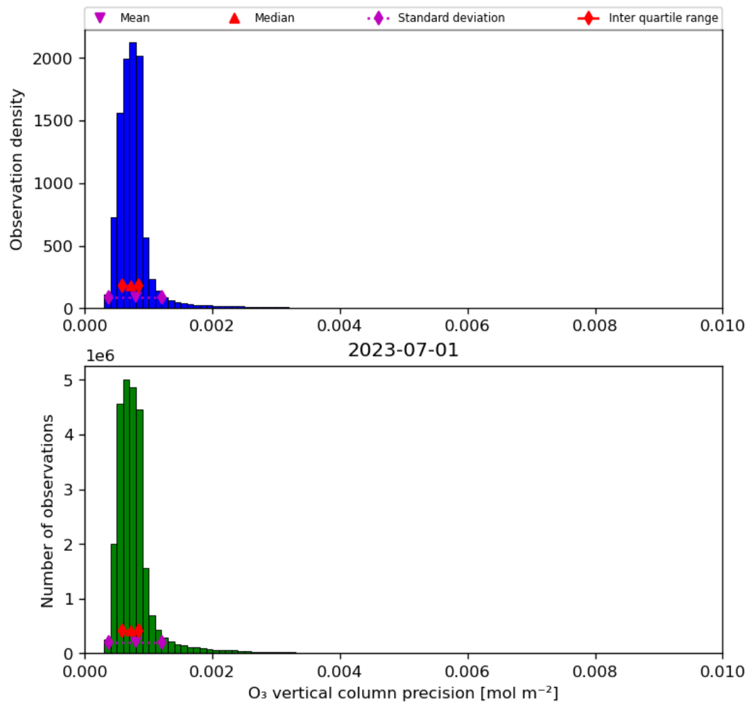
Figure 22: Histogram of “O 3 vertical column precision” for 2023-06-30 to 2023-07-02
