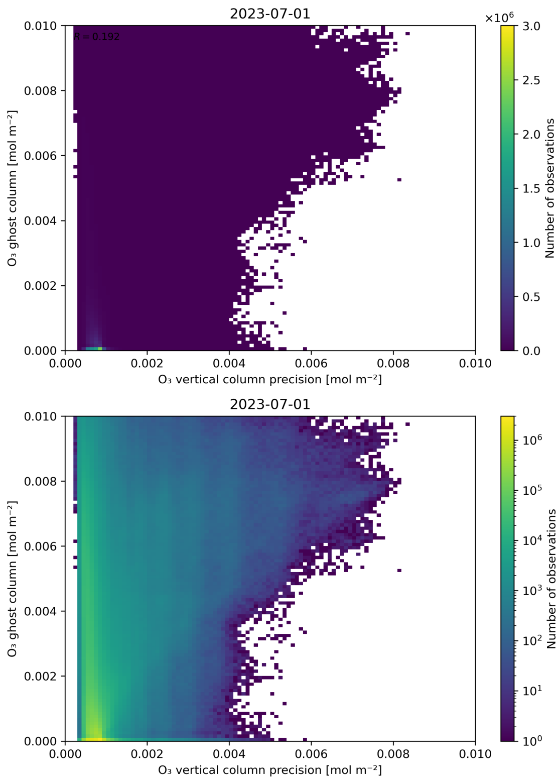
Figure 43: Scatter density plot of “ \text{O}_3 vertical column precision” against “ \text{O}_3 ghost column” for 2023-06-30 to 2023-07-02.
