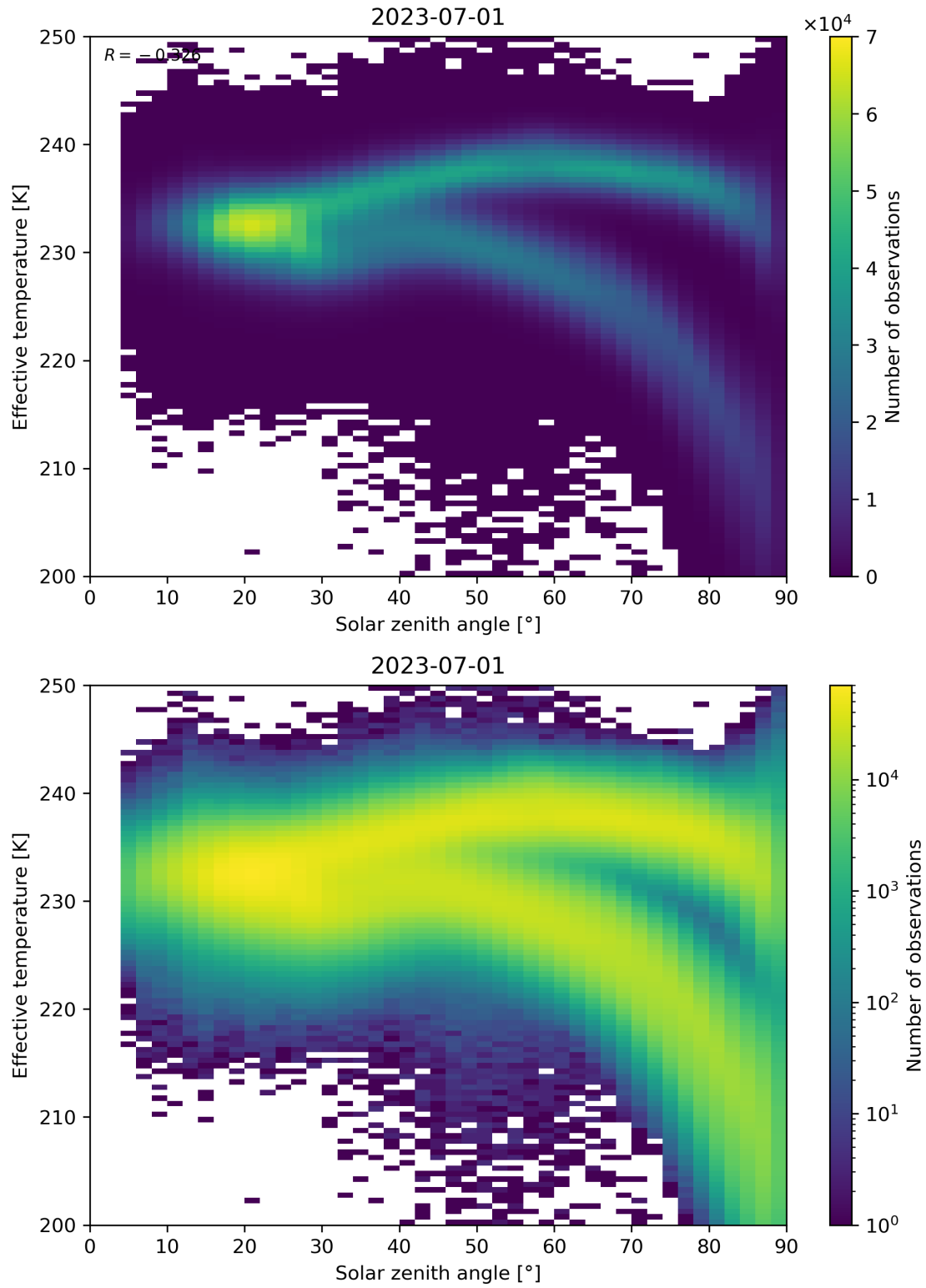
Figure 45: Scatter density plot of “Solar zenith angle” against “Effective temperature” for 2023-06-30 to 2023-07-02.
