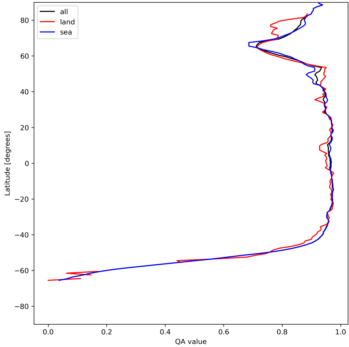
Figure 13: Zonal average of “QA value” for 2023-06-30 to 2023-07-02.
