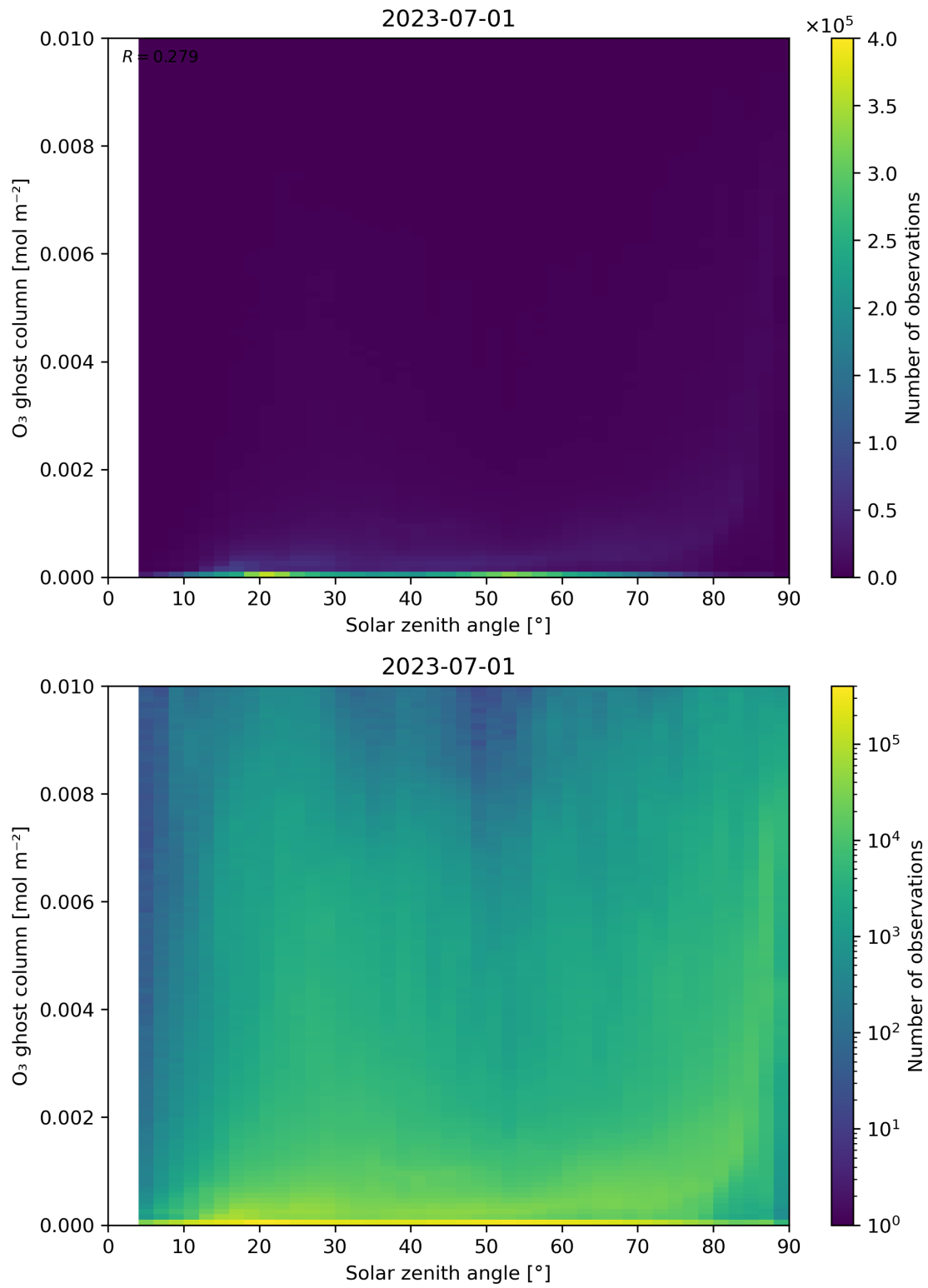
Figure 46: Scatter density plot of “Solar zenith angle” against “O 3 ghost column” for 2023-06-30 to 2023-07-02.
