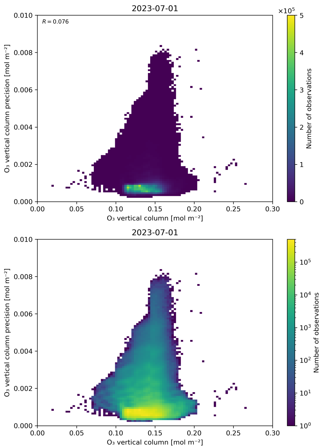
Figure 41: Scatter density plot of “O 3 vertical column” against “O 3 vertical column precision” for 2023-06-30 to 2023-07-02.
