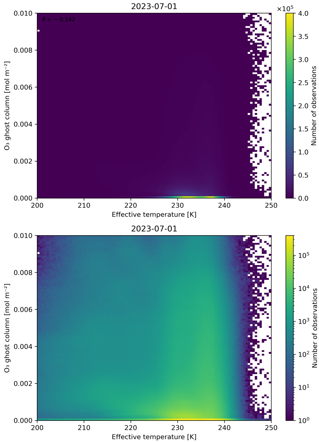
Figure 38: Scatter density plot of “Effective temperature” against “O 3 ghost column” for 2023-06-30 to 2023-07-02.
