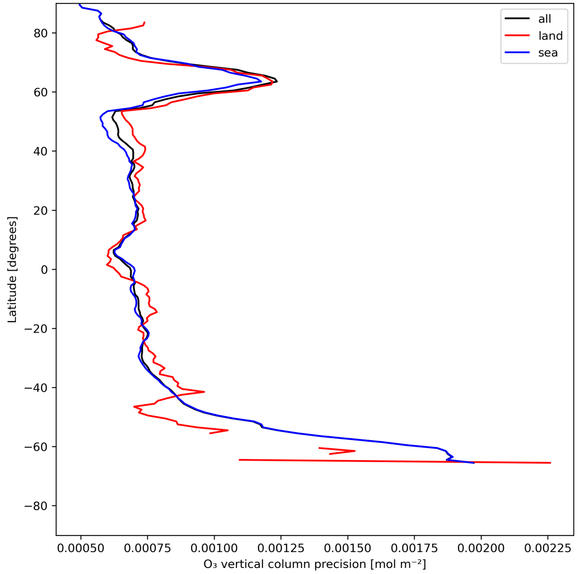
Figure 15: Zonal average of “O 3 vertical column precision” for 2023-06-30 to 2023-07-02.
