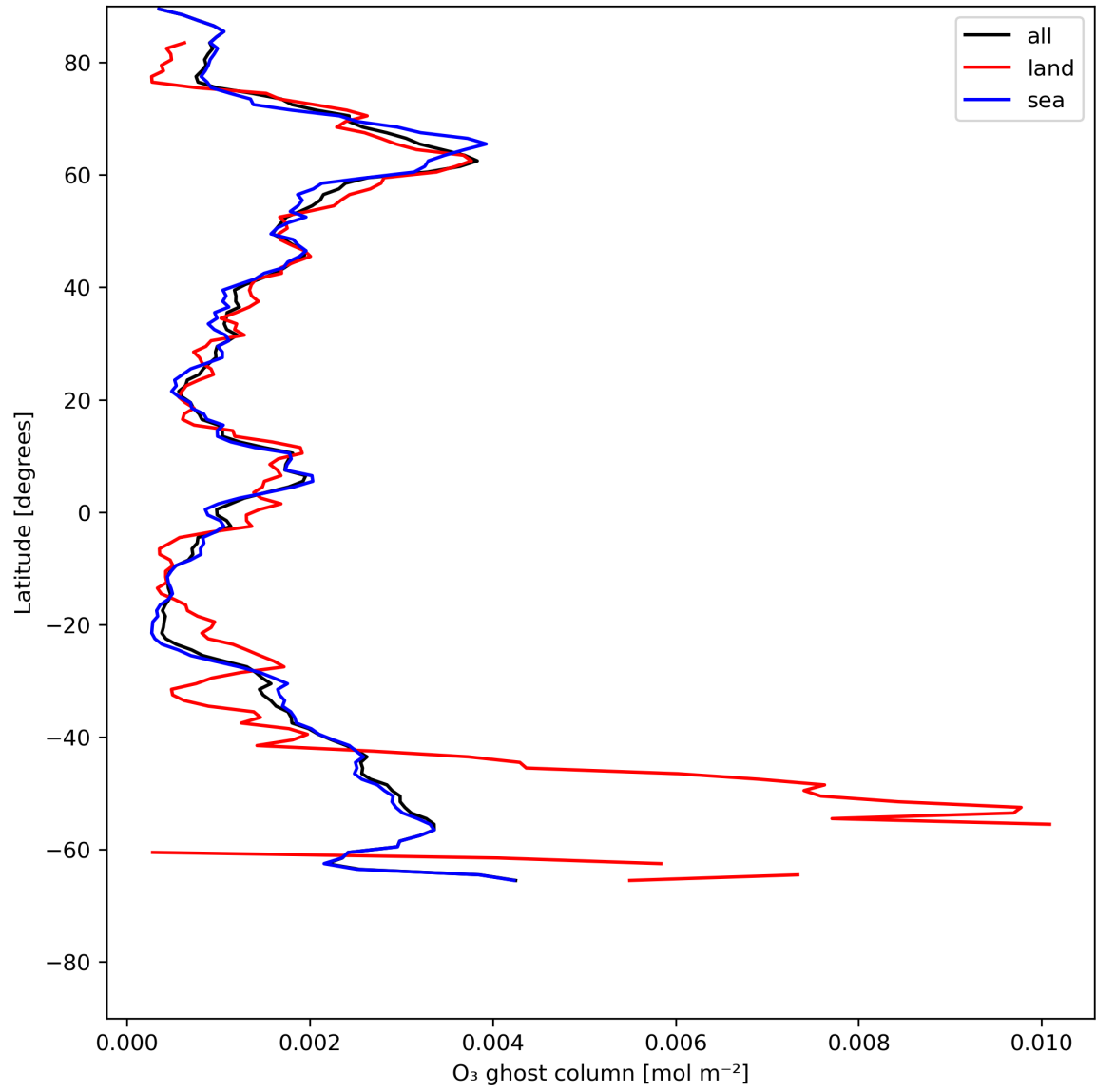
Figure 18: Zonal average of “O 3 ghost column” for 2023-06-30 to 2023-07-02.
