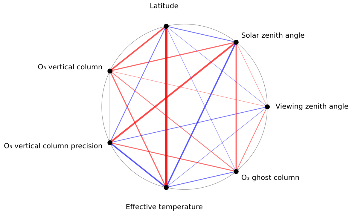
Figure 1: Map of correlation graph for 2023-06-30 to 2023-07-02.
