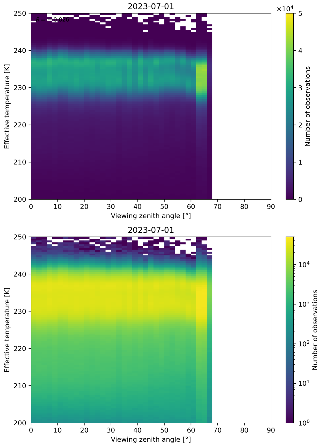
Figure 50: Scatter density plot of “Viewing zenith angle” against “Effective temperature” for 2023-06-30 to 2023-07-02.
