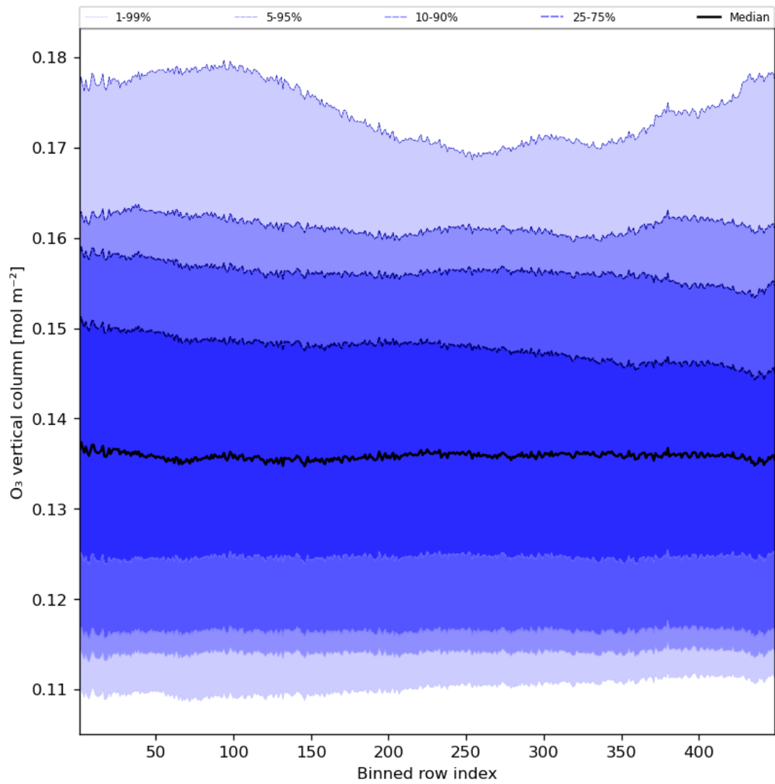
Figure 28: Along track statistics of “O 3 vertical column” for 2023-06-30 to 2023-07-02
