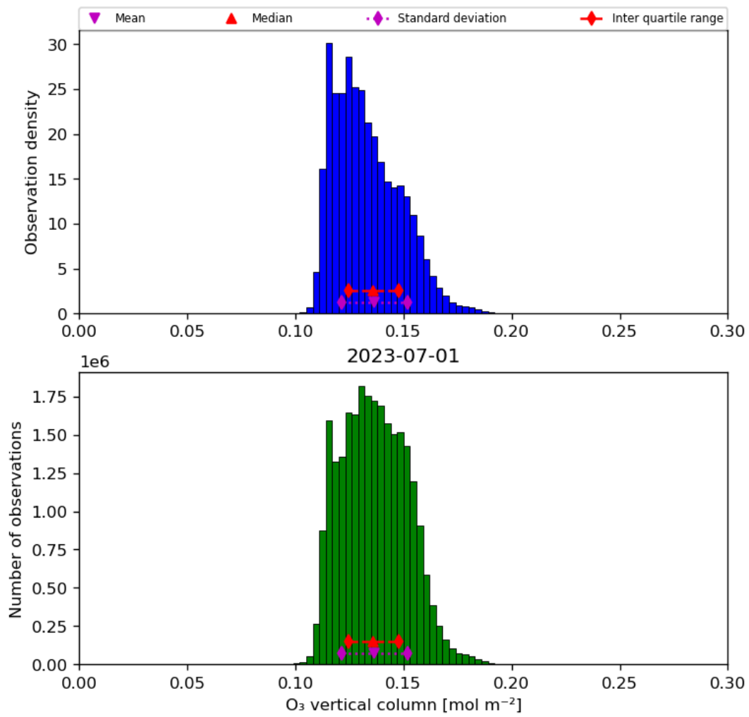
Figure 21: Histogram of “O 3 vertical column” for 2023-06-30 to 2023-07-02
