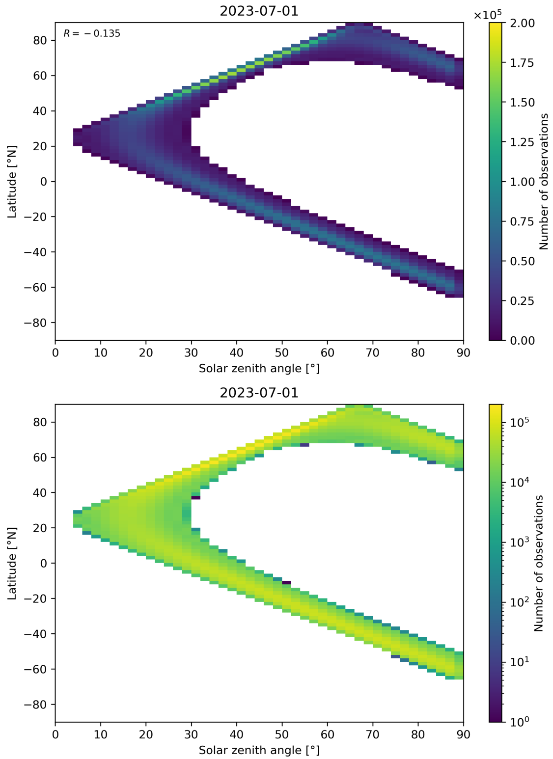
Figure 44: Scatter density plot of “Solar zenith angle” against “Latitude” for 2023-06-30 to 2023-07-02.
