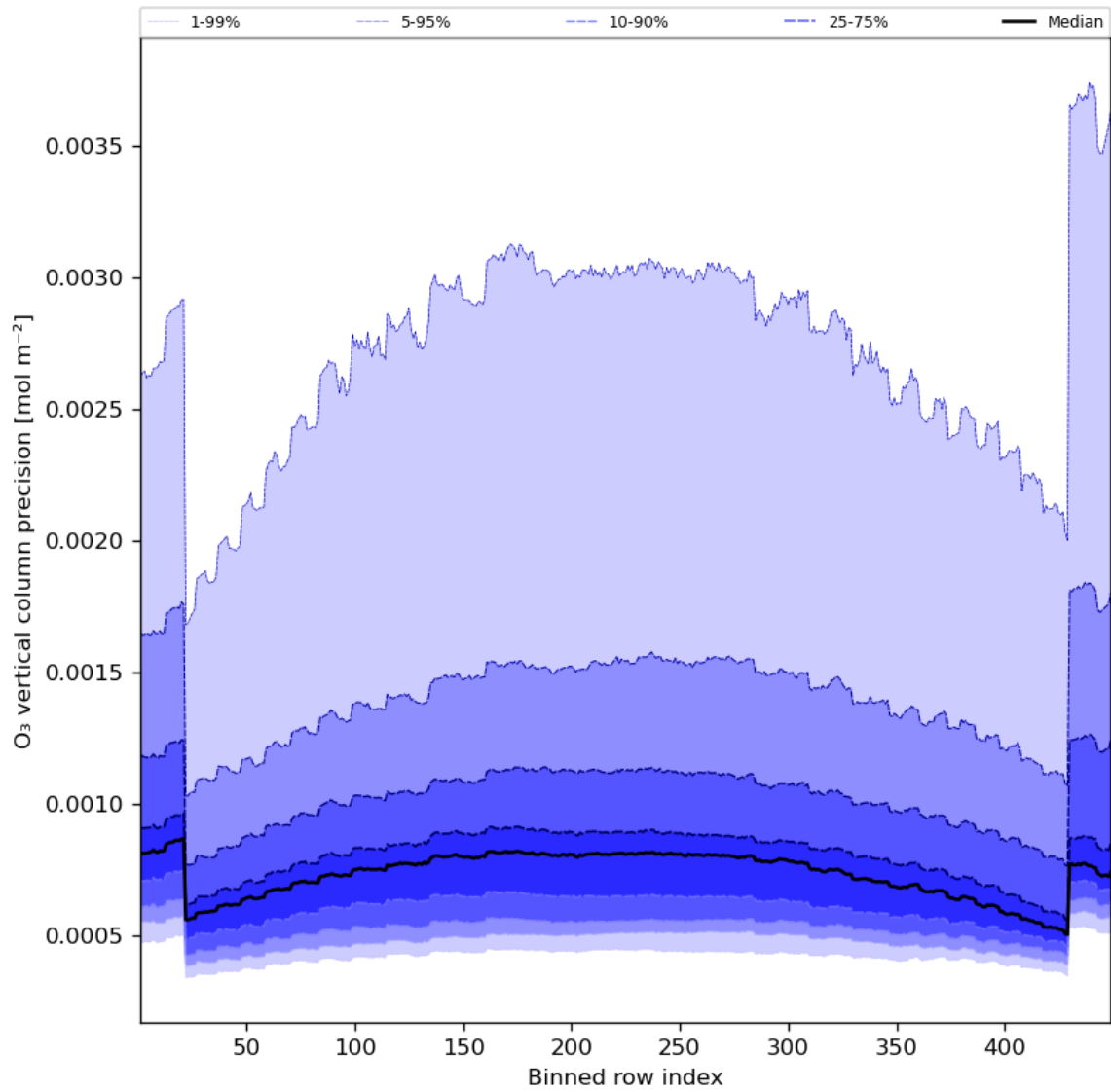
Figure 29: Along track statistics of “O 3 vertical column precision” for 2023-06-30 to 2023-07-02
