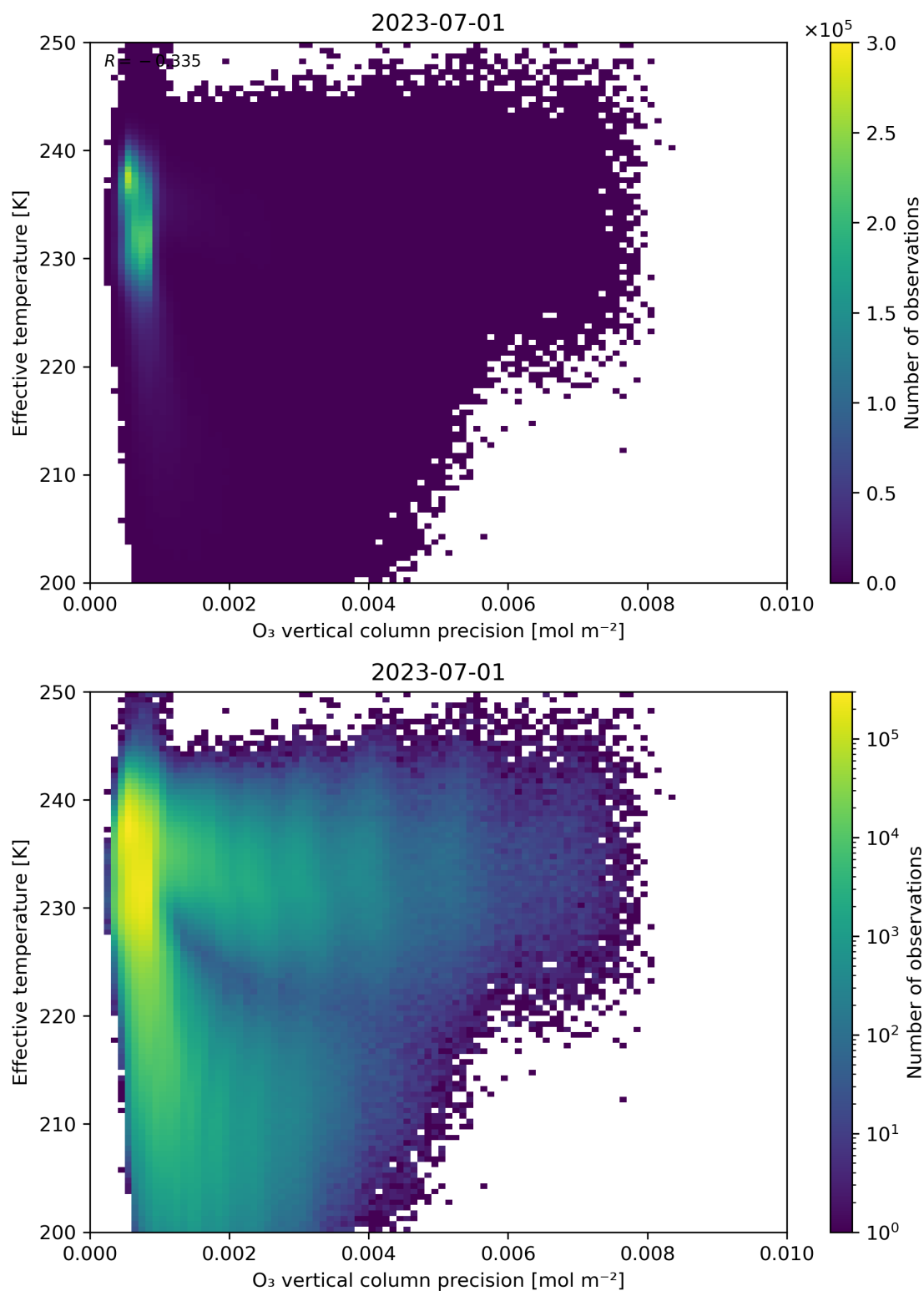
Figure 42: Scatter density plot of “O 3 vertical column precision” against “Effective temperature” for 2023-06-30 to 2023-07-02.
