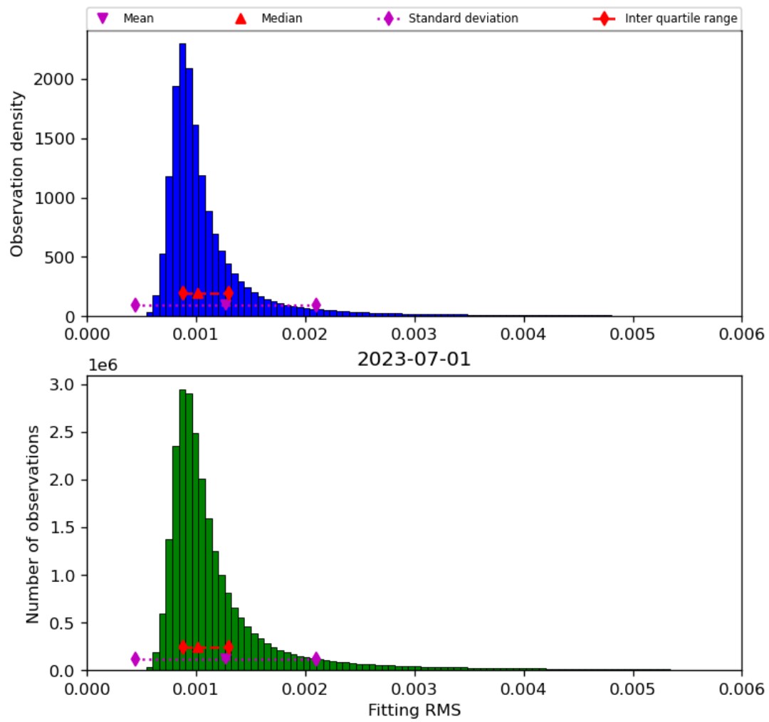
Figure 23: Histogram of “Fitting RMS” for 2023-06-30 to 2023-07-02
