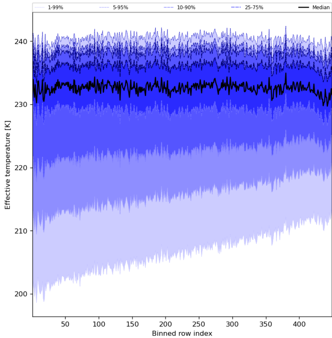
Figure 31: Along track statistics of “Effective temperature” for 2023-06-30 to 2023-07-02
