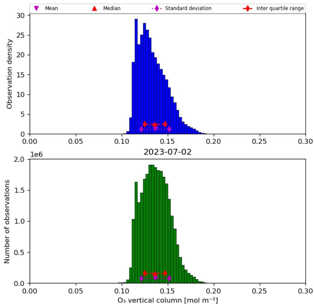
Figure 21: Histogram of “O 3 vertical column” for 2023-07-01 to 2023-07-03
