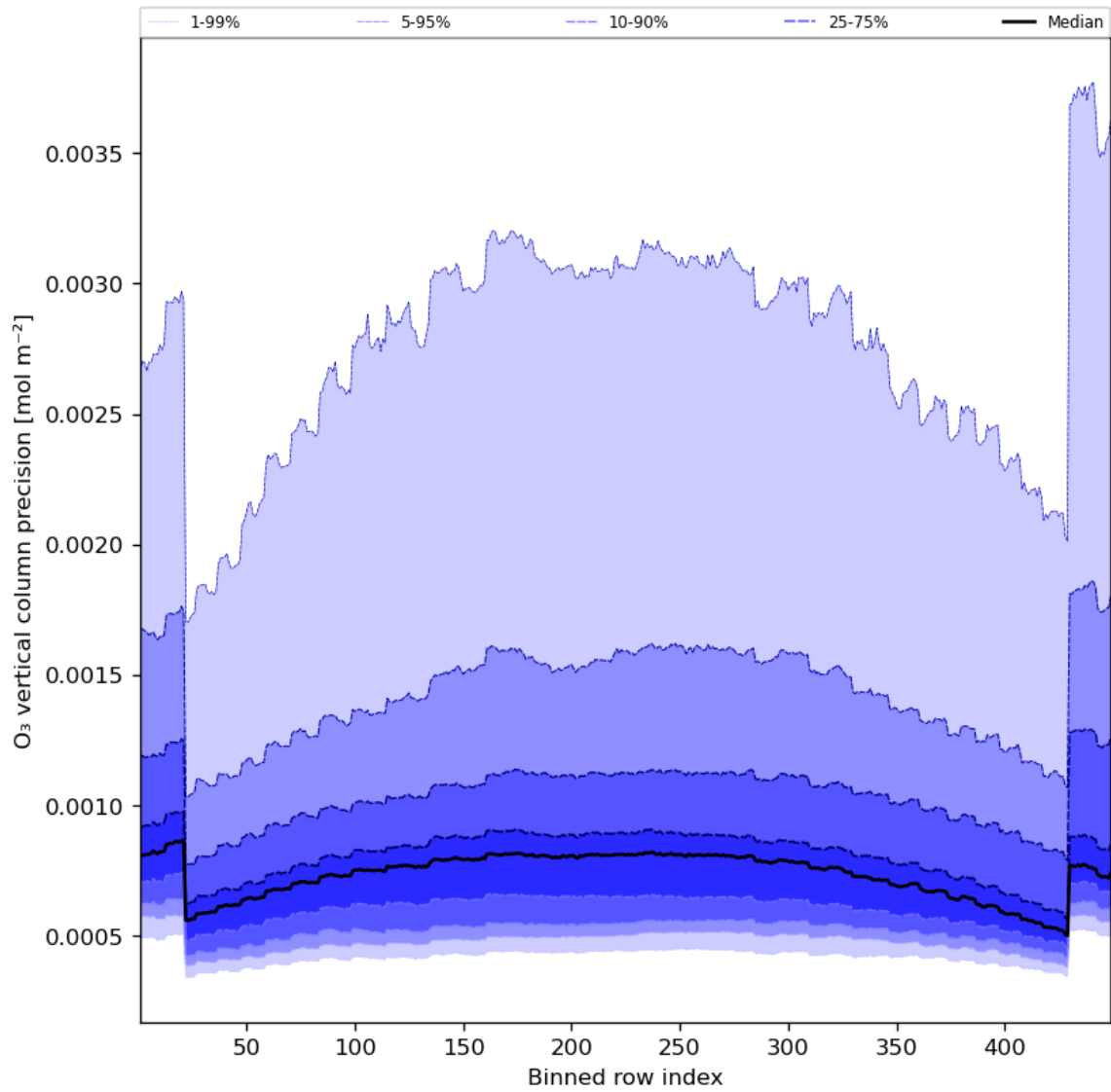
Figure 29: Along track statistics of “O 3 vertical column precision” for 2023-07-01 to 2023-07-03
