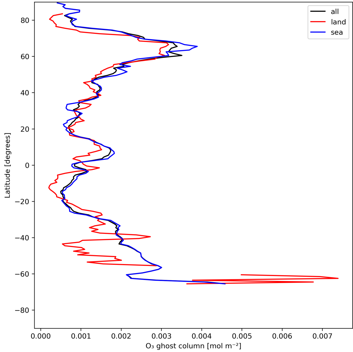
Figure 18: Zonal average of “O 3 ghost column” for 2023-07-01 to 2023-07-03.
