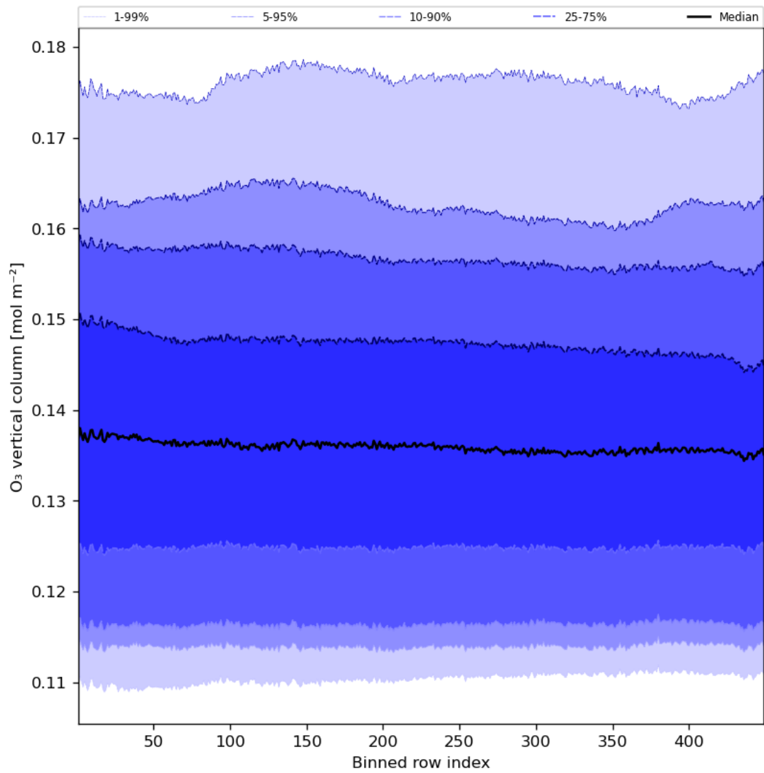
Figure 28: Along track statistics of “O 3 vertical column” for 2023-07-01 to 2023-07-03
