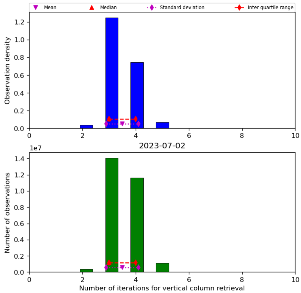
Figure 26: Histogram of “Number of iterations for vertical column retrieval” for 2023-07-01 to 2023-07-03
