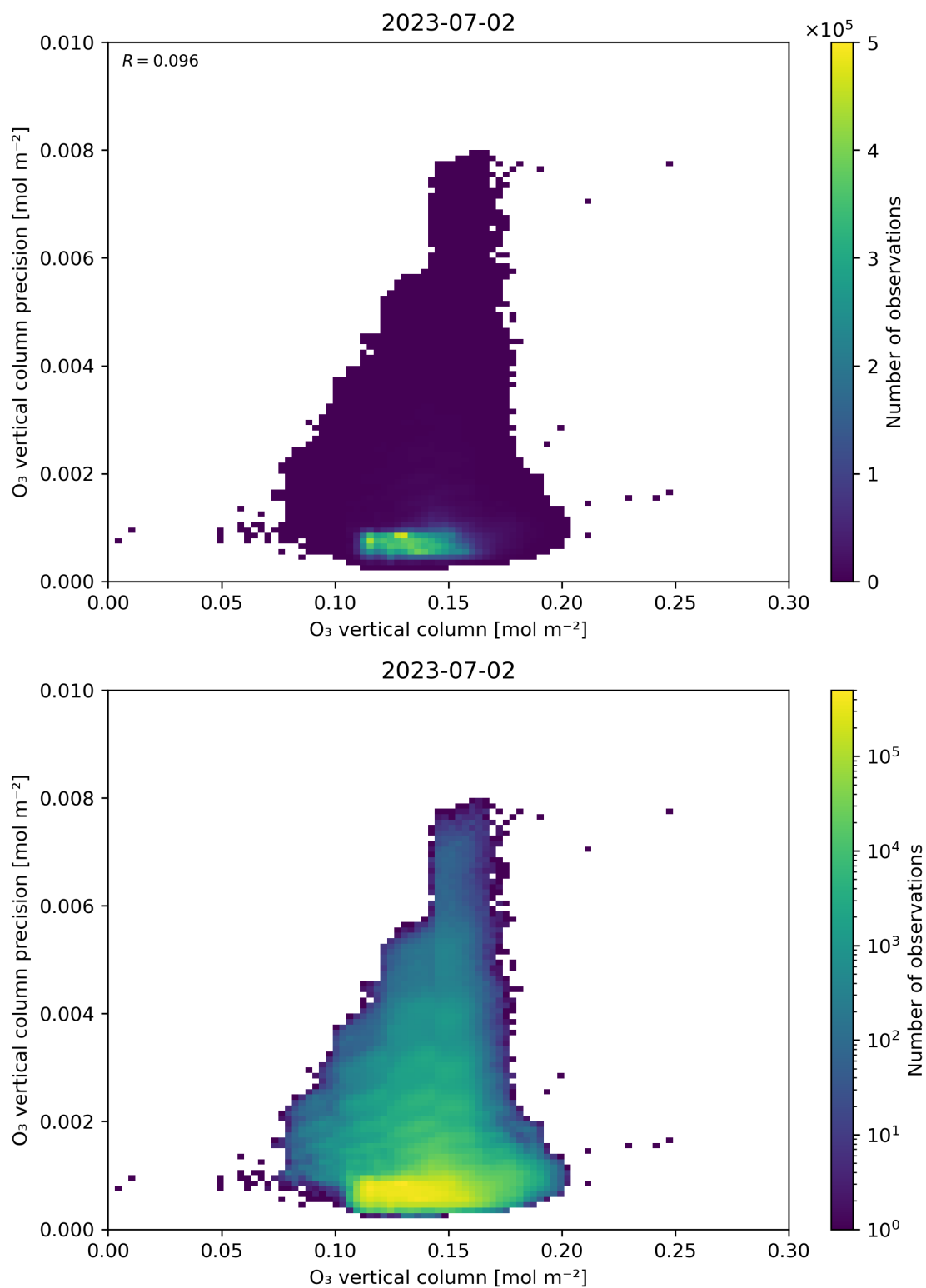
Figure 41: Scatter density plot of “O 3 vertical column” against “O 3 vertical column precision” for 2023-07-01 to 2023-07-03.
