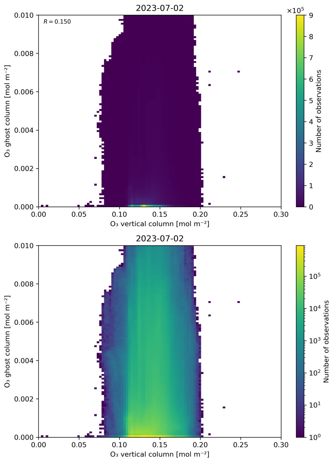
Figure 40: Scatter density plot of “O 3 vertical column” against “O 3 ghost column” for 2023-07-01 to 2023-07-03.
