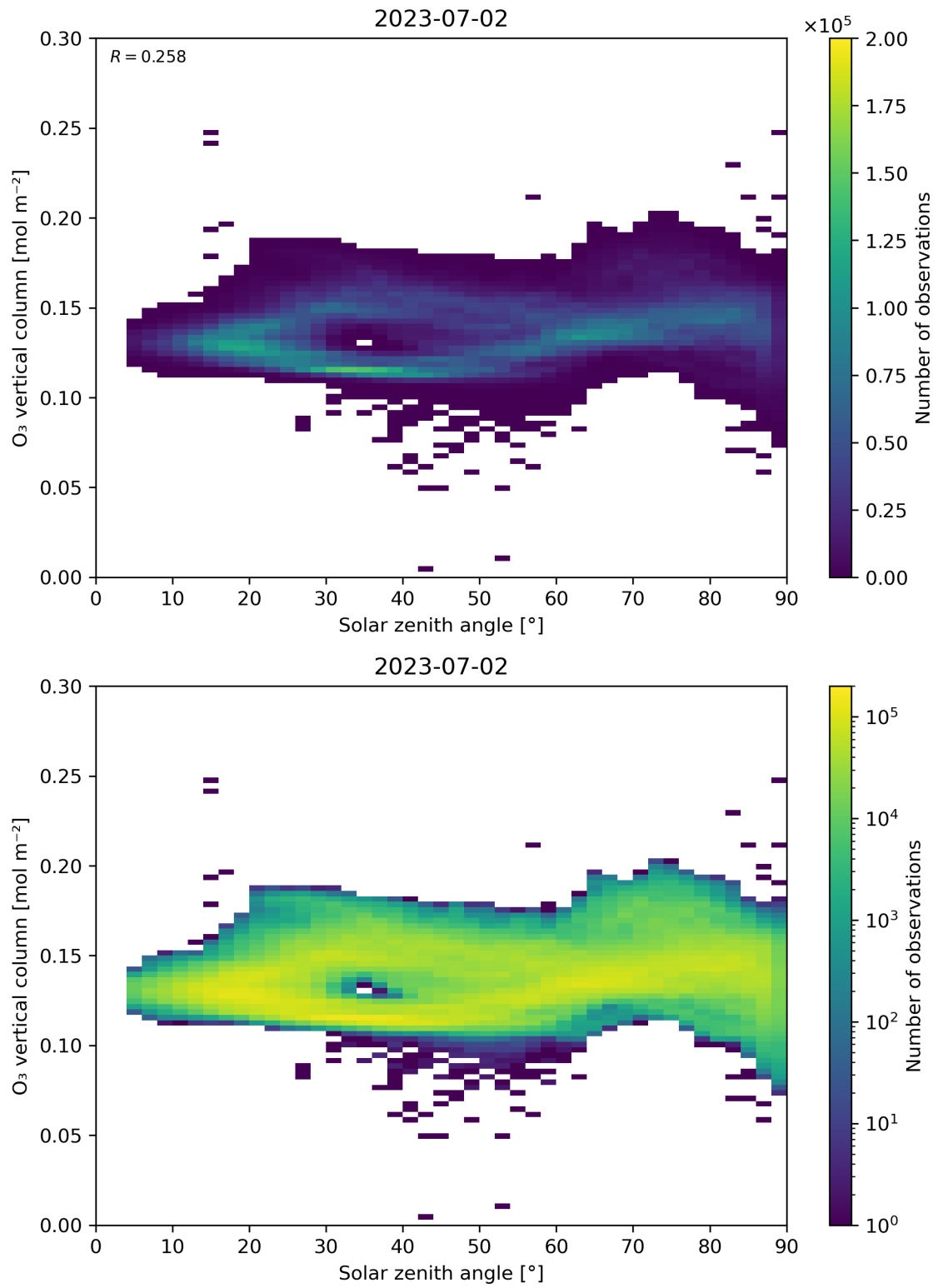
Figure 47: Scatter density plot of “Solar zenith angle” against “O 3 vertical column” for 2023-07-01 to 2023-07-03.
