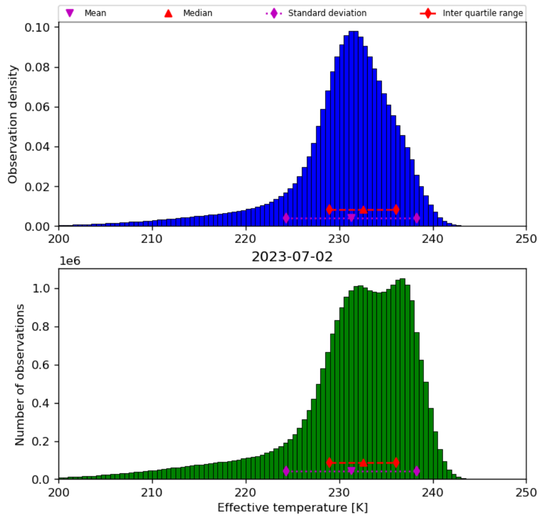
Figure 24: Histogram of “Effective temperature” for 2023-07-01 to 2023-07-03
