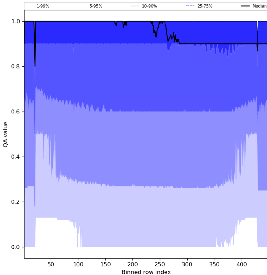
Figure 27: Along track statistics of “QA value” for 2023-07-01 to 2023-07-03
