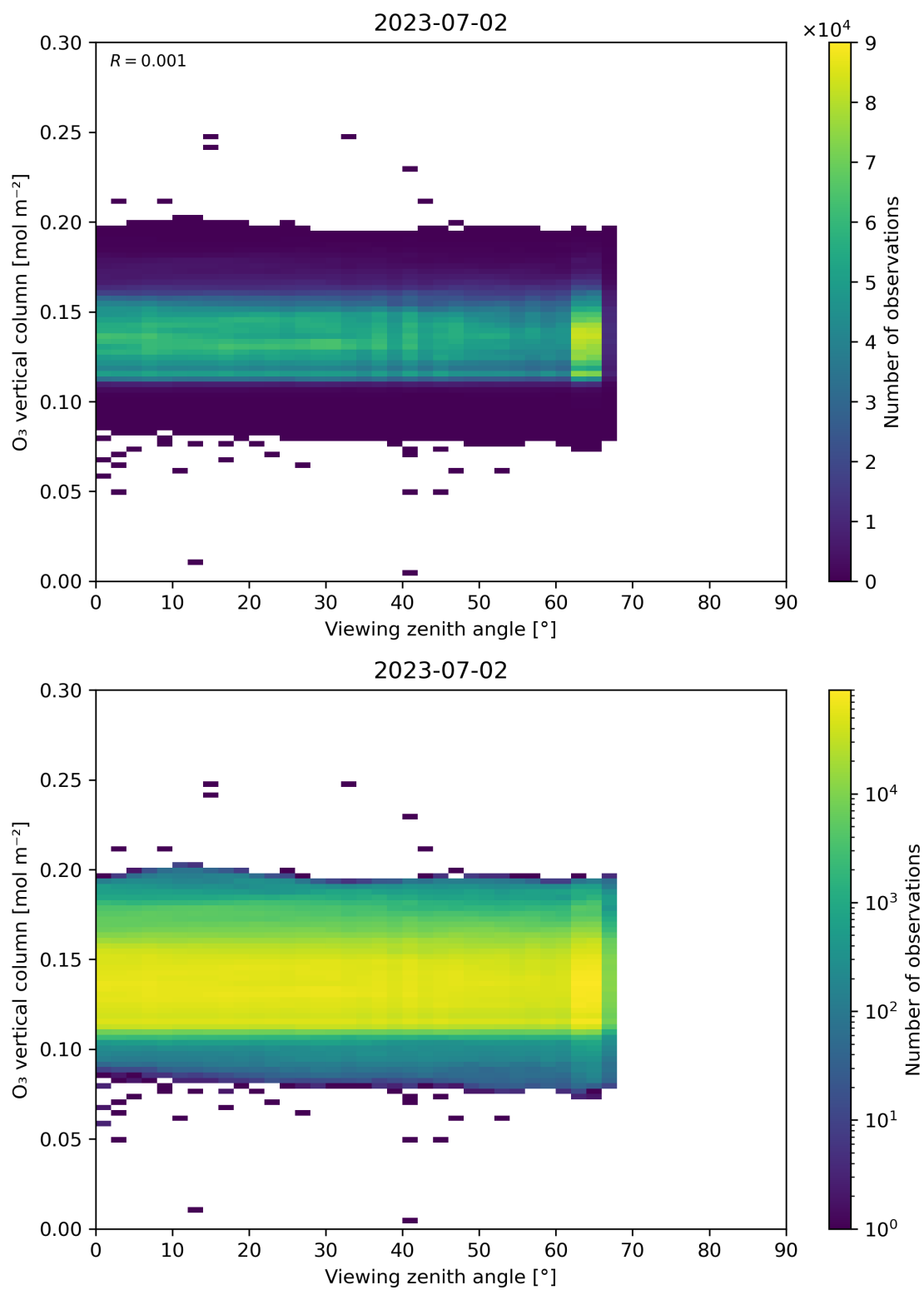
Figure 52: Scatter density plot of “Viewing zenith angle” against “O 3 vertical column” for 2023-07-01 to 2023-07-03.
