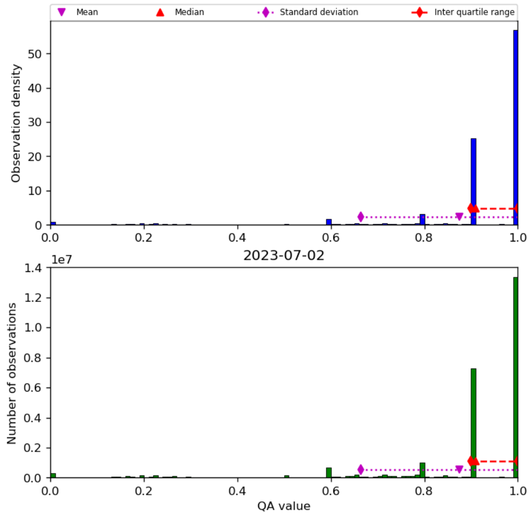
Figure 20: Histogram of “QA value” for 2023-07-01 to 2023-07-03
