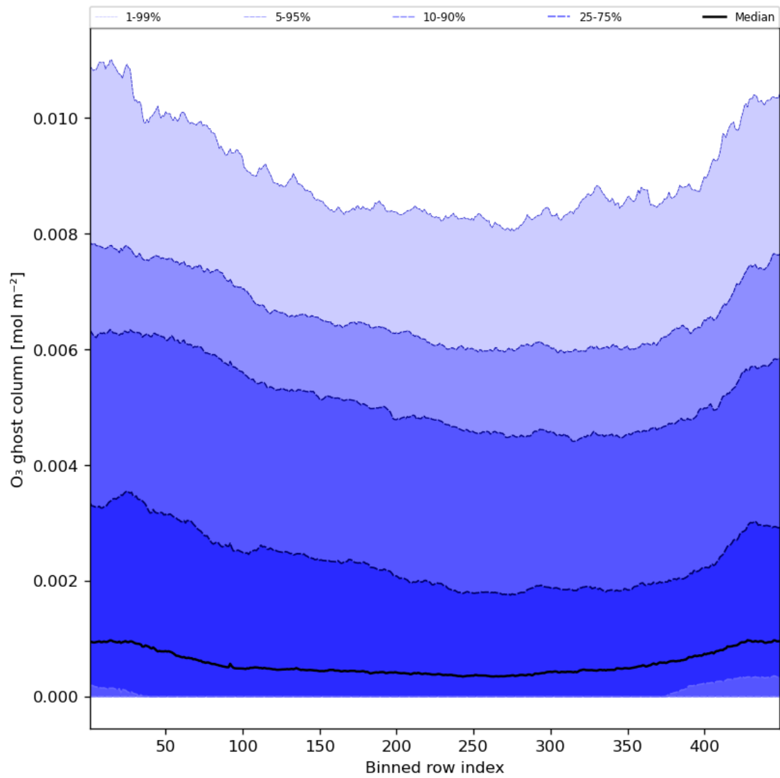
Figure 32: Along track statistics of “O 3 ghost column” for 2023-07-01 to 2023-07-03
