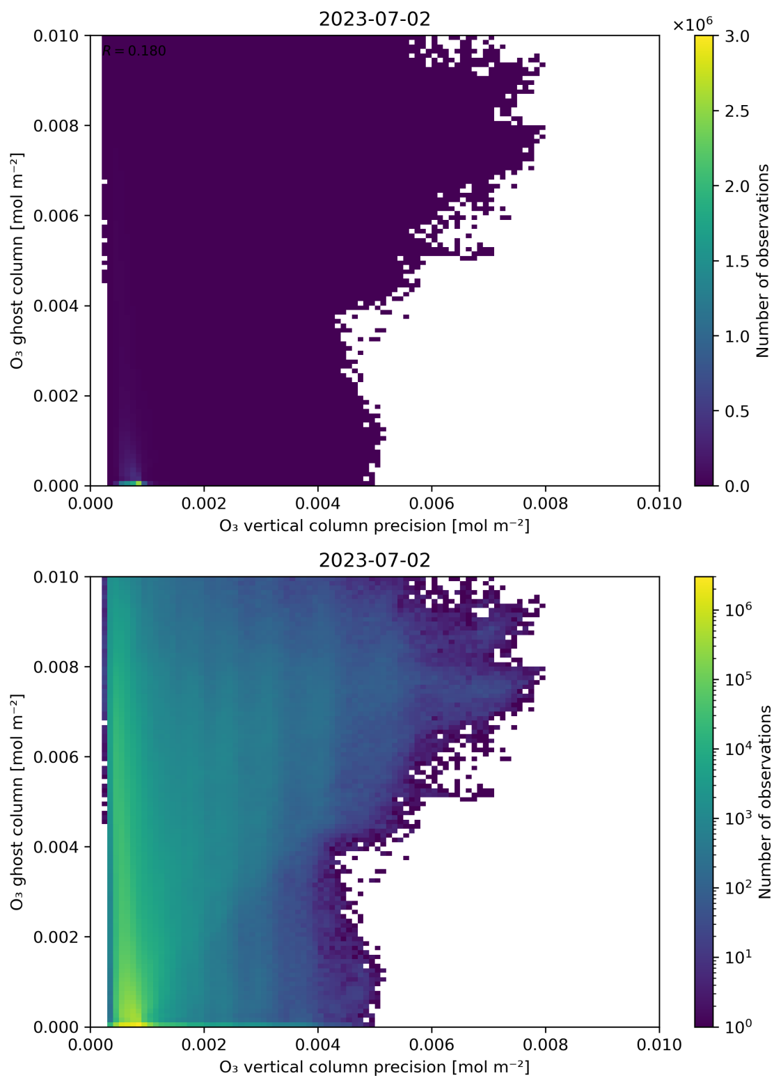
Figure 43: Scatter density plot of “ \text{O}_3 vertical column precision” against “ \text{O}_3 ghost column” for 2023-07-01 to 2023-07-03.
