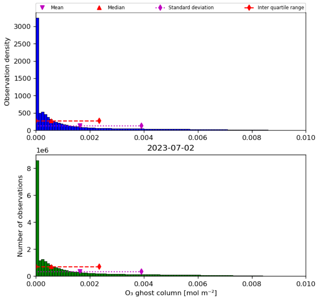
Figure 25: Histogram of “O 3 ghost column” for 2023-07-01 to 2023-07-03
