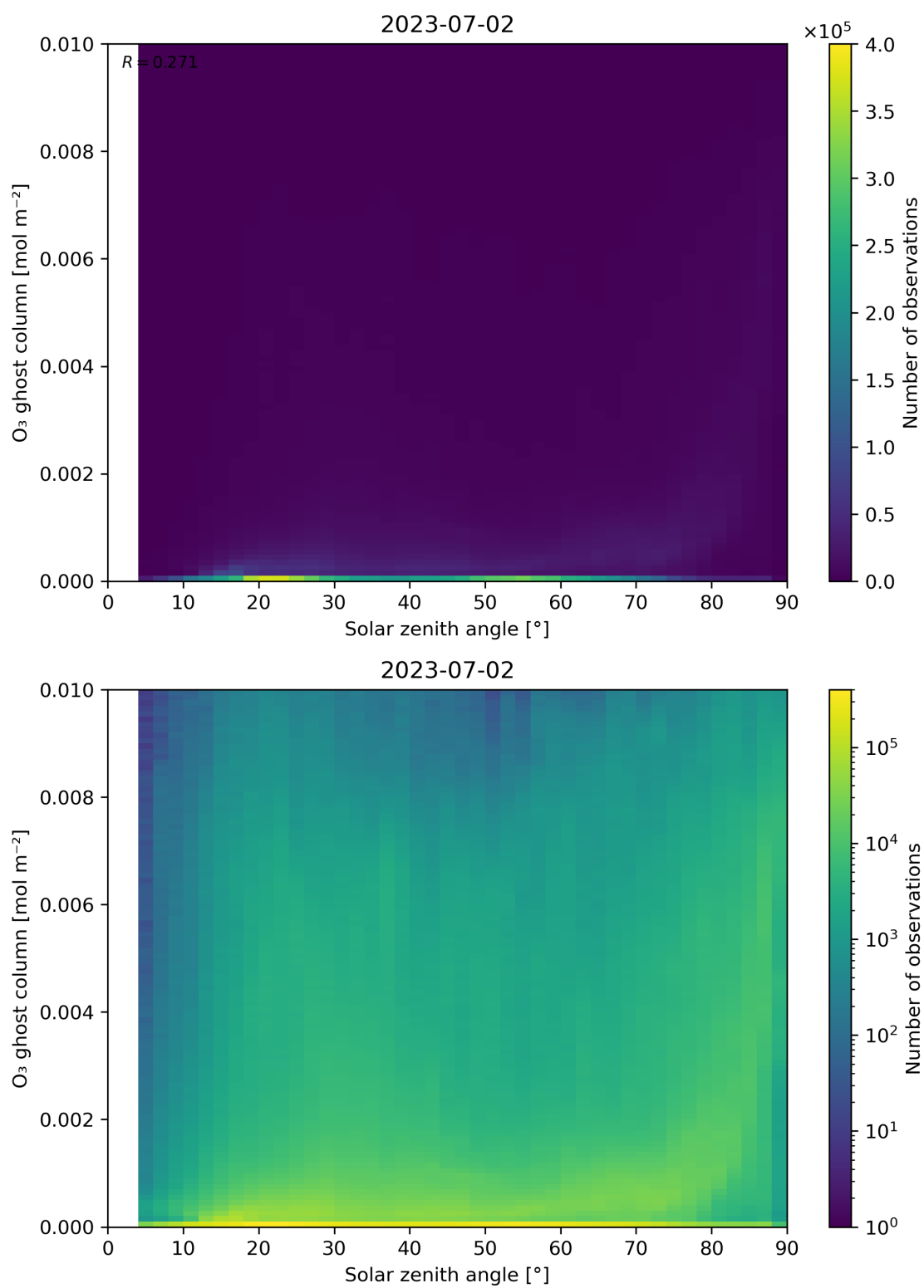
Figure 46: Scatter density plot of “Solar zenith angle” against “O 3 ghost column” for 2023-07-01 to 2023-07-03.
