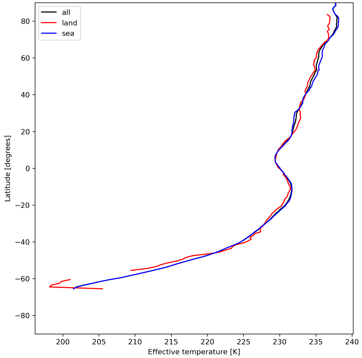
Figure 17: Zonal average of “Effective temperature” for 2023-07-01 to 2023-07-03.
