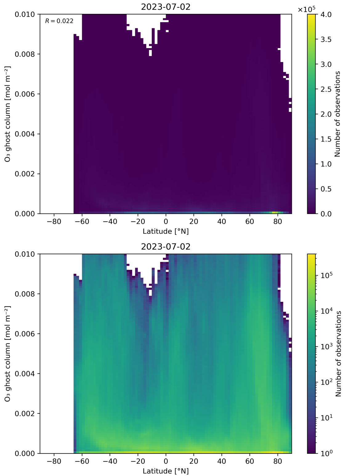
Figure 35: Scatter density plot of “Latitude” against “O 3 ghost column” for 2023-07-01 to 2023-07-03.
