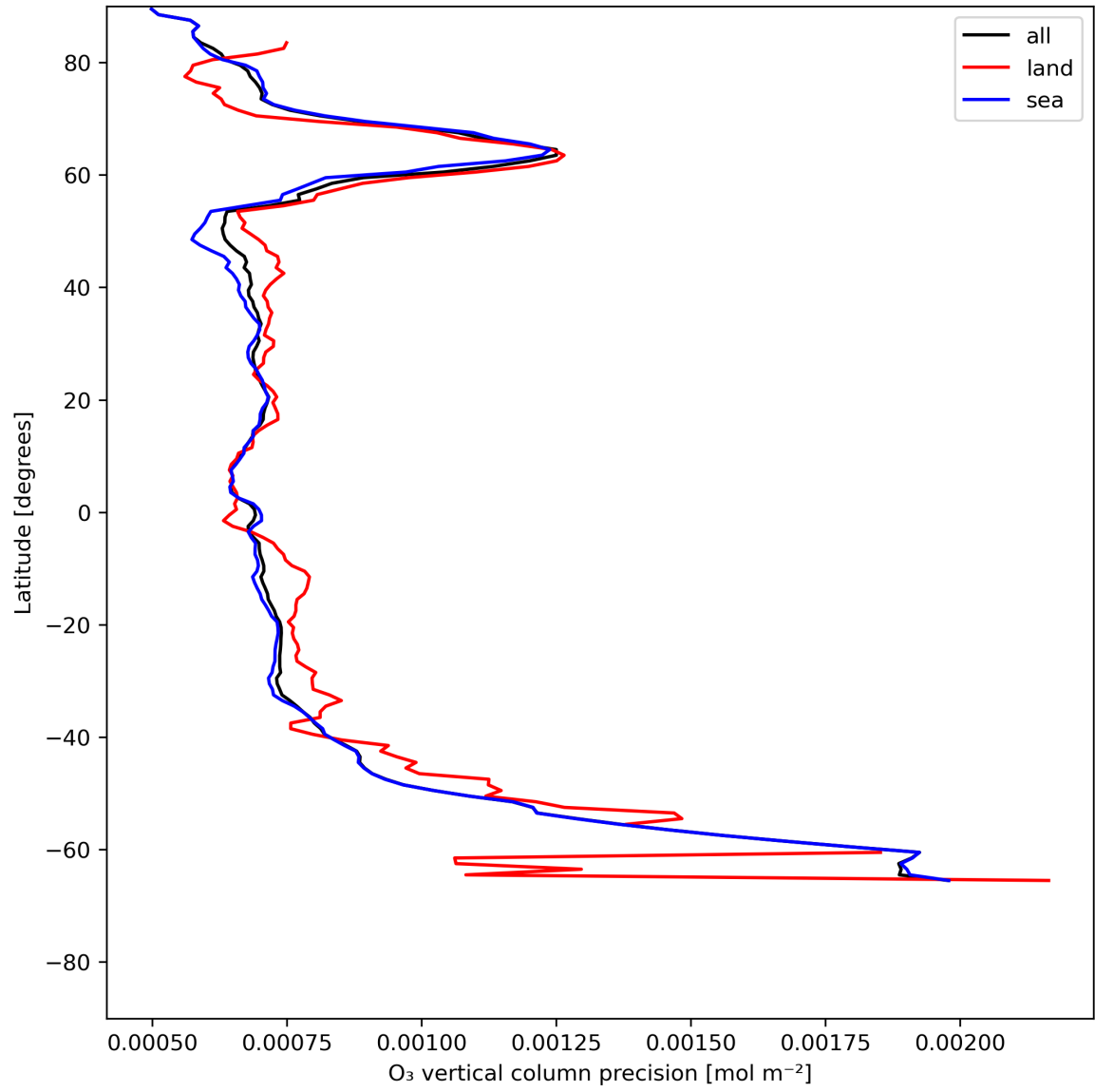
Figure 15: Zonal average of “O 3 vertical column precision” for 2023-07-01 to 2023-07-03.
