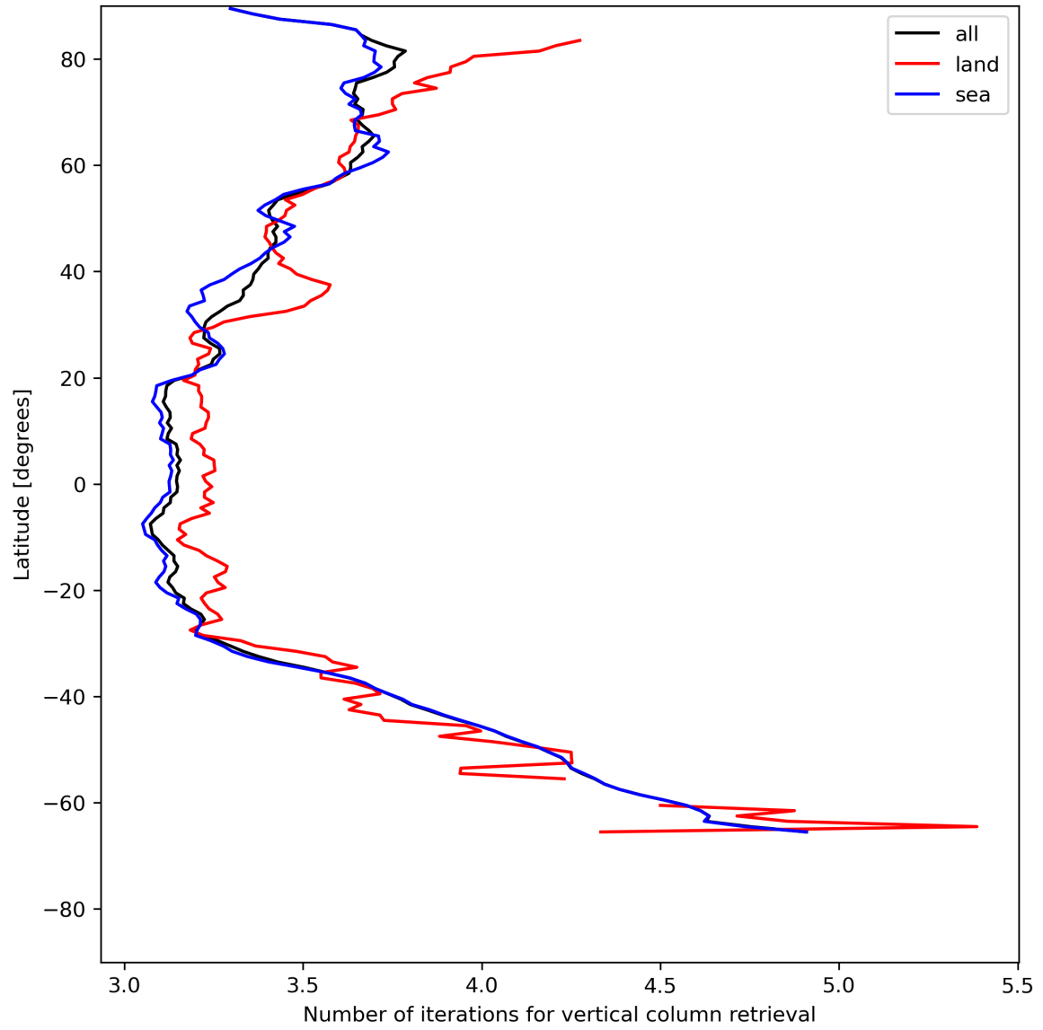
Figure 19: Zonal average of “Number of iterations for vertical column retrieval” for 2023-07-01 to 2023-07-03.
