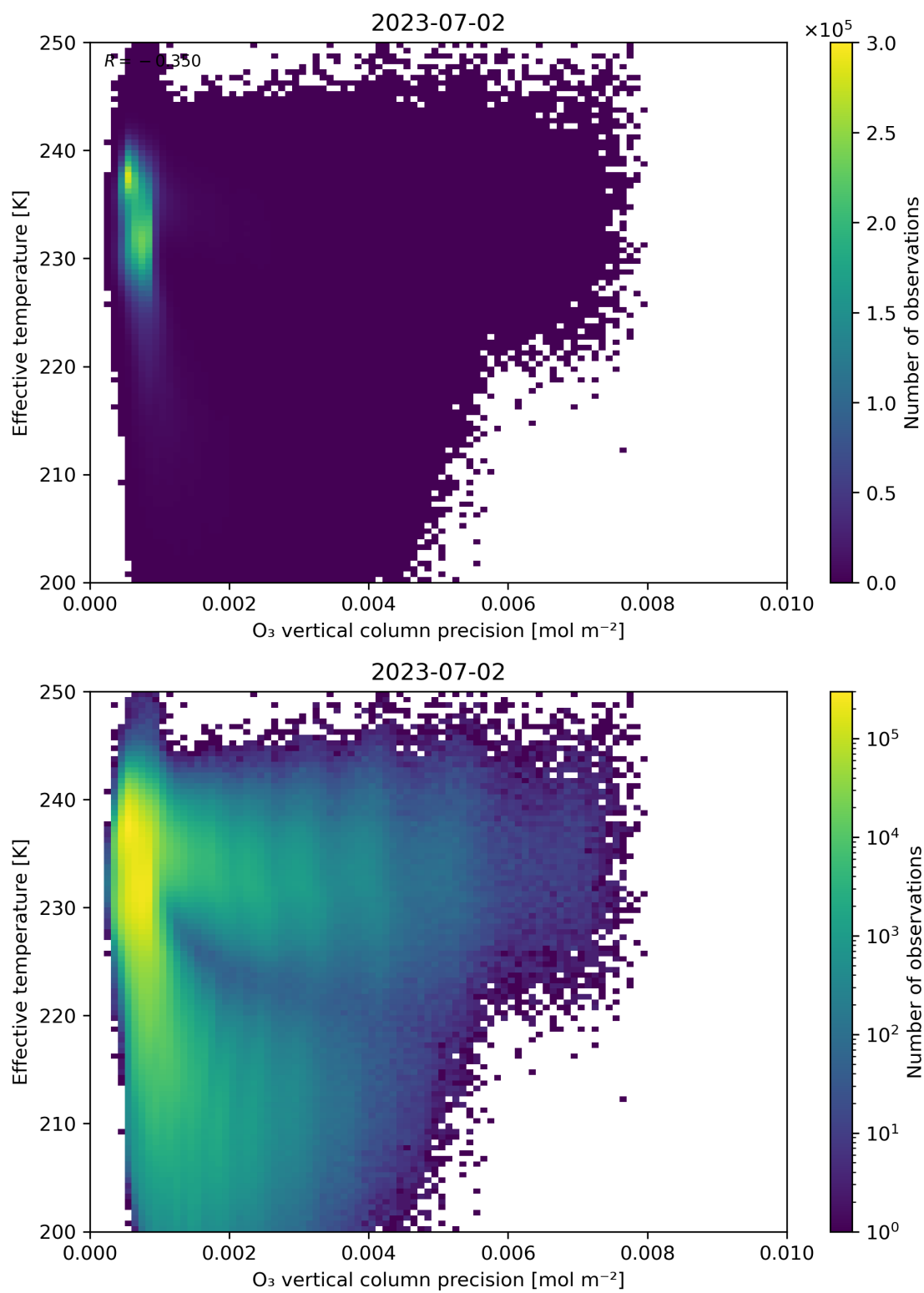
Figure 42: Scatter density plot of “O 3 vertical column precision” against “Effective temperature” for 2023-07-01 to 2023-07-03.
