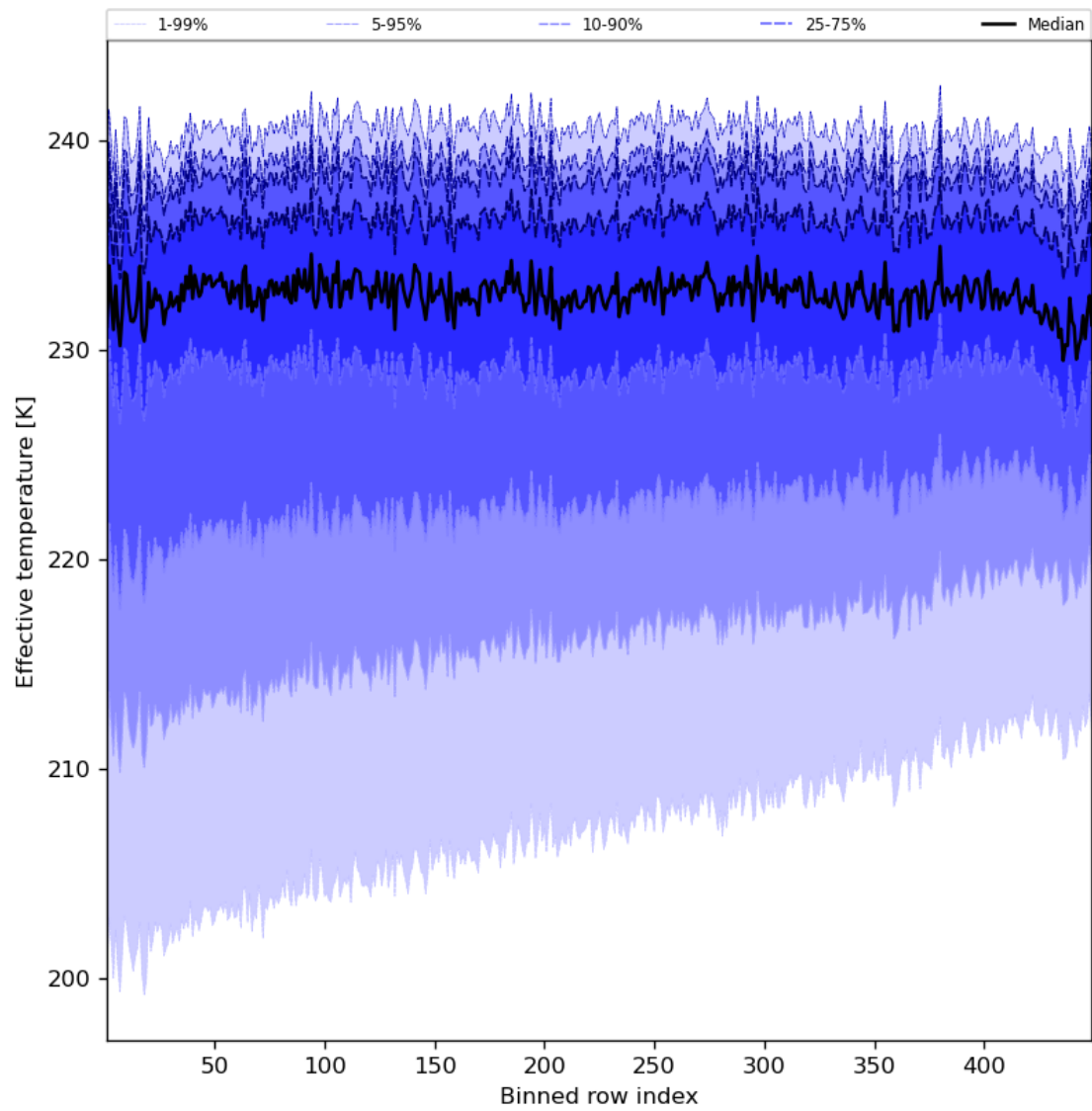
Figure 31: Along track statistics of “Effective temperature” for 2023-07-01 to 2023-07-03
