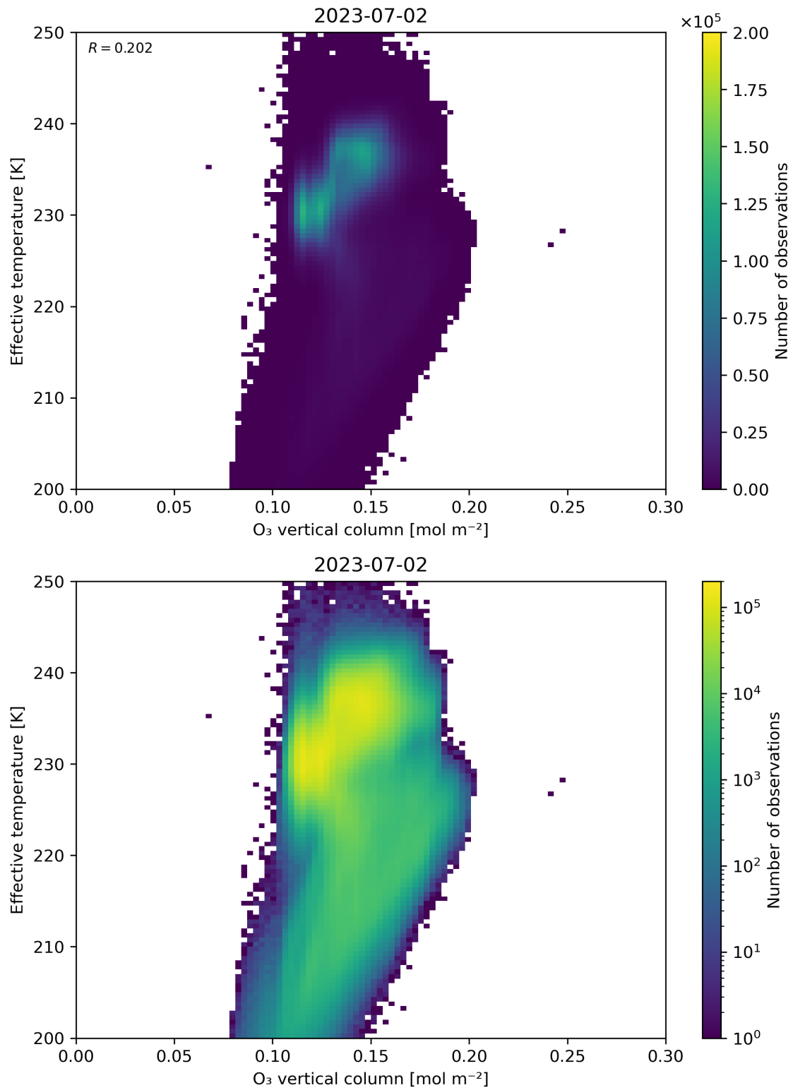
Figure 39: Scatter density plot of “O 3 vertical column” against “Effective temperature” for 2023-07-01 to 2023-07-03.
