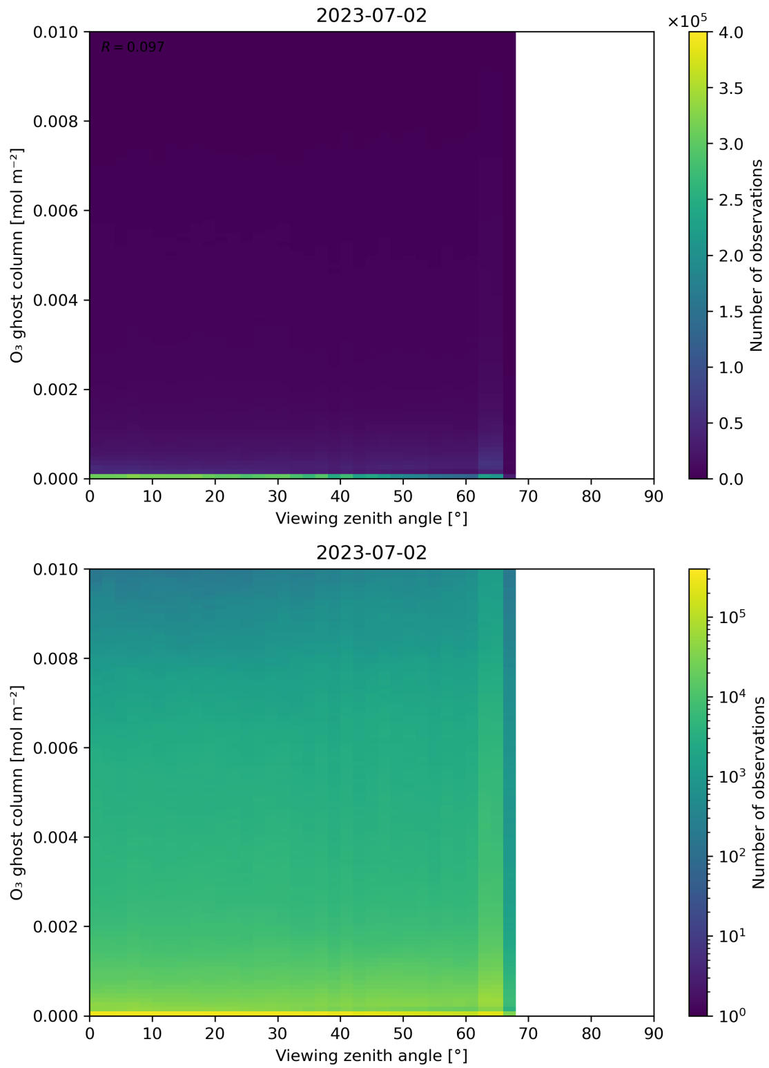
Figure 51: Scatter density plot of “Viewing zenith angle” against “O 3 ghost column” for 2023-07-01 to 2023-07-03.
