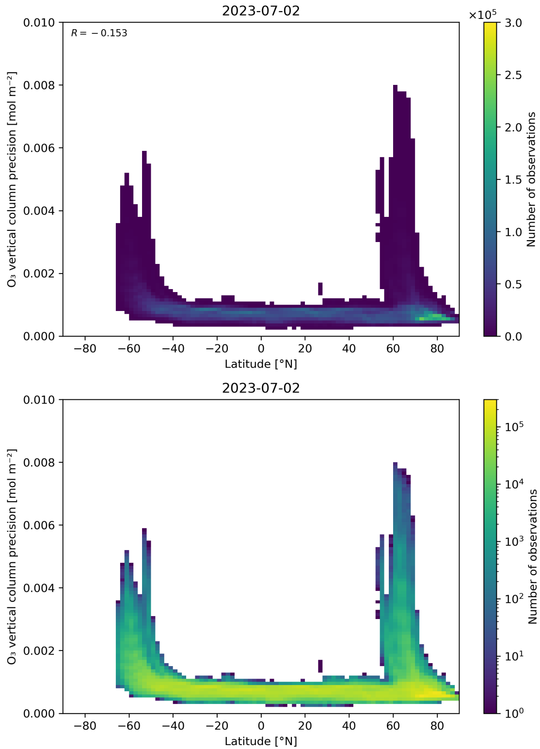
Figure 37: Scatter density plot of “Latitude” against “O 3 vertical column precision” for 2023-07-01 to 2023-07-03.
