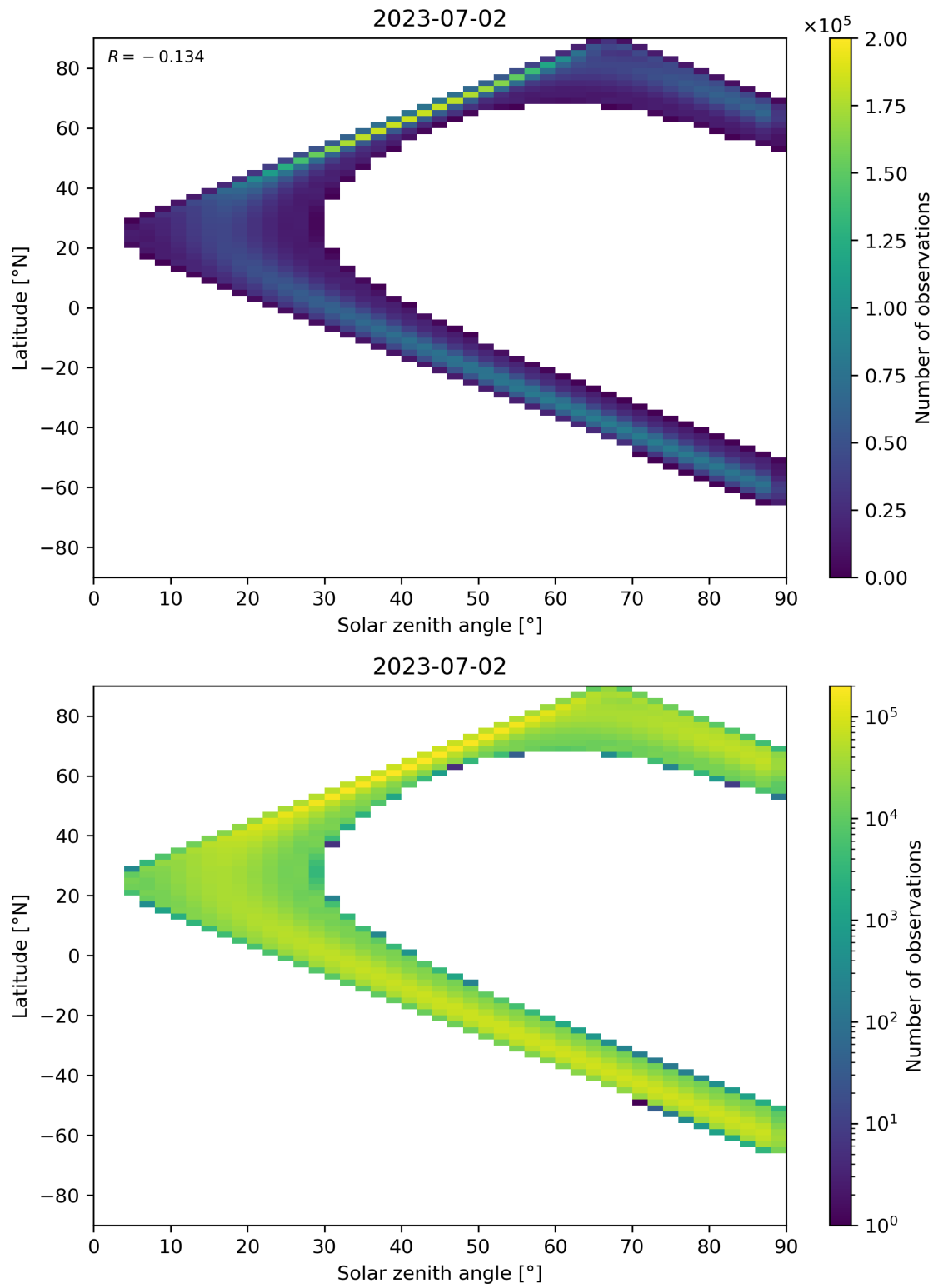
Figure 44: Scatter density plot of “Solar zenith angle” against “Latitude” for 2023-07-01 to 2023-07-03.
