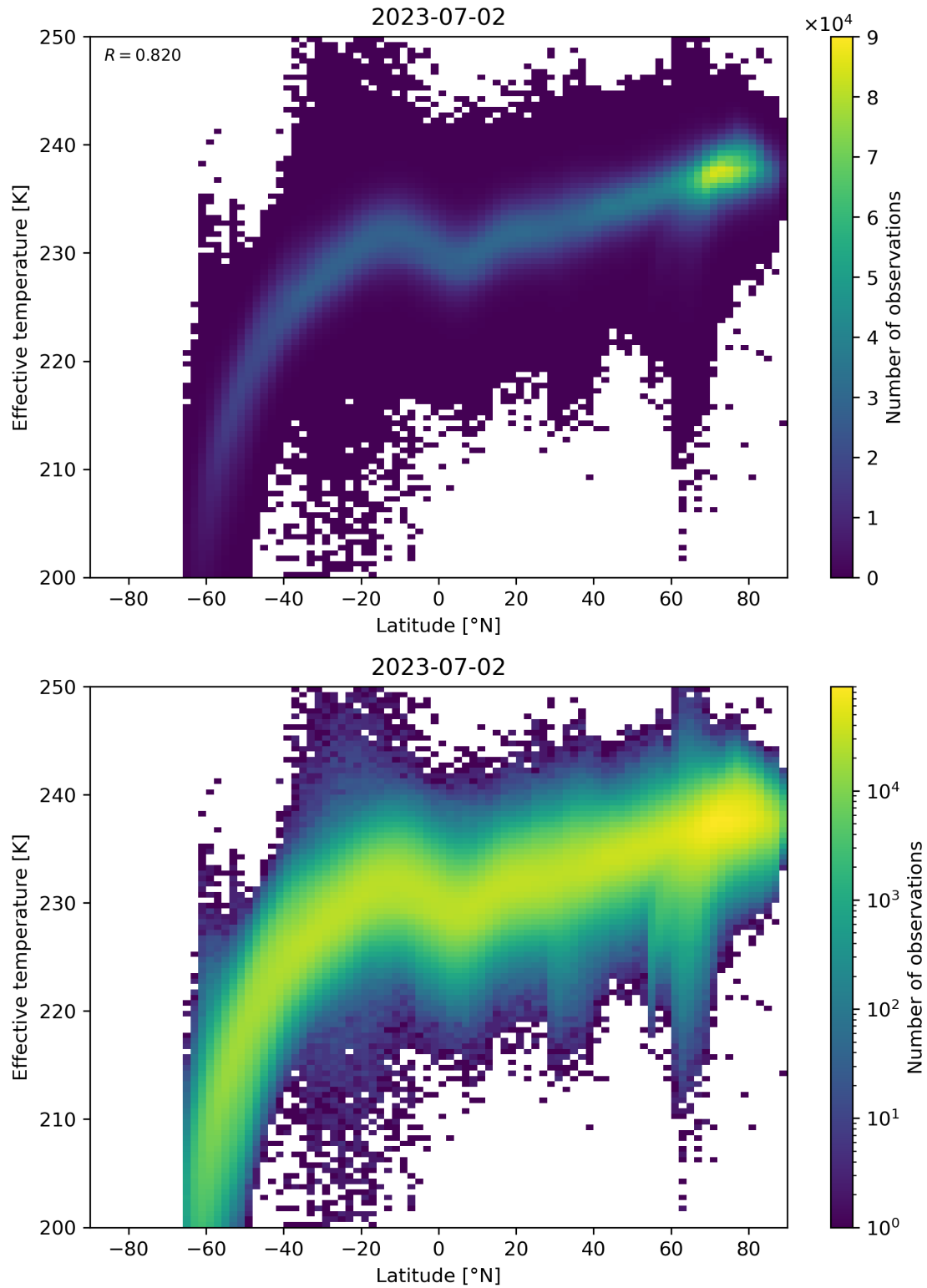
Figure 34: Scatter density plot of “Latitude” against “Effective temperature” for 2023-07-01 to 2023-07-03.
