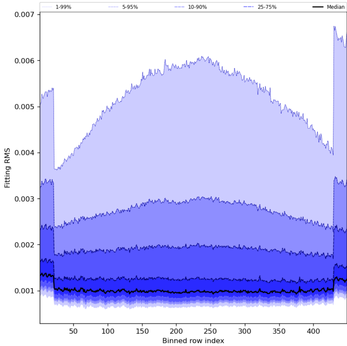
Figure 30: Along track statistics of “Fitting RMS” for 2023-07-01 to 2023-07-03
