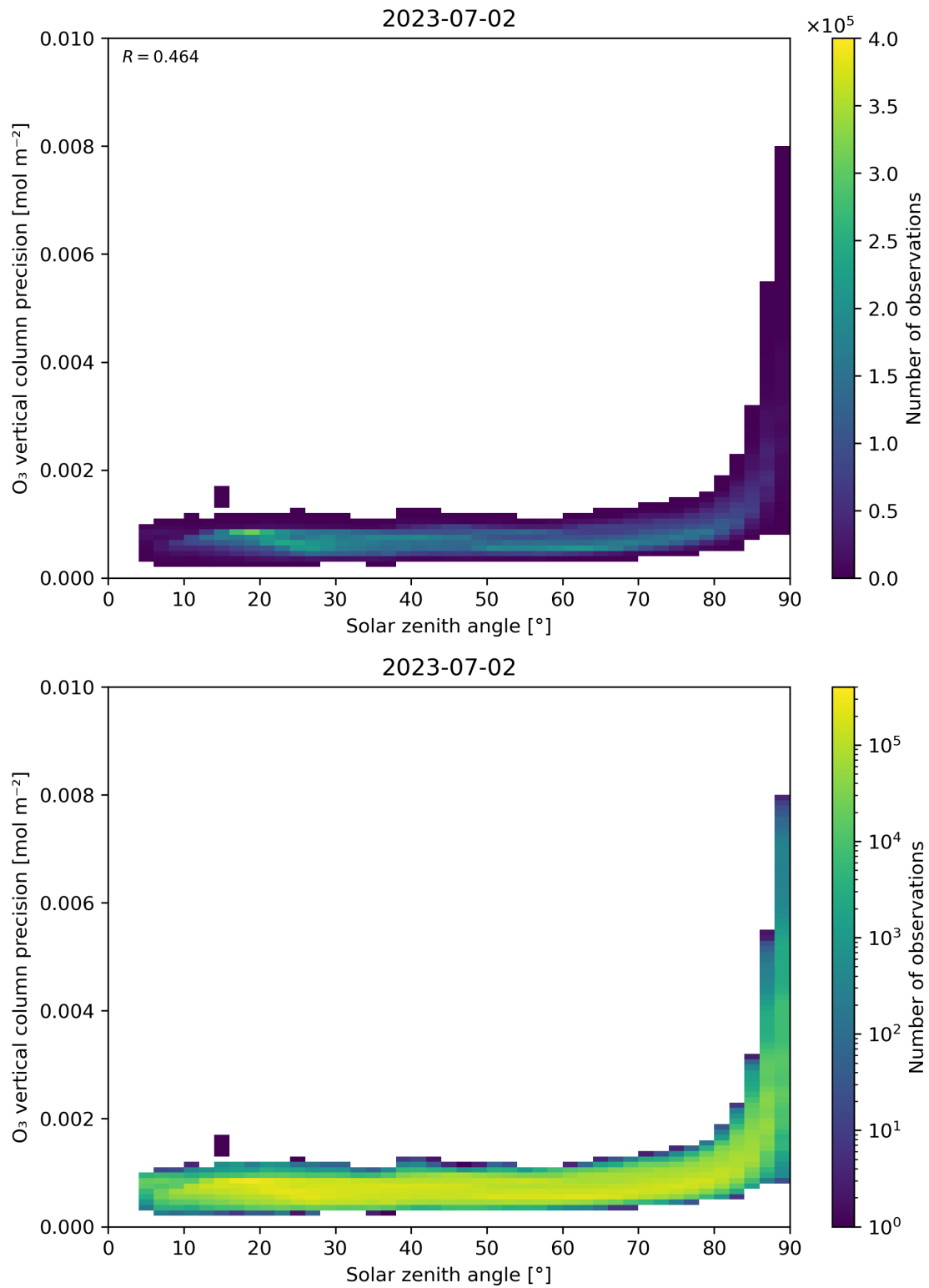
Figure 48: Scatter density plot of “Solar zenith angle” against “O 3 vertical column precision” for 2023-07-01 to 2023-07-03.
