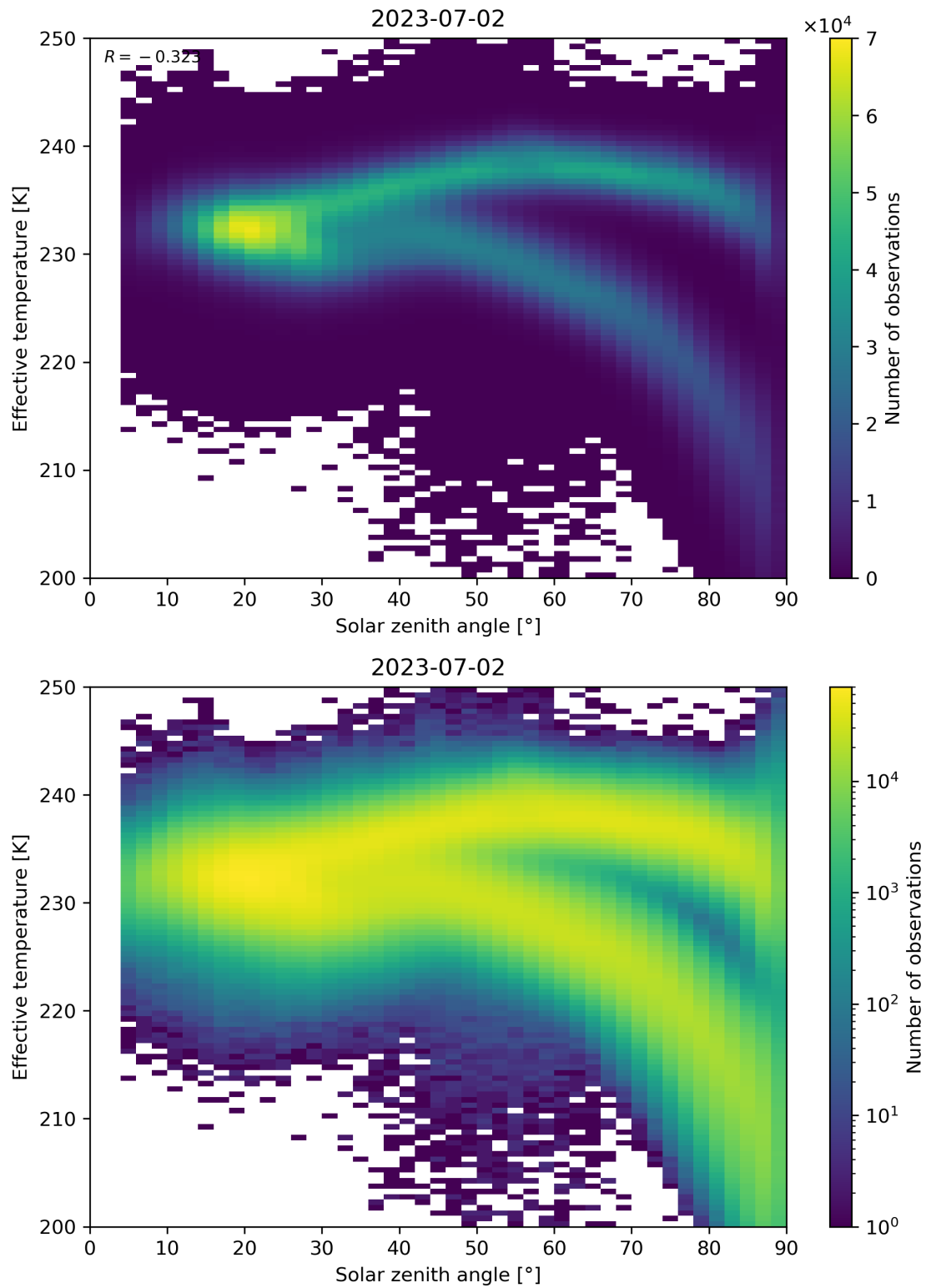
Figure 45: Scatter density plot of “Solar zenith angle” against “Effective temperature” for 2023-07-01 to 2023-07-03.
