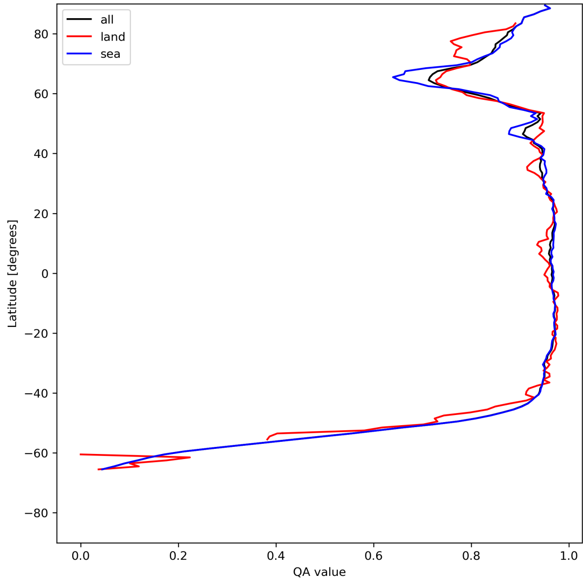
Figure 13: Zonal average of “QA value” for 2023-07-01 to 2023-07-03.
