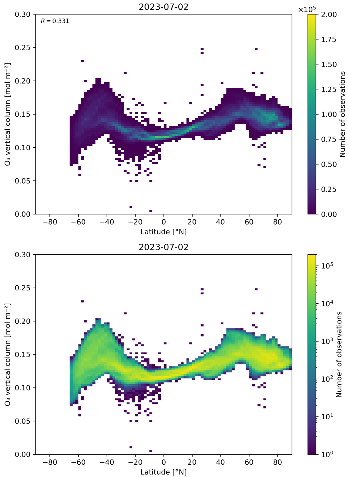
Figure 36: Scatter density plot of “Latitude” against “O 3 vertical column” for 2023-07-01 to 2023-07-03.
