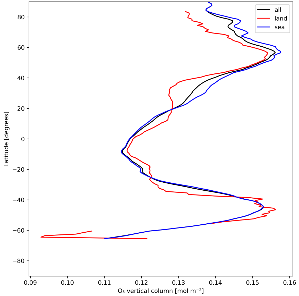
Figure 14: Zonal average of “O 3 vertical column” for 2023-07-01 to 2023-07-03.
