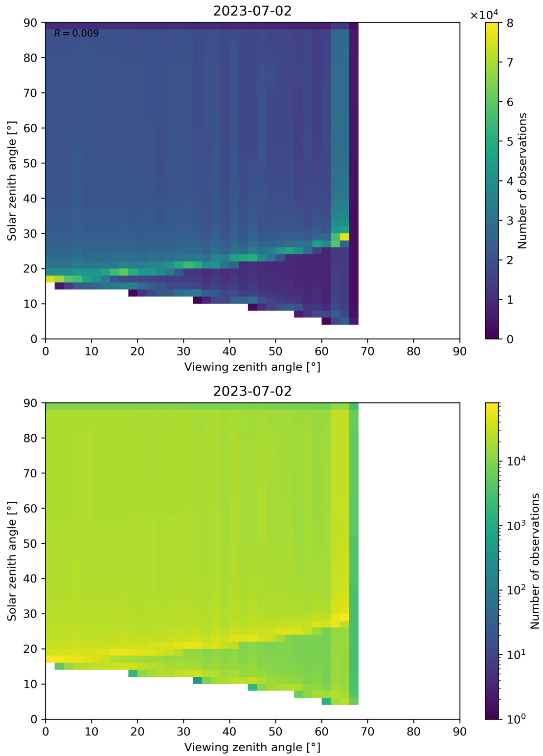
Figure 54: Scatter density plot of “Viewing zenith angle” against “Solar zenith angle” for 2023-07-01 to 2023-07-03.
