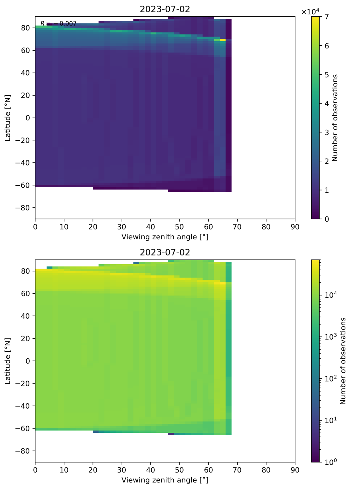
Figure 49: Scatter density plot of “Viewing zenith angle” against “Latitude” for 2023-07-01 to 2023-07-03.
