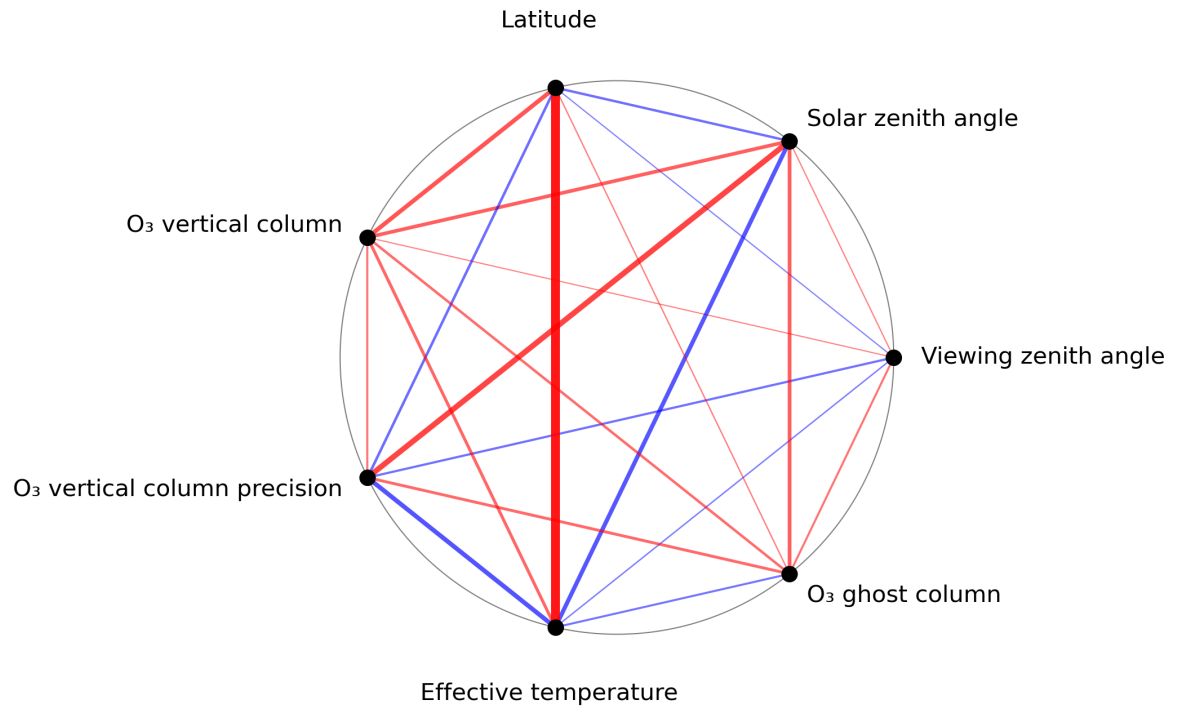
Figure 1: Map of correlation graph for 2023-07-01 to 2023-07-03.
