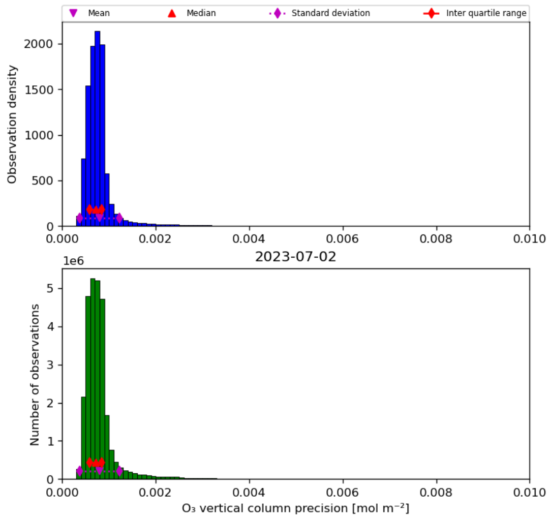
Figure 22: Histogram of “O 3 vertical column precision” for 2023-07-01 to 2023-07-03
