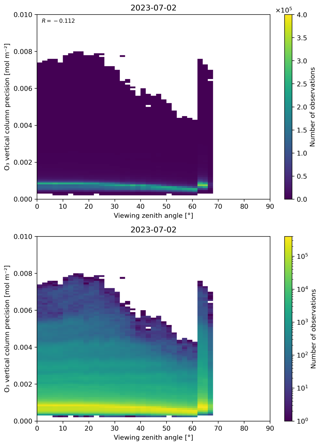
Figure 53: Scatter density plot of “Viewing zenith angle” against “O 3 vertical column precision” for 2023-07-01 to 2023-07-03.
