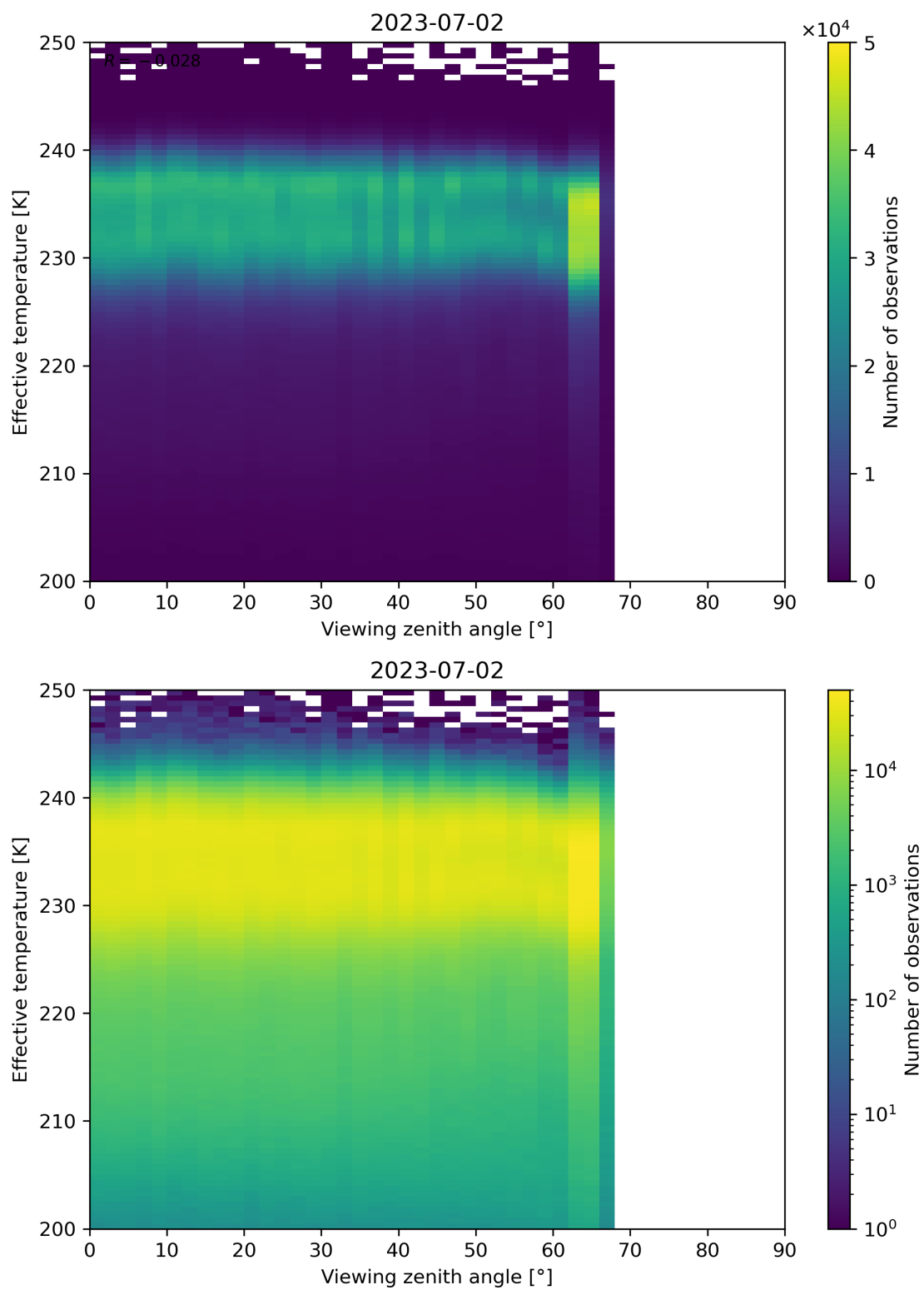
Figure 50: Scatter density plot of “Viewing zenith angle” against “Effective temperature” for 2023-07-01 to 2023-07-03.
