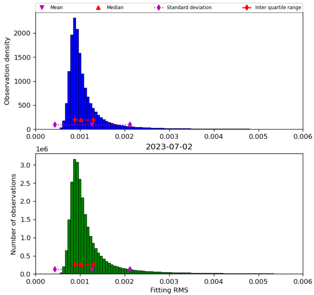
Figure 23: Histogram of “Fitting RMS” for 2023-07-01 to 2023-07-03
