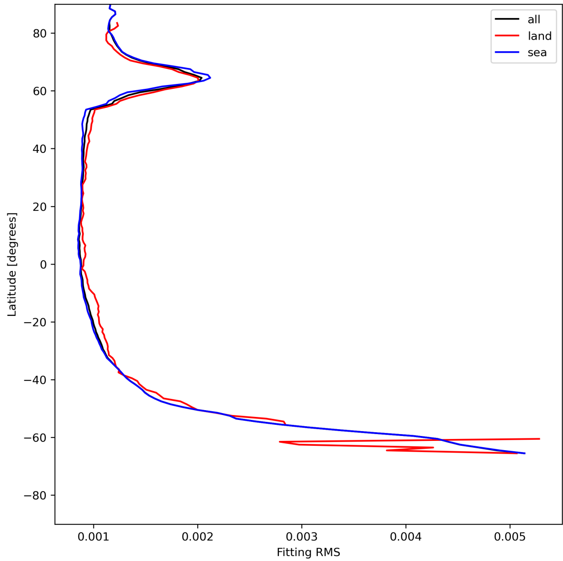
Figure 16: Zonal average of “Fitting RMS” for 2023-07-01 to 2023-07-03.
