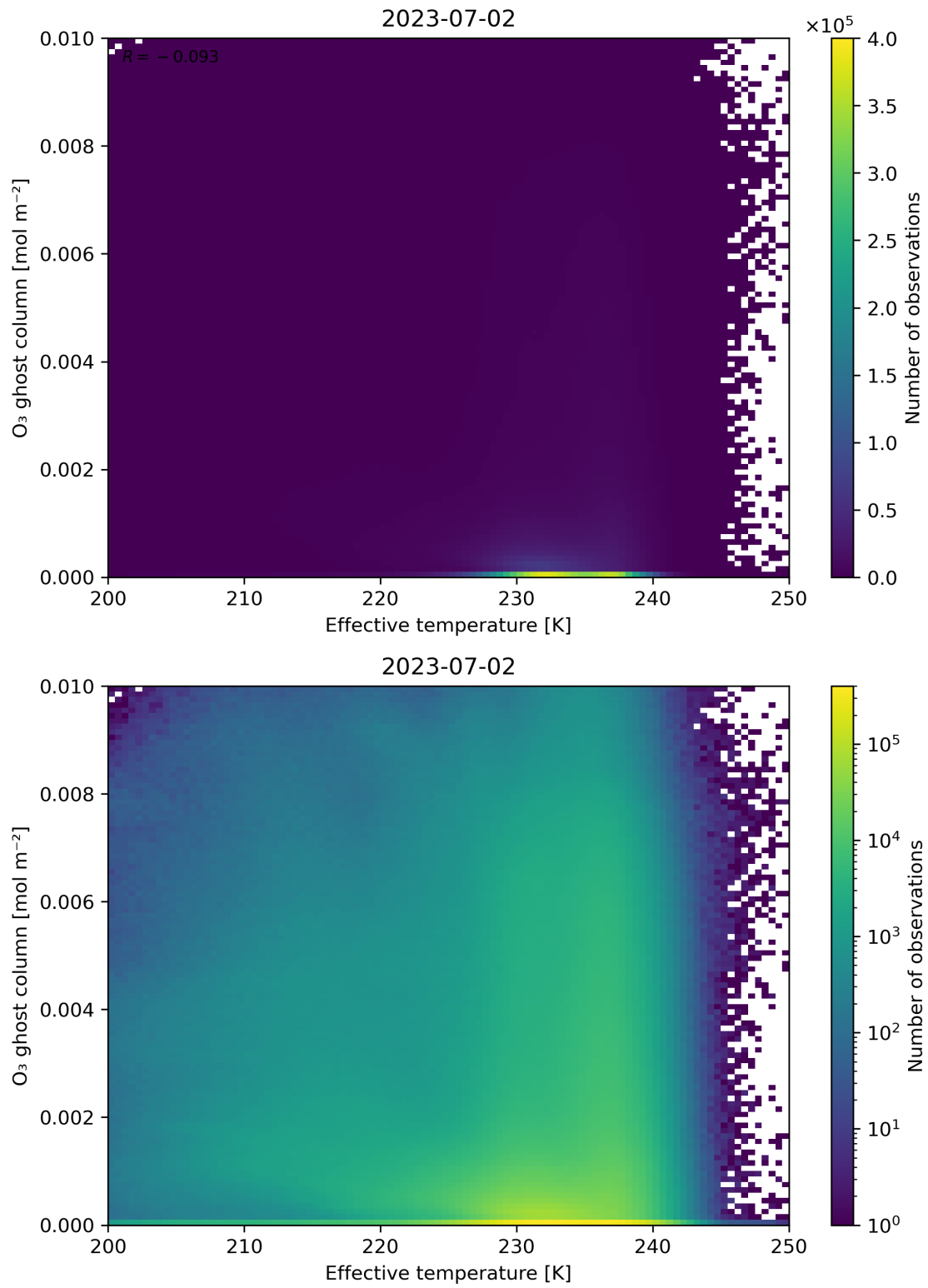
Figure 38: Scatter density plot of “Effective temperature” against “O 3 ghost column” for 2023-07-01 to 2023-07-03.
