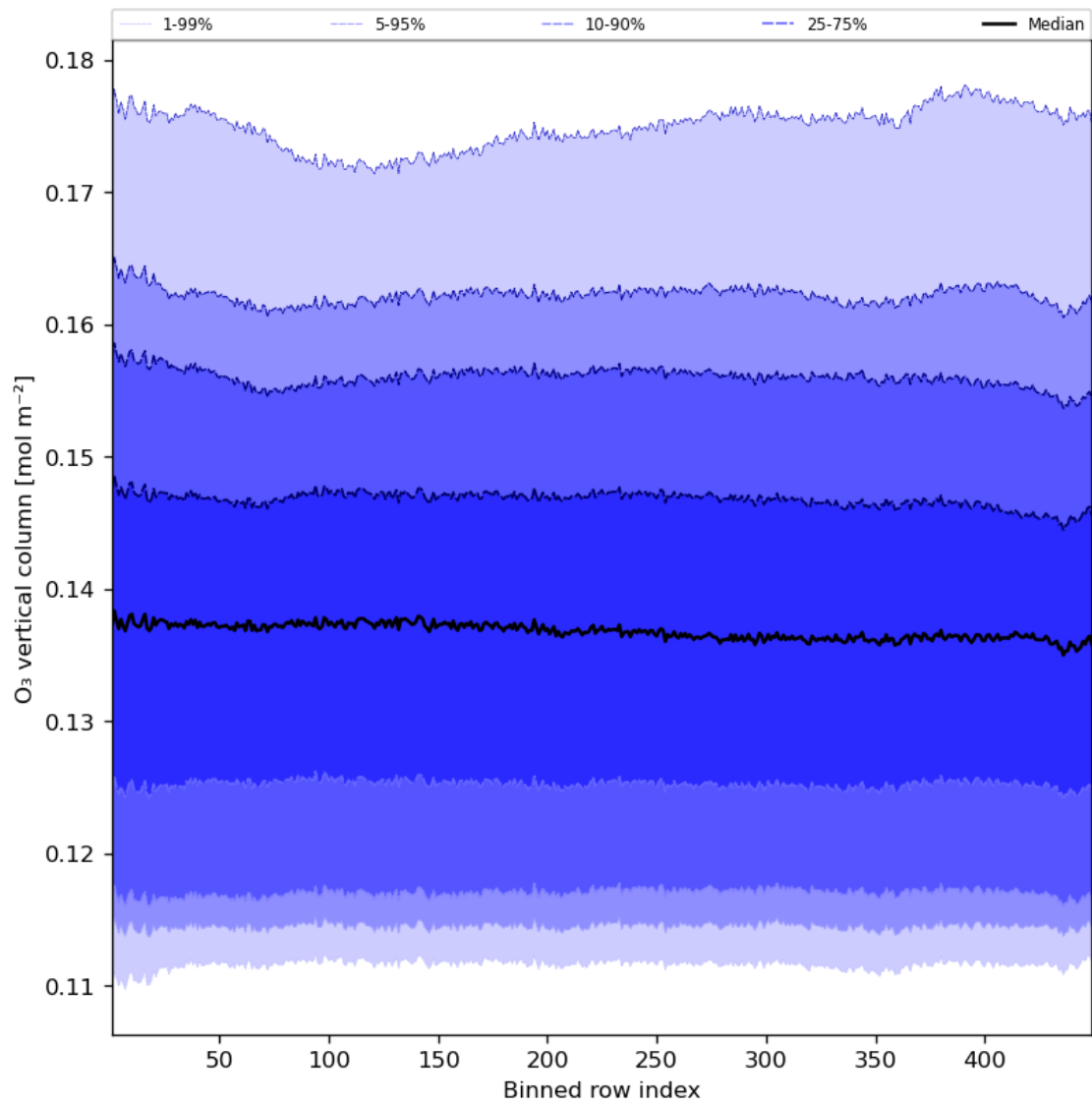
Figure 28: Along track statistics of “O 3 vertical column” for 2023-07-03 to 2023-07-04
