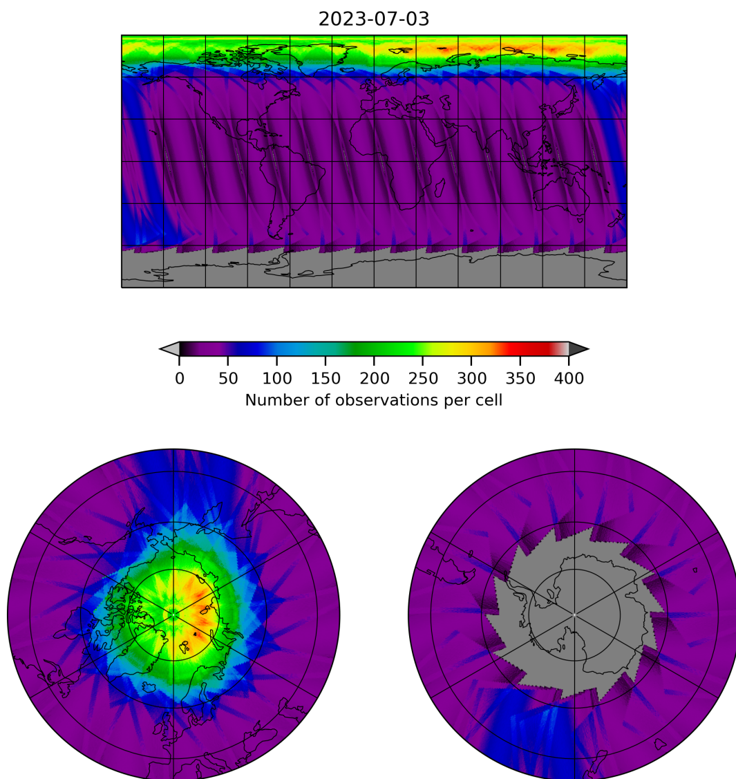
Figure 12: Map of the number of observations for 2023-07-03 to 2023-07-04
