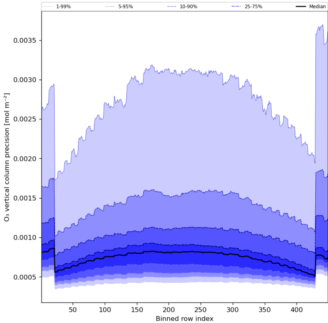
Figure 29: Along track statistics of “O 3 vertical column precision” for 2023-07-03 to 2023-07-04
