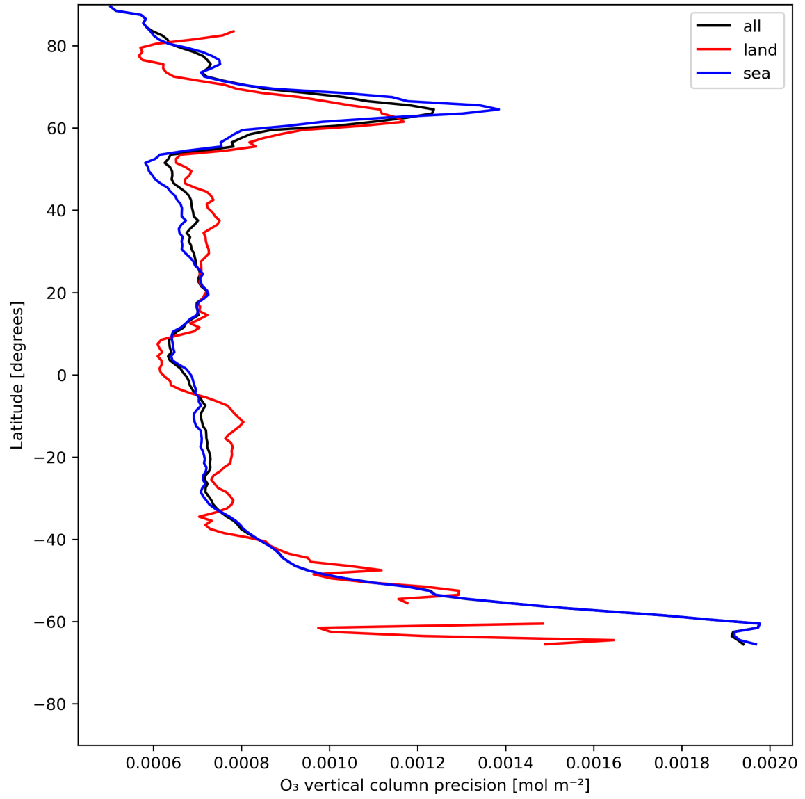
Figure 15: Zonal average of "O 3 vertical column precision" for 2023-07-03 to 2023-07-04.
