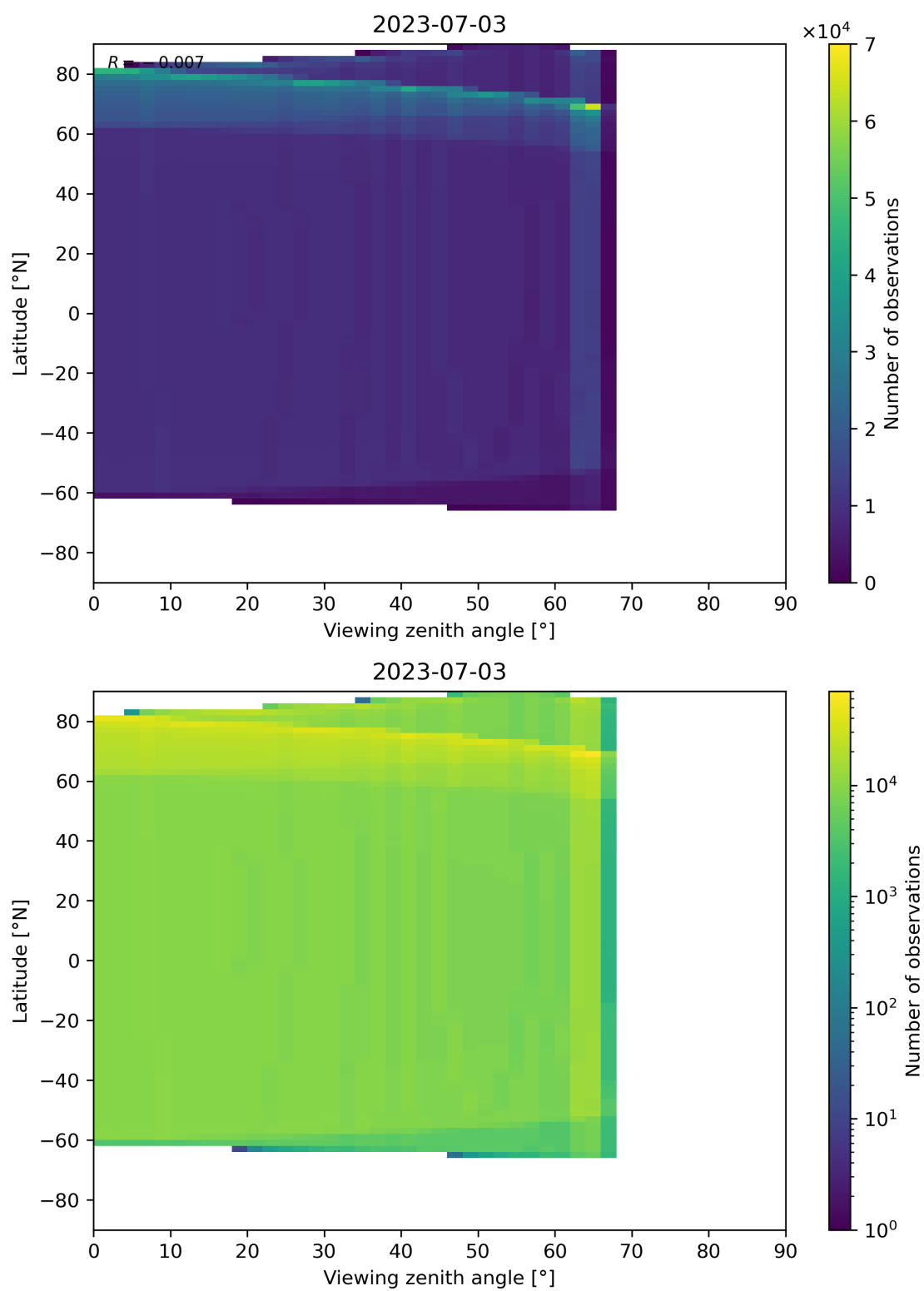
Figure 49: Scatter density plot of “Viewing zenith angle” against “Latitude” for 2023-07-03 to 2023-07-04.
