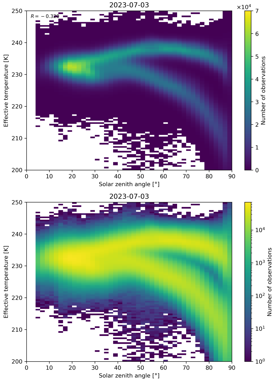
Figure 45: Scatter density plot of “Solar zenith angle” against “Effective temperature” for 2023-07-03 to 2023-07-04.
