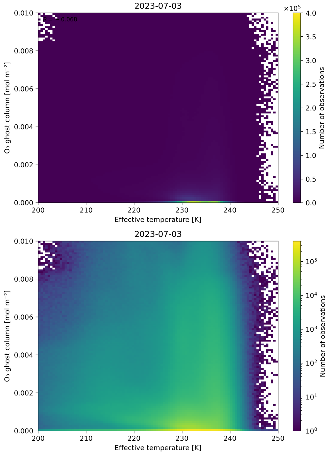
Figure 38: Scatter density plot of “Effective temperature” against “O 3 ghost column” for 2023-07-03 to 2023-07-04.
