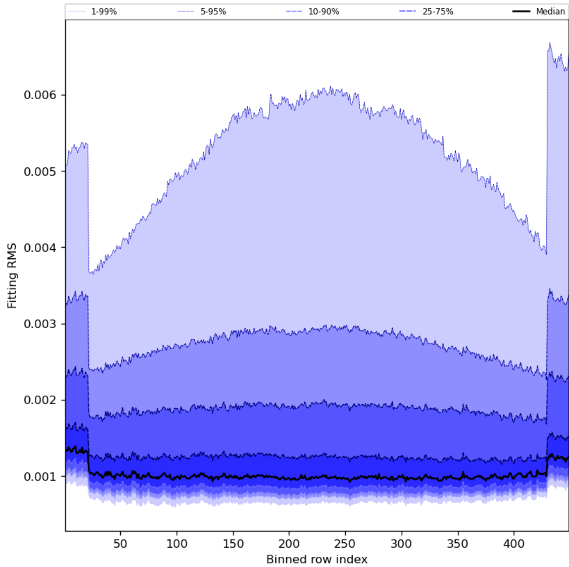
Figure 30: Along track statistics of “Fitting RMS” for 2023-07-03 to 2023-07-04
