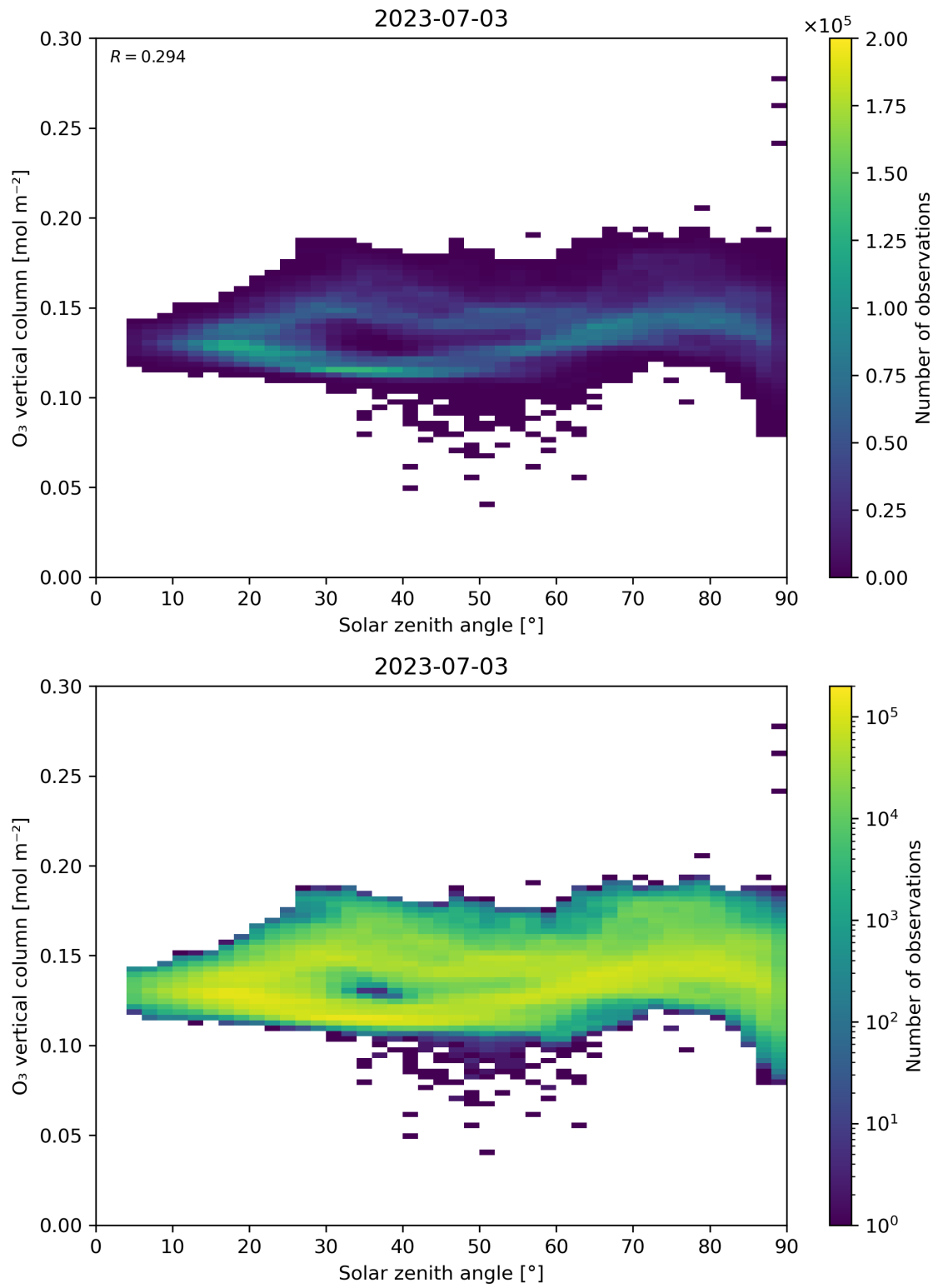
Figure 47: Scatter density plot of “Solar zenith angle” against “O 3 vertical column” for 2023-07-03 to 2023-07-04.
