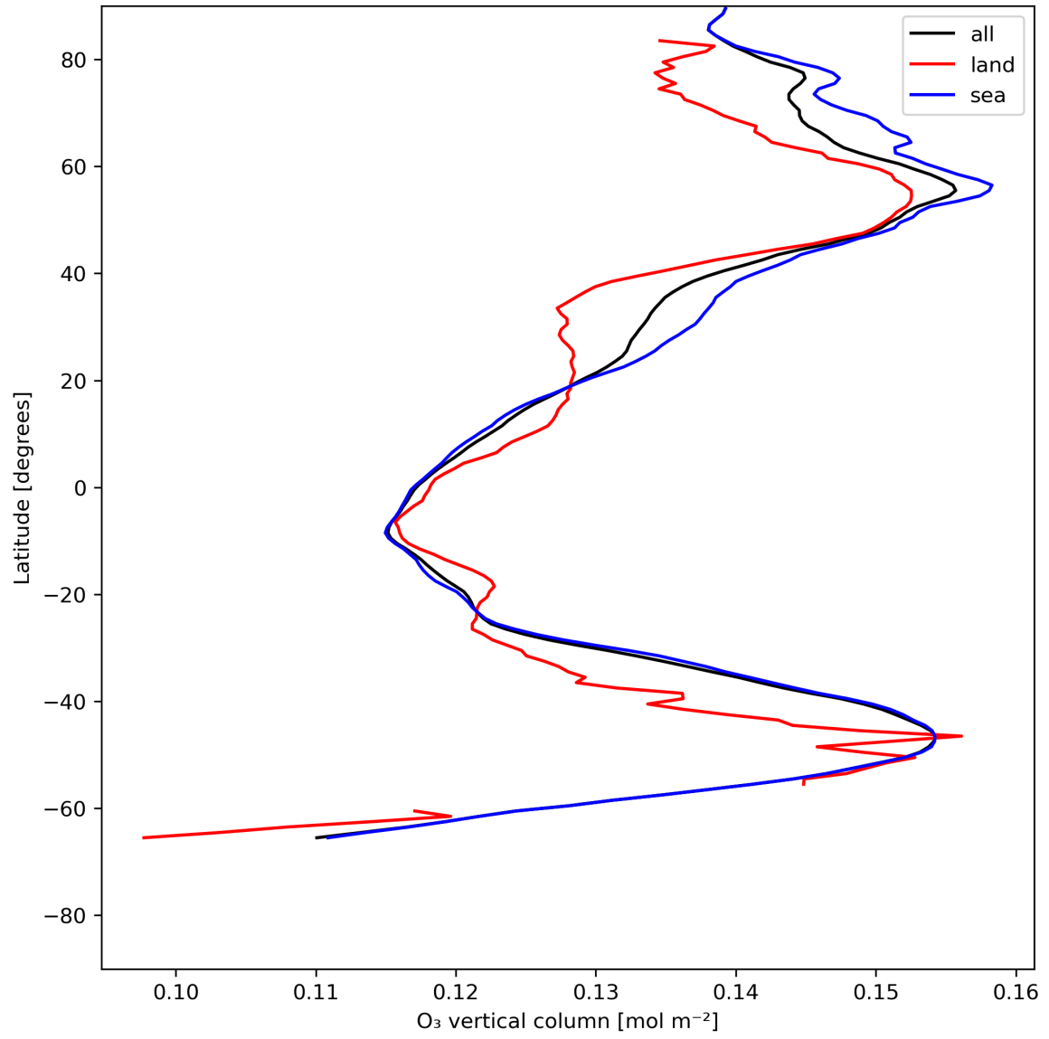
Figure 14: Zonal average of “O 3 vertical column” for 2023-07-03 to 2023-07-04.
