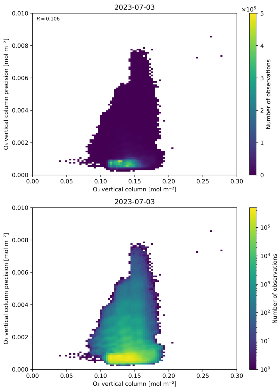
Figure 41: Scatter density plot of “O 3 vertical column” against “O 3 vertical column precision” for 2023-07-03 to 2023-07-04.
