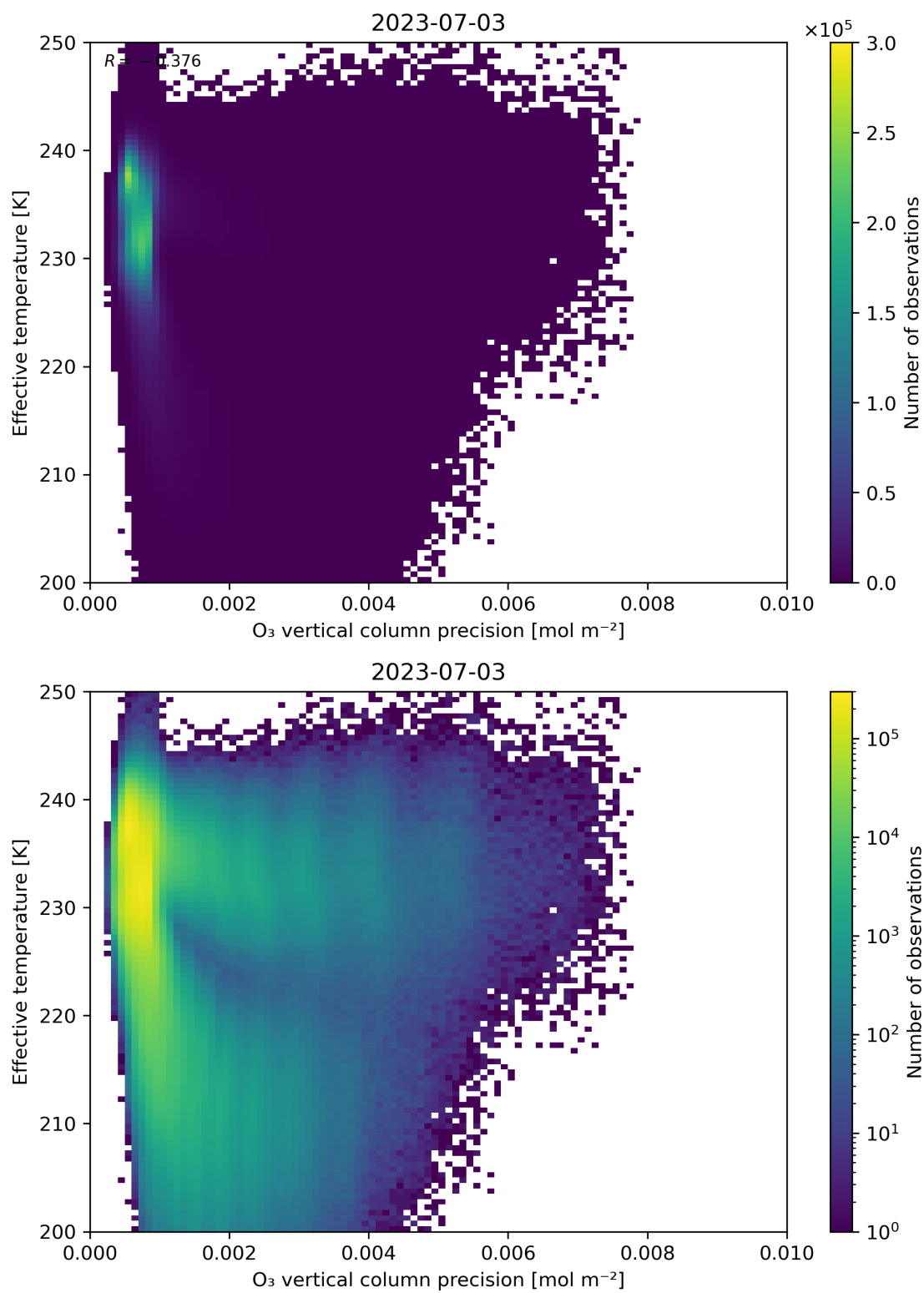
Figure 42: Scatter density plot of “O 3 vertical column precision” against “Effective temperature” for 2023-07-03 to 2023-07-04.
