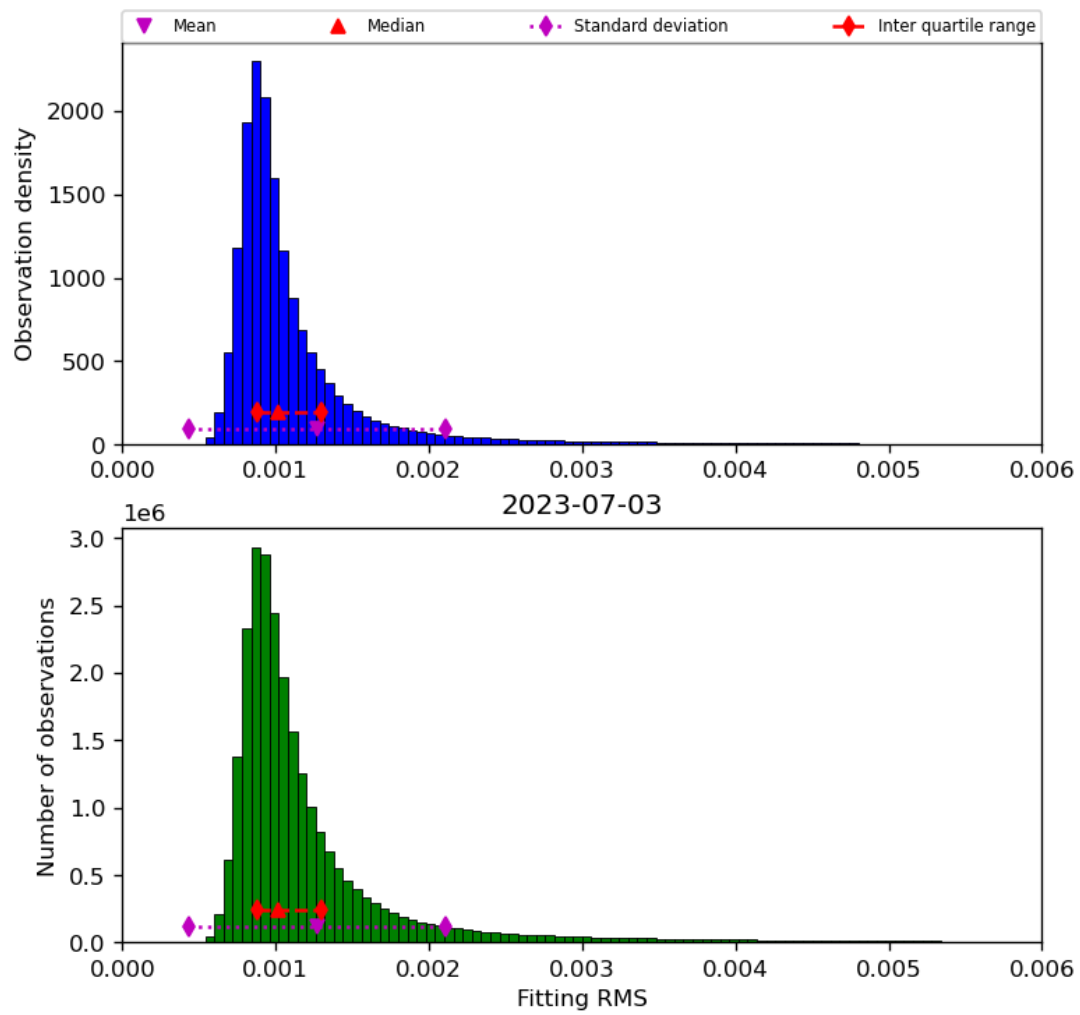
Figure 23: Histogram of “Fitting RMS” for 2023-07-03 to 2023-07-04
