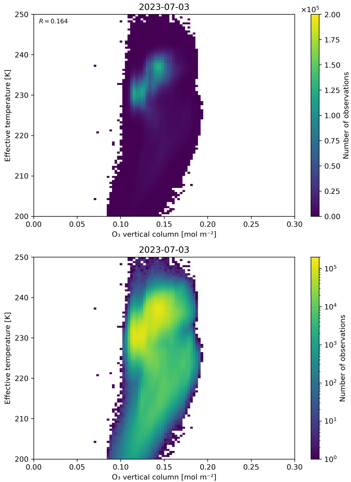
Figure 39: Scatter density plot of “O 3 vertical column” against “Effective temperature” for 2023-07-03 to 2023-07-04.
