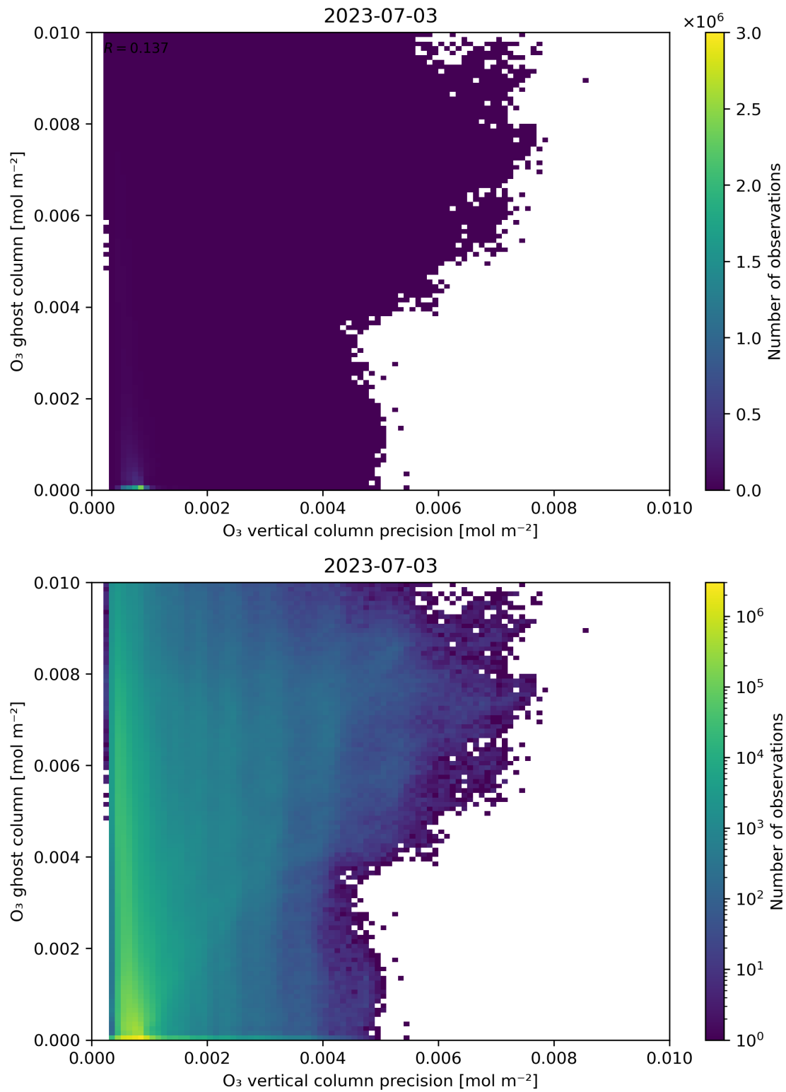
Figure 43: Scatter density plot of “ \text{O}_3 vertical column precision” against “ \text{O}_3 ghost column” for 2023-07-03 to 2023-07-04.
