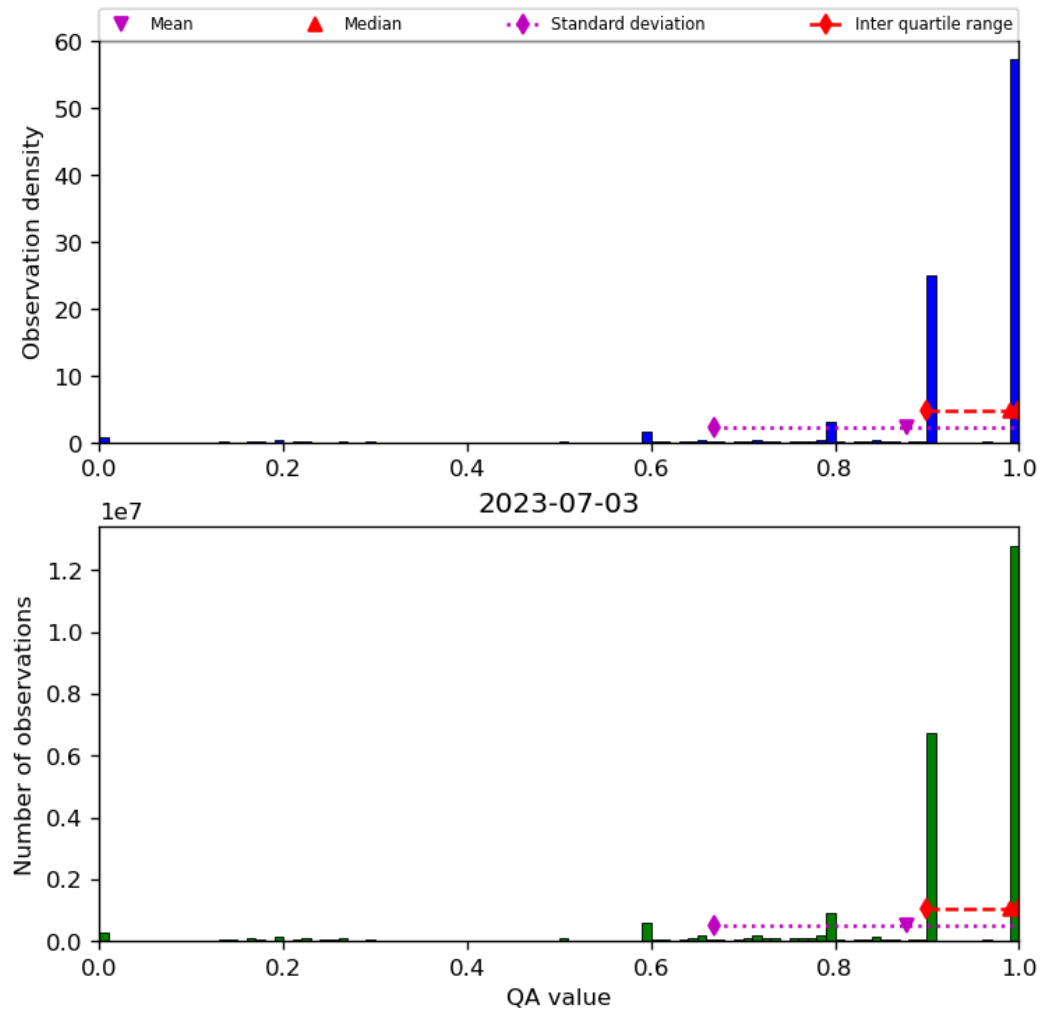
Figure 20: Histogram of “QA value” for 2023-07-03 to 2023-07-04
