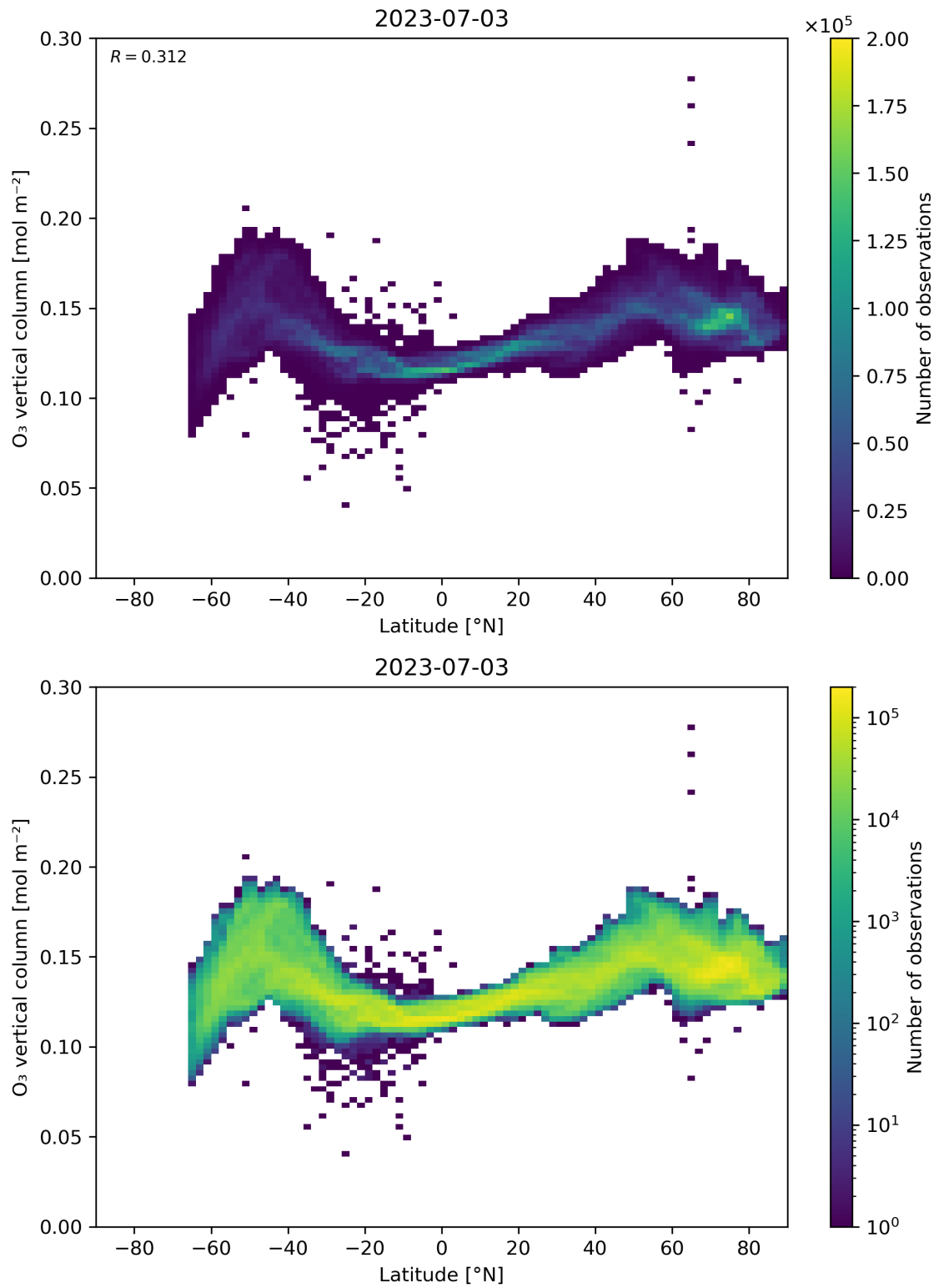
Figure 36: Scatter density plot of “Latitude” against “O 3 vertical column” for 2023-07-03 to 2023-07-04.
