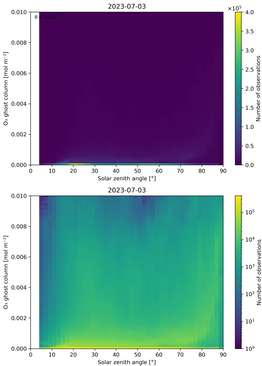
Figure 46: Scatter density plot of “Solar zenith angle” against “O 3 ghost column” for 2023-07-03 to 2023-07-04.
