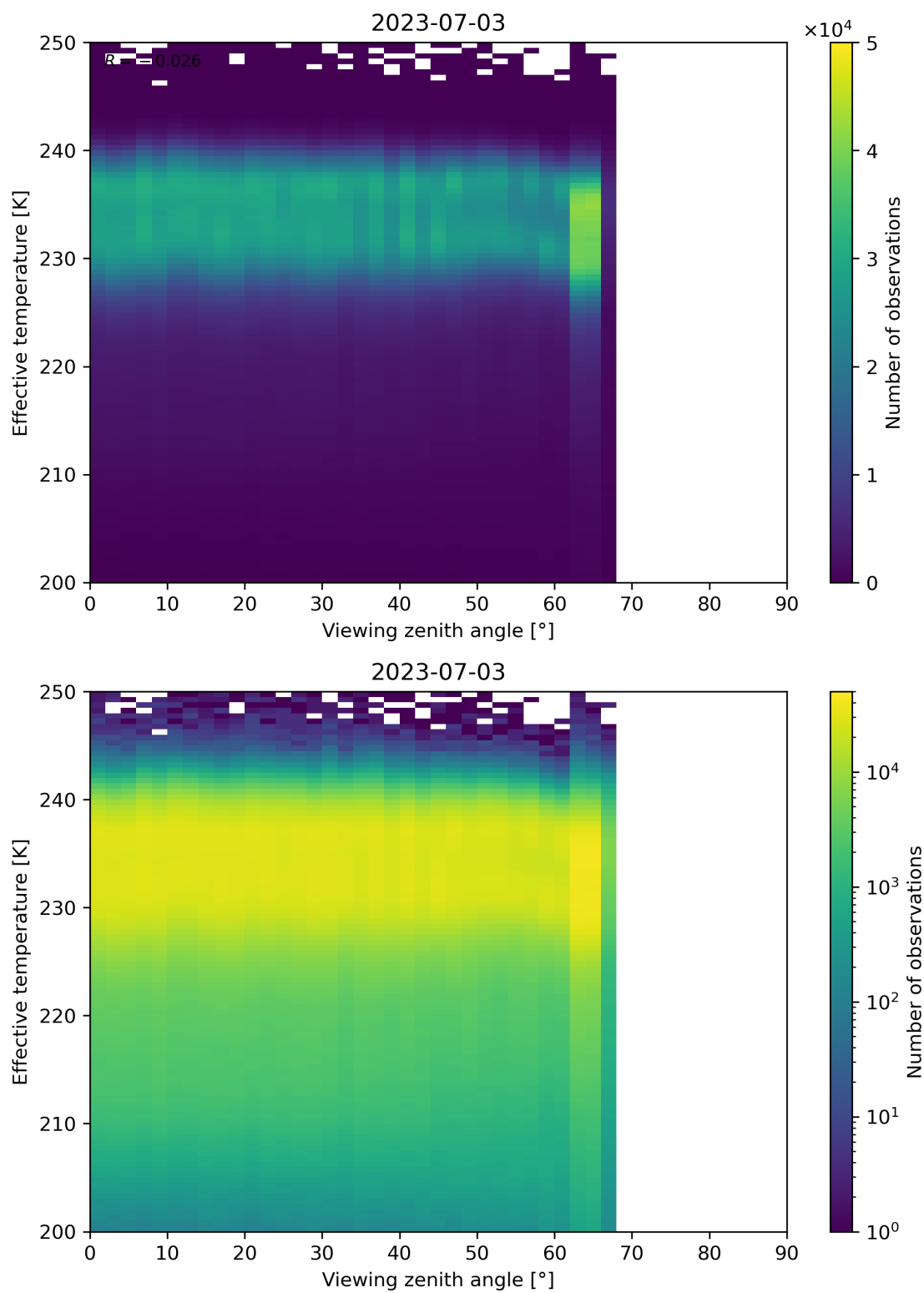
Figure 50: Scatter density plot of “Viewing zenith angle” against “Effective temperature” for 2023-07-03 to 2023-07-04.
