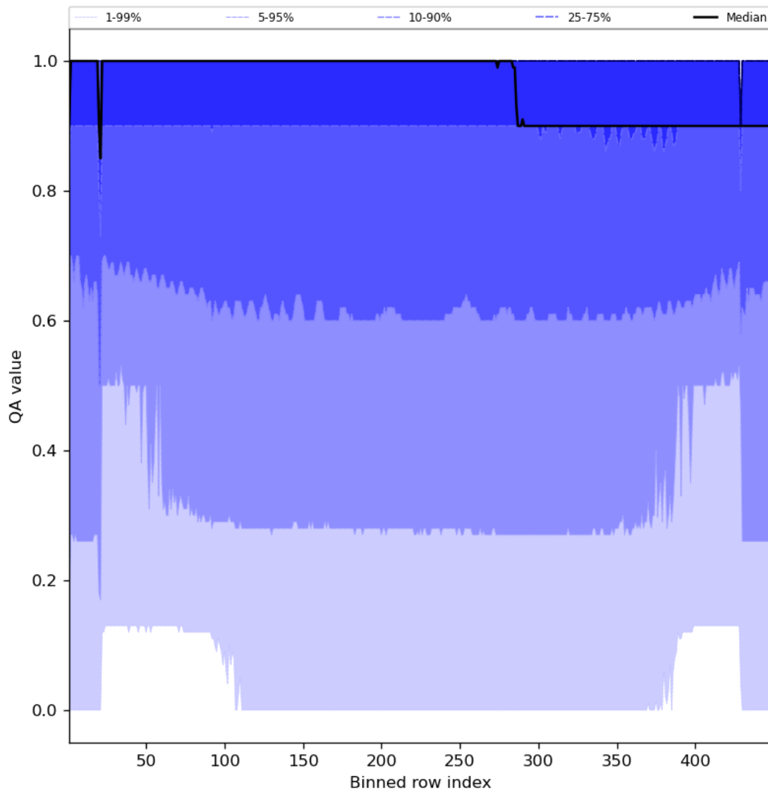
Figure 27: Along track statistics of “QA value” for 2023-07-03 to 2023-07-04
