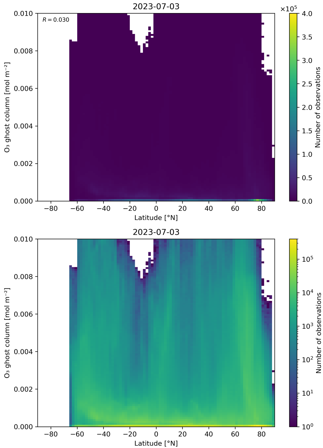
Figure 35: Scatter density plot of “Latitude” against “O 3 ghost column” for 2023-07-03 to 2023-07-04.
