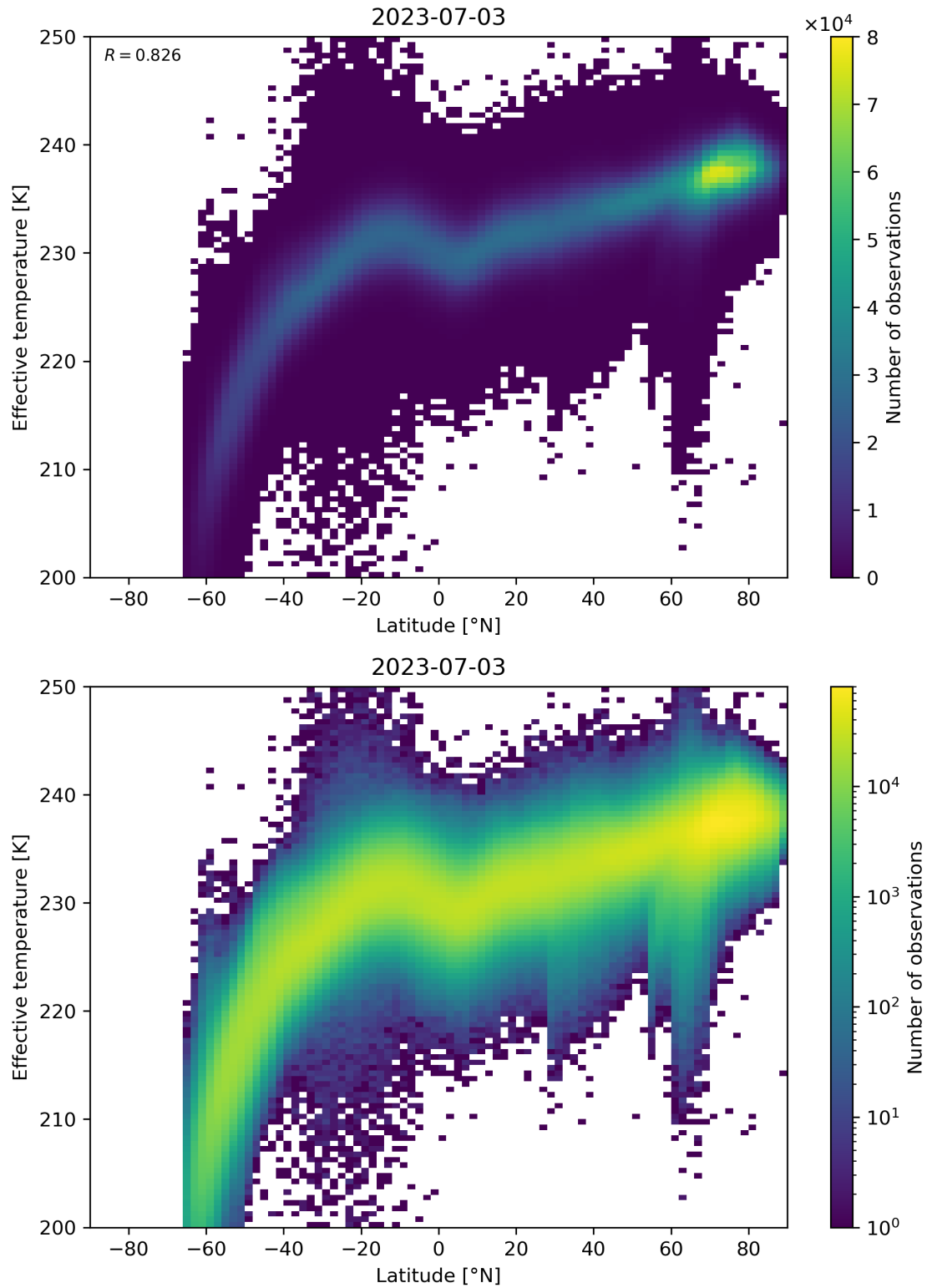
Figure 34: Scatter density plot of “Latitude” against “Effective temperature” for 2023-07-03 to 2023-07-04.
