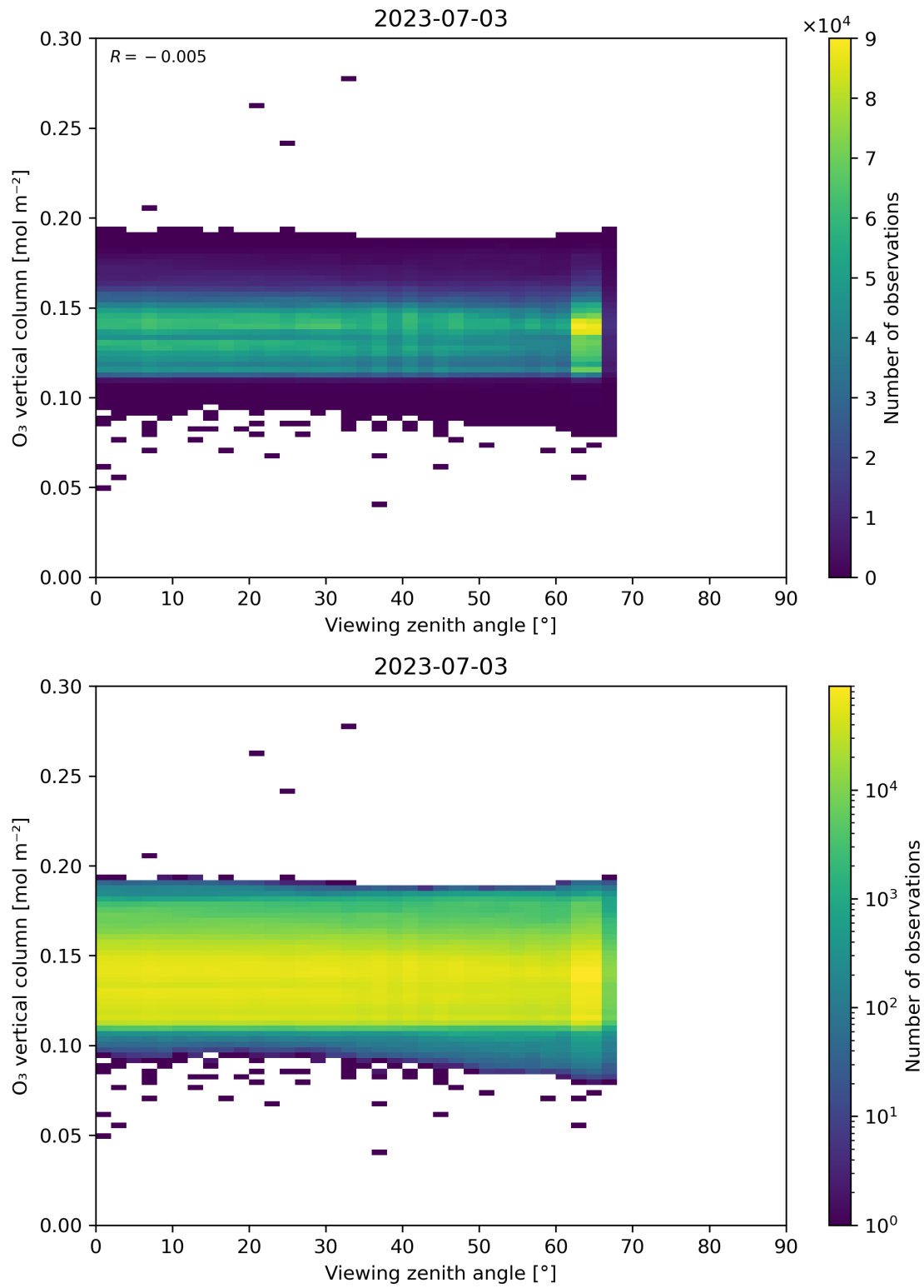
Figure 52: Scatter density plot of “Viewing zenith angle” against “O 3 vertical column” for 2023-07-03 to 2023-07-04.
