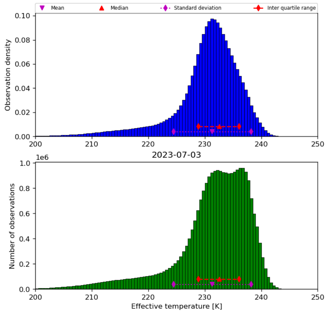
Figure 24: Histogram of “Effective temperature” for 2023-07-03 to 2023-07-04
