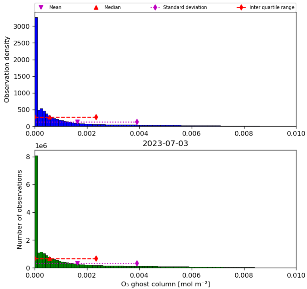
Figure 25: Histogram of “O 3 ghost column” for 2023-07-03 to 2023-07-04
