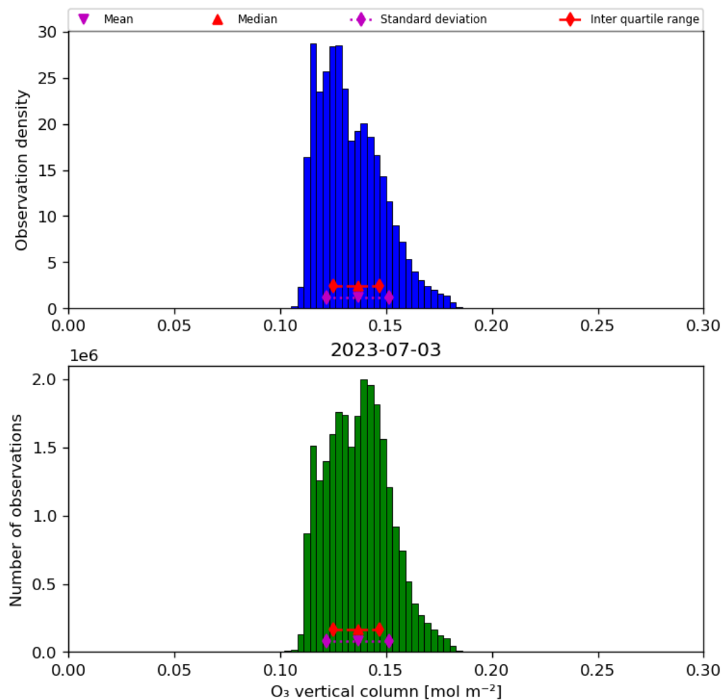
Figure 21: Histogram of “O 3 vertical column” for 2023-07-03 to 2023-07-04
