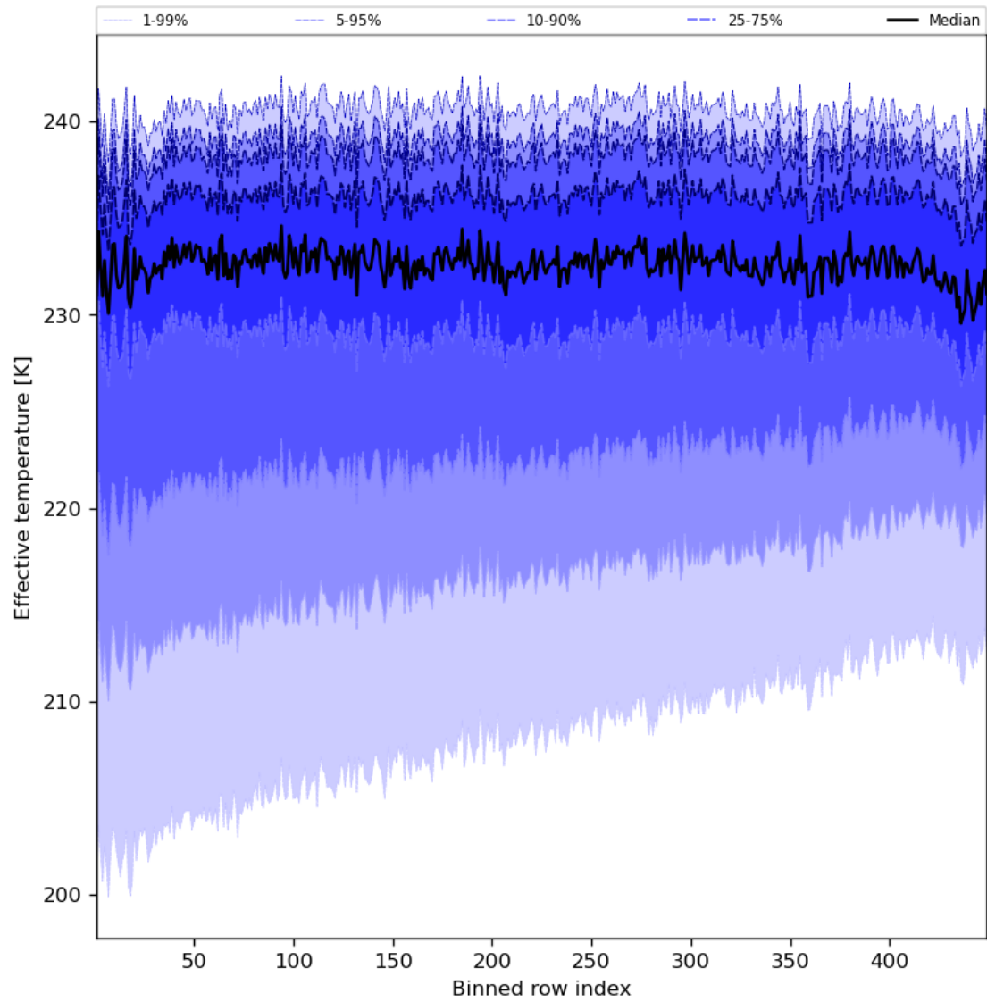
Figure 31: Along track statistics of “Effective temperature” for 2023-07-03 to 2023-07-04
