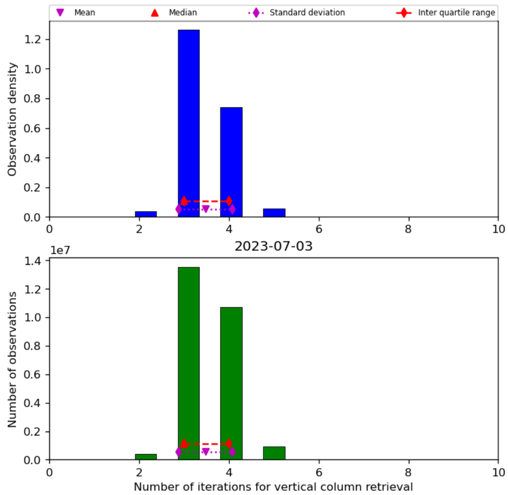
Figure 26: Histogram of “Number of iterations for vertical column retrieval” for 2023-07-03 to 2023-07-04
