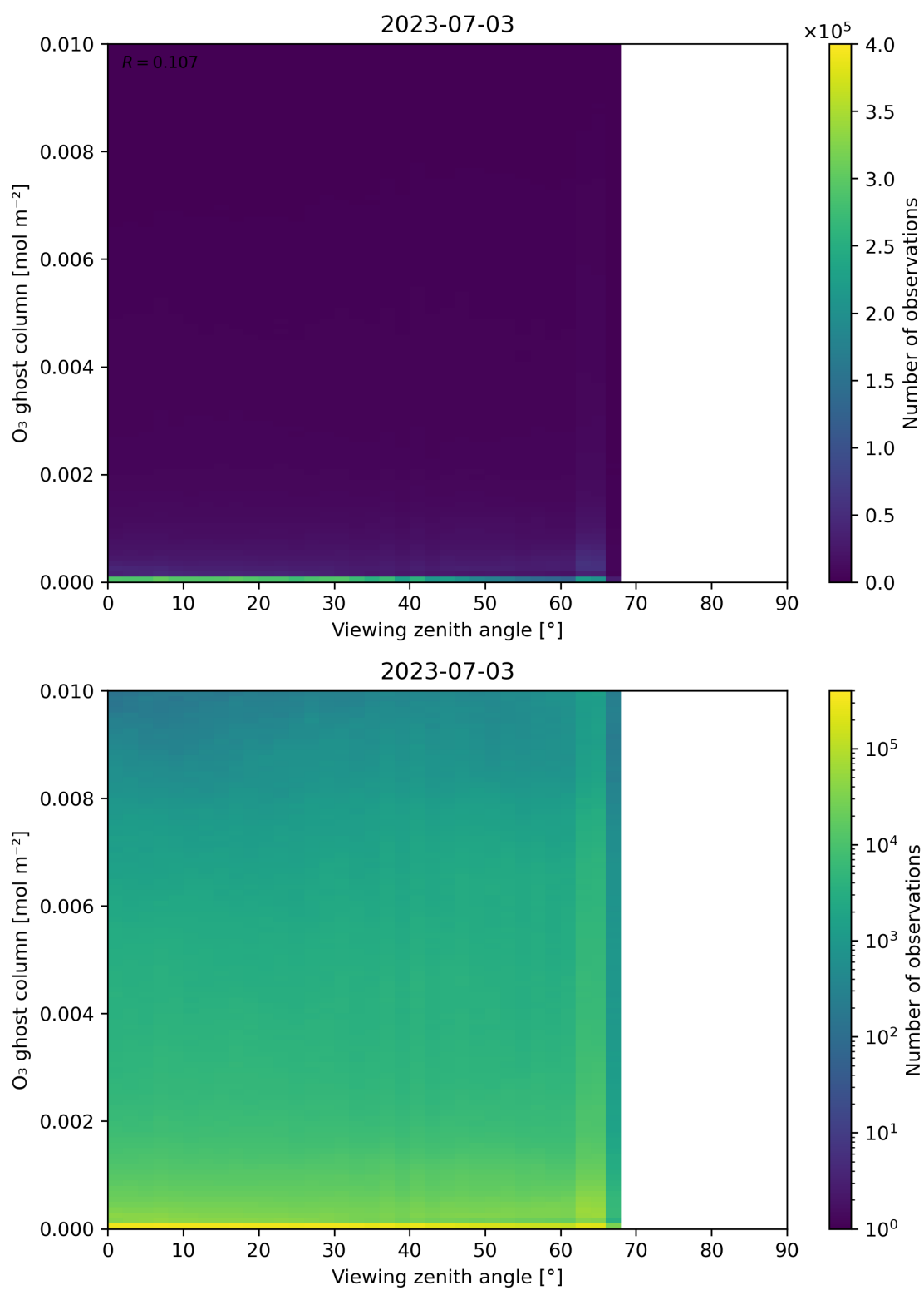
Figure 51: Scatter density plot of “Viewing zenith angle” against “O 3 ghost column” for 2023-07-03 to 2023-07-04.
