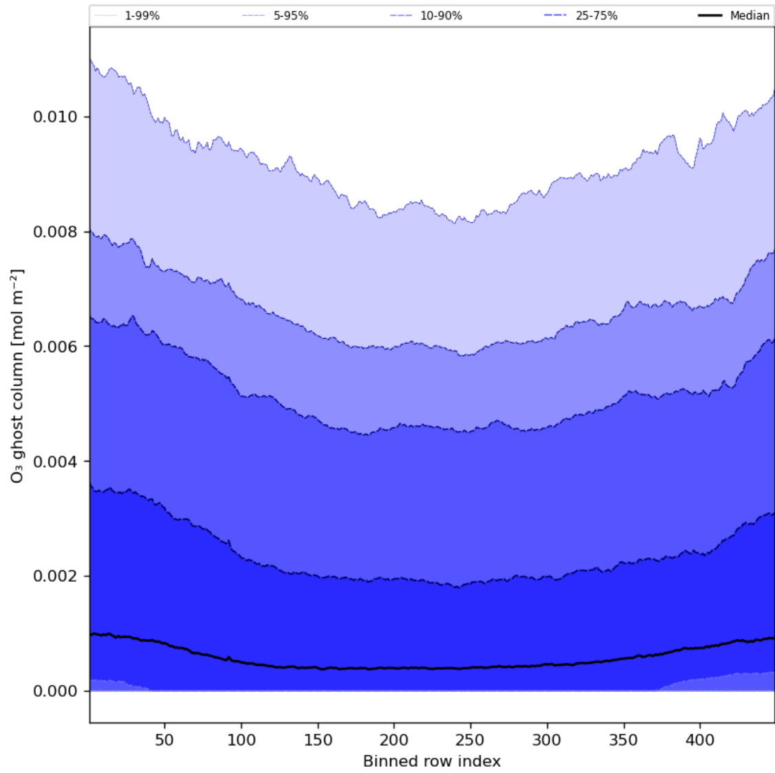
Figure 32: Along track statistics of “O 3 ghost column” for 2023-07-03 to 2023-07-04
