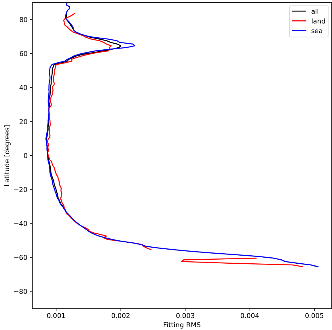
Figure 16: Zonal average of “Fitting RMS” for 2023-07-03 to 2023-07-04.
