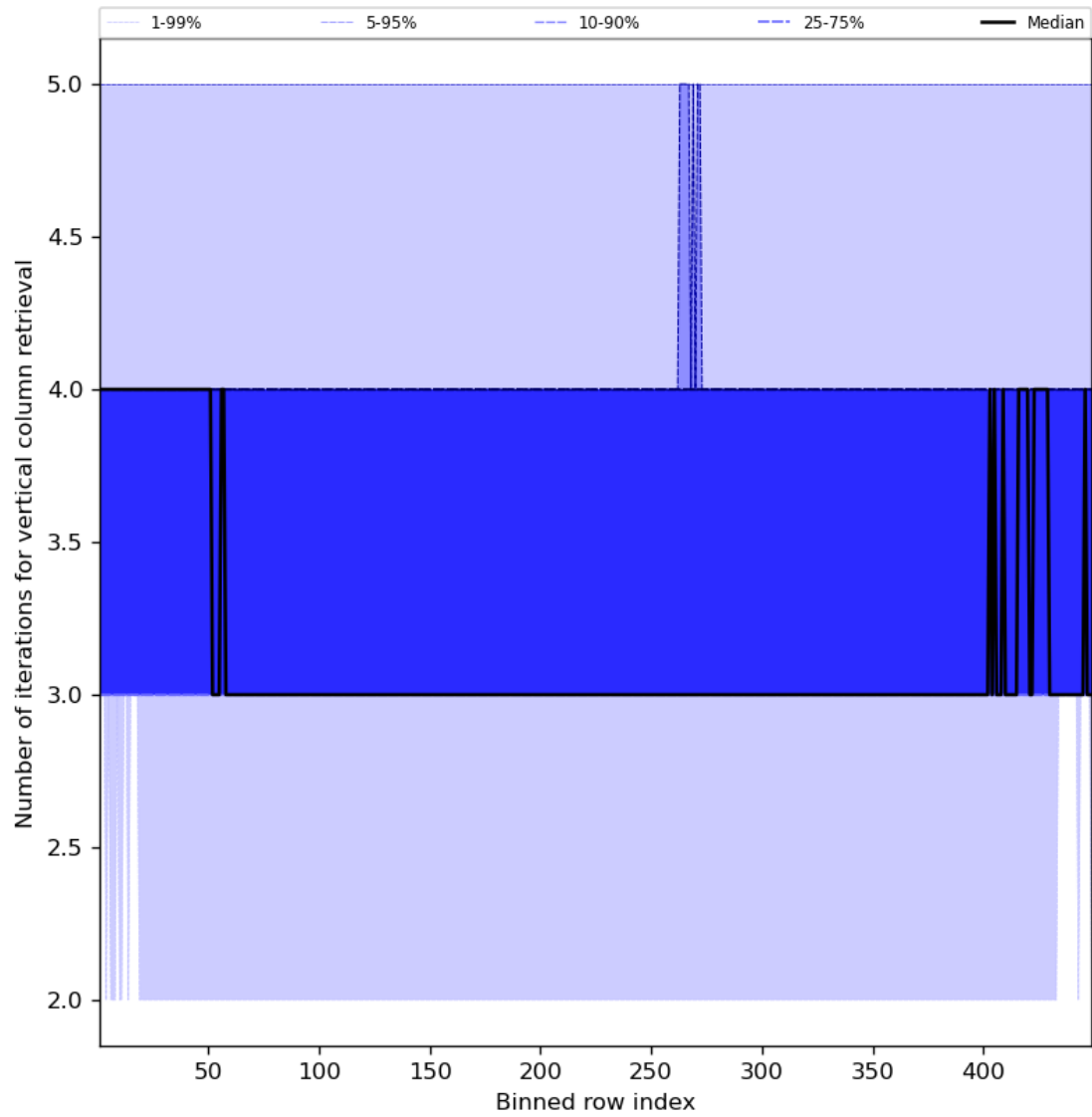
Figure 33: Along track statistics of “Number of iterations for vertical column retrieval” for 2023-07-03 to 2023-07-04
