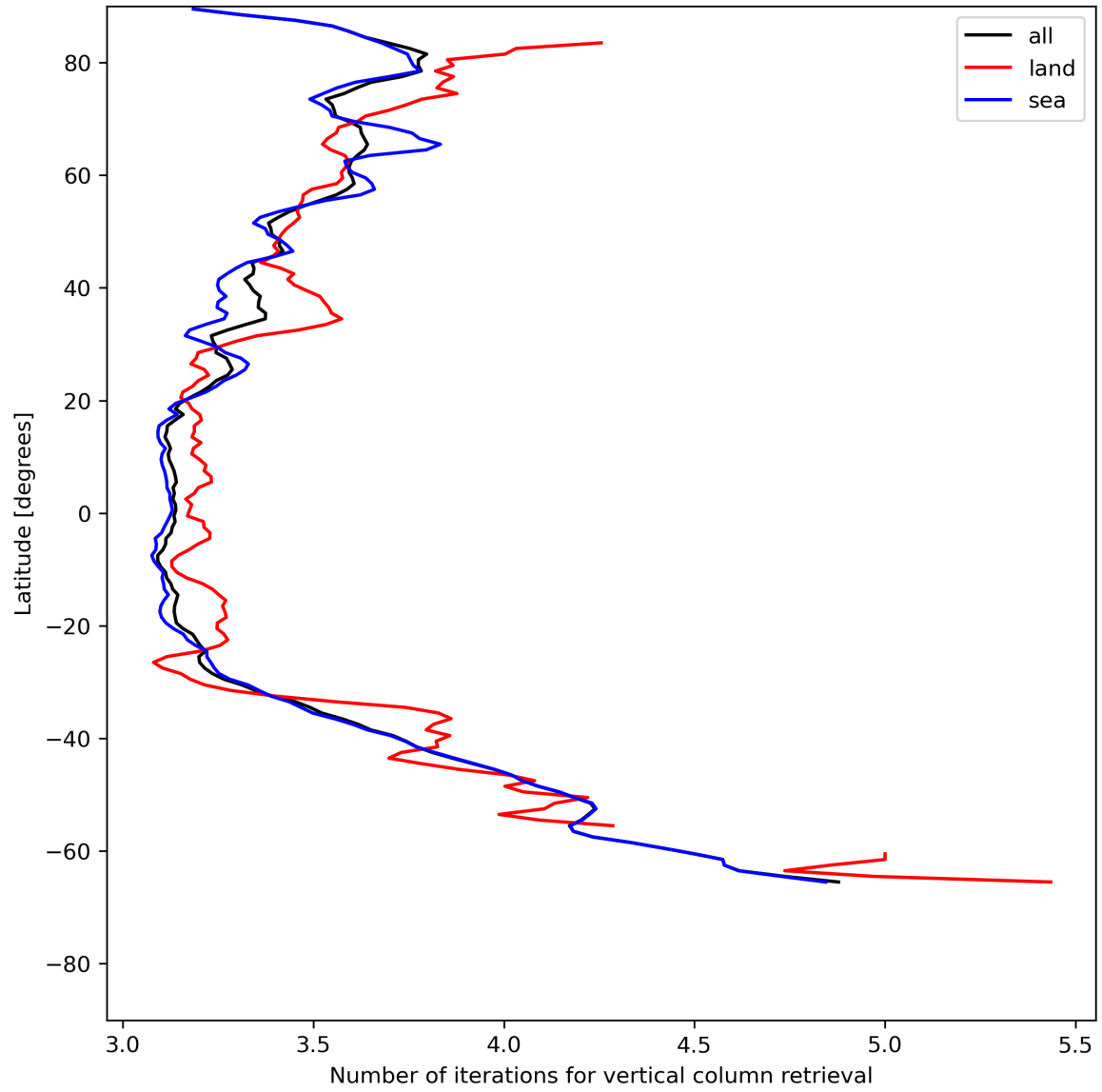
Figure 19: Zonal average of “Number of iterations for vertical column retrieval” for 2023-07-03 to 2023-07-04.
