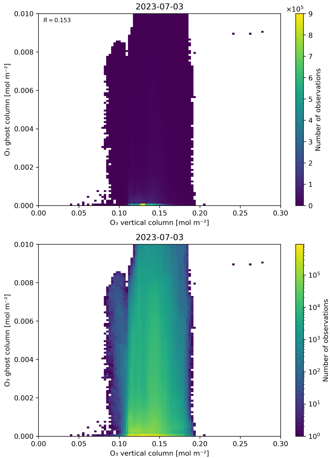
Figure 40: Scatter density plot of “O 3 vertical column” against “O 3 ghost column” for 2023-07-03 to 2023-07-04.
