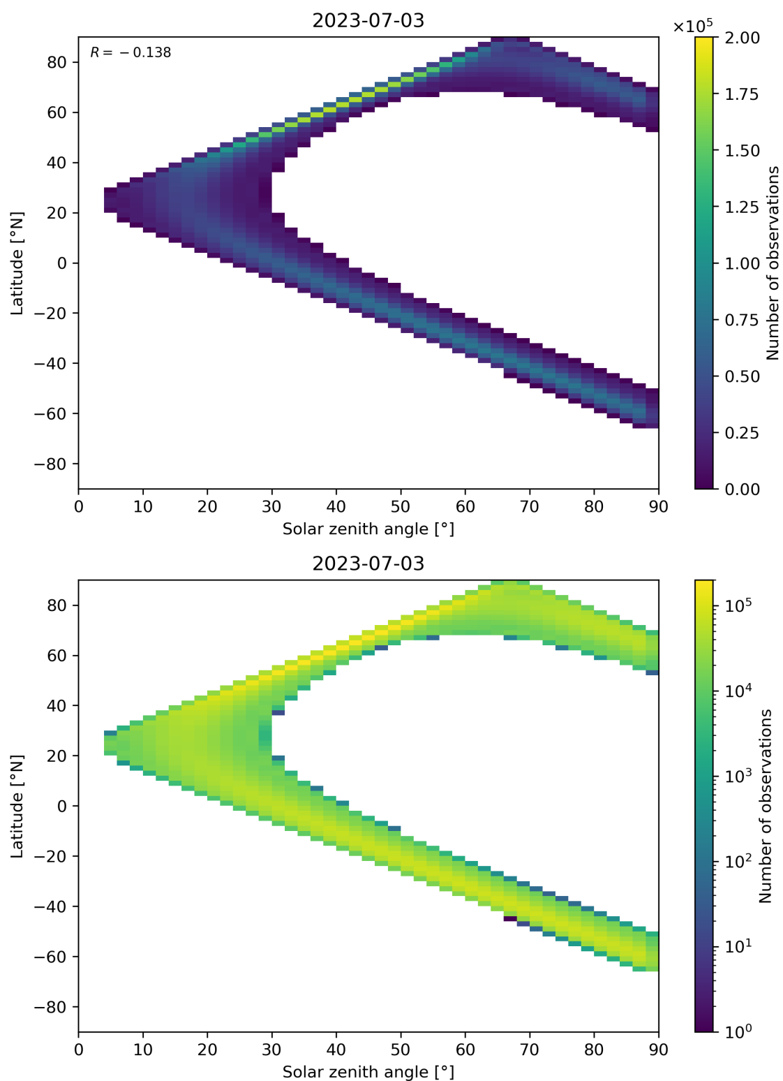
Figure 44: Scatter density plot of “Solar zenith angle” against “Latitude” for 2023-07-03 to 2023-07-04.
