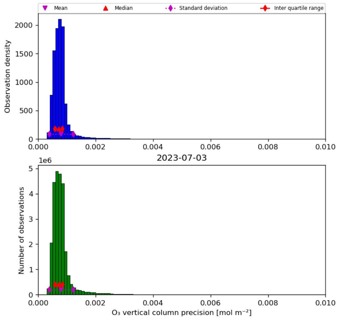
Figure 22: Histogram of “O 3 vertical column precision” for 2023-07-03 to 2023-07-04
