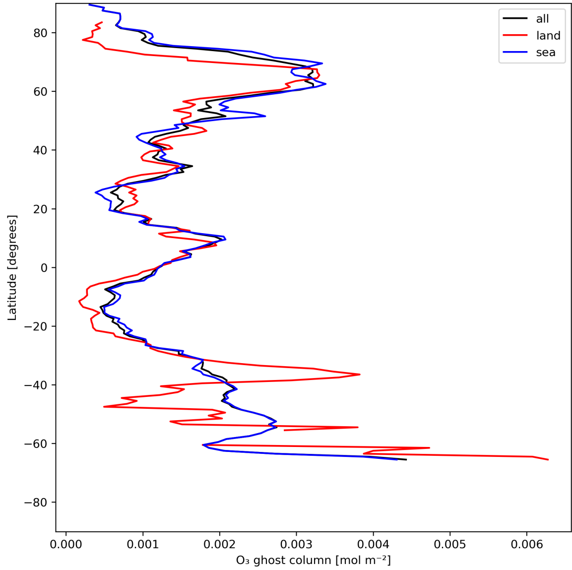
Figure 18: Zonal average of “O 3 ghost column” for 2023-07-03 to 2023-07-04.
