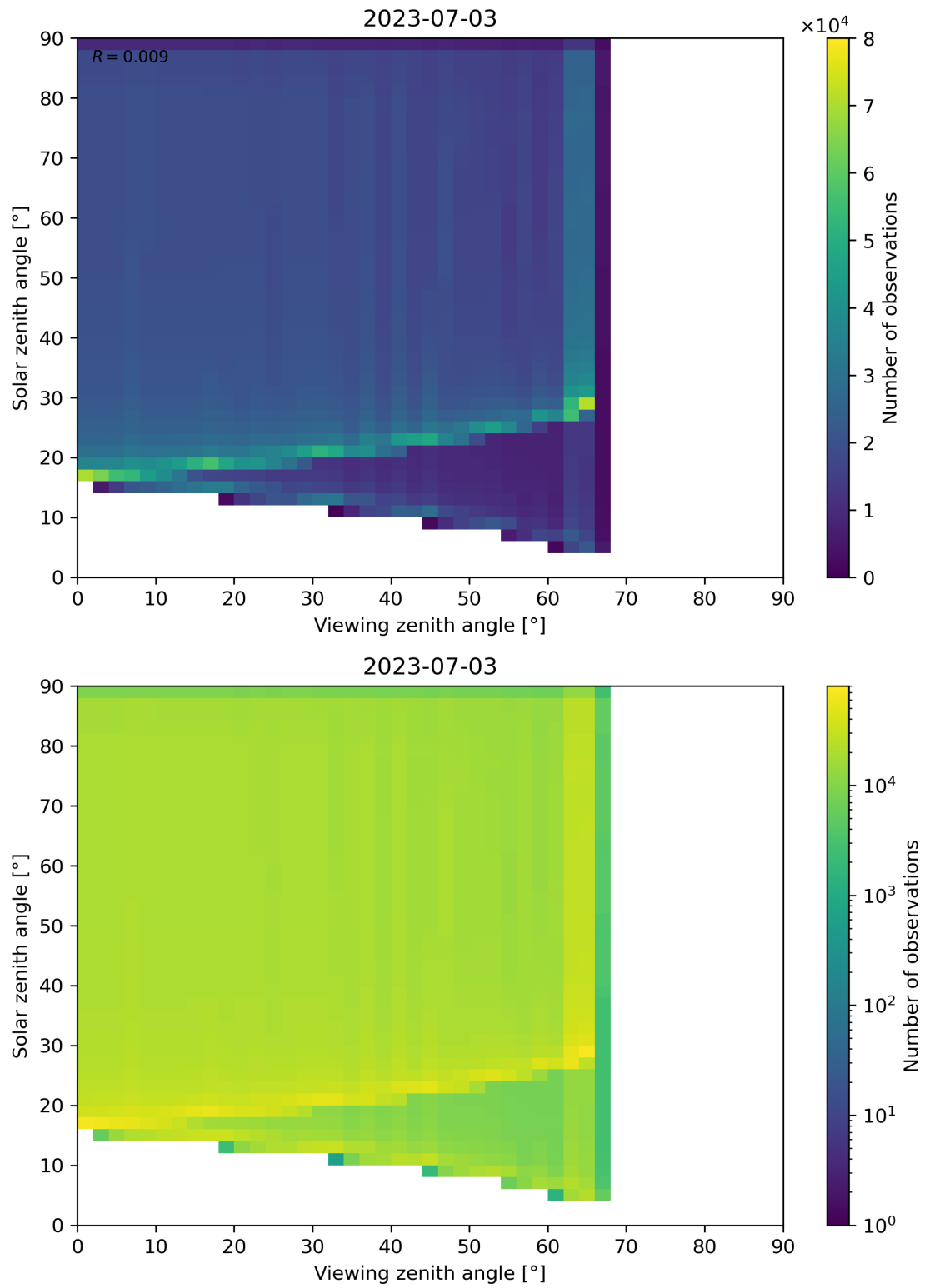
Figure 54: Scatter density plot of “Viewing zenith angle” against “Solar zenith angle” for 2023-07-03 to 2023-07-04.
