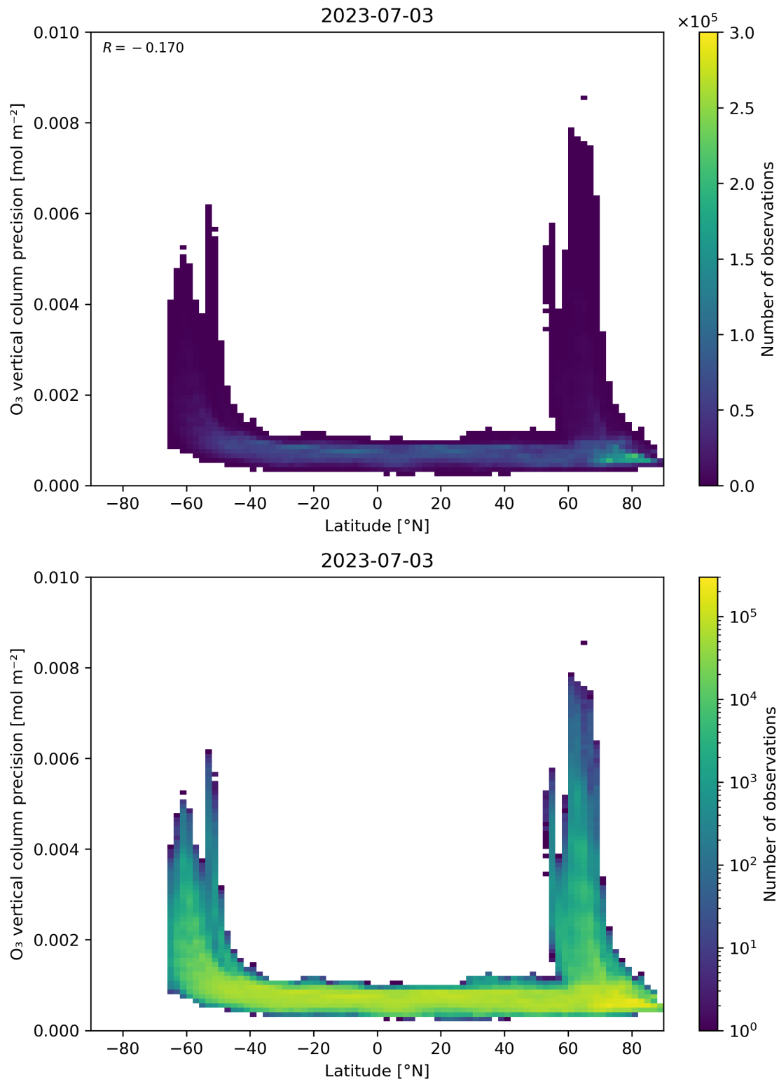
Figure 37: Scatter density plot of “Latitude” against “O 3 vertical column precision” for 2023-07-03 to 2023-07-04.
