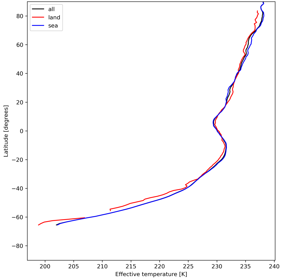
Figure 17: Zonal average of "Effective temperature" for 2023-07-03 to 2023-07-04.
