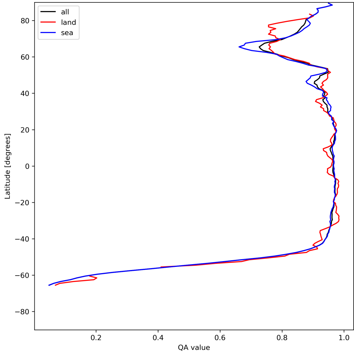
Figure 13: Zonal average of “QA value” for 2023-07-03 to 2023-07-04.
