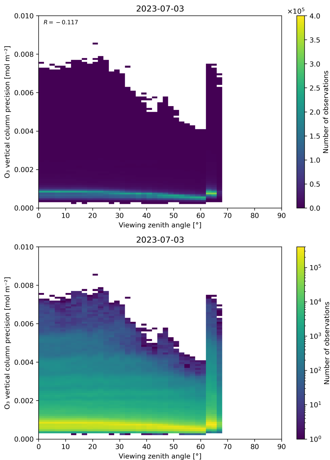
Figure 53: Scatter density plot of “Viewing zenith angle” against “O 3 vertical column precision” for 2023-07-03 to 2023-07-04.
