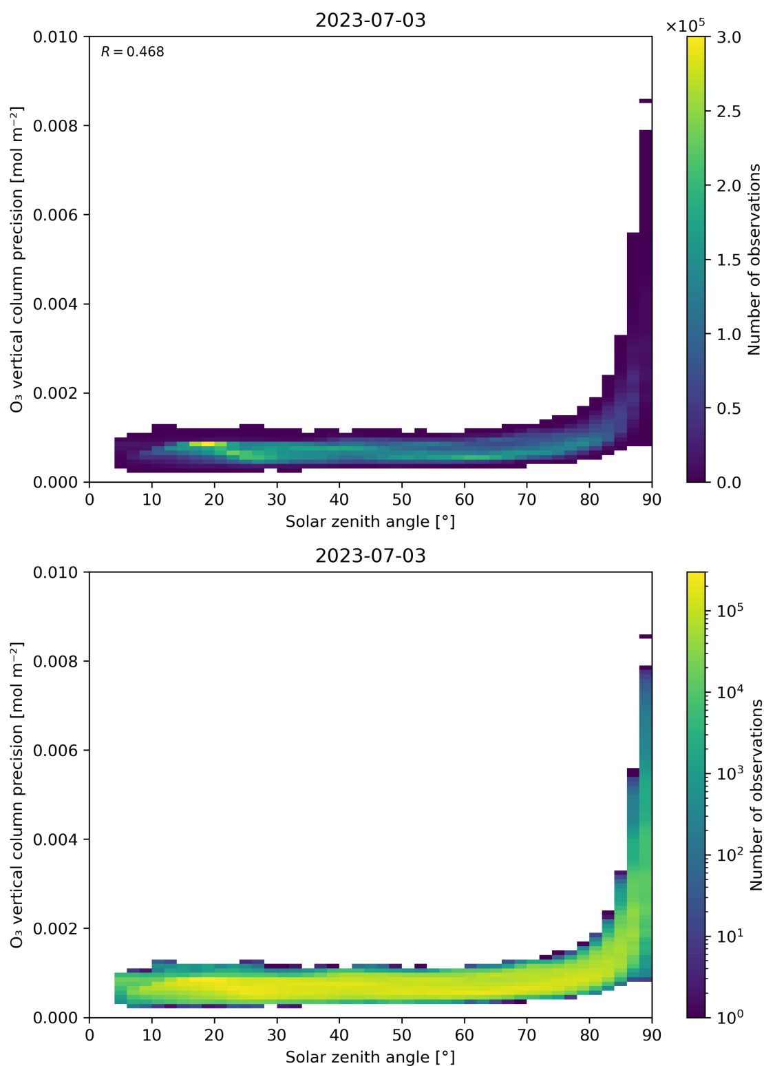
Figure 48: Scatter density plot of “Solar zenith angle” against “O 3 vertical column precision” for 2023-07-03 to 2023-07-04.
