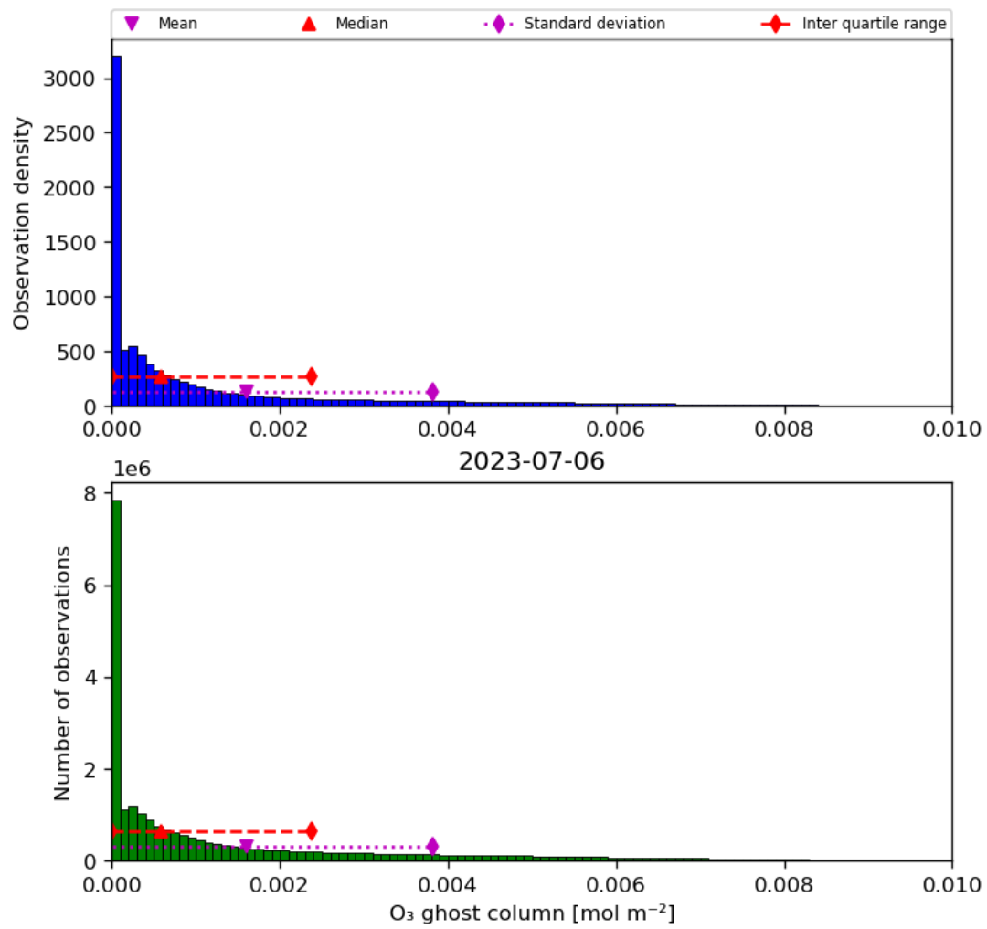
Figure 25: Histogram of “O 3 ghost column” for 2023-07-05 to 2023-07-07
