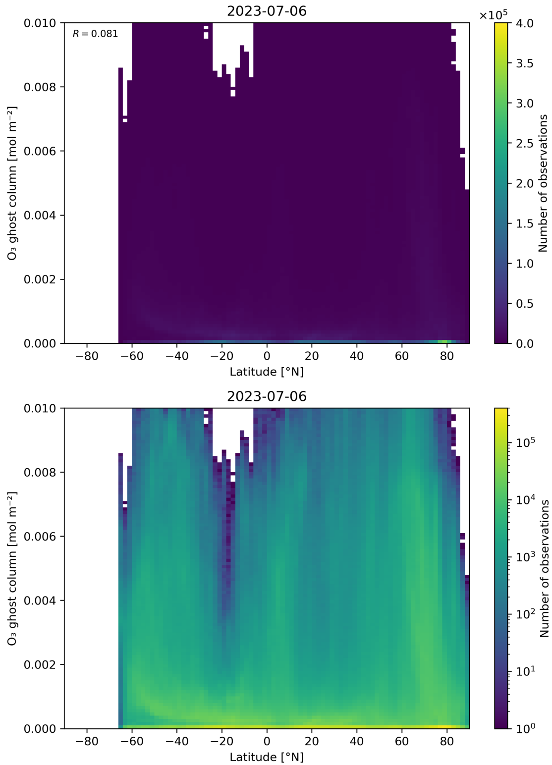
Figure 35: Scatter density plot of “Latitude” against “O 3 ghost column” for 2023-07-05 to 2023-07-07.
