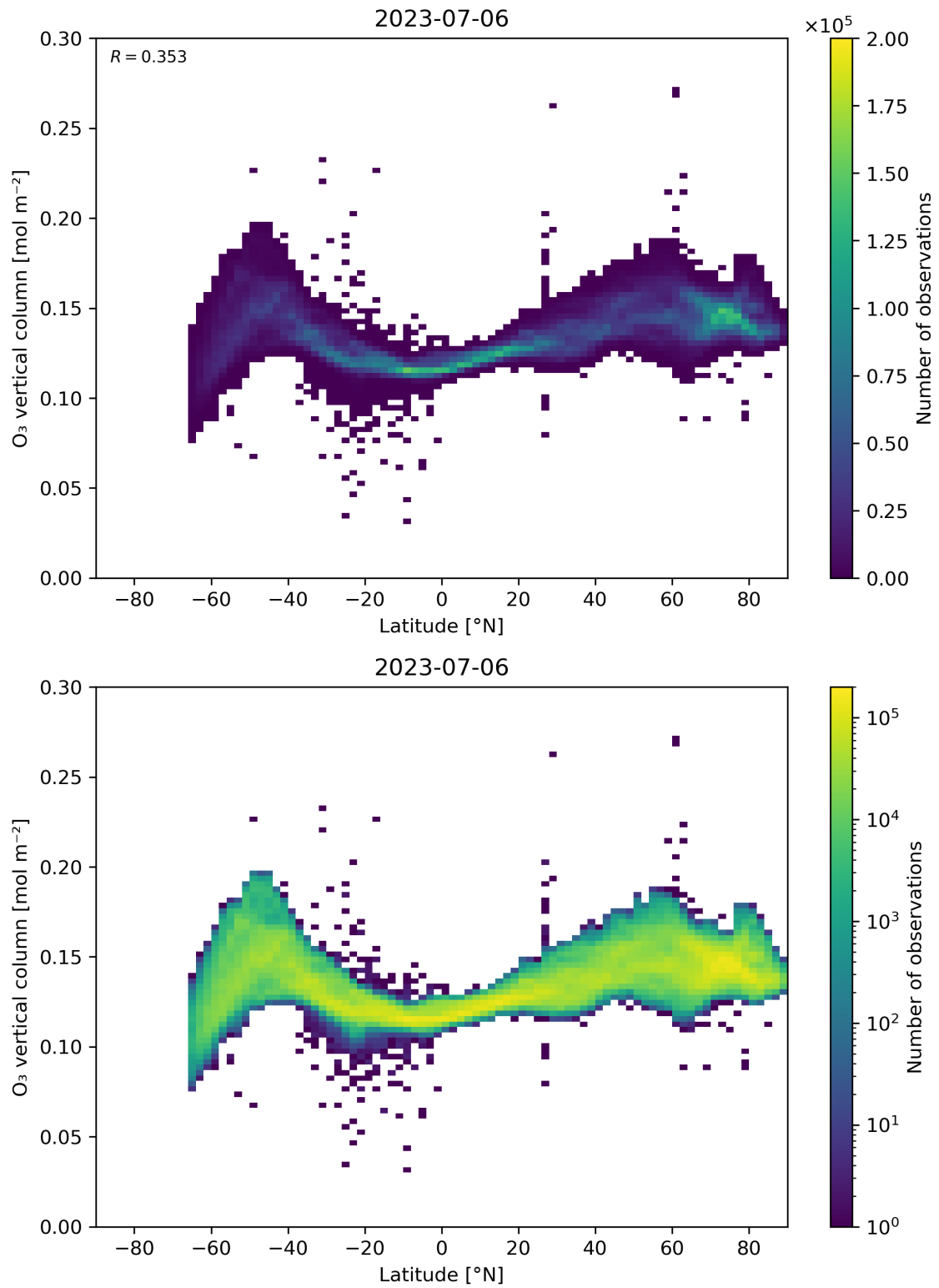
Figure 36: Scatter density plot of “Latitude” against “O 3 vertical column” for 2023-07-05 to 2023-07-07.
