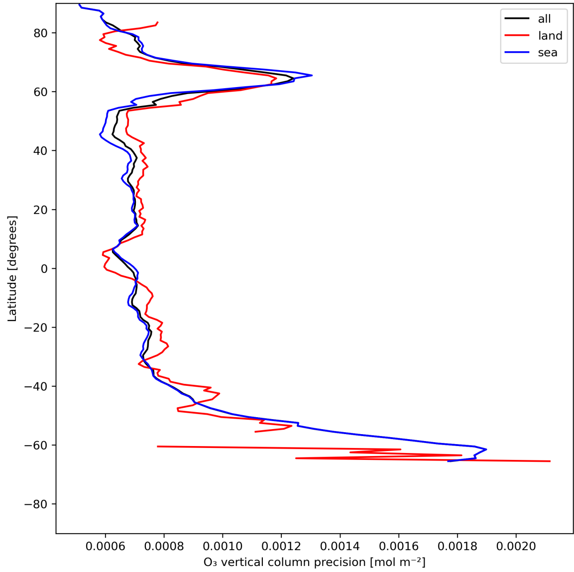
Figure 15: Zonal average of "O 3 vertical column precision" for 2023-07-05 to 2023-07-07.
