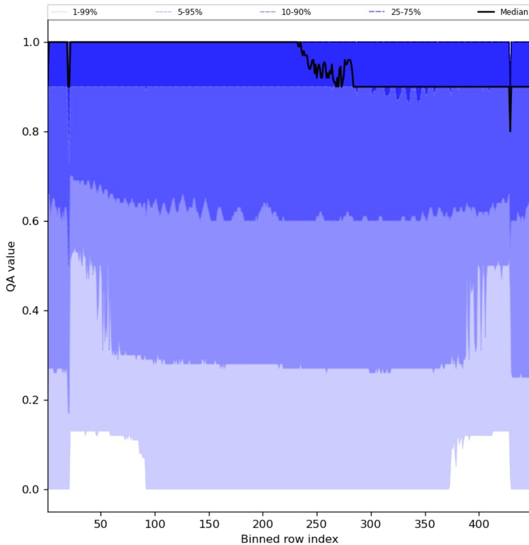
Figure 27: Along track statistics of “QA value” for 2023-07-05 to 2023-07-07
