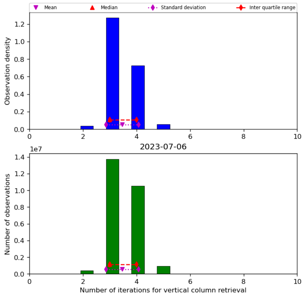
Figure 26: Histogram of “Number of iterations for vertical column retrieval” for 2023-07-05 to 2023-07-07
