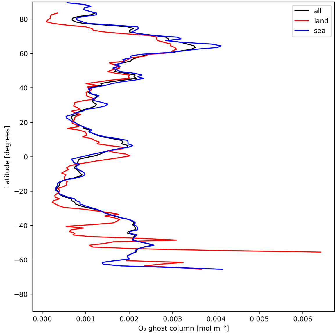
Figure 18: Zonal average of “O 3 ghost column” for 2023-07-05 to 2023-07-07.
