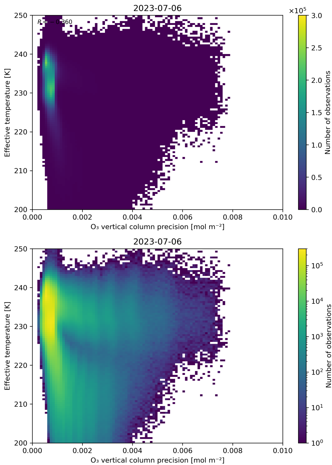
Figure 42: Scatter density plot of “O 3 vertical column precision” against “Effective temperature” for 2023-07-05 to 2023-07-07.
