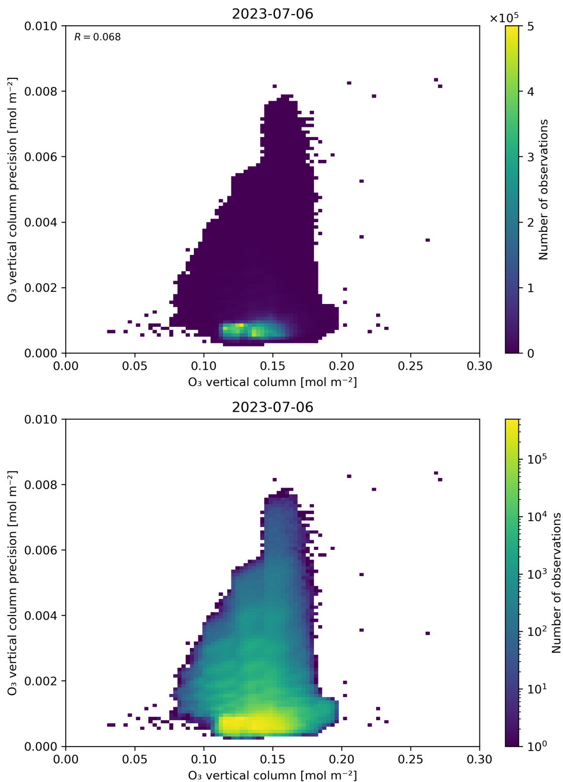
Figure 41: Scatter density plot of “O 3 vertical column” against “O 3 vertical column precision” for 2023-07-05 to 2023-07-07.
