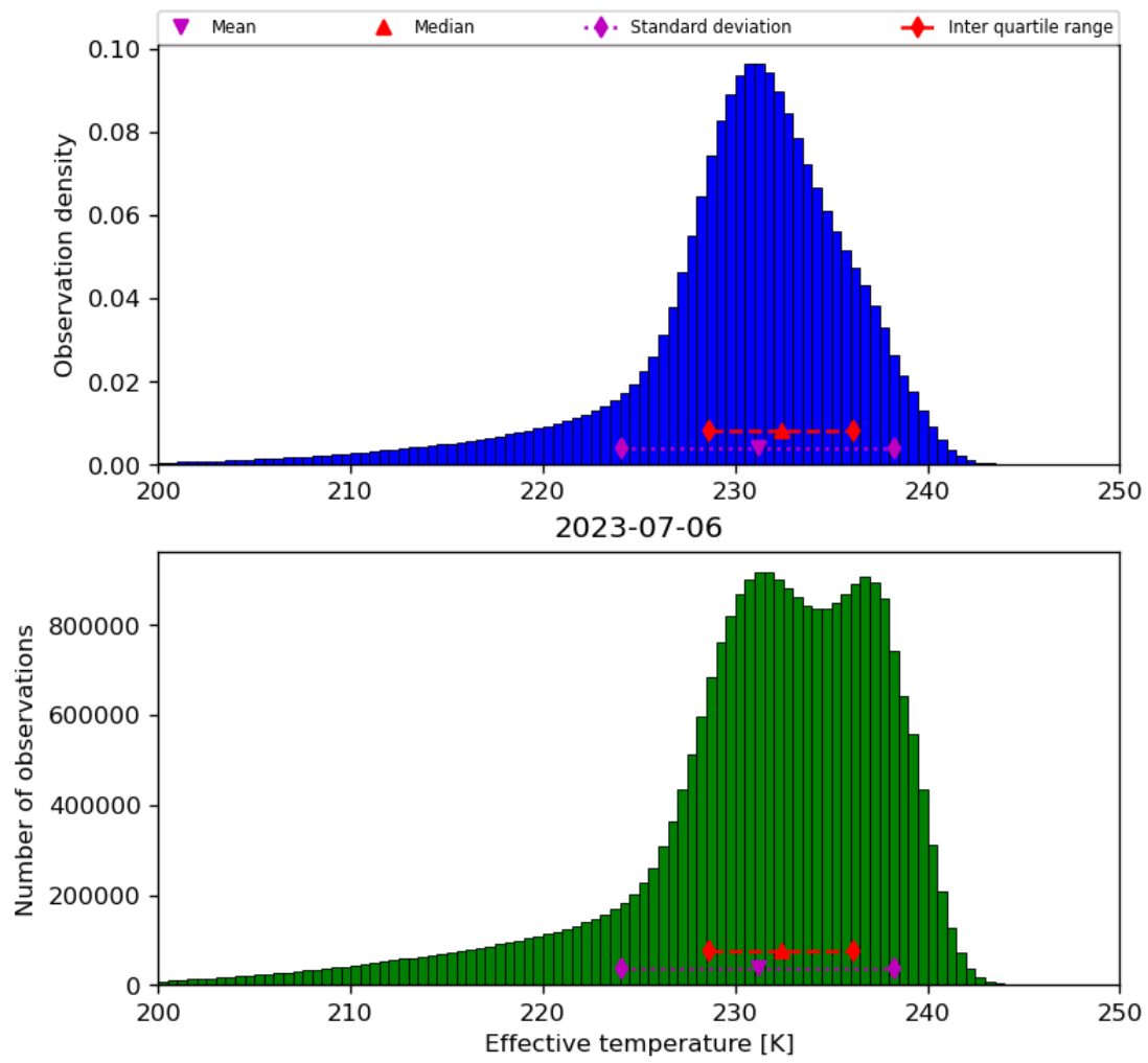
Figure 24: Histogram of “Effective temperature” for 2023-07-05 to 2023-07-07
