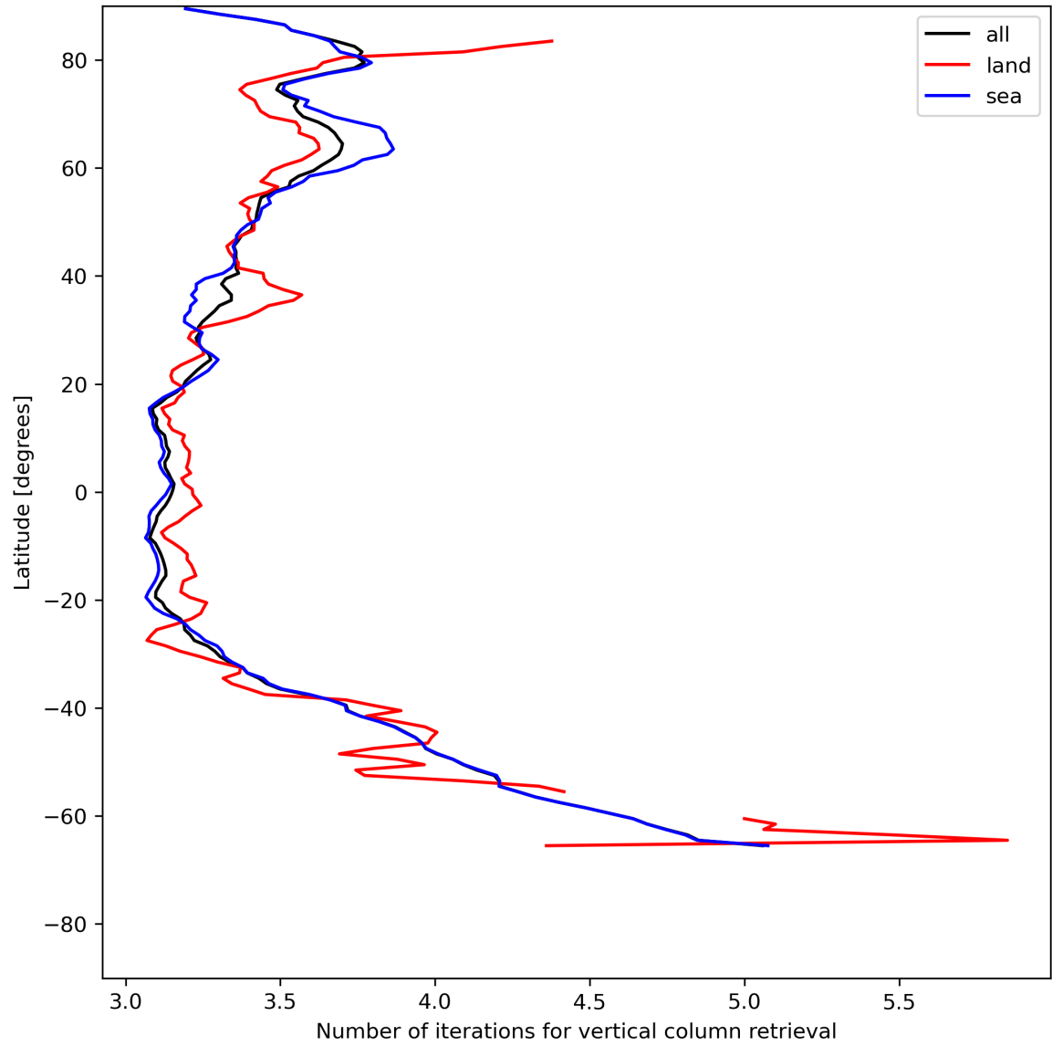
Figure 19: Zonal average of “Number of iterations for vertical column retrieval” for 2023-07-05 to 2023-07-07.
