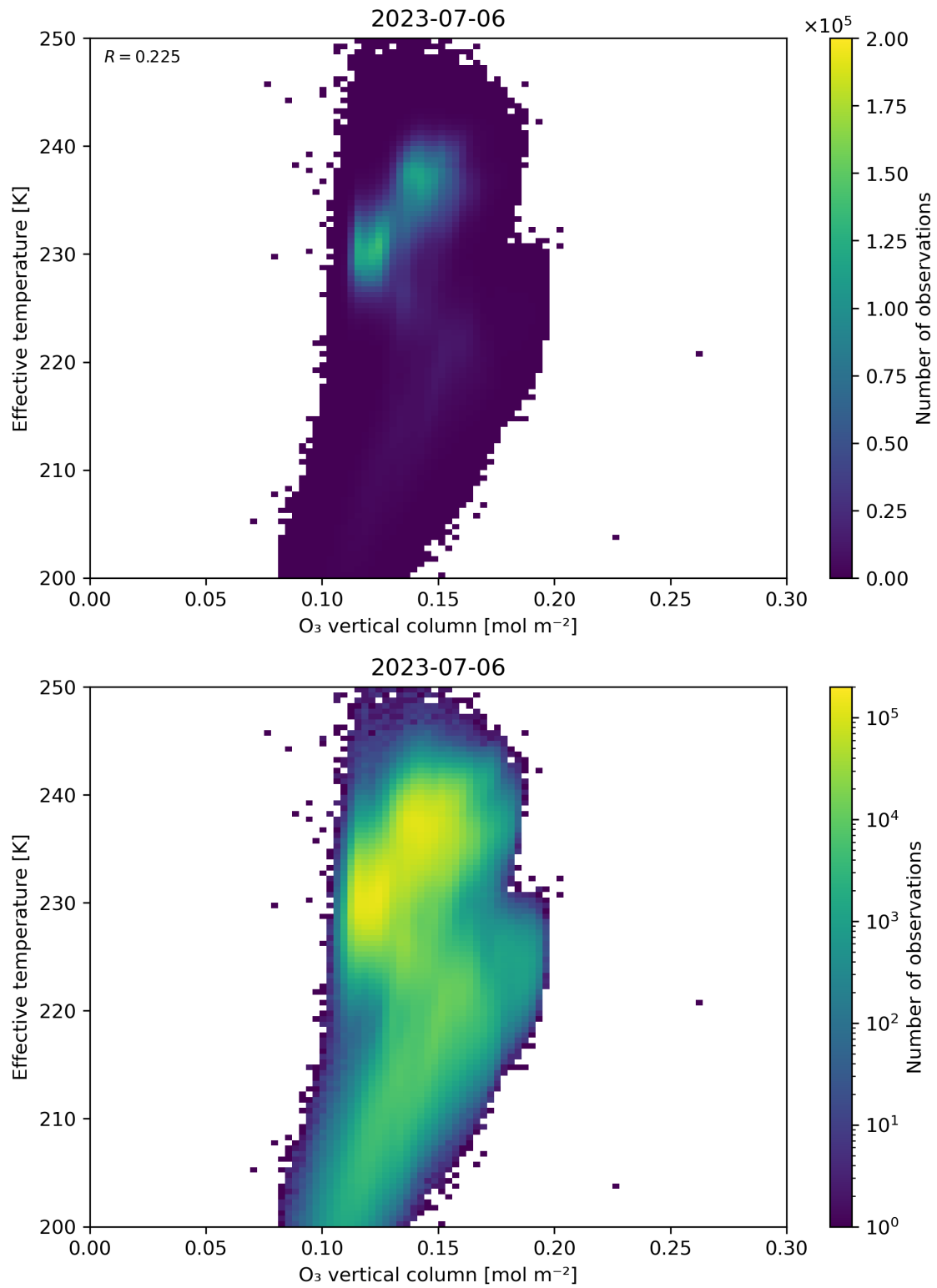
Figure 39: Scatter density plot of “O 3 vertical column” against “Effective temperature” for 2023-07-05 to 2023-07-07.
