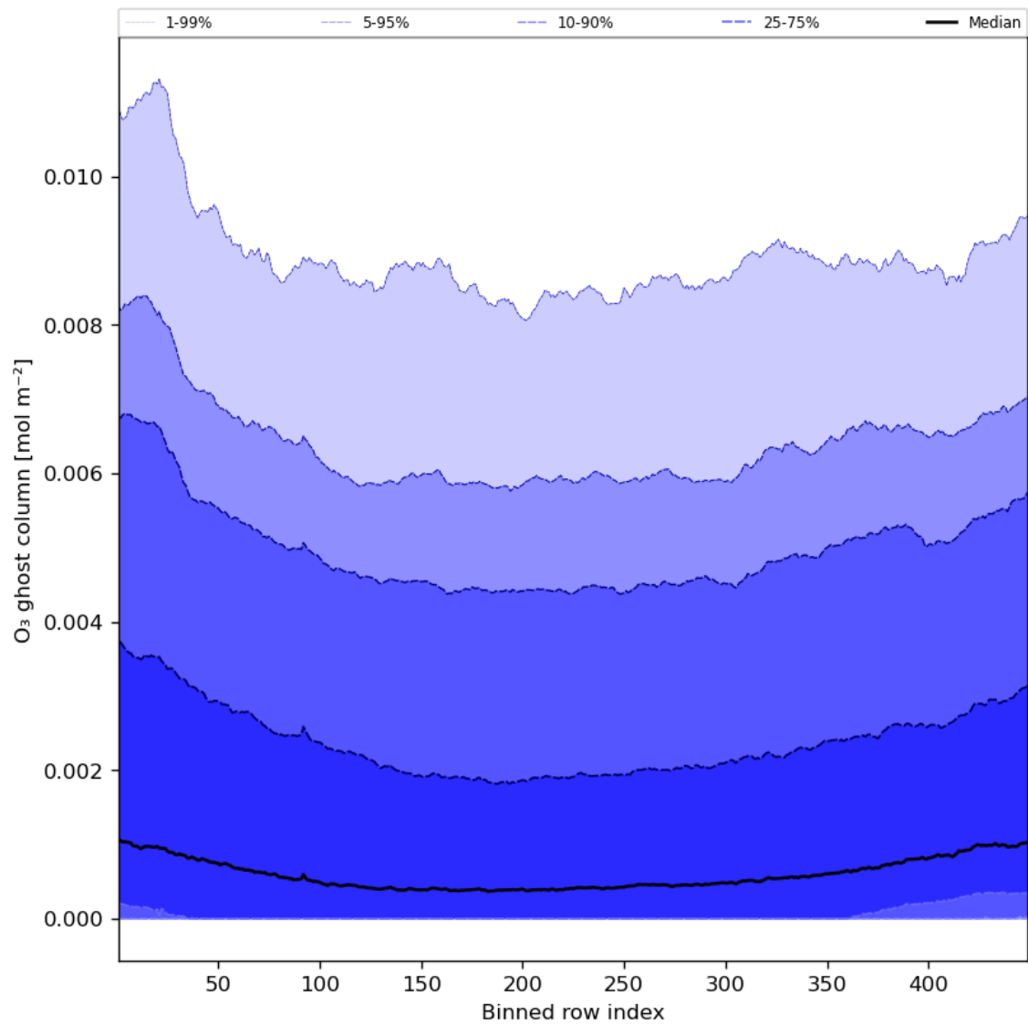
Figure 32: Along track statistics of “O 3 ghost column” for 2023-07-05 to 2023-07-07
