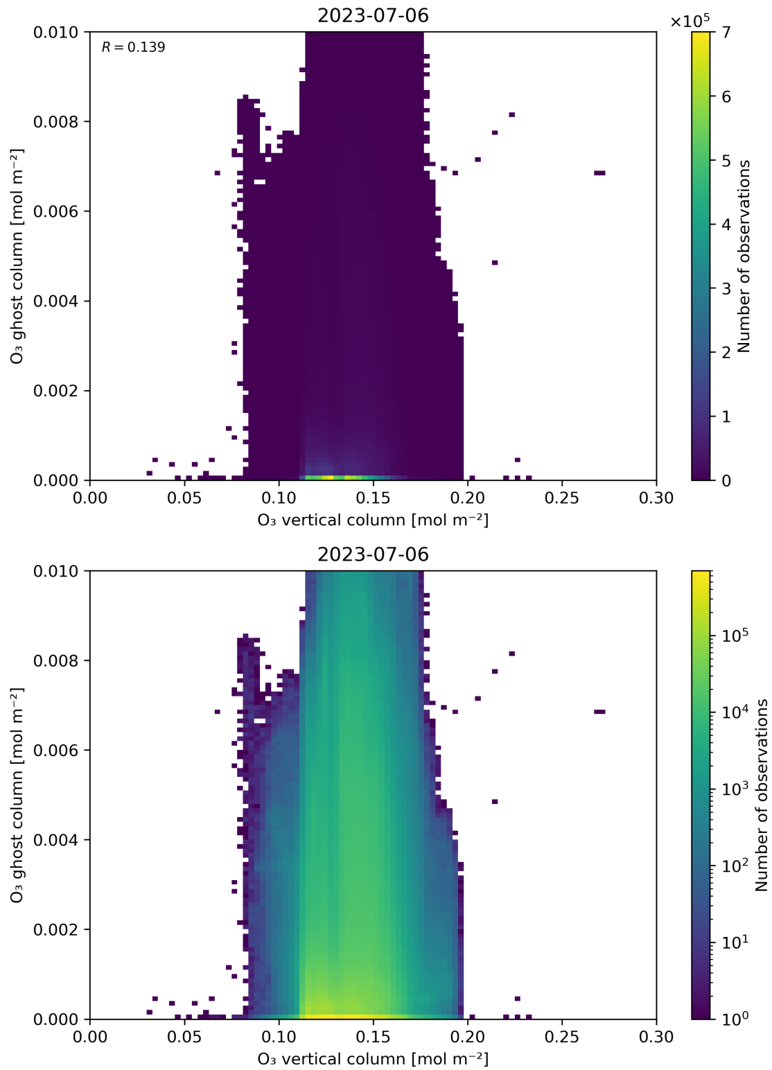
Figure 40: Scatter density plot of “O 3 vertical column” against “O 3 ghost column” for 2023-07-05 to 2023-07-07.
