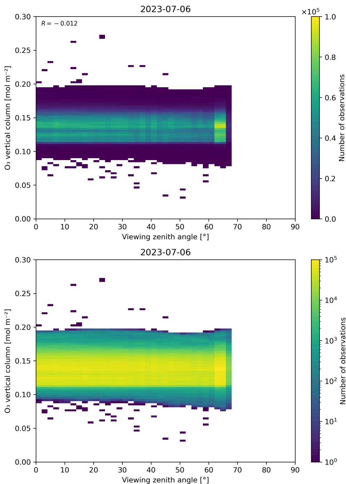
Figure 52: Scatter density plot of “Viewing zenith angle” against “O 3 vertical column” for 2023-07-05 to 2023-07-07.
