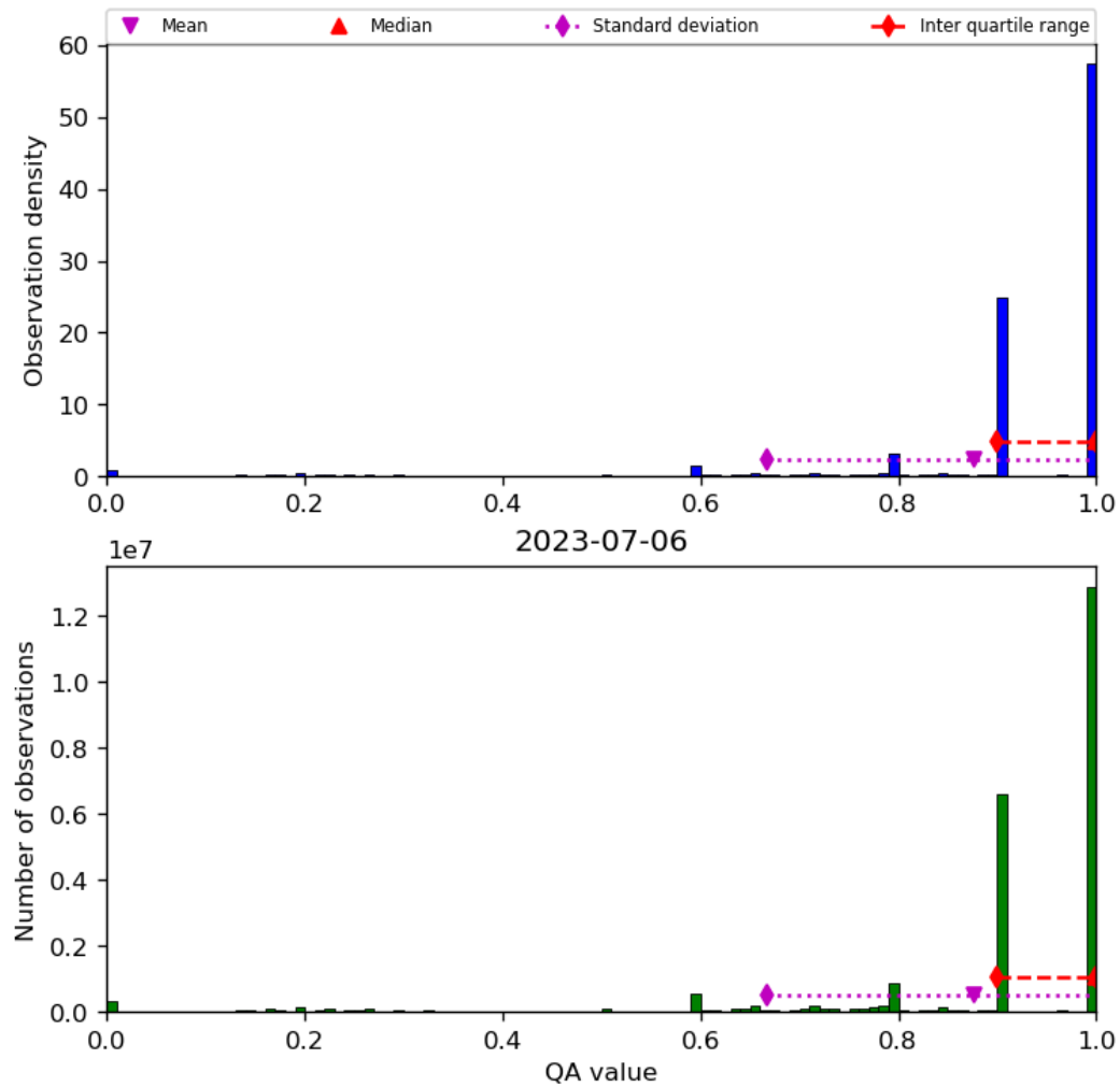
Figure 20: Histogram of “QA value” for 2023-07-05 to 2023-07-07
