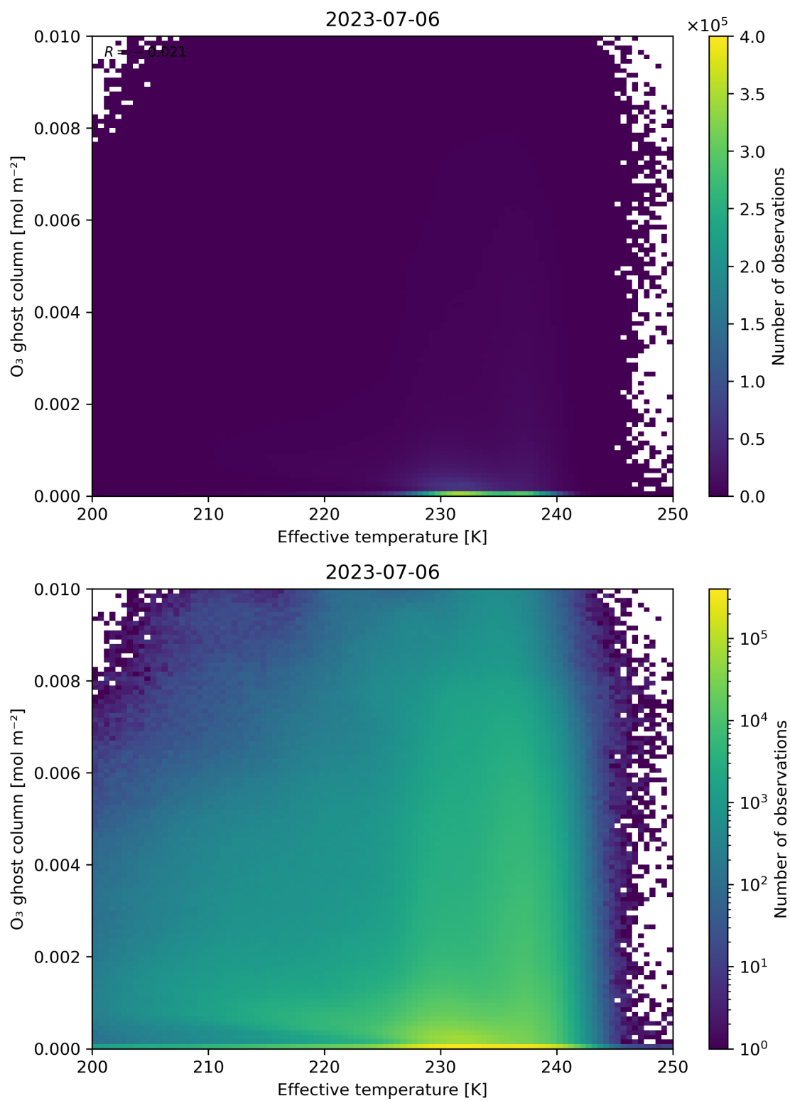
Figure 38: Scatter density plot of “Effective temperature” against “O 3 ghost column” for 2023-07-05 to 2023-07-07.
