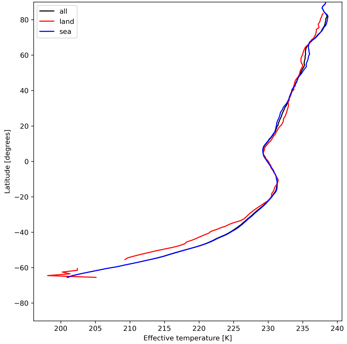
Figure 17: Zonal average of "Effective temperature" for 2023-07-05 to 2023-07-07.
