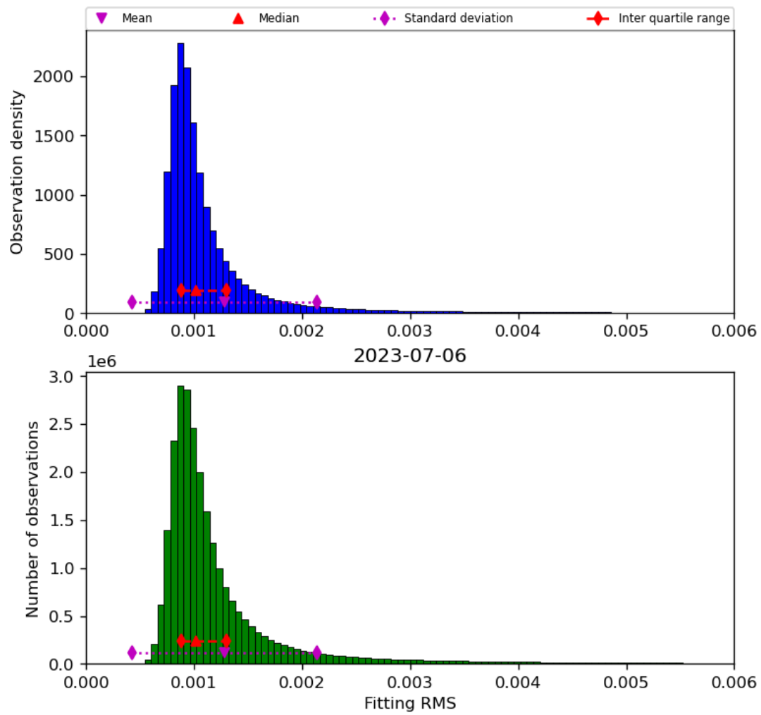
Figure 23: Histogram of “Fitting RMS” for 2023-07-05 to 2023-07-07
