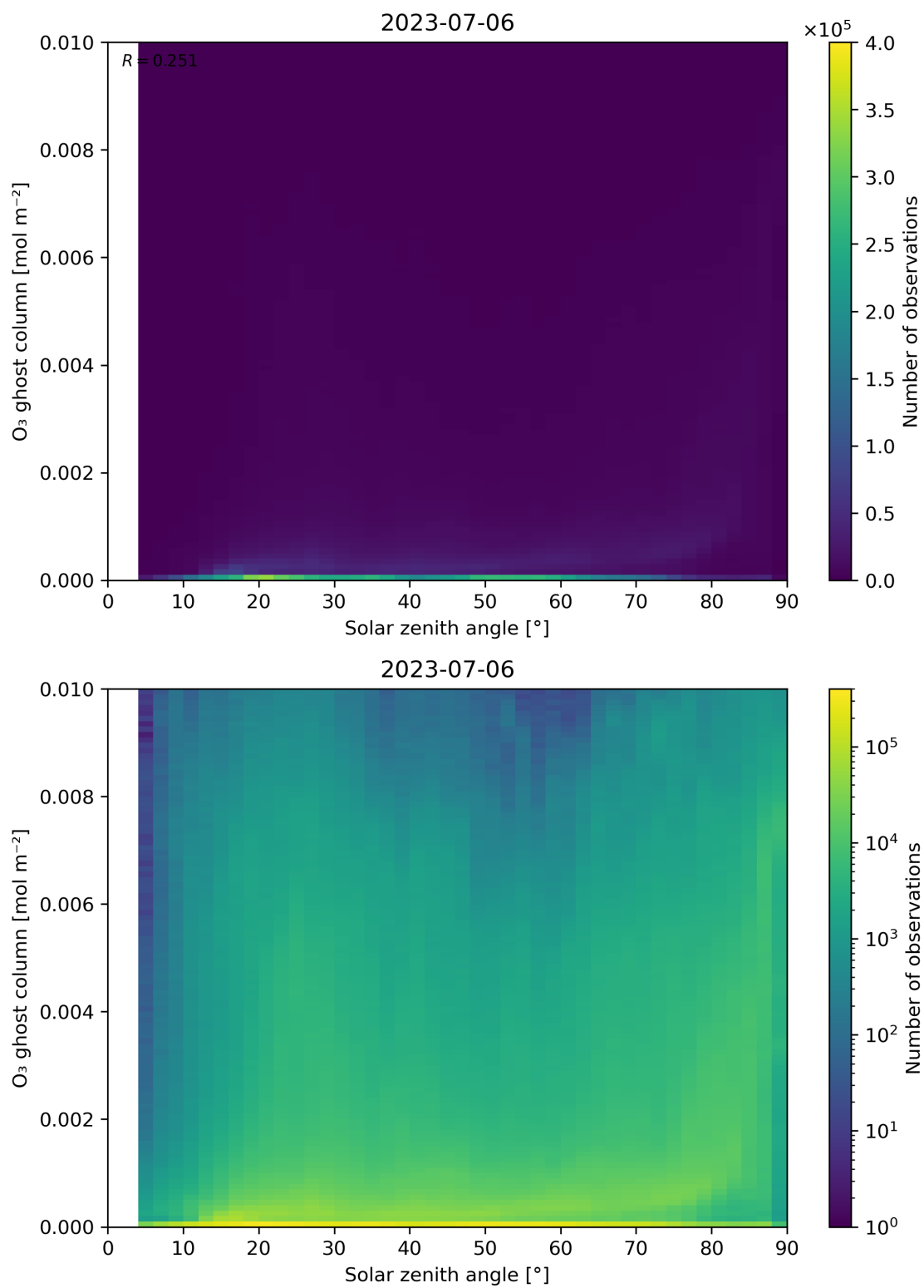
Figure 46: Scatter density plot of “Solar zenith angle” against “O 3 ghost column” for 2023-07-05 to 2023-07-07.
