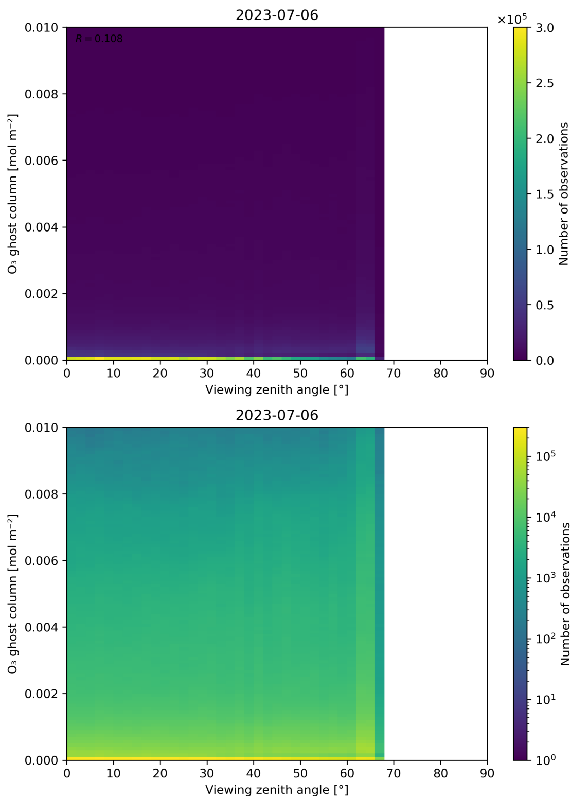
Figure 51: Scatter density plot of “Viewing zenith angle” against “O 3 ghost column” for 2023-07-05 to 2023-07-07.
