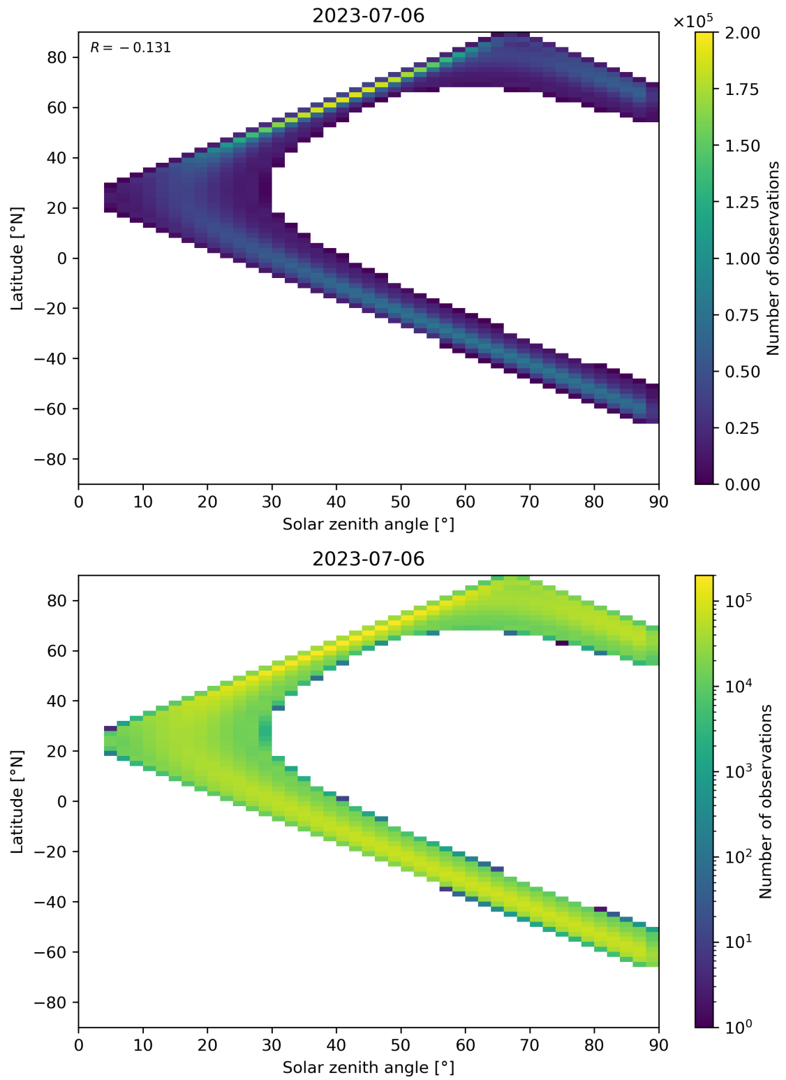
Figure 44: Scatter density plot of “Solar zenith angle” against “Latitude” for 2023-07-05 to 2023-07-07.
