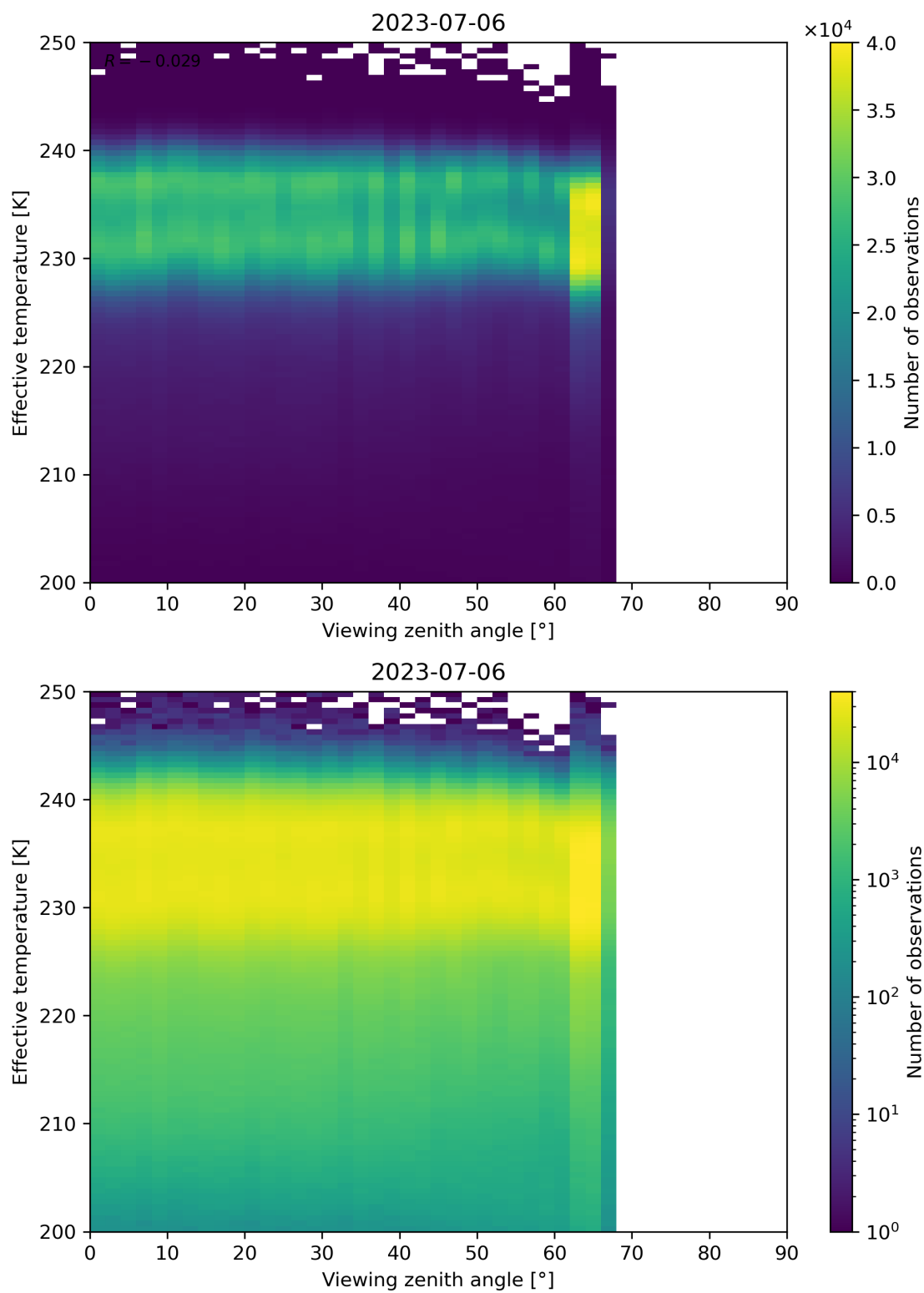
Figure 50: Scatter density plot of “Viewing zenith angle” against “Effective temperature” for 2023-07-05 to 2023-07-07.
