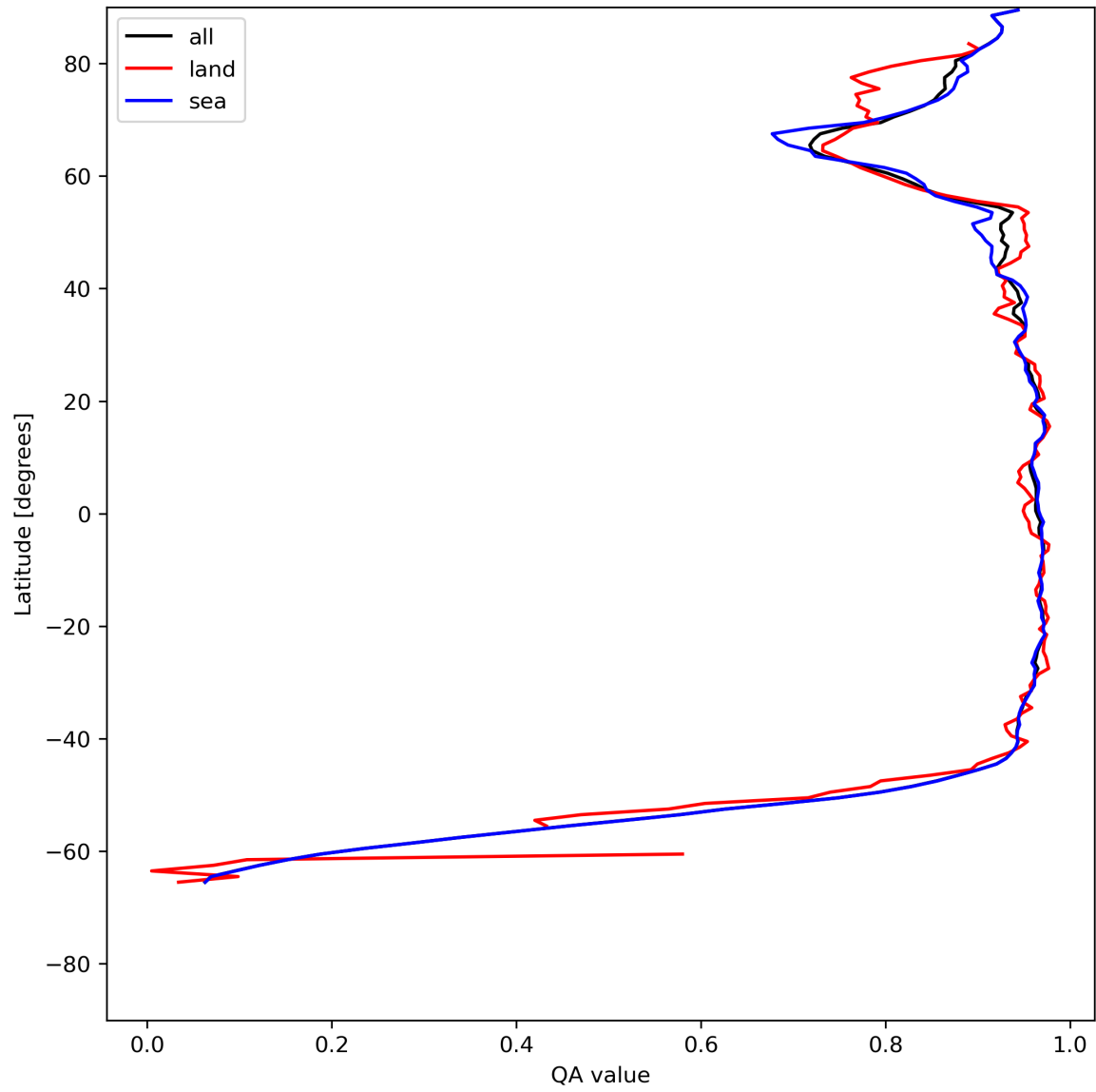
Figure 13: Zonal average of “QA value” for 2023-07-05 to 2023-07-07.
