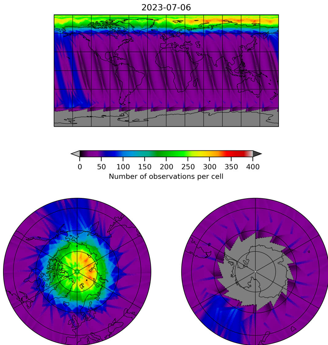
Figure 12: Map of the number of observations for 2023-07-05 to 2023-07-07
