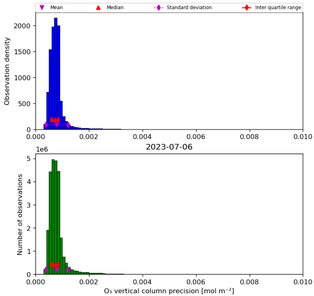
Figure 22: Histogram of “O 3 vertical column precision” for 2023-07-05 to 2023-07-07
