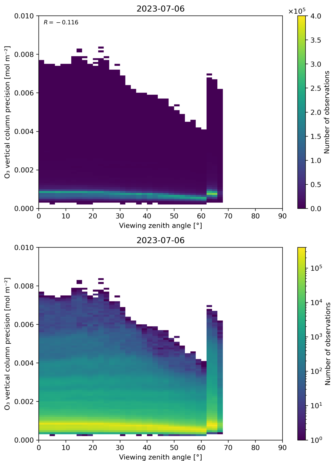
Figure 53: Scatter density plot of “Viewing zenith angle” against “O 3 vertical column precision” for 2023-07-05 to 2023-07-07.
