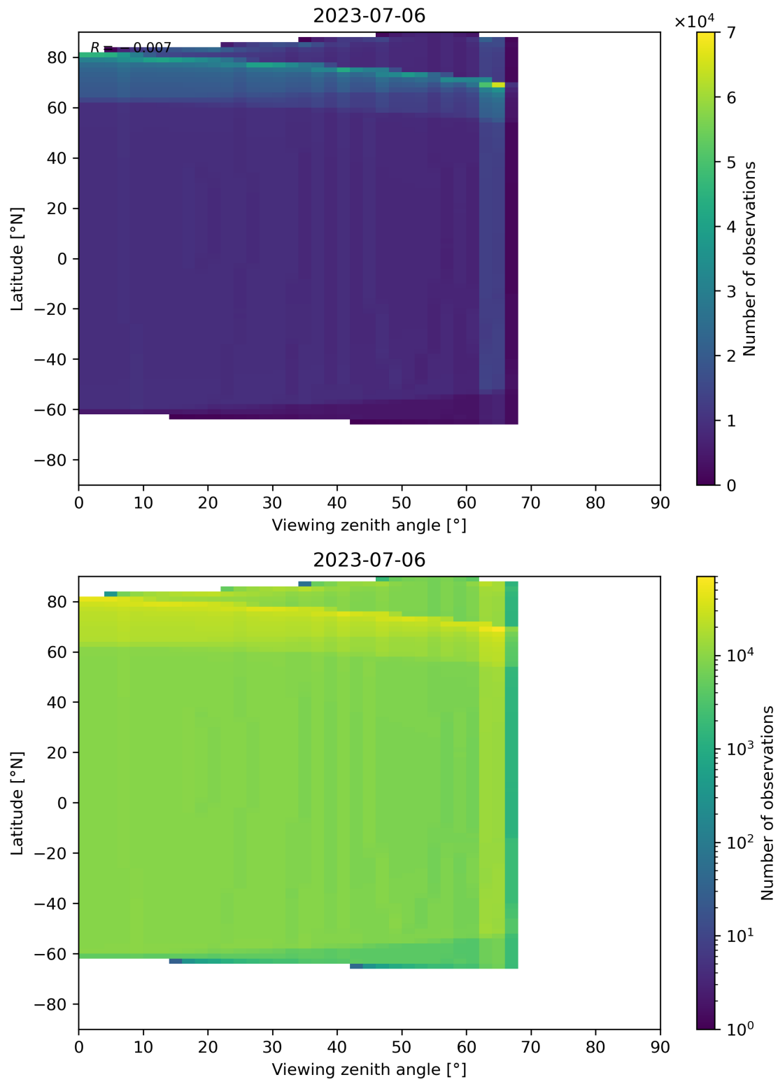
Figure 49: Scatter density plot of “Viewing zenith angle” against “Latitude” for 2023-07-05 to 2023-07-07.
