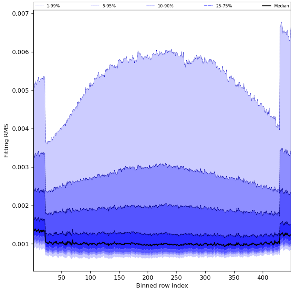
Figure 30: Along track statistics of “Fitting RMS” for 2023-07-05 to 2023-07-07
