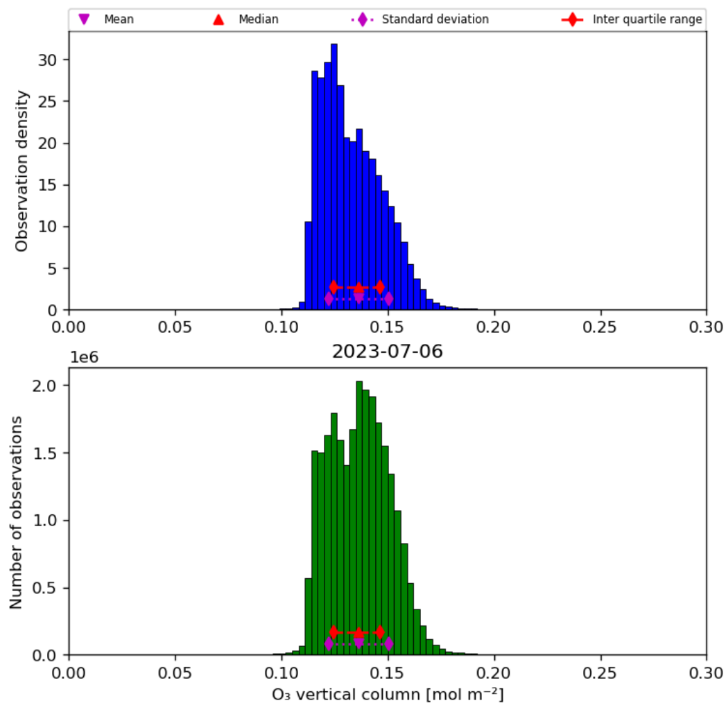
Figure 21: Histogram of “O 3 vertical column” for 2023-07-05 to 2023-07-07
