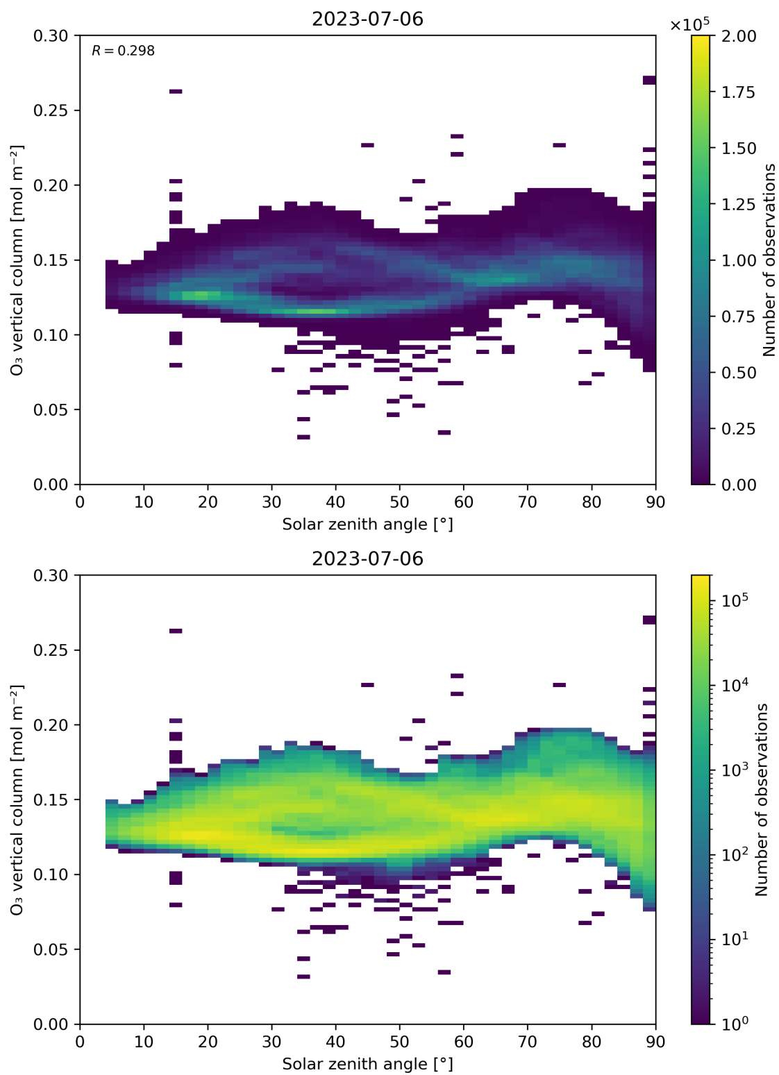
Figure 47: Scatter density plot of “Solar zenith angle” against “O 3 vertical column” for 2023-07-05 to 2023-07-07.
