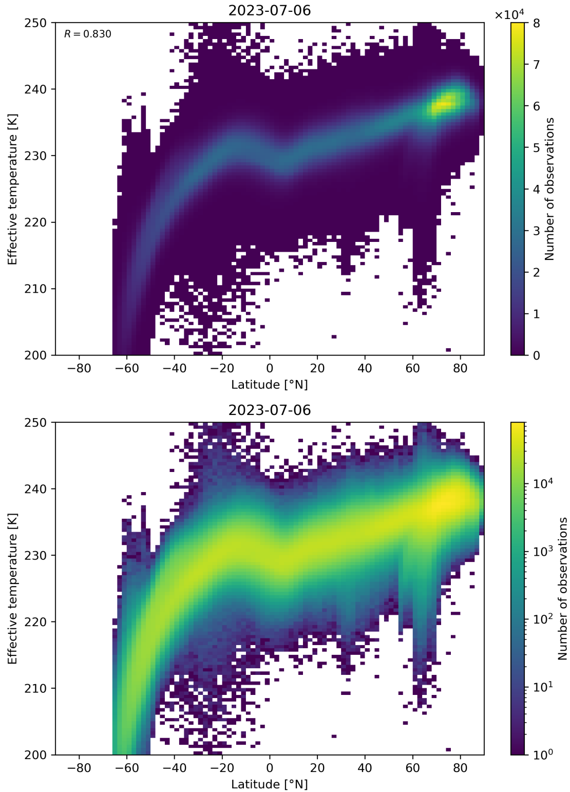
Figure 34: Scatter density plot of “Latitude” against “Effective temperature” for 2023-07-05 to 2023-07-07.
