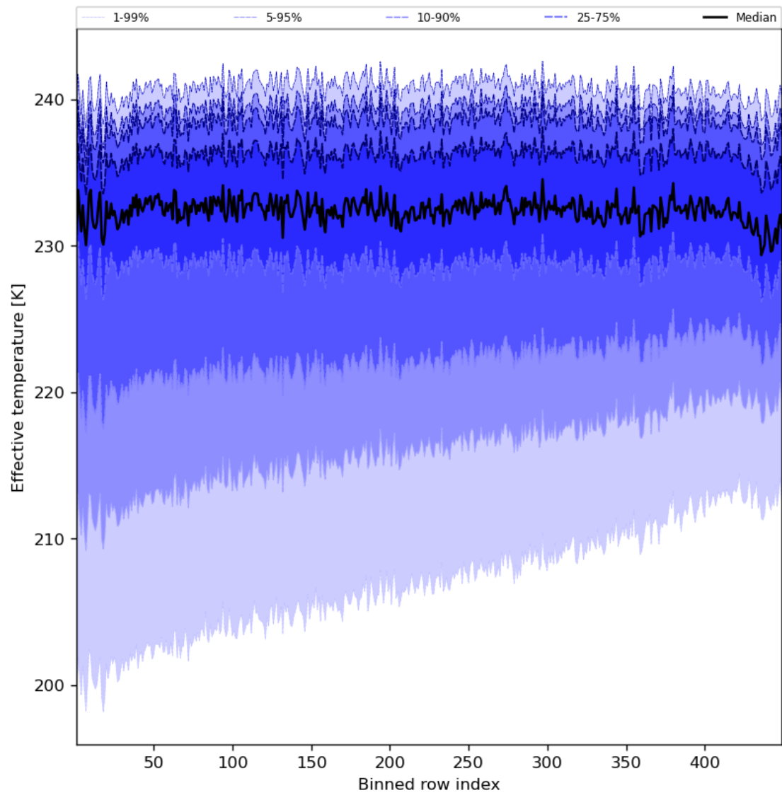
Figure 31: Along track statistics of “Effective temperature” for 2023-07-05 to 2023-07-07
