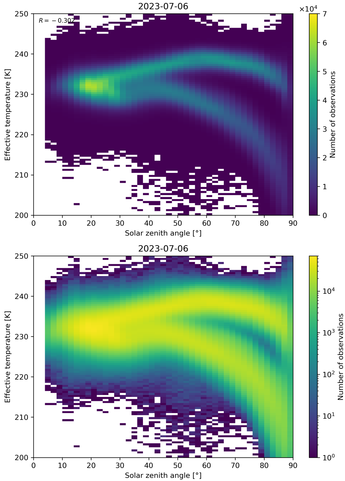
Figure 45: Scatter density plot of “Solar zenith angle” against “Effective temperature” for 2023-07-05 to 2023-07-07.
