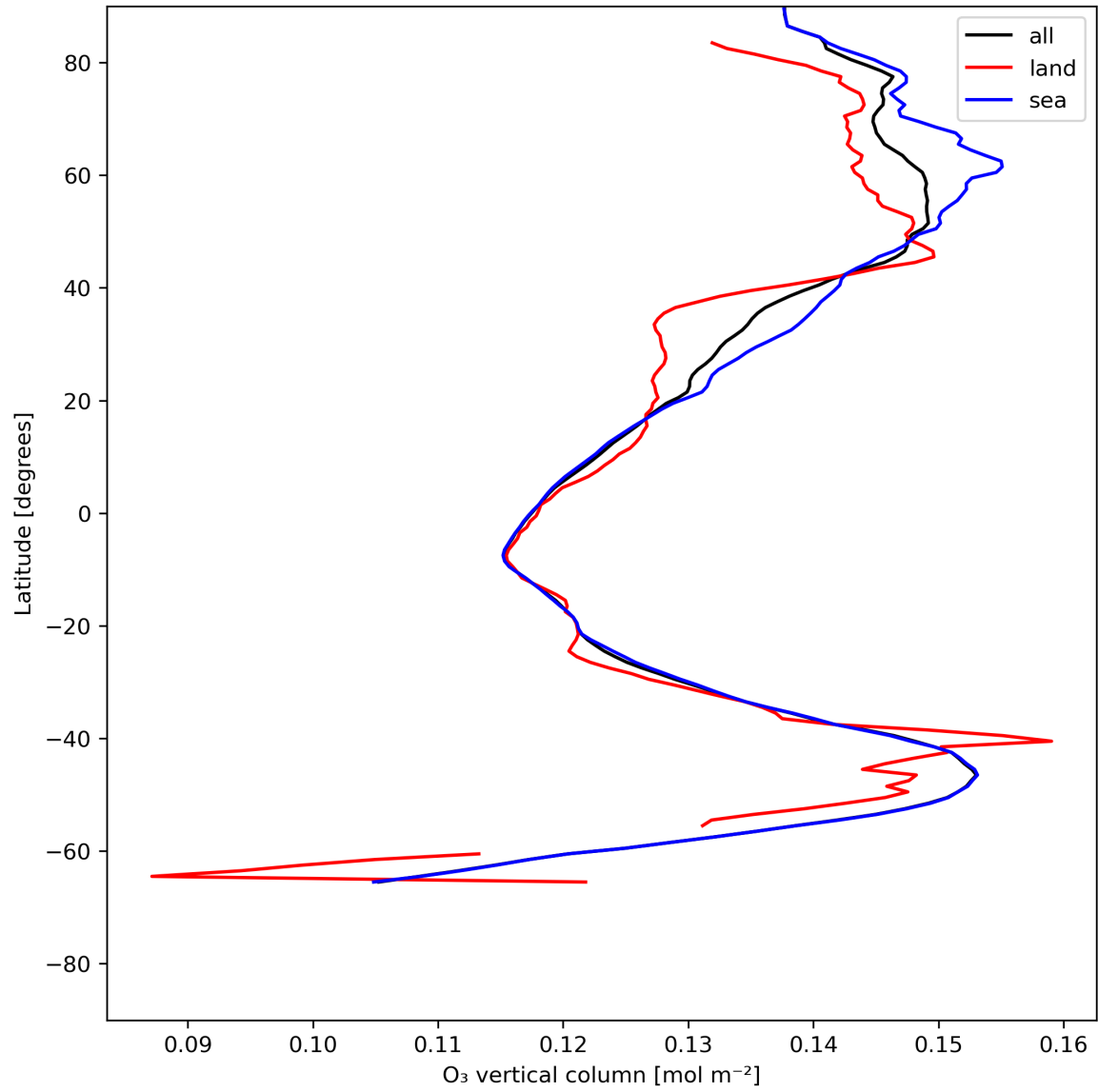
Figure 14: Zonal average of “O 3 vertical column” for 2023-07-05 to 2023-07-07.
