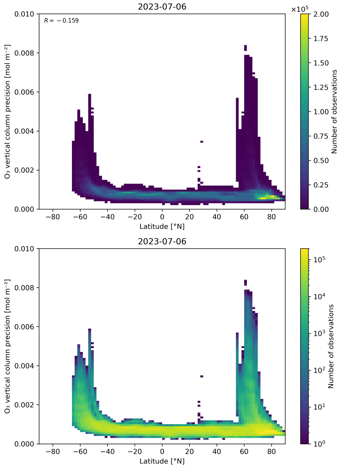
Figure 37: Scatter density plot of “Latitude” against “O 3 vertical column precision” for 2023-07-05 to 2023-07-07.
