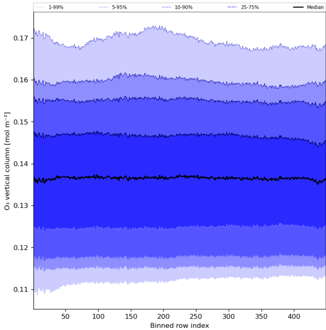
Figure 28: Along track statistics of “O 3 vertical column” for 2023-07-05 to 2023-07-07
