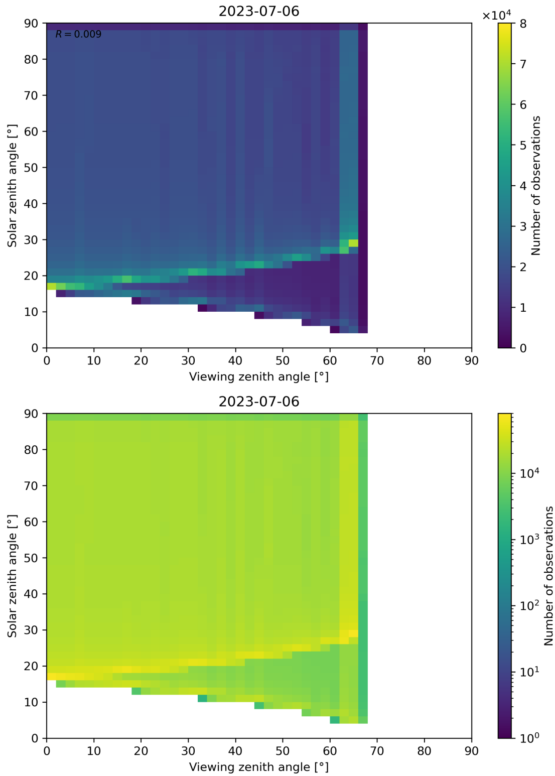
Figure 54: Scatter density plot of “Viewing zenith angle” against “Solar zenith angle” for 2023-07-05 to 2023-07-07.
