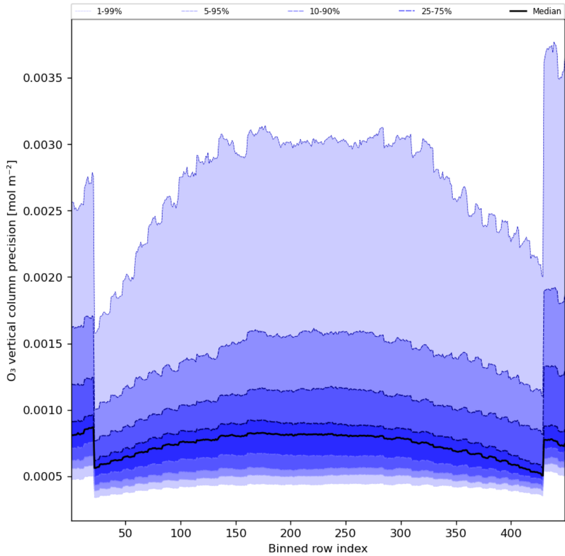
Figure 29: Along track statistics of “O 3 vertical column precision” for 2023-07-05 to 2023-07-07
