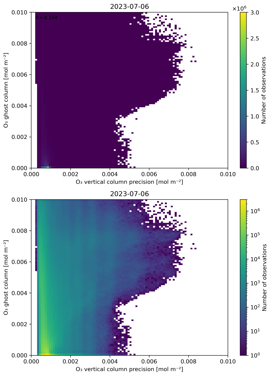
Figure 43: Scatter density plot of “ \text{O}_3 vertical column precision” against “ \text{O}_3 ghost column” for 2023-07-05 to 2023-07-07.
