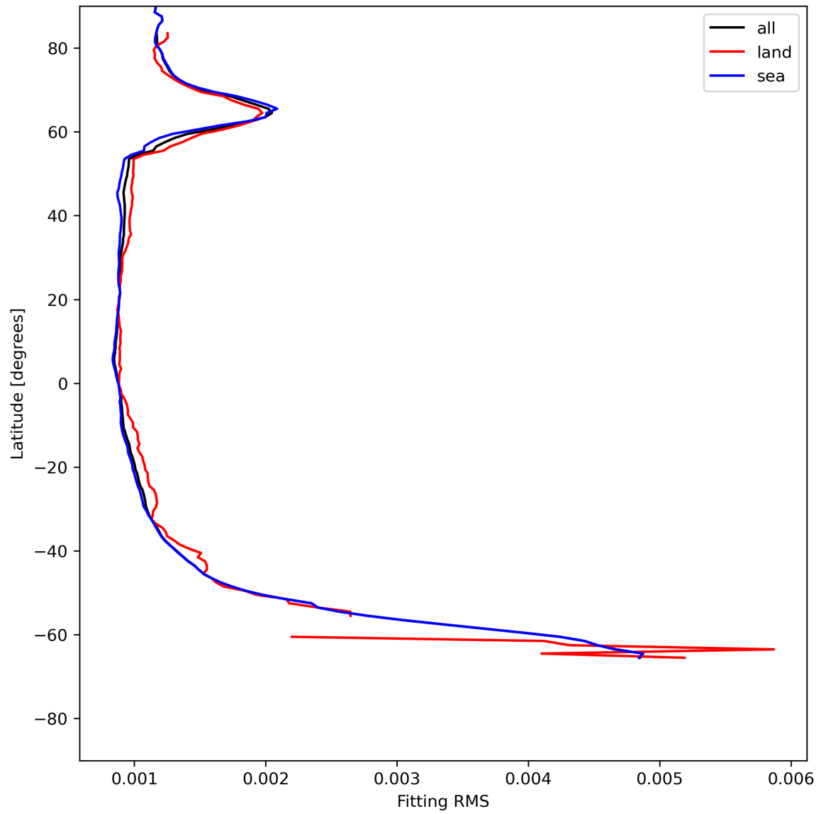
Figure 16: Zonal average of “Fitting RMS” for 2023-07-05 to 2023-07-07.
