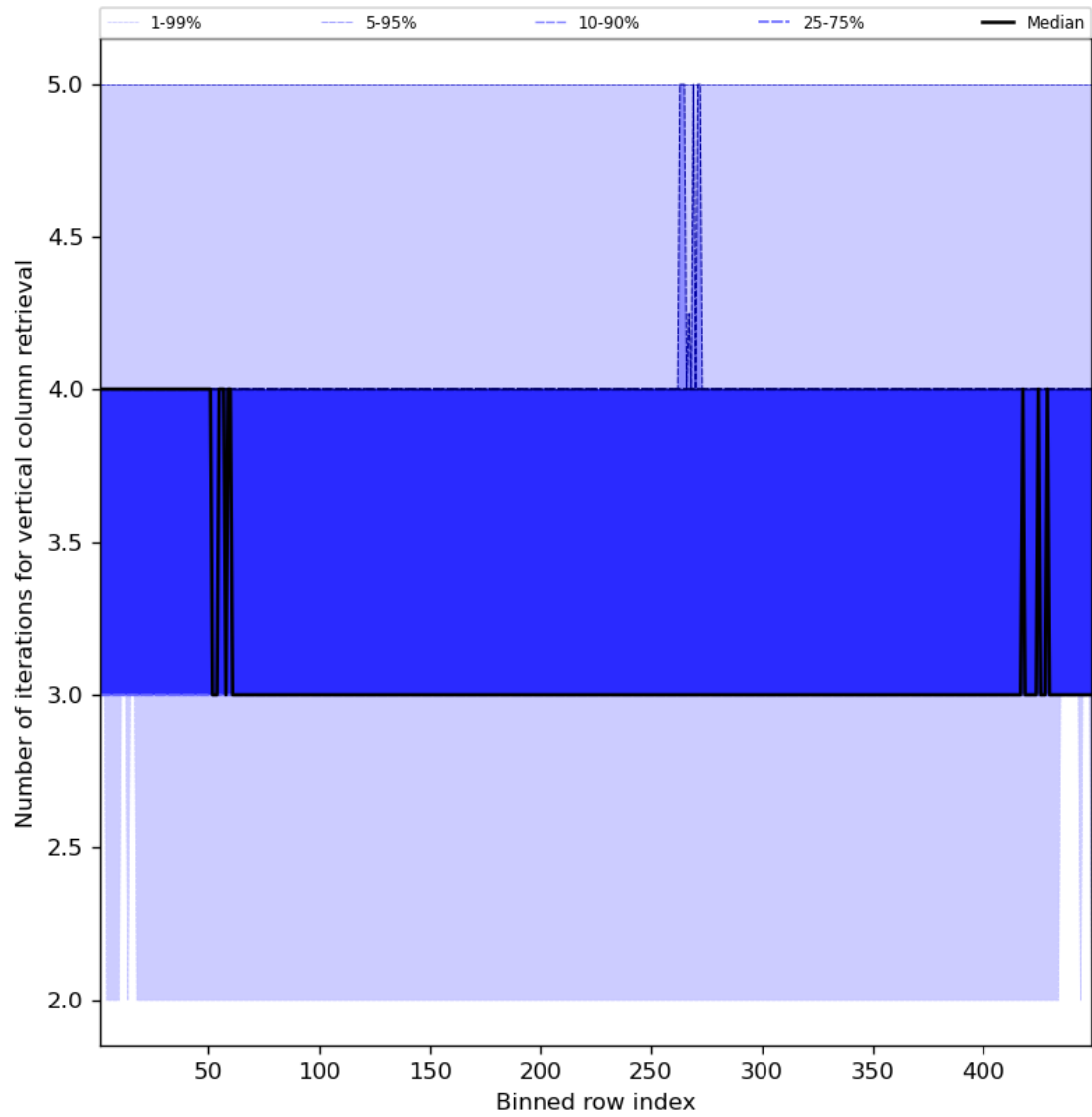
Figure 33: Along track statistics of “Number of iterations for vertical column retrieval” for 2023-07-05 to 2023-07-07
