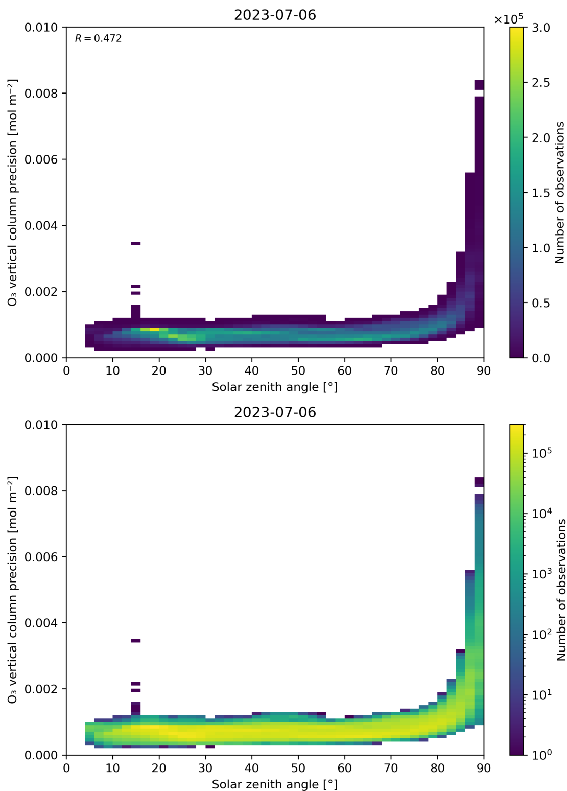
Figure 48: Scatter density plot of “Solar zenith angle” against “O 3 vertical column precision” for 2023-07-05 to 2023-07-07.
