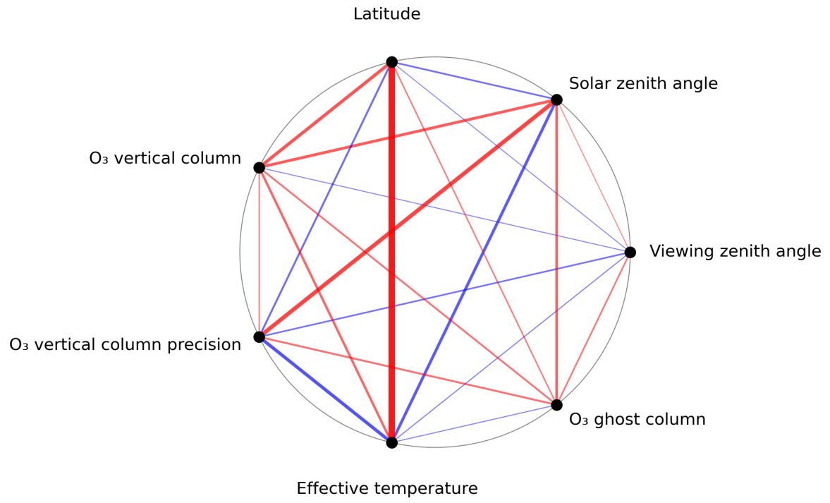
Figure 1: Map of correlation graph for 2023-07-05 to 2023-07-07.
