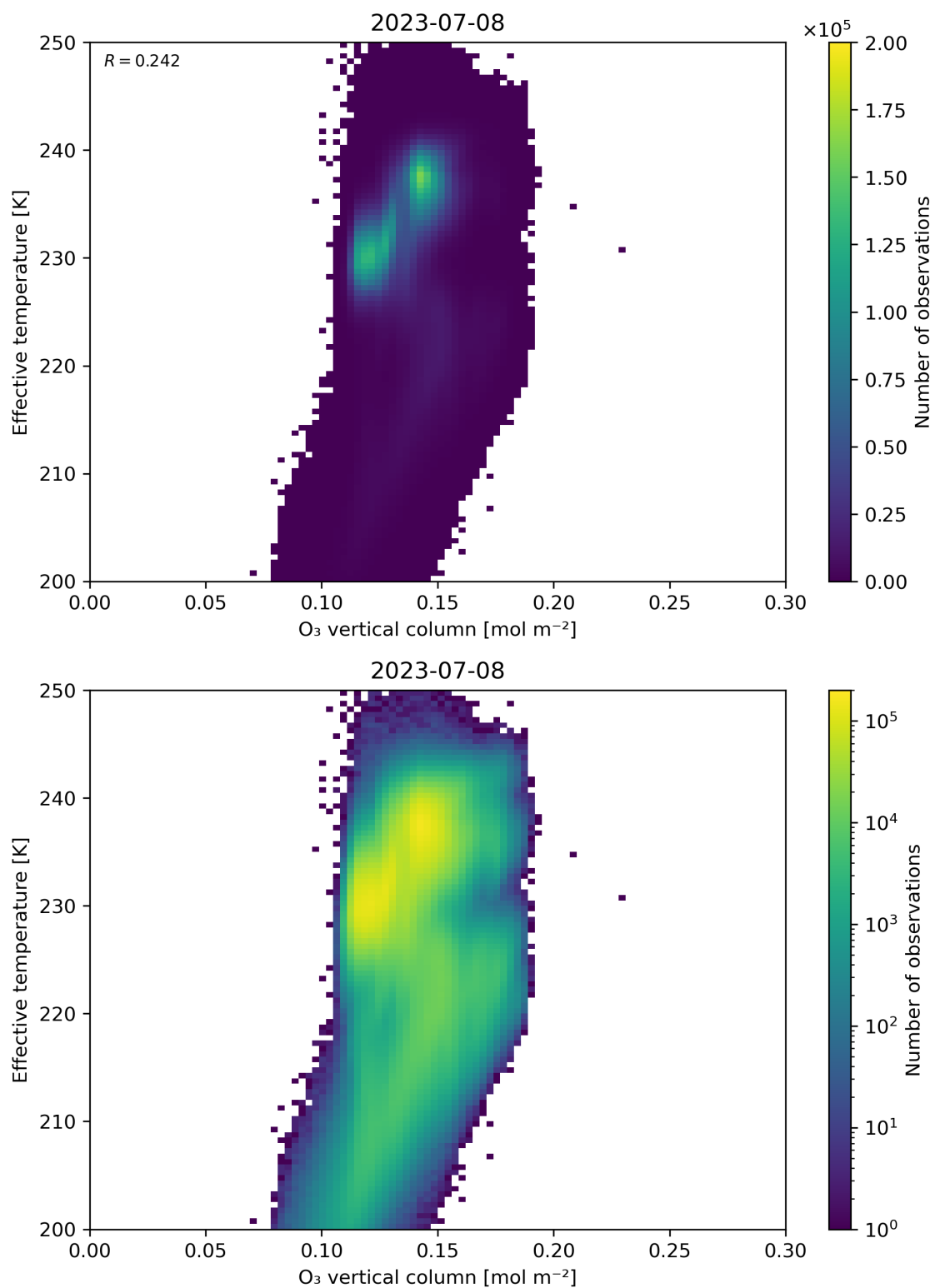
Figure 39: Scatter density plot of “O 3 vertical column” against “Effective temperature” for 2023-07-08 to 2023-07-09.
