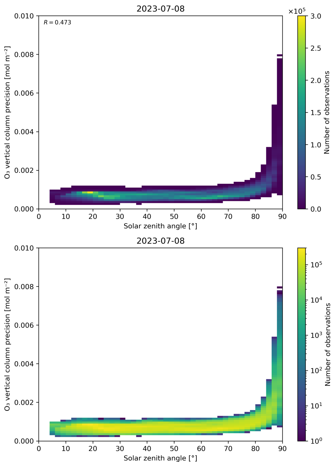
Figure 48: Scatter density plot of “Solar zenith angle” against “O 3 vertical column precision” for 2023-07-08 to 2023-07-09.
