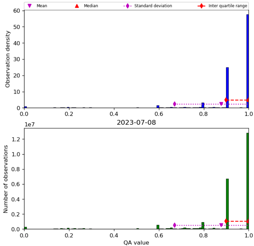
Figure 20: Histogram of “QA value” for 2023-07-08 to 2023-07-09
