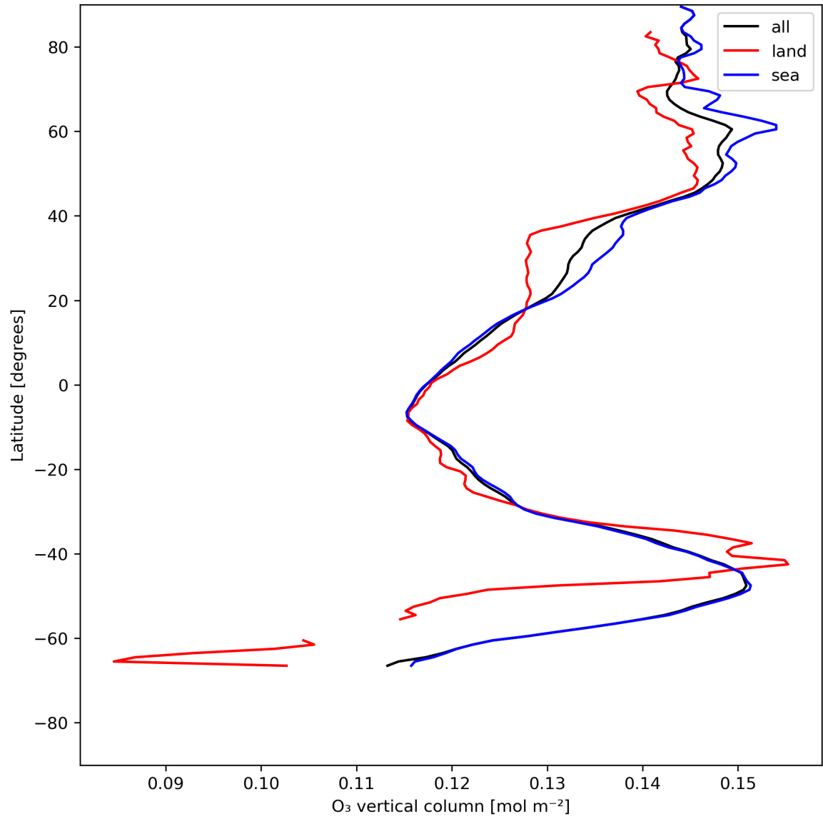
Figure 14: Zonal average of “O 3 vertical column” for 2023-07-08 to 2023-07-09.
