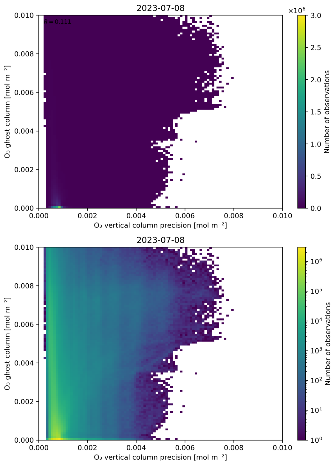
Figure 43: Scatter density plot of “O 3 vertical column precision” against “O 3 ghost column” for 2023-07-08 to 2023-07-09.
