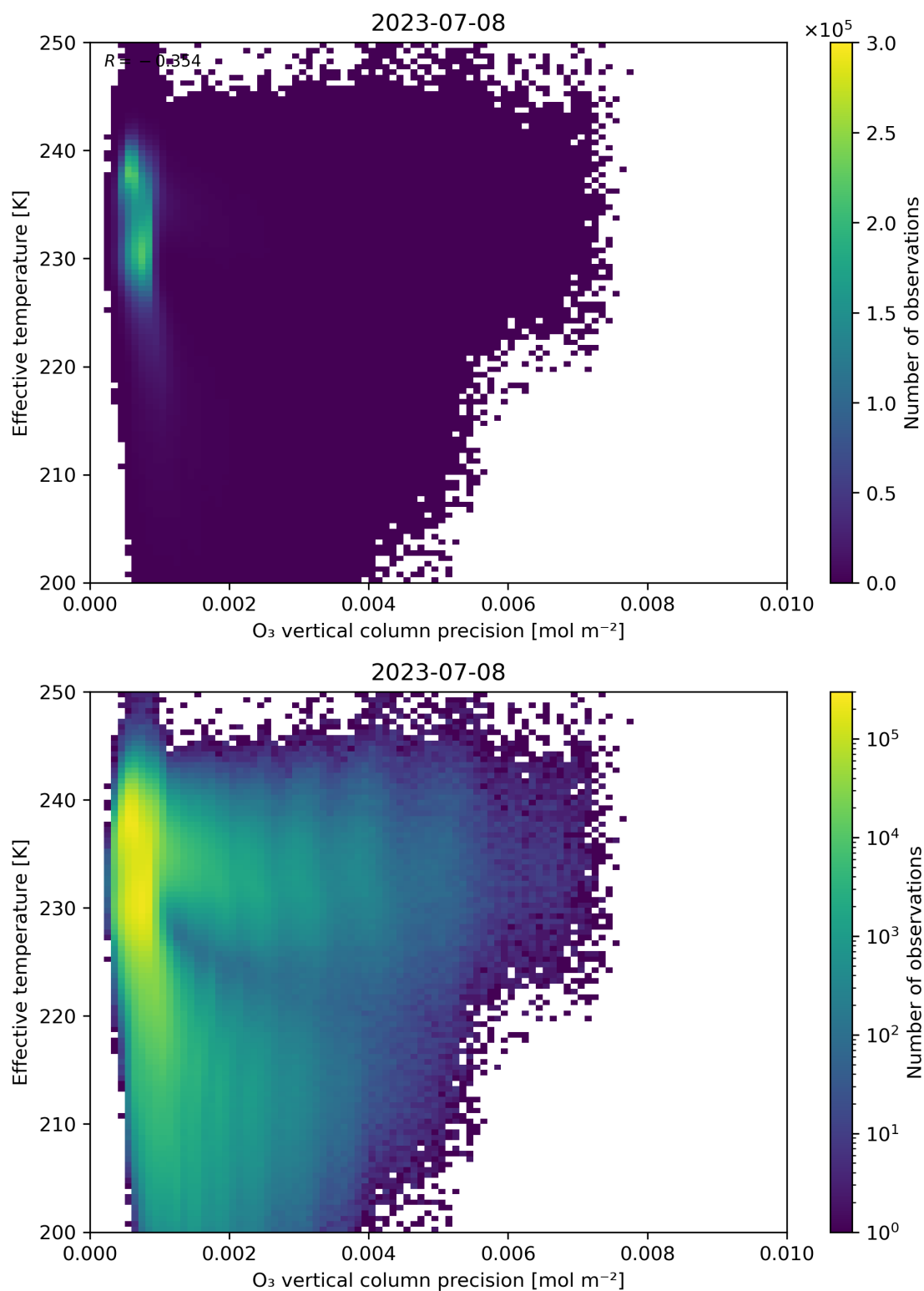
Figure 42: Scatter density plot of “O 3 vertical column precision” against “Effective temperature” for 2023-07-08 to 2023-07-09.
