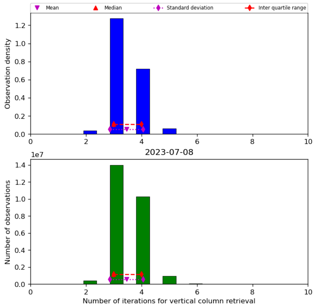
Figure 26: Histogram of “Number of iterations for vertical column retrieval” for 2023-07-08 to 2023-07-09
