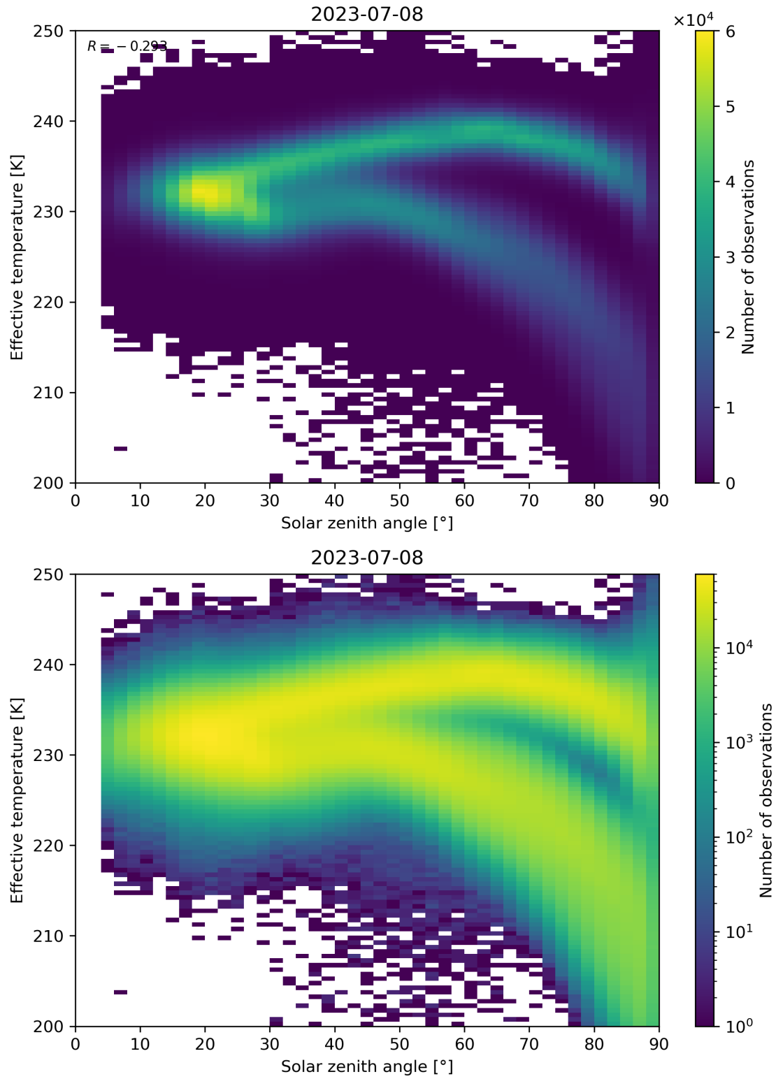
Figure 45: Scatter density plot of “Solar zenith angle” against “Effective temperature” for 2023-07-08 to 2023-07-09.
