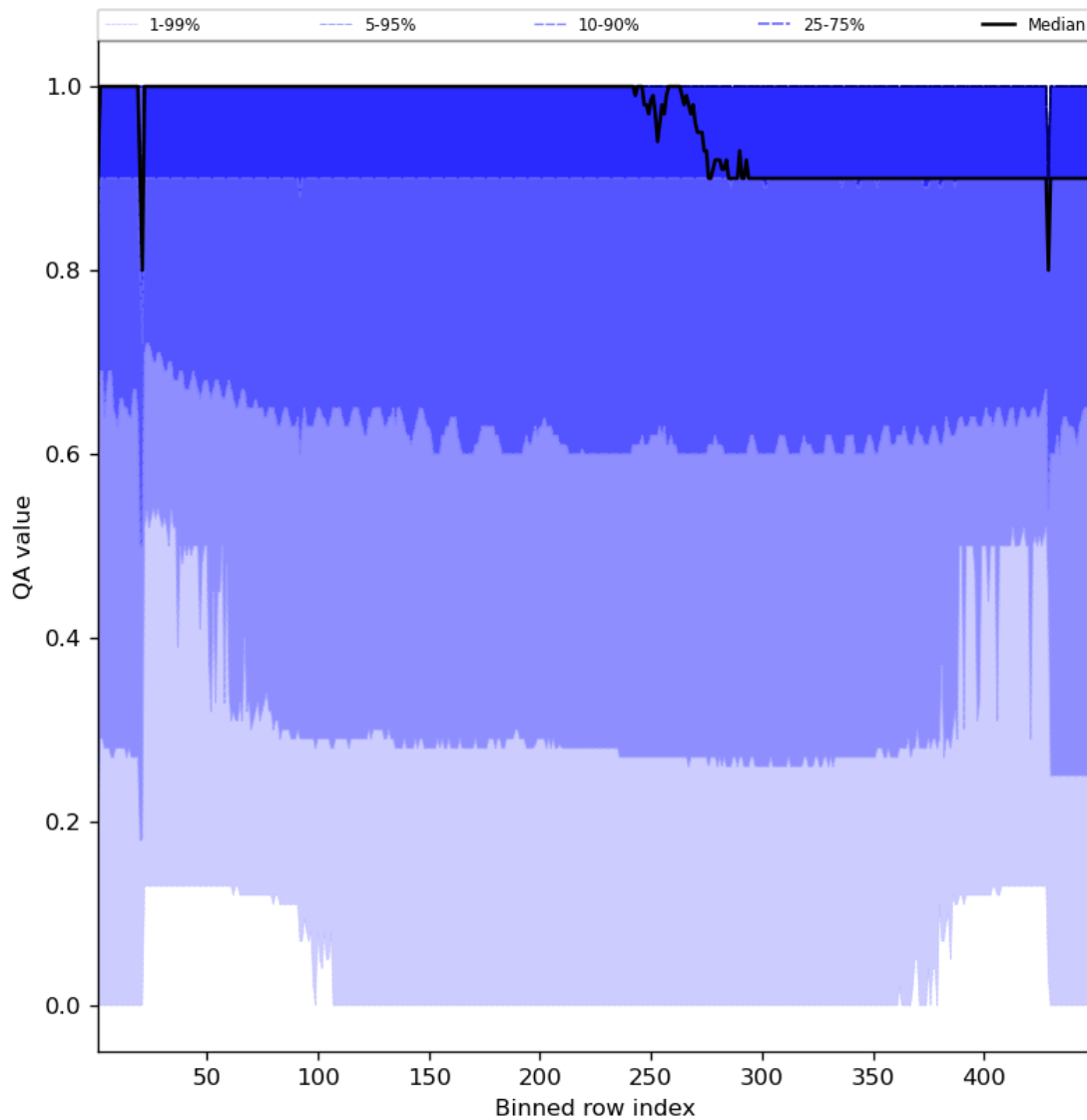
Figure 27: Along track statistics of “QA value” for 2023-07-08 to 2023-07-09
