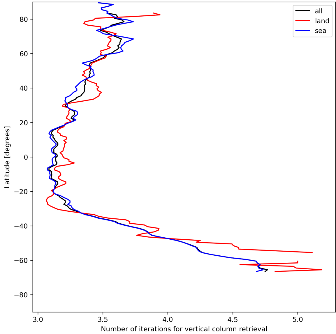
Figure 19: Zonal average of “Number of iterations for vertical column retrieval” for 2023-07-08 to 2023-07-09.
