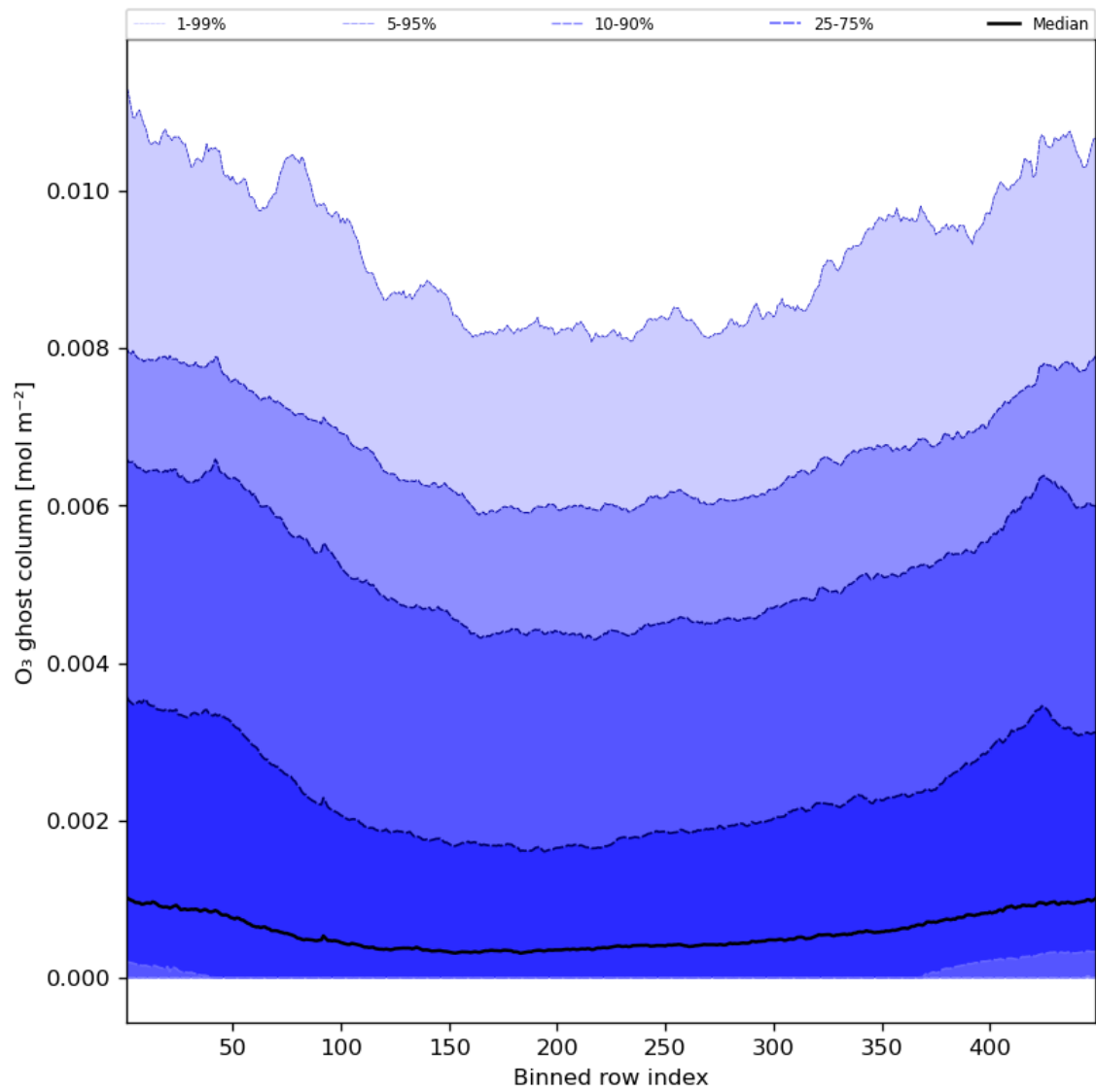
Figure 32: Along track statistics of “O 3 ghost column” for 2023-07-08 to 2023-07-09
