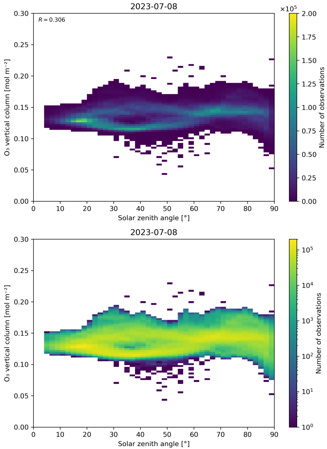
Figure 47: Scatter density plot of “Solar zenith angle” against “O 3 vertical column” for 2023-07-08 to 2023-07-09.
