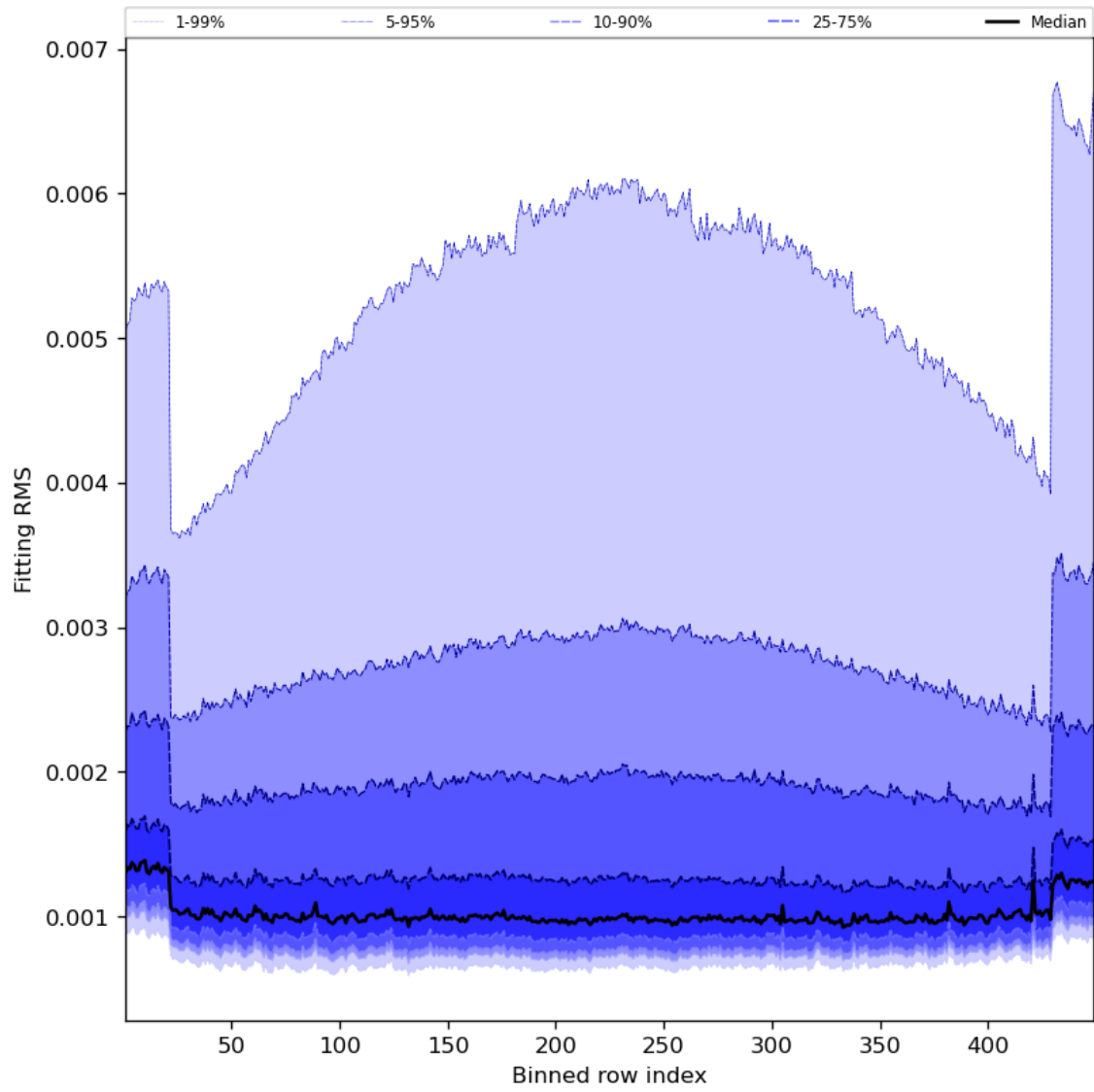
Figure 30: Along track statistics of “Fitting RMS” for 2023-07-08 to 2023-07-09
