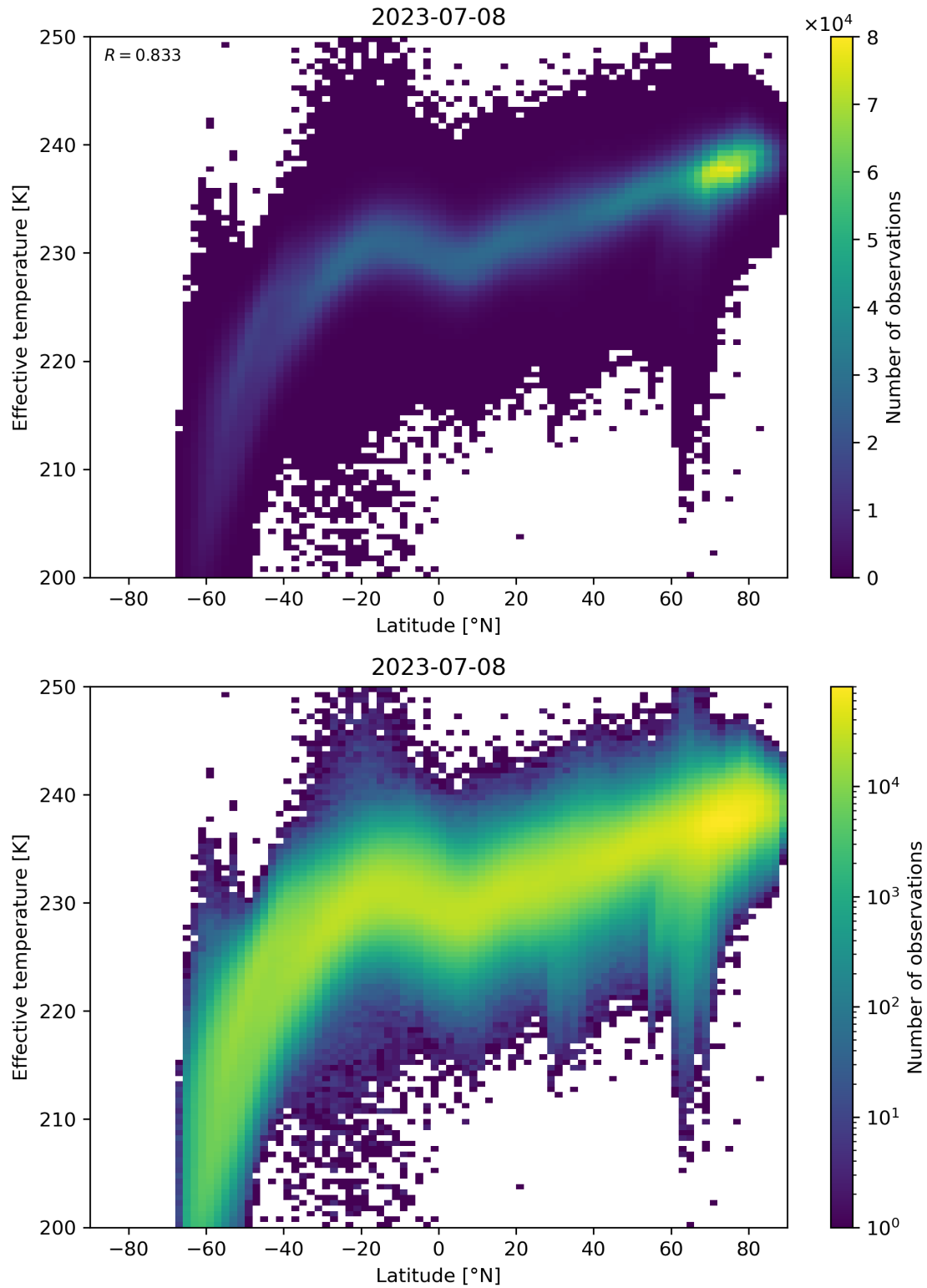
Figure 34: Scatter density plot of “Latitude” against “Effective temperature” for 2023-07-08 to 2023-07-09.
