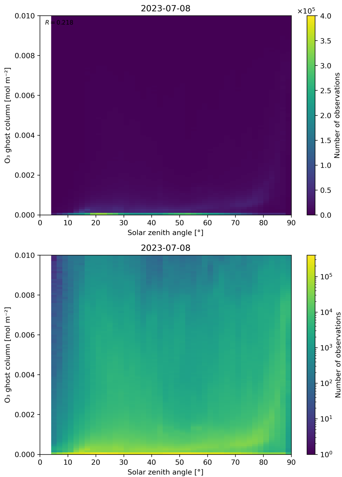
Figure 46: Scatter density plot of “Solar zenith angle” against “O 3 ghost column” for 2023-07-08 to 2023-07-09.
