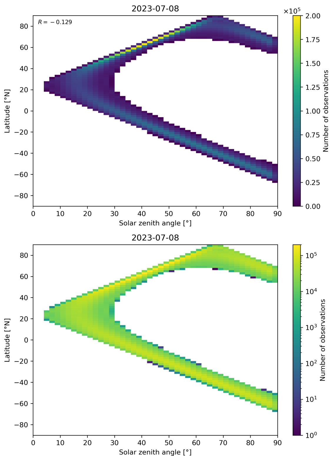
Figure 44: Scatter density plot of “Solar zenith angle” against “Latitude” for 2023-07-08 to 2023-07-09.
