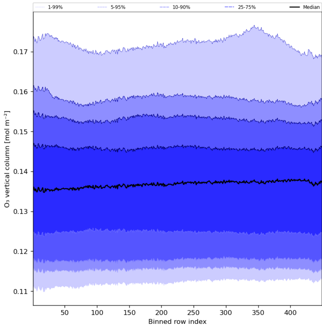
Figure 28: Along track statistics of “O 3 vertical column” for 2023-07-08 to 2023-07-09
