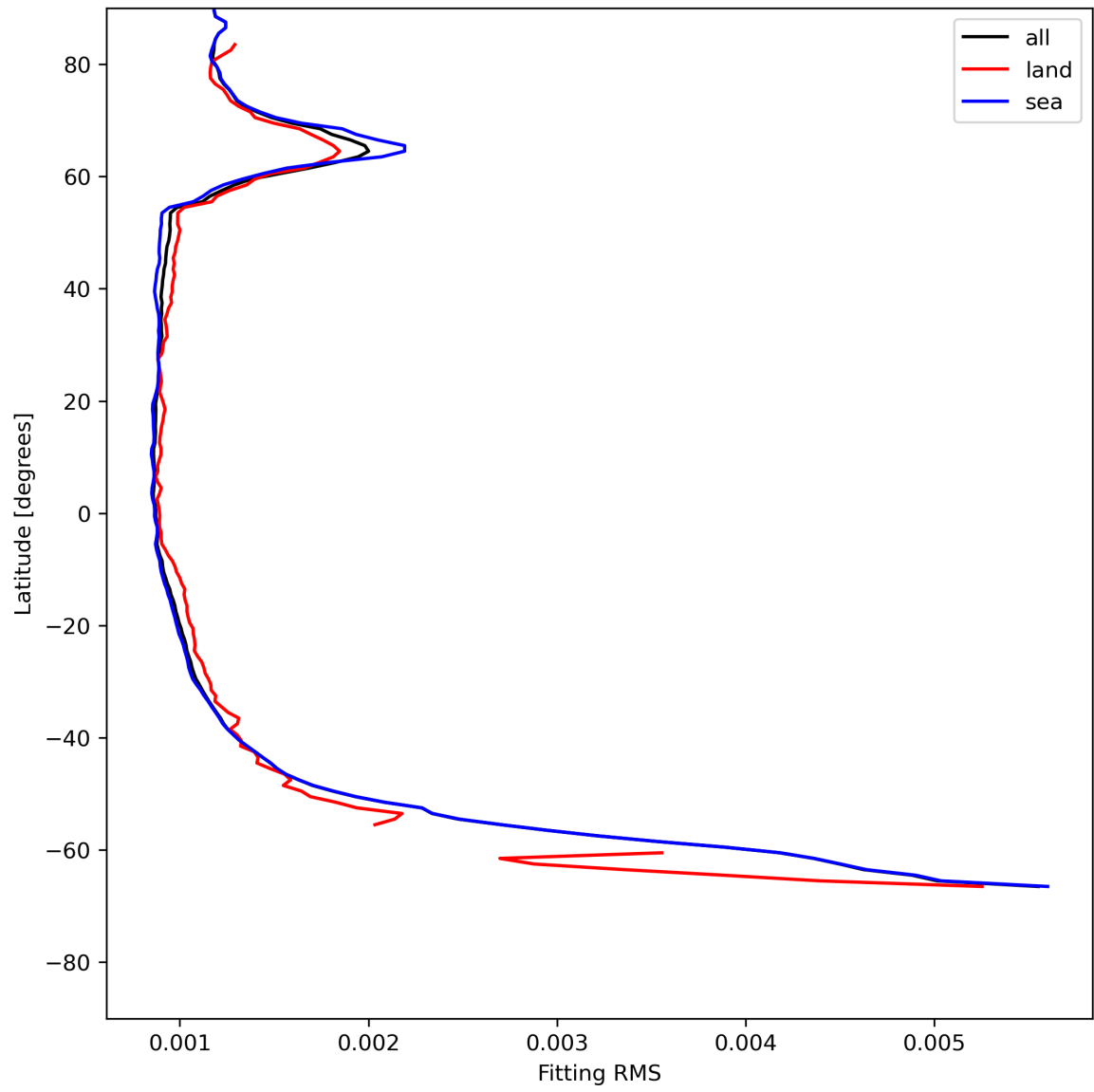
Figure 16: Zonal average of “Fitting RMS” for 2023-07-08 to 2023-07-09.
