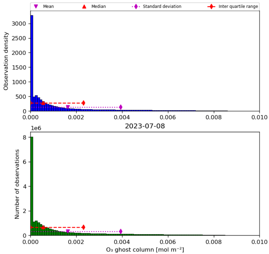
Figure 25: Histogram of “O 3 ghost column” for 2023-07-08 to 2023-07-09
