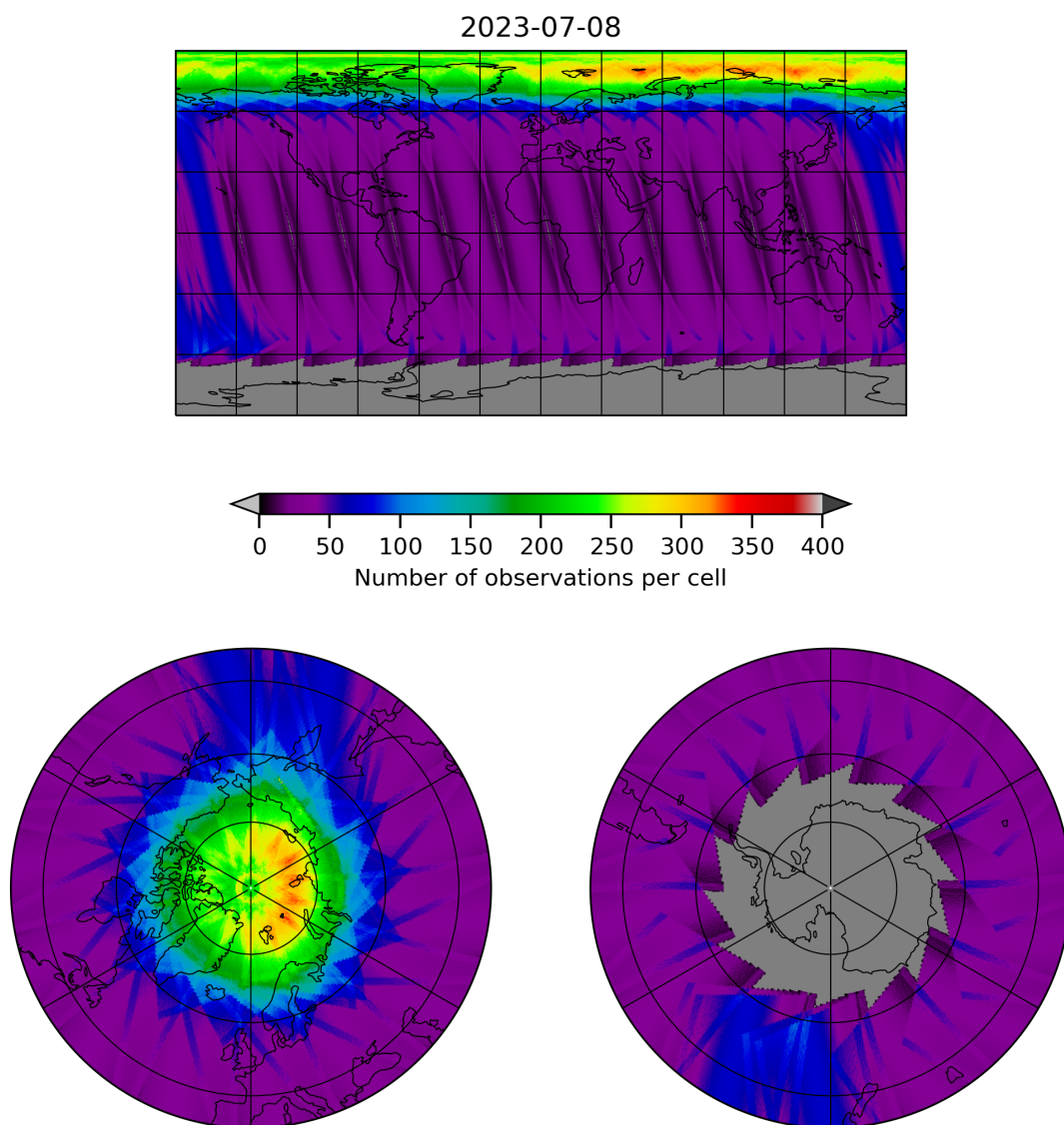
Figure 12: Map of the number of observations for 2023-07-08 to 2023-07-09
