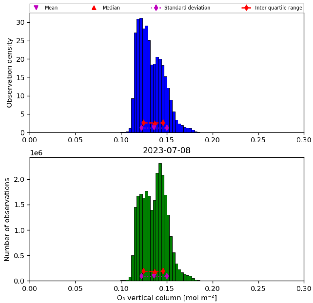
Figure 21: Histogram of “O 3 vertical column” for 2023-07-08 to 2023-07-09
