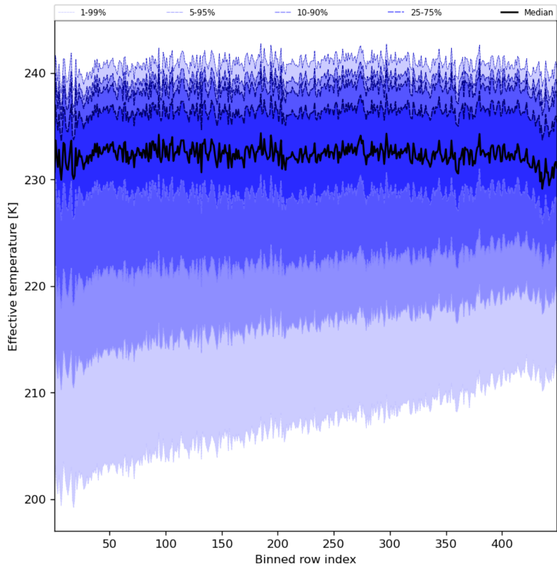
Figure 31: Along track statistics of “Effective temperature” for 2023-07-08 to 2023-07-09
