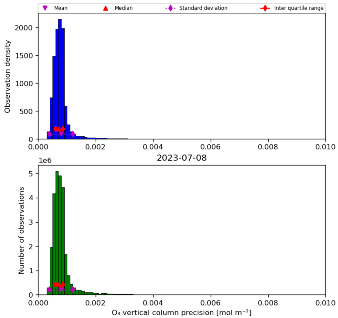
Figure 22: Histogram of “O 3 vertical column precision” for 2023-07-08 to 2023-07-09
