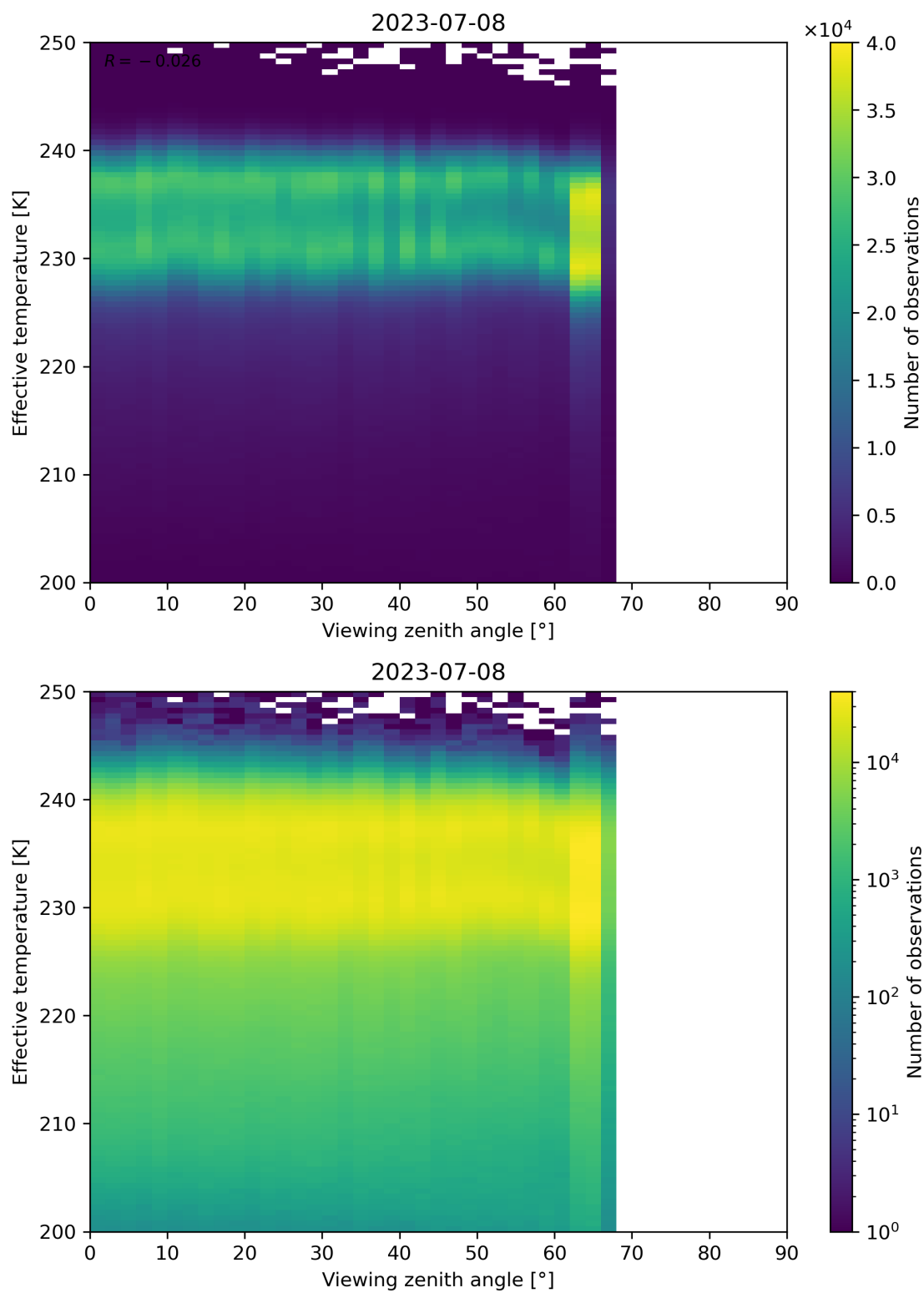
Figure 50: Scatter density plot of “Viewing zenith angle” against “Effective temperature” for 2023-07-08 to 2023-07-09.
