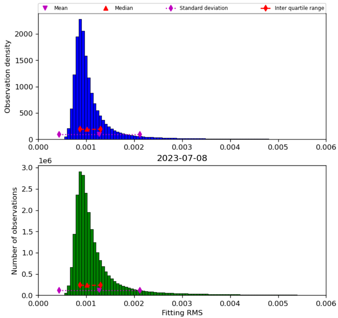
Figure 23: Histogram of “Fitting RMS” for 2023-07-08 to 2023-07-09
