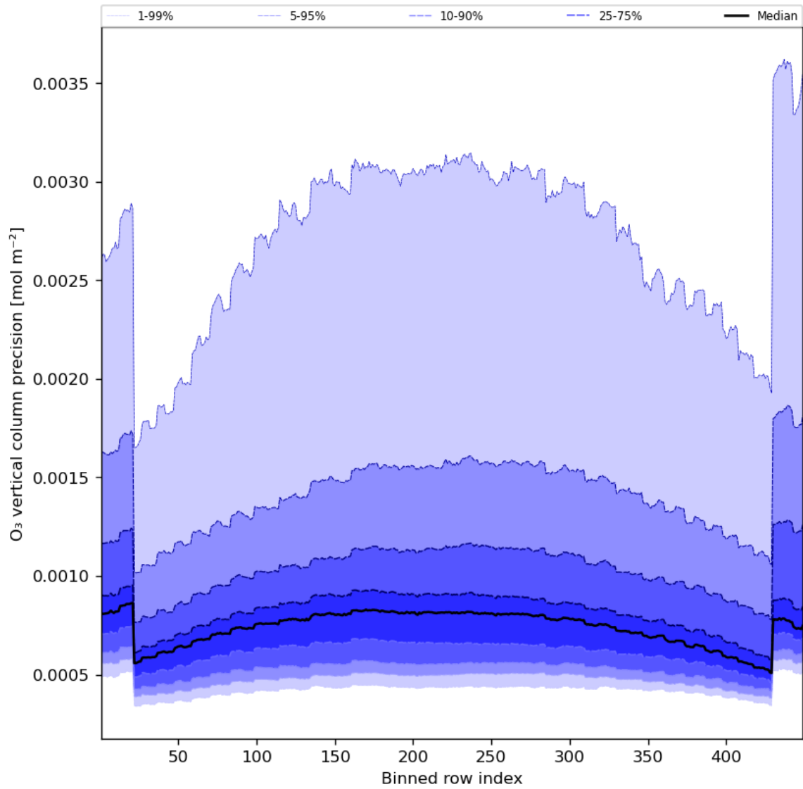
Figure 29: Along track statistics of “O 3 vertical column precision” for 2023-07-08 to 2023-07-09
