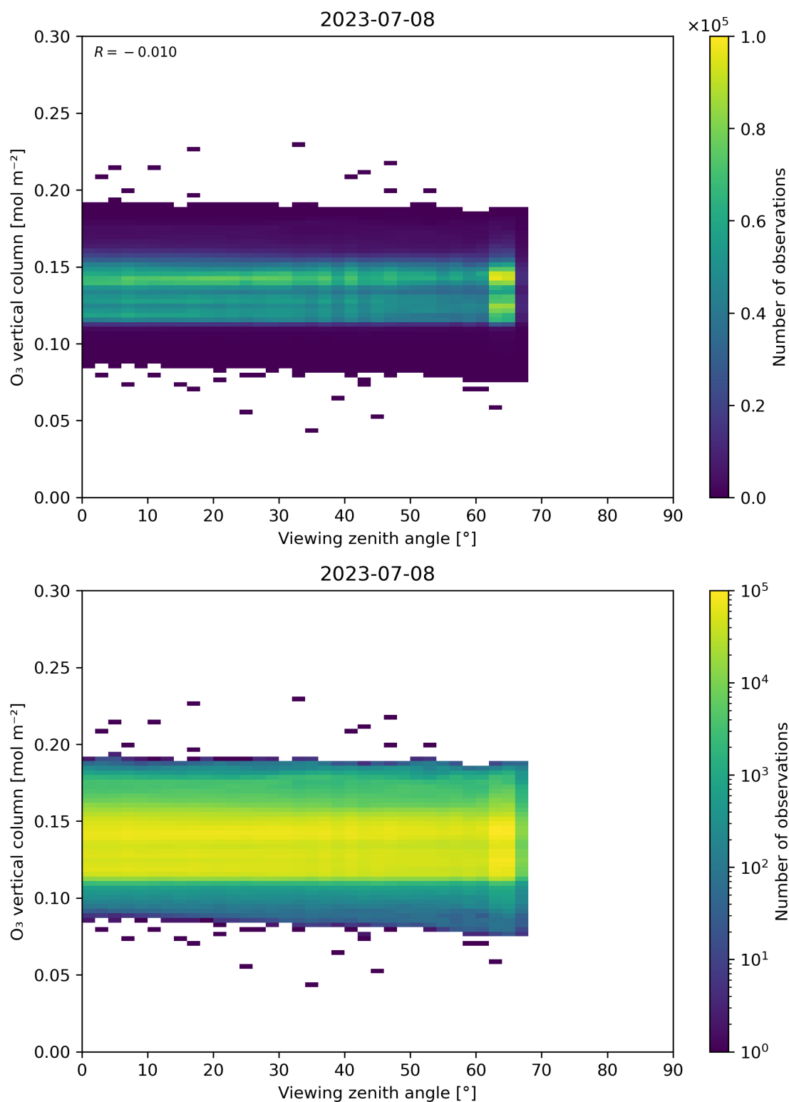
Figure 52: Scatter density plot of “Viewing zenith angle” against “O 3 vertical column” for 2023-07-08 to 2023-07-09.
