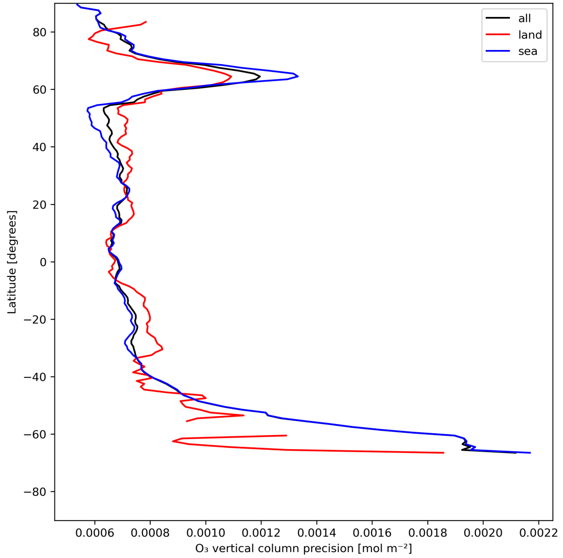
Figure 15: Zonal average of “O 3 vertical column precision” for 2023-07-08 to 2023-07-09.
