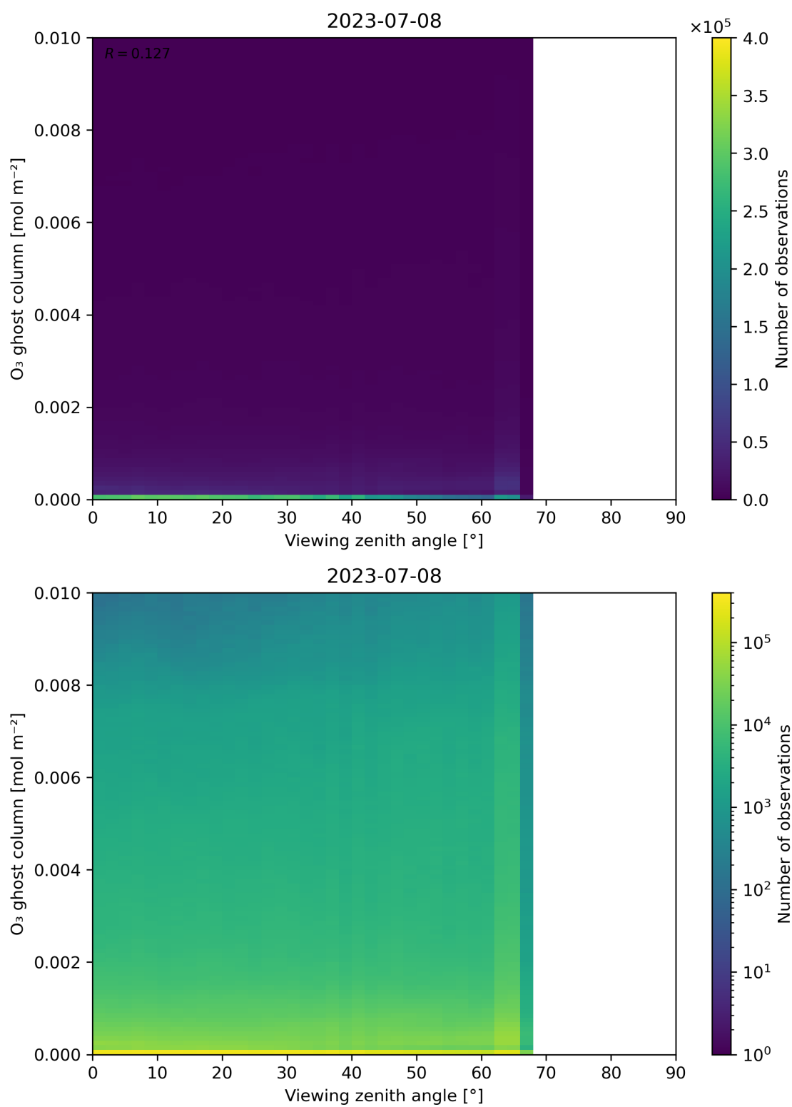
Figure 51: Scatter density plot of “Viewing zenith angle” against “O 3 ghost column” for 2023-07-08 to 2023-07-09.
