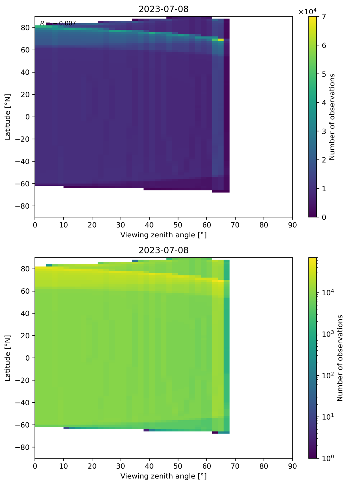
Figure 49: Scatter density plot of “Viewing zenith angle” against “Latitude” for 2023-07-08 to 2023-07-09.
