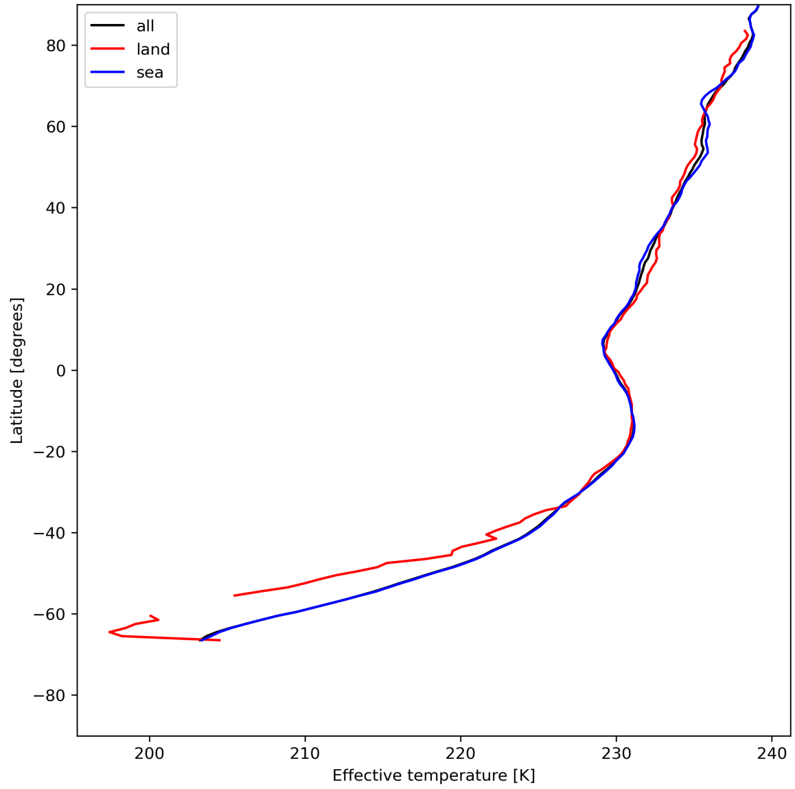
Figure 17: Zonal average of "Effective temperature" for 2023-07-08 to 2023-07-09.
