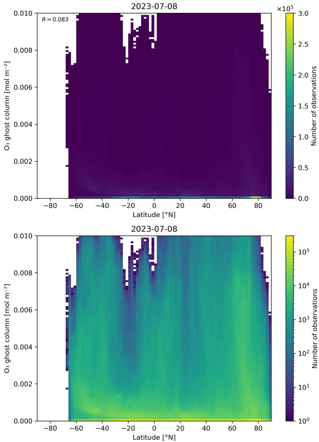
Figure 35: Scatter density plot of “Latitude” against “O 3 ghost column” for 2023-07-08 to 2023-07-09.
