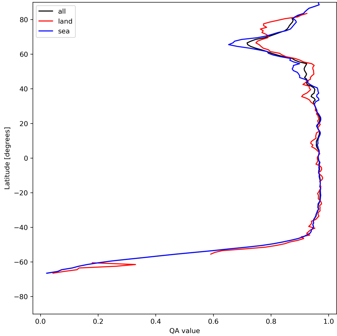
Figure 13: Zonal average of “QA value” for 2023-07-08 to 2023-07-09.
