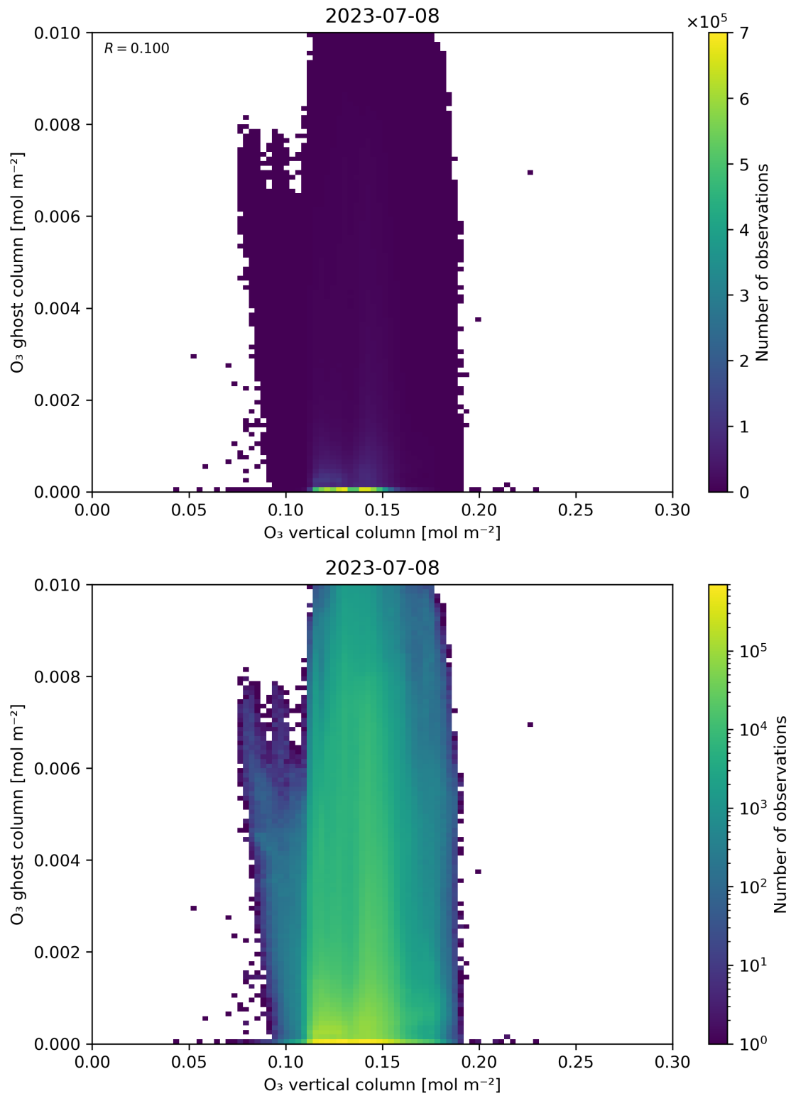
Figure 40: Scatter density plot of “O 3 vertical column” against “O 3 ghost column” for 2023-07-08 to 2023-07-09.
