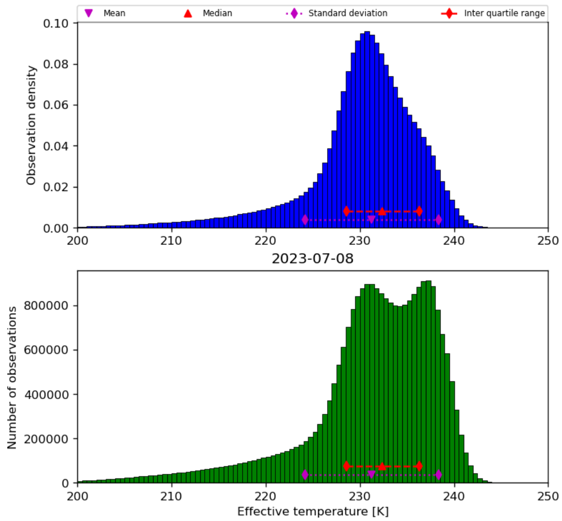
Figure 24: Histogram of “Effective temperature” for 2023-07-08 to 2023-07-09
