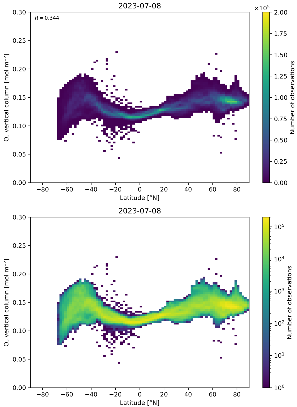
Figure 36: Scatter density plot of “Latitude” against “O 3 vertical column” for 2023-07-08 to 2023-07-09.
