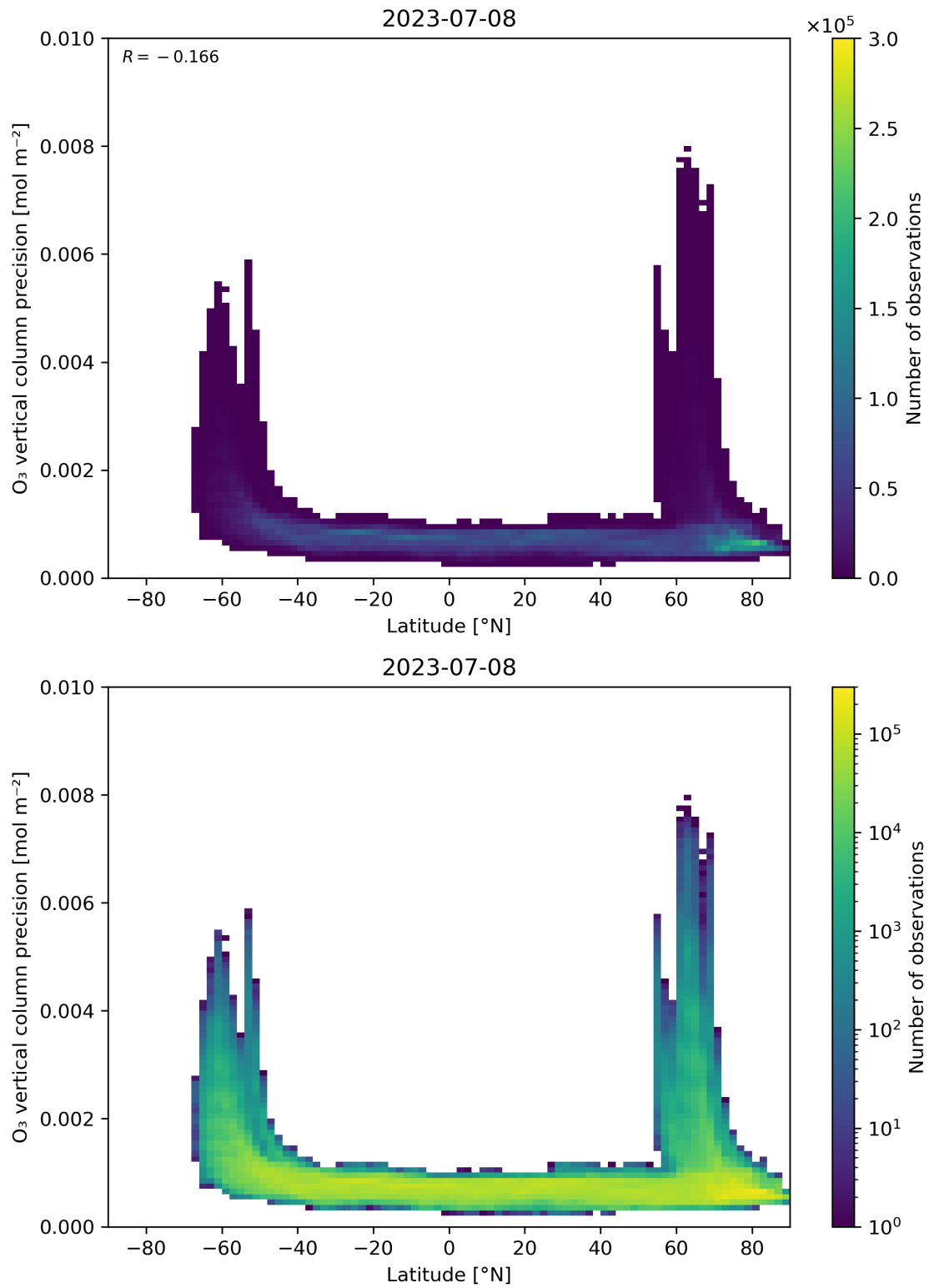
Figure 37: Scatter density plot of “Latitude” against “O 3 vertical column precision” for 2023-07-08 to 2023-07-09.
