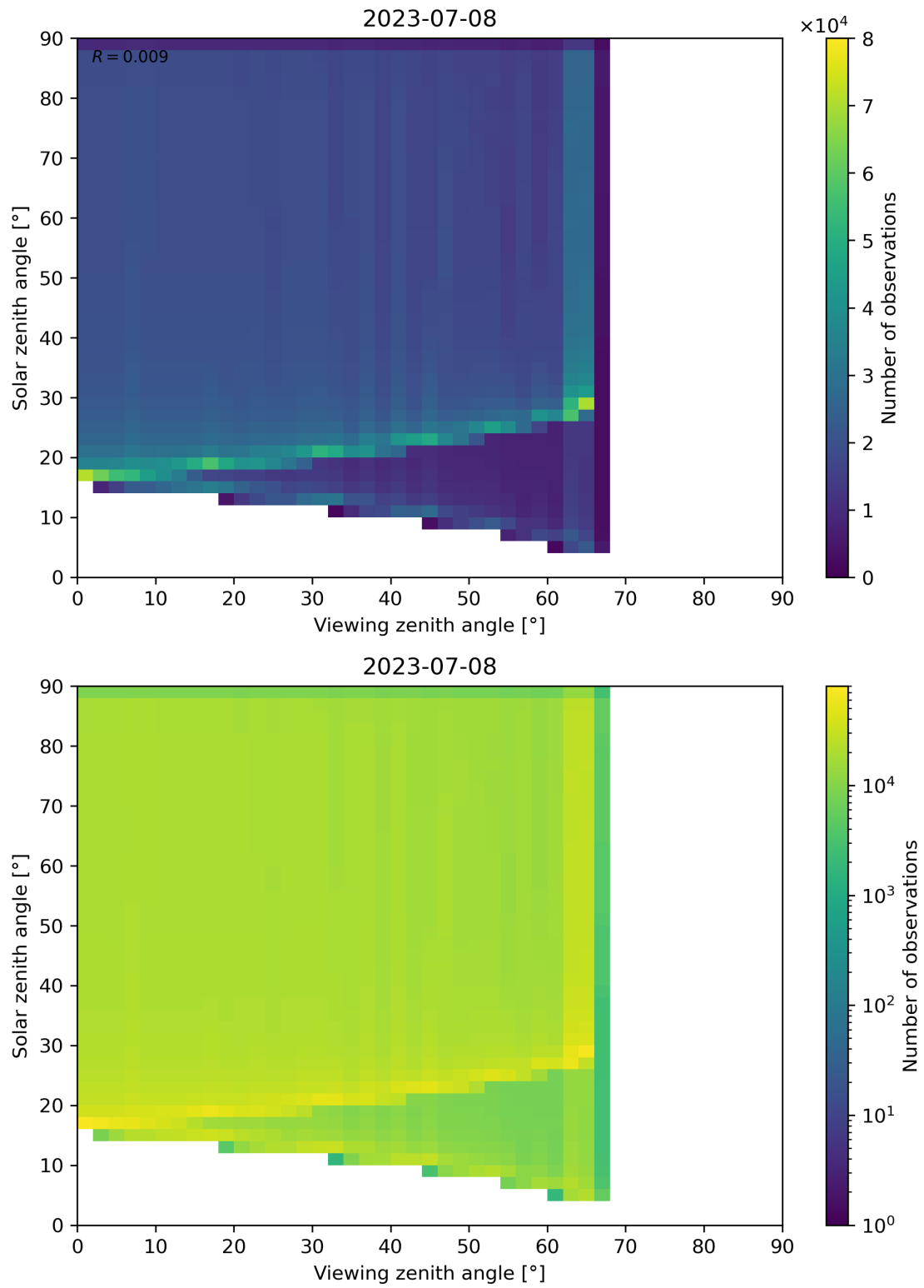
Figure 54: Scatter density plot of “Viewing zenith angle” against “Solar zenith angle” for 2023-07-08 to 2023-07-09.
