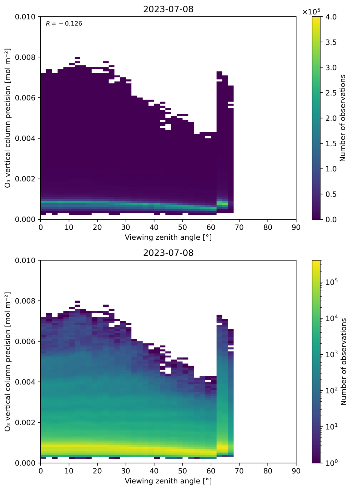
Figure 53: Scatter density plot of “Viewing zenith angle” against “O 3 vertical column precision” for 2023-07-08 to 2023-07-09.
