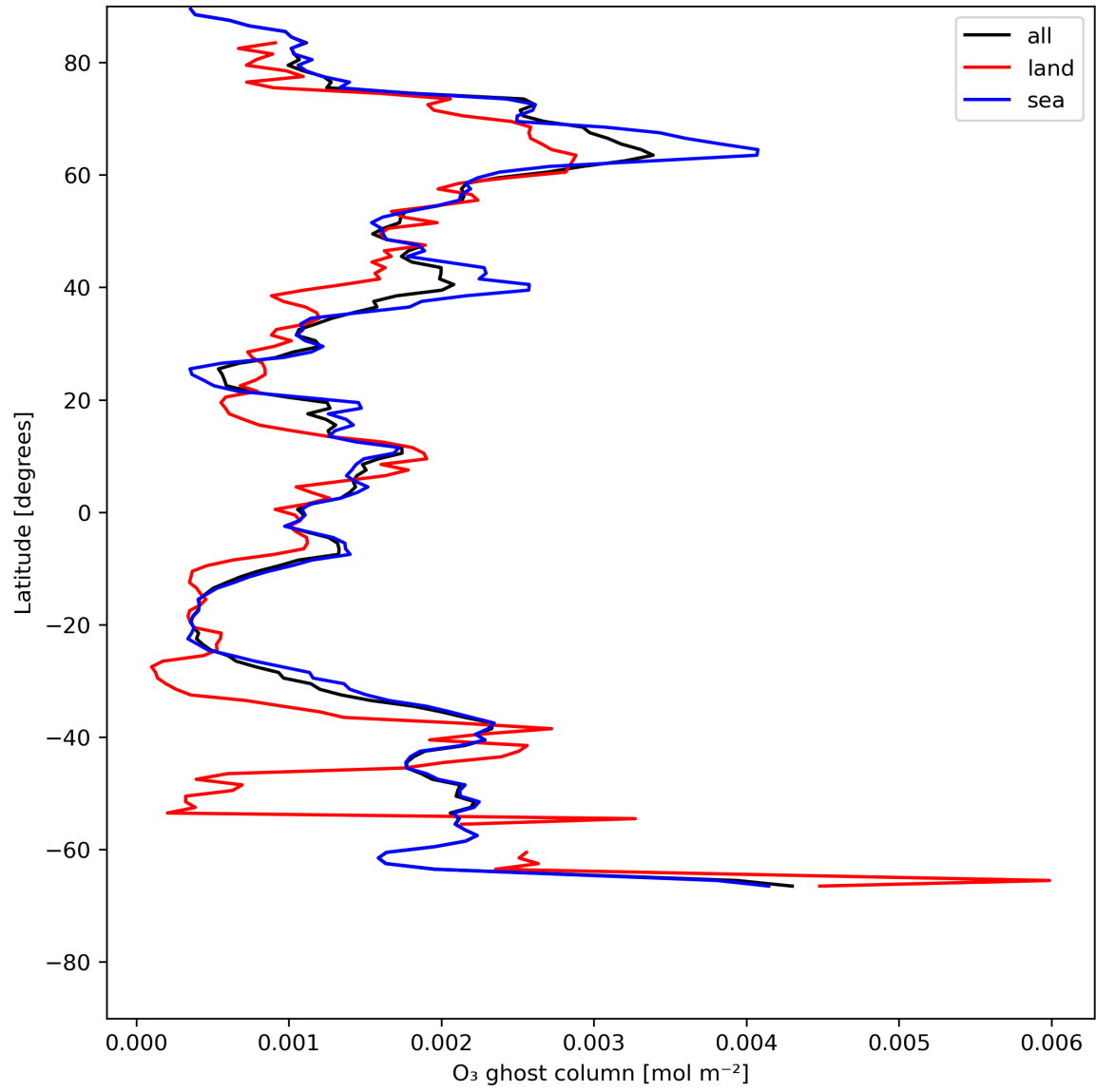
Figure 18: Zonal average of “O 3 ghost column” for 2023-07-08 to 2023-07-09.
