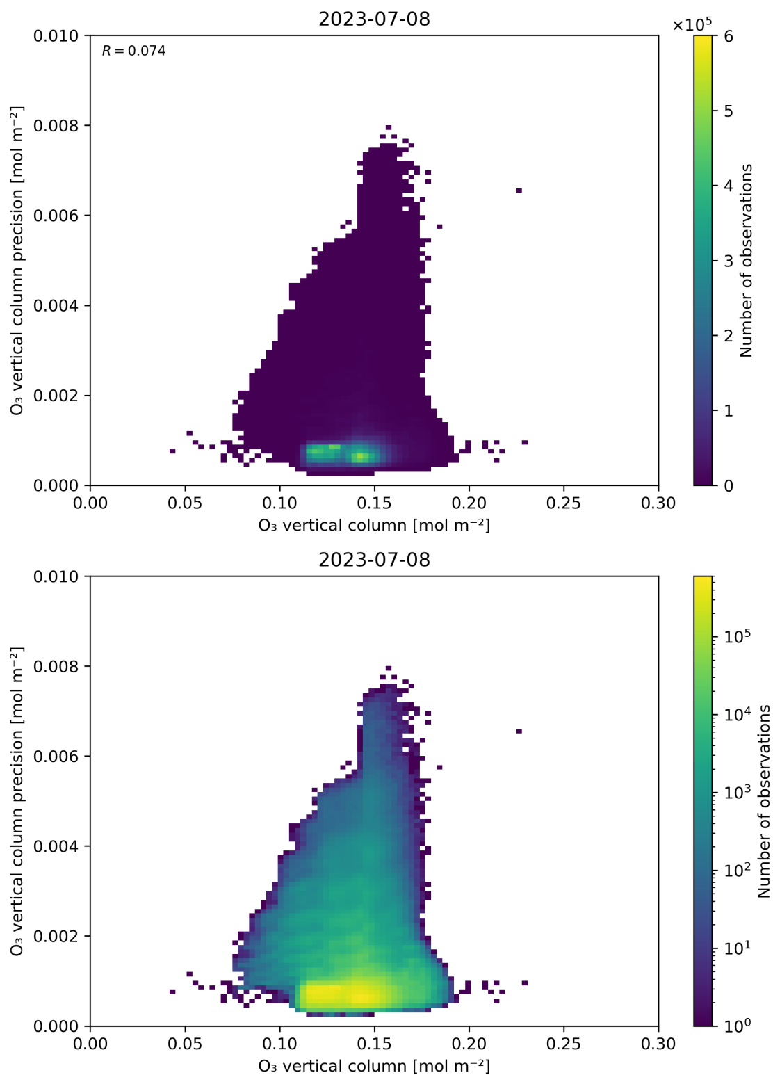
Figure 41: Scatter density plot of “O 3 vertical column” against “O 3 vertical column precision” for 2023-07-08 to 2023-07-09.
