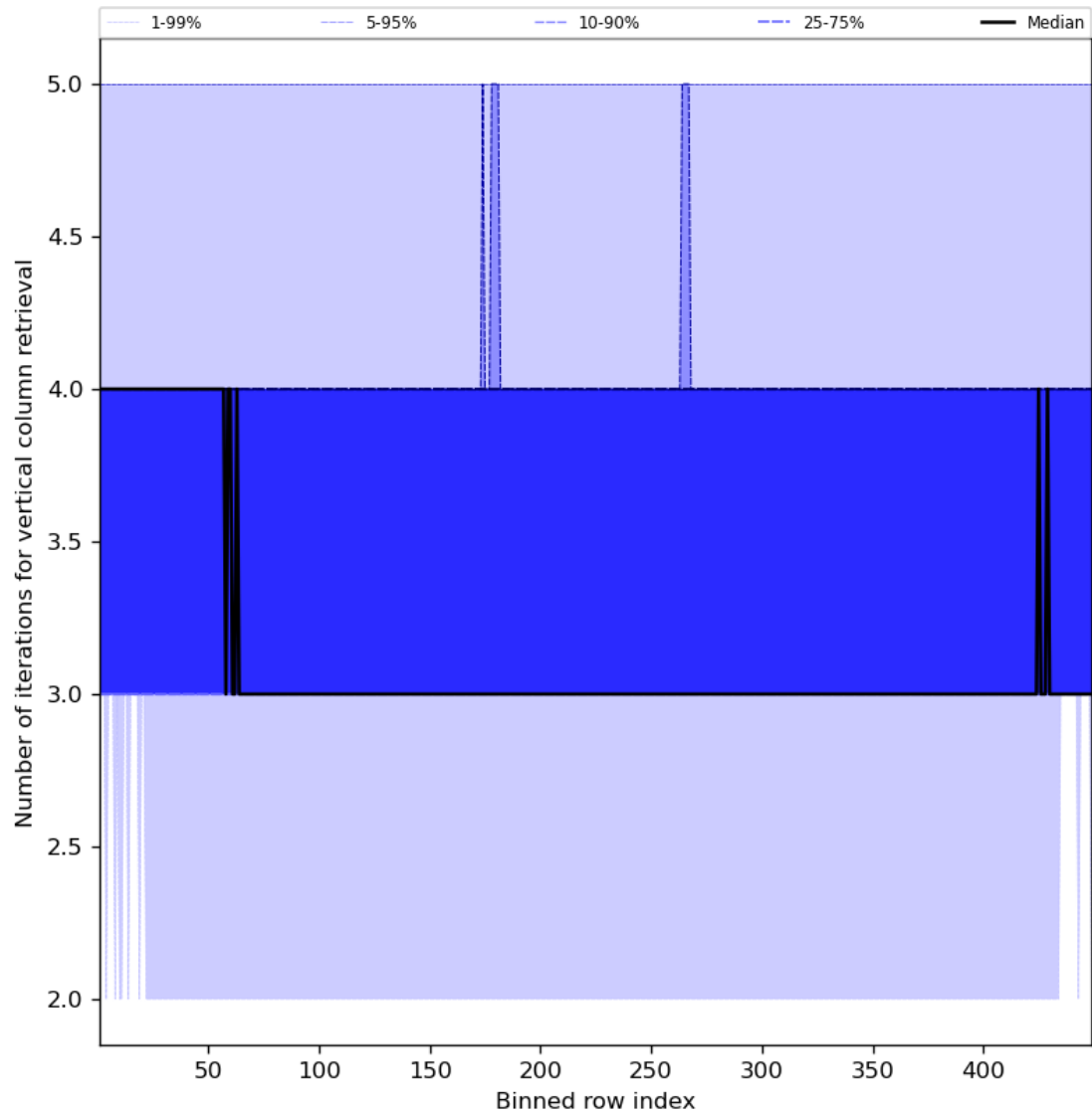
Figure 33: Along track statistics of “Number of iterations for vertical column retrieval” for 2023-07-08 to 2023-07-09
