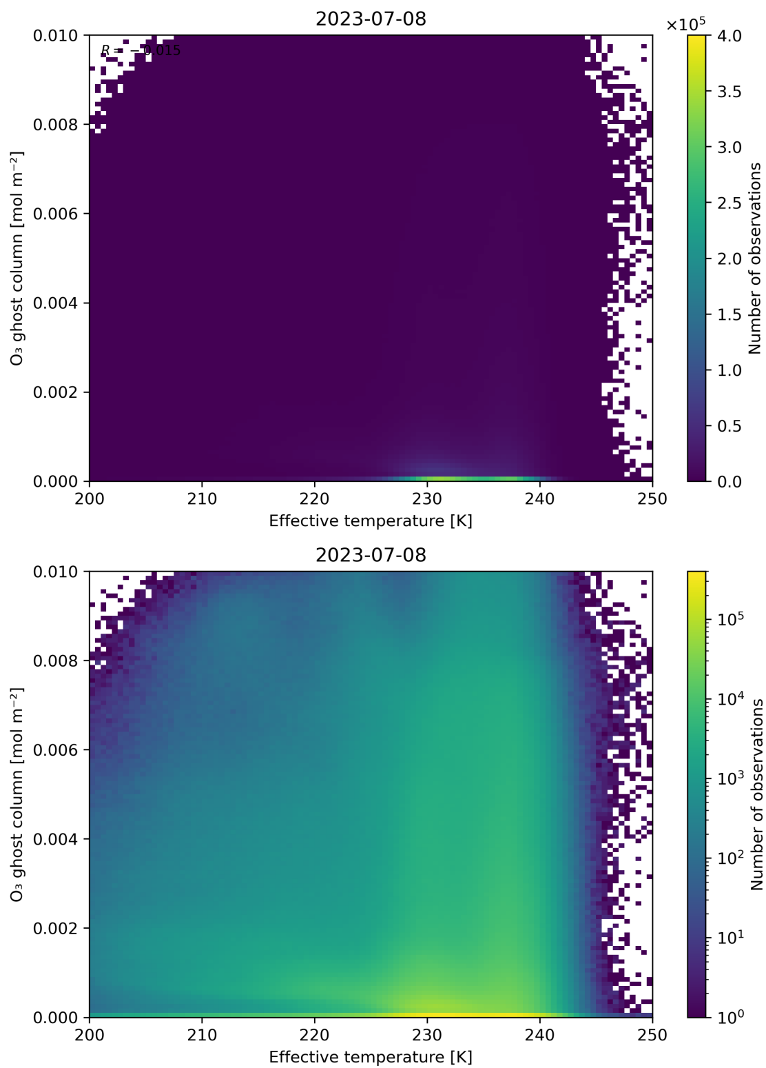
Figure 38: Scatter density plot of “Effective temperature” against “O 3 ghost column” for 2023-07-08 to 2023-07-09.
