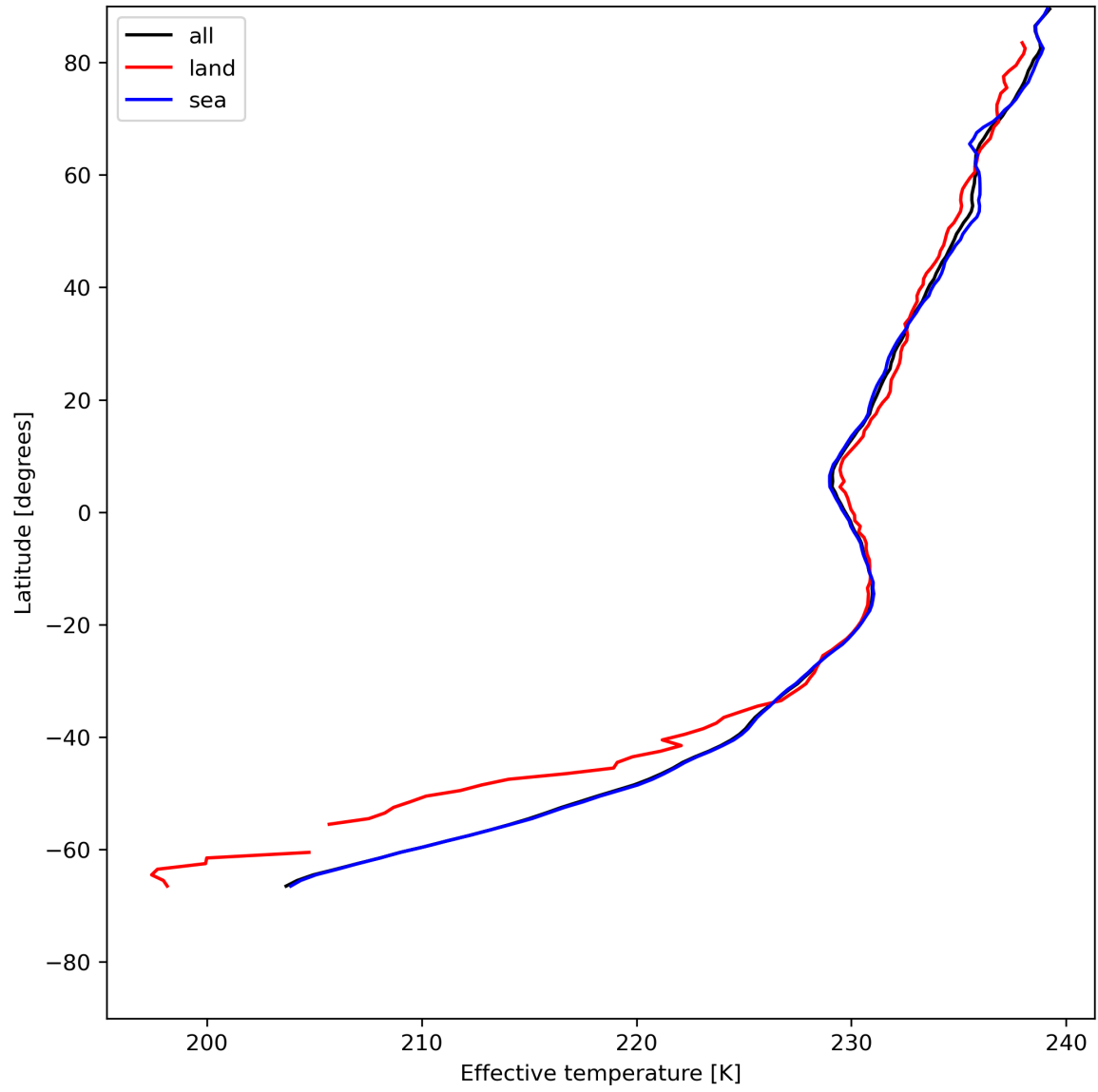
Figure 17: Zonal average of "Effective temperature" for 2023-07-08 to 2023-07-10.
