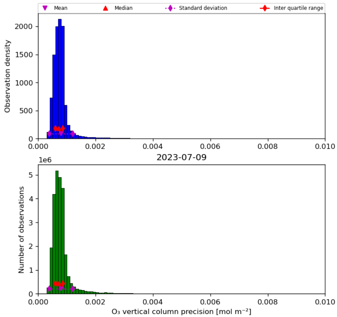
Figure 22: Histogram of “O 3 vertical column precision” for 2023-07-08 to 2023-07-10
