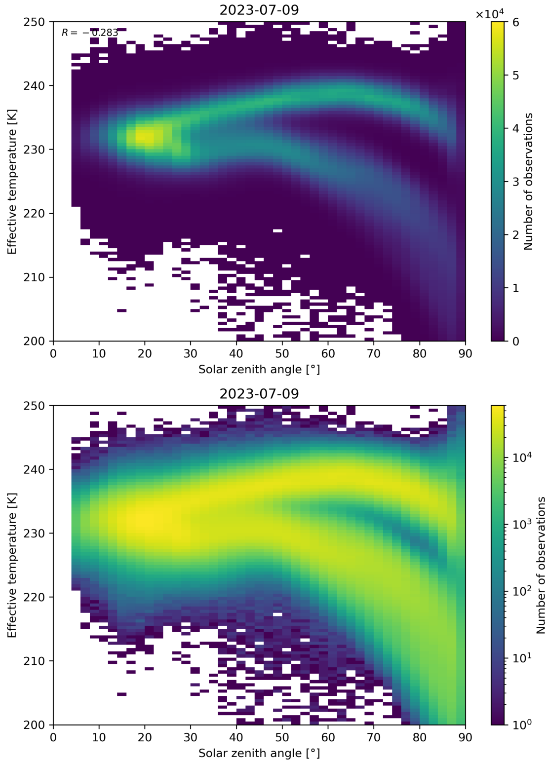
Figure 45: Scatter density plot of “Solar zenith angle” against “Effective temperature” for 2023-07-08 to 2023-07-10.
