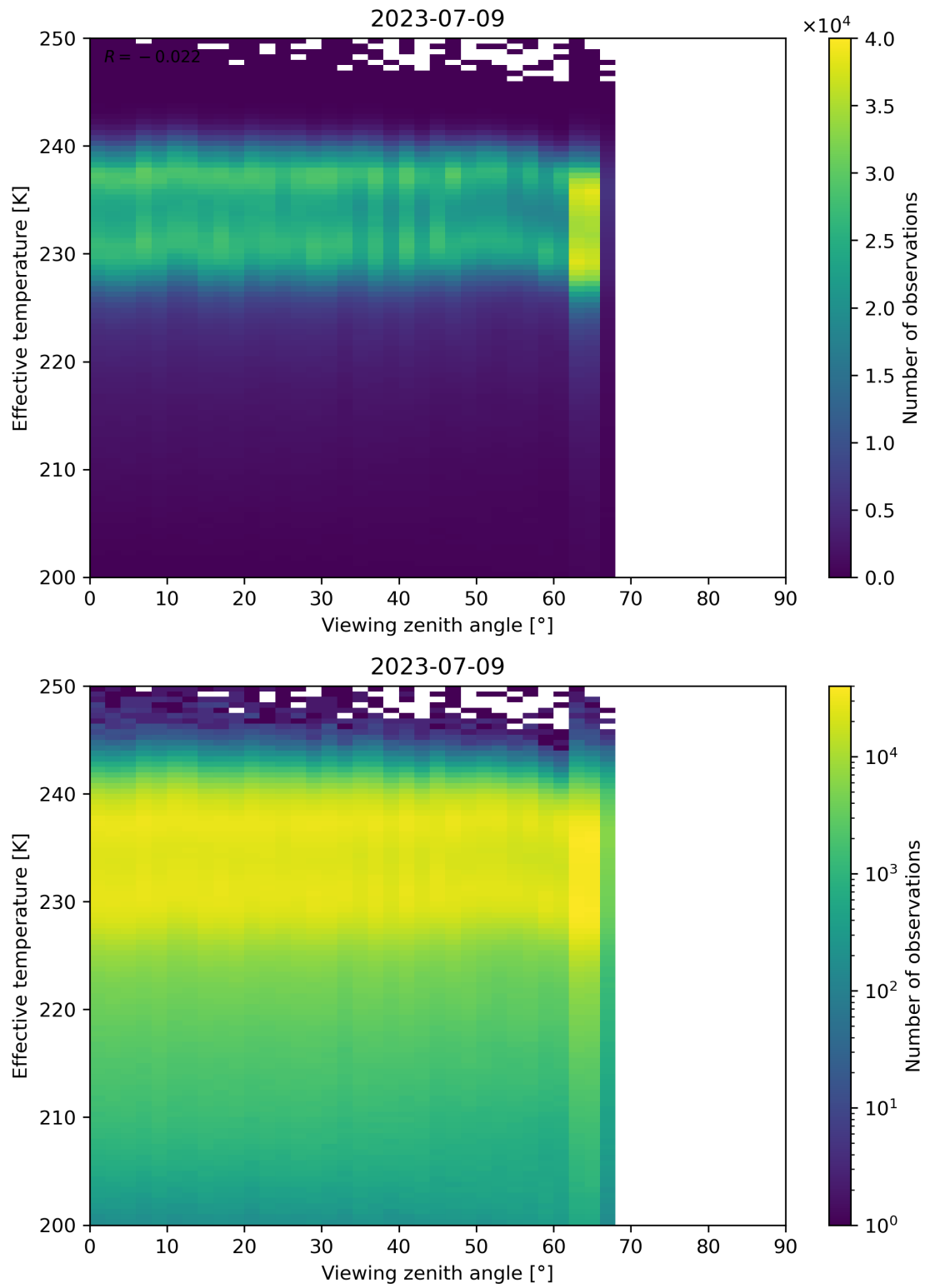
Figure 50: Scatter density plot of “Viewing zenith angle” against “Effective temperature” for 2023-07-08 to 2023-07-10.
