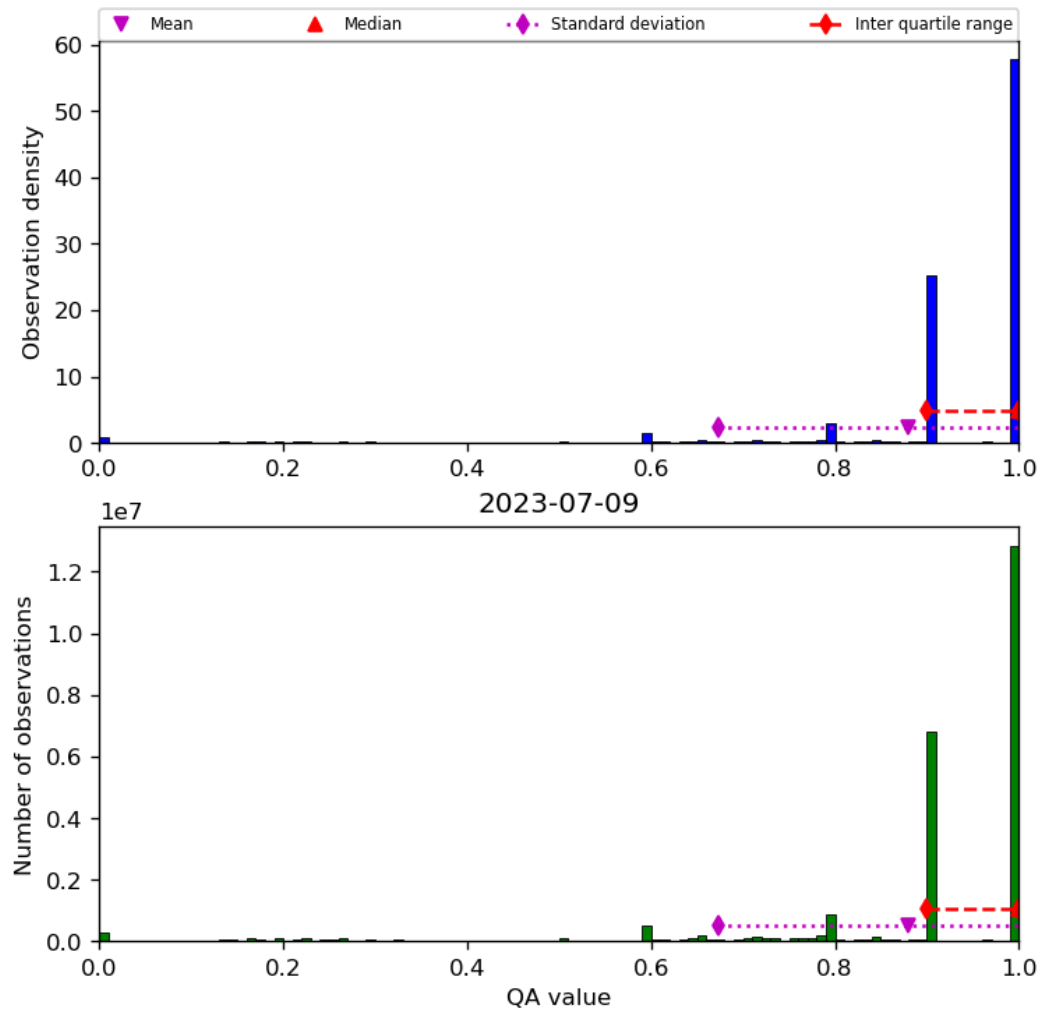
Figure 20: Histogram of “QA value” for 2023-07-08 to 2023-07-10
