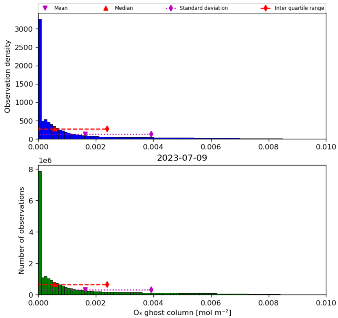
Figure 25: Histogram of “O 3 ghost column” for 2023-07-08 to 2023-07-10
