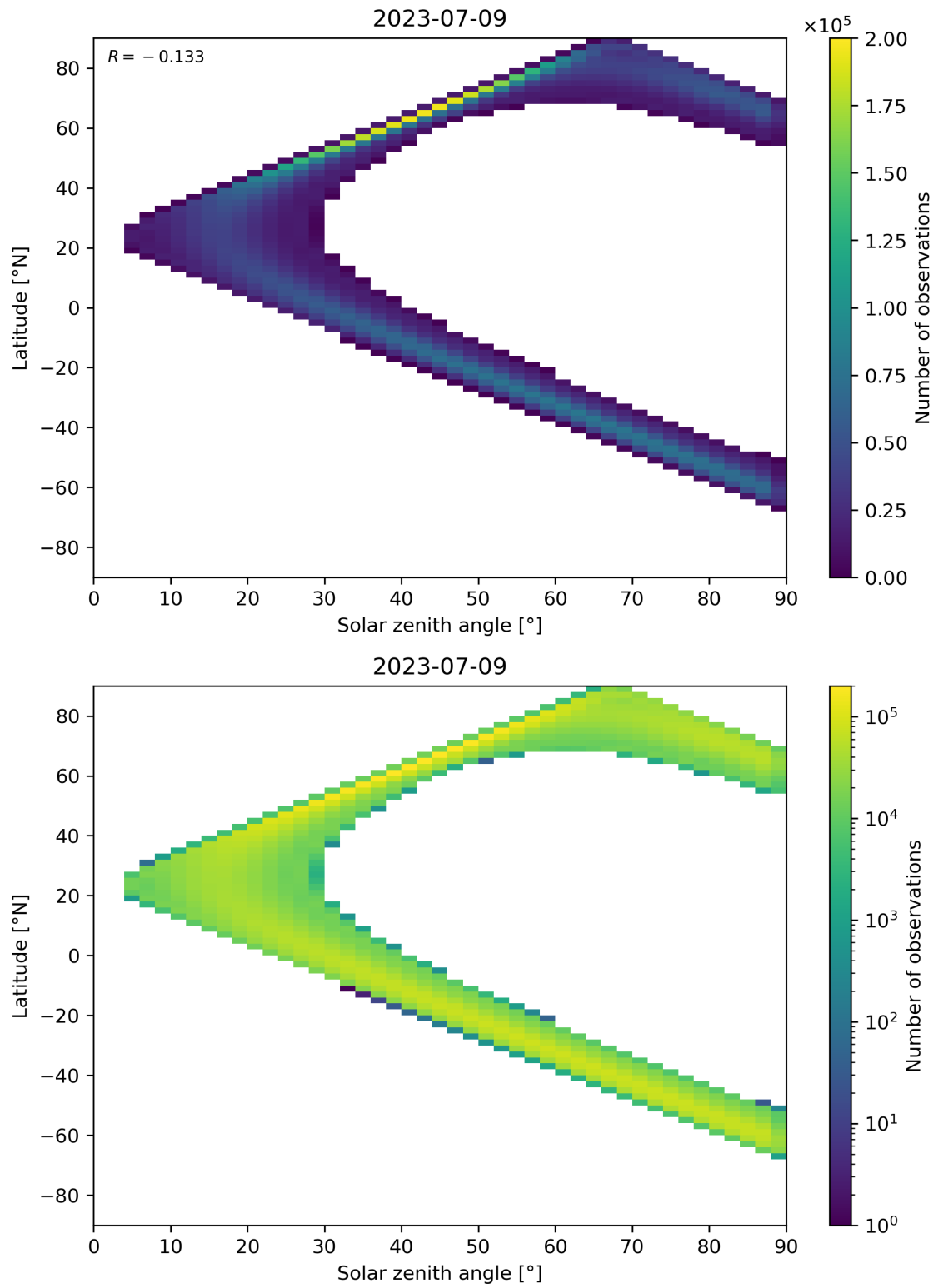
Figure 44: Scatter density plot of “Solar zenith angle” against “Latitude” for 2023-07-08 to 2023-07-10.
