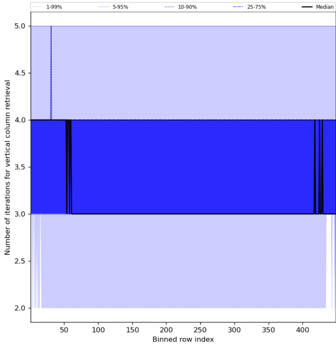
Figure 33: Along track statistics of “Number of iterations for vertical column retrieval” for 2023-07-08 to 2023-07-10
