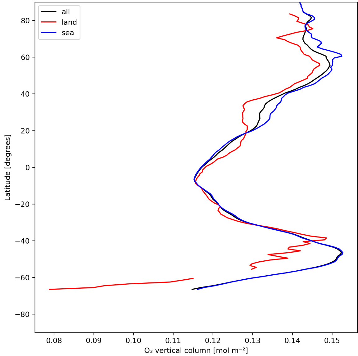
Figure 14: Zonal average of “O 3 vertical column” for 2023-07-08 to 2023-07-10.
