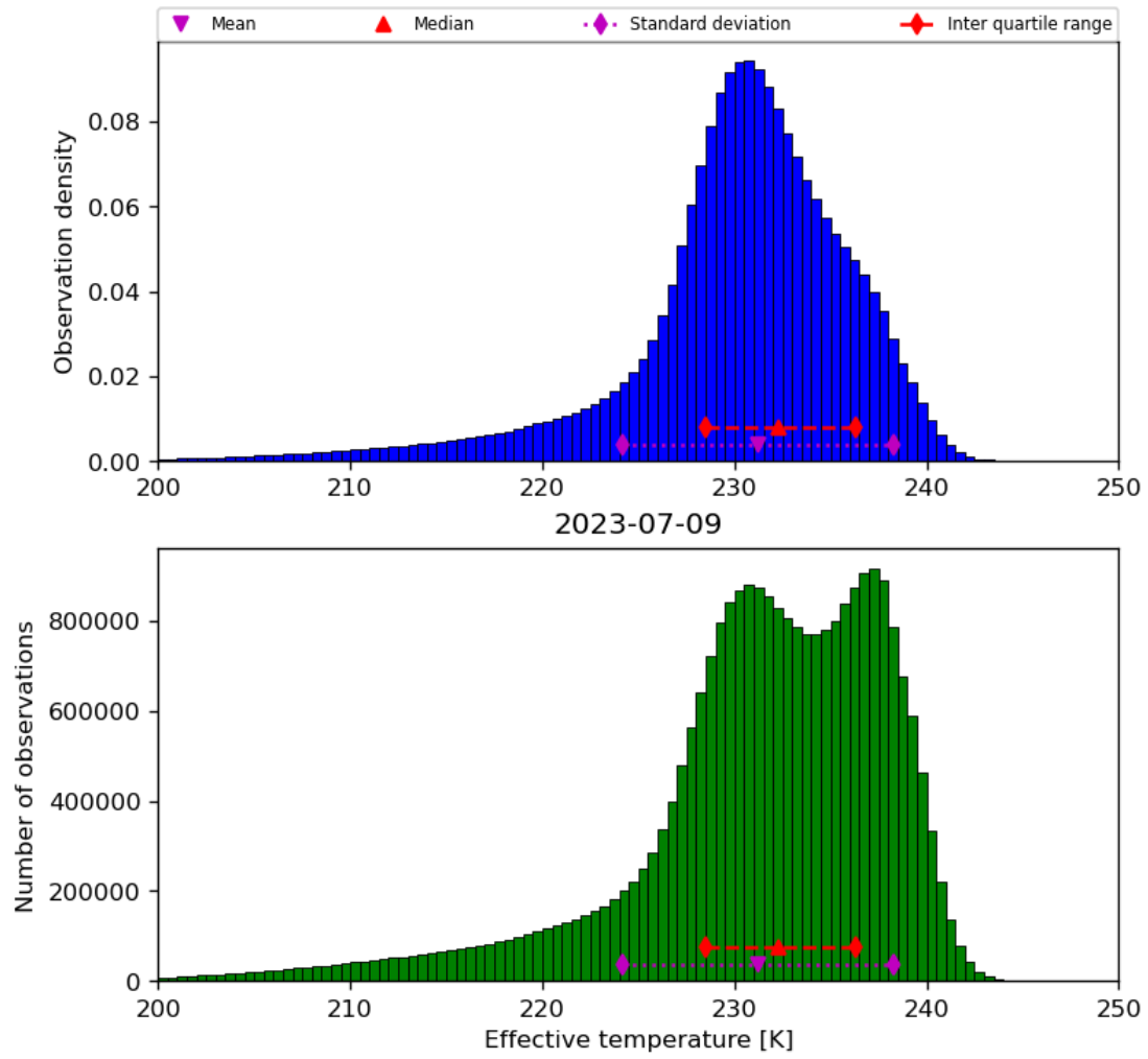
Figure 24: Histogram of “Effective temperature” for 2023-07-08 to 2023-07-10
