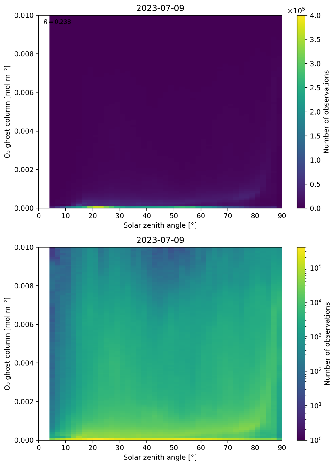
Figure 46: Scatter density plot of “Solar zenith angle” against “O 3 ghost column” for 2023-07-08 to 2023-07-10.
