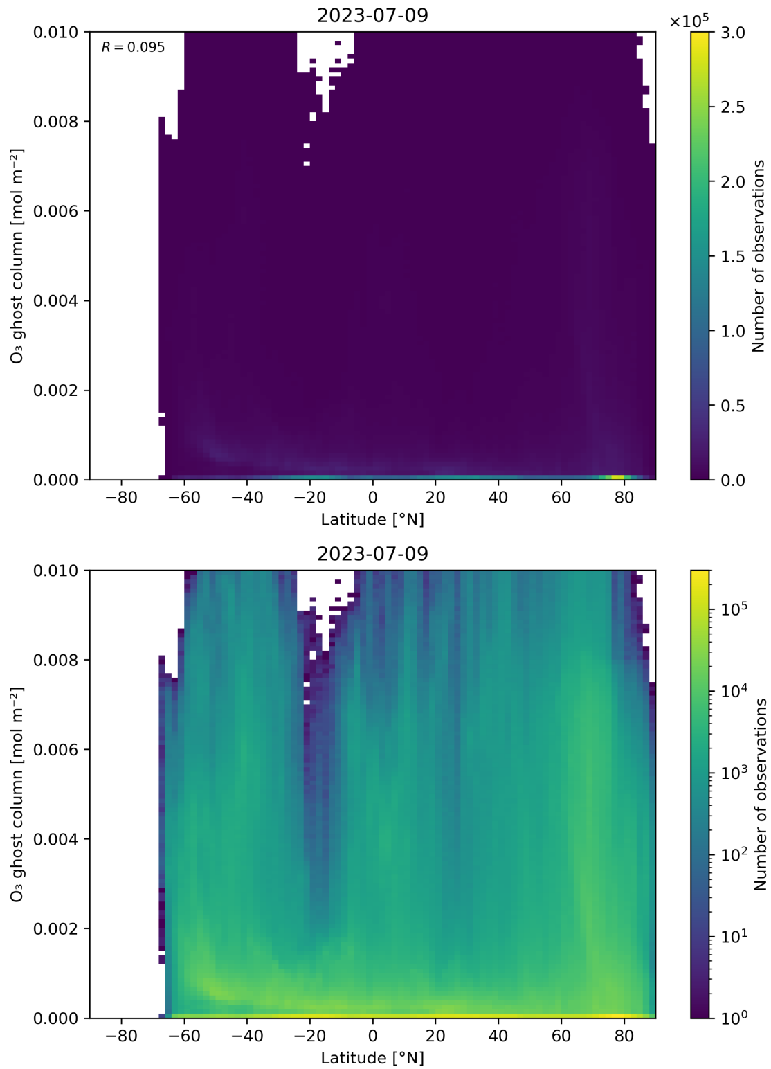
Figure 35: Scatter density plot of “Latitude” against “O 3 ghost column” for 2023-07-08 to 2023-07-10.
