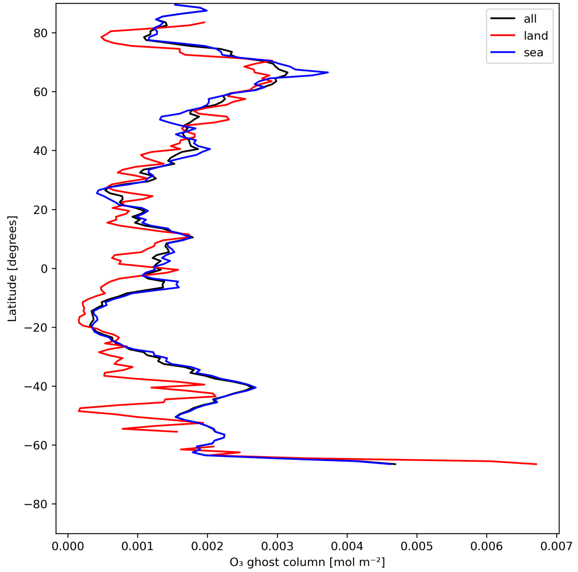
Figure 18: Zonal average of “O 3 ghost column” for 2023-07-08 to 2023-07-10.
