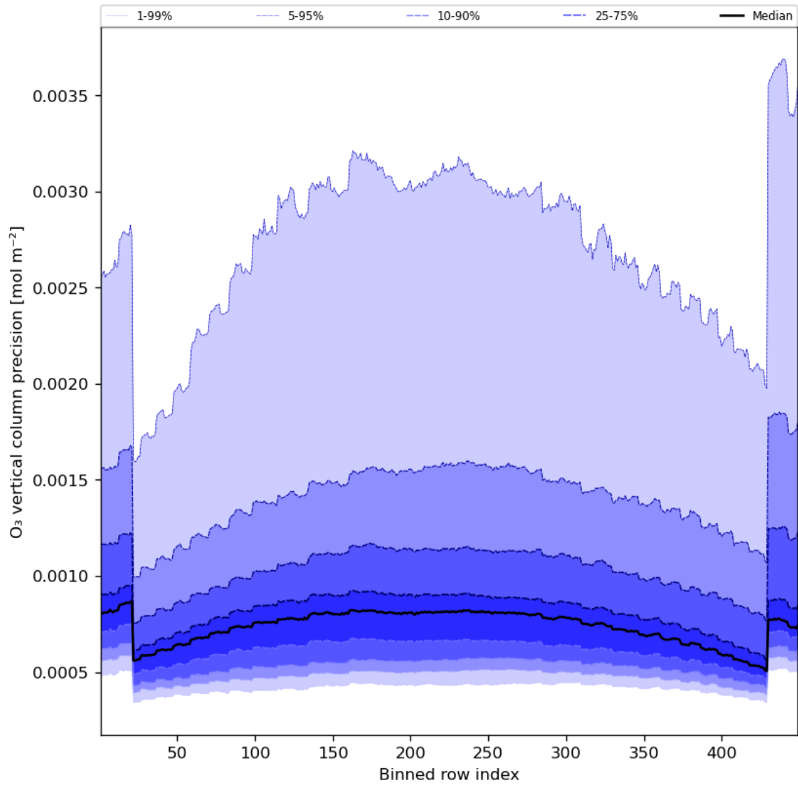
Figure 29: Along track statistics of “O 3 vertical column precision” for 2023-07-08 to 2023-07-10
