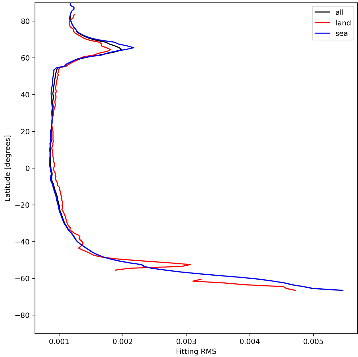
Figure 16: Zonal average of “Fitting RMS” for 2023-07-08 to 2023-07-10.
