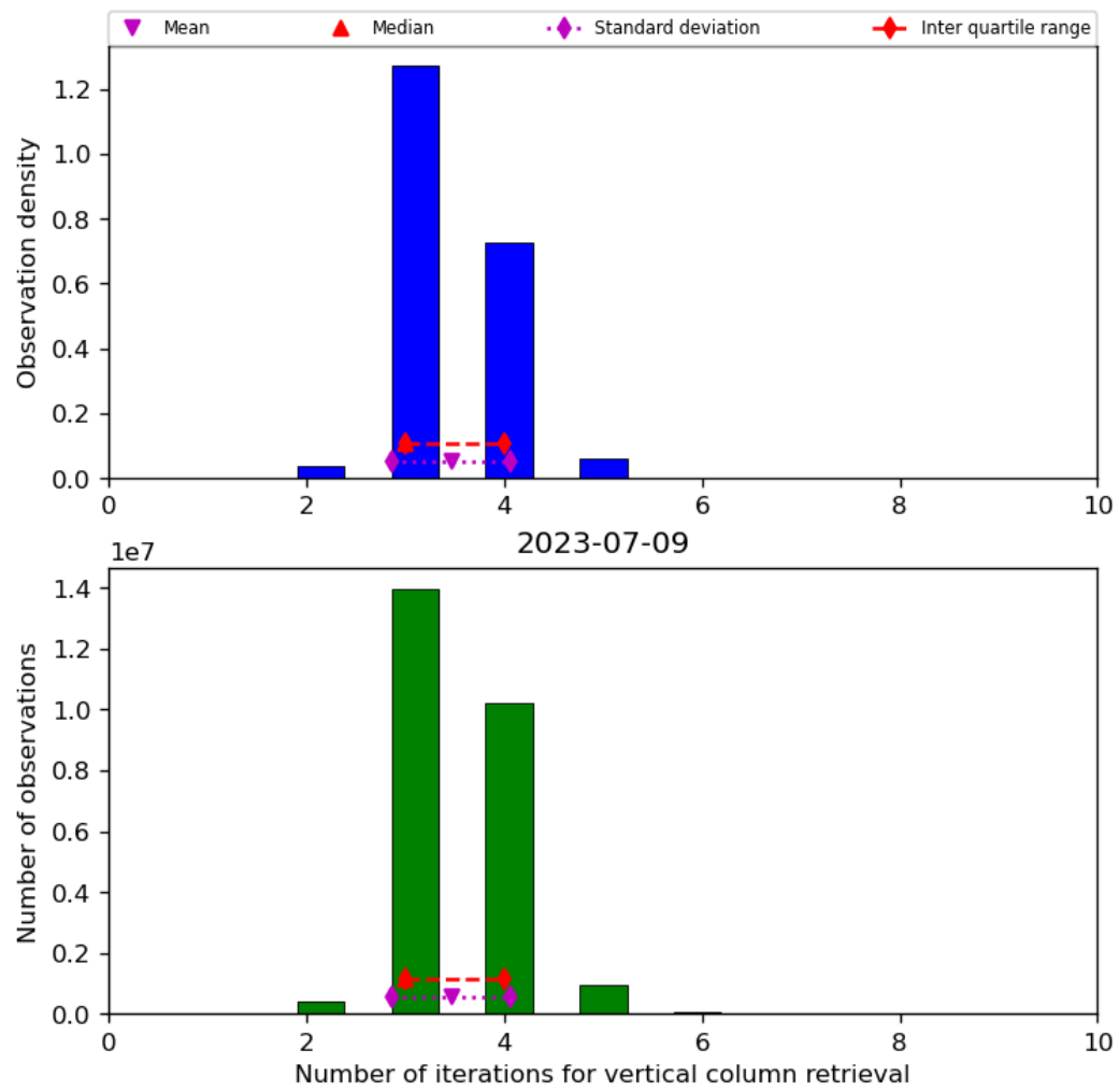
Figure 26: Histogram of “Number of iterations for vertical column retrieval” for 2023-07-08 to 2023-07-10
