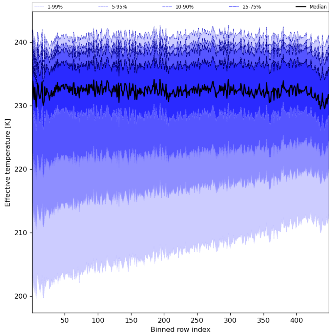
Figure 31: Along track statistics of “Effective temperature” for 2023-07-08 to 2023-07-10
