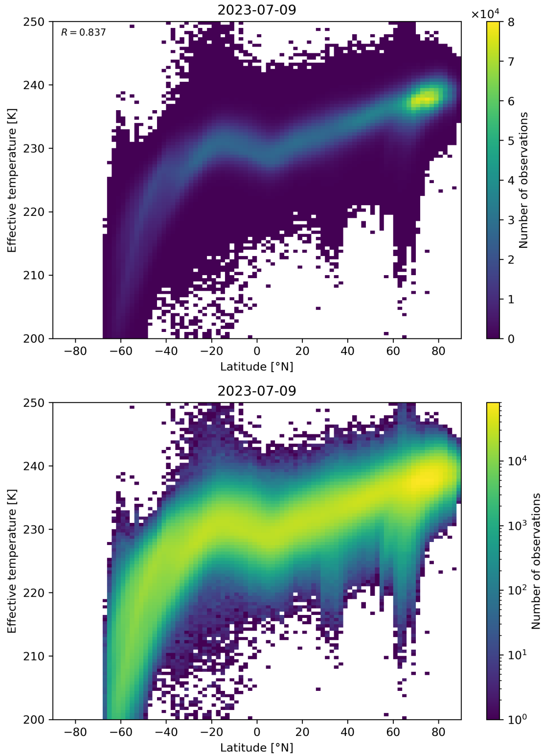
Figure 34: Scatter density plot of “Latitude” against “Effective temperature” for 2023-07-08 to 2023-07-10.
