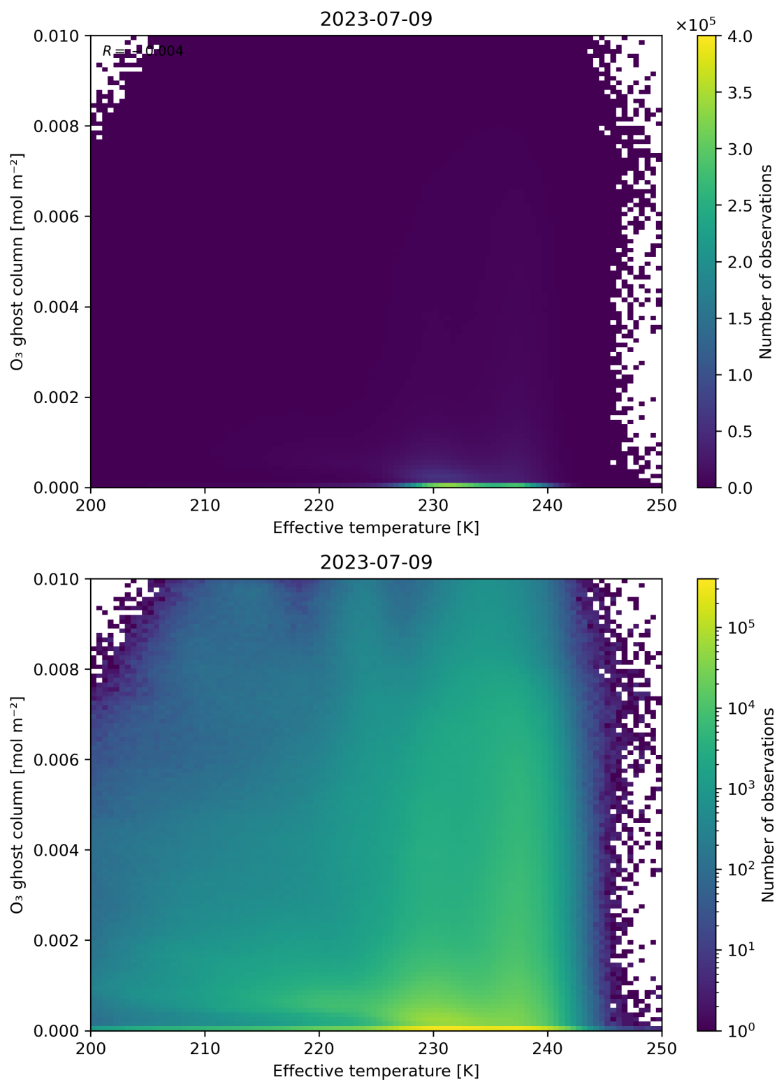
Figure 38: Scatter density plot of “Effective temperature” against “O 3 ghost column” for 2023-07-08 to 2023-07-10.
