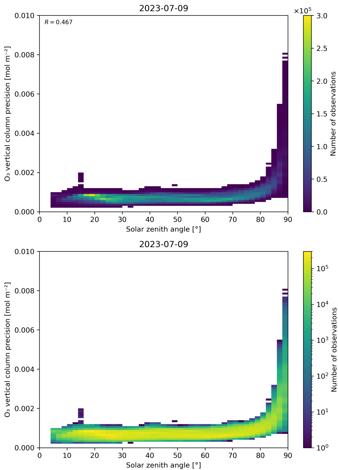
Figure 48: Scatter density plot of “Solar zenith angle” against “O 3 vertical column precision” for 2023-07-08 to 2023-07-10.
