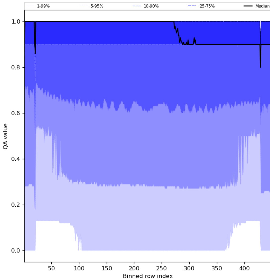
Figure 27: Along track statistics of “QA value” for 2023-07-08 to 2023-07-10
