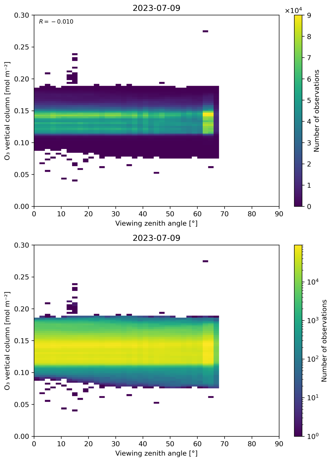
Figure 52: Scatter density plot of “Viewing zenith angle” against “O 3 vertical column” for 2023-07-08 to 2023-07-10.
