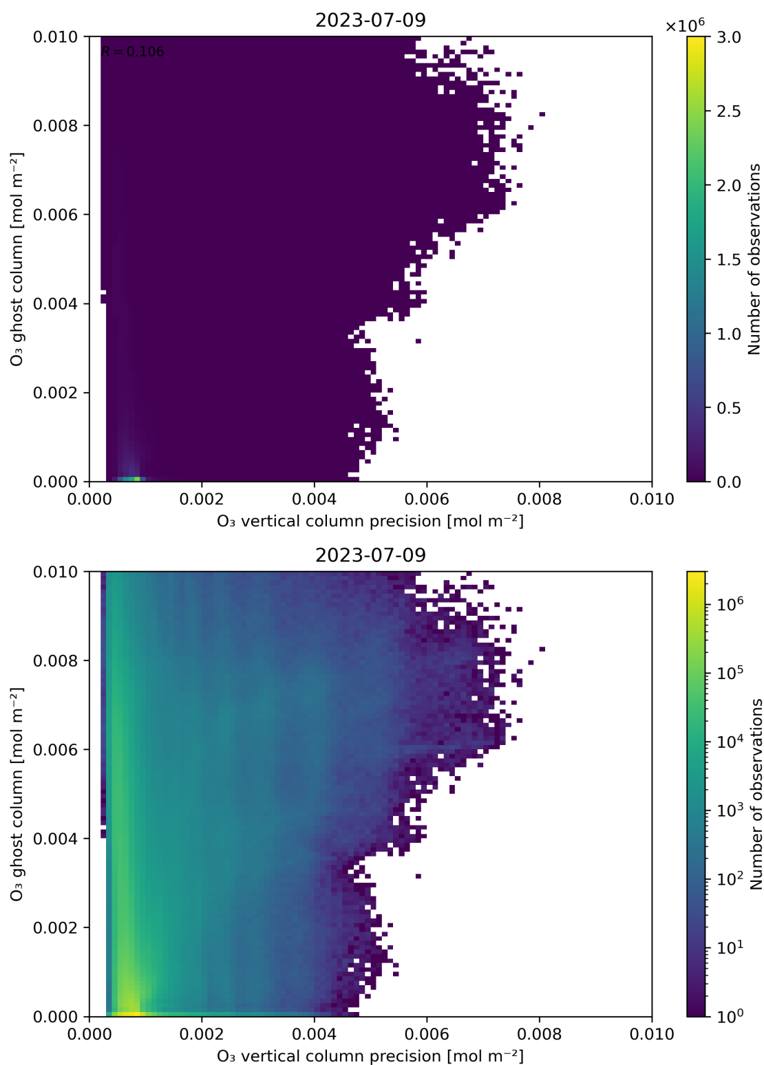
Figure 43: Scatter density plot of “ \text{O}_3 vertical column precision” against “ \text{O}_3 ghost column” for 2023-07-08 to 2023-07-10.
