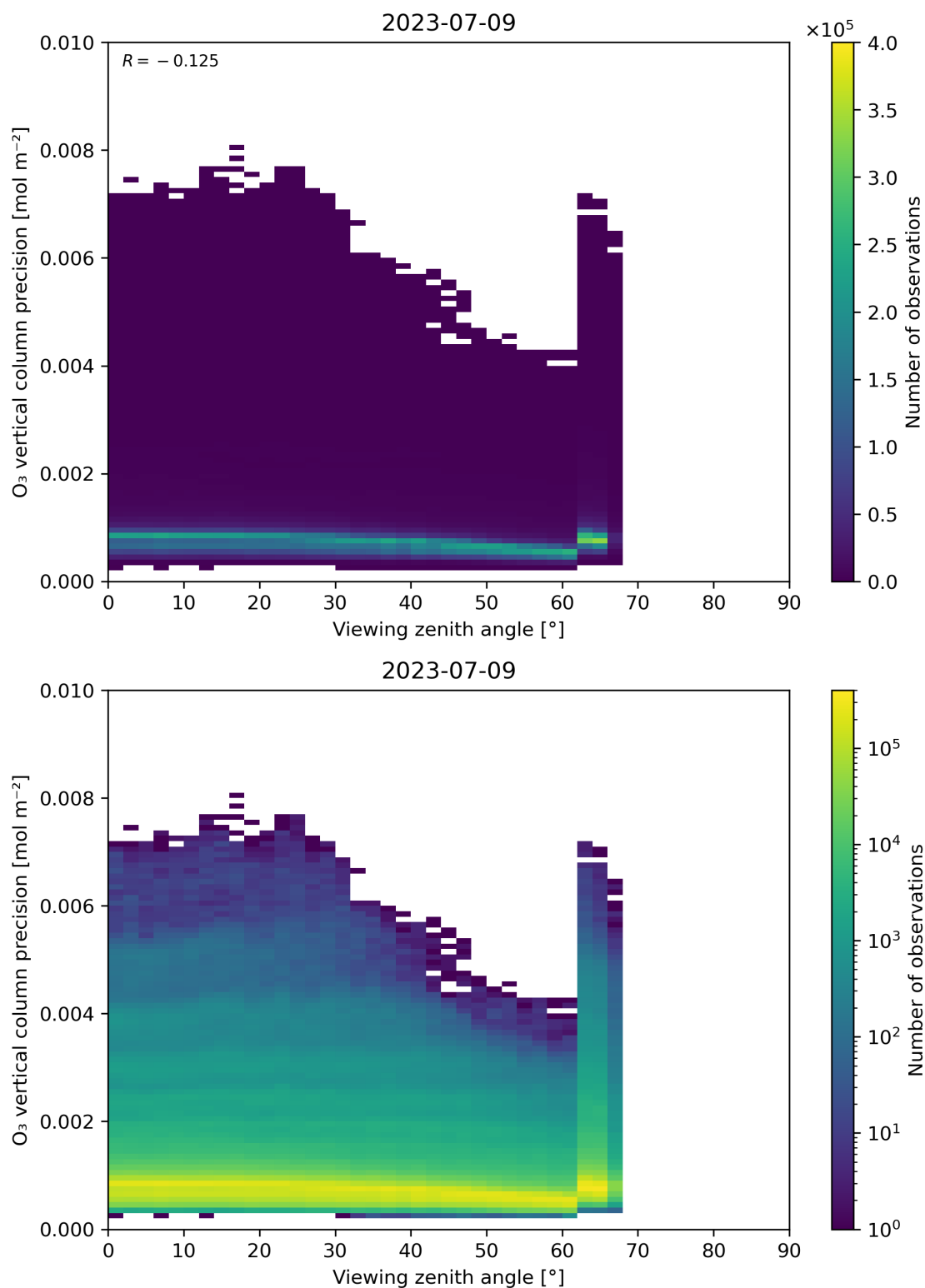
Figure 53: Scatter density plot of “Viewing zenith angle” against “O 3 vertical column precision” for 2023-07-08 to 2023-07-10.
