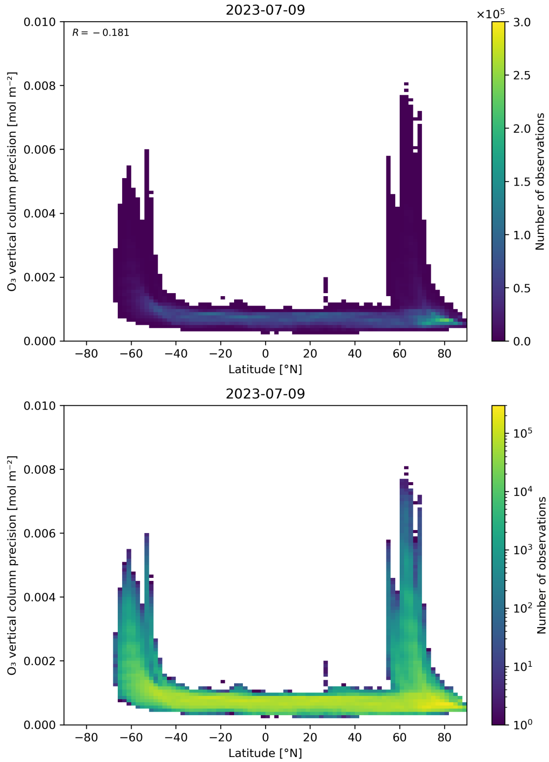
Figure 37: Scatter density plot of “Latitude” against “O 3 vertical column precision” for 2023-07-08 to 2023-07-10.
