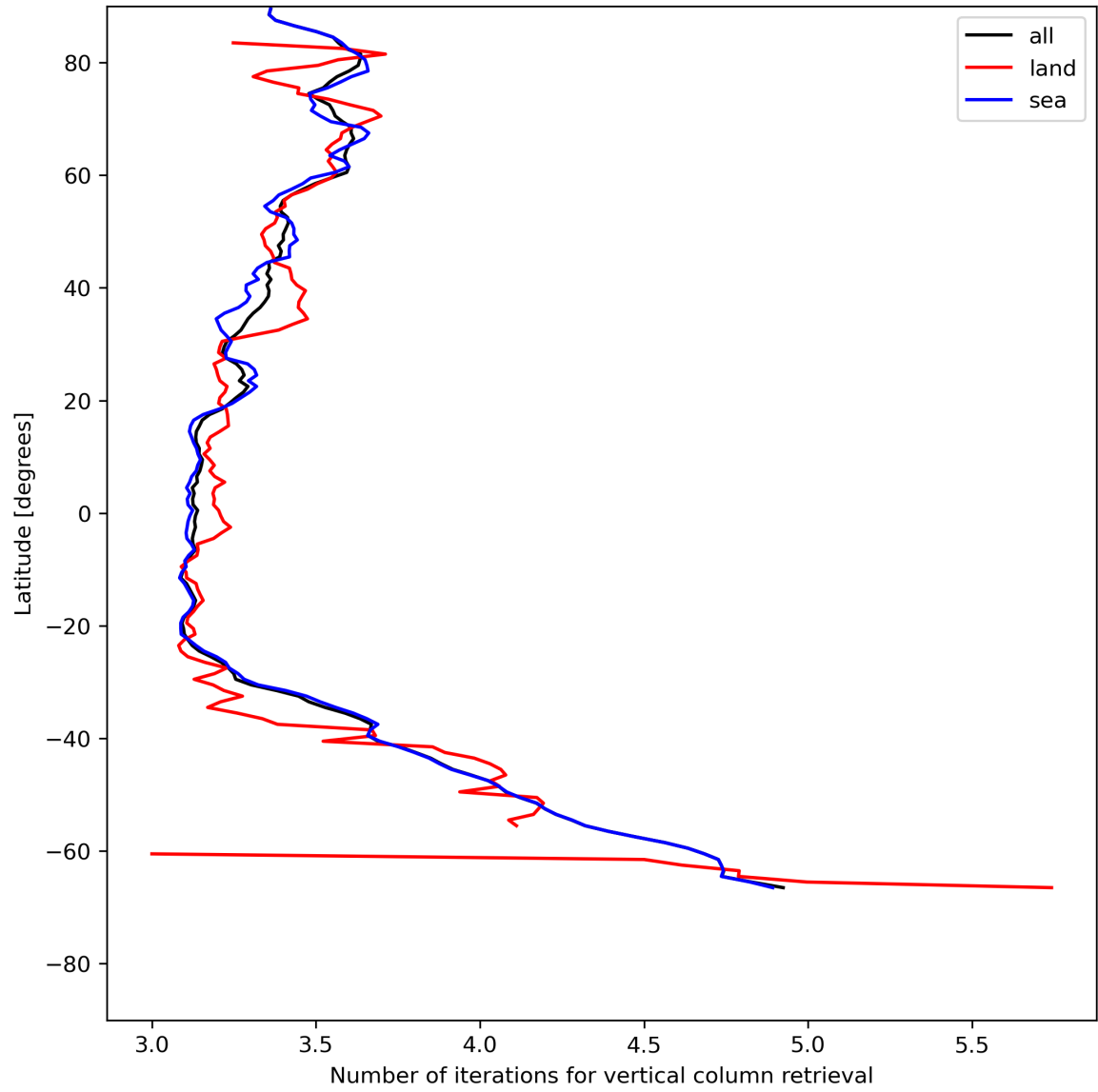
Figure 19: Zonal average of “Number of iterations for vertical column retrieval” for 2023-07-08 to 2023-07-10.
