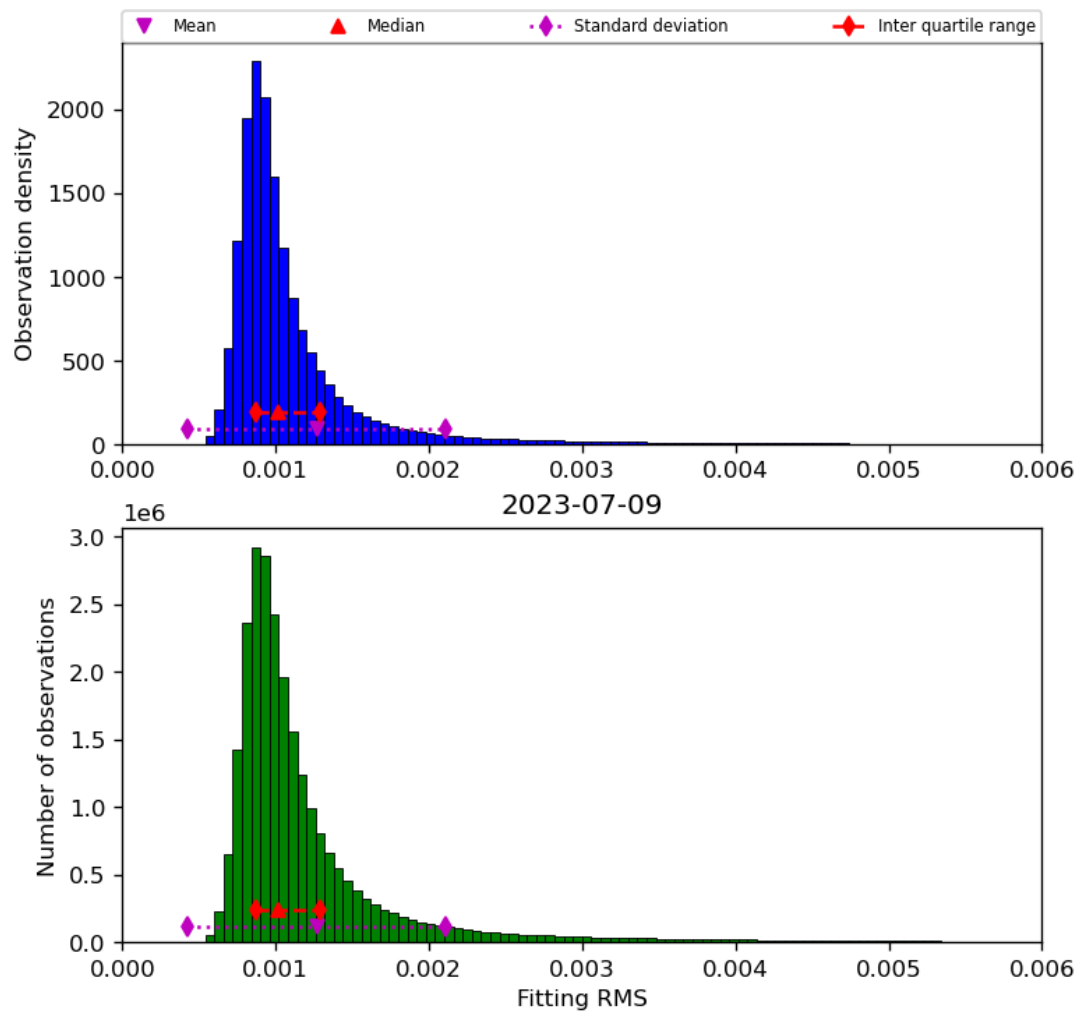
Figure 23: Histogram of “Fitting RMS” for 2023-07-08 to 2023-07-10
