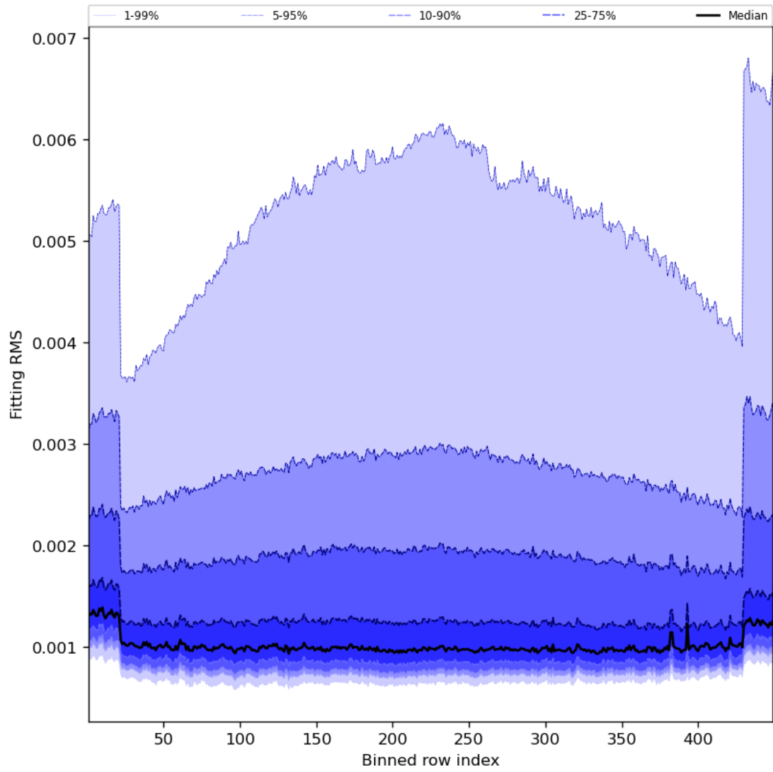
Figure 30: Along track statistics of “Fitting RMS” for 2023-07-08 to 2023-07-10
