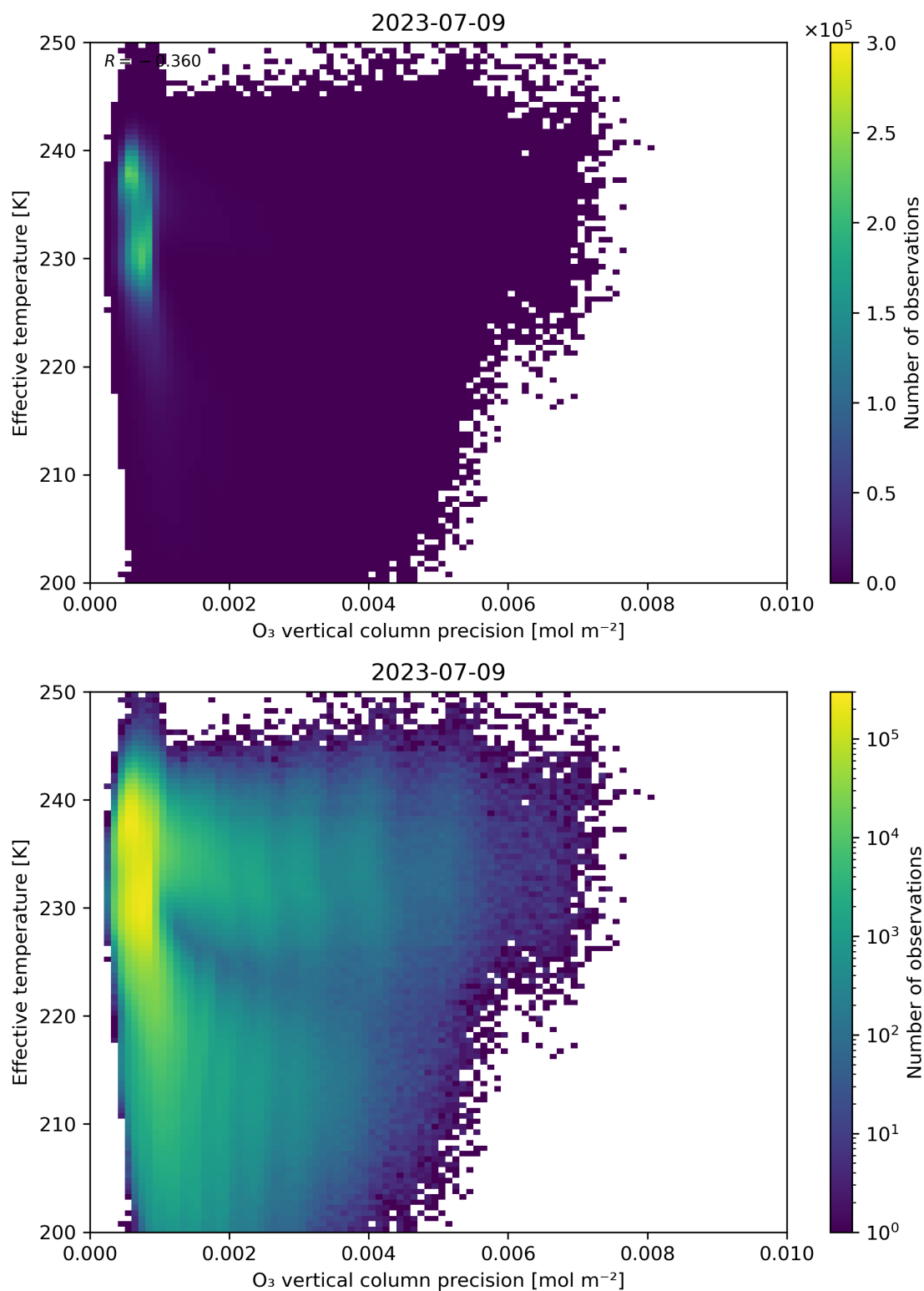
Figure 42: Scatter density plot of “O 3 vertical column precision” against “Effective temperature” for 2023-07-08 to 2023-07-10.
