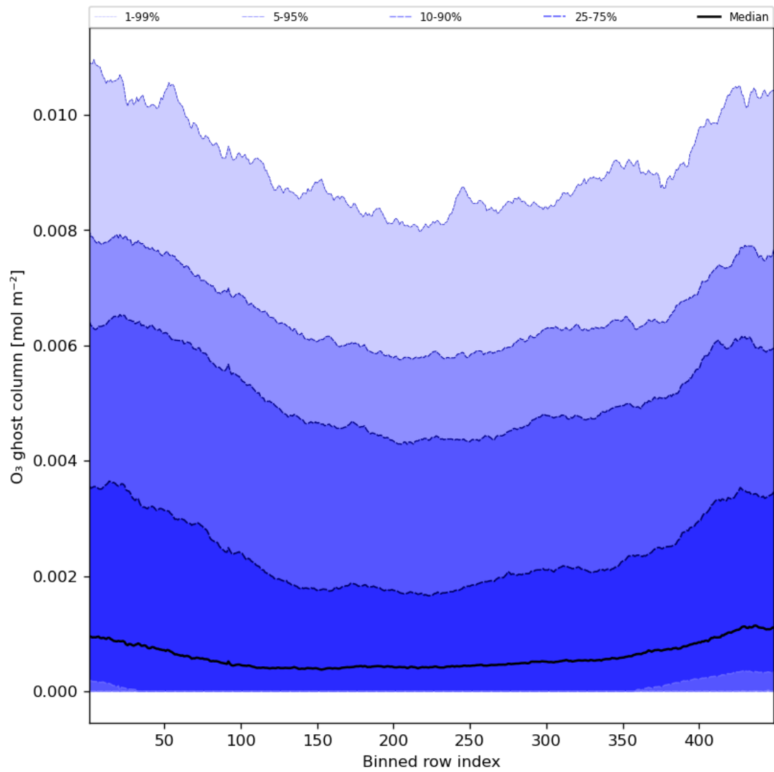
Figure 32: Along track statistics of “O 3 ghost column” for 2023-07-08 to 2023-07-10
