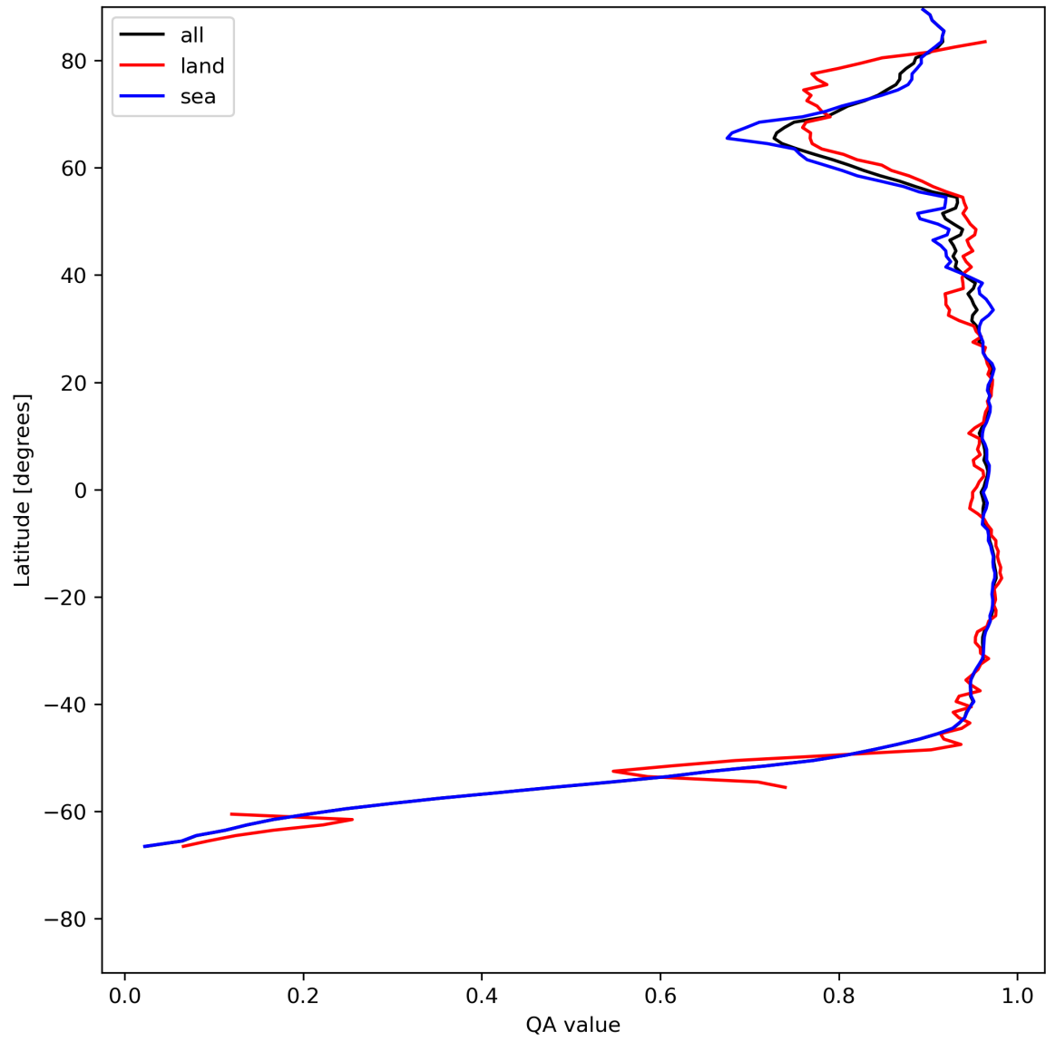
Figure 13: Zonal average of “QA value” for 2023-07-08 to 2023-07-10.
