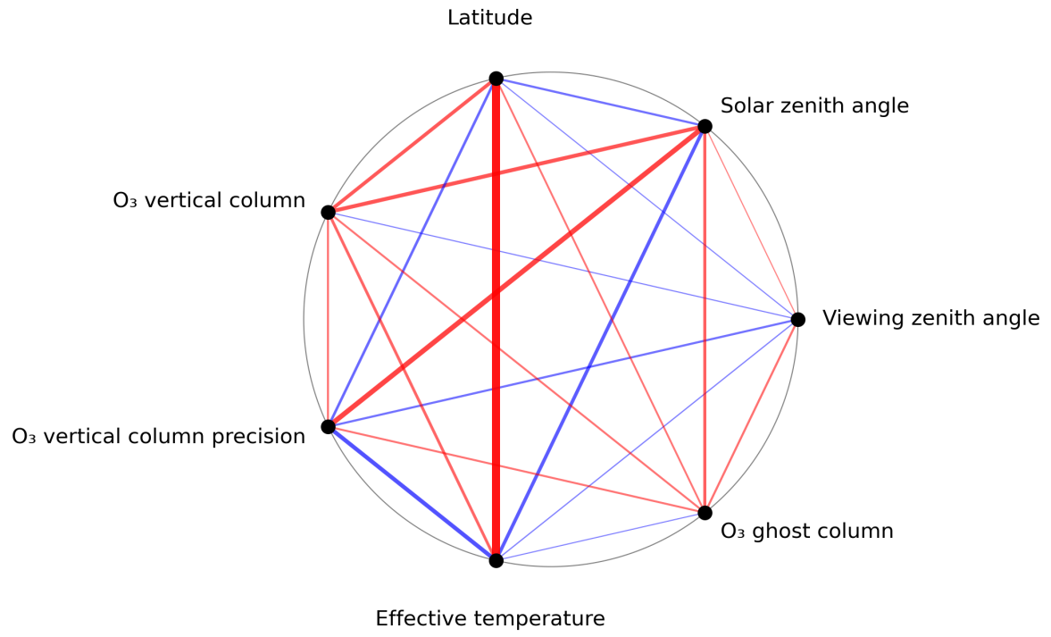
Figure 1: Map of correlation graph for 2023-07-08 to 2023-07-10.
