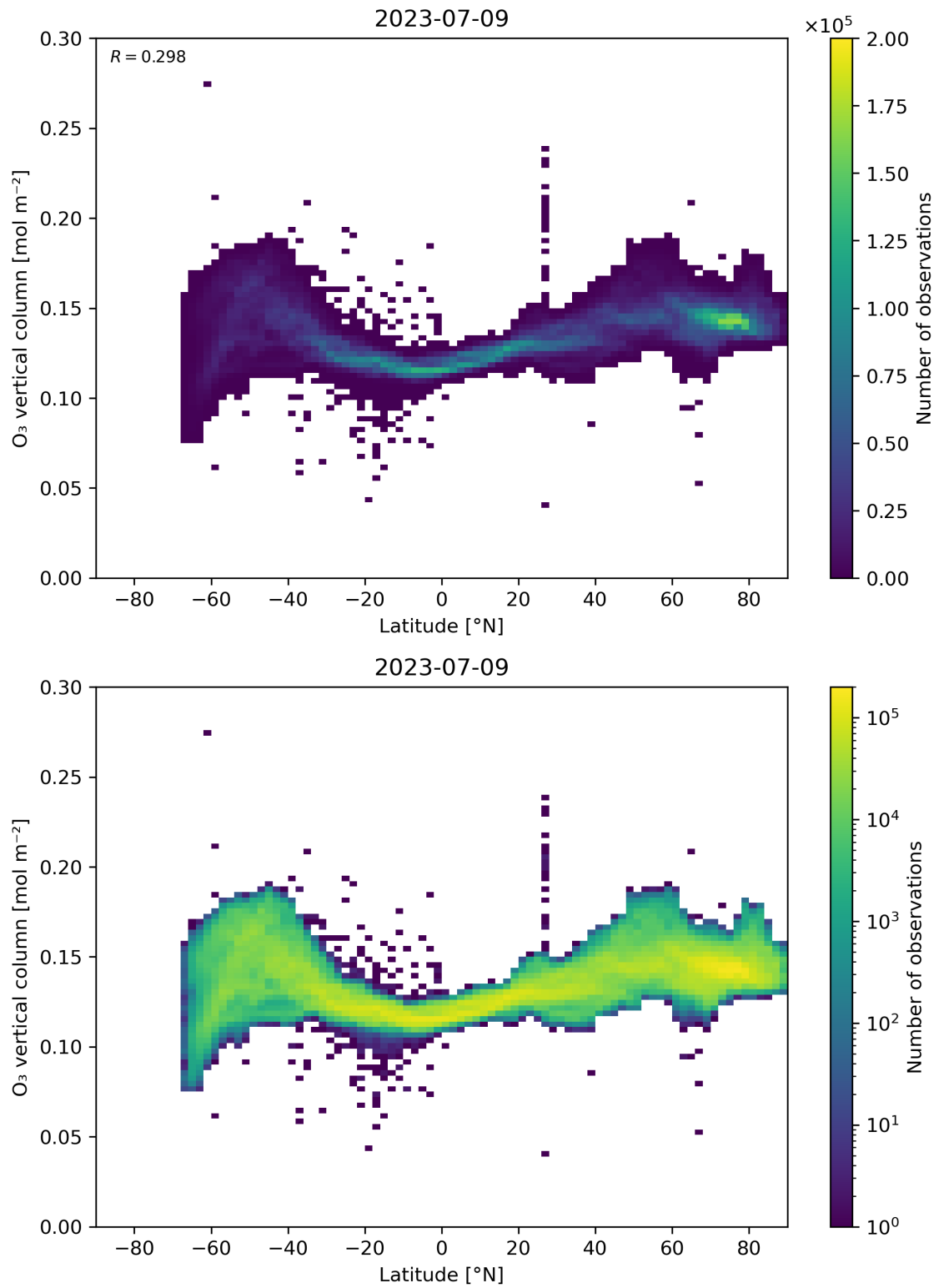
Figure 36: Scatter density plot of “Latitude” against “O 3 vertical column” for 2023-07-08 to 2023-07-10.
