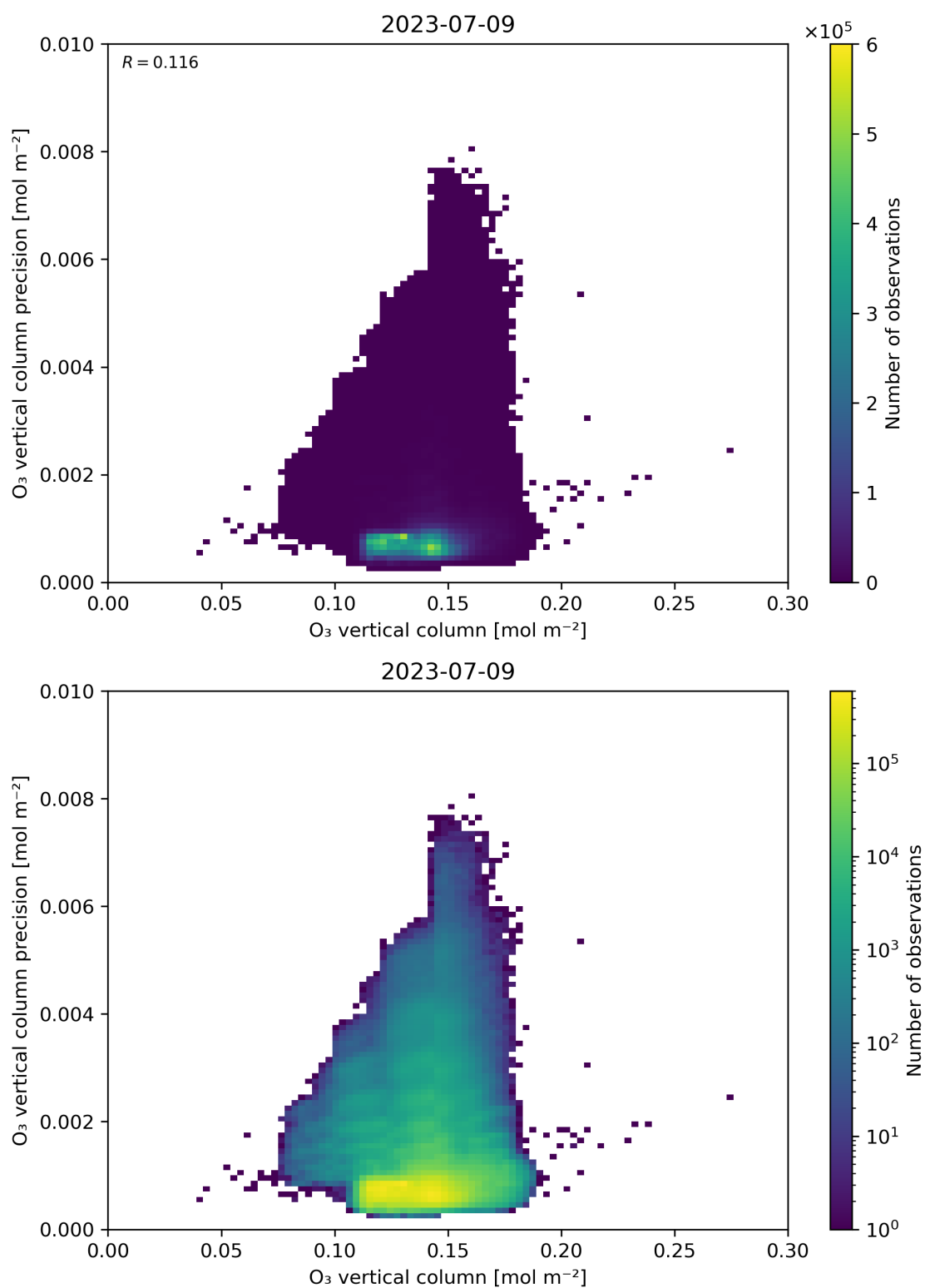
Figure 41: Scatter density plot of “O 3 vertical column” against “O 3 vertical column precision” for 2023-07-08 to 2023-07-10.
