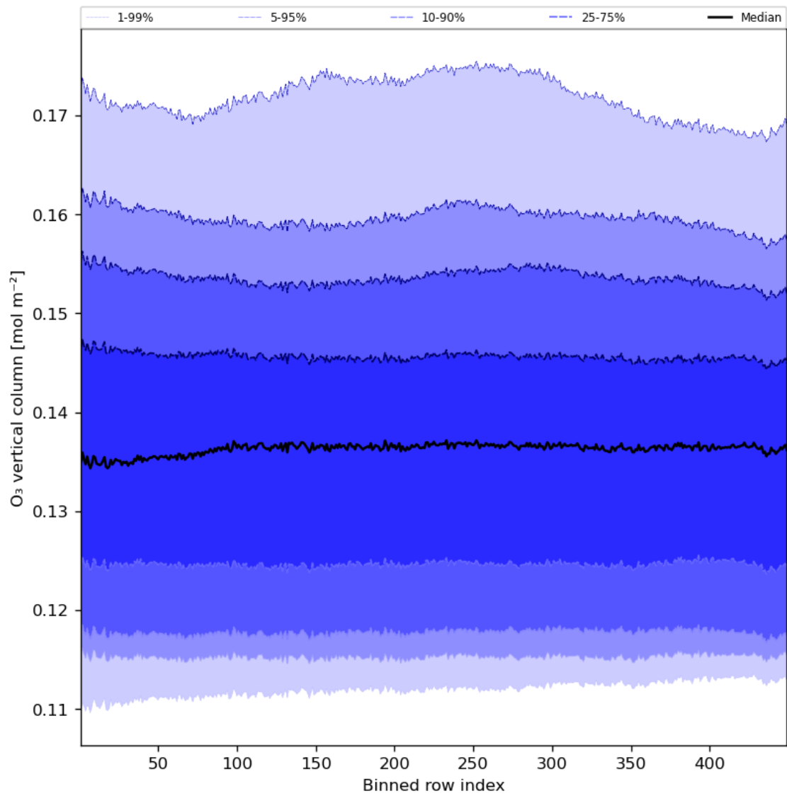
Figure 28: Along track statistics of “O 3 vertical column” for 2023-07-08 to 2023-07-10
