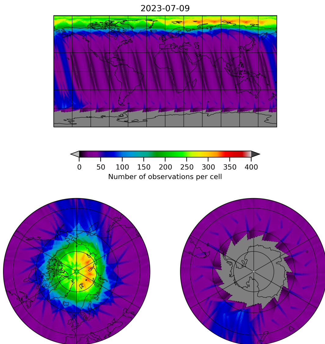
Figure 12: Map of the number of observations for 2023-07-08 to 2023-07-10
