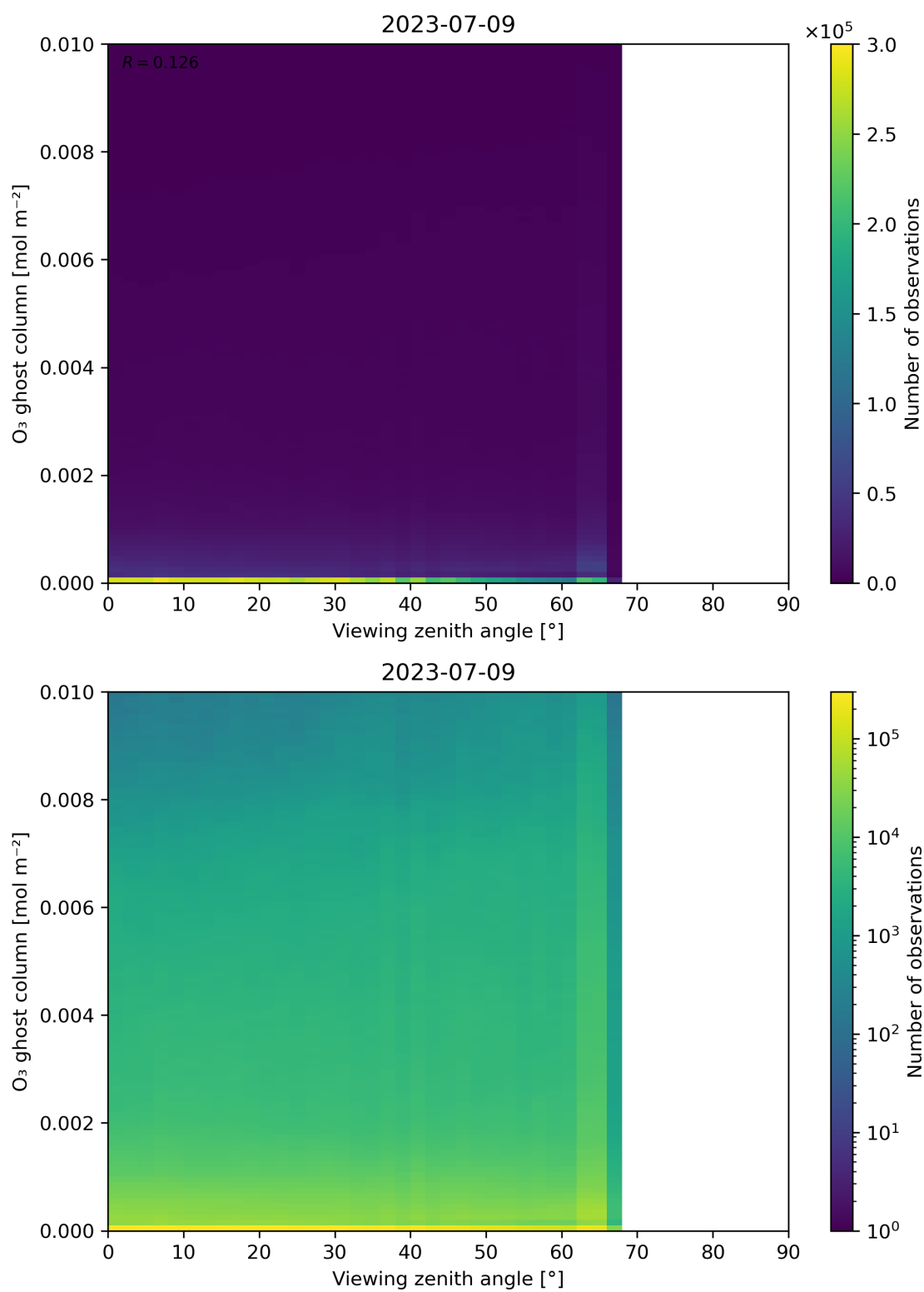
Figure 51: Scatter density plot of “Viewing zenith angle” against “O 3 ghost column” for 2023-07-08 to 2023-07-10.
