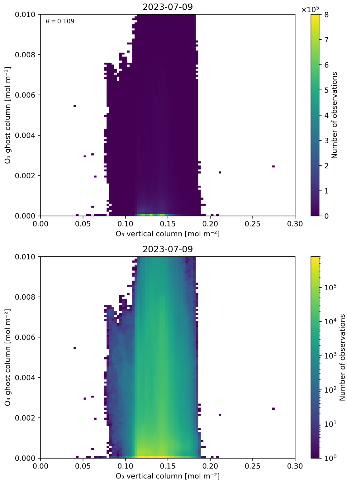
Figure 40: Scatter density plot of “O 3 vertical column” against “O 3 ghost column” for 2023-07-08 to 2023-07-10.
