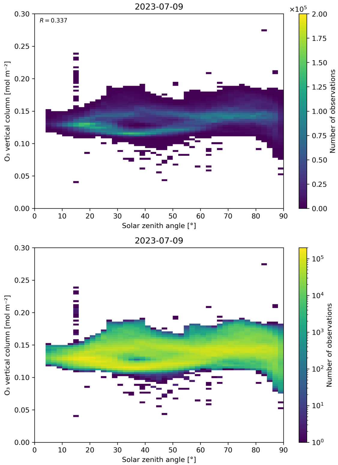
Figure 47: Scatter density plot of “Solar zenith angle” against “O 3 vertical column” for 2023-07-08 to 2023-07-10.
