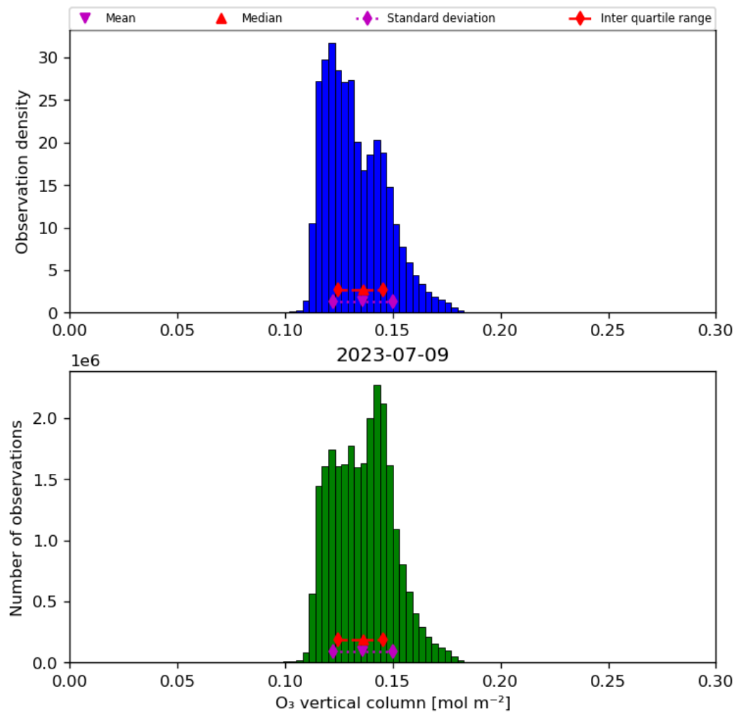
Figure 21: Histogram of “O 3 vertical column” for 2023-07-08 to 2023-07-10
