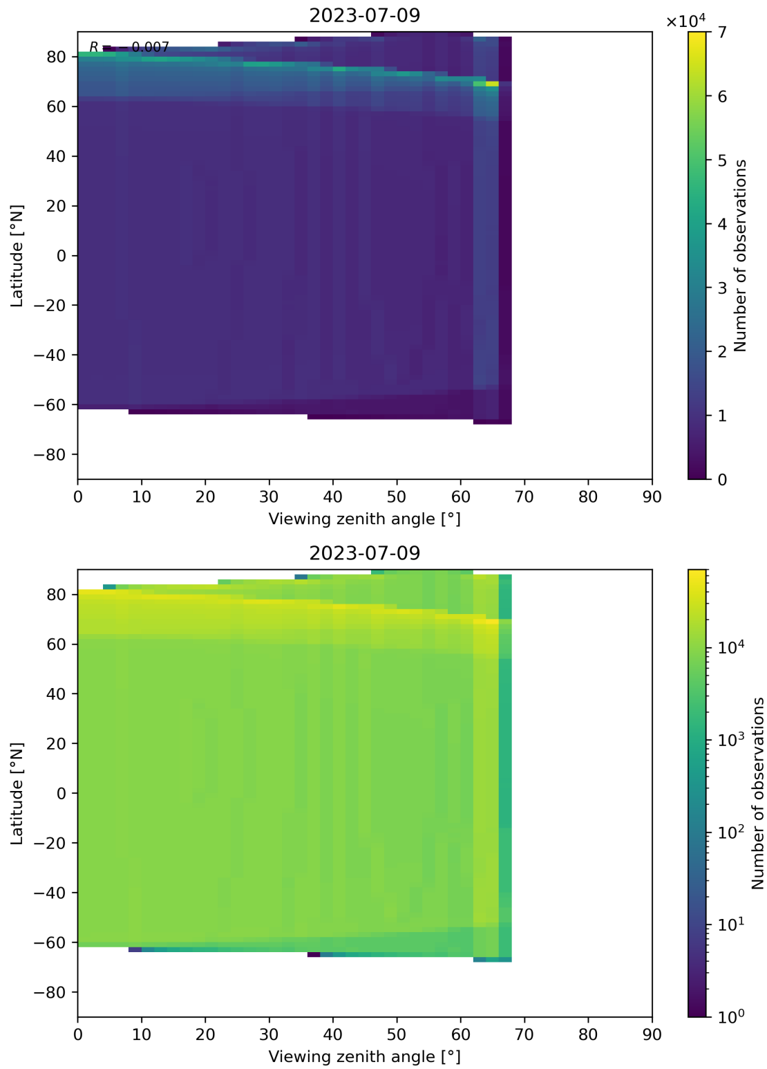
Figure 49: Scatter density plot of “Viewing zenith angle” against “Latitude” for 2023-07-08 to 2023-07-10.
