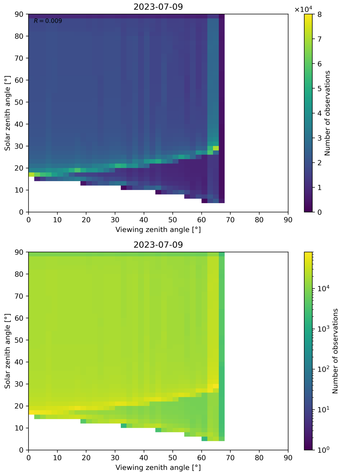
Figure 54: Scatter density plot of “Viewing zenith angle” against “Solar zenith angle” for 2023-07-08 to 2023-07-10.
