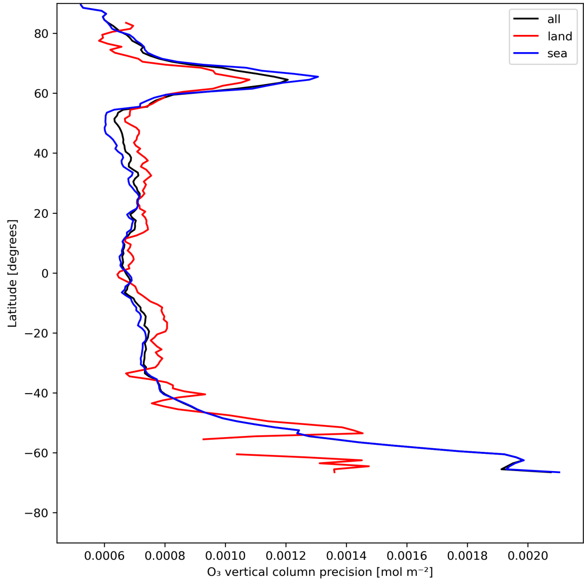
Figure 15: Zonal average of “O 3 vertical column precision” for 2023-07-08 to 2023-07-10.
