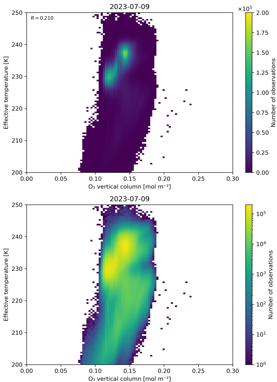
Figure 39: Scatter density plot of “O 3 vertical column” against “Effective temperature” for 2023-07-08 to 2023-07-10.
