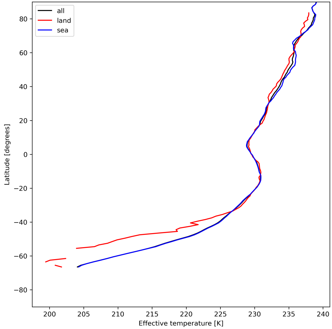
Figure 17: Zonal average of "Effective temperature" for 2023-07-09 to 2023-07-11.
