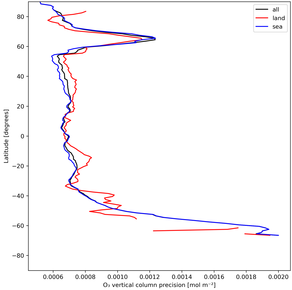
Figure 15: Zonal average of “O 3 vertical column precision” for 2023-07-09 to 2023-07-11.
