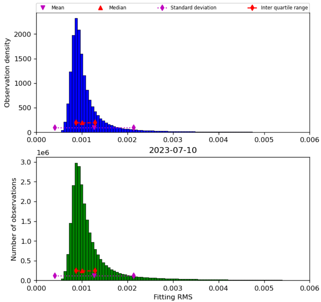
Figure 23: Histogram of “Fitting RMS” for 2023-07-09 to 2023-07-11
