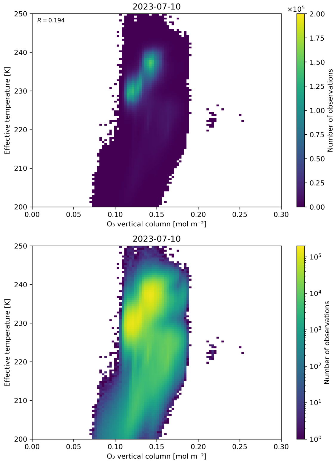
Figure 39: Scatter density plot of “O 3 vertical column” against “Effective temperature” for 2023-07-09 to 2023-07-11.
