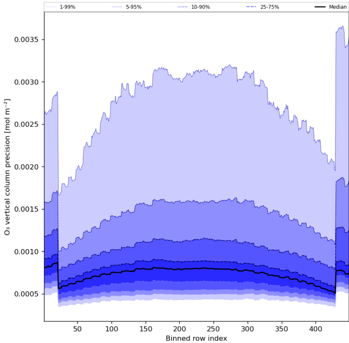
Figure 29: Along track statistics of “O 3 vertical column precision” for 2023-07-09 to 2023-07-11
