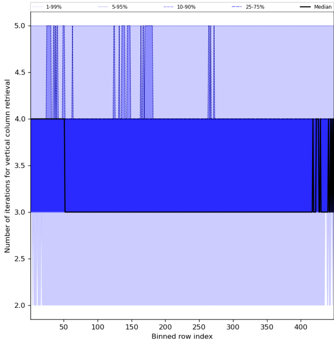
Figure 33: Along track statistics of “Number of iterations for vertical column retrieval” for 2023-07-09 to 2023-07-11
