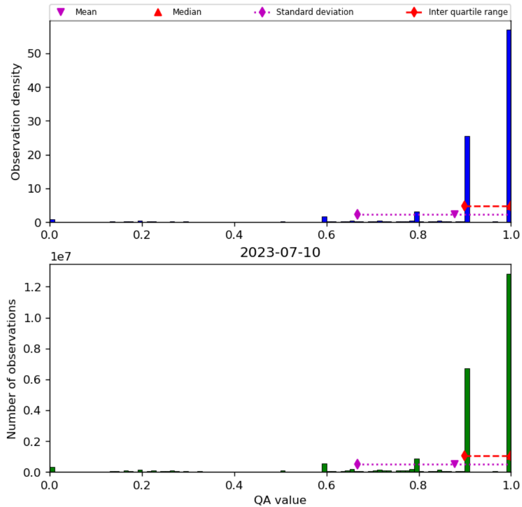
Figure 20: Histogram of “QA value” for 2023-07-09 to 2023-07-11
