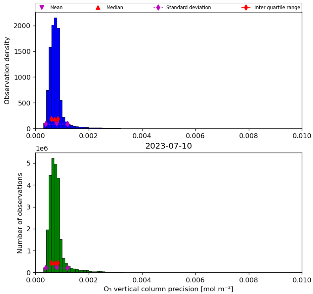
Figure 22: Histogram of “O 3 vertical column precision” for 2023-07-09 to 2023-07-11
