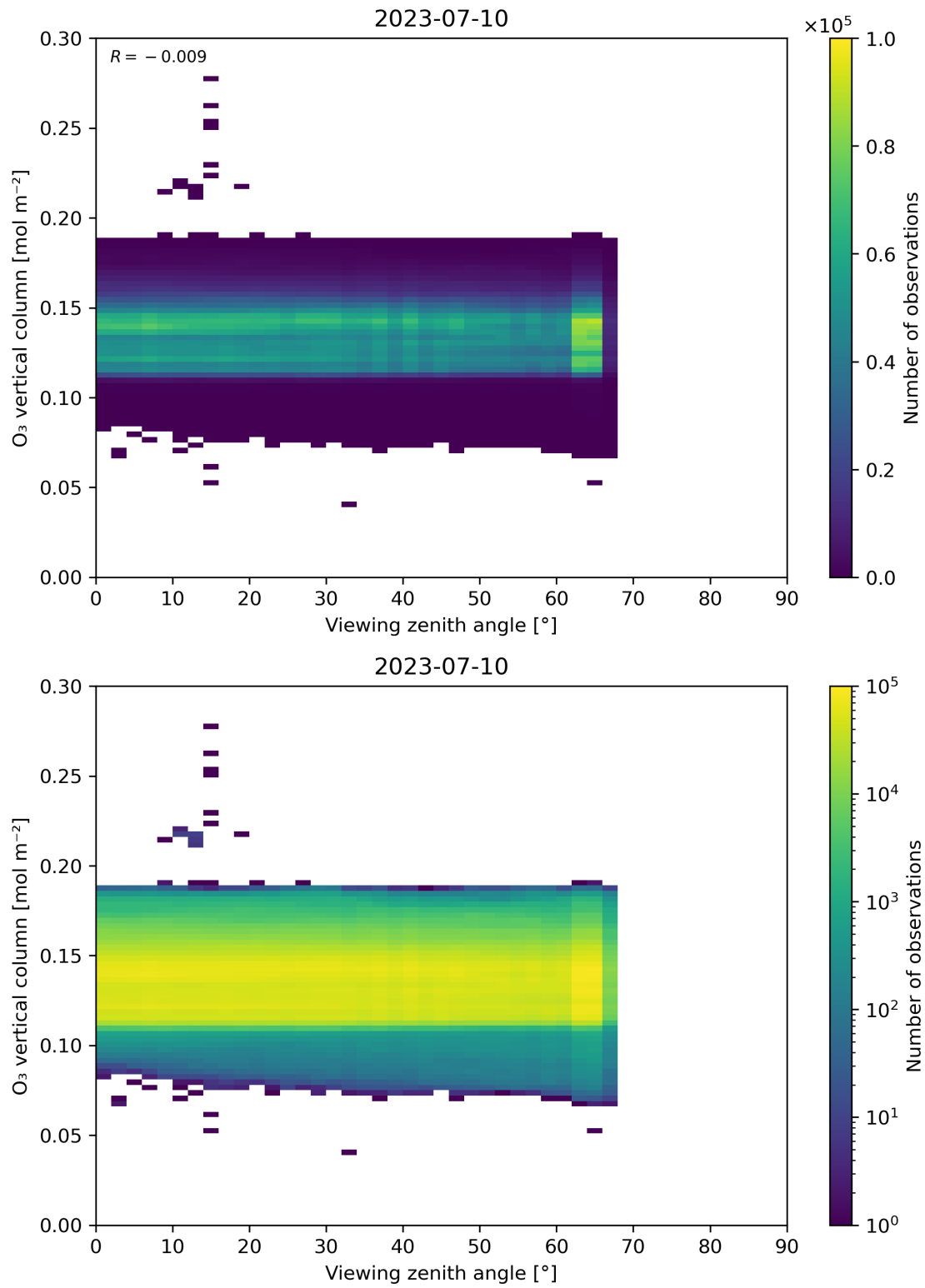
Figure 52: Scatter density plot of “Viewing zenith angle” against “O 3 vertical column” for 2023-07-09 to 2023-07-11.
