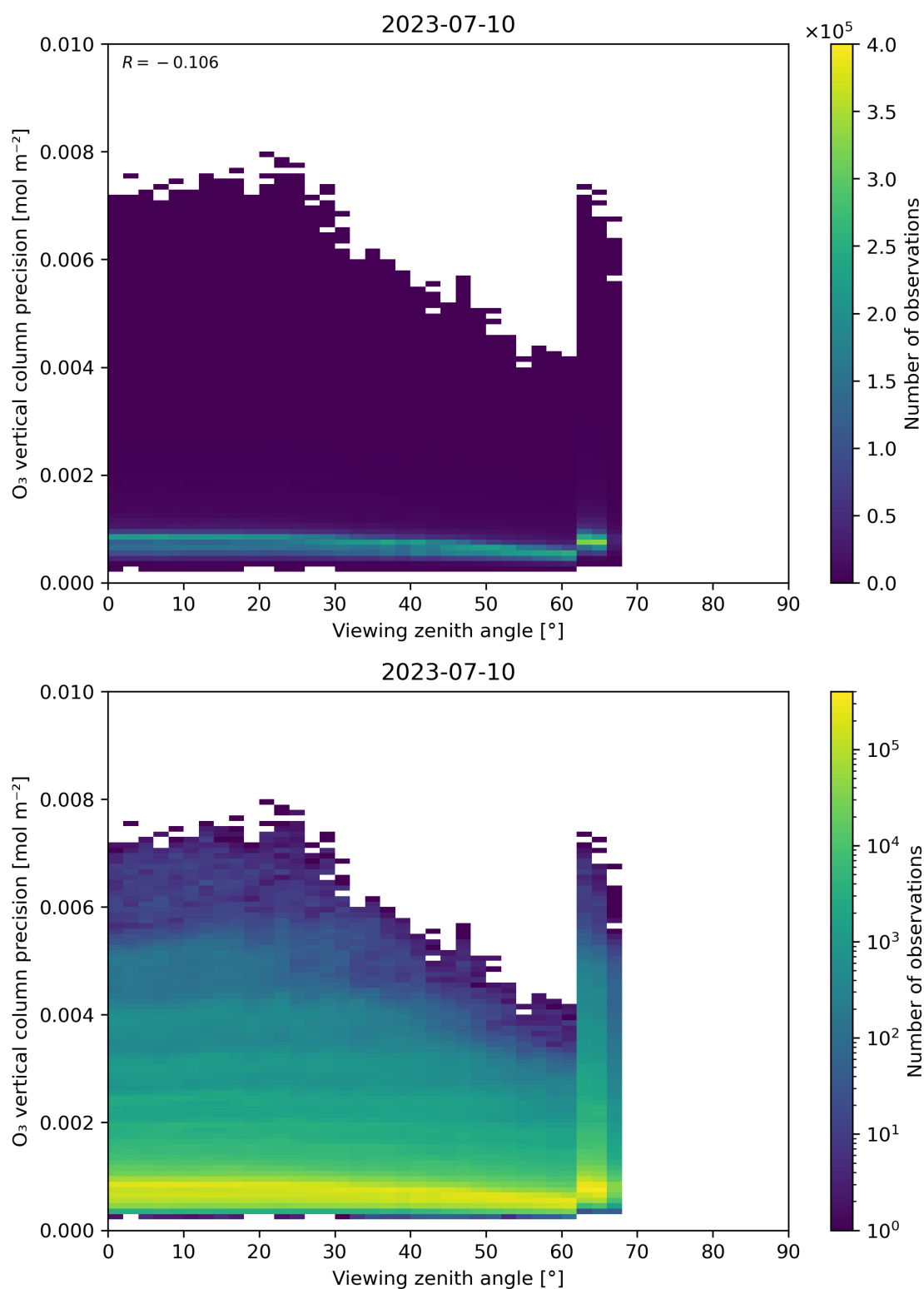
Figure 53: Scatter density plot of “Viewing zenith angle” against “O 3 vertical column precision” for 2023-07-09 to 2023-07-11.
