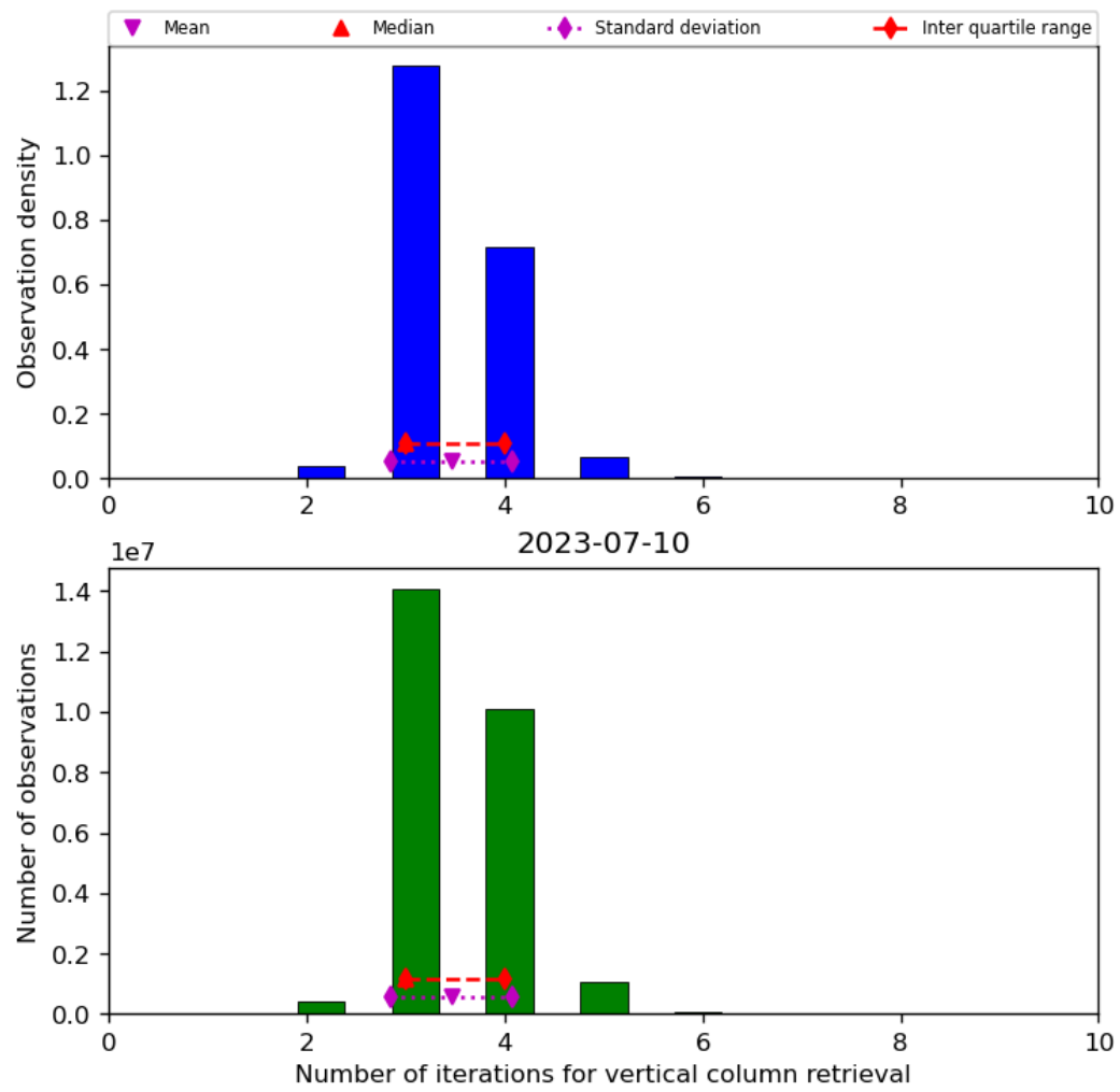
Figure 26: Histogram of “Number of iterations for vertical column retrieval” for 2023-07-09 to 2023-07-11
