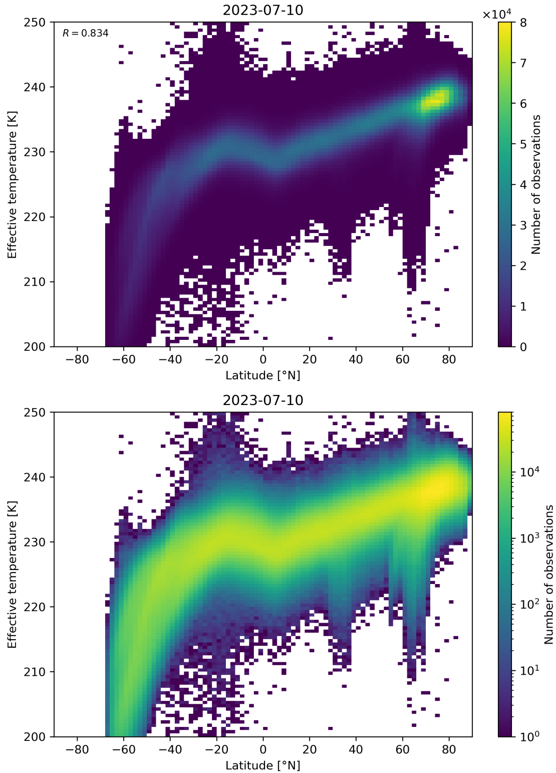
Figure 34: Scatter density plot of “Latitude” against “Effective temperature” for 2023-07-09 to 2023-07-11.
