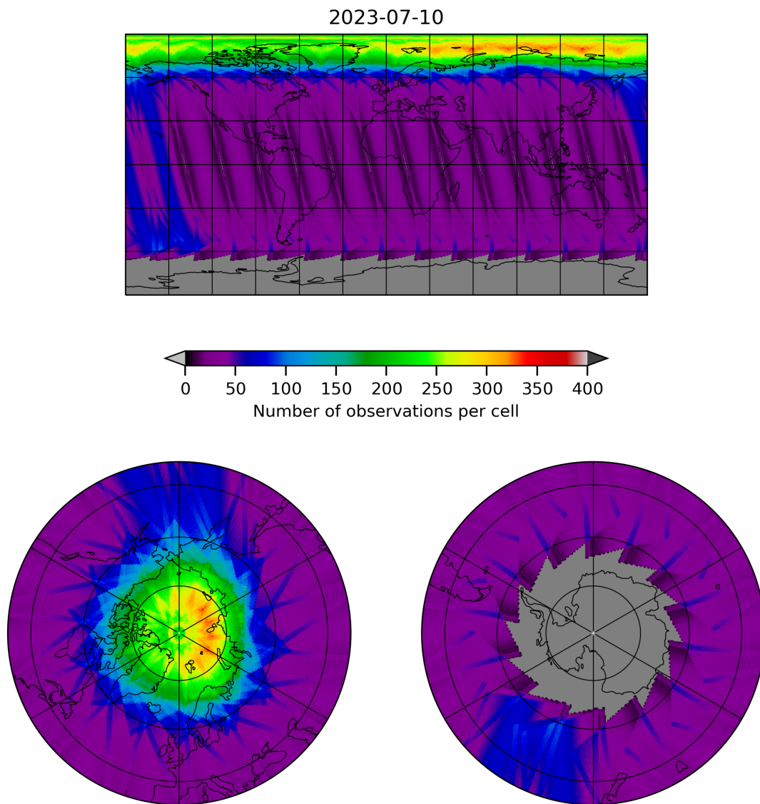
Figure 12: Map of the number of observations for 2023-07-09 to 2023-07-11
