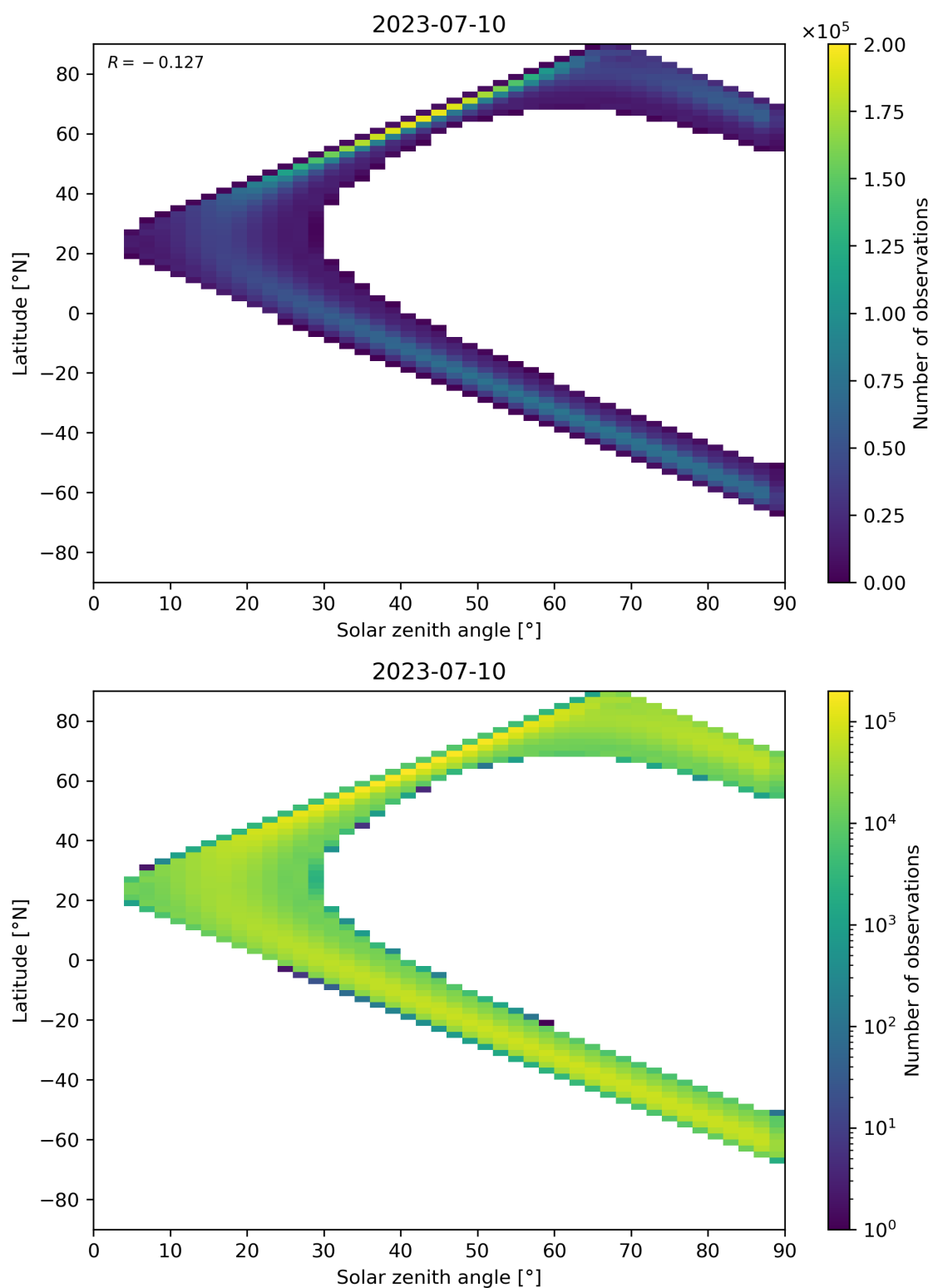
Figure 44: Scatter density plot of “Solar zenith angle” against “Latitude” for 2023-07-09 to 2023-07-11.
