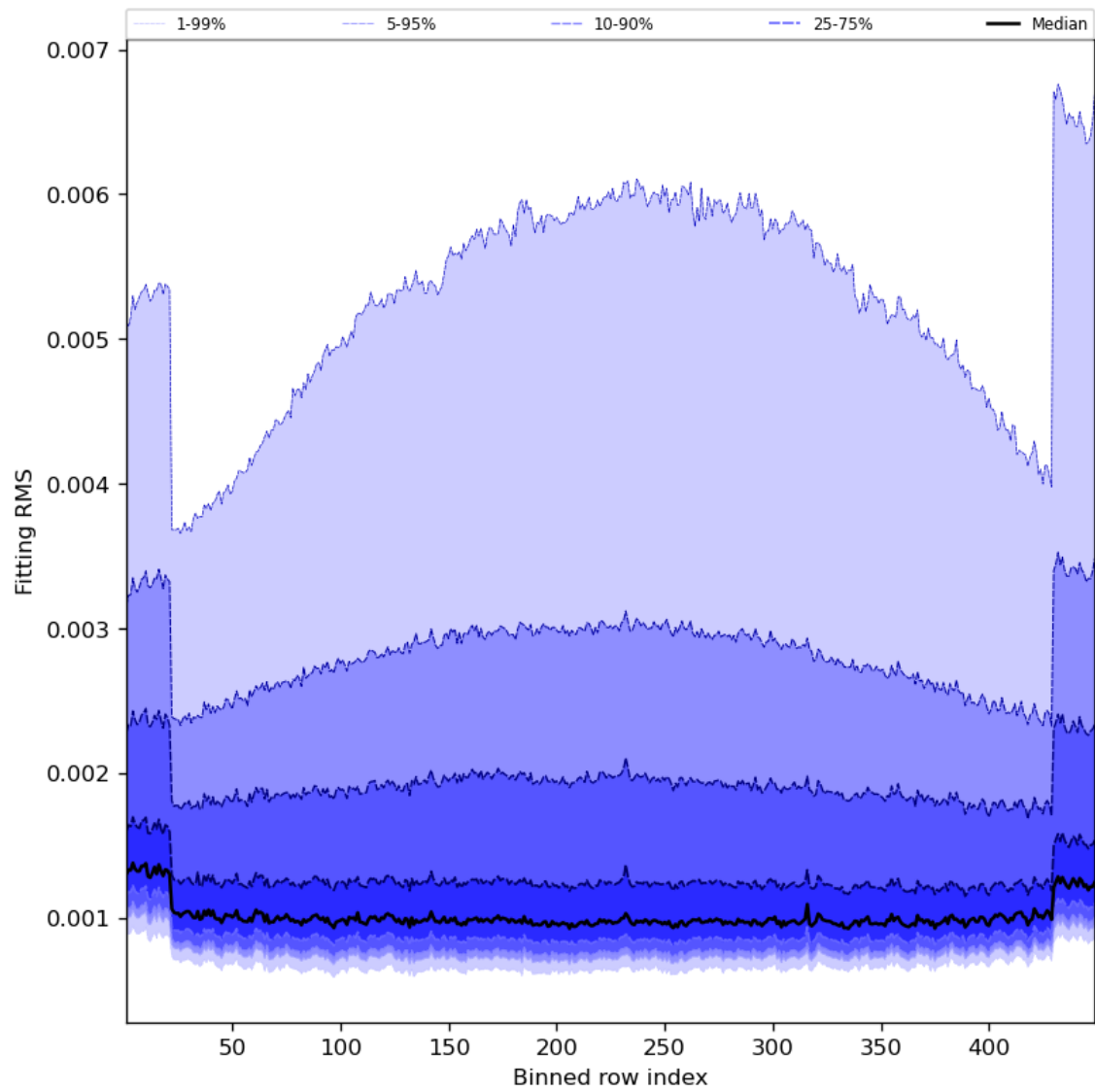
Figure 30: Along track statistics of “Fitting RMS” for 2023-07-09 to 2023-07-11
