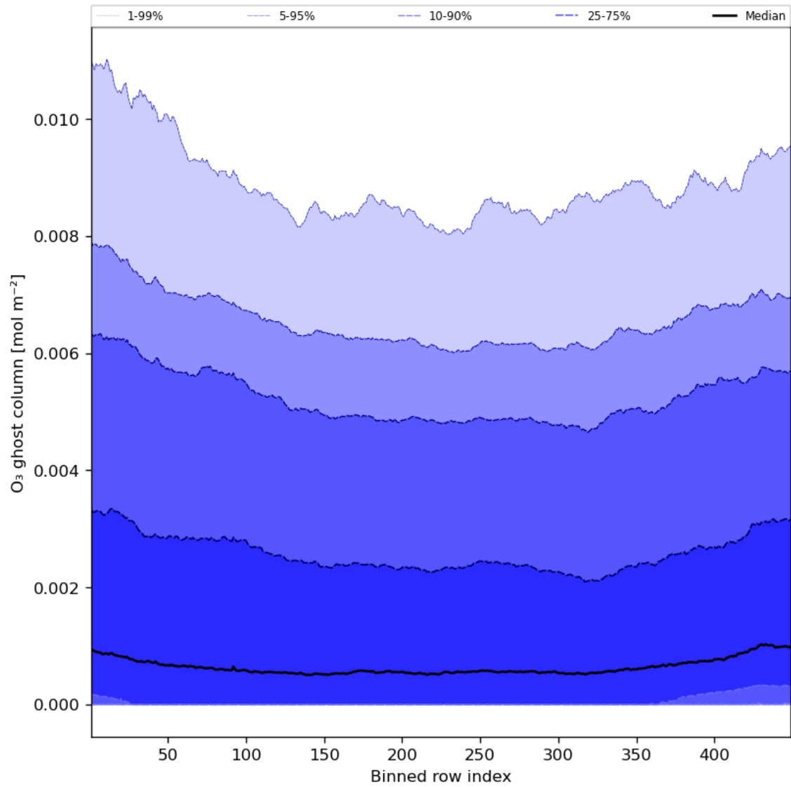
Figure 32: Along track statistics of “O 3 ghost column” for 2023-07-09 to 2023-07-11
