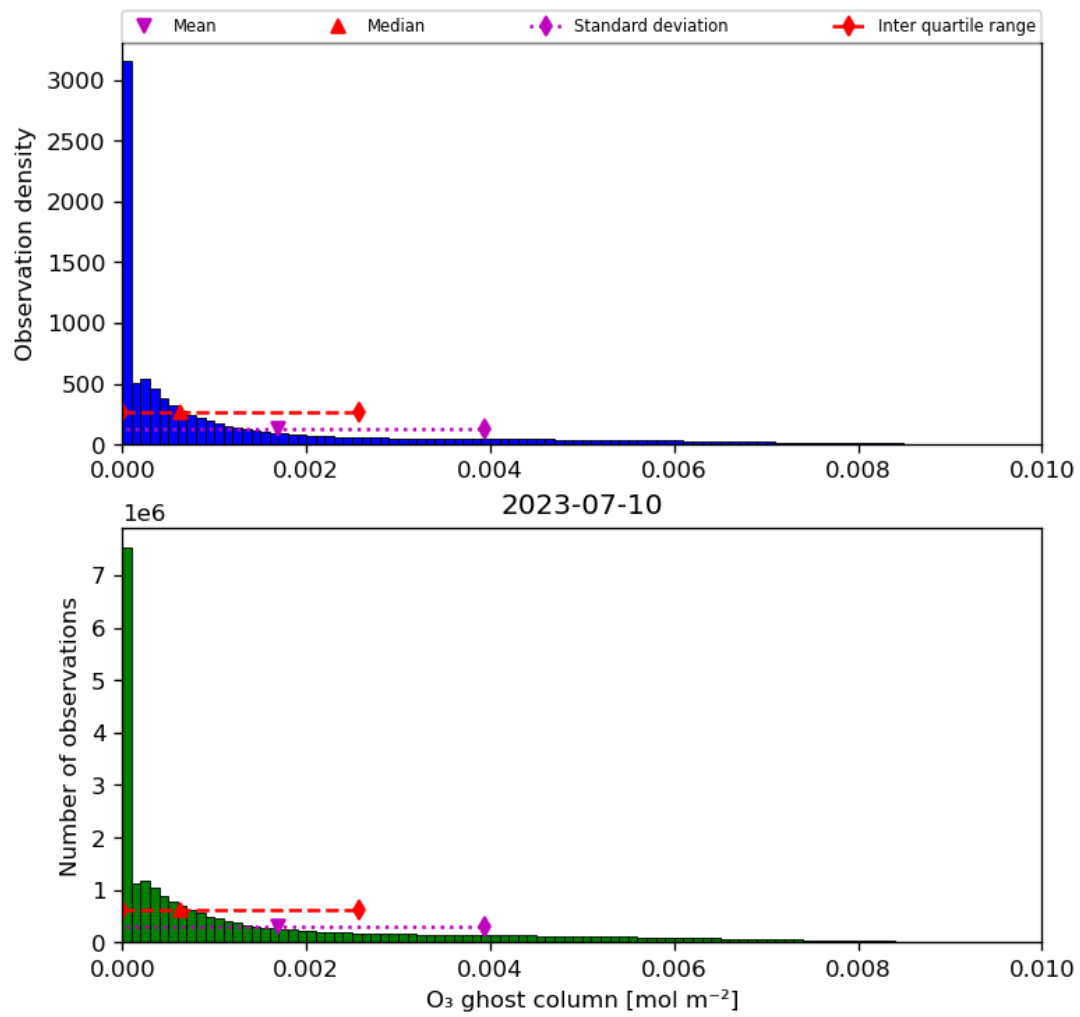
Figure 25: Histogram of “O 3 ghost column” for 2023-07-09 to 2023-07-11
