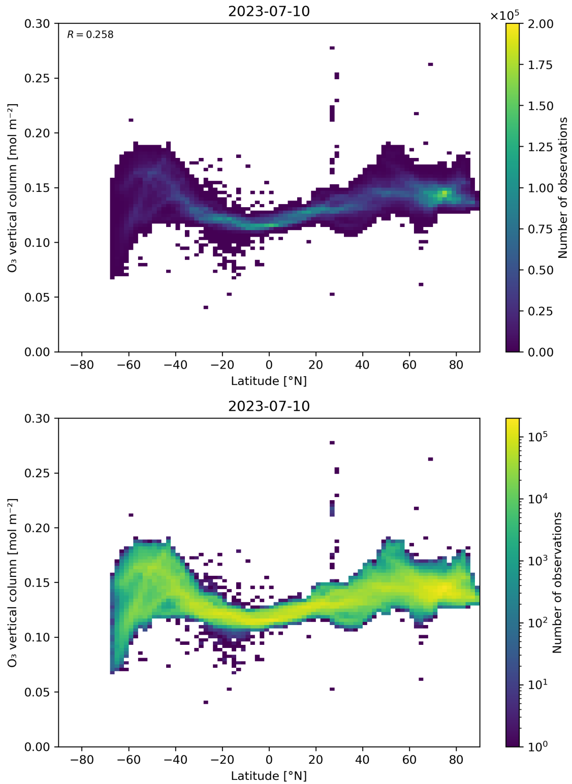
Figure 36: Scatter density plot of “Latitude” against “O 3 vertical column” for 2023-07-09 to 2023-07-11.
