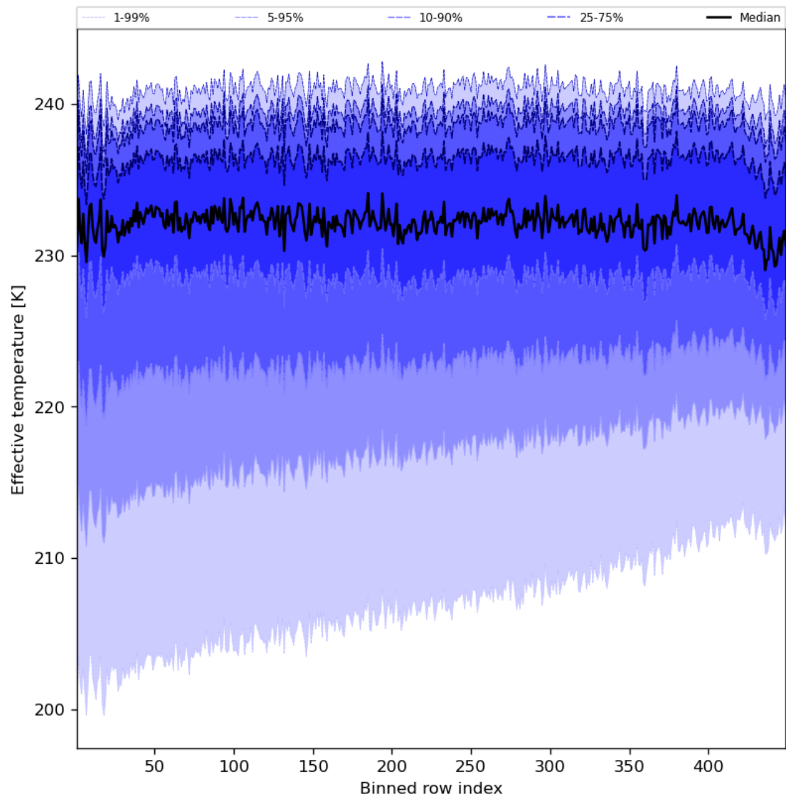
Figure 31: Along track statistics of “Effective temperature” for 2023-07-09 to 2023-07-11
