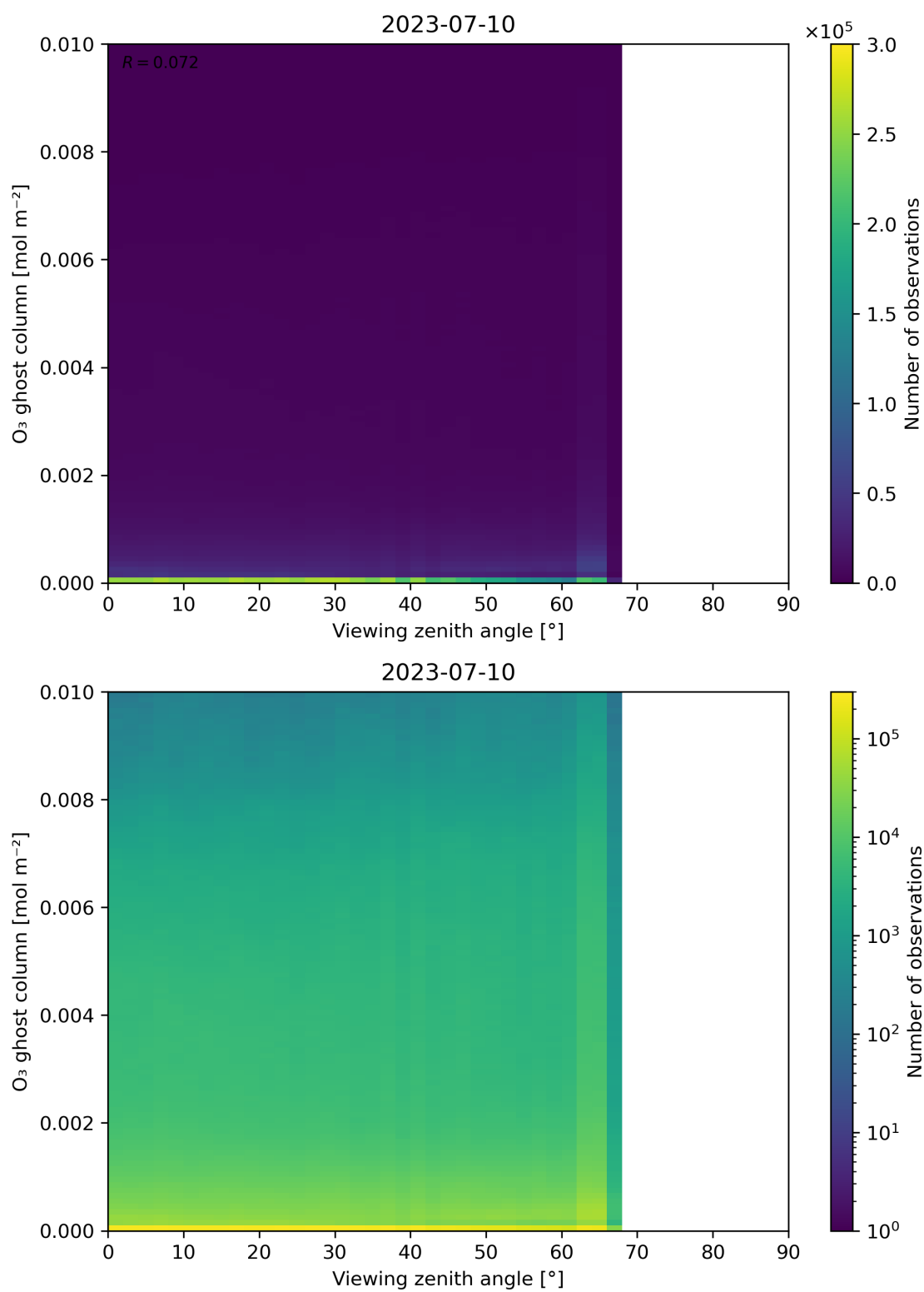
Figure 51: Scatter density plot of “Viewing zenith angle” against “O 3 ghost column” for 2023-07-09 to 2023-07-11.
