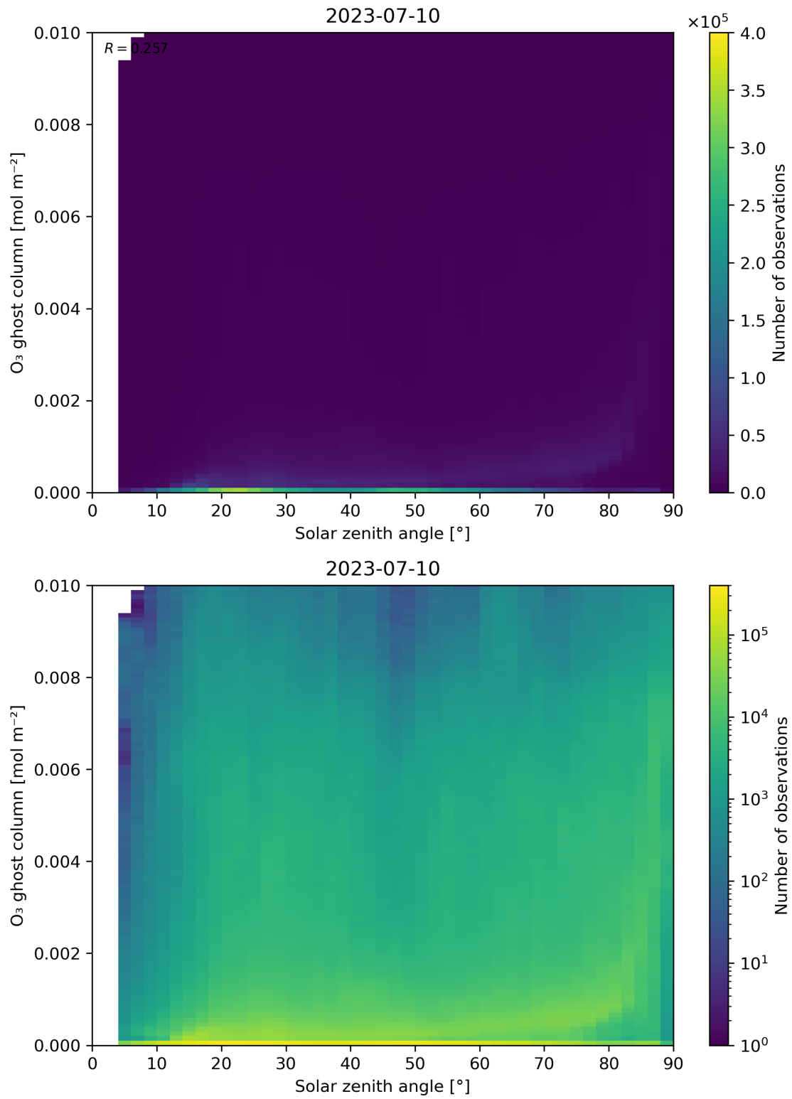
Figure 46: Scatter density plot of “Solar zenith angle” against “O 3 ghost column” for 2023-07-09 to 2023-07-11.
