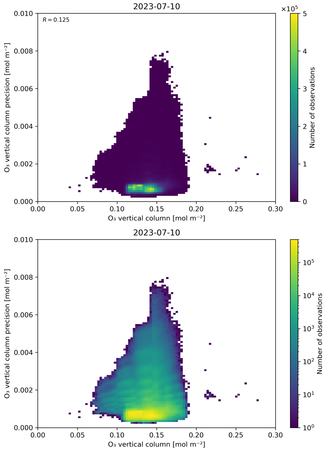
Figure 41: Scatter density plot of “O 3 vertical column” against “O 3 vertical column precision” for 2023-07-09 to 2023-07-11.
