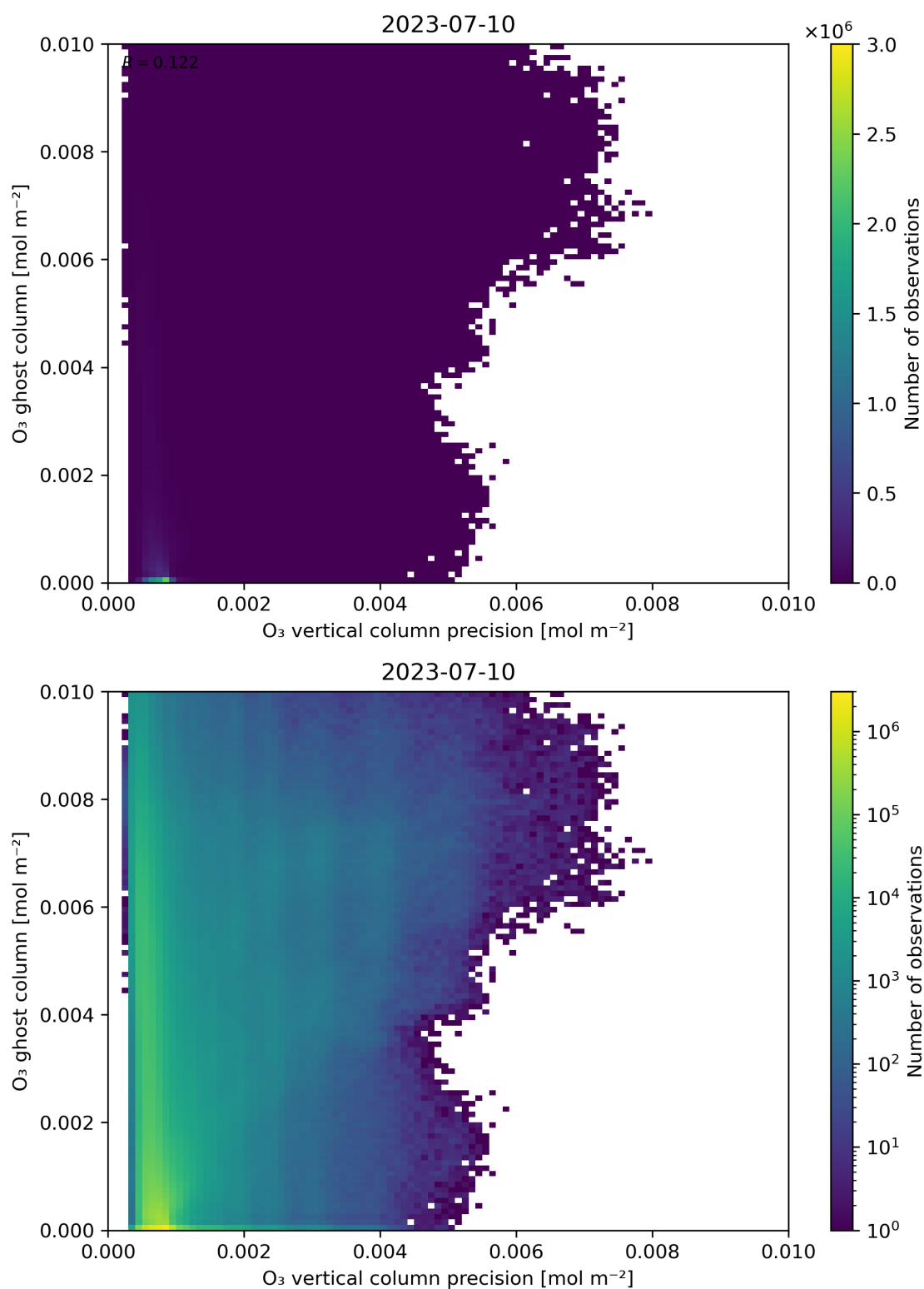
Figure 43: Scatter density plot of “ \text{O}_3 vertical column precision” against “ \text{O}_3 ghost column” for 2023-07-09 to 2023-07-11.
