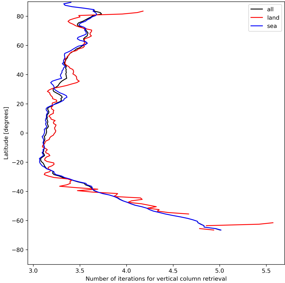
Figure 19: Zonal average of “Number of iterations for vertical column retrieval” for 2023-07-09 to 2023-07-11.
