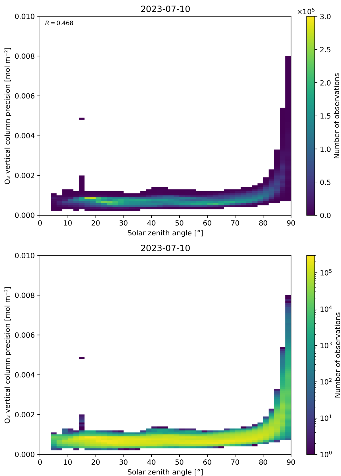
Figure 48: Scatter density plot of “Solar zenith angle” against “O 3 vertical column precision” for 2023-07-09 to 2023-07-11.
