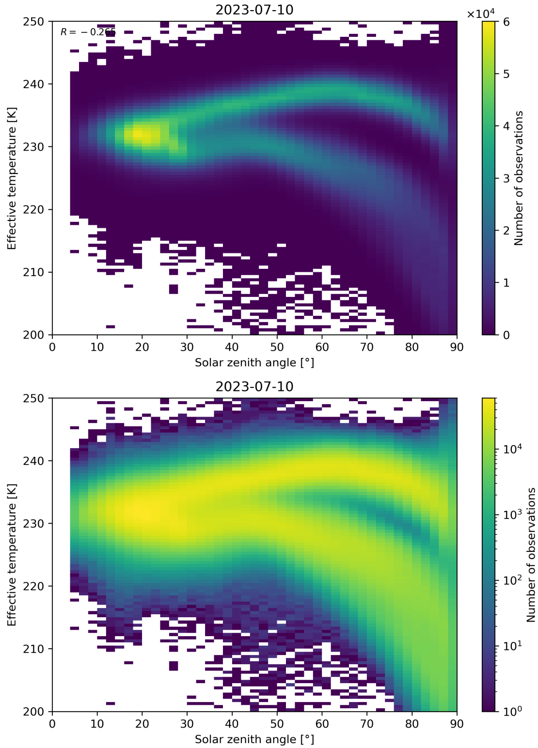
Figure 45: Scatter density plot of “Solar zenith angle” against “Effective temperature” for 2023-07-09 to 2023-07-11.
