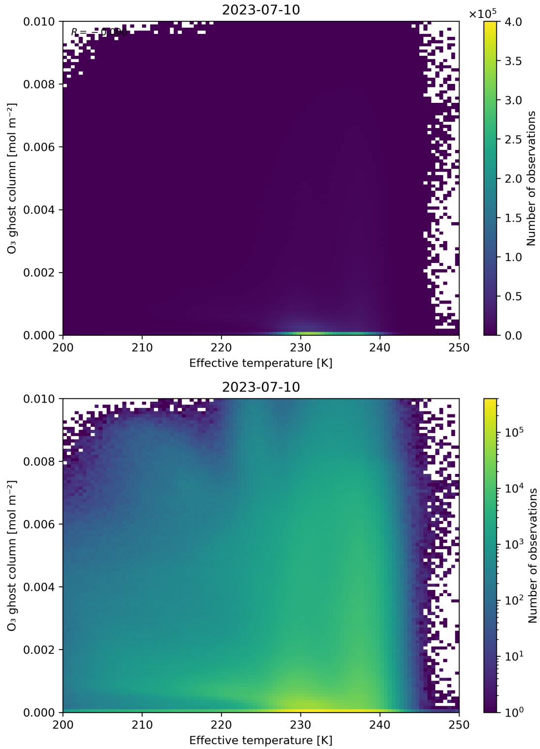
Figure 38: Scatter density plot of “Effective temperature” against “O 3 ghost column” for 2023-07-09 to 2023-07-11.
