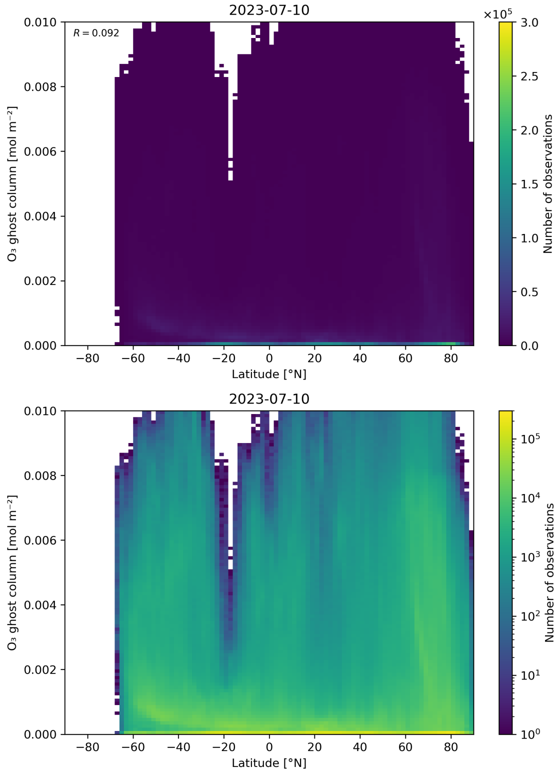
Figure 35: Scatter density plot of “Latitude” against “O 3 ghost column” for 2023-07-09 to 2023-07-11.
