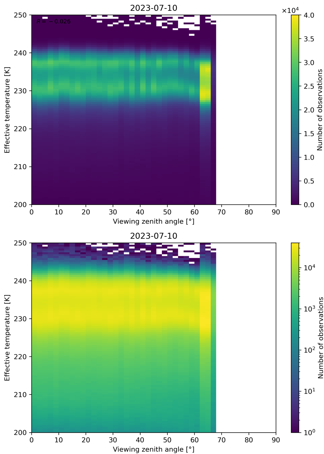
Figure 50: Scatter density plot of “Viewing zenith angle” against “Effective temperature” for 2023-07-09 to 2023-07-11.
