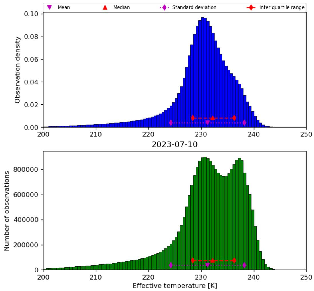
Figure 24: Histogram of “Effective temperature” for 2023-07-09 to 2023-07-11
