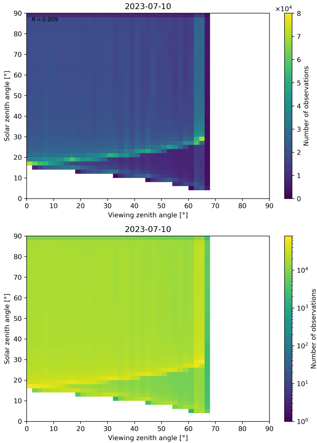
Figure 54: Scatter density plot of “Viewing zenith angle” against “Solar zenith angle” for 2023-07-09 to 2023-07-11.
