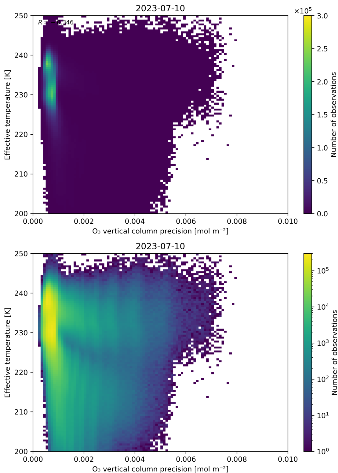
Figure 42: Scatter density plot of “O 3 vertical column precision” against “Effective temperature” for 2023-07-09 to 2023-07-11.
