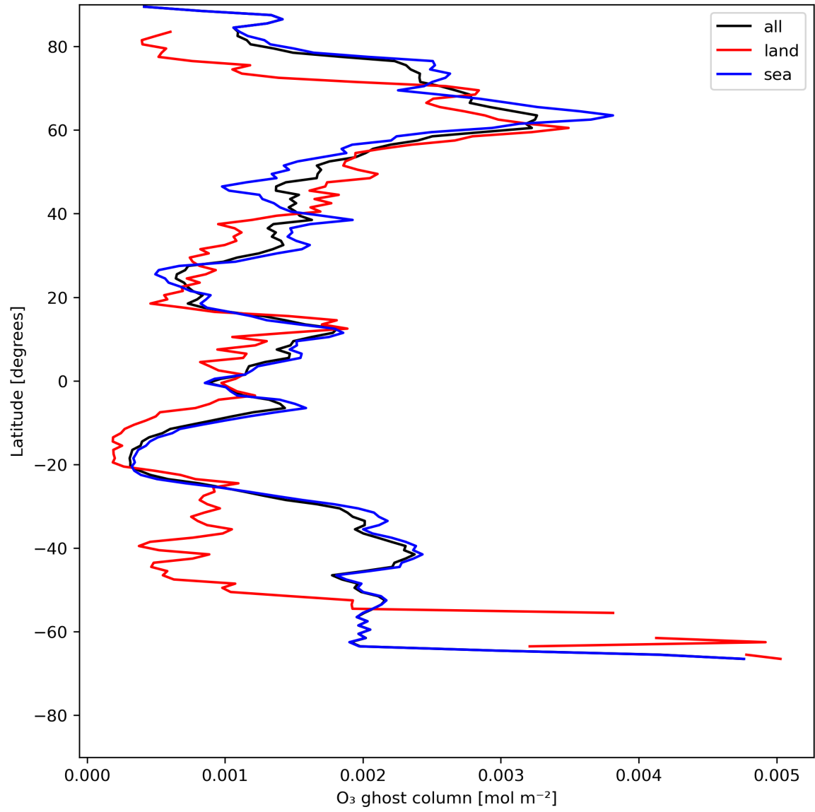
Figure 18: Zonal average of “O 3 ghost column” for 2023-07-09 to 2023-07-11.
