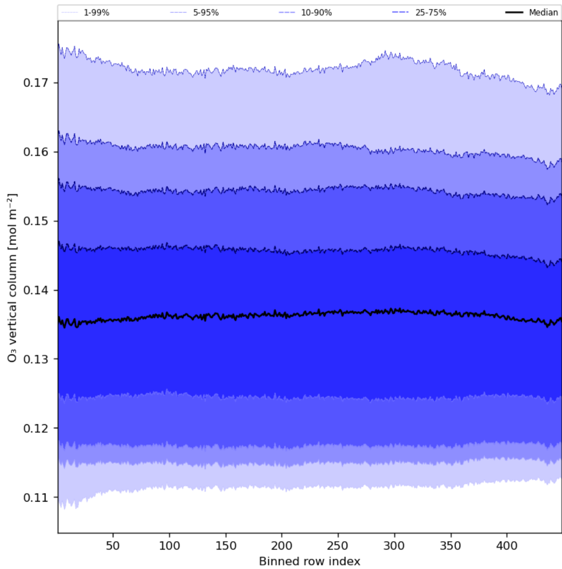
Figure 28: Along track statistics of “O 3 vertical column” for 2023-07-09 to 2023-07-11
