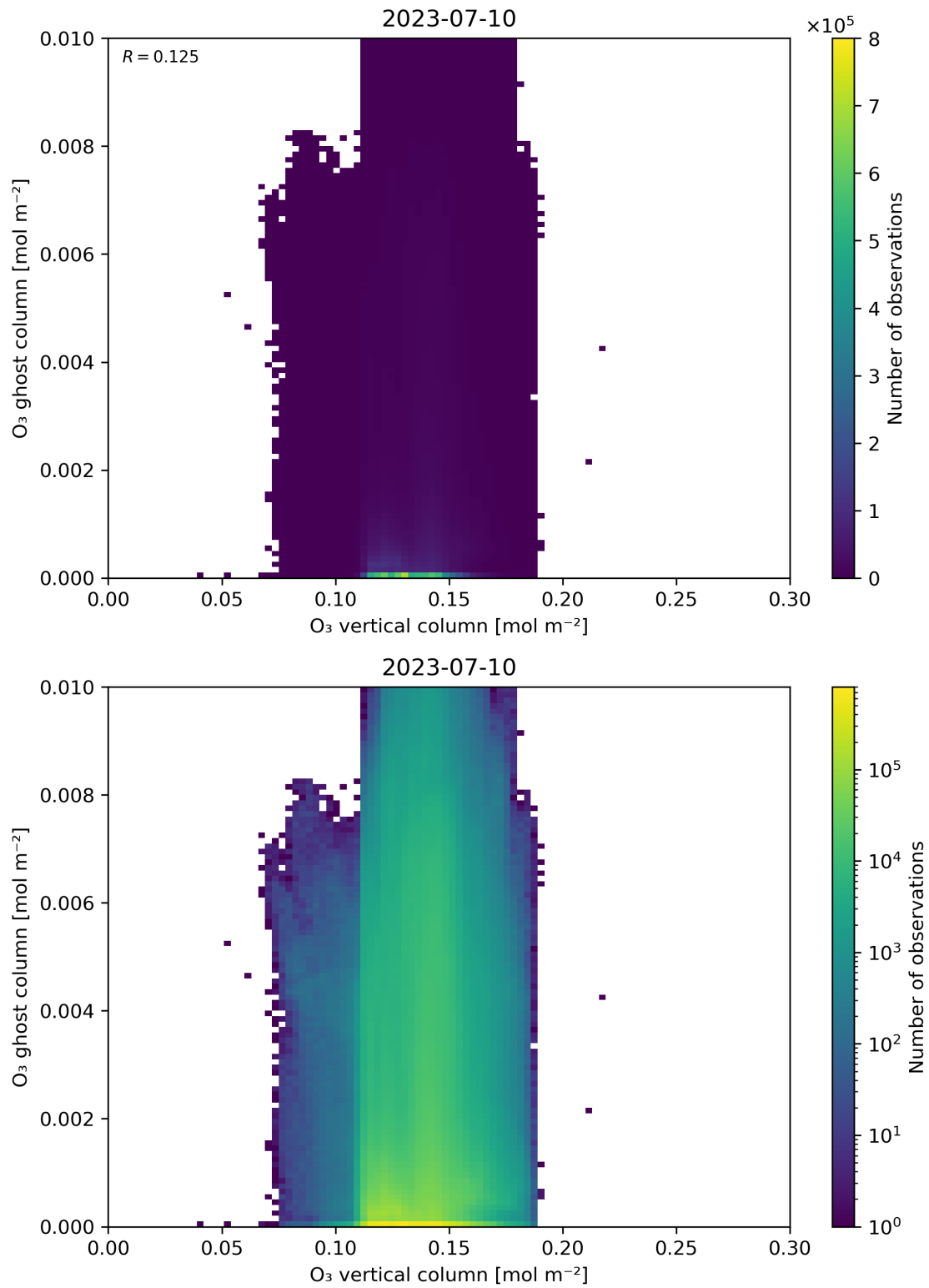
Figure 40: Scatter density plot of “O 3 vertical column” against “O 3 ghost column” for 2023-07-09 to 2023-07-11.
