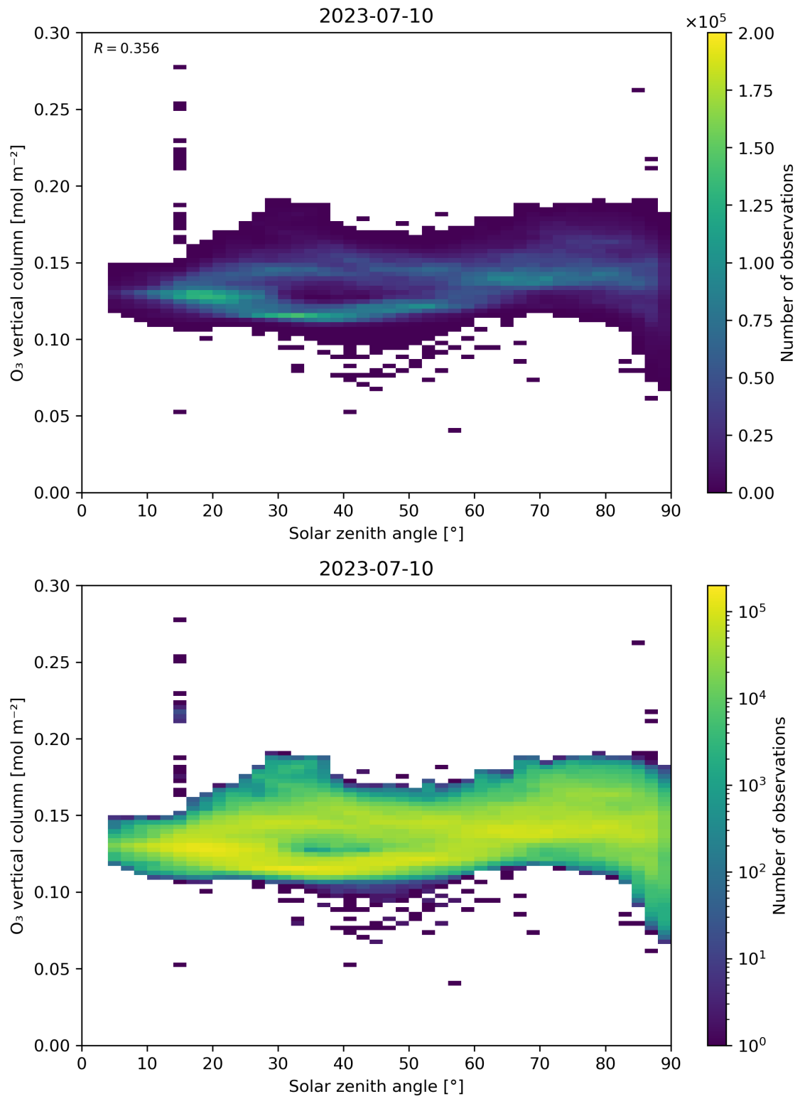
Figure 47: Scatter density plot of “Solar zenith angle” against “O 3 vertical column” for 2023-07-09 to 2023-07-11.
