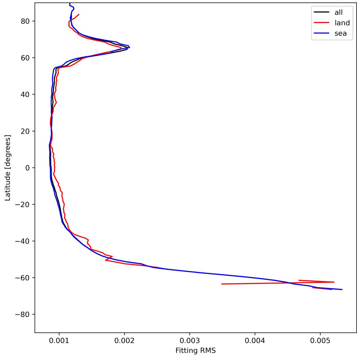
Figure 16: Zonal average of “Fitting RMS” for 2023-07-09 to 2023-07-11.
