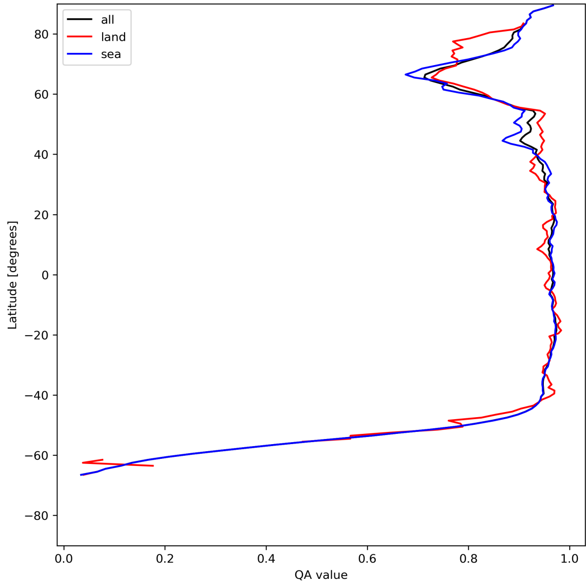
Figure 13: Zonal average of “QA value” for 2023-07-09 to 2023-07-11.
