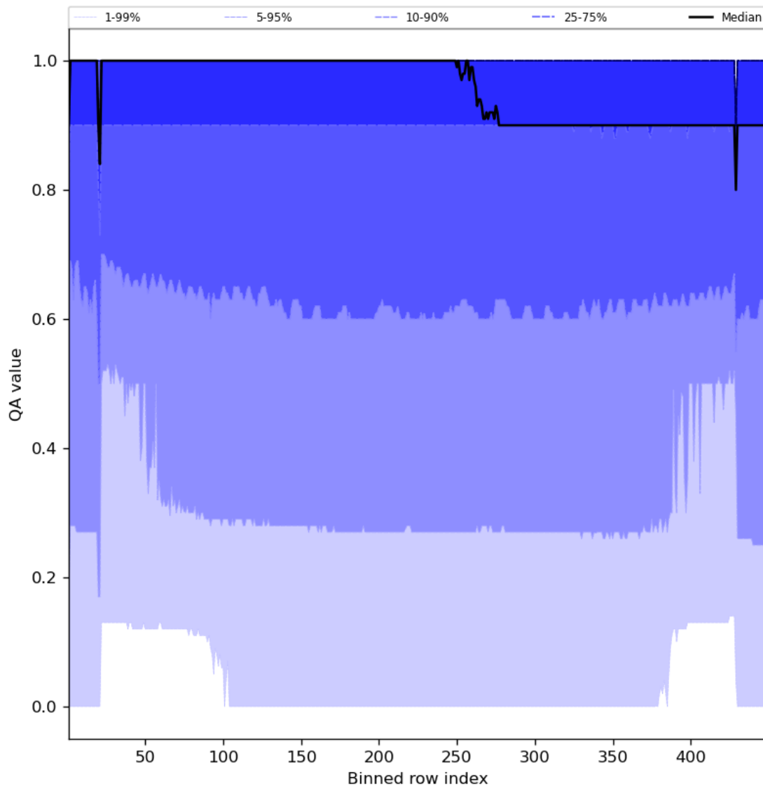
Figure 27: Along track statistics of “QA value” for 2023-07-09 to 2023-07-11
