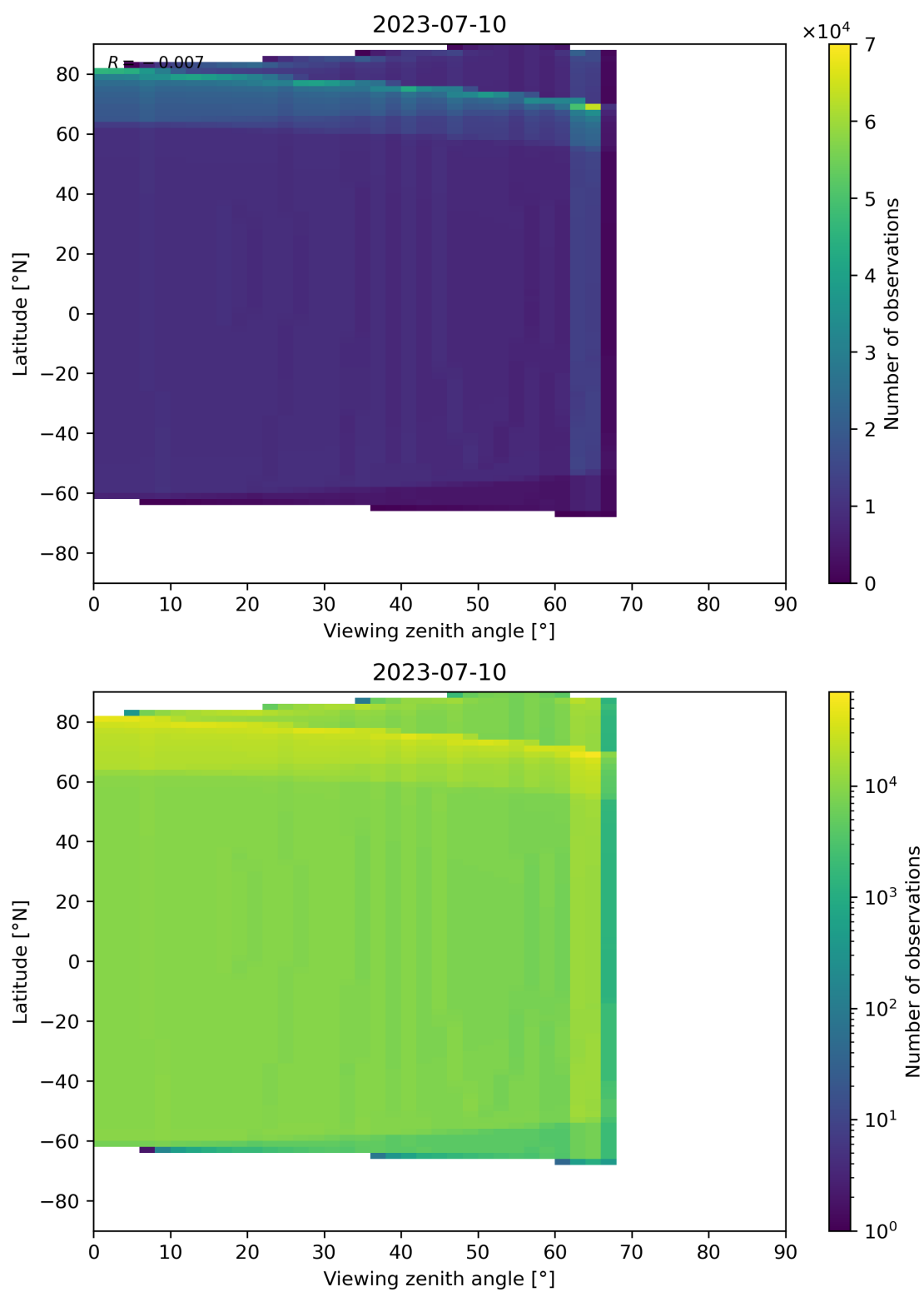
Figure 49: Scatter density plot of “Viewing zenith angle” against “Latitude” for 2023-07-09 to 2023-07-11.
