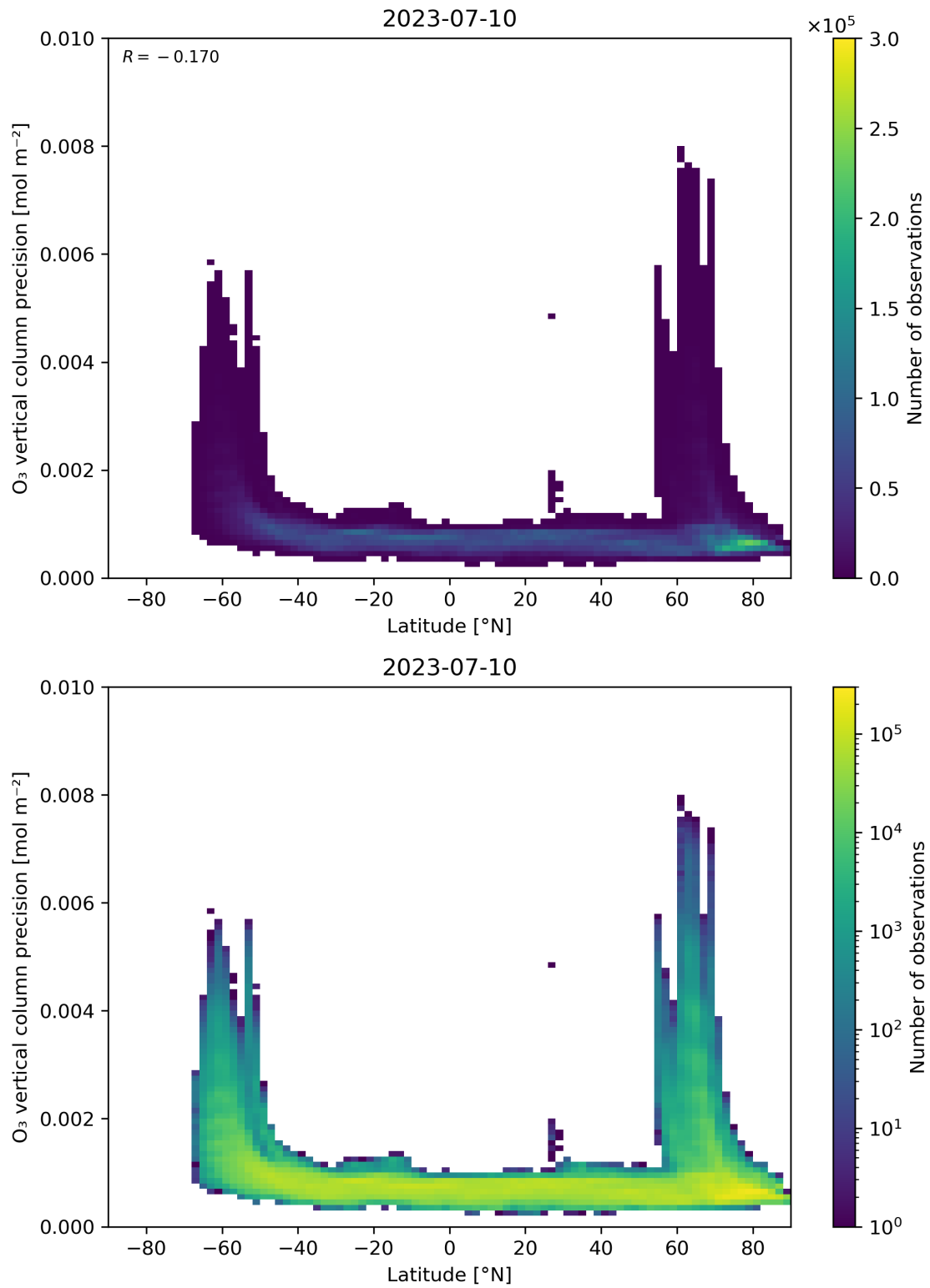
Figure 37: Scatter density plot of “Latitude” against “O 3 vertical column precision” for 2023-07-09 to 2023-07-11.
