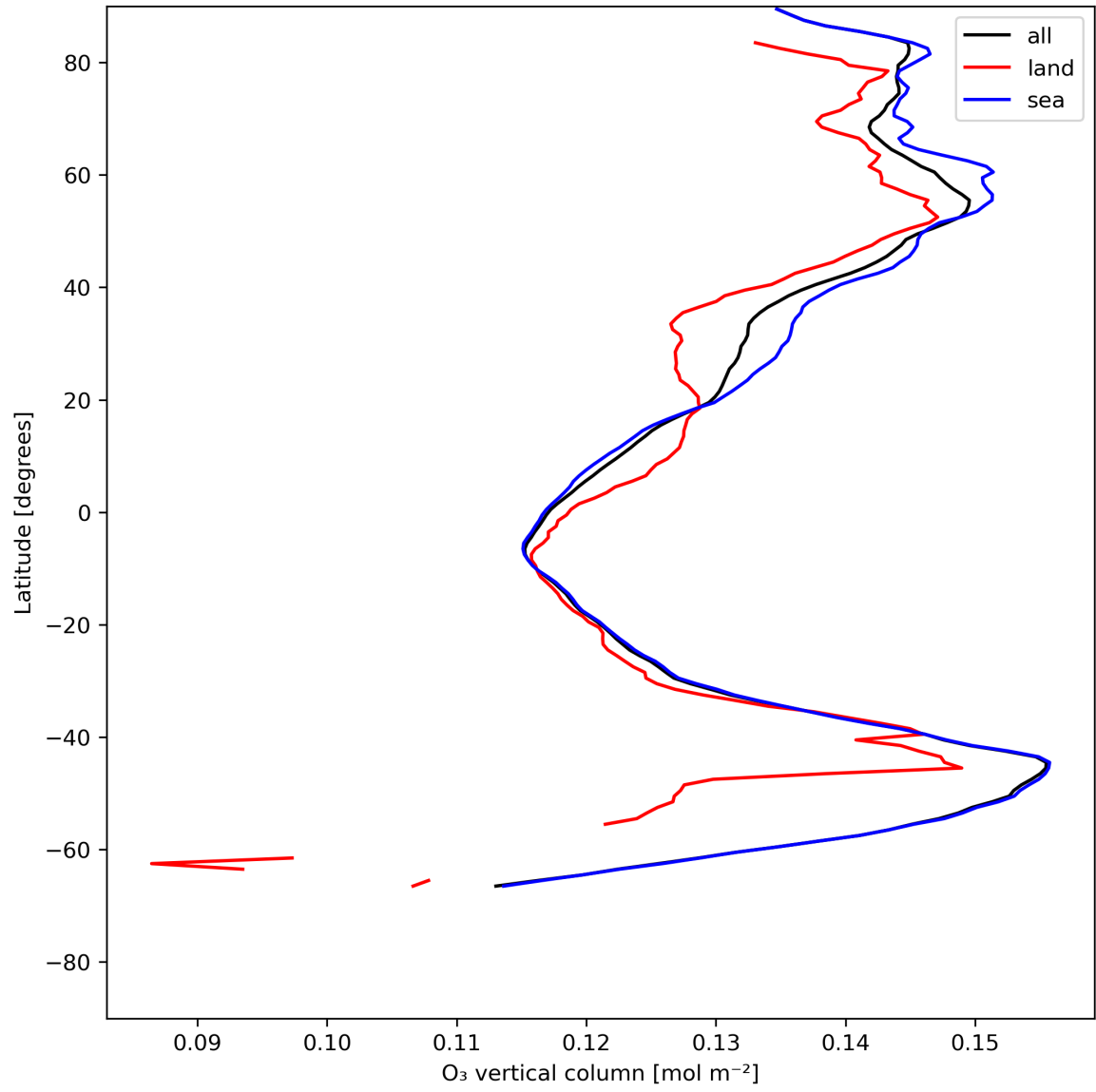
Figure 14: Zonal average of “O 3 vertical column” for 2023-07-09 to 2023-07-11.
