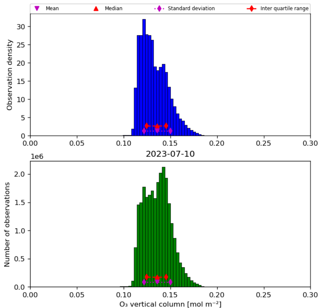
Figure 21: Histogram of “O 3 vertical column” for 2023-07-09 to 2023-07-11
