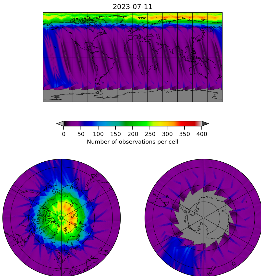
Figure 12: Map of the number of observations for 2023-07-10 to 2023-07-12
