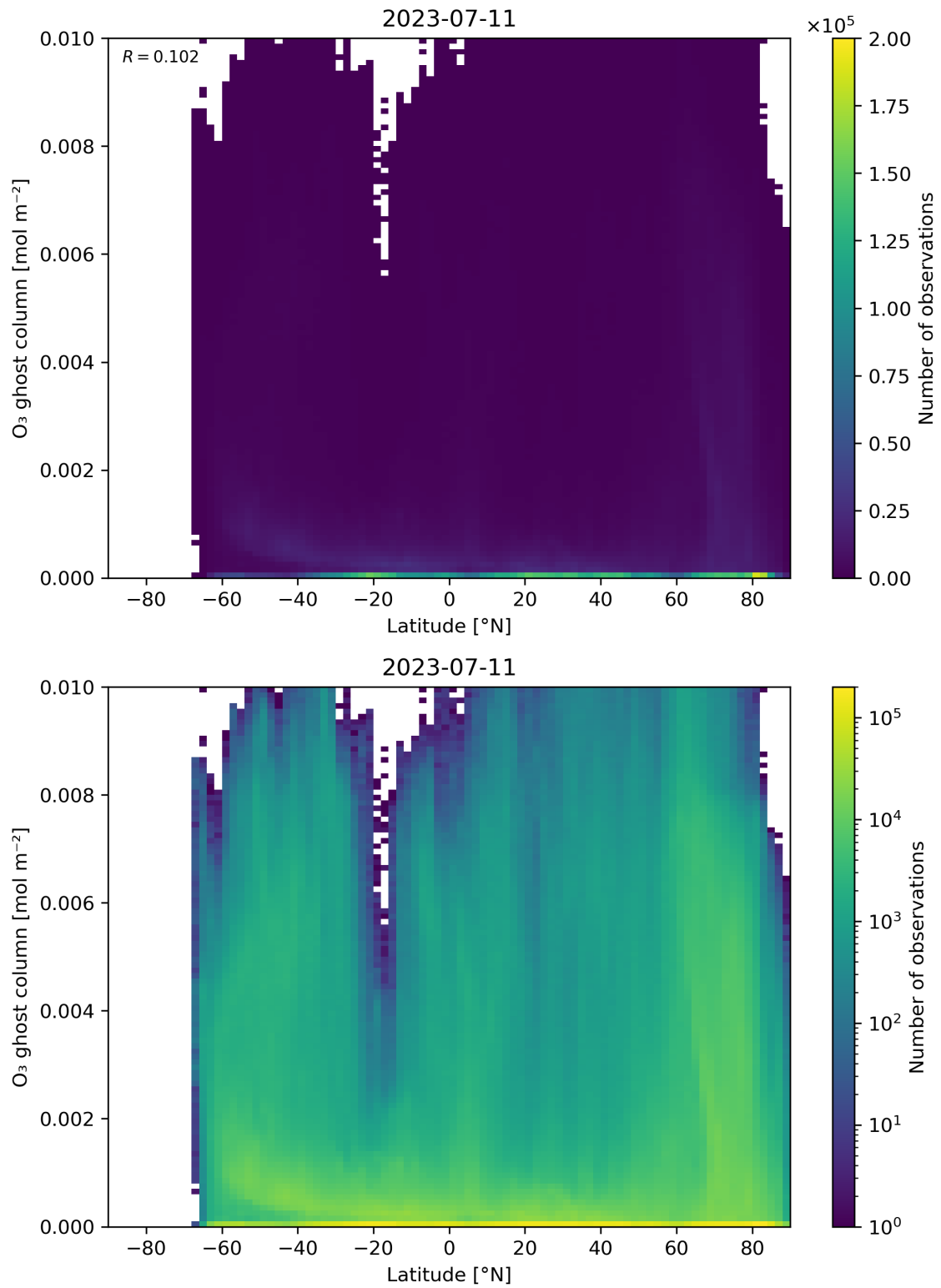
Figure 35: Scatter density plot of “Latitude” against “O 3 ghost column” for 2023-07-10 to 2023-07-12.
