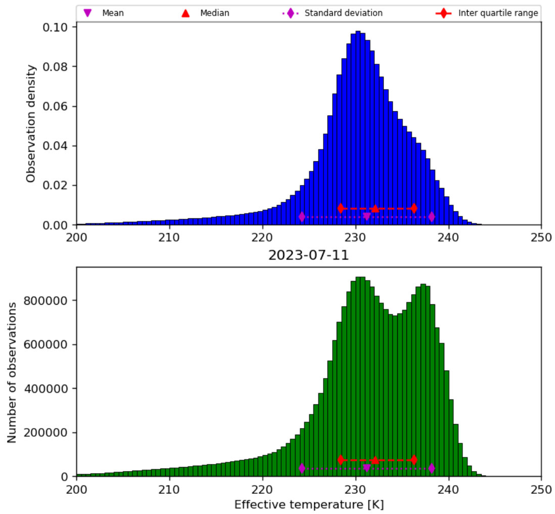
Figure 24: Histogram of “Effective temperature” for 2023-07-10 to 2023-07-12
