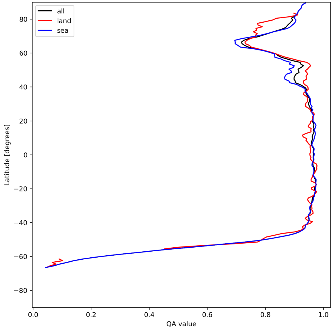
Figure 13: Zonal average of “QA value” for 2023-07-10 to 2023-07-12.
