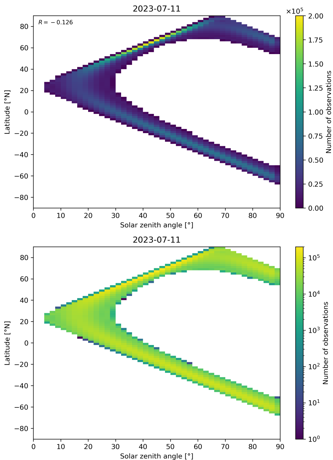
Figure 44: Scatter density plot of “Solar zenith angle” against “Latitude” for 2023-07-10 to 2023-07-12.
