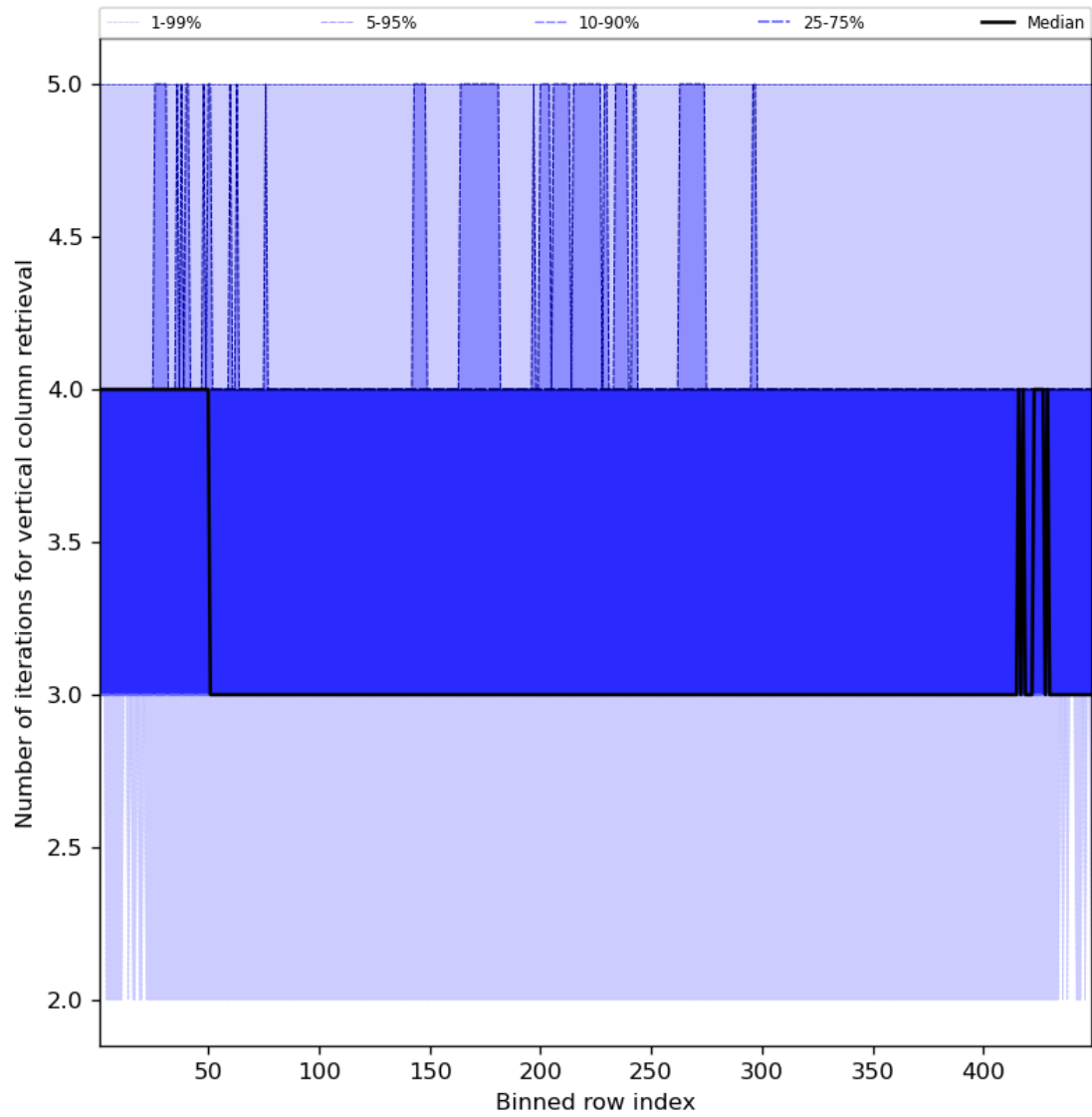
Figure 33: Along track statistics of “Number of iterations for vertical column retrieval” for 2023-07-10 to 2023-07-12
