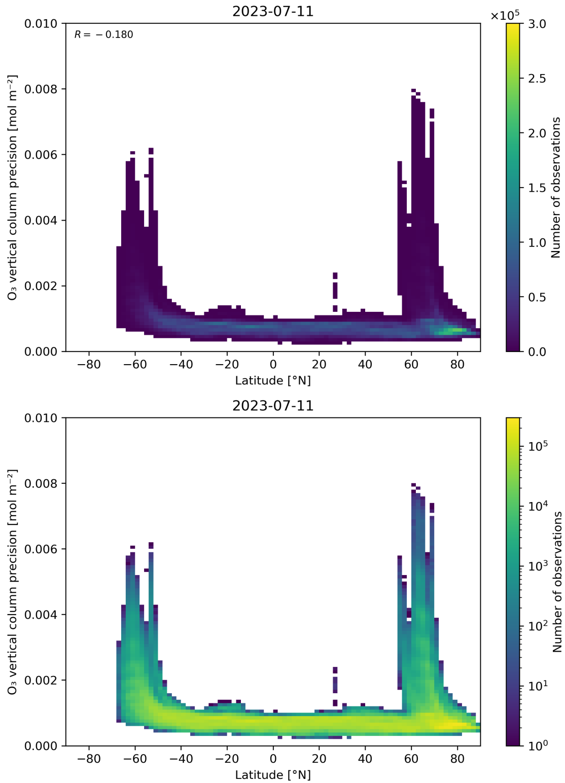
Figure 37: Scatter density plot of “Latitude” against “O 3 vertical column precision” for 2023-07-10 to 2023-07-12.
