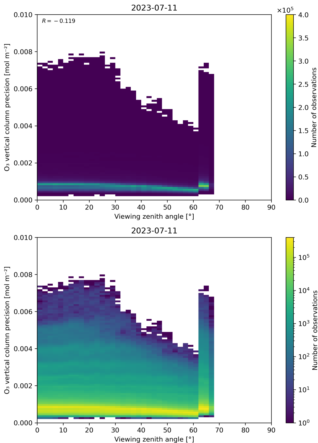
Figure 53: Scatter density plot of “Viewing zenith angle” against “O 3 vertical column precision” for 2023-07-10 to 2023-07-12.
