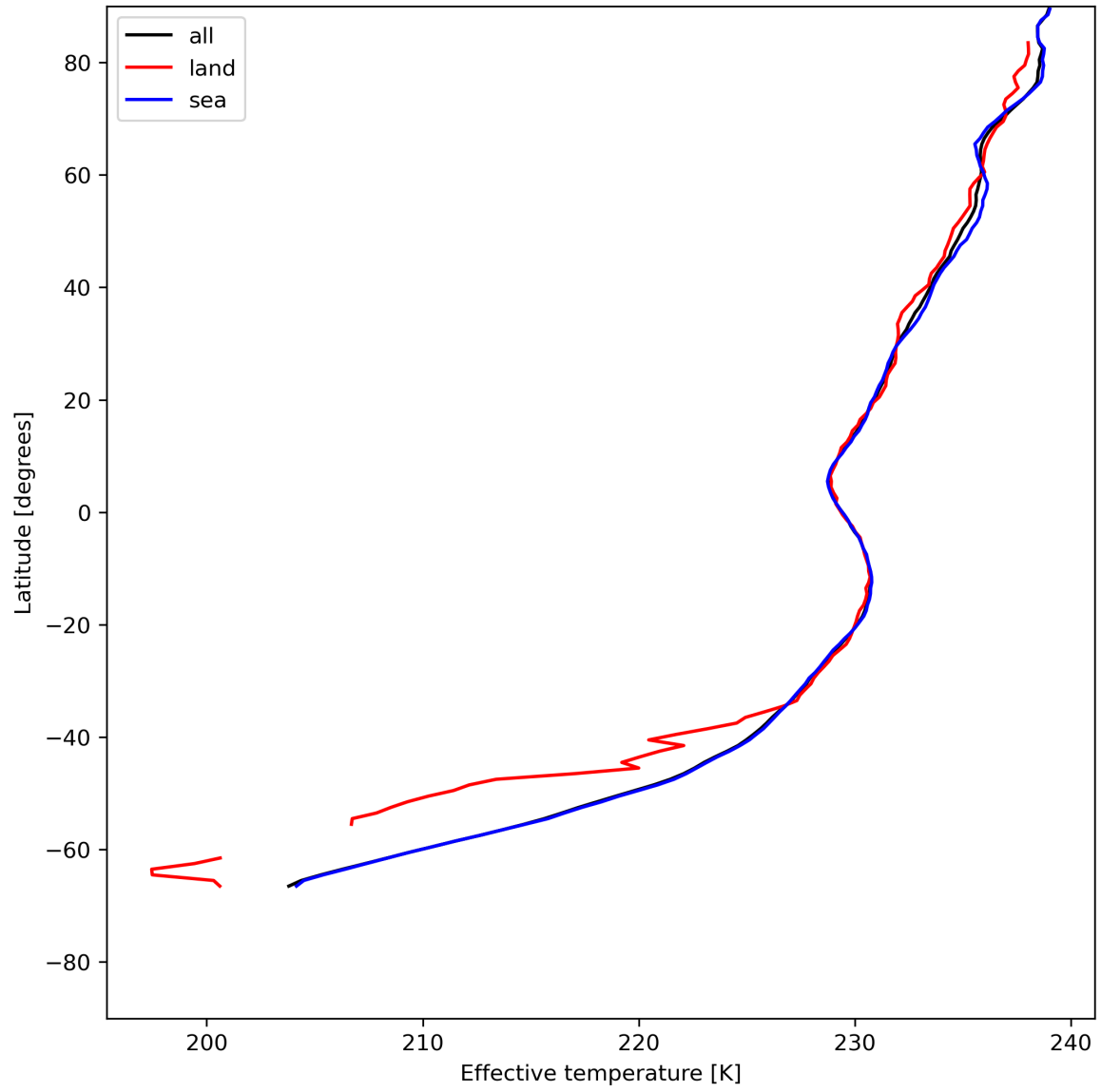
Figure 17: Zonal average of "Effective temperature" for 2023-07-10 to 2023-07-12.
