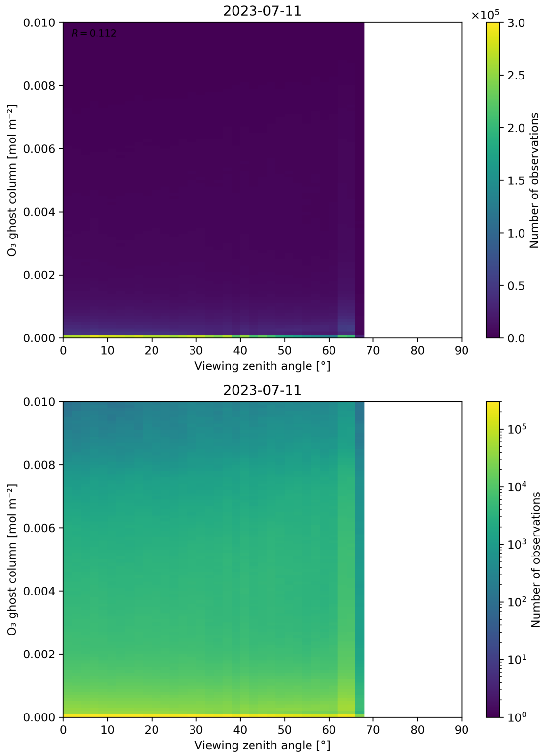
Figure 51: Scatter density plot of “Viewing zenith angle” against “O 3 ghost column” for 2023-07-10 to 2023-07-12.
