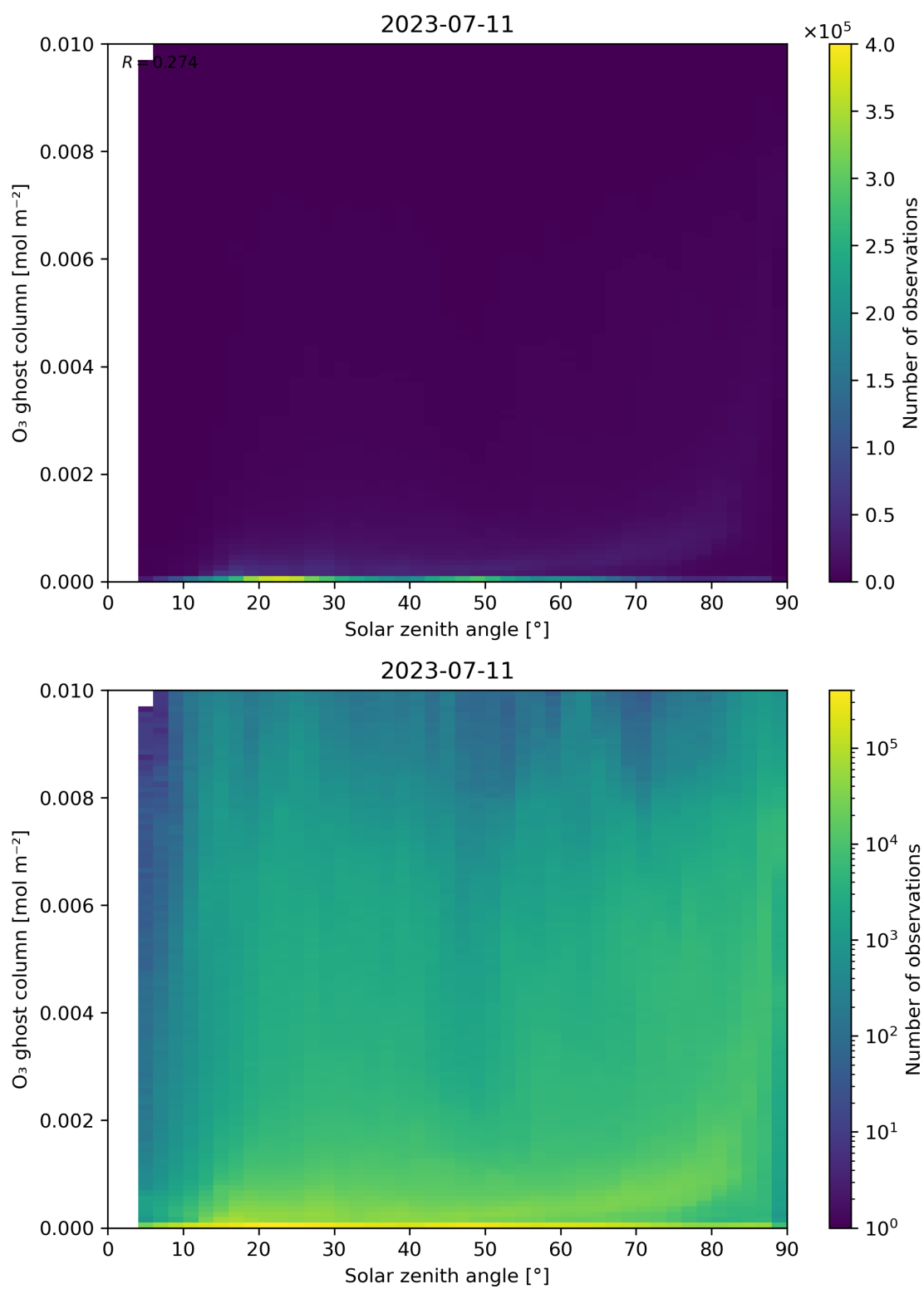
Figure 46: Scatter density plot of “Solar zenith angle” against “O 3 ghost column” for 2023-07-10 to 2023-07-12.
