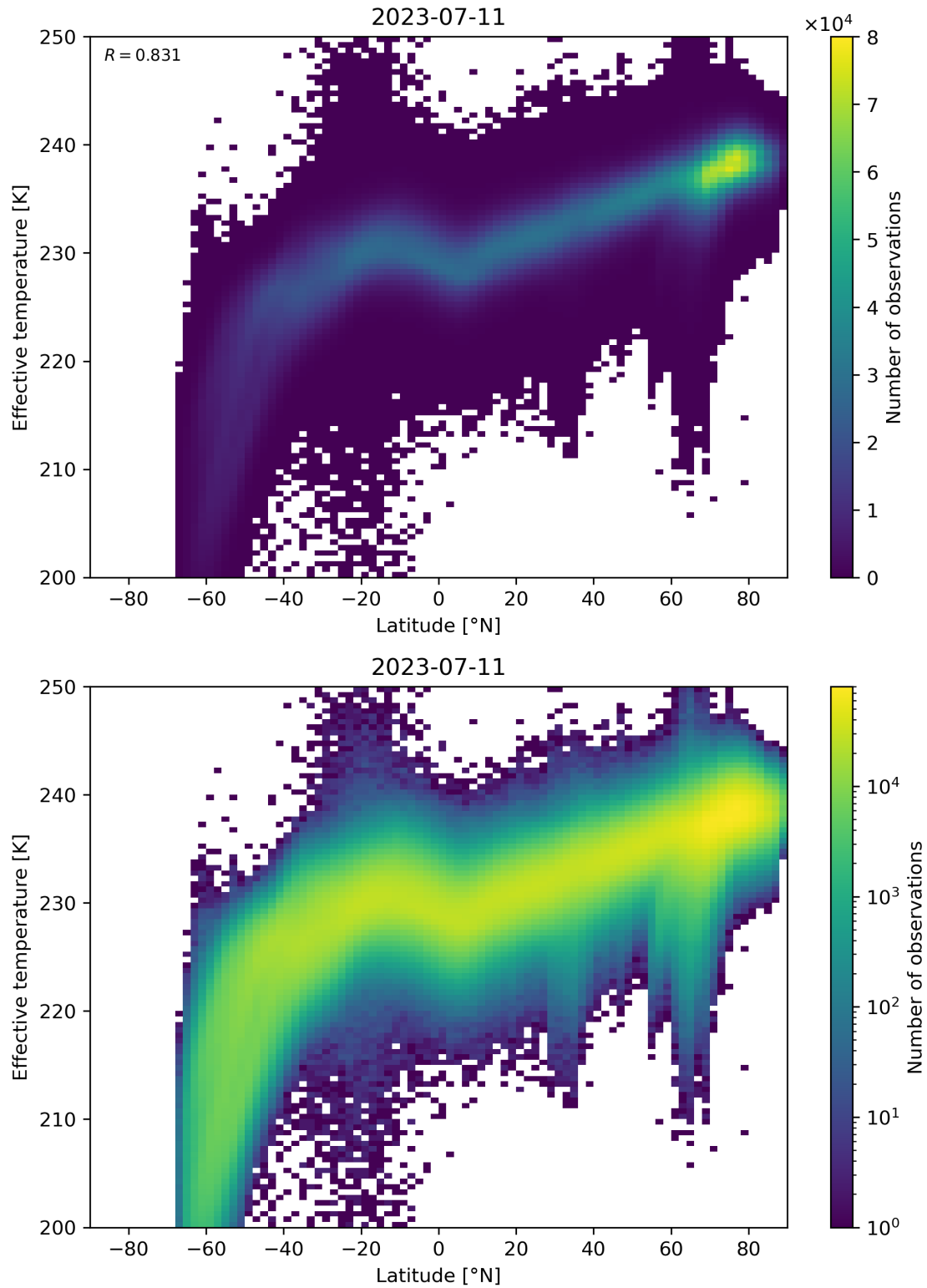
Figure 34: Scatter density plot of “Latitude” against “Effective temperature” for 2023-07-10 to 2023-07-12.
