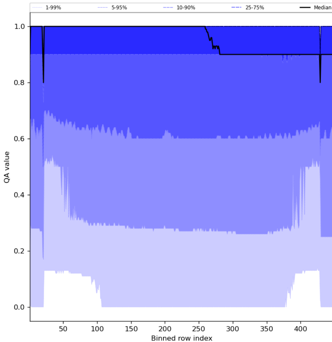
Figure 27: Along track statistics of “QA value” for 2023-07-10 to 2023-07-12
