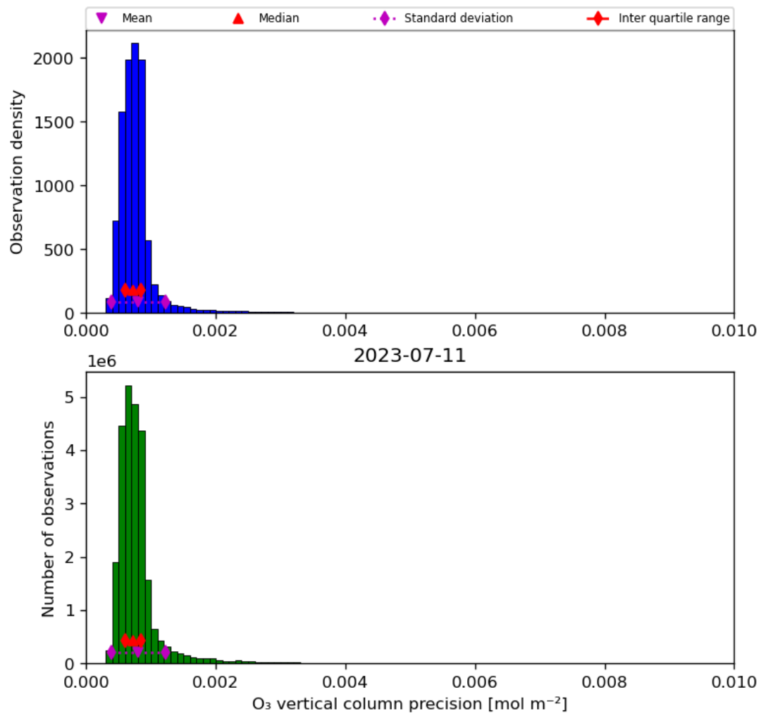
Figure 22: Histogram of “O 3 vertical column precision” for 2023-07-10 to 2023-07-12
