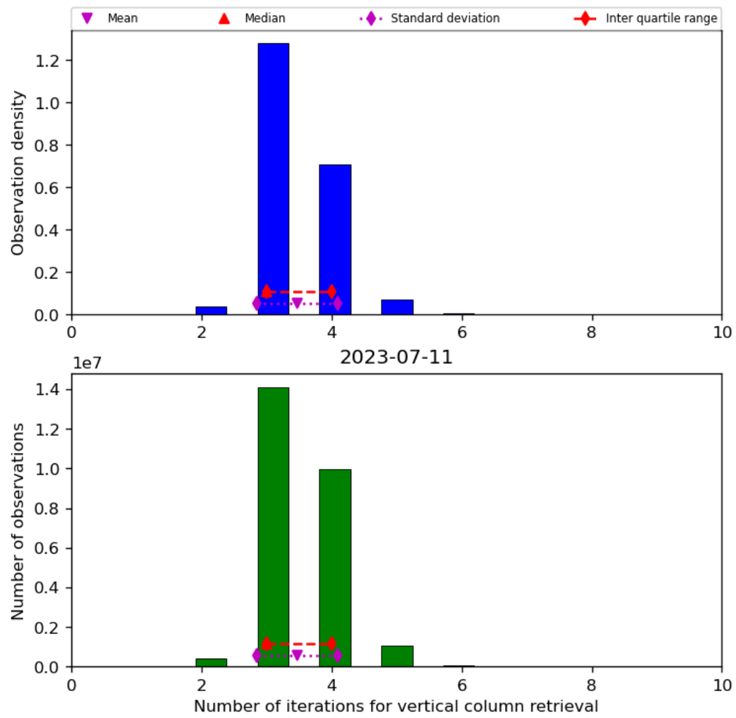
Figure 26: Histogram of “Number of iterations for vertical column retrieval” for 2023-07-10 to 2023-07-12
