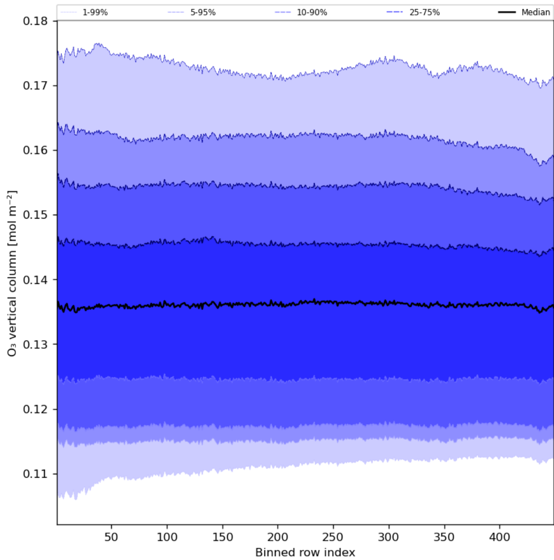
Figure 28: Along track statistics of “O 3 vertical column” for 2023-07-10 to 2023-07-12
