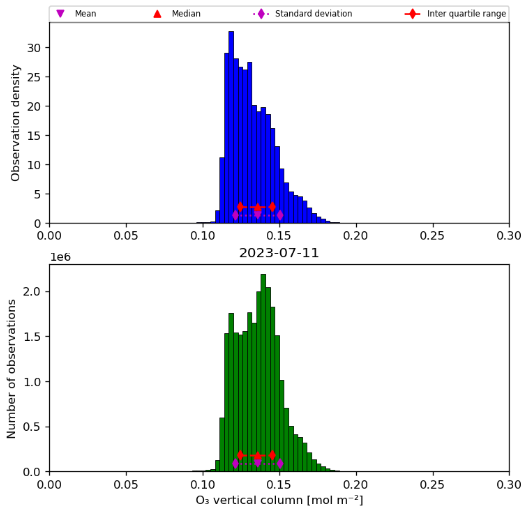
Figure 21: Histogram of “O 3 vertical column” for 2023-07-10 to 2023-07-12
