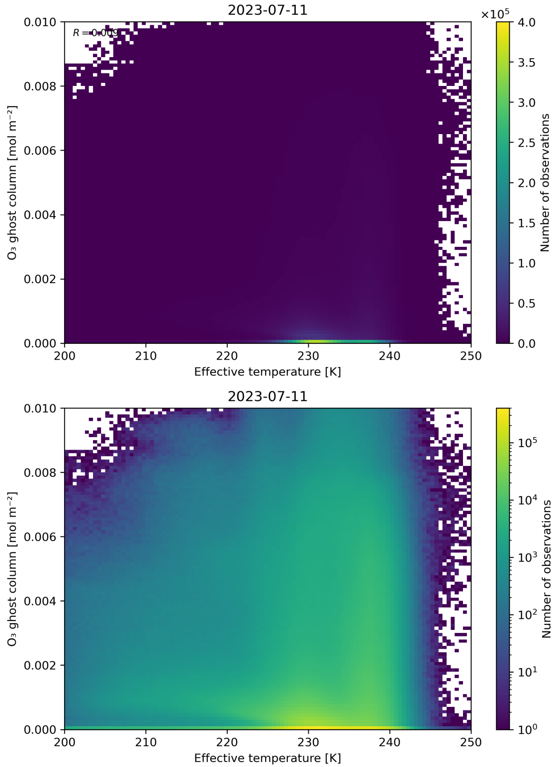
Figure 38: Scatter density plot of “Effective temperature” against “O 3 ghost column” for 2023-07-10 to 2023-07-12.
