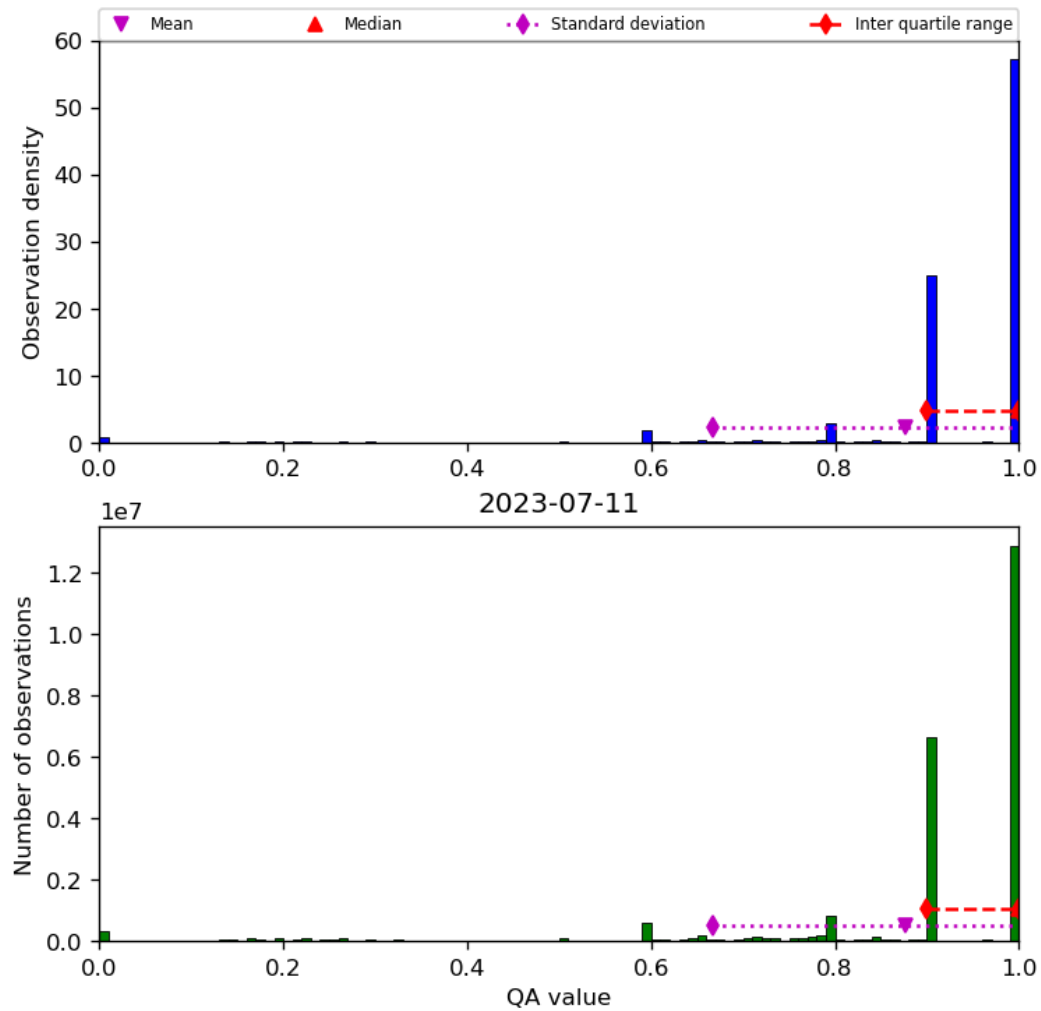
Figure 20: Histogram of “QA value” for 2023-07-10 to 2023-07-12
