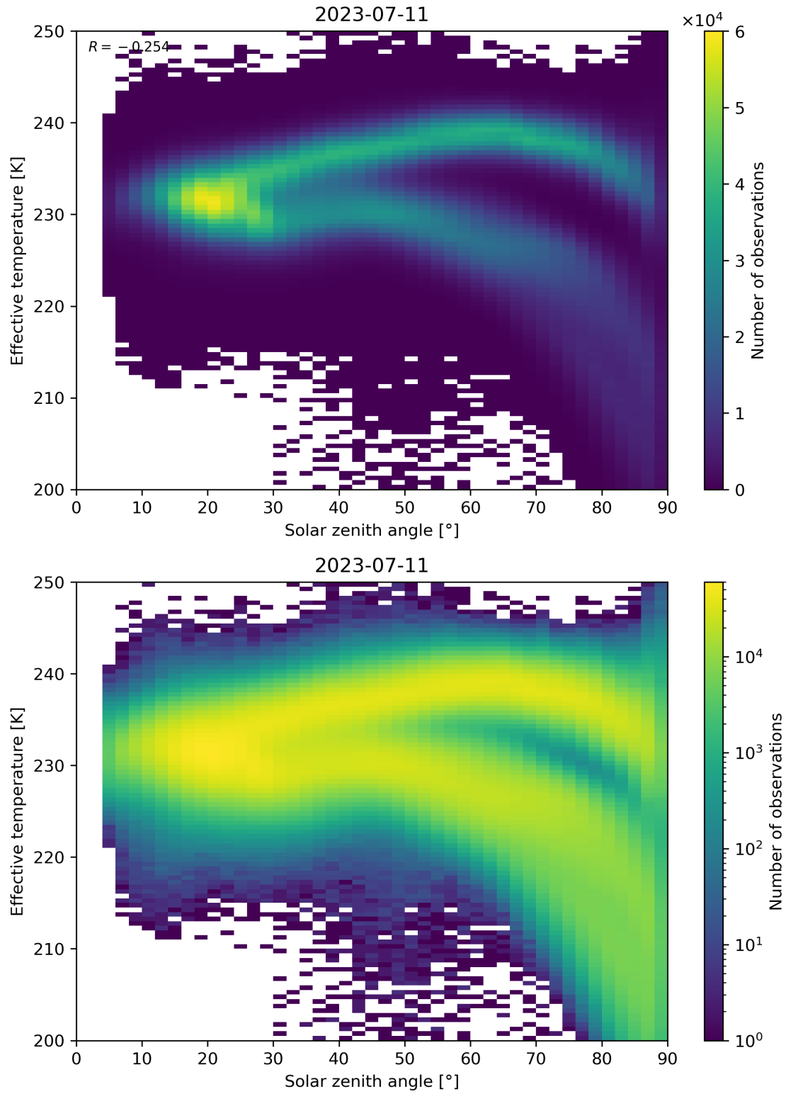
Figure 45: Scatter density plot of “Solar zenith angle” against “Effective temperature” for 2023-07-10 to 2023-07-12.
