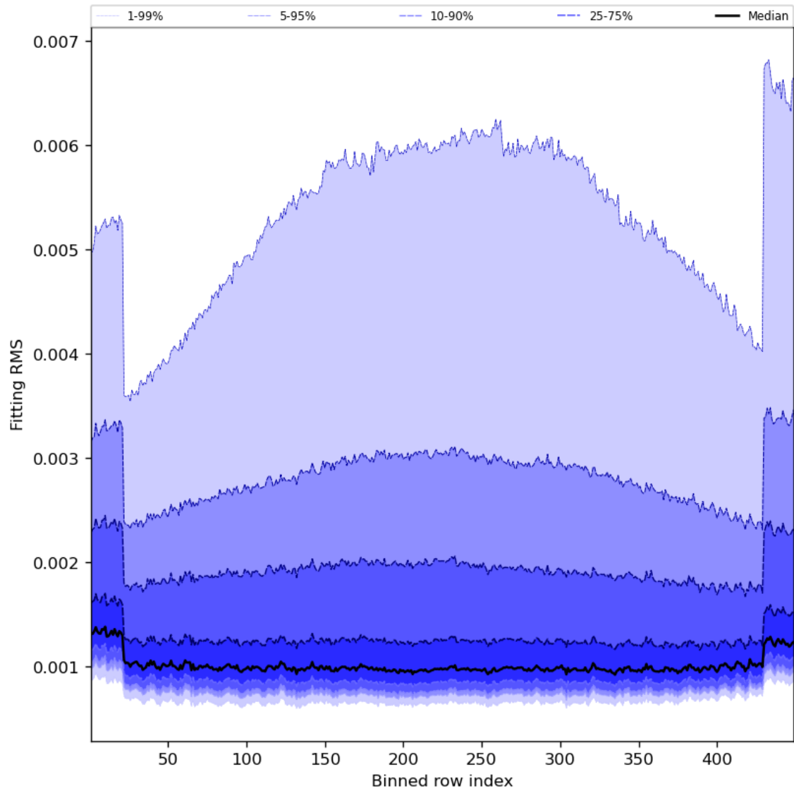
Figure 30: Along track statistics of “Fitting RMS” for 2023-07-10 to 2023-07-12
