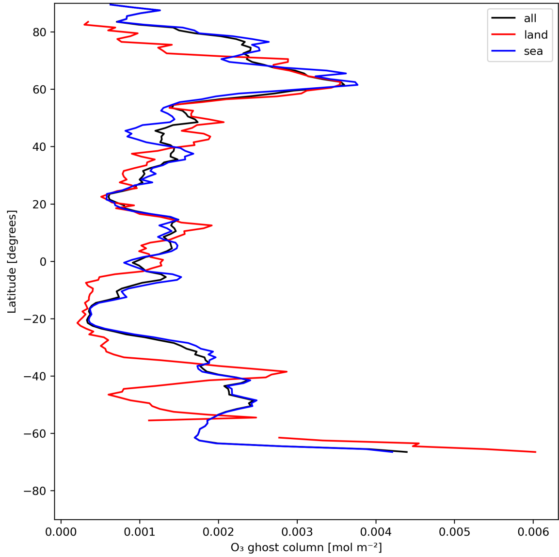
Figure 18: Zonal average of “O 3 ghost column” for 2023-07-10 to 2023-07-12.
