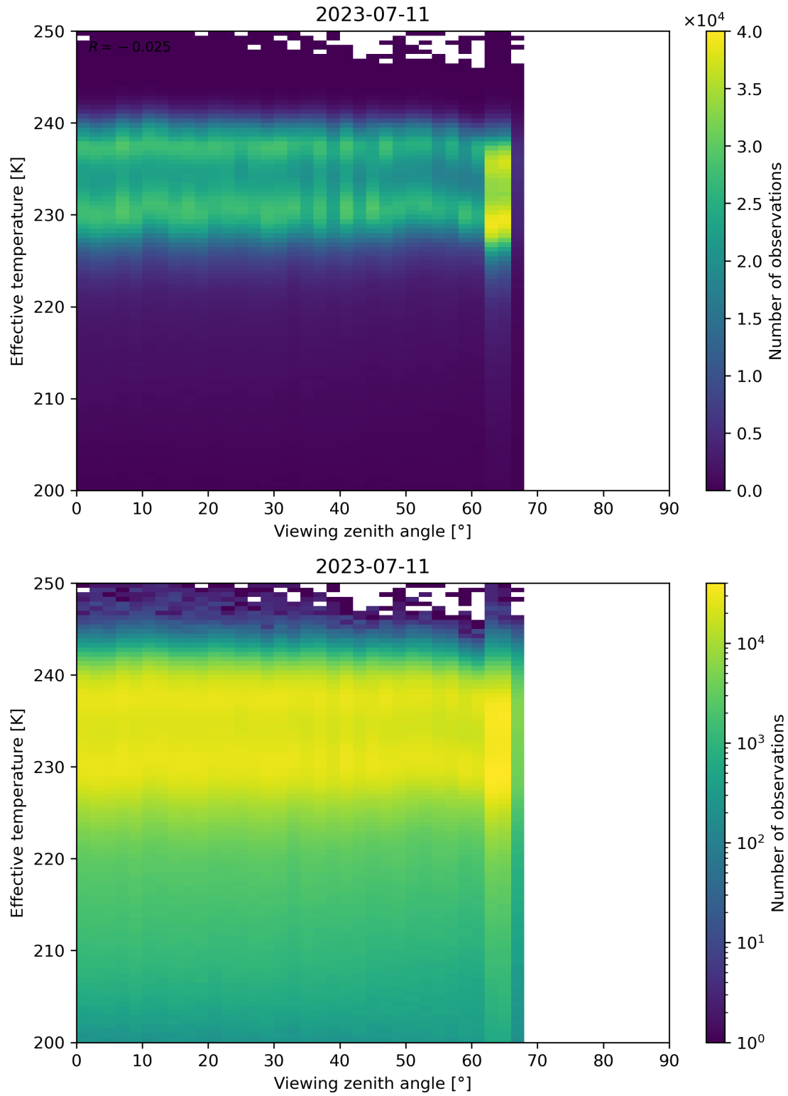
Figure 50: Scatter density plot of “Viewing zenith angle” against “Effective temperature” for 2023-07-10 to 2023-07-12.
