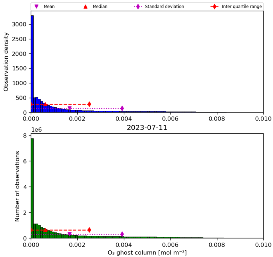
Figure 25: Histogram of “O 3 ghost column” for 2023-07-10 to 2023-07-12
