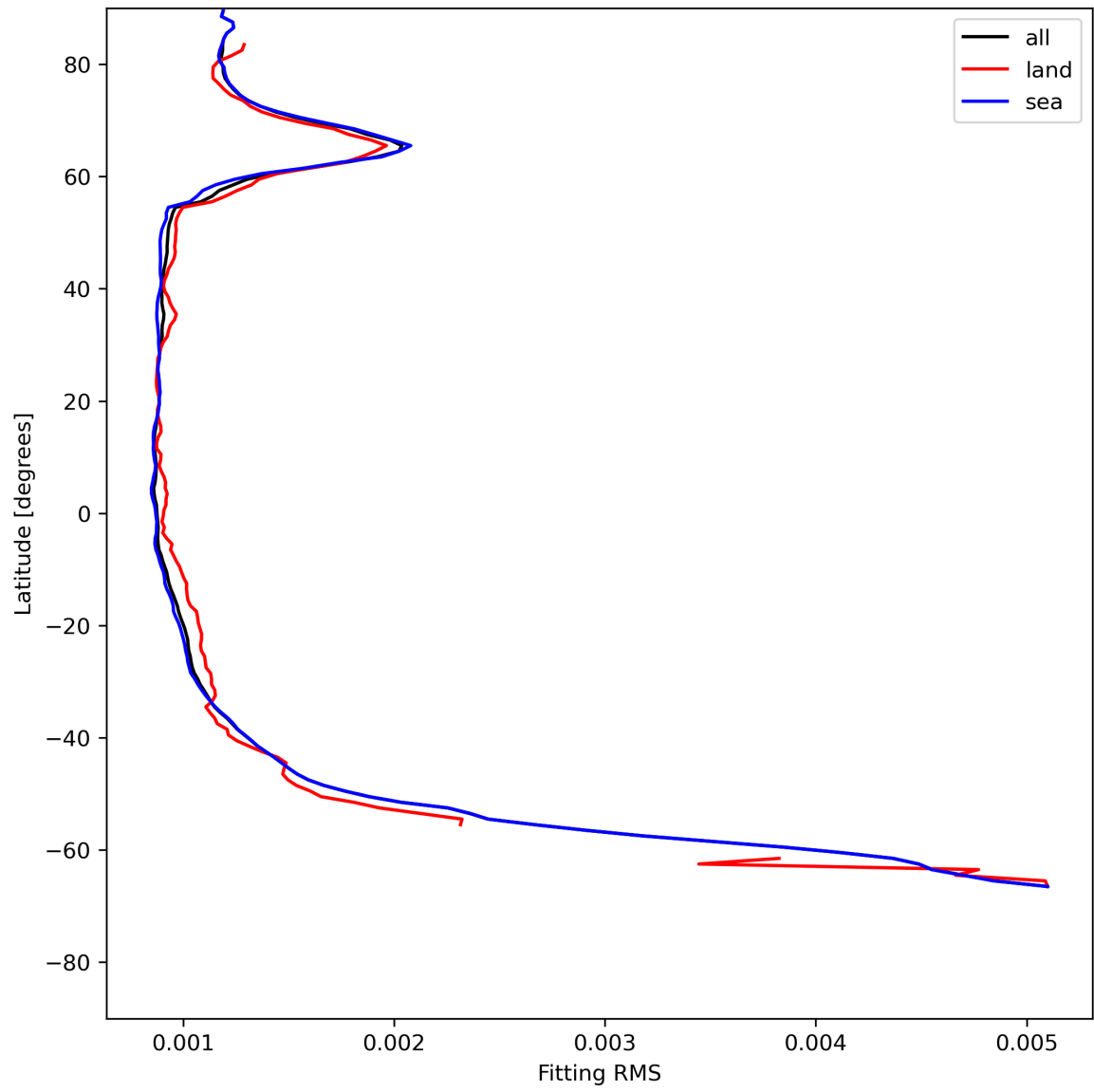
Figure 16: Zonal average of “Fitting RMS” for 2023-07-10 to 2023-07-12.
