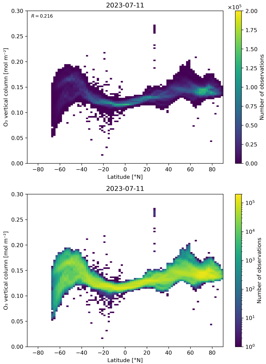
Figure 36: Scatter density plot of “Latitude” against “O 3 vertical column” for 2023-07-10 to 2023-07-12.
