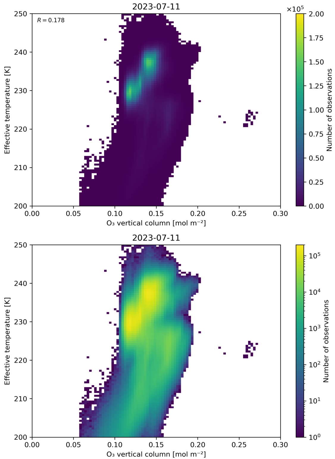
Figure 39: Scatter density plot of “O 3 vertical column” against “Effective temperature” for 2023-07-10 to 2023-07-12.
