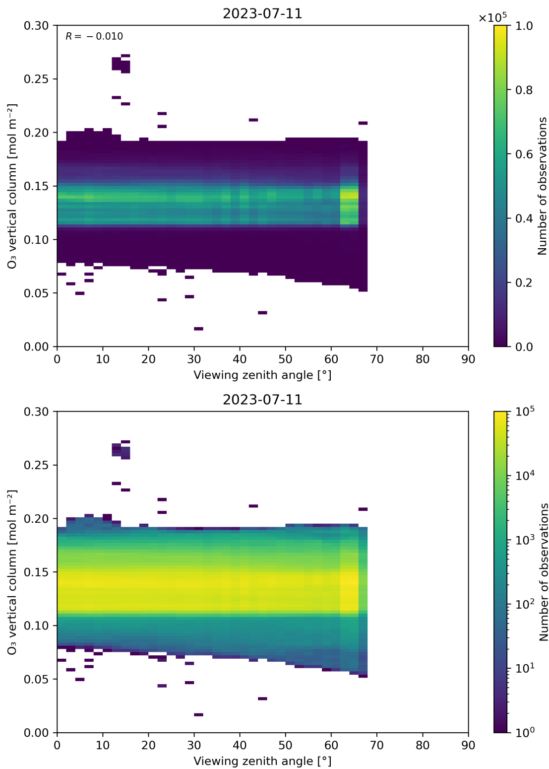
Figure 52: Scatter density plot of “Viewing zenith angle” against “O 3 vertical column” for 2023-07-10 to 2023-07-12.
