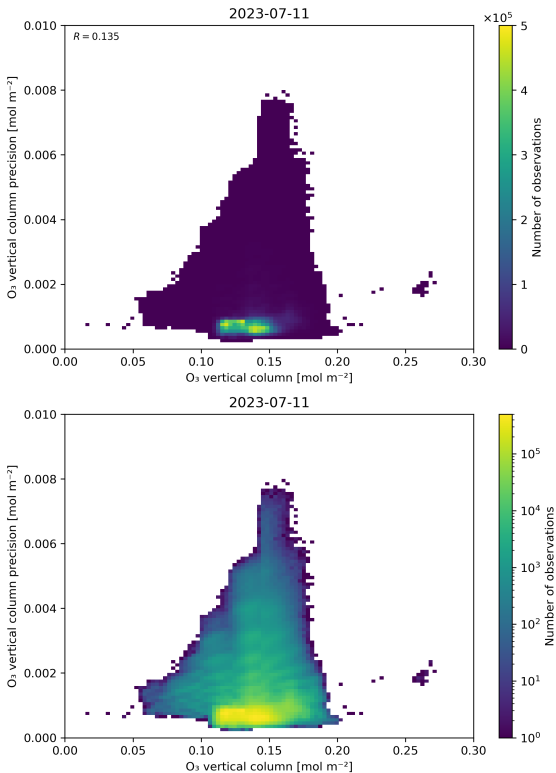
Figure 41: Scatter density plot of “O 3 vertical column” against “O 3 vertical column precision” for 2023-07-10 to 2023-07-12.
