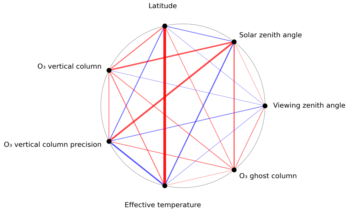
Figure 1: Map of correlation graph for 2023-07-10 to 2023-07-12.
