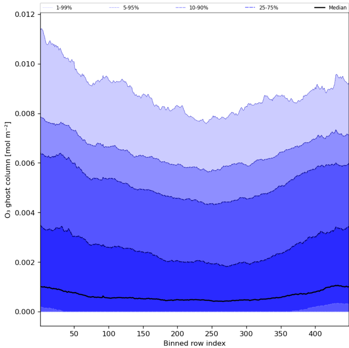
Figure 32: Along track statistics of “O 3 ghost column” for 2023-07-10 to 2023-07-12
