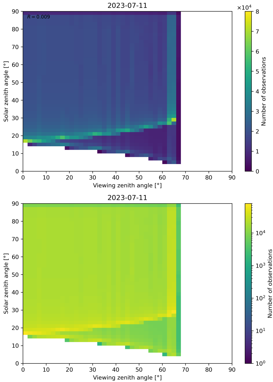
Figure 54: Scatter density plot of “Viewing zenith angle” against “Solar zenith angle” for 2023-07-10 to 2023-07-12.
