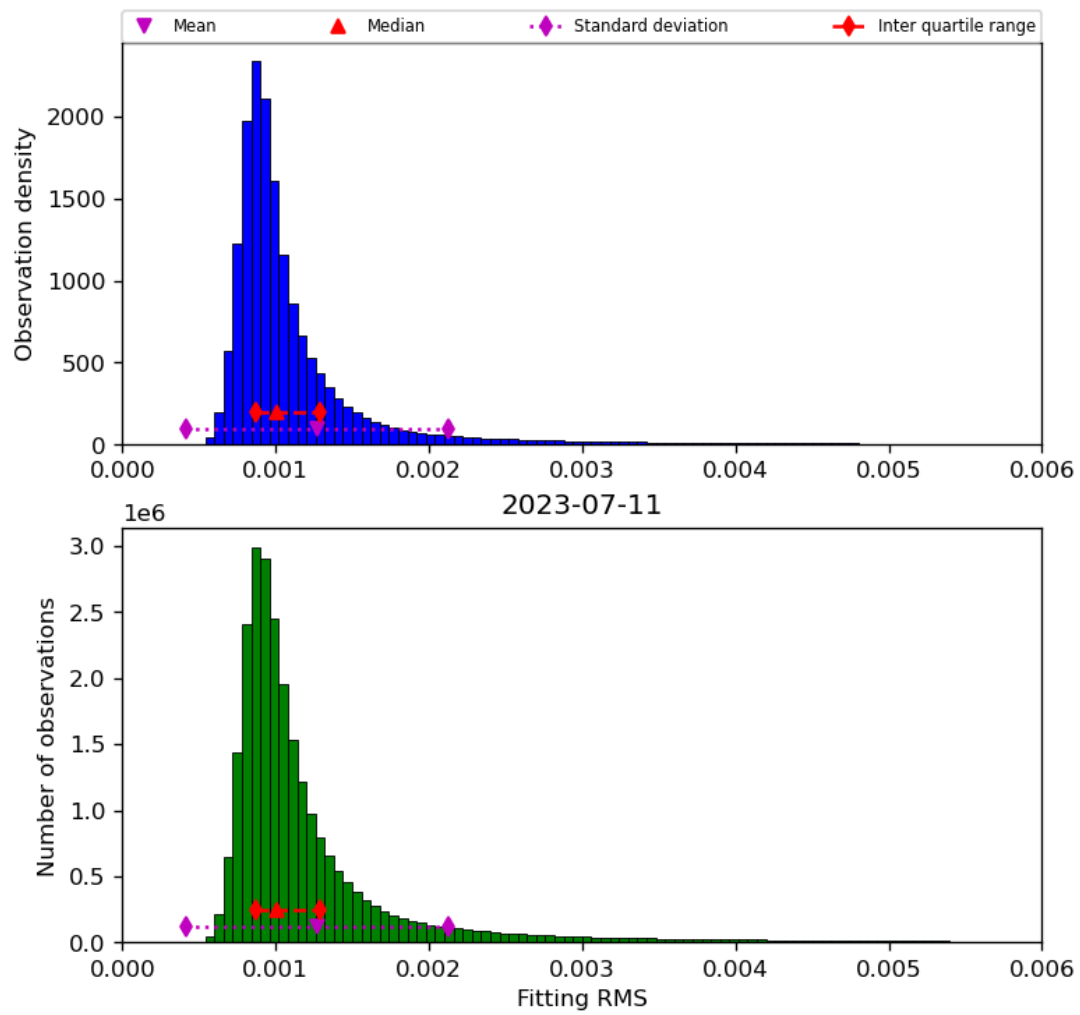
Figure 23: Histogram of “Fitting RMS” for 2023-07-10 to 2023-07-12
