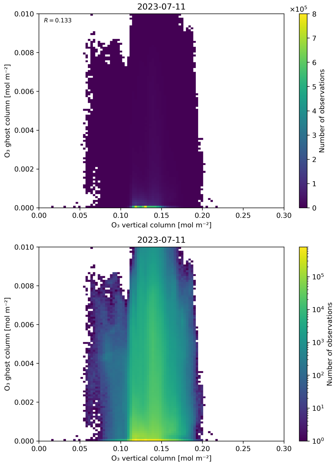
Figure 40: Scatter density plot of “O 3 vertical column” against “O 3 ghost column” for 2023-07-10 to 2023-07-12.
