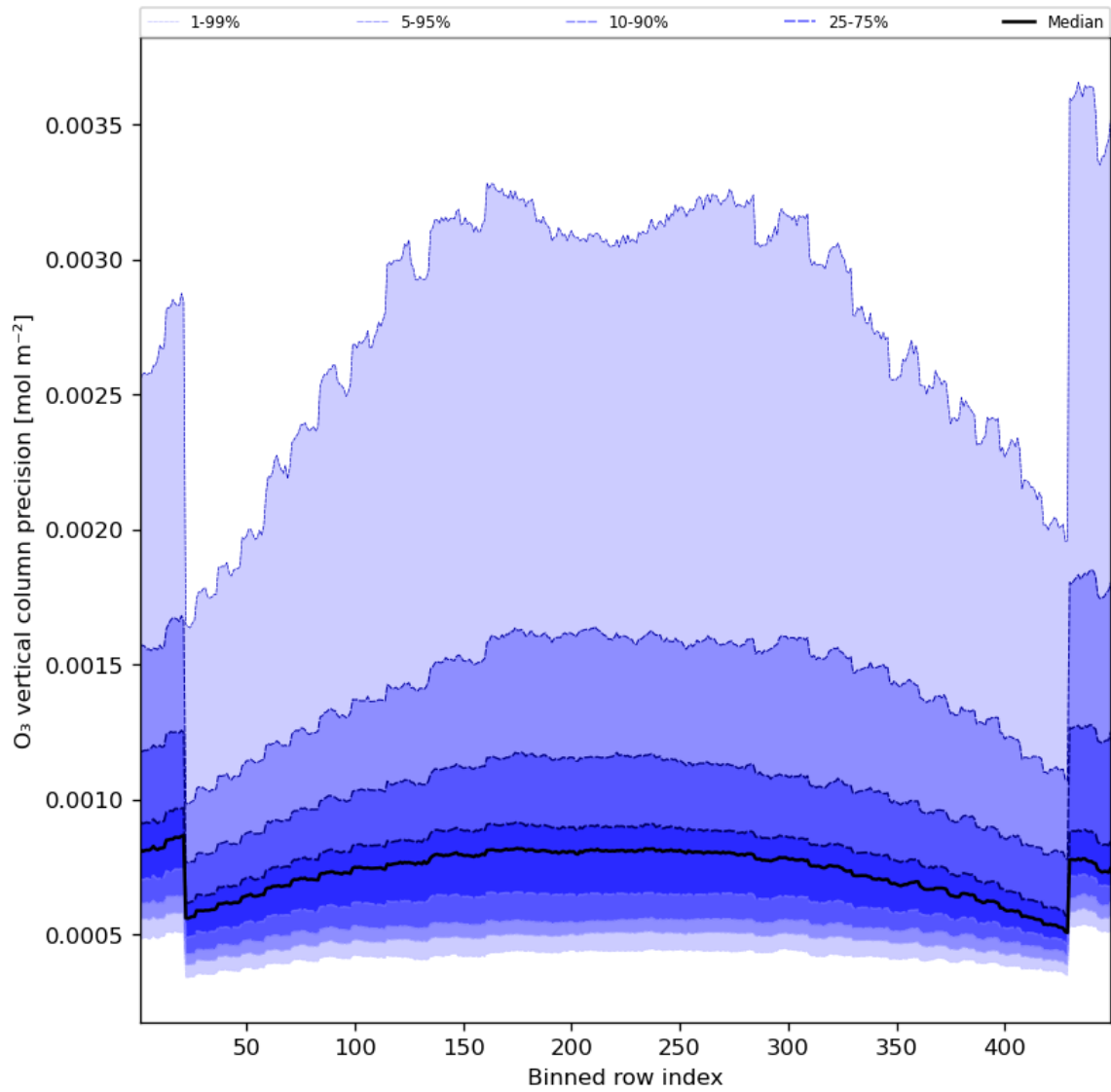
Figure 29: Along track statistics of “O 3 vertical column precision” for 2023-07-10 to 2023-07-12
