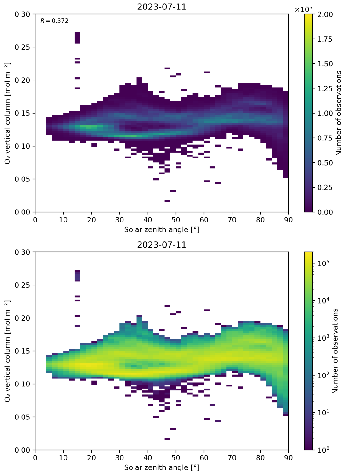
Figure 47: Scatter density plot of “Solar zenith angle” against “O 3 vertical column” for 2023-07-10 to 2023-07-12.
