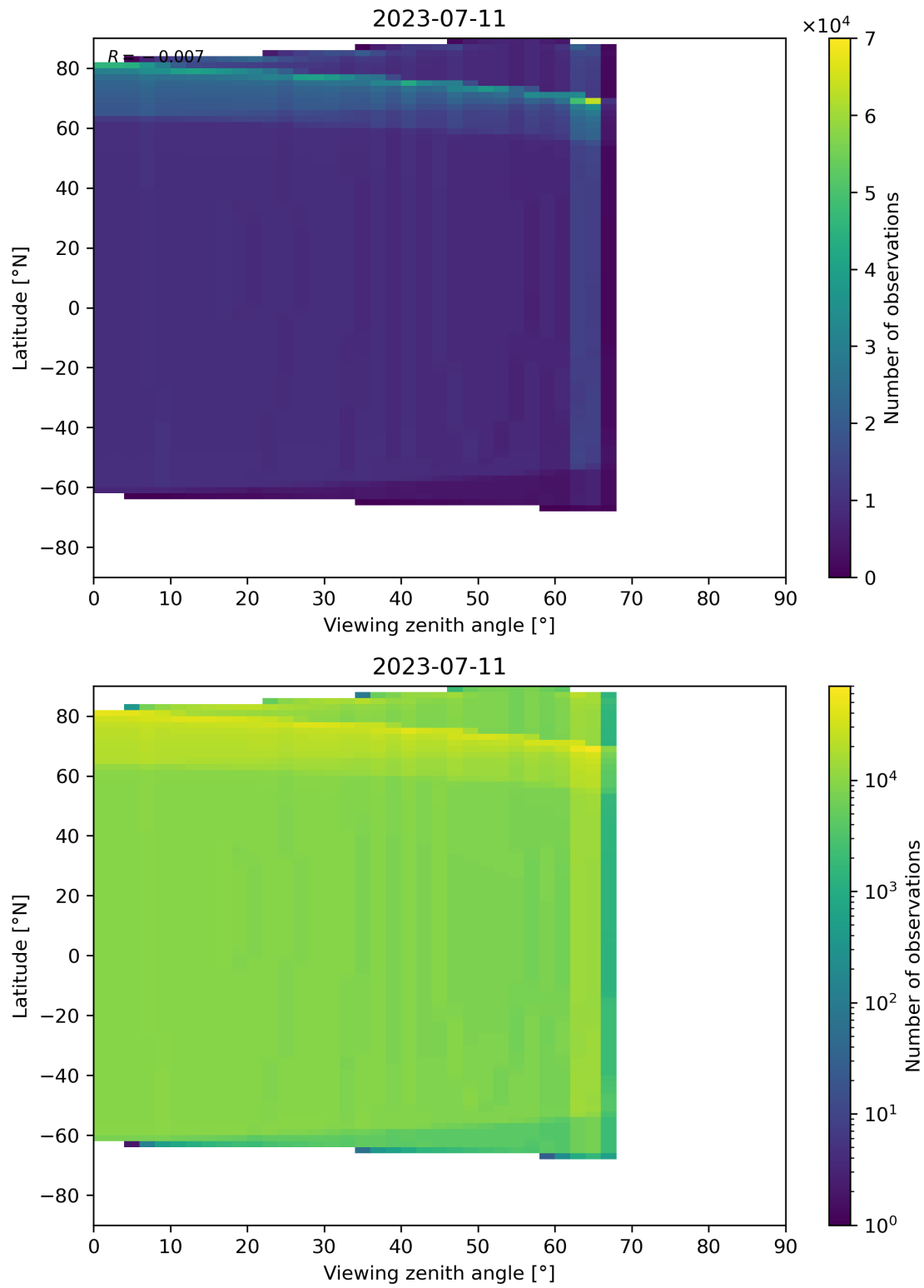
Figure 49: Scatter density plot of “Viewing zenith angle” against “Latitude” for 2023-07-10 to 2023-07-12.
