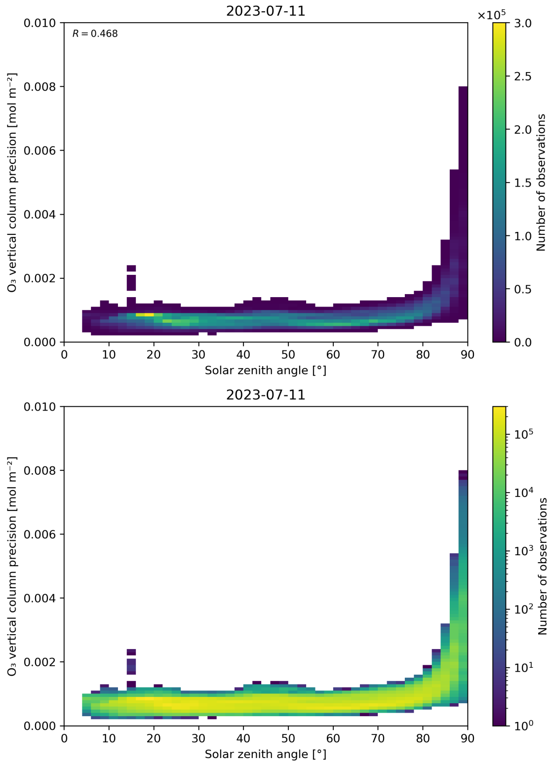
Figure 48: Scatter density plot of “Solar zenith angle” against “O 3 vertical column precision” for 2023-07-10 to 2023-07-12.
