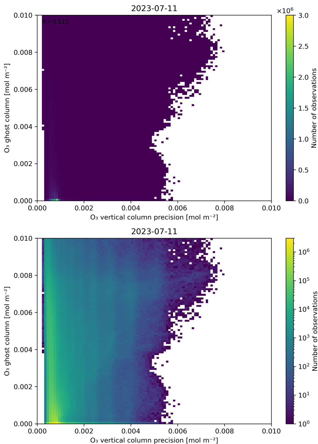
Figure 43: Scatter density plot of “ \text{O}_3 vertical column precision” against “ \text{O}_3 ghost column” for 2023-07-10 to 2023-07-12.
