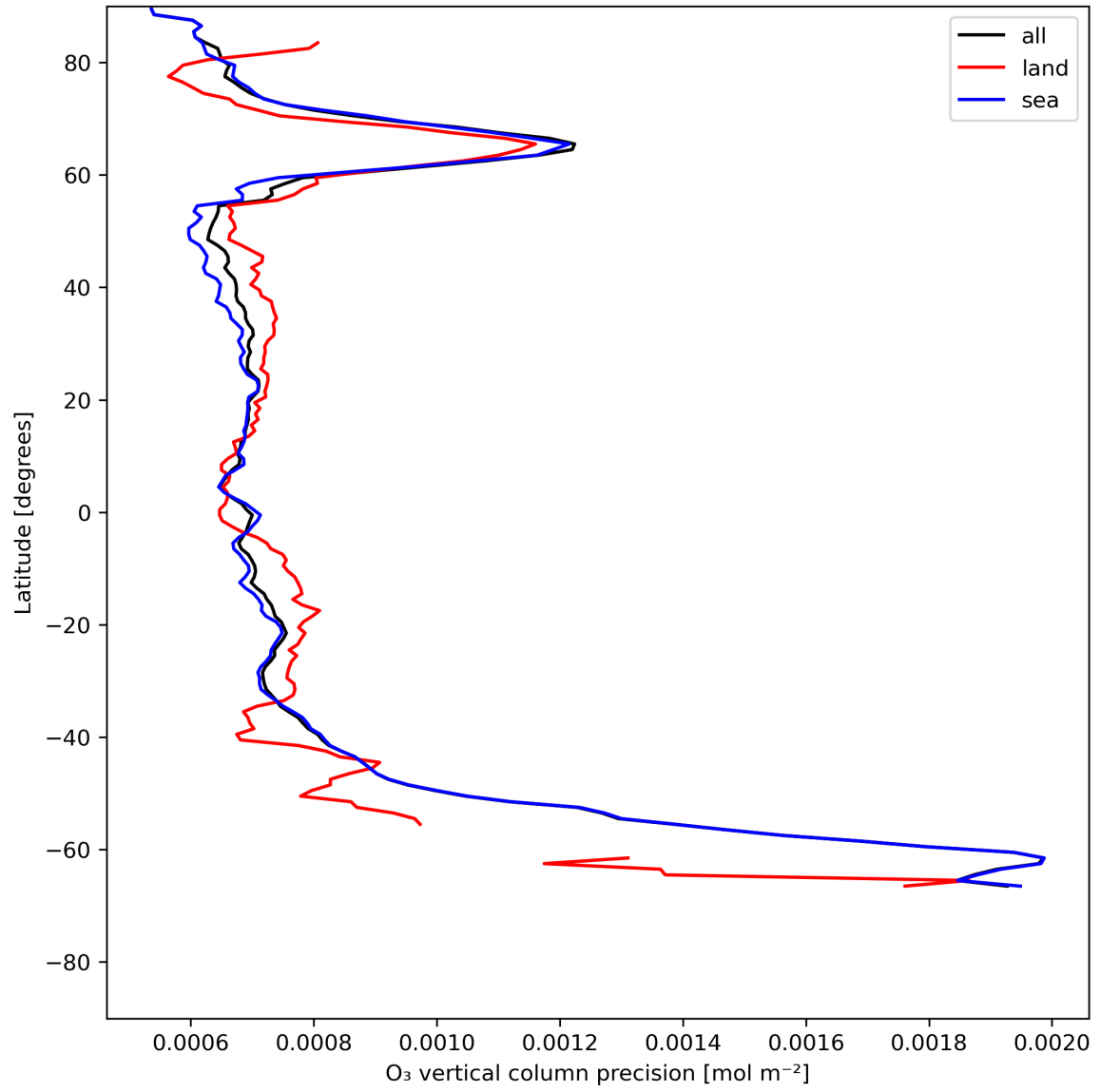
Figure 15: Zonal average of “O 3 vertical column precision” for 2023-07-10 to 2023-07-12.
