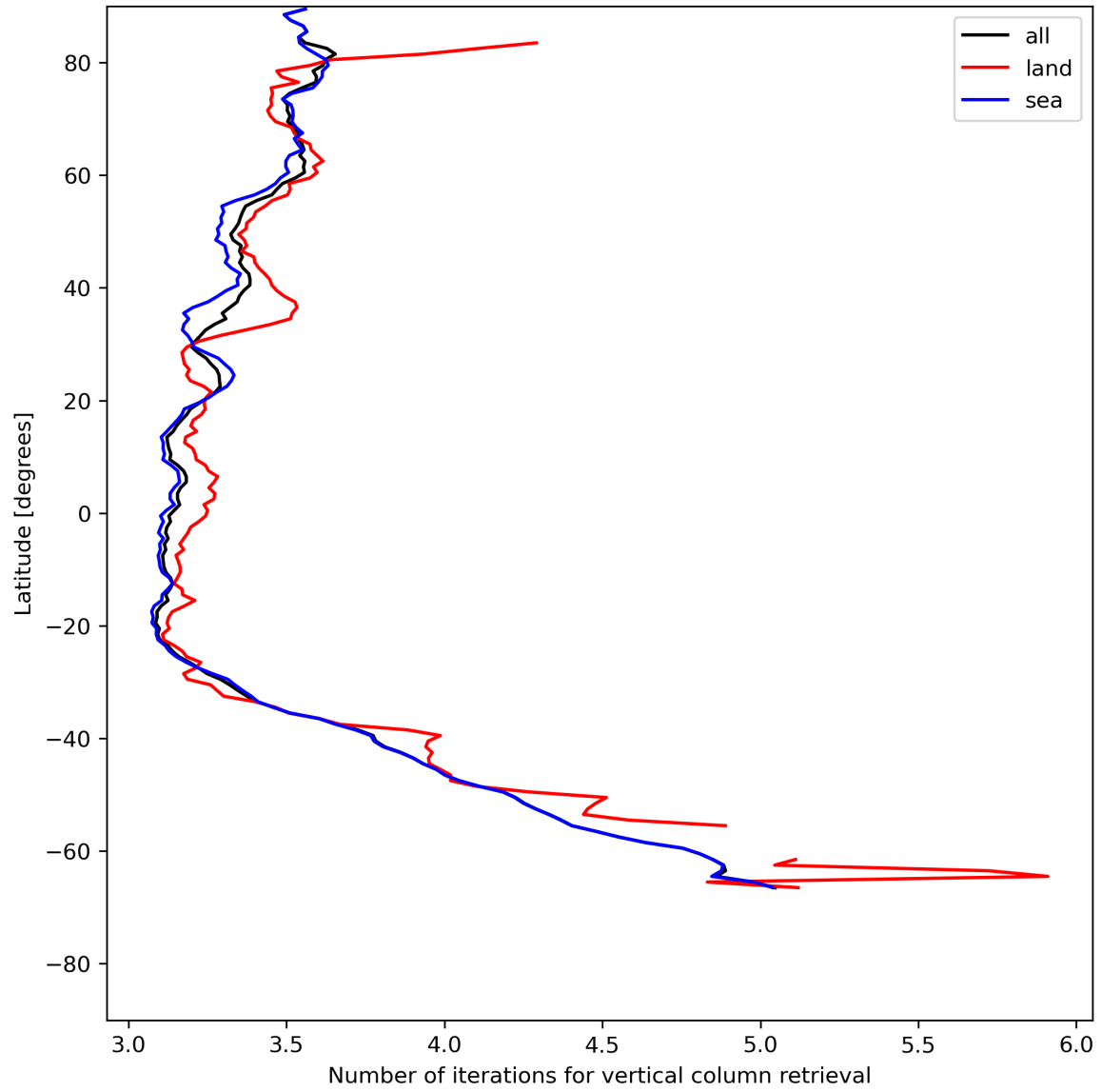
Figure 19: Zonal average of “Number of iterations for vertical column retrieval” for 2023-07-10 to 2023-07-12.
