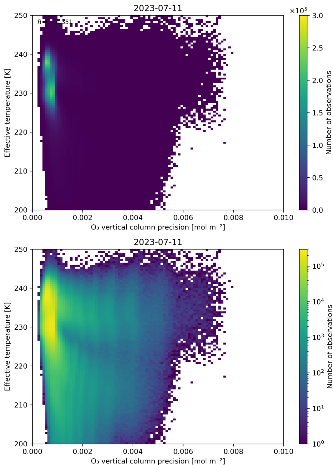
Figure 42: Scatter density plot of “O 3 vertical column precision” against “Effective temperature” for 2023-07-10 to 2023-07-12.
