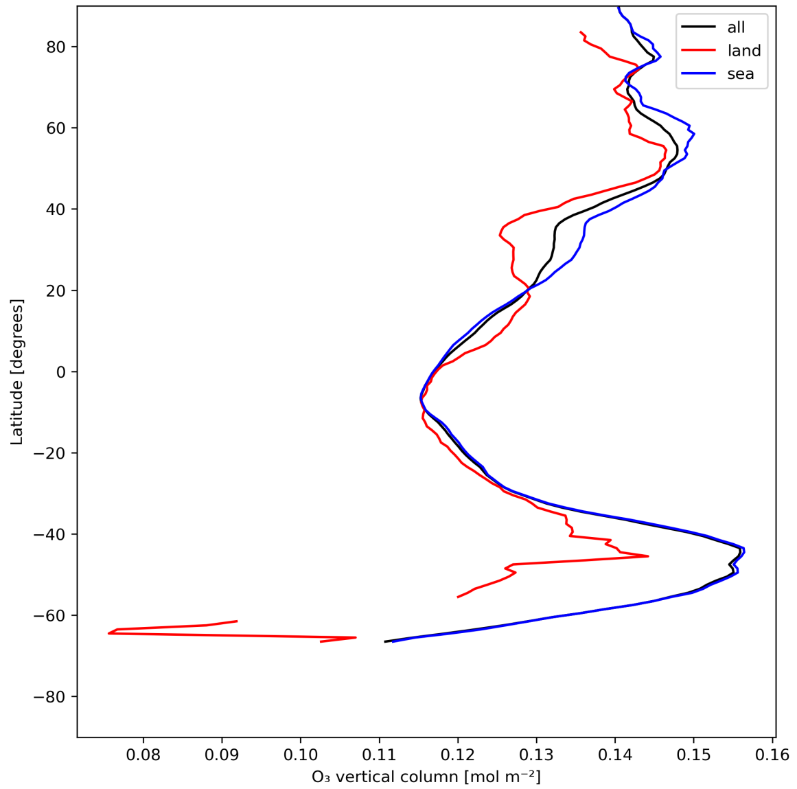
Figure 14: Zonal average of “O 3 vertical column” for 2023-07-10 to 2023-07-12.
