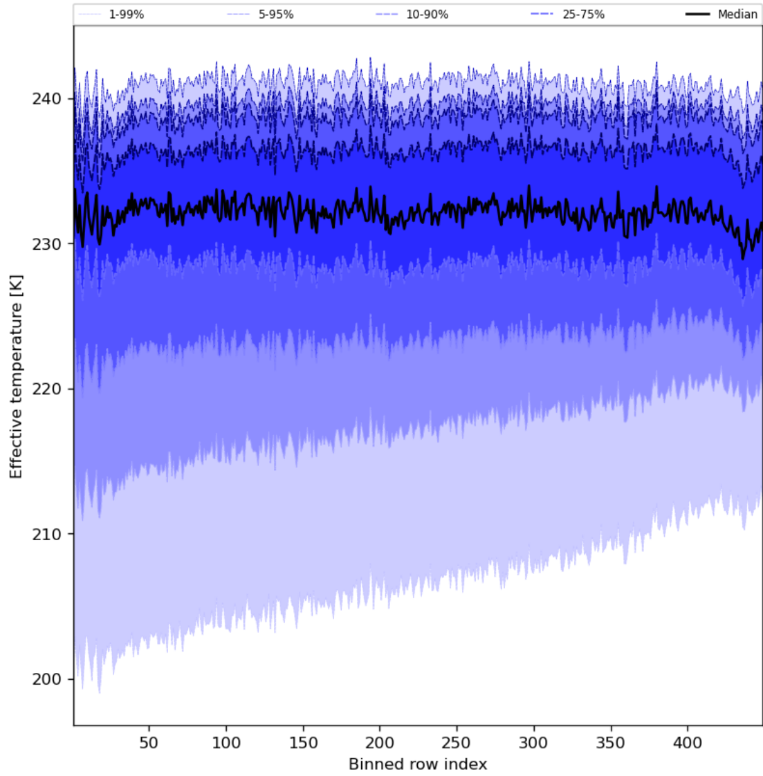
Figure 31: Along track statistics of “Effective temperature” for 2023-07-10 to 2023-07-12
