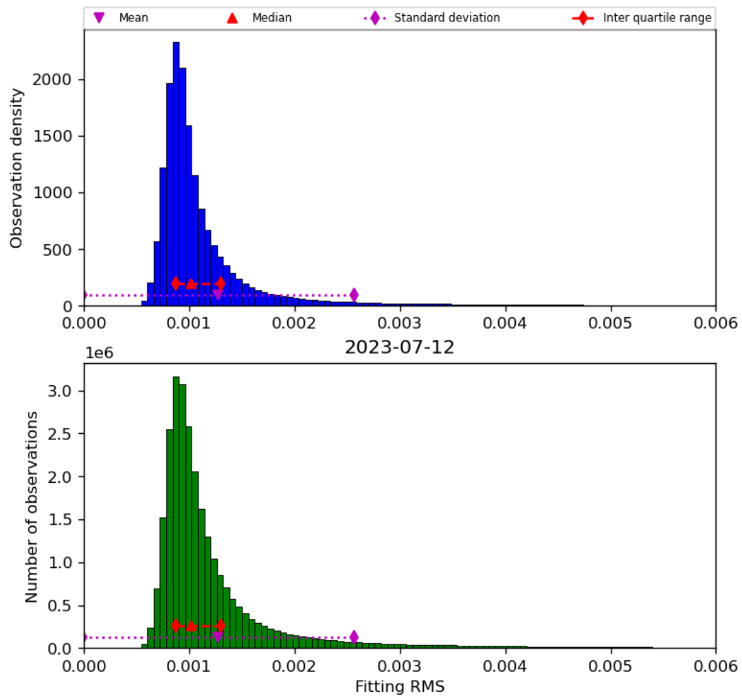
Figure 23: Histogram of “Fitting RMS” for 2023-07-11 to 2023-07-13
