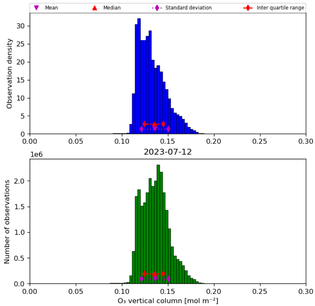
Figure 21: Histogram of “O 3 vertical column” for 2023-07-11 to 2023-07-13
