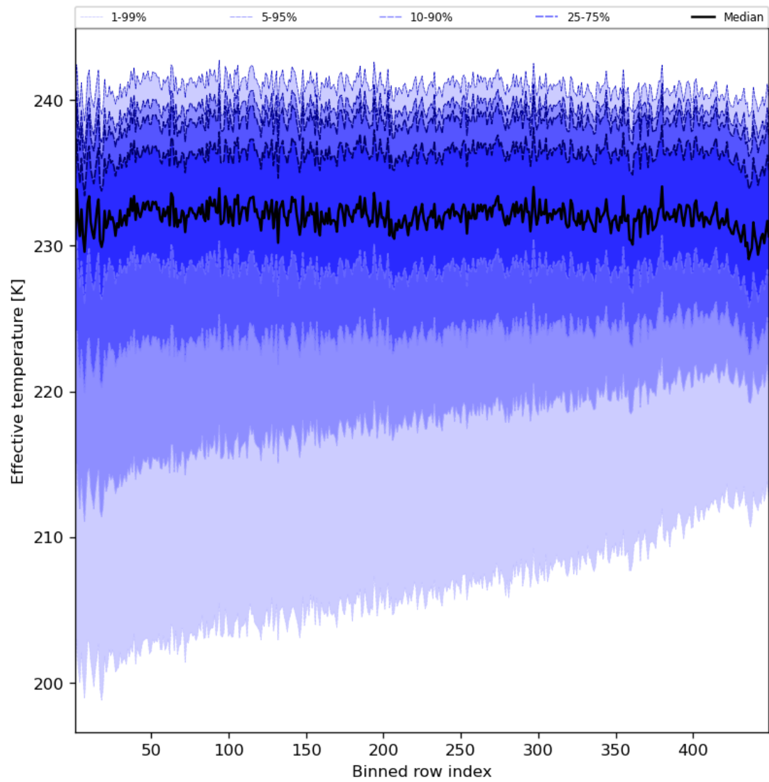
Figure 31: Along track statistics of “Effective temperature” for 2023-07-11 to 2023-07-13
