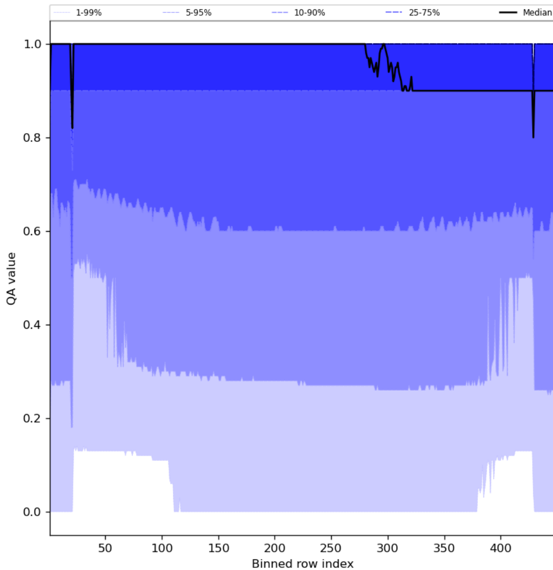
Figure 27: Along track statistics of “QA value” for 2023-07-11 to 2023-07-13
