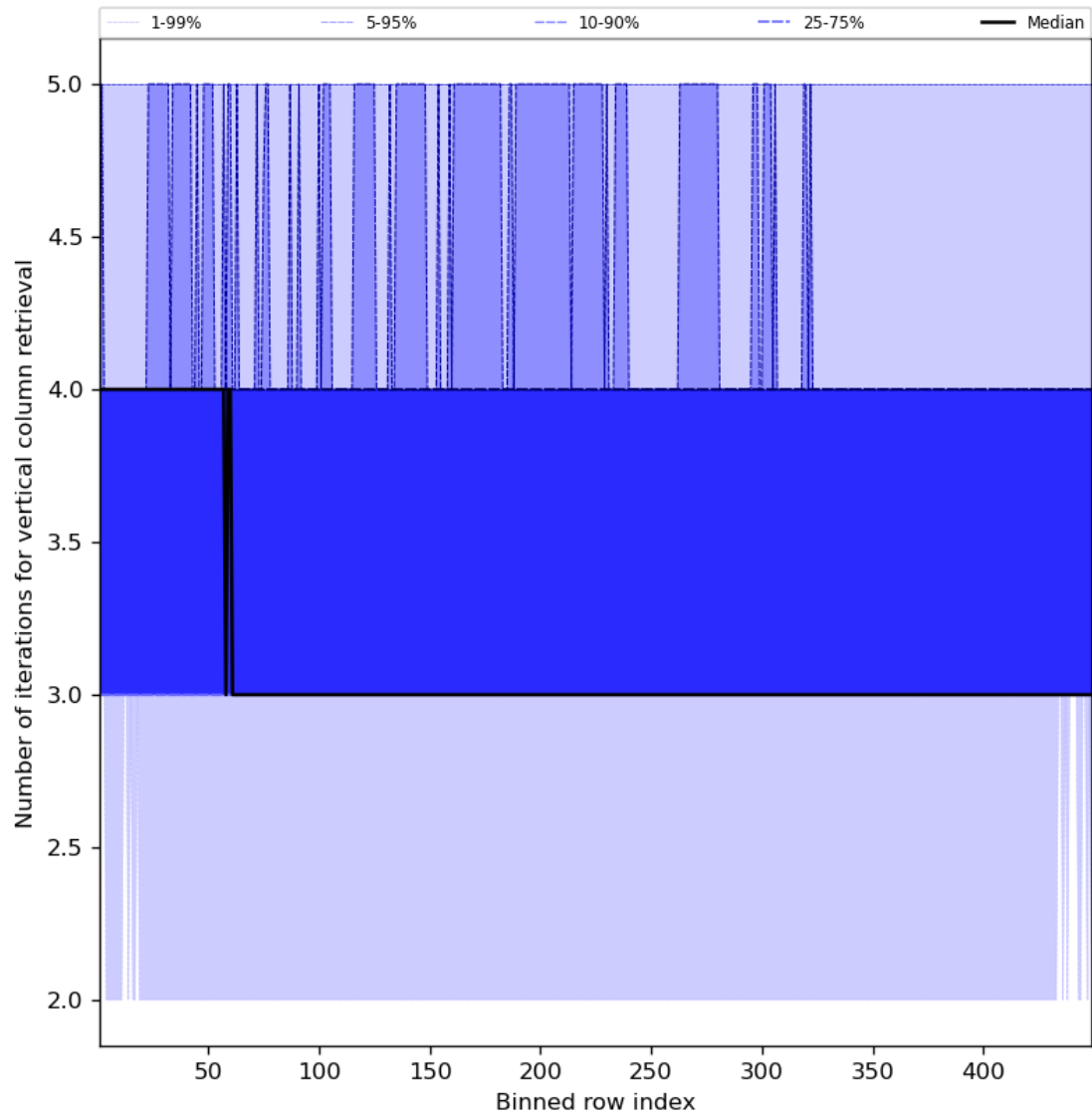
Figure 33: Along track statistics of “Number of iterations for vertical column retrieval” for 2023-07-11 to 2023-07-13
