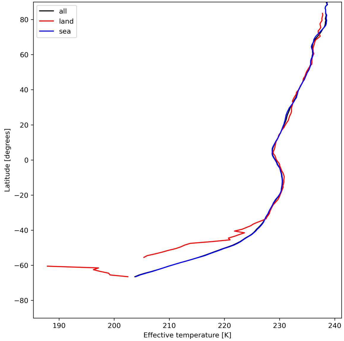
Figure 17: Zonal average of “Effective temperature” for 2023-07-11 to 2023-07-13.
