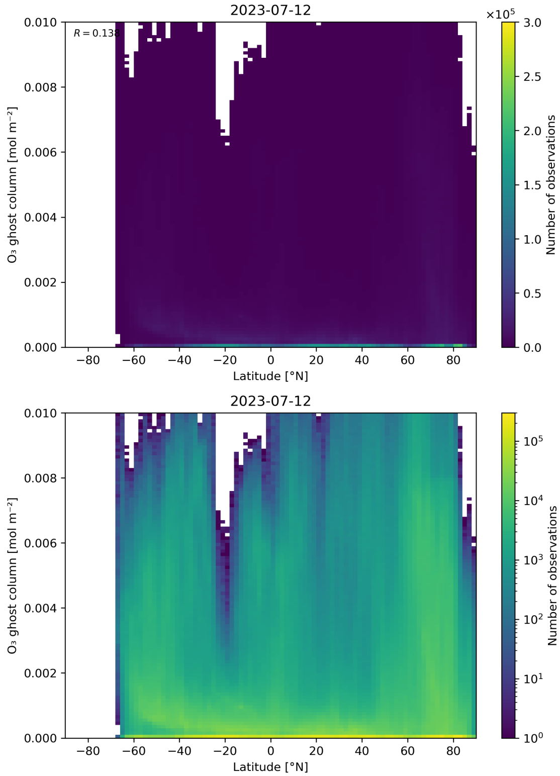
Figure 35: Scatter density plot of “Latitude” against “O 3 ghost column” for 2023-07-11 to 2023-07-13.
