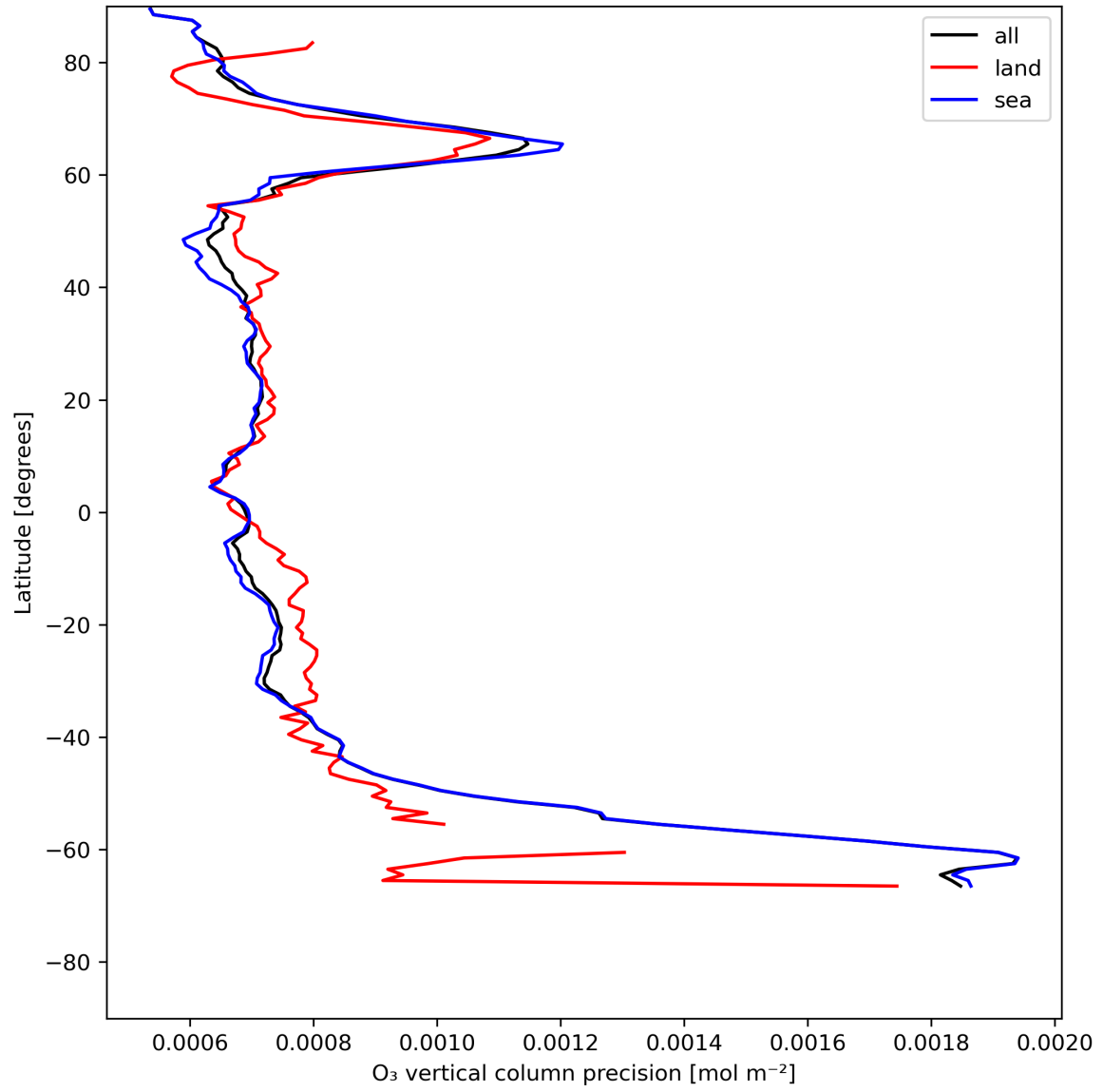
Figure 15: Zonal average of “O 3 vertical column precision” for 2023-07-11 to 2023-07-13.
