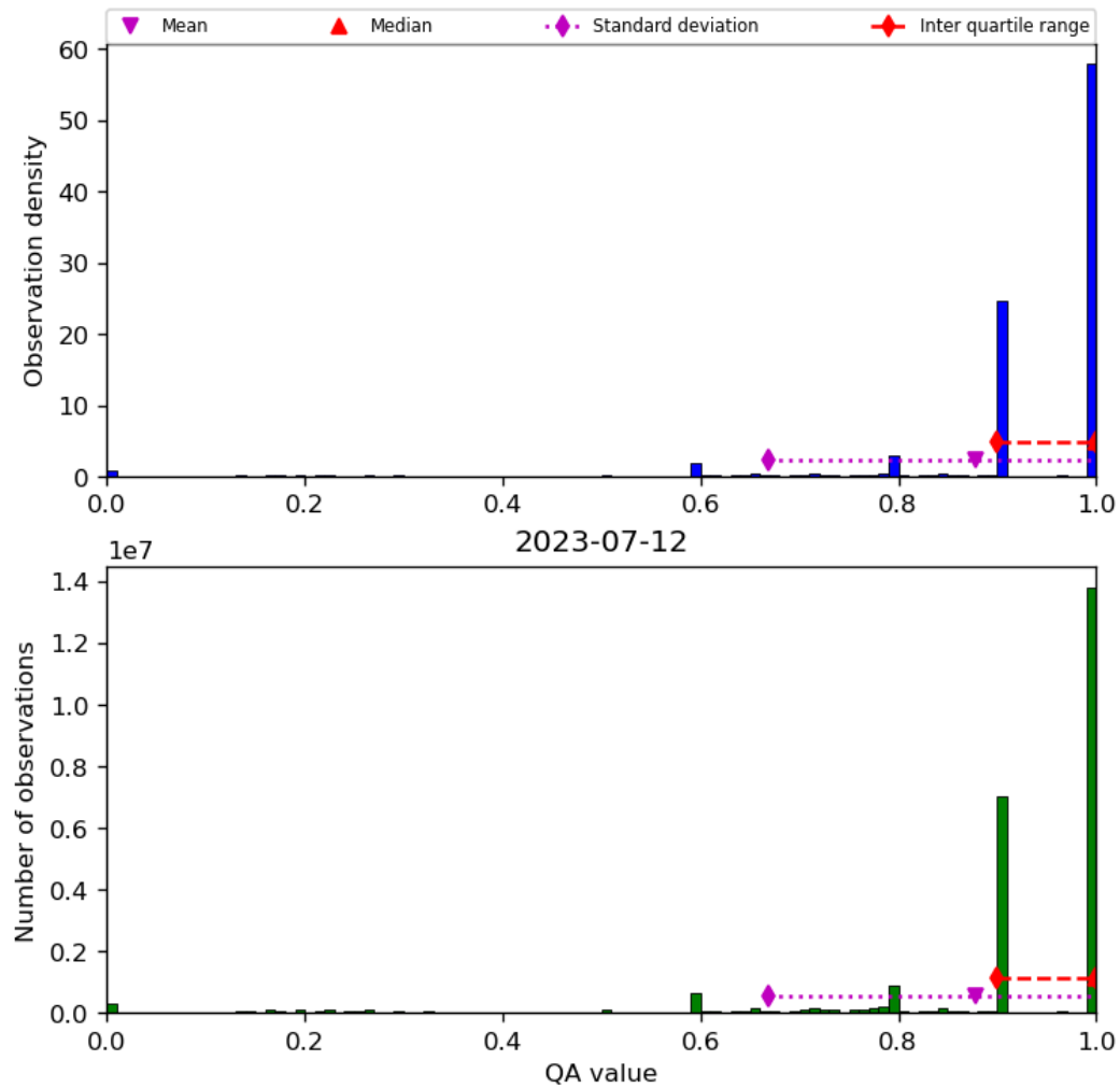
Figure 20: Histogram of “QA value” for 2023-07-11 to 2023-07-13
