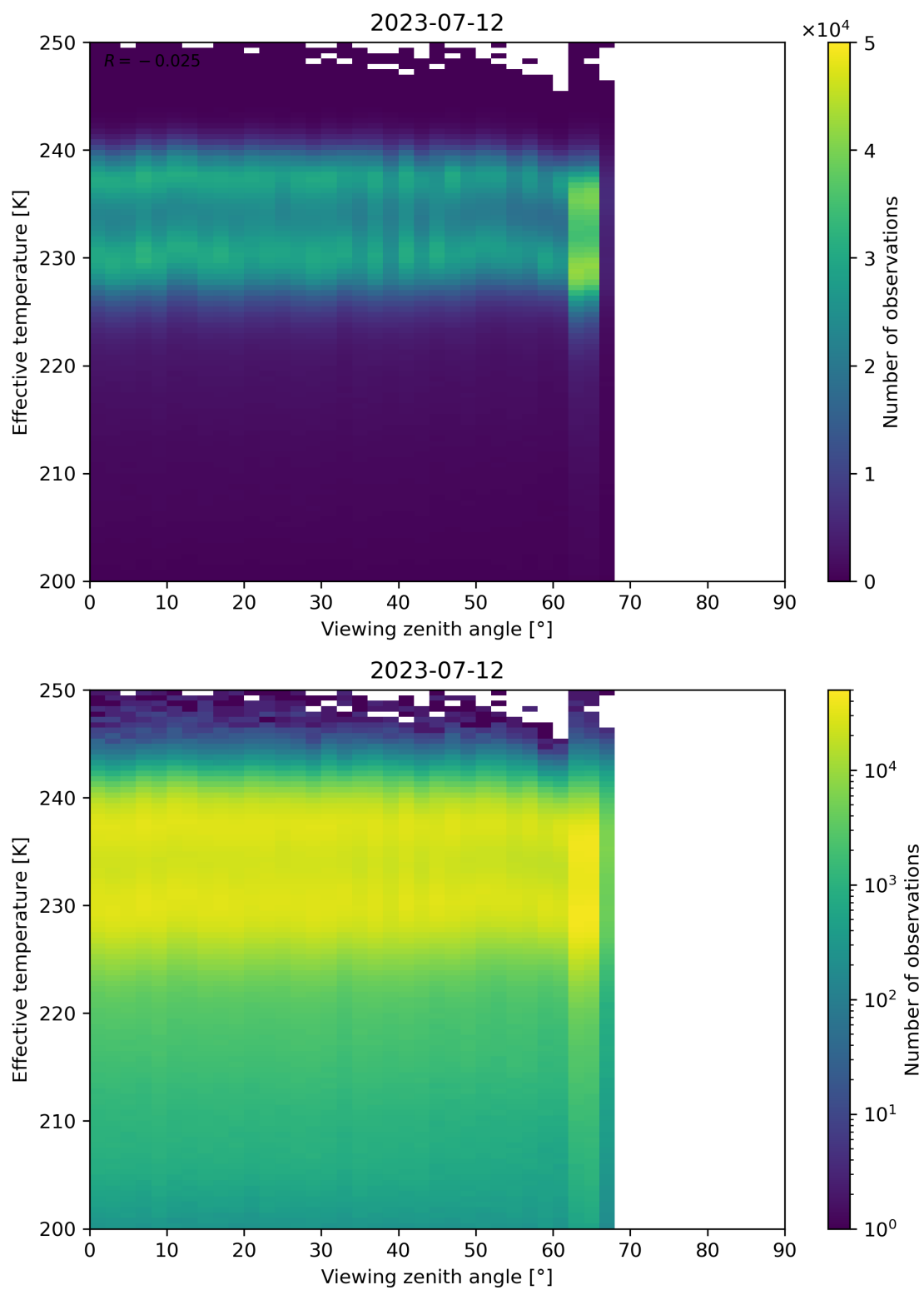
Figure 50: Scatter density plot of “Viewing zenith angle” against “Effective temperature” for 2023-07-11 to 2023-07-13.
