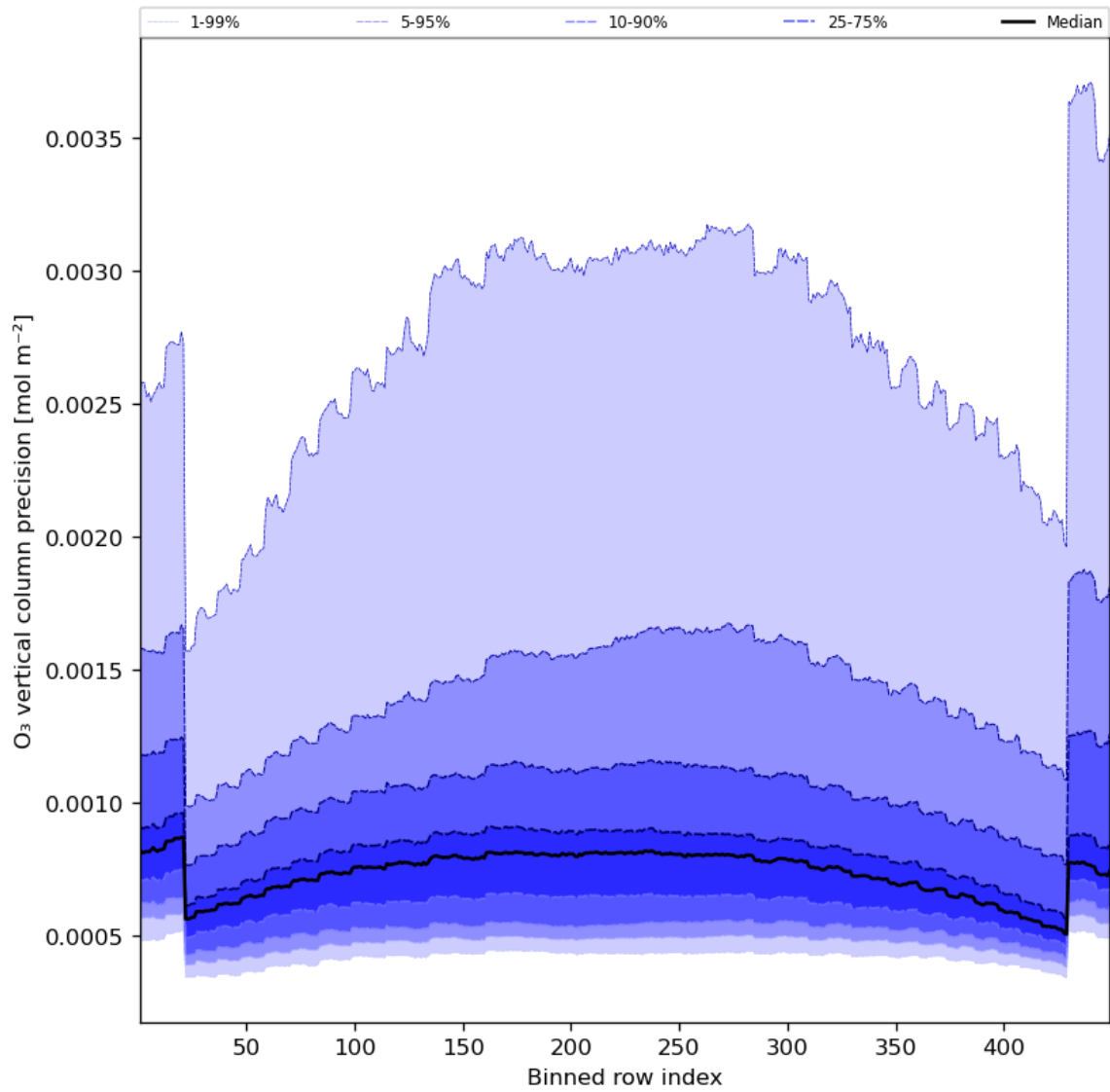
Figure 29: Along track statistics of “O 3 vertical column precision” for 2023-07-11 to 2023-07-13
