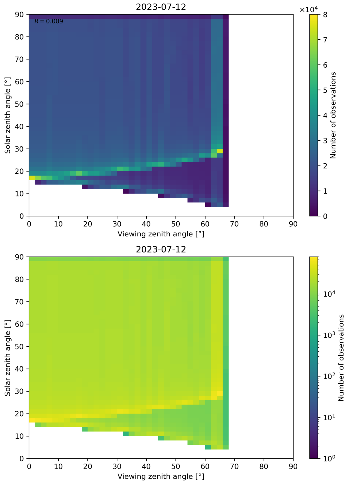
Figure 54: Scatter density plot of “Viewing zenith angle” against “Solar zenith angle” for 2023-07-11 to 2023-07-13.
