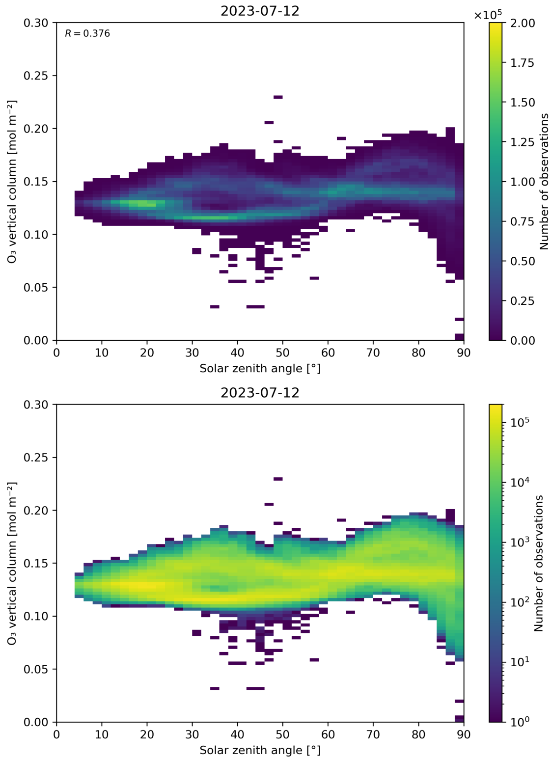
Figure 47: Scatter density plot of “Solar zenith angle” against “O 3 vertical column” for 2023-07-11 to 2023-07-13.
