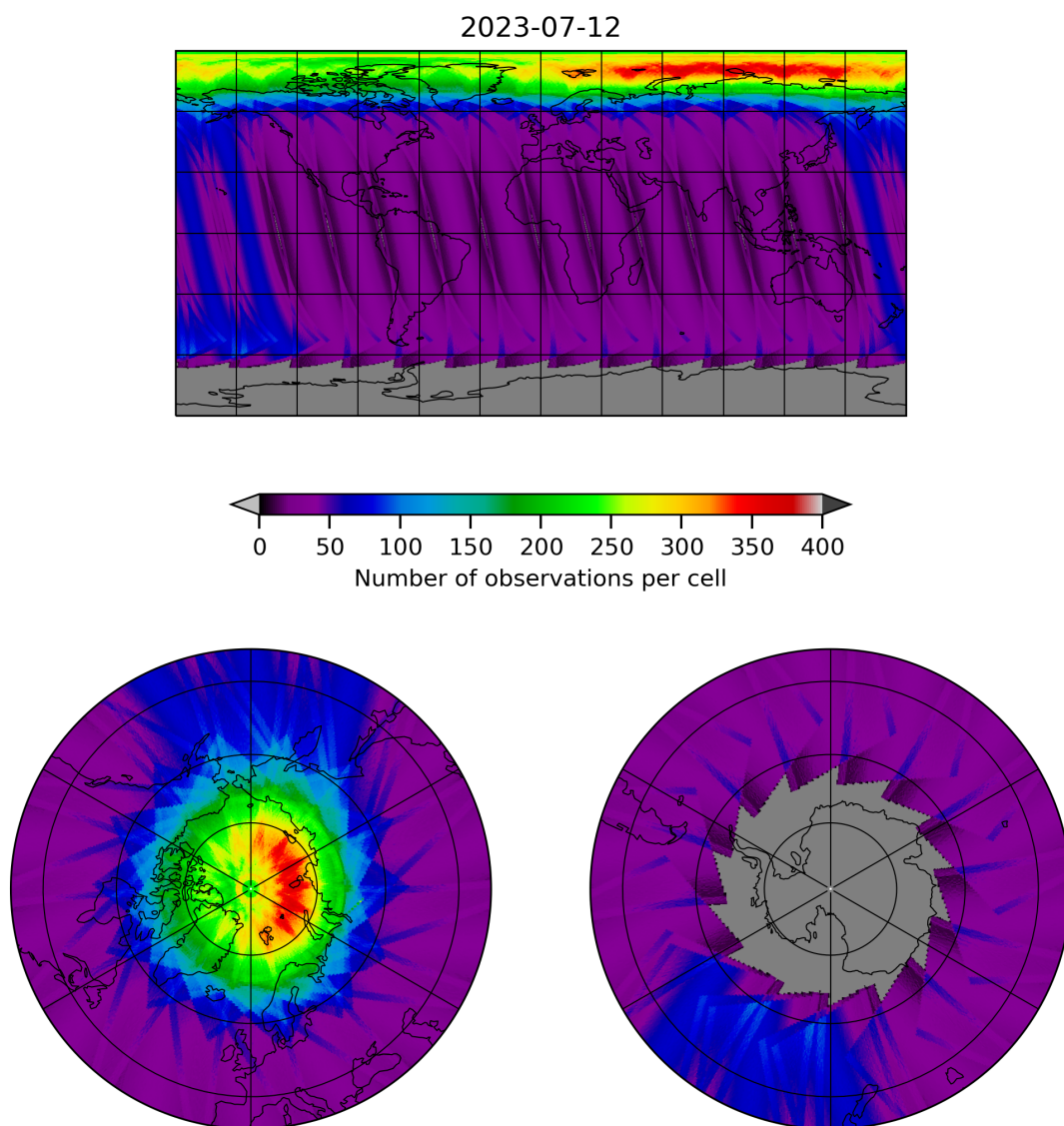
Figure 12: Map of the number of observations for 2023-07-11 to 2023-07-13
