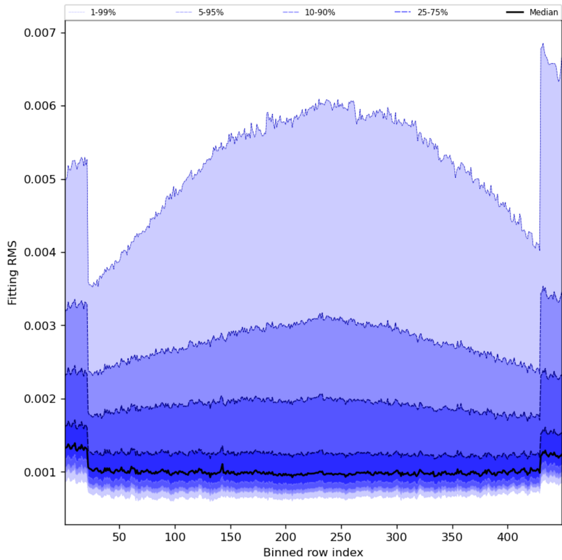
Figure 30: Along track statistics of “Fitting RMS” for 2023-07-11 to 2023-07-13
