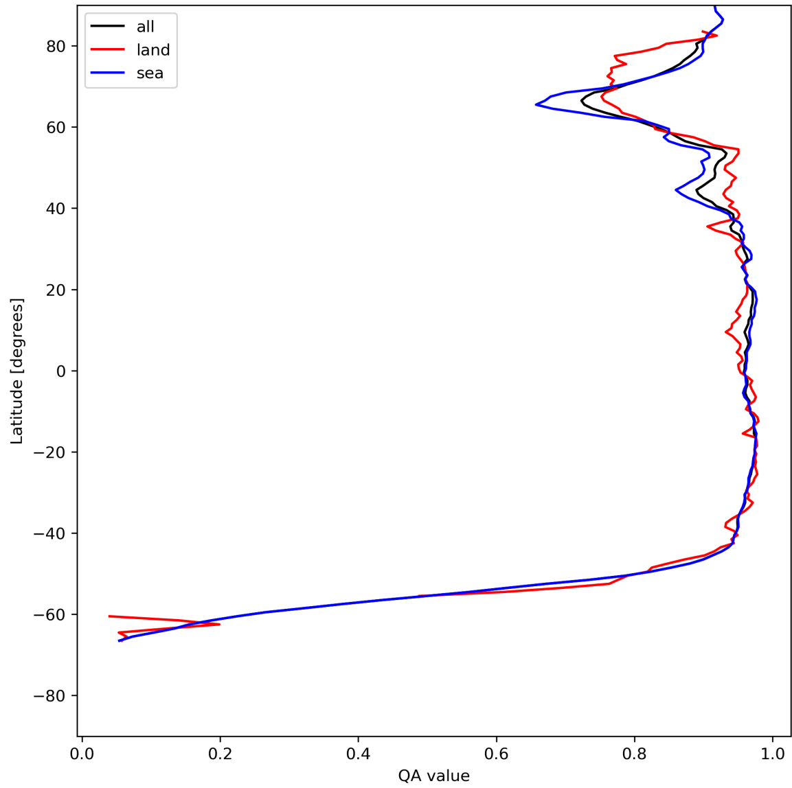
Figure 13: Zonal average of “QA value” for 2023-07-11 to 2023-07-13.
