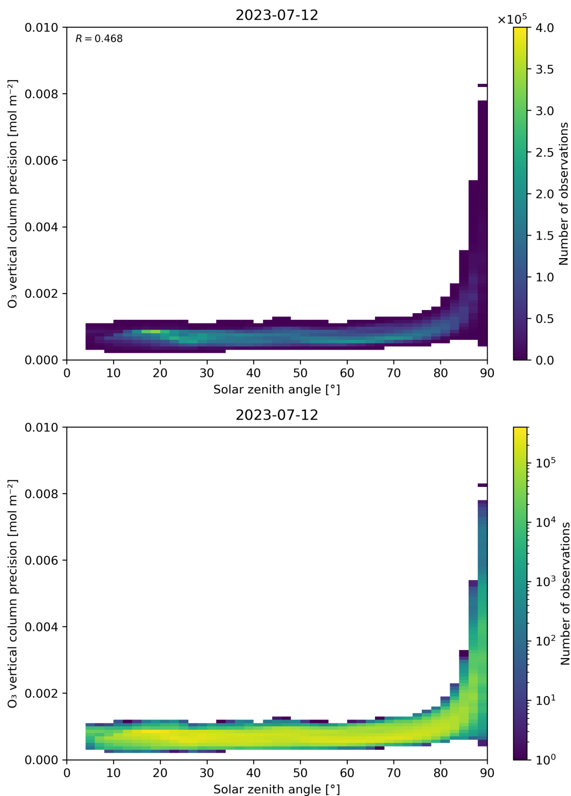
Figure 48: Scatter density plot of “Solar zenith angle” against “O 3 vertical column precision” for 2023-07-11 to 2023-07-13.
