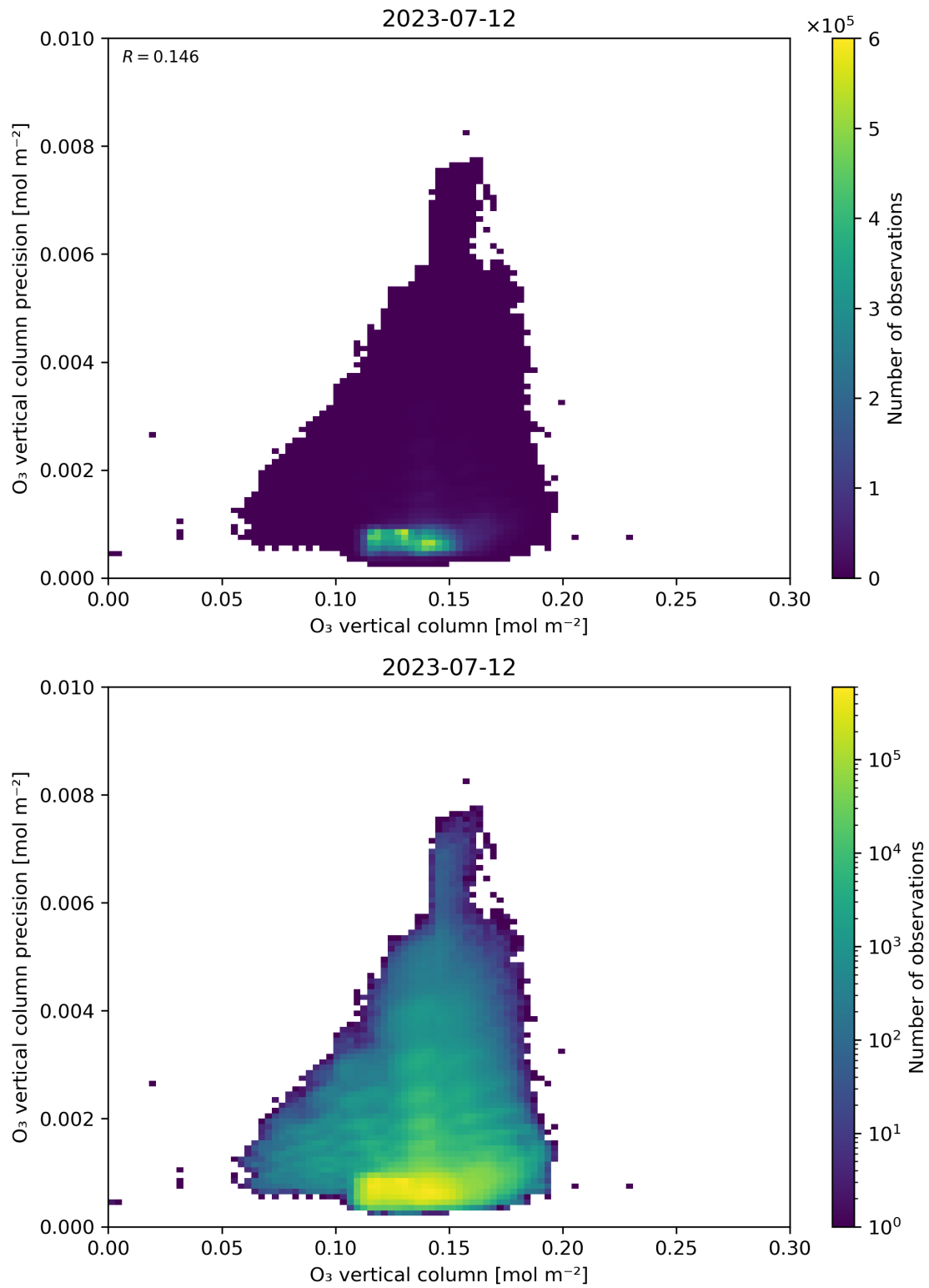
Figure 41: Scatter density plot of “O 3 vertical column” against “O 3 vertical column precision” for 2023-07-11 to 2023-07-13.
