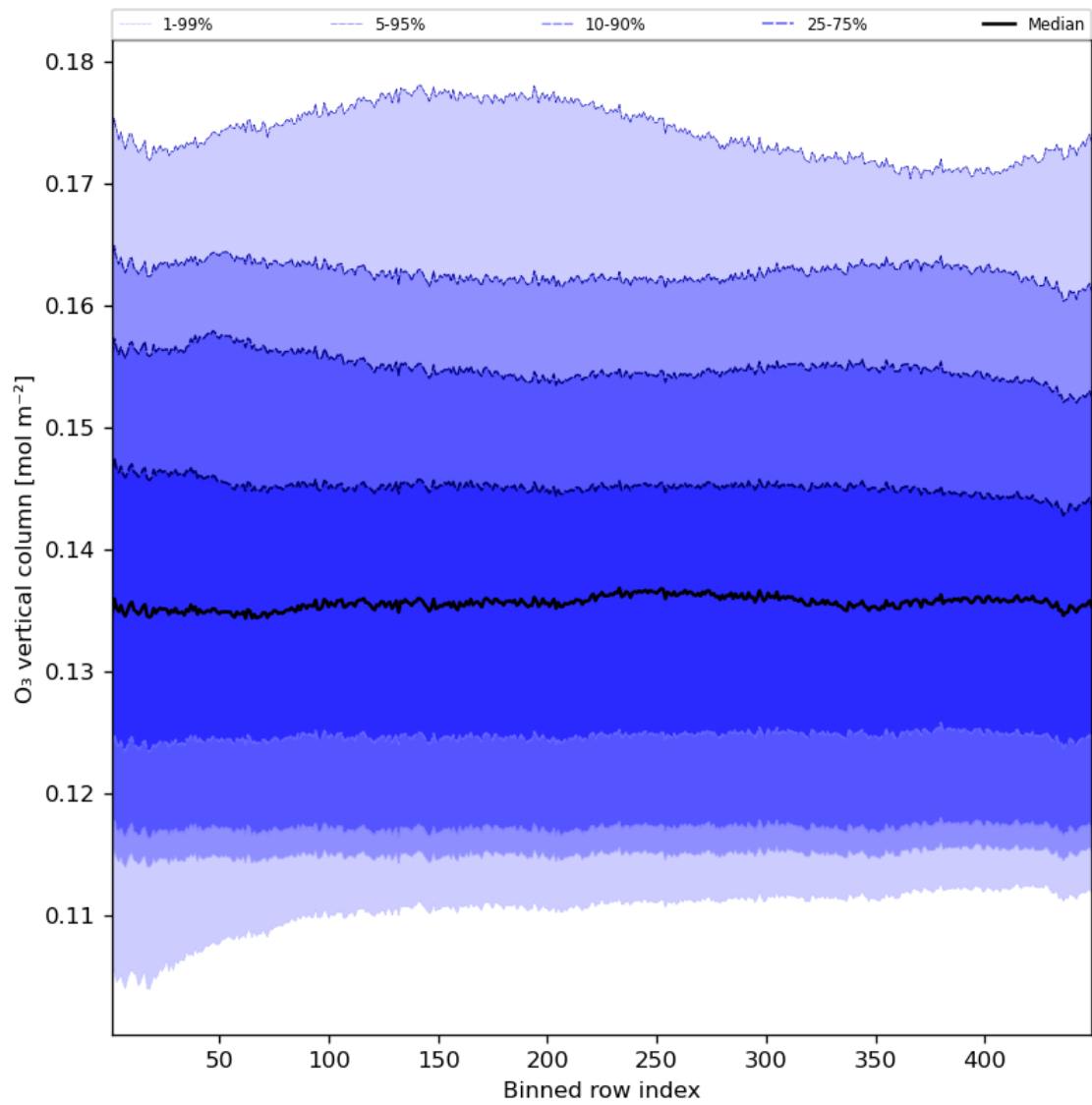
Figure 28: Along track statistics of “O 3 vertical column” for 2023-07-11 to 2023-07-13
