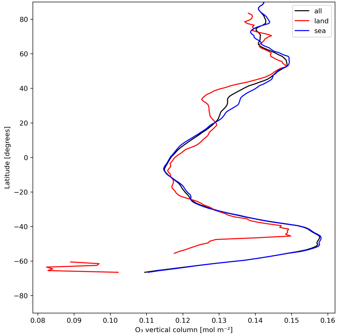
Figure 14: Zonal average of “O 3 vertical column” for 2023-07-11 to 2023-07-13.
