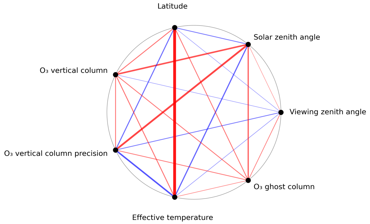
Figure 1: Map of correlation graph for 2023-07-11 to 2023-07-13.
