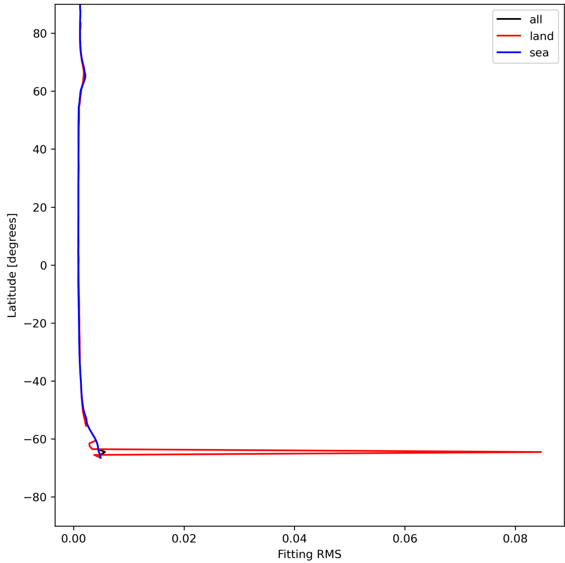
Figure 16: Zonal average of “Fitting RMS” for 2023-07-11 to 2023-07-13.
