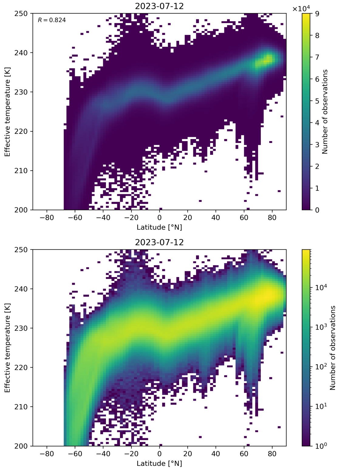
Figure 34: Scatter density plot of “Latitude” against “Effective temperature” for 2023-07-11 to 2023-07-13.
