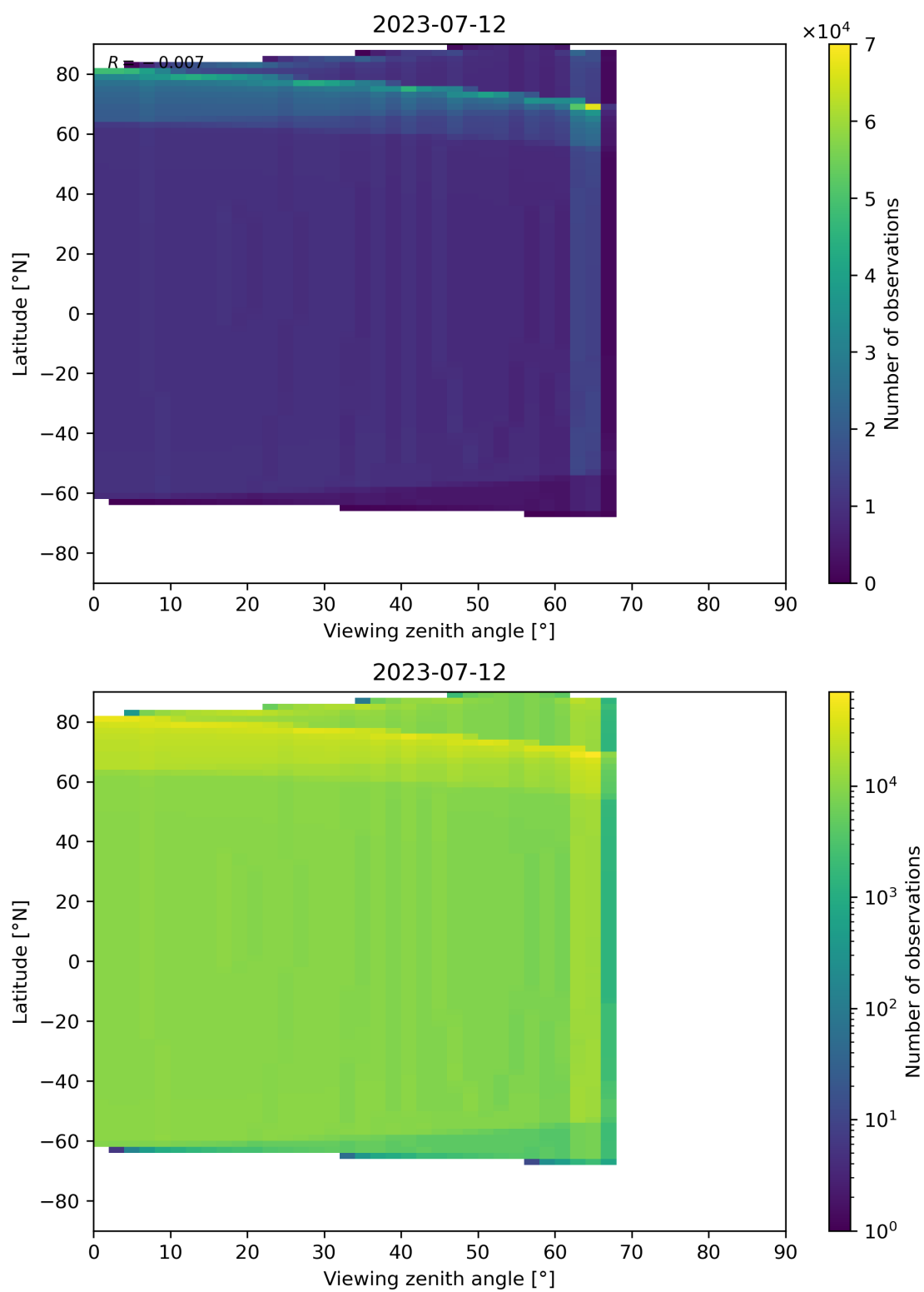
Figure 49: Scatter density plot of “Viewing zenith angle” against “Latitude” for 2023-07-11 to 2023-07-13.
