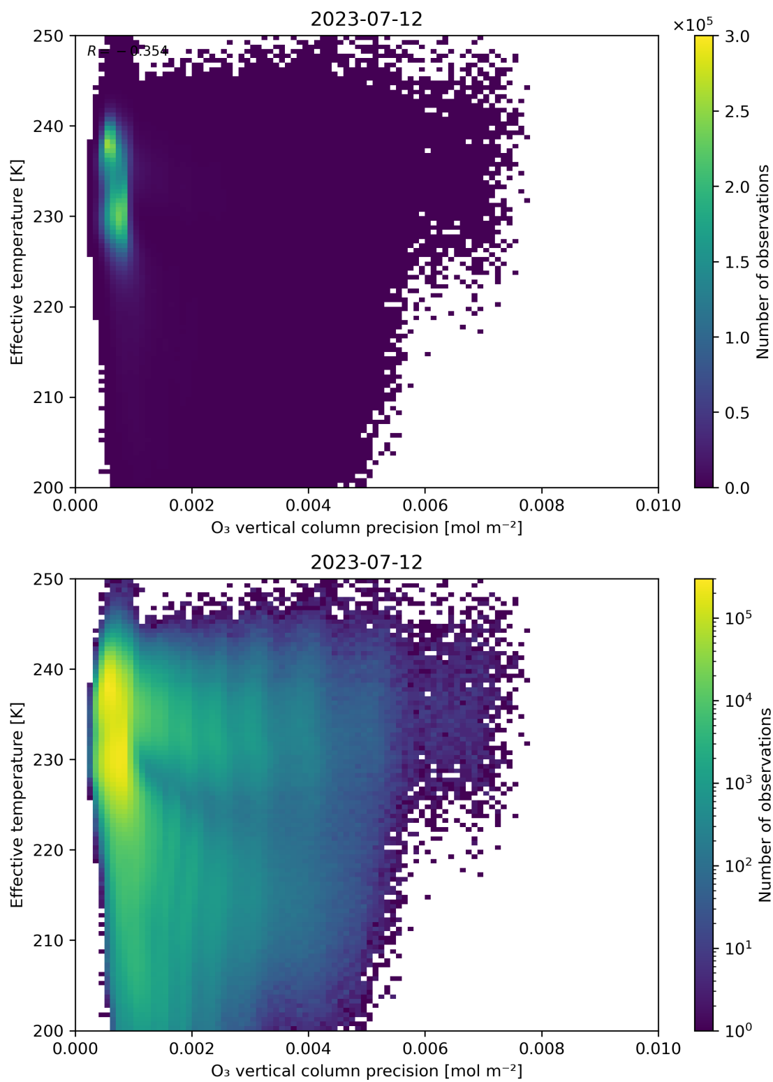
Figure 42: Scatter density plot of “O 3 vertical column precision” against “Effective temperature” for 2023-07-11 to 2023-07-13.
