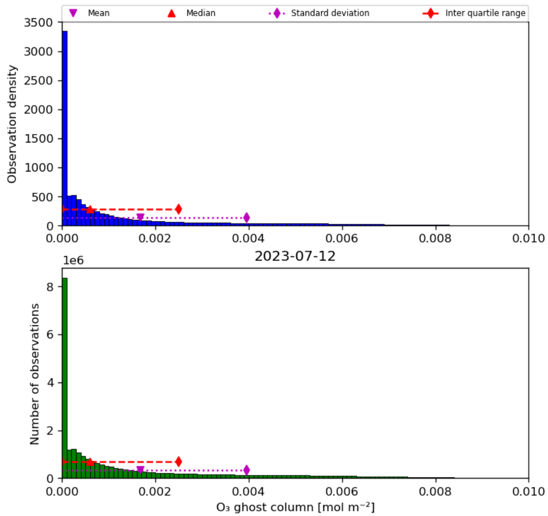
Figure 25: Histogram of “O 3 ghost column” for 2023-07-11 to 2023-07-13
