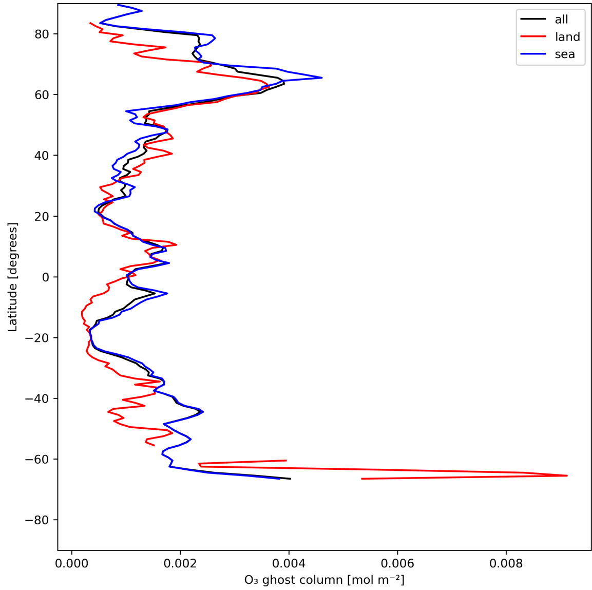
Figure 18: Zonal average of "O 3 ghost column" for 2023-07-11 to 2023-07-13.
