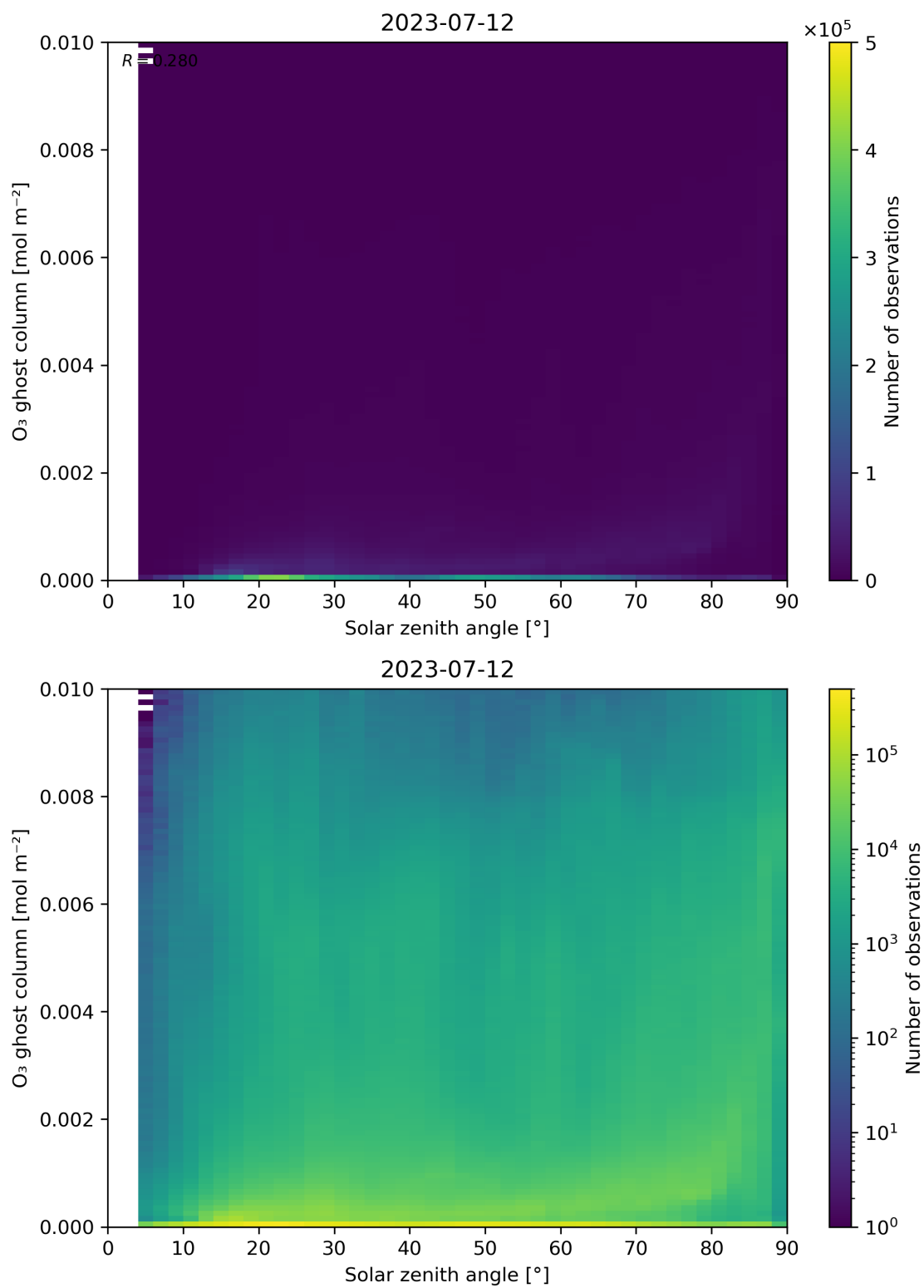
Figure 46: Scatter density plot of “Solar zenith angle” against “O 3 ghost column” for 2023-07-11 to 2023-07-13.
