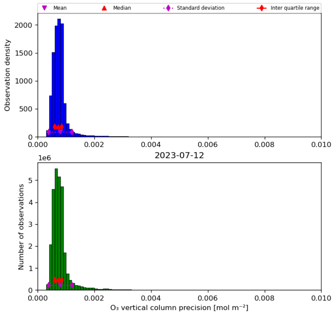
Figure 22: Histogram of “O 3 vertical column precision” for 2023-07-11 to 2023-07-13
