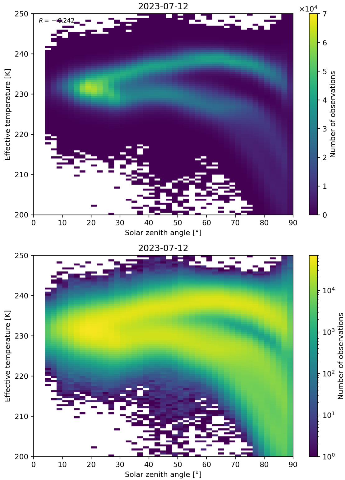
Figure 45: Scatter density plot of “Solar zenith angle” against “Effective temperature” for 2023-07-11 to 2023-07-13.
