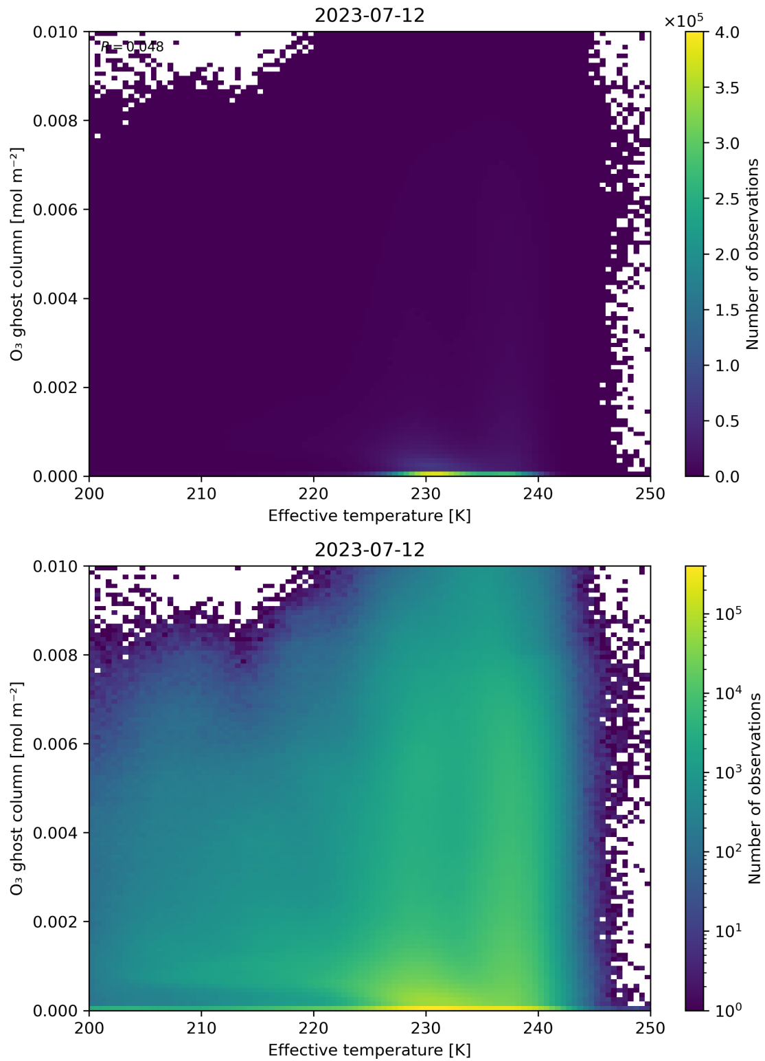
Figure 38: Scatter density plot of “Effective temperature” against “O 3 ghost column” for 2023-07-11 to 2023-07-13.
