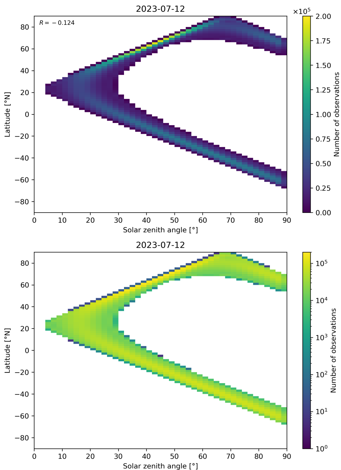
Figure 44: Scatter density plot of “Solar zenith angle” against “Latitude” for 2023-07-11 to 2023-07-13.
