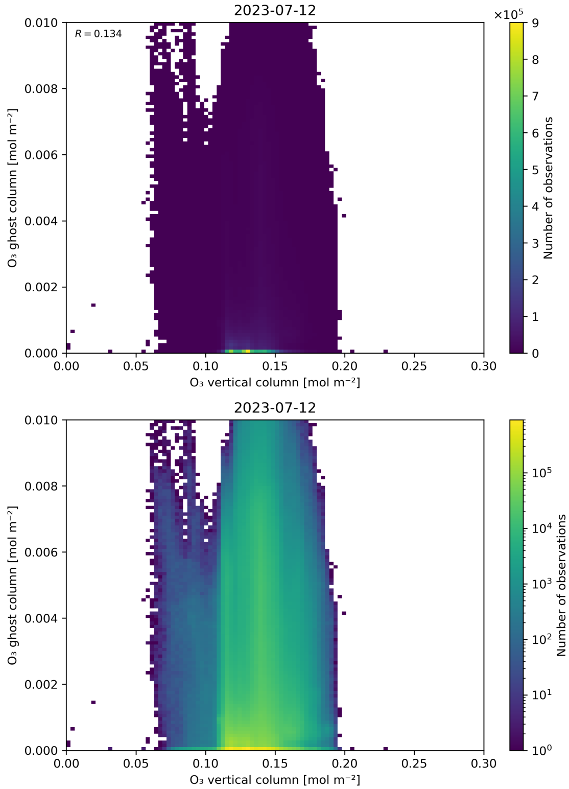
Figure 40: Scatter density plot of “O 3 vertical column” against “O 3 ghost column” for 2023-07-11 to 2023-07-13.
