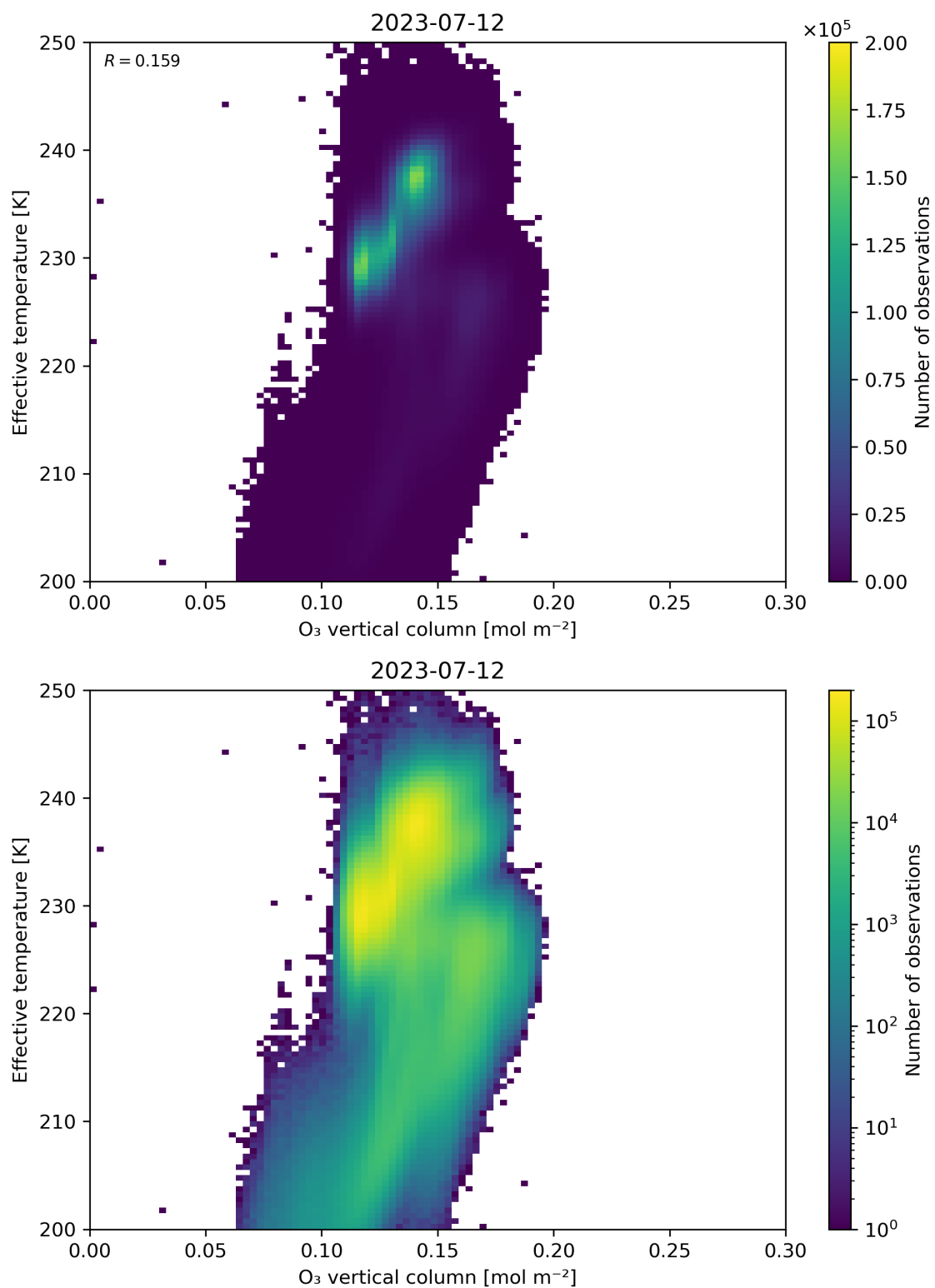
Figure 39: Scatter density plot of “O 3 vertical column” against “Effective temperature” for 2023-07-11 to 2023-07-13.
