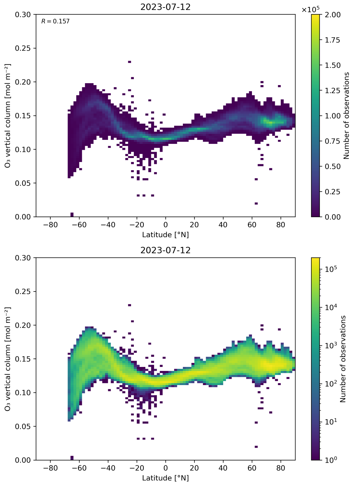
Figure 36: Scatter density plot of “Latitude” against “O 3 vertical column” for 2023-07-11 to 2023-07-13.
