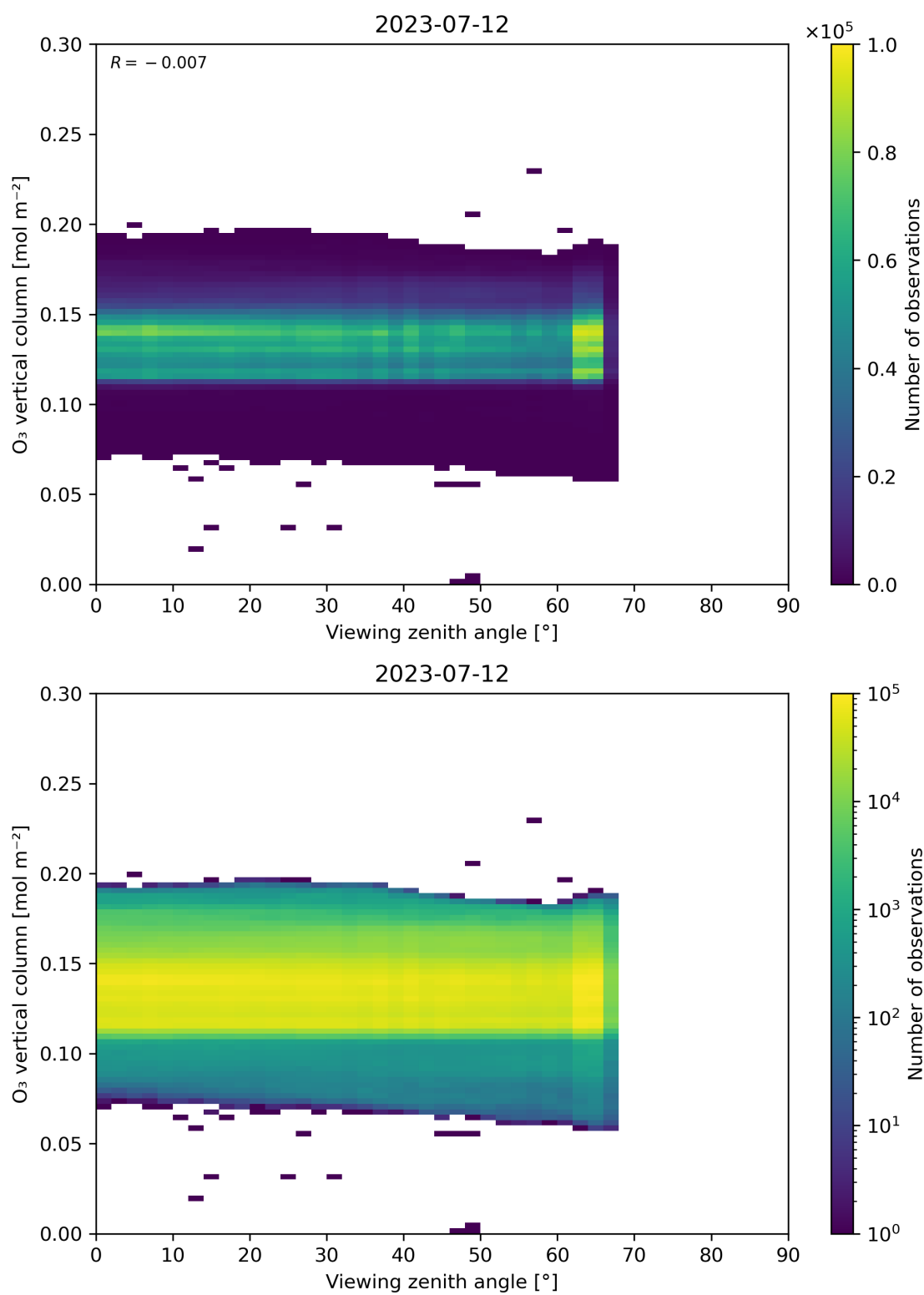
Figure 52: Scatter density plot of “Viewing zenith angle” against “O 3 vertical column” for 2023-07-11 to 2023-07-13.
