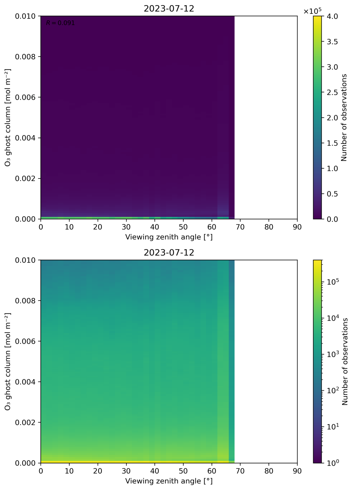
Figure 51: Scatter density plot of “Viewing zenith angle” against “O 3 ghost column” for 2023-07-11 to 2023-07-13.
