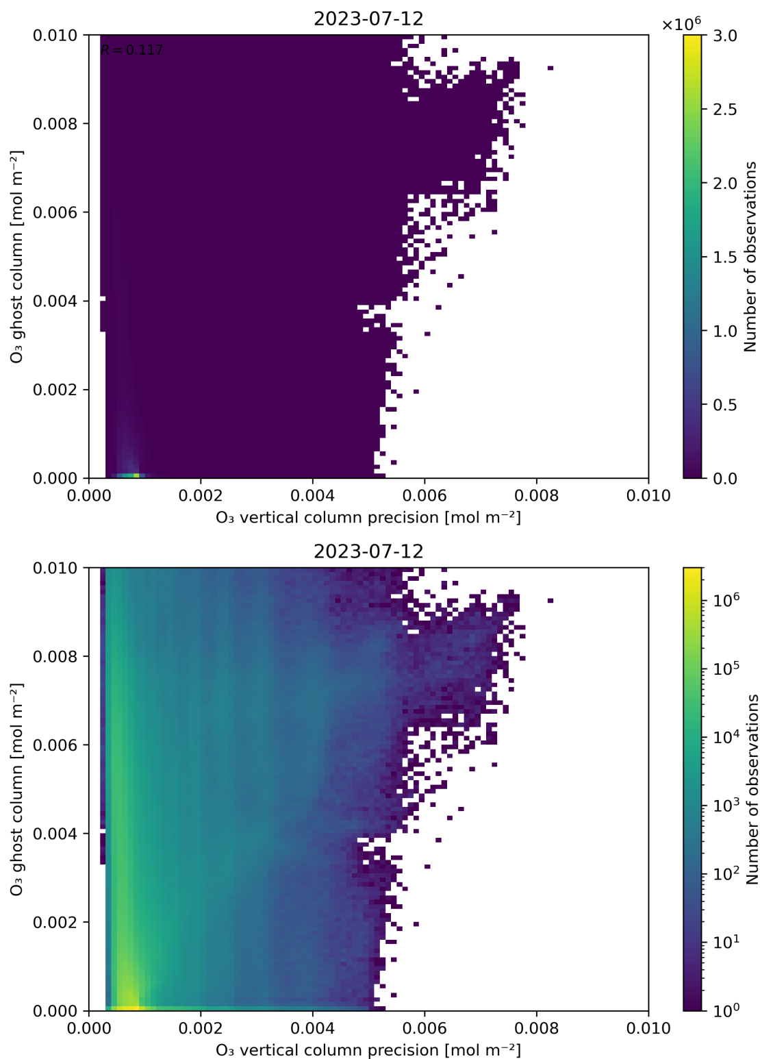
Figure 43: Scatter density plot of “ \text{O}_3 vertical column precision” against “ \text{O}_3 ghost column” for 2023-07-11 to 2023-07-13.
