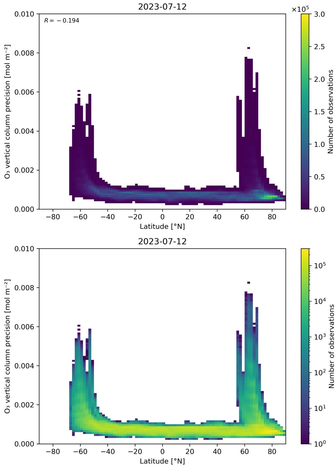
Figure 37: Scatter density plot of “Latitude” against “O 3 vertical column precision” for 2023-07-11 to 2023-07-13.
