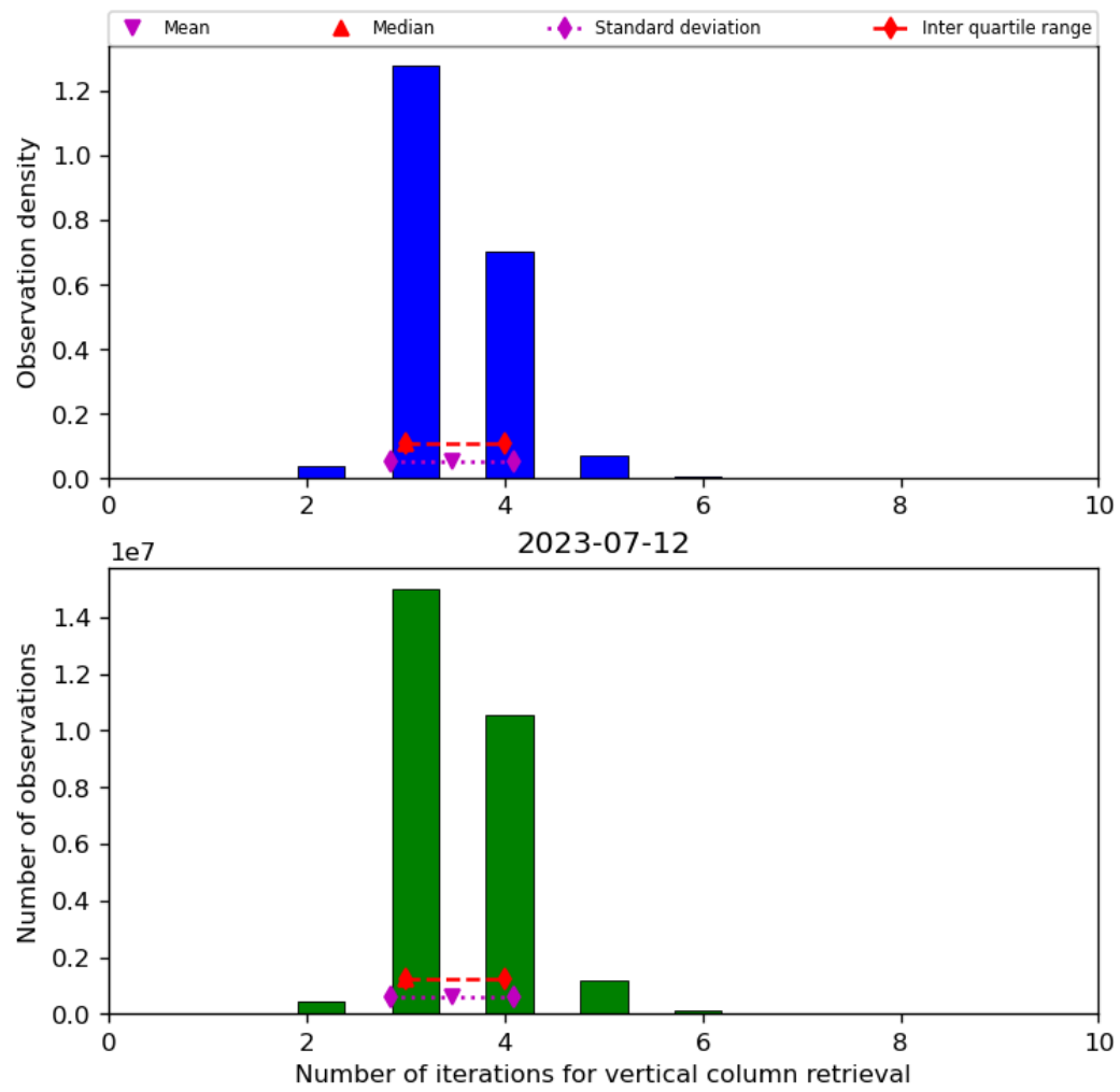
Figure 26: Histogram of “Number of iterations for vertical column retrieval” for 2023-07-11 to 2023-07-13
