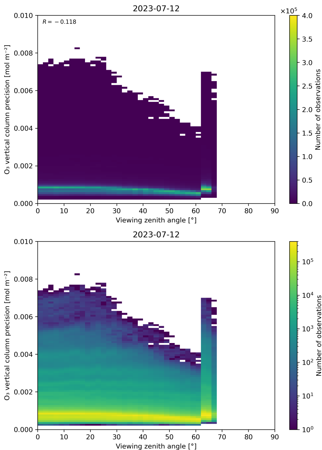
Figure 53: Scatter density plot of “Viewing zenith angle” against “O 3 vertical column precision” for 2023-07-11 to 2023-07-13.
