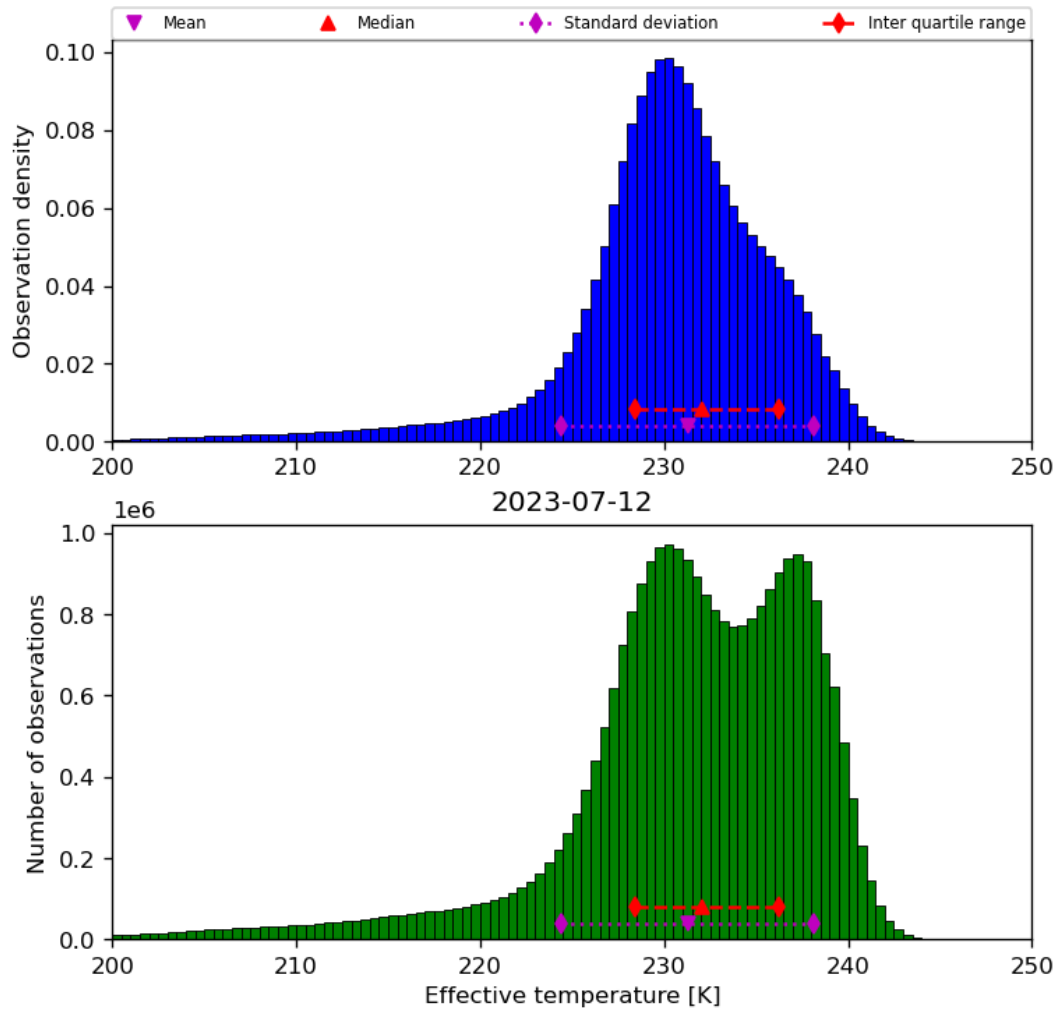
Figure 24: Histogram of “Effective temperature” for 2023-07-11 to 2023-07-13
