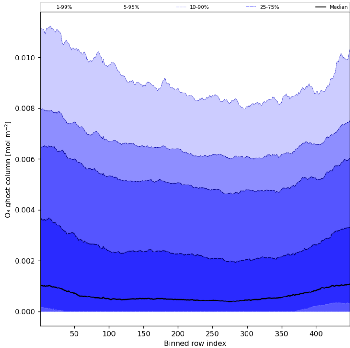
Figure 32: Along track statistics of “O 3 ghost column” for 2023-07-11 to 2023-07-13
