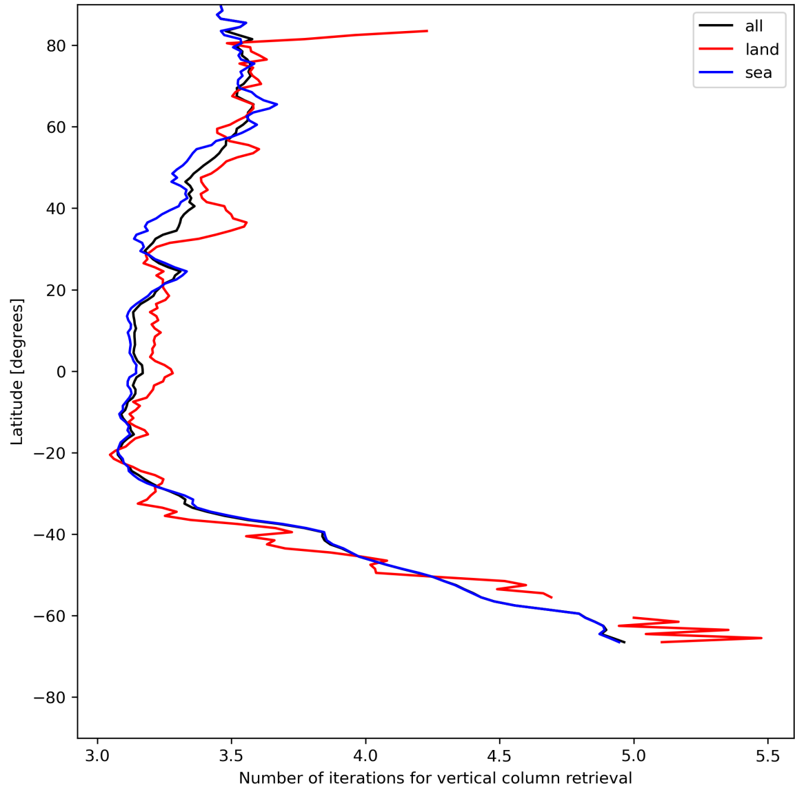
Figure 19: Zonal average of “Number of iterations for vertical column retrieval” for 2023-07-11 to 2023-07-13.
