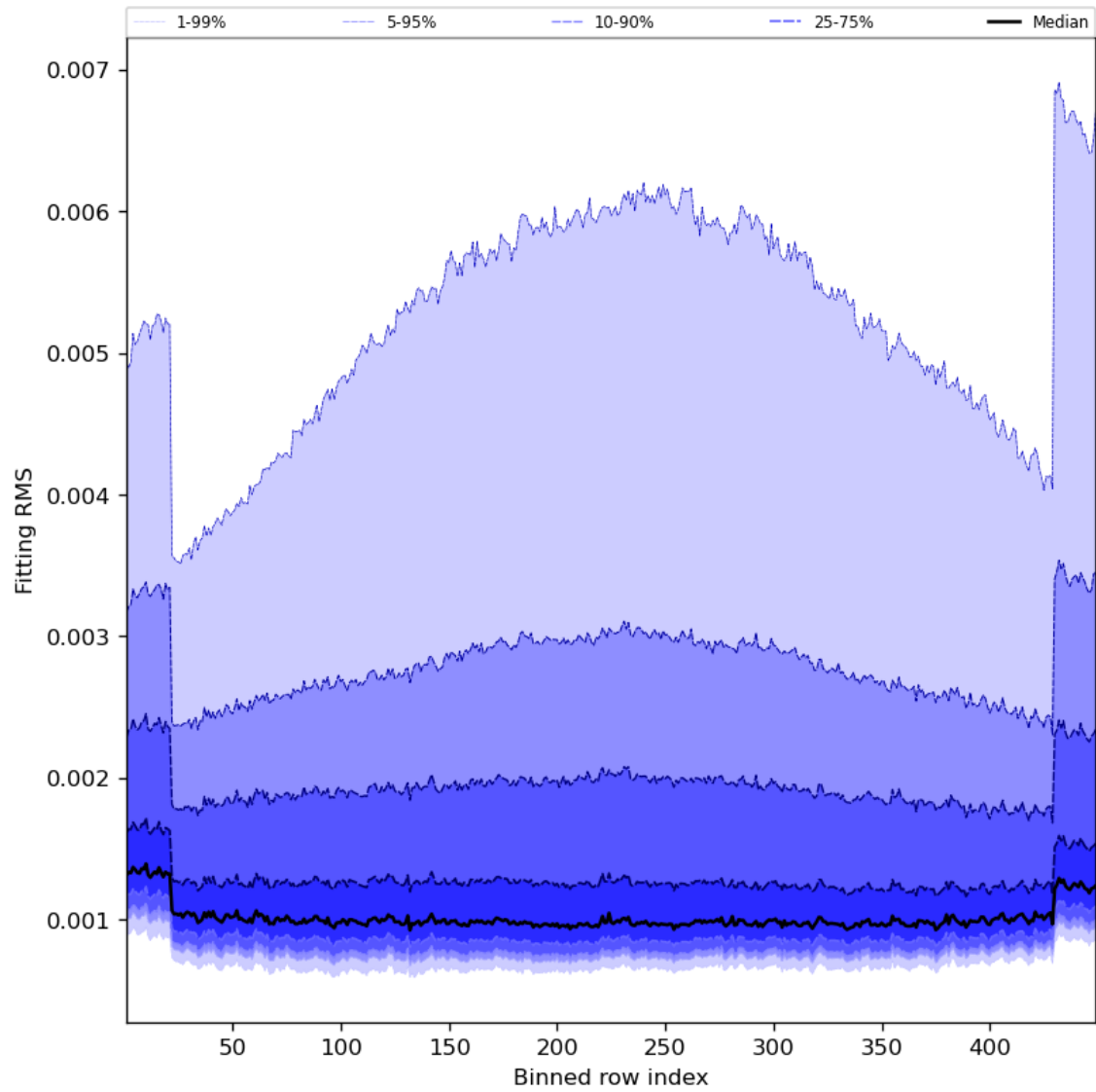
Figure 30: Along track statistics of “Fitting RMS” for 2023-07-13 to 2023-07-14
