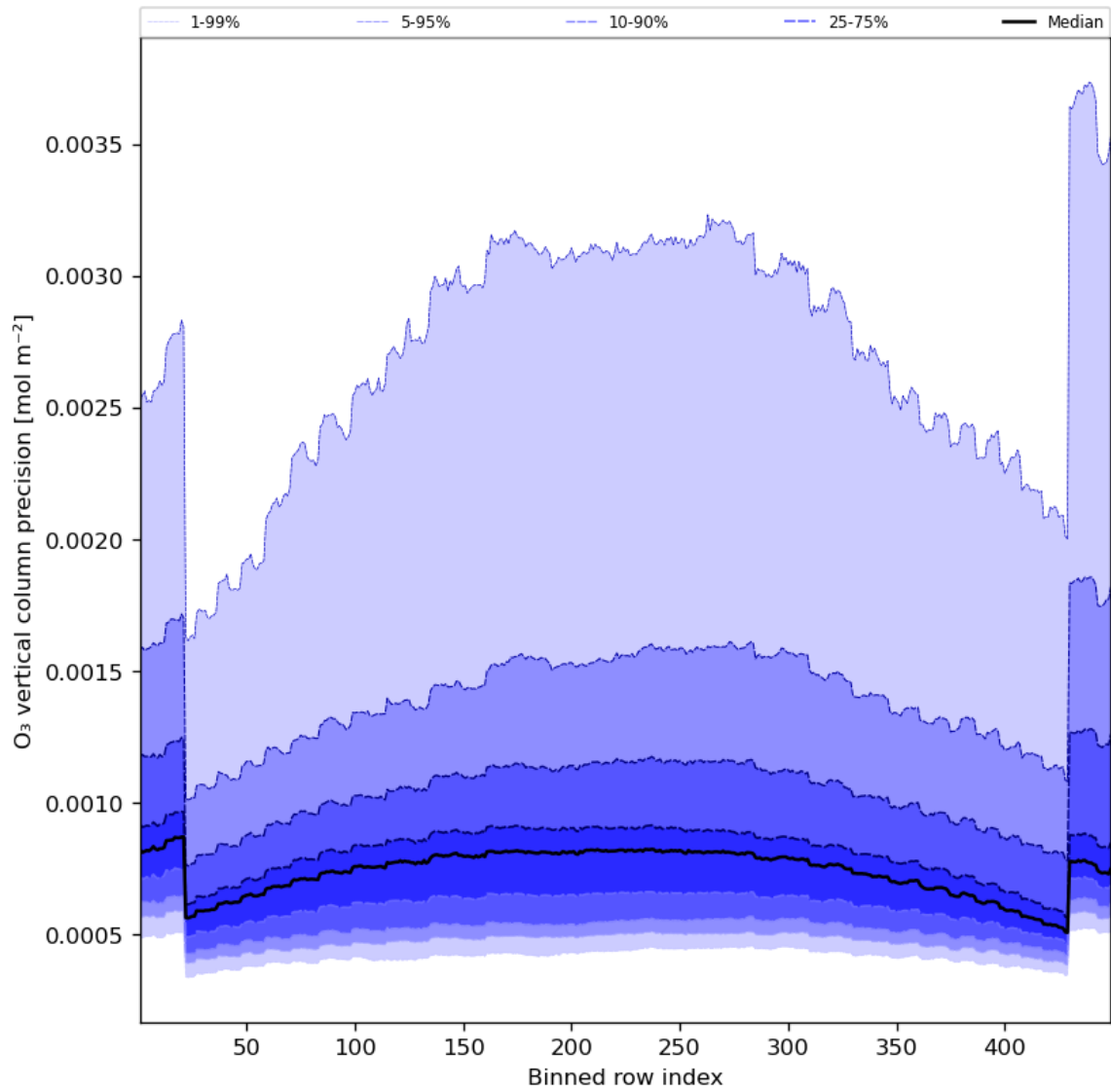
Figure 29: Along track statistics of “O 3 vertical column precision” for 2023-07-13 to 2023-07-14
