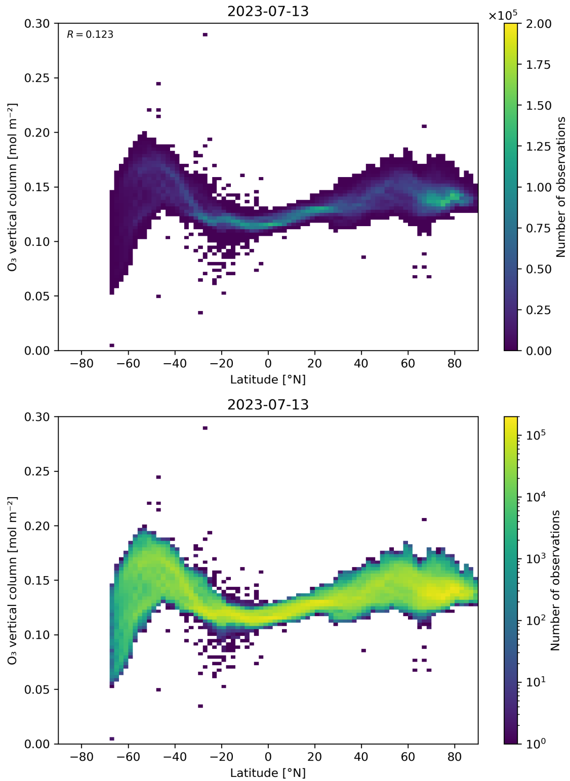
Figure 36: Scatter density plot of “Latitude” against “O 3 vertical column” for 2023-07-13 to 2023-07-14.
