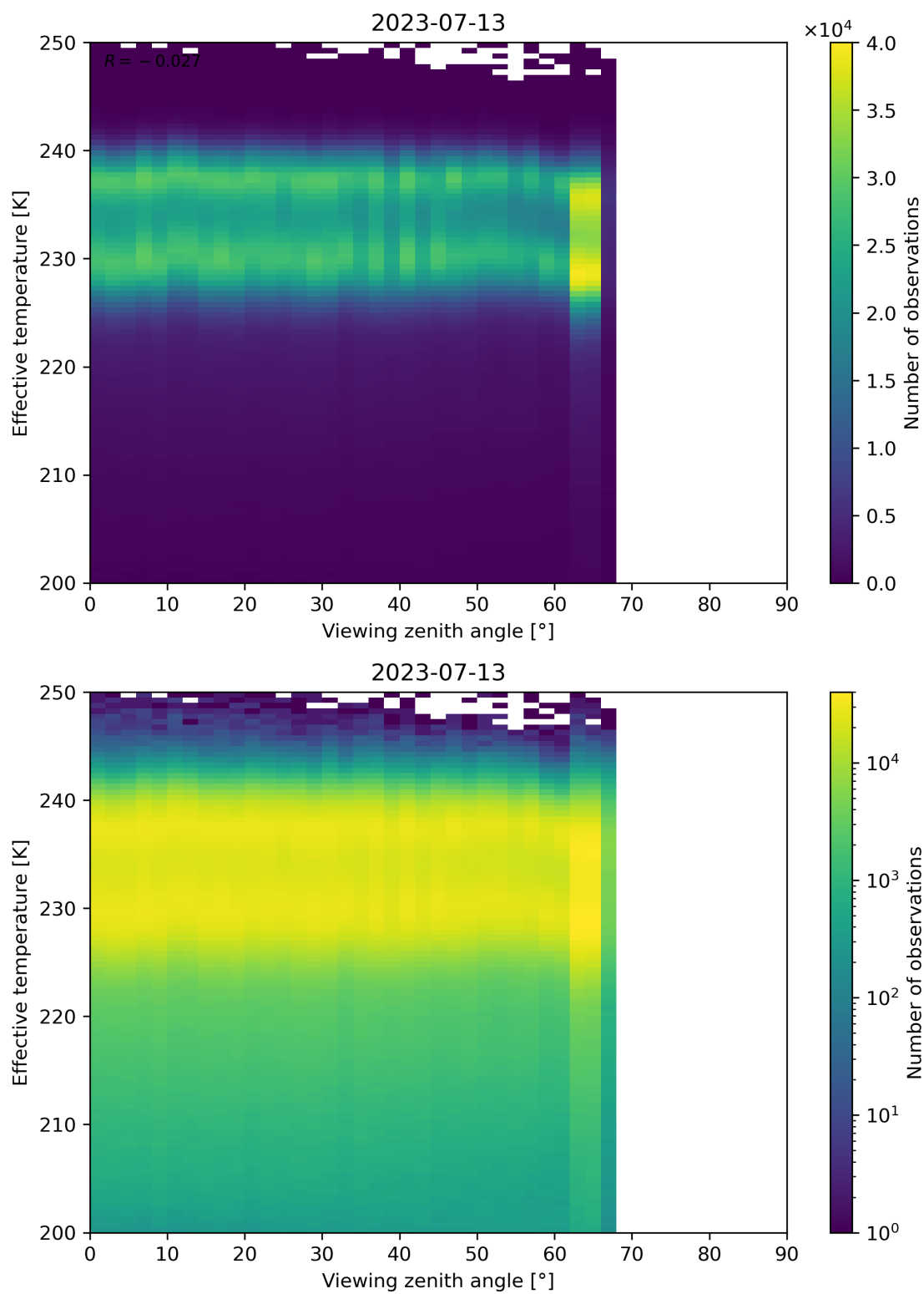
Figure 50: Scatter density plot of “Viewing zenith angle” against “Effective temperature” for 2023-07-13 to 2023-07-14.
