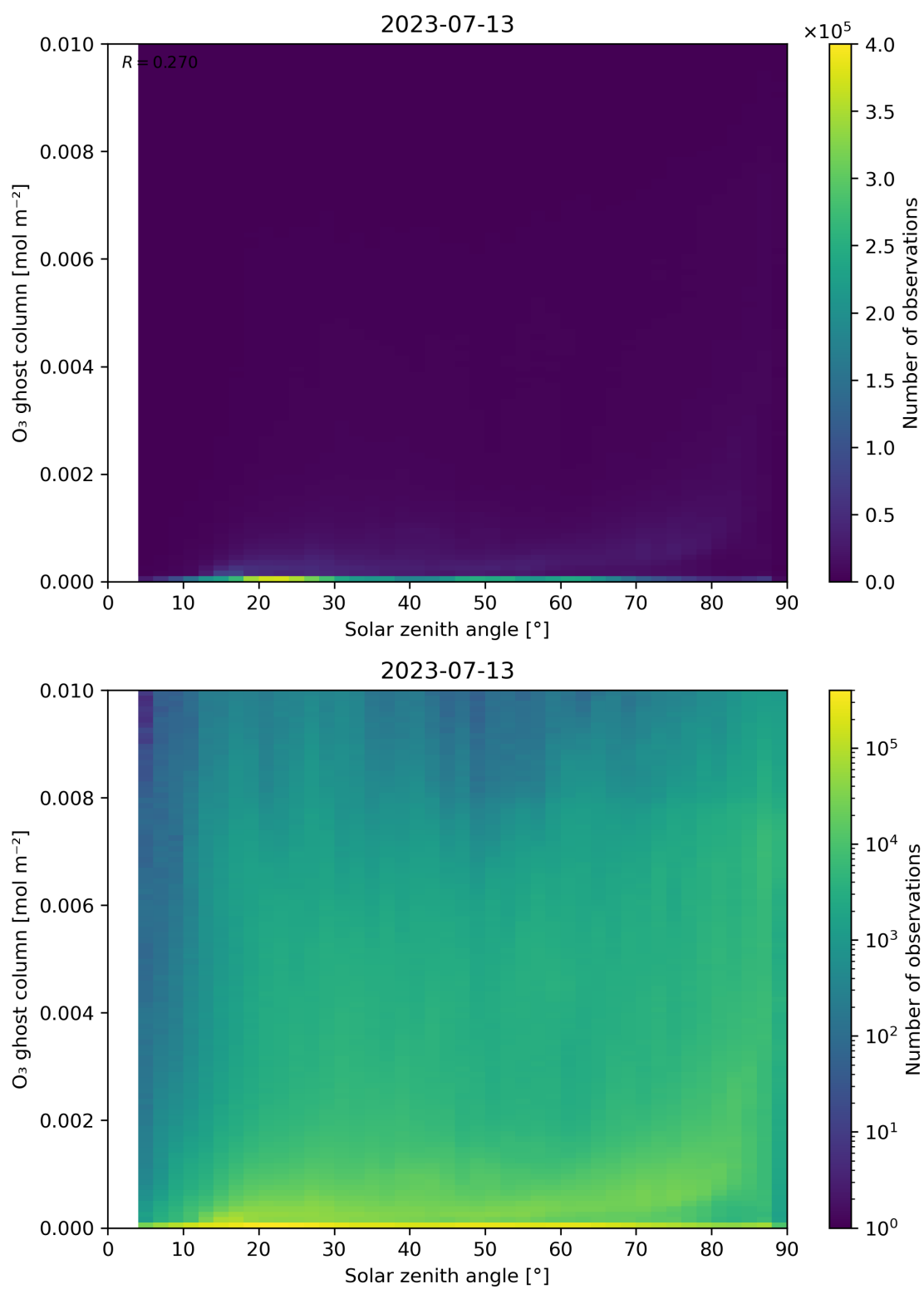
Figure 46: Scatter density plot of “Solar zenith angle” against “O 3 ghost column” for 2023-07-13 to 2023-07-14.
