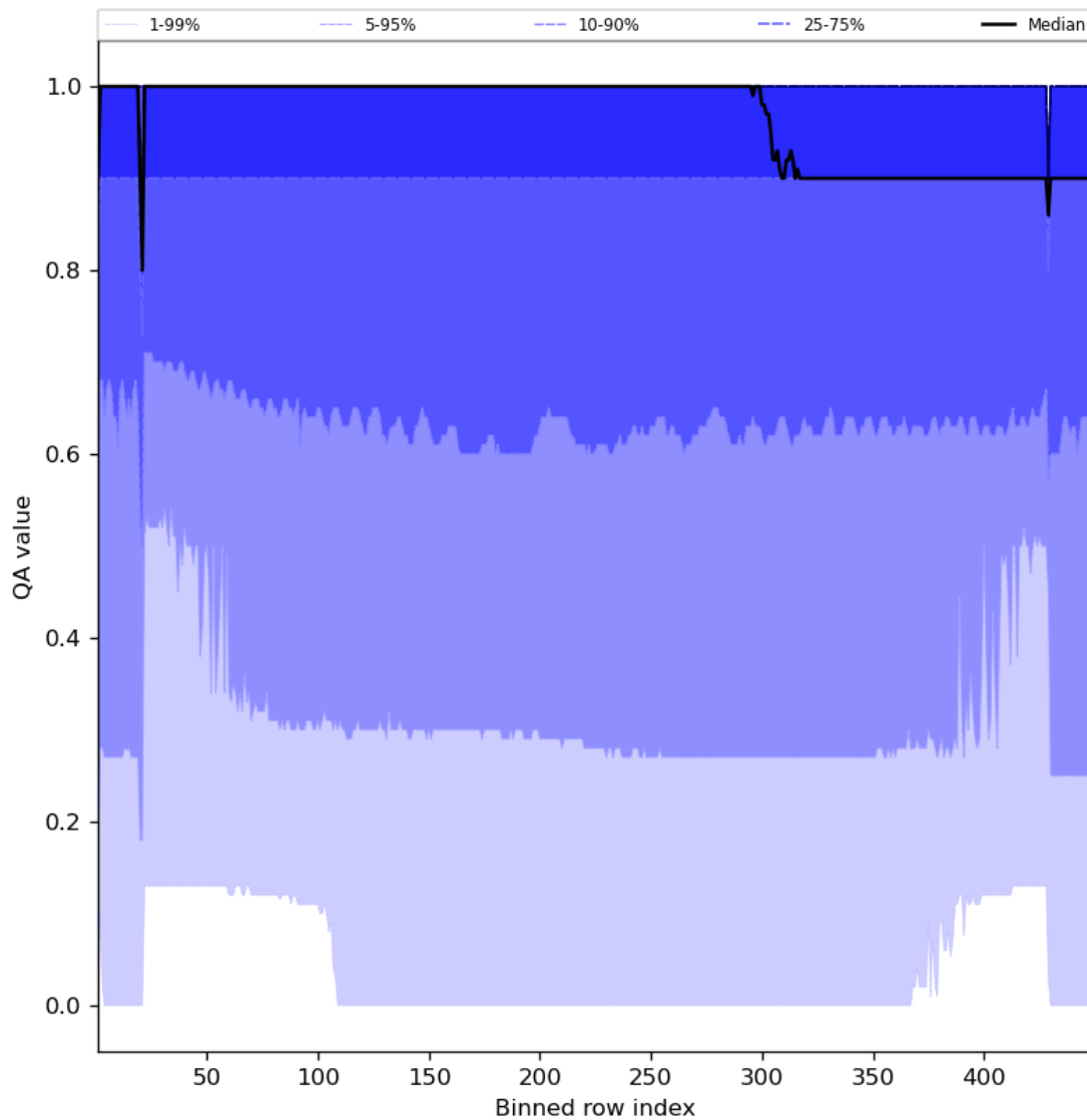
Figure 27: Along track statistics of “QA value” for 2023-07-13 to 2023-07-14
