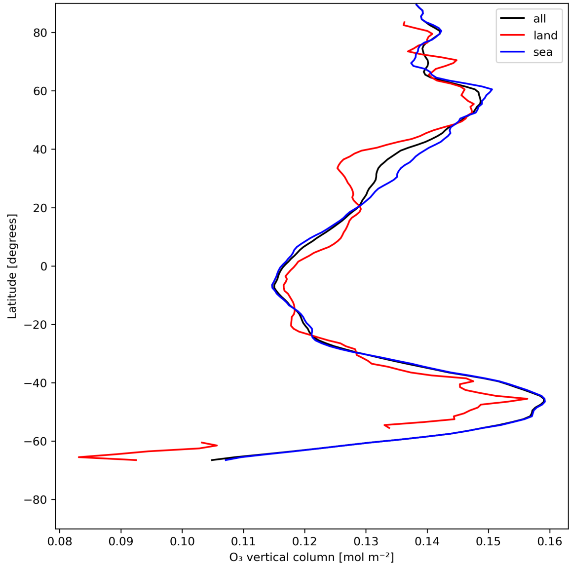
Figure 14: Zonal average of “O 3 vertical column” for 2023-07-13 to 2023-07-14.
