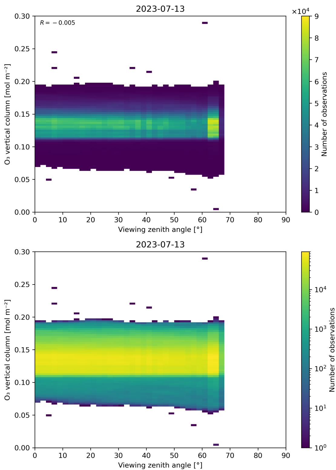
Figure 52: Scatter density plot of “Viewing zenith angle” against “O 3 vertical column” for 2023-07-13 to 2023-07-14.
