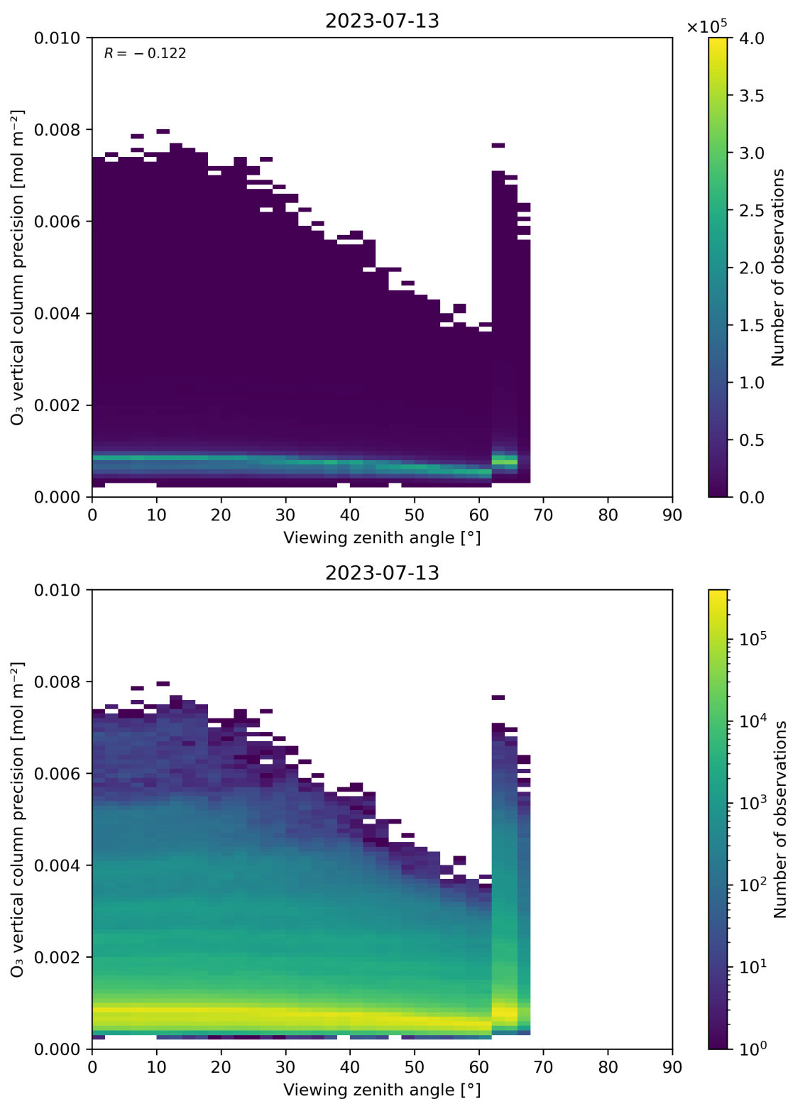
Figure 53: Scatter density plot of “Viewing zenith angle” against “O 3 vertical column precision” for 2023-07-13 to 2023-07-14.
