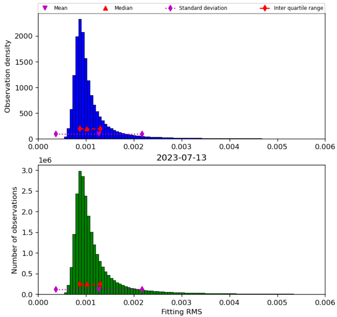
Figure 23: Histogram of “Fitting RMS” for 2023-07-13 to 2023-07-14
