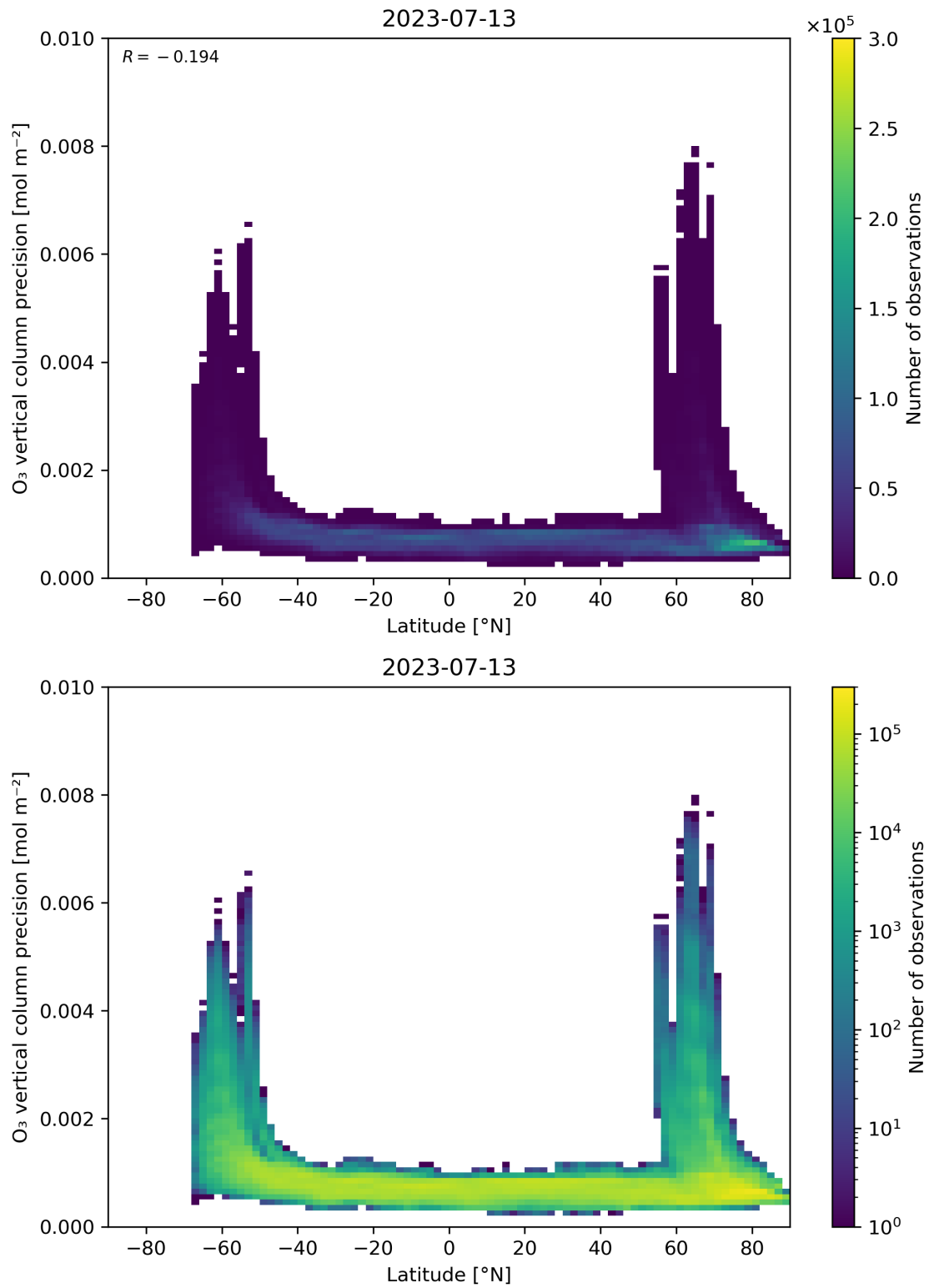
Figure 37: Scatter density plot of “Latitude” against “O 3 vertical column precision” for 2023-07-13 to 2023-07-14.
