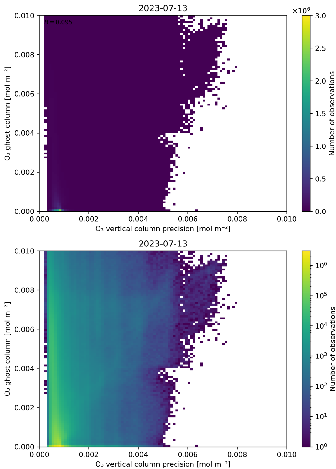
Figure 43: Scatter density plot of “ \text{O}_3 vertical column precision” against “ \text{O}_3 ghost column” for 2023-07-13 to 2023-07-14.
