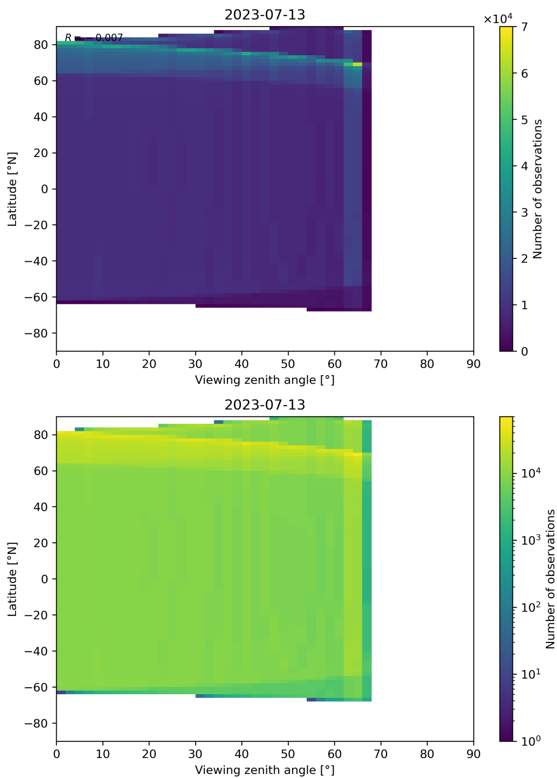
Figure 49: Scatter density plot of “Viewing zenith angle” against “Latitude” for 2023-07-13 to 2023-07-14.
