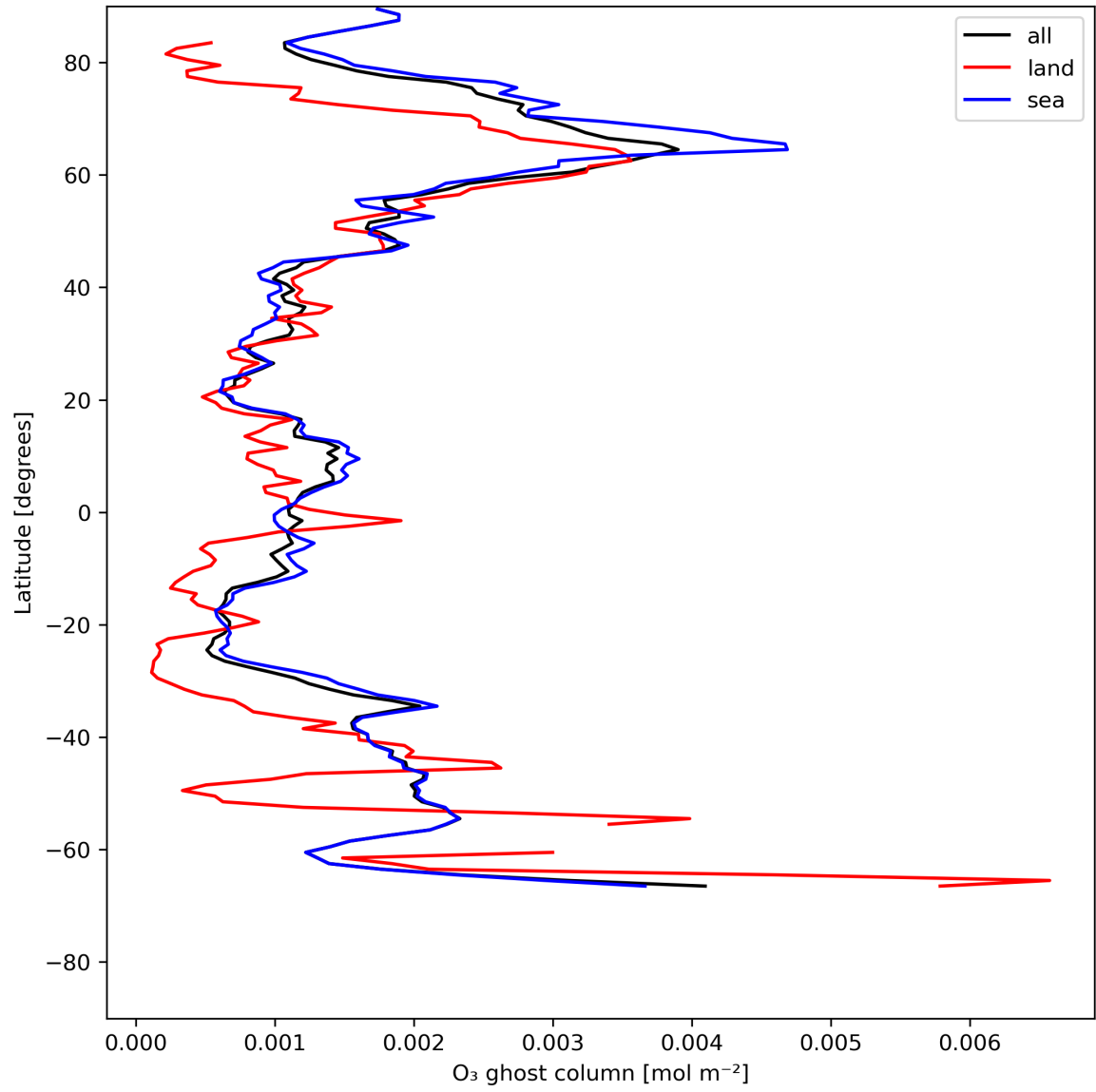
Figure 18: Zonal average of “O 3 ghost column” for 2023-07-13 to 2023-07-14.
