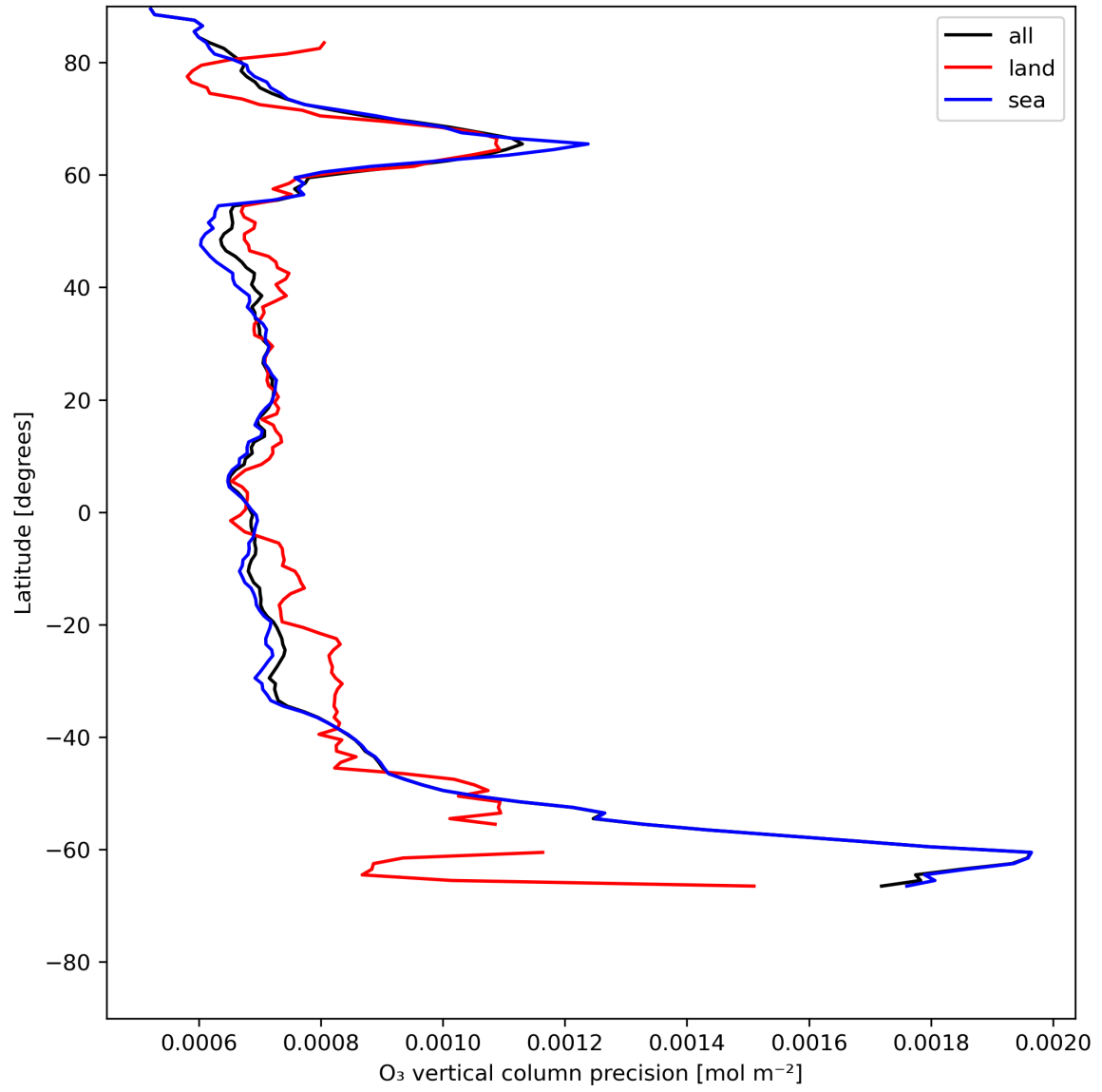
Figure 15: Zonal average of “O 3 vertical column precision” for 2023-07-13 to 2023-07-14.
