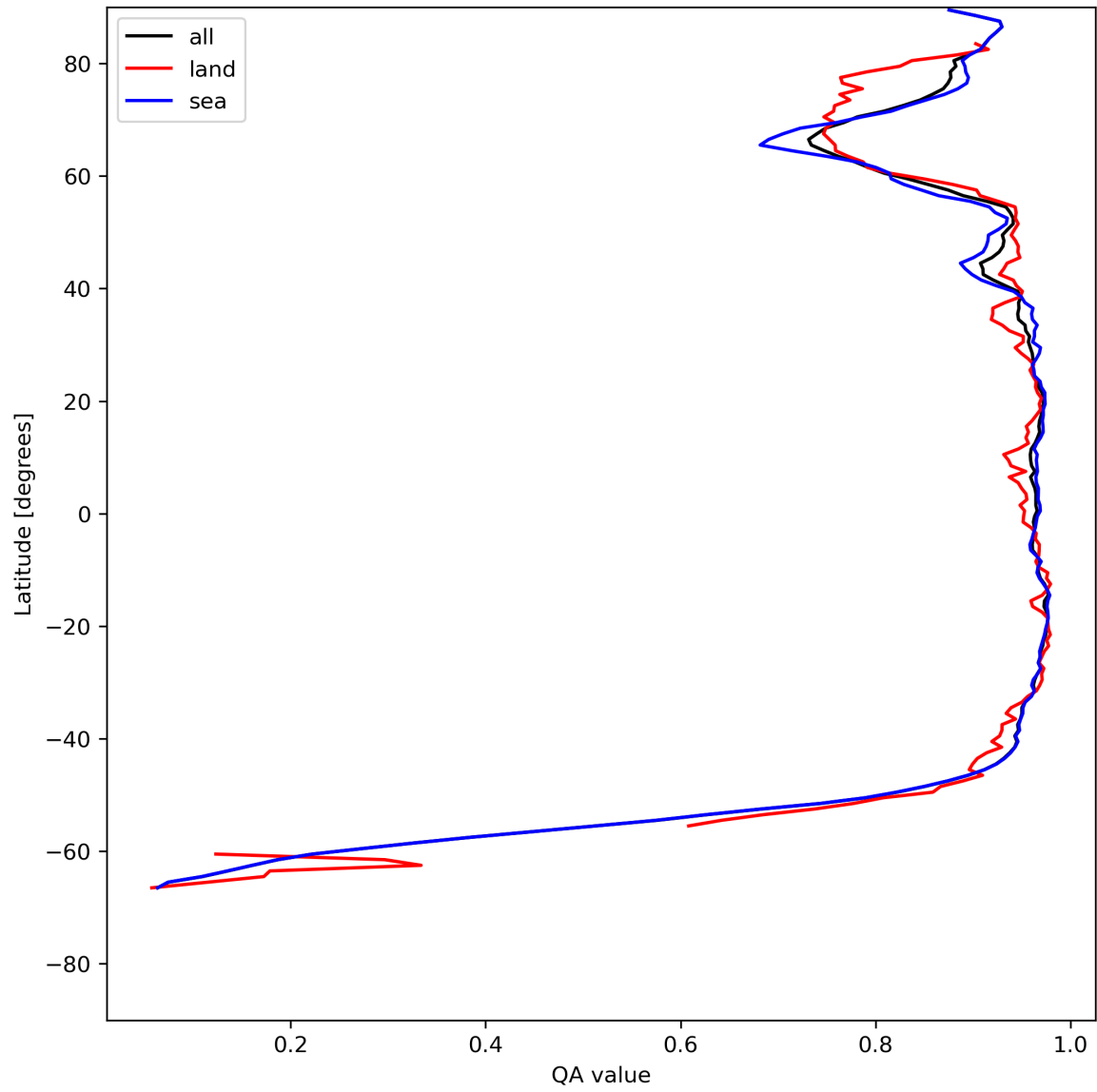
Figure 13: Zonal average of “QA value” for 2023-07-13 to 2023-07-14.
