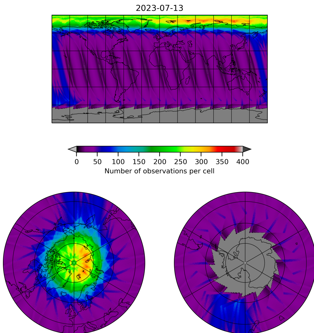
Figure 12: Map of the number of observations for 2023-07-13 to 2023-07-14
