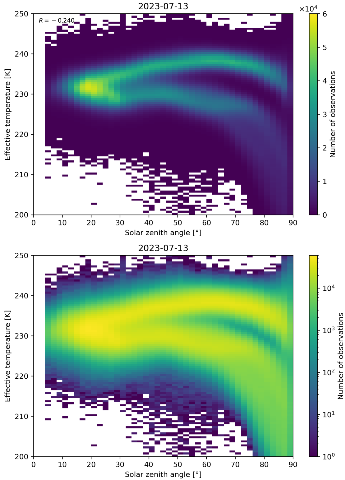
Figure 45: Scatter density plot of “Solar zenith angle” against “Effective temperature” for 2023-07-13 to 2023-07-14.
