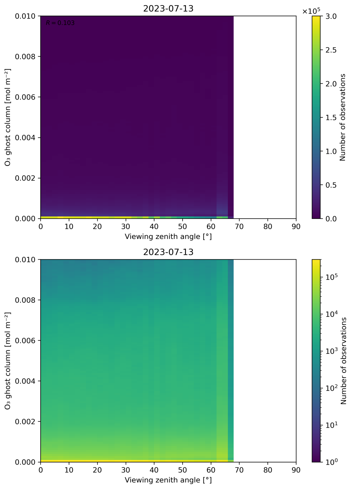
Figure 51: Scatter density plot of “Viewing zenith angle” against “O 3 ghost column” for 2023-07-13 to 2023-07-14.
