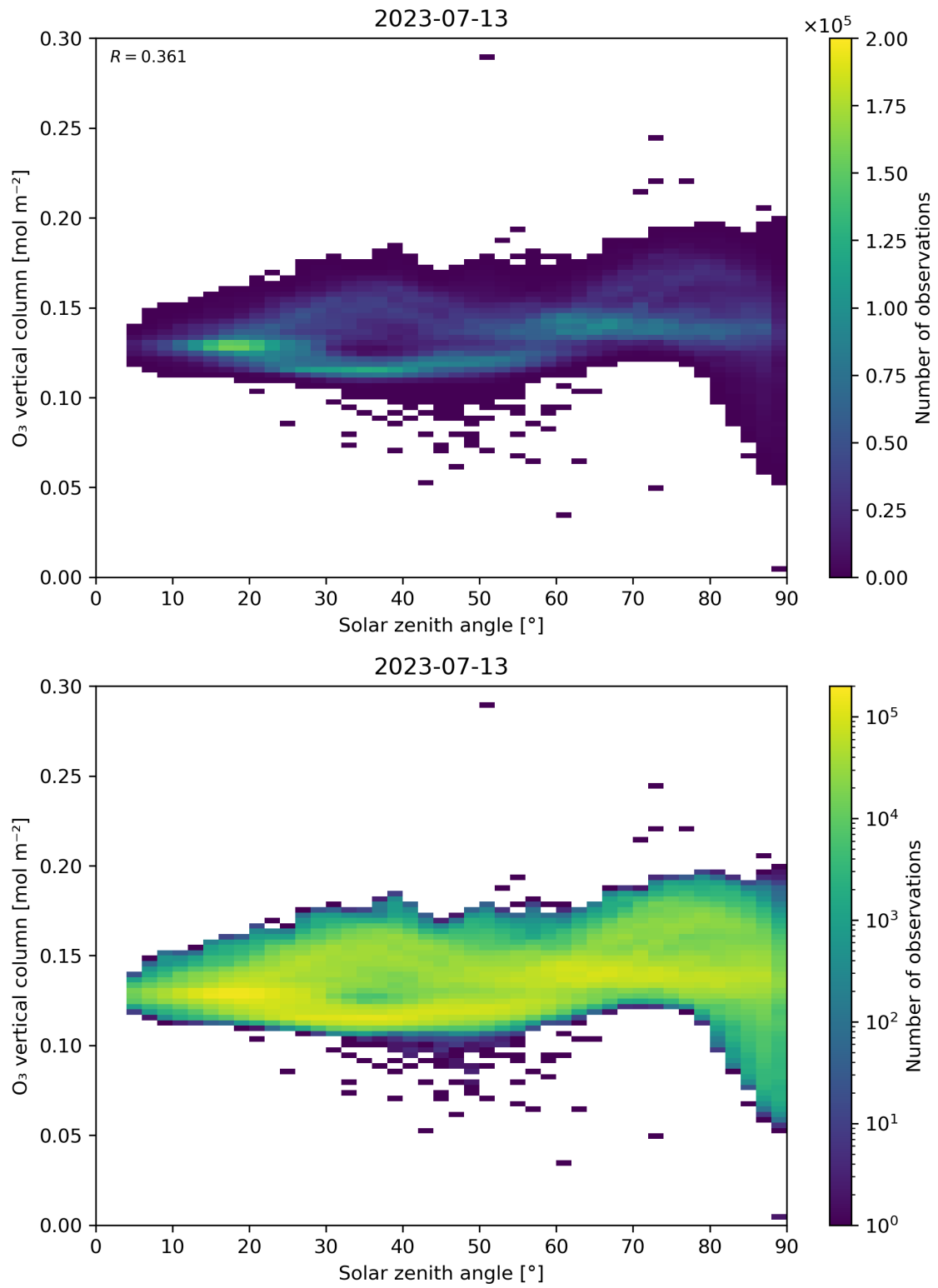
Figure 47: Scatter density plot of “Solar zenith angle” against “O 3 vertical column” for 2023-07-13 to 2023-07-14.
