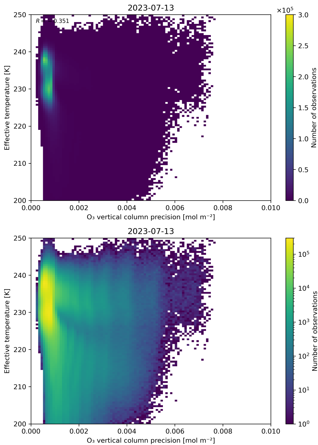
Figure 42: Scatter density plot of “O 3 vertical column precision” against “Effective temperature” for 2023-07-13 to 2023-07-14.
