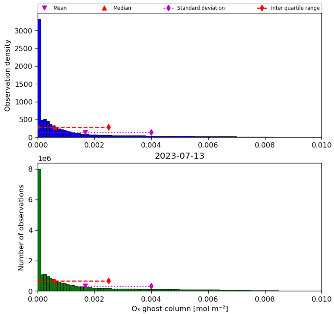
Figure 25: Histogram of "O 3 ghost column" for 2023-07-13 to 2023-07-14
