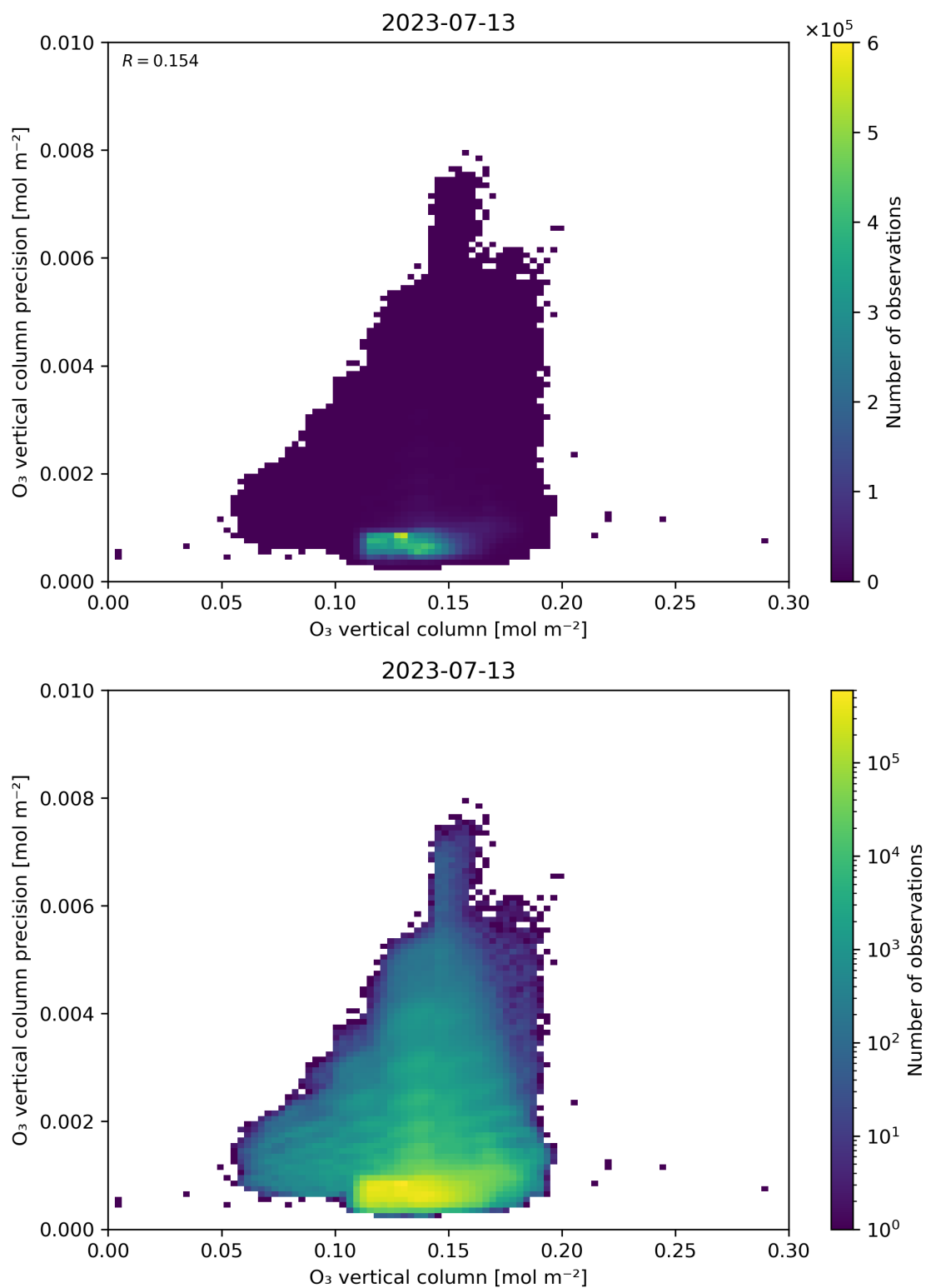
Figure 41: Scatter density plot of “O 3 vertical column” against “O 3 vertical column precision” for 2023-07-13 to 2023-07-14.
