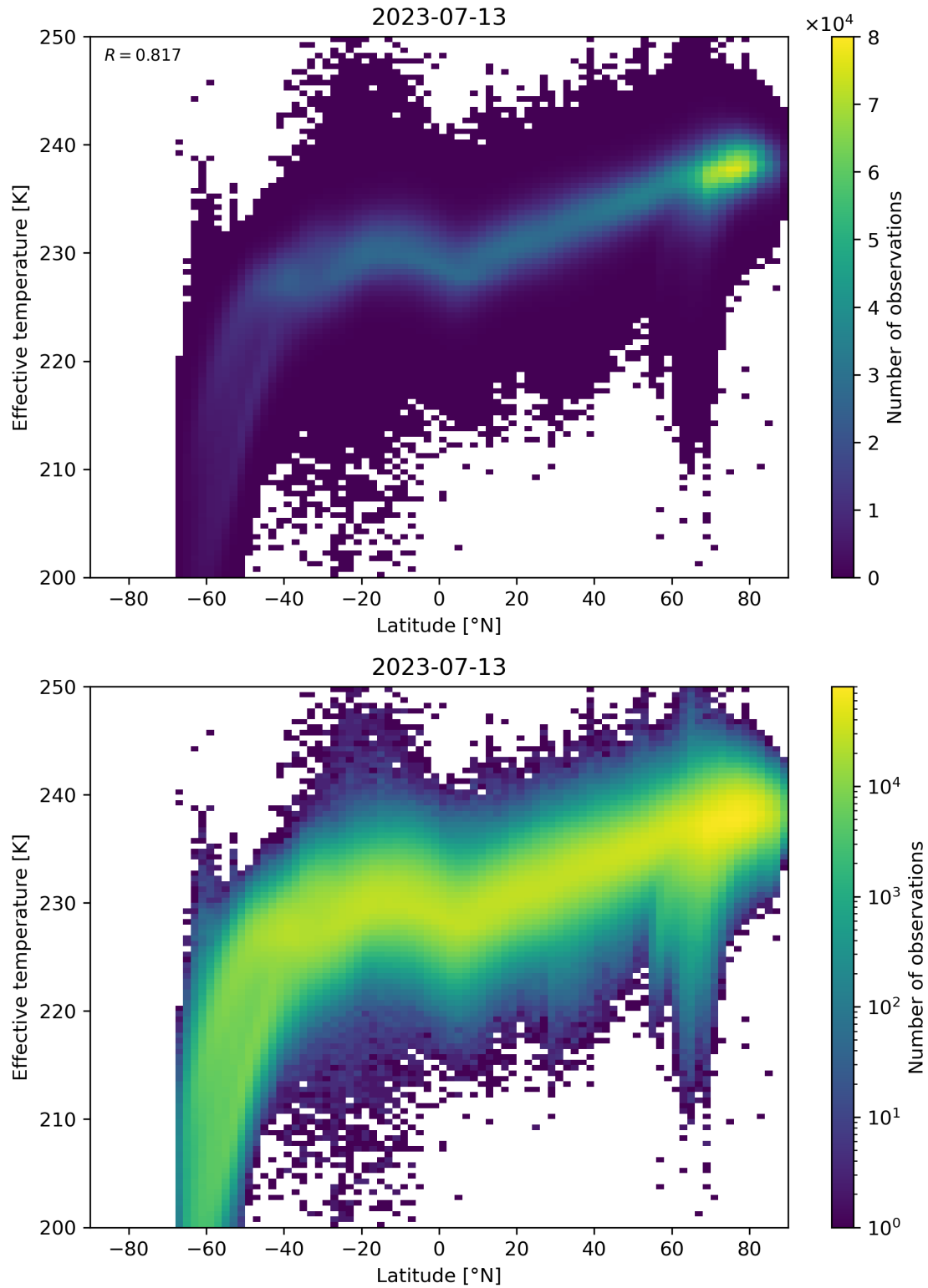
Figure 34: Scatter density plot of “Latitude” against “Effective temperature” for 2023-07-13 to 2023-07-14.
