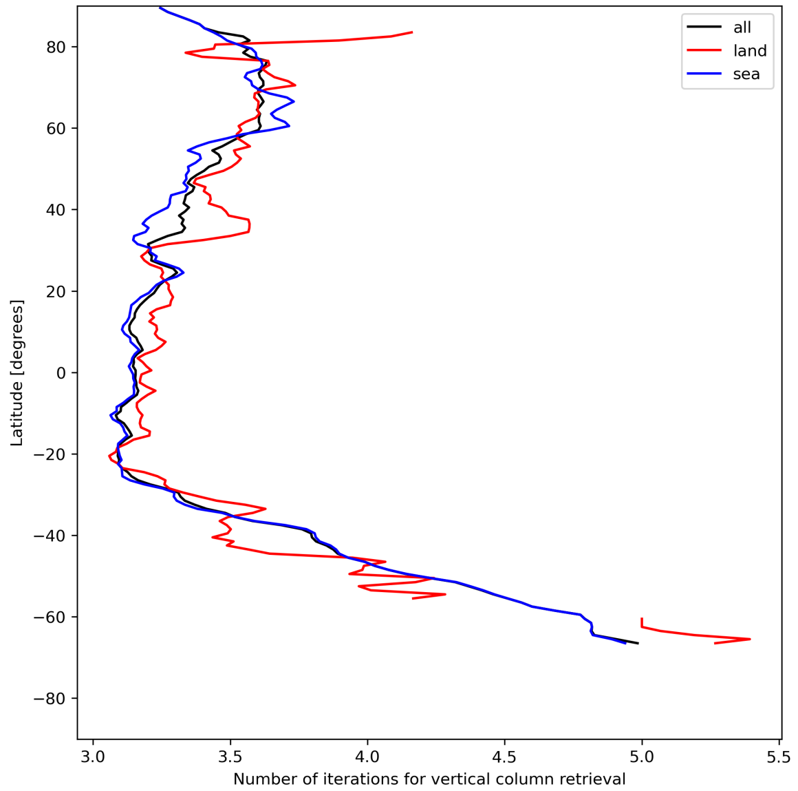
Figure 19: Zonal average of “Number of iterations for vertical column retrieval” for 2023-07-13 to 2023-07-14.
