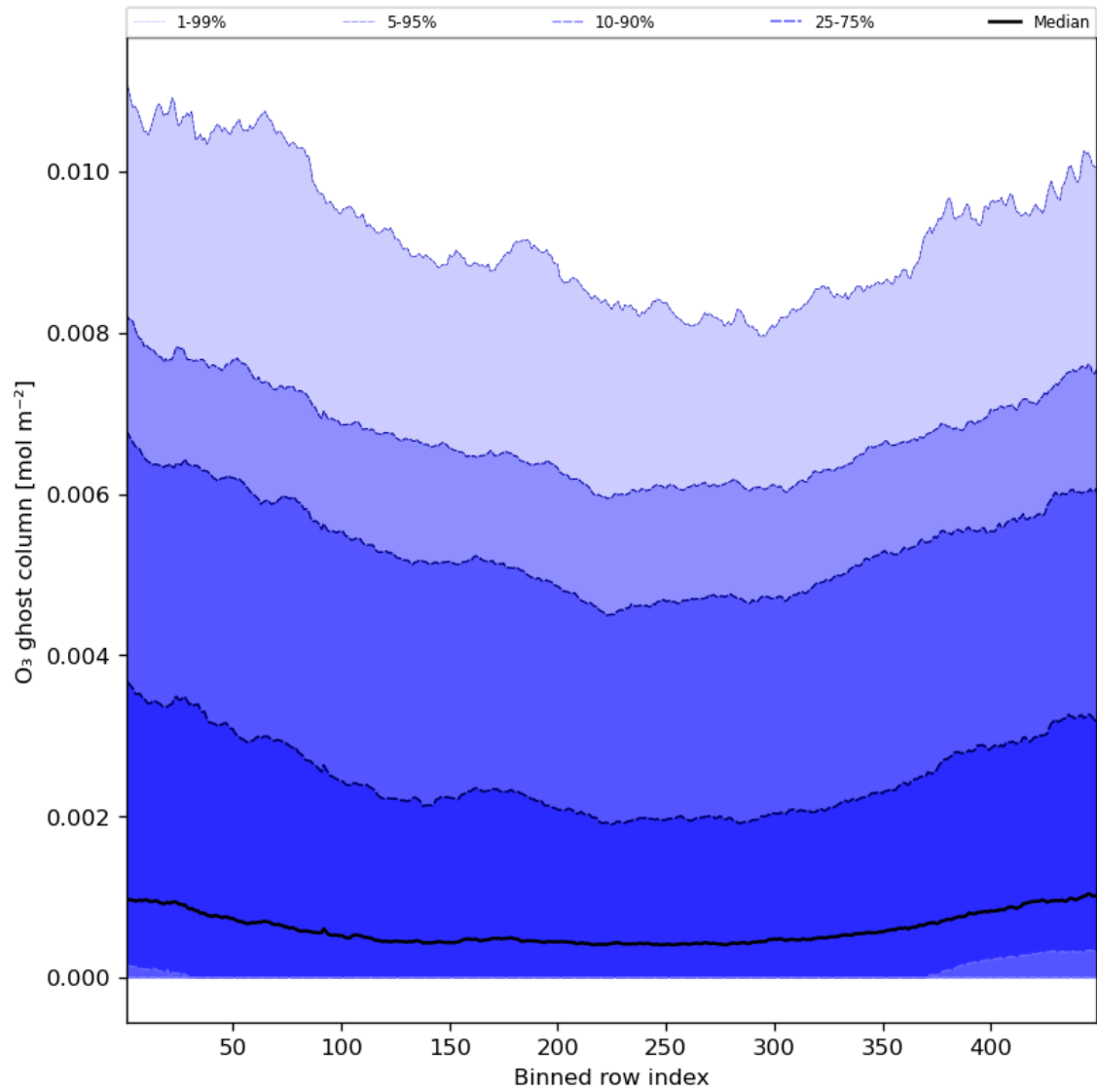
Figure 32: Along track statistics of “O 3 ghost column” for 2023-07-13 to 2023-07-14
