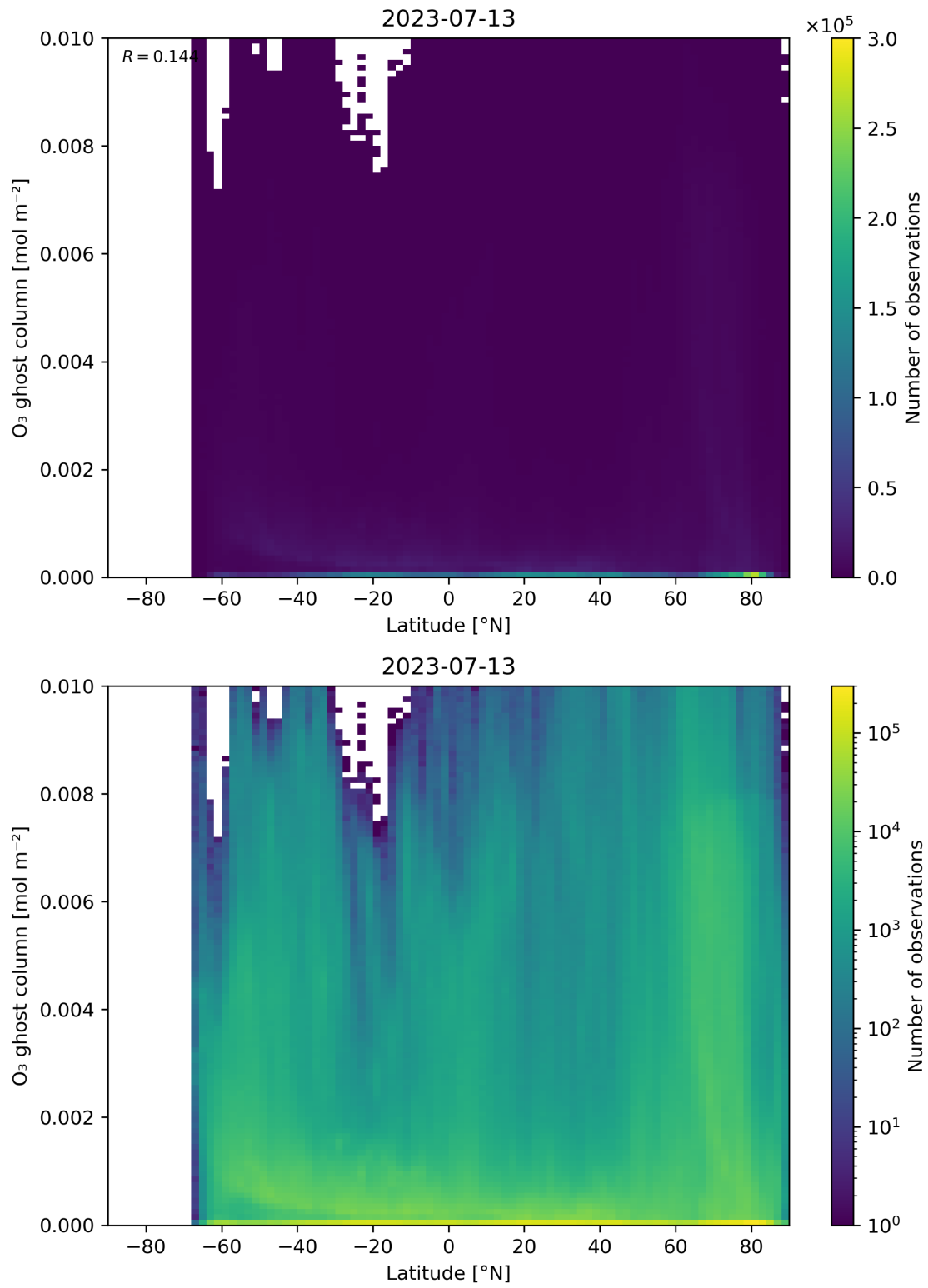
Figure 35: Scatter density plot of “Latitude” against “O 3 ghost column” for 2023-07-13 to 2023-07-14.
