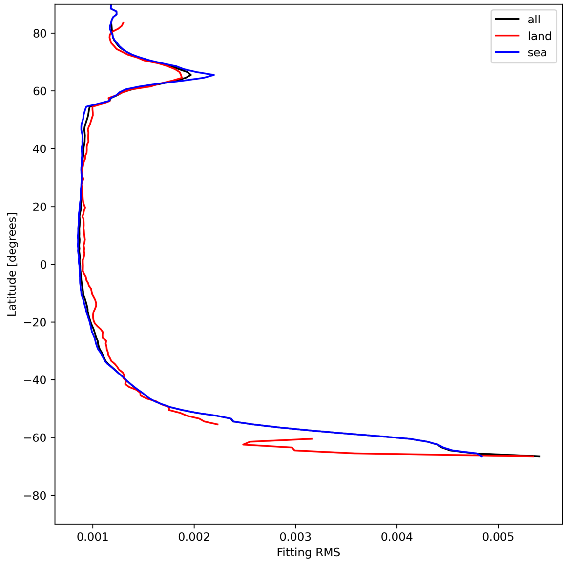
Figure 16: Zonal average of “Fitting RMS” for 2023-07-13 to 2023-07-14.
