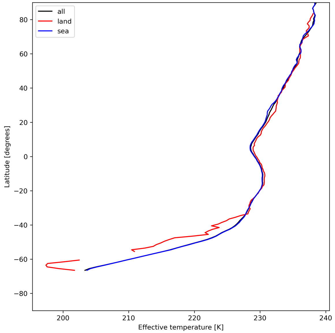
Figure 17: Zonal average of "Effective temperature" for 2023-07-13 to 2023-07-14.
