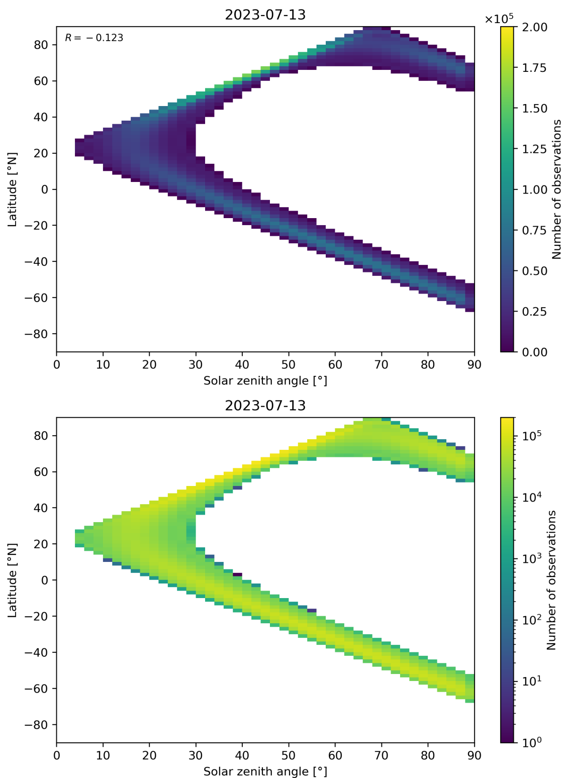
Figure 44: Scatter density plot of “Solar zenith angle” against “Latitude” for 2023-07-13 to 2023-07-14.
