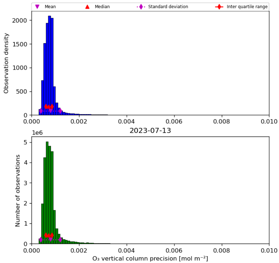
Figure 22: Histogram of “O 3 vertical column precision” for 2023-07-13 to 2023-07-14
