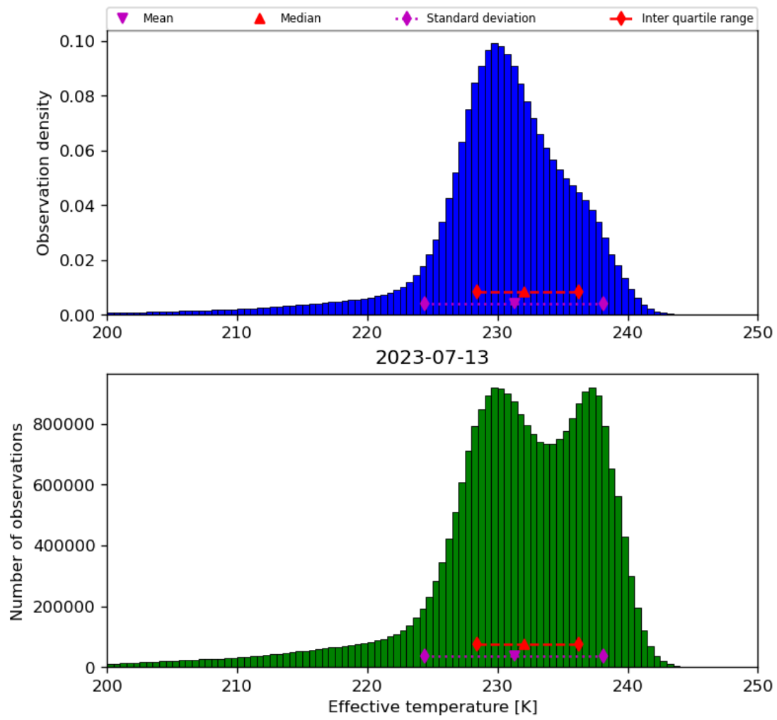
Figure 24: Histogram of “Effective temperature” for 2023-07-13 to 2023-07-14
