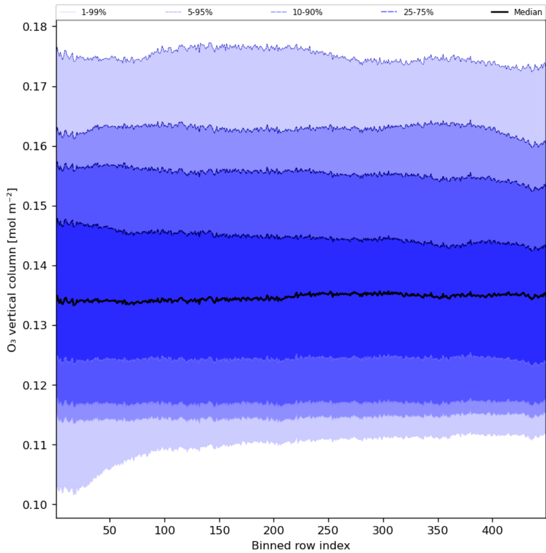
Figure 28: Along track statistics of “O 3 vertical column” for 2023-07-13 to 2023-07-14
