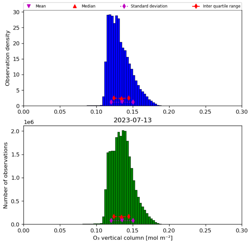
Figure 21: Histogram of “O 3 vertical column” for 2023-07-13 to 2023-07-14
