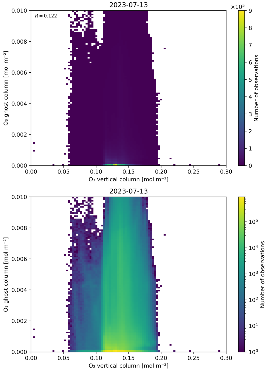
Figure 40: Scatter density plot of “O 3 vertical column” against “O 3 ghost column” for 2023-07-13 to 2023-07-14.
