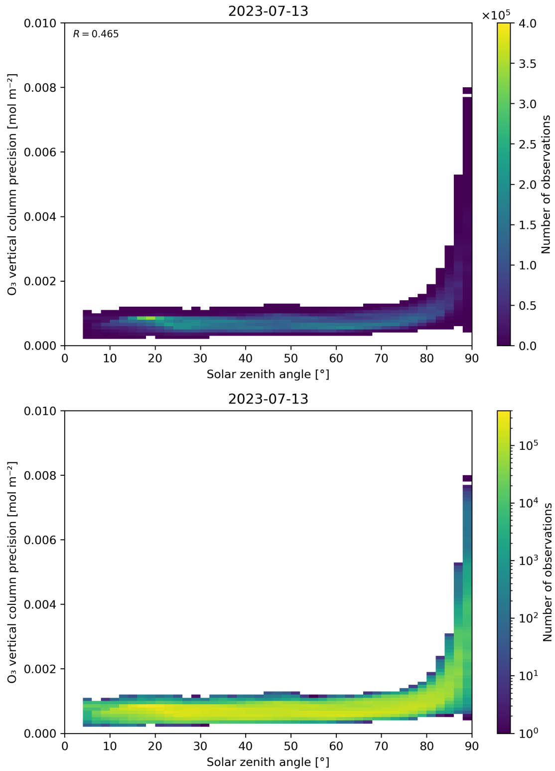
Figure 48: Scatter density plot of “Solar zenith angle” against “O 3 vertical column precision” for 2023-07-13 to 2023-07-14.
