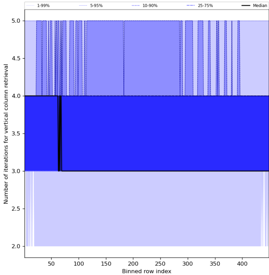
Figure 33: Along track statistics of “Number of iterations for vertical column retrieval” for 2023-07-13 to 2023-07-14
