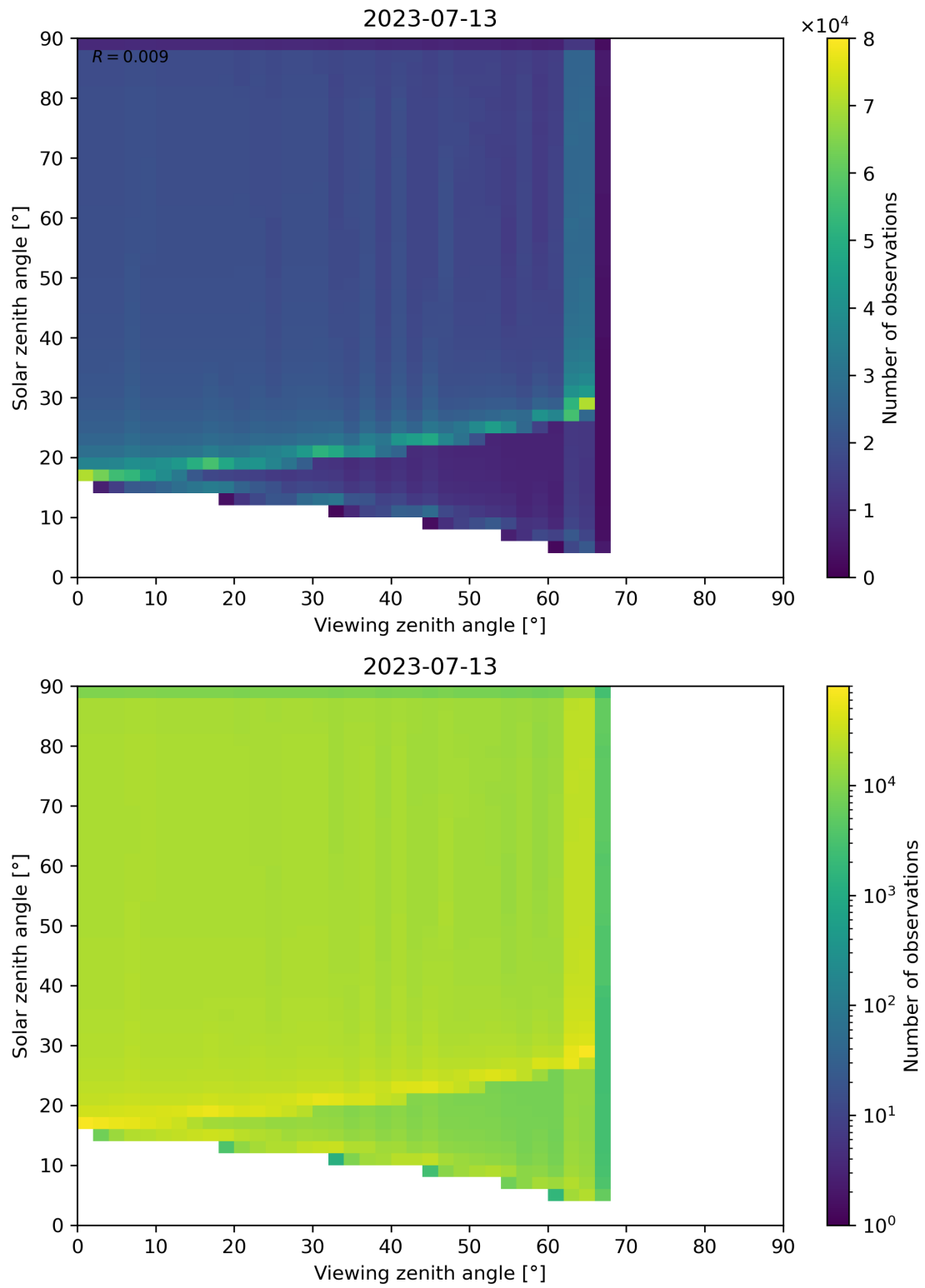
Figure 54: Scatter density plot of “Viewing zenith angle” against “Solar zenith angle” for 2023-07-13 to 2023-07-14.
