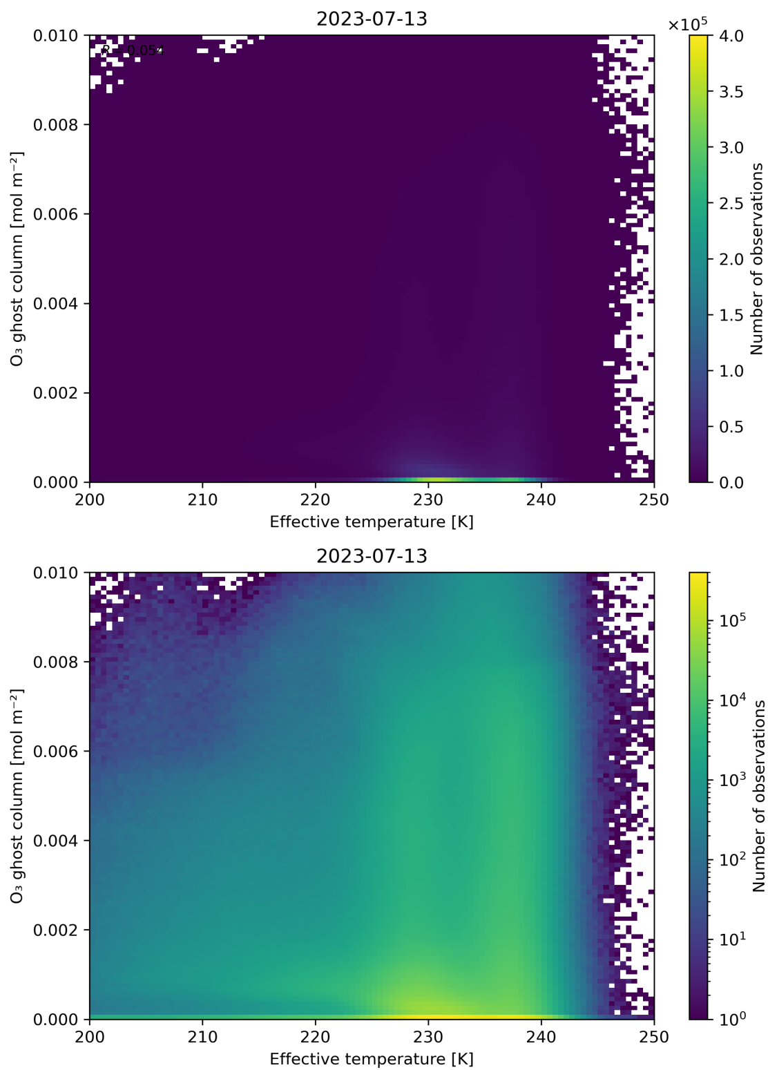
Figure 38: Scatter density plot of “Effective temperature” against “O 3 ghost column” for 2023-07-13 to 2023-07-14.
