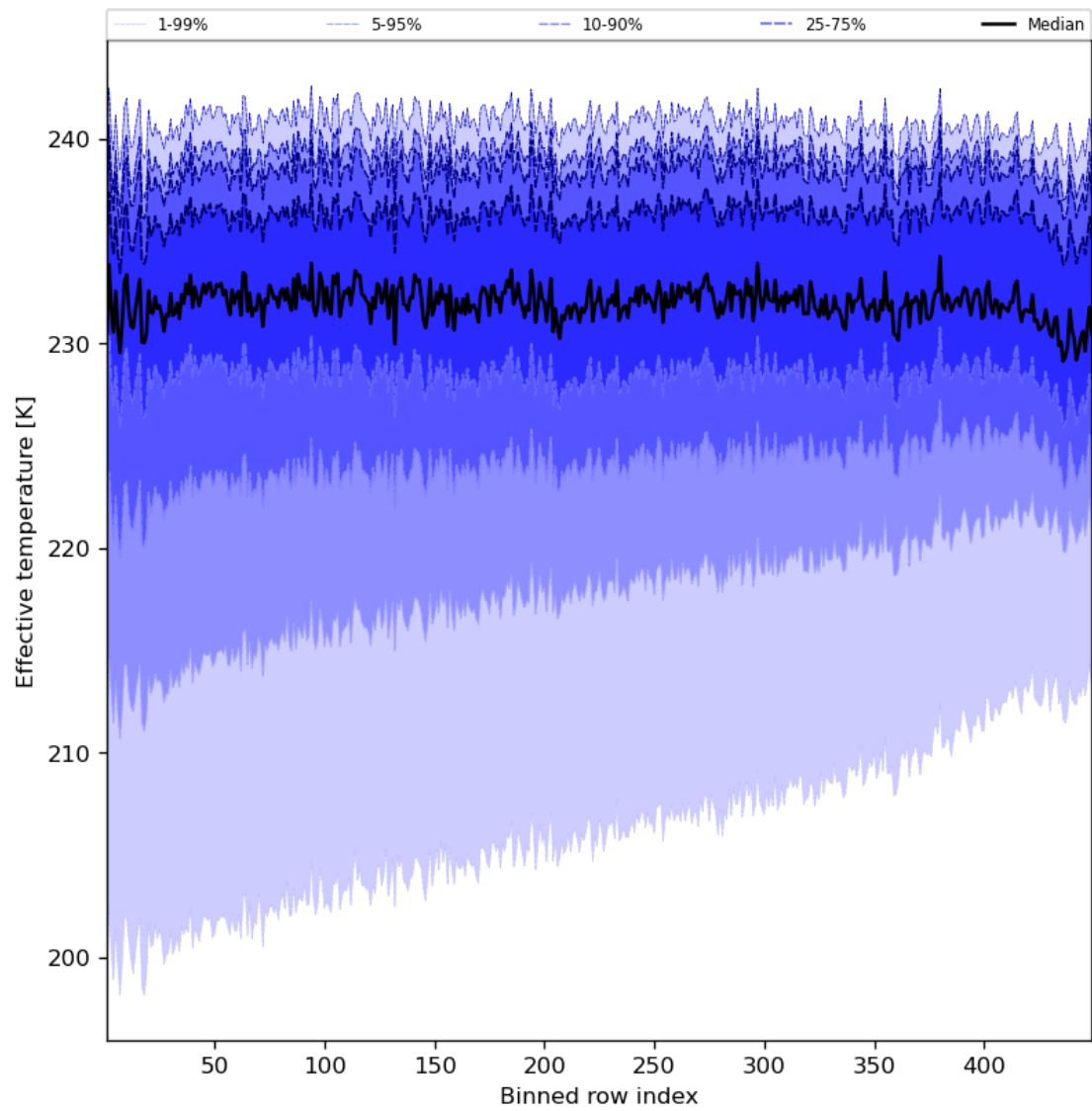
Figure 31: Along track statistics of “Effective temperature” for 2023-07-13 to 2023-07-14
