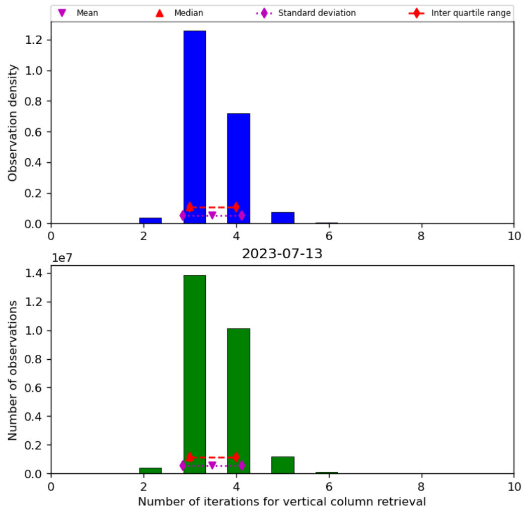
Figure 26: Histogram of “Number of iterations for vertical column retrieval” for 2023-07-13 to 2023-07-14
