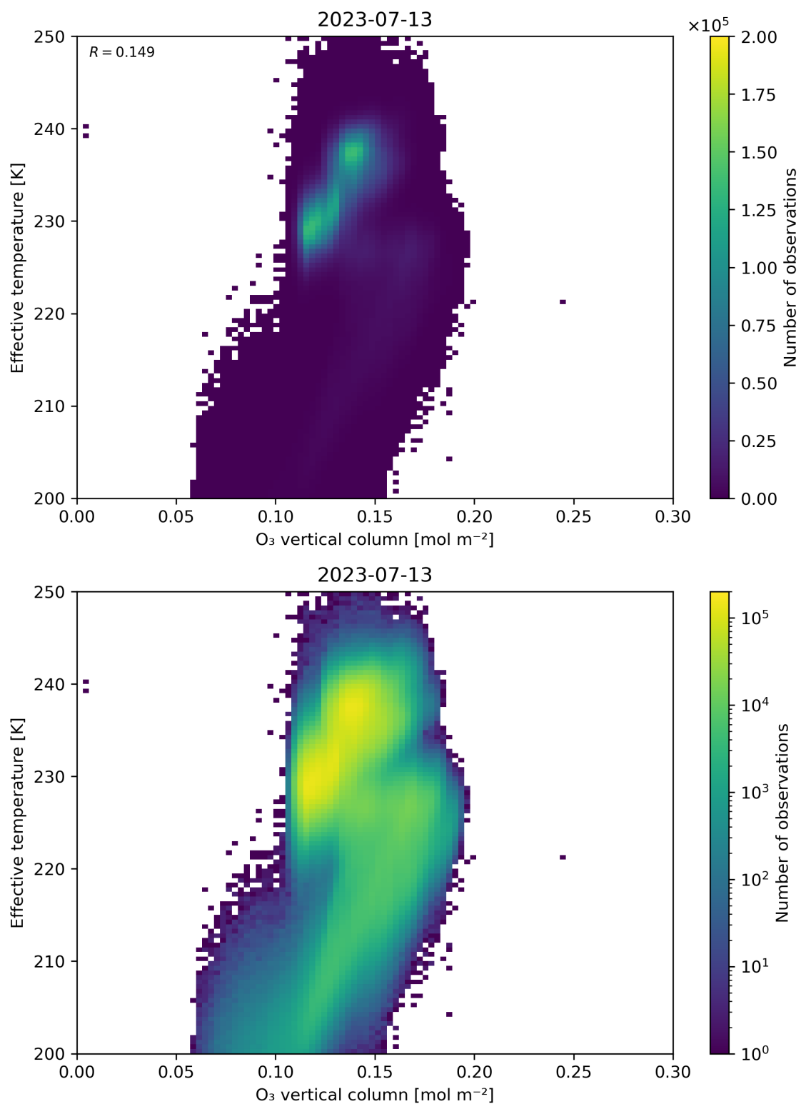
Figure 39: Scatter density plot of “O 3 vertical column” against “Effective temperature” for 2023-07-13 to 2023-07-14.
