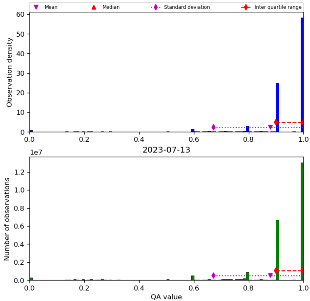
Figure 20: Histogram of “QA value” for 2023-07-13 to 2023-07-14
