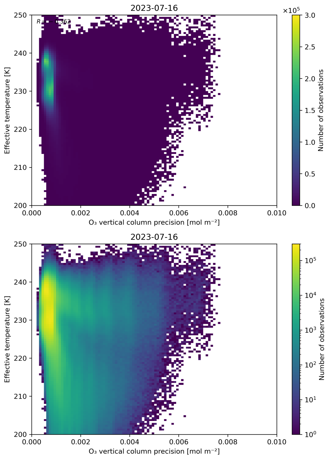
Figure 42: Scatter density plot of “O 3 vertical column precision” against “Effective temperature” for 2023-07-15 to 2023-07-17.
