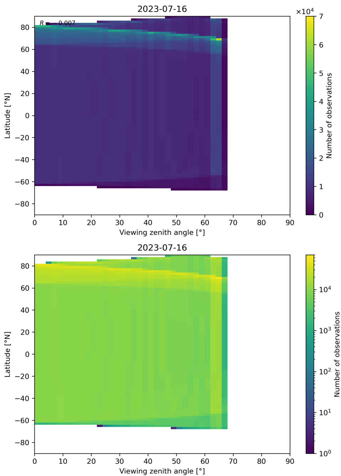
Figure 49: Scatter density plot of “Viewing zenith angle” against “Latitude” for 2023-07-15 to 2023-07-17.
