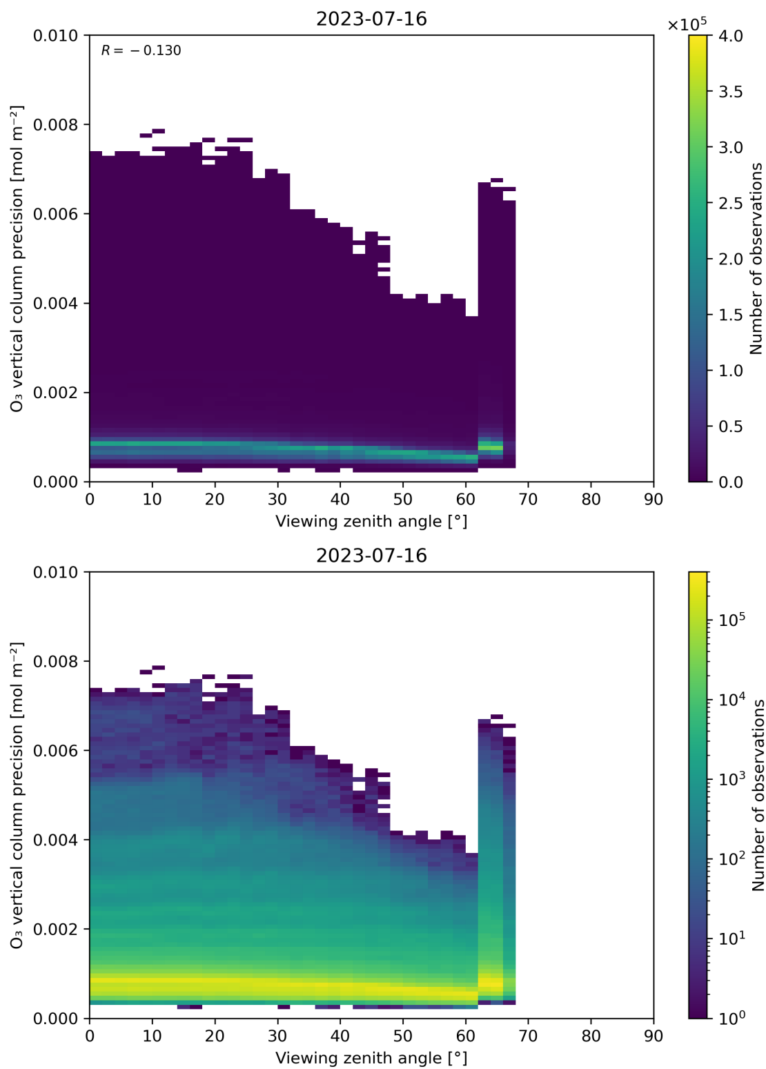
Figure 53: Scatter density plot of “Viewing zenith angle” against “O 3 vertical column precision” for 2023-07-15 to 2023-07-17.
