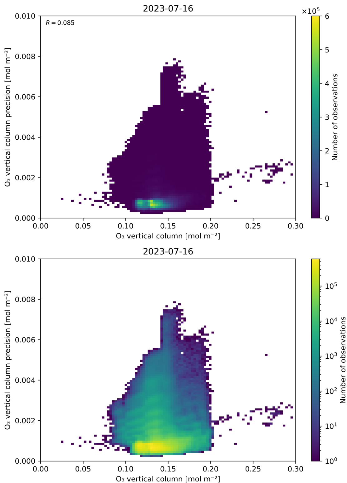
Figure 41: Scatter density plot of “O 3 vertical column” against “O 3 vertical column precision” for 2023-07-15 to 2023-07-17.
