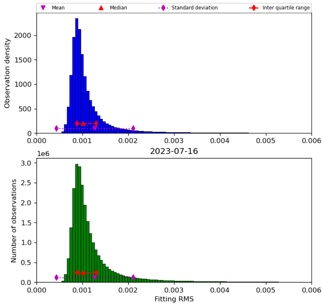
Figure 23: Histogram of “Fitting RMS” for 2023-07-15 to 2023-07-17
