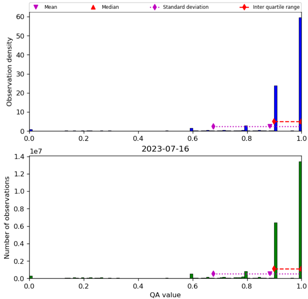
Figure 20: Histogram of “QA value” for 2023-07-15 to 2023-07-17
