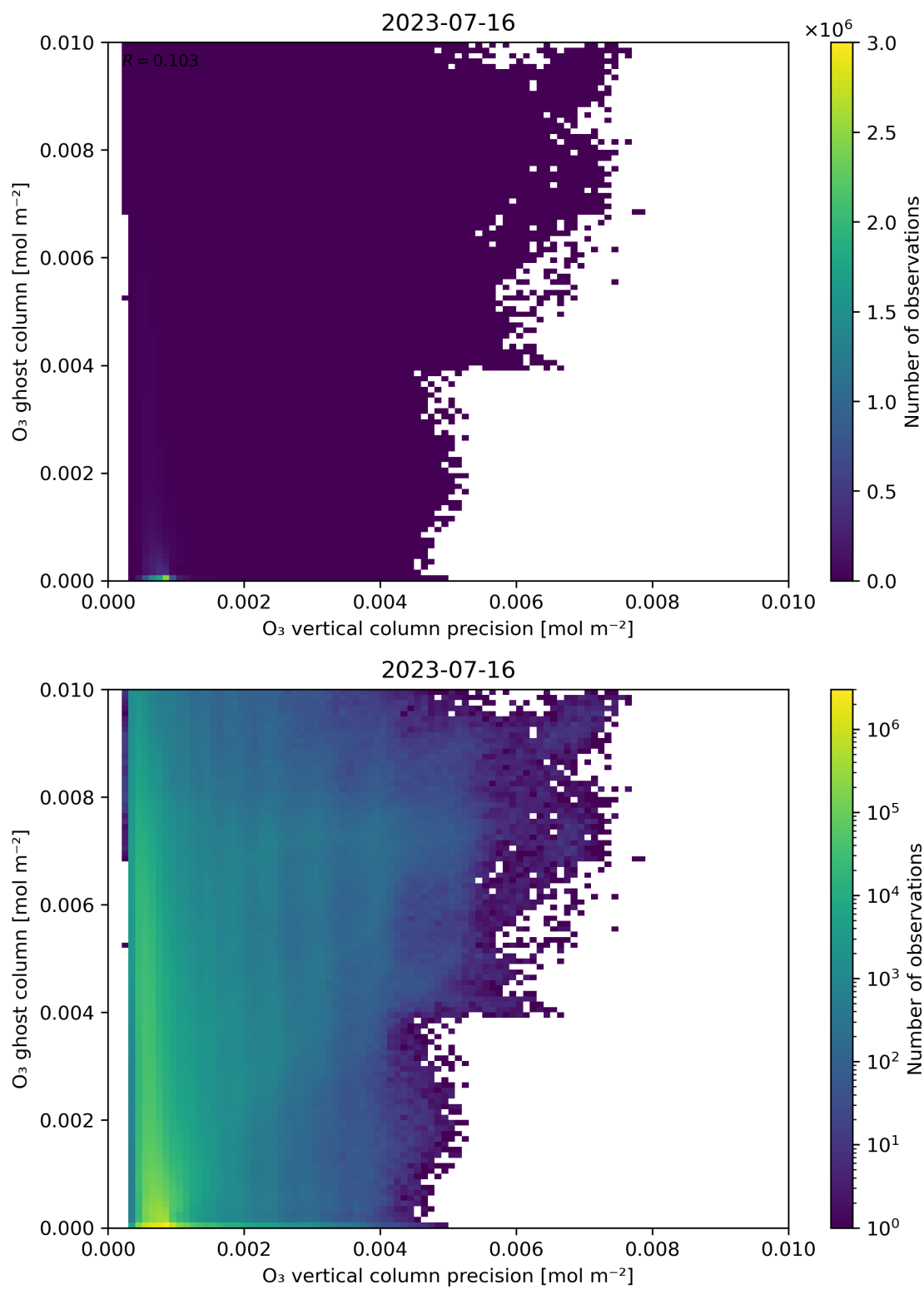
Figure 43: Scatter density plot of “ \text{O}_3 vertical column precision” against “ \text{O}_3 ghost column” for 2023-07-15 to 2023-07-17.
