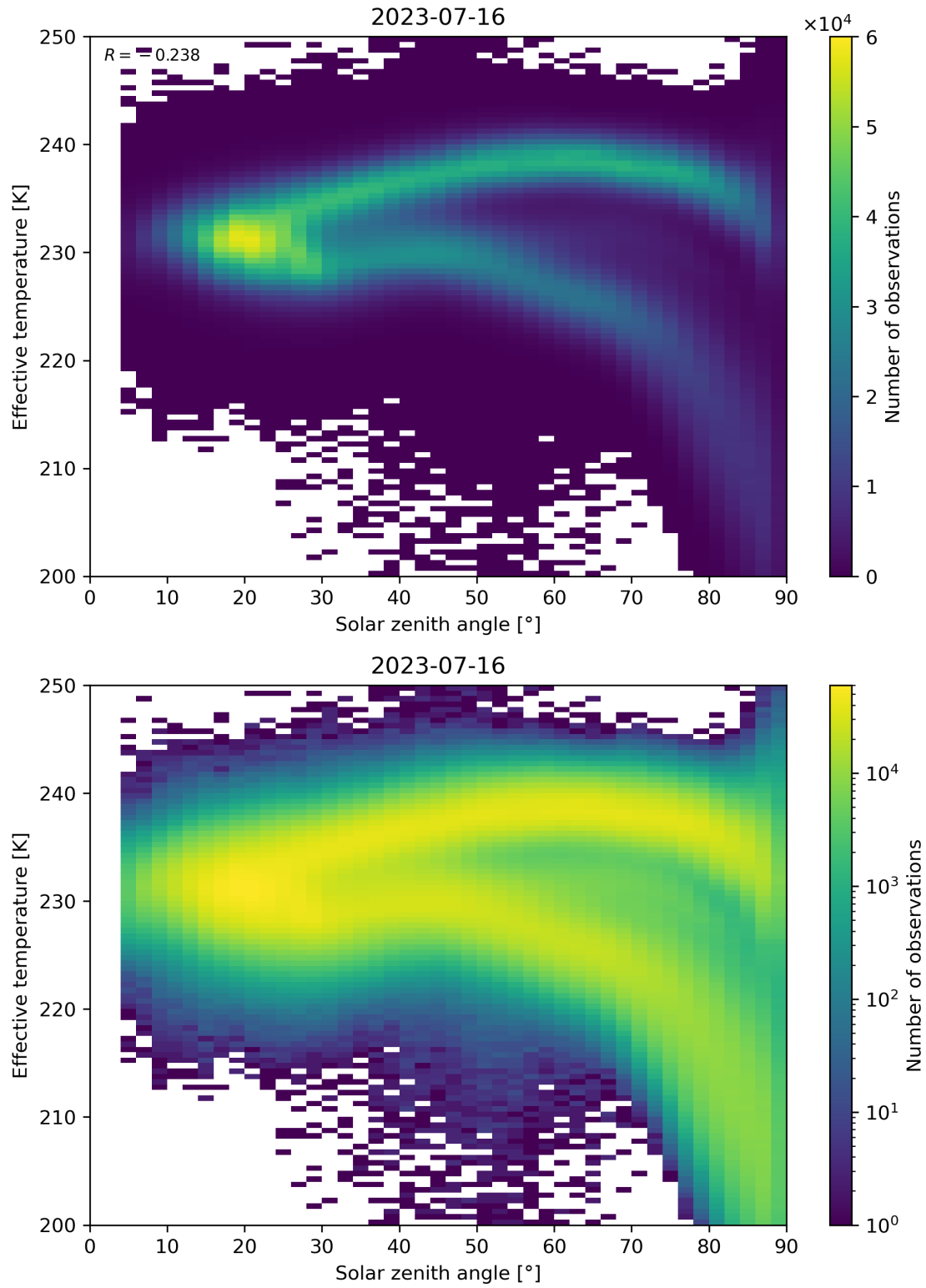
Figure 45: Scatter density plot of “Solar zenith angle” against “Effective temperature” for 2023-07-15 to 2023-07-17.
