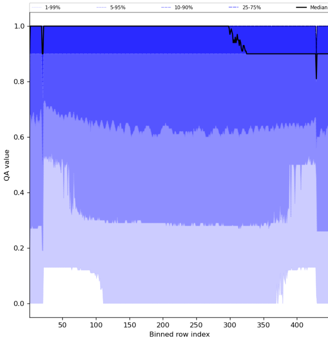
Figure 27: Along track statistics of “QA value” for 2023-07-15 to 2023-07-17
