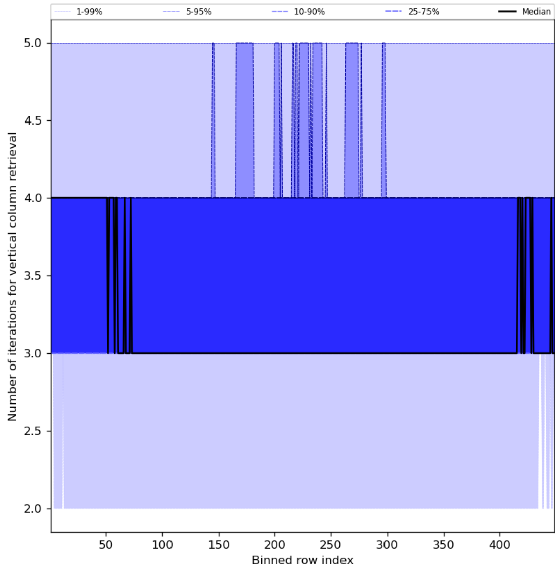
Figure 33: Along track statistics of “Number of iterations for vertical column retrieval” for 2023-07-15 to 2023-07-17
