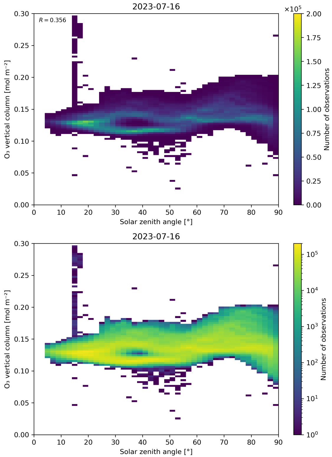
Figure 47: Scatter density plot of “Solar zenith angle” against “O 3 vertical column” for 2023-07-15 to 2023-07-17.
