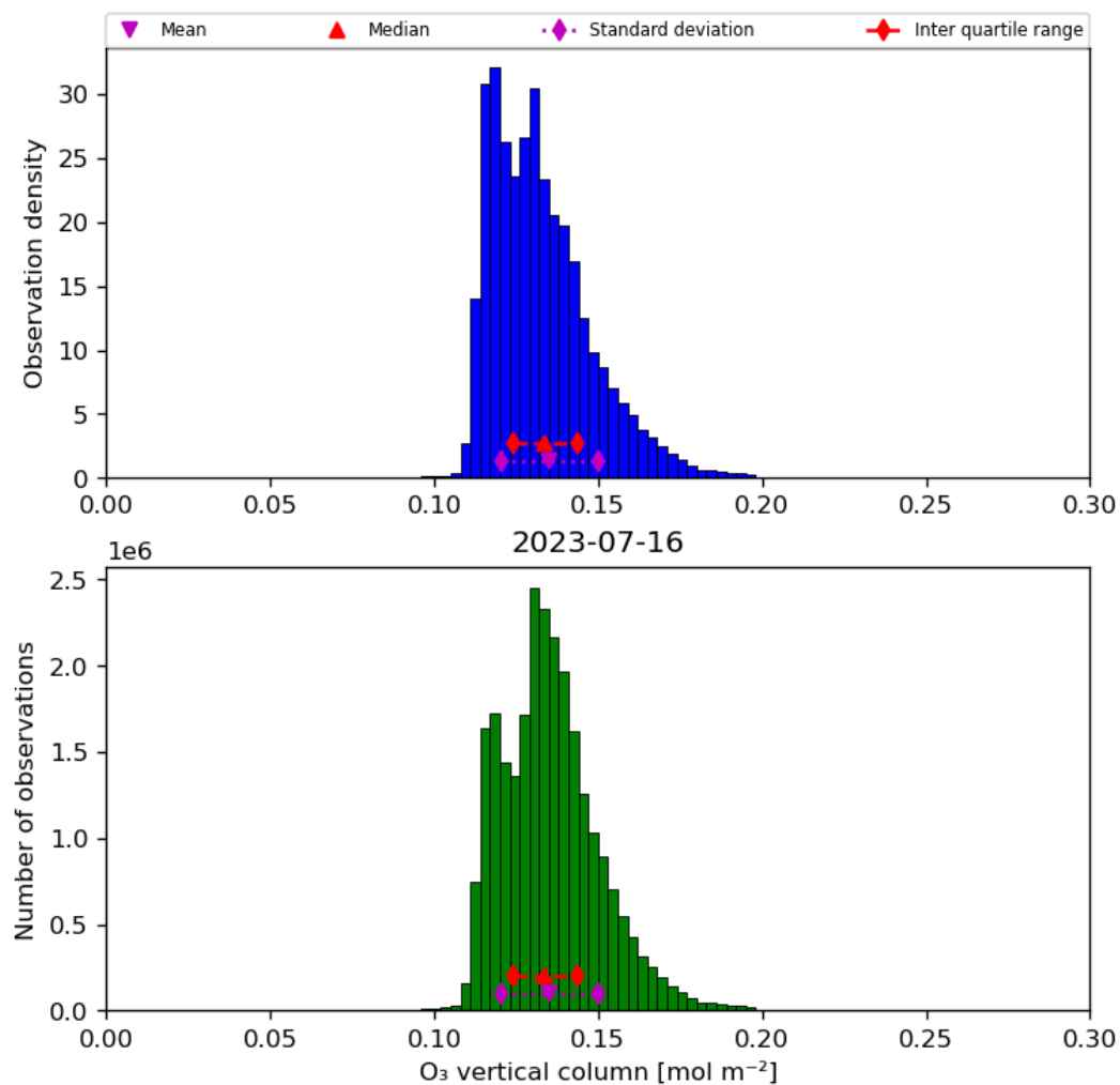
Figure 21: Histogram of “O 3 vertical column” for 2023-07-15 to 2023-07-17
