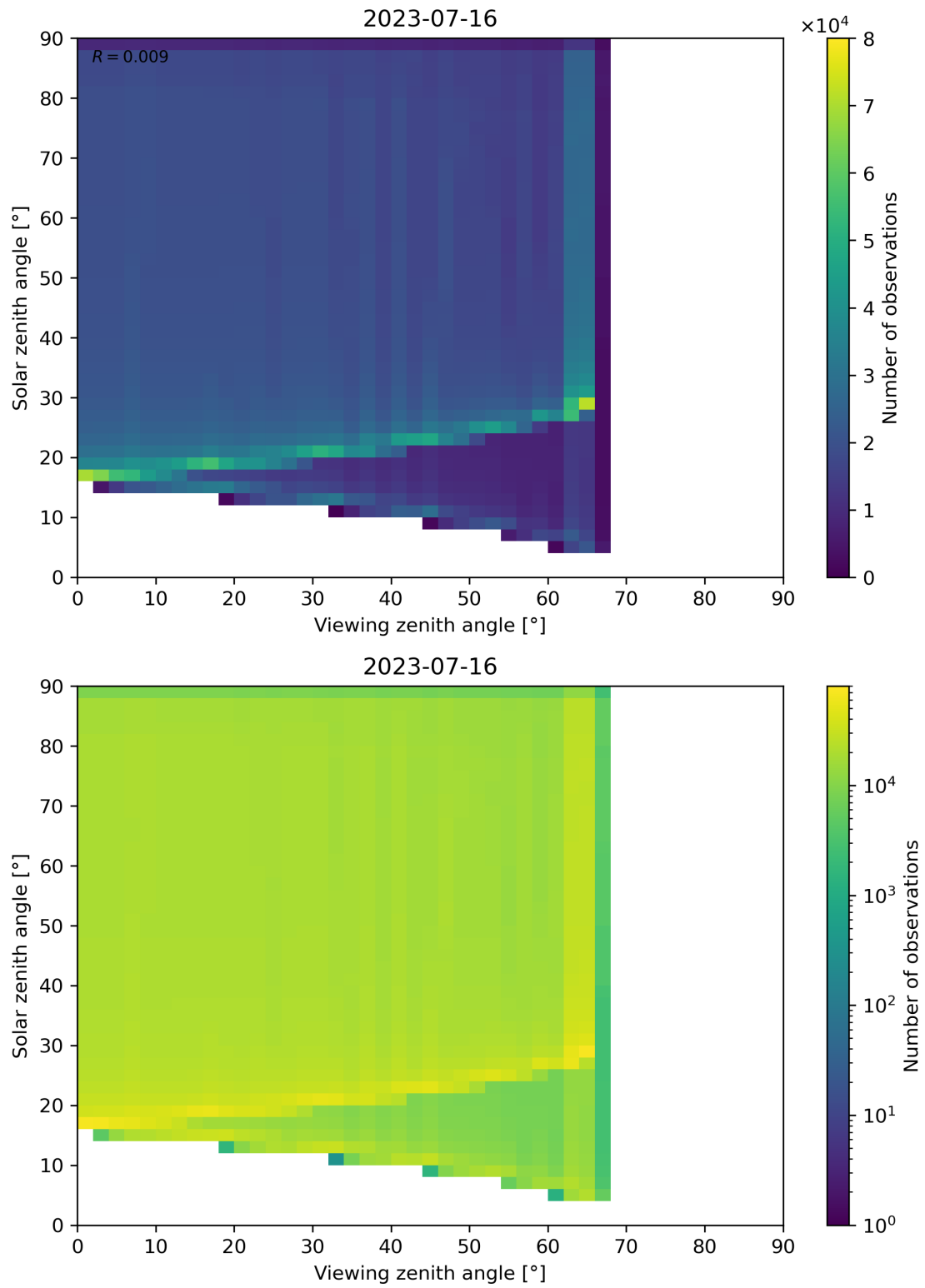
Figure 54: Scatter density plot of “Viewing zenith angle” against “Solar zenith angle” for 2023-07-15 to 2023-07-17.
