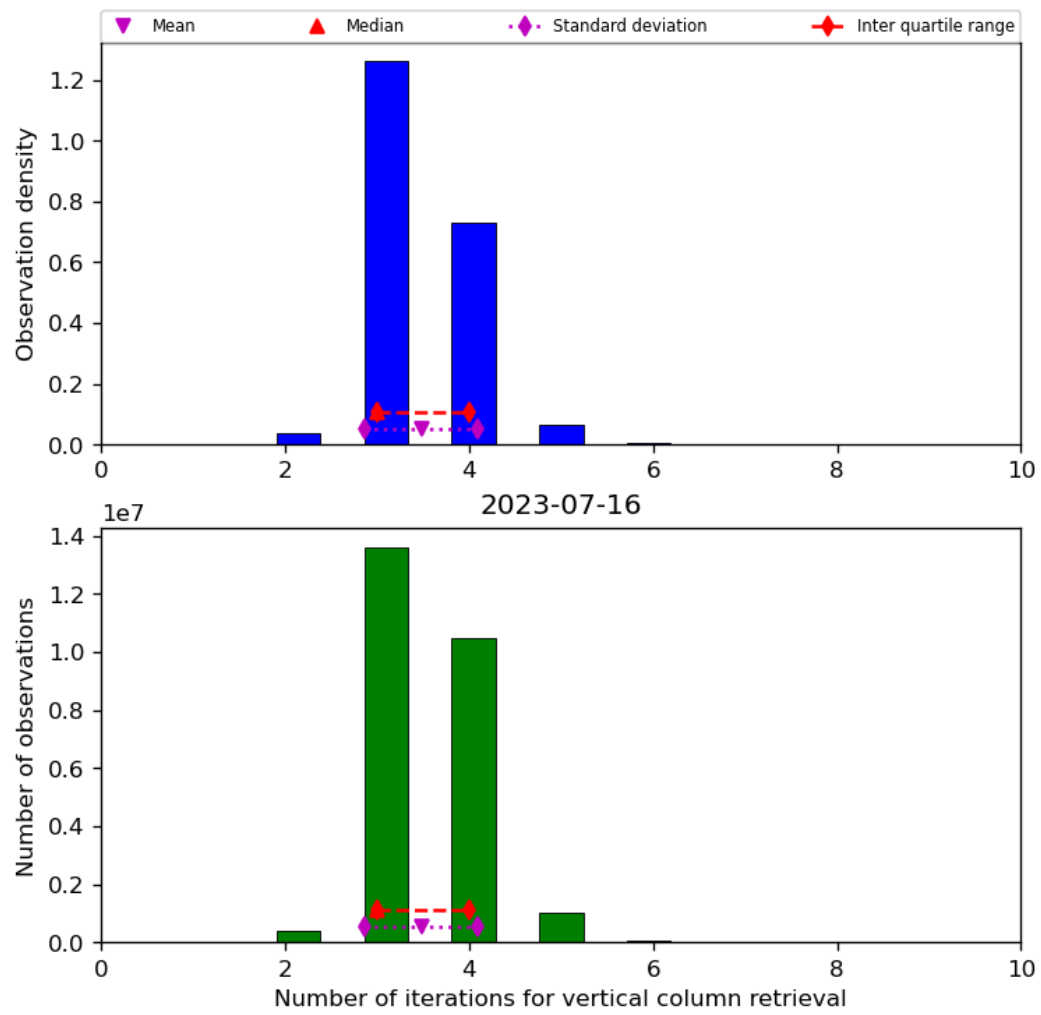
Figure 26: Histogram of “Number of iterations for vertical column retrieval” for 2023-07-15 to 2023-07-17
