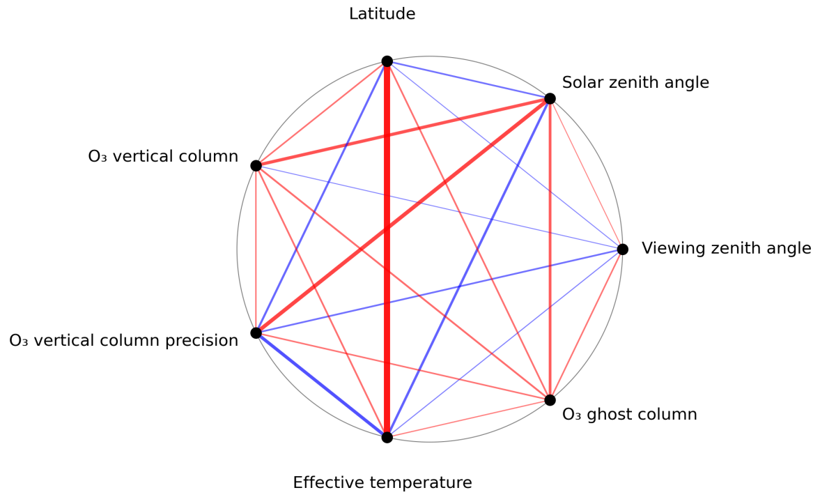
Figure 1: Map of correlation graph for 2023-07-15 to 2023-07-17.
