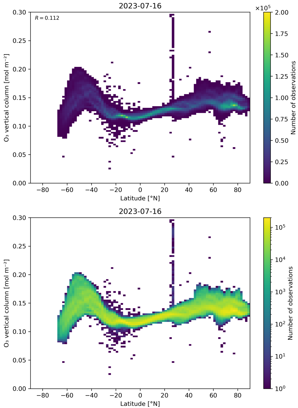
Figure 36: Scatter density plot of “Latitude” against “O 3 vertical column” for 2023-07-15 to 2023-07-17.
