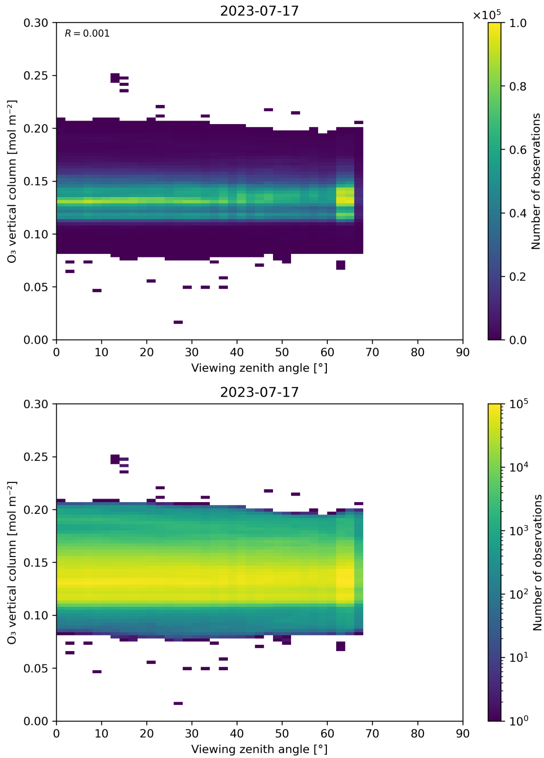
Figure 52: Scatter density plot of “Viewing zenith angle” against “O 3 vertical column” for 2023-07-16 to 2023-07-18.
