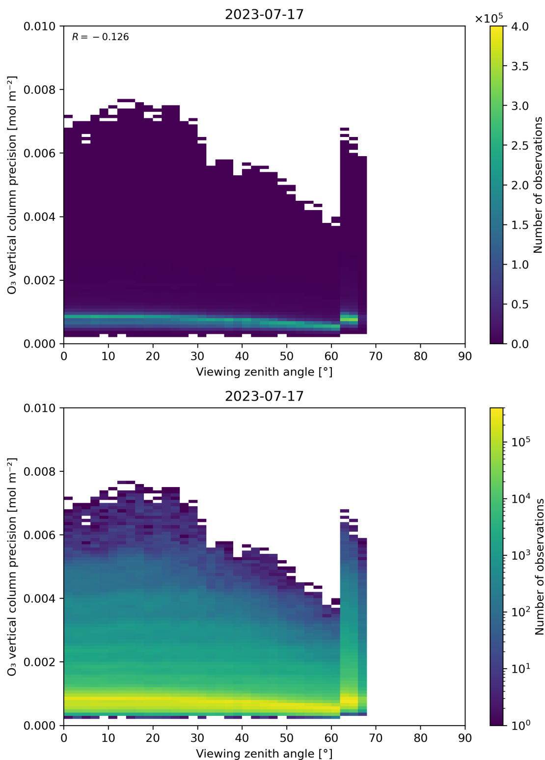
Figure 53: Scatter density plot of “Viewing zenith angle” against “O 3 vertical column precision” for 2023-07-16 to 2023-07-18.
