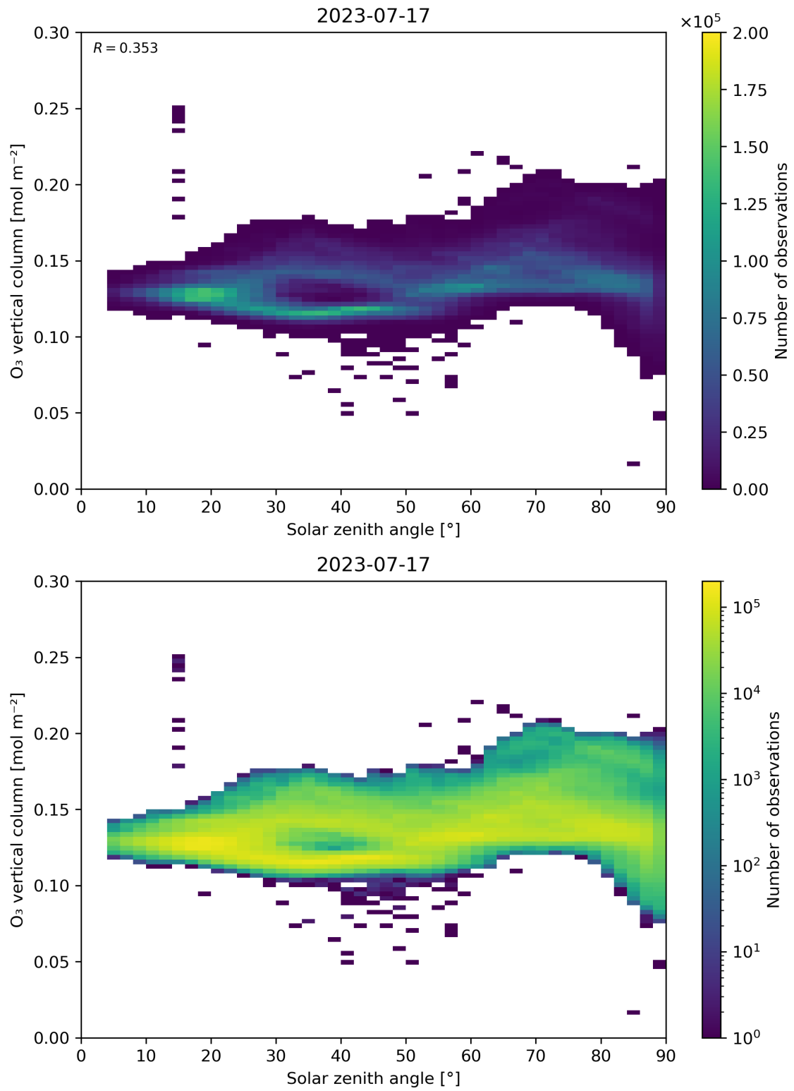
Figure 47: Scatter density plot of “Solar zenith angle” against “O 3 vertical column” for 2023-07-16 to 2023-07-18.
