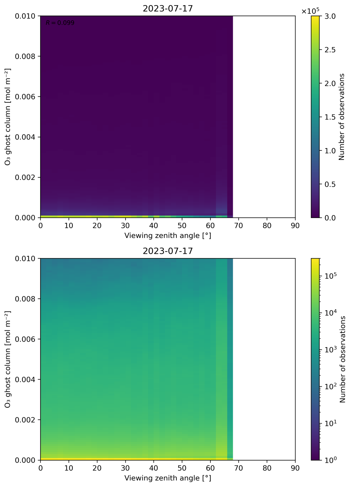
Figure 51: Scatter density plot of “Viewing zenith angle” against “O 3 ghost column” for 2023-07-16 to 2023-07-18.
