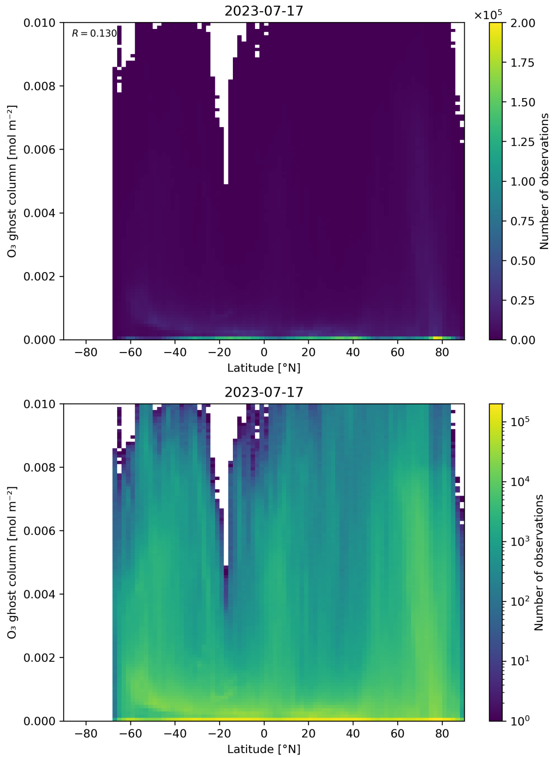
Figure 35: Scatter density plot of “Latitude” against “O 3 ghost column” for 2023-07-16 to 2023-07-18.
