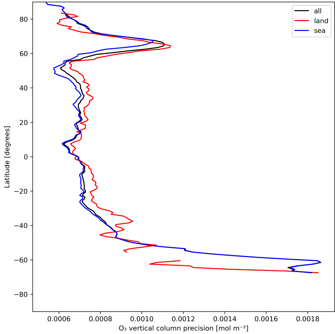
Figure 15: Zonal average of “O 3 vertical column precision” for 2023-07-16 to 2023-07-18.
