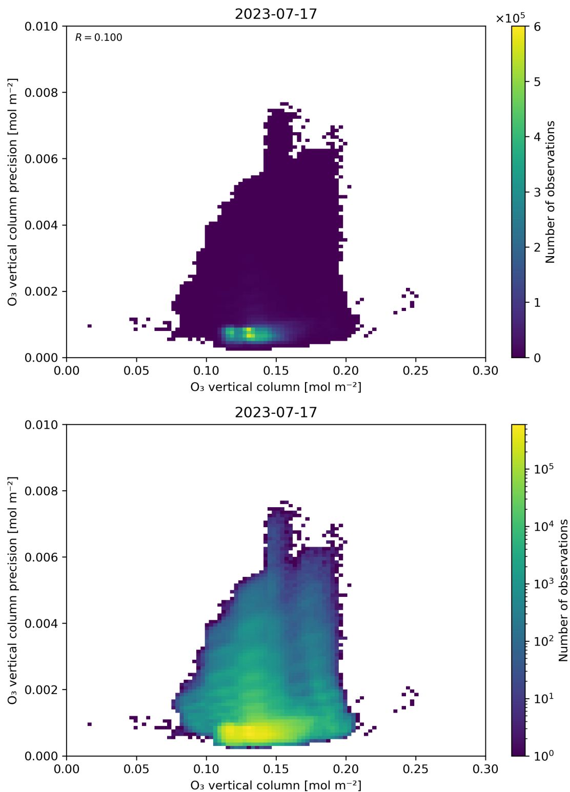
Figure 41: Scatter density plot of “O 3 vertical column” against “O 3 vertical column precision” for 2023-07-16 to 2023-07-18.
