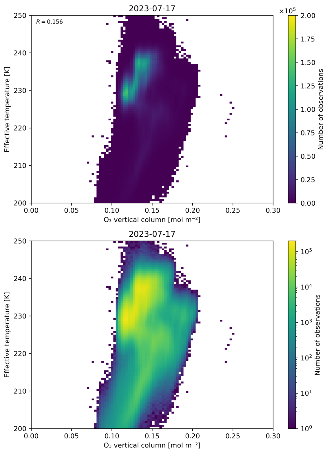
Figure 39: Scatter density plot of “O 3 vertical column” against “Effective temperature” for 2023-07-16 to 2023-07-18.
