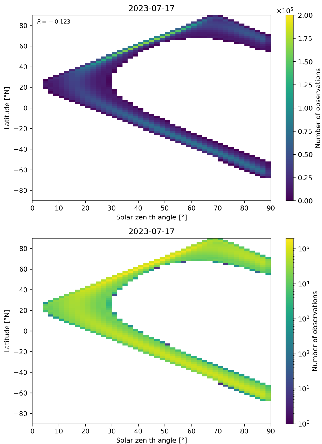
Figure 44: Scatter density plot of “Solar zenith angle” against “Latitude” for 2023-07-16 to 2023-07-18.
