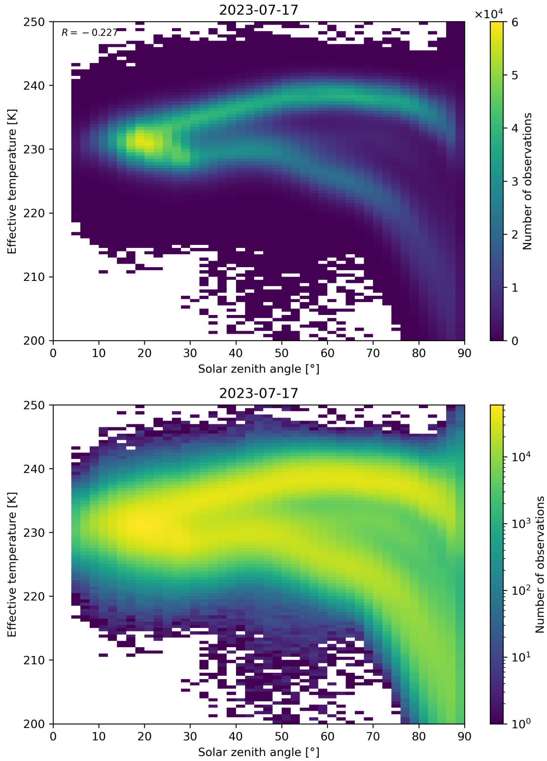
Figure 45: Scatter density plot of “Solar zenith angle” against “Effective temperature” for 2023-07-16 to 2023-07-18.
