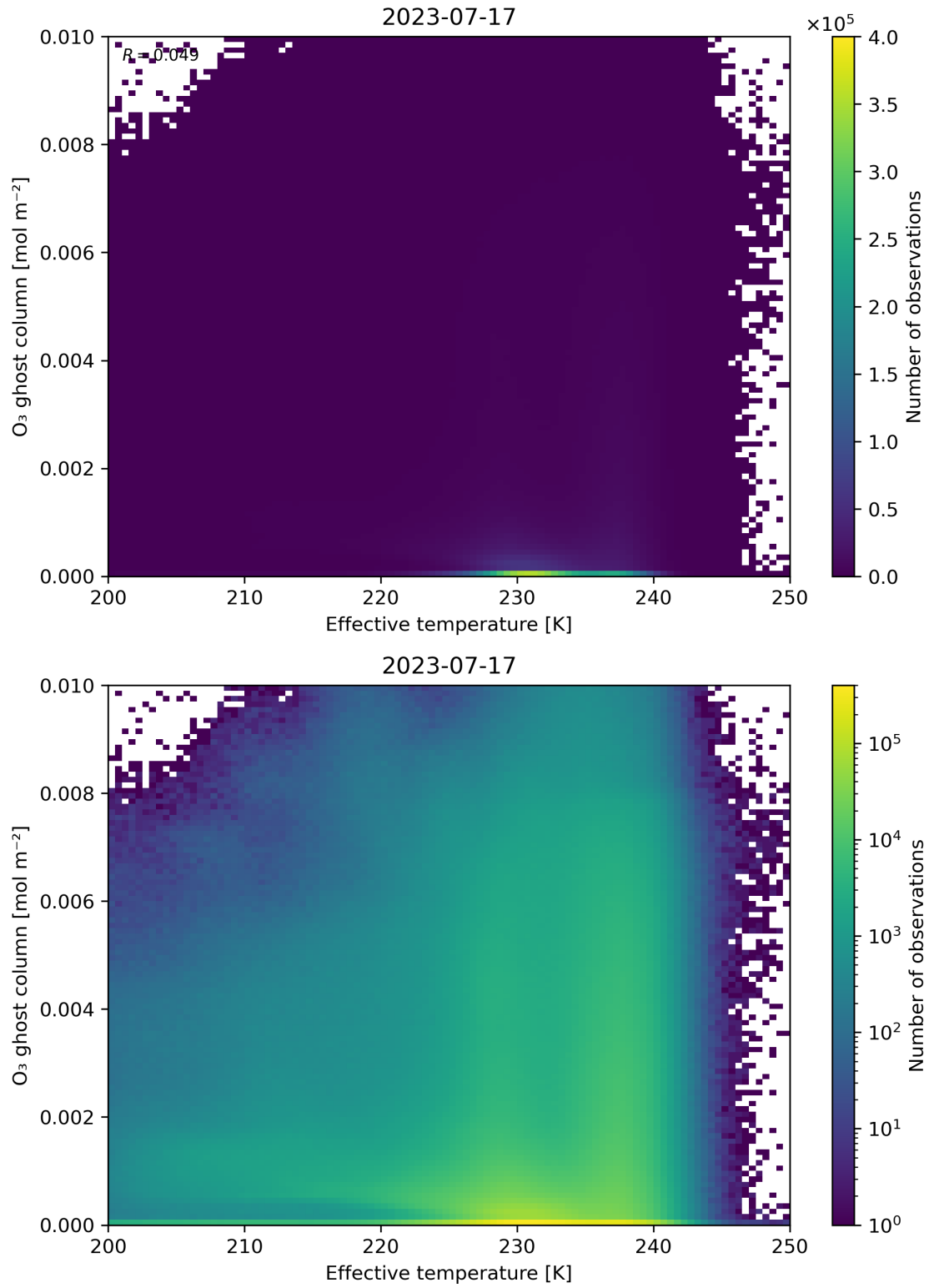
Figure 38: Scatter density plot of “Effective temperature” against “O 3 ghost column” for 2023-07-16 to 2023-07-18.
