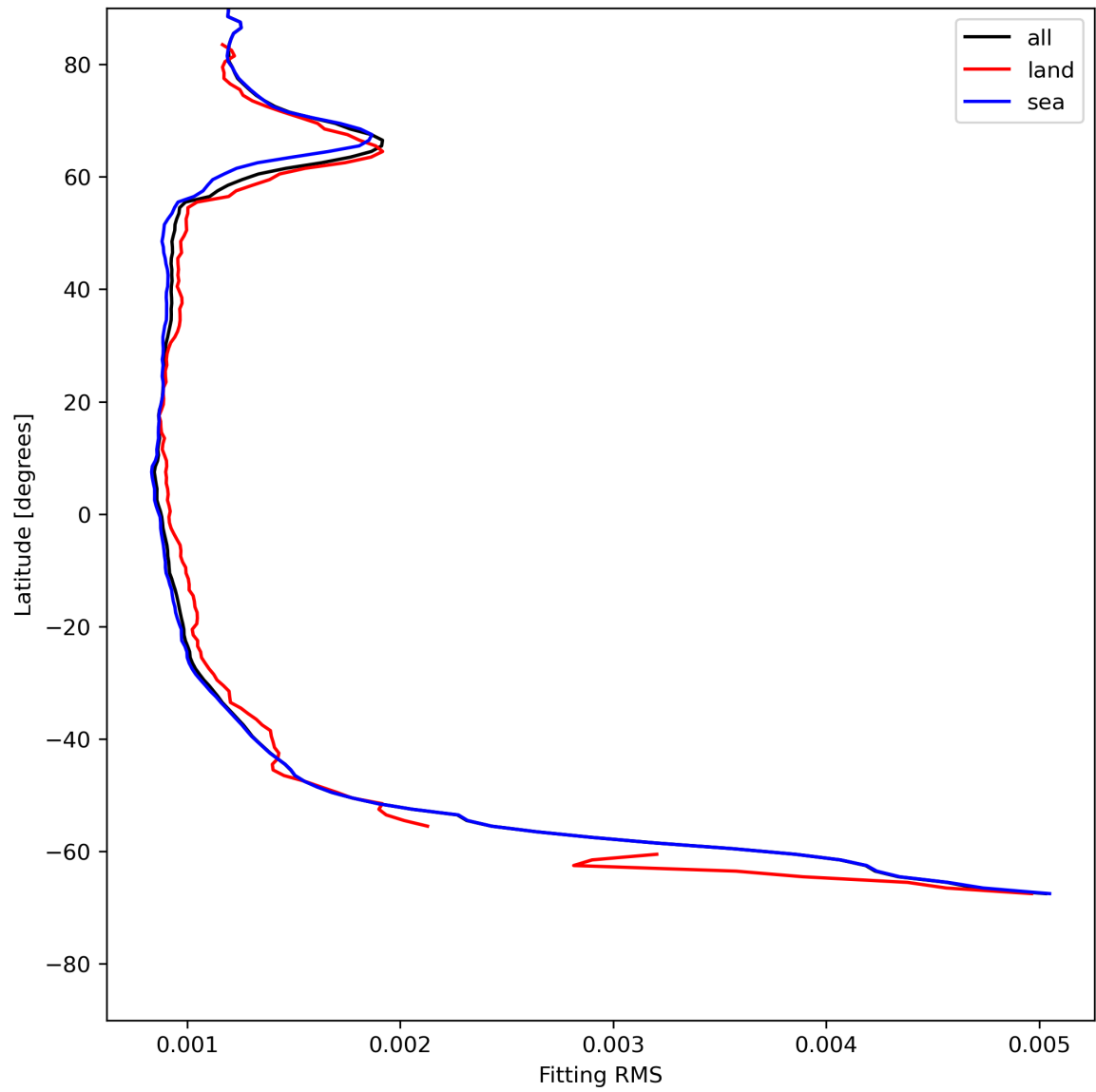
Figure 16: Zonal average of “Fitting RMS” for 2023-07-16 to 2023-07-18.
