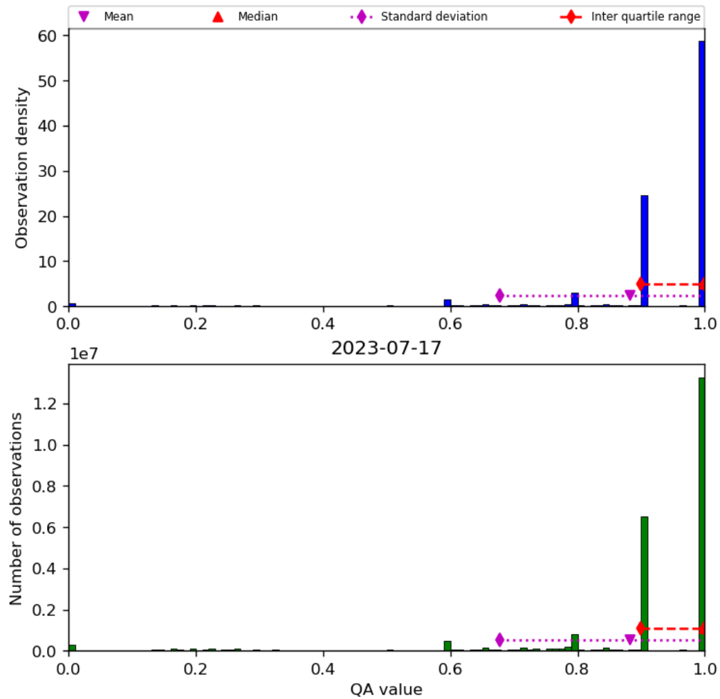
Figure 20: Histogram of “QA value” for 2023-07-16 to 2023-07-18
