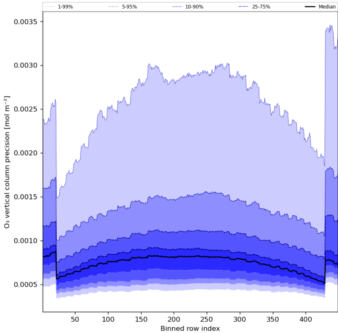
Figure 29: Along track statistics of “O 3 vertical column precision” for 2023-07-16 to 2023-07-18
