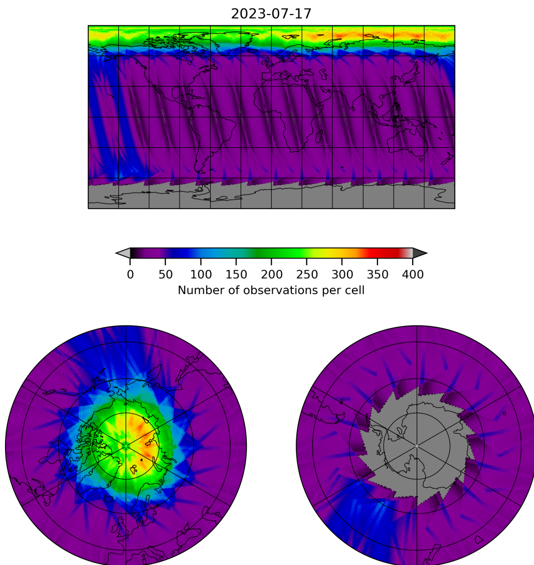
Figure 12: Map of the number of observations for 2023-07-16 to 2023-07-18
