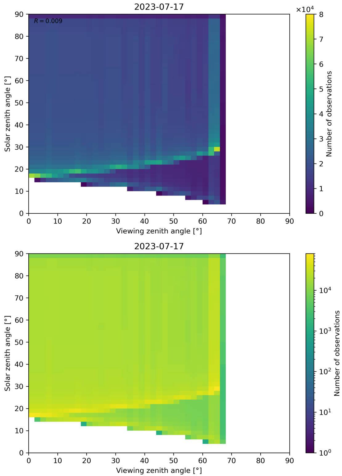
Figure 54: Scatter density plot of “Viewing zenith angle” against “Solar zenith angle” for 2023-07-16 to 2023-07-18.
