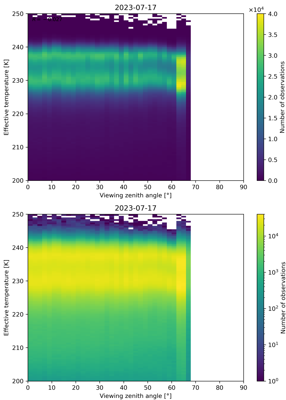
Figure 50: Scatter density plot of “Viewing zenith angle” against “Effective temperature” for 2023-07-16 to 2023-07-18.
