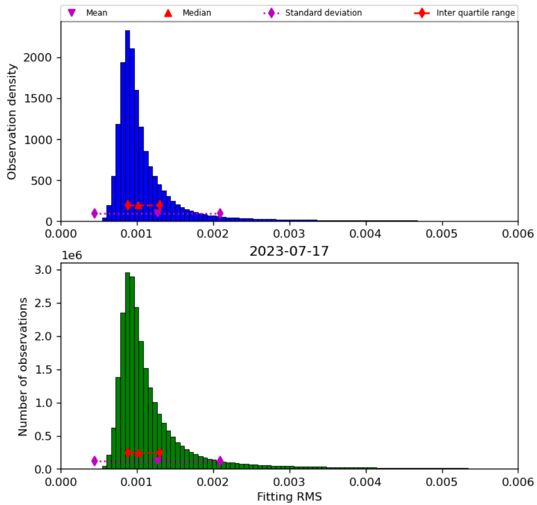
Figure 23: Histogram of “Fitting RMS” for 2023-07-16 to 2023-07-18
