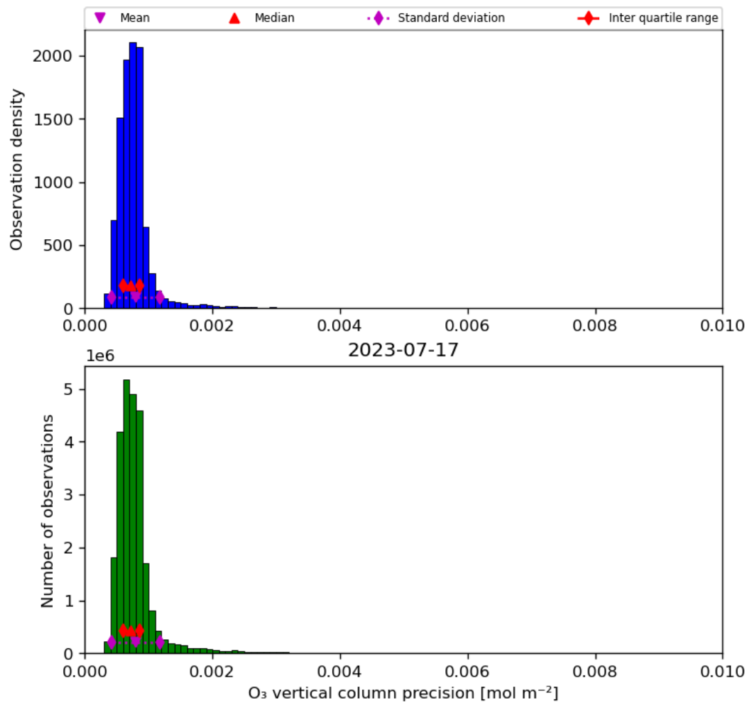
Figure 22: Histogram of “O 3 vertical column precision” for 2023-07-16 to 2023-07-18
