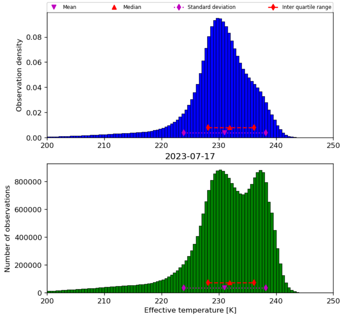
Figure 24: Histogram of “Effective temperature” for 2023-07-16 to 2023-07-18
