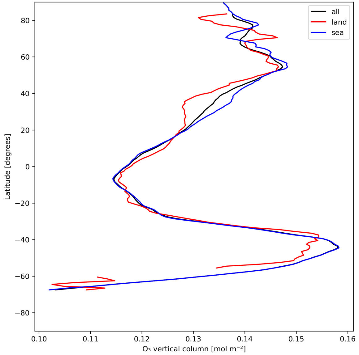
Figure 14: Zonal average of “O 3 vertical column” for 2023-07-16 to 2023-07-18.
