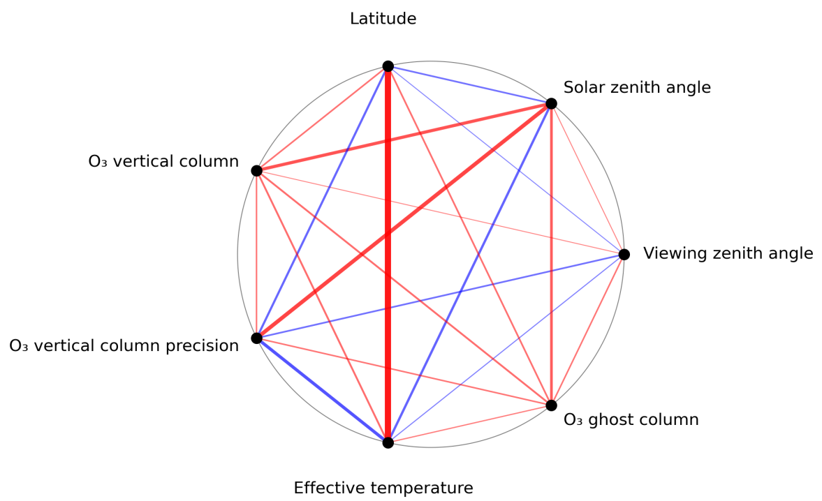
Figure 1: Map of correlation graph for 2023-07-16 to 2023-07-18.
