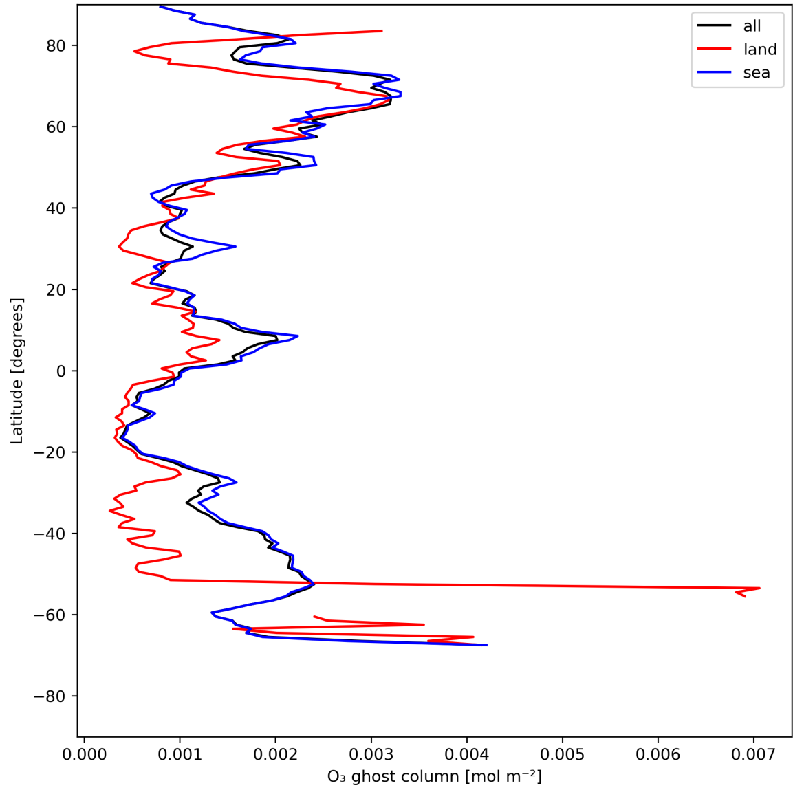
Figure 18: Zonal average of “O 3 ghost column” for 2023-07-16 to 2023-07-18.
