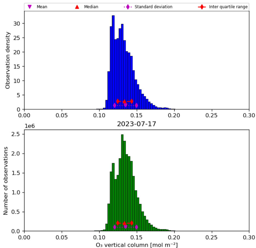
Figure 21: Histogram of “O 3 vertical column” for 2023-07-16 to 2023-07-18
