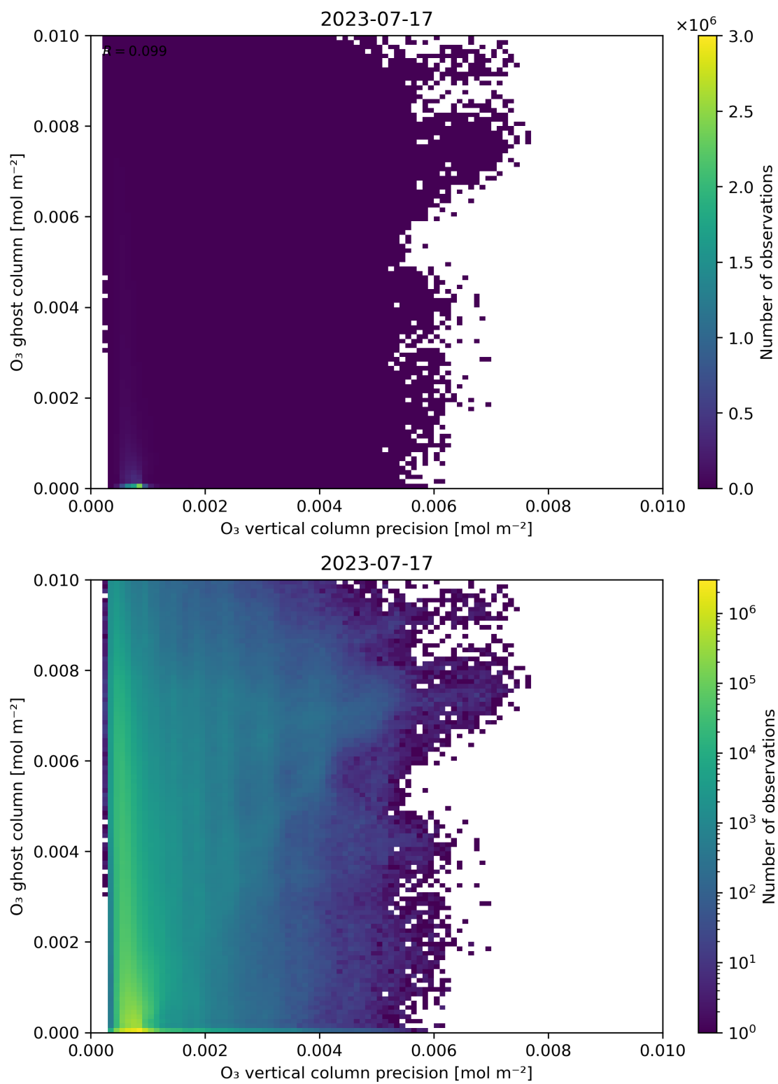
Figure 43: Scatter density plot of “O 3 vertical column precision” against “O 3 ghost column” for 2023-07-16 to 2023-07-18.
