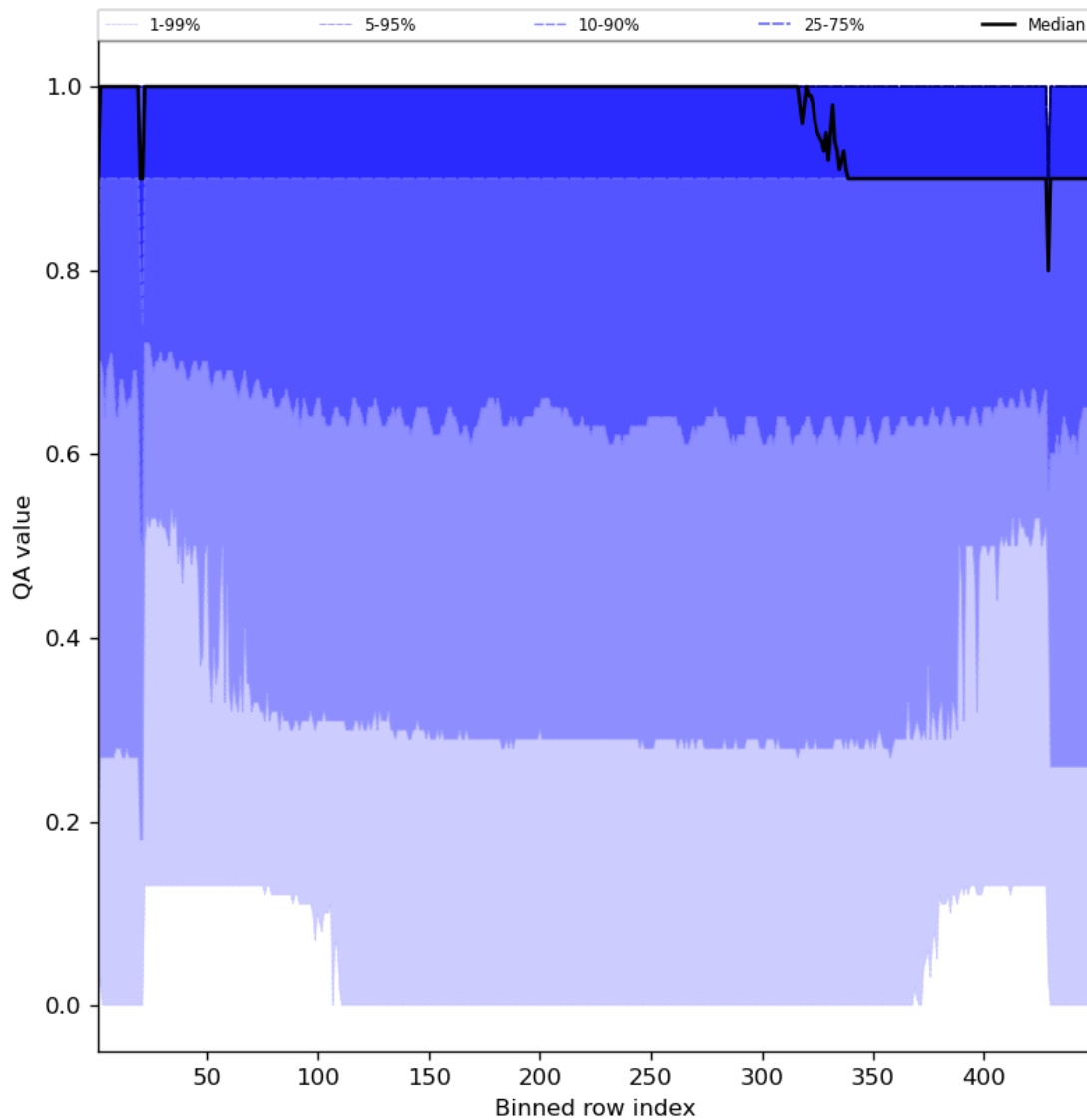
Figure 27: Along track statistics of “QA value” for 2023-07-16 to 2023-07-18
