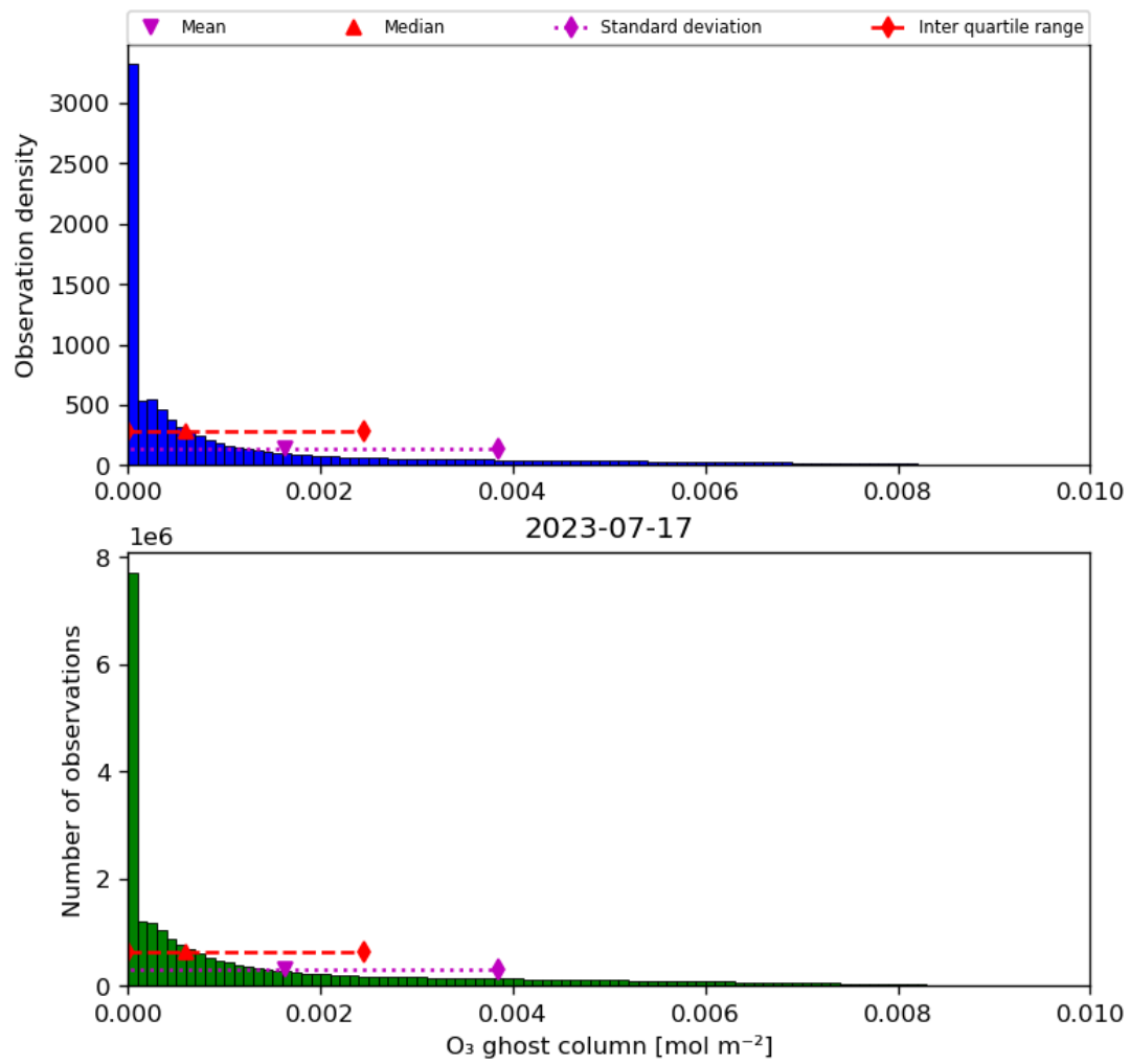
Figure 25: Histogram of “O 3 ghost column” for 2023-07-16 to 2023-07-18
