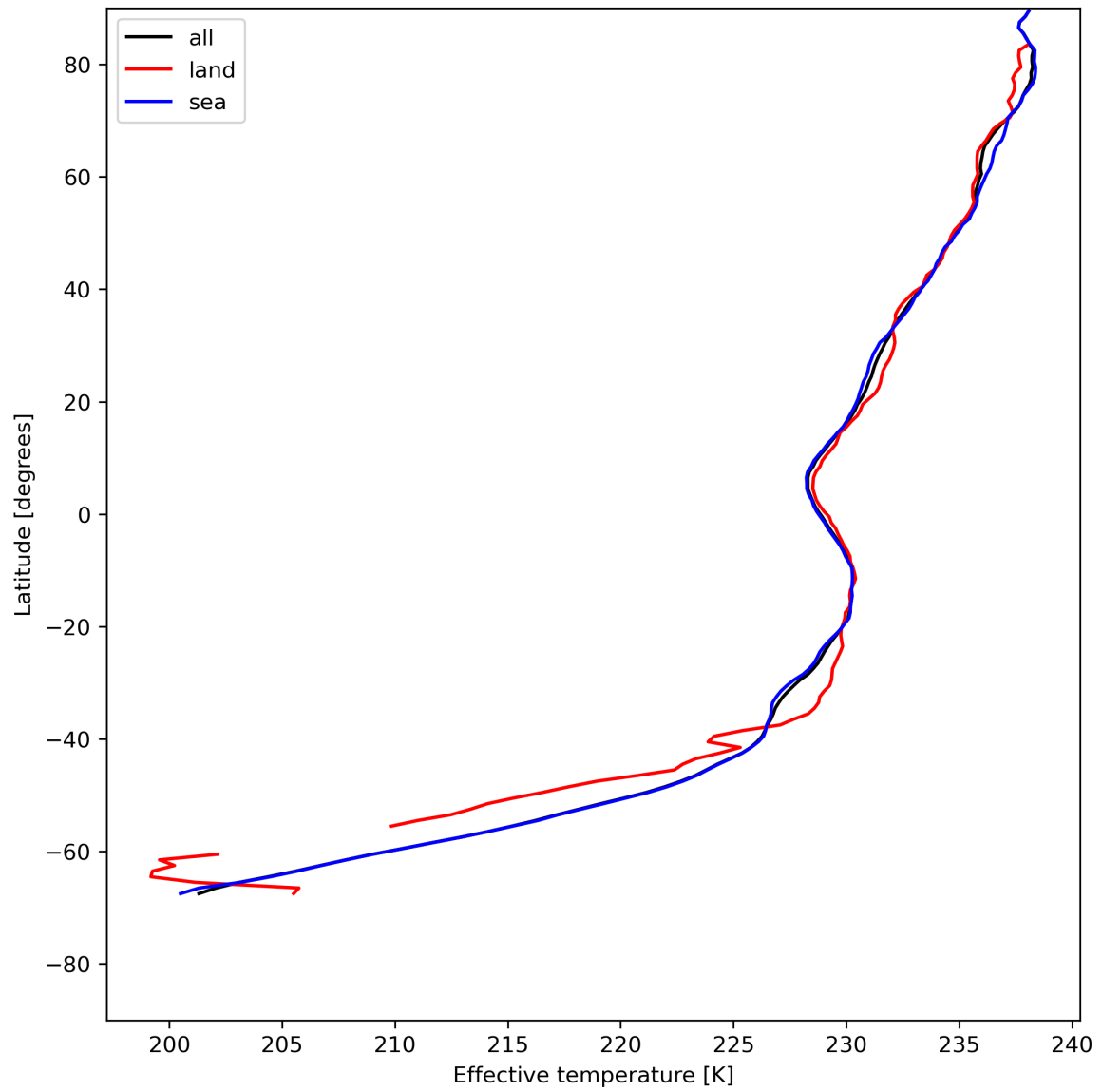
Figure 17: Zonal average of "Effective temperature" for 2023-07-16 to 2023-07-18.
