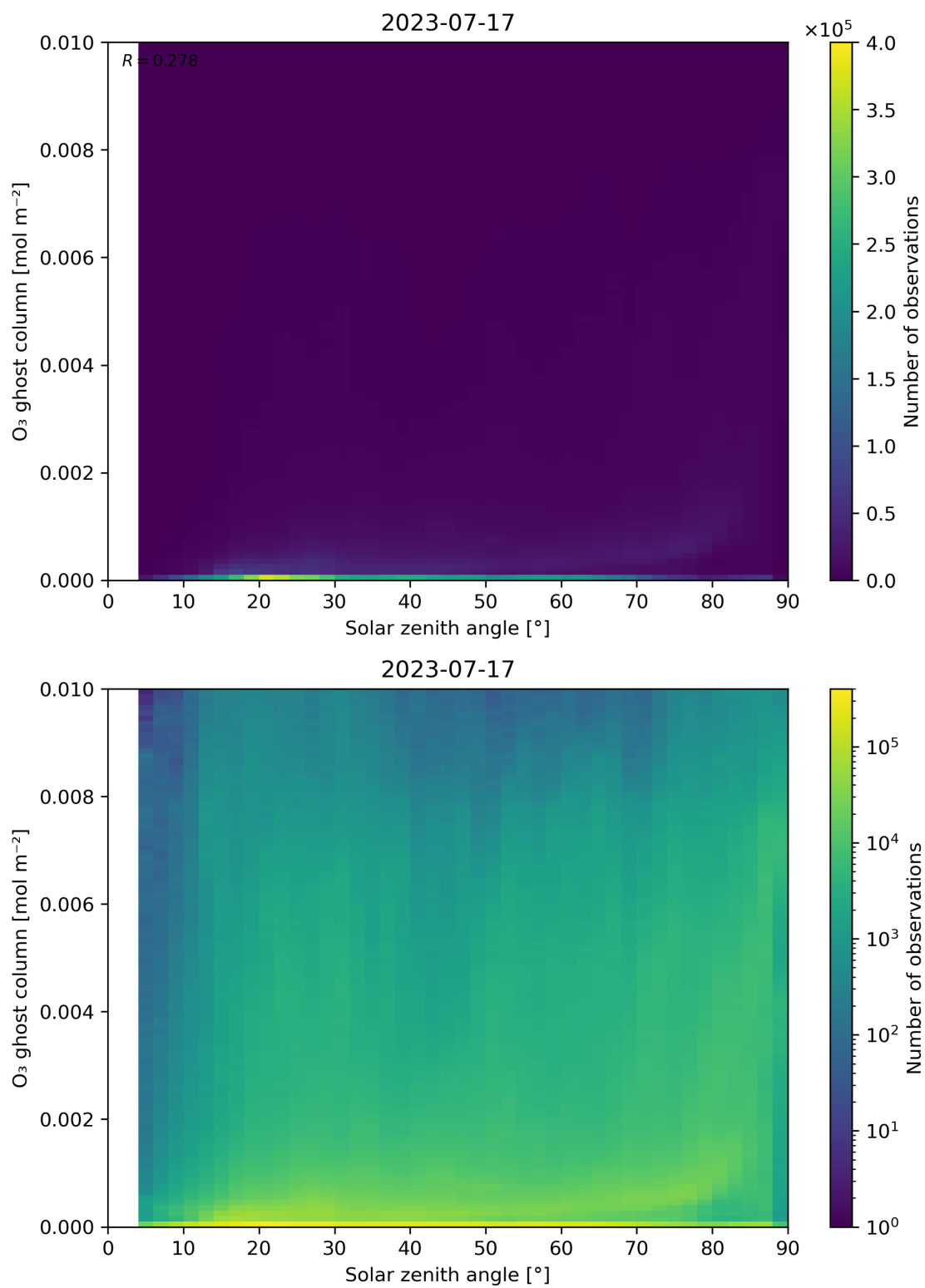
Figure 46: Scatter density plot of “Solar zenith angle” against “O 3 ghost column” for 2023-07-16 to 2023-07-18.
