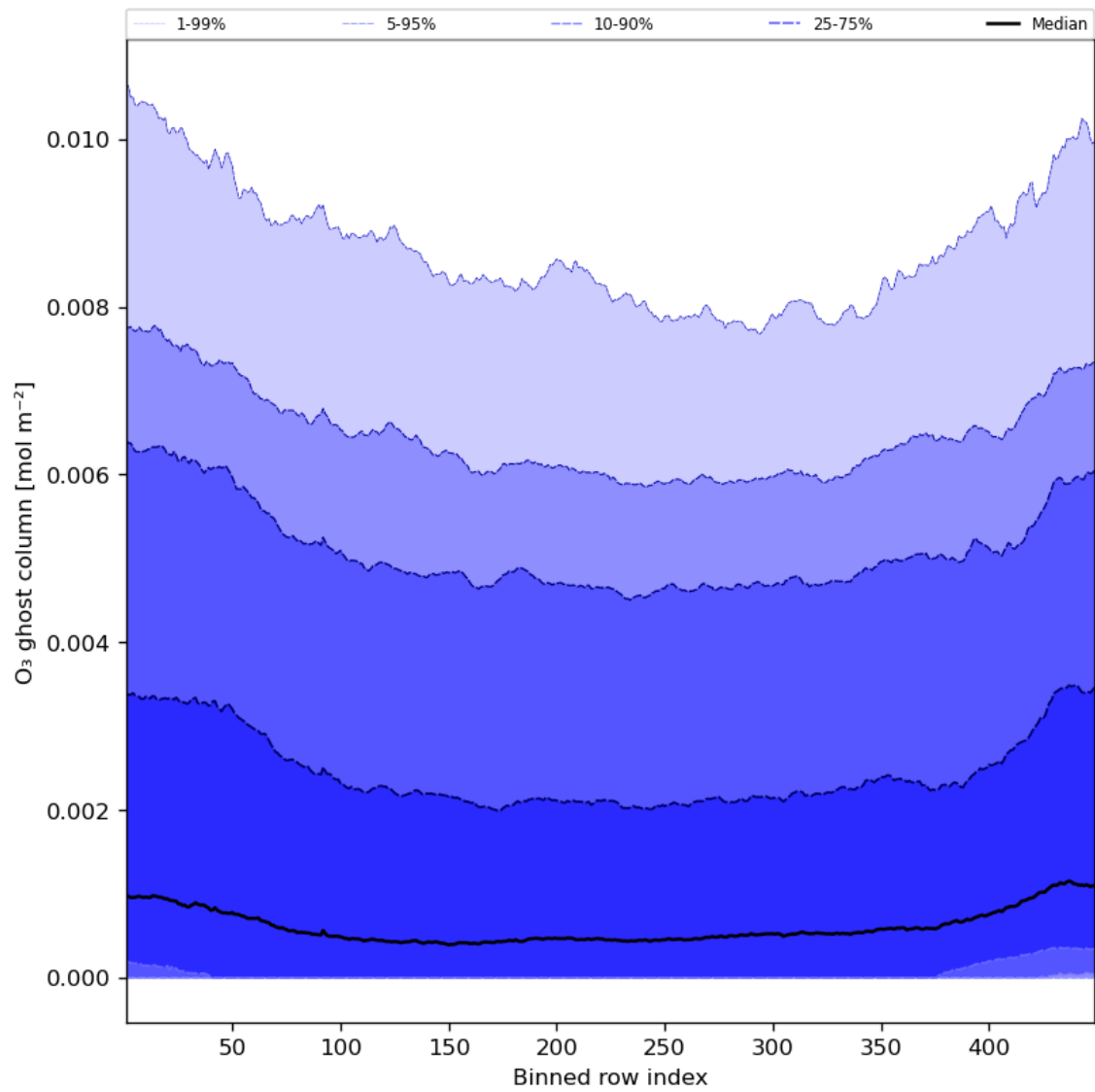
Figure 32: Along track statistics of “O 3 ghost column” for 2023-07-16 to 2023-07-18
