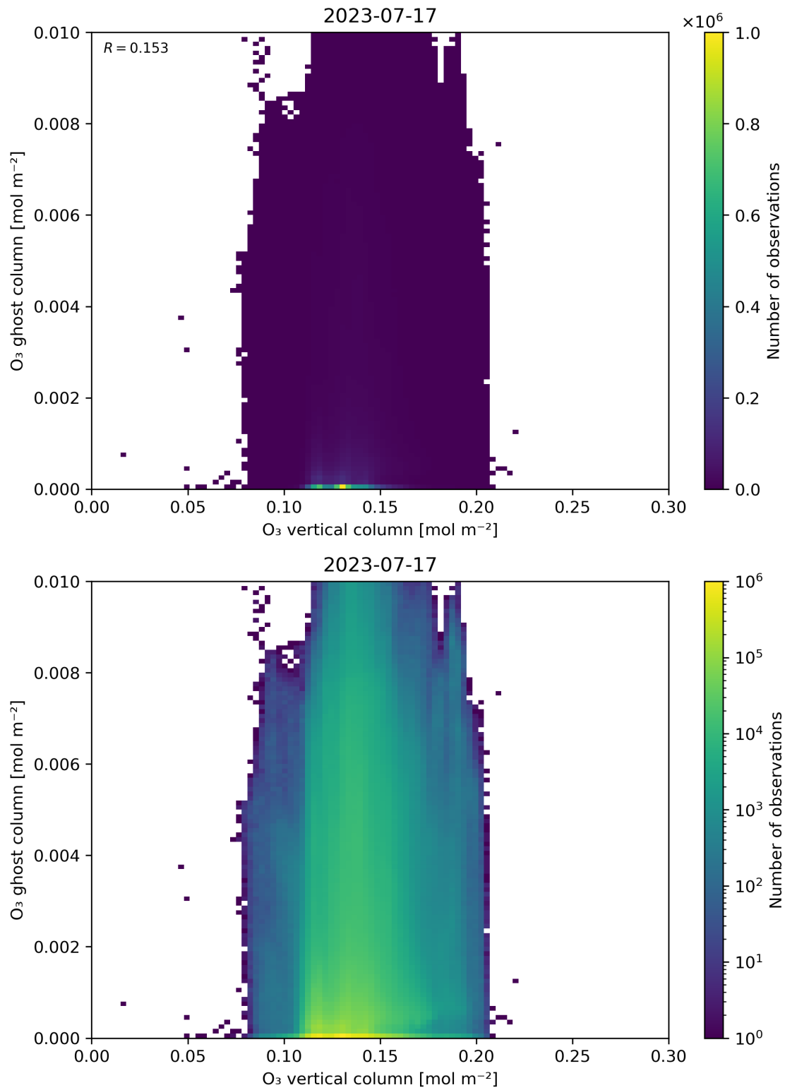
Figure 40: Scatter density plot of “O 3 vertical column” against “O 3 ghost column” for 2023-07-16 to 2023-07-18.
