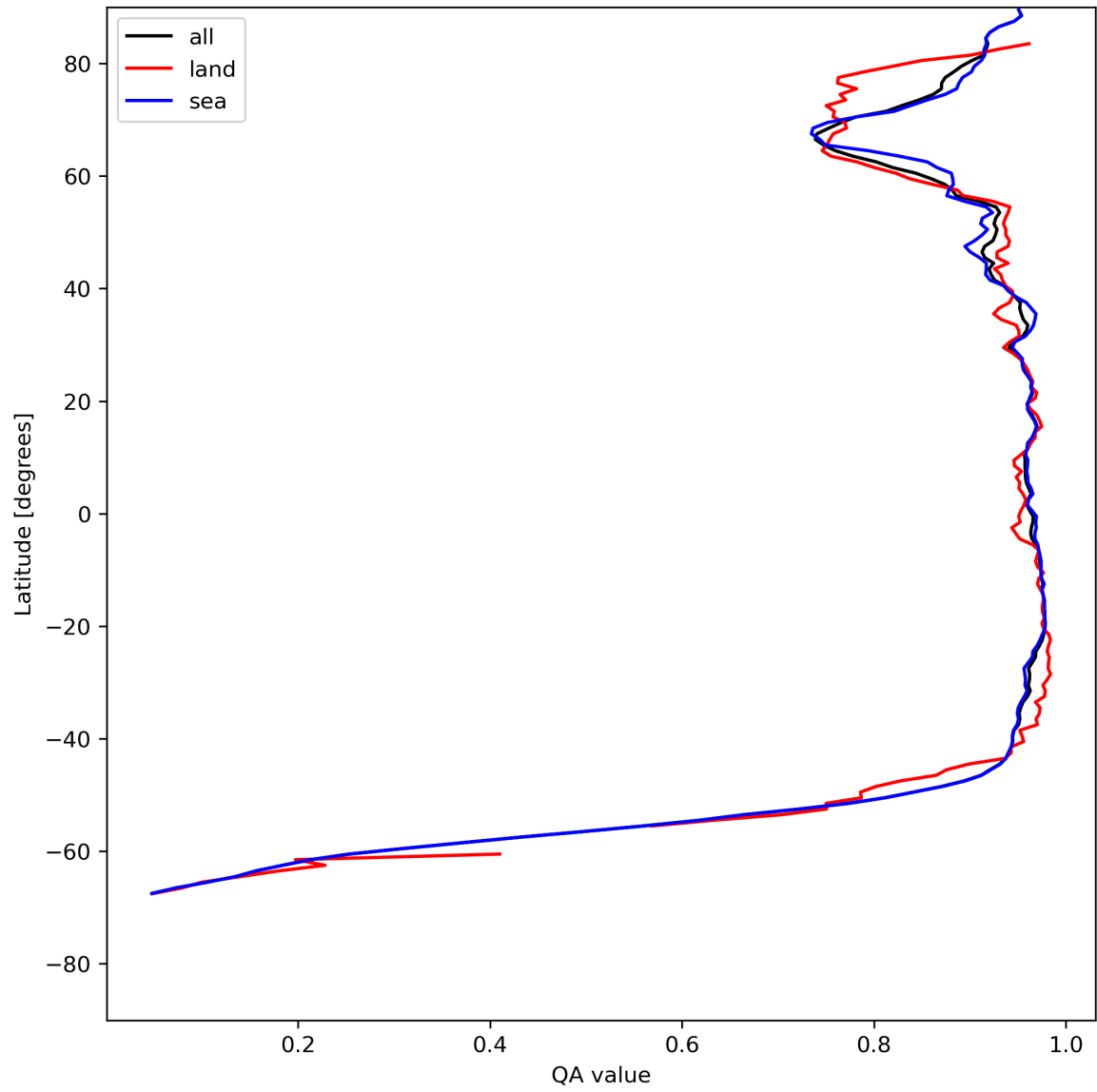
Figure 13: Zonal average of “QA value” for 2023-07-16 to 2023-07-18.
