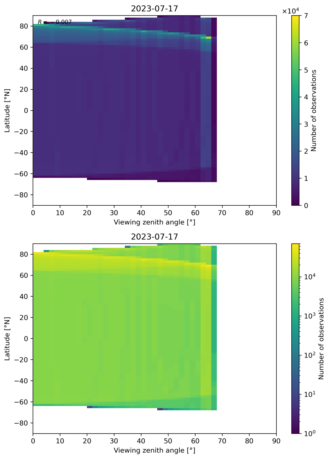
Figure 49: Scatter density plot of “Viewing zenith angle” against “Latitude” for 2023-07-16 to 2023-07-18.
