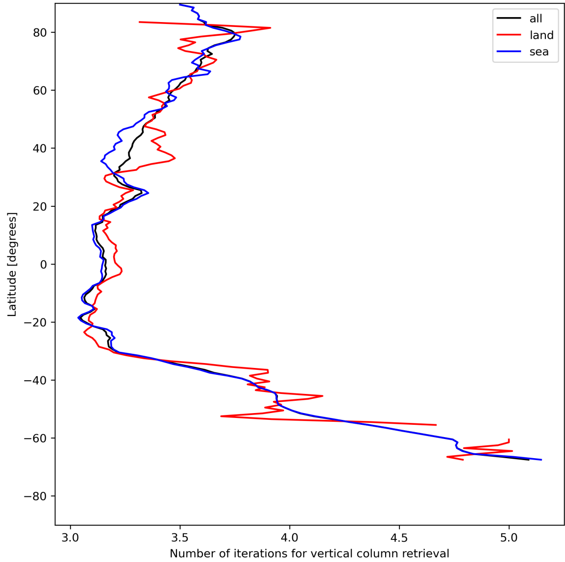
Figure 19: Zonal average of “Number of iterations for vertical column retrieval” for 2023-07-16 to 2023-07-18.
