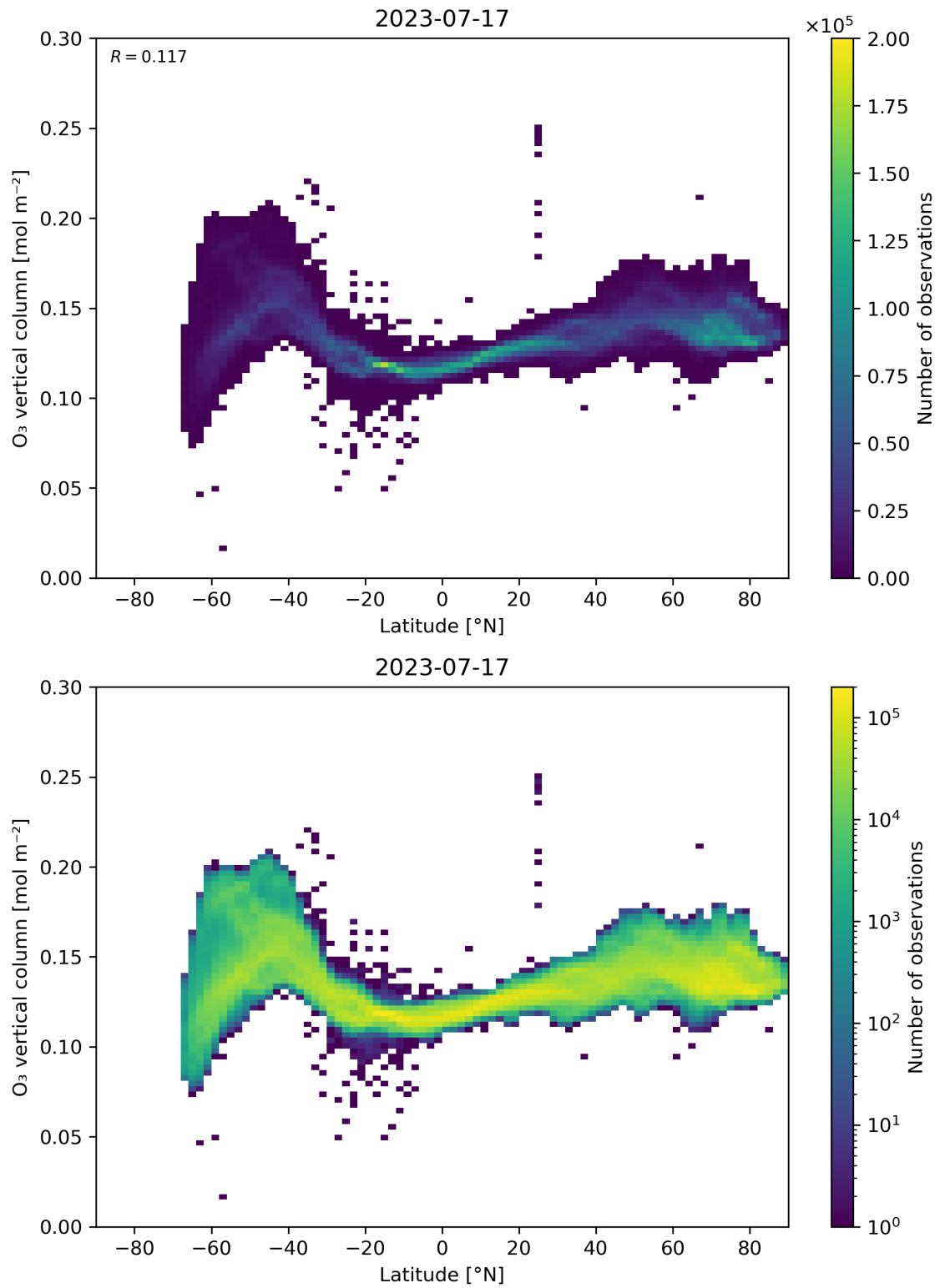
Figure 36: Scatter density plot of “Latitude” against “O 3 vertical column” for 2023-07-16 to 2023-07-18.
