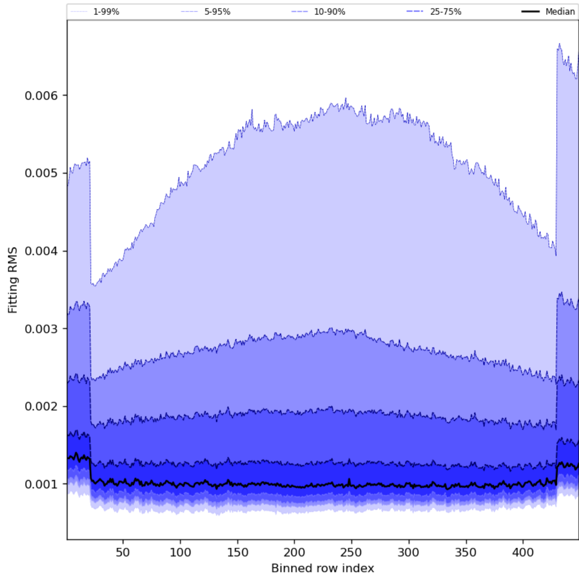
Figure 30: Along track statistics of “Fitting RMS” for 2023-07-16 to 2023-07-18
