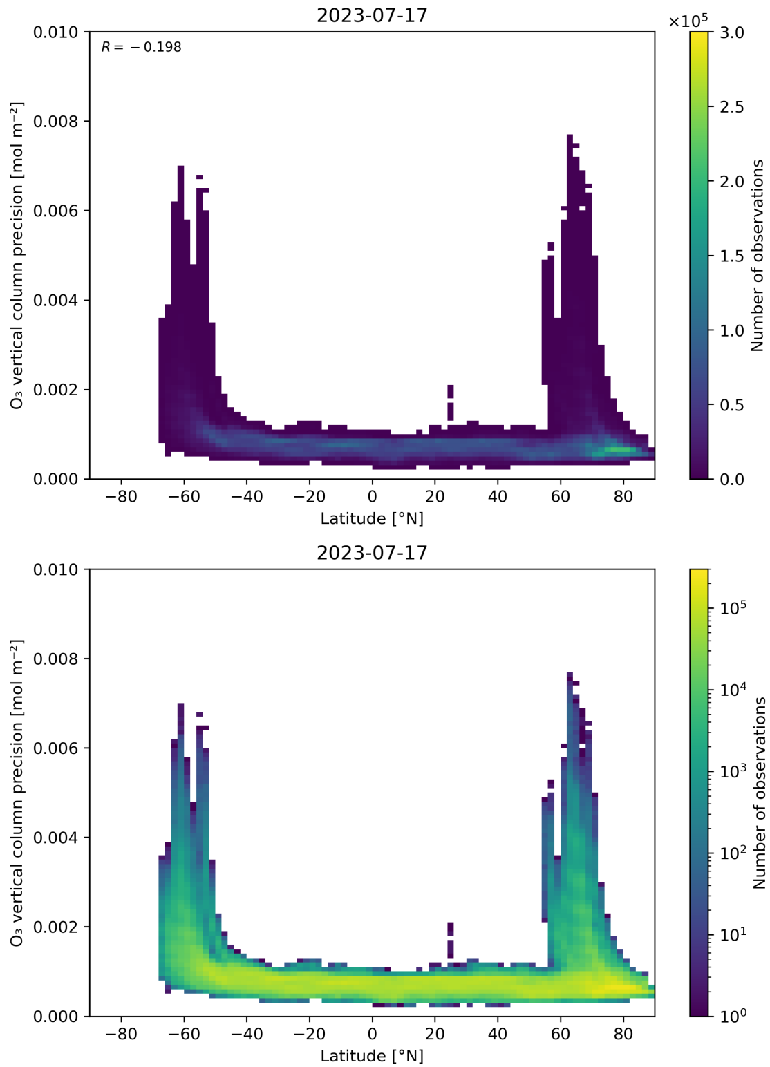
Figure 37: Scatter density plot of “Latitude” against “O 3 vertical column precision” for 2023-07-16 to 2023-07-18.
