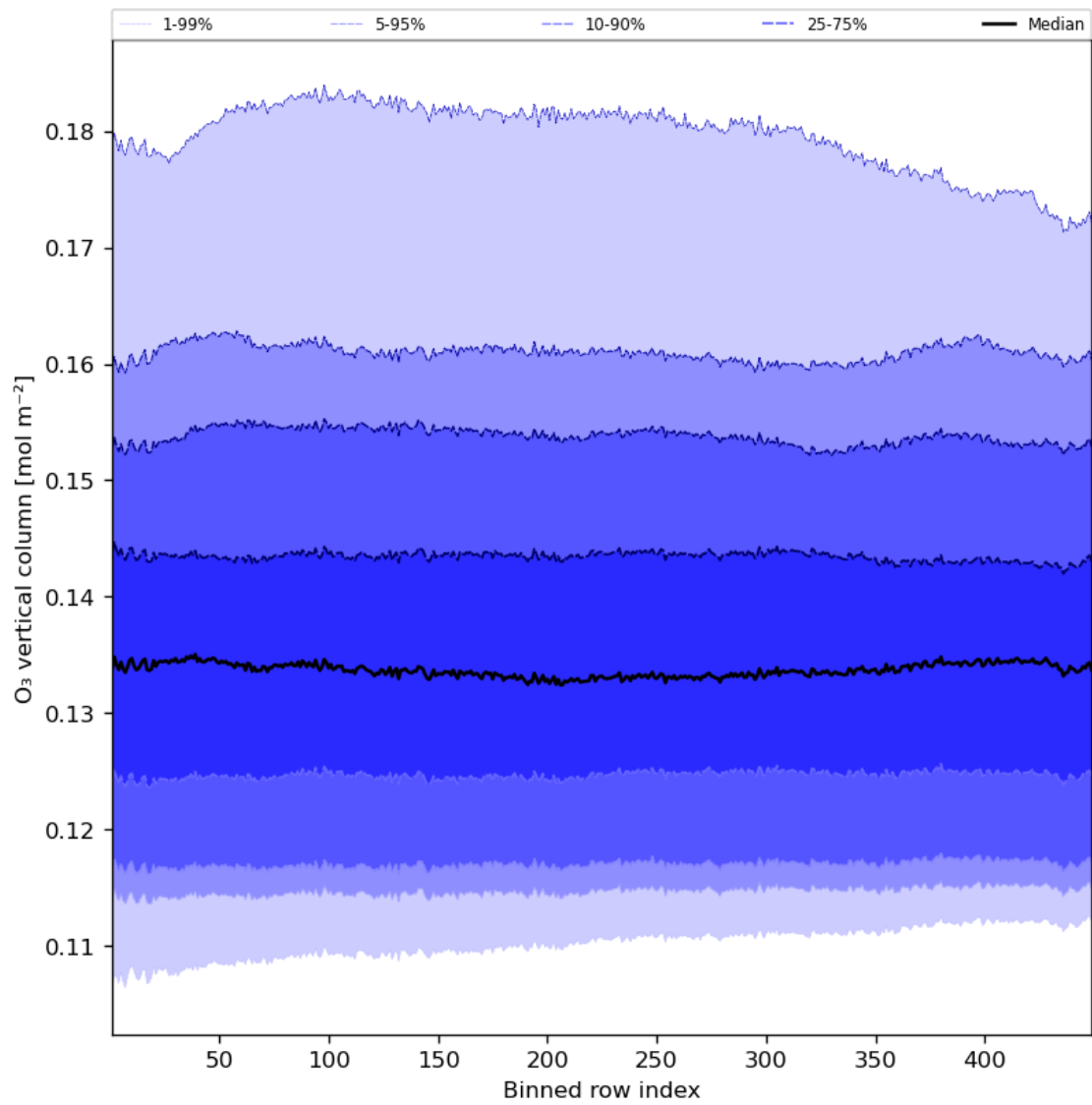
Figure 28: Along track statistics of “O 3 vertical column” for 2023-07-16 to 2023-07-18
