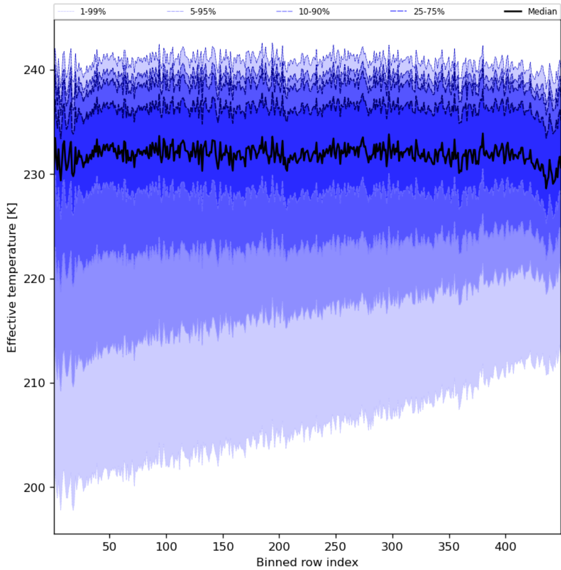
Figure 31: Along track statistics of “Effective temperature” for 2023-07-16 to 2023-07-18
