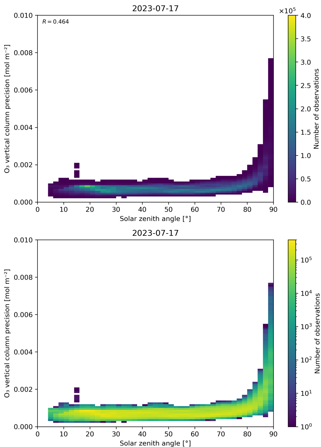
Figure 48: Scatter density plot of “Solar zenith angle” against “O 3 vertical column precision” for 2023-07-16 to 2023-07-18.
