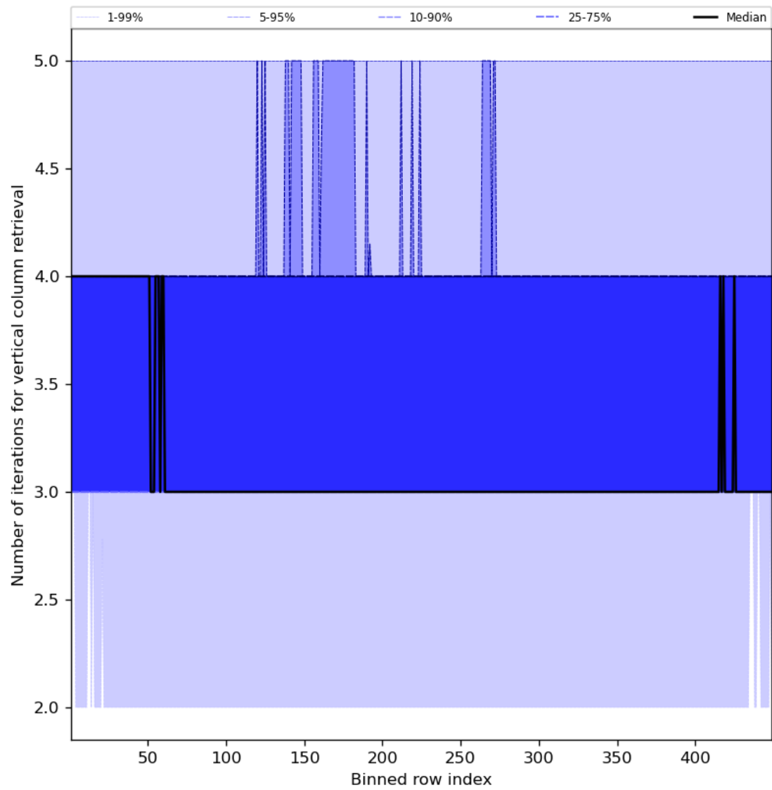
Figure 33: Along track statistics of “Number of iterations for vertical column retrieval” for 2023-07-16 to 2023-07-18
