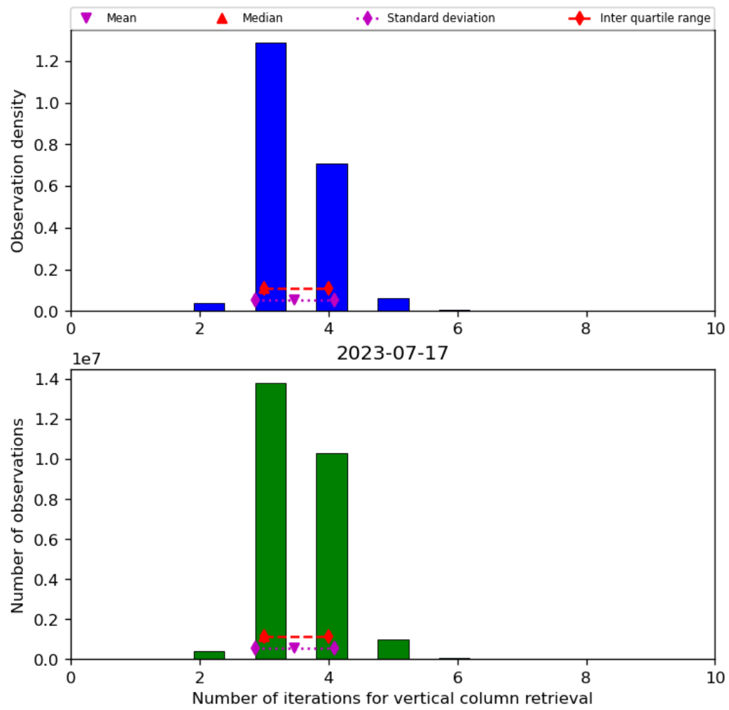
Figure 26: Histogram of “Number of iterations for vertical column retrieval” for 2023-07-16 to 2023-07-18
