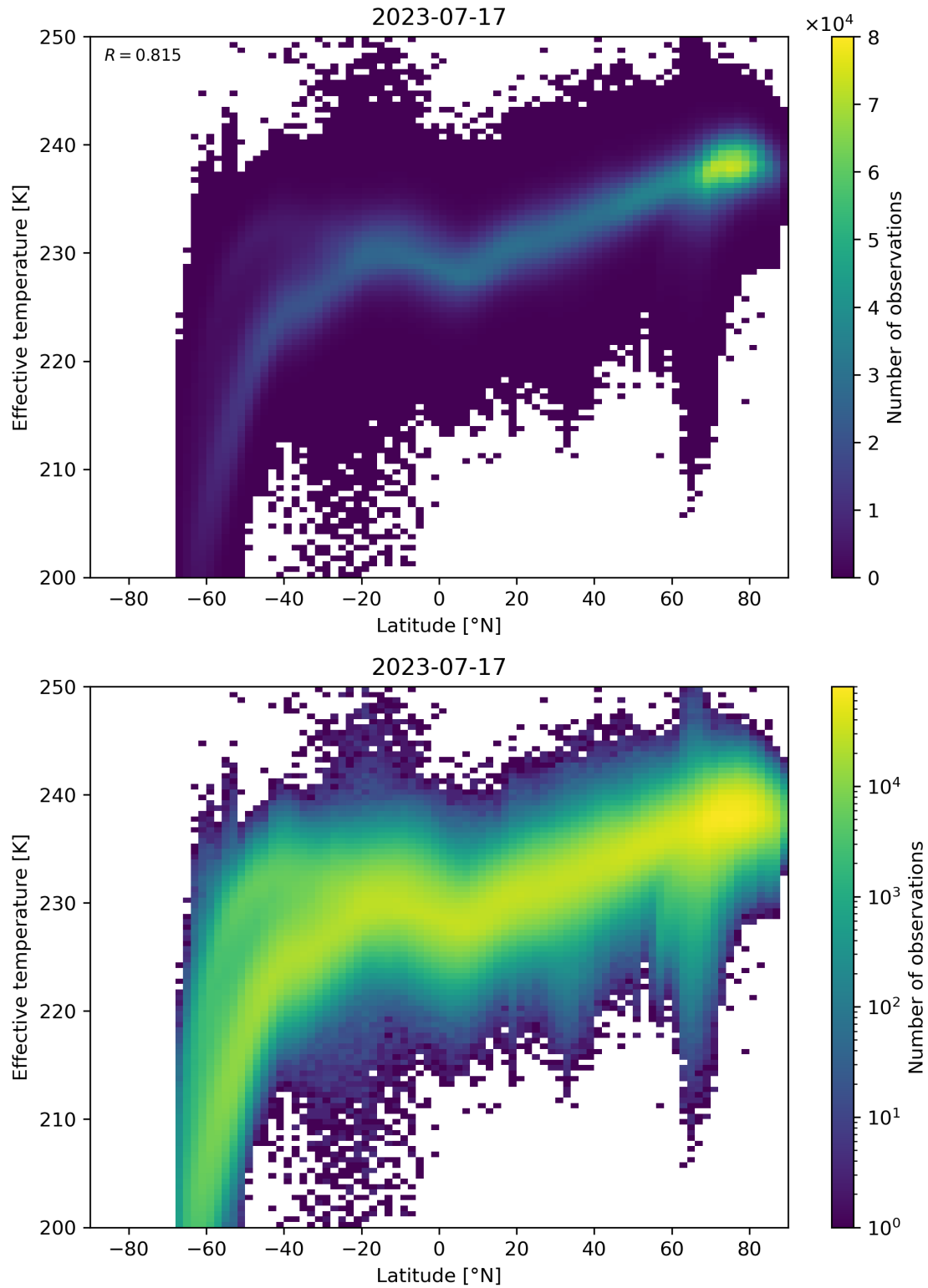
Figure 34: Scatter density plot of “Latitude” against “Effective temperature” for 2023-07-16 to 2023-07-18.
