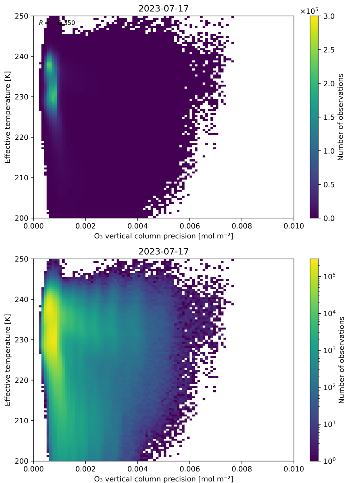
Figure 42: Scatter density plot of “O 3 vertical column precision” against “Effective temperature” for 2023-07-16 to 2023-07-18.
