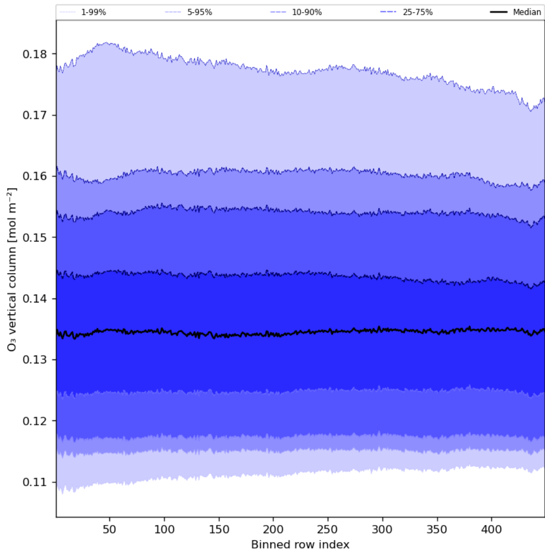
Figure 28: Along track statistics of “O 3 vertical column” for 2023-07-19 to 2023-07-20
