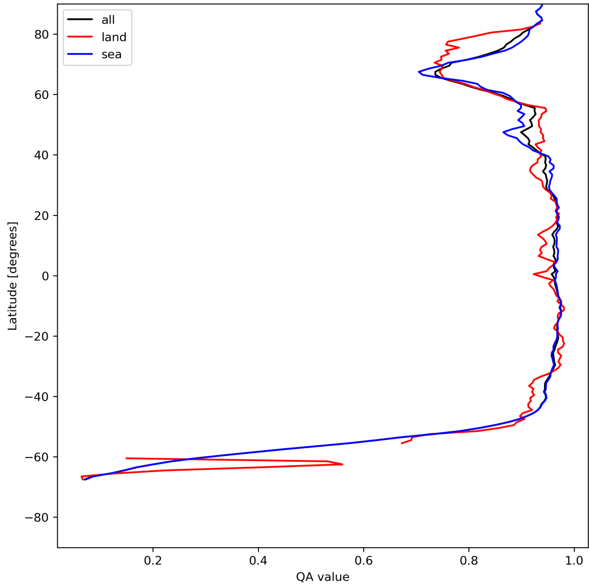
Figure 13: Zonal average of “QA value” for 2023-07-19 to 2023-07-20.
