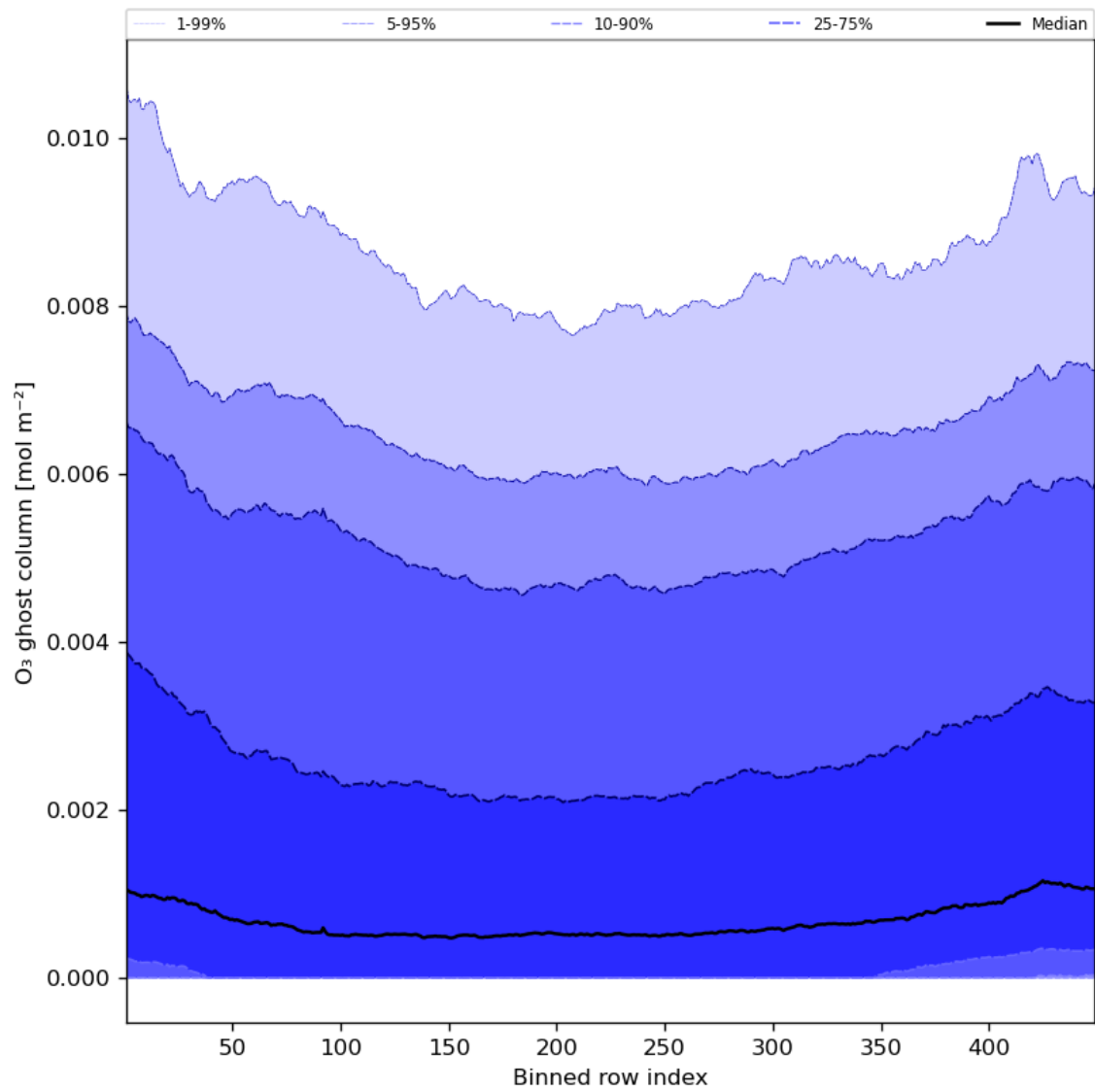
Figure 32: Along track statistics of “O 3 ghost column” for 2023-07-19 to 2023-07-20
