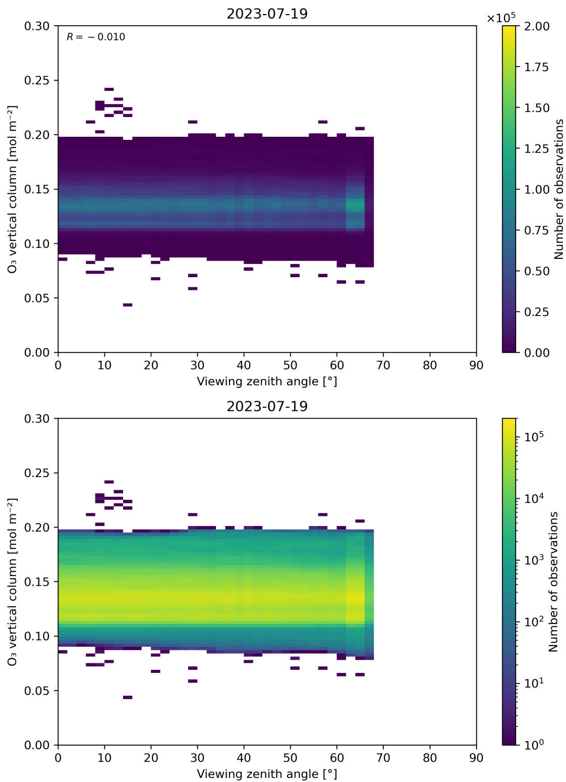
Figure 52: Scatter density plot of “Viewing zenith angle” against “O 3 vertical column” for 2023-07-19 to 2023-07-20.
