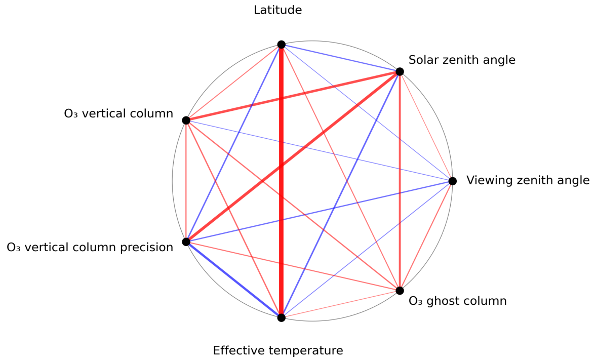
Figure 1: Map of correlation graph for 2023-07-19 to 2023-07-20.
