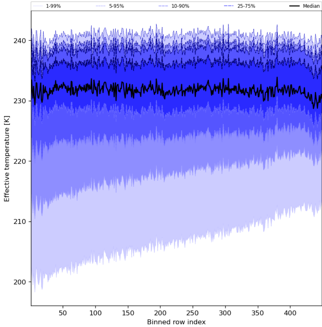
Figure 31: Along track statistics of “Effective temperature” for 2023-07-19 to 2023-07-20
