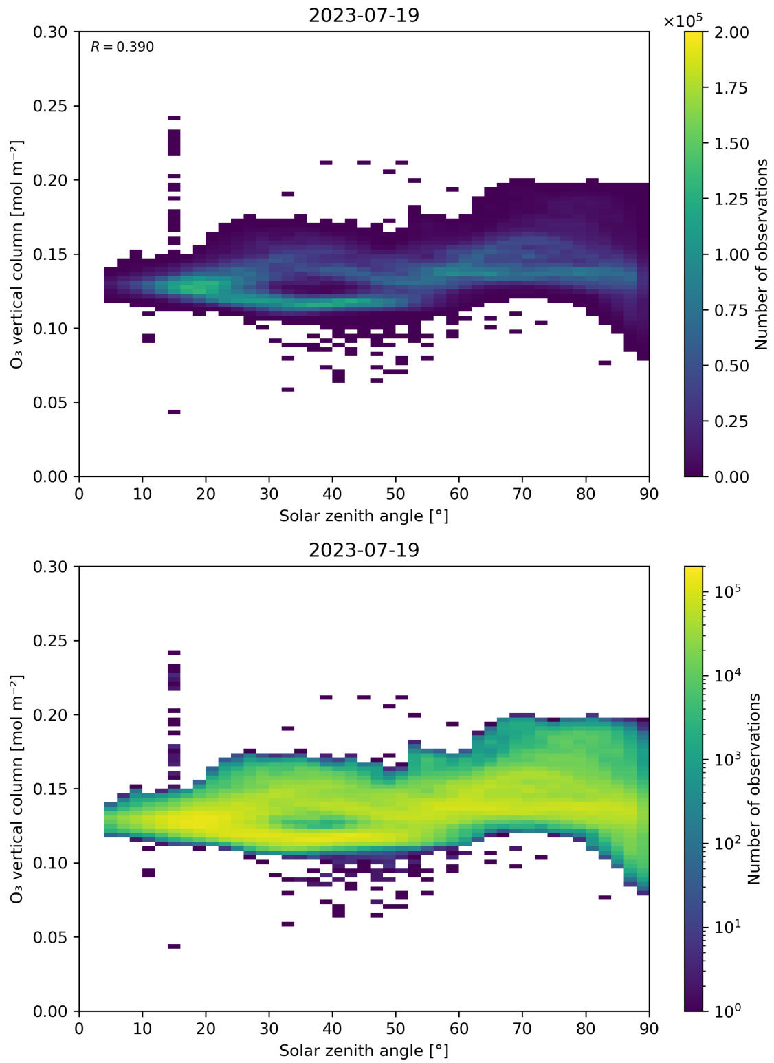
Figure 47: Scatter density plot of “Solar zenith angle” against “O 3 vertical column” for 2023-07-19 to 2023-07-20.
