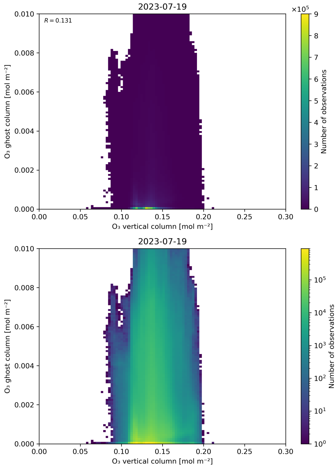
Figure 40: Scatter density plot of “O 3 vertical column” against “O 3 ghost column” for 2023-07-19 to 2023-07-20.
