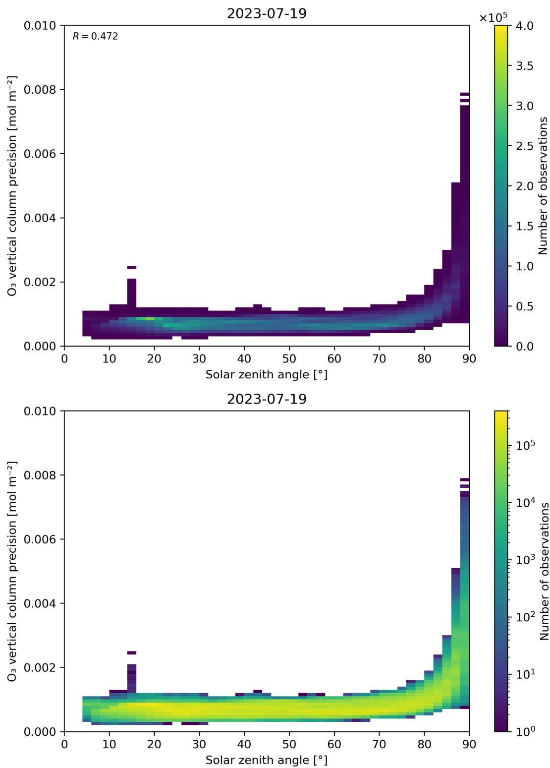
Figure 48: Scatter density plot of “Solar zenith angle” against “O 3 vertical column precision” for 2023-07-19 to 2023-07-20.
