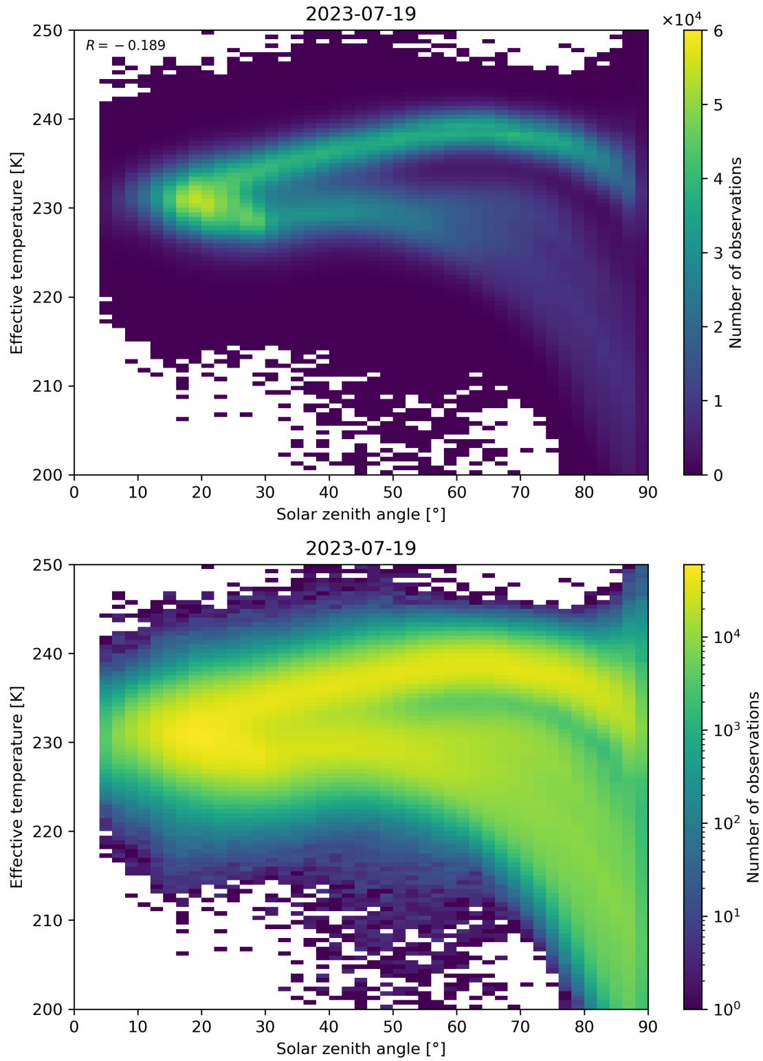
Figure 45: Scatter density plot of “Solar zenith angle” against “Effective temperature” for 2023-07-19 to 2023-07-20.
