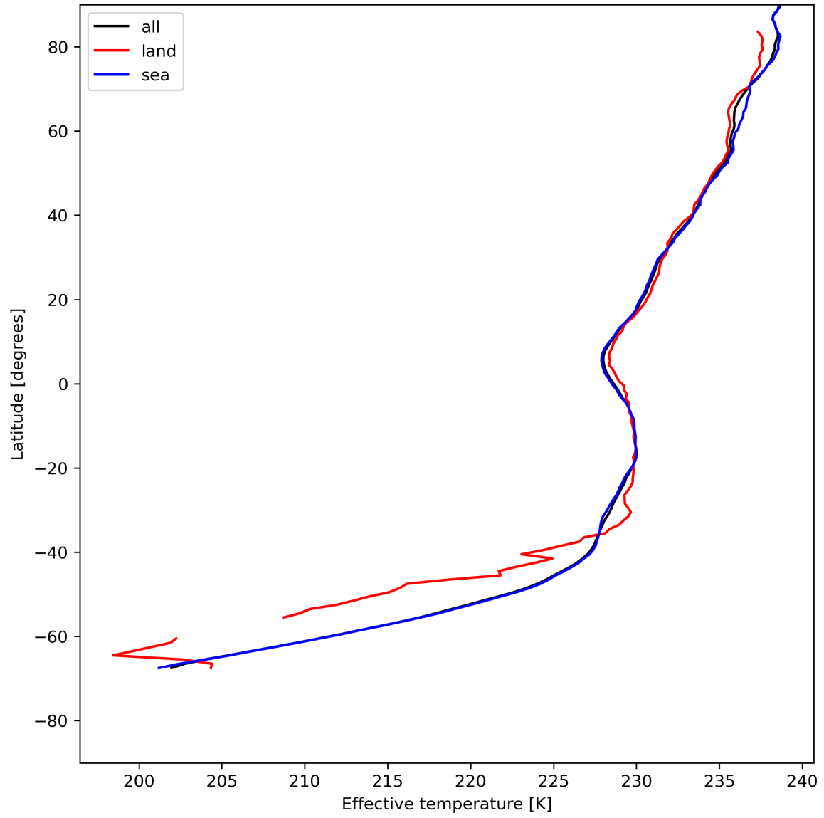
Figure 17: Zonal average of "Effective temperature" for 2023-07-19 to 2023-07-20.
