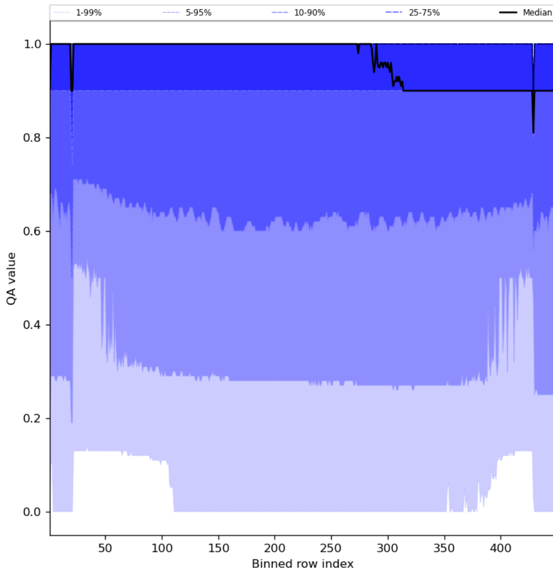
Figure 27: Along track statistics of “QA value” for 2023-07-19 to 2023-07-20
