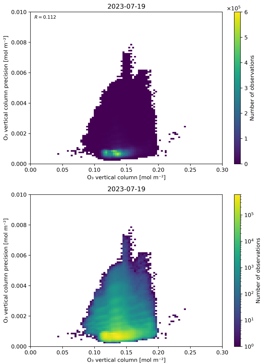
Figure 41: Scatter density plot of “O 3 vertical column” against “O 3 vertical column precision” for 2023-07-19 to 2023-07-20.
