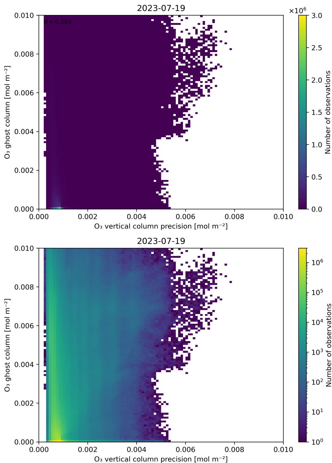
Figure 43: Scatter density plot of “ O_3 vertical column precision” against “ O_3 ghost column” for 2023-07-19 to 2023-07-20.
