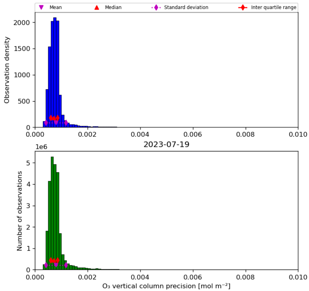
Figure 22: Histogram of “O 3 vertical column precision” for 2023-07-19 to 2023-07-20
