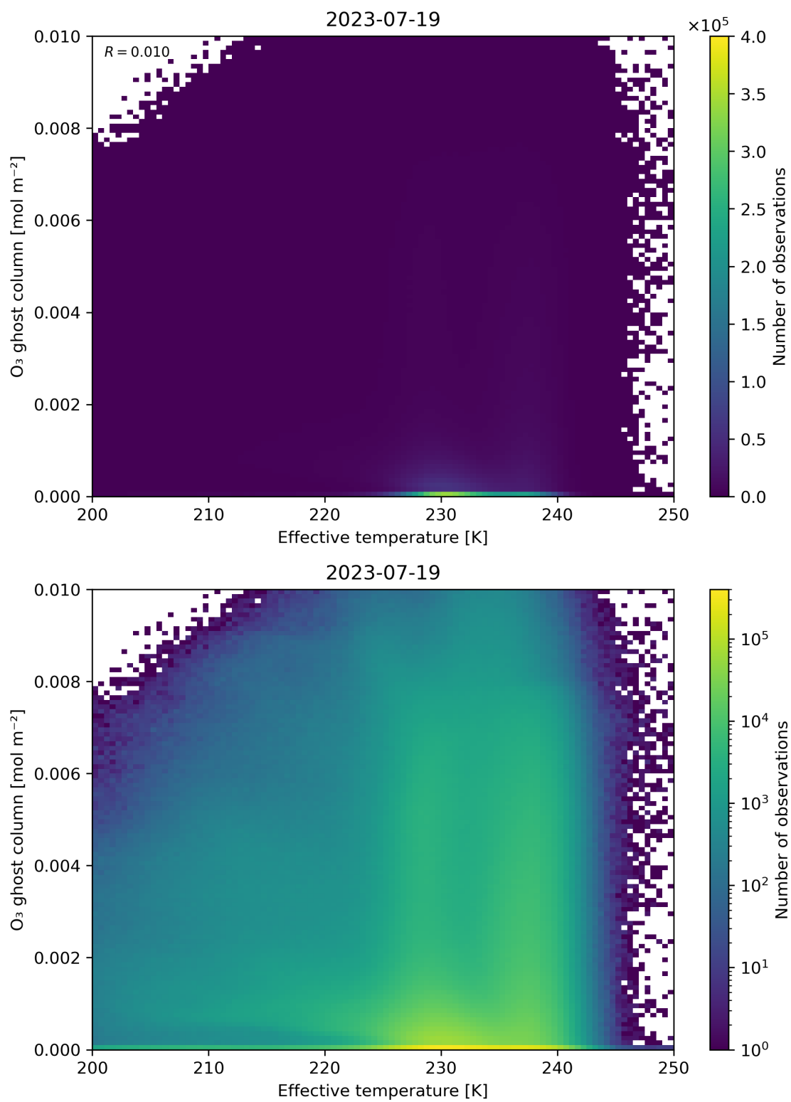
Figure 38: Scatter density plot of “Effective temperature” against “O 3 ghost column” for 2023-07-19 to 2023-07-20.
