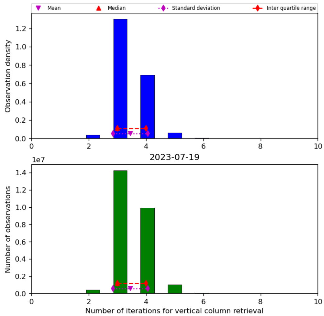
Figure 26: Histogram of “Number of iterations for vertical column retrieval” for 2023-07-19 to 2023-07-20
