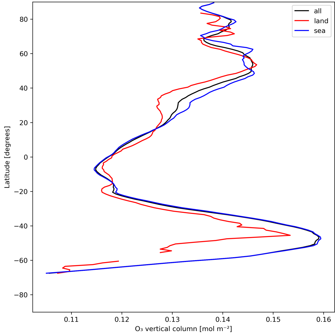
Figure 14: Zonal average of “O 3 vertical column” for 2023-07-19 to 2023-07-20.
