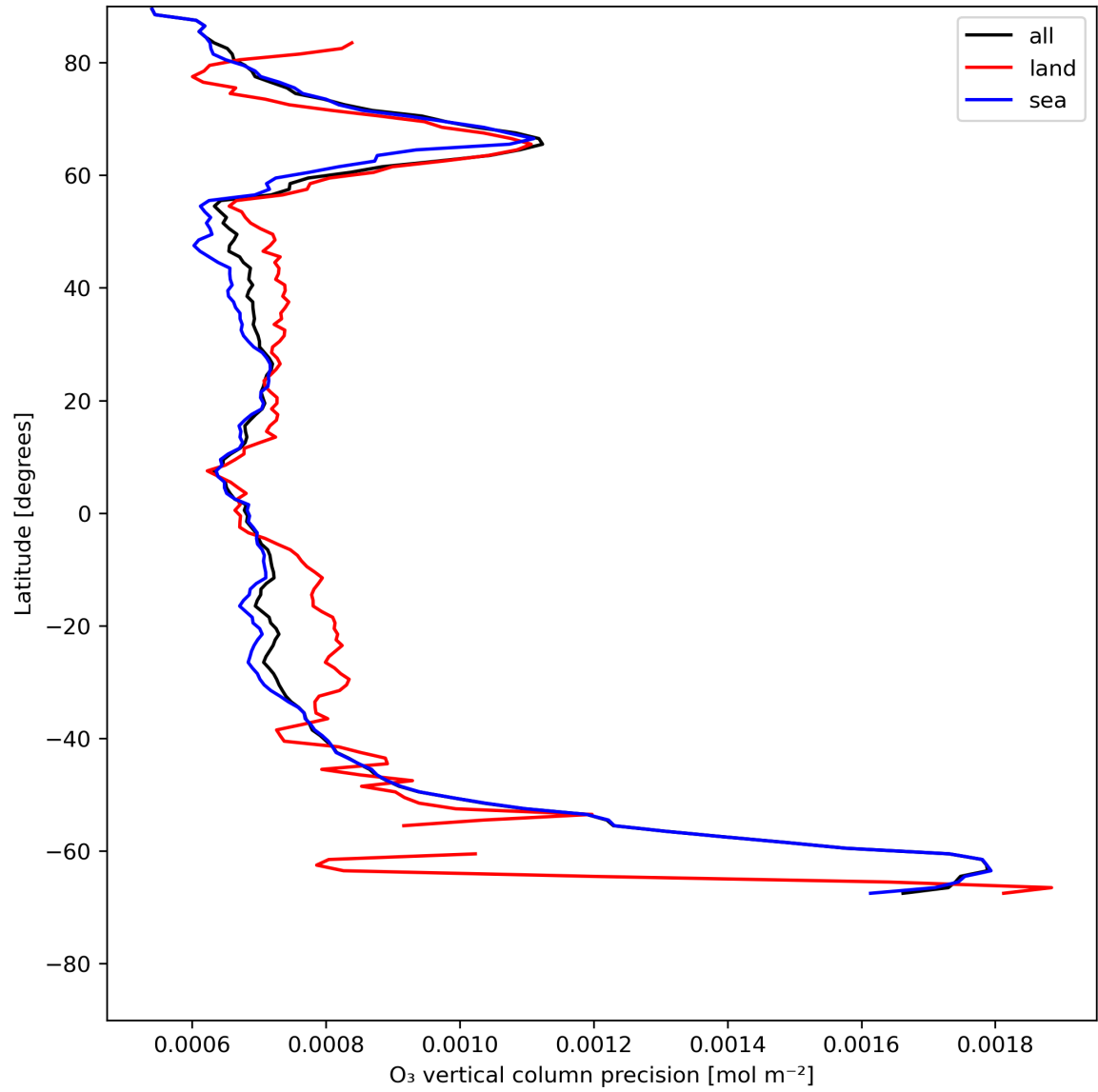
Figure 15: Zonal average of "O 3 vertical column precision" for 2023-07-19 to 2023-07-20.
