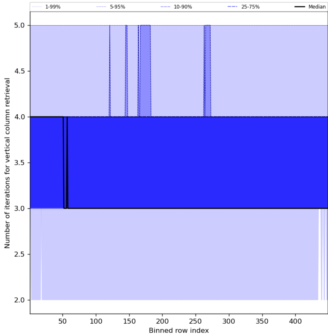
Figure 33: Along track statistics of “Number of iterations for vertical column retrieval” for 2023-07-19 to 2023-07-20
