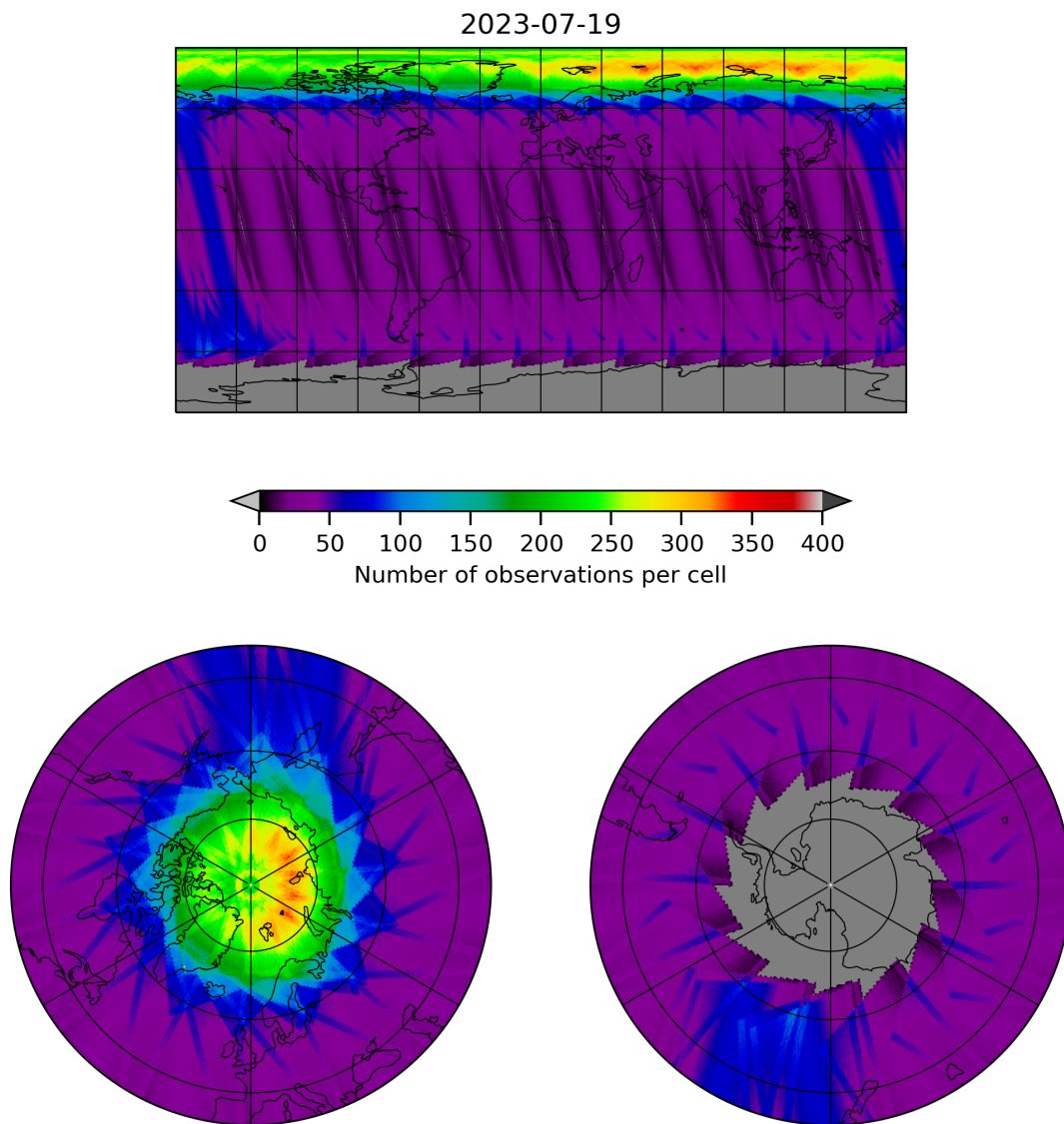
Figure 12: Map of the number of observations for 2023-07-19 to 2023-07-20
