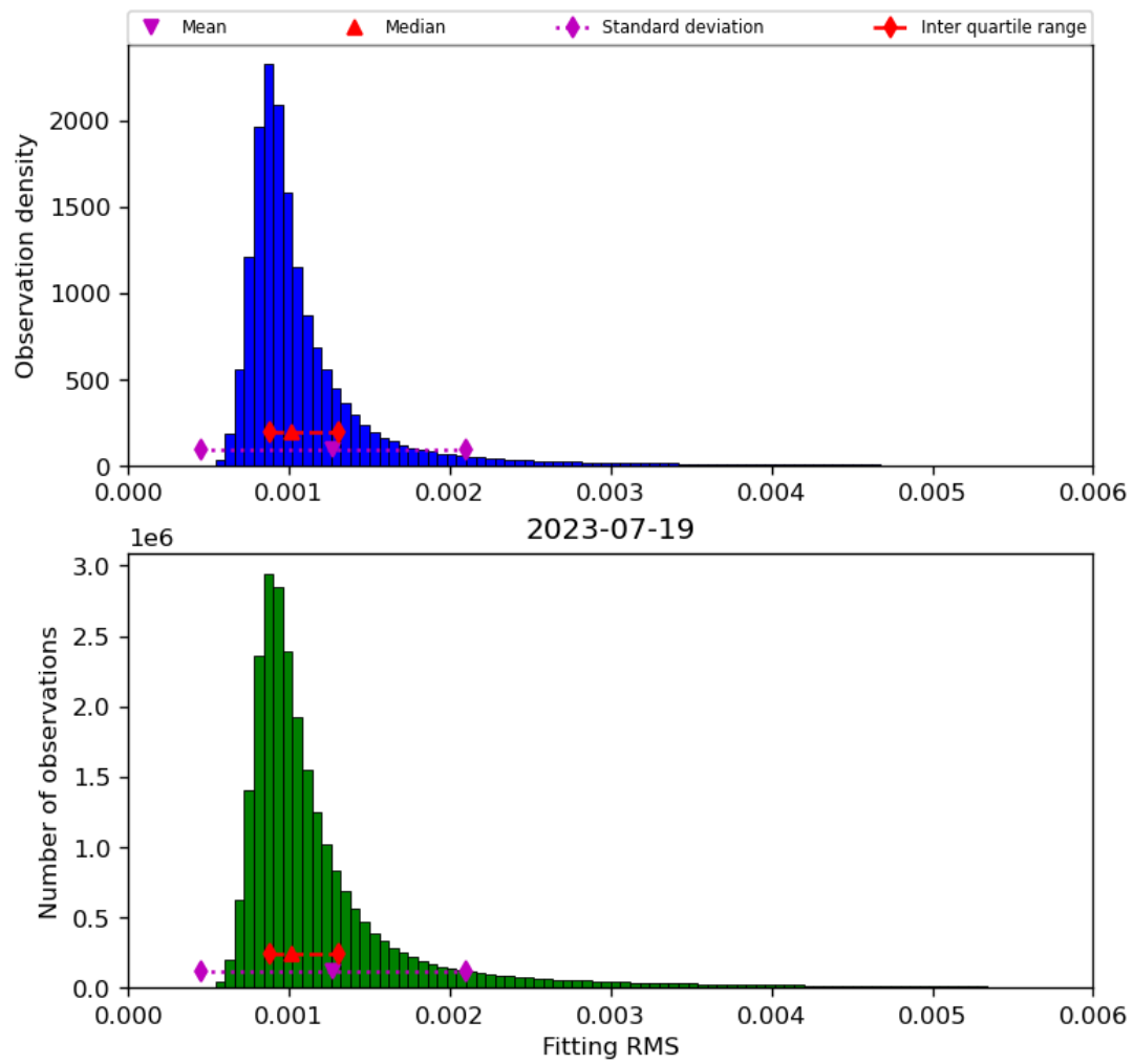
Figure 23: Histogram of “Fitting RMS” for 2023-07-19 to 2023-07-20
