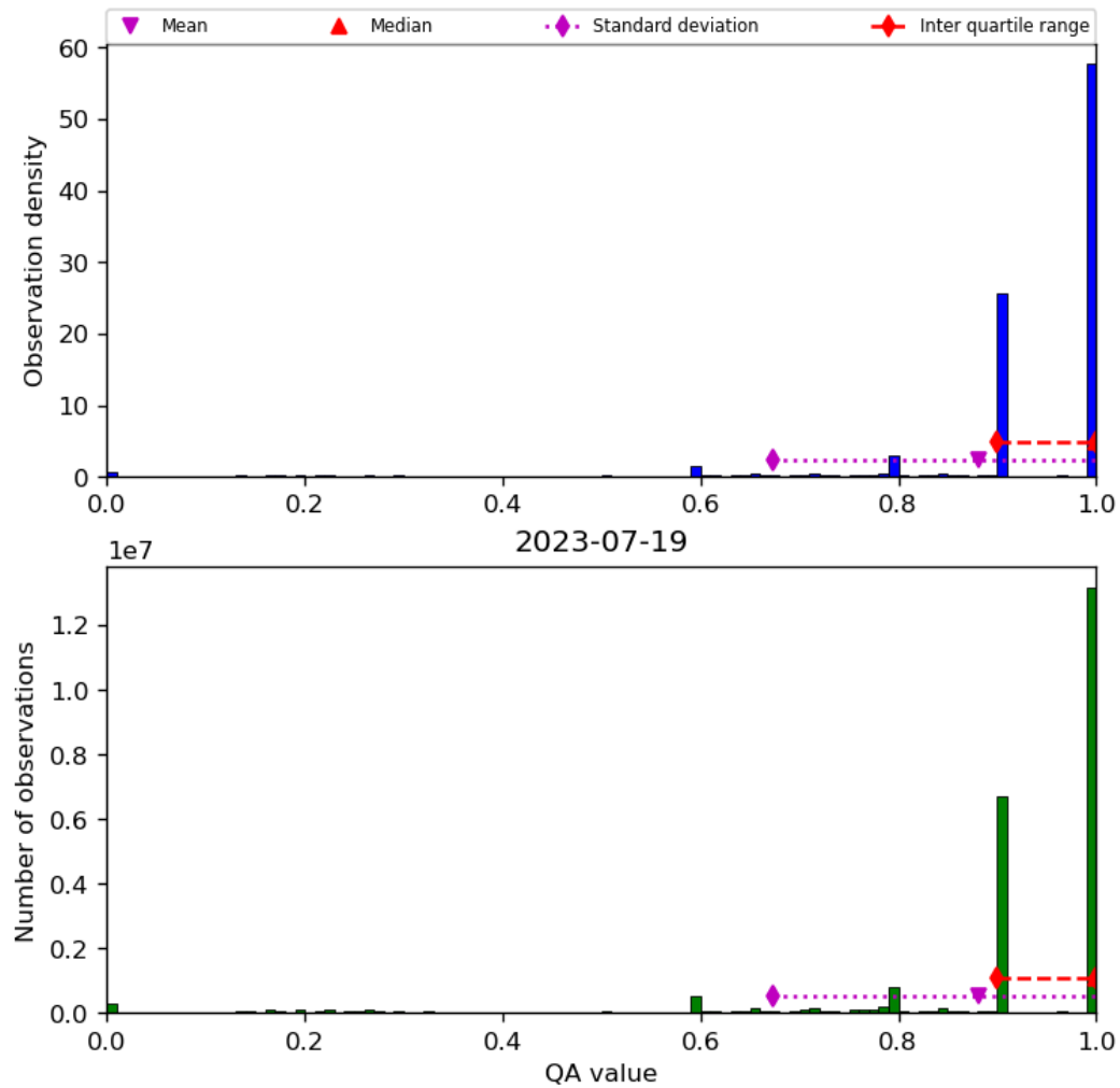
Figure 20: Histogram of “QA value” for 2023-07-19 to 2023-07-20
