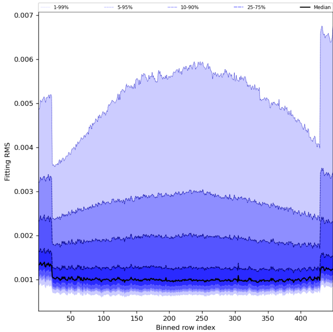
Figure 30: Along track statistics of “Fitting RMS” for 2023-07-19 to 2023-07-20
