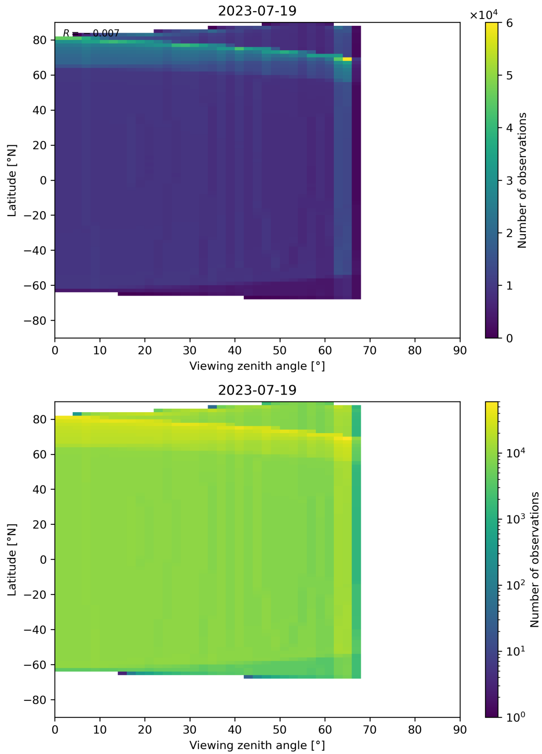
Figure 49: Scatter density plot of “Viewing zenith angle” against “Latitude” for 2023-07-19 to 2023-07-20.
