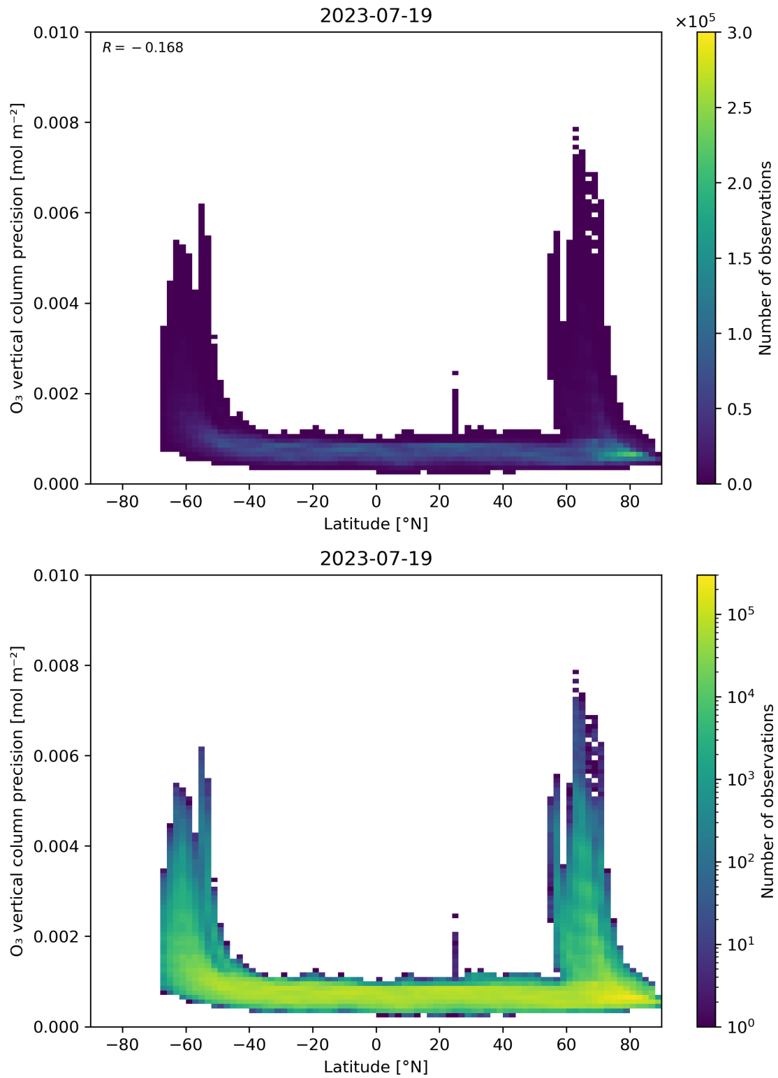
Figure 37: Scatter density plot of “Latitude” against “O 3 vertical column precision” for 2023-07-19 to 2023-07-20.
