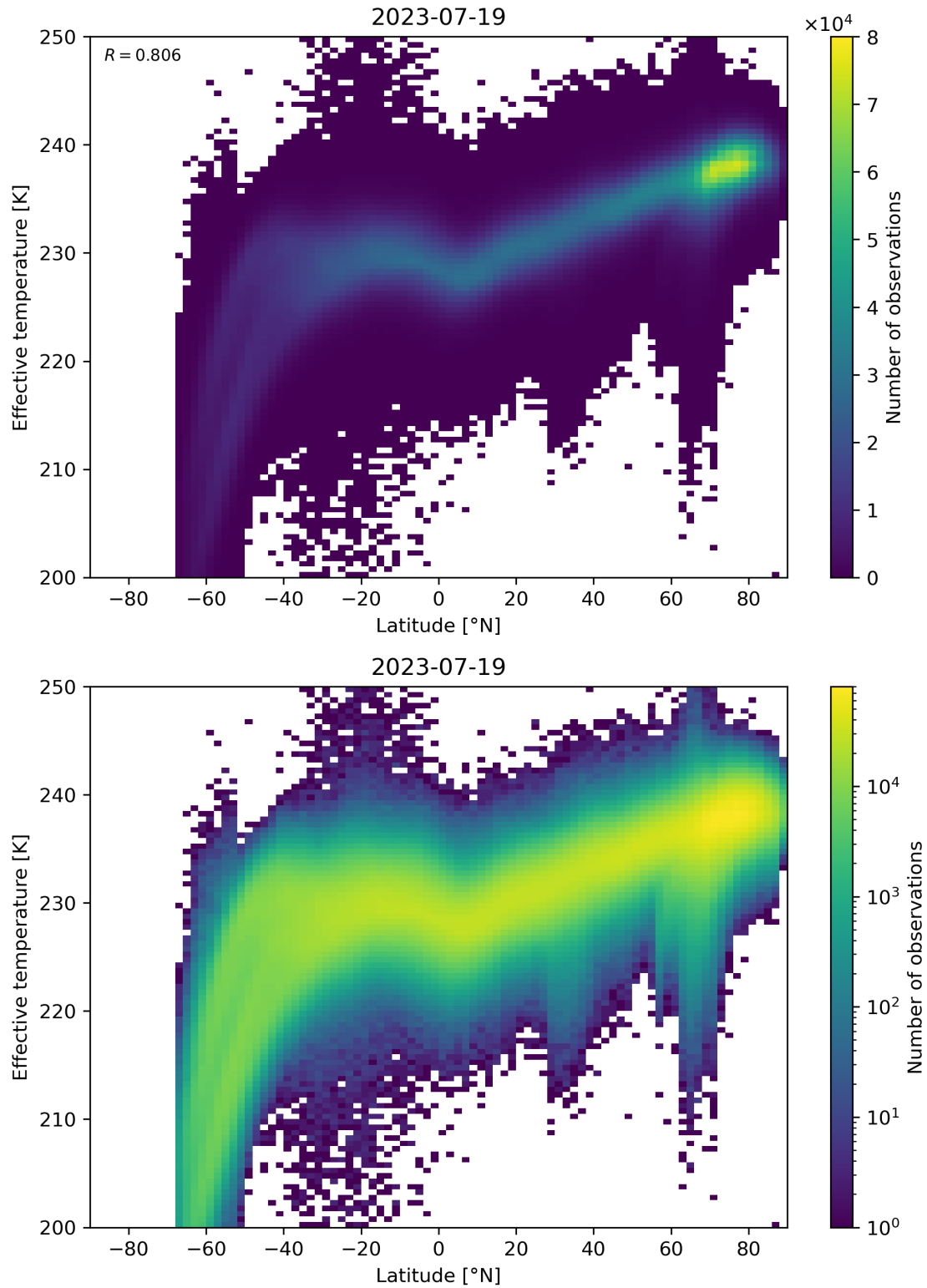
Figure 34: Scatter density plot of “Latitude” against “Effective temperature” for 2023-07-19 to 2023-07-20.
