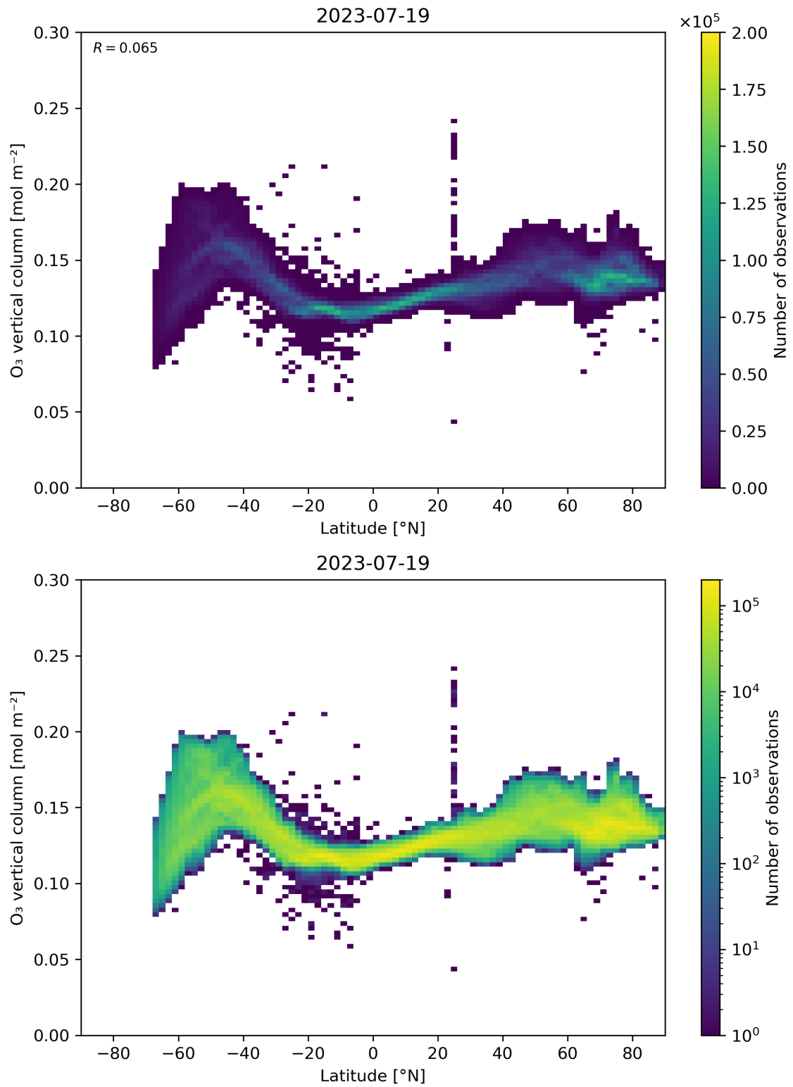
Figure 36: Scatter density plot of “Latitude” against “O 3 vertical column” for 2023-07-19 to 2023-07-20.
