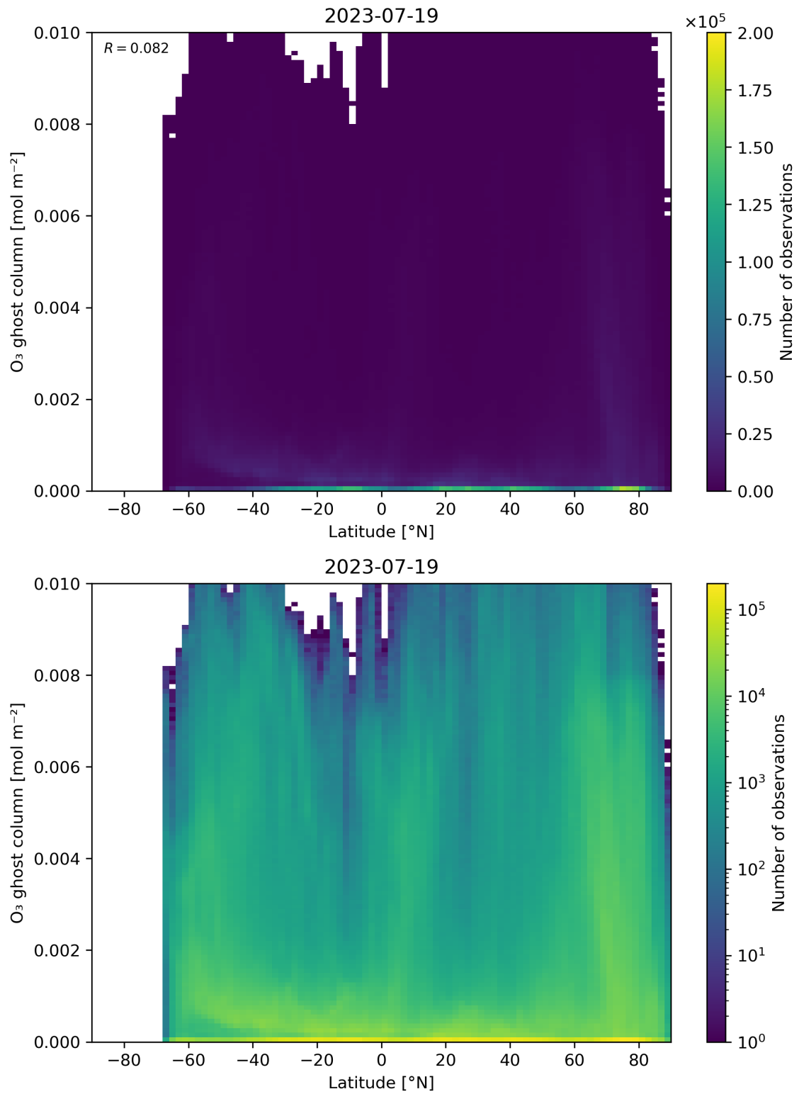
Figure 35: Scatter density plot of “Latitude” against “O 3 ghost column” for 2023-07-19 to 2023-07-20.
