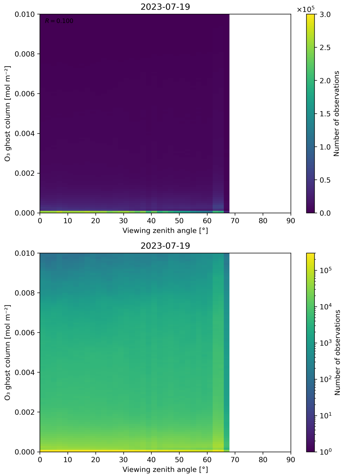
Figure 51: Scatter density plot of “Viewing zenith angle” against “O 3 ghost column” for 2023-07-19 to 2023-07-20.
