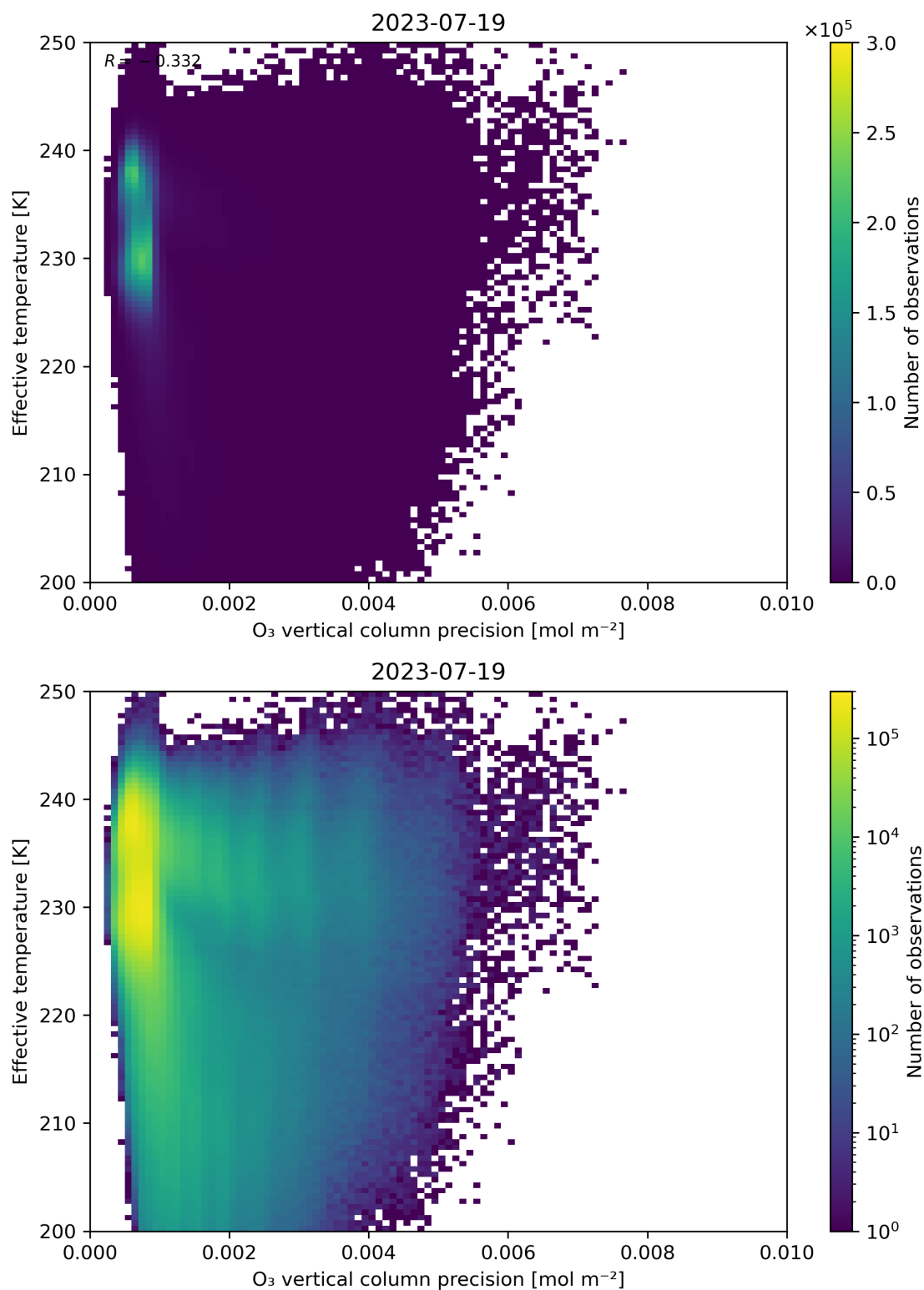
Figure 42: Scatter density plot of “O 3 vertical column precision” against “Effective temperature” for 2023-07-19 to 2023-07-20.
