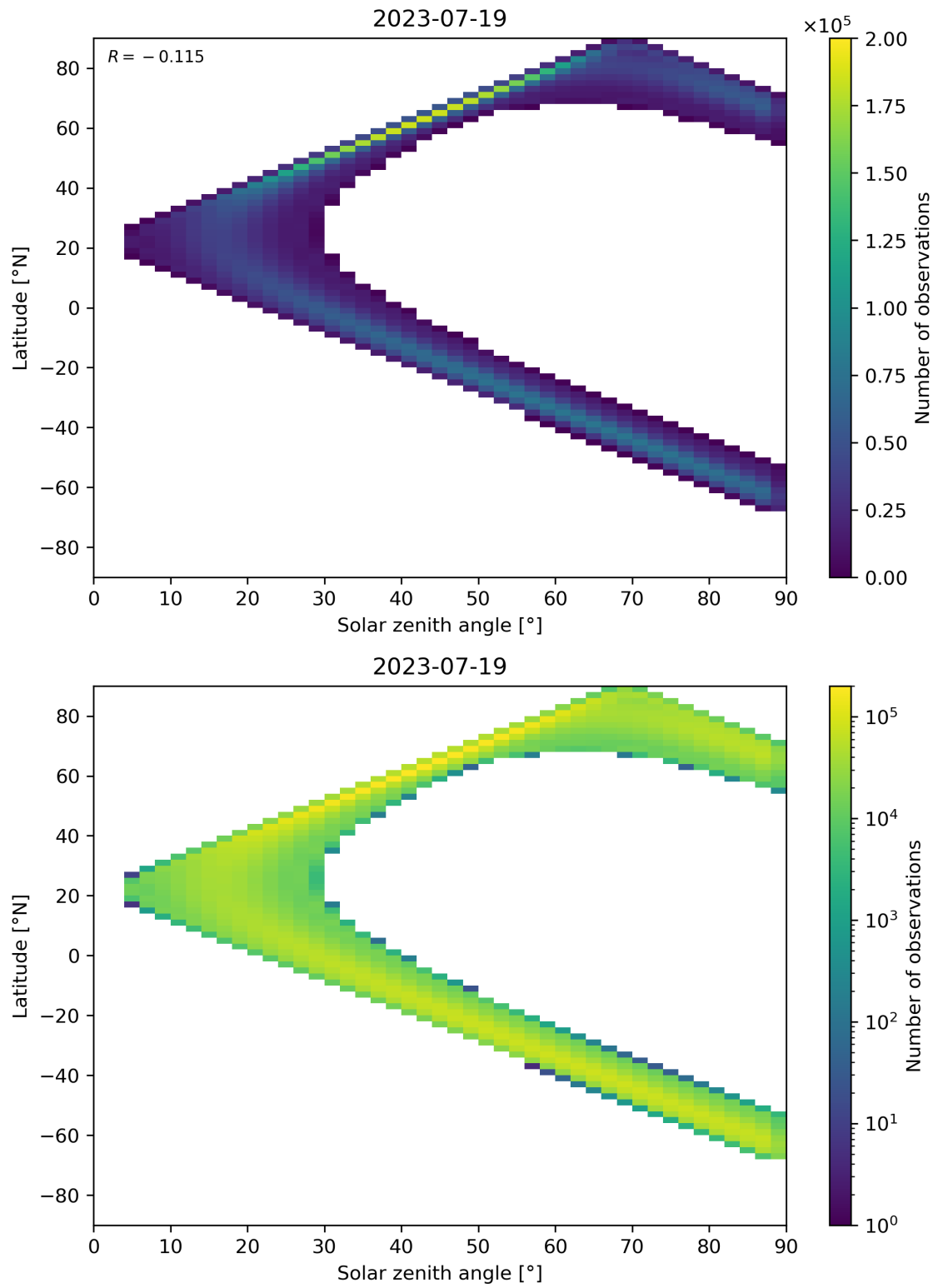
Figure 44: Scatter density plot of “Solar zenith angle” against “Latitude” for 2023-07-19 to 2023-07-20.
