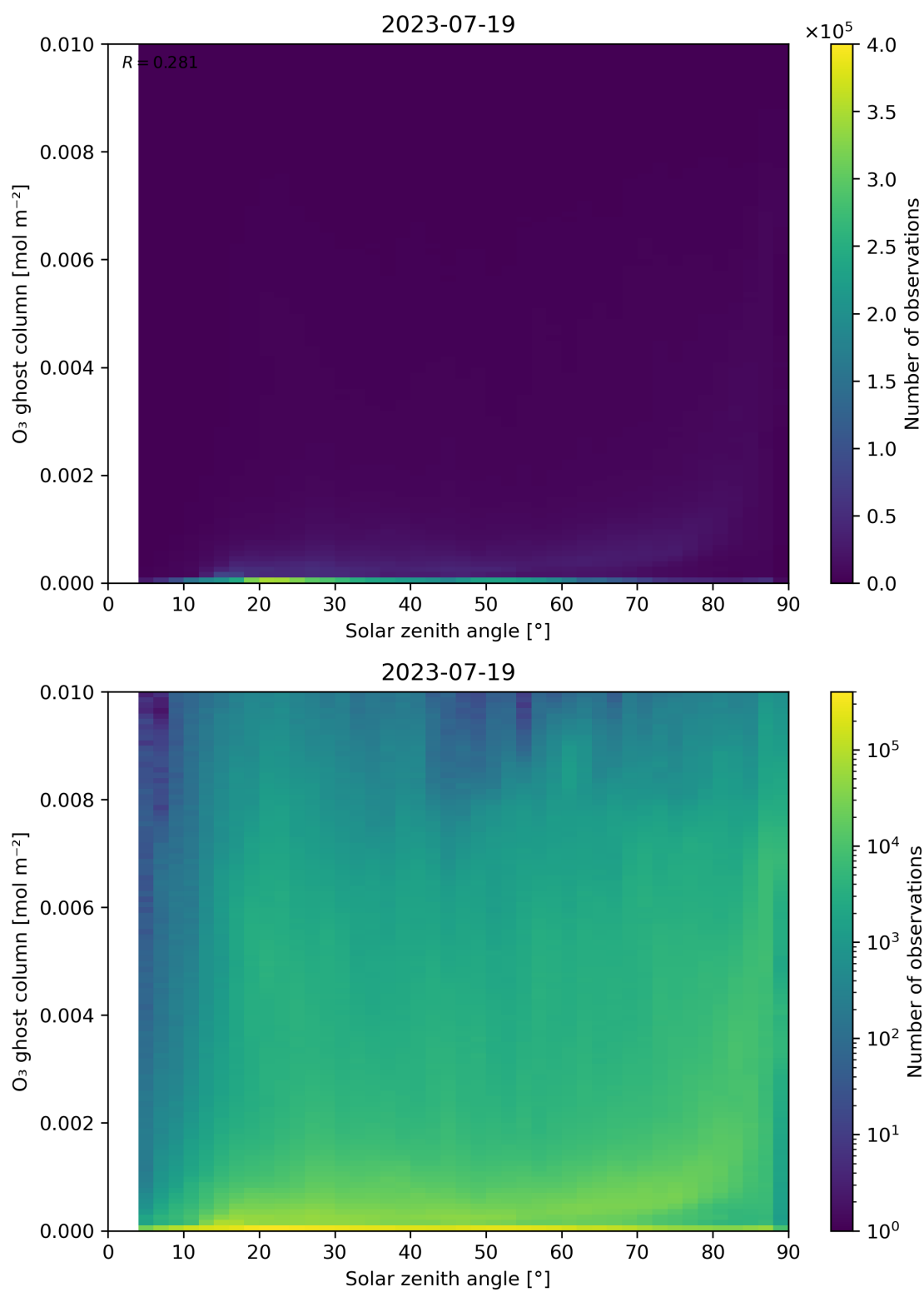
Figure 46: Scatter density plot of “Solar zenith angle” against “O 3 ghost column” for 2023-07-19 to 2023-07-20.
