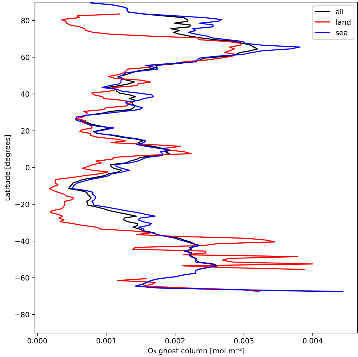
Figure 18: Zonal average of “O 3 ghost column” for 2023-07-19 to 2023-07-20.
