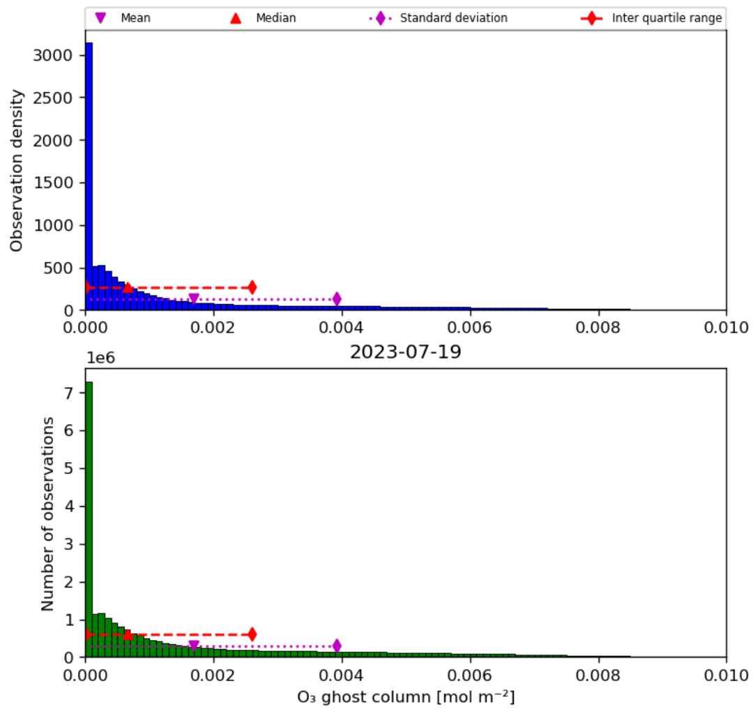
Figure 25: Histogram of “O 3 ghost column” for 2023-07-19 to 2023-07-20
