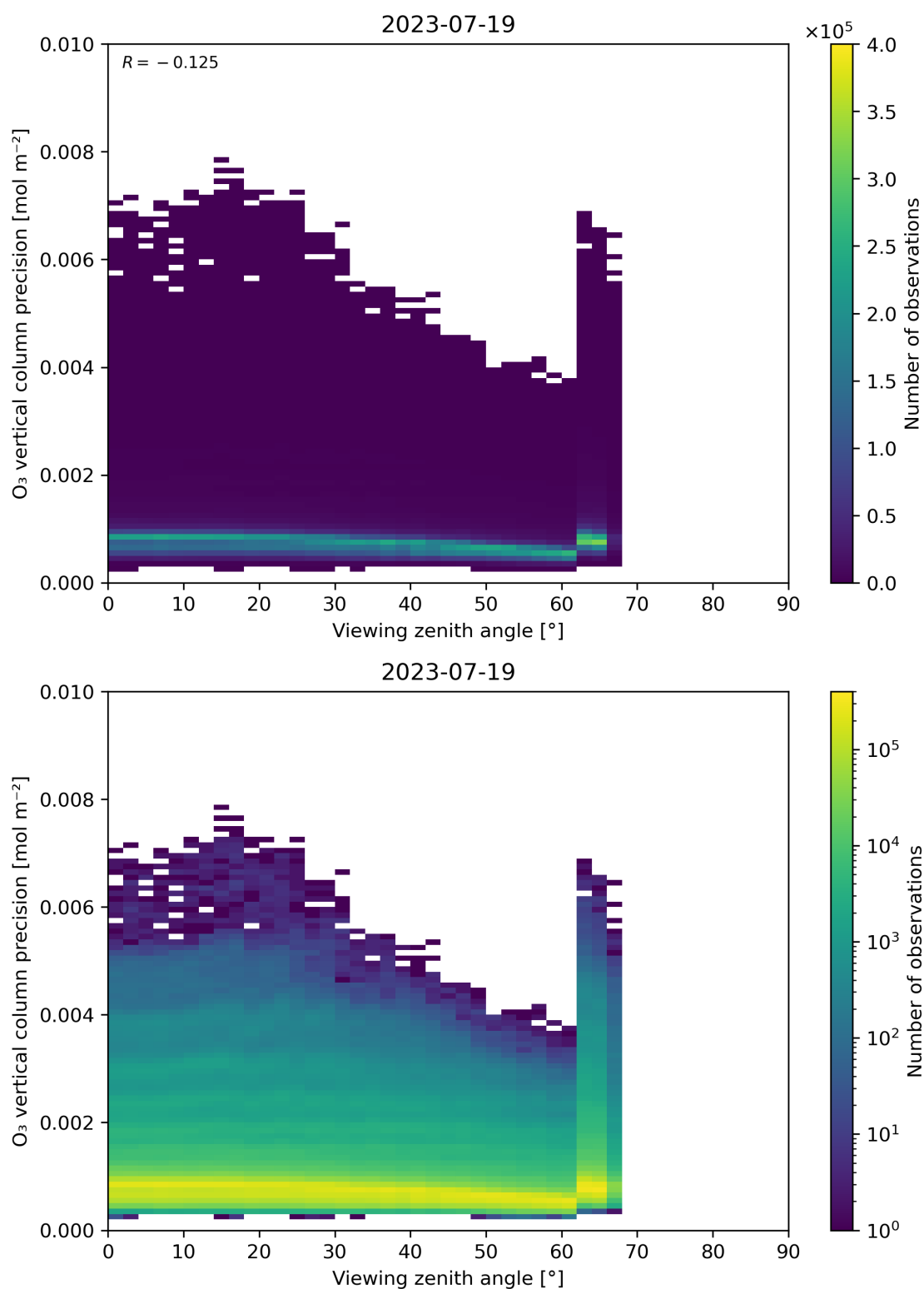
Figure 53: Scatter density plot of “Viewing zenith angle” against “O 3 vertical column precision” for 2023-07-19 to 2023-07-20.
