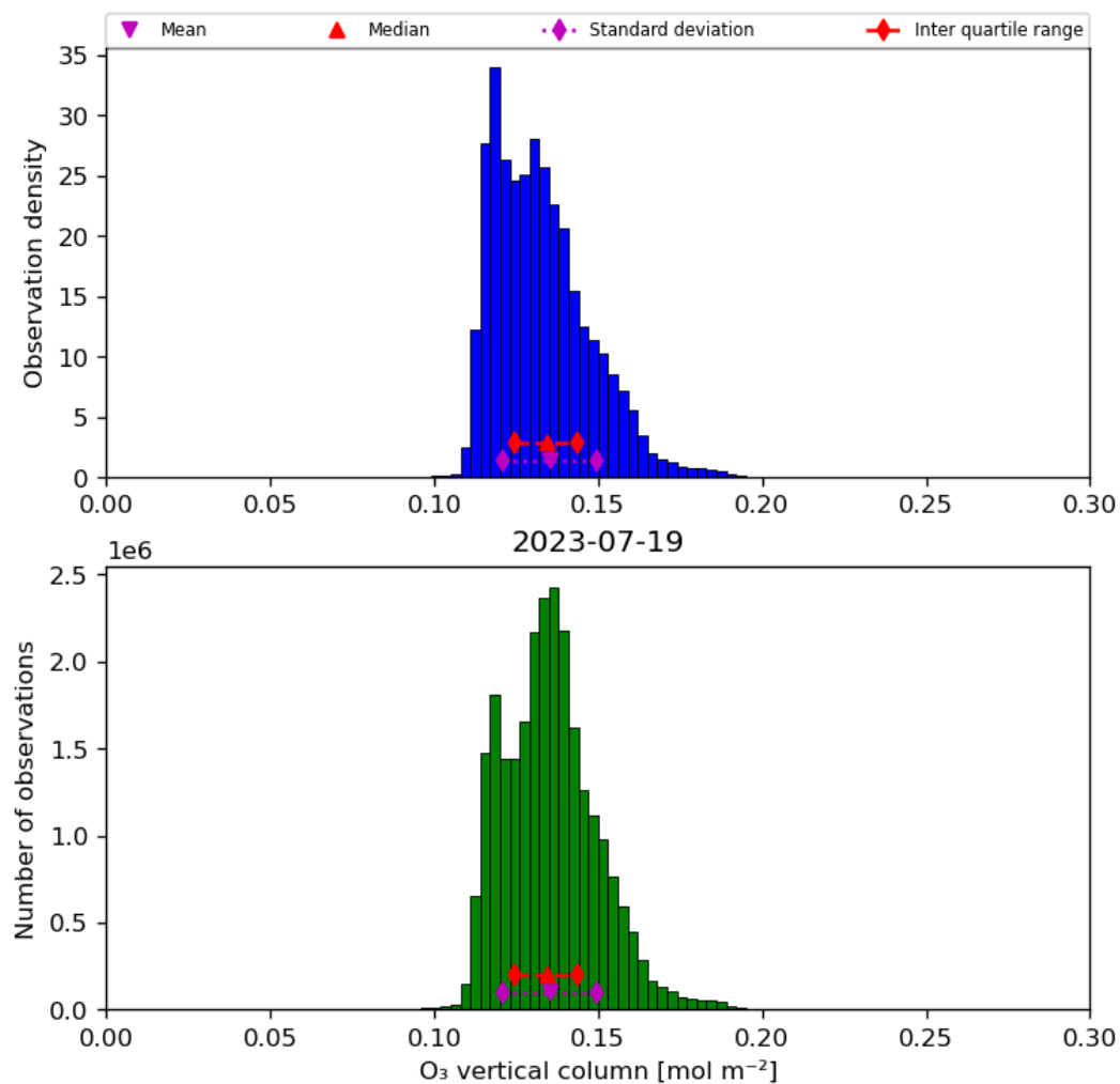
Figure 21: Histogram of “O 3 vertical column” for 2023-07-19 to 2023-07-20
