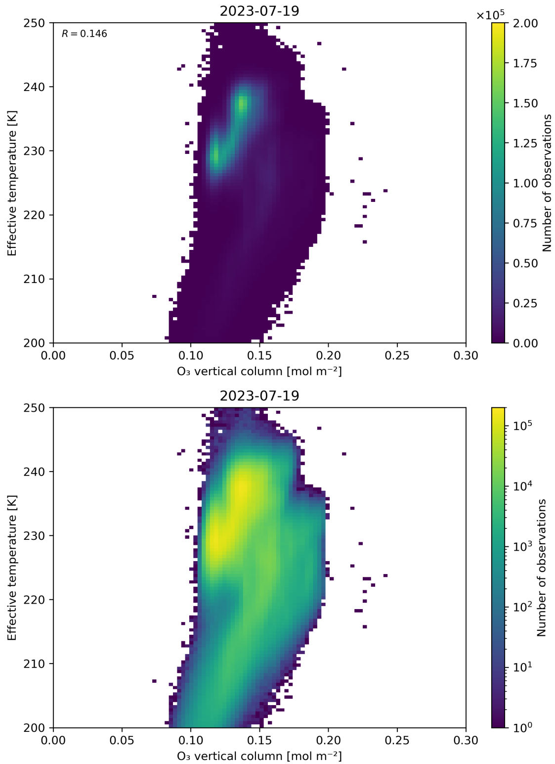
Figure 39: Scatter density plot of “O 3 vertical column” against “Effective temperature” for 2023-07-19 to 2023-07-20.
