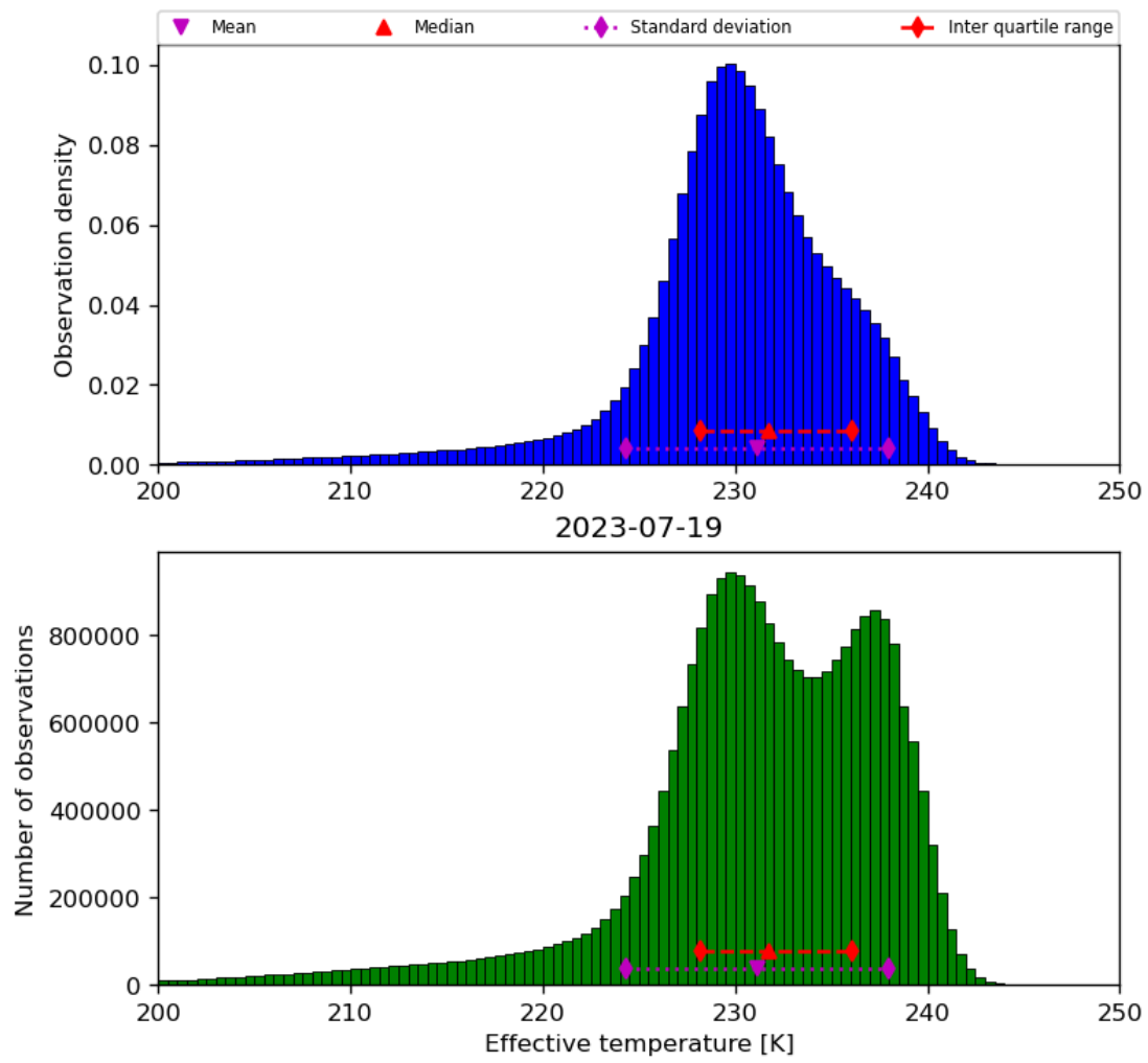
Figure 24: Histogram of “Effective temperature” for 2023-07-19 to 2023-07-20
