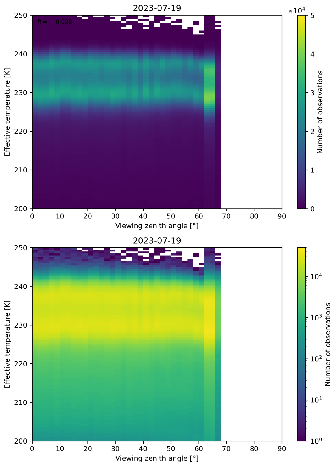
Figure 50: Scatter density plot of “Viewing zenith angle” against “Effective temperature” for 2023-07-19 to 2023-07-20.
