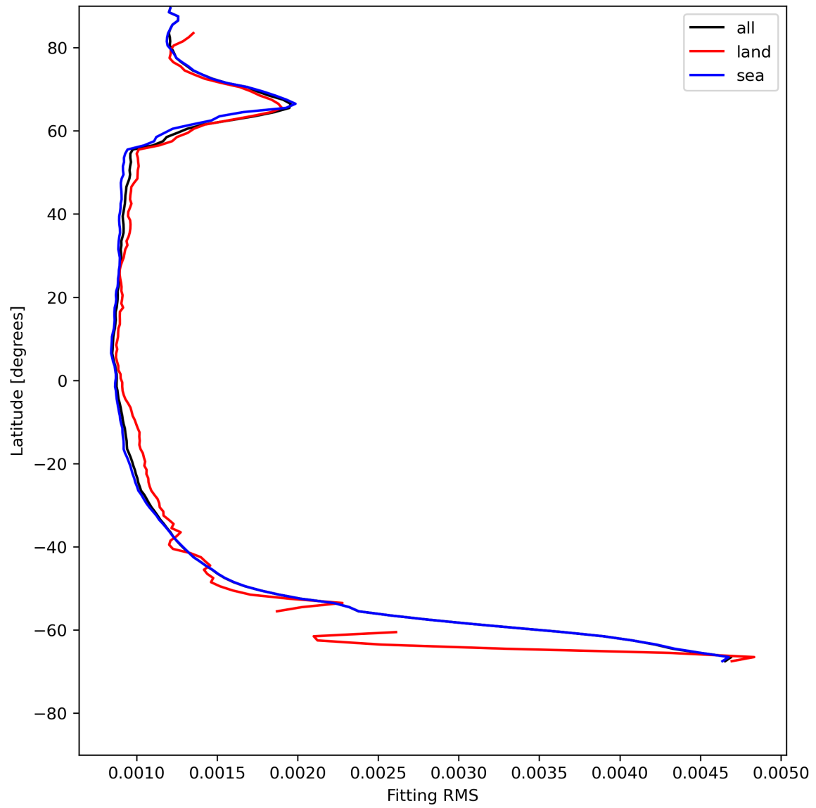
Figure 16: Zonal average of “Fitting RMS” for 2023-07-19 to 2023-07-20.
