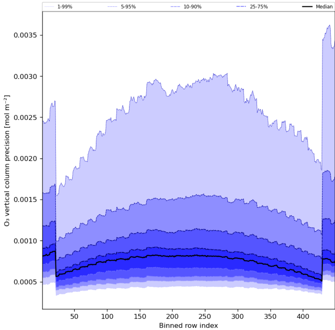
Figure 29: Along track statistics of “O 3 vertical column precision” for 2023-07-19 to 2023-07-20
