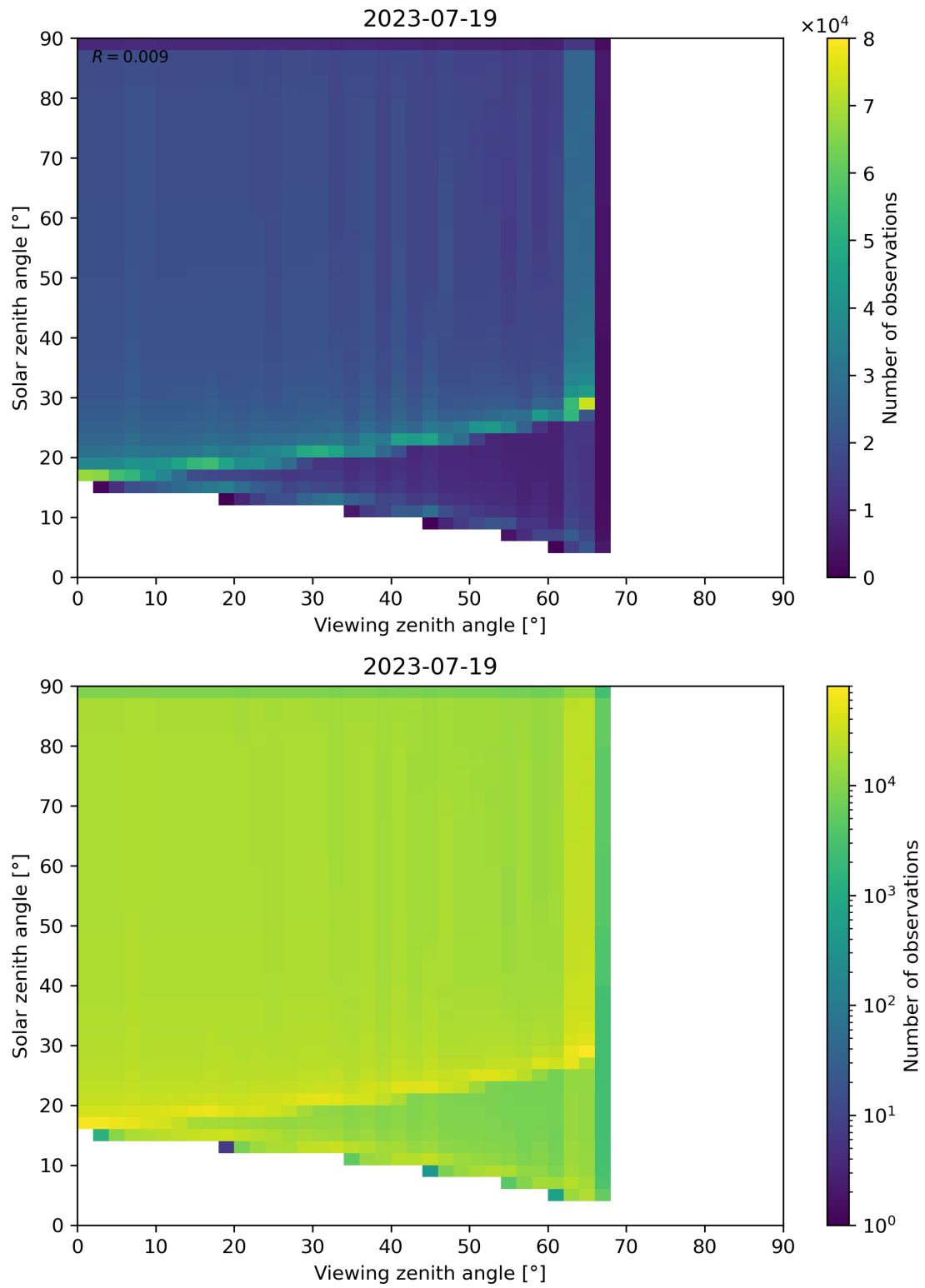
Figure 54: Scatter density plot of “Viewing zenith angle” against “Solar zenith angle” for 2023-07-19 to 2023-07-20.
