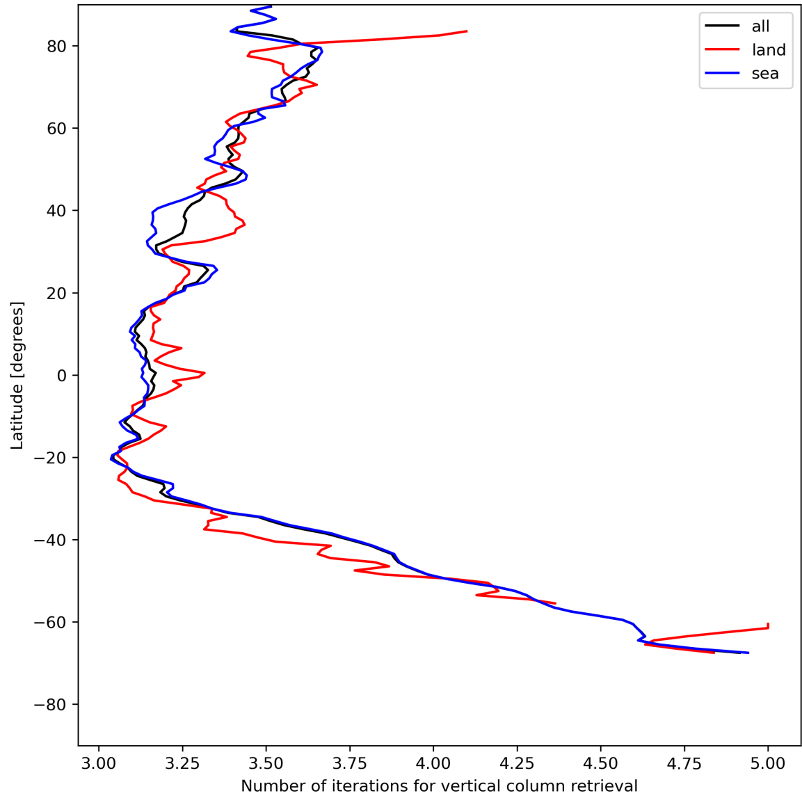
Figure 19: Zonal average of “Number of iterations for vertical column retrieval” for 2023-07-19 to 2023-07-20.
