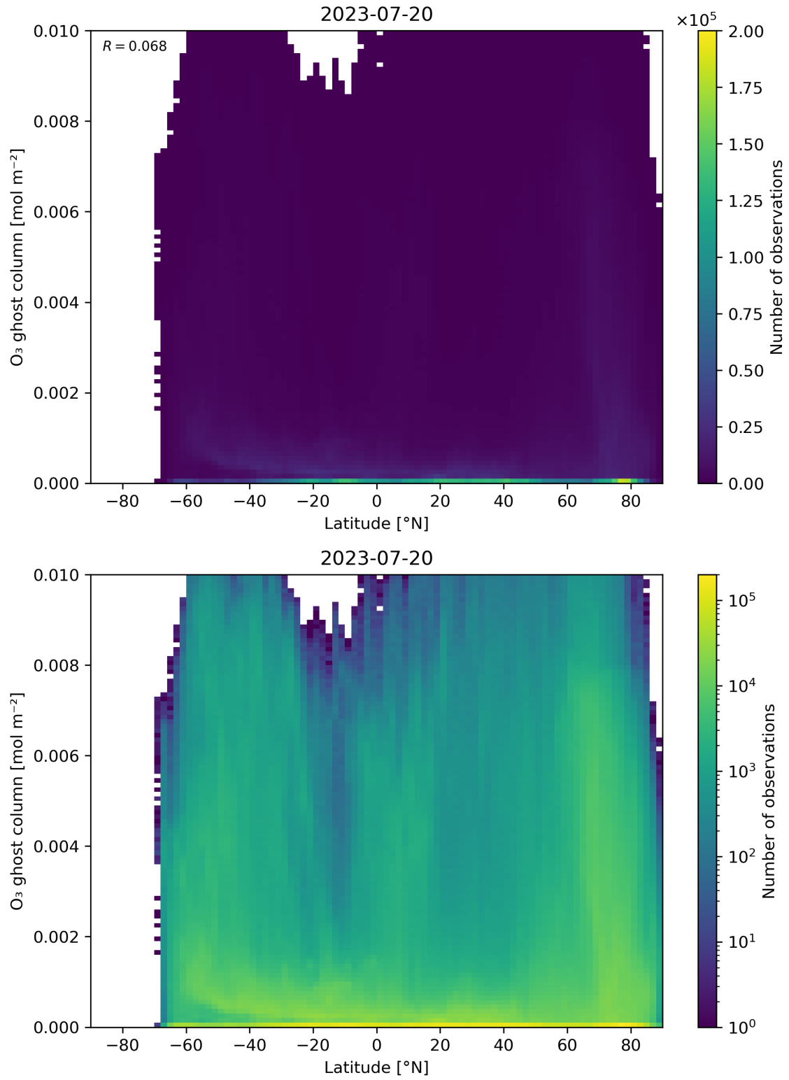
Figure 35: Scatter density plot of “Latitude” against “O 3 ghost column” for 2023-07-19 to 2023-07-21.
