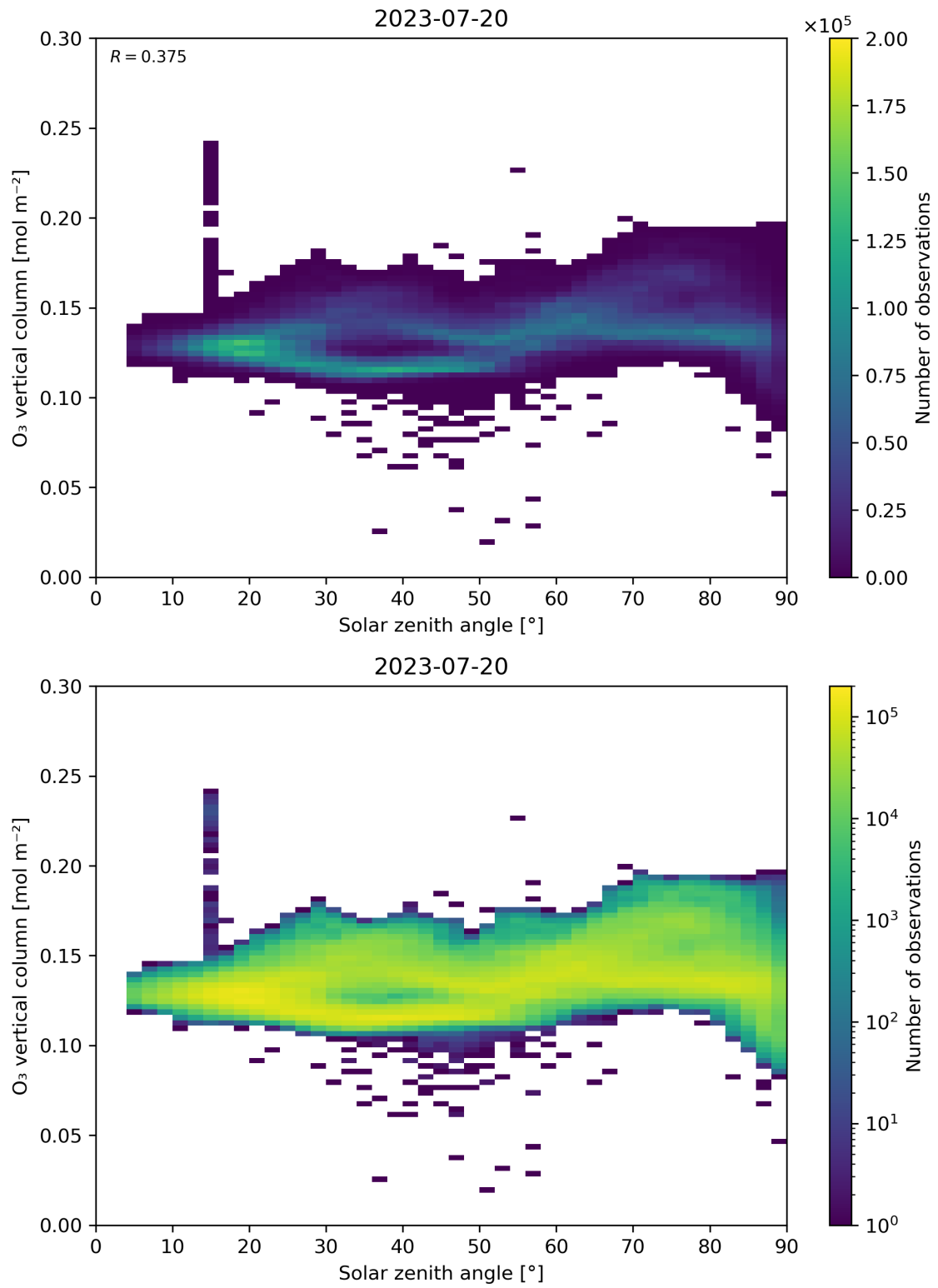
Figure 47: Scatter density plot of “Solar zenith angle” against “O 3 vertical column” for 2023-07-19 to 2023-07-21.
