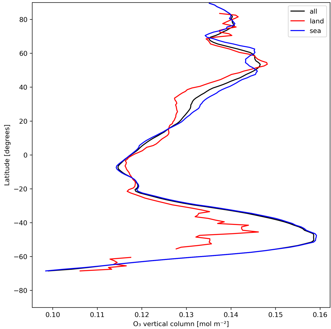
Figure 14: Zonal average of “O 3 vertical column” for 2023-07-19 to 2023-07-21.
