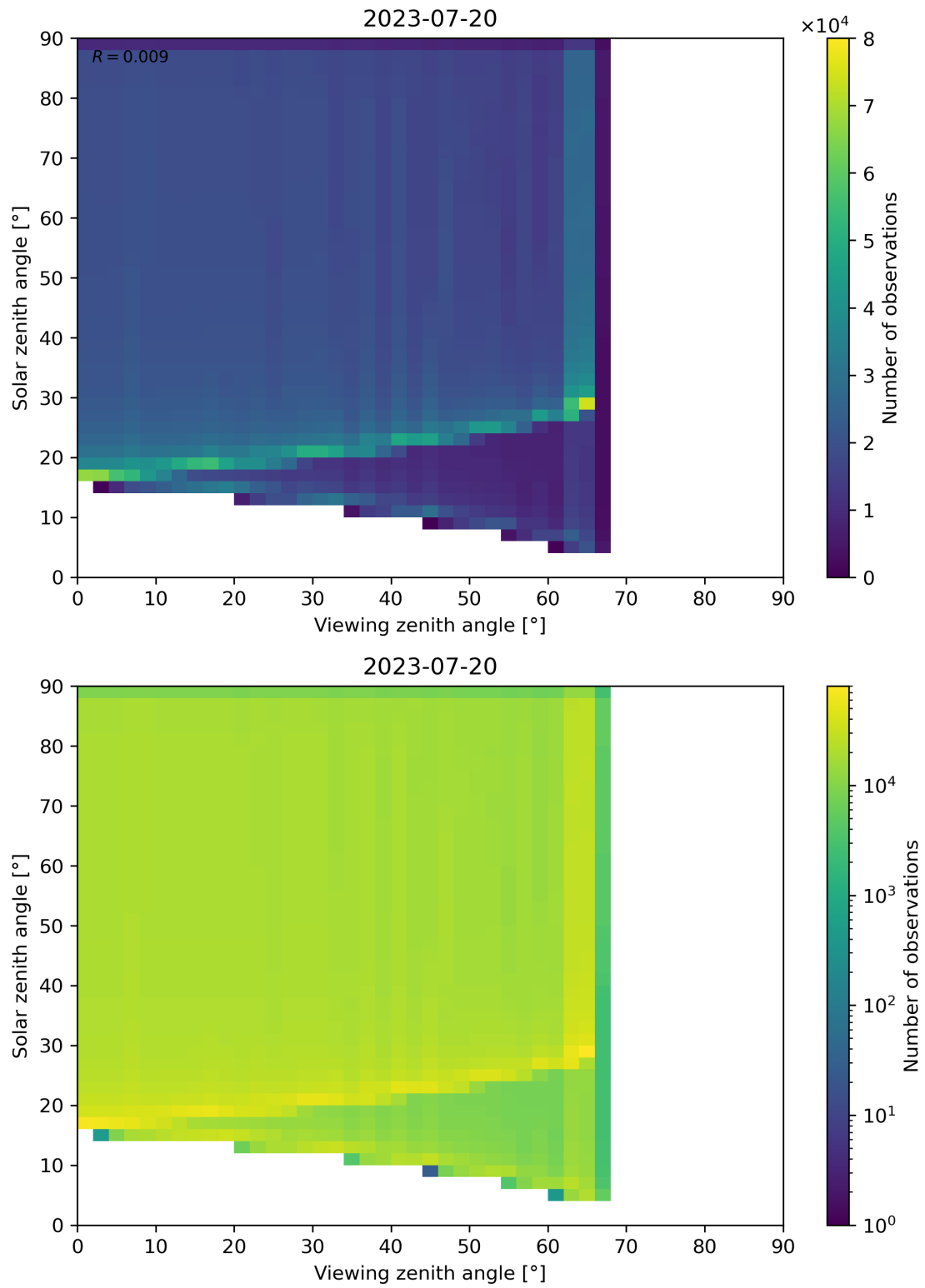
Figure 54: Scatter density plot of “Viewing zenith angle” against “Solar zenith angle” for 2023-07-19 to 2023-07-21.
