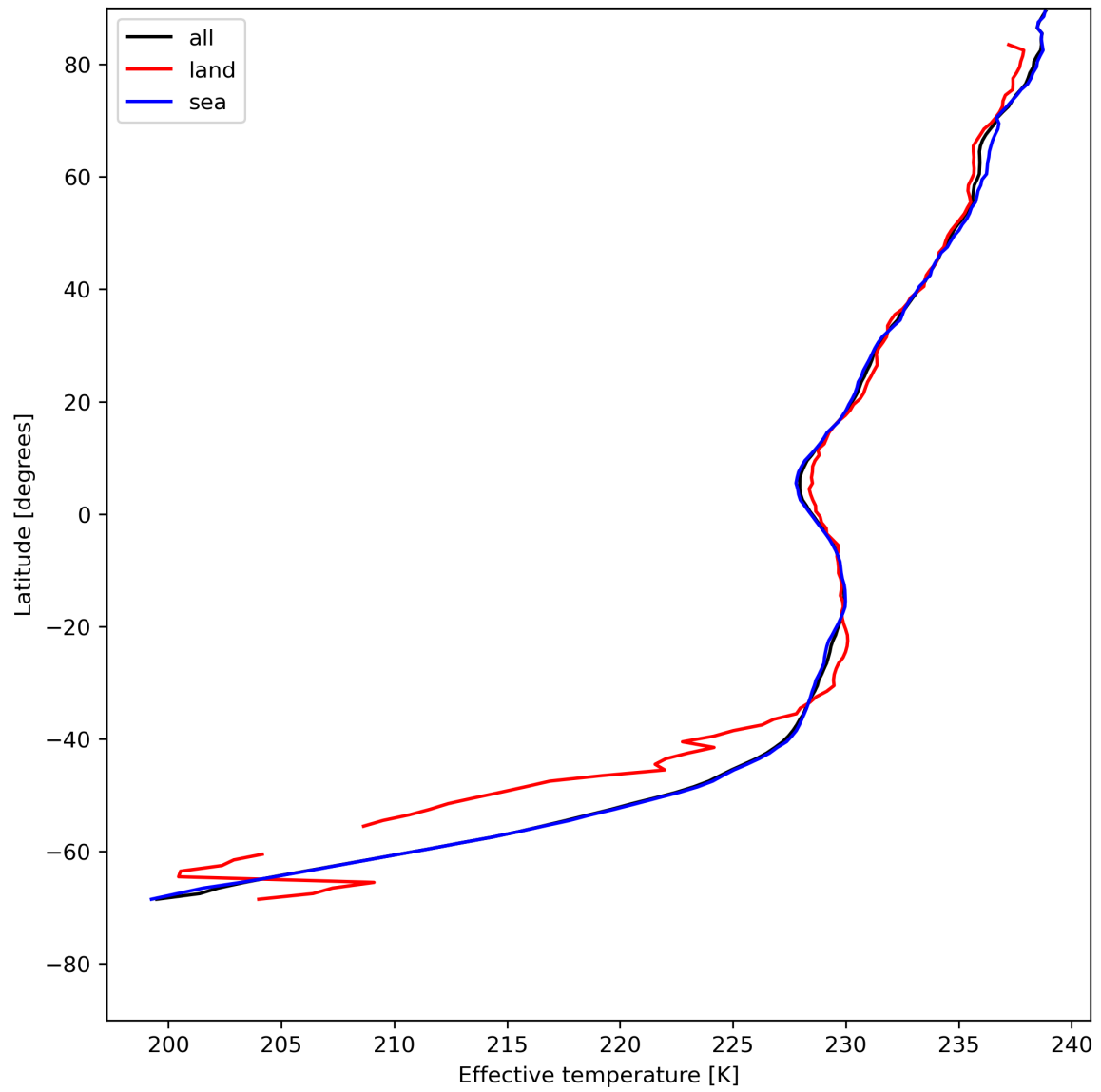
Figure 17: Zonal average of "Effective temperature" for 2023-07-19 to 2023-07-21.
