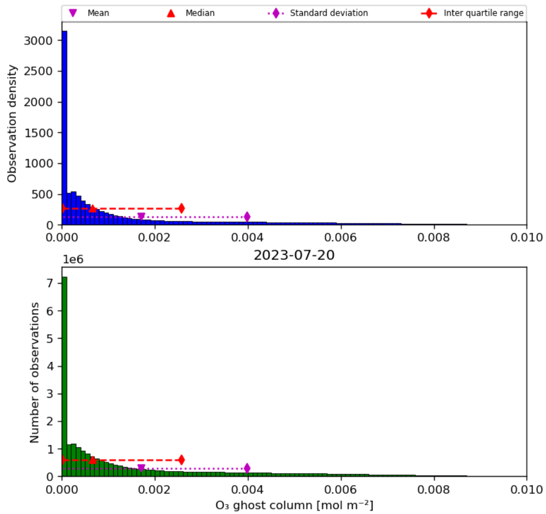
Figure 25: Histogram of “O 3 ghost column” for 2023-07-19 to 2023-07-21
