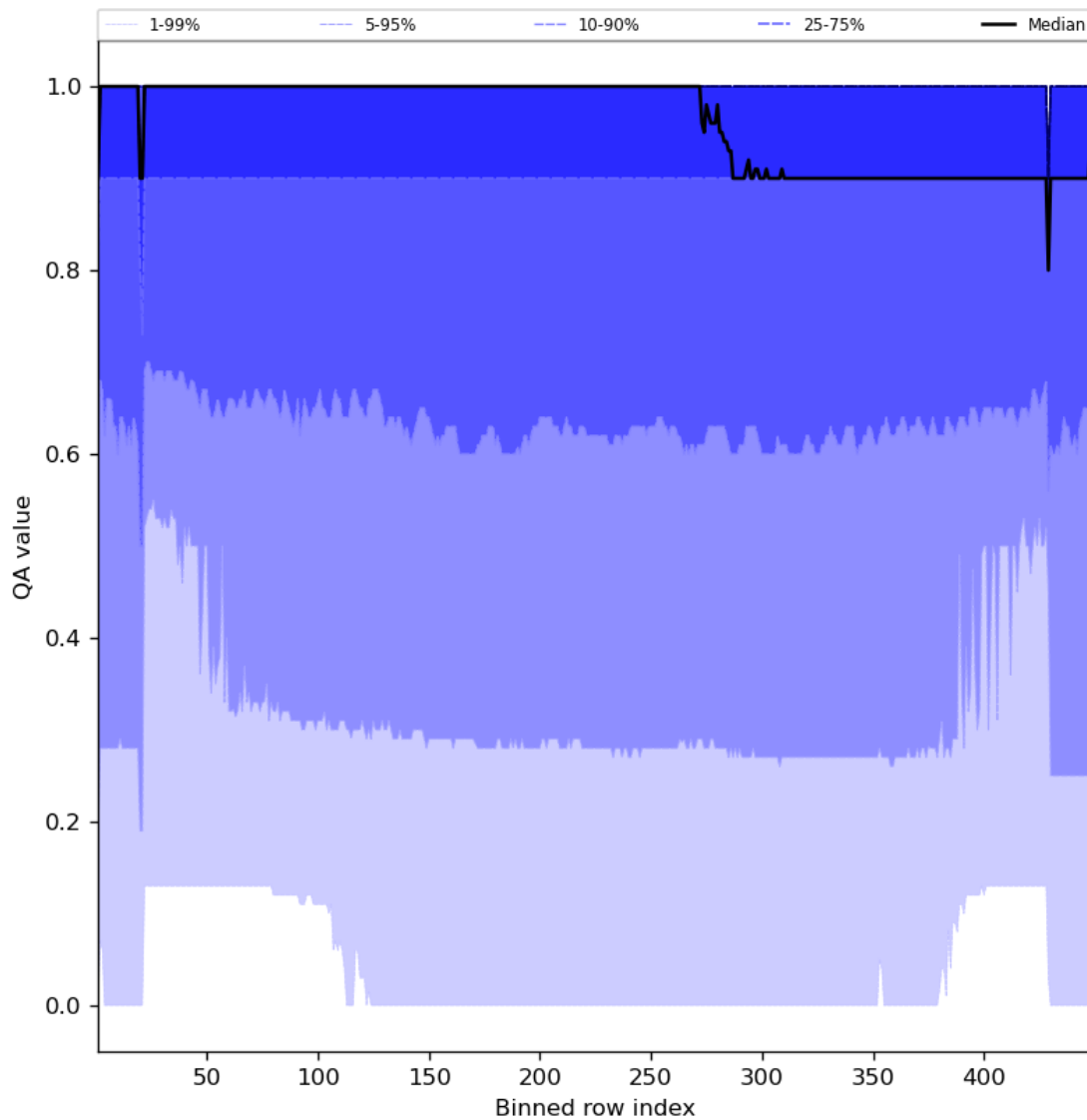
Figure 27: Along track statistics of “QA value” for 2023-07-19 to 2023-07-21
