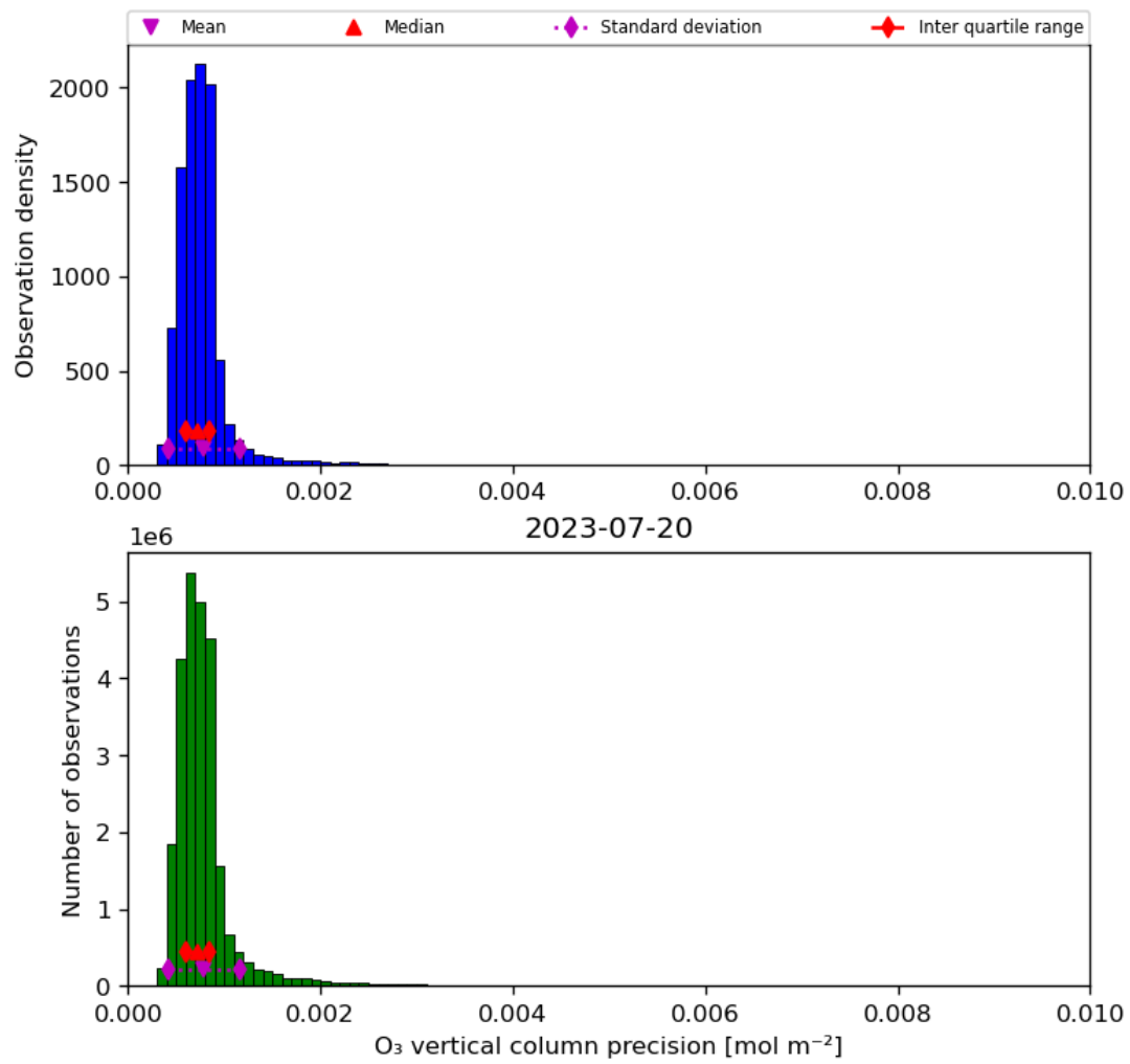
Figure 22: Histogram of “O 3 vertical column precision” for 2023-07-19 to 2023-07-21
