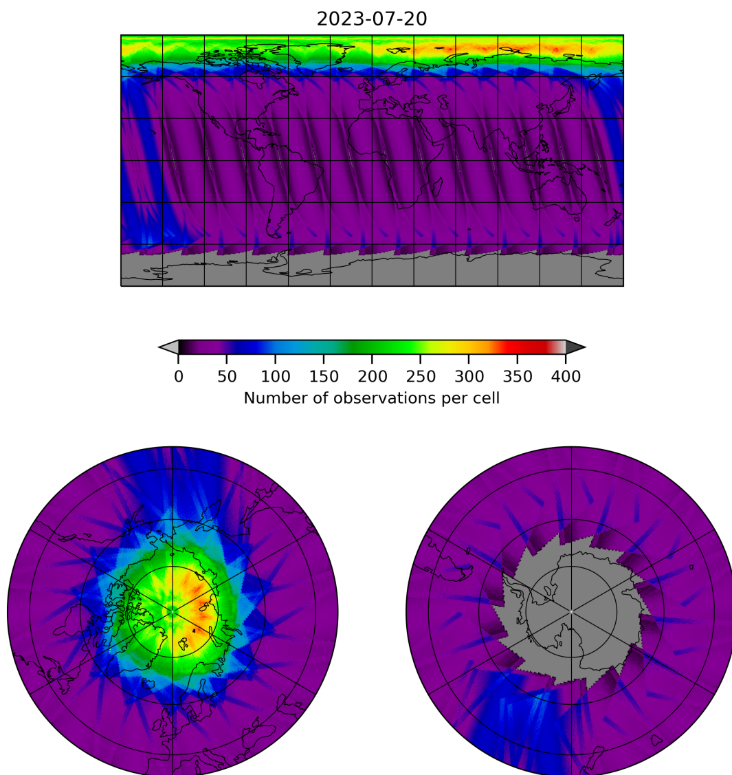
Figure 12: Map of the number of observations for 2023-07-19 to 2023-07-21
