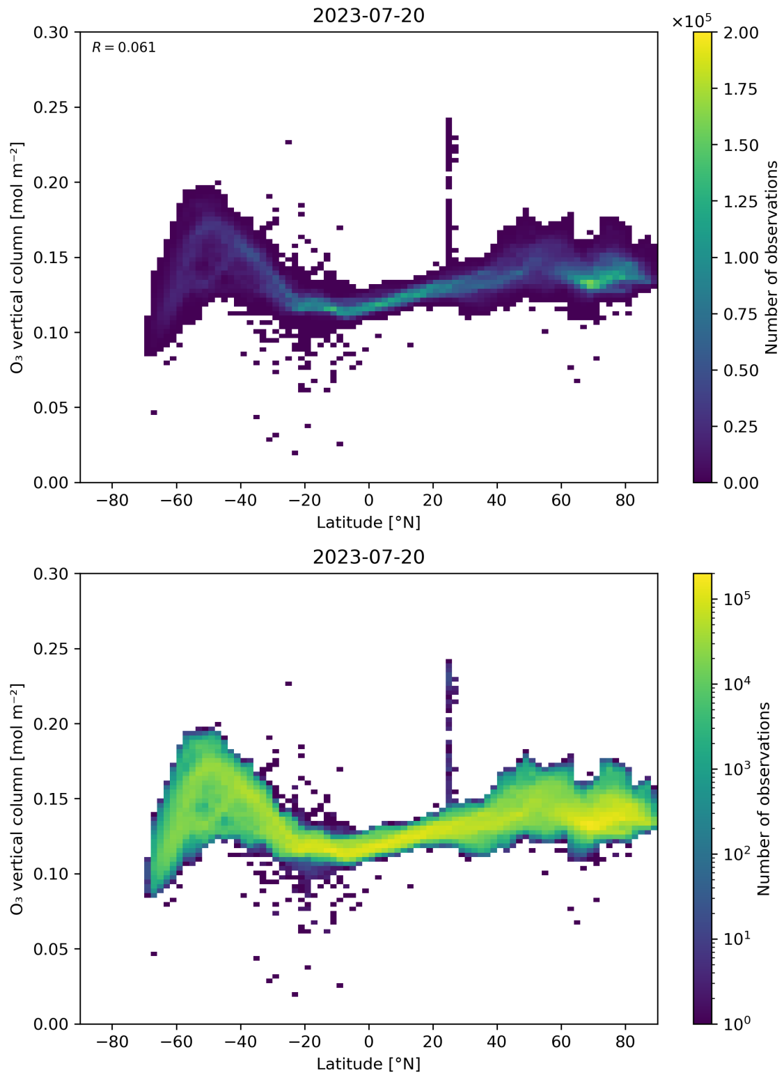
Figure 36: Scatter density plot of “Latitude” against “O 3 vertical column” for 2023-07-19 to 2023-07-21.
