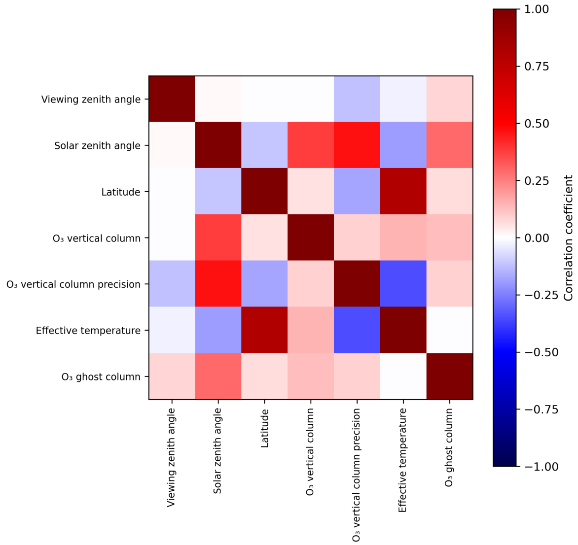
Figure 2: Map of correlation matrix for 2023-07-19 to 2023-07-21.
