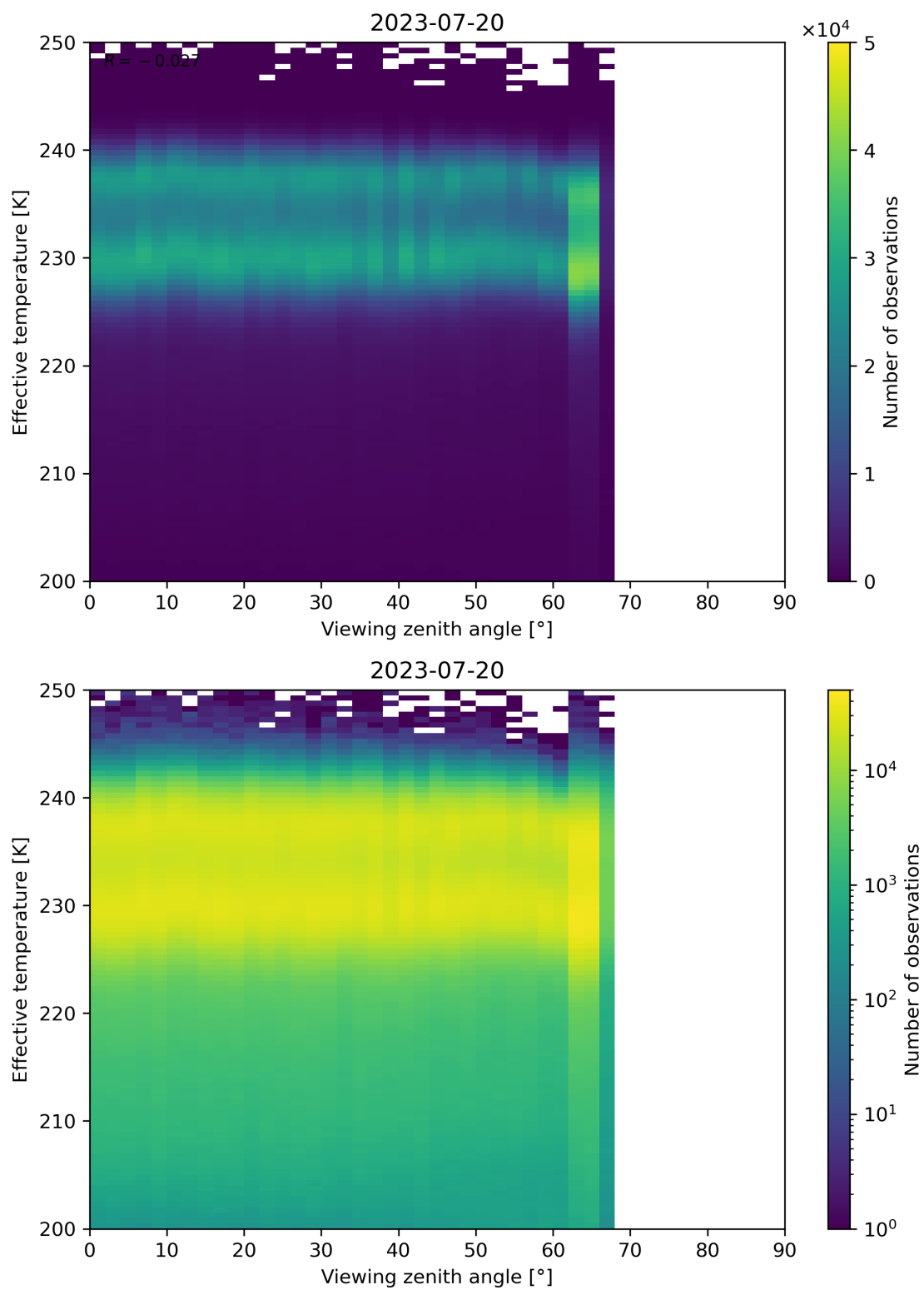
Figure 50: Scatter density plot of “Viewing zenith angle” against “Effective temperature” for 2023-07-19 to 2023-07-21.
