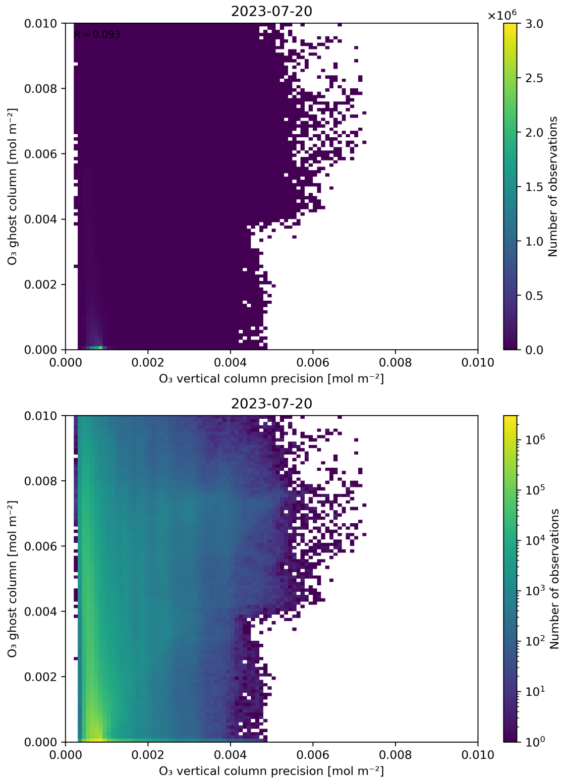
Figure 43: Scatter density plot of “ \text{O}_3 vertical column precision” against “ \text{O}_3 ghost column” for 2023-07-19 to 2023-07-21.
