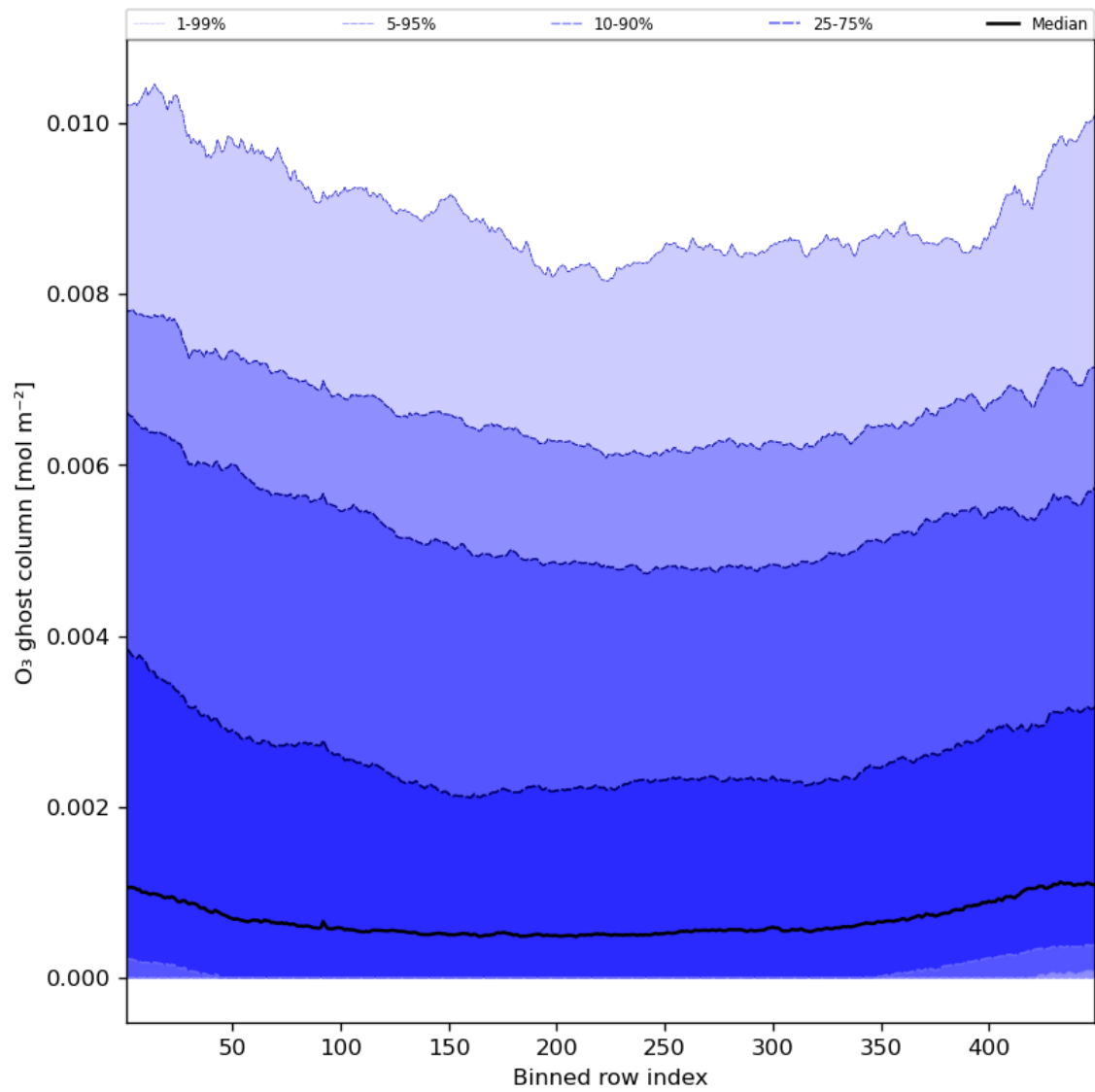
Figure 32: Along track statistics of “O 3 ghost column” for 2023-07-19 to 2023-07-21
