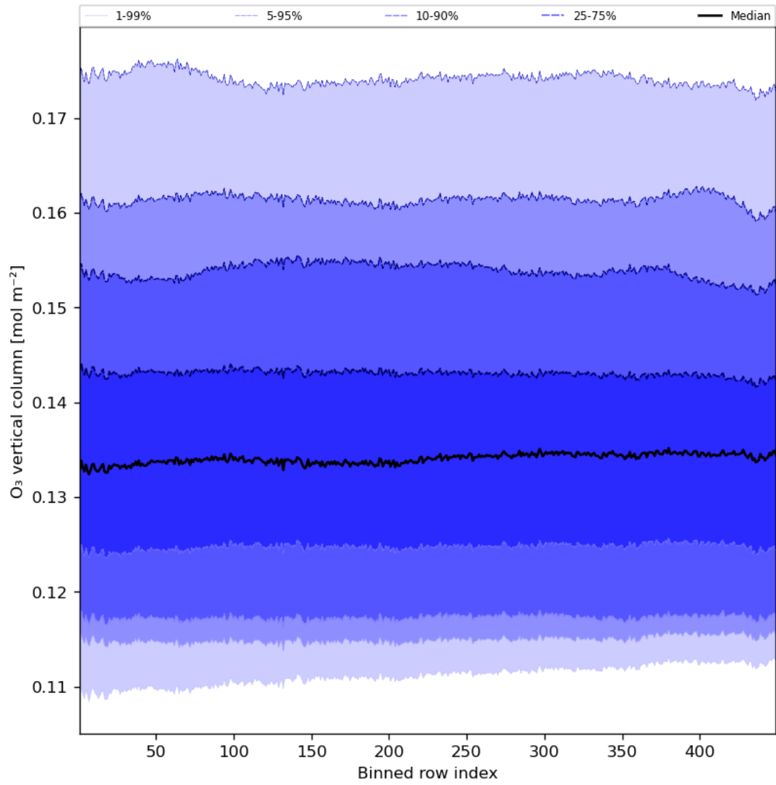
Figure 28: Along track statistics of “O 3 vertical column” for 2023-07-19 to 2023-07-21
