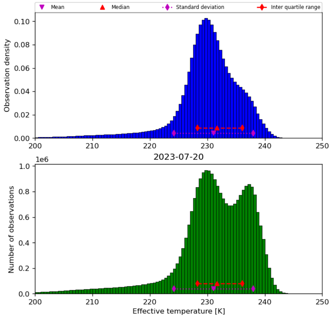
Figure 24: Histogram of “Effective temperature” for 2023-07-19 to 2023-07-21
