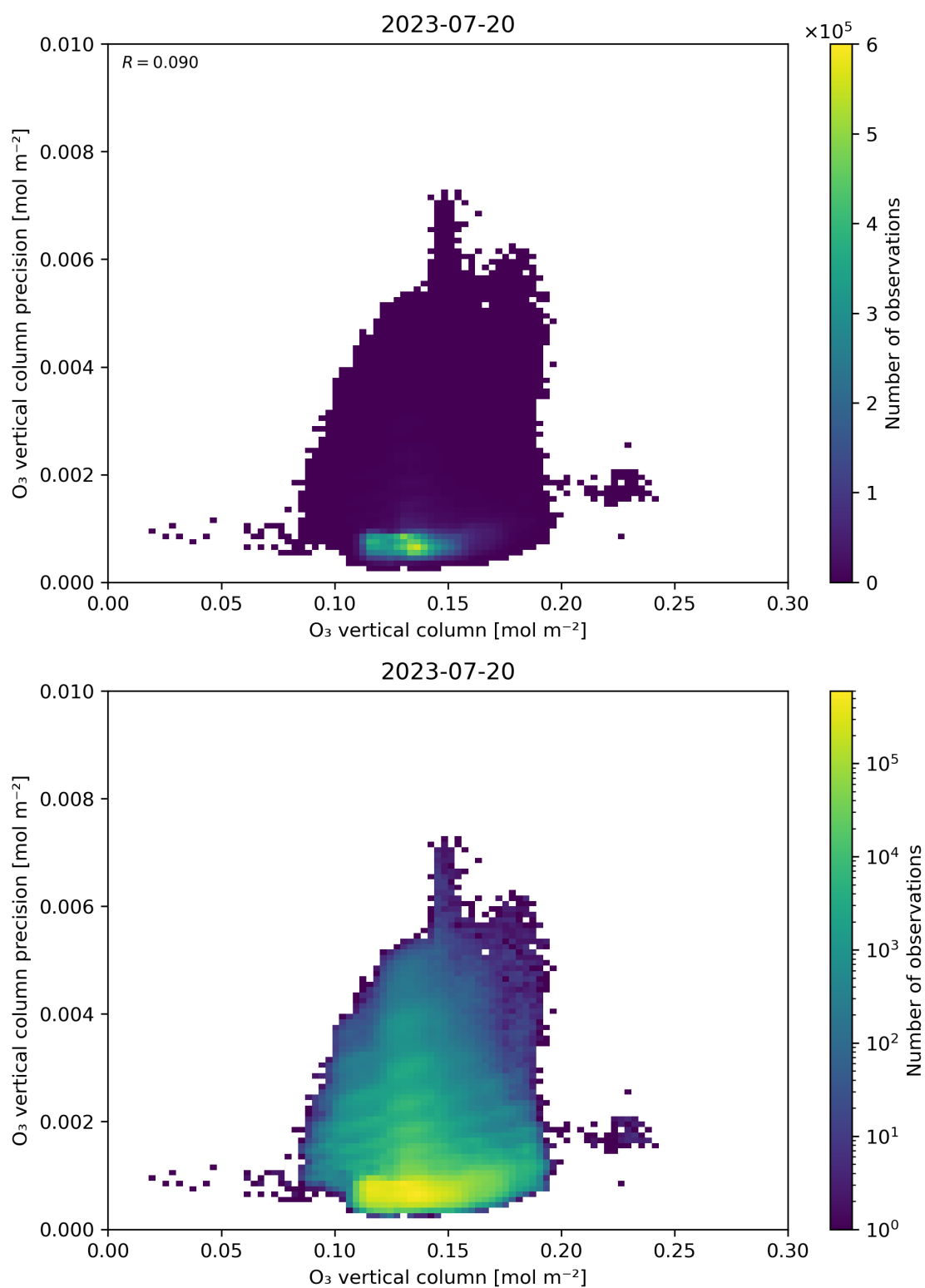
Figure 41: Scatter density plot of “O 3 vertical column” against “O 3 vertical column precision” for 2023-07-19 to 2023-07-21.
