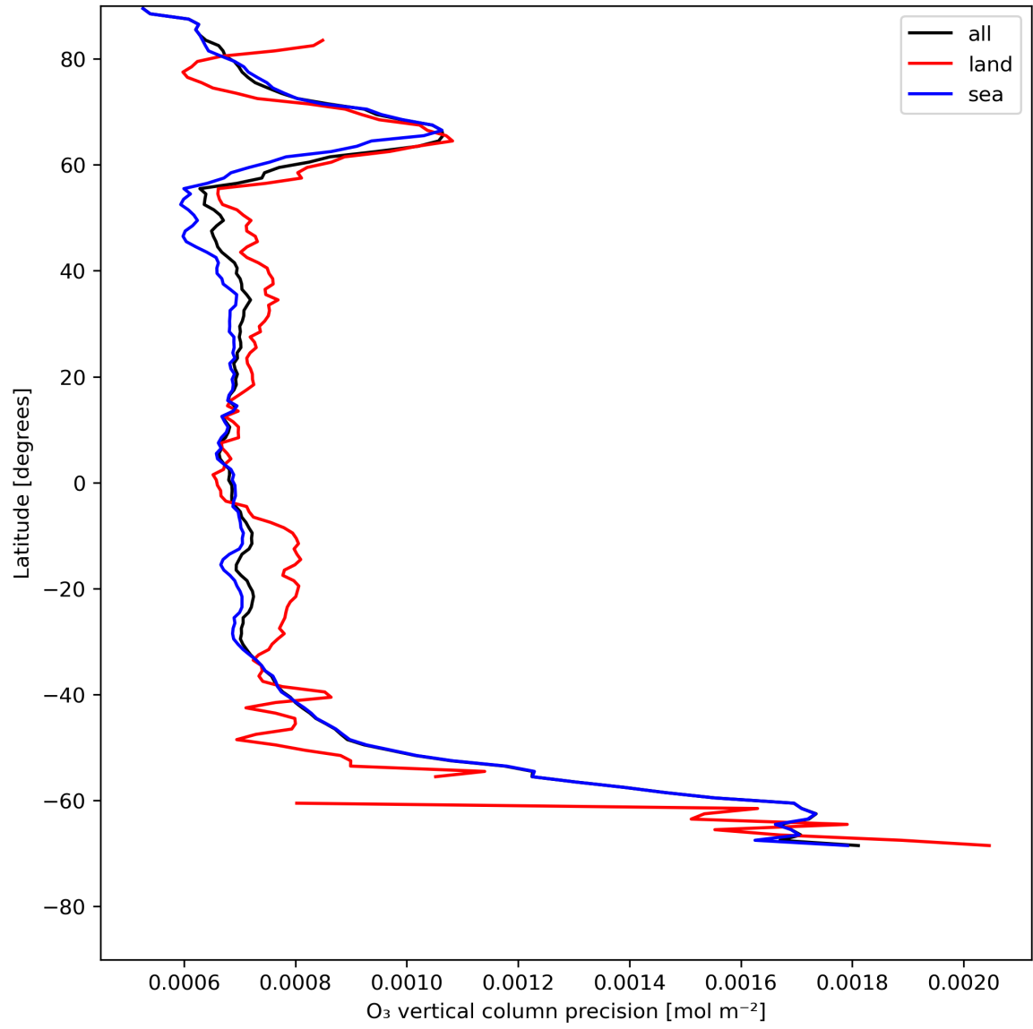
Figure 15: Zonal average of "O 3 vertical column precision" for 2023-07-19 to 2023-07-21.
