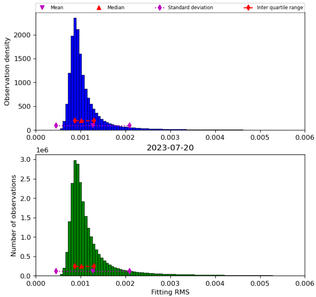
Figure 23: Histogram of “Fitting RMS” for 2023-07-19 to 2023-07-21
