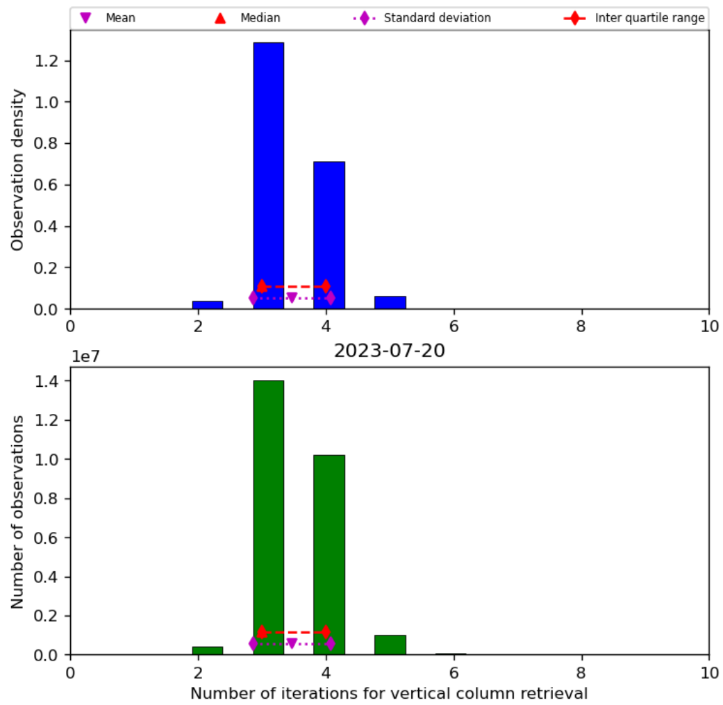
Figure 26: Histogram of “Number of iterations for vertical column retrieval” for 2023-07-19 to 2023-07-21
