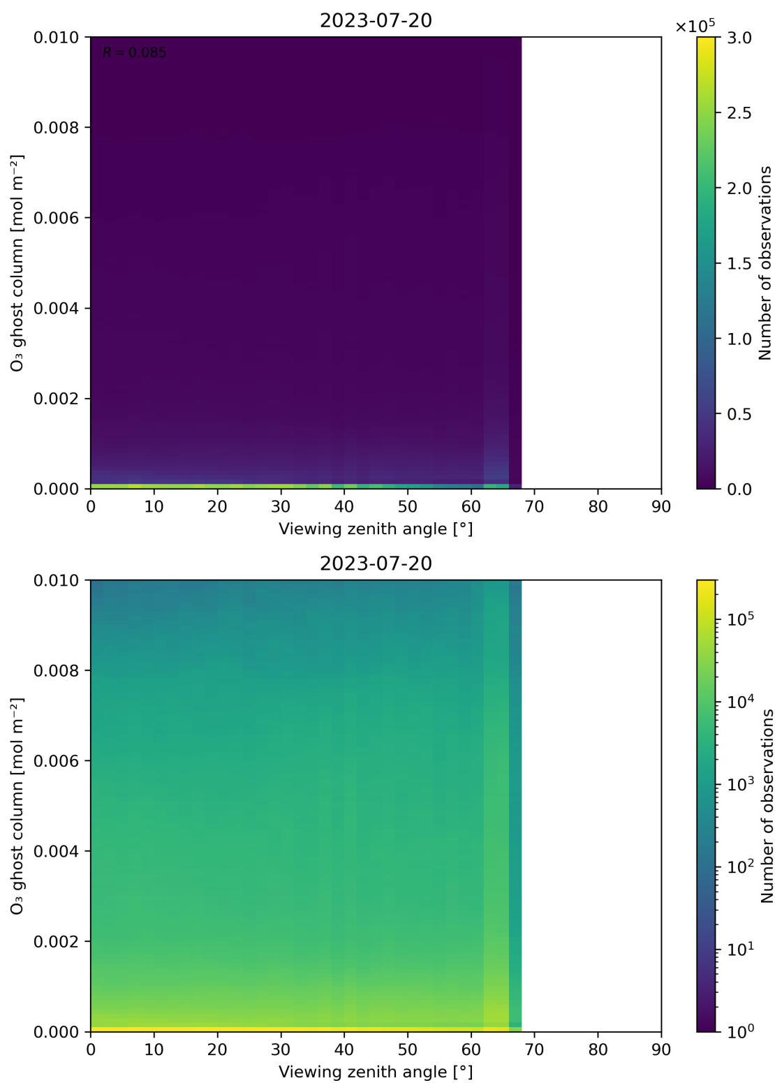
Figure 51: Scatter density plot of “Viewing zenith angle” against “O 3 ghost column” for 2023-07-19 to 2023-07-21.
