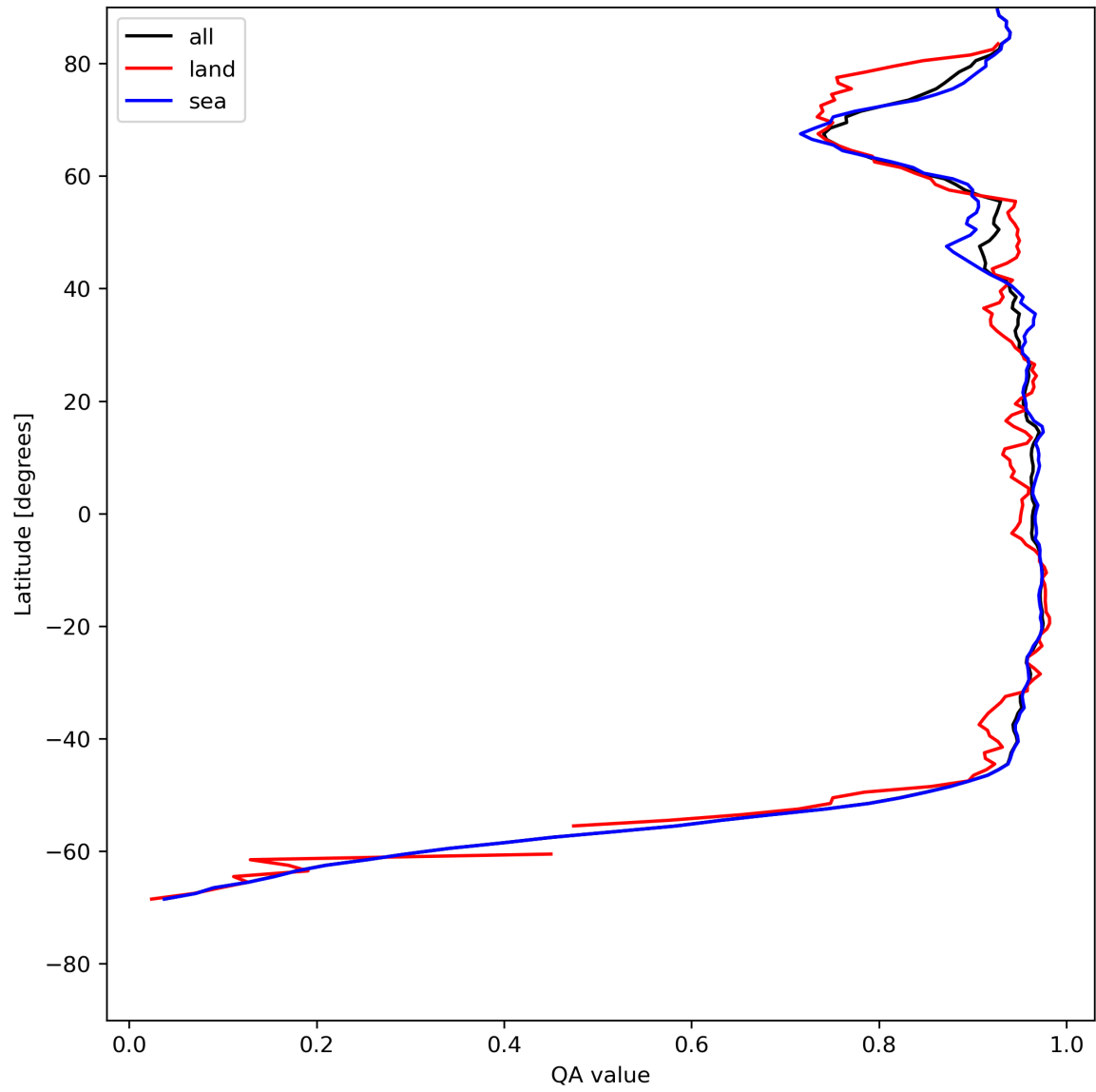
Figure 13: Zonal average of “QA value” for 2023-07-19 to 2023-07-21.
