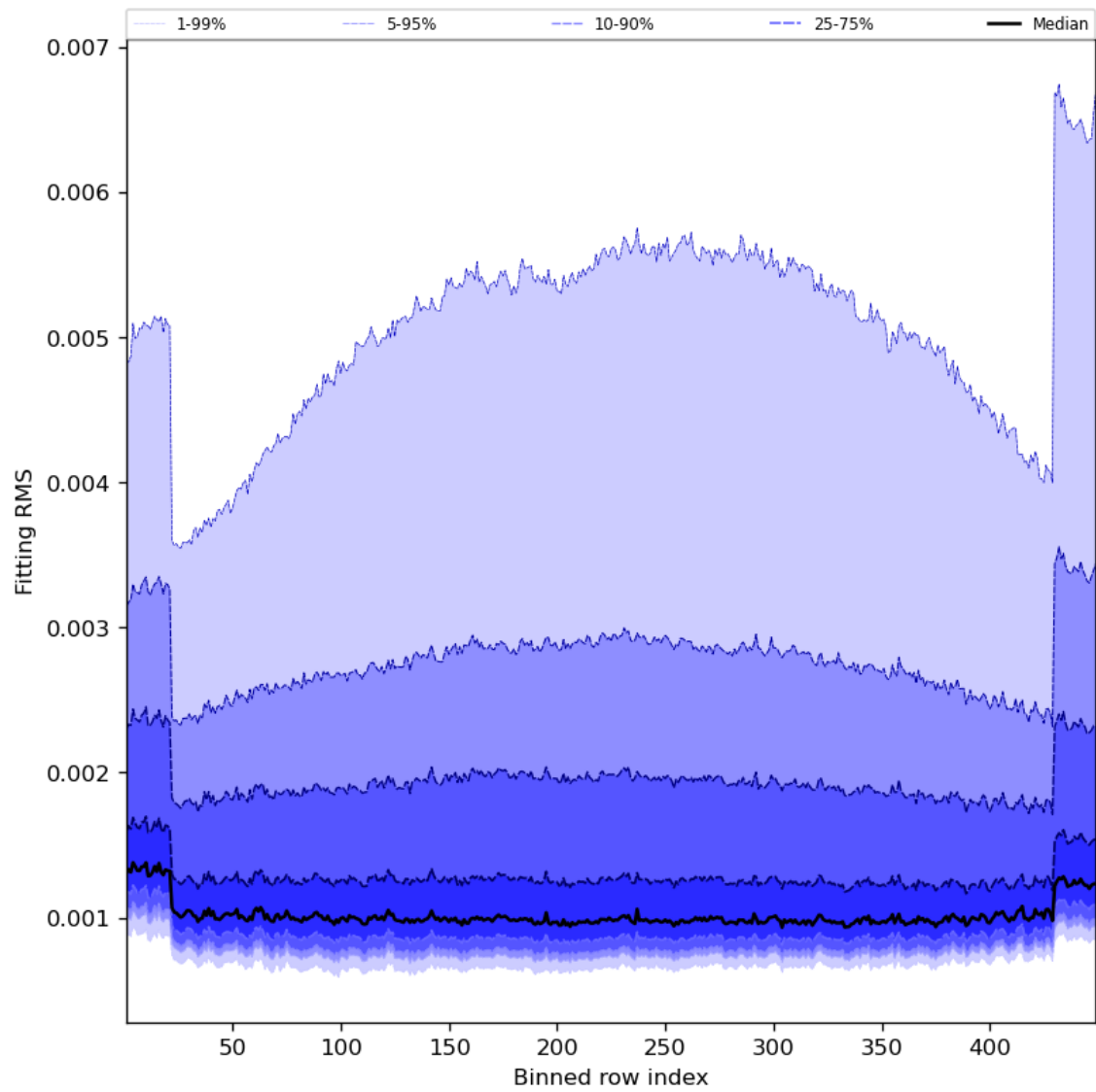
Figure 30: Along track statistics of “Fitting RMS” for 2023-07-19 to 2023-07-21
