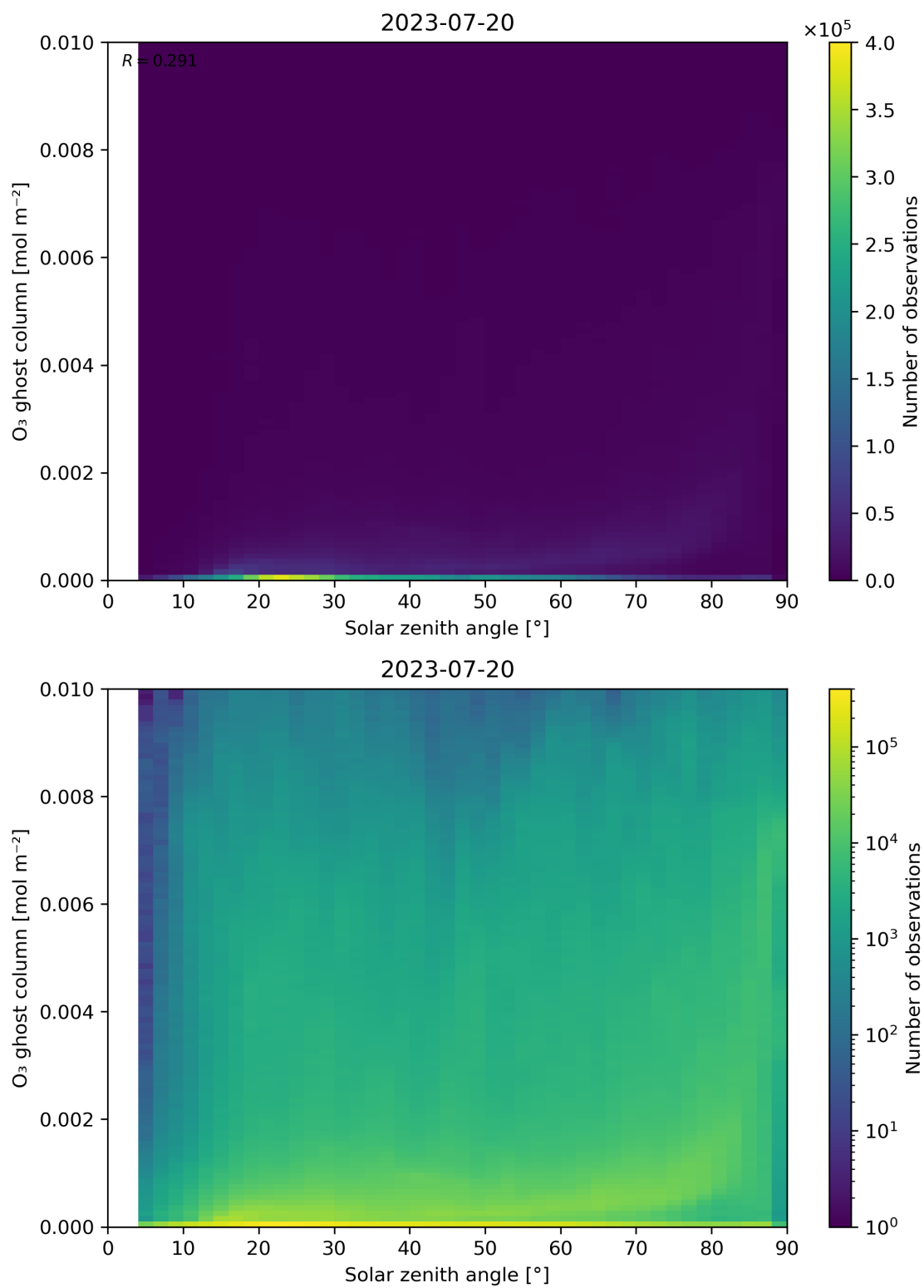
Figure 46: Scatter density plot of “Solar zenith angle” against “O 3 ghost column” for 2023-07-19 to 2023-07-21.
