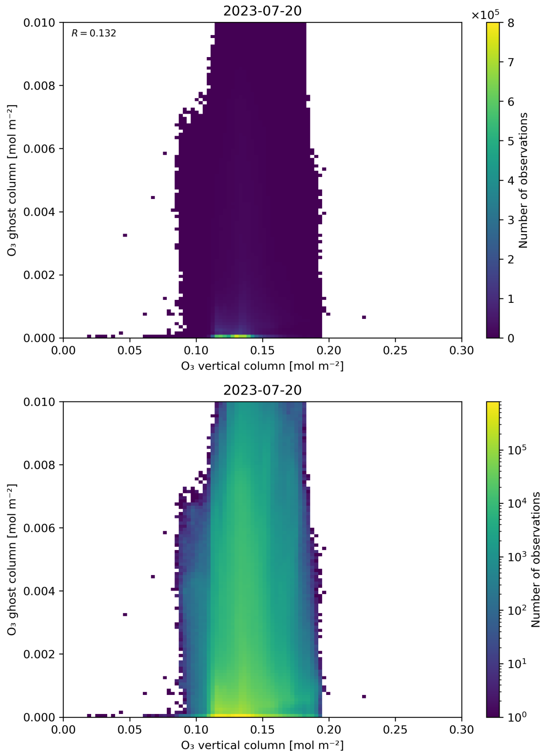
Figure 40: Scatter density plot of “O 3 vertical column” against “O 3 ghost column” for 2023-07-19 to 2023-07-21.
