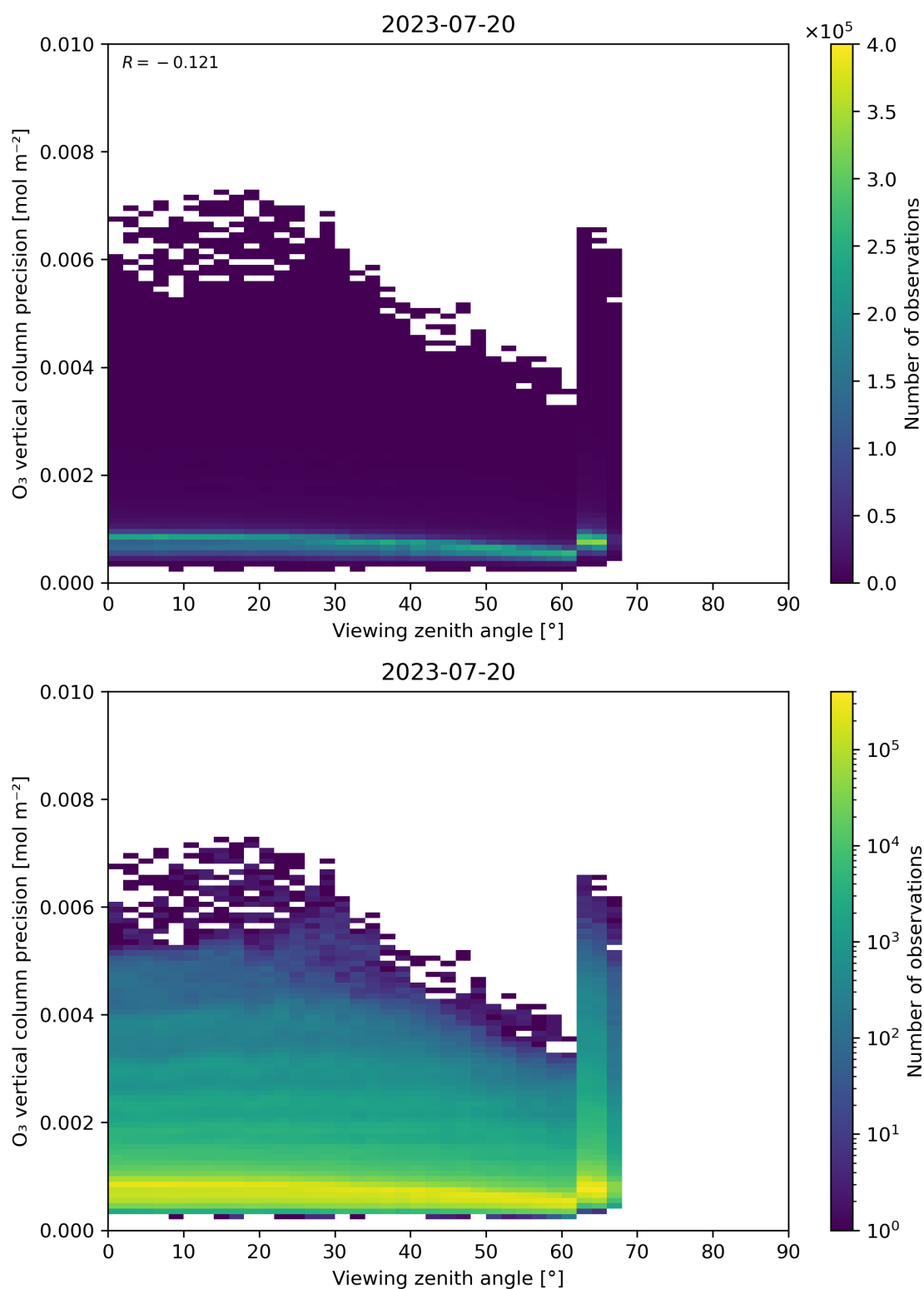
Figure 53: Scatter density plot of “Viewing zenith angle” against “O 3 vertical column precision” for 2023-07-19 to 2023-07-21.
