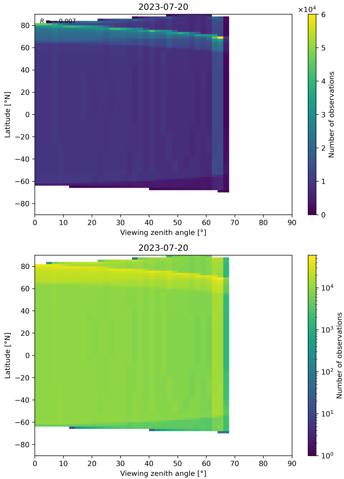
Figure 49: Scatter density plot of “Viewing zenith angle” against “Latitude” for 2023-07-19 to 2023-07-21.
