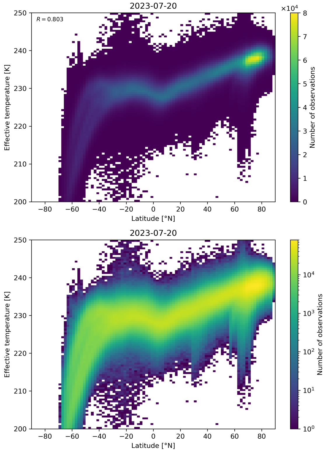
Figure 34: Scatter density plot of “Latitude” against “Effective temperature” for 2023-07-19 to 2023-07-21.
