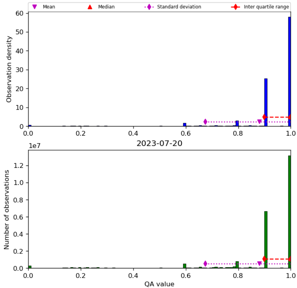
Figure 20: Histogram of “QA value” for 2023-07-19 to 2023-07-21
