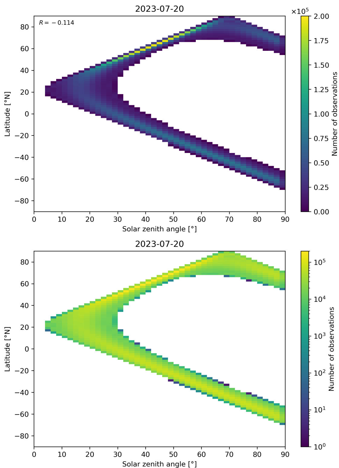
Figure 44: Scatter density plot of “Solar zenith angle” against “Latitude” for 2023-07-19 to 2023-07-21.
