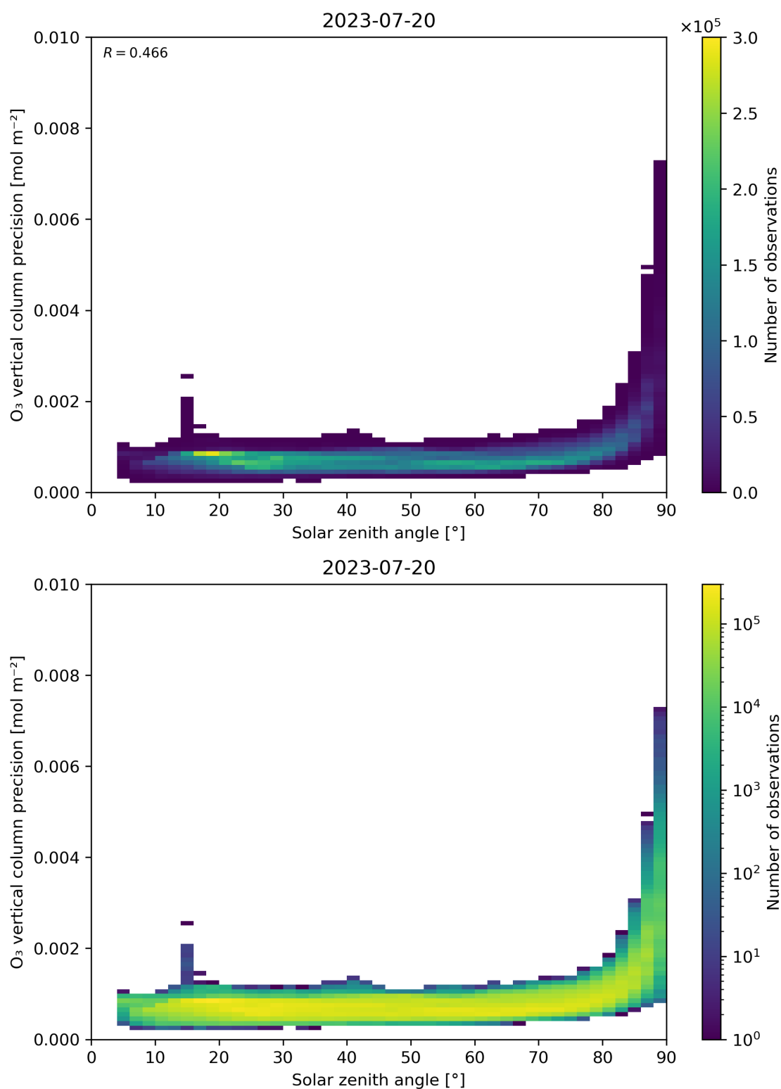
Figure 48: Scatter density plot of “Solar zenith angle” against “O 3 vertical column precision” for 2023-07-19 to 2023-07-21.
