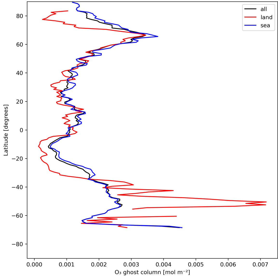
Figure 18: Zonal average of “O 3 ghost column” for 2023-07-19 to 2023-07-21.
