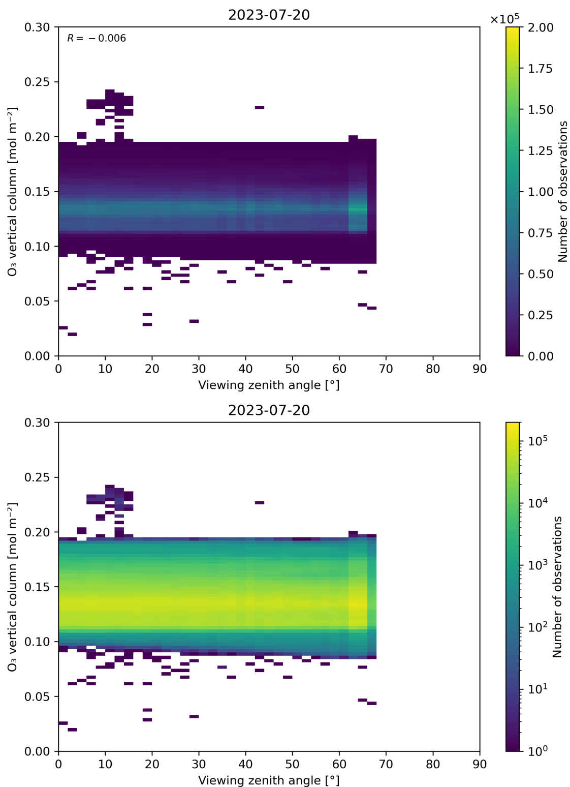
Figure 52: Scatter density plot of “Viewing zenith angle” against “O 3 vertical column” for 2023-07-19 to 2023-07-21.
