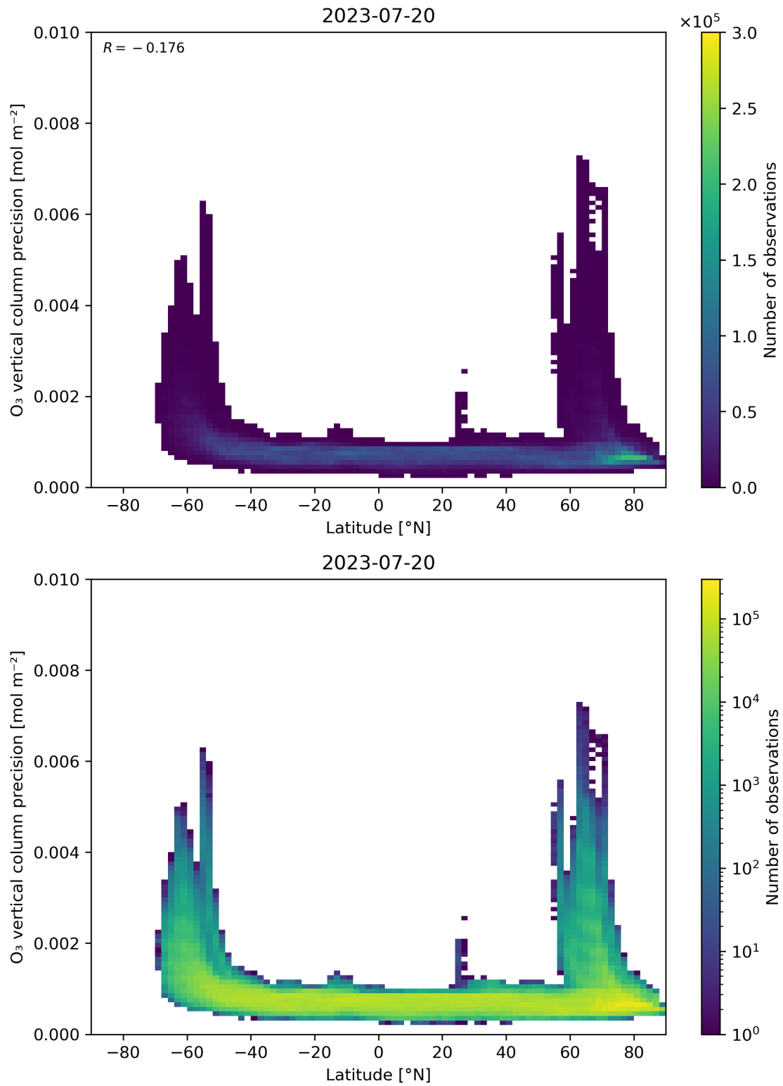
Figure 37: Scatter density plot of “Latitude” against “O 3 vertical column precision” for 2023-07-19 to 2023-07-21.
