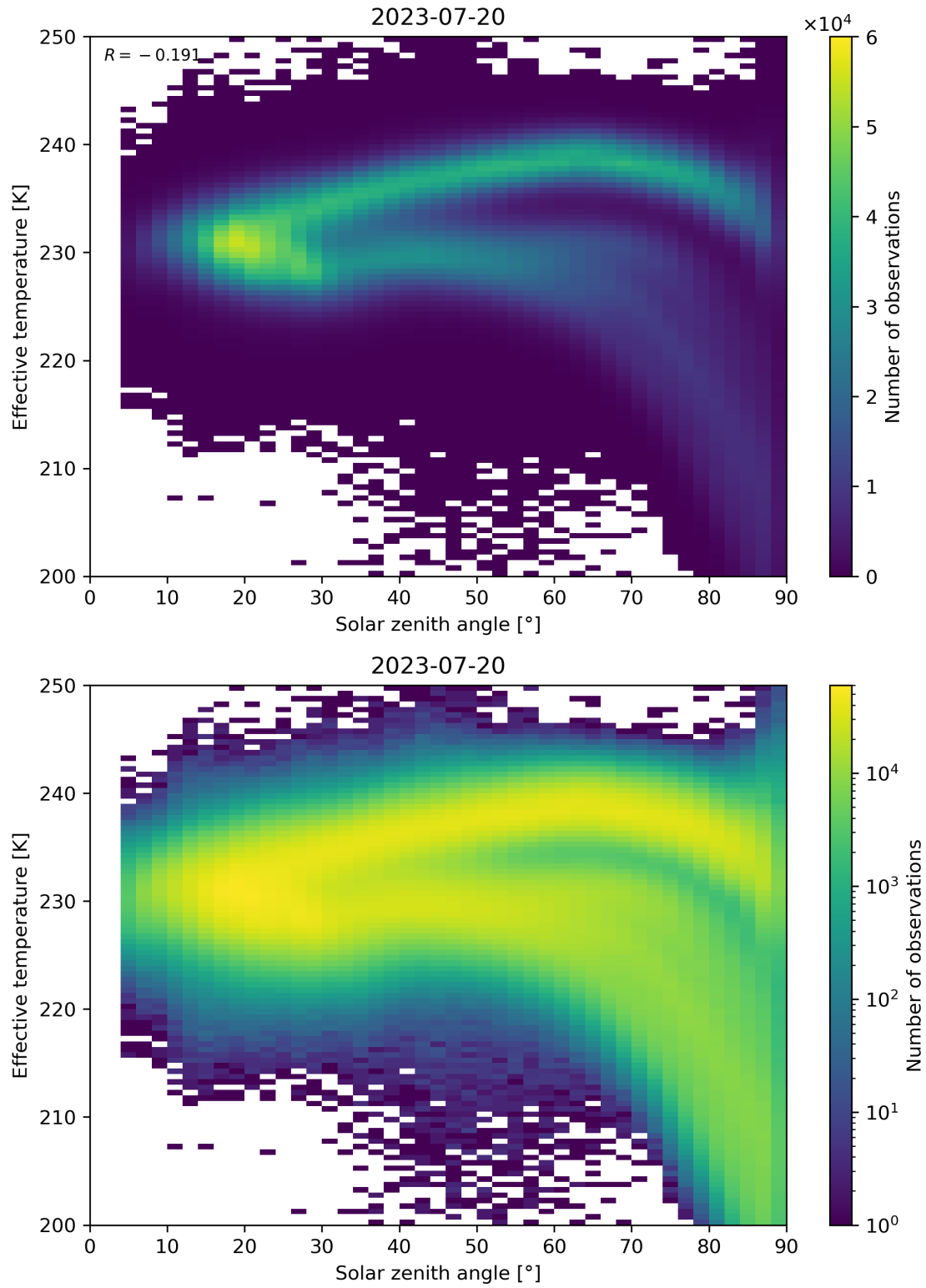
Figure 45: Scatter density plot of “Solar zenith angle” against “Effective temperature” for 2023-07-19 to 2023-07-21.
