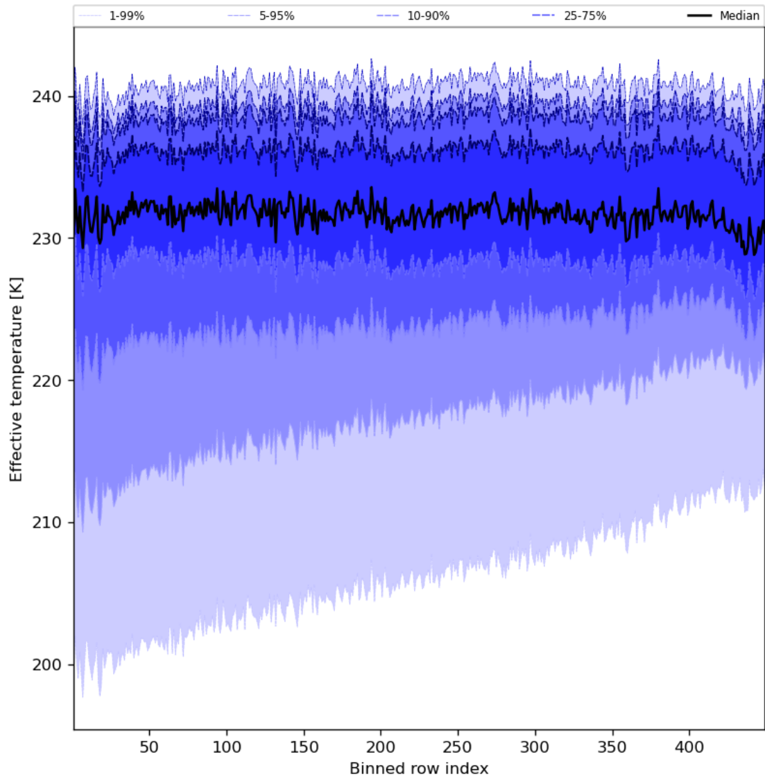
Figure 31: Along track statistics of “Effective temperature” for 2023-07-19 to 2023-07-21
