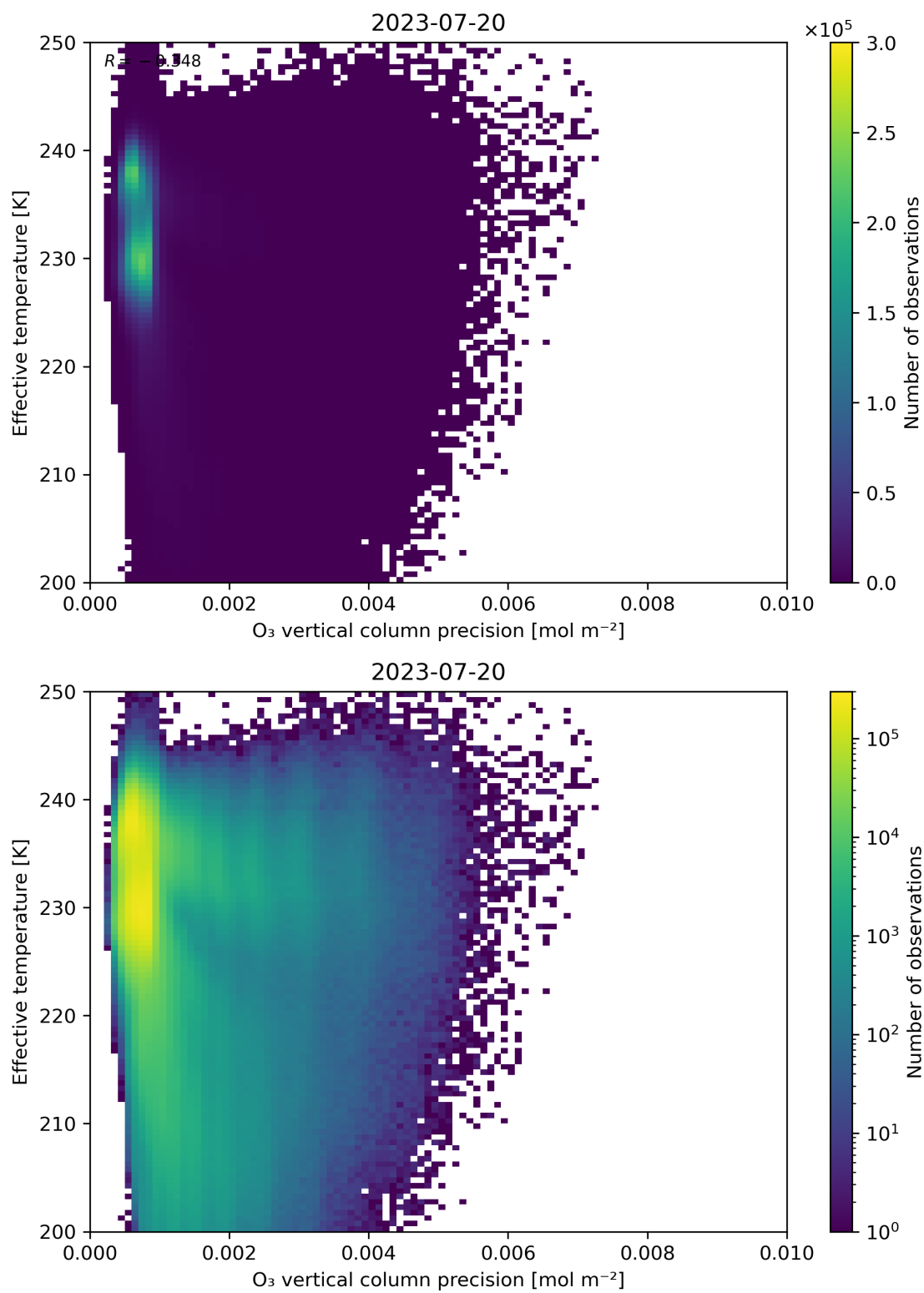
Figure 42: Scatter density plot of “O 3 vertical column precision” against “Effective temperature” for 2023-07-19 to 2023-07-21.
