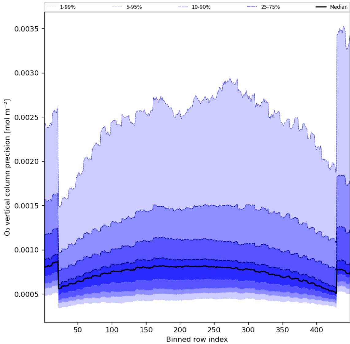
Figure 29: Along track statistics of “O 3 vertical column precision” for 2023-07-19 to 2023-07-21
