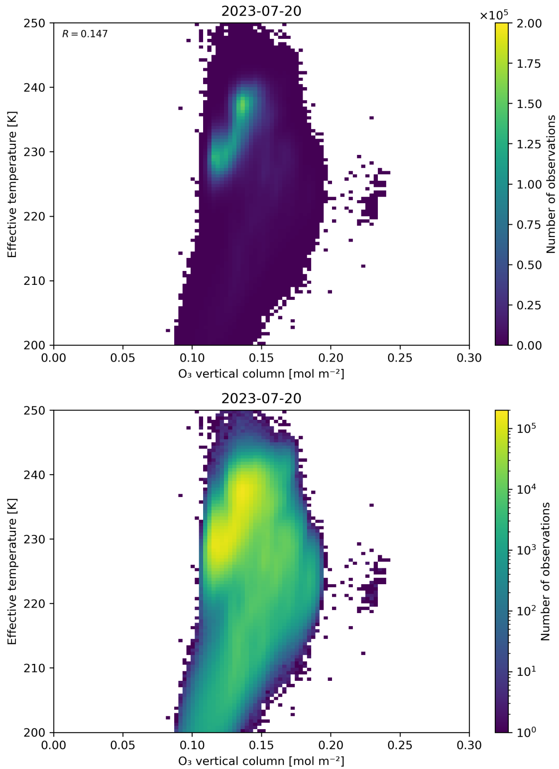
Figure 39: Scatter density plot of “O 3 vertical column” against “Effective temperature” for 2023-07-19 to 2023-07-21.
