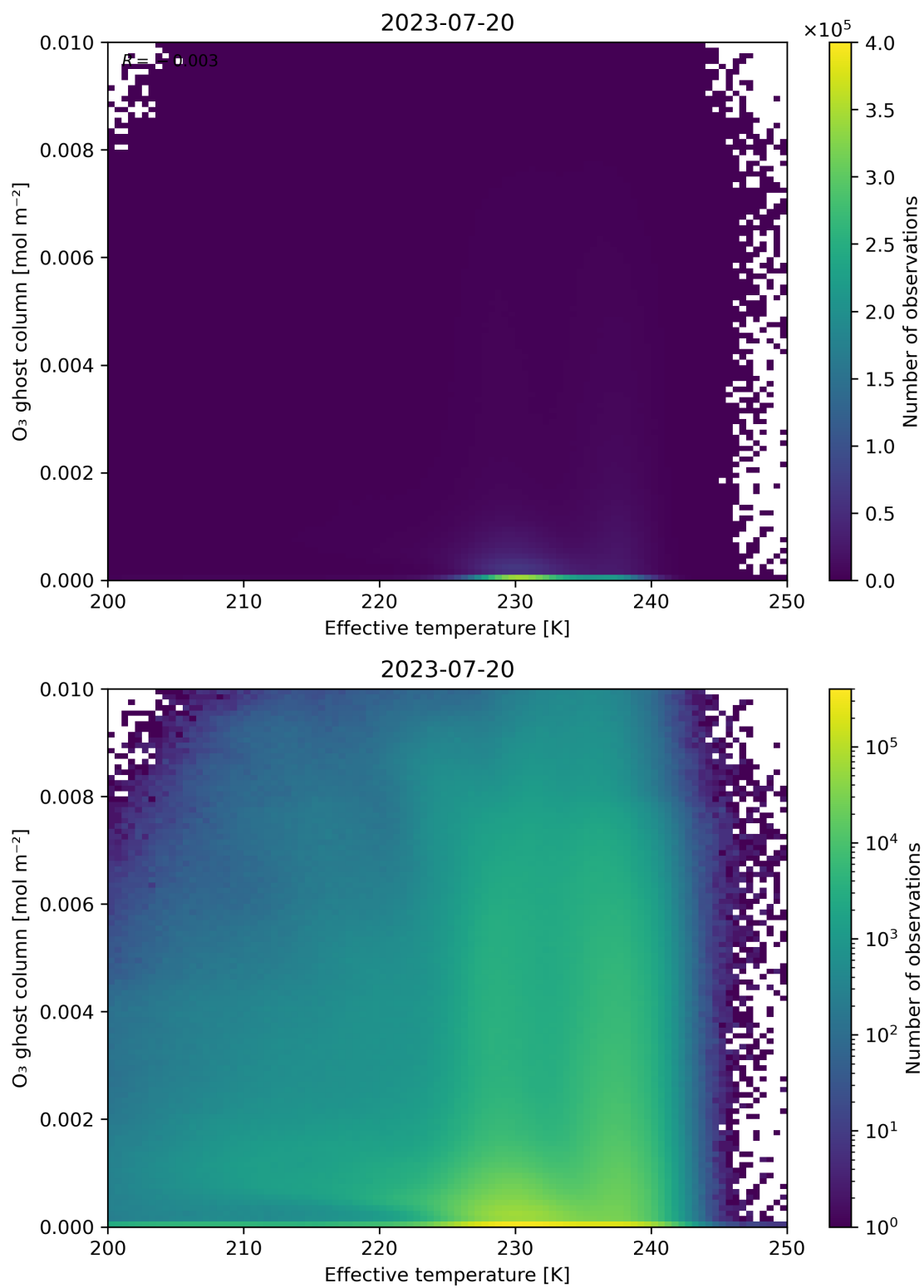
Figure 38: Scatter density plot of “Effective temperature” against “O 3 ghost column” for 2023-07-19 to 2023-07-21.
