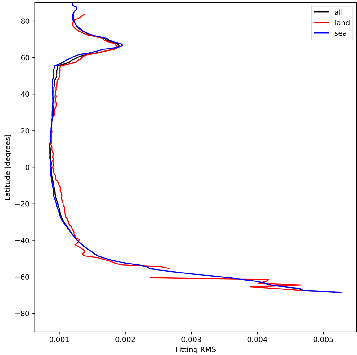
Figure 16: Zonal average of “Fitting RMS” for 2023-07-19 to 2023-07-21.
