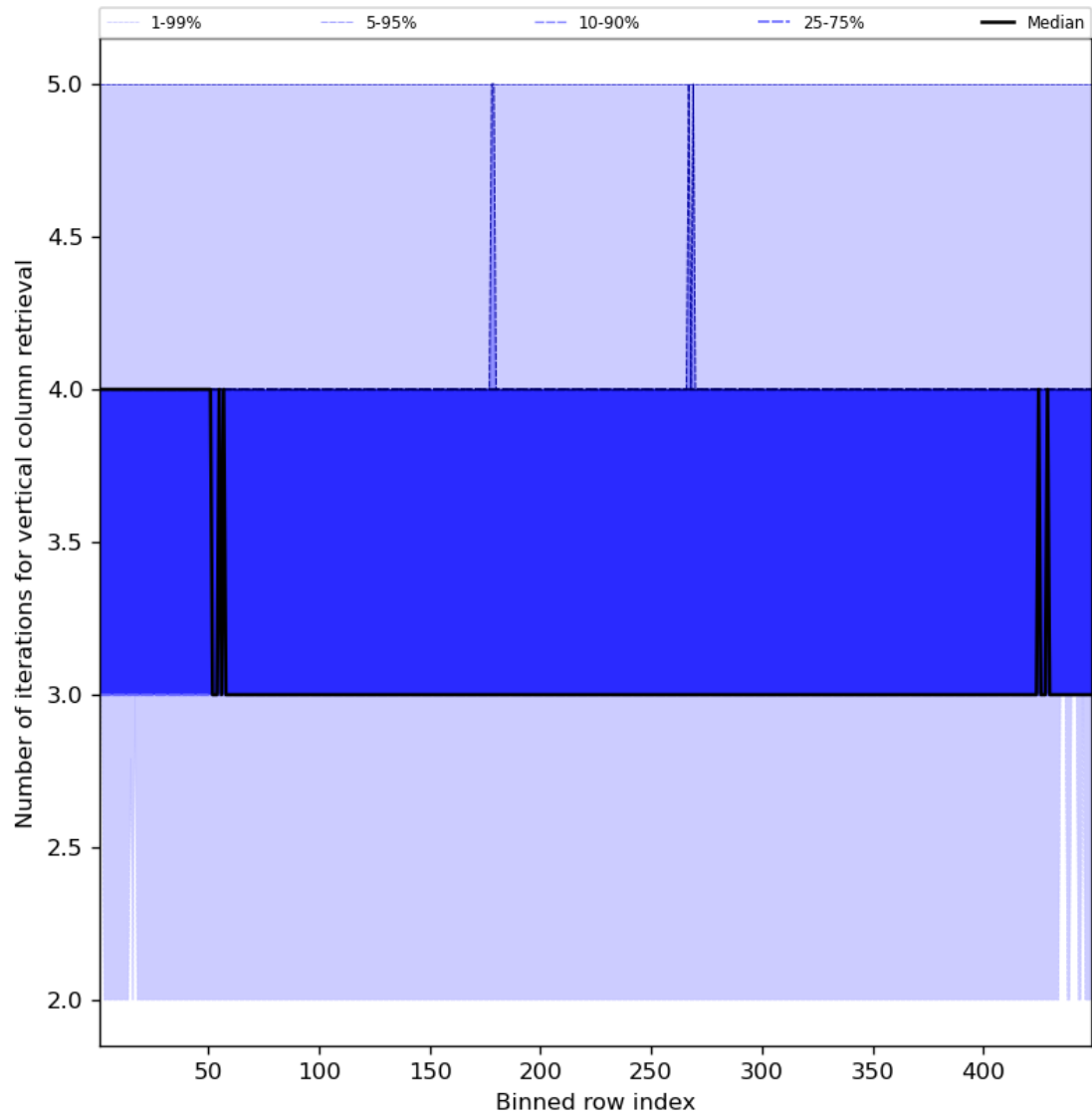
Figure 33: Along track statistics of “Number of iterations for vertical column retrieval” for 2023-07-19 to 2023-07-21
