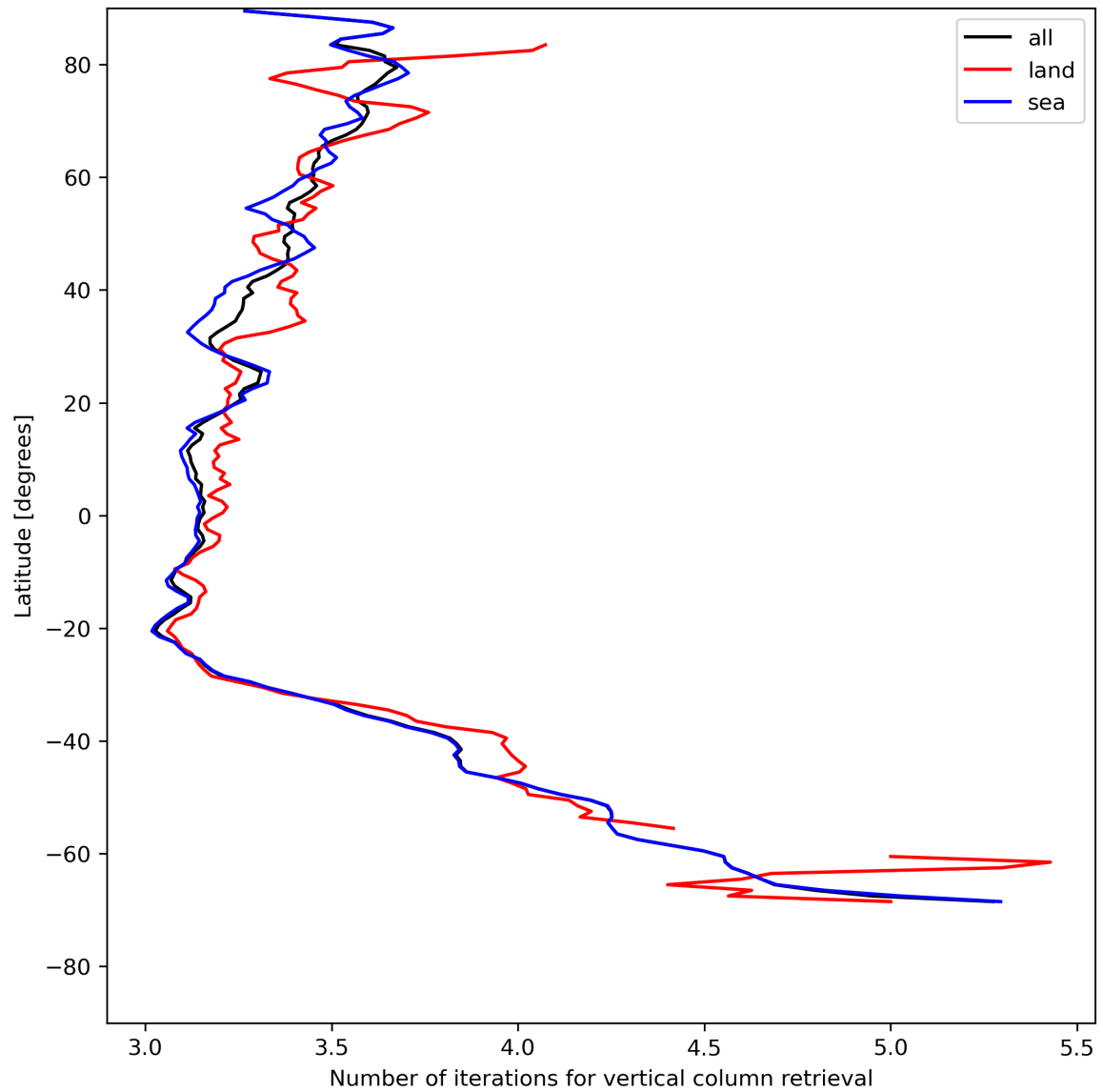
Figure 19: Zonal average of “Number of iterations for vertical column retrieval” for 2023-07-19 to 2023-07-21.
