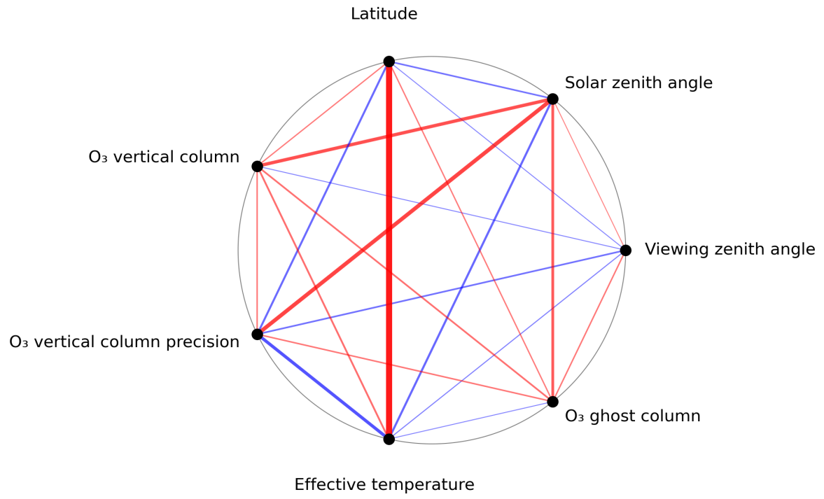
Figure 1: Map of correlation graph for 2023-07-19 to 2023-07-21.
