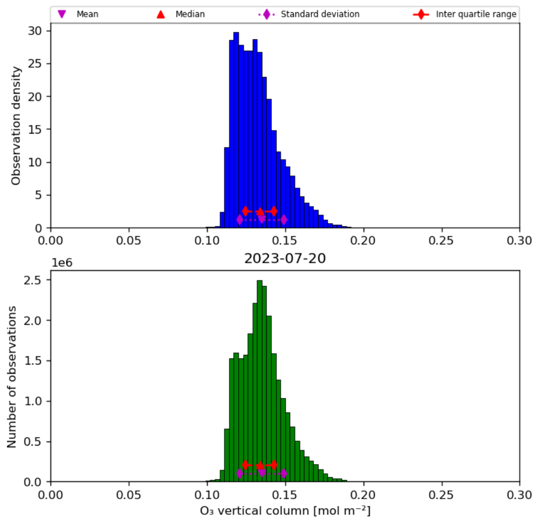
Figure 21: Histogram of “O 3 vertical column” for 2023-07-19 to 2023-07-21
