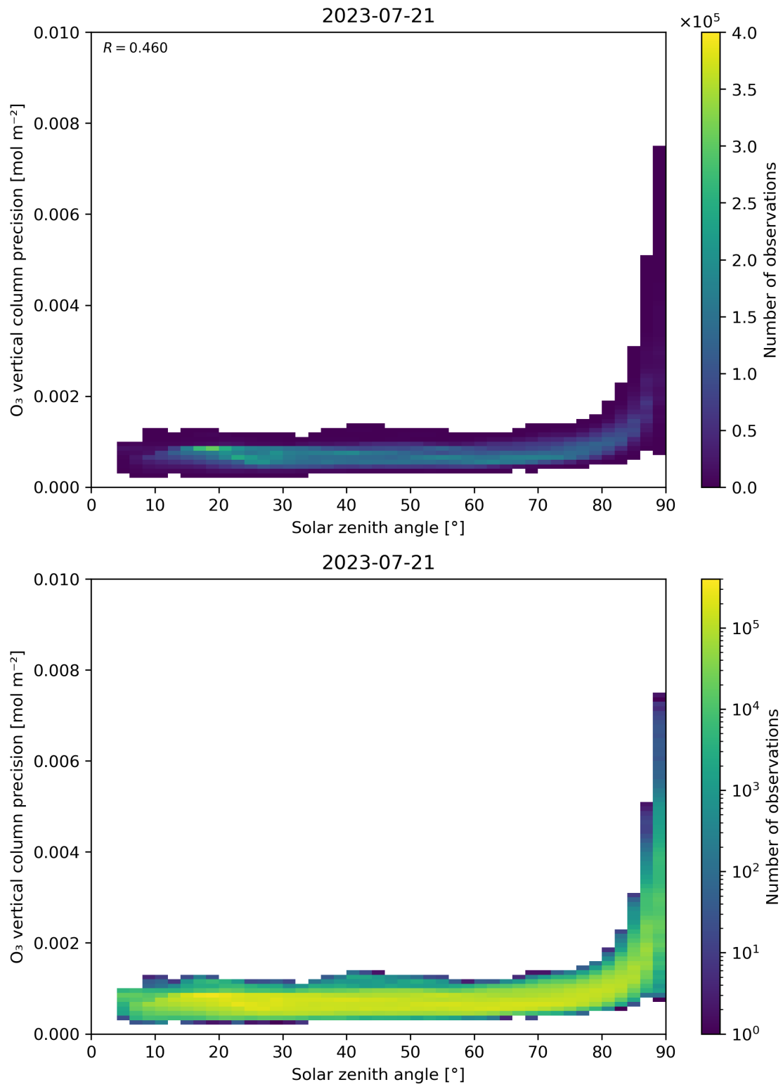
Figure 48: Scatter density plot of “Solar zenith angle” against “O 3 vertical column precision” for 2023-07-20 to 2023-07-22.
