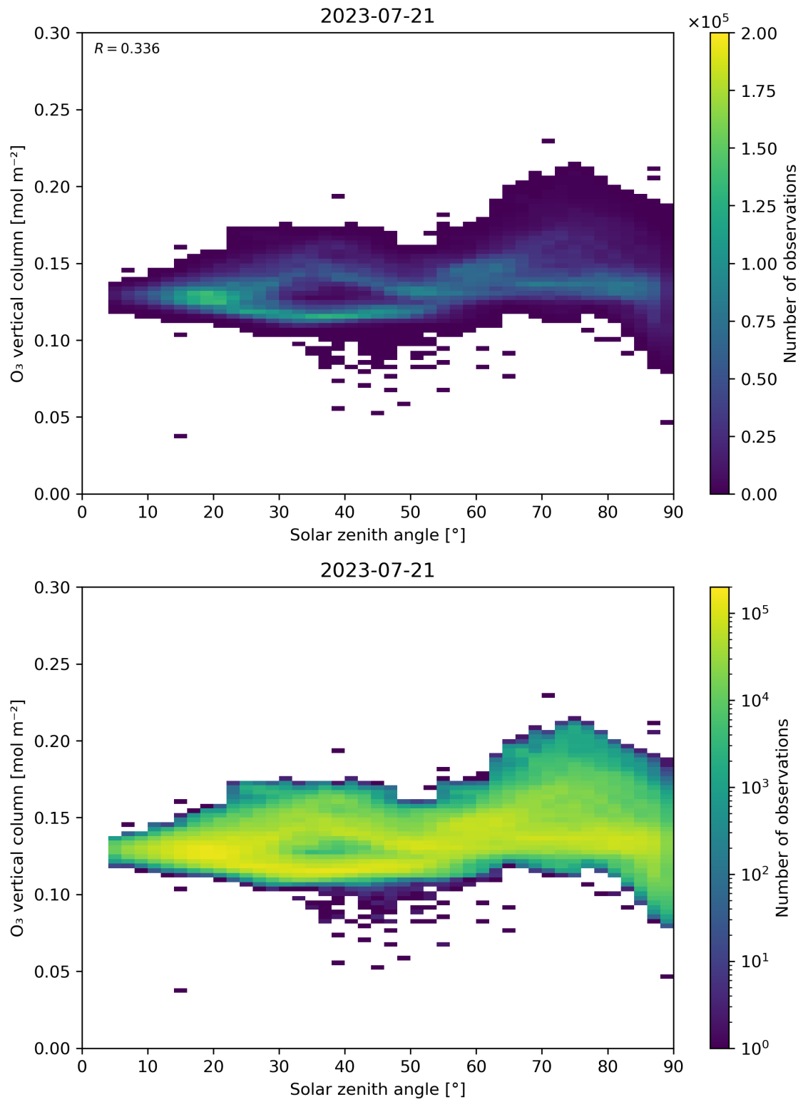
Figure 47: Scatter density plot of “Solar zenith angle” against “O 3 vertical column” for 2023-07-20 to 2023-07-22.
