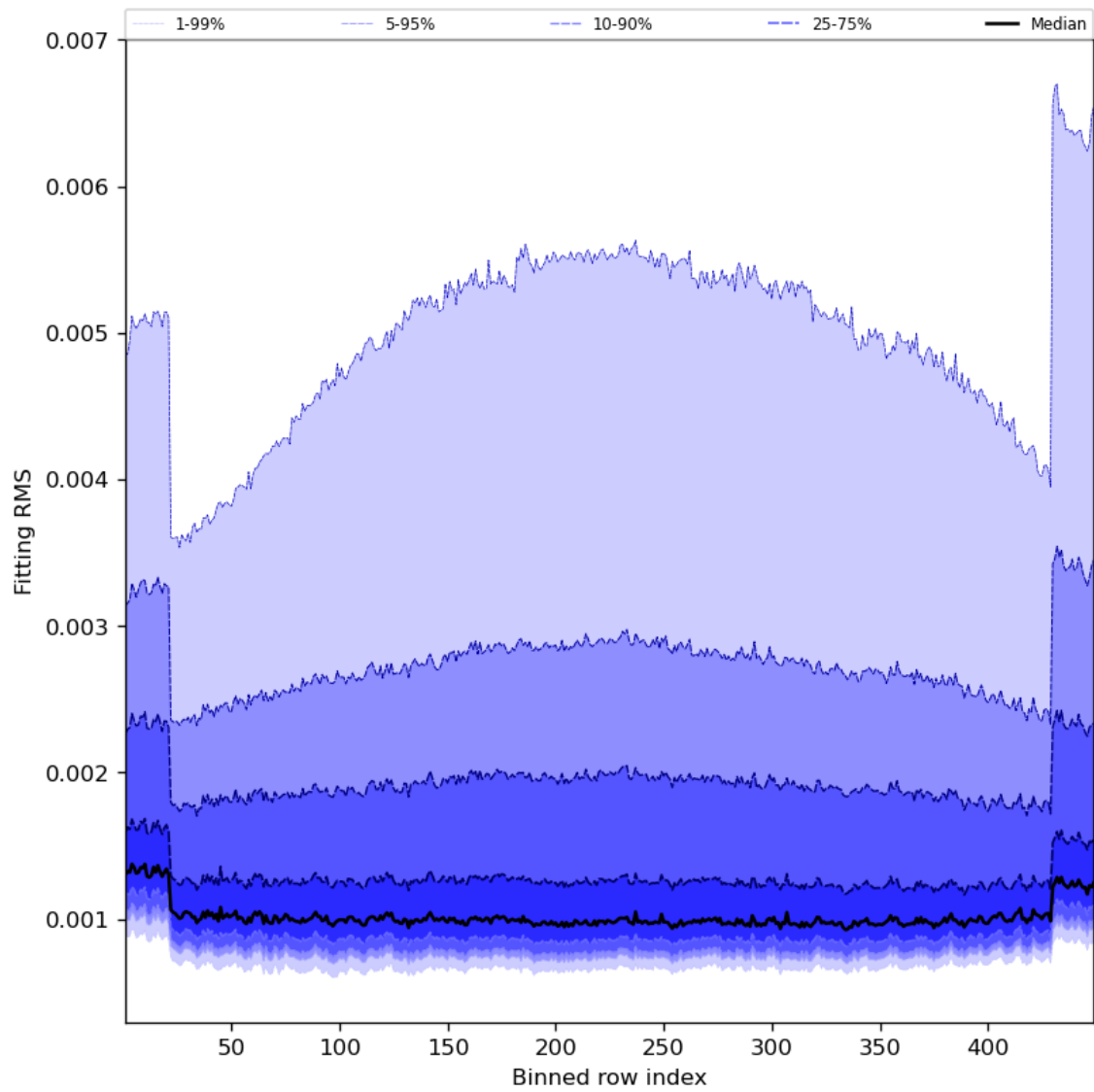
Figure 30: Along track statistics of “Fitting RMS” for 2023-07-20 to 2023-07-22
