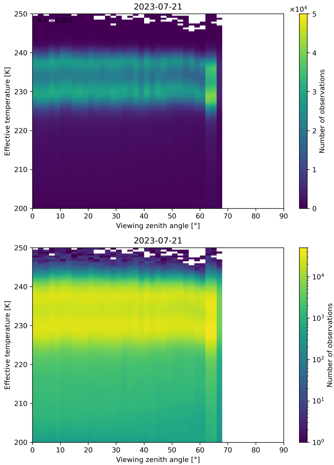
Figure 50: Scatter density plot of “Viewing zenith angle” against “Effective temperature” for 2023-07-20 to 2023-07-22.
