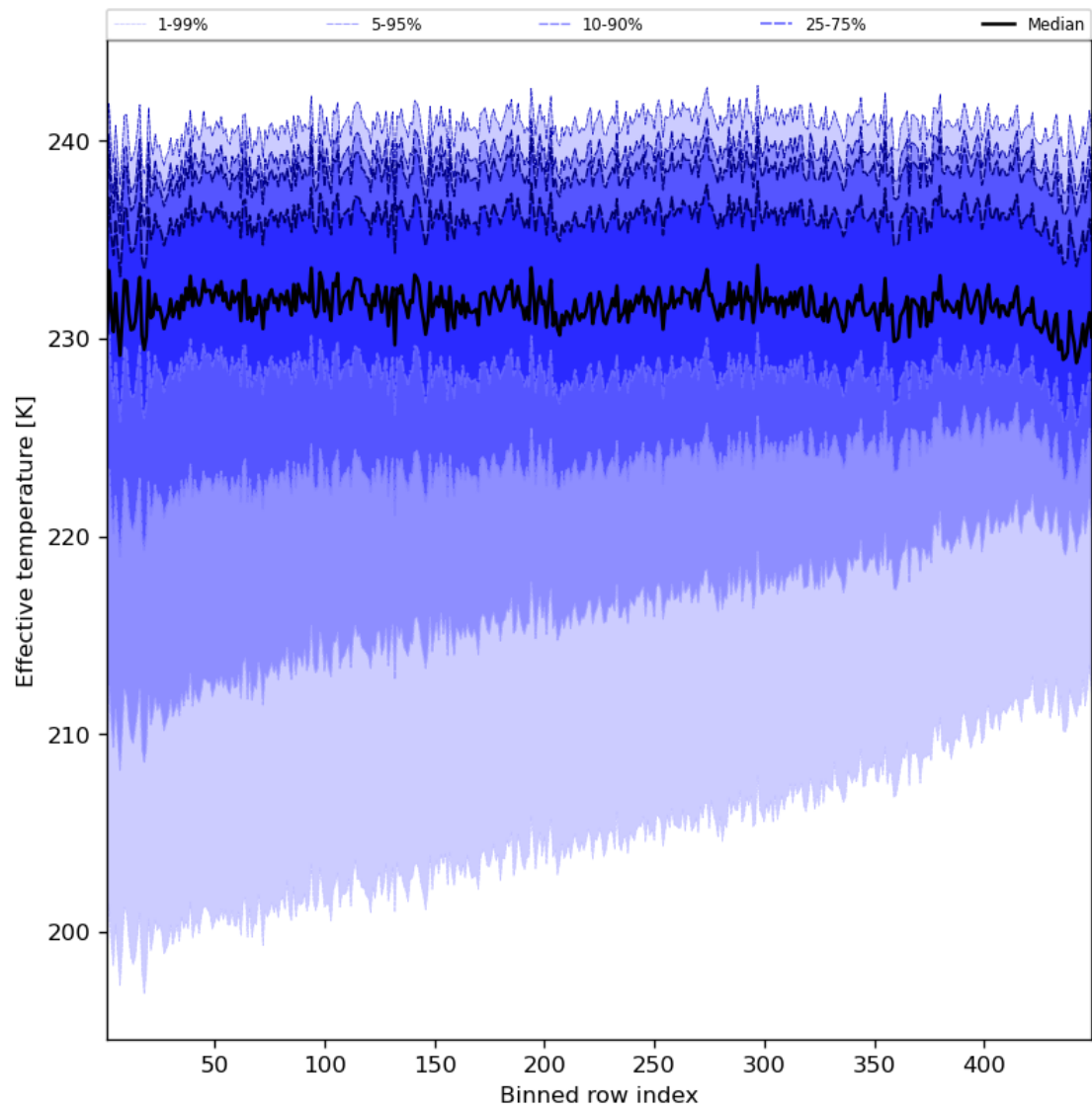
Figure 31: Along track statistics of “Effective temperature” for 2023-07-20 to 2023-07-22
