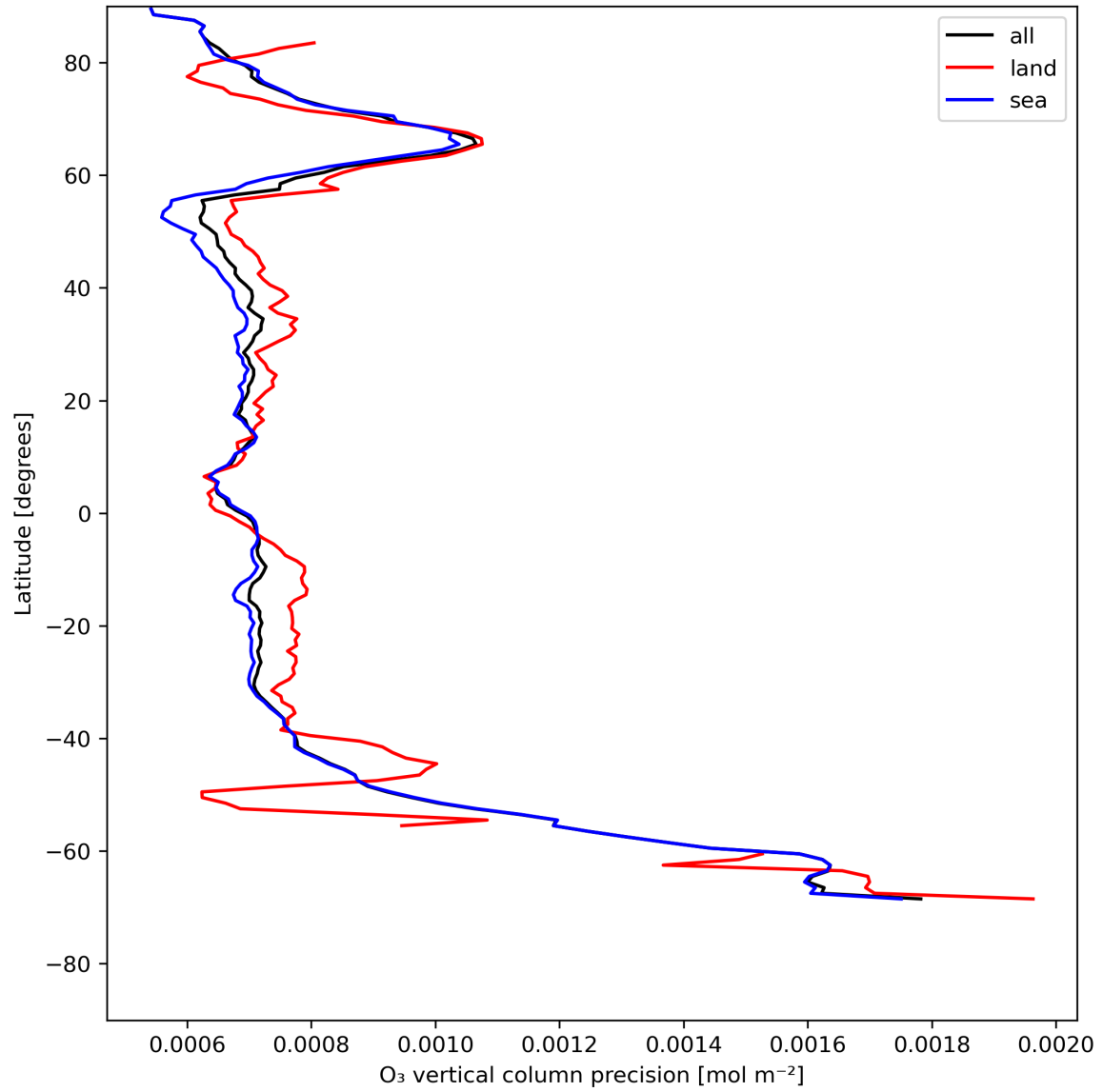
Figure 15: Zonal average of “O 3 vertical column precision” for 2023-07-20 to 2023-07-22.
