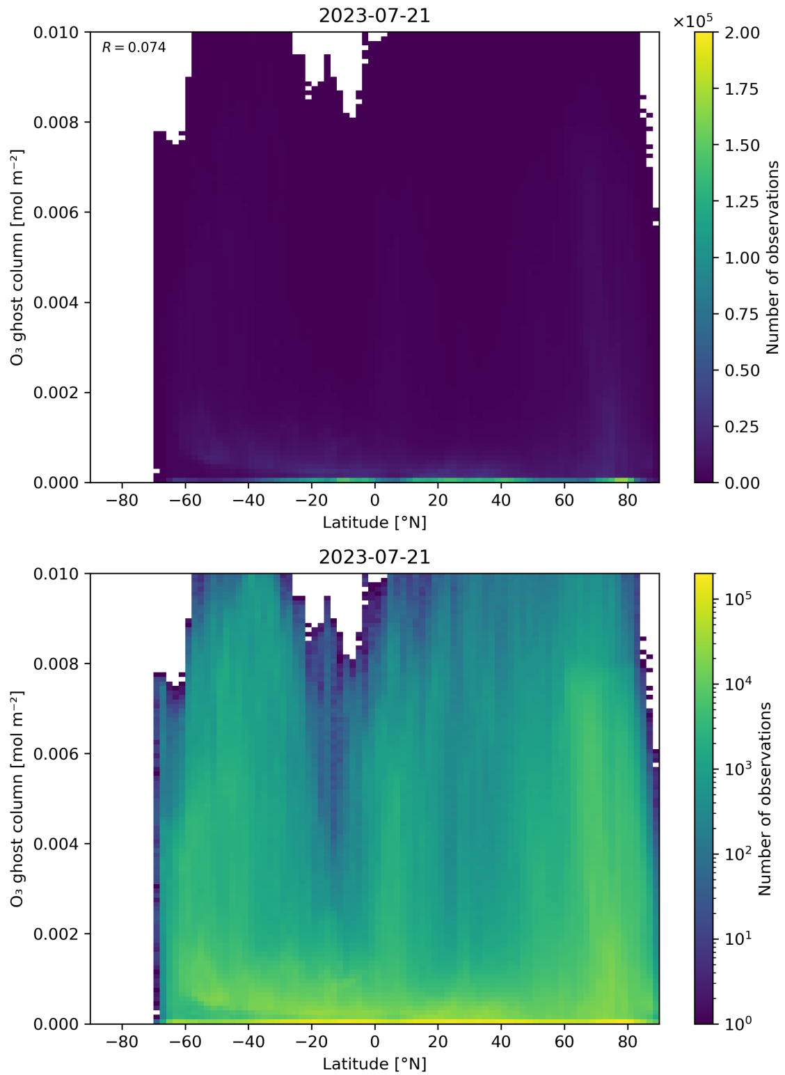
Figure 35: Scatter density plot of “Latitude” against “O 3 ghost column” for 2023-07-20 to 2023-07-22.
