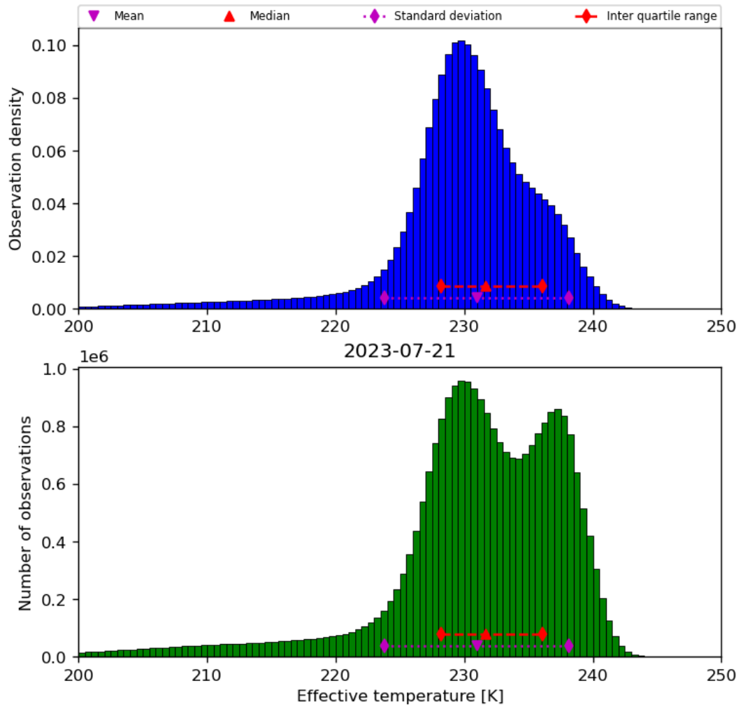
Figure 24: Histogram of “Effective temperature” for 2023-07-20 to 2023-07-22
