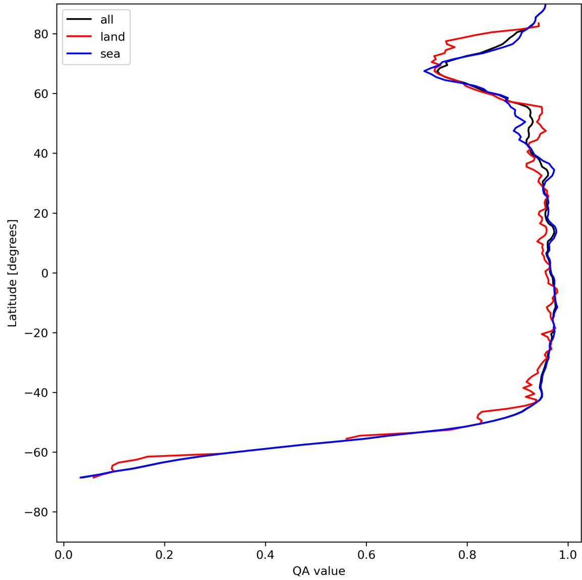
Figure 13: Zonal average of “QA value” for 2023-07-20 to 2023-07-22.
