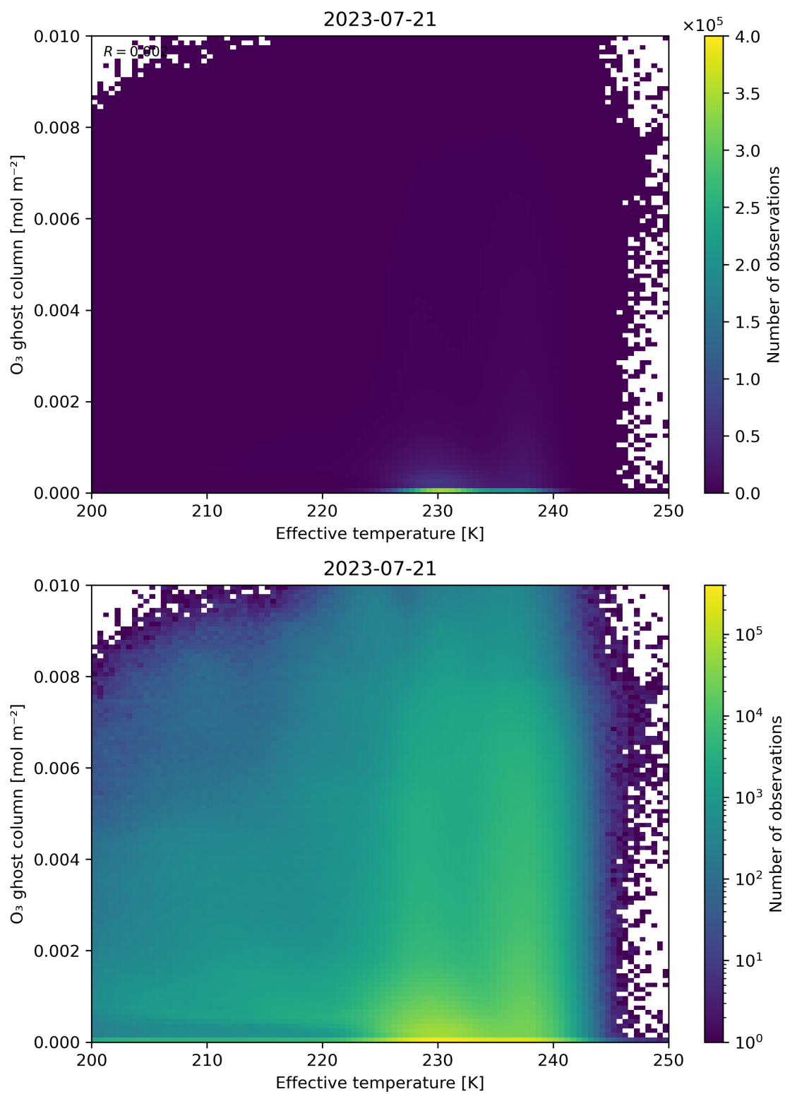
Figure 38: Scatter density plot of “Effective temperature” against “O 3 ghost column” for 2023-07-20 to 2023-07-22.
