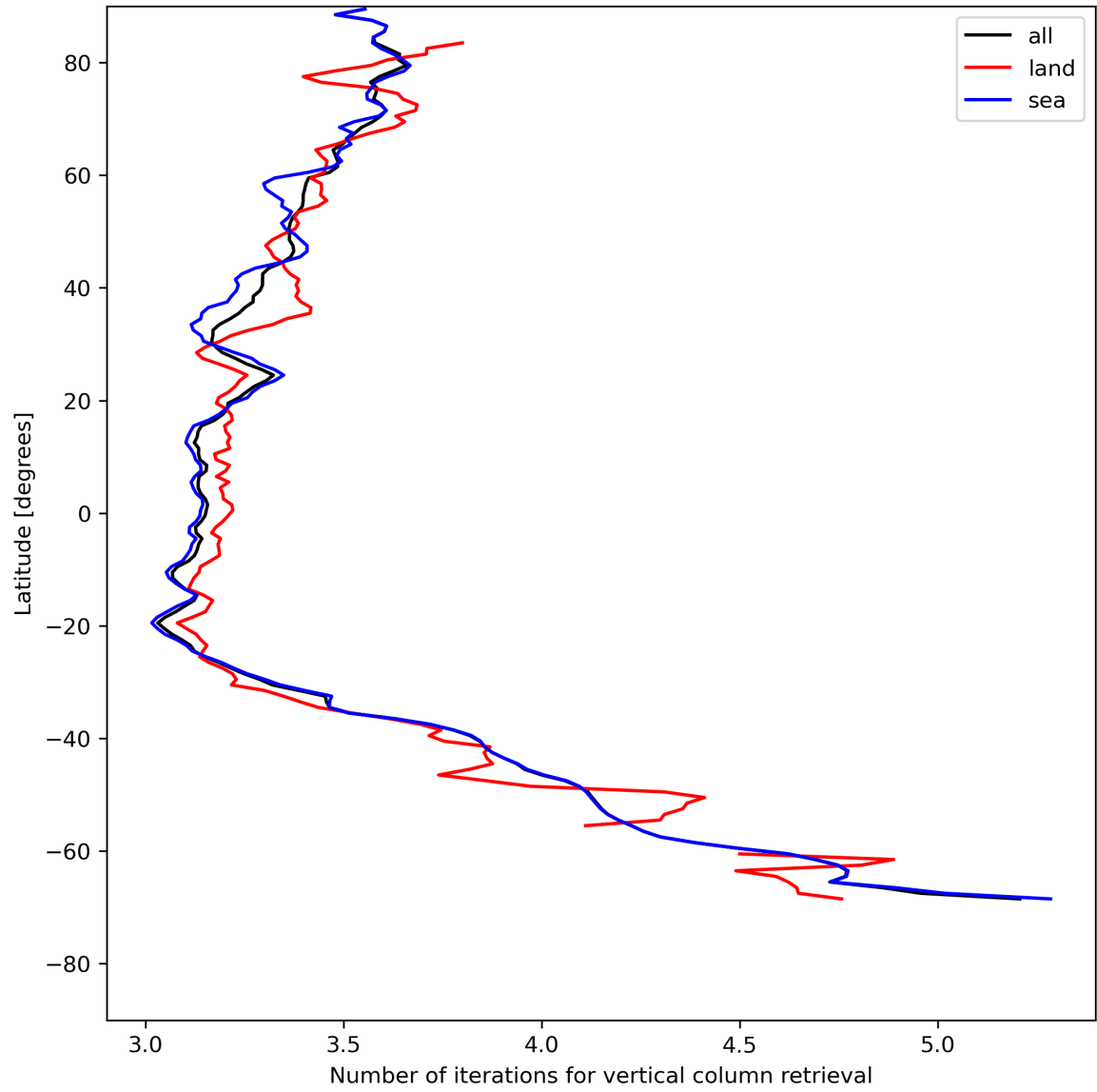
Figure 19: Zonal average of “Number of iterations for vertical column retrieval” for 2023-07-20 to 2023-07-22.
