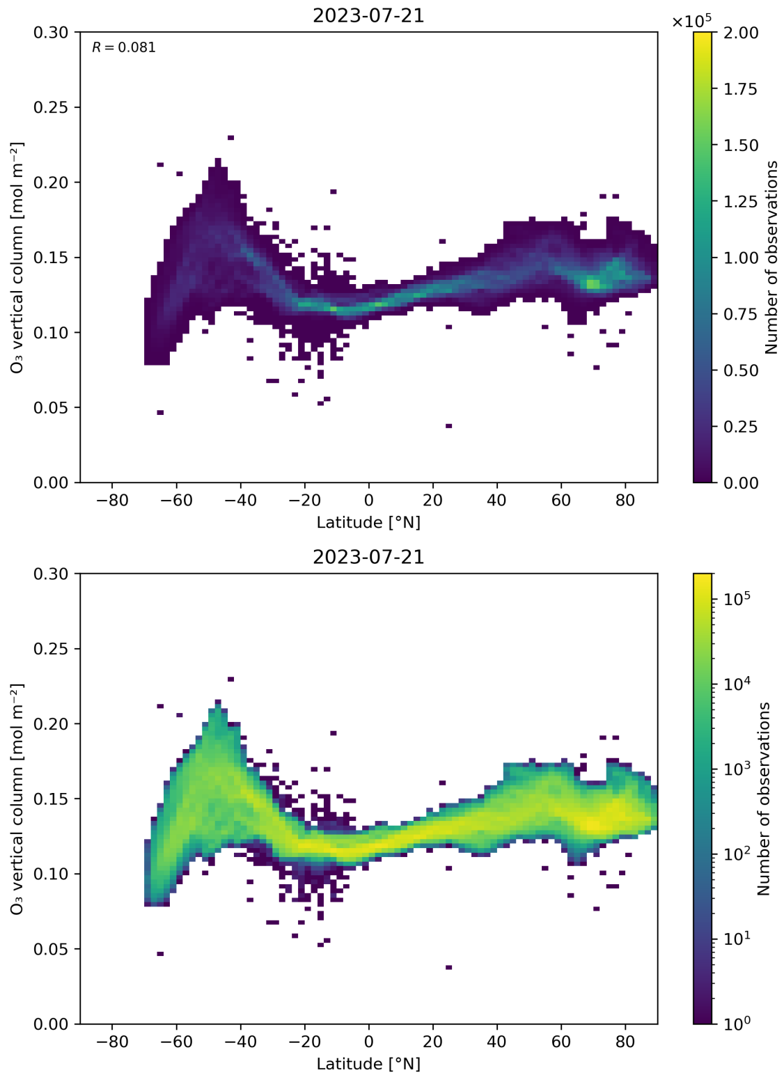
Figure 36: Scatter density plot of “Latitude” against “O 3 vertical column” for 2023-07-20 to 2023-07-22.
