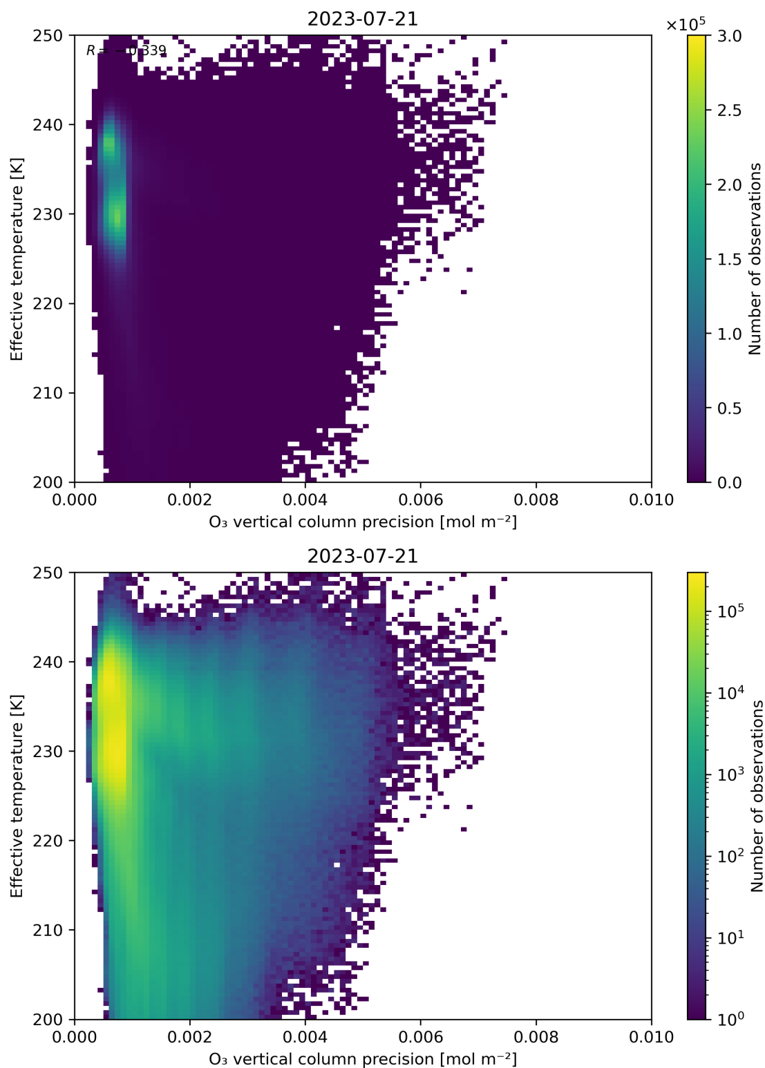
Figure 42: Scatter density plot of “O 3 vertical column precision” against “Effective temperature” for 2023-07-20 to 2023-07-22.
