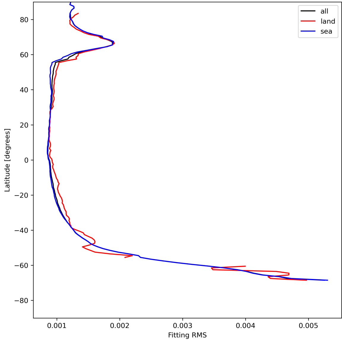
Figure 16: Zonal average of “Fitting RMS” for 2023-07-20 to 2023-07-22.
