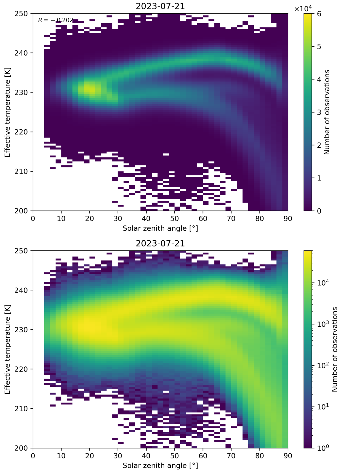
Figure 45: Scatter density plot of “Solar zenith angle” against “Effective temperature” for 2023-07-20 to 2023-07-22.
