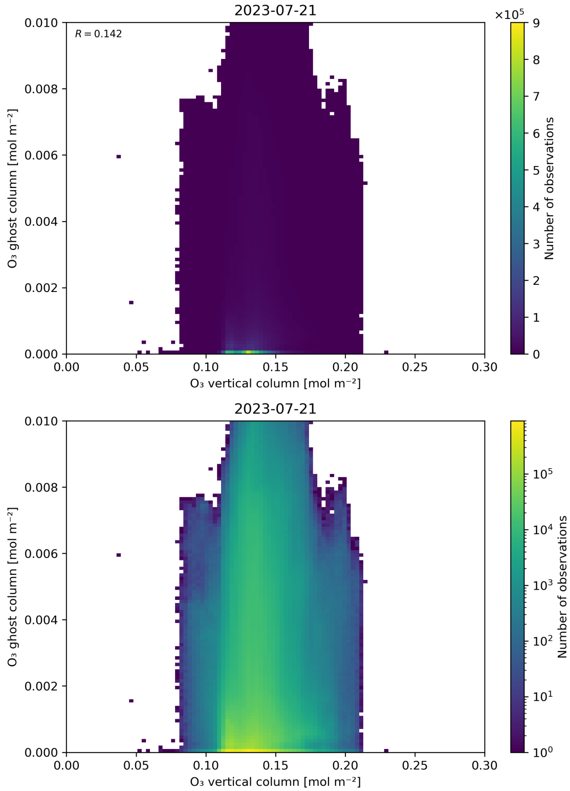
Figure 40: Scatter density plot of “O 3 vertical column” against “O 3 ghost column” for 2023-07-20 to 2023-07-22.
