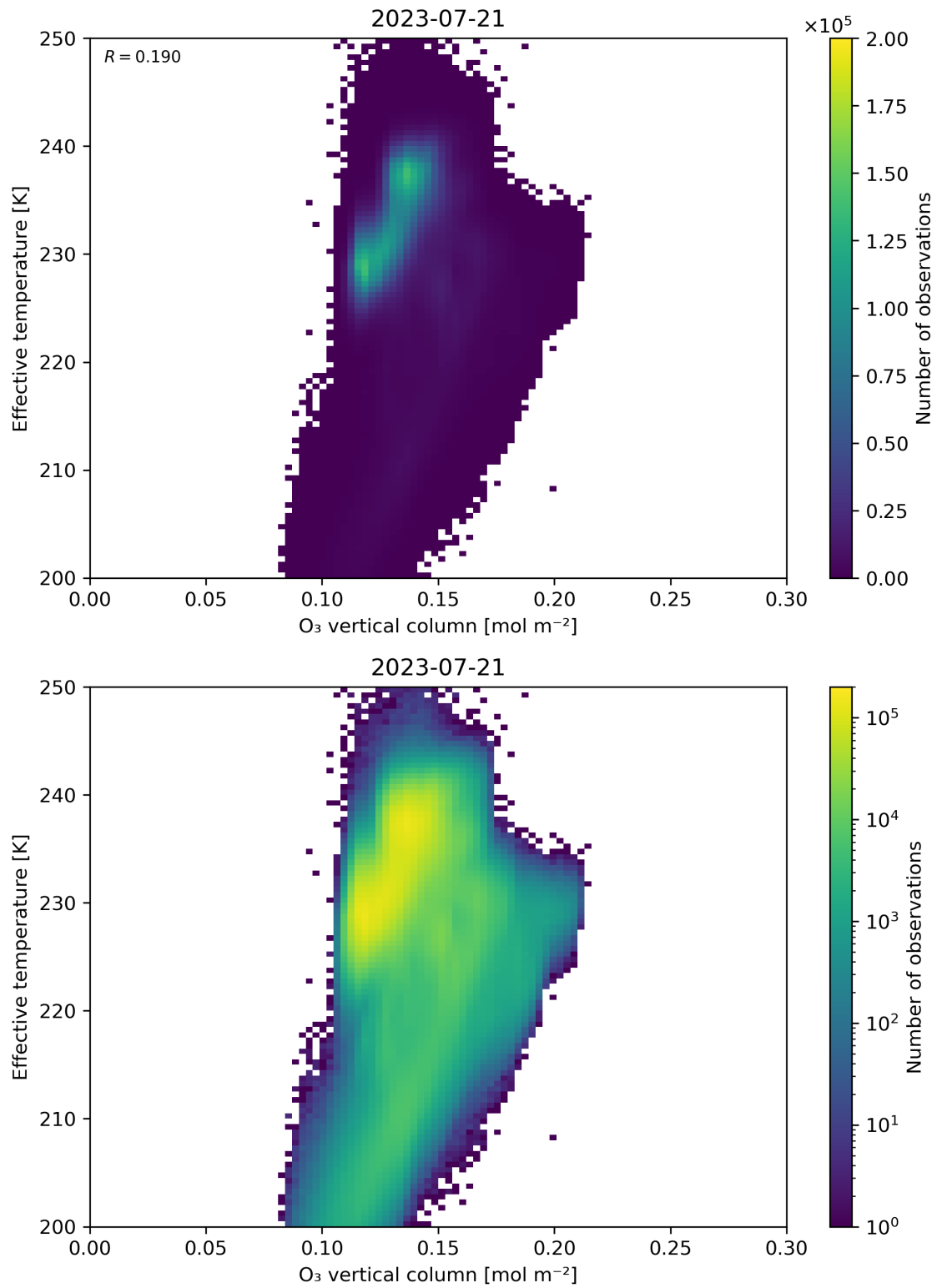
Figure 39: Scatter density plot of “O 3 vertical column” against “Effective temperature” for 2023-07-20 to 2023-07-22.
