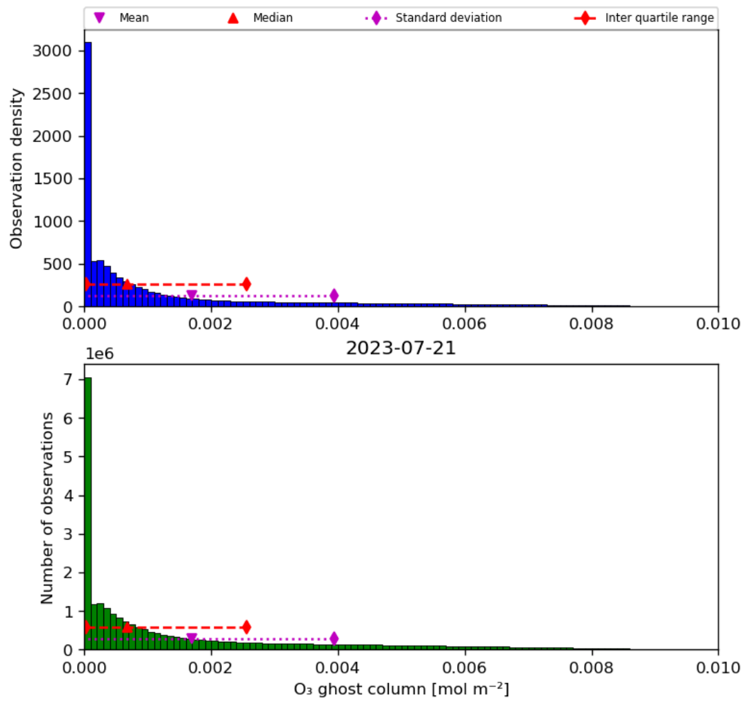
Figure 25: Histogram of “O 3 ghost column” for 2023-07-20 to 2023-07-22
