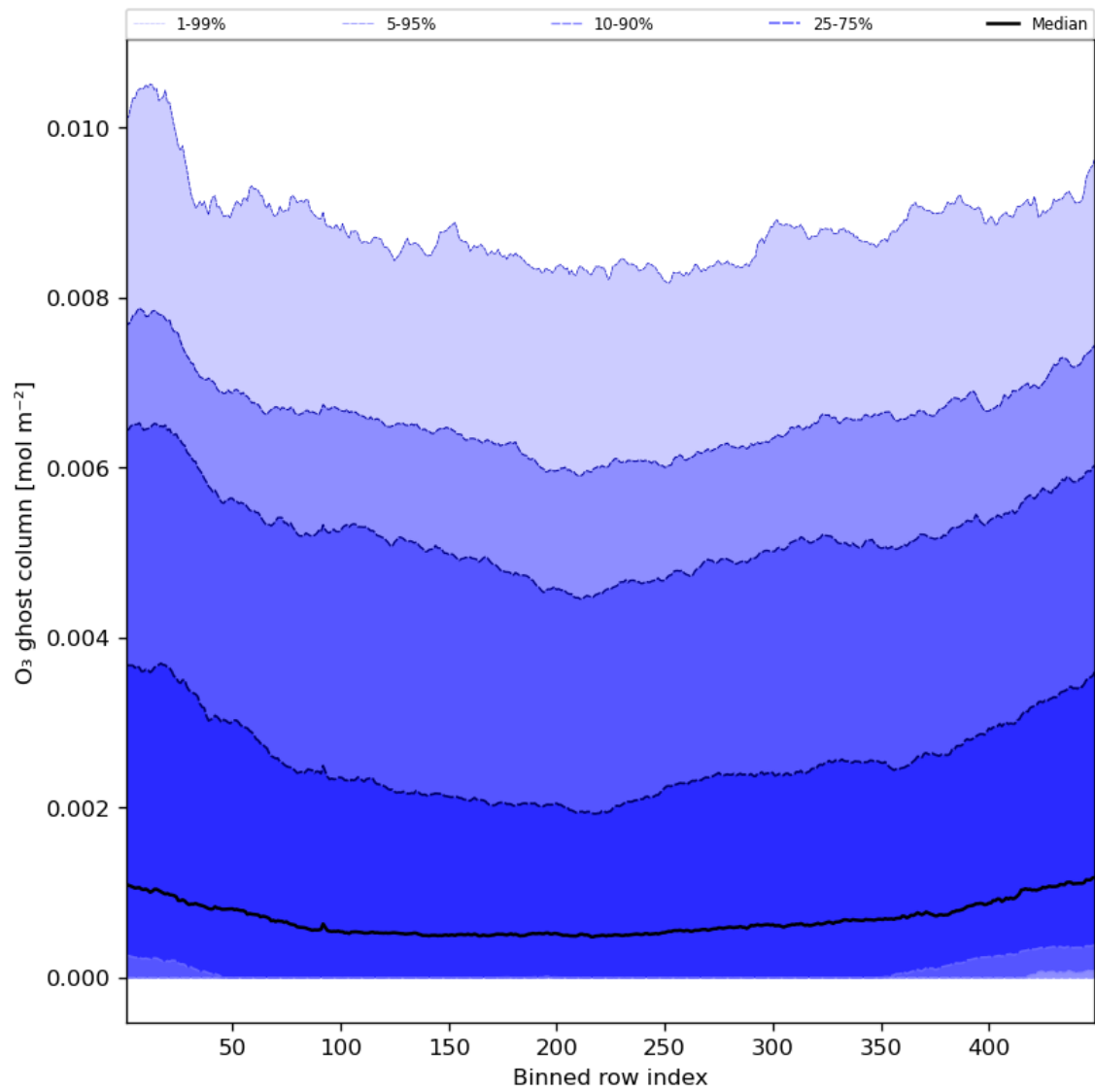
Figure 32: Along track statistics of “O 3 ghost column” for 2023-07-20 to 2023-07-22
