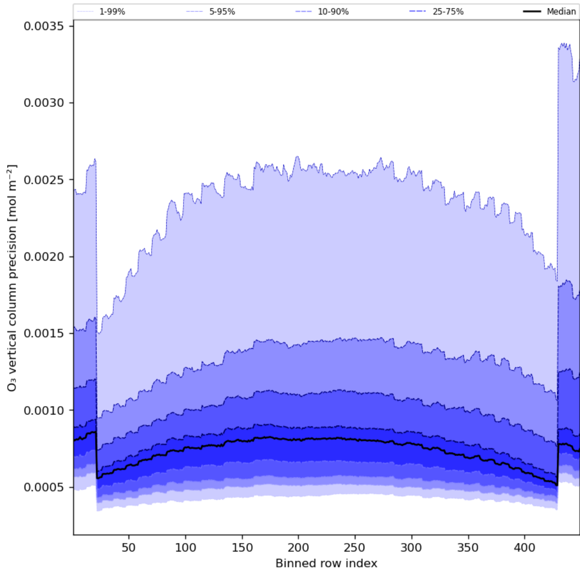
Figure 29: Along track statistics of “O 3 vertical column precision” for 2023-07-20 to 2023-07-22
