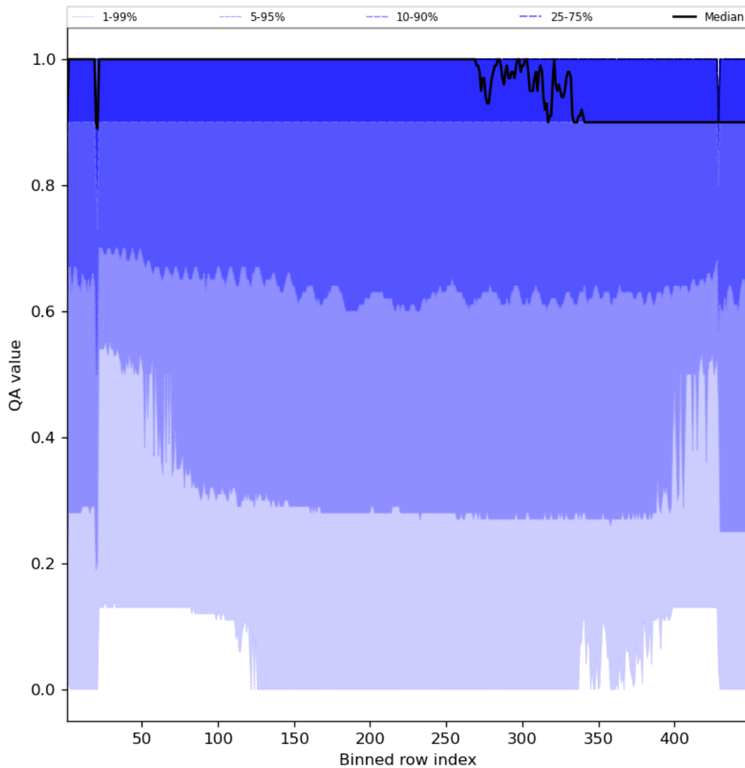
Figure 27: Along track statistics of “QA value” for 2023-07-20 to 2023-07-22
