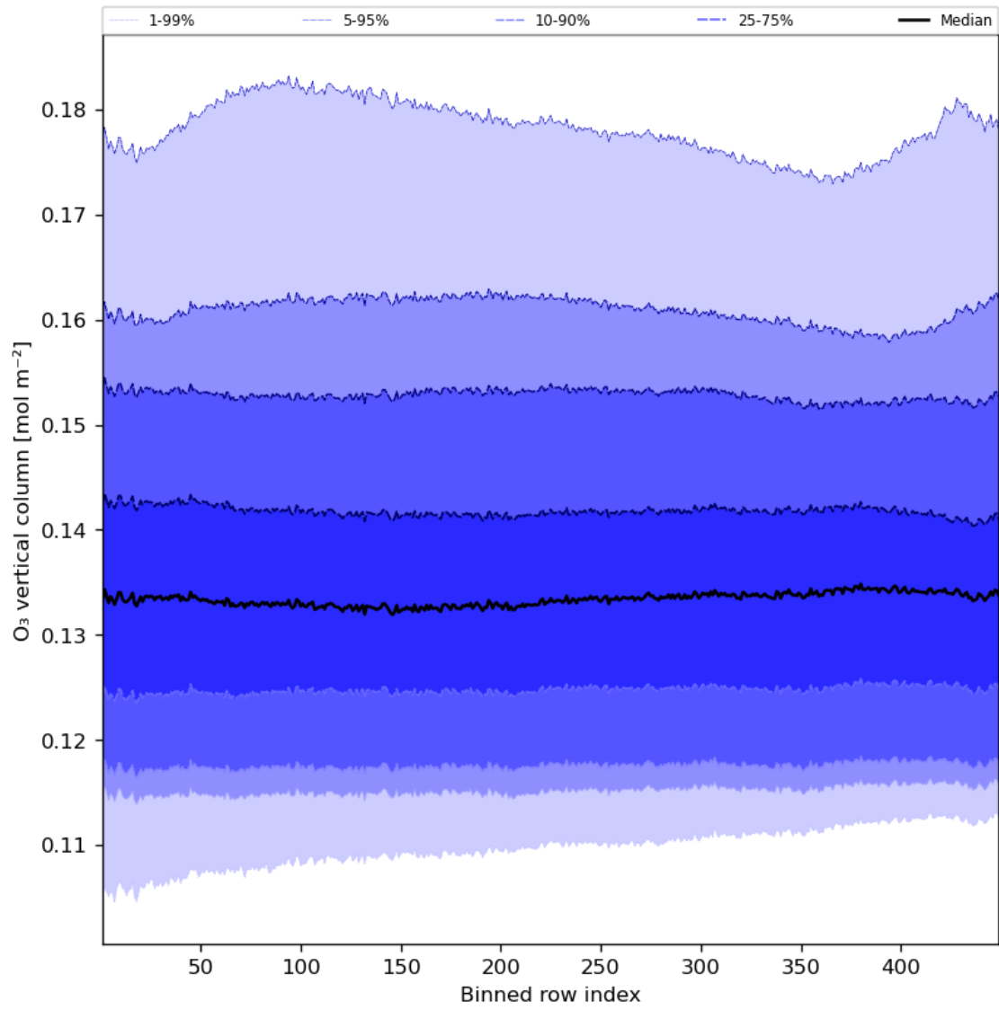
Figure 28: Along track statistics of “O 3 vertical column” for 2023-07-21 to 2023-07-23
