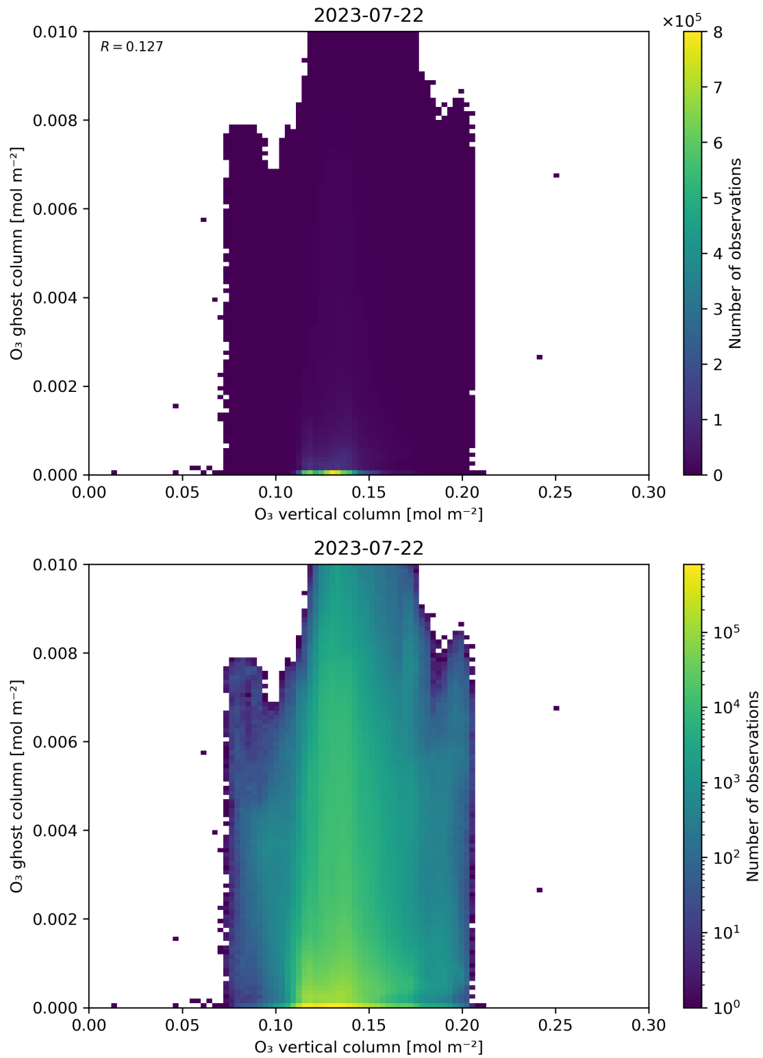
Figure 40: Scatter density plot of “O 3 vertical column” against “O 3 ghost column” for 2023-07-21 to 2023-07-23.
