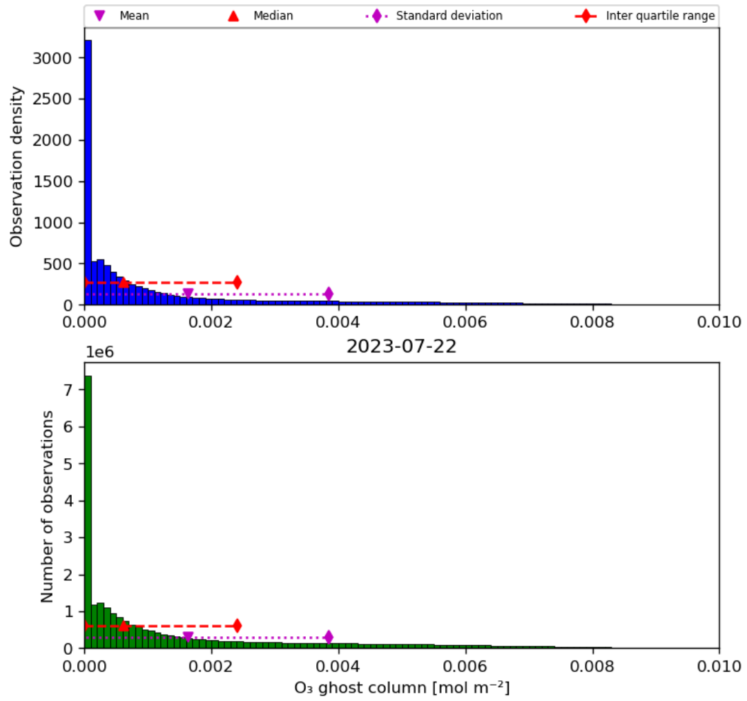
Figure 25: Histogram of “O 3 ghost column” for 2023-07-21 to 2023-07-23
