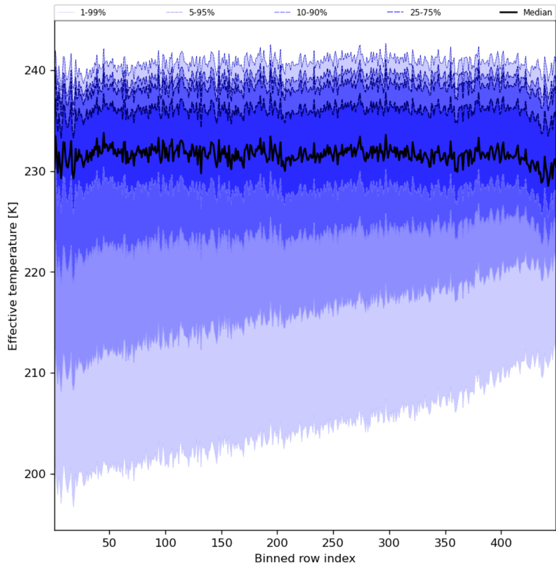
Figure 31: Along track statistics of “Effective temperature” for 2023-07-21 to 2023-07-23
