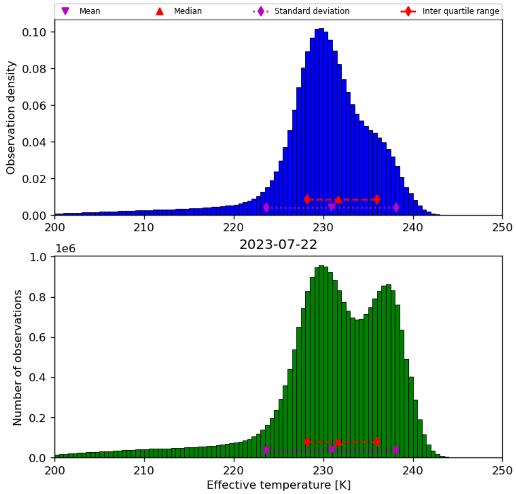
Figure 24: Histogram of “Effective temperature” for 2023-07-21 to 2023-07-23
