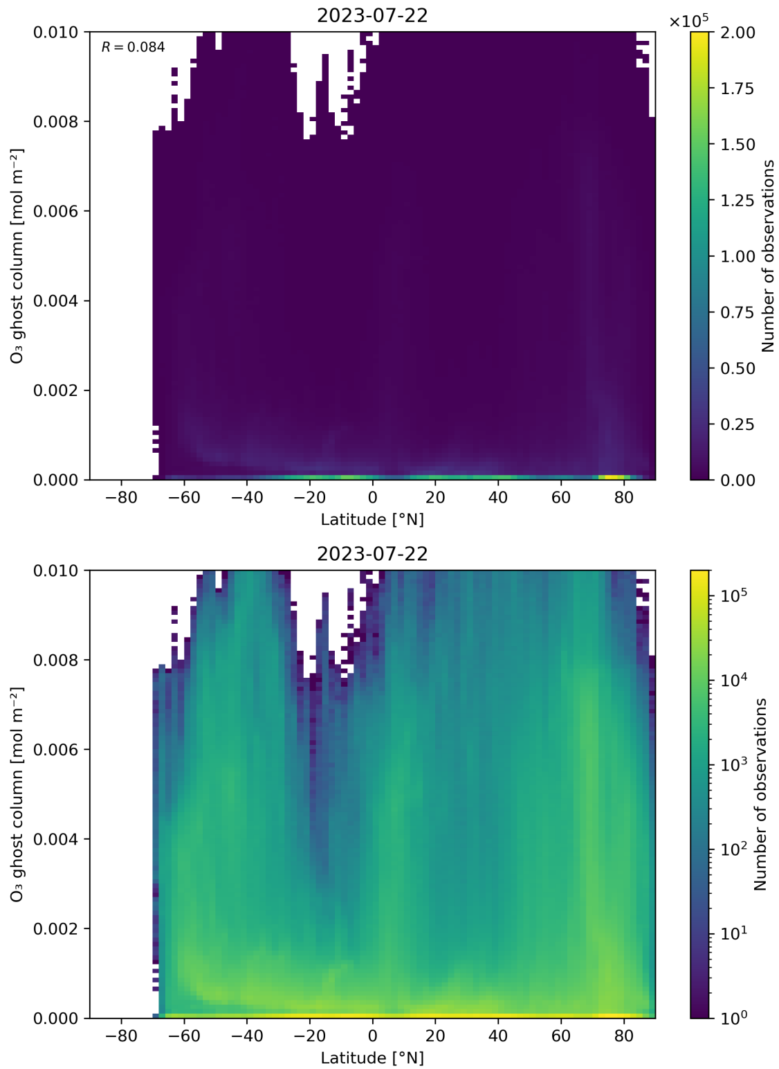
Figure 35: Scatter density plot of “Latitude” against “O 3 ghost column” for 2023-07-21 to 2023-07-23.
