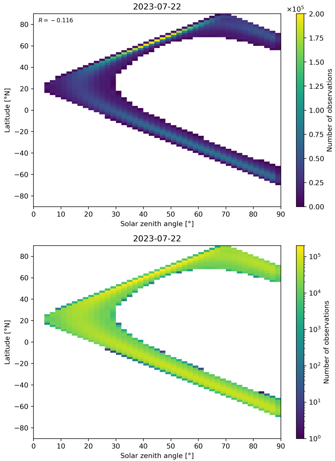
Figure 44: Scatter density plot of “Solar zenith angle” against “Latitude” for 2023-07-21 to 2023-07-23.
