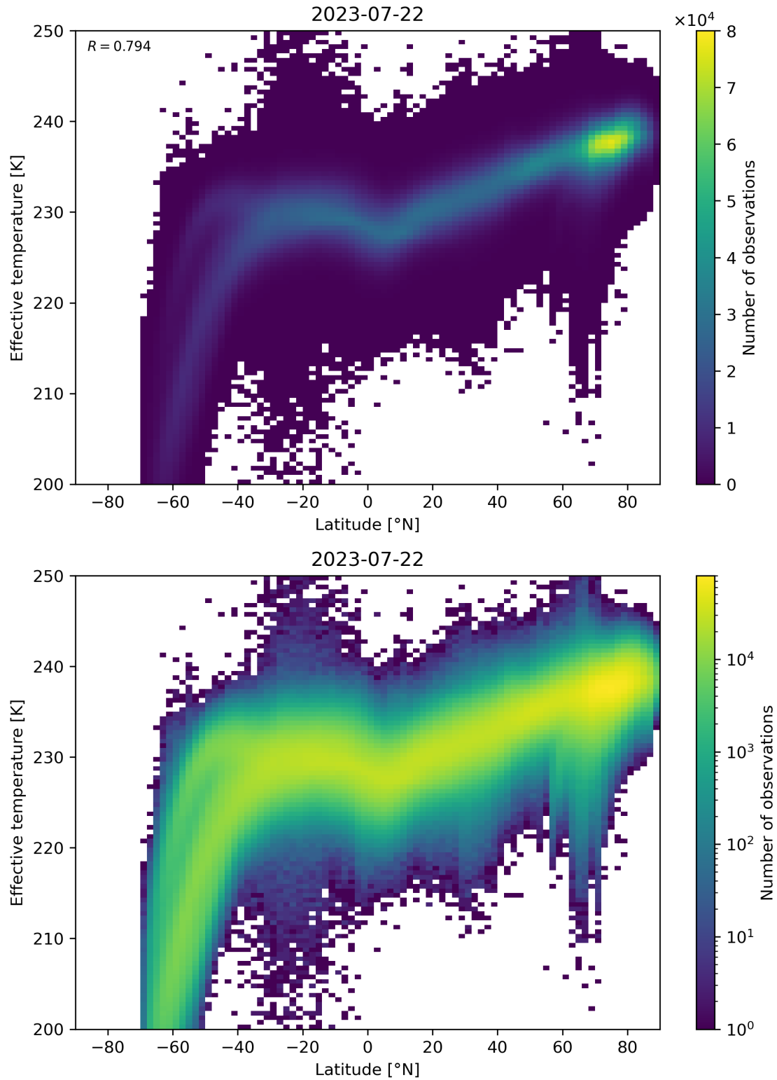
Figure 34: Scatter density plot of “Latitude” against “Effective temperature” for 2023-07-21 to 2023-07-23.
