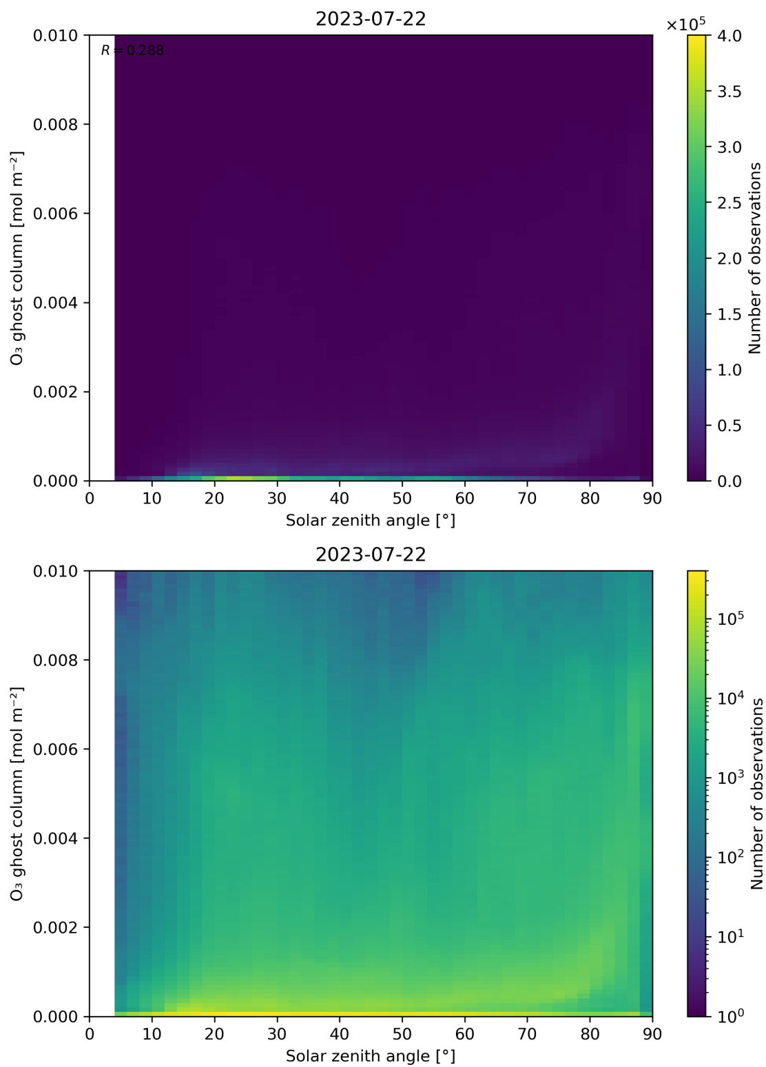
Figure 46: Scatter density plot of “Solar zenith angle” against “O 3 ghost column” for 2023-07-21 to 2023-07-23.
