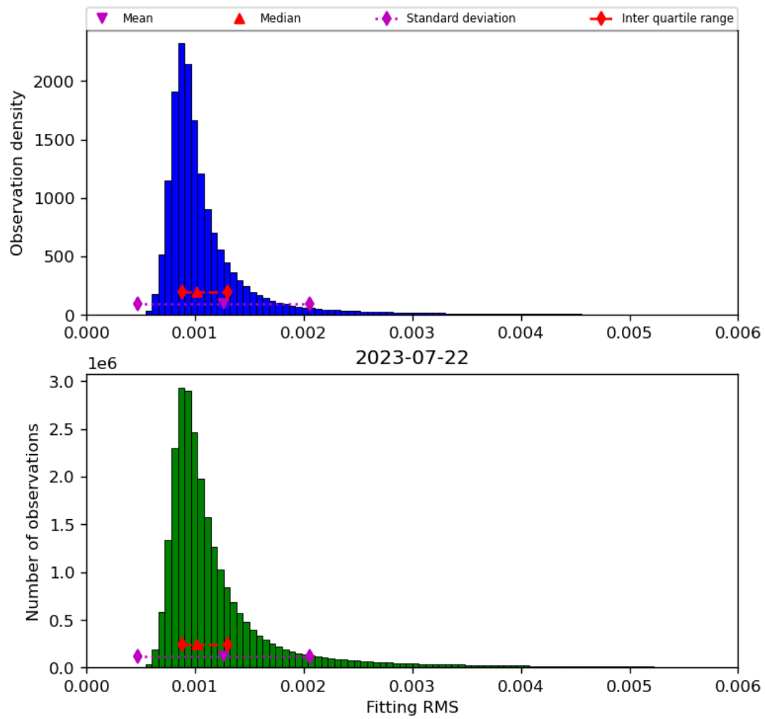
Figure 23: Histogram of “Fitting RMS” for 2023-07-21 to 2023-07-23
