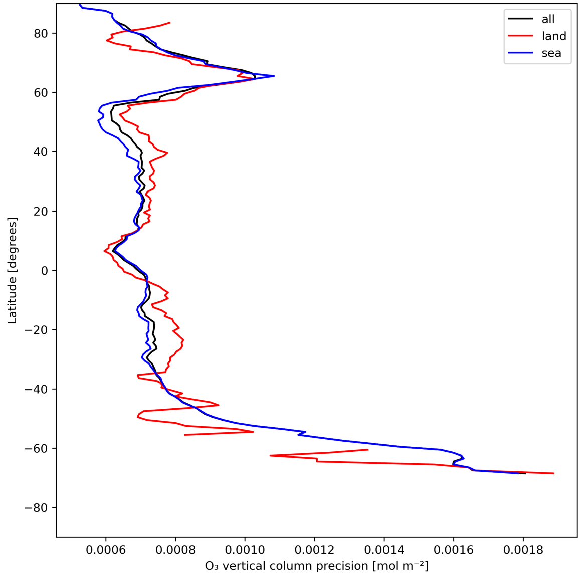
Figure 15: Zonal average of "O 3 vertical column precision" for 2023-07-21 to 2023-07-23.
