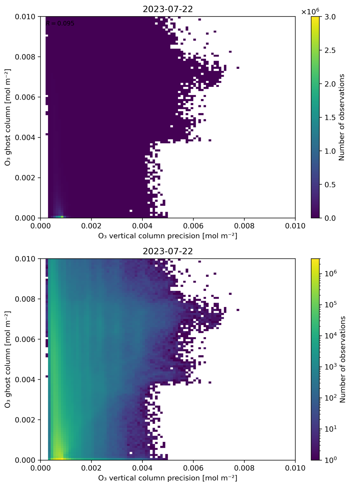
Figure 43: Scatter density plot of “O 3 vertical column precision” against “O 3 ghost column” for 2023-07-21 to 2023-07-23.
