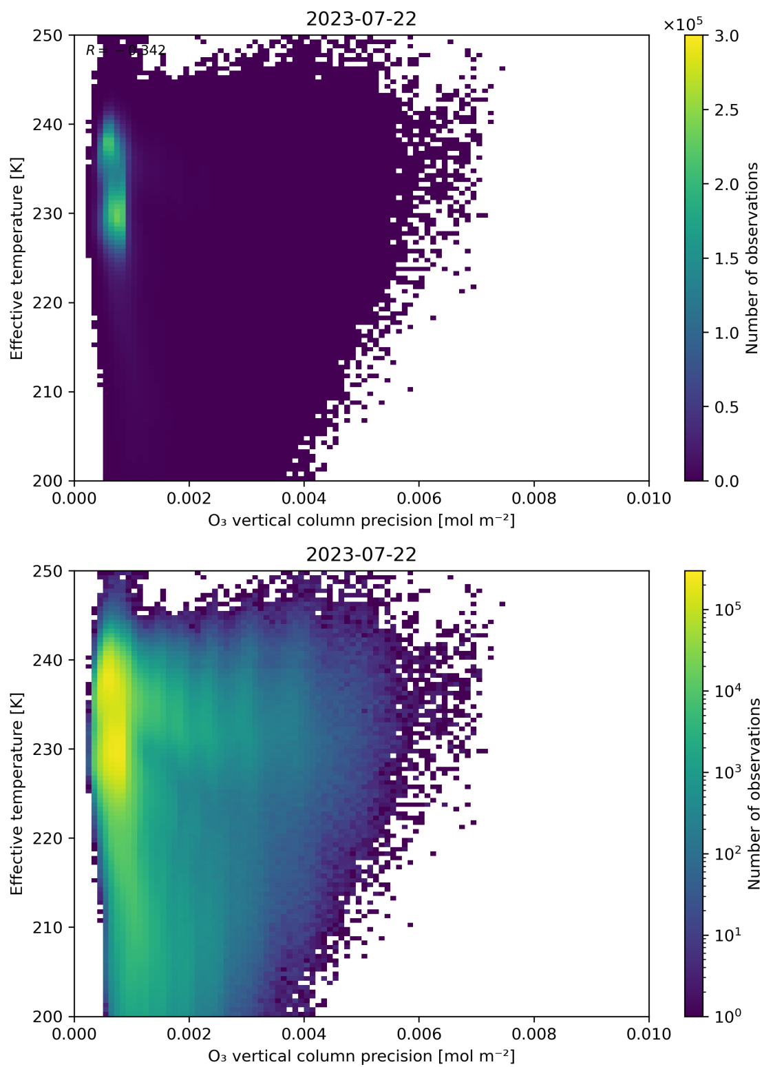
Figure 42: Scatter density plot of “O 3 vertical column precision” against “Effective temperature” for 2023-07-21 to 2023-07-23.
