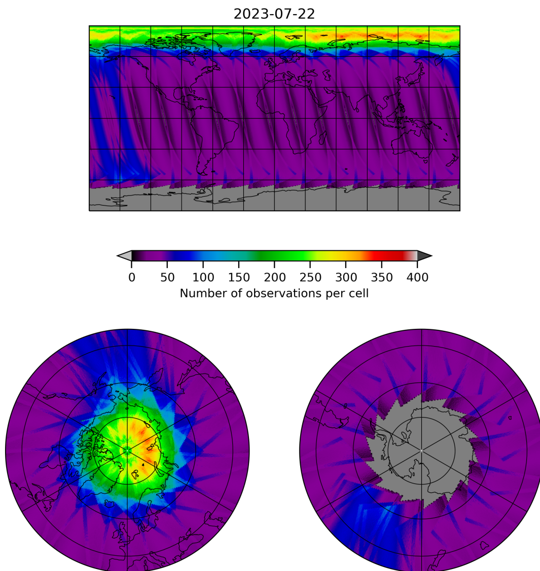
Figure 12: Map of the number of observations for 2023-07-21 to 2023-07-23
