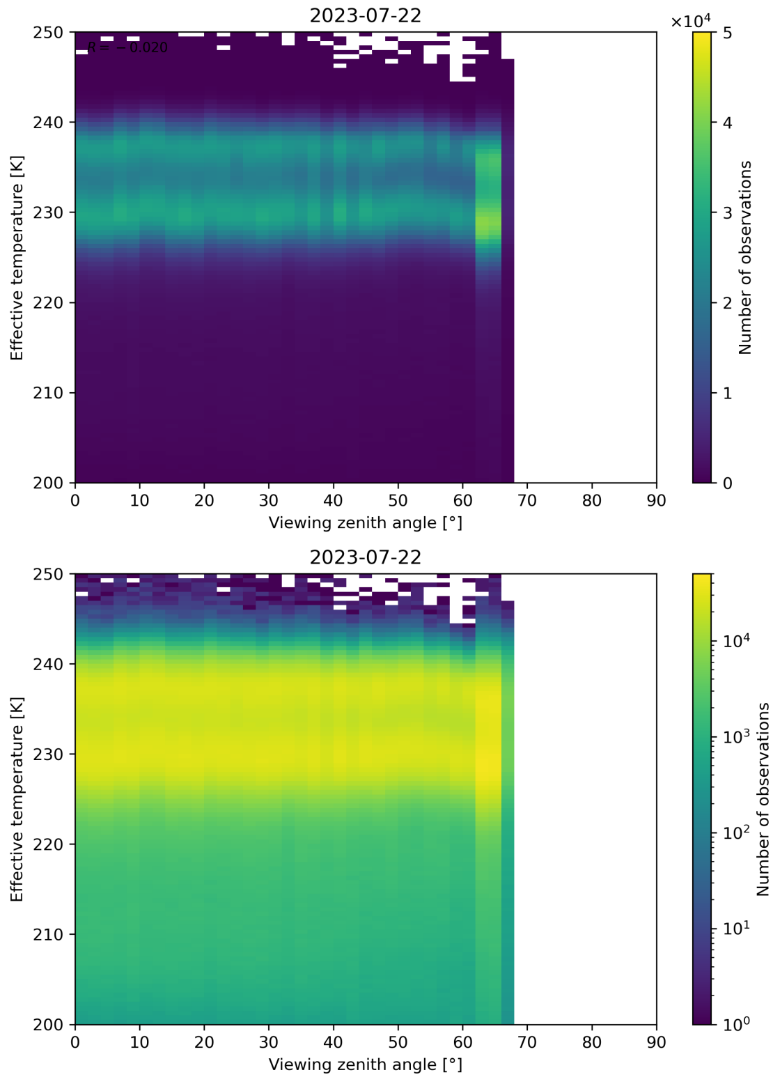
Figure 50: Scatter density plot of “Viewing zenith angle” against “Effective temperature” for 2023-07-21 to 2023-07-23.
