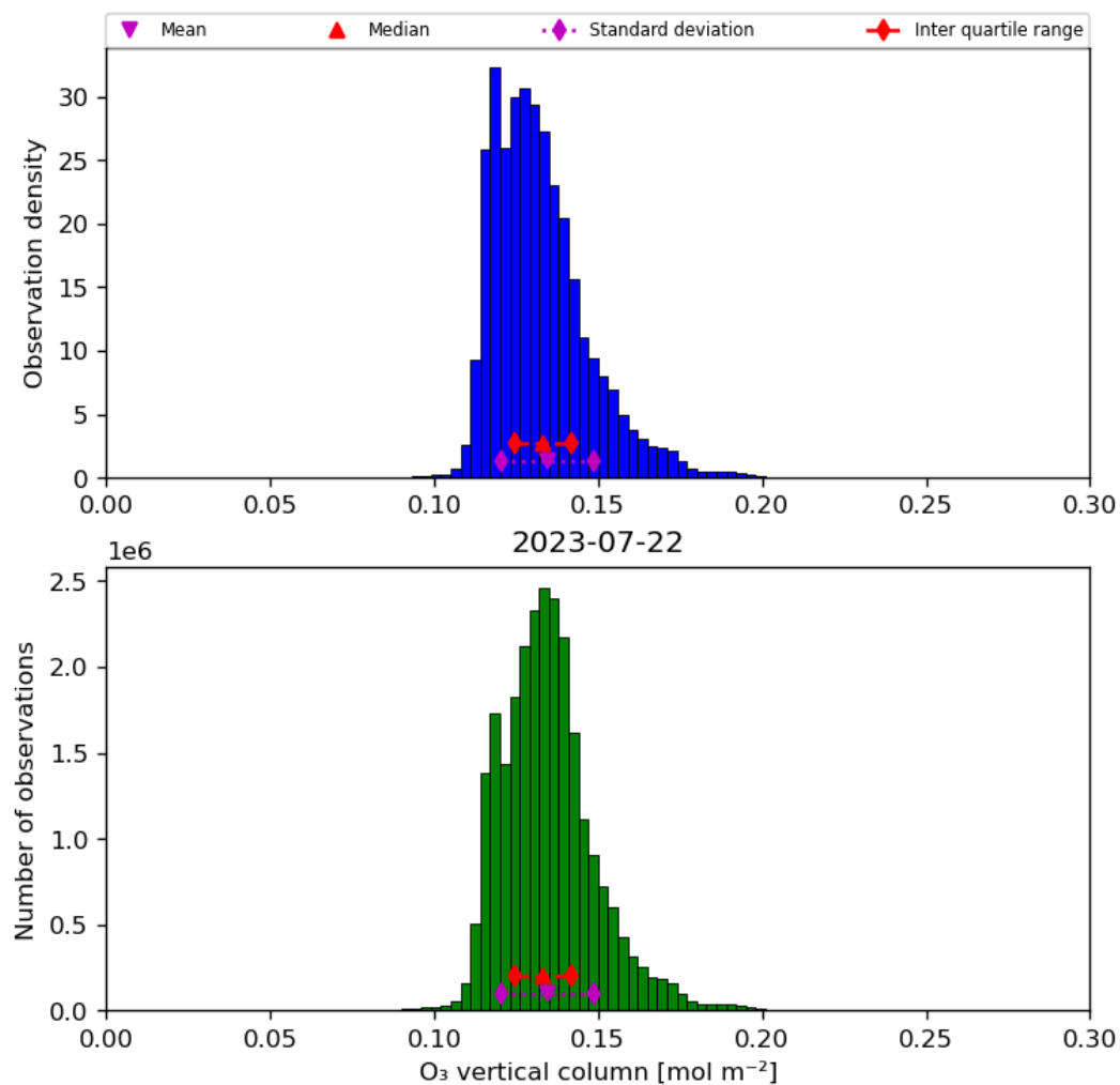
Figure 21: Histogram of “O 3 vertical column” for 2023-07-21 to 2023-07-23
