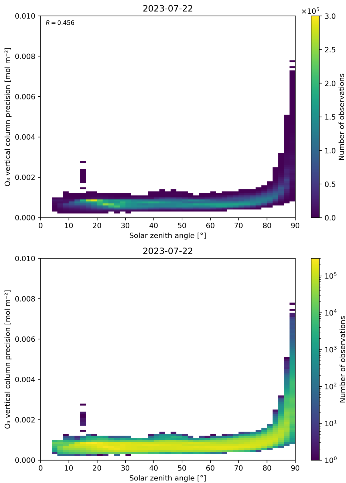
Figure 48: Scatter density plot of “Solar zenith angle” against “O 3 vertical column precision” for 2023-07-21 to 2023-07-23.
