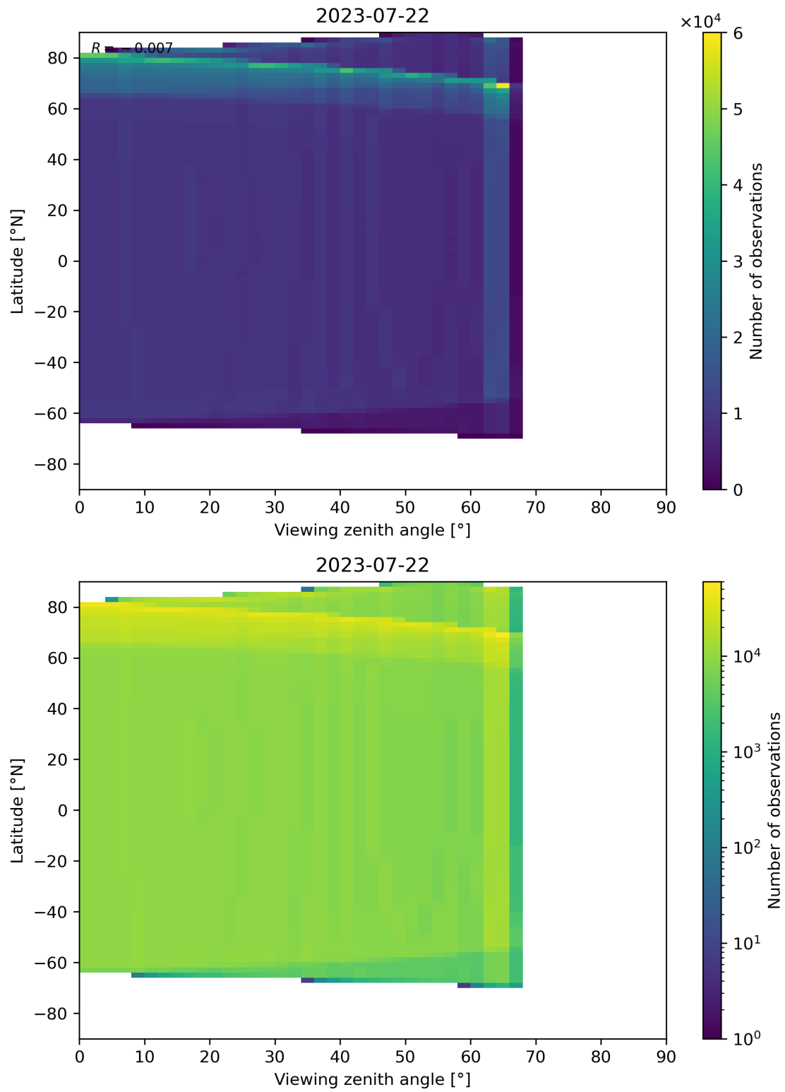
Figure 49: Scatter density plot of “Viewing zenith angle” against “Latitude” for 2023-07-21 to 2023-07-23.
