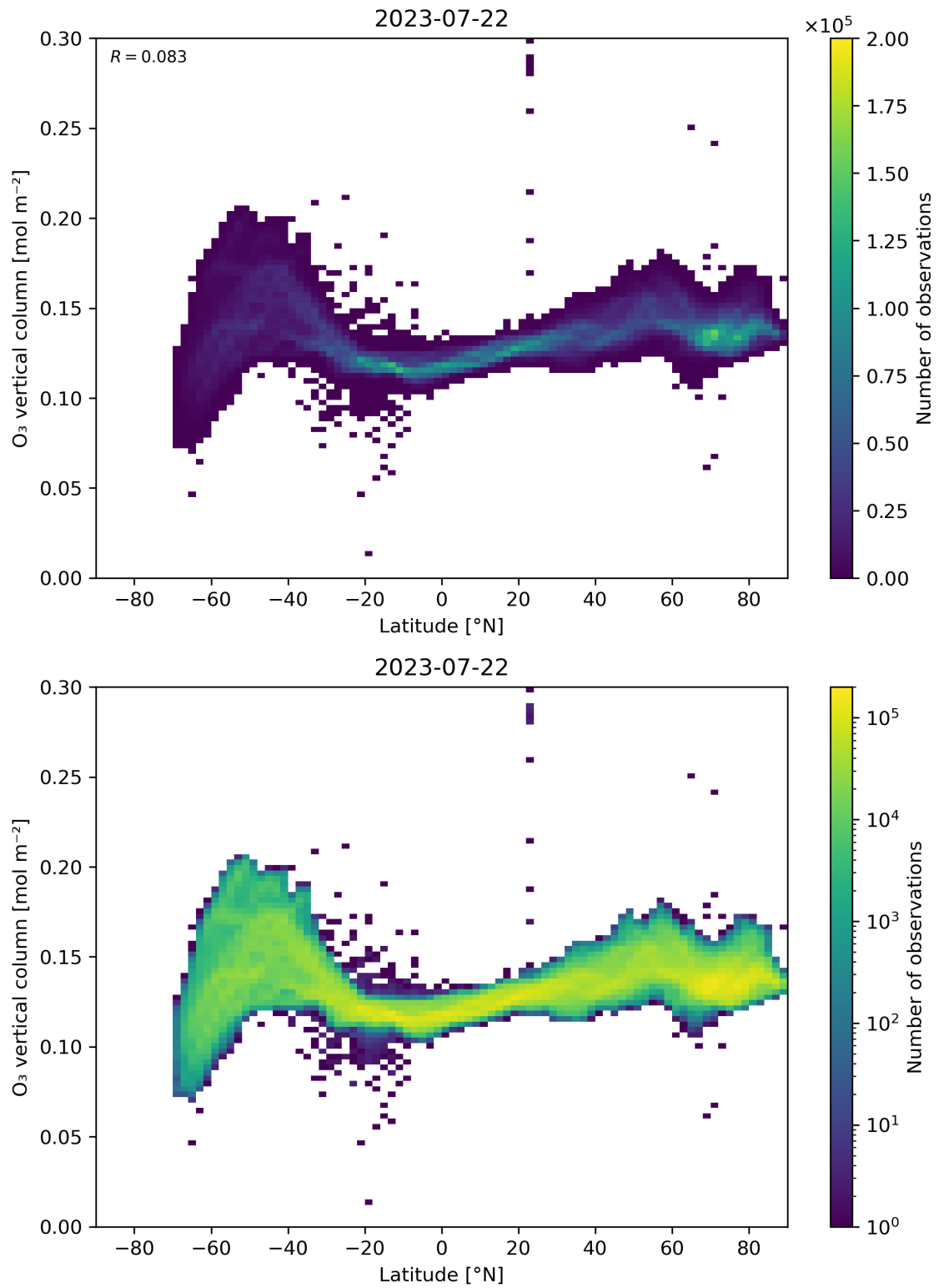
Figure 36: Scatter density plot of “Latitude” against “O 3 vertical column” for 2023-07-21 to 2023-07-23.
