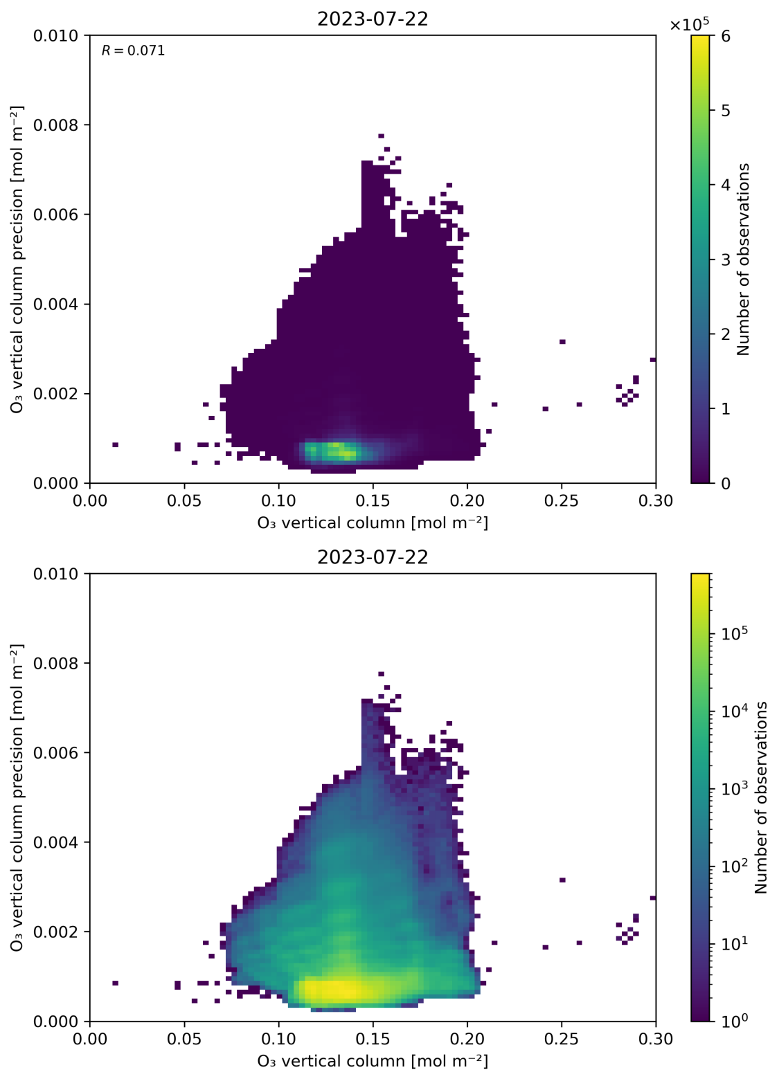
Figure 41: Scatter density plot of “O 3 vertical column” against “O 3 vertical column precision” for 2023-07-21 to 2023-07-23.
