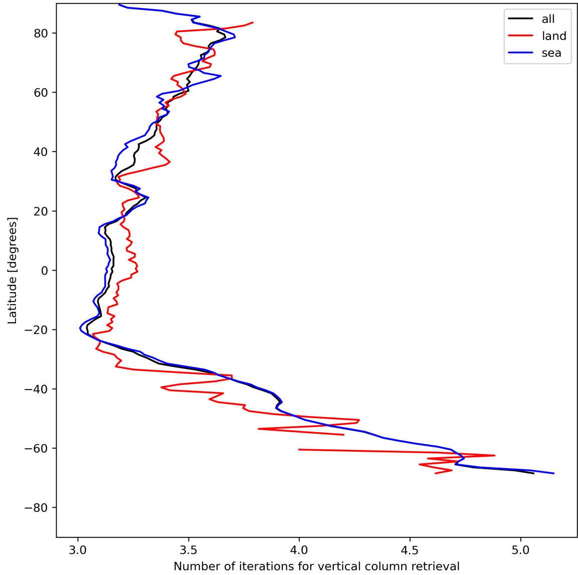
Figure 19: Zonal average of “Number of iterations for vertical column retrieval” for 2023-07-21 to 2023-07-23.
