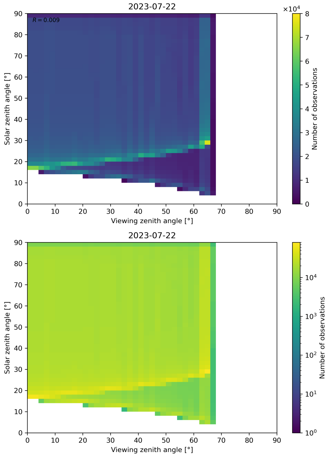
Figure 54: Scatter density plot of “Viewing zenith angle” against “Solar zenith angle” for 2023-07-21 to 2023-07-23.
