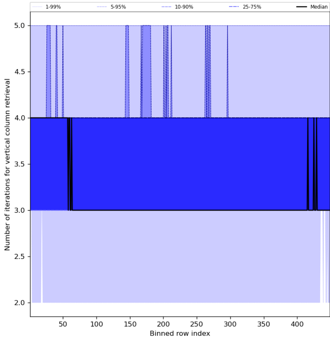
Figure 33: Along track statistics of “Number of iterations for vertical column retrieval” for 2023-07-21 to 2023-07-23
