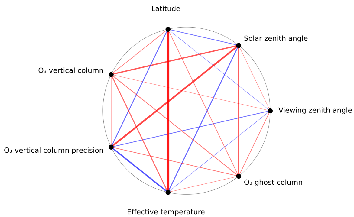
Figure 1: Map of correlation graph for 2023-07-21 to 2023-07-23.
