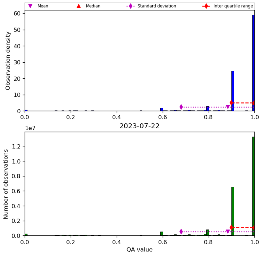
Figure 20: Histogram of “QA value” for 2023-07-21 to 2023-07-23
