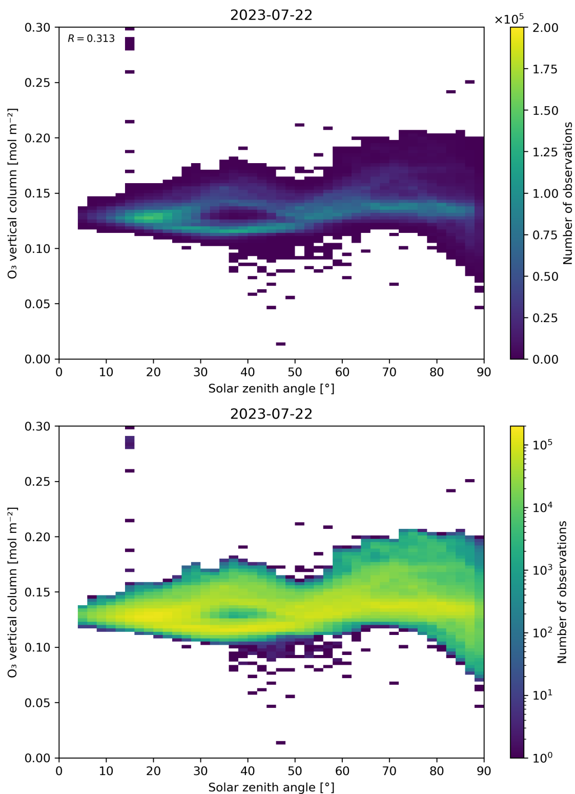
Figure 47: Scatter density plot of “Solar zenith angle” against “O 3 vertical column” for 2023-07-21 to 2023-07-23.
