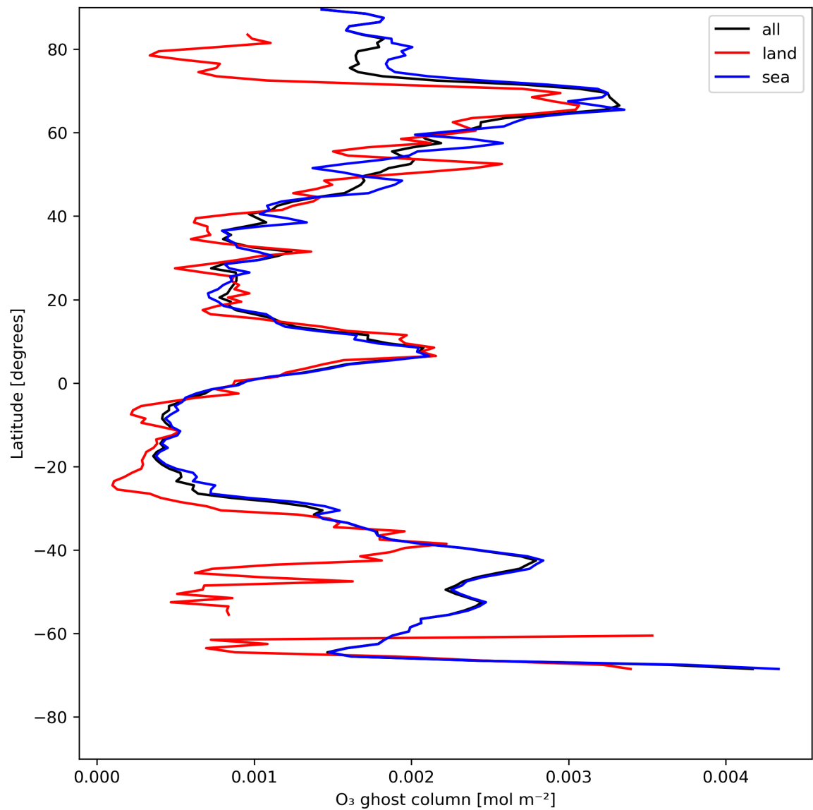
Figure 18: Zonal average of “O 3 ghost column” for 2023-07-21 to 2023-07-23.
