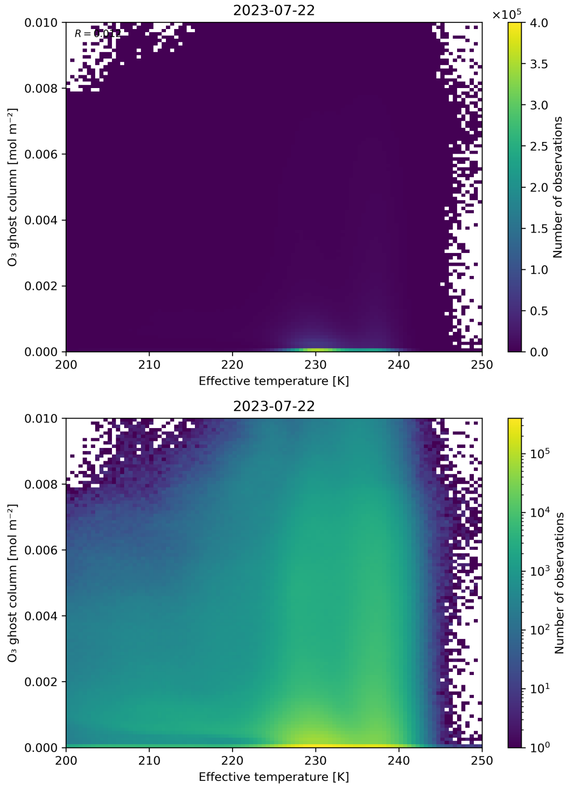
Figure 38: Scatter density plot of “Effective temperature” against “O 3 ghost column” for 2023-07-21 to 2023-07-23.
