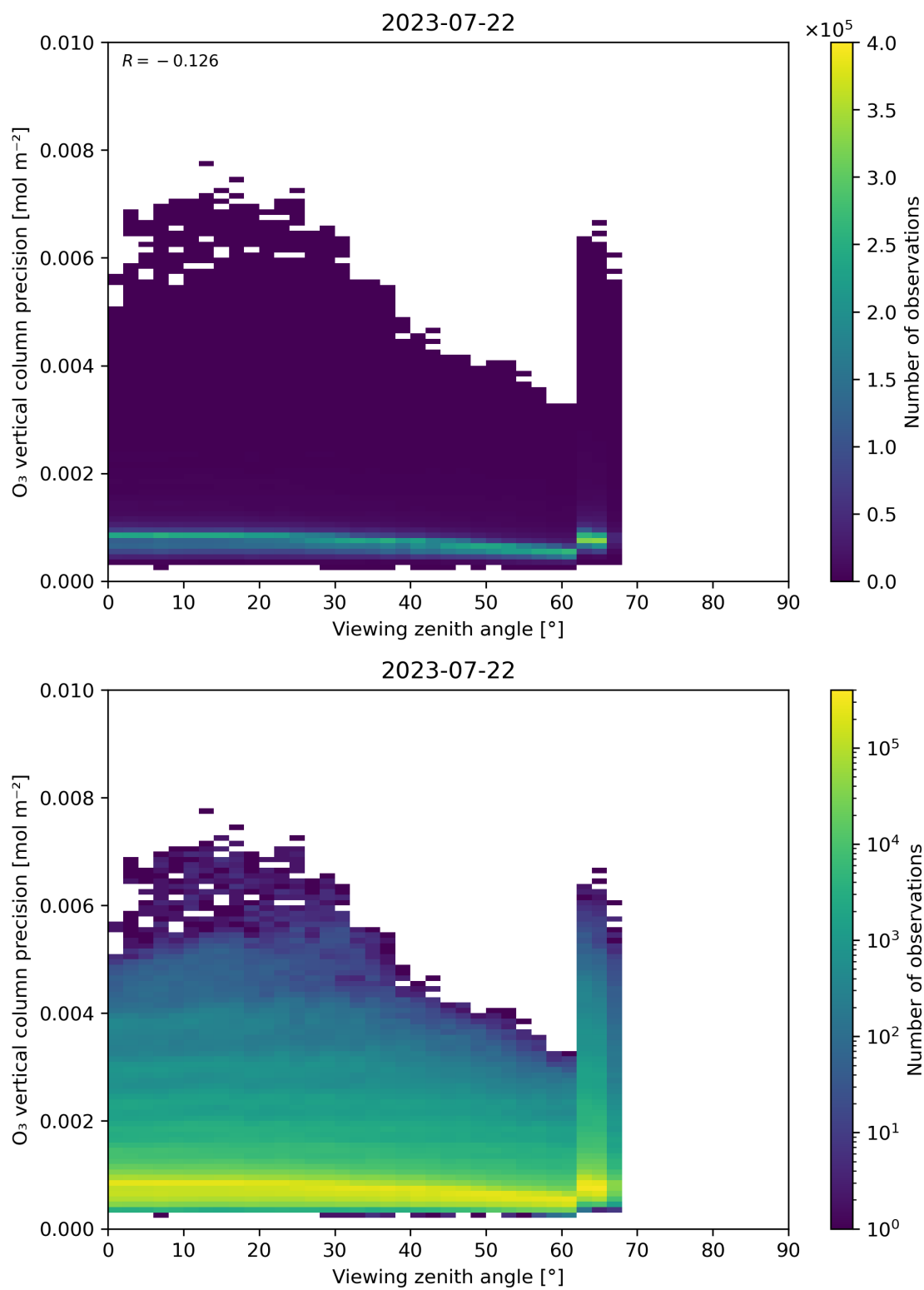
Figure 53: Scatter density plot of “Viewing zenith angle” against “O 3 vertical column precision” for 2023-07-21 to 2023-07-23.
