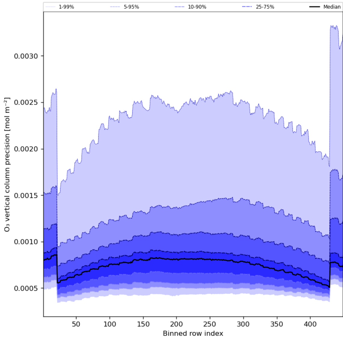
Figure 29: Along track statistics of “O 3 vertical column precision” for 2023-07-21 to 2023-07-23
