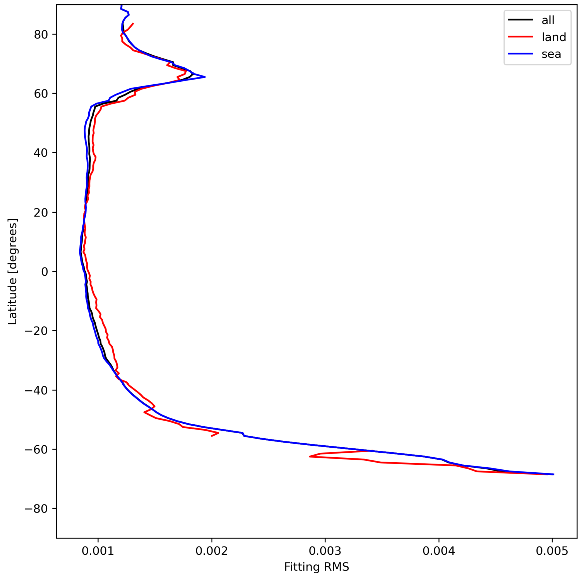
Figure 16: Zonal average of “Fitting RMS” for 2023-07-21 to 2023-07-23.
