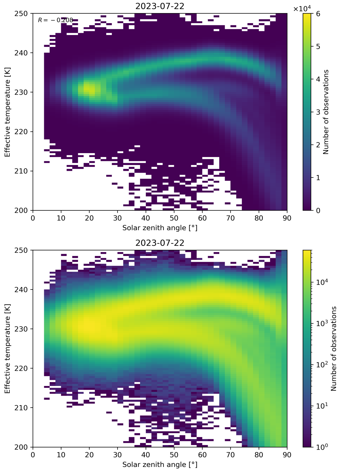
Figure 45: Scatter density plot of “Solar zenith angle” against “Effective temperature” for 2023-07-21 to 2023-07-23.
