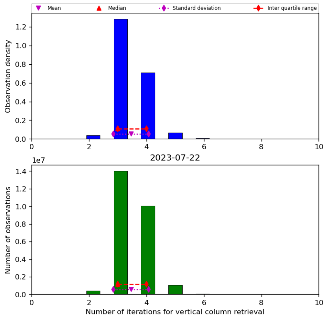
Figure 26: Histogram of “Number of iterations for vertical column retrieval” for 2023-07-21 to 2023-07-23
