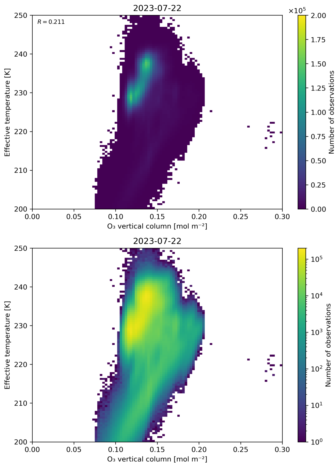
Figure 39: Scatter density plot of “O 3 vertical column” against “Effective temperature” for 2023-07-21 to 2023-07-23.
