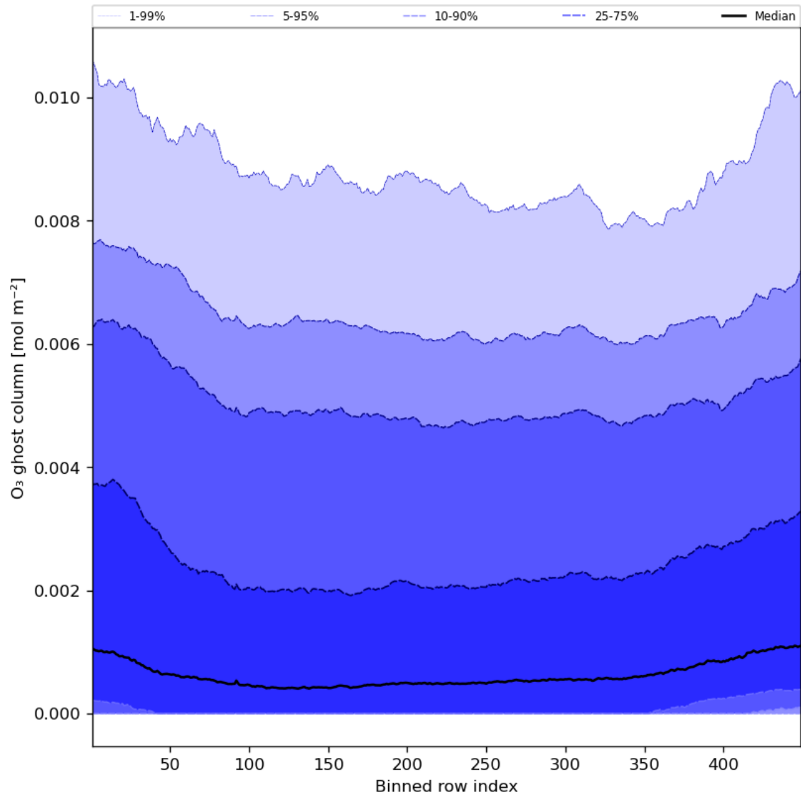
Figure 32: Along track statistics of “O 3 ghost column” for 2023-07-21 to 2023-07-23
