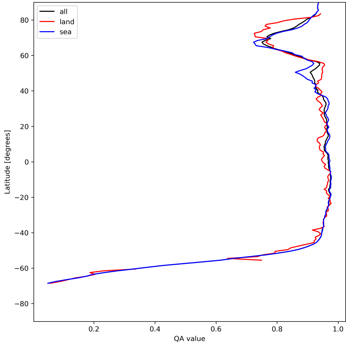
Figure 13: Zonal average of “QA value” for 2023-07-21 to 2023-07-23.
