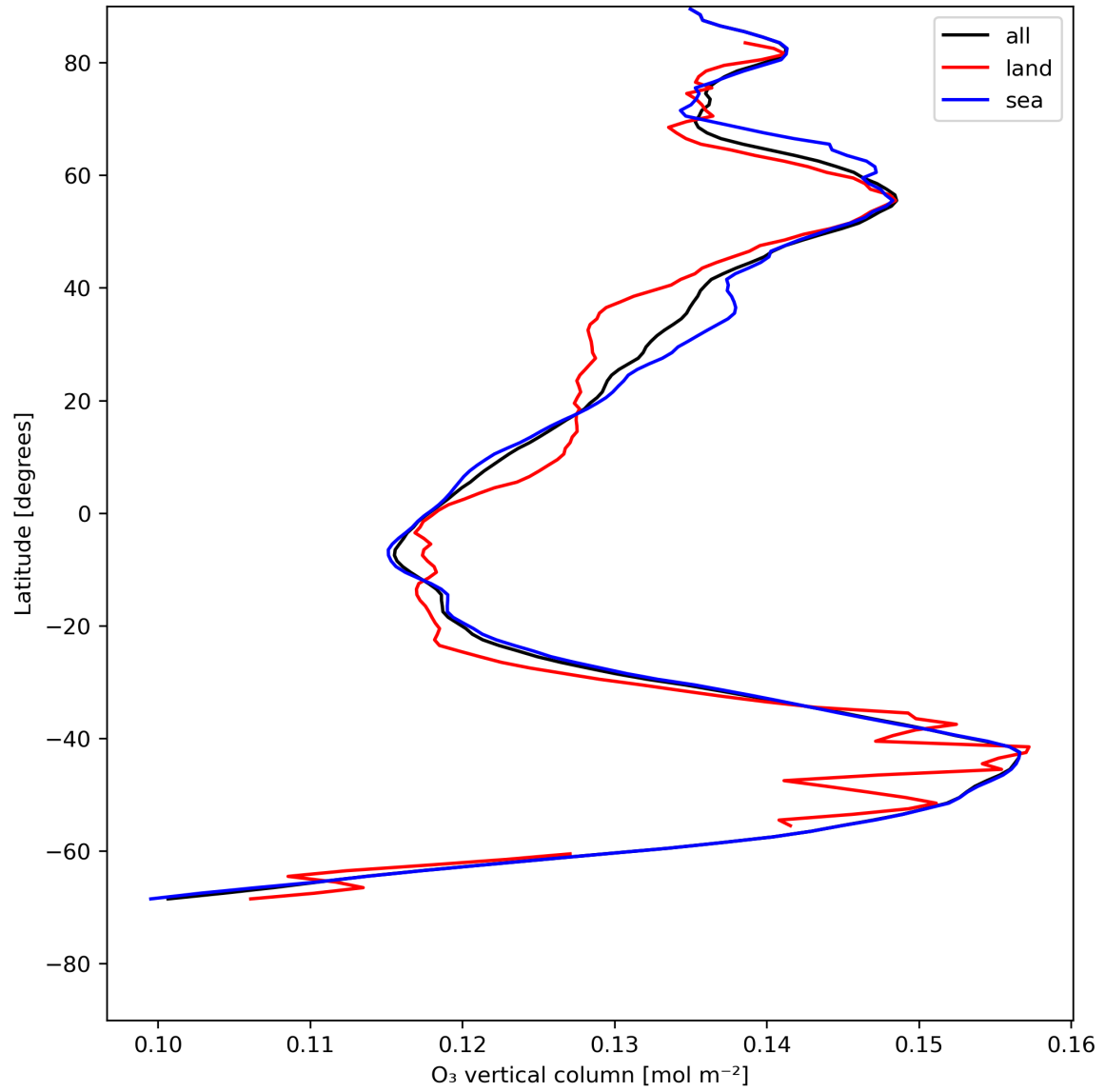
Figure 14: Zonal average of “O 3 vertical column” for 2023-07-21 to 2023-07-23.
