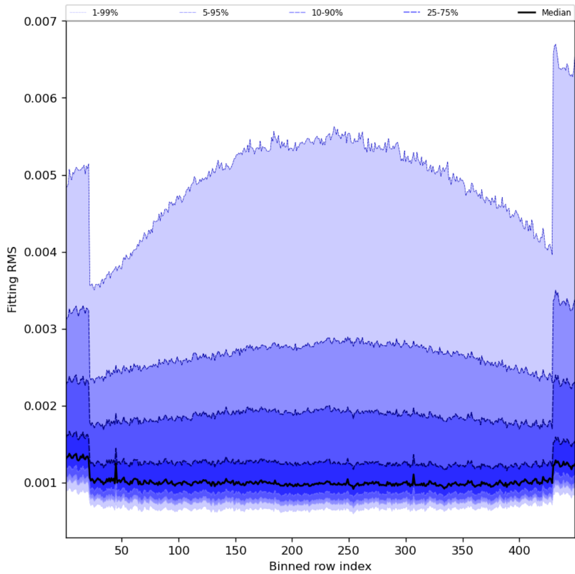
Figure 30: Along track statistics of “Fitting RMS” for 2023-07-21 to 2023-07-23
