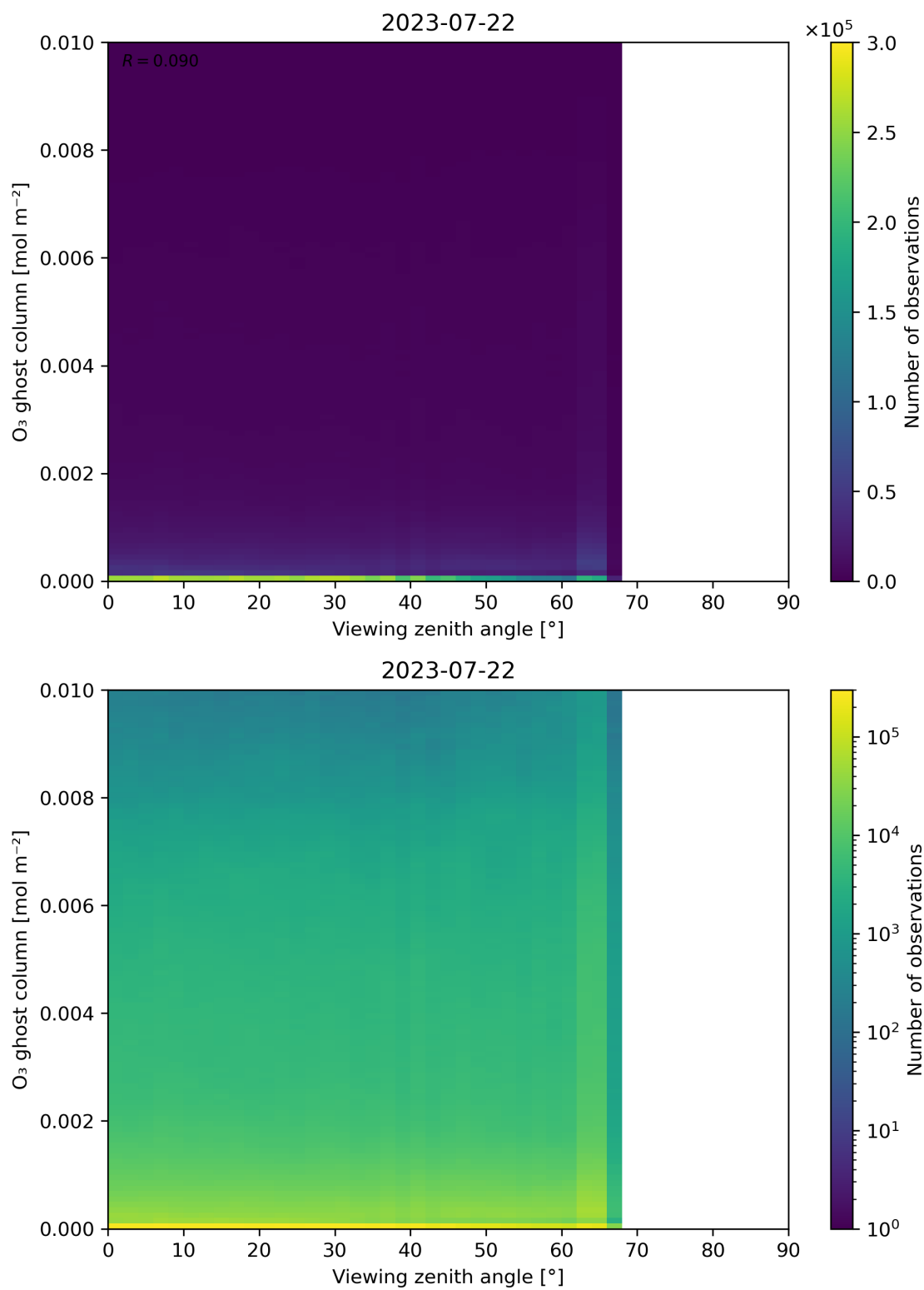
Figure 51: Scatter density plot of “Viewing zenith angle” against “O 3 ghost column” for 2023-07-21 to 2023-07-23.
