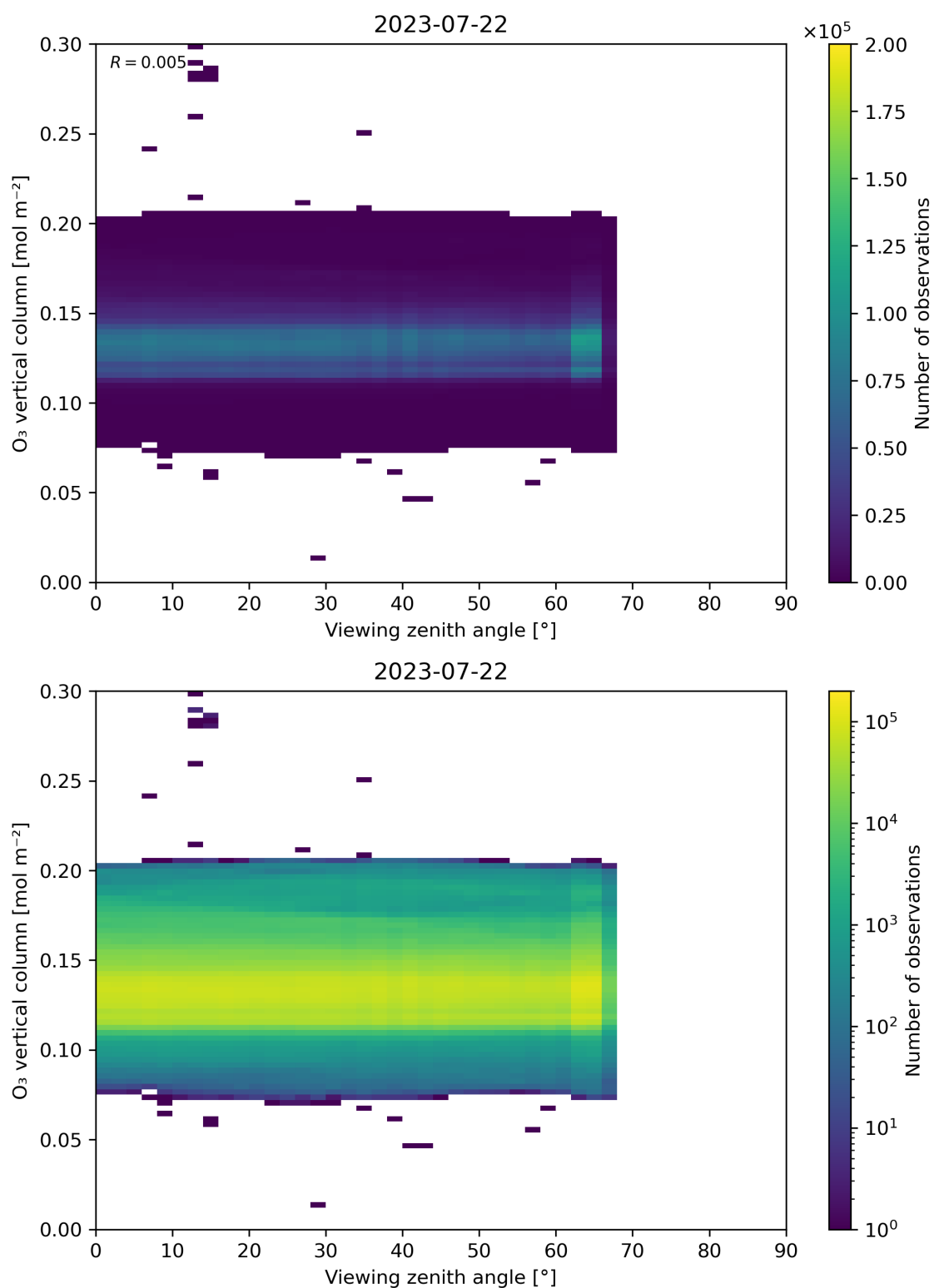
Figure 52: Scatter density plot of “Viewing zenith angle” against “O 3 vertical column” for 2023-07-21 to 2023-07-23.
