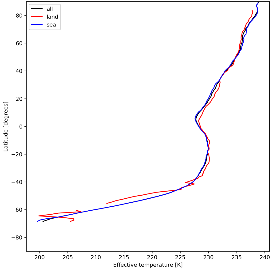
Figure 17: Zonal average of “Effective temperature” for 2023-07-21 to 2023-07-23.
