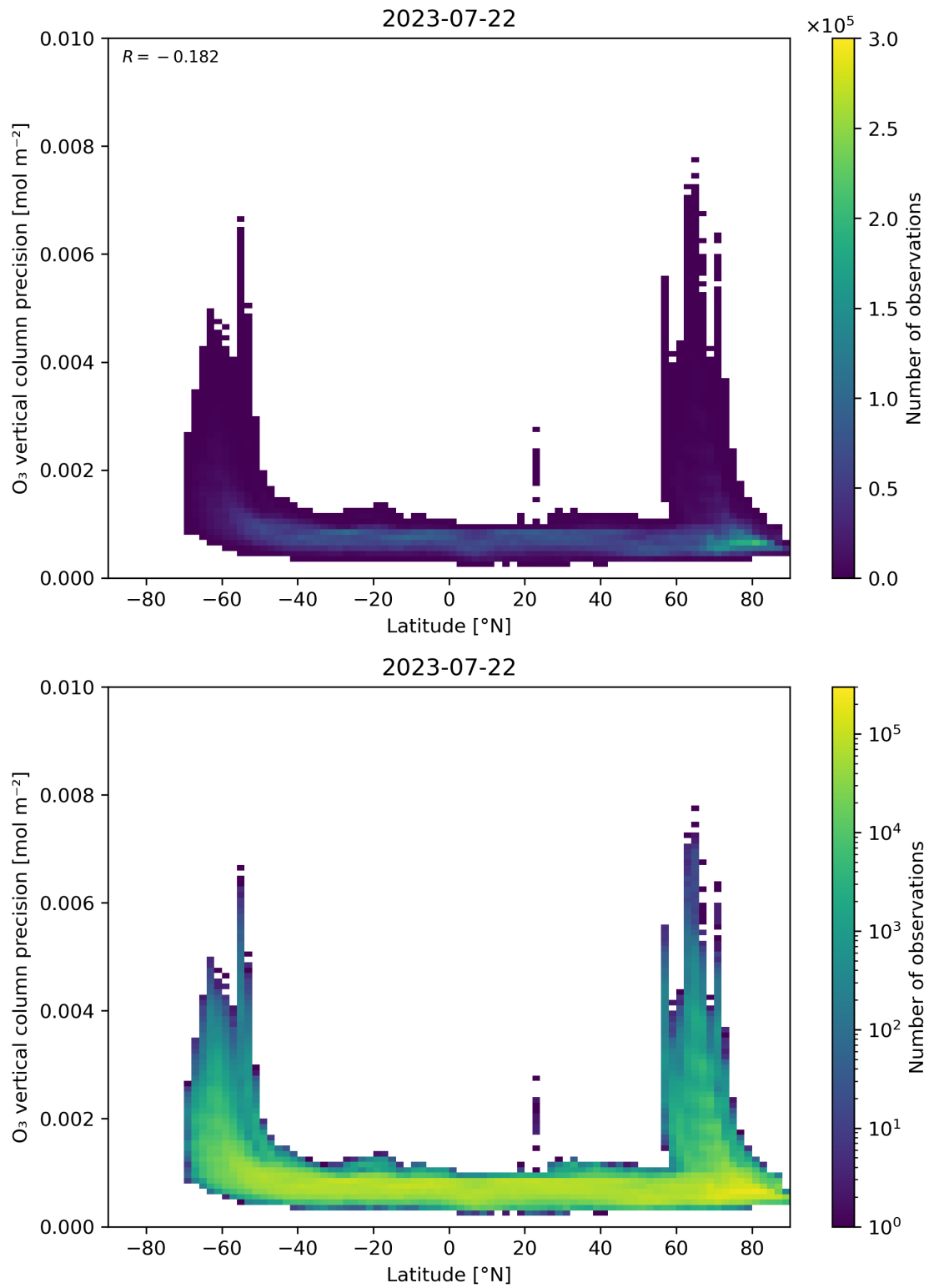
Figure 37: Scatter density plot of “Latitude” against “O 3 vertical column precision” for 2023-07-21 to 2023-07-23.
