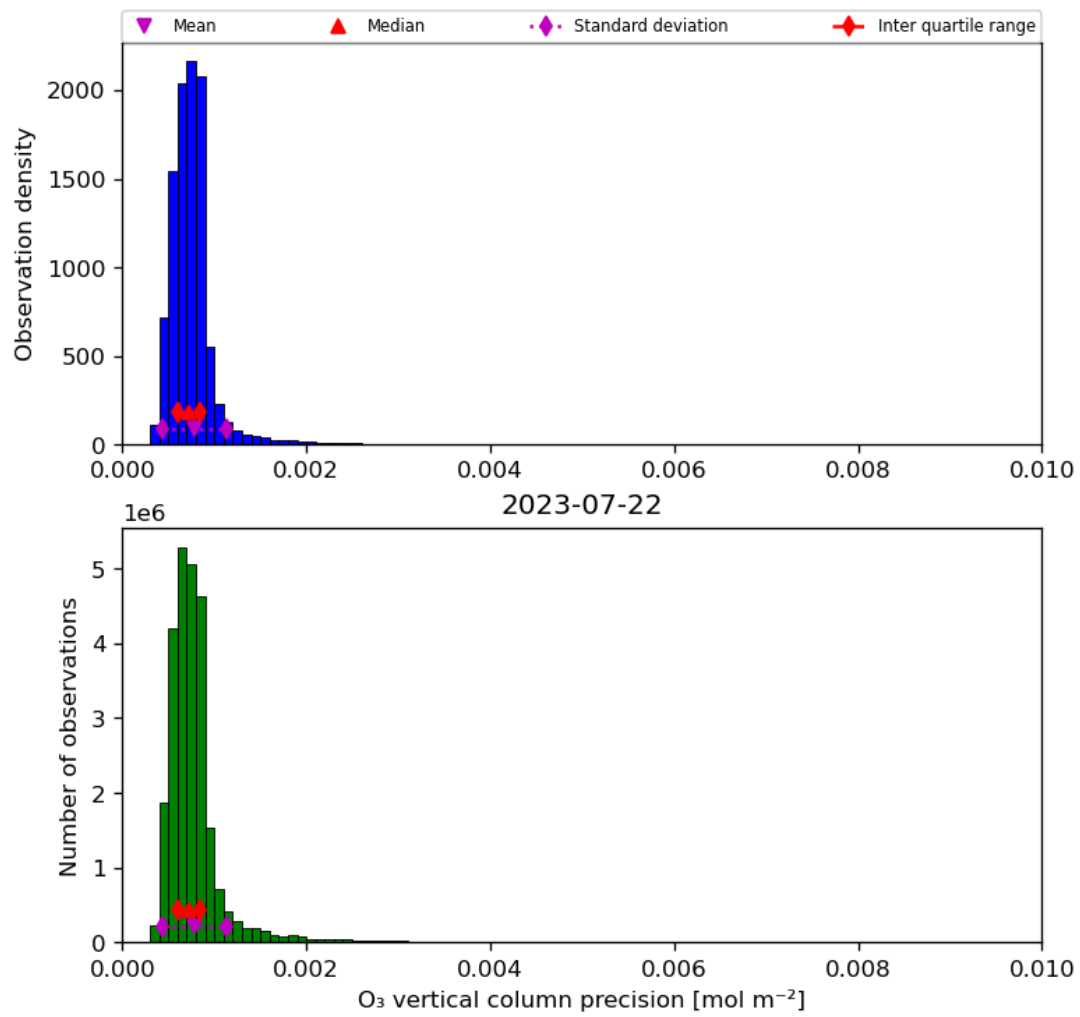
Figure 22: Histogram of “O 3 vertical column precision” for 2023-07-21 to 2023-07-23
