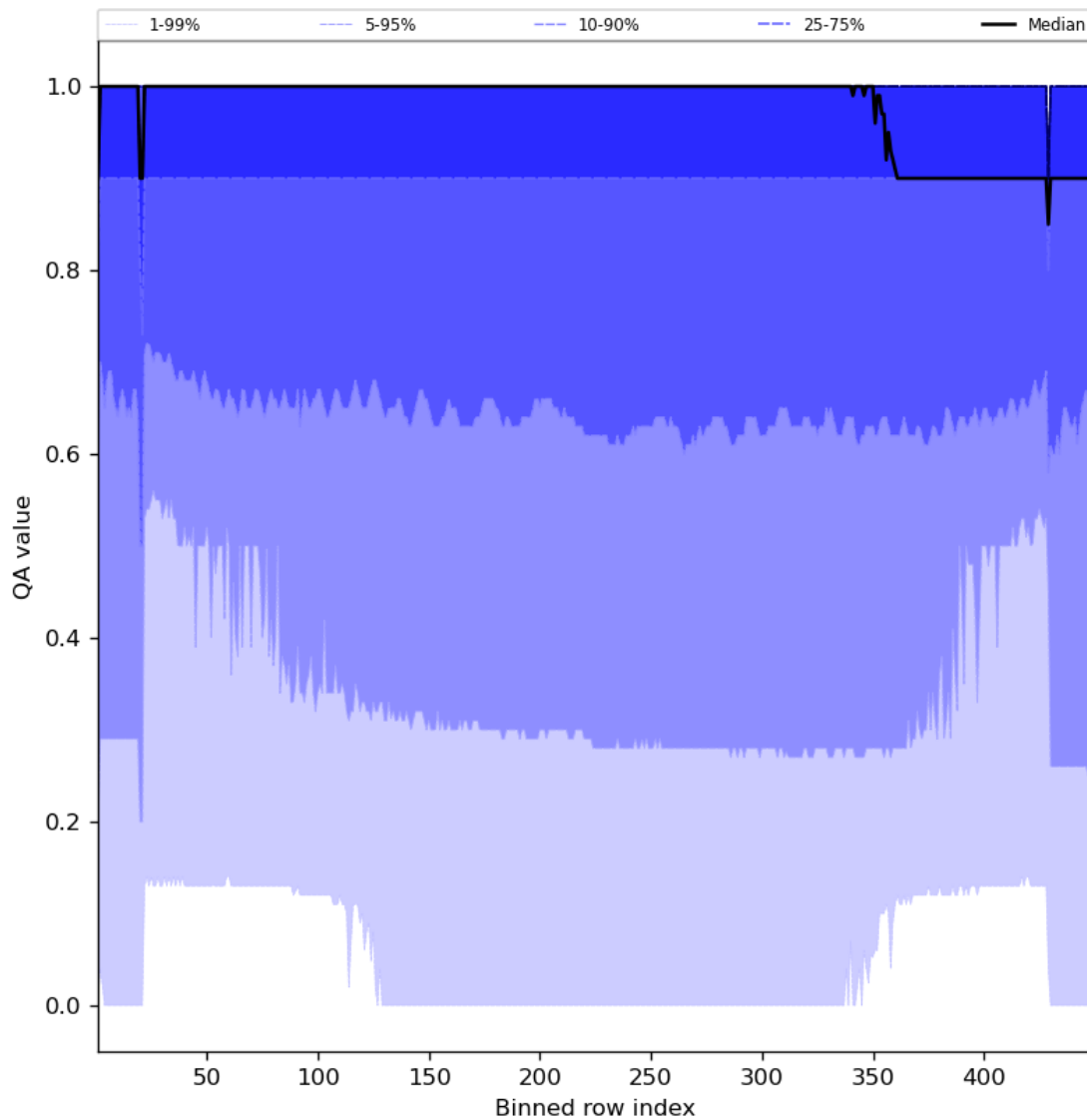
Figure 27: Along track statistics of “QA value” for 2023-07-21 to 2023-07-23
