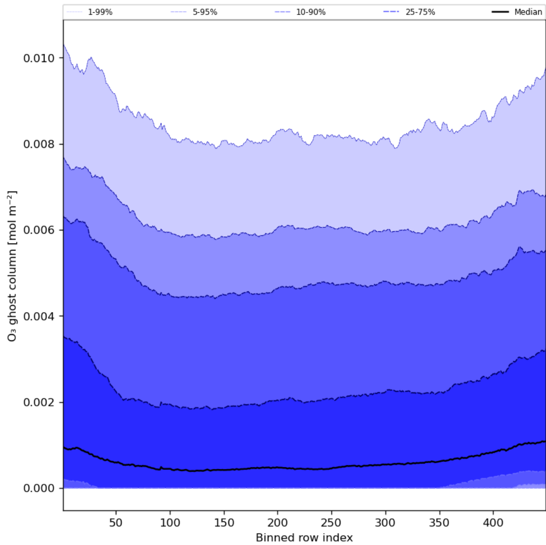
Figure 32: Along track statistics of “O 3 ghost column” for 2023-07-22 to 2023-07-24
