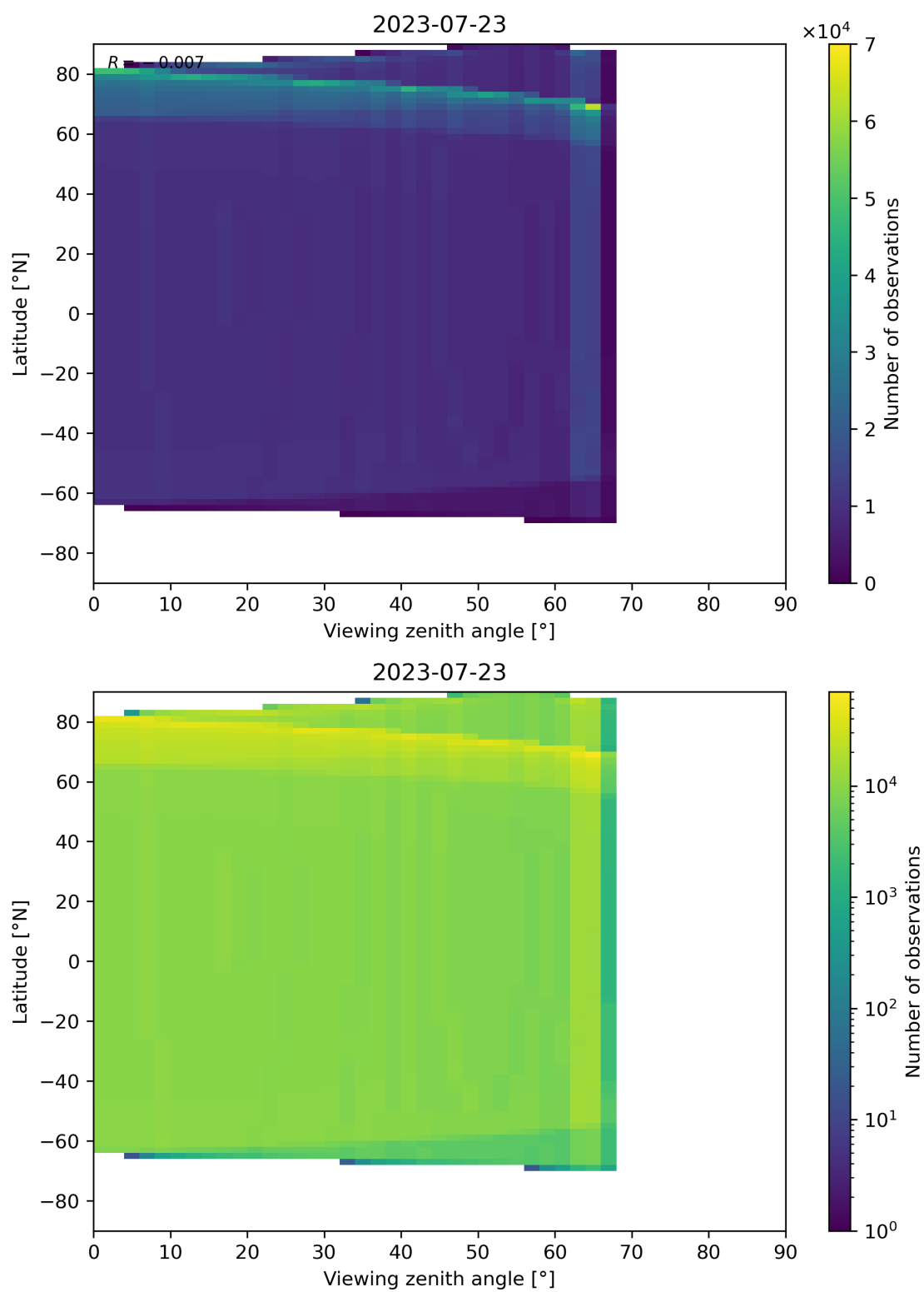
Figure 49: Scatter density plot of “Viewing zenith angle” against “Latitude” for 2023-07-22 to 2023-07-24.
