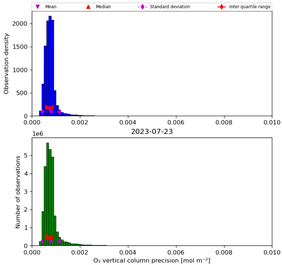
Figure 22: Histogram of “O 3 vertical column precision” for 2023-07-22 to 2023-07-24
