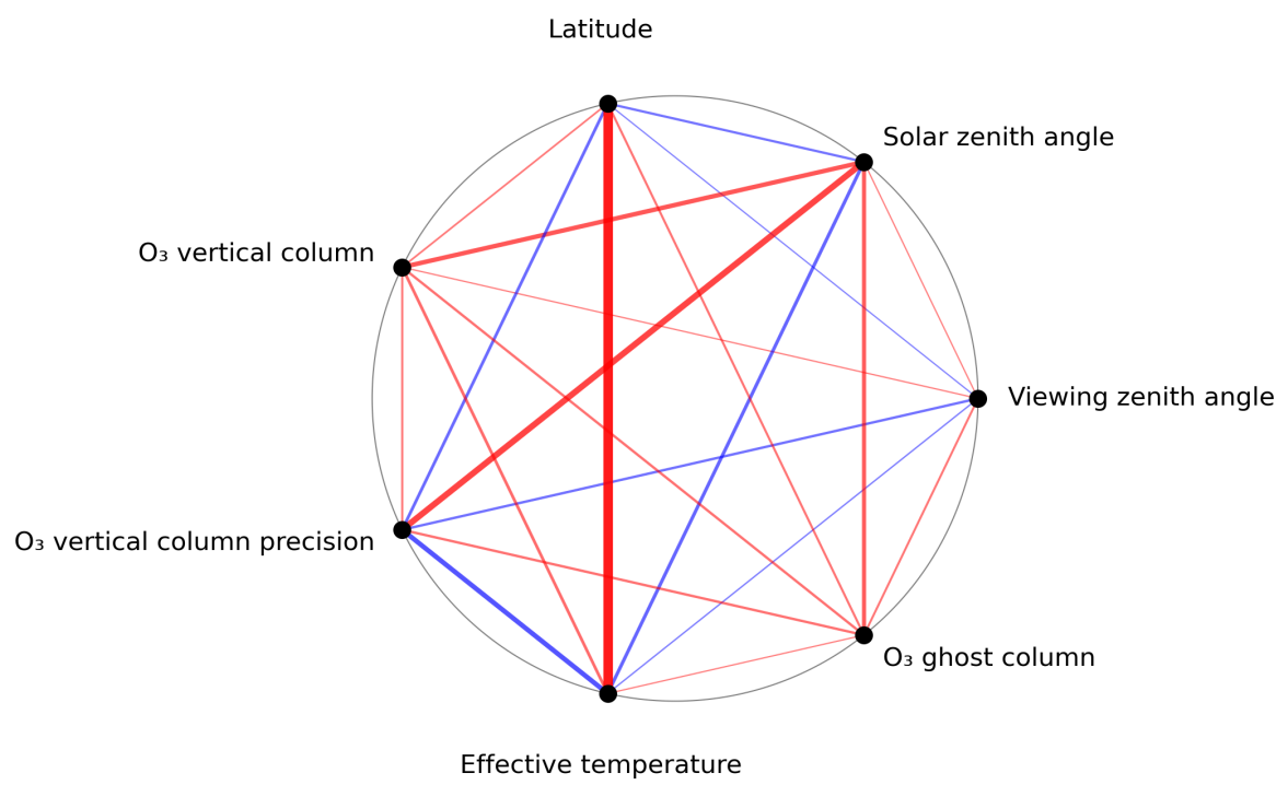
Figure 1: Map of correlation graph for 2023-07-22 to 2023-07-24.
