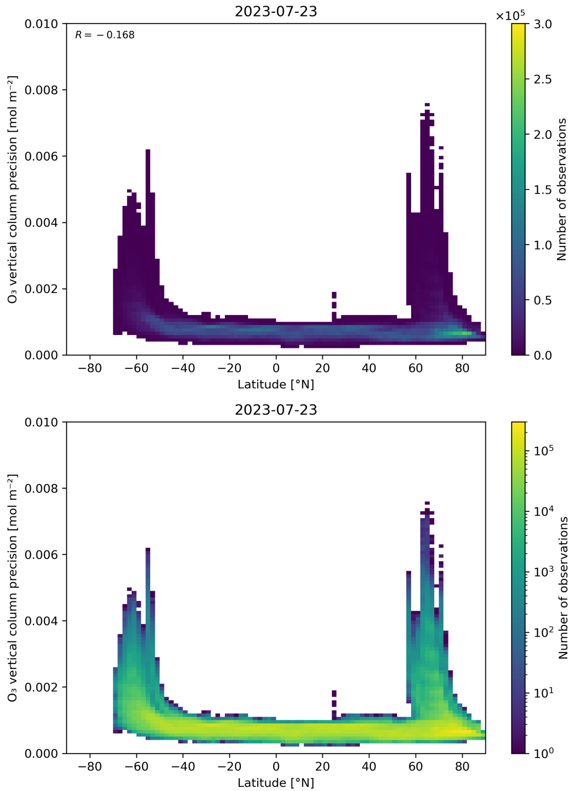
Figure 37: Scatter density plot of “Latitude” against “O 3 vertical column precision” for 2023-07-22 to 2023-07-24.
