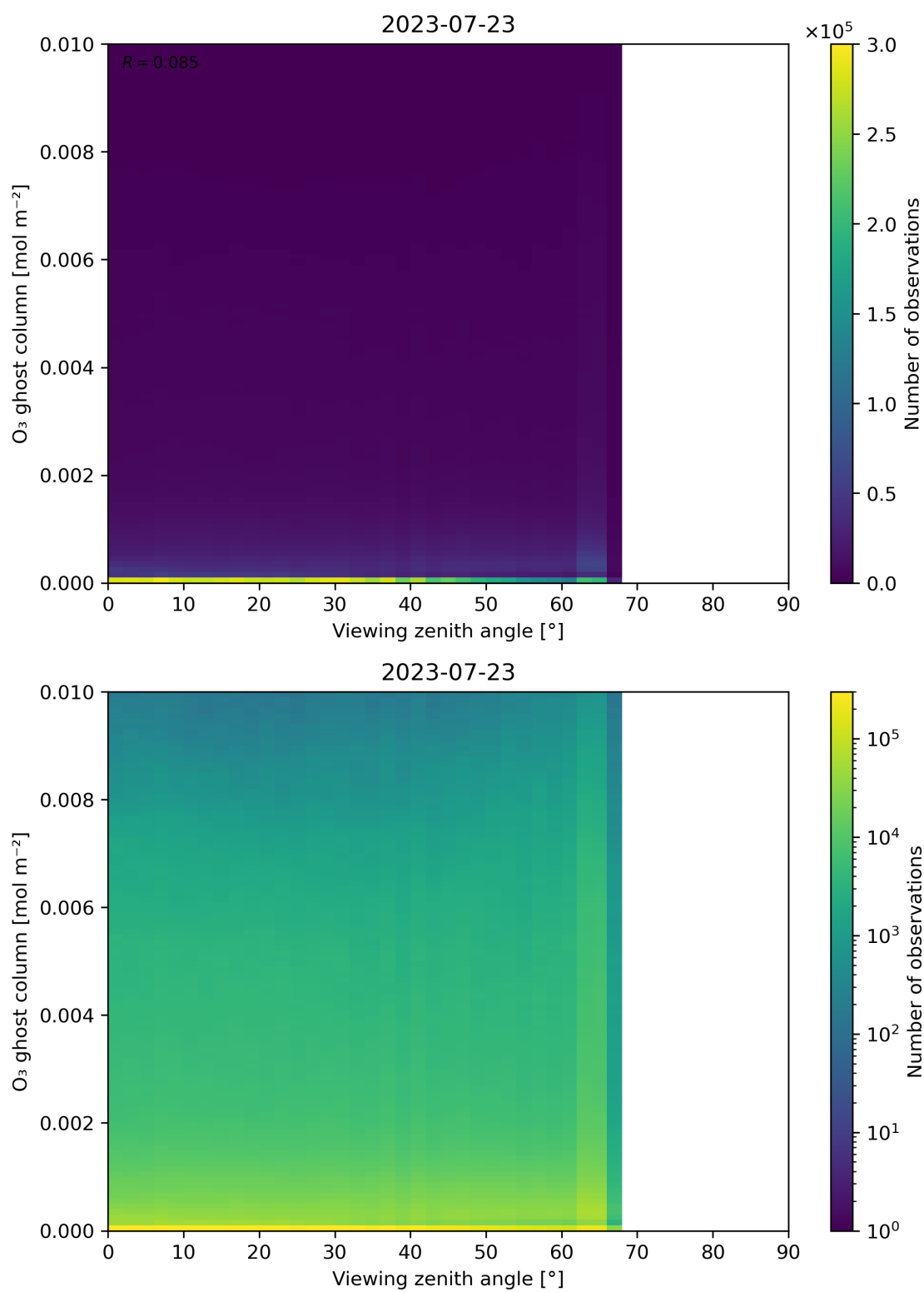
Figure 51: Scatter density plot of “Viewing zenith angle” against “O 3 ghost column” for 2023-07-22 to 2023-07-24.
