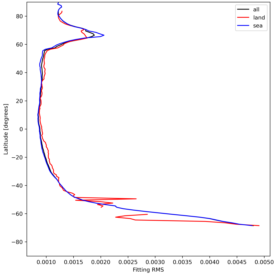
Figure 16: Zonal average of “Fitting RMS” for 2023-07-22 to 2023-07-24.
