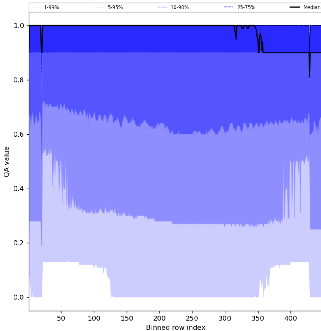
Figure 27: Along track statistics of “QA value” for 2023-07-22 to 2023-07-24
