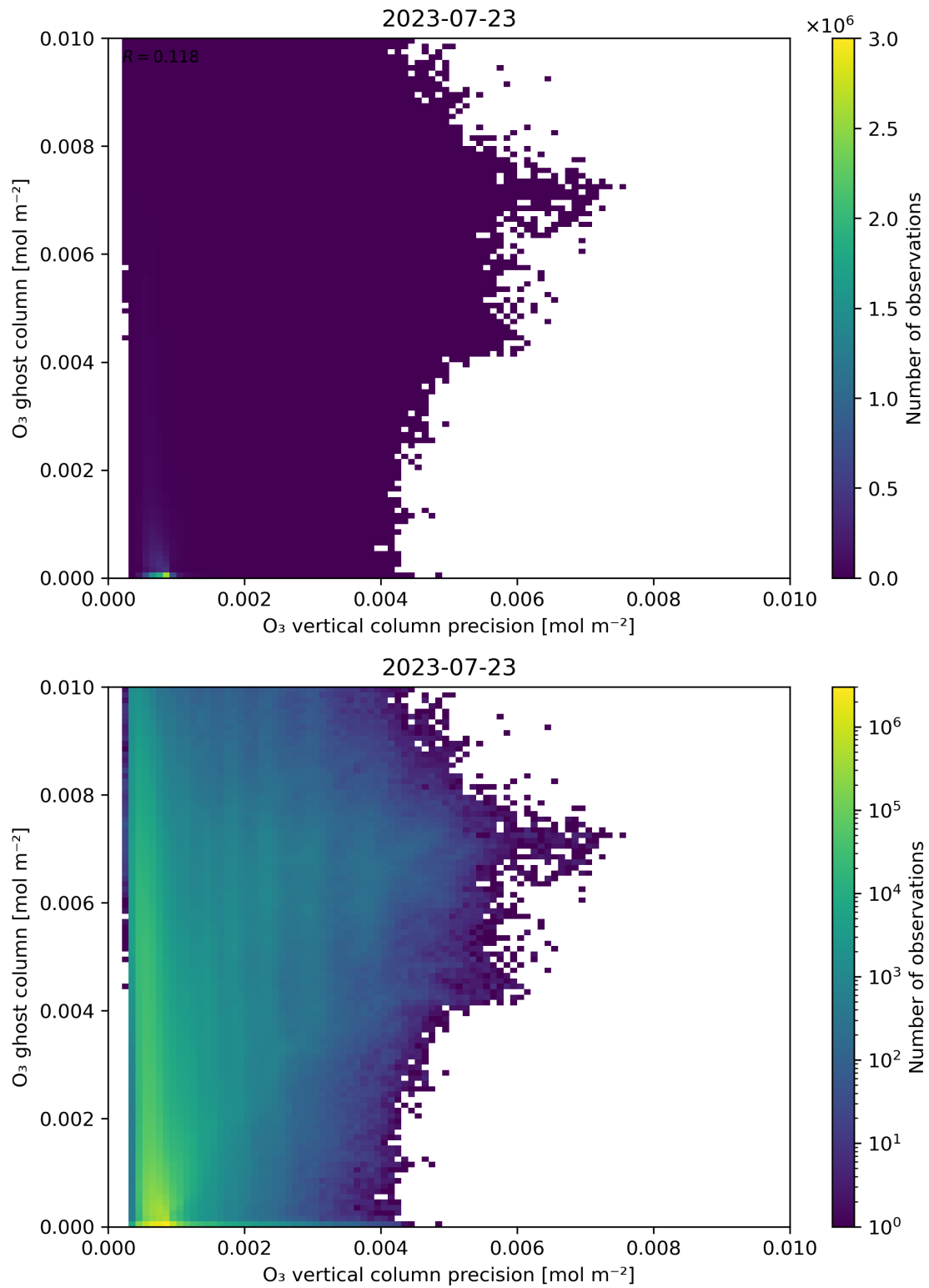
Figure 43: Scatter density plot of “ \text{O}_3 vertical column precision” against “ \text{O}_3 ghost column” for 2023-07-22 to 2023-07-24.
