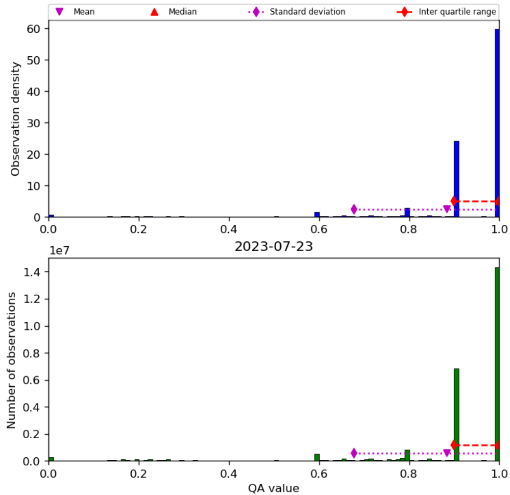
Figure 20: Histogram of “QA value” for 2023-07-22 to 2023-07-24
