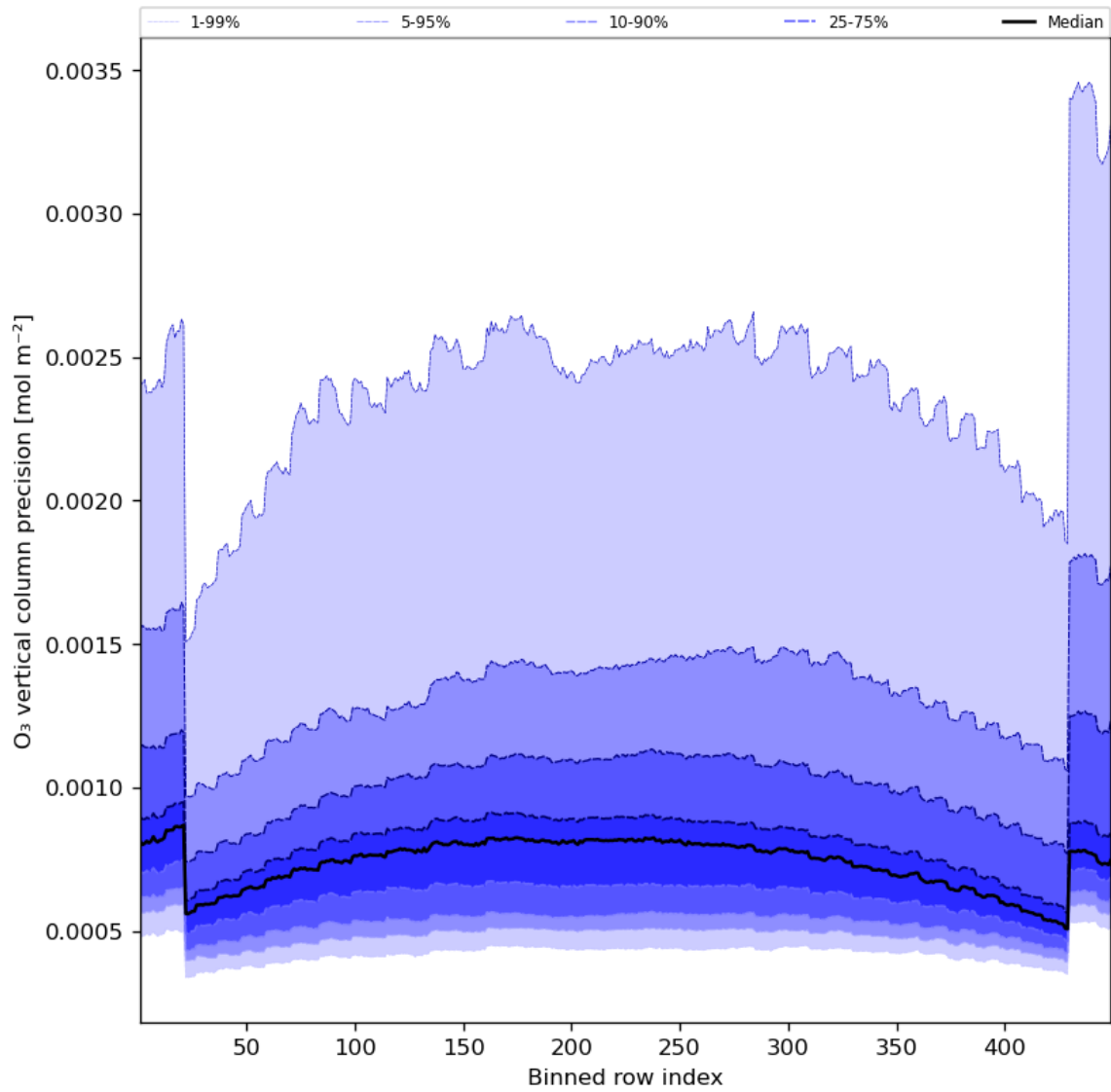
Figure 29: Along track statistics of “O 3 vertical column precision” for 2023-07-22 to 2023-07-24
