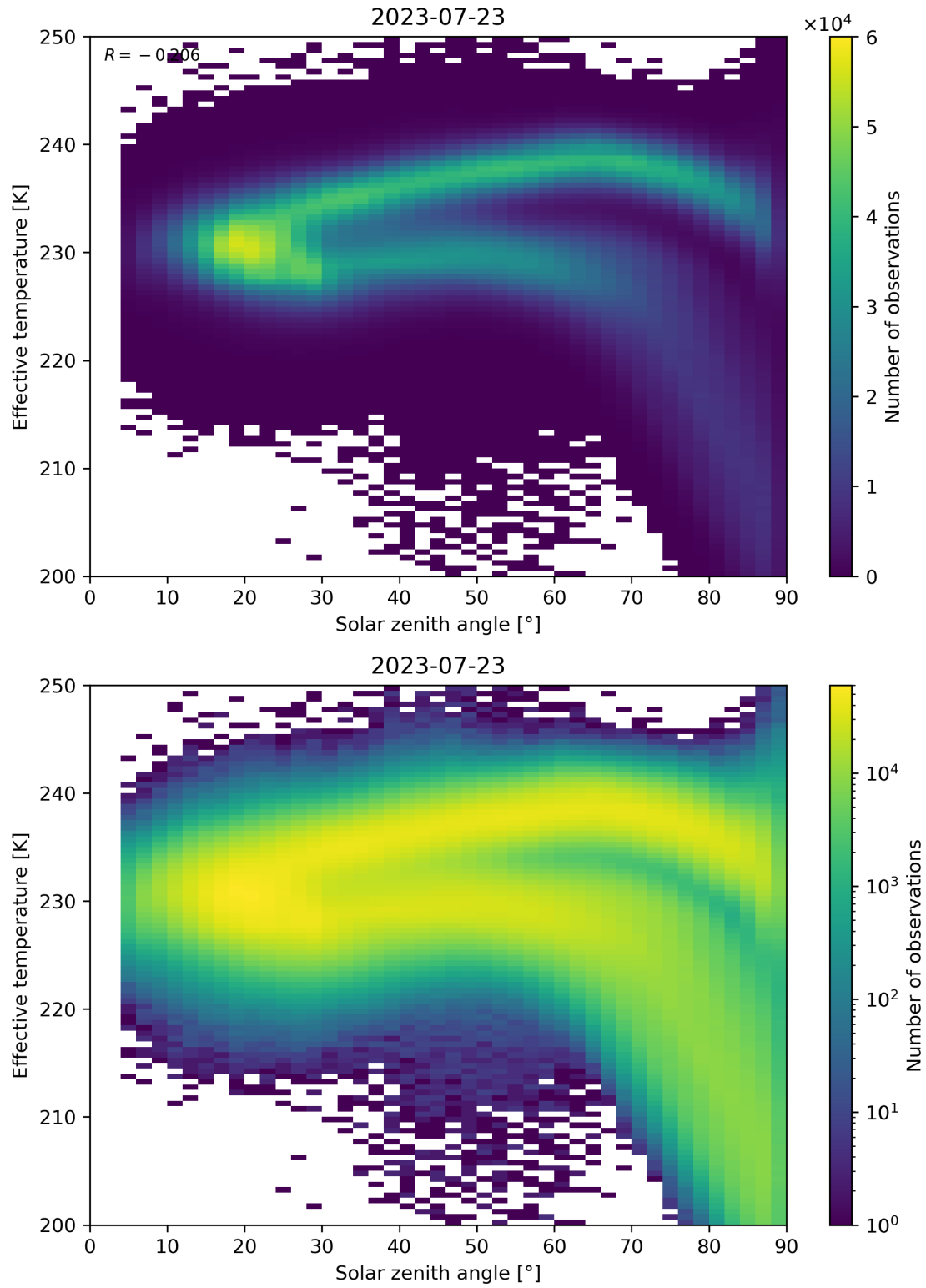
Figure 45: Scatter density plot of “Solar zenith angle” against “Effective temperature” for 2023-07-22 to 2023-07-24.
