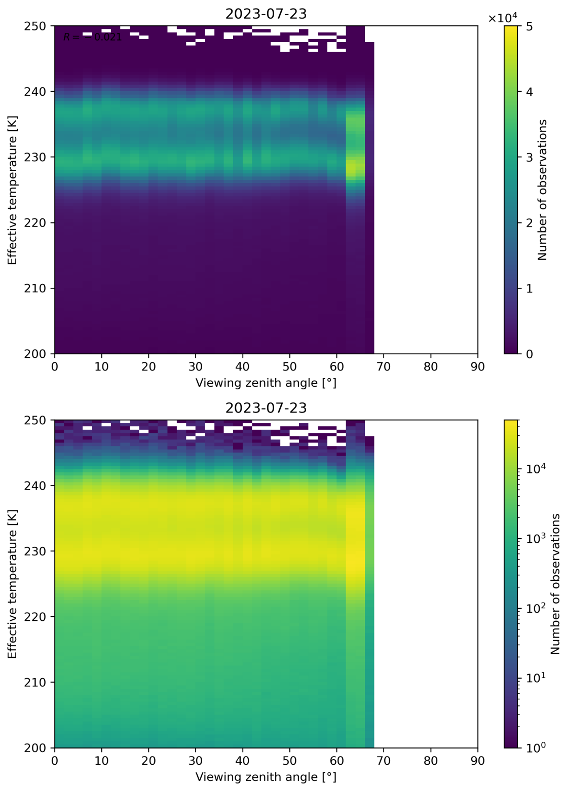
Figure 50: Scatter density plot of “Viewing zenith angle” against “Effective temperature” for 2023-07-22 to 2023-07-24.
