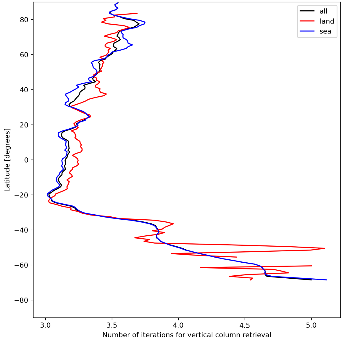
Figure 19: Zonal average of “Number of iterations for vertical column retrieval” for 2023-07-22 to 2023-07-24.
