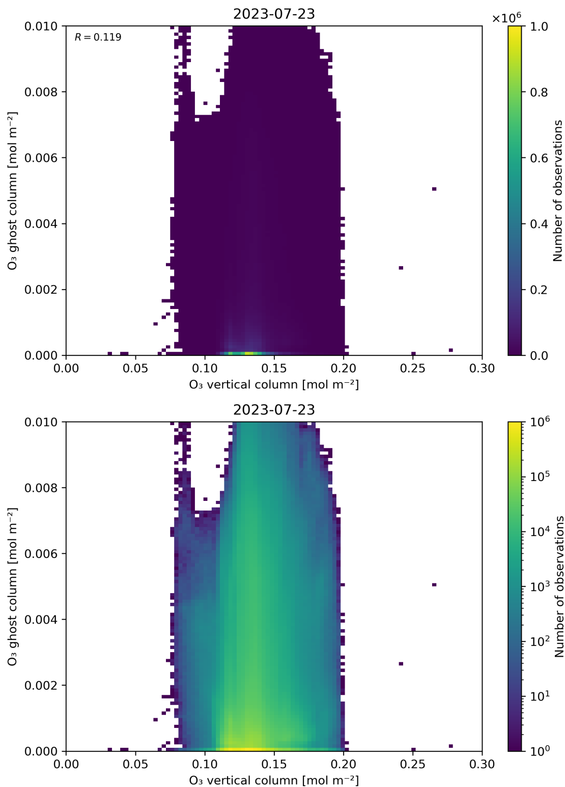
Figure 40: Scatter density plot of “O 3 vertical column” against “O 3 ghost column” for 2023-07-22 to 2023-07-24.
