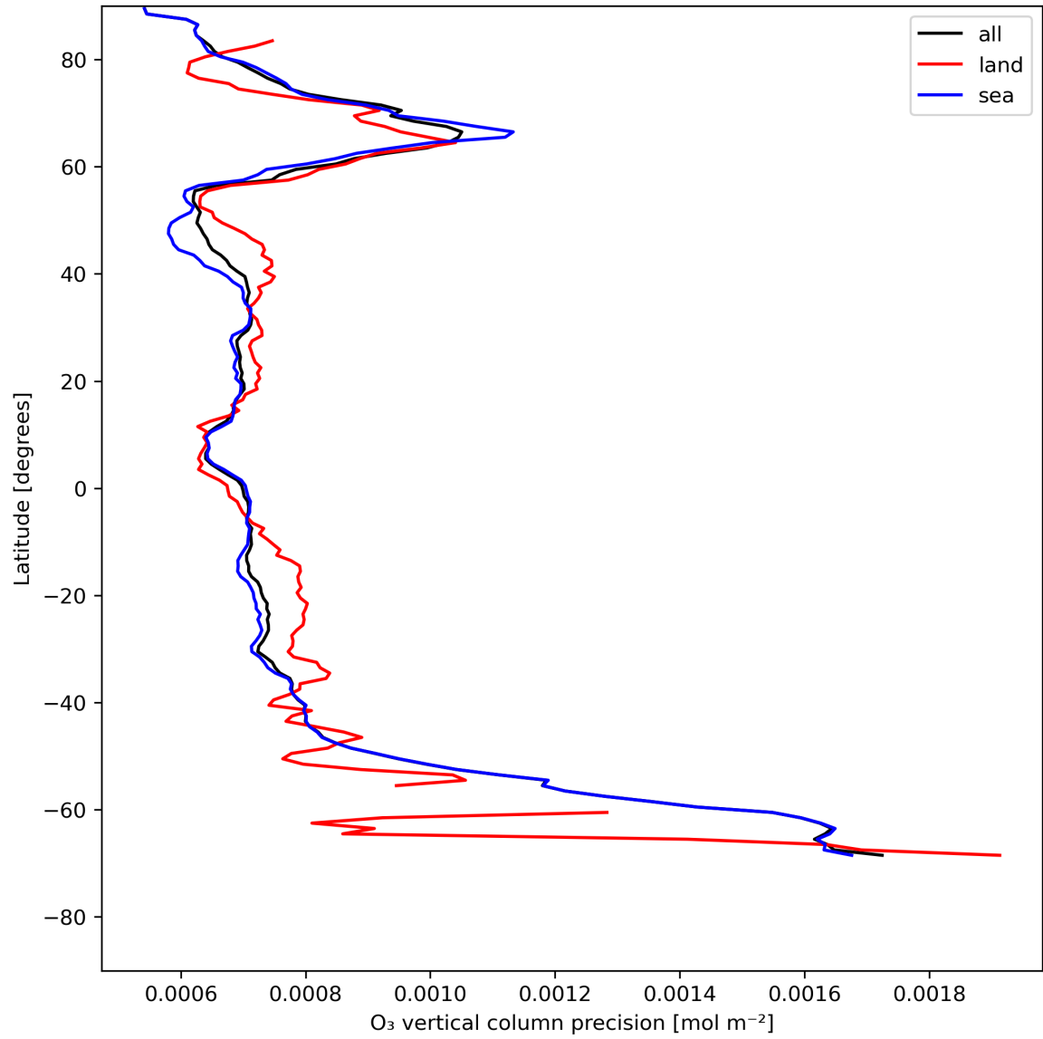
Figure 15: Zonal average of “O 3 vertical column precision” for 2023-07-22 to 2023-07-24.
