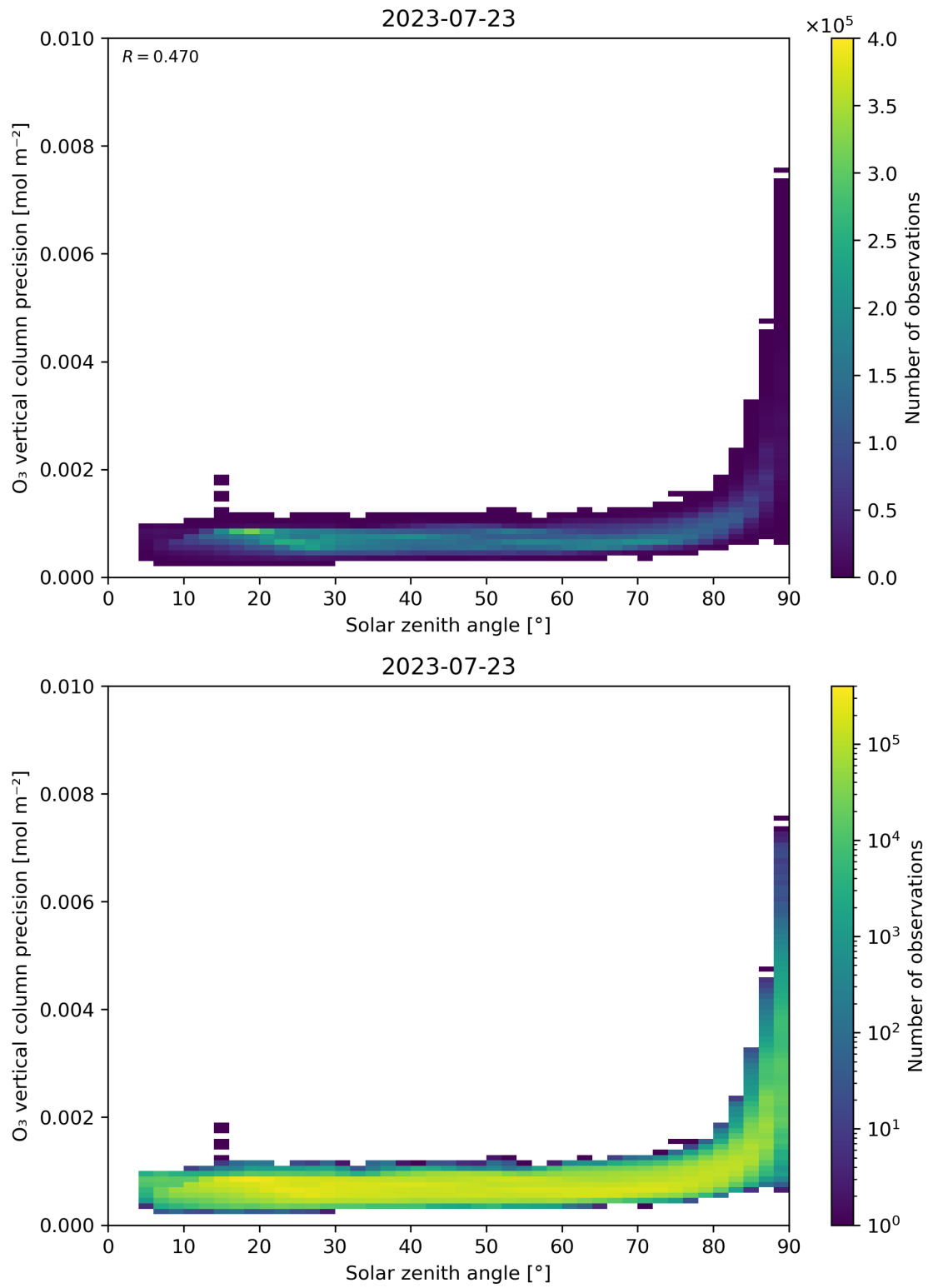
Figure 48: Scatter density plot of “Solar zenith angle” against “O 3 vertical column precision” for 2023-07-22 to 2023-07-24.
