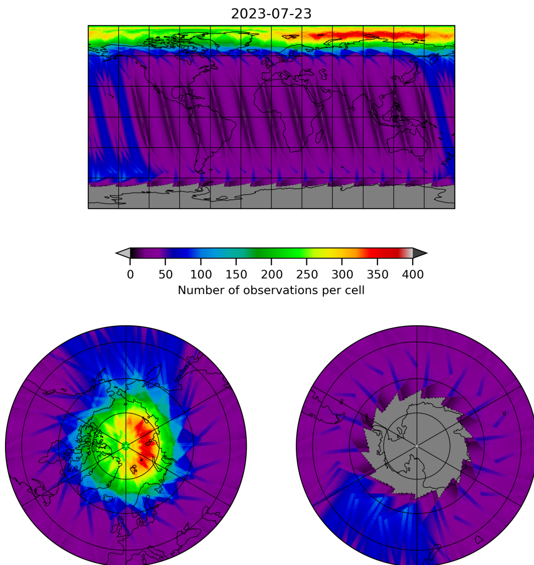
Figure 12: Map of the number of observations for 2023-07-22 to 2023-07-24
