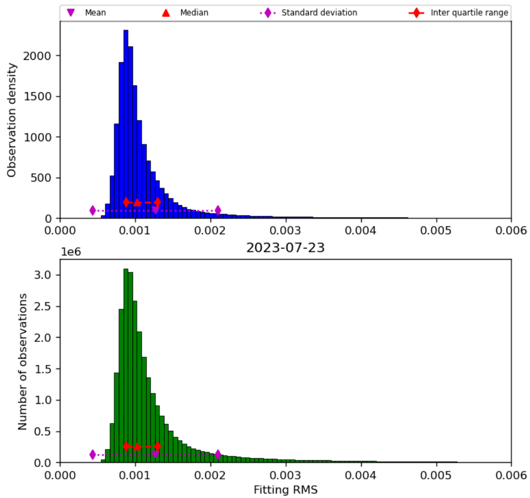
Figure 23: Histogram of “Fitting RMS” for 2023-07-22 to 2023-07-24
