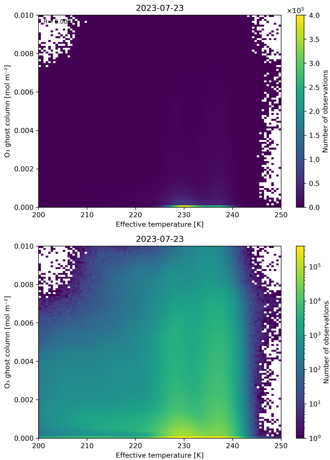
Figure 38: Scatter density plot of “Effective temperature” against “O 3 ghost column” for 2023-07-22 to 2023-07-24.
