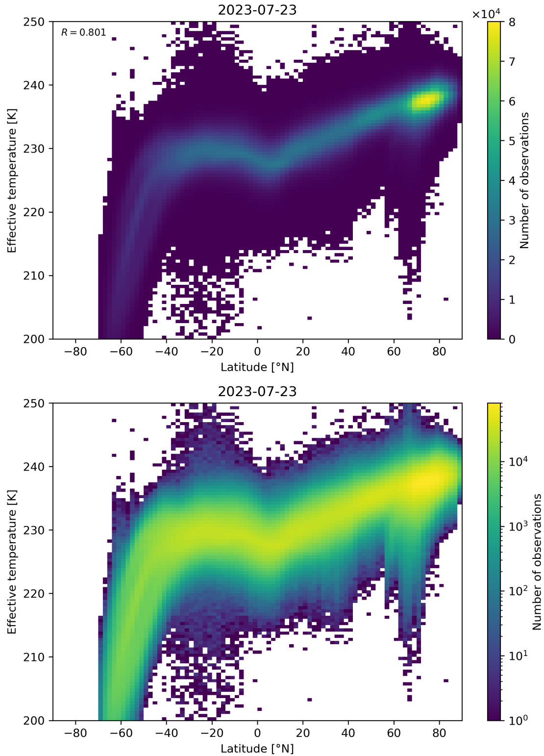
Figure 34: Scatter density plot of “Latitude” against “Effective temperature” for 2023-07-22 to 2023-07-24.
