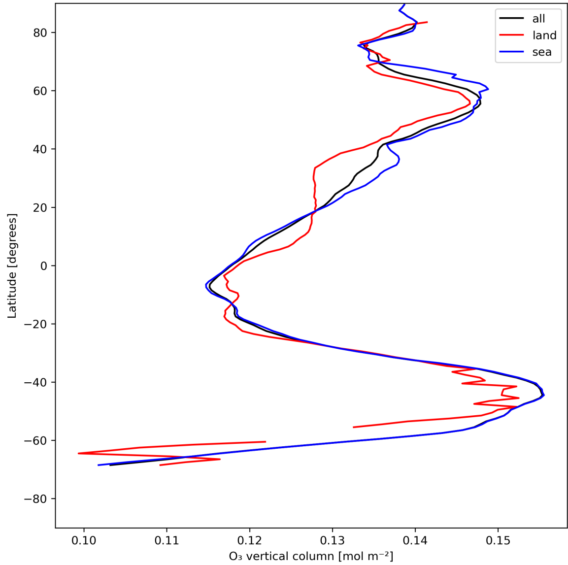
Figure 14: Zonal average of “O 3 vertical column” for 2023-07-22 to 2023-07-24.
