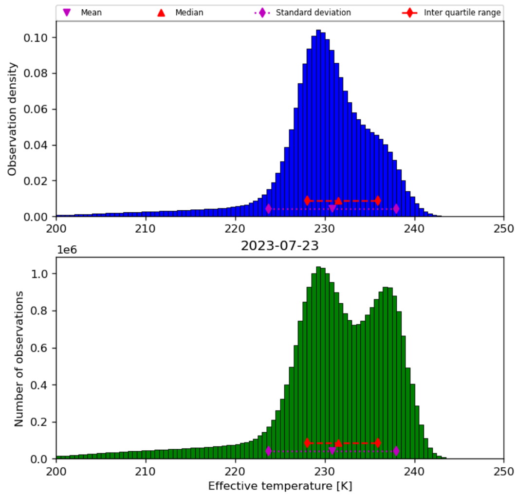
Figure 24: Histogram of “Effective temperature” for 2023-07-22 to 2023-07-24
