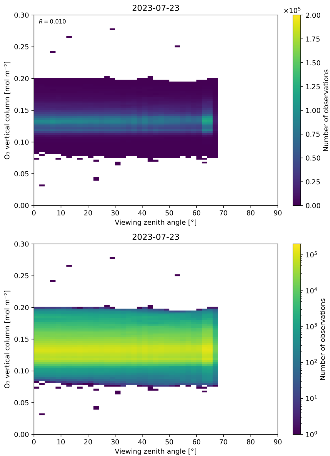
Figure 52: Scatter density plot of “Viewing zenith angle” against “O 3 vertical column” for 2023-07-22 to 2023-07-24.
