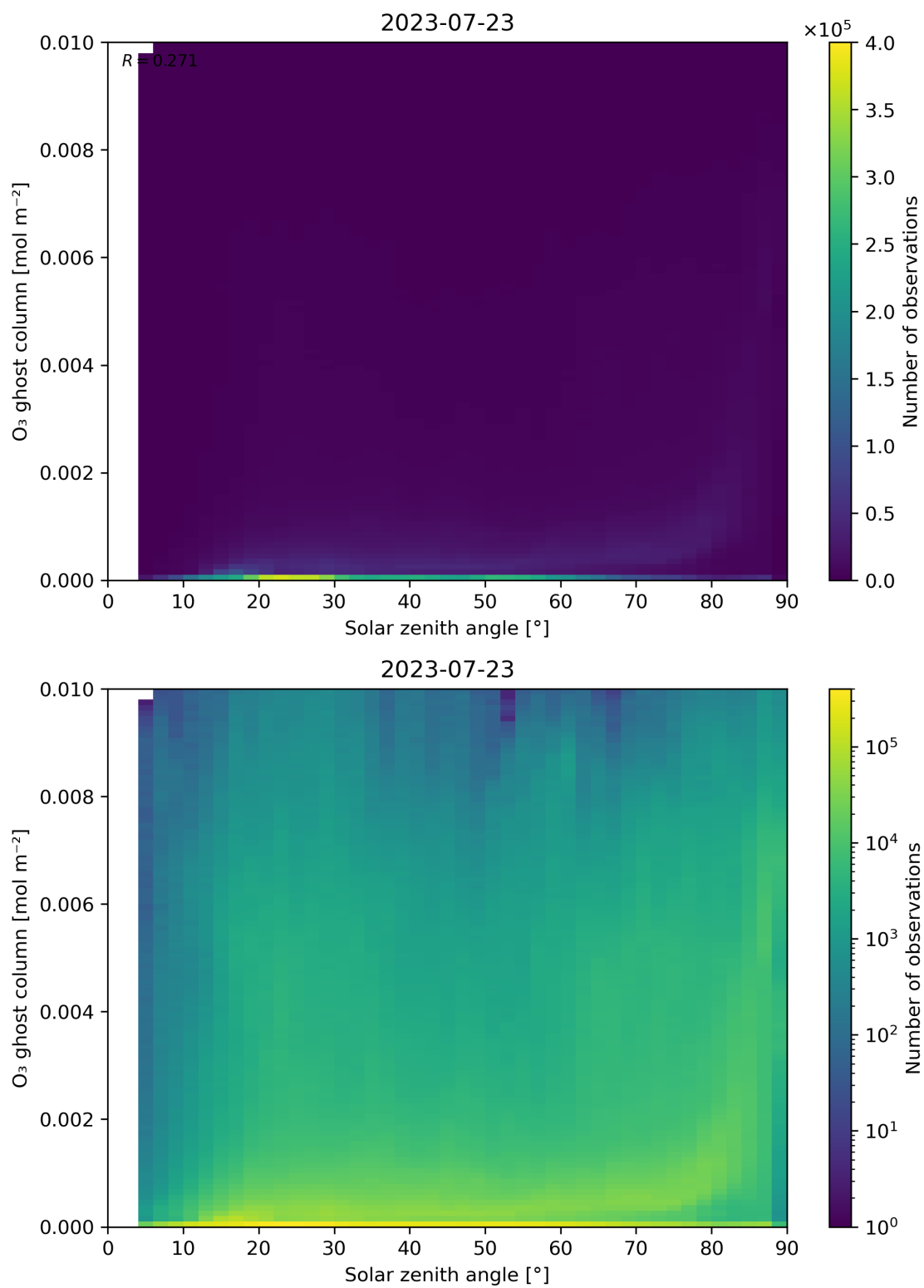
Figure 46: Scatter density plot of “Solar zenith angle” against “O 3 ghost column” for 2023-07-22 to 2023-07-24.
