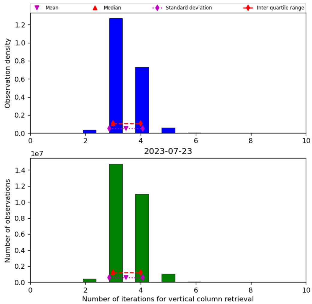
Figure 26: Histogram of “Number of iterations for vertical column retrieval” for 2023-07-22 to 2023-07-24
