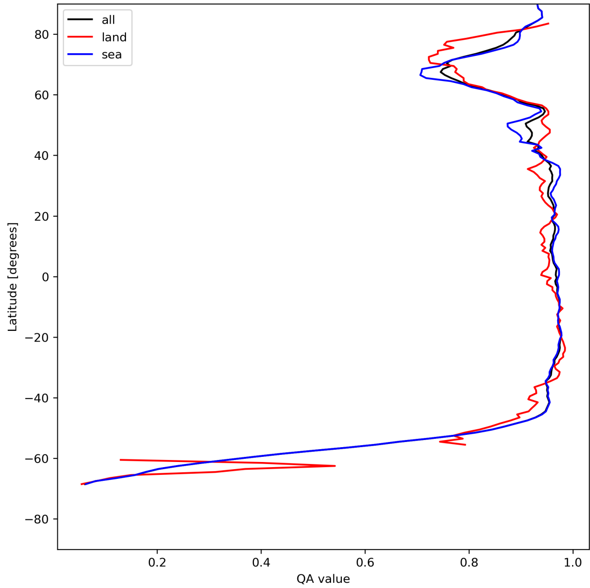
Figure 13: Zonal average of “QA value” for 2023-07-22 to 2023-07-24.
