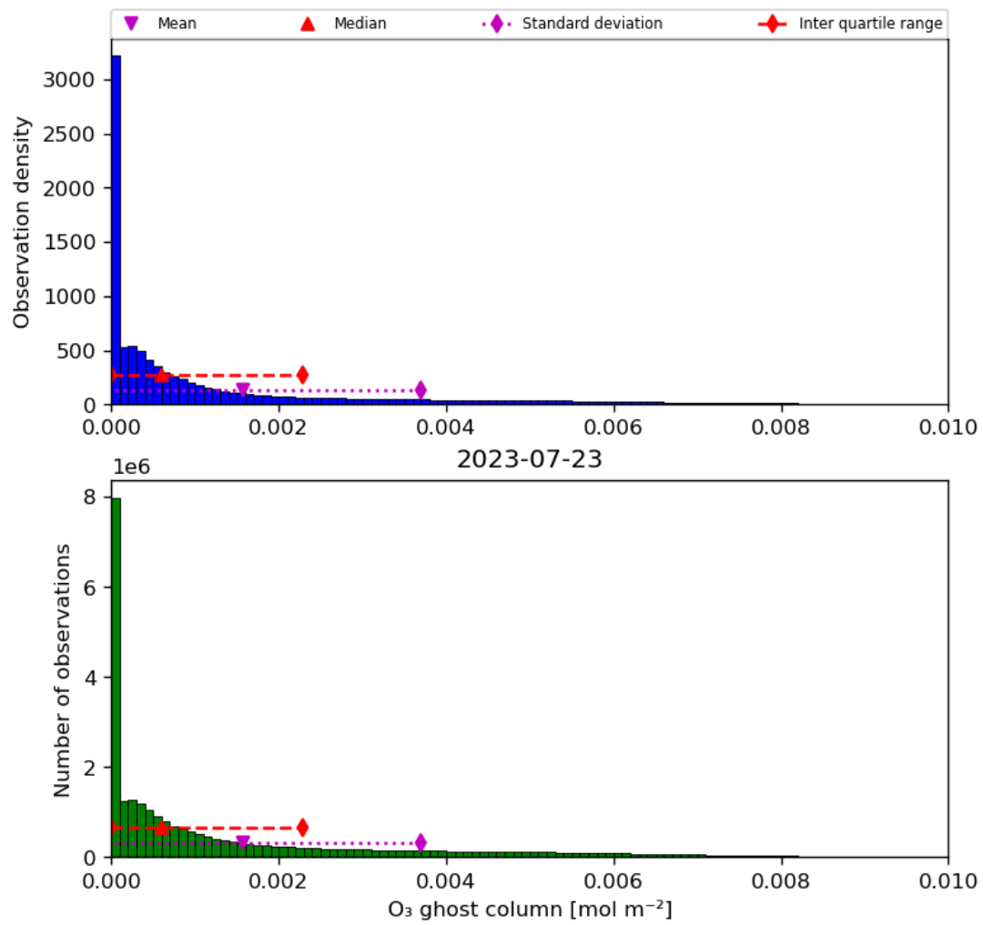
Figure 25: Histogram of “O 3 ghost column” for 2023-07-22 to 2023-07-24
