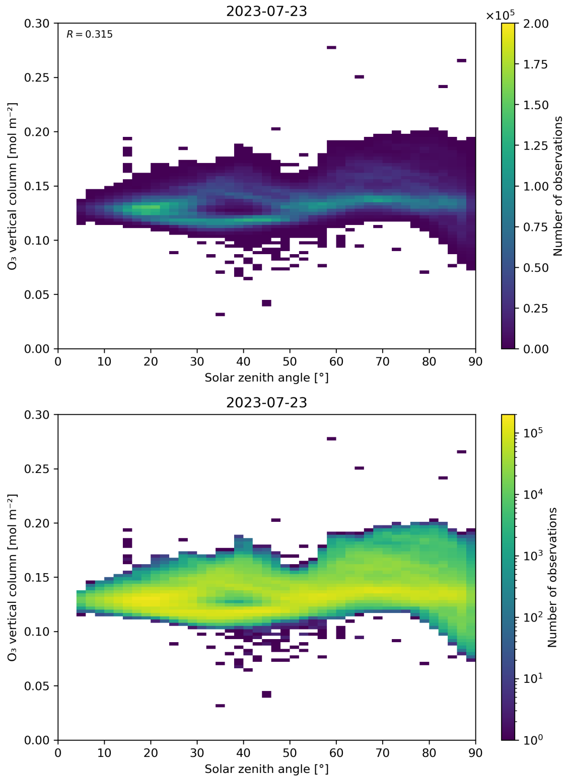
Figure 47: Scatter density plot of “Solar zenith angle” against “O 3 vertical column” for 2023-07-22 to 2023-07-24.
