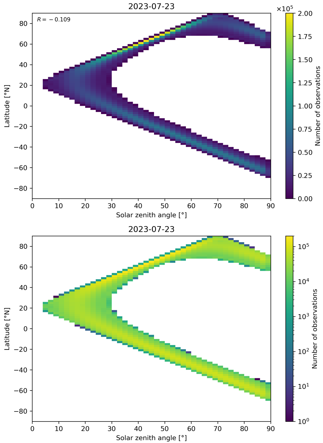
Figure 44: Scatter density plot of “Solar zenith angle” against “Latitude” for 2023-07-22 to 2023-07-24.
