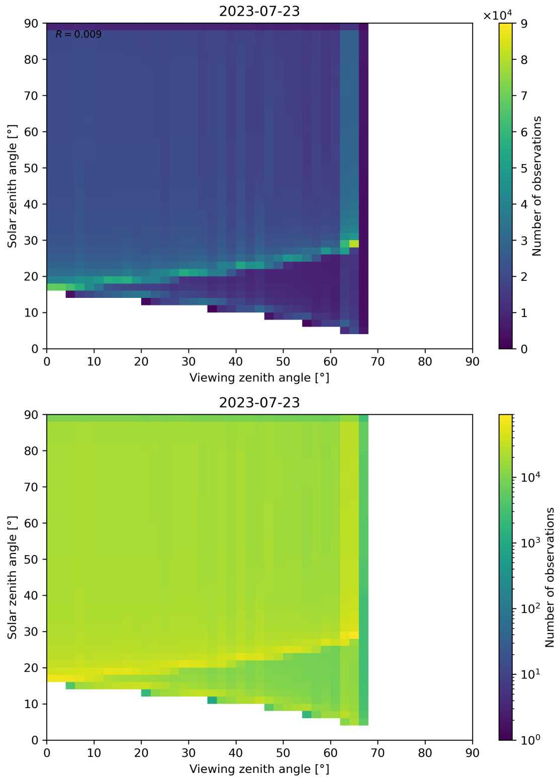
Figure 54: Scatter density plot of “Viewing zenith angle” against “Solar zenith angle” for 2023-07-22 to 2023-07-24.
