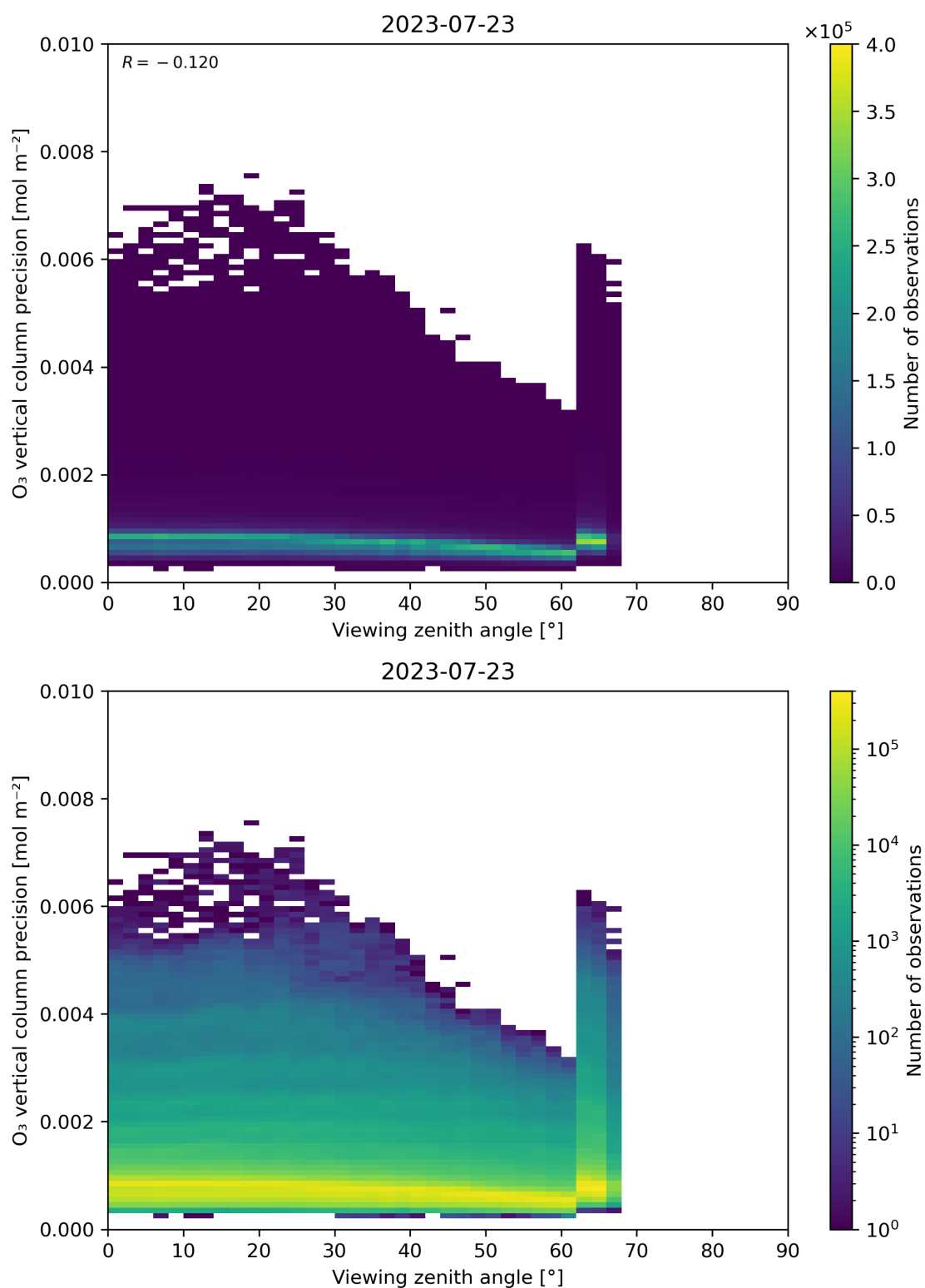
Figure 53: Scatter density plot of “Viewing zenith angle” against “O 3 vertical column precision” for 2023-07-22 to 2023-07-24.
