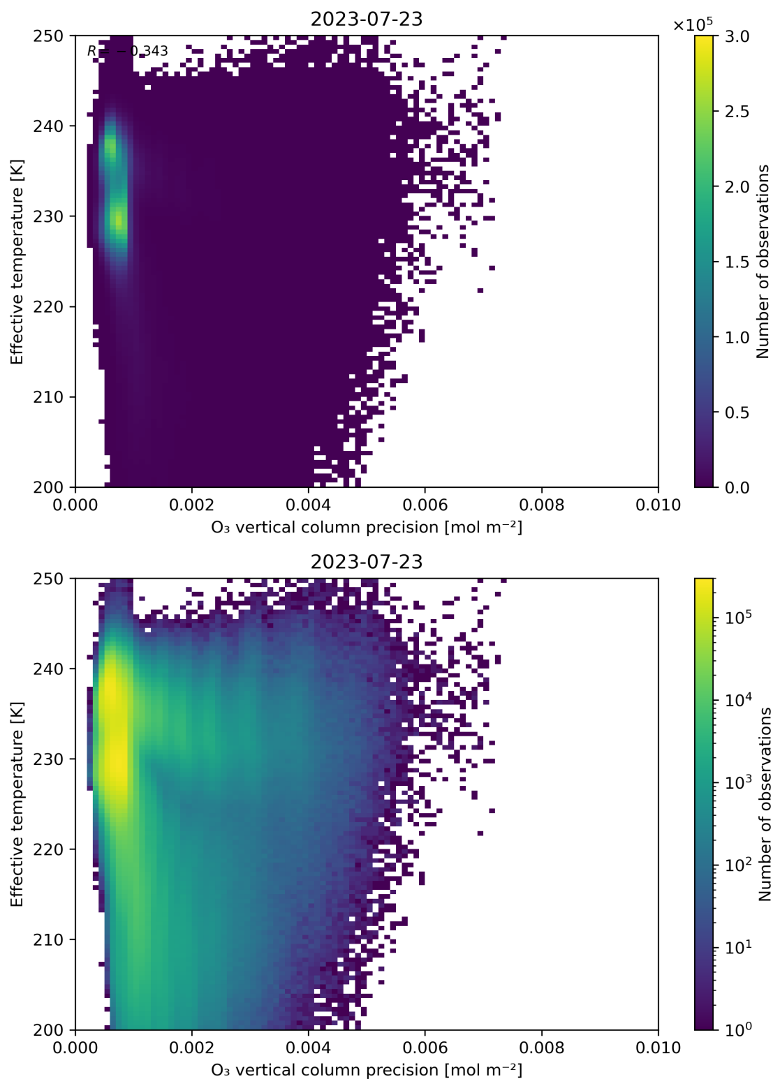
Figure 42: Scatter density plot of “O 3 vertical column precision” against “Effective temperature” for 2023-07-22 to 2023-07-24.
