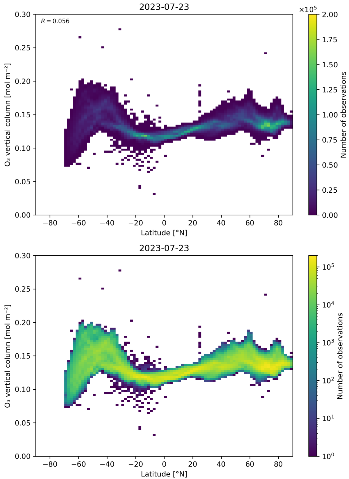
Figure 36: Scatter density plot of “Latitude” against “O 3 vertical column” for 2023-07-22 to 2023-07-24.
