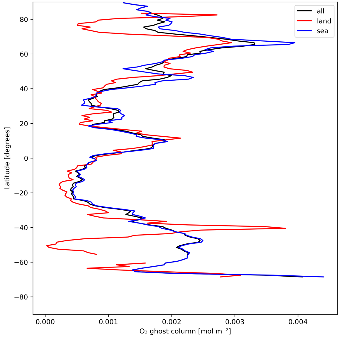
Figure 18: Zonal average of “O 3 ghost column” for 2023-07-22 to 2023-07-24.
