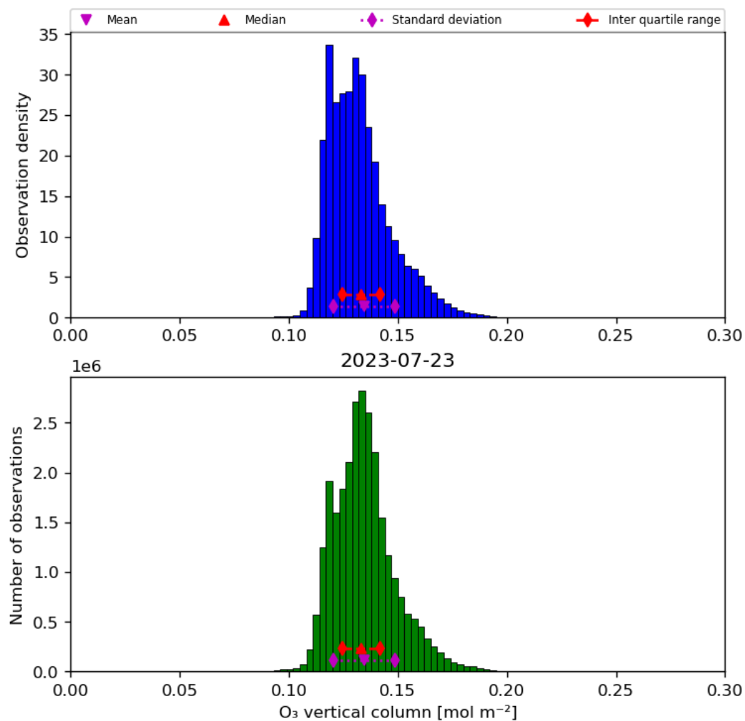
Figure 21: Histogram of “O 3 vertical column” for 2023-07-22 to 2023-07-24
