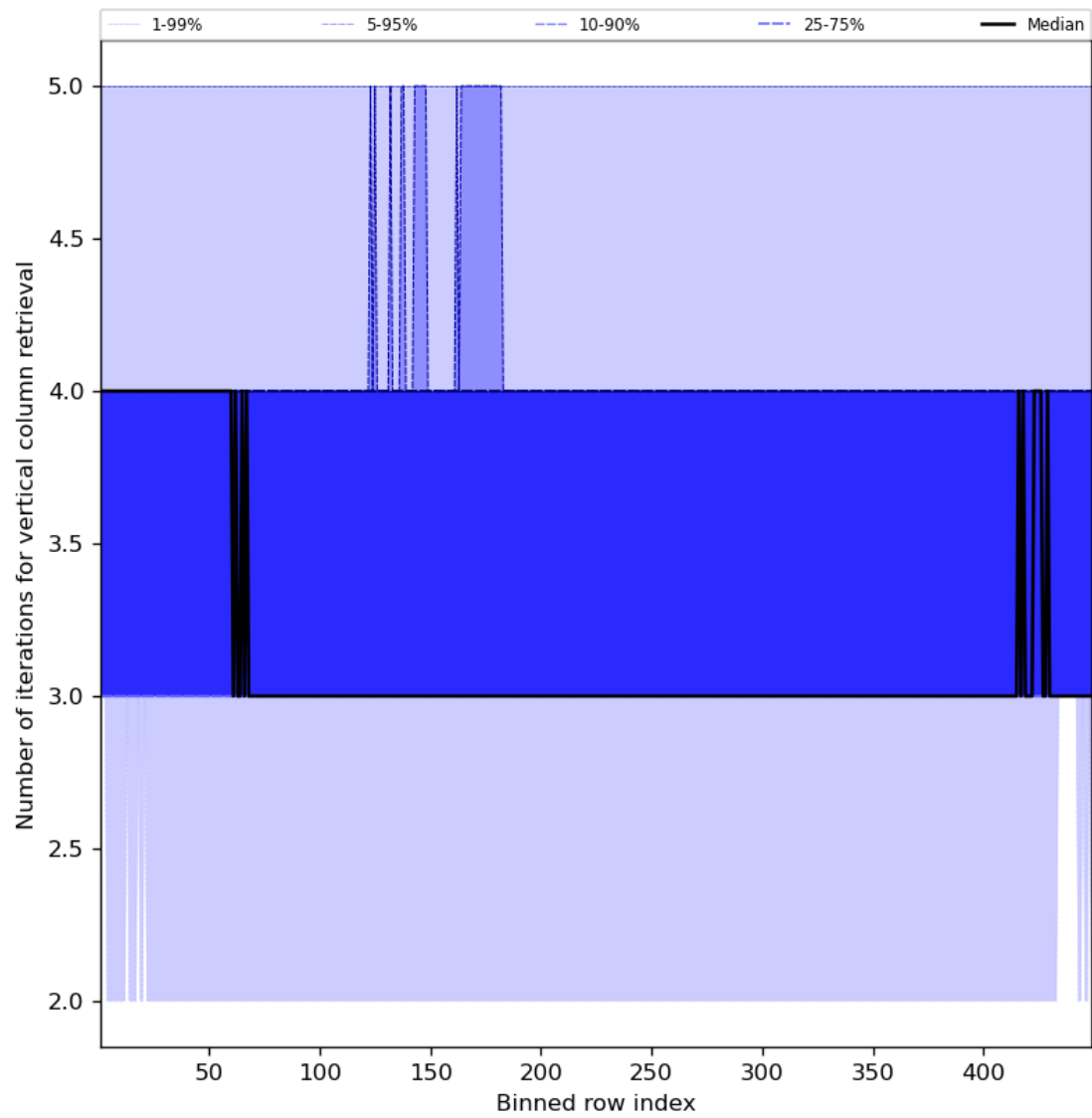
Figure 33: Along track statistics of “Number of iterations for vertical column retrieval” for 2023-07-22 to 2023-07-24
