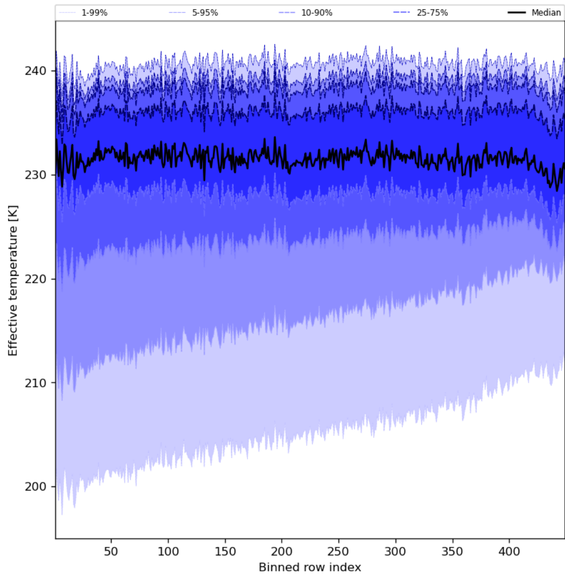
Figure 31: Along track statistics of “Effective temperature” for 2023-07-22 to 2023-07-24
