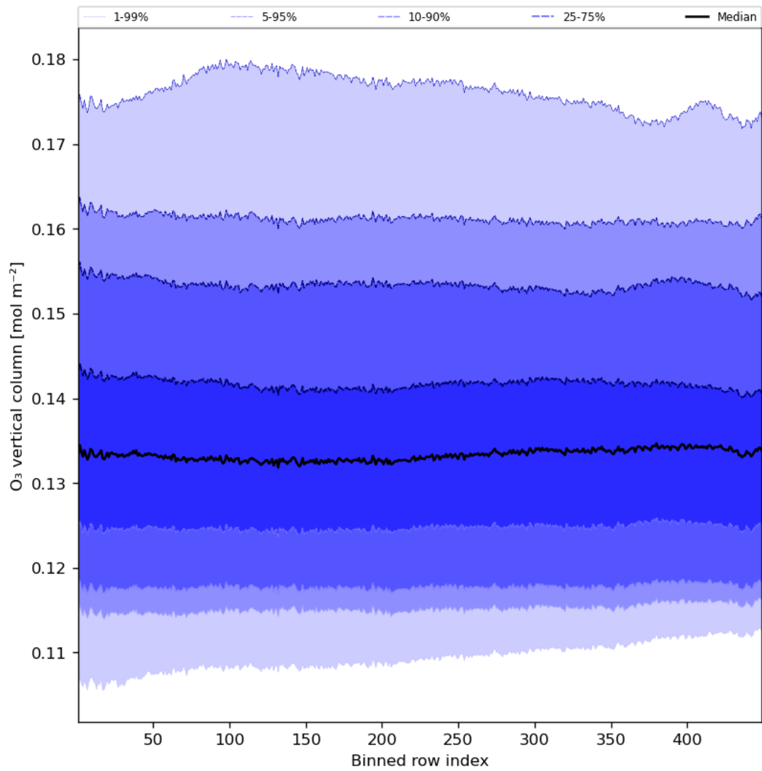
Figure 28: Along track statistics of “O 3 vertical column” for 2023-07-22 to 2023-07-24
