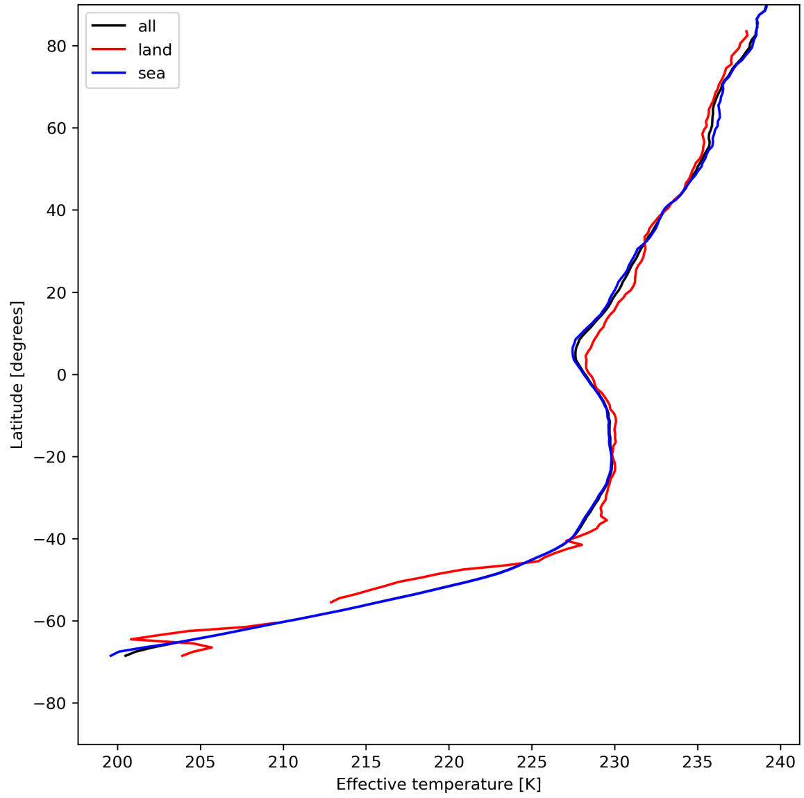
Figure 17: Zonal average of "Effective temperature" for 2023-07-22 to 2023-07-24.
