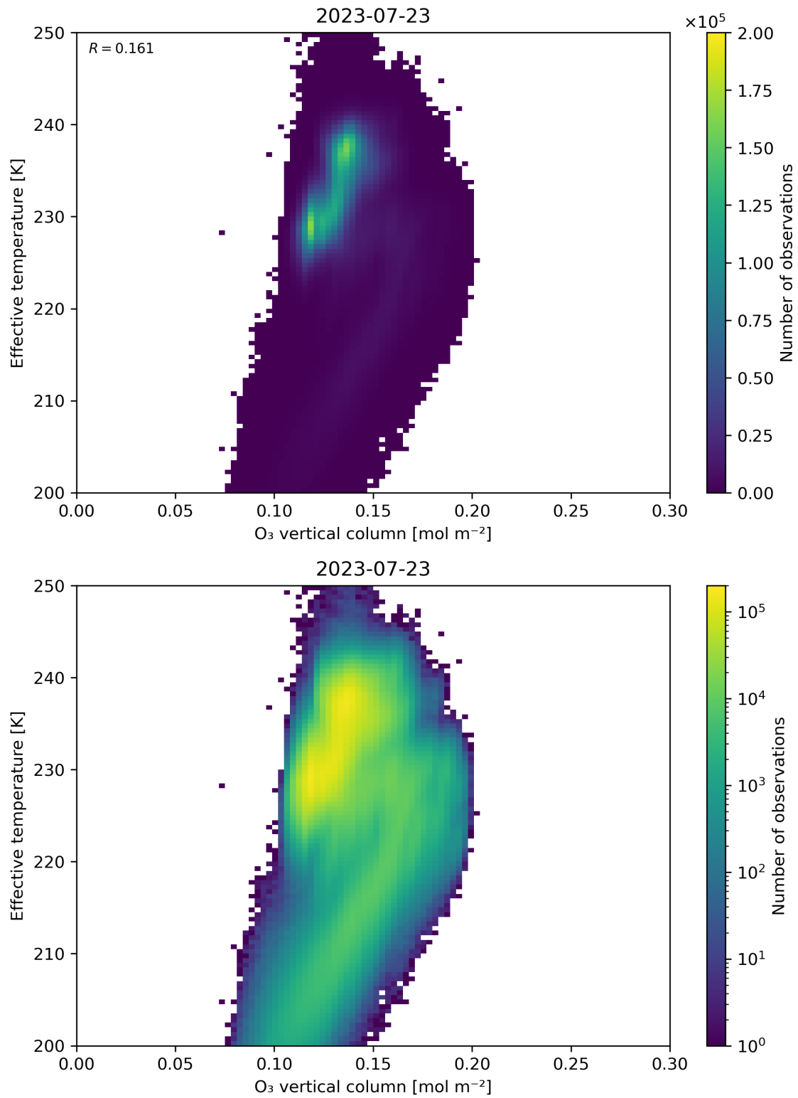
Figure 39: Scatter density plot of “O 3 vertical column” against “Effective temperature” for 2023-07-22 to 2023-07-24.
