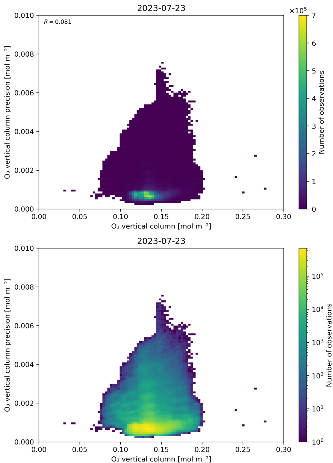
Figure 41: Scatter density plot of “O 3 vertical column” against “O 3 vertical column precision” for 2023-07-22 to 2023-07-24.
