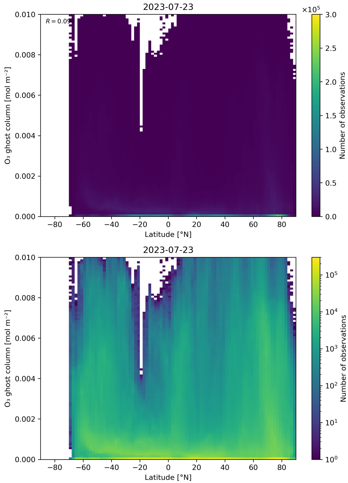
Figure 35: Scatter density plot of “Latitude” against “O 3 ghost column” for 2023-07-22 to 2023-07-24.
