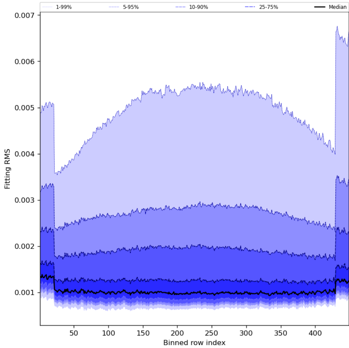
Figure 30: Along track statistics of “Fitting RMS” for 2023-07-22 to 2023-07-24
