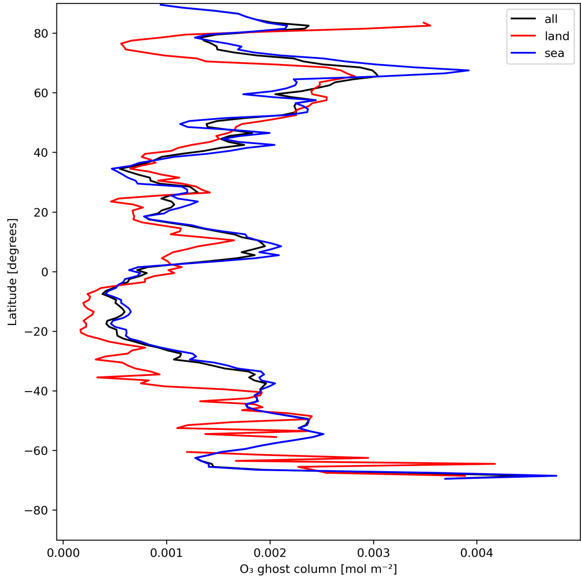
Figure 18: Zonal average of "O 3 ghost column" for 2023-07-24 to 2023-07-25.
