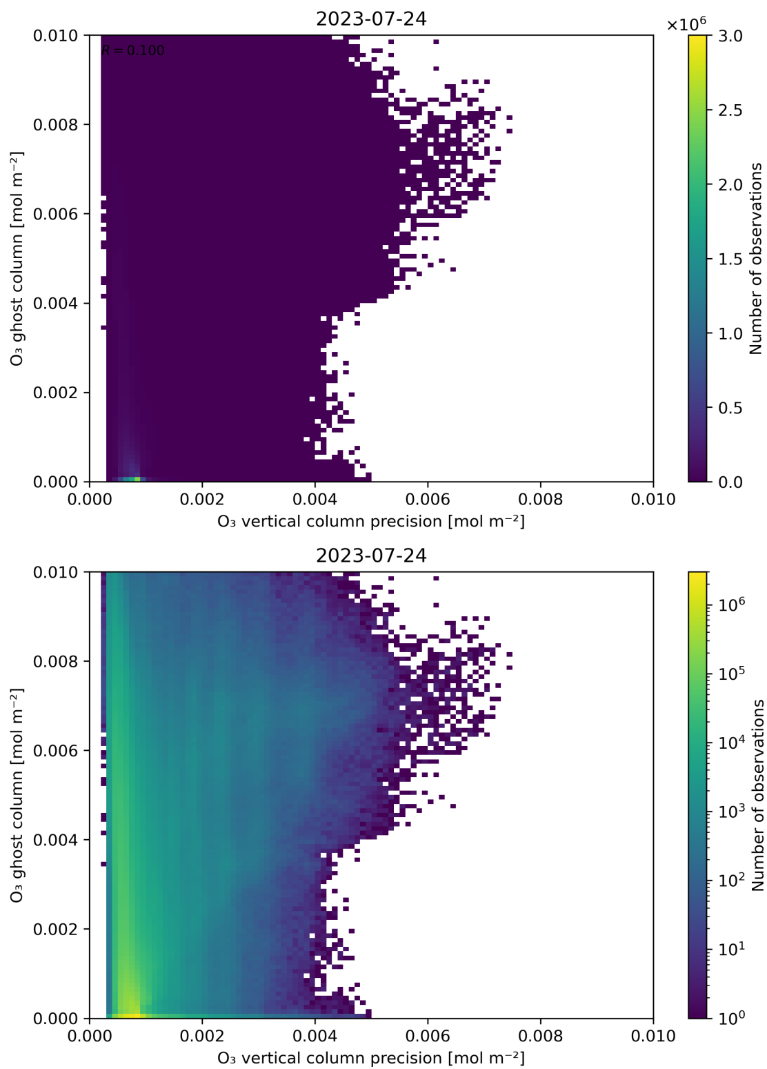
Figure 43: Scatter density plot of “ O_3 vertical column precision” against “ O_3 ghost column” for 2023-07-24 to 2023-07-25.
