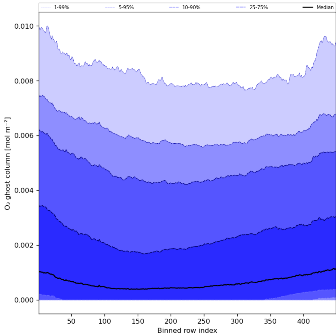
Figure 32: Along track statistics of “O 3 ghost column” for 2023-07-24 to 2023-07-25
