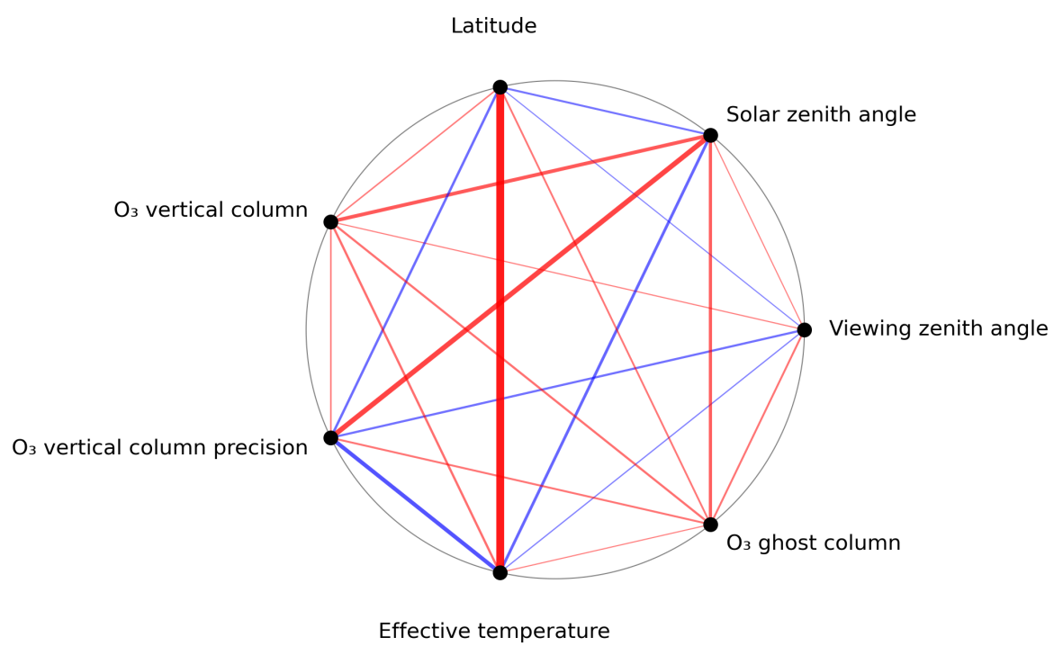
Figure 1: Map of correlation graph for 2023-07-24 to 2023-07-25.
