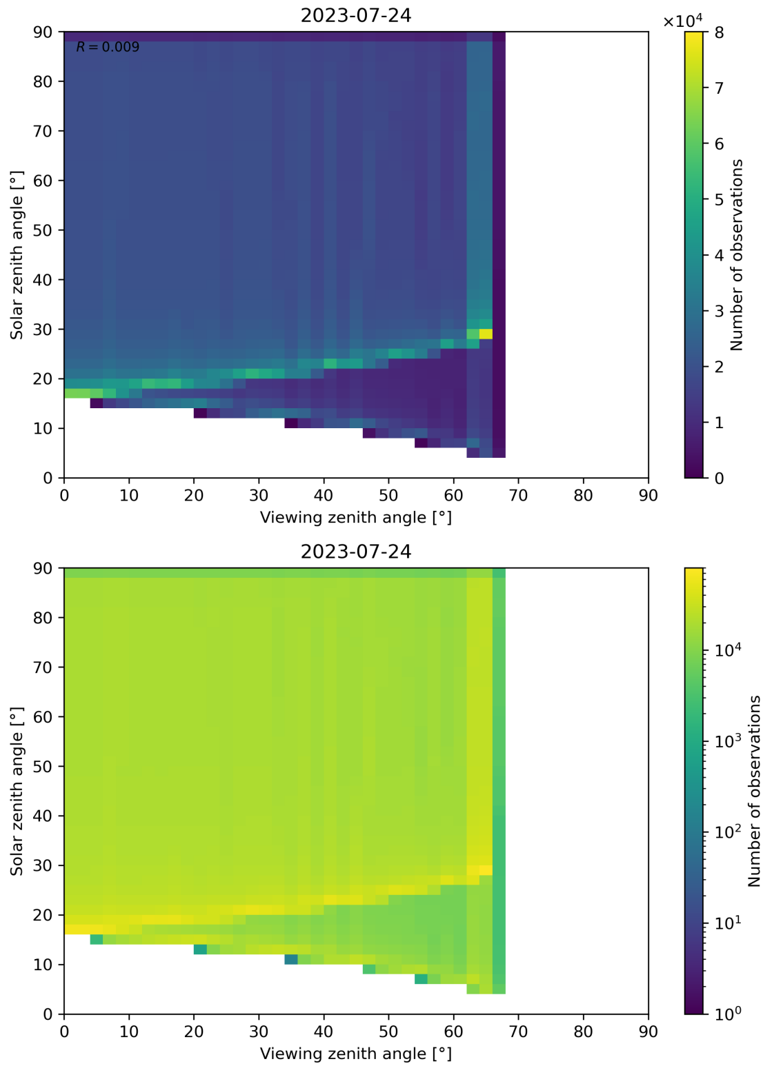
Figure 54: Scatter density plot of “Viewing zenith angle” against “Solar zenith angle” for 2023-07-24 to 2023-07-25.
