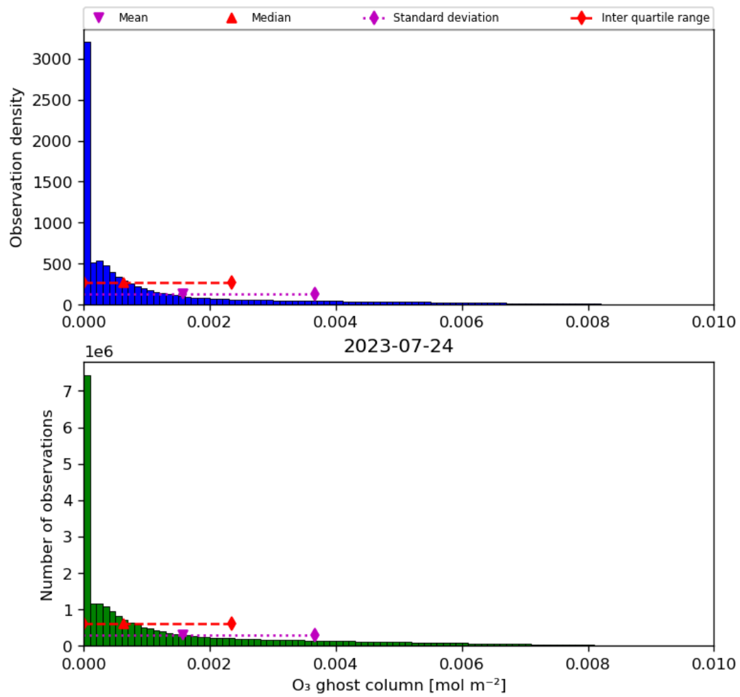
Figure 25: Histogram of “O 3 ghost column” for 2023-07-24 to 2023-07-25
