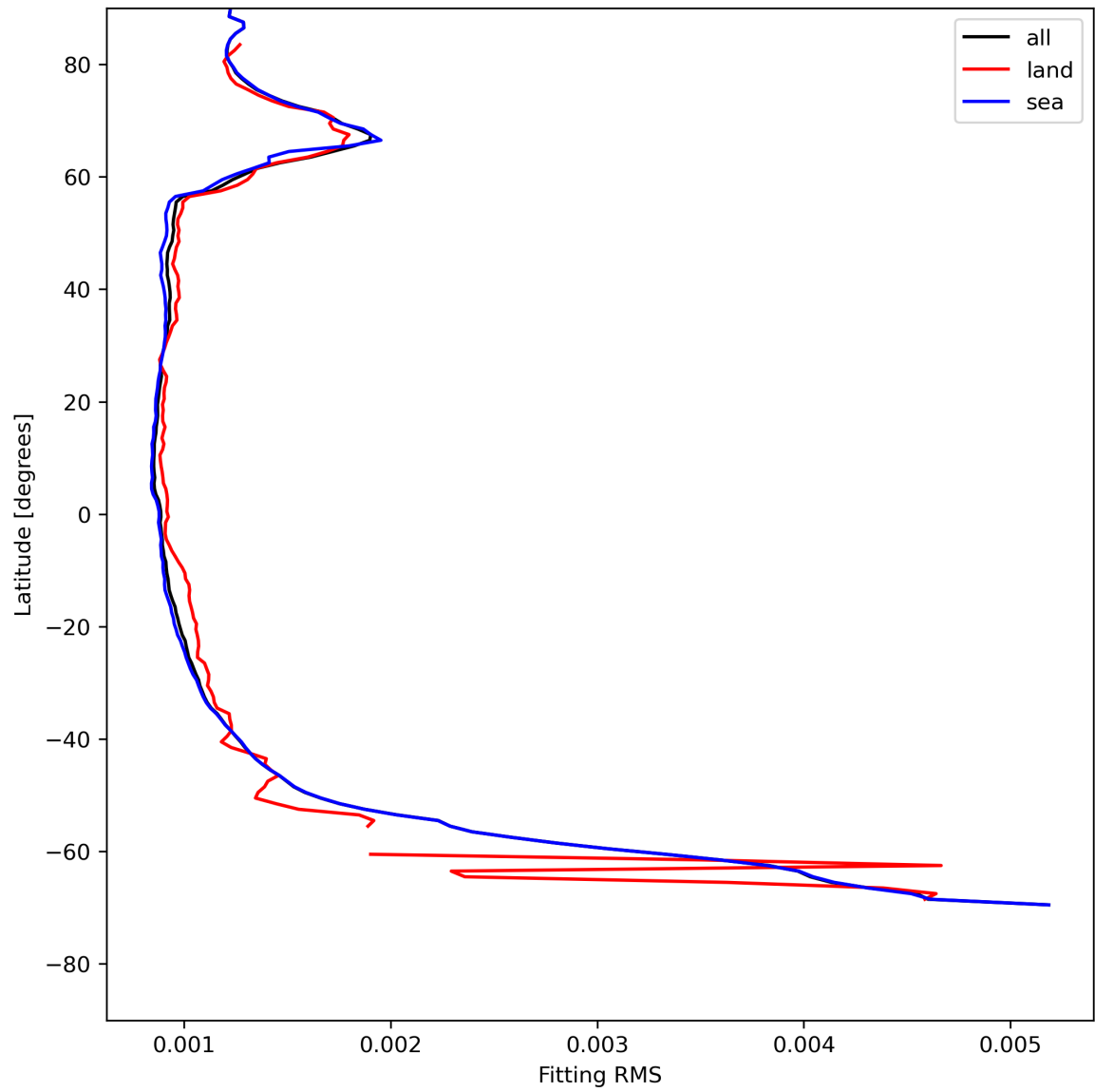
Figure 16: Zonal average of “Fitting RMS” for 2023-07-24 to 2023-07-25.
