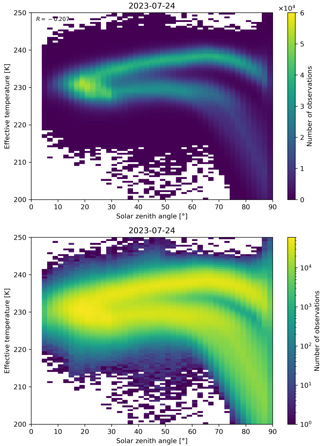
Figure 45: Scatter density plot of “Solar zenith angle” against “Effective temperature” for 2023-07-24 to 2023-07-25.
