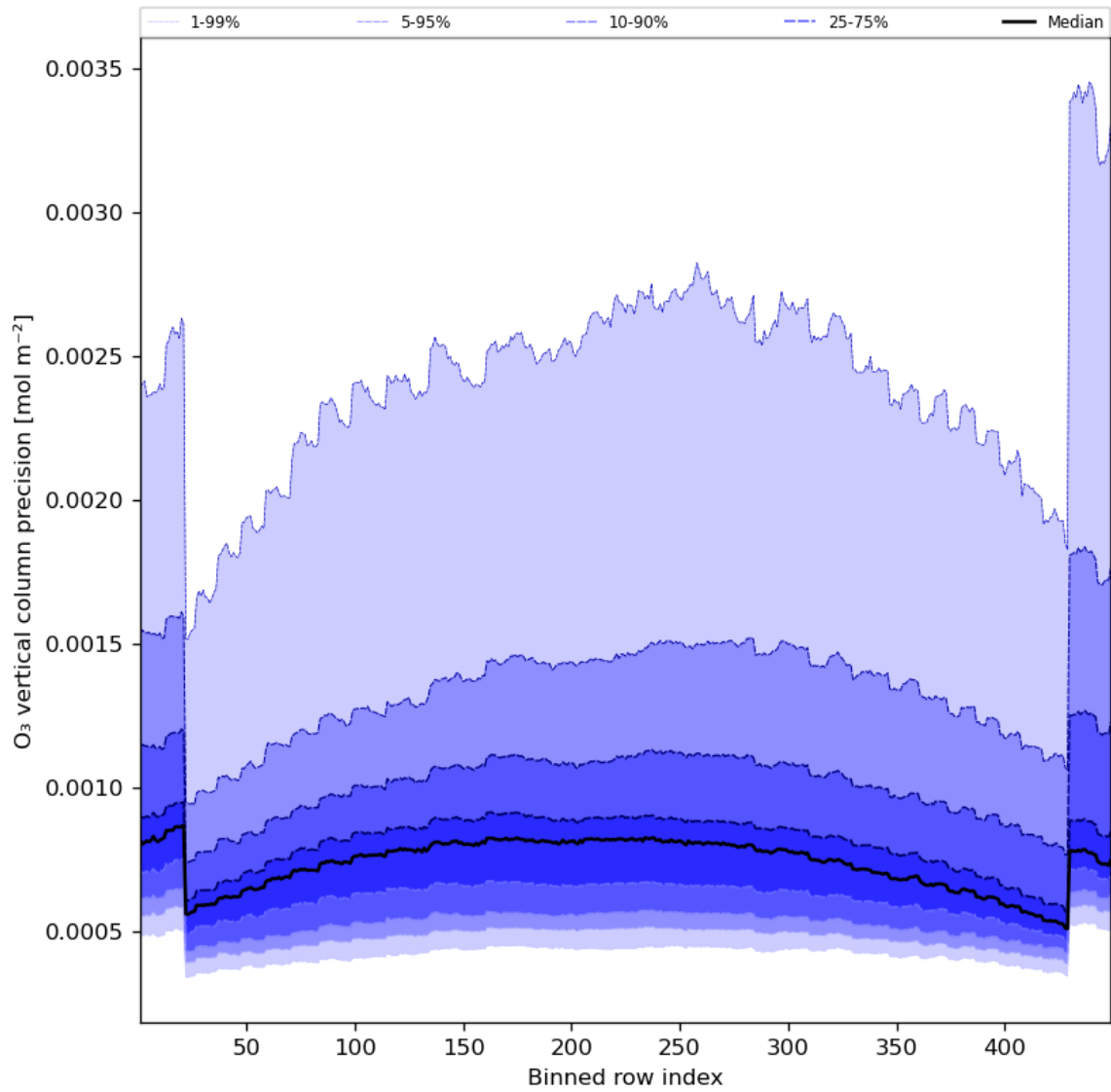
Figure 29: Along track statistics of “O 3 vertical column precision” for 2023-07-24 to 2023-07-25
