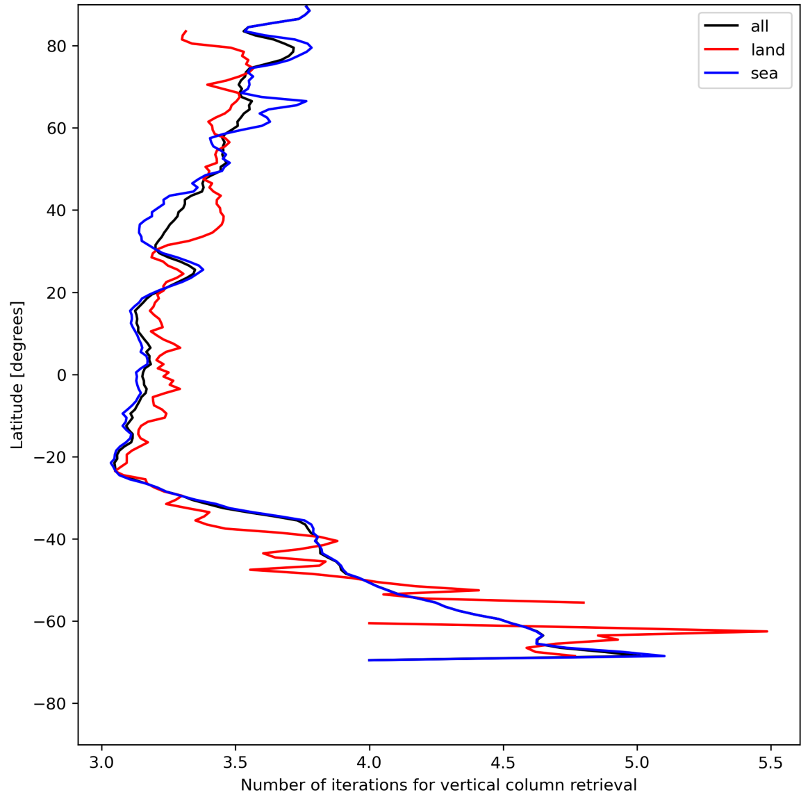
Figure 19: Zonal average of “Number of iterations for vertical column retrieval” for 2023-07-24 to 2023-07-25.
