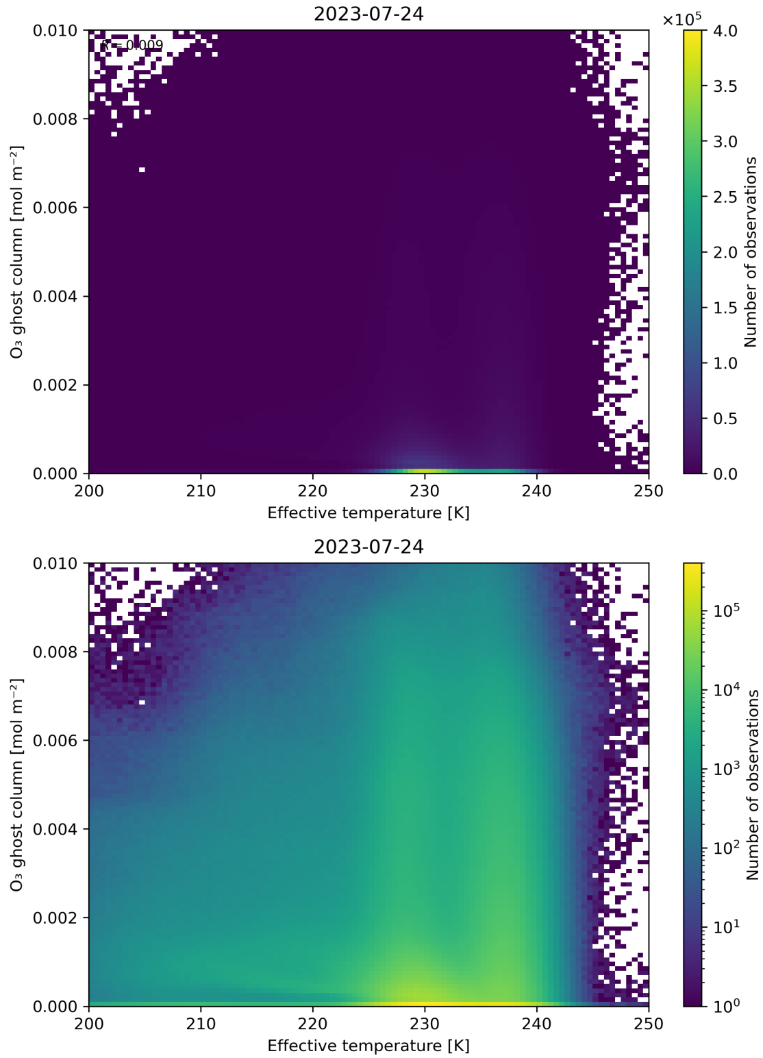
Figure 38: Scatter density plot of “Effective temperature” against “O 3 ghost column” for 2023-07-24 to 2023-07-25.
