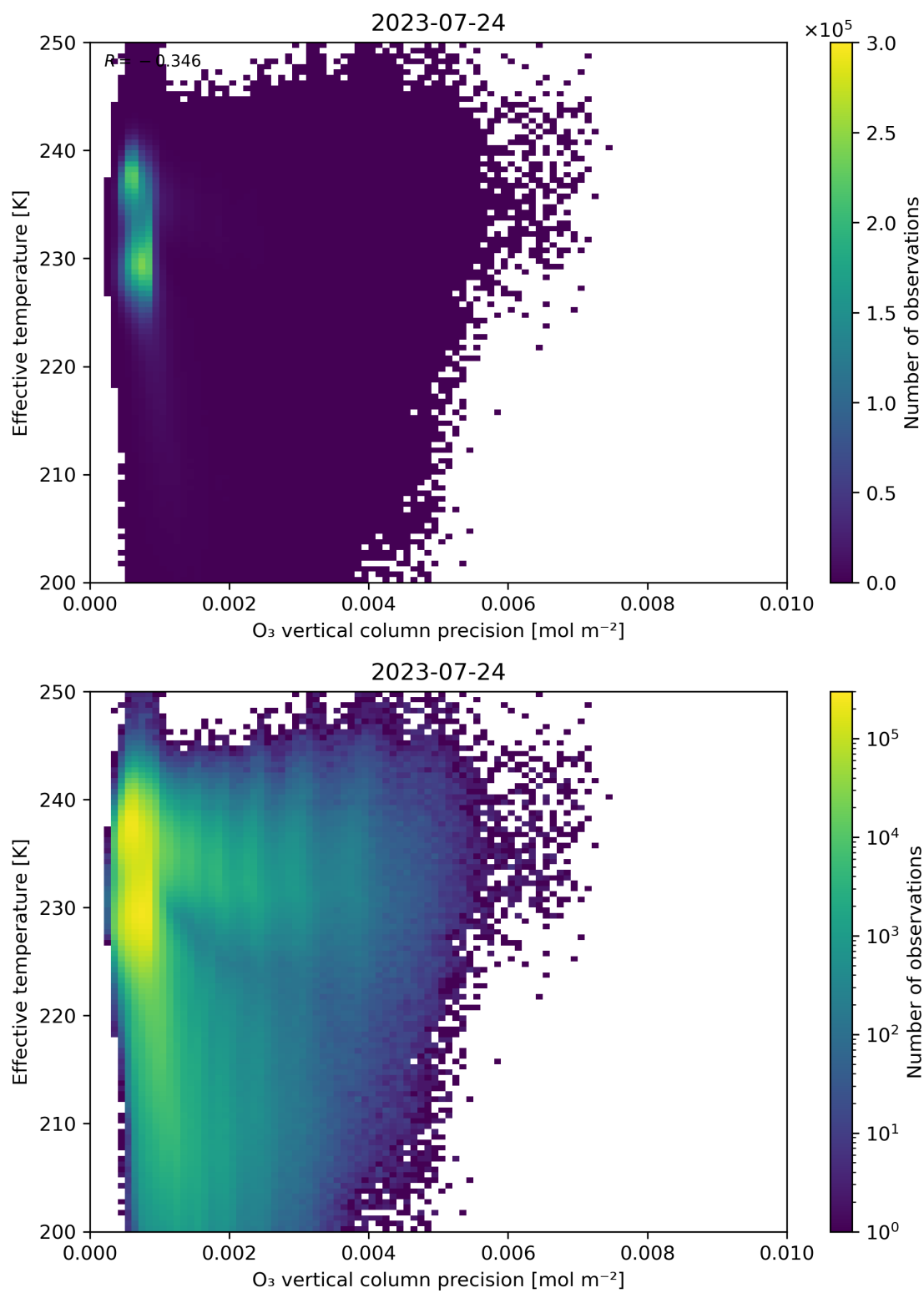
Figure 42: Scatter density plot of “O 3 vertical column precision” against “Effective temperature” for 2023-07-24 to 2023-07-25.
