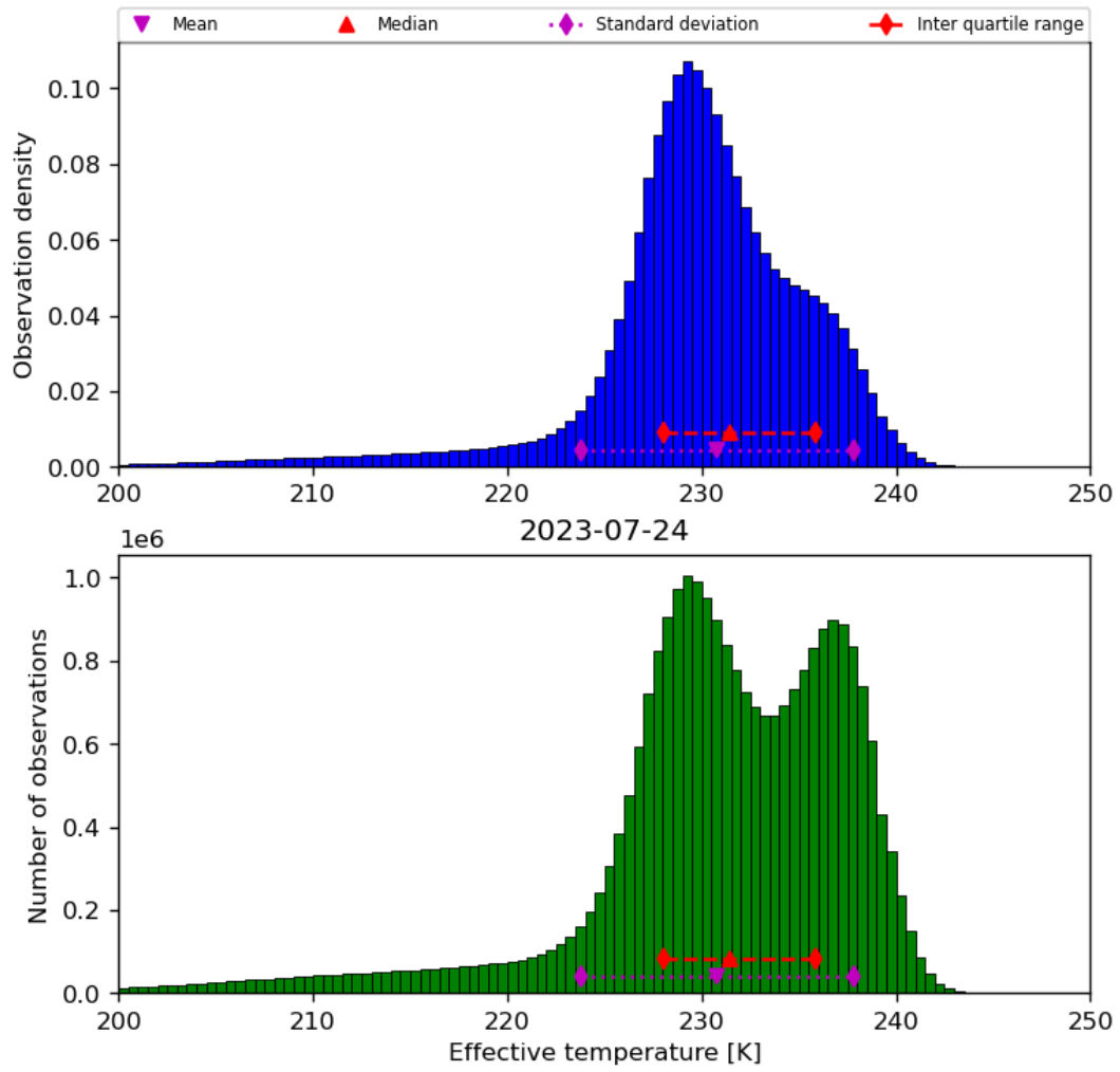
Figure 24: Histogram of “Effective temperature” for 2023-07-24 to 2023-07-25
