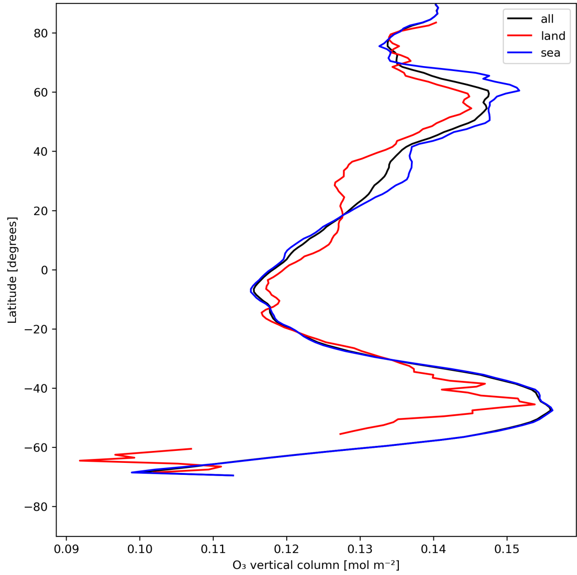
Figure 14: Zonal average of “O 3 vertical column” for 2023-07-24 to 2023-07-25.
