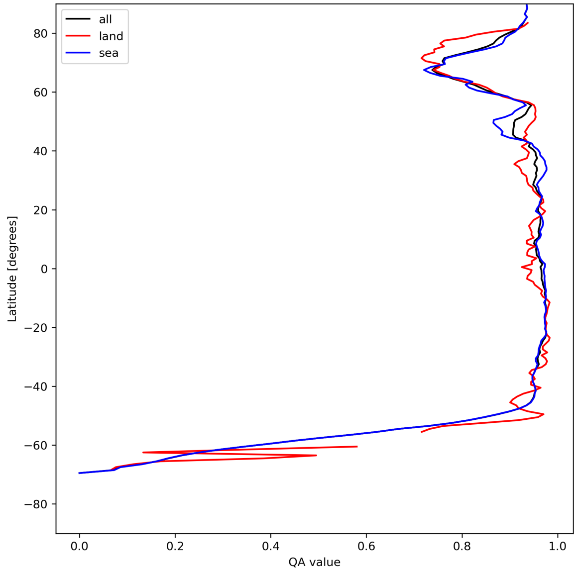
Figure 13: Zonal average of “QA value” for 2023-07-24 to 2023-07-25.
