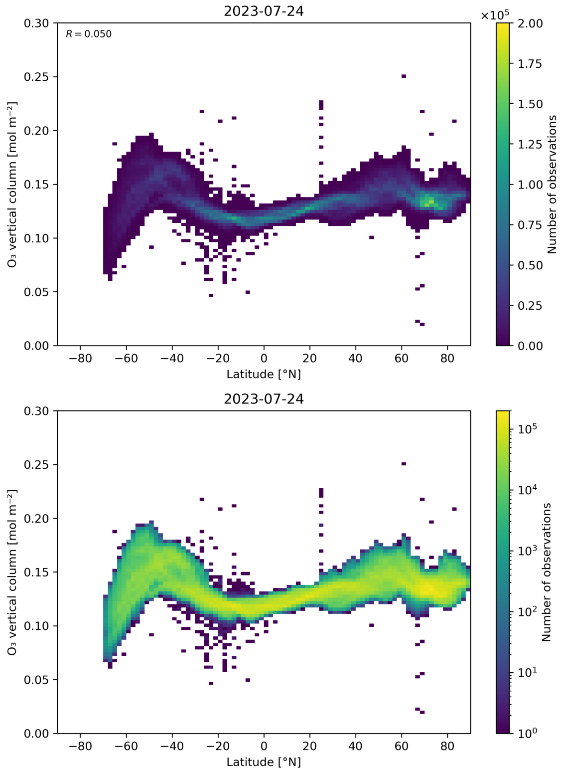
Figure 36: Scatter density plot of “Latitude” against “O 3 vertical column” for 2023-07-24 to 2023-07-25.
