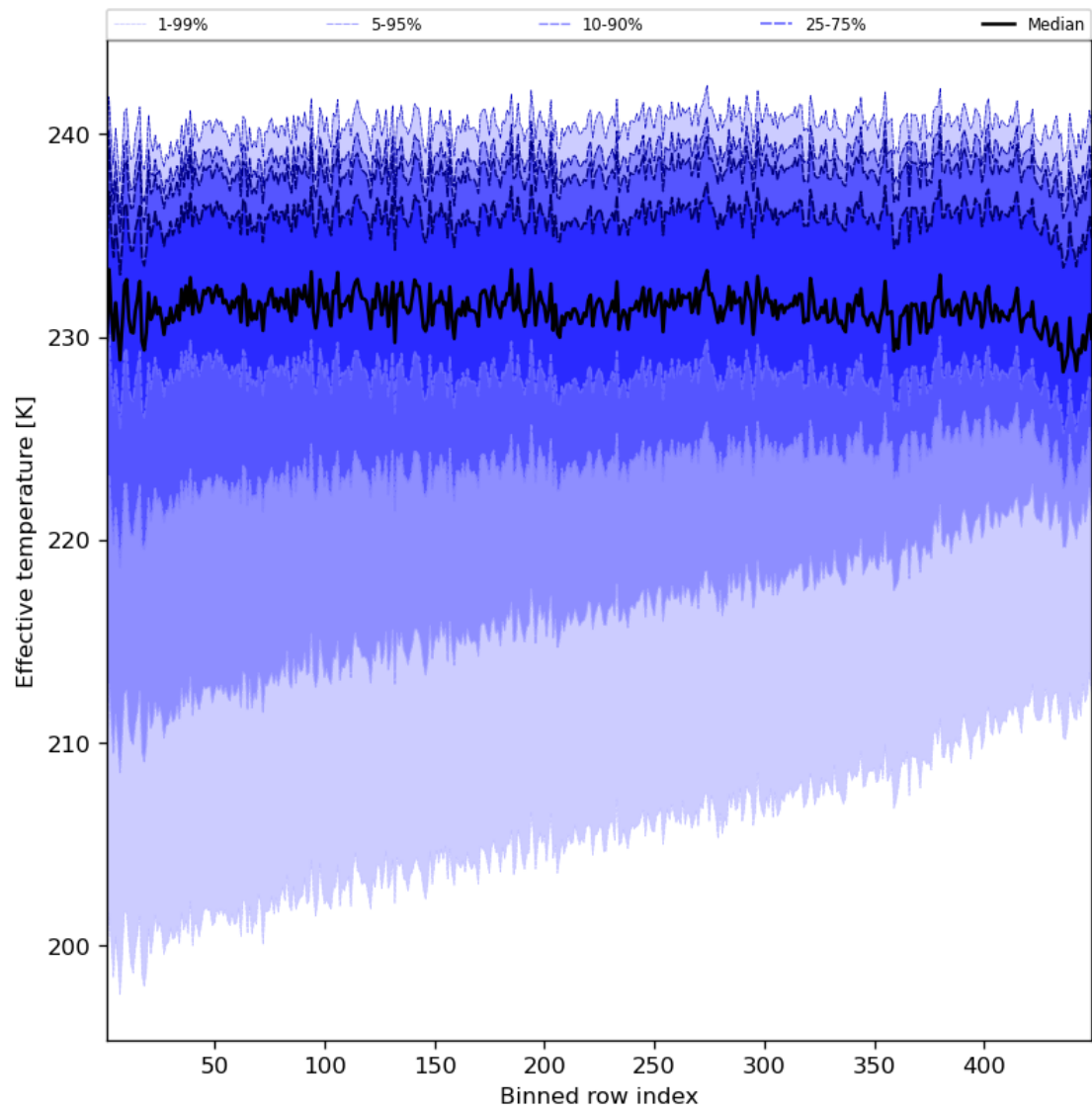
Figure 31: Along track statistics of “Effective temperature” for 2023-07-24 to 2023-07-25
