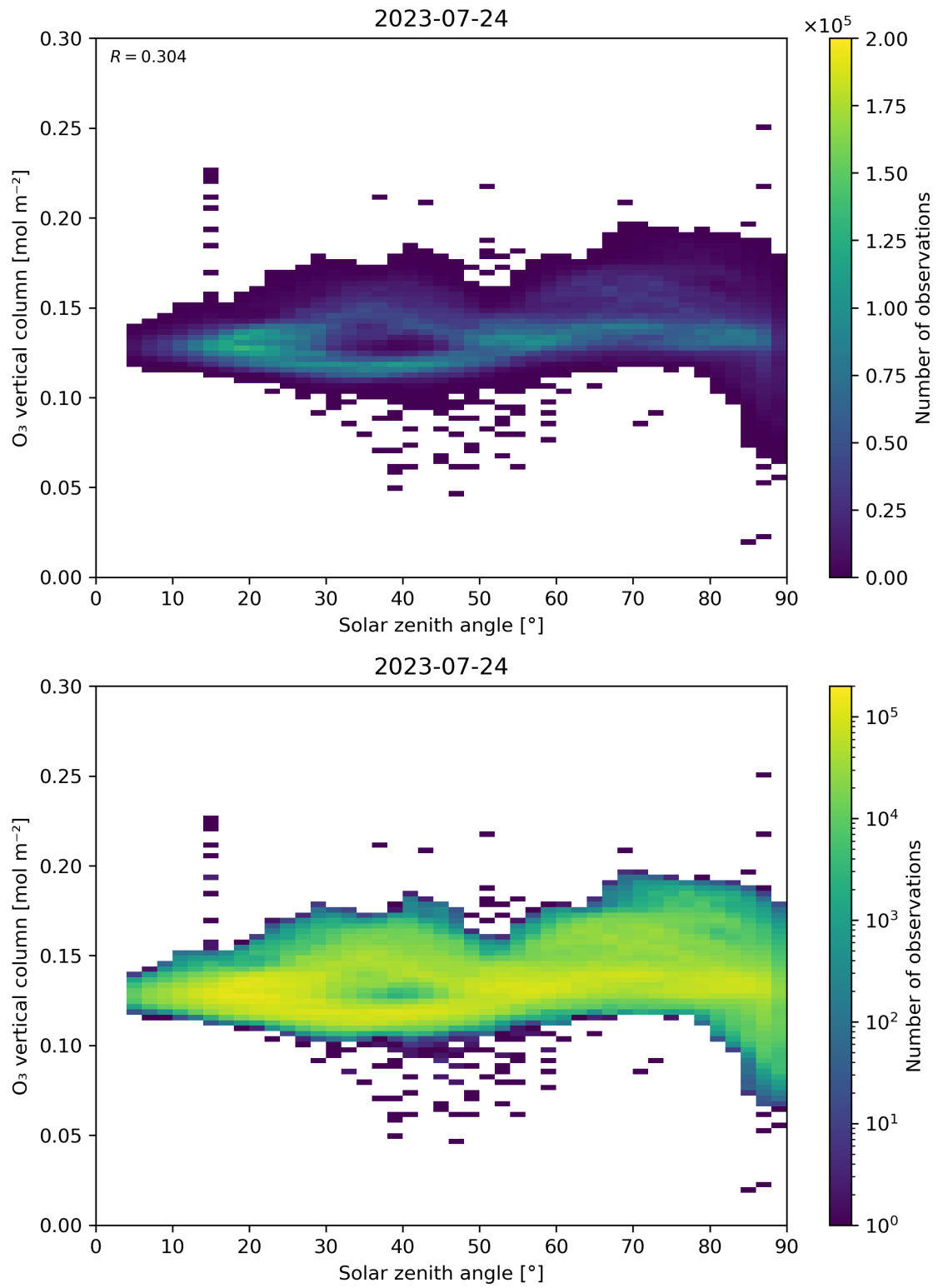
Figure 47: Scatter density plot of “Solar zenith angle” against “O 3 vertical column” for 2023-07-24 to 2023-07-25.
