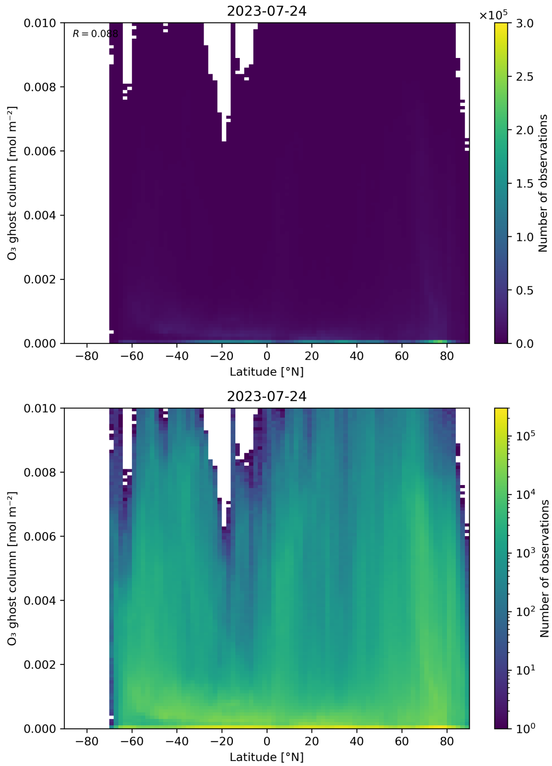
Figure 35: Scatter density plot of “Latitude” against “O 3 ghost column” for 2023-07-24 to 2023-07-25.
