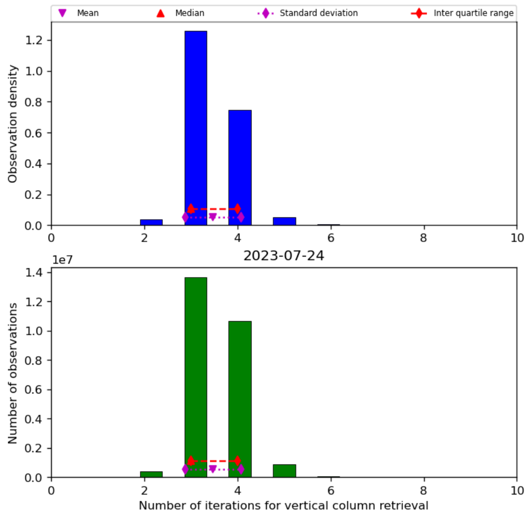
Figure 26: Histogram of “Number of iterations for vertical column retrieval” for 2023-07-24 to 2023-07-25
