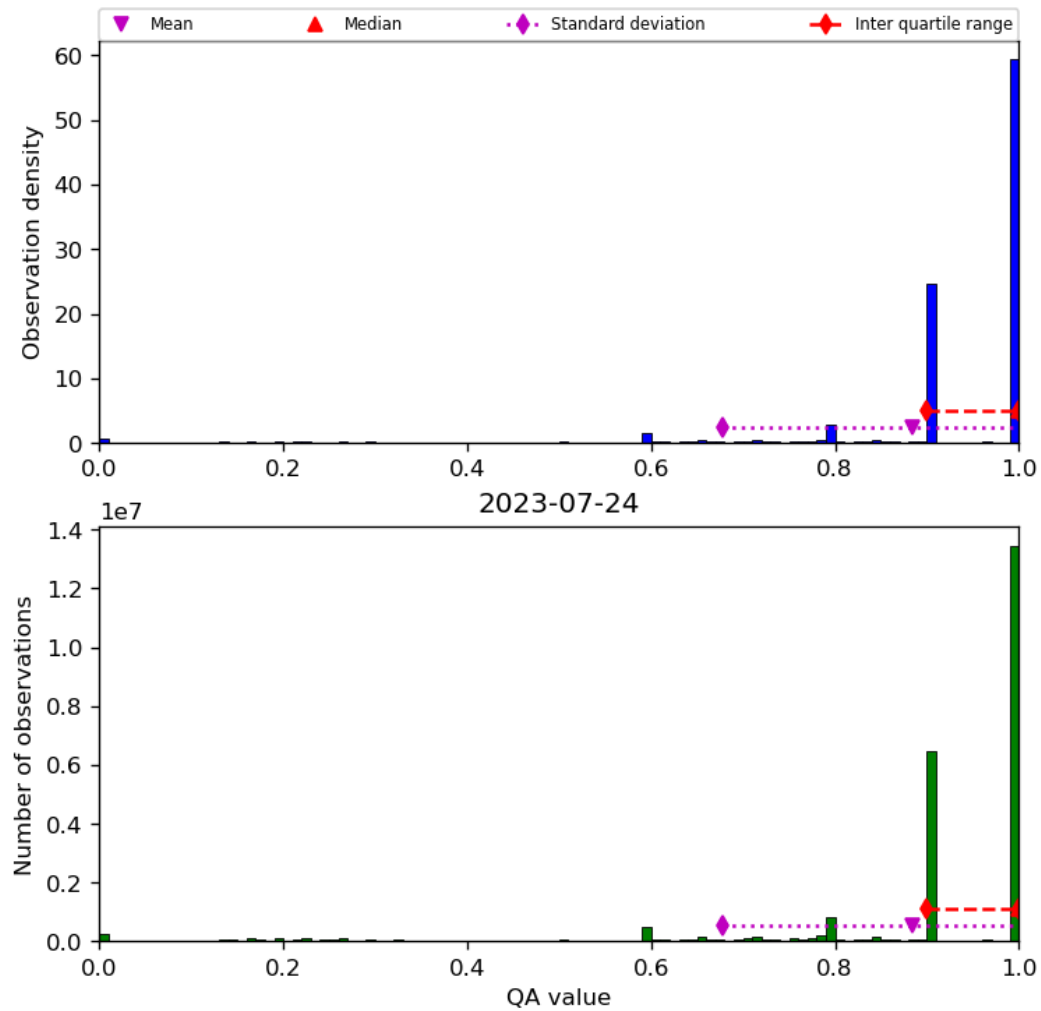
Figure 20: Histogram of “QA value” for 2023-07-24 to 2023-07-25
