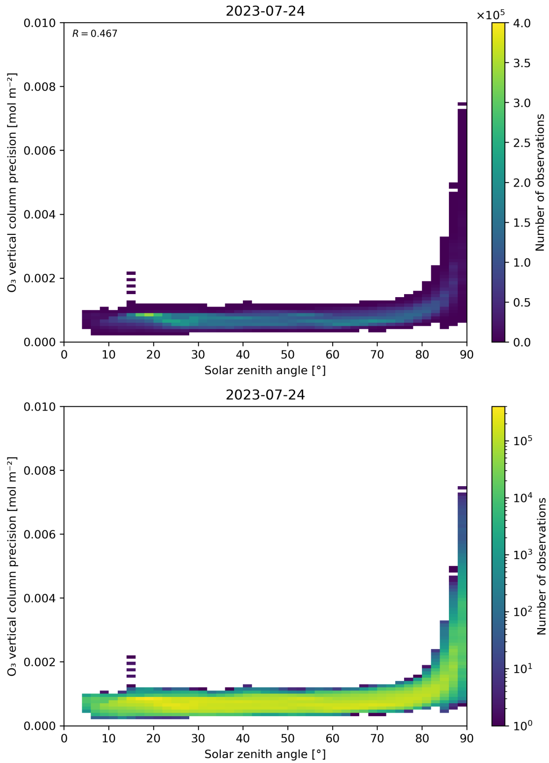
Figure 48: Scatter density plot of “Solar zenith angle” against “O 3 vertical column precision” for 2023-07-24 to 2023-07-25.
