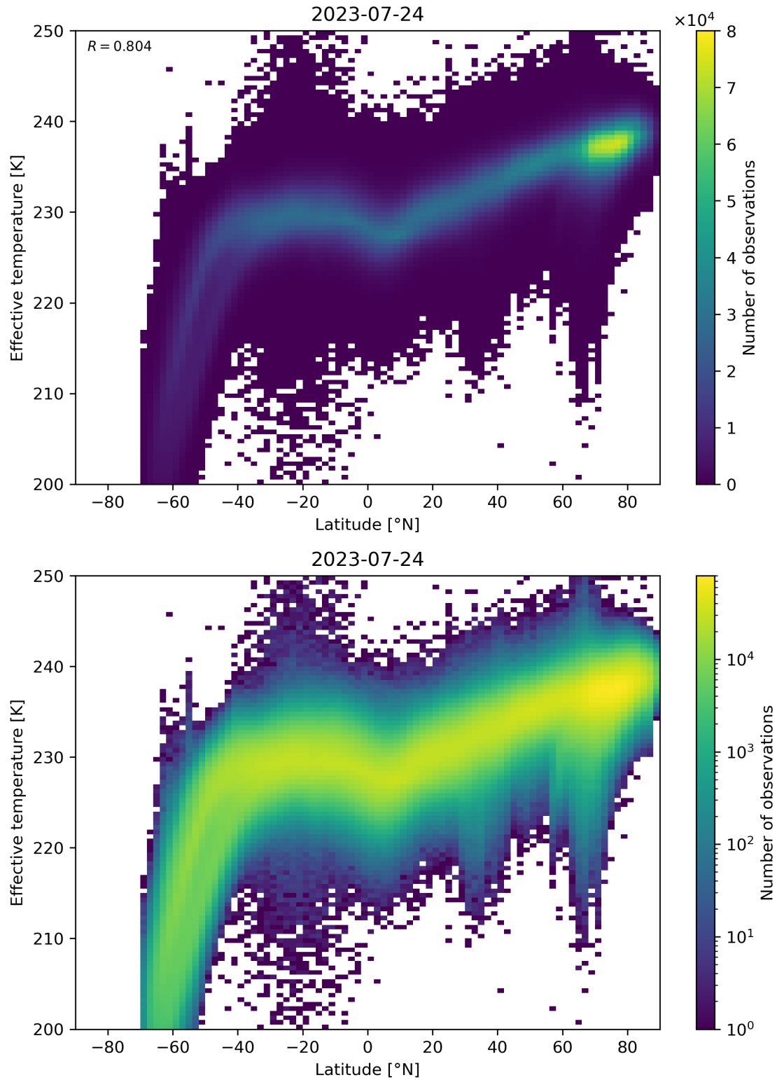
Figure 34: Scatter density plot of “Latitude” against “Effective temperature” for 2023-07-24 to 2023-07-25.
