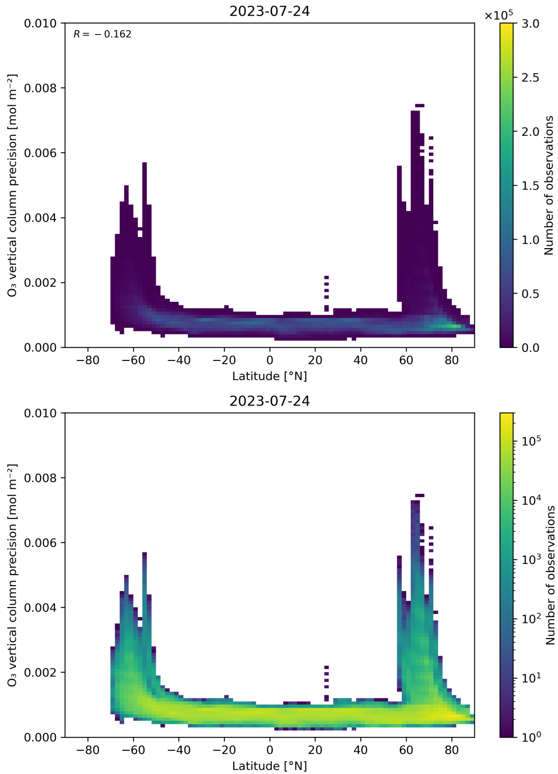
Figure 37: Scatter density plot of “Latitude” against “O 3 vertical column precision” for 2023-07-24 to 2023-07-25.
