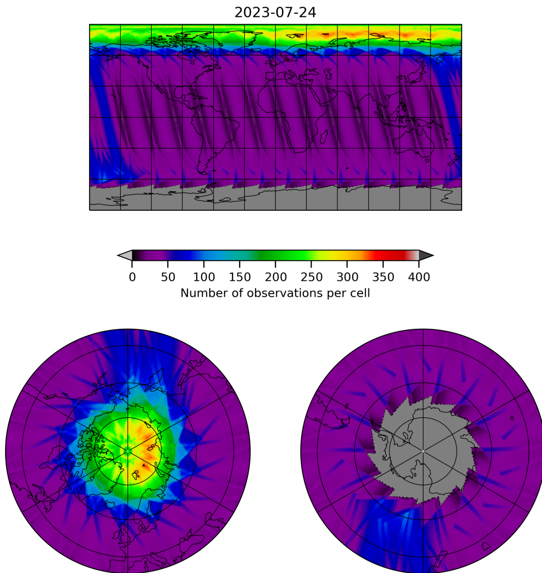
Figure 12: Map of the number of observations for 2023-07-24 to 2023-07-25
