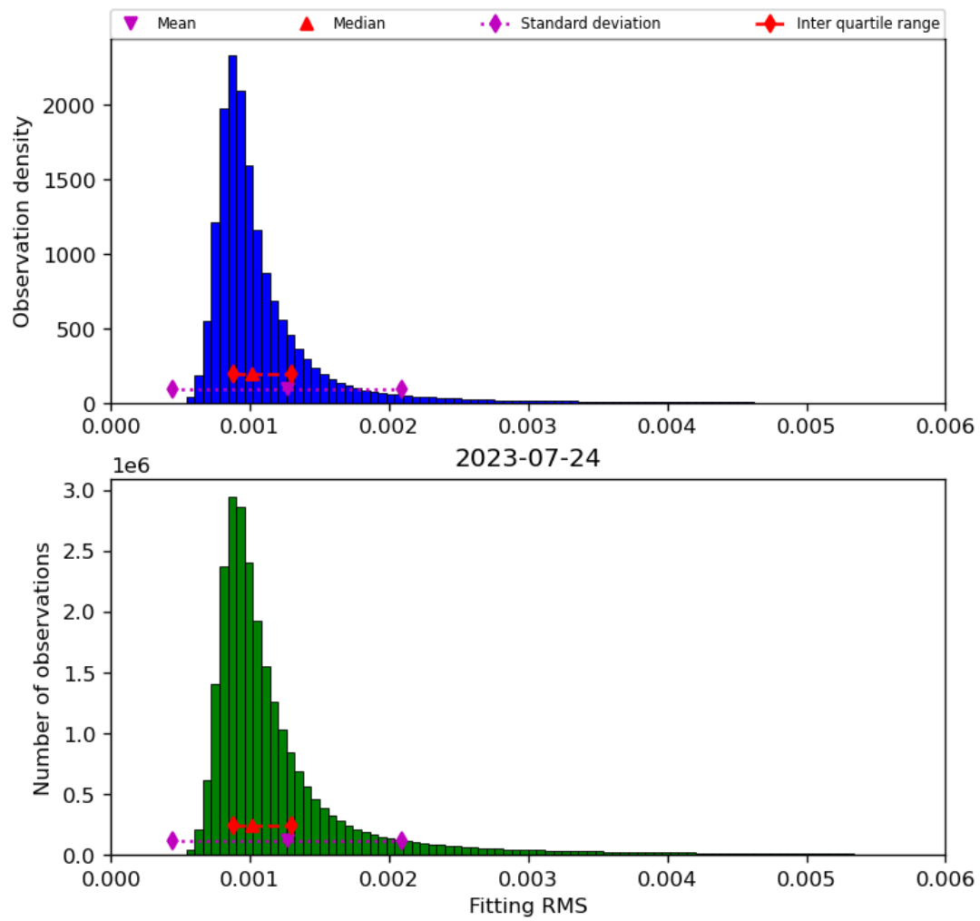
Figure 23: Histogram of “Fitting RMS” for 2023-07-24 to 2023-07-25
