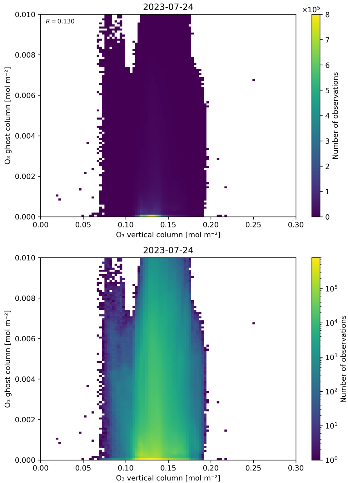
Figure 40: Scatter density plot of “O 3 vertical column” against “O 3 ghost column” for 2023-07-24 to 2023-07-25.
