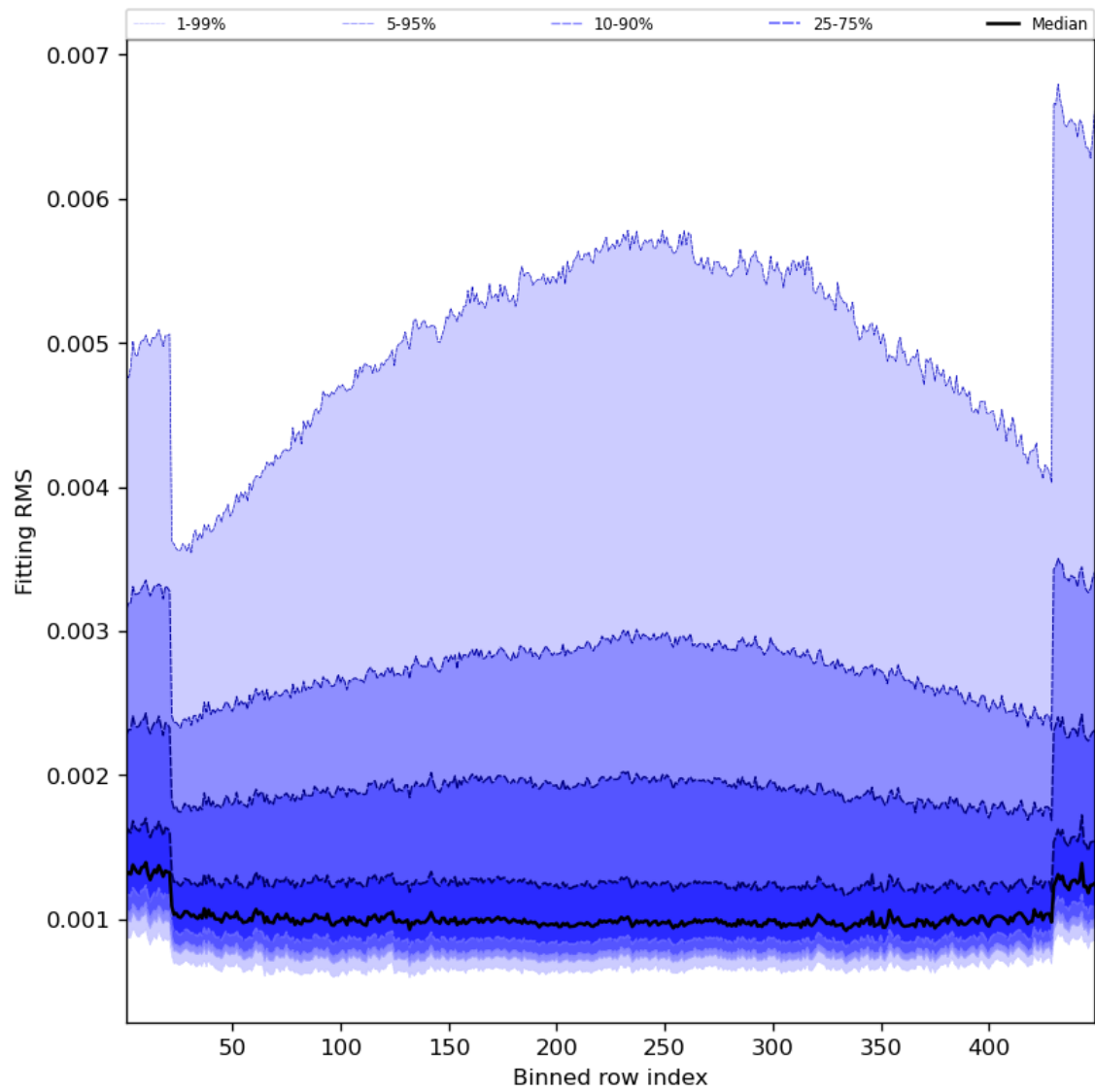
Figure 30: Along track statistics of “Fitting RMS” for 2023-07-24 to 2023-07-25
