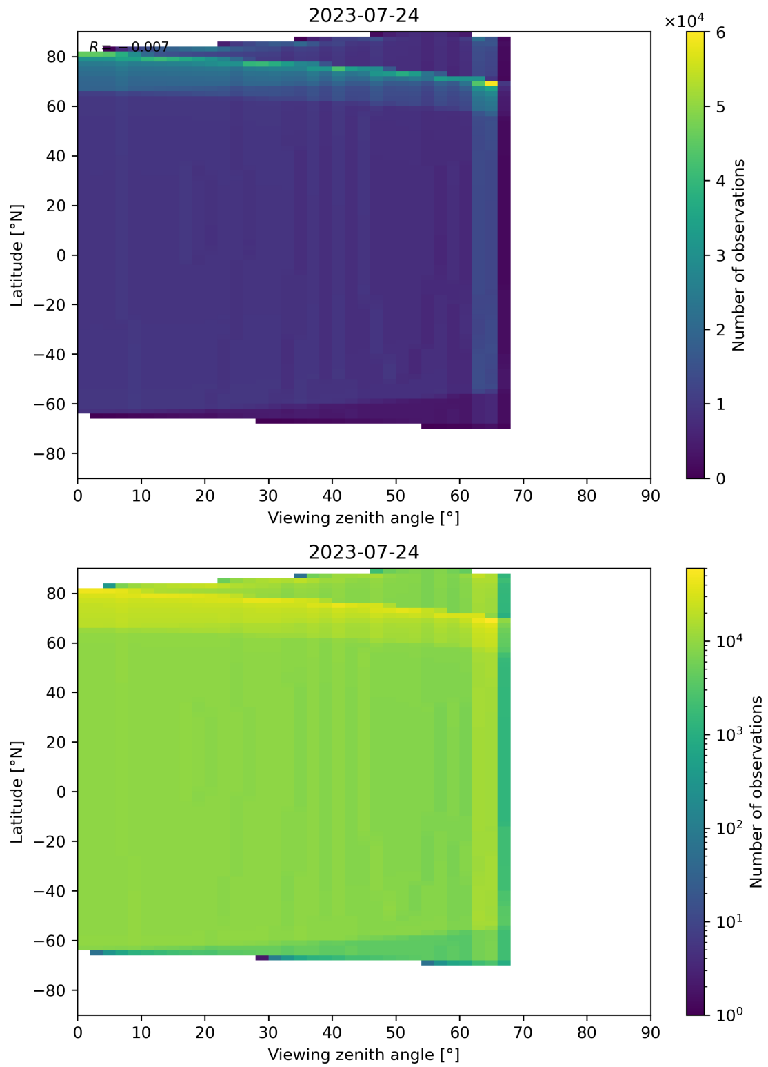
Figure 49: Scatter density plot of “Viewing zenith angle” against “Latitude” for 2023-07-24 to 2023-07-25.
