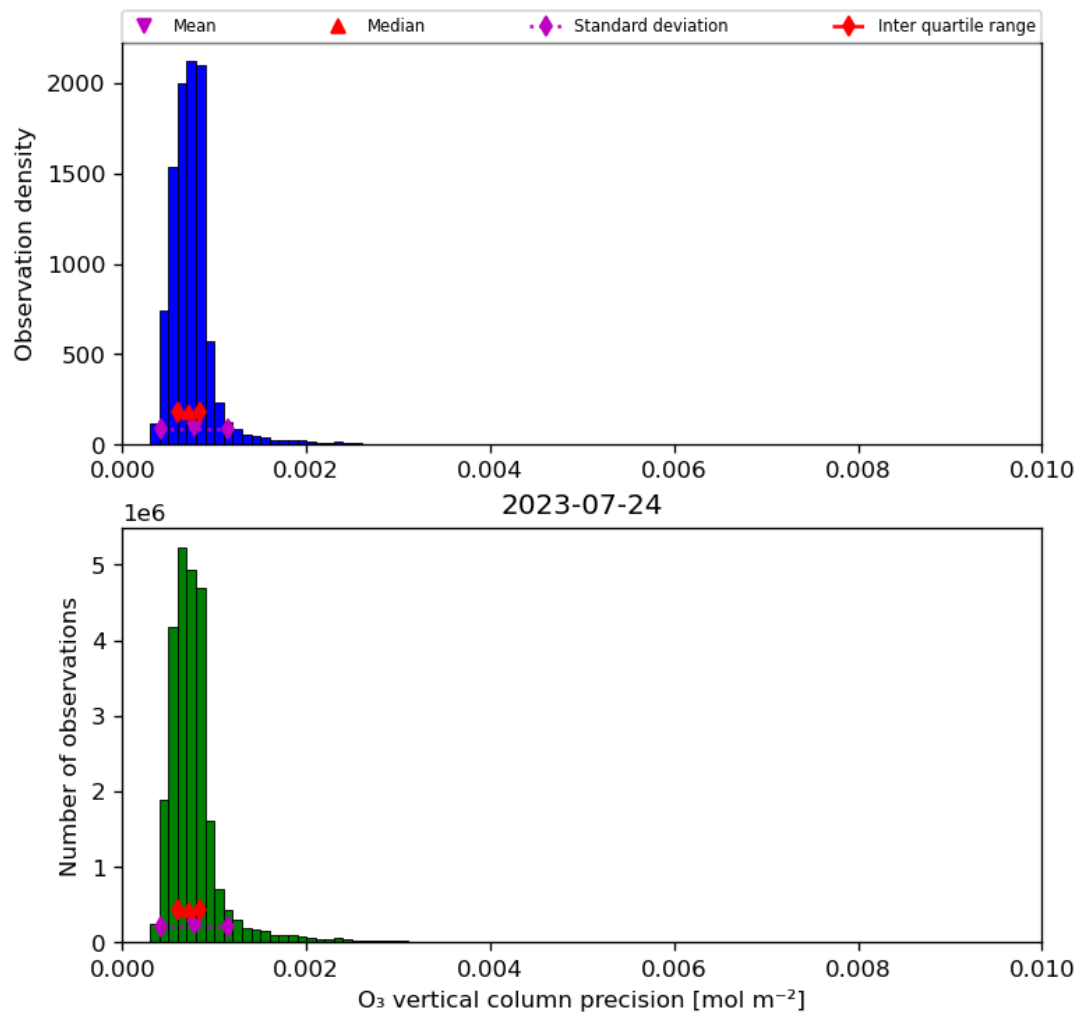
Figure 22: Histogram of “O 3 vertical column precision” for 2023-07-24 to 2023-07-25
