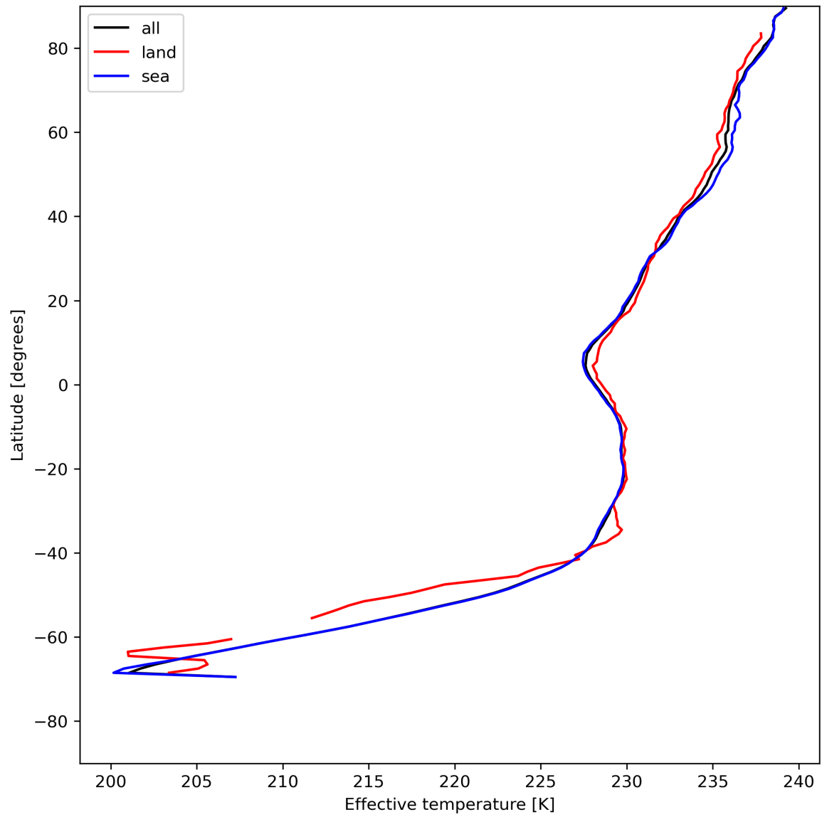
Figure 17: Zonal average of “Effective temperature” for 2023-07-24 to 2023-07-25.
