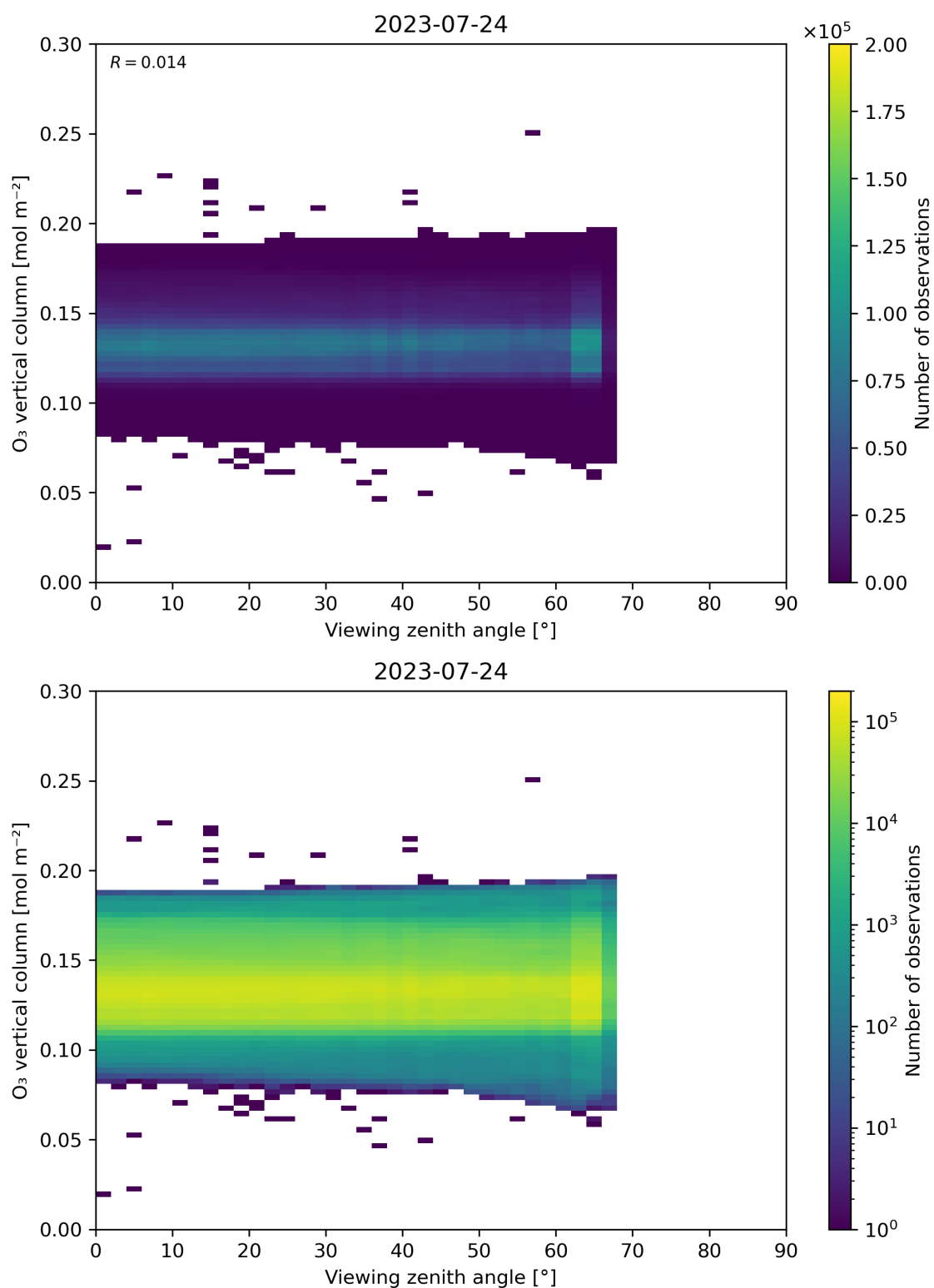
Figure 52: Scatter density plot of “Viewing zenith angle” against “O 3 vertical column” for 2023-07-24 to 2023-07-25.
