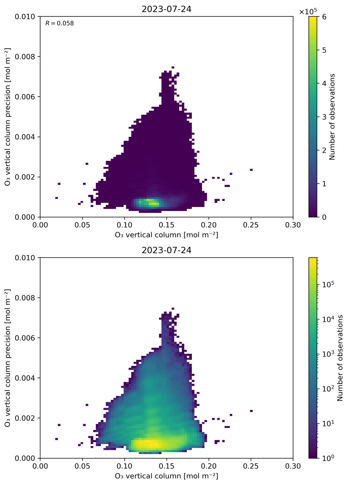
Figure 41: Scatter density plot of “O 3 vertical column” against “O 3 vertical column precision” for 2023-07-24 to 2023-07-25.
