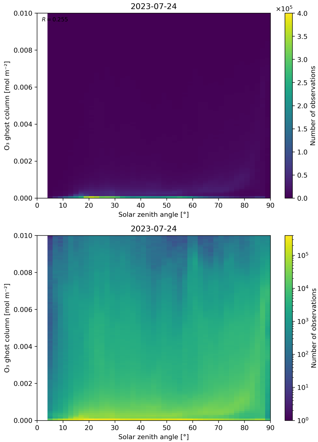
Figure 46: Scatter density plot of “Solar zenith angle” against “O 3 ghost column” for 2023-07-24 to 2023-07-25.
