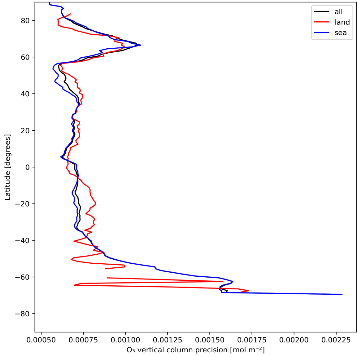
Figure 15: Zonal average of “O 3 vertical column precision” for 2023-07-24 to 2023-07-25.
