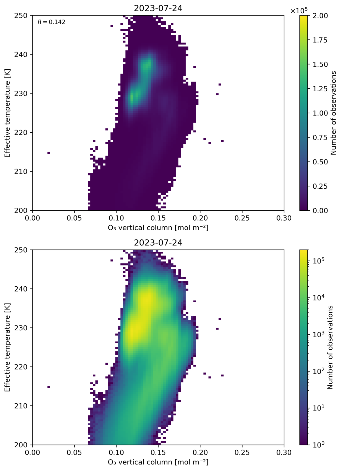
Figure 39: Scatter density plot of “O 3 vertical column” against “Effective temperature” for 2023-07-24 to 2023-07-25.
