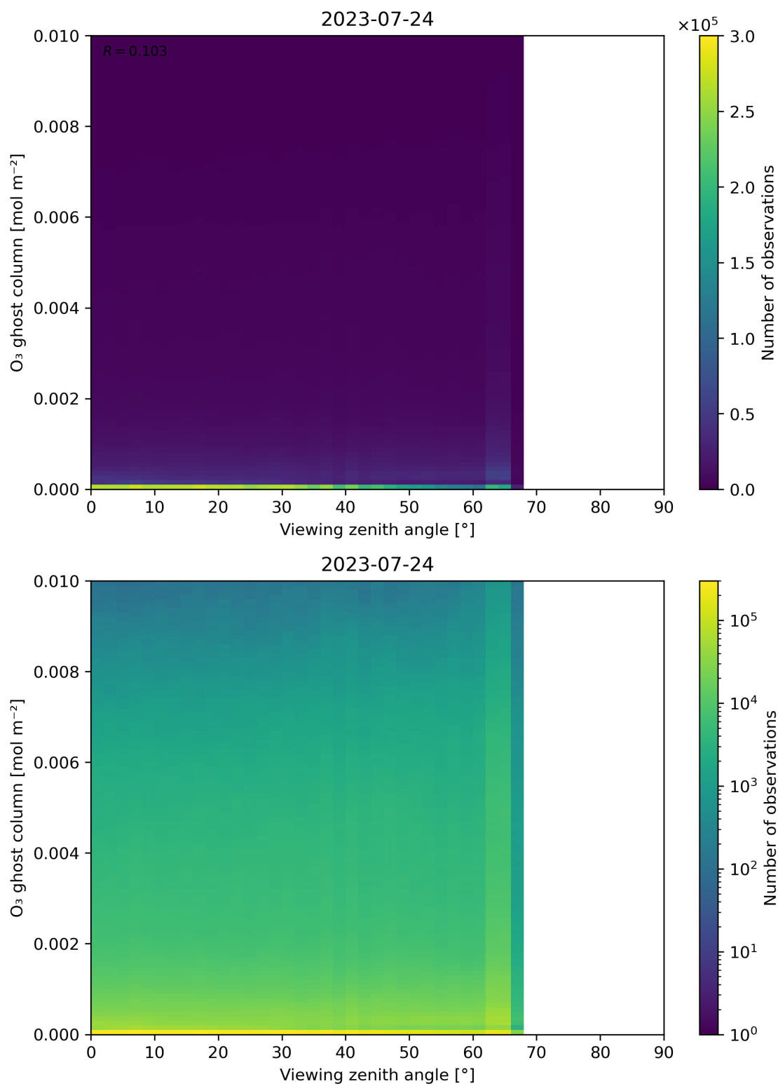
Figure 51: Scatter density plot of “Viewing zenith angle” against “O 3 ghost column” for 2023-07-24 to 2023-07-25.
