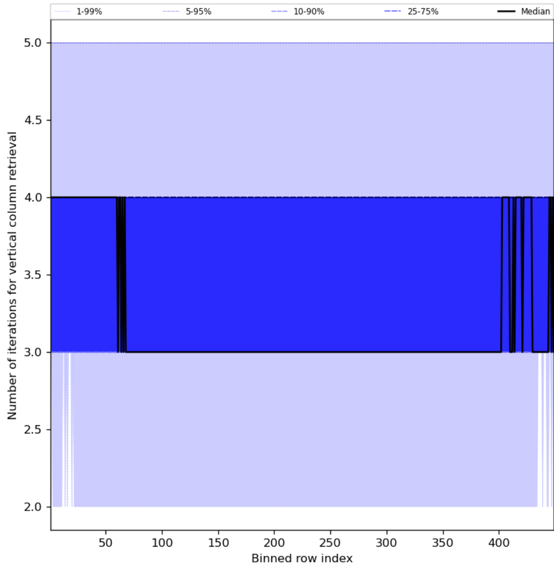
Figure 33: Along track statistics of “Number of iterations for vertical column retrieval” for 2023-07-24 to 2023-07-25
