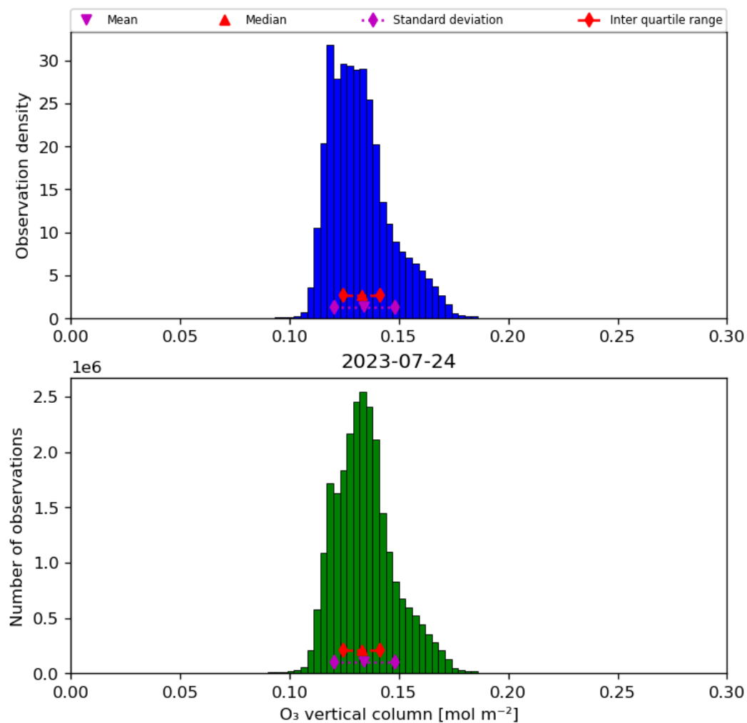
Figure 21: Histogram of “O 3 vertical column” for 2023-07-24 to 2023-07-25
