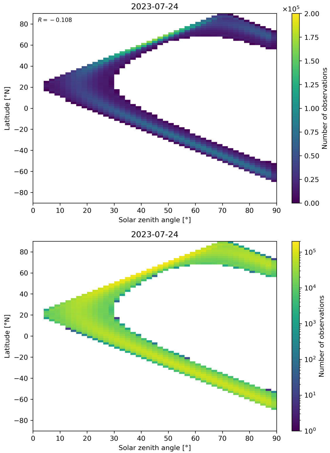
Figure 44: Scatter density plot of “Solar zenith angle” against “Latitude” for 2023-07-24 to 2023-07-25.
