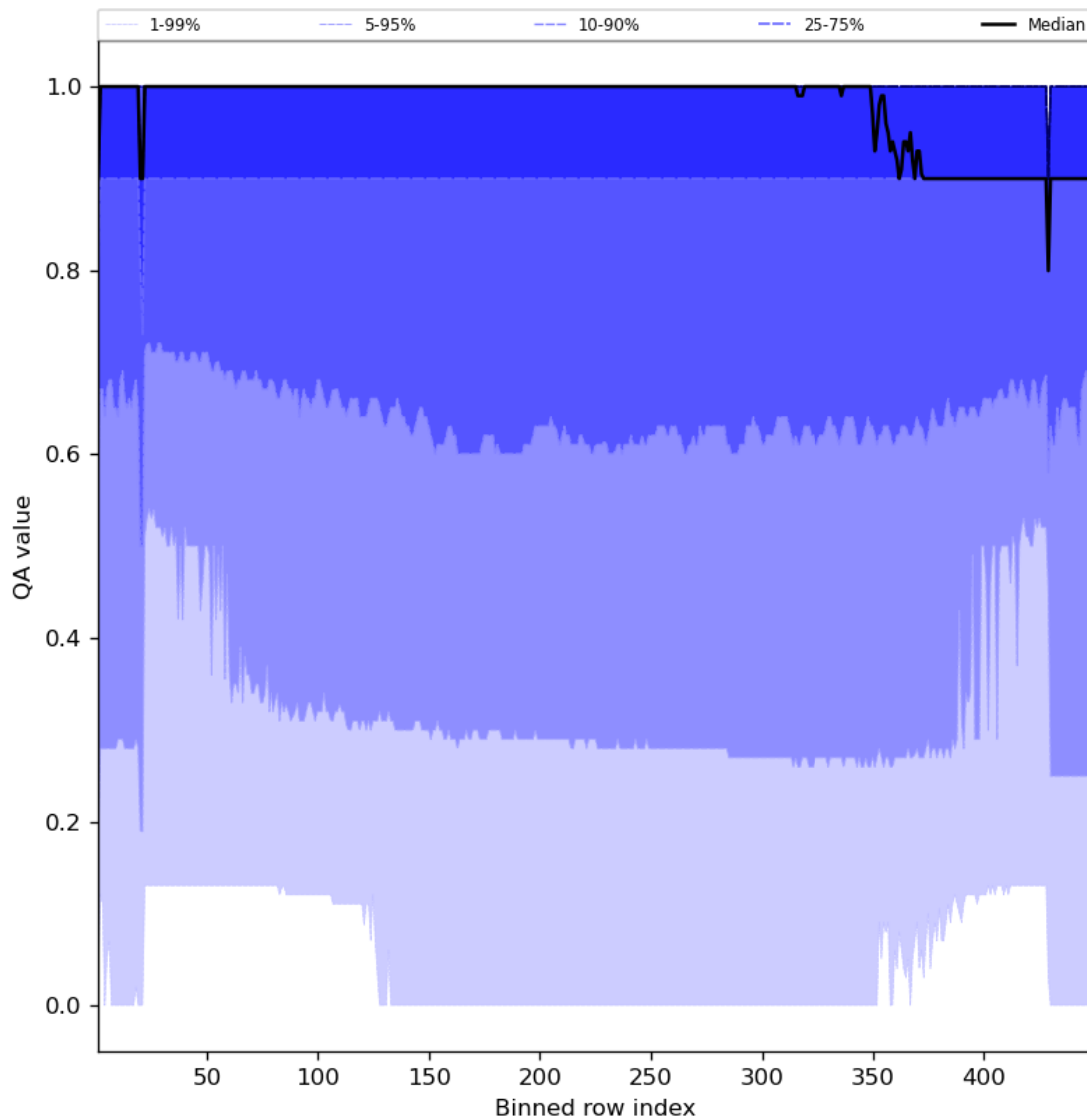
Figure 27: Along track statistics of “QA value” for 2023-07-24 to 2023-07-25
