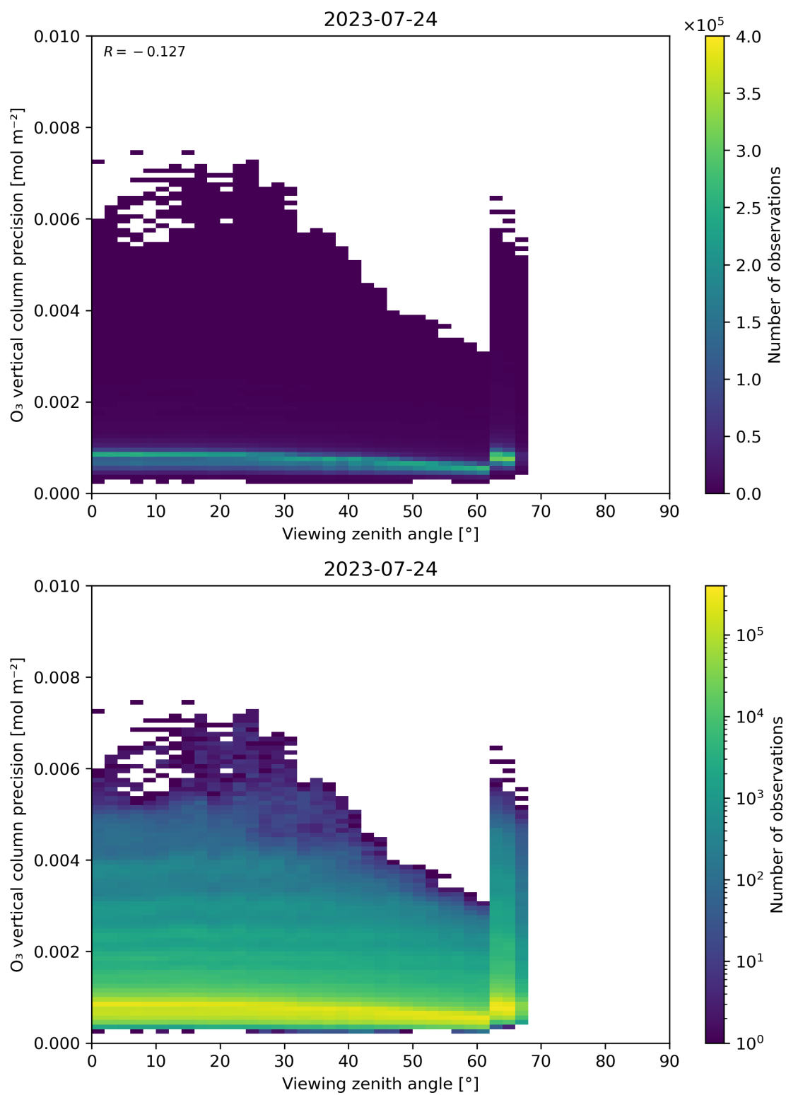
Figure 53: Scatter density plot of “Viewing zenith angle” against “O 3 vertical column precision” for 2023-07-24 to 2023-07-25.
