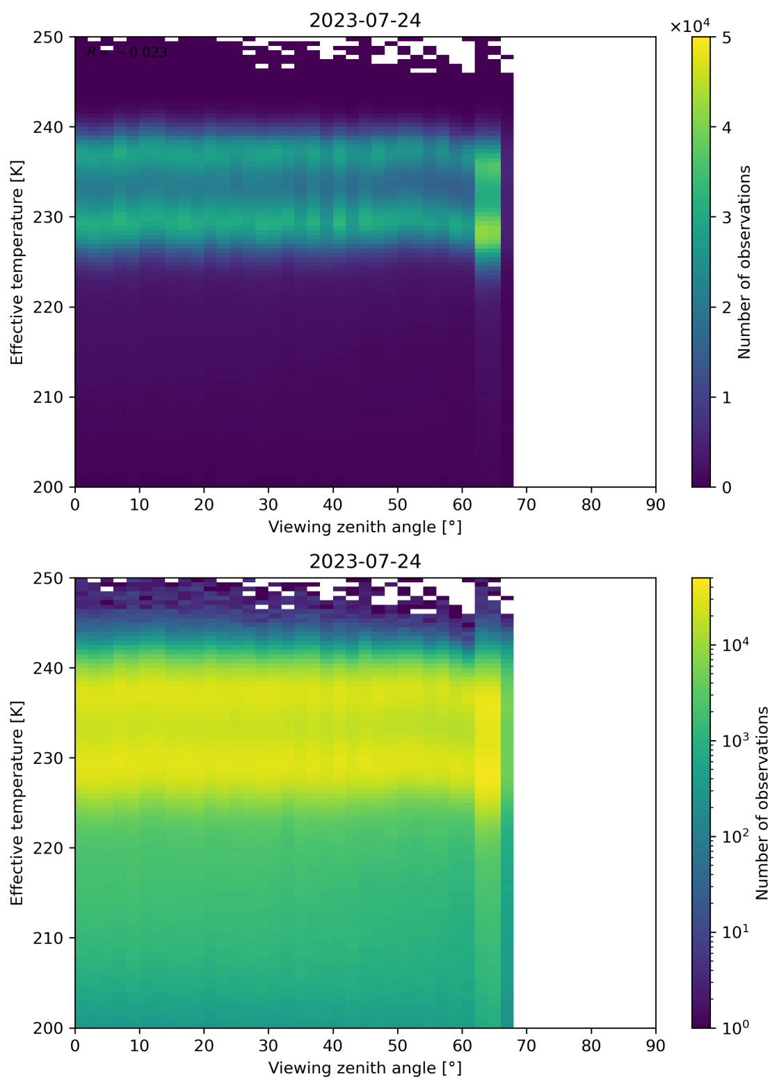
Figure 50: Scatter density plot of “Viewing zenith angle” against “Effective temperature” for 2023-07-24 to 2023-07-25.
