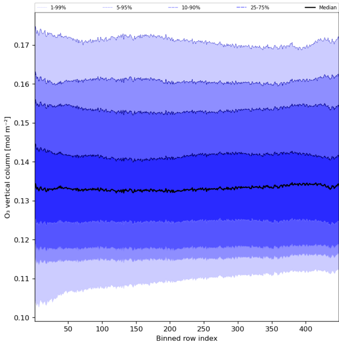
Figure 28: Along track statistics of “O 3 vertical column” for 2023-07-24 to 2023-07-25
