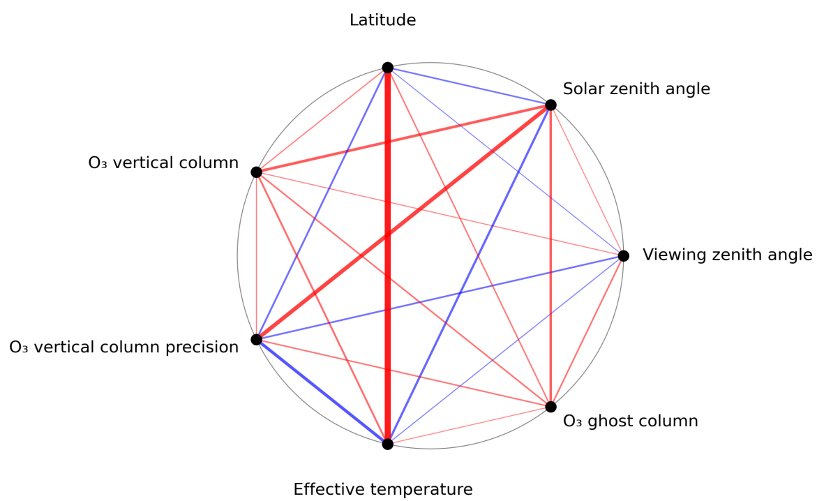
Figure 1: Map of correlation graph for 2023-07-24 to 2023-07-26.
