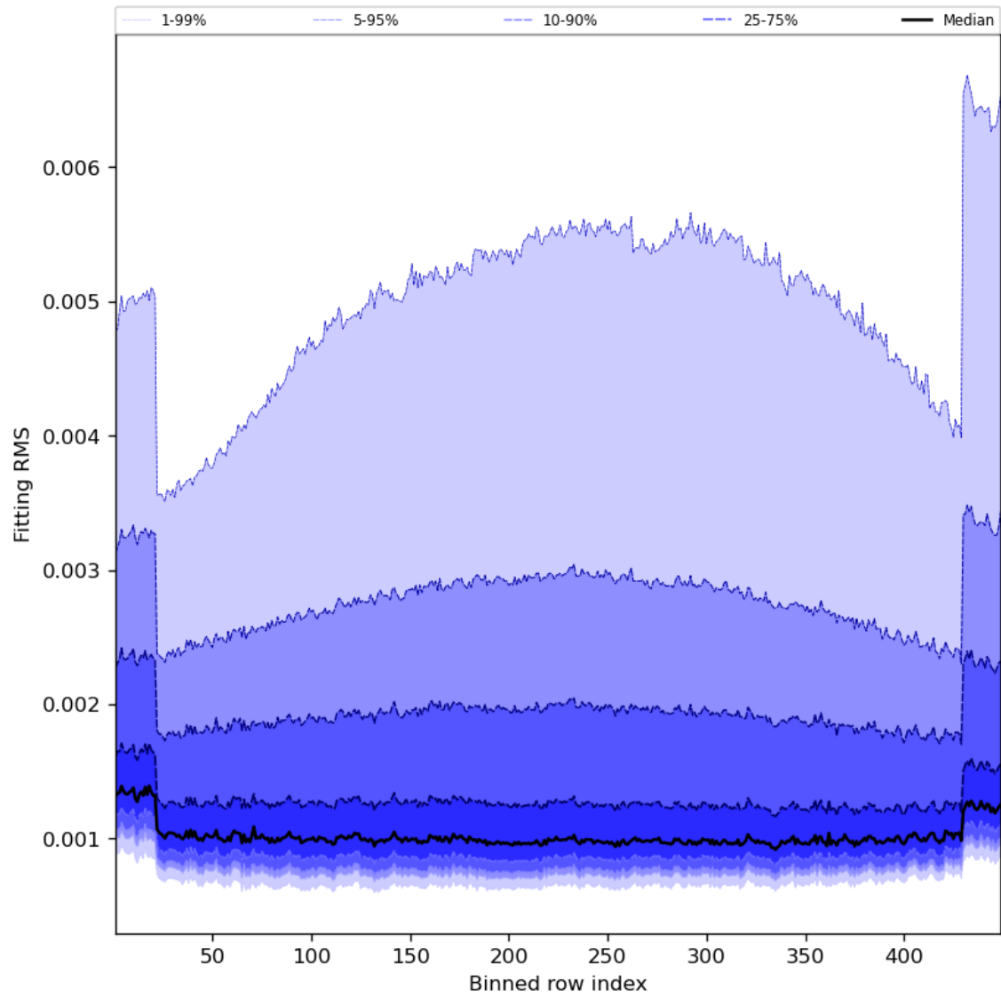
Figure 30: Along track statistics of “Fitting RMS” for 2023-07-24 to 2023-07-26
