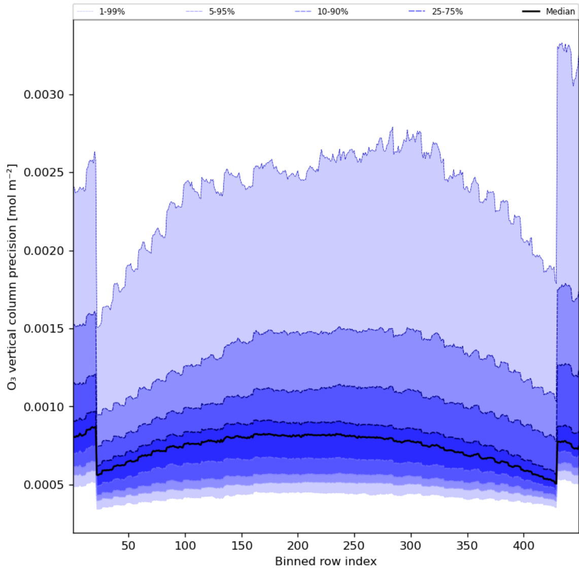
Figure 29: Along track statistics of “O 3 vertical column precision” for 2023-07-24 to 2023-07-26
