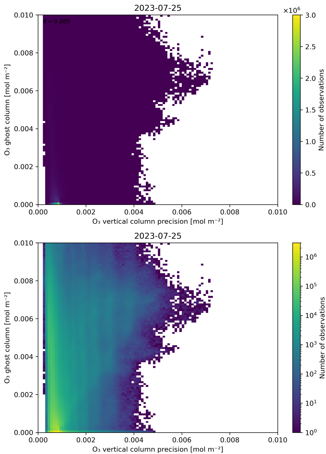
Figure 43: Scatter density plot of “ \text{O}_3 vertical column precision” against “ \text{O}_3 ghost column” for 2023-07-24 to 2023-07-26.
