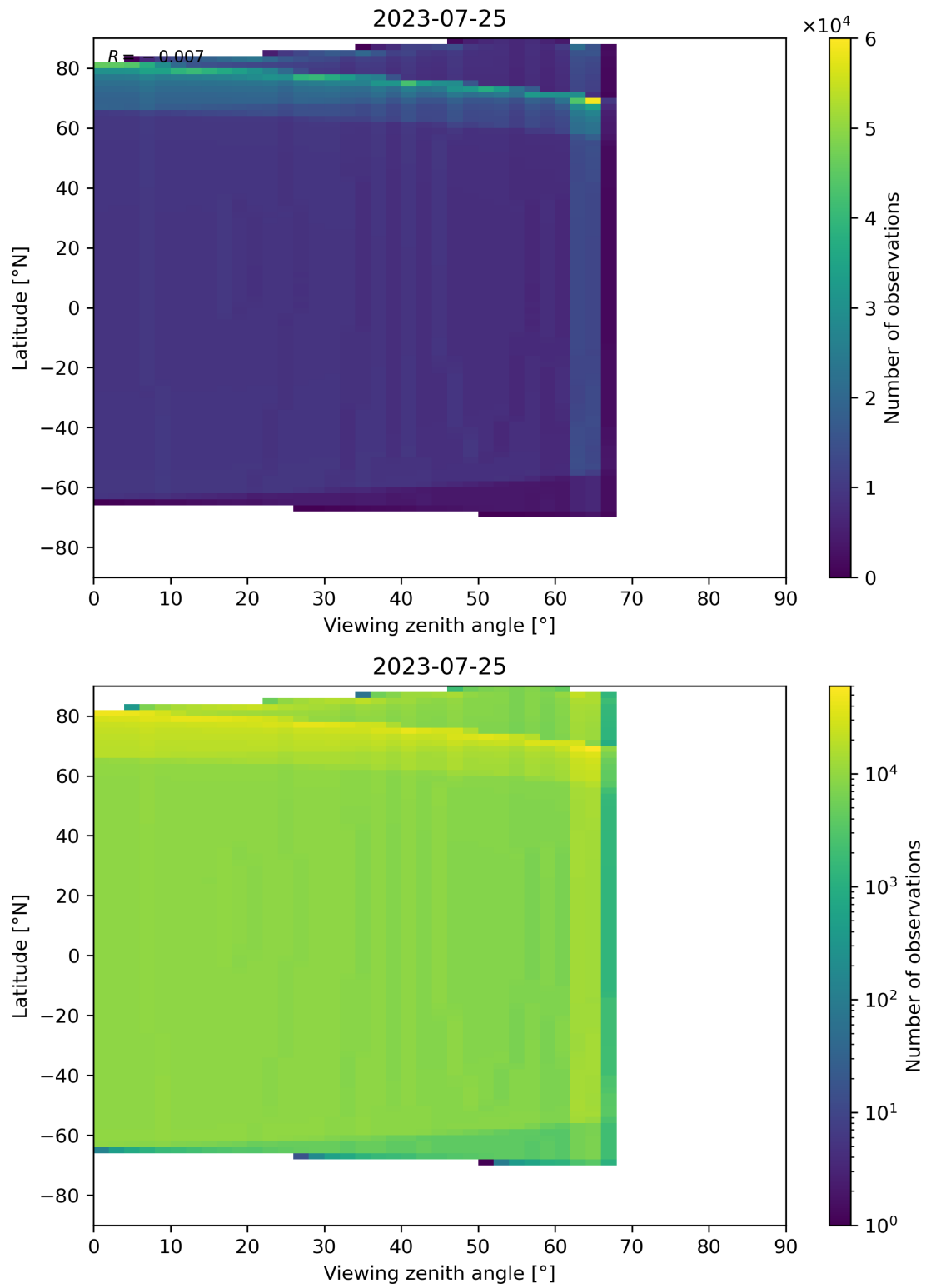
Figure 49: Scatter density plot of “Viewing zenith angle” against “Latitude” for 2023-07-24 to 2023-07-26.
