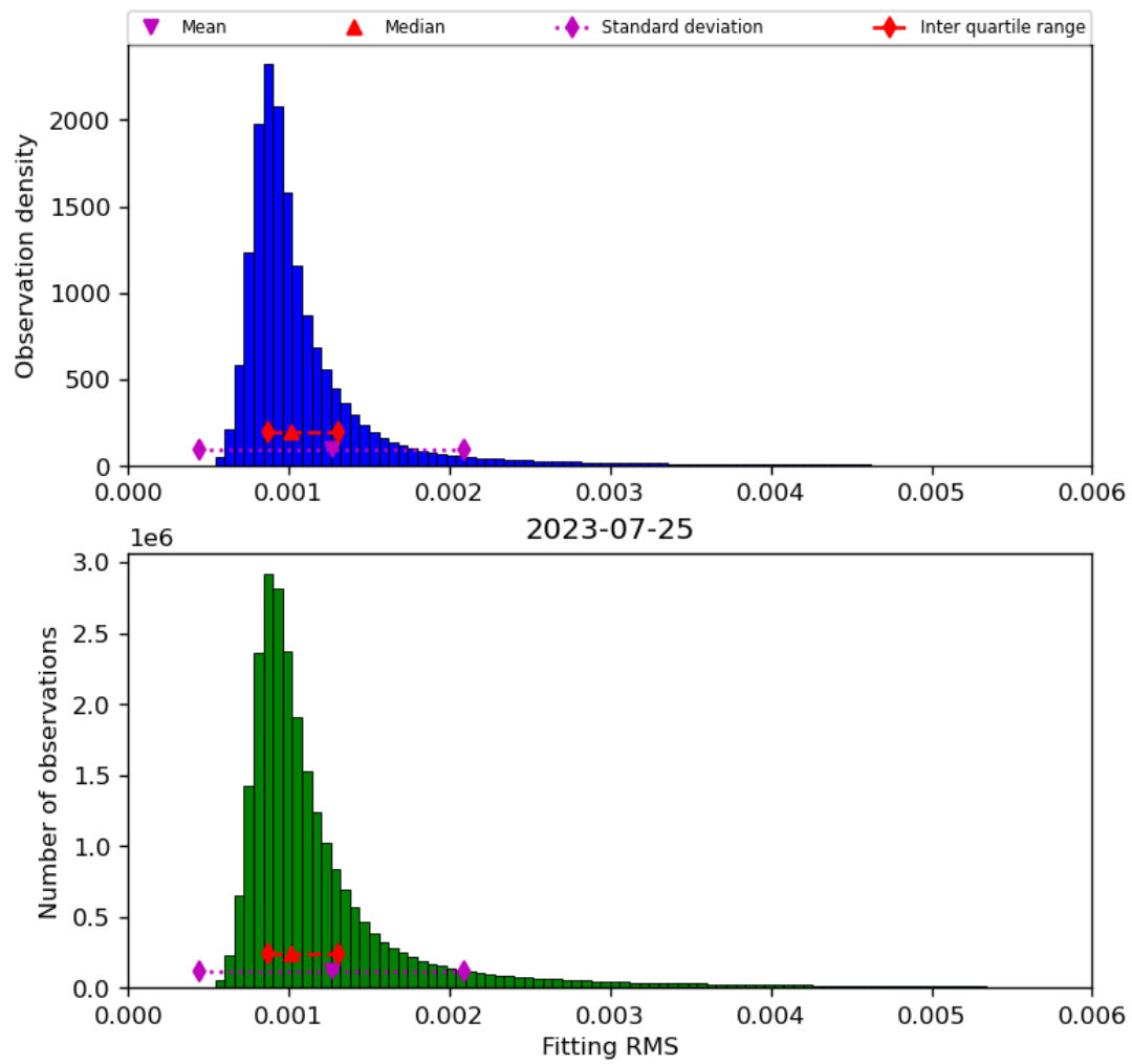
Figure 23: Histogram of “Fitting RMS” for 2023-07-24 to 2023-07-26
