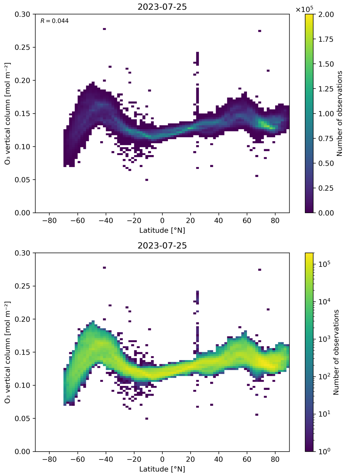
Figure 36: Scatter density plot of “Latitude” against “O 3 vertical column” for 2023-07-24 to 2023-07-26.
