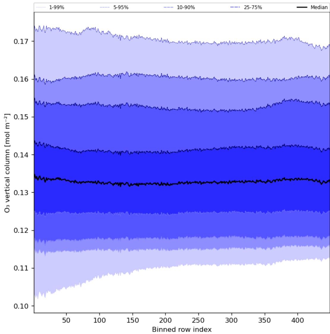
Figure 28: Along track statistics of “O 3 vertical column” for 2023-07-24 to 2023-07-26
