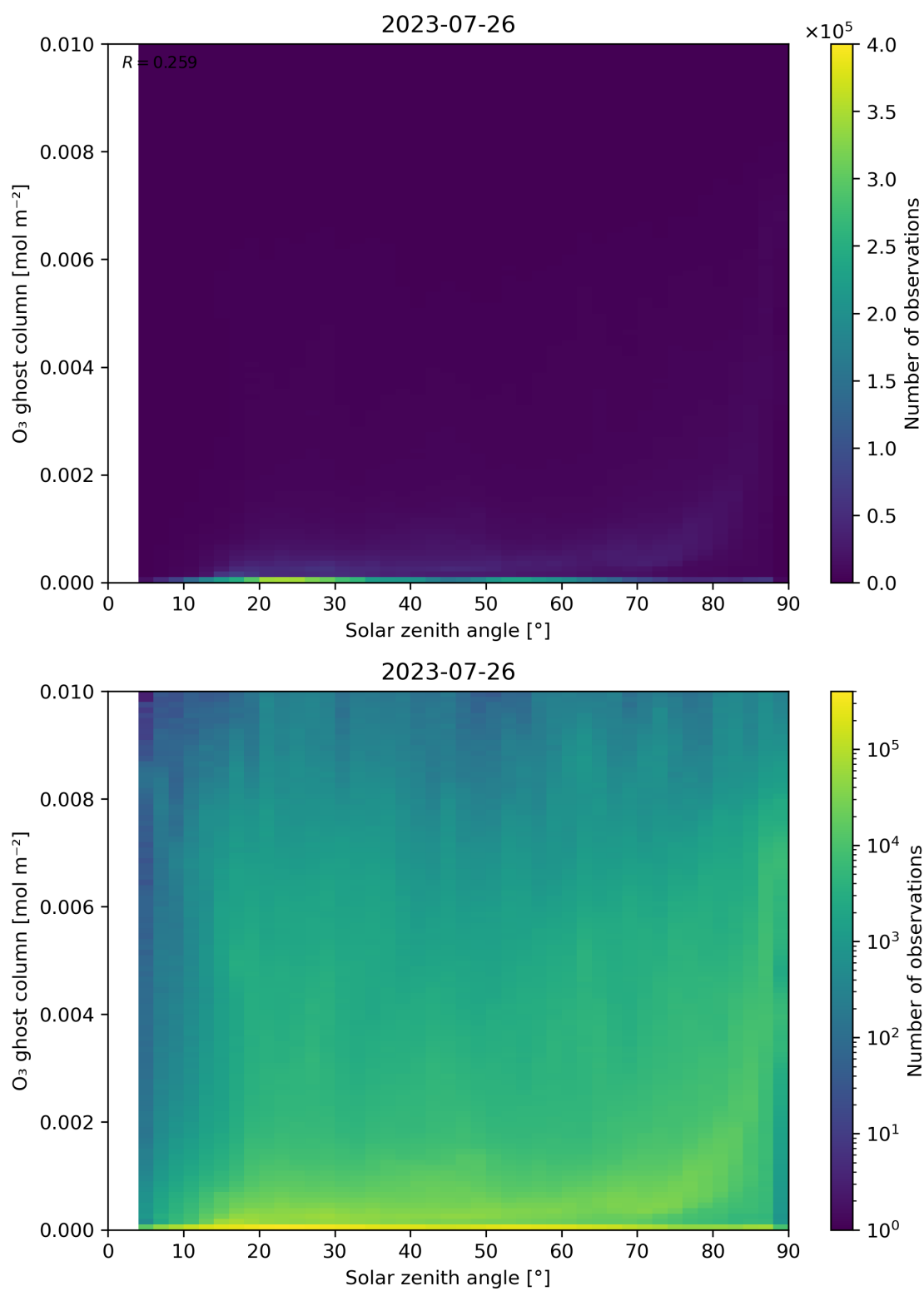
Figure 46: Scatter density plot of “Solar zenith angle” against “O 3 ghost column” for 2023-07-25 to 2023-07-27.
