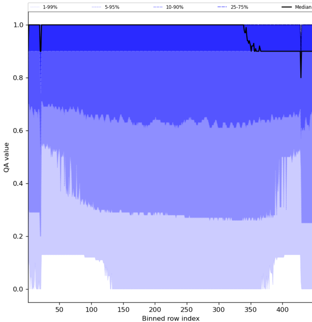
Figure 27: Along track statistics of “QA value” for 2023-07-25 to 2023-07-27
