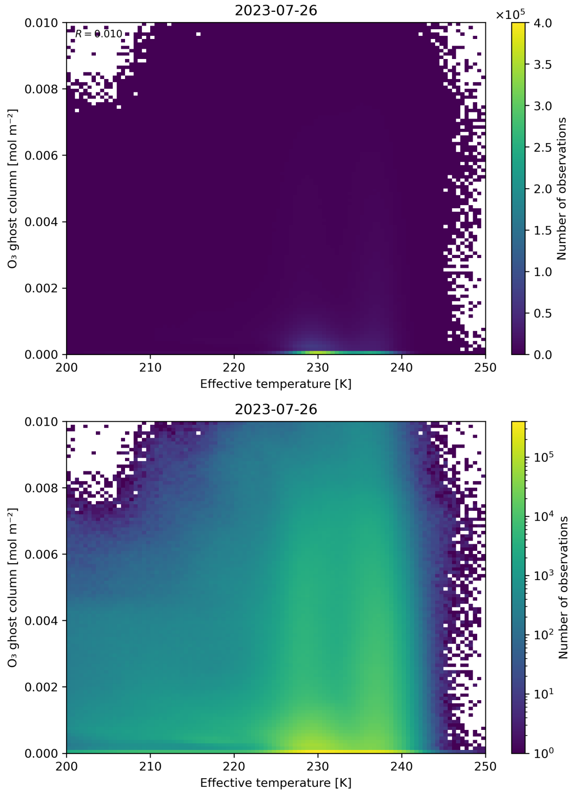
Figure 38: Scatter density plot of “Effective temperature” against “O 3 ghost column” for 2023-07-25 to 2023-07-27.
