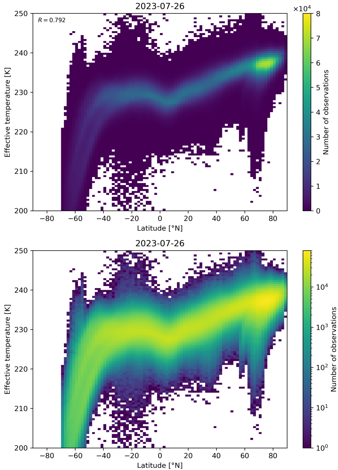
Figure 34: Scatter density plot of “Latitude” against “Effective temperature” for 2023-07-25 to 2023-07-27.
