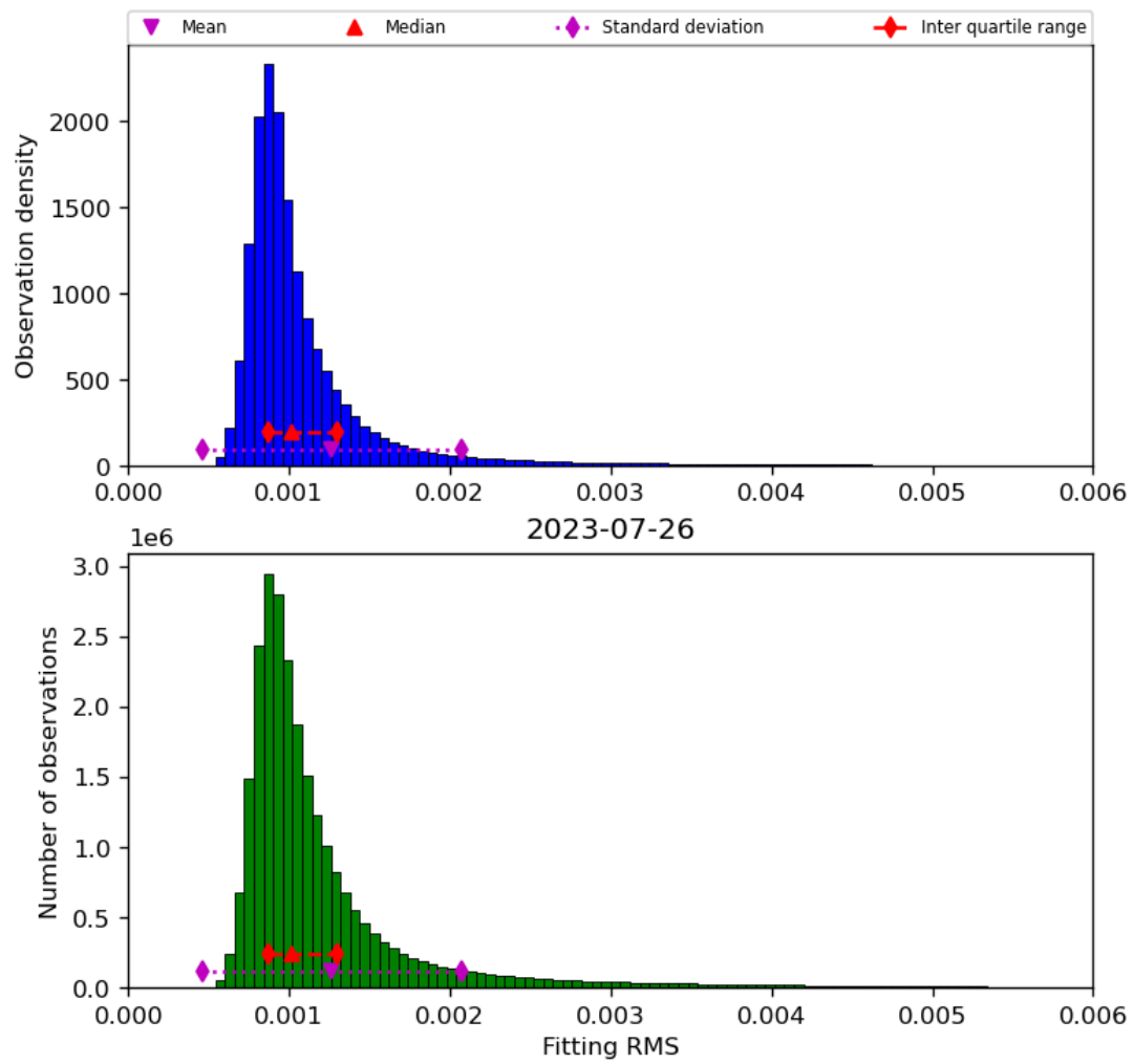
Figure 23: Histogram of “Fitting RMS” for 2023-07-25 to 2023-07-27
