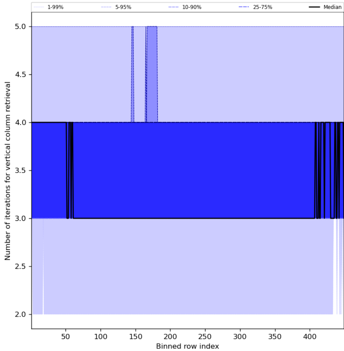
Figure 33: Along track statistics of “Number of iterations for vertical column retrieval” for 2023-07-25 to 2023-07-27
