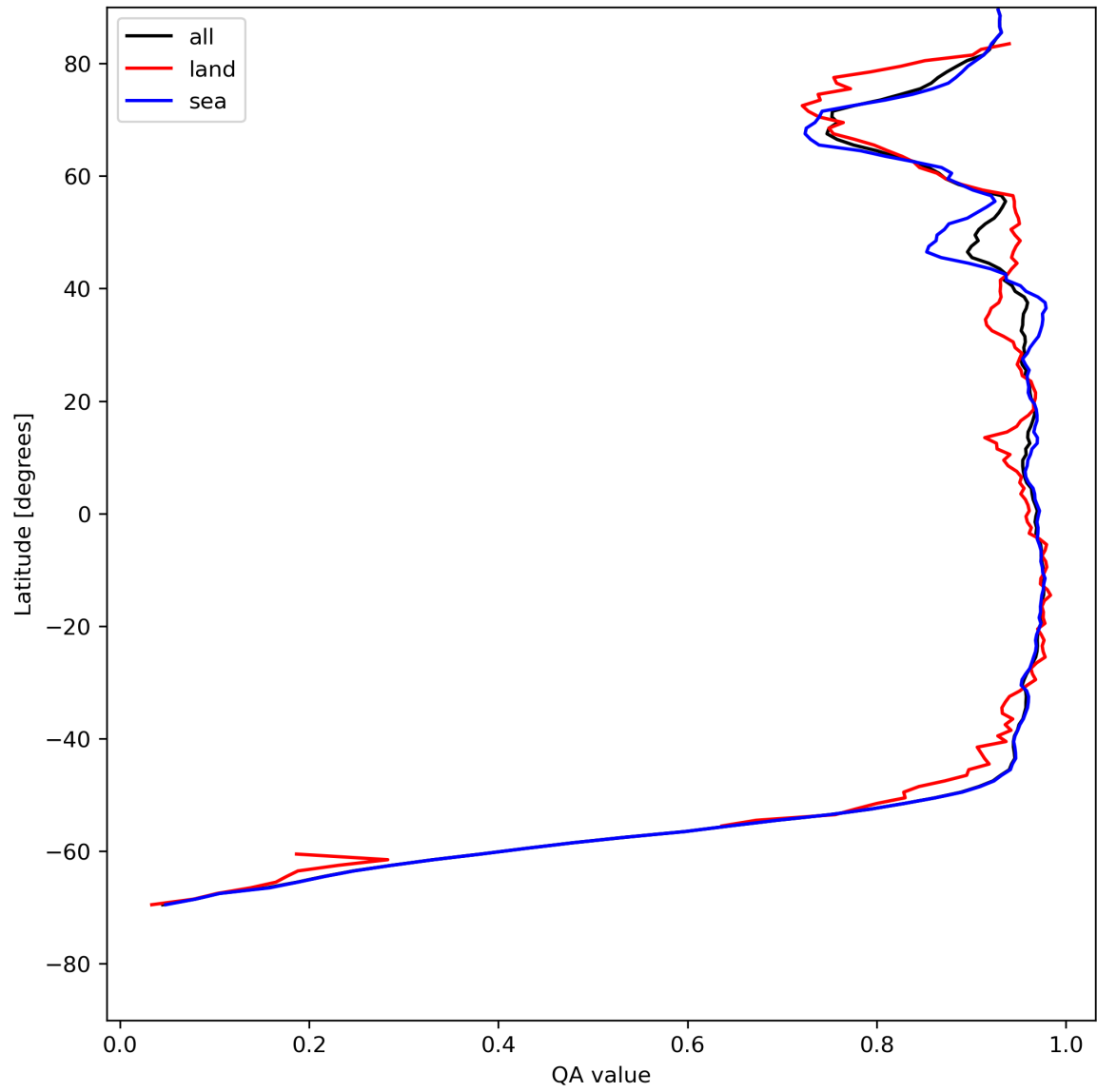
Figure 13: Zonal average of “QA value” for 2023-07-25 to 2023-07-27.
