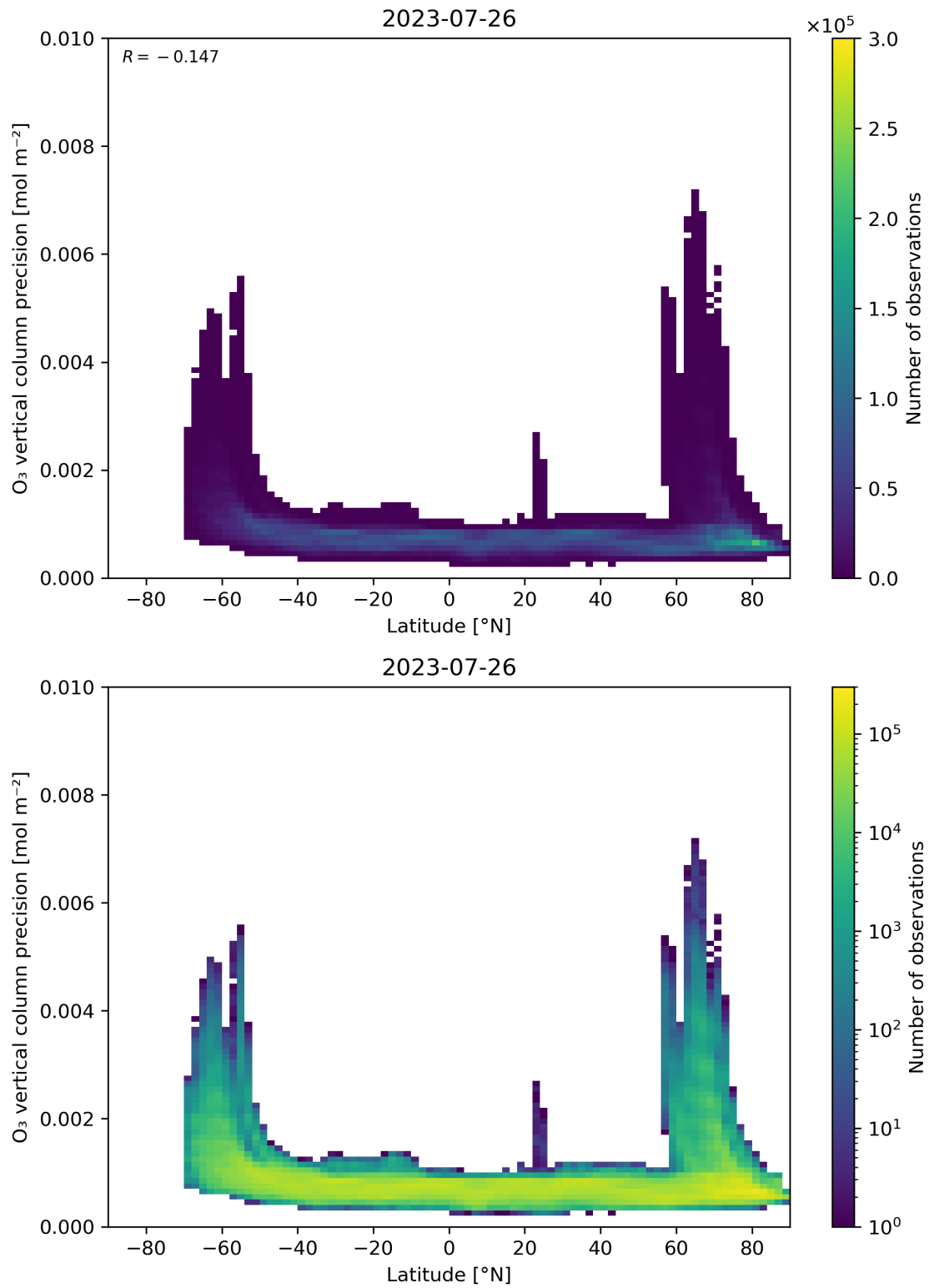
Figure 37: Scatter density plot of “Latitude” against “O 3 vertical column precision” for 2023-07-25 to 2023-07-27.
