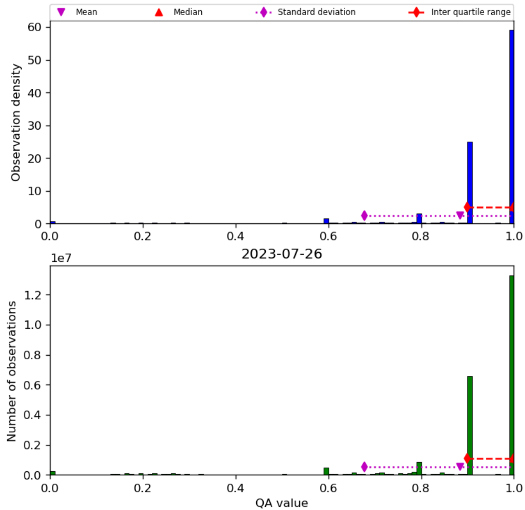
Figure 20: Histogram of “QA value” for 2023-07-25 to 2023-07-27
