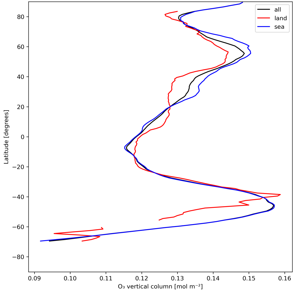
Figure 14: Zonal average of “O 3 vertical column” for 2023-07-25 to 2023-07-27.
