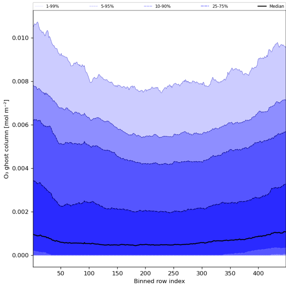
Figure 32: Along track statistics of “O 3 ghost column” for 2023-07-25 to 2023-07-27
