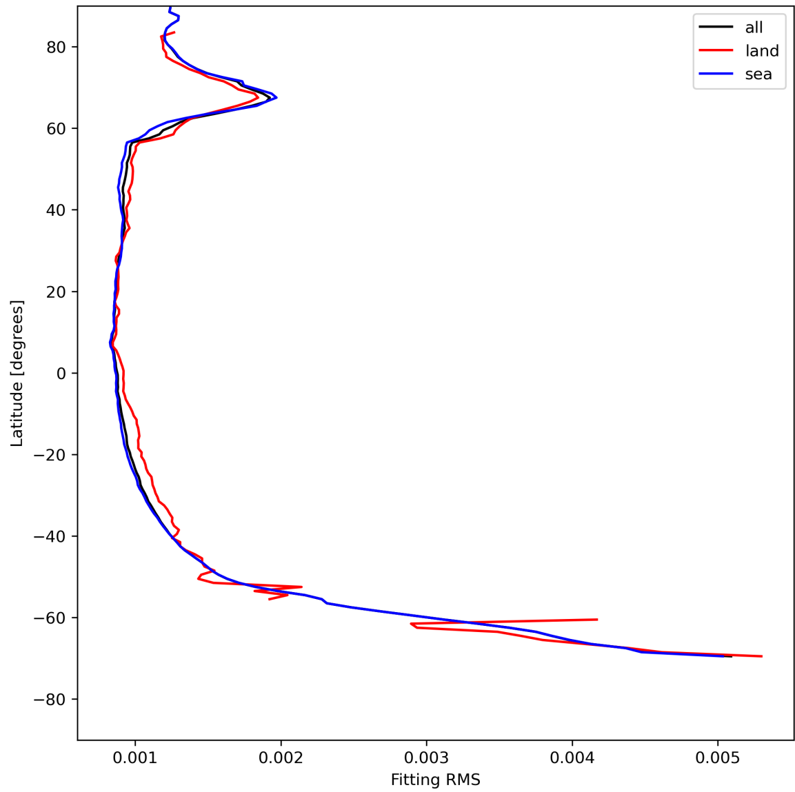
Figure 16: Zonal average of “Fitting RMS” for 2023-07-25 to 2023-07-27.
