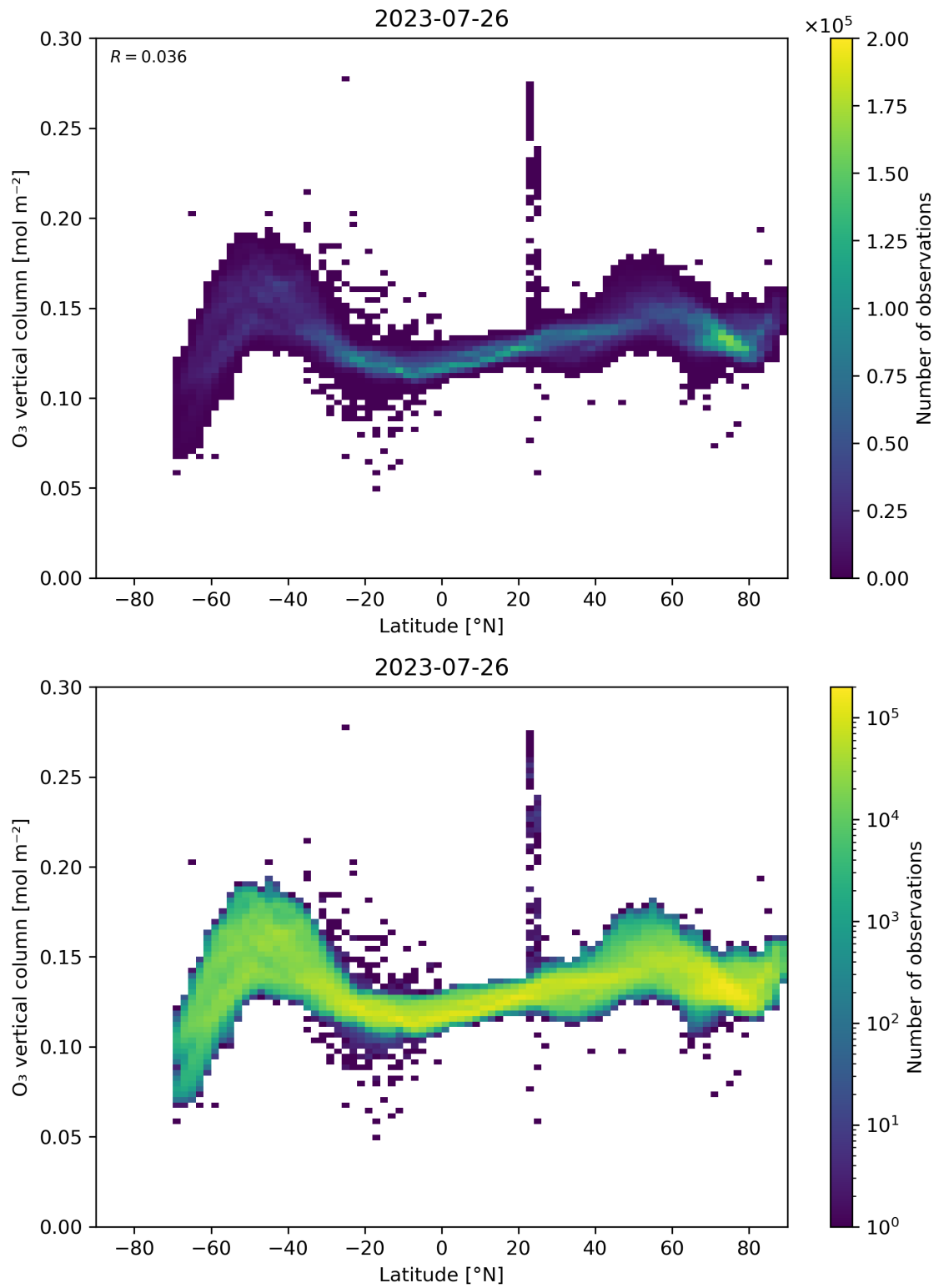
Figure 36: Scatter density plot of “Latitude” against “O 3 vertical column” for 2023-07-25 to 2023-07-27.
