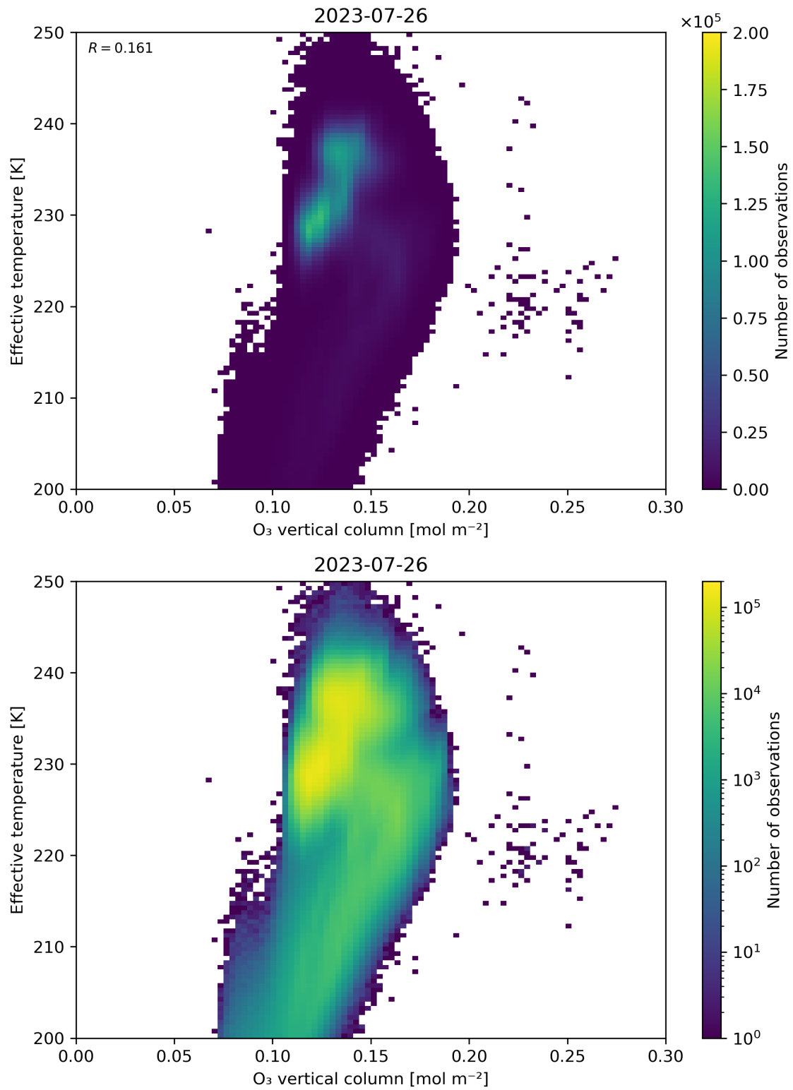
Figure 39: Scatter density plot of “O 3 vertical column” against “Effective temperature” for 2023-07-25 to 2023-07-27.
