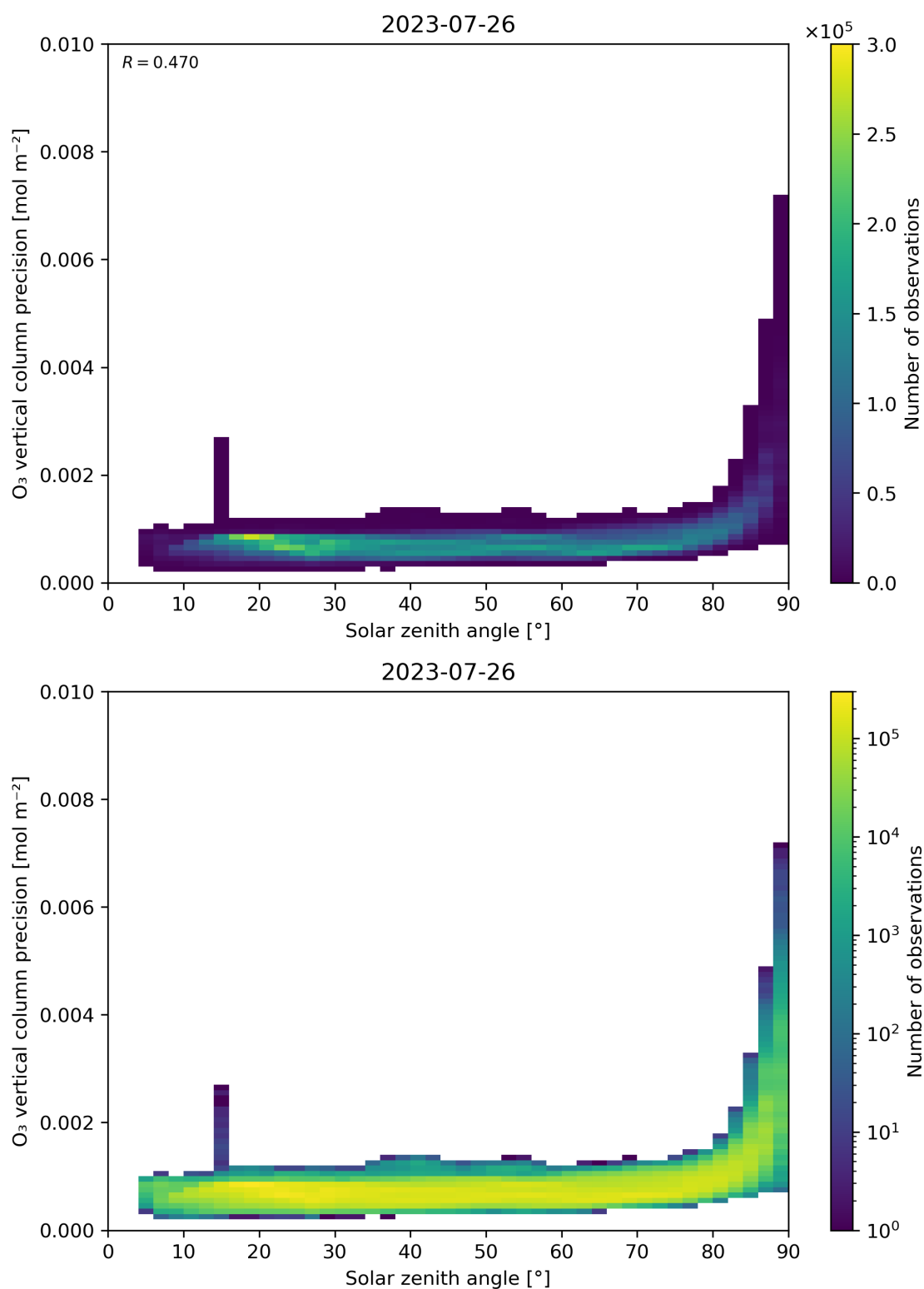
Figure 48: Scatter density plot of “Solar zenith angle” against “O 3 vertical column precision” for 2023-07-25 to 2023-07-27.
