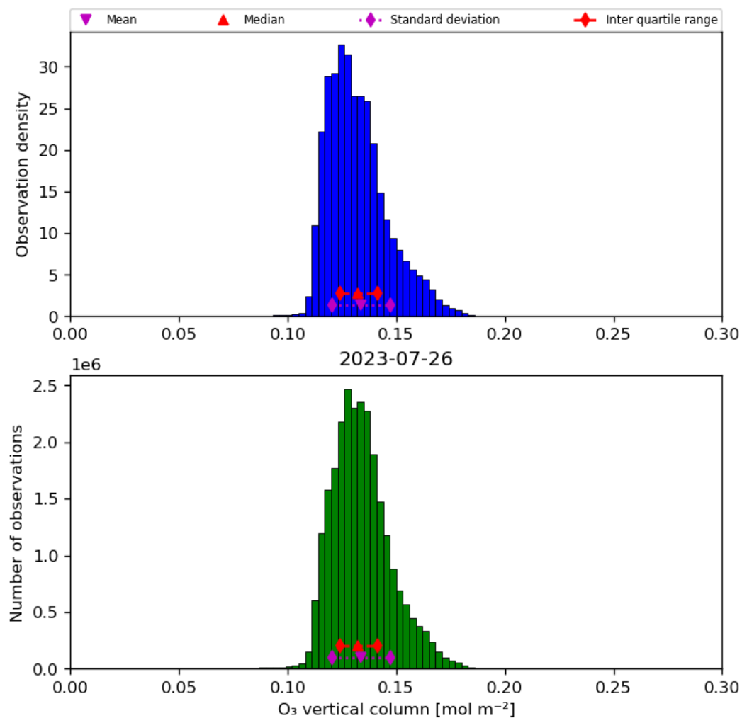
Figure 21: Histogram of “O 3 vertical column” for 2023-07-25 to 2023-07-27
