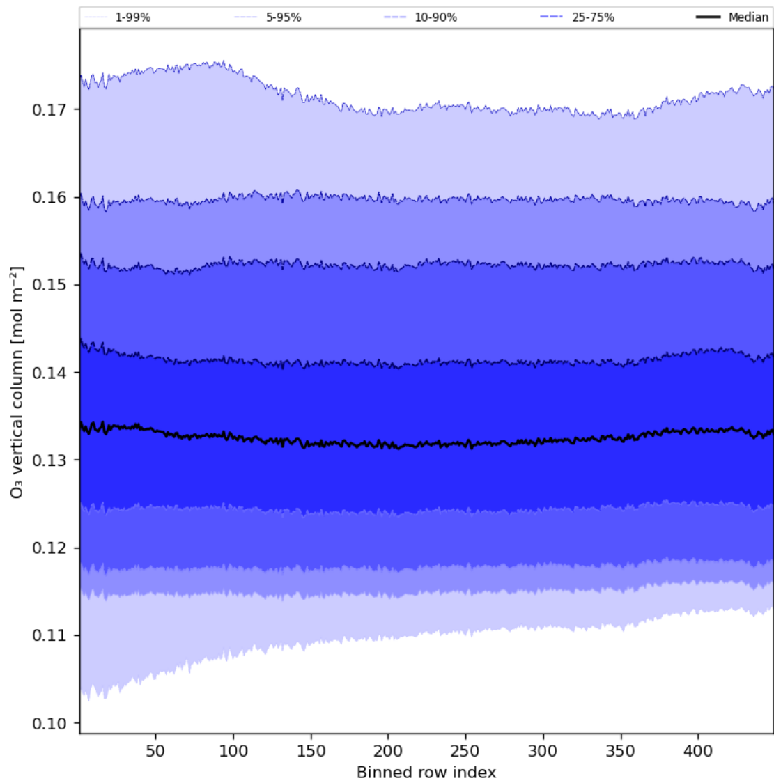
Figure 28: Along track statistics of “O 3 vertical column” for 2023-07-25 to 2023-07-27
