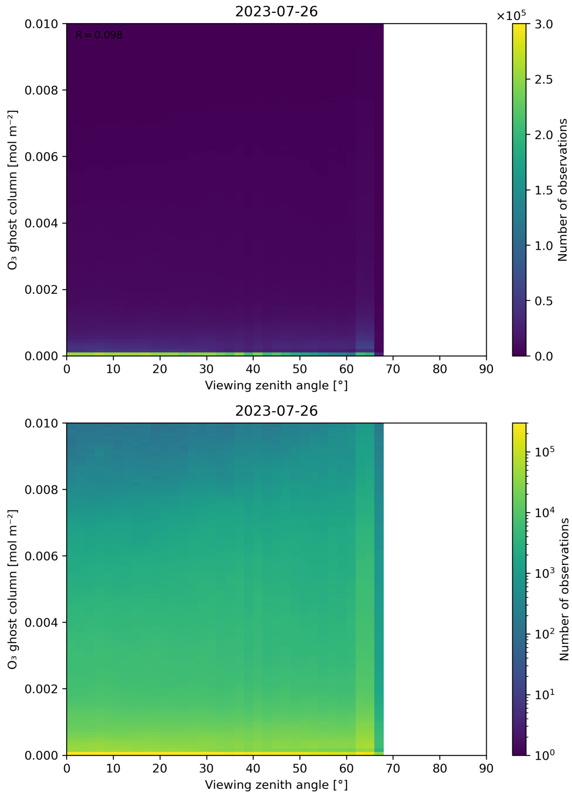
Figure 51: Scatter density plot of “Viewing zenith angle” against “O 3 ghost column” for 2023-07-25 to 2023-07-27.
