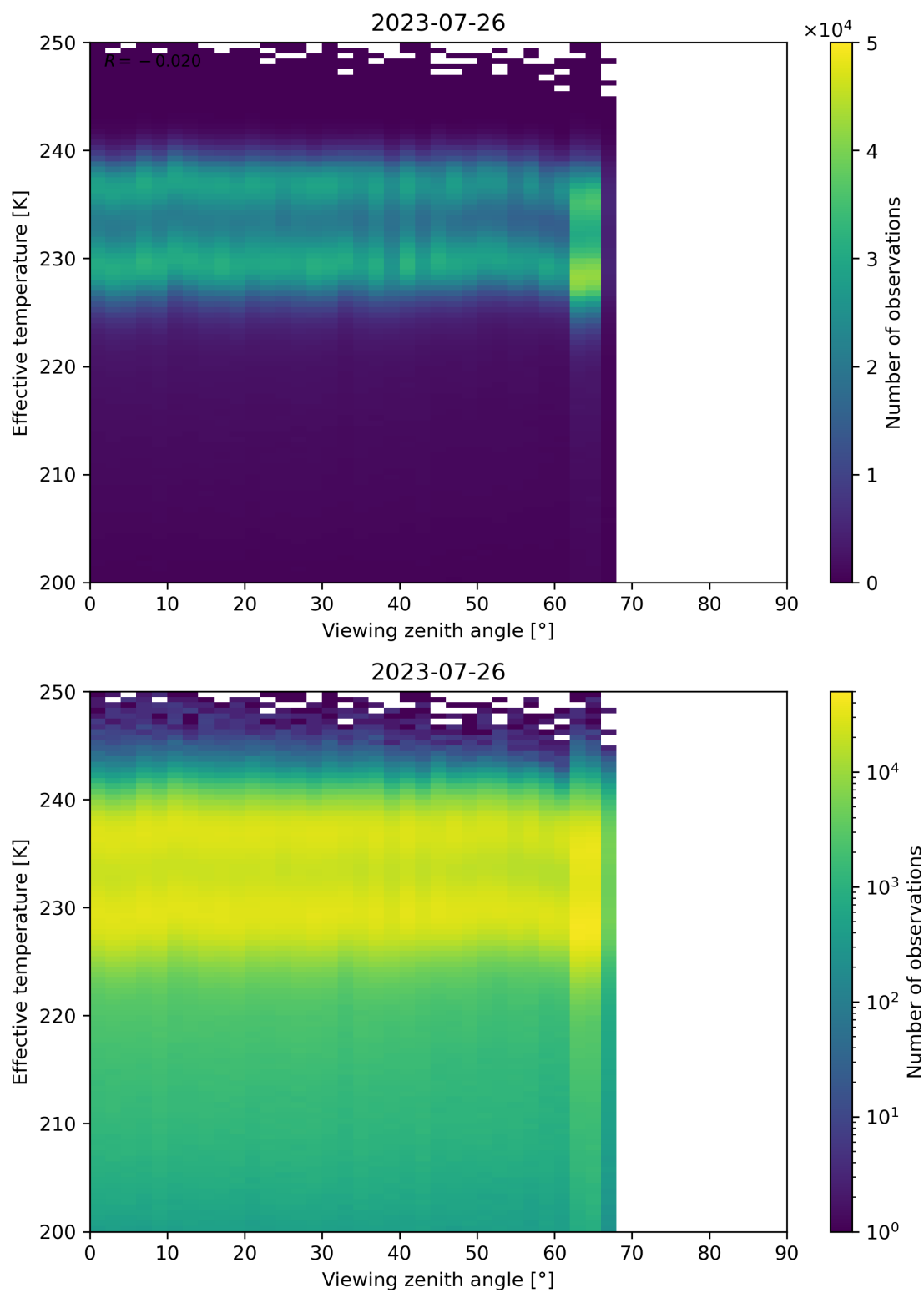
Figure 50: Scatter density plot of “Viewing zenith angle” against “Effective temperature” for 2023-07-25 to 2023-07-27.
