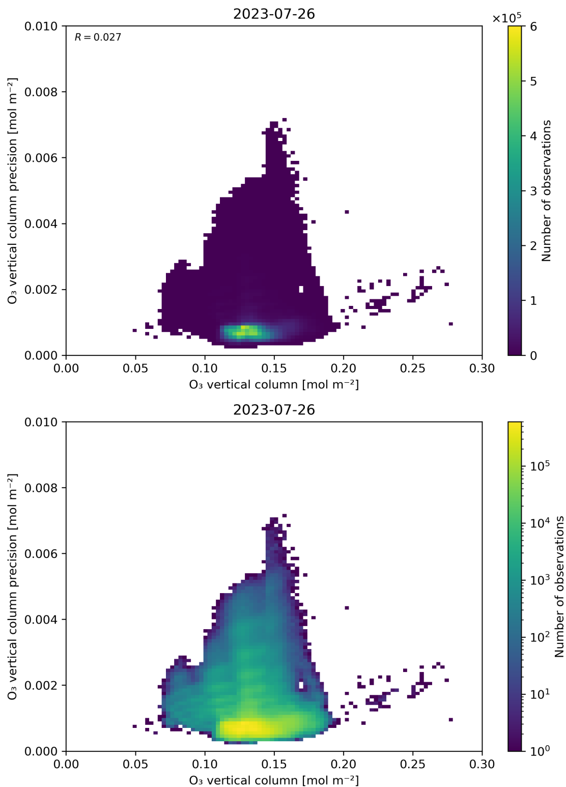
Figure 41: Scatter density plot of “O 3 vertical column” against “O 3 vertical column precision” for 2023-07-25 to 2023-07-27.
