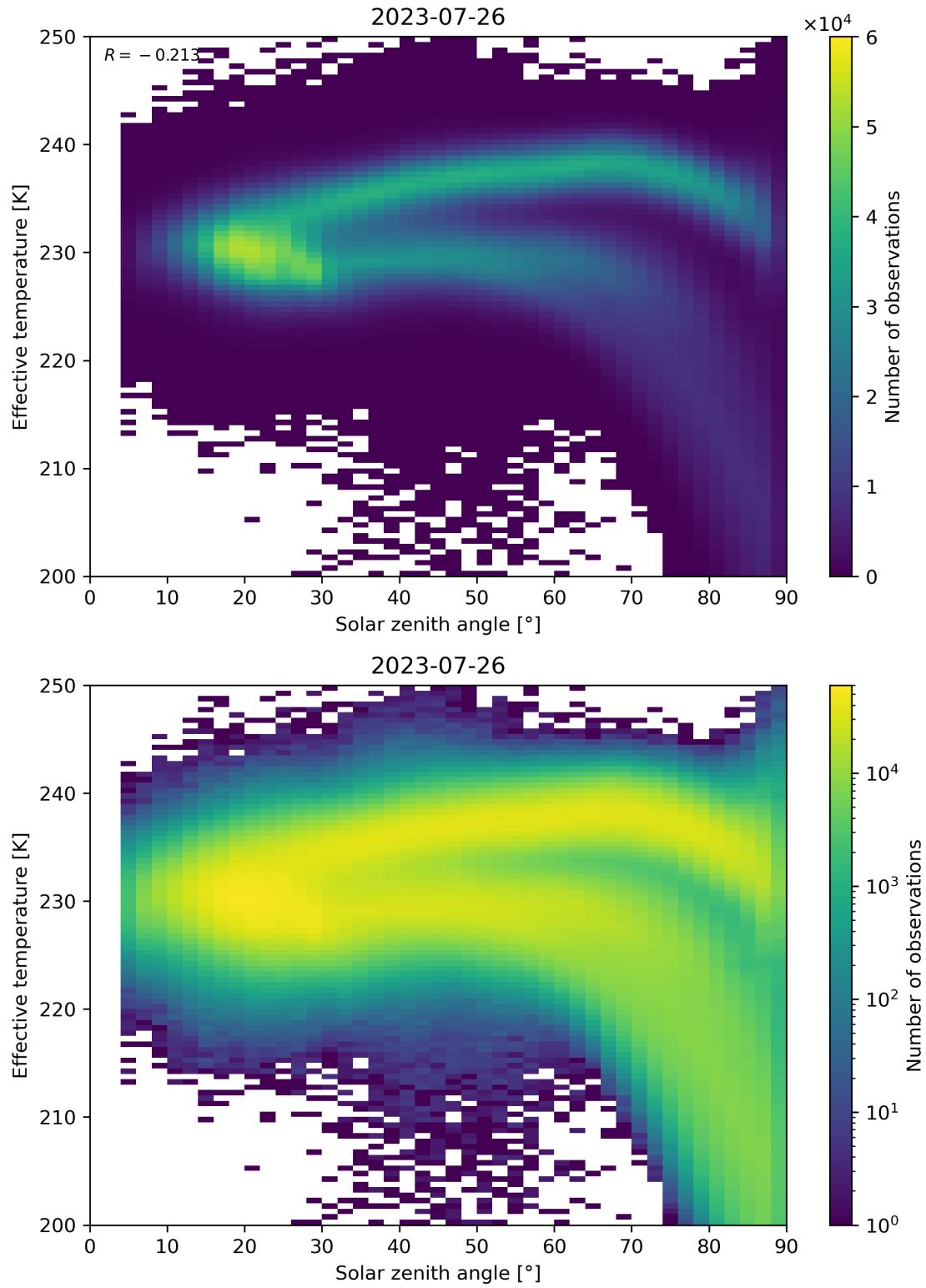
Figure 45: Scatter density plot of “Solar zenith angle” against “Effective temperature” for 2023-07-25 to 2023-07-27.
