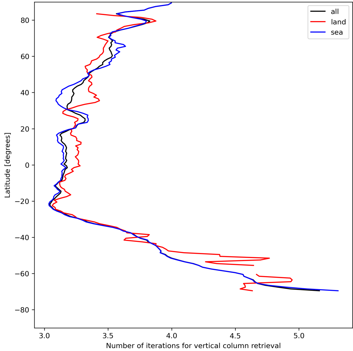
Figure 19: Zonal average of “Number of iterations for vertical column retrieval” for 2023-07-25 to 2023-07-27.
