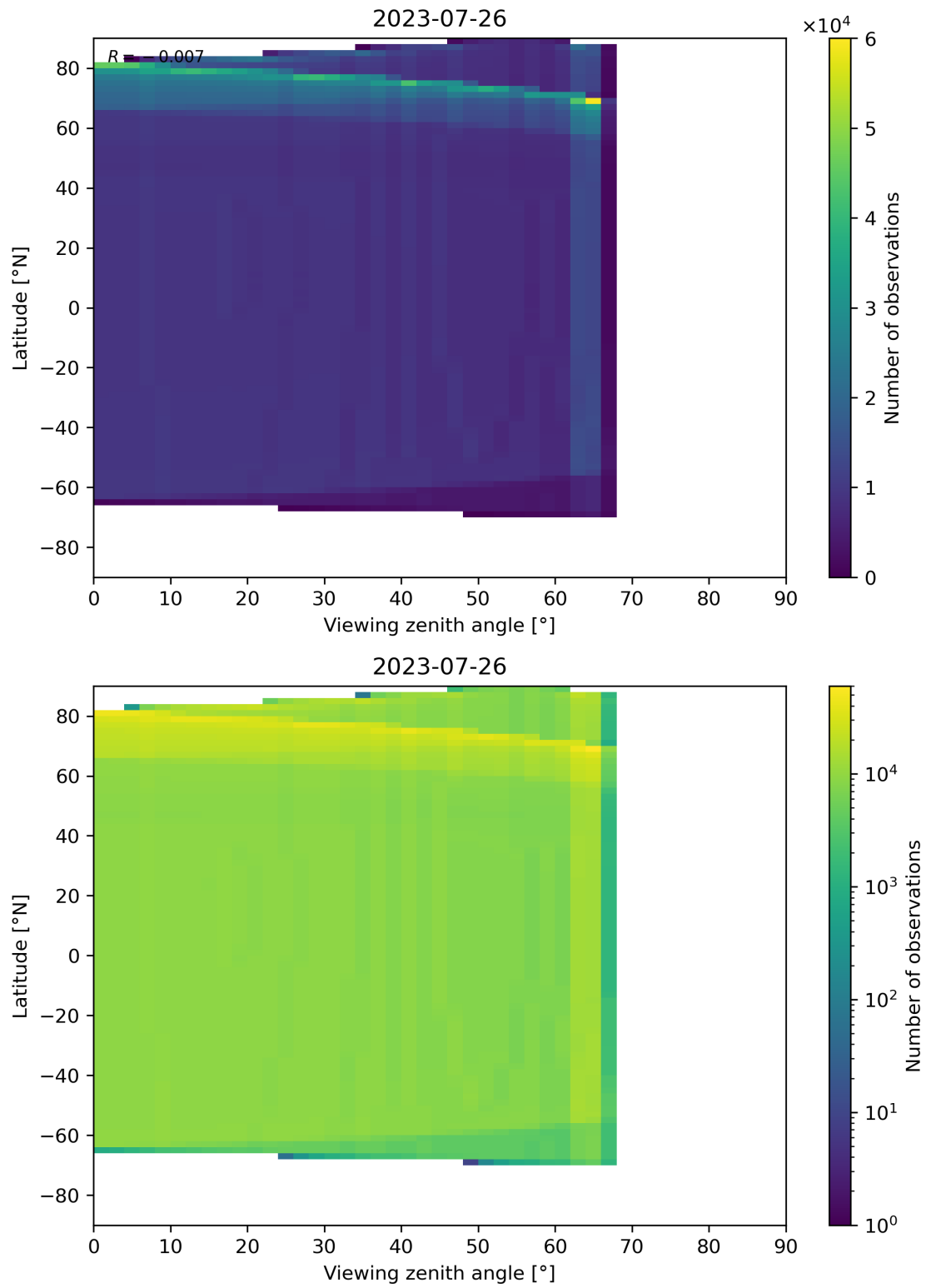
Figure 49: Scatter density plot of “Viewing zenith angle” against “Latitude” for 2023-07-25 to 2023-07-27.
