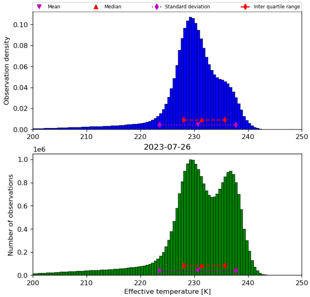
Figure 24: Histogram of “Effective temperature” for 2023-07-25 to 2023-07-27
