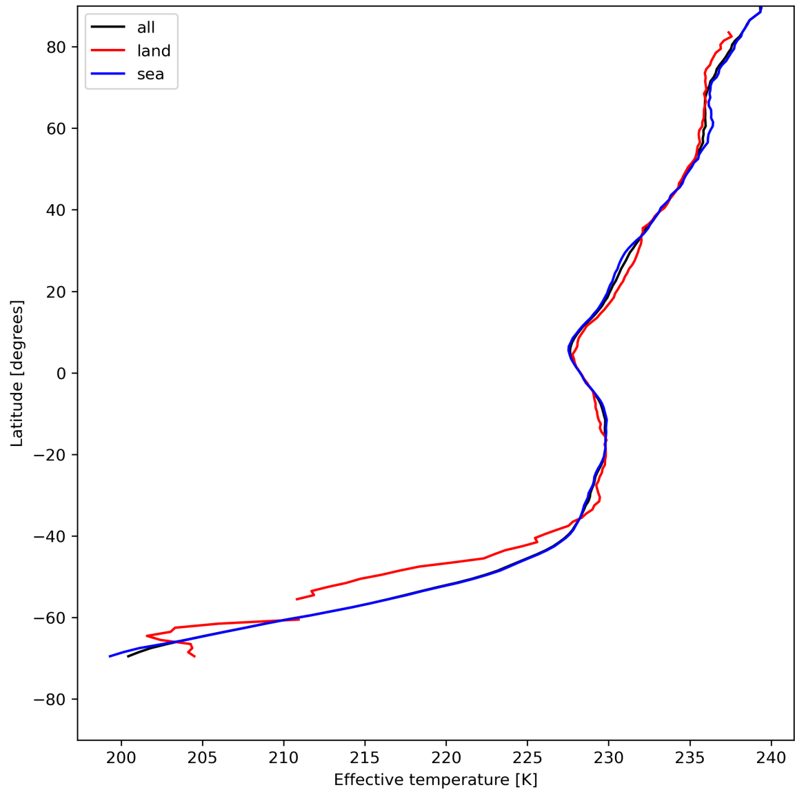
Figure 17: Zonal average of "Effective temperature" for 2023-07-25 to 2023-07-27.
