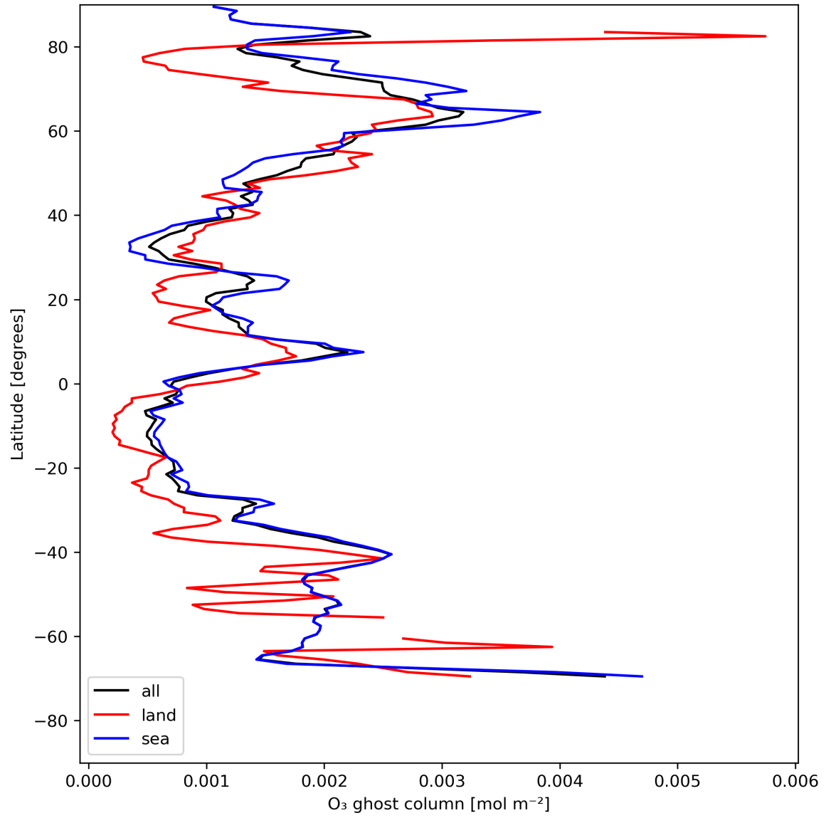
Figure 18: Zonal average of “O 3 ghost column” for 2023-07-25 to 2023-07-27.
