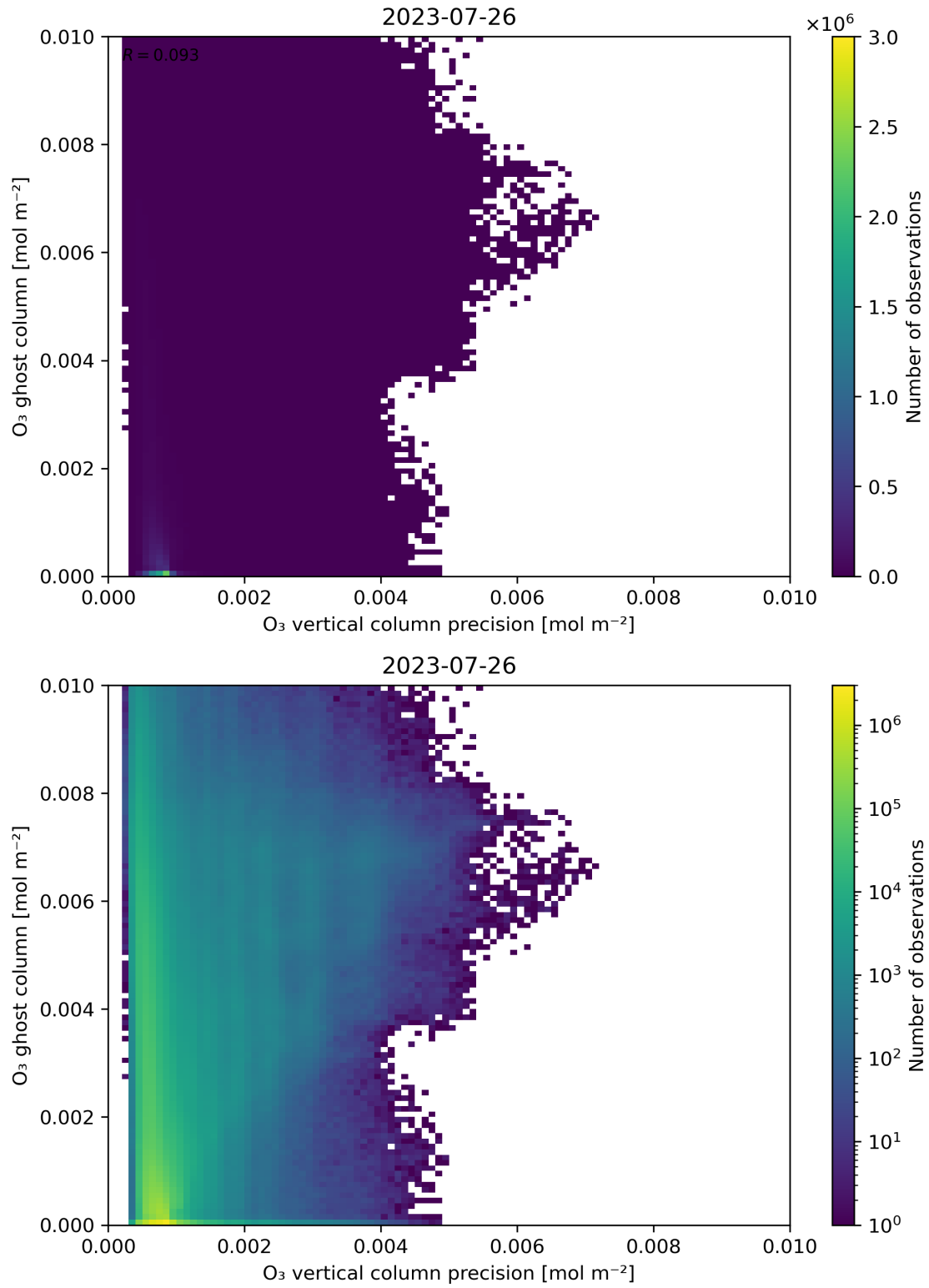
Figure 43: Scatter density plot of “O 3 vertical column precision” against “O 3 ghost column” for 2023-07-25 to 2023-07-27.
