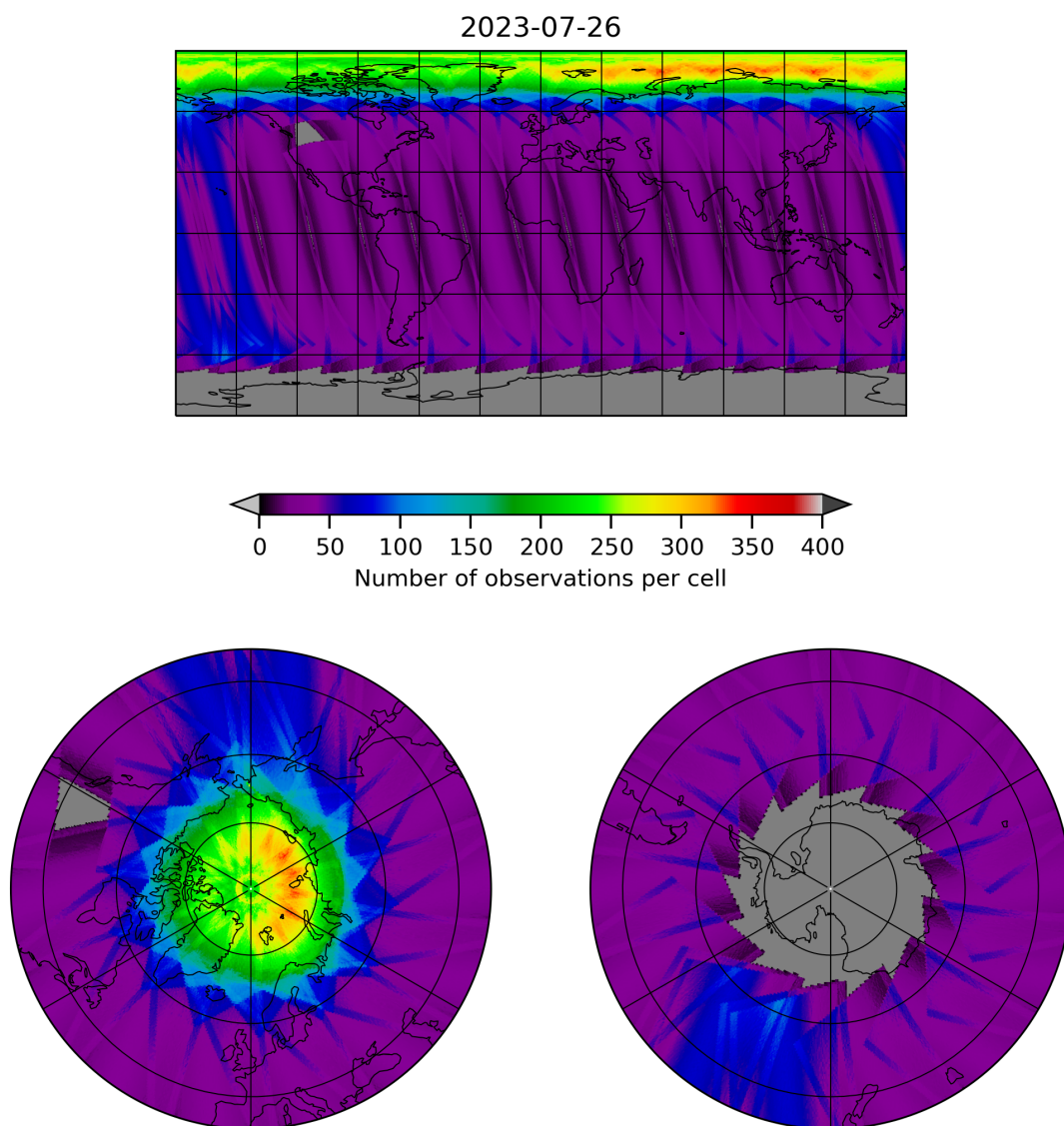
Figure 12: Map of the number of observations for 2023-07-25 to 2023-07-27
