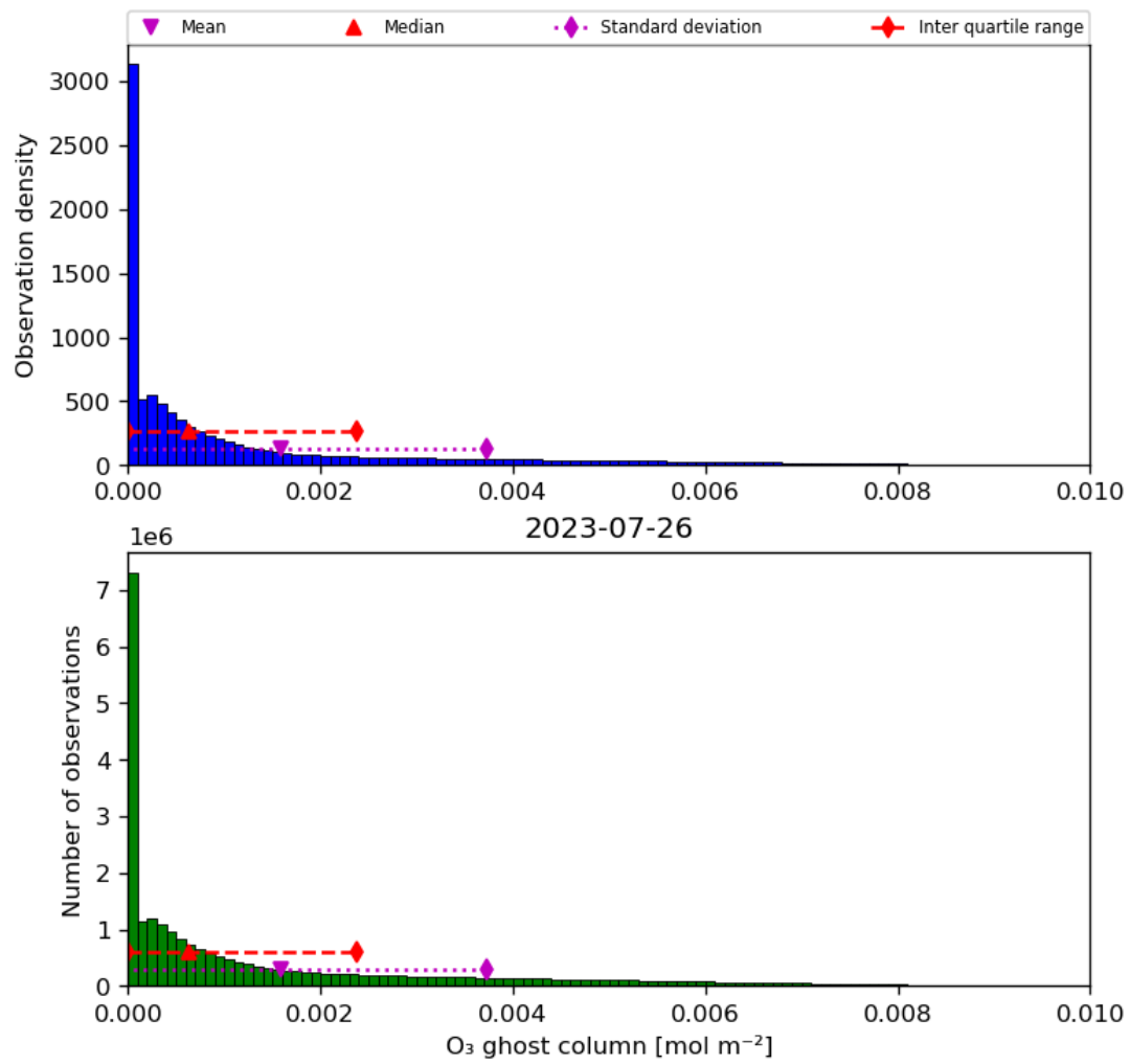
Figure 25: Histogram of "O 3 ghost column" for 2023-07-25 to 2023-07-27
