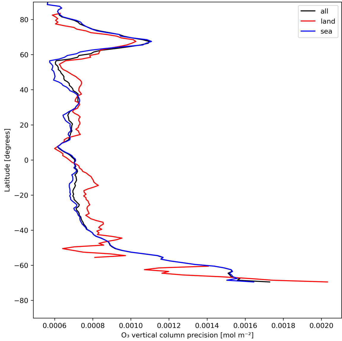
Figure 15: Zonal average of “O 3 vertical column precision” for 2023-07-25 to 2023-07-27.
