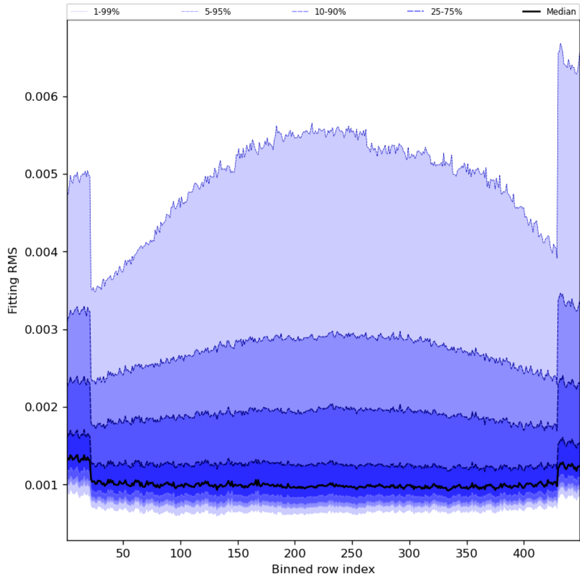
Figure 30: Along track statistics of “Fitting RMS” for 2023-07-25 to 2023-07-27
