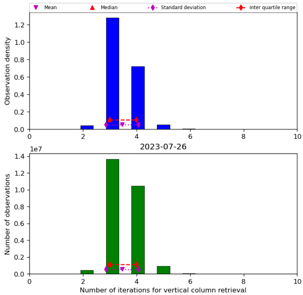
Figure 26: Histogram of “Number of iterations for vertical column retrieval” for 2023-07-25 to 2023-07-27
