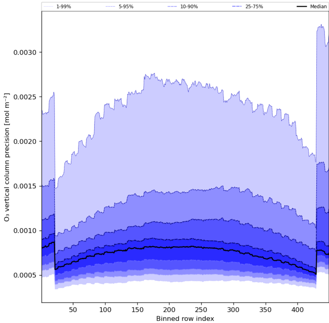
Figure 29: Along track statistics of “O 3 vertical column precision” for 2023-07-25 to 2023-07-27
