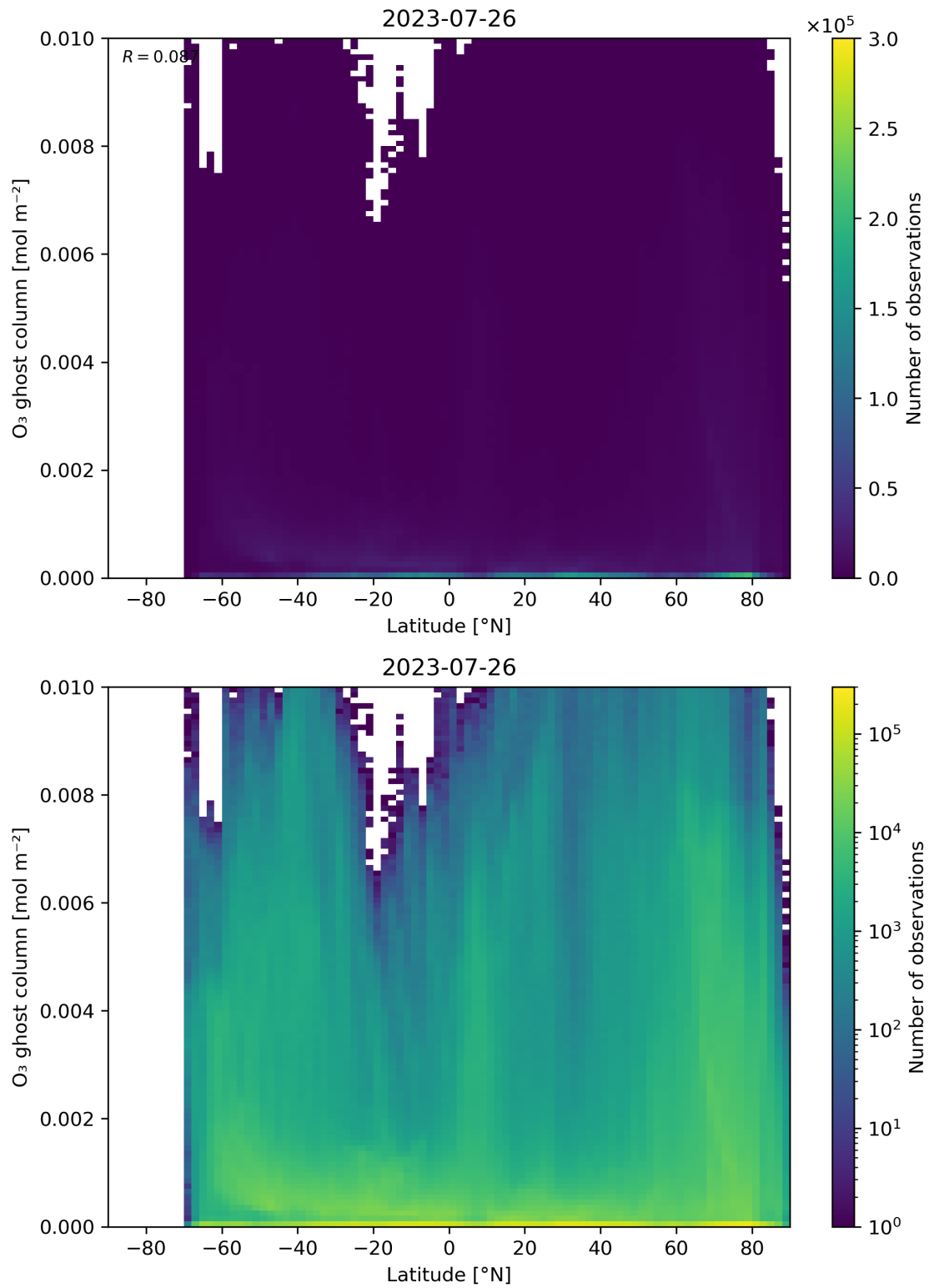
Figure 35: Scatter density plot of “Latitude” against “O 3 ghost column” for 2023-07-25 to 2023-07-27.
