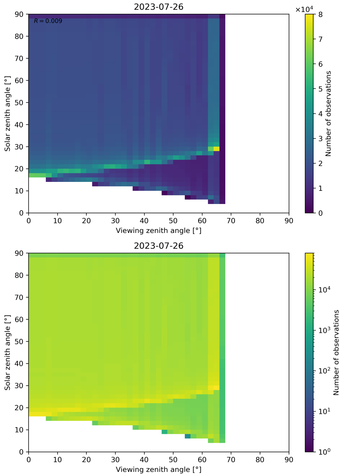
Figure 54: Scatter density plot of “Viewing zenith angle” against “Solar zenith angle” for 2023-07-25 to 2023-07-27.
