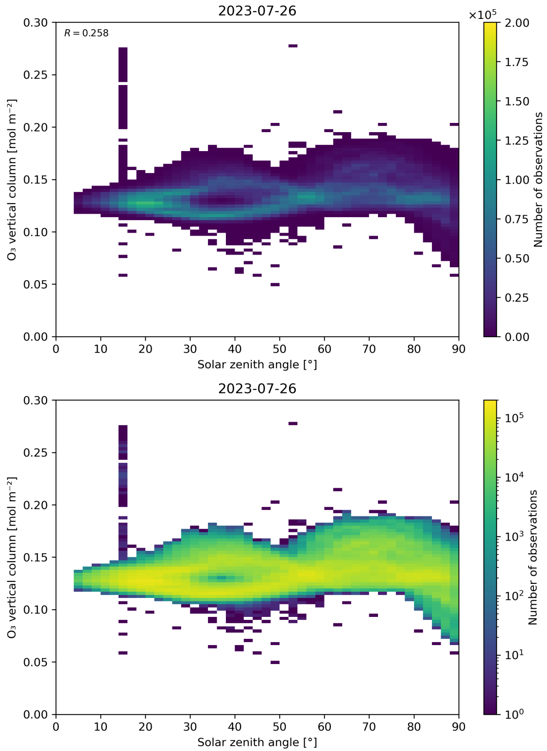
Figure 47: Scatter density plot of “Solar zenith angle” against “O 3 vertical column” for 2023-07-25 to 2023-07-27.
