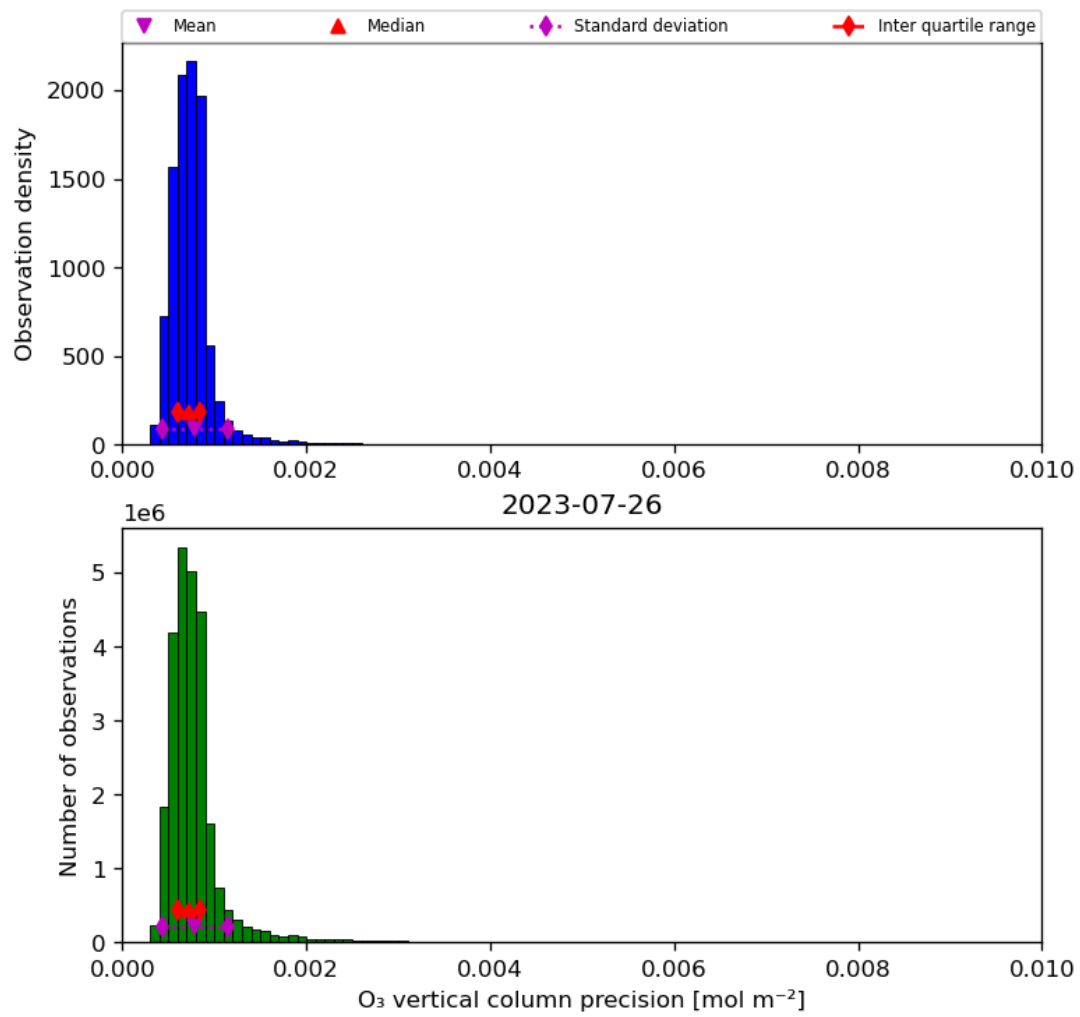
Figure 22: Histogram of “O 3 vertical column precision” for 2023-07-25 to 2023-07-27
