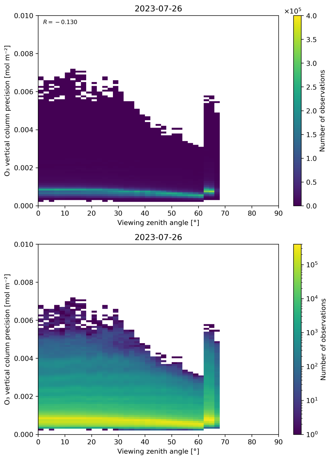
Figure 53: Scatter density plot of “Viewing zenith angle” against “O 3 vertical column precision” for 2023-07-25 to 2023-07-27.
