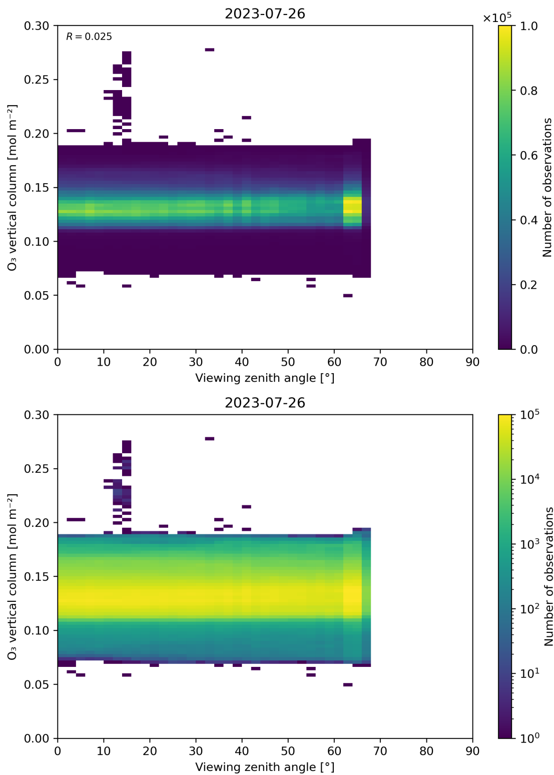
Figure 52: Scatter density plot of “Viewing zenith angle” against “O 3 vertical column” for 2023-07-25 to 2023-07-27.
