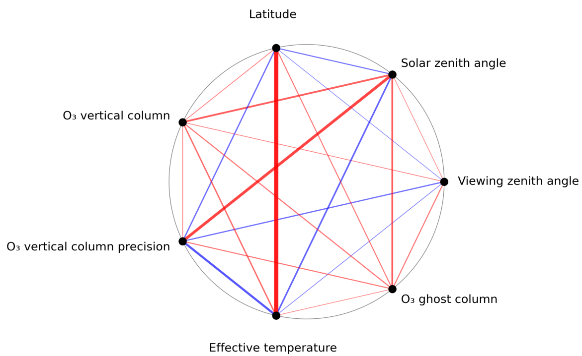
Figure 1: Map of correlation graph for 2023-07-25 to 2023-07-27.
