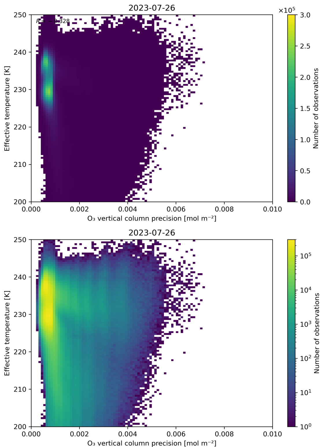
Figure 42: Scatter density plot of “O 3 vertical column precision” against “Effective temperature” for 2023-07-25 to 2023-07-27.
