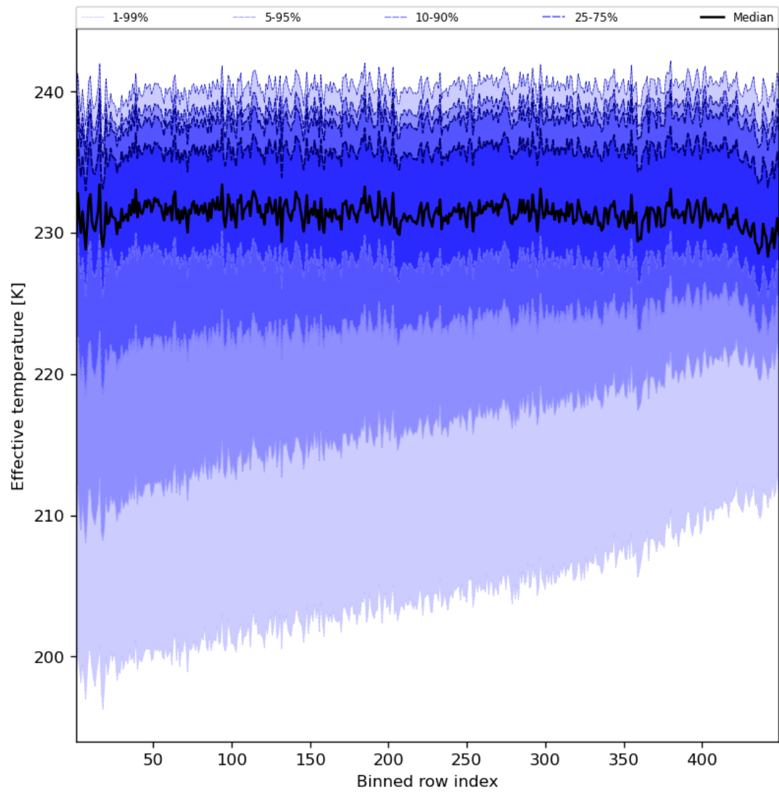
Figure 31: Along track statistics of “Effective temperature” for 2023-07-25 to 2023-07-27
