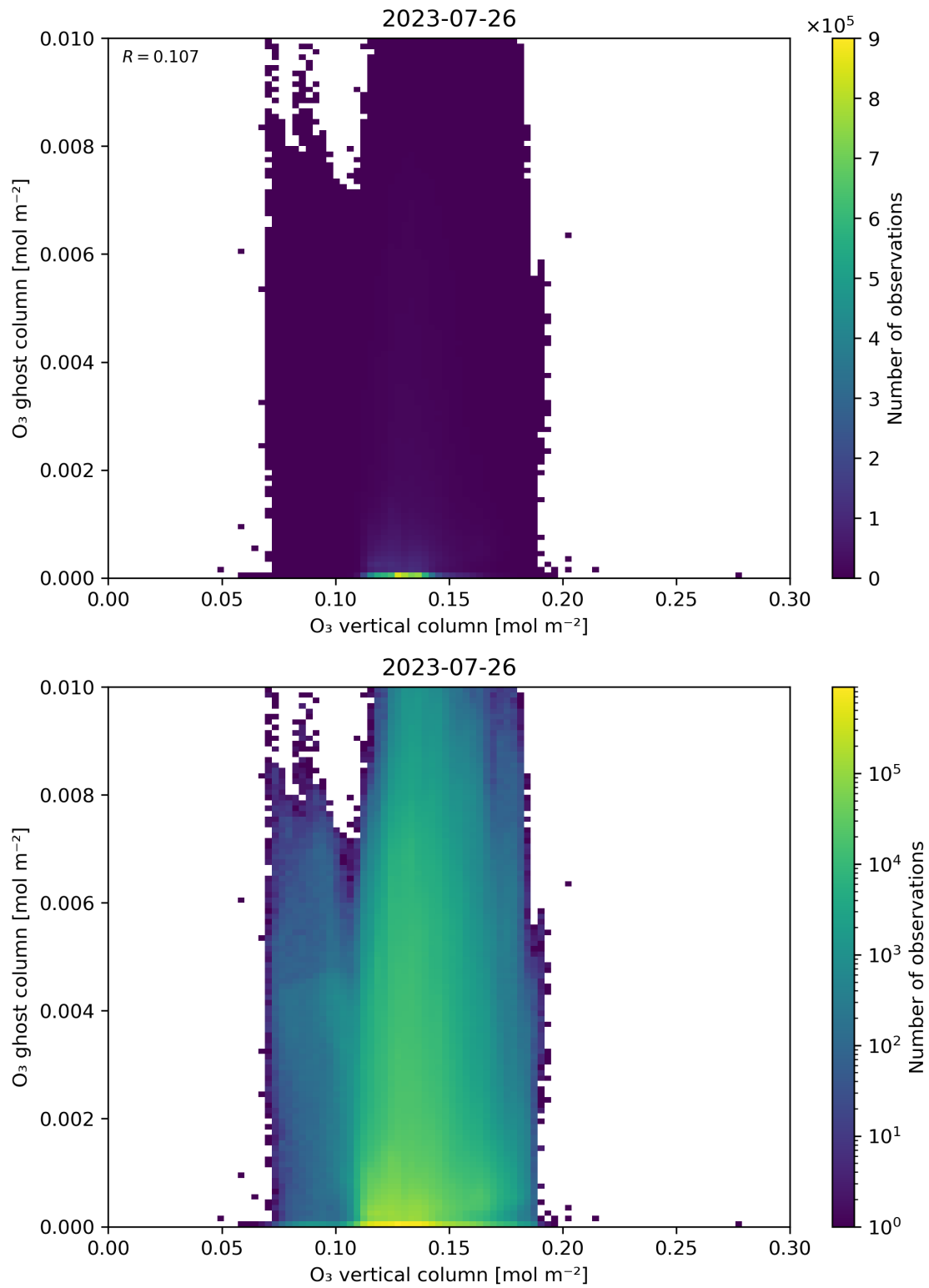
Figure 40: Scatter density plot of “O 3 vertical column” against “O 3 ghost column” for 2023-07-25 to 2023-07-27.
