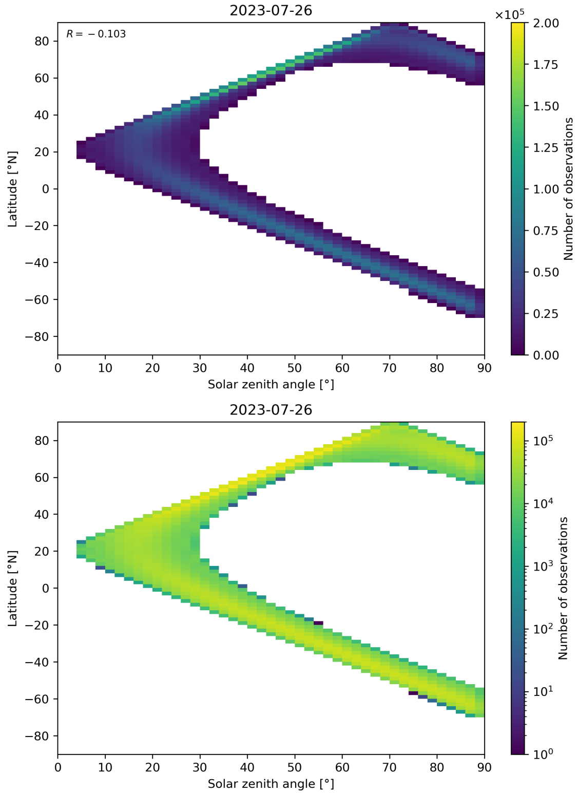
Figure 44: Scatter density plot of “Solar zenith angle” against “Latitude” for 2023-07-25 to 2023-07-27.
