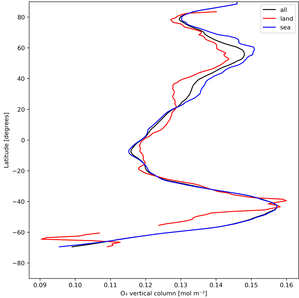
Figure 14: Zonal average of “O 3 vertical column” for 2023-07-26 to 2023-07-28.
