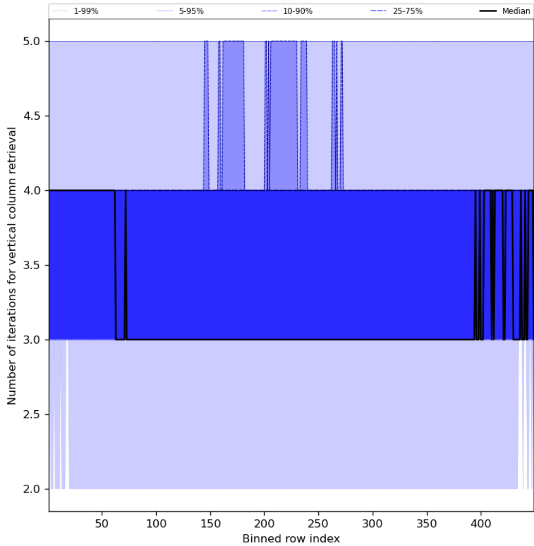
Figure 33: Along track statistics of “Number of iterations for vertical column retrieval” for 2023-07-26 to 2023-07-28
