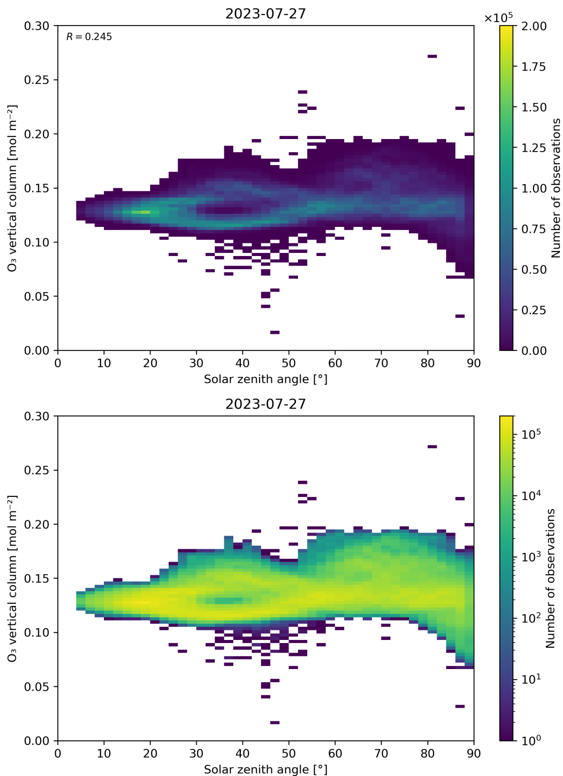
Figure 47: Scatter density plot of “Solar zenith angle” against “O 3 vertical column” for 2023-07-26 to 2023-07-28.
