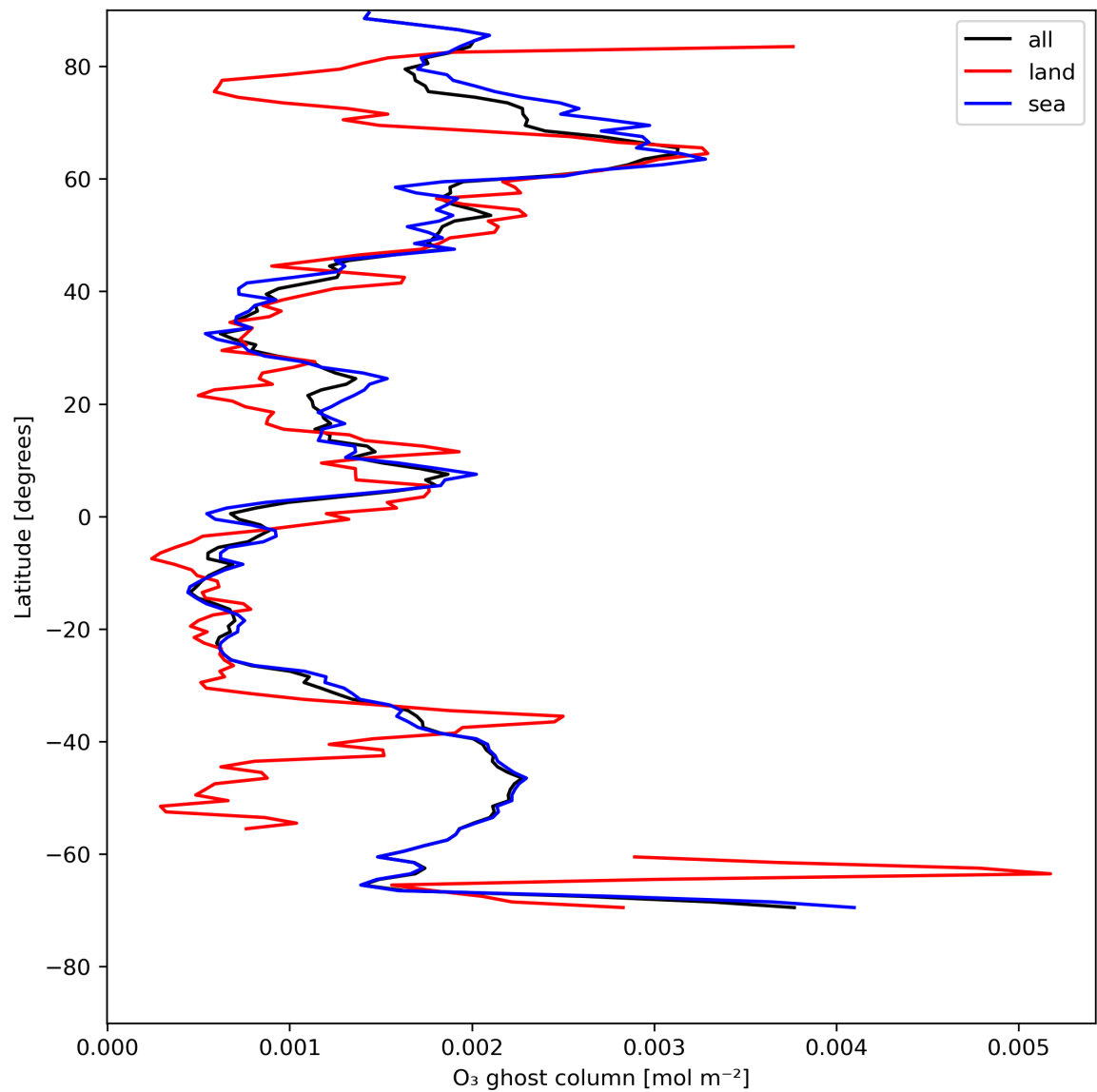
Figure 18: Zonal average of “O 3 ghost column” for 2023-07-26 to 2023-07-28.
