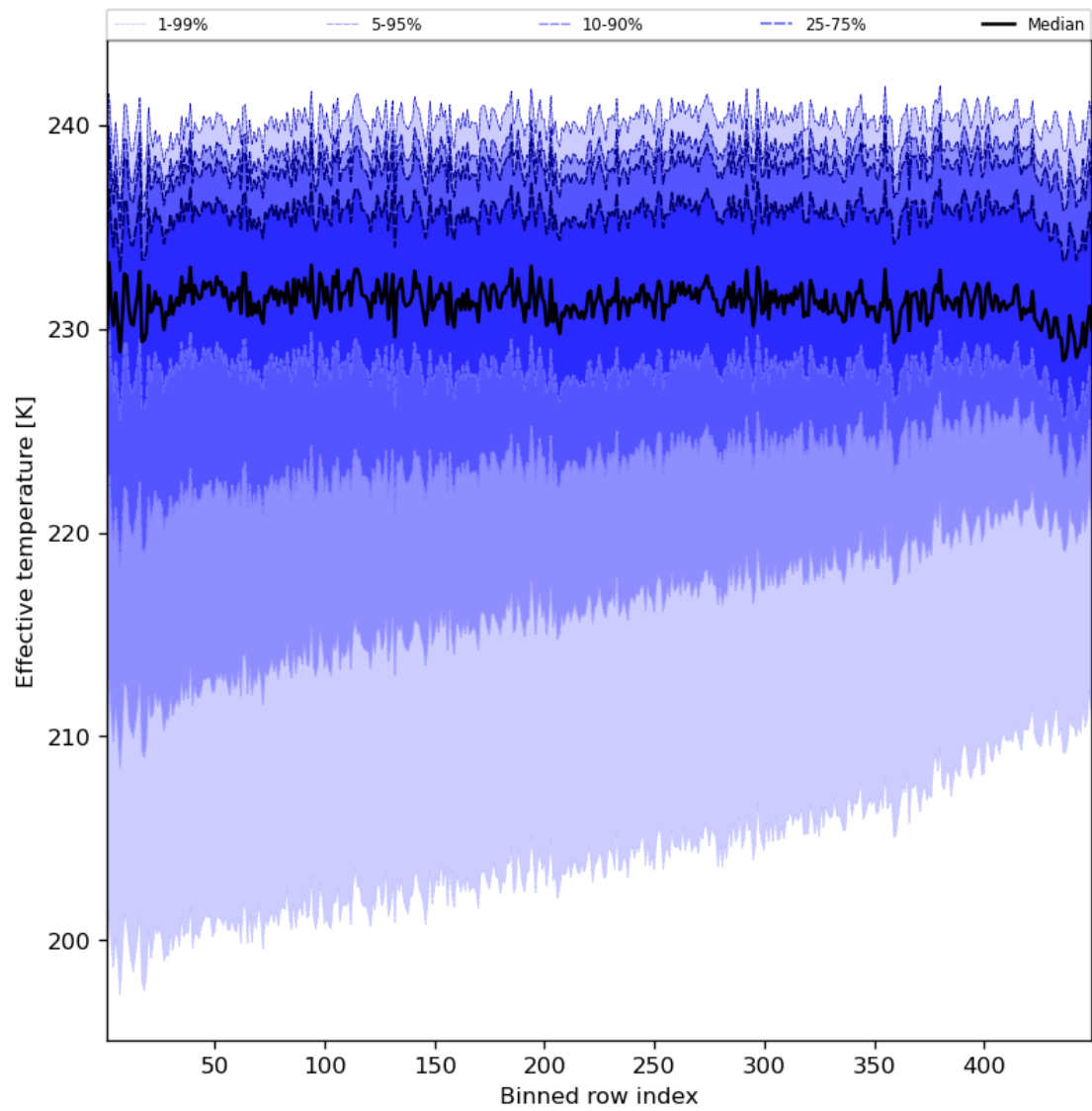
Figure 31: Along track statistics of “Effective temperature” for 2023-07-26 to 2023-07-28
