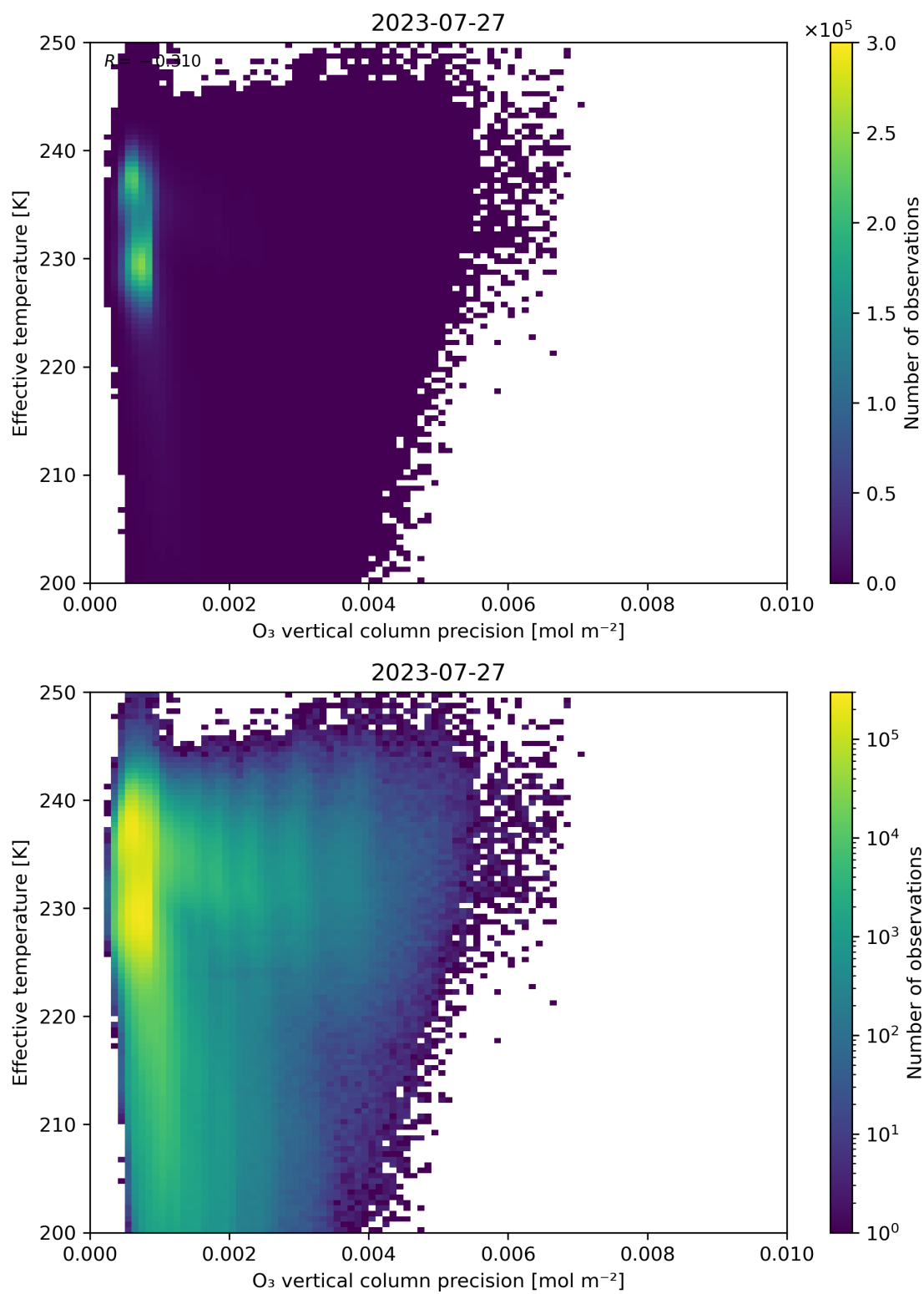
Figure 42: Scatter density plot of “O 3 vertical column precision” against “Effective temperature” for 2023-07-26 to 2023-07-28.
