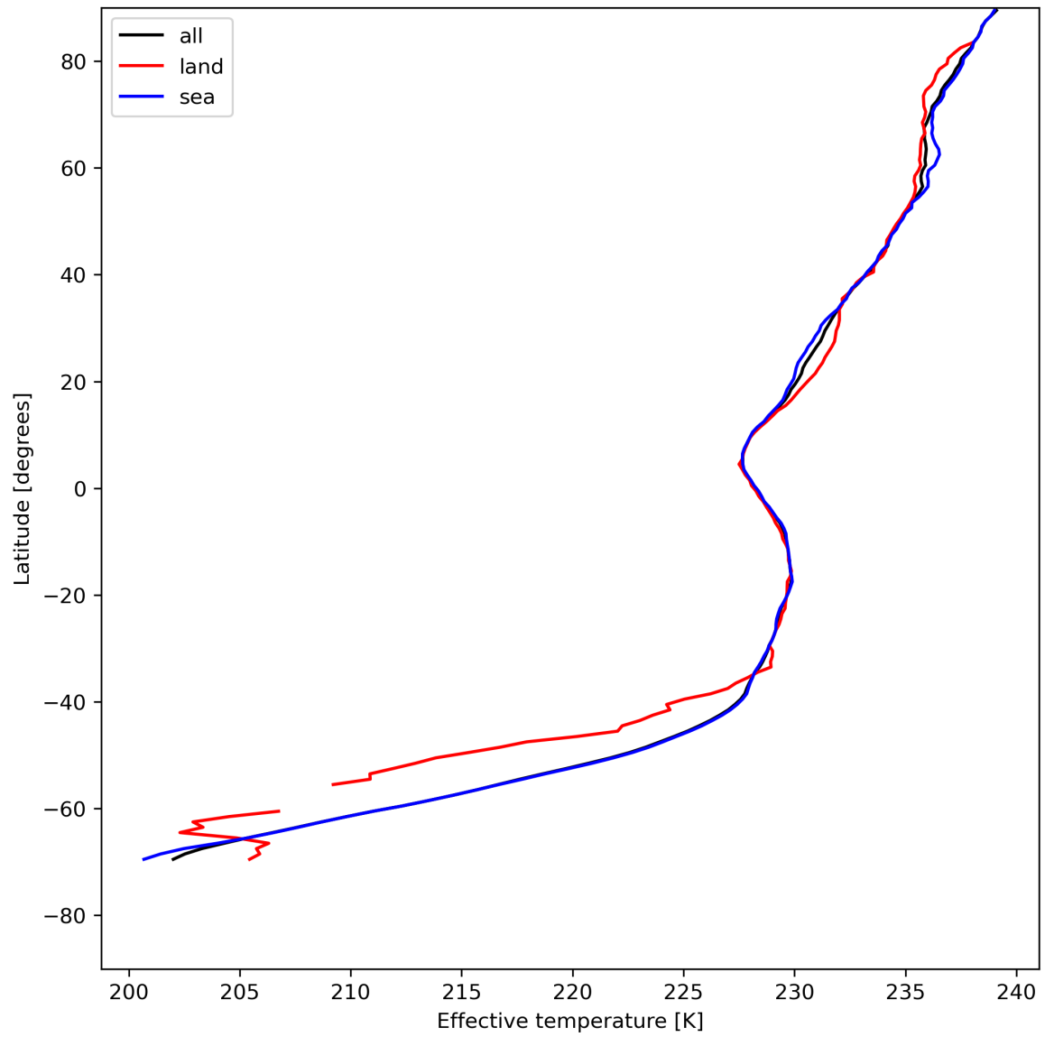
Figure 17: Zonal average of “Effective temperature” for 2023-07-26 to 2023-07-28.
