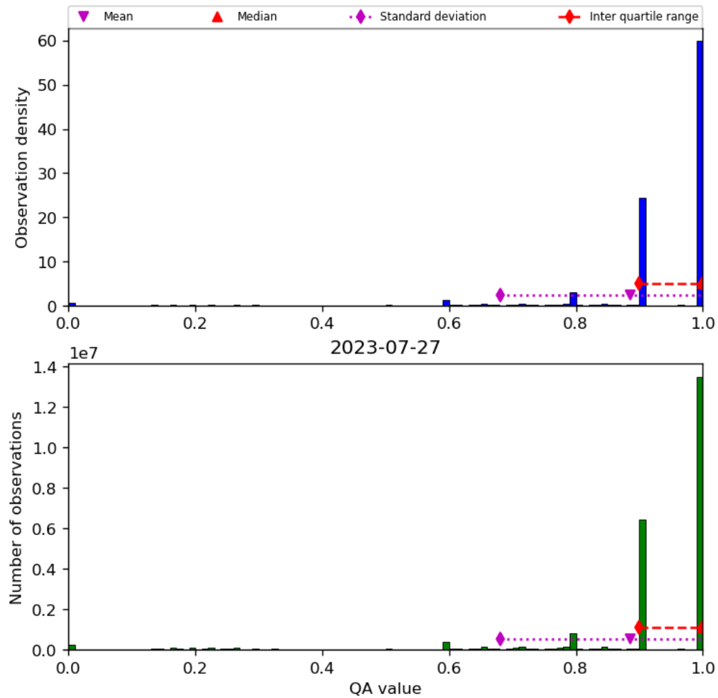
Figure 20: Histogram of “QA value” for 2023-07-26 to 2023-07-28
