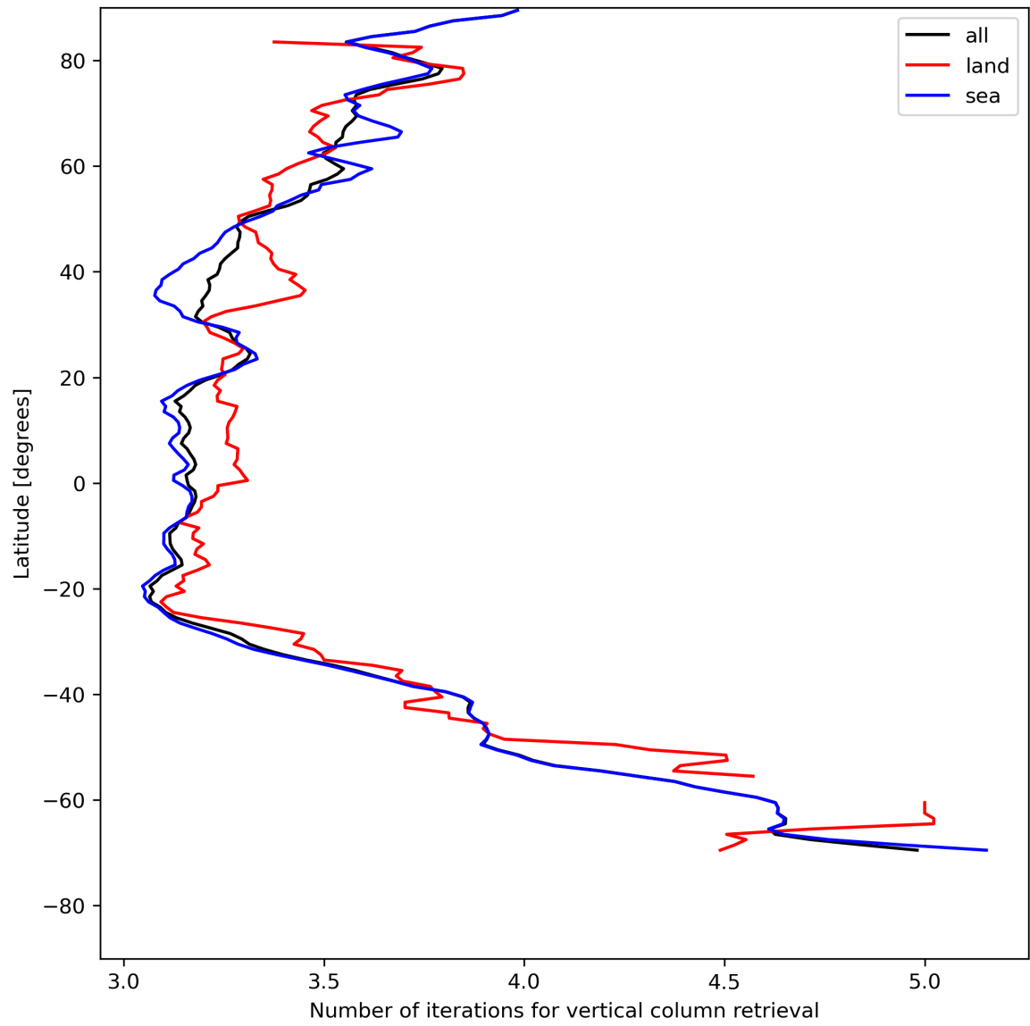
Figure 19: Zonal average of “Number of iterations for vertical column retrieval” for 2023-07-26 to 2023-07-28.
