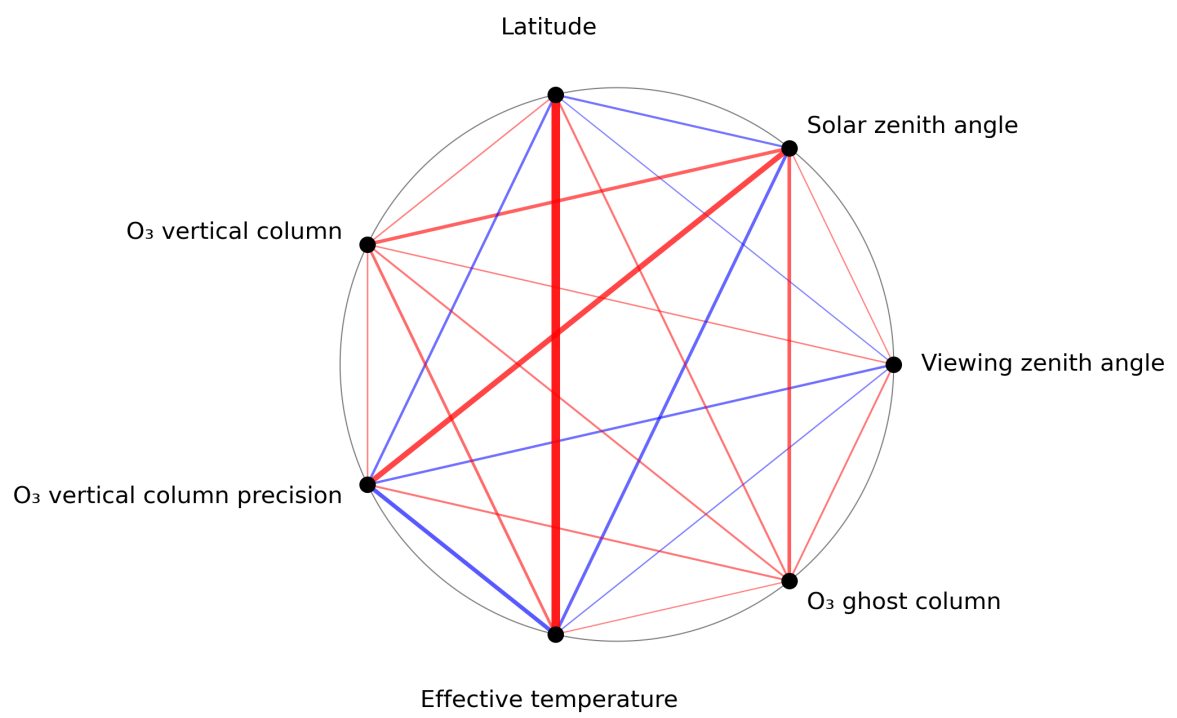
Figure 1: Map of correlation graph for 2023-07-26 to 2023-07-28.
