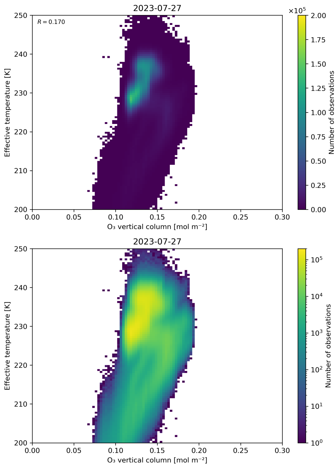
Figure 39: Scatter density plot of “O 3 vertical column” against “Effective temperature” for 2023-07-26 to 2023-07-28.
