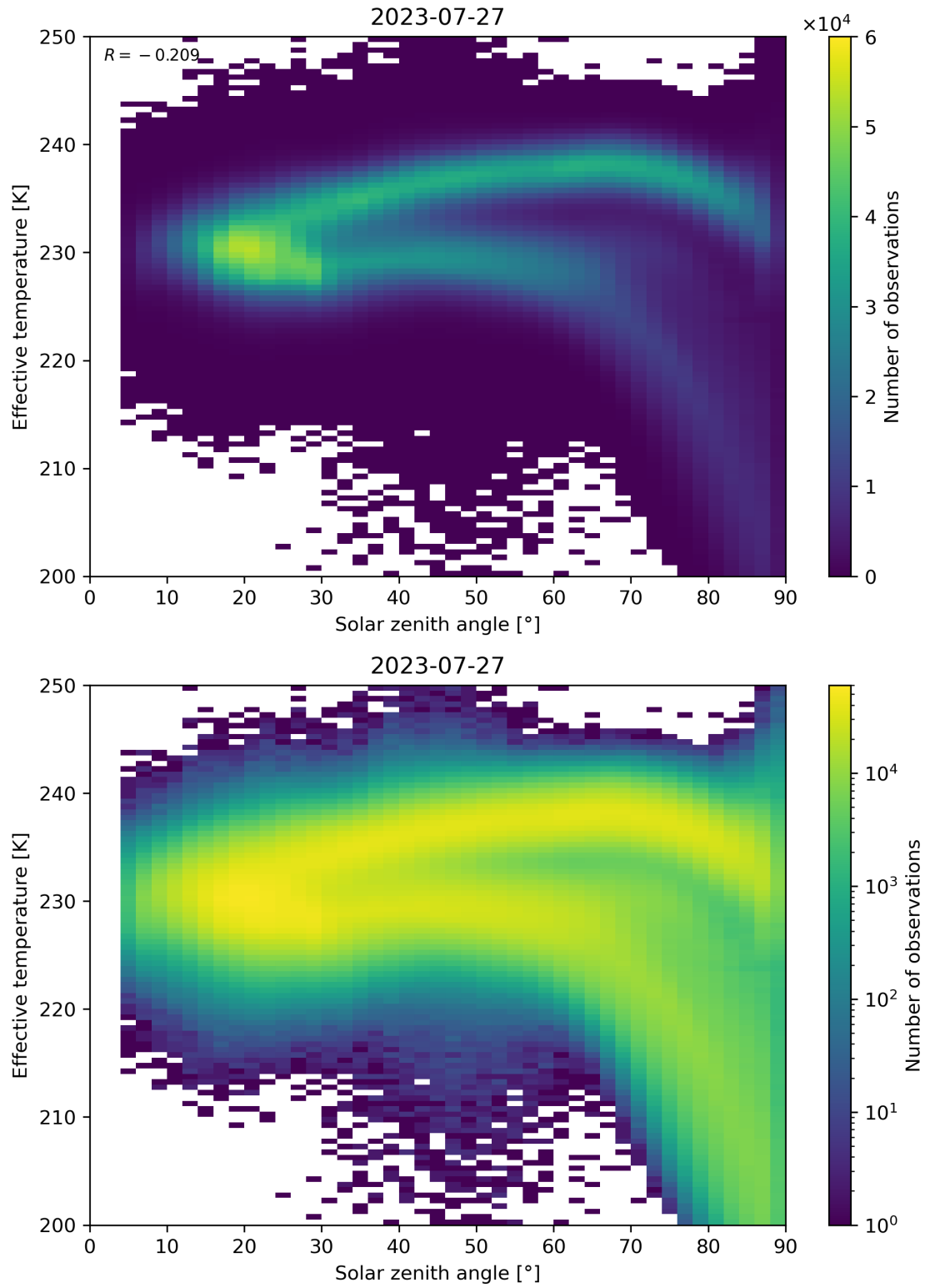
Figure 45: Scatter density plot of “Solar zenith angle” against “Effective temperature” for 2023-07-26 to 2023-07-28.
