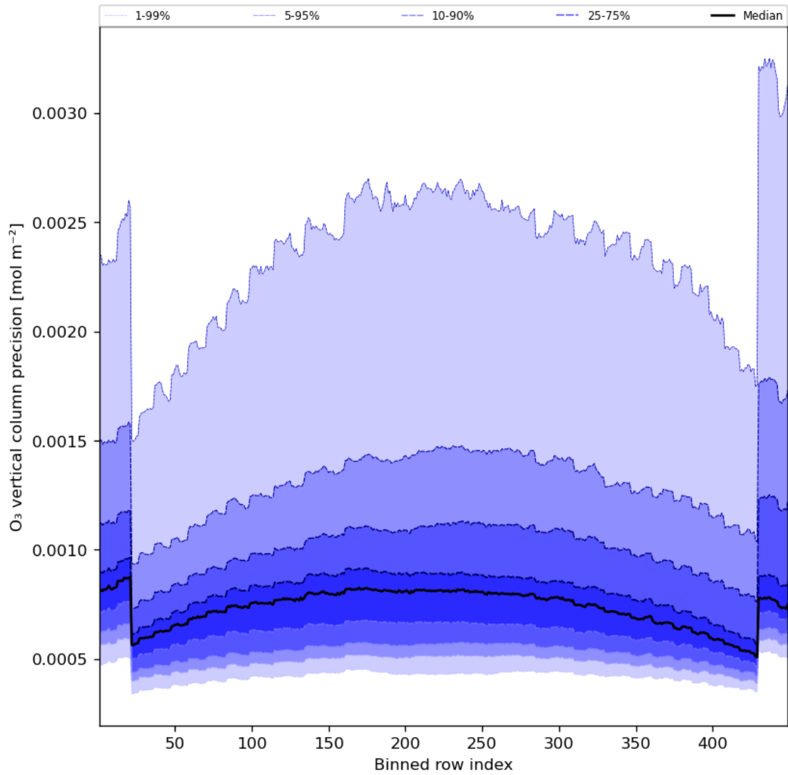
Figure 29: Along track statistics of “O 3 vertical column precision” for 2023-07-26 to 2023-07-28
