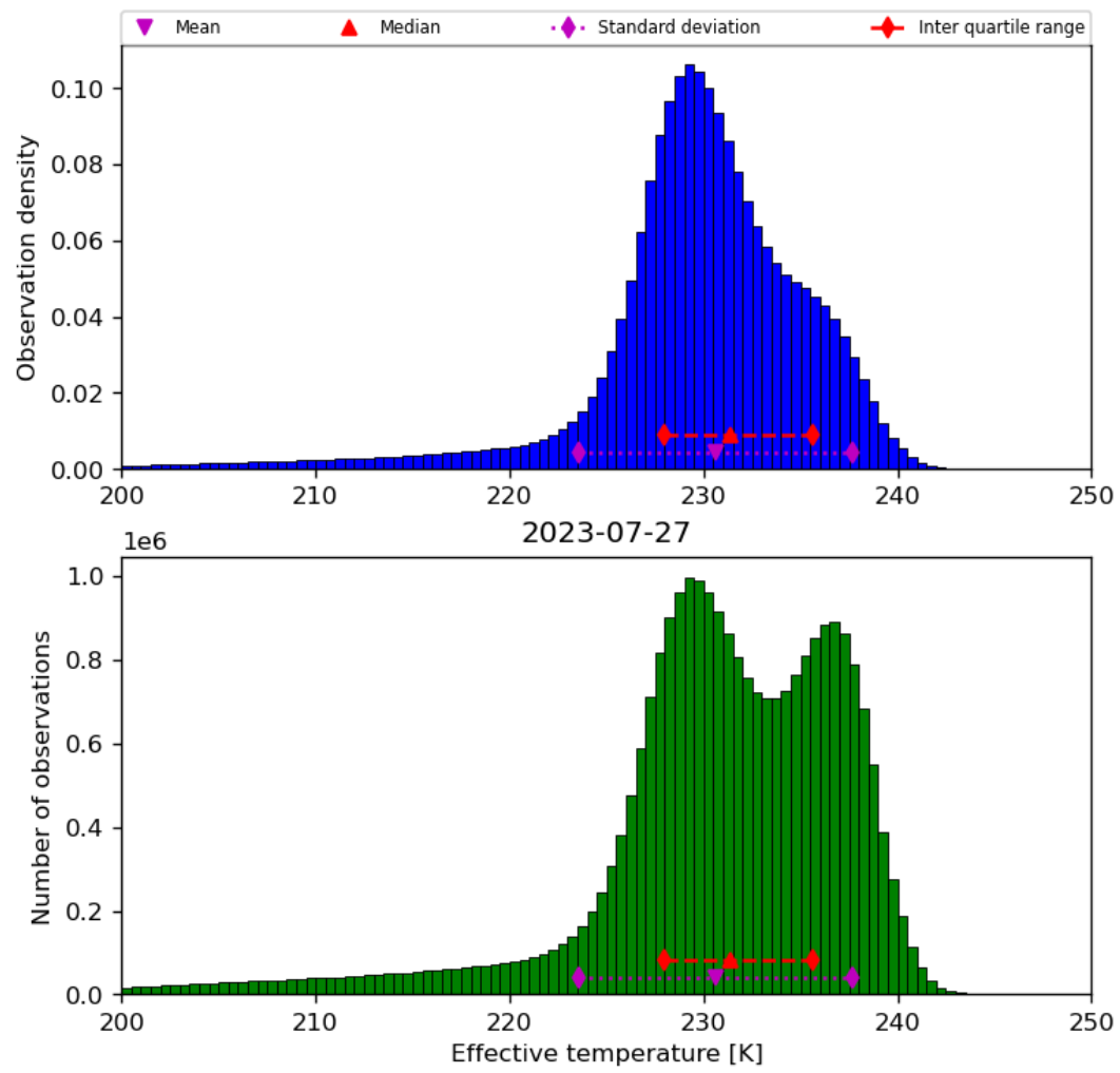
Figure 24: Histogram of “Effective temperature” for 2023-07-26 to 2023-07-28
