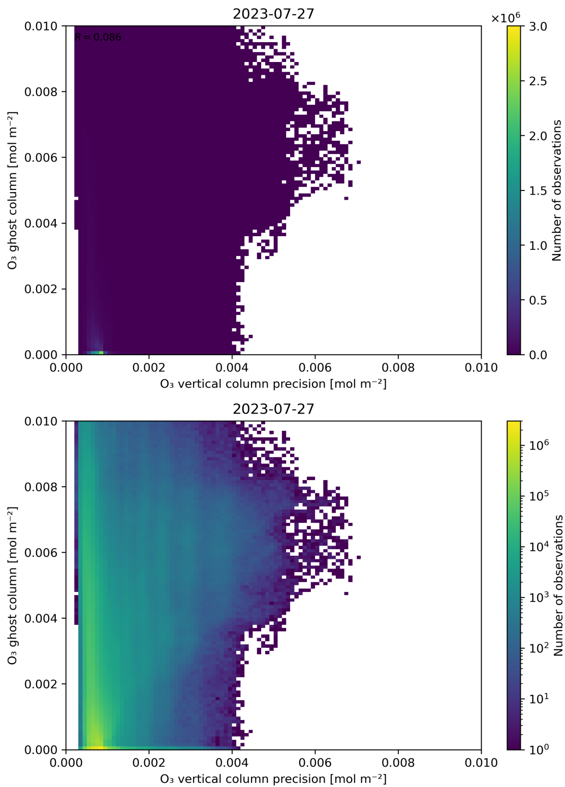
Figure 43: Scatter density plot of “O 3 vertical column precision” against “O 3 ghost column” for 2023-07-26 to 2023-07-28.
