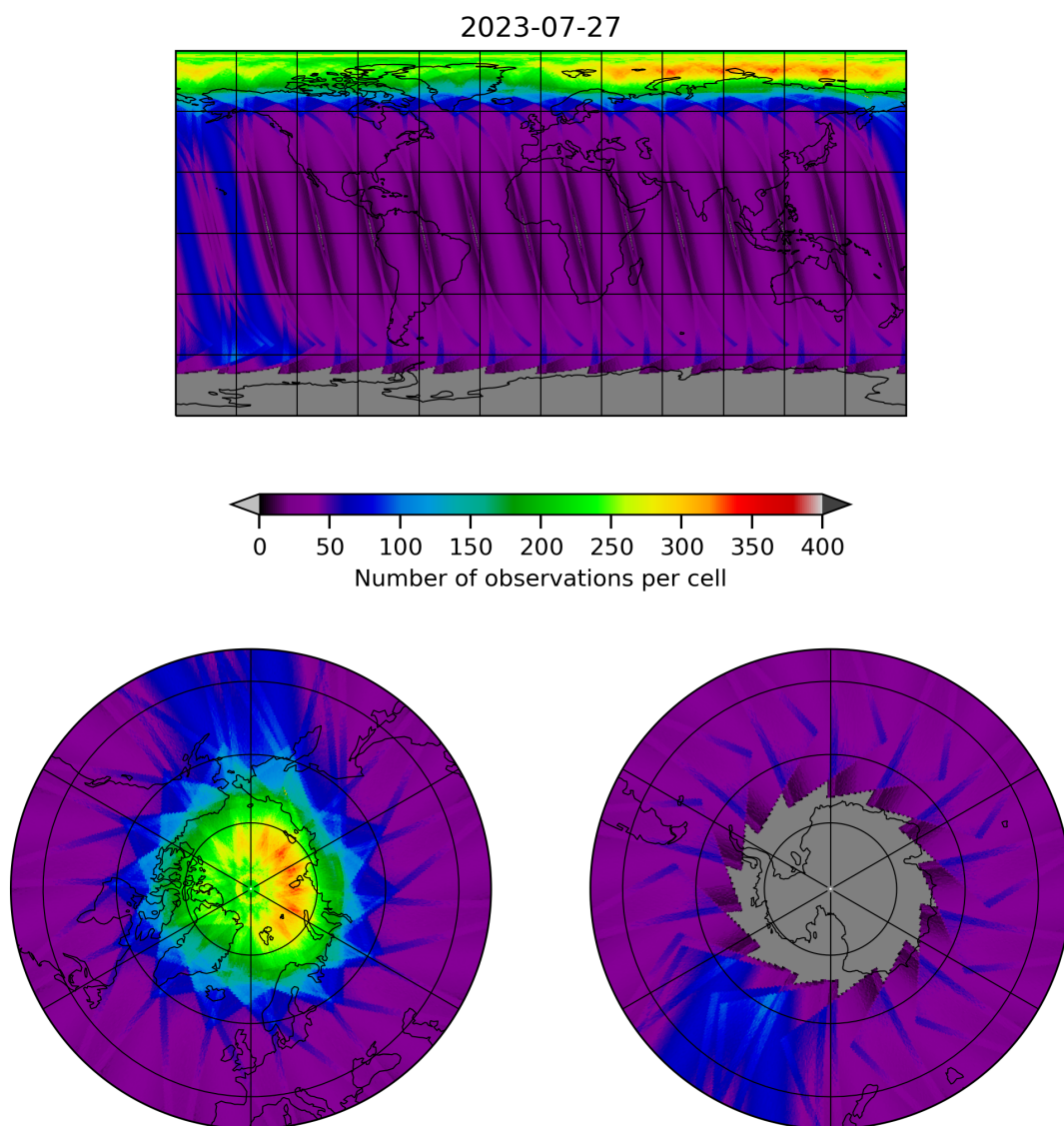
Figure 12: Map of the number of observations for 2023-07-26 to 2023-07-28
