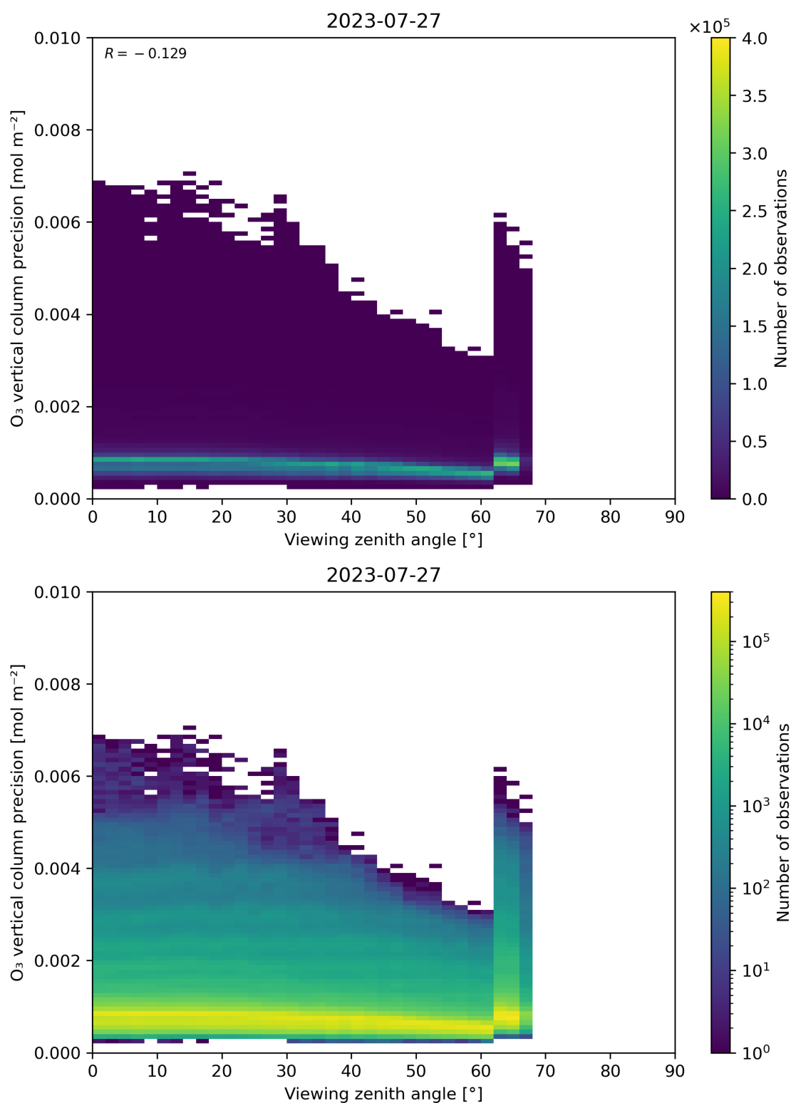
Figure 53: Scatter density plot of “Viewing zenith angle” against “O 3 vertical column precision” for 2023-07-26 to 2023-07-28.
