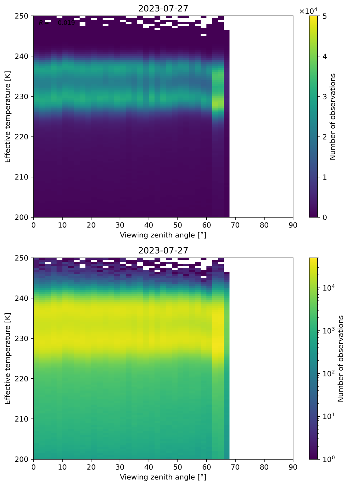
Figure 50: Scatter density plot of “Viewing zenith angle” against “Effective temperature” for 2023-07-26 to 2023-07-28.
