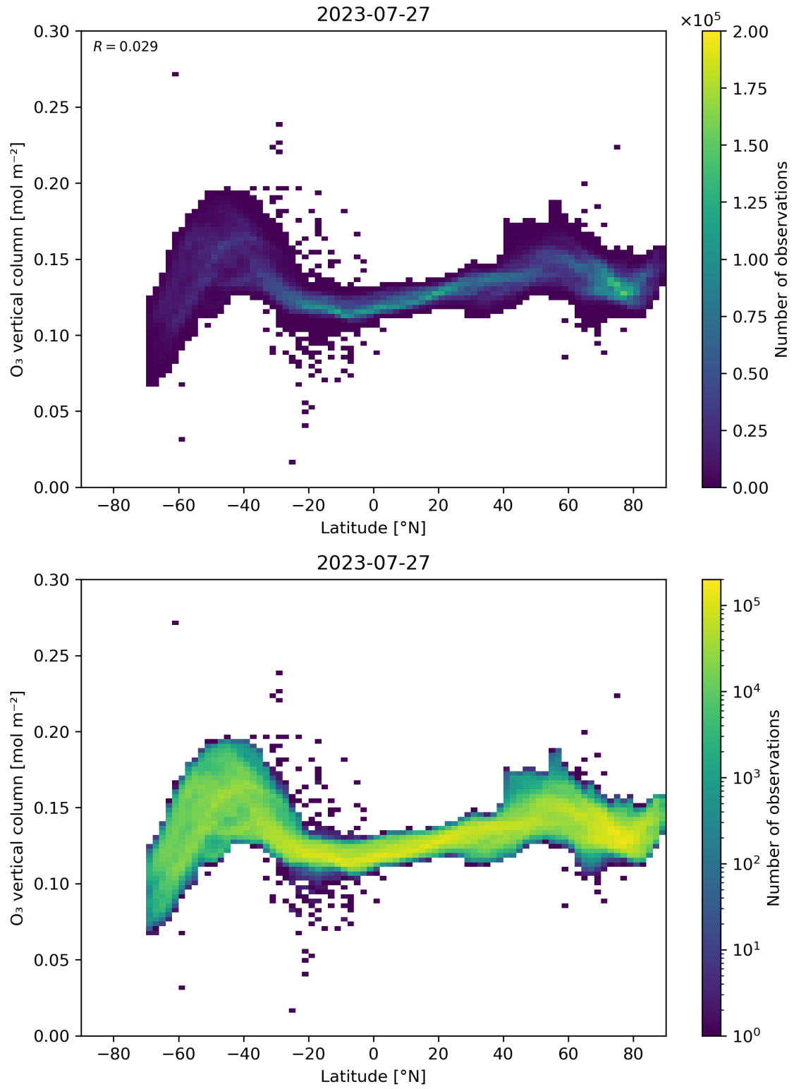
Figure 36: Scatter density plot of “Latitude” against “O 3 vertical column” for 2023-07-26 to 2023-07-28.
