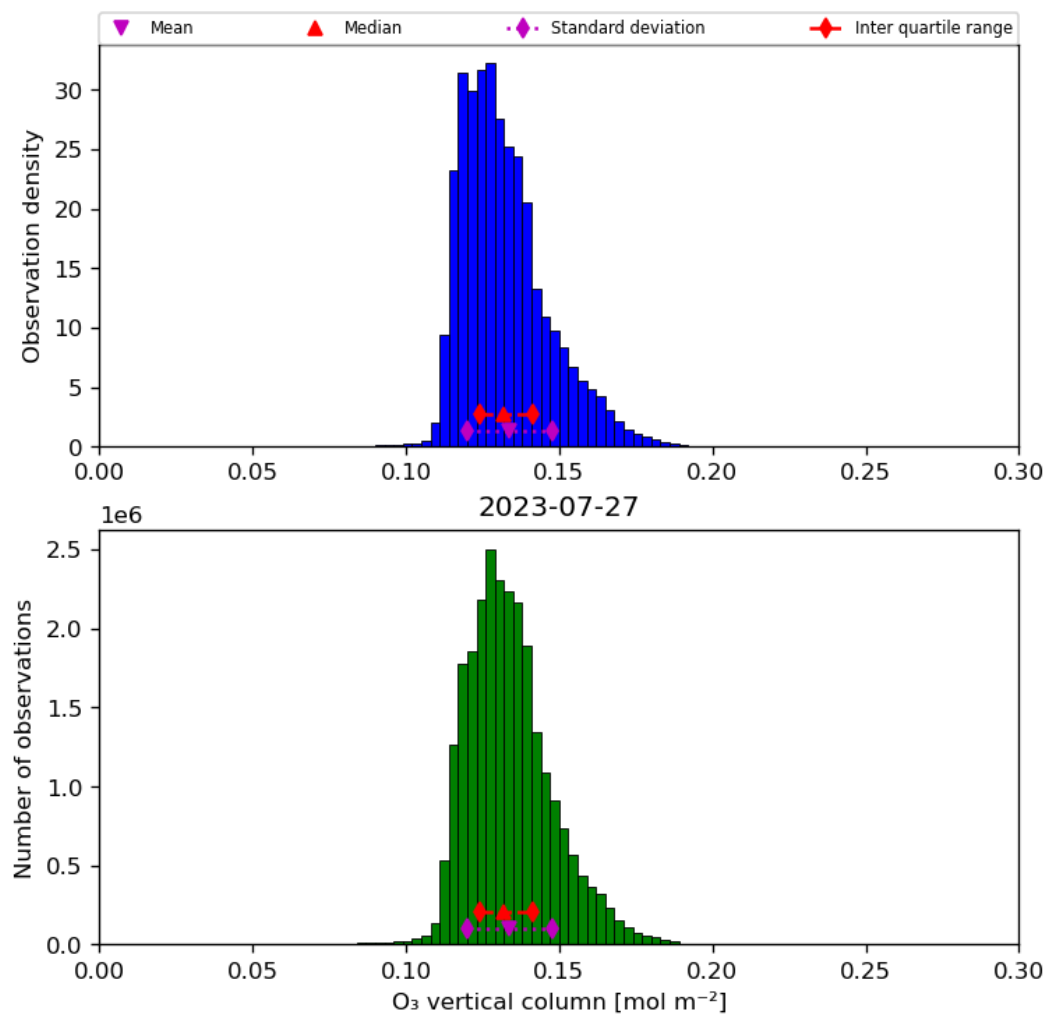
Figure 21: Histogram of “O 3 vertical column” for 2023-07-26 to 2023-07-28
