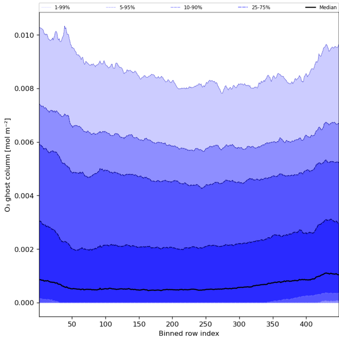
Figure 32: Along track statistics of “O 3 ghost column” for 2023-07-26 to 2023-07-28
