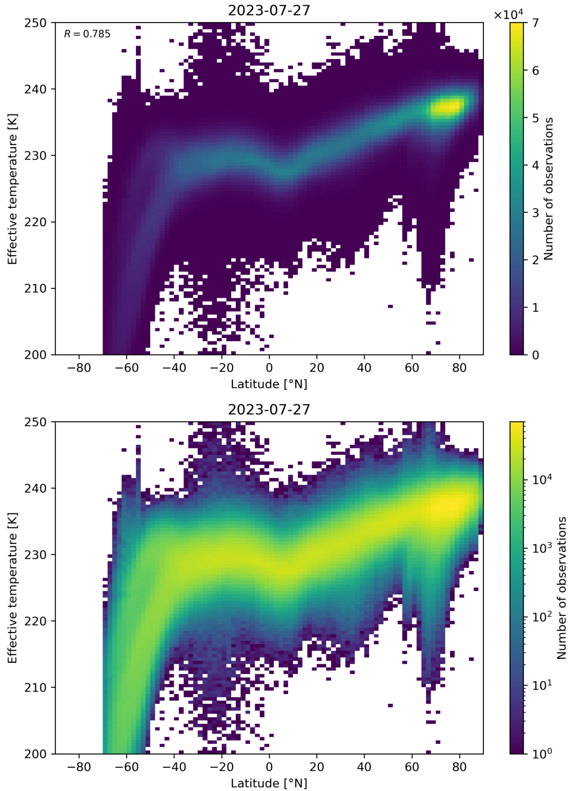
Figure 34: Scatter density plot of “Latitude” against “Effective temperature” for 2023-07-26 to 2023-07-28.
