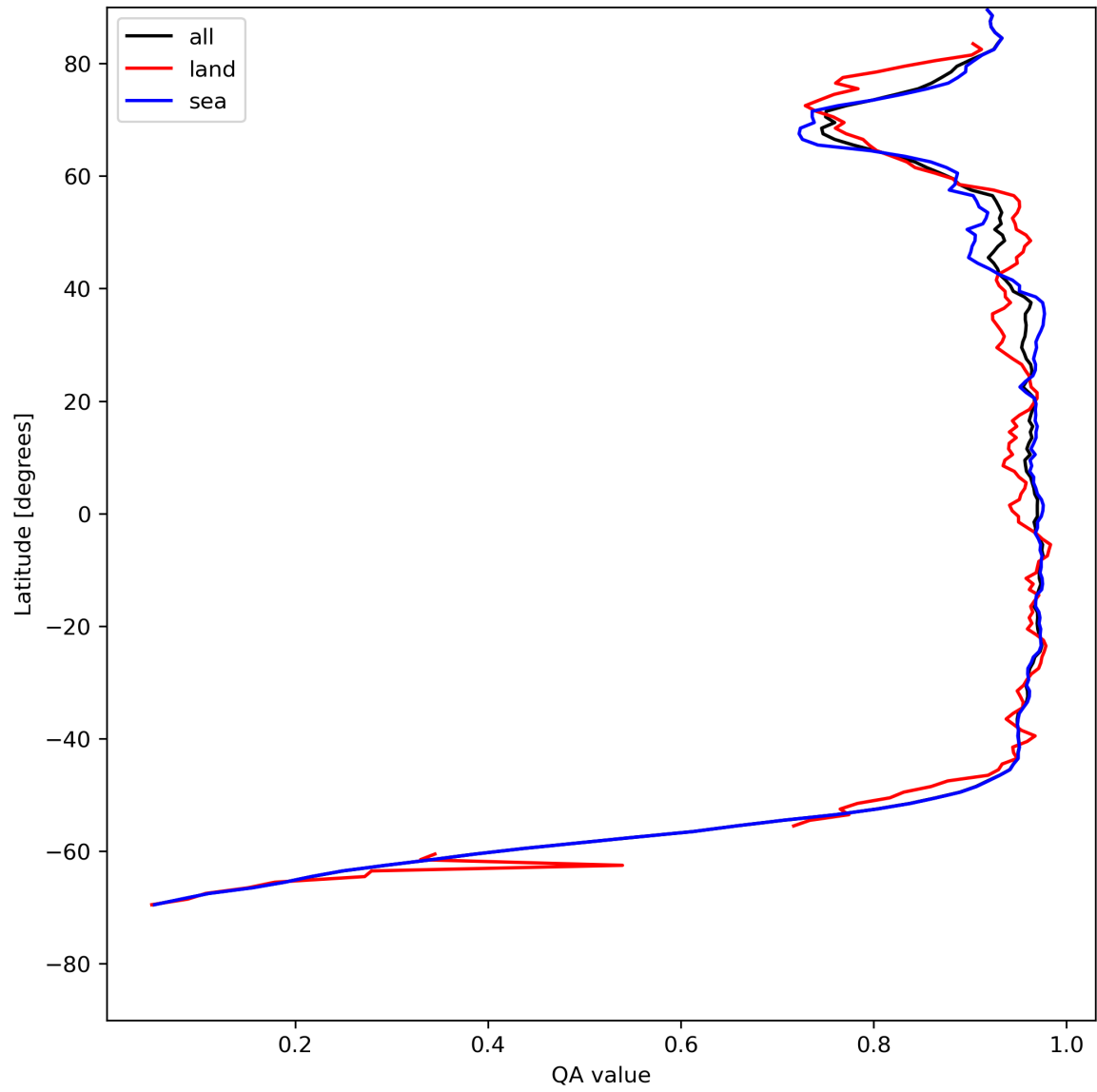
Figure 13: Zonal average of “QA value” for 2023-07-26 to 2023-07-28.
