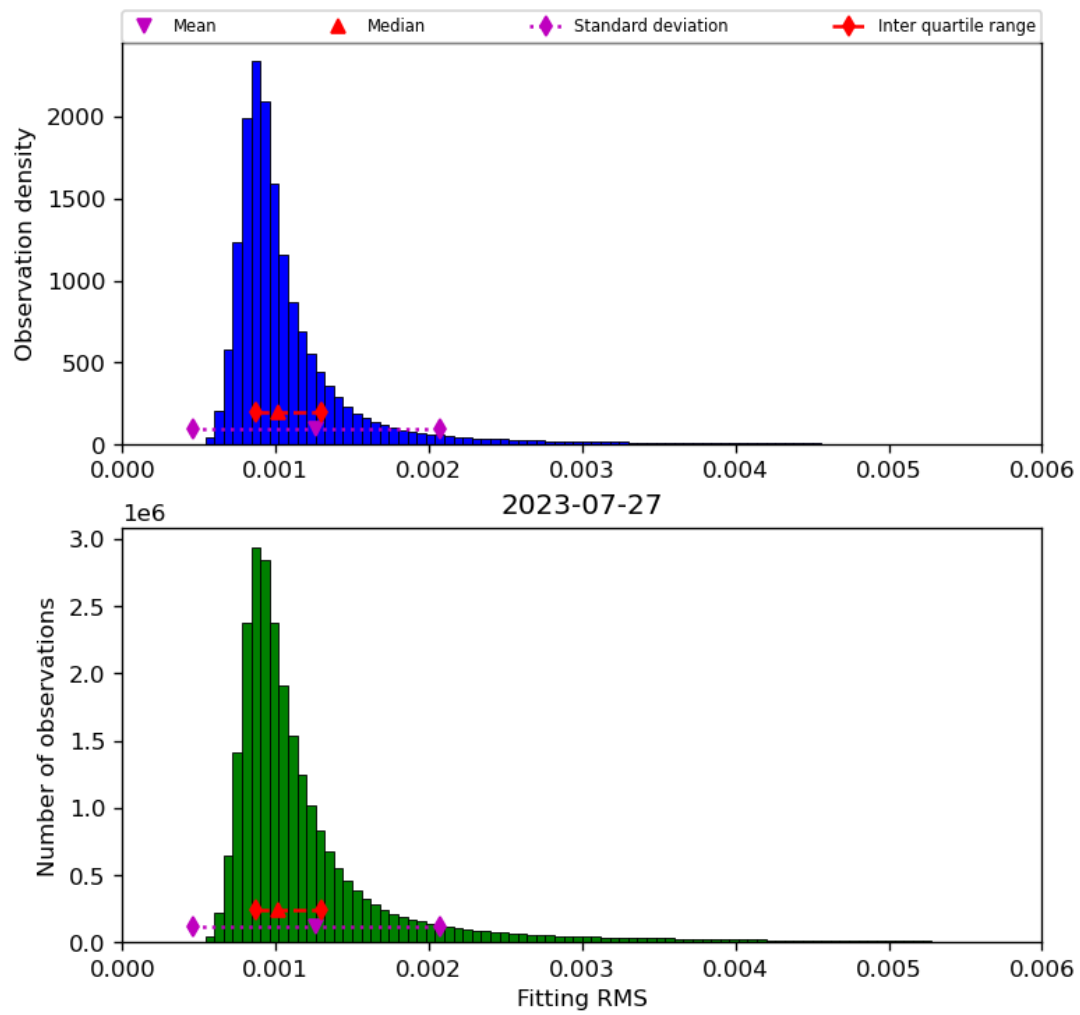
Figure 23: Histogram of “Fitting RMS” for 2023-07-26 to 2023-07-28
