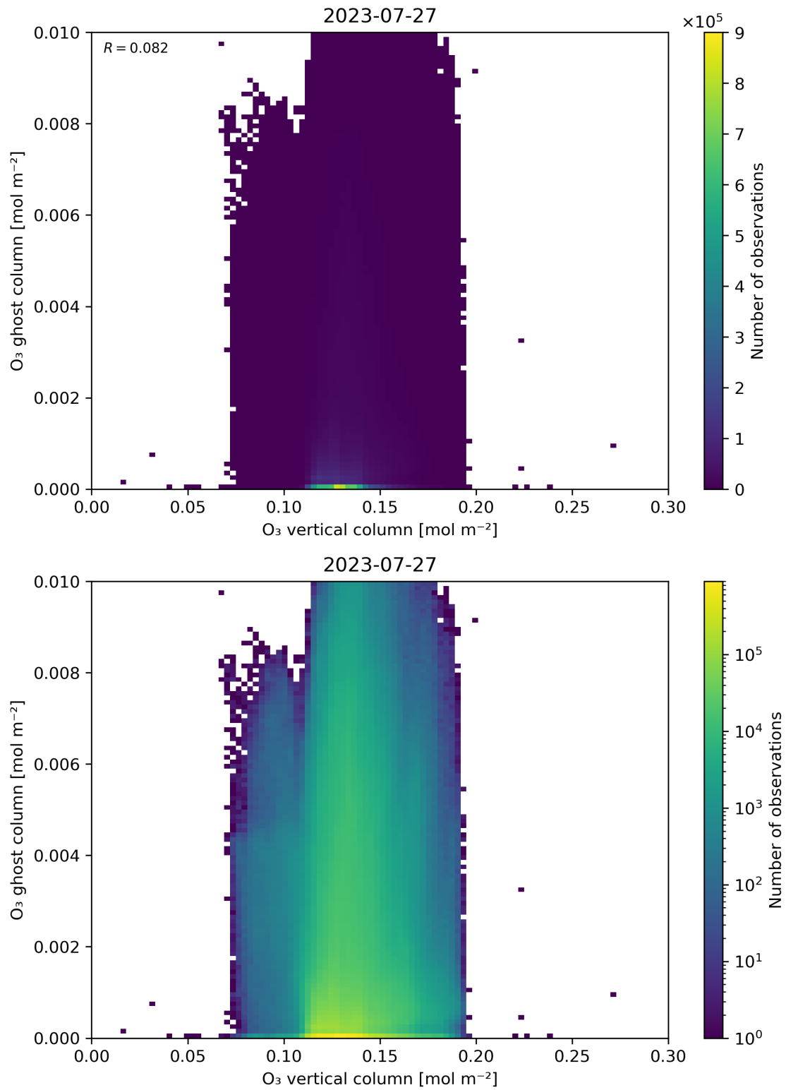
Figure 40: Scatter density plot of “O 3 vertical column” against “O 3 ghost column” for 2023-07-26 to 2023-07-28.
