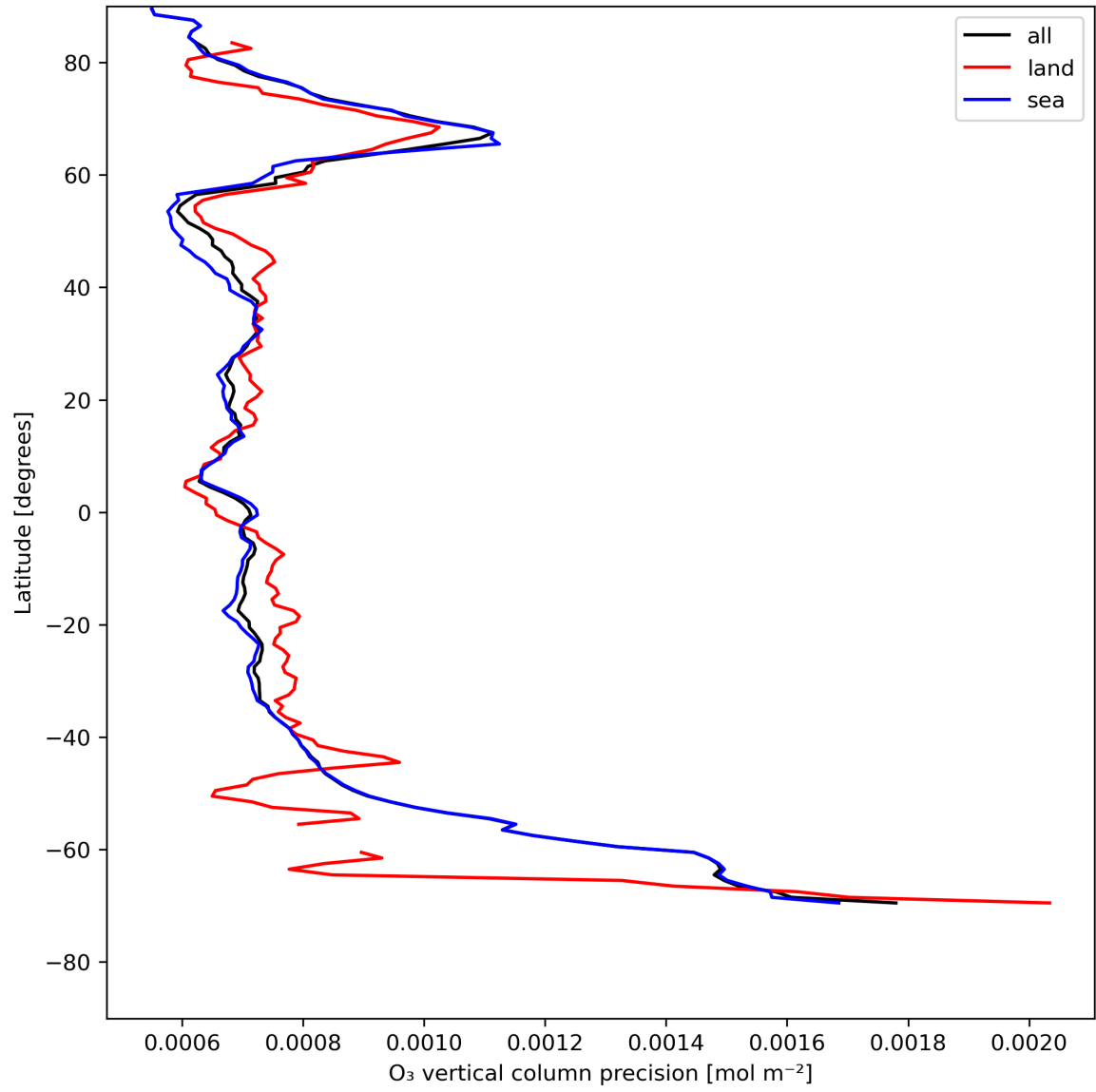
Figure 15: Zonal average of “O 3 vertical column precision” for 2023-07-26 to 2023-07-28.
