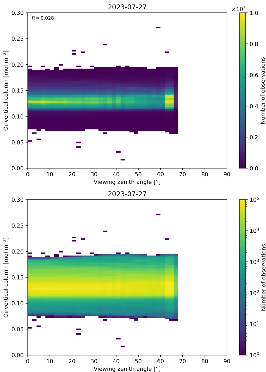
Figure 52: Scatter density plot of “Viewing zenith angle” against “O 3 vertical column” for 2023-07-26 to 2023-07-28.
