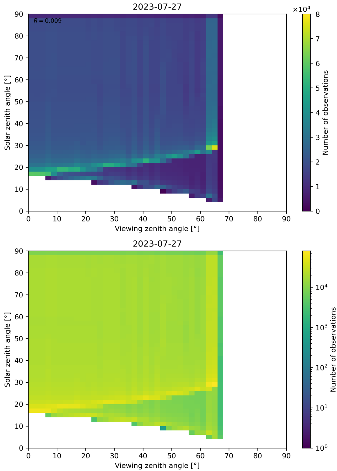
Figure 54: Scatter density plot of “Viewing zenith angle” against “Solar zenith angle” for 2023-07-26 to 2023-07-28.
