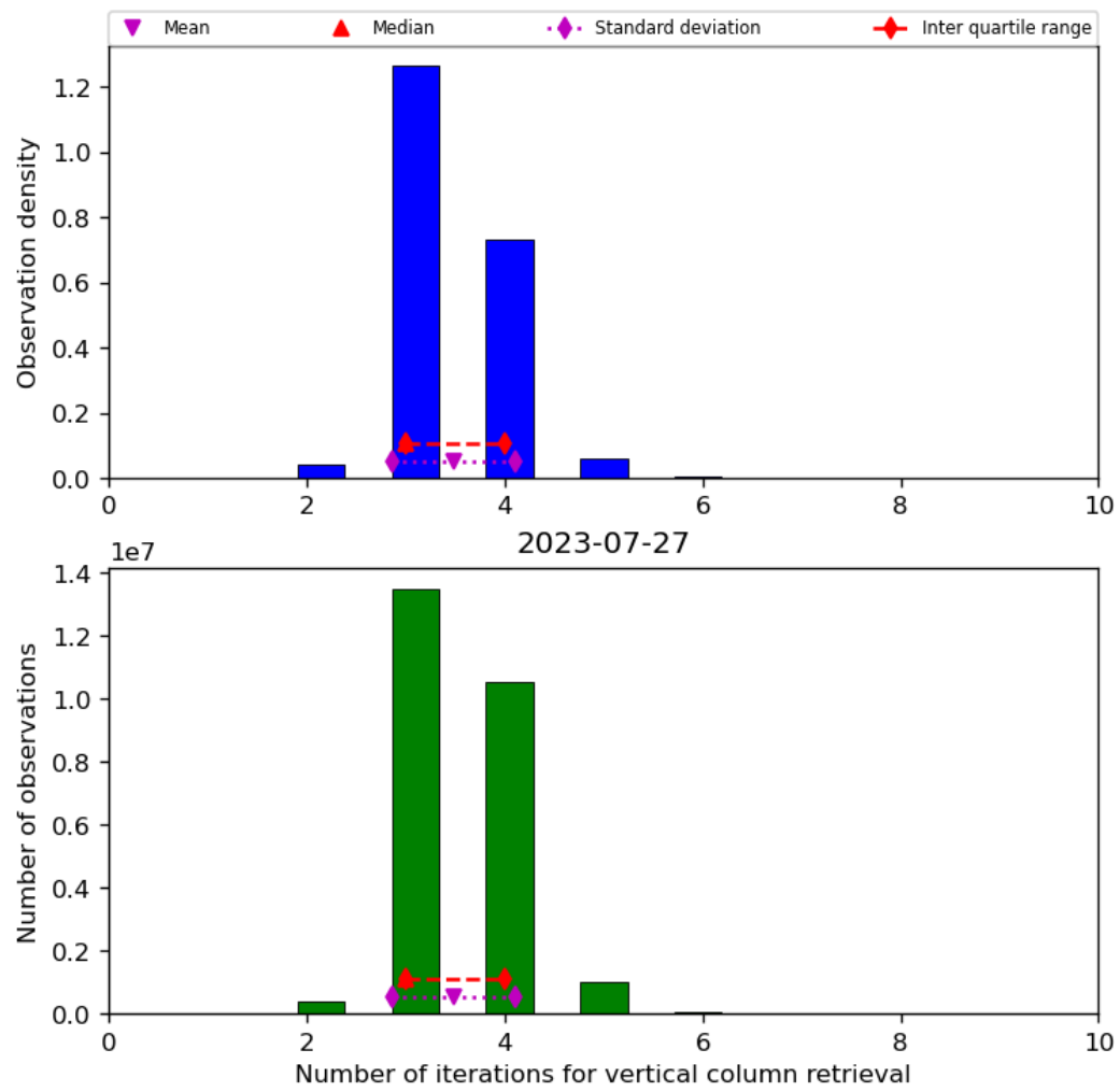
Figure 26: Histogram of “Number of iterations for vertical column retrieval” for 2023-07-26 to 2023-07-28
