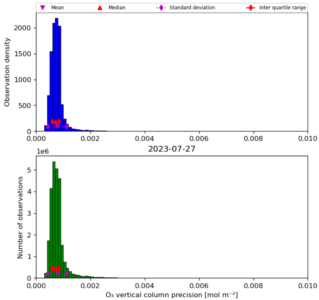
Figure 22: Histogram of “O 3 vertical column precision” for 2023-07-26 to 2023-07-28
