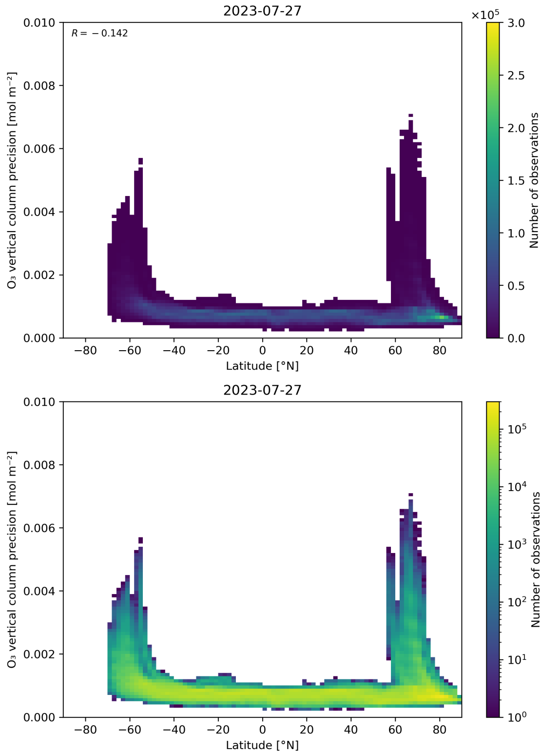
Figure 37: Scatter density plot of “Latitude” against “O 3 vertical column precision” for 2023-07-26 to 2023-07-28.
