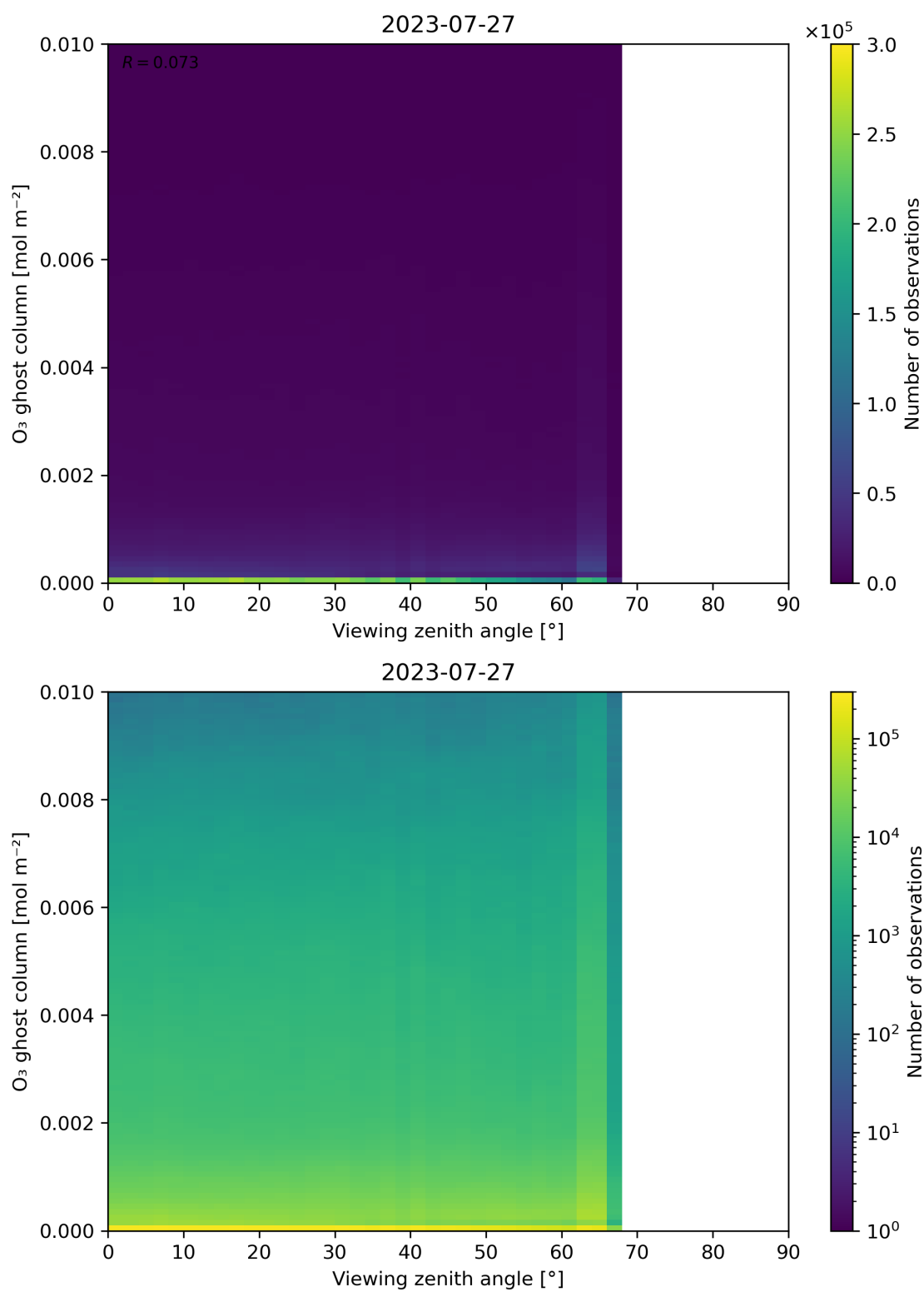
Figure 51: Scatter density plot of “Viewing zenith angle” against “O 3 ghost column” for 2023-07-26 to 2023-07-28.
