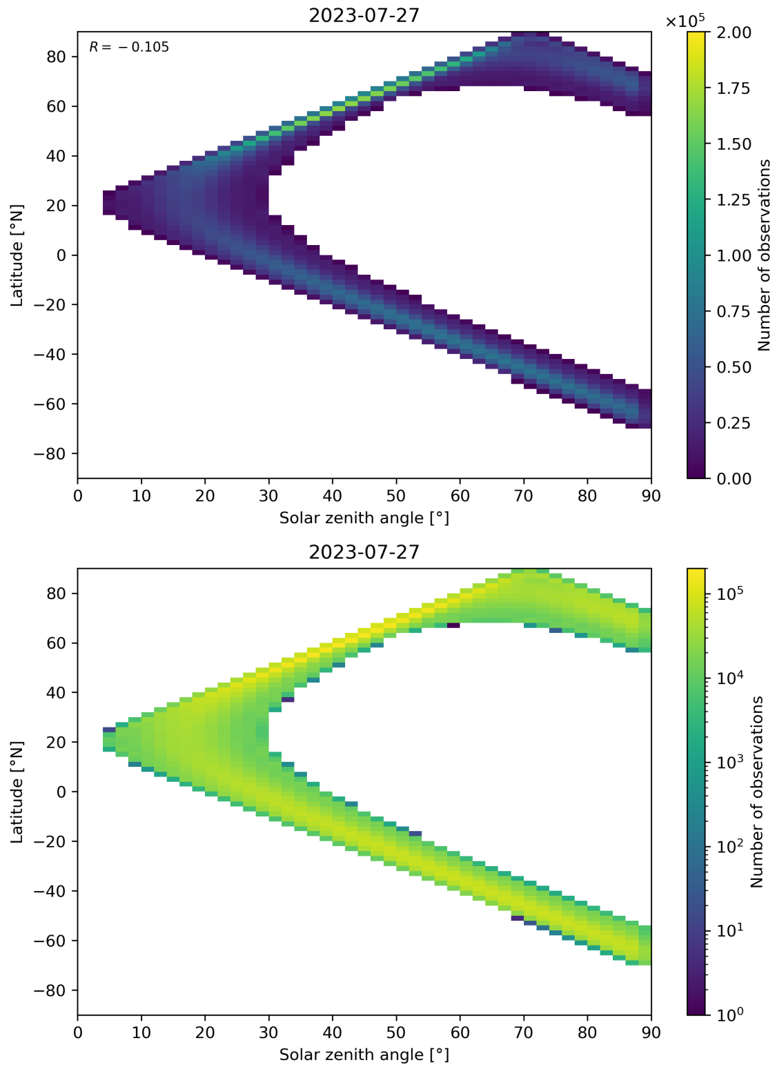
Figure 44: Scatter density plot of “Solar zenith angle” against “Latitude” for 2023-07-26 to 2023-07-28.
