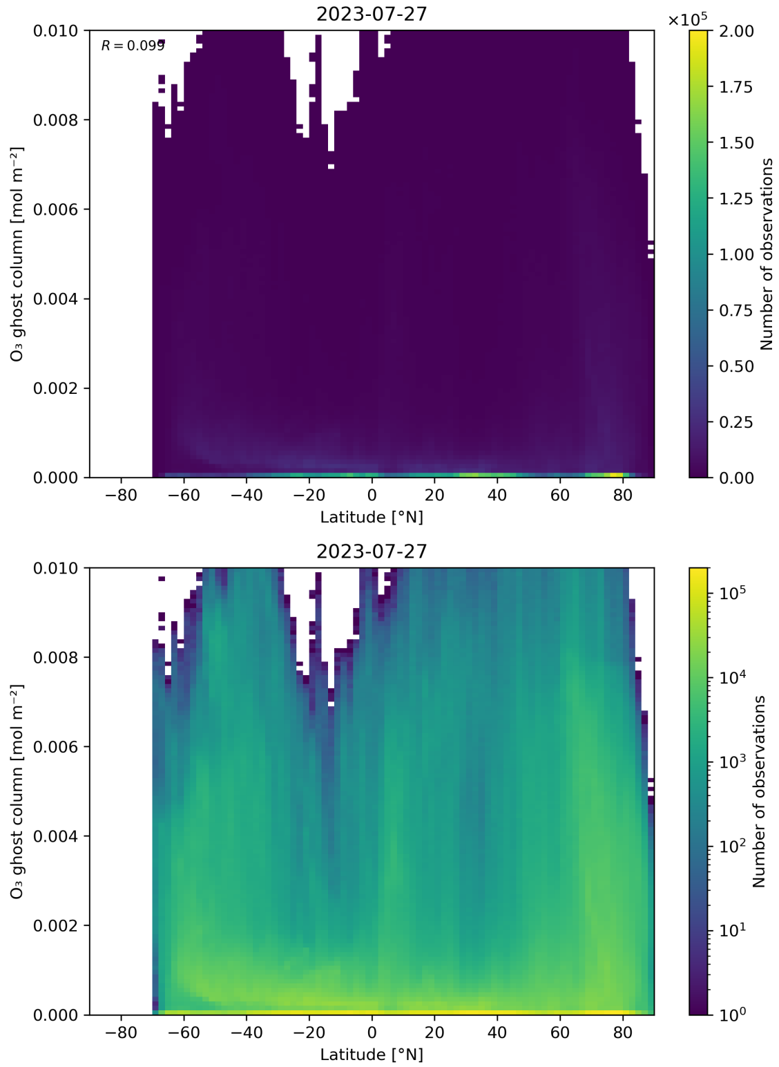
Figure 35: Scatter density plot of “Latitude” against “O 3 ghost column” for 2023-07-26 to 2023-07-28.
