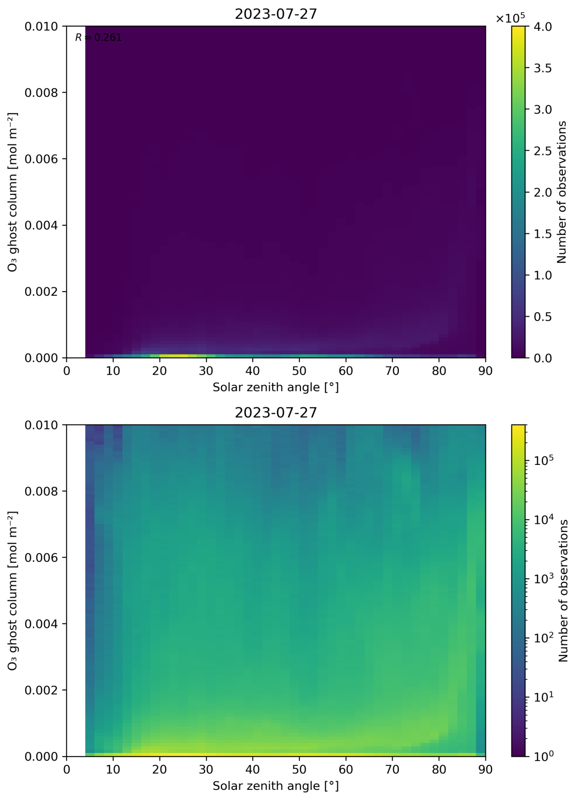
Figure 46: Scatter density plot of “Solar zenith angle” against “O 3 ghost column” for 2023-07-26 to 2023-07-28.
