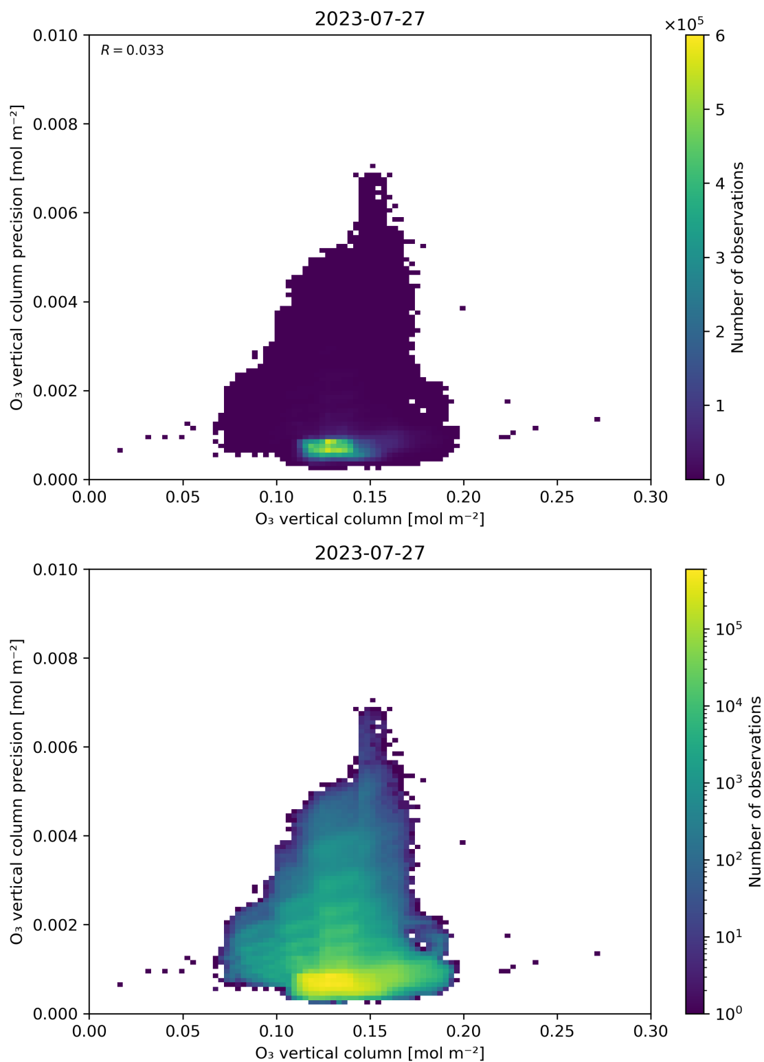
Figure 41: Scatter density plot of “O 3 vertical column” against “O 3 vertical column precision” for 2023-07-26 to 2023-07-28.
