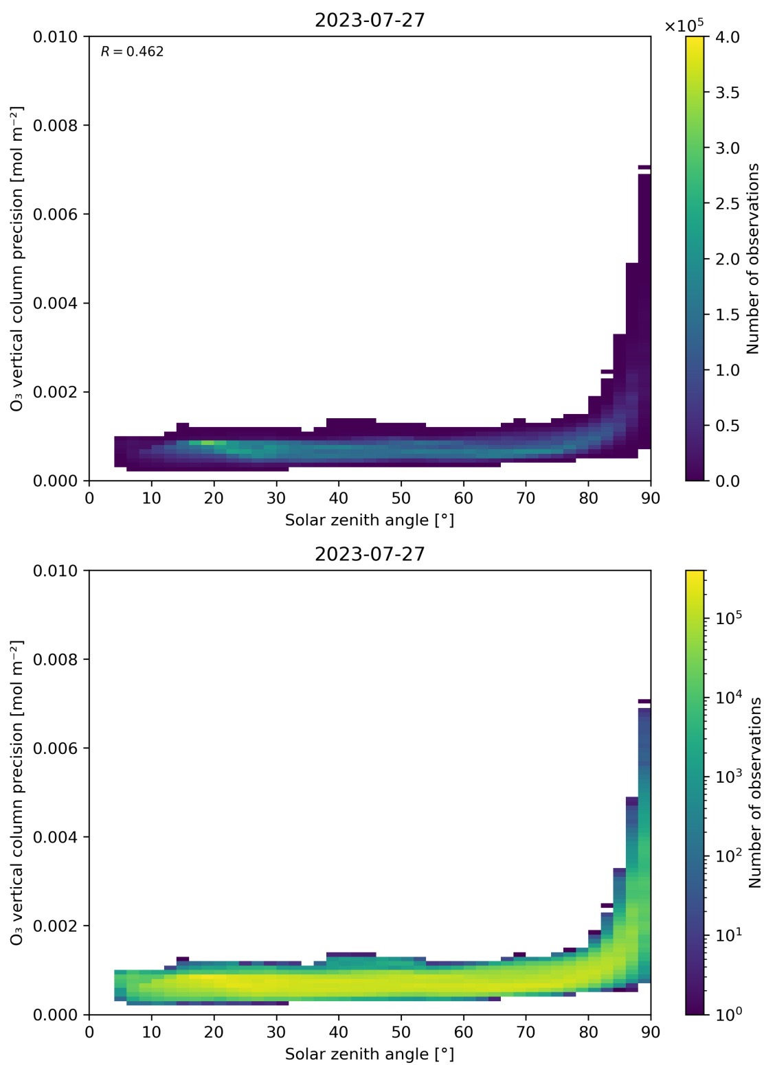
Figure 48: Scatter density plot of “Solar zenith angle” against “O 3 vertical column precision” for 2023-07-26 to 2023-07-28.
