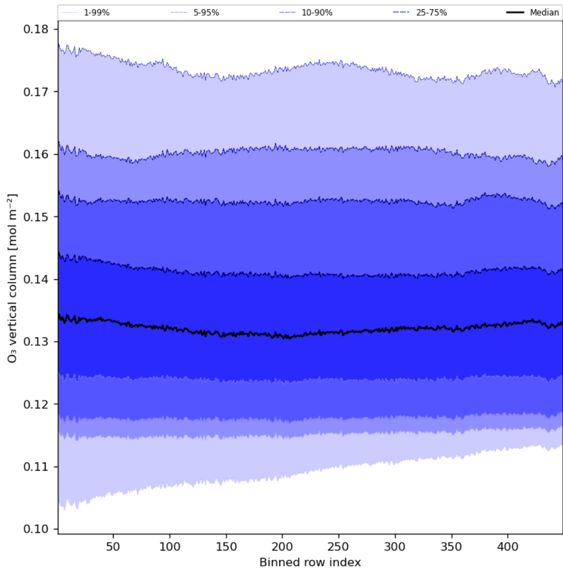
Figure 28: Along track statistics of “ O_3 vertical column” for 2023-07-26 to 2023-07-28
