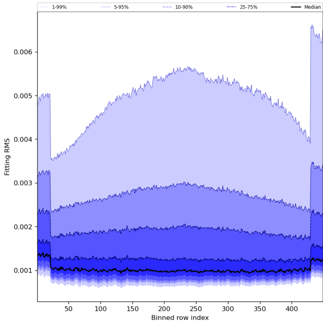
Figure 30: Along track statistics of “Fitting RMS” for 2023-07-26 to 2023-07-28
