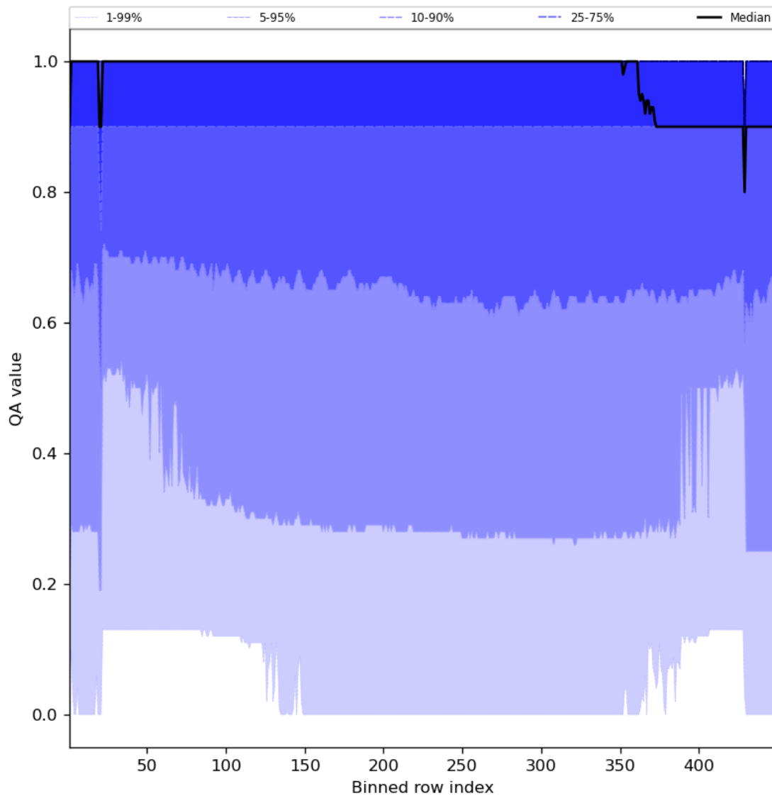
Figure 27: Along track statistics of “QA value” for 2023-07-26 to 2023-07-28
