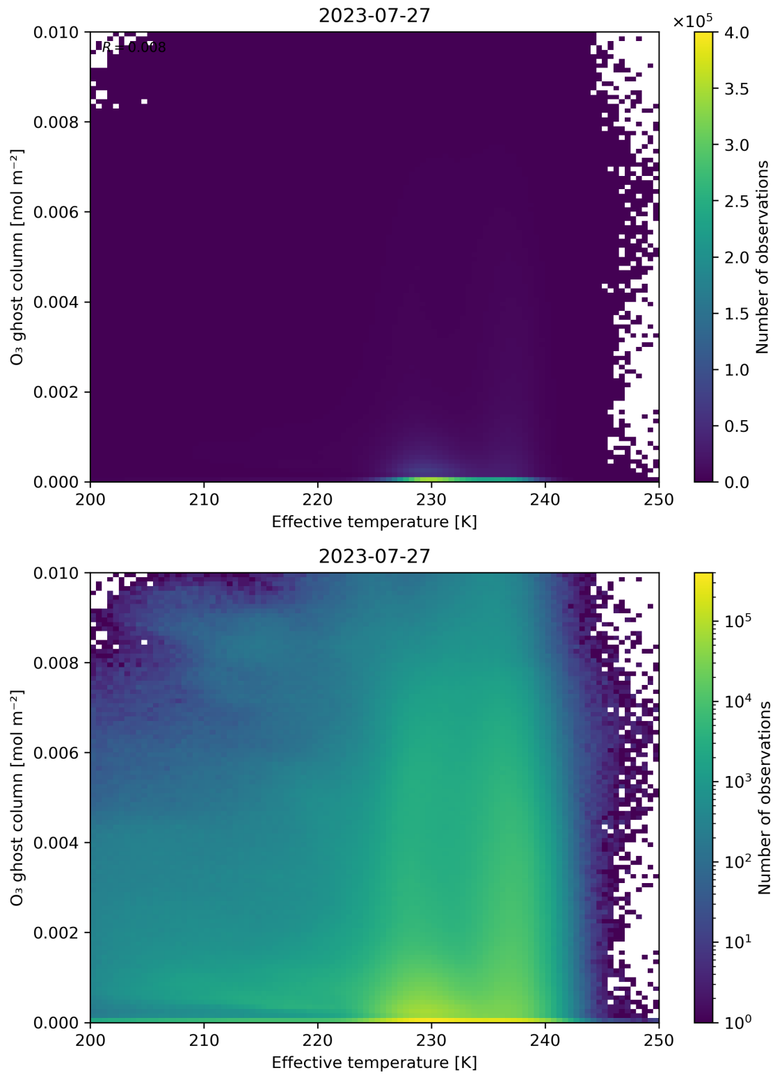
Figure 38: Scatter density plot of “Effective temperature” against “O 3 ghost column” for 2023-07-26 to 2023-07-28.
