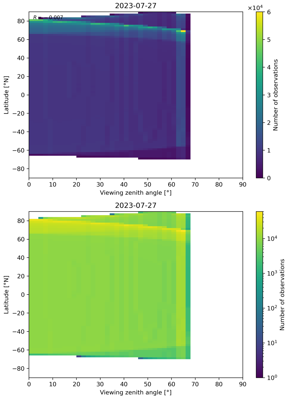
Figure 49: Scatter density plot of “Viewing zenith angle” against “Latitude” for 2023-07-26 to 2023-07-28.
