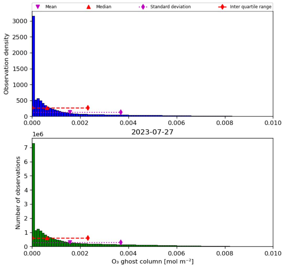
Figure 25: Histogram of “O 3 ghost column” for 2023-07-26 to 2023-07-28
