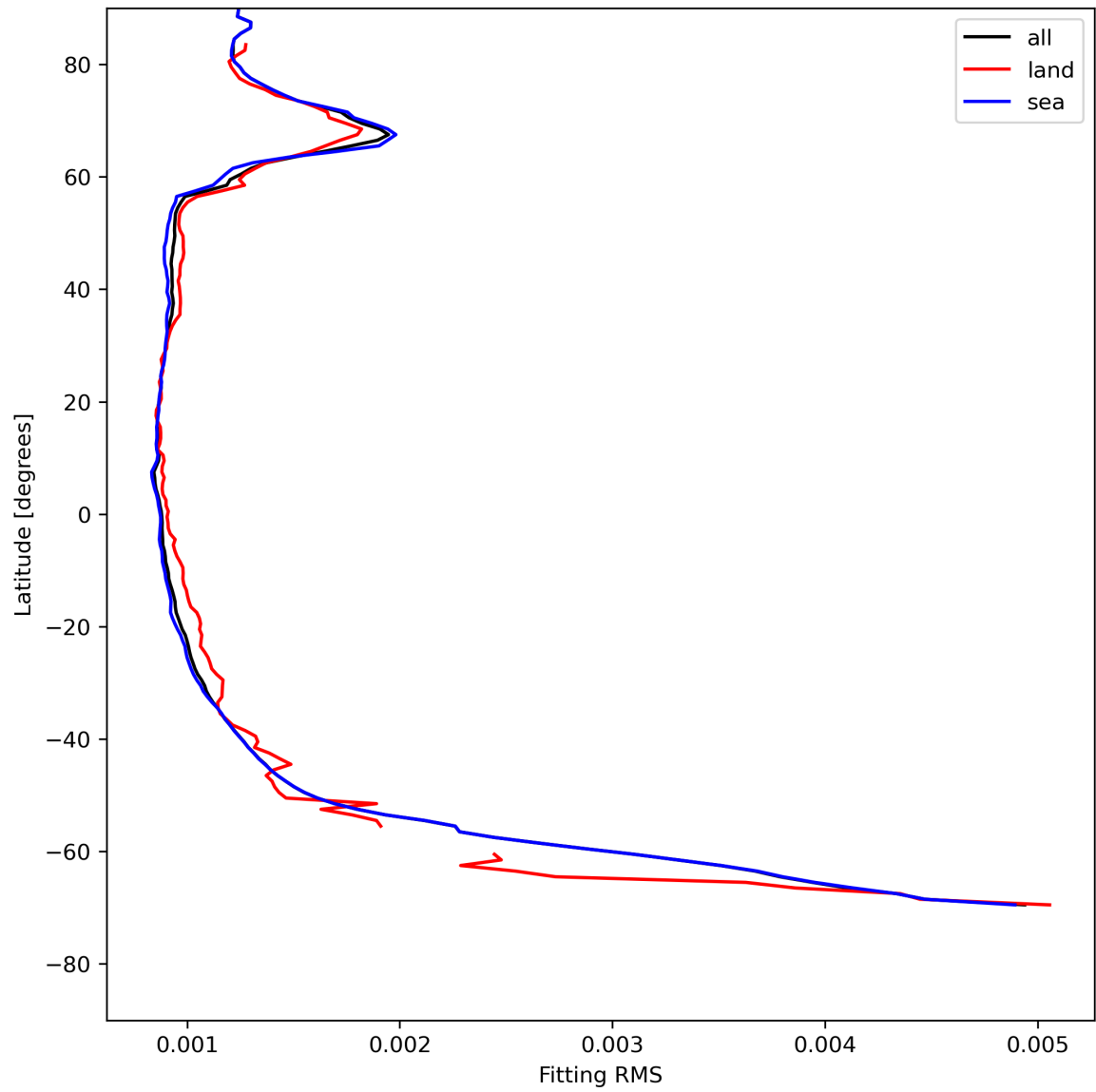
Figure 16: Zonal average of “Fitting RMS” for 2023-07-26 to 2023-07-28.
