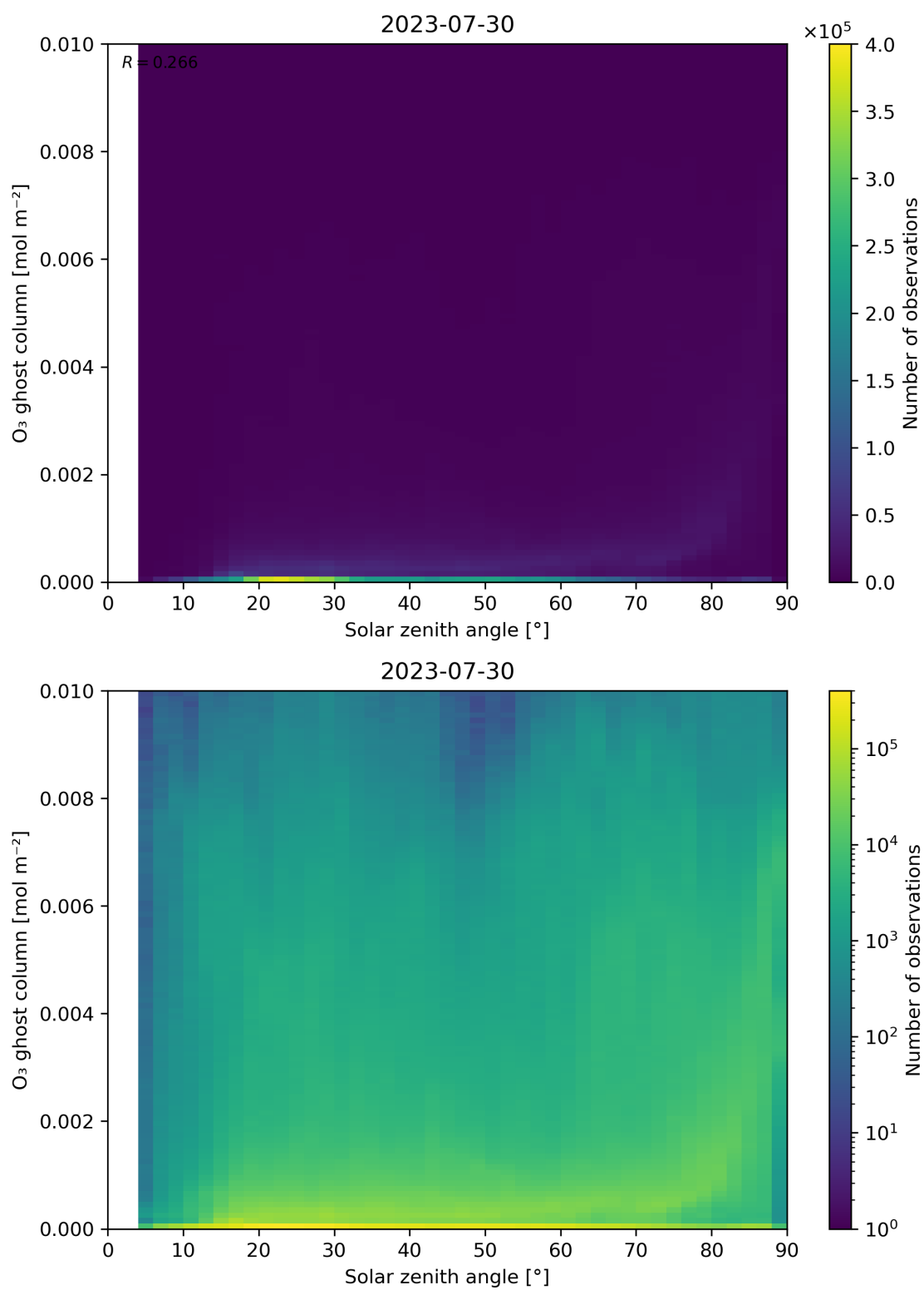
Figure 46: Scatter density plot of “Solar zenith angle” against “O 3 ghost column” for 2023-07-29 to 2023-07-31.
