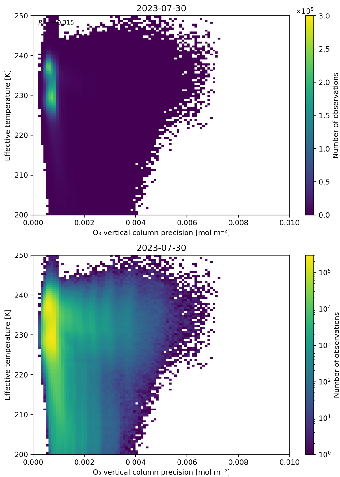
Figure 42: Scatter density plot of “O 3 vertical column precision” against “Effective temperature” for 2023-07-29 to 2023-07-31.
