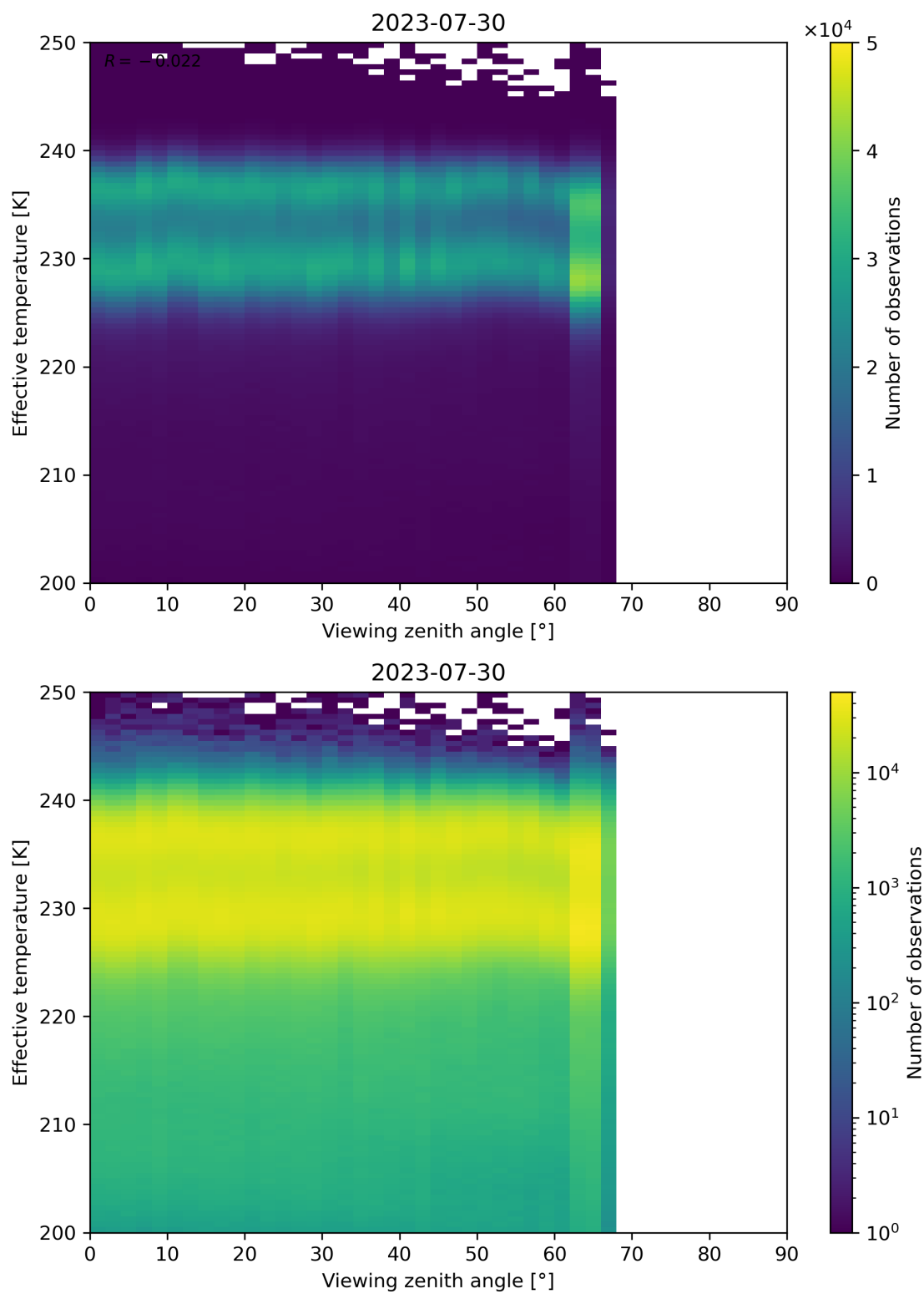
Figure 50: Scatter density plot of “Viewing zenith angle” against “Effective temperature” for 2023-07-29 to 2023-07-31.
