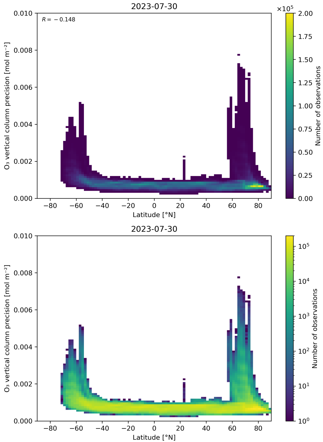
Figure 37: Scatter density plot of “Latitude” against “O 3 vertical column precision” for 2023-07-29 to 2023-07-31.
