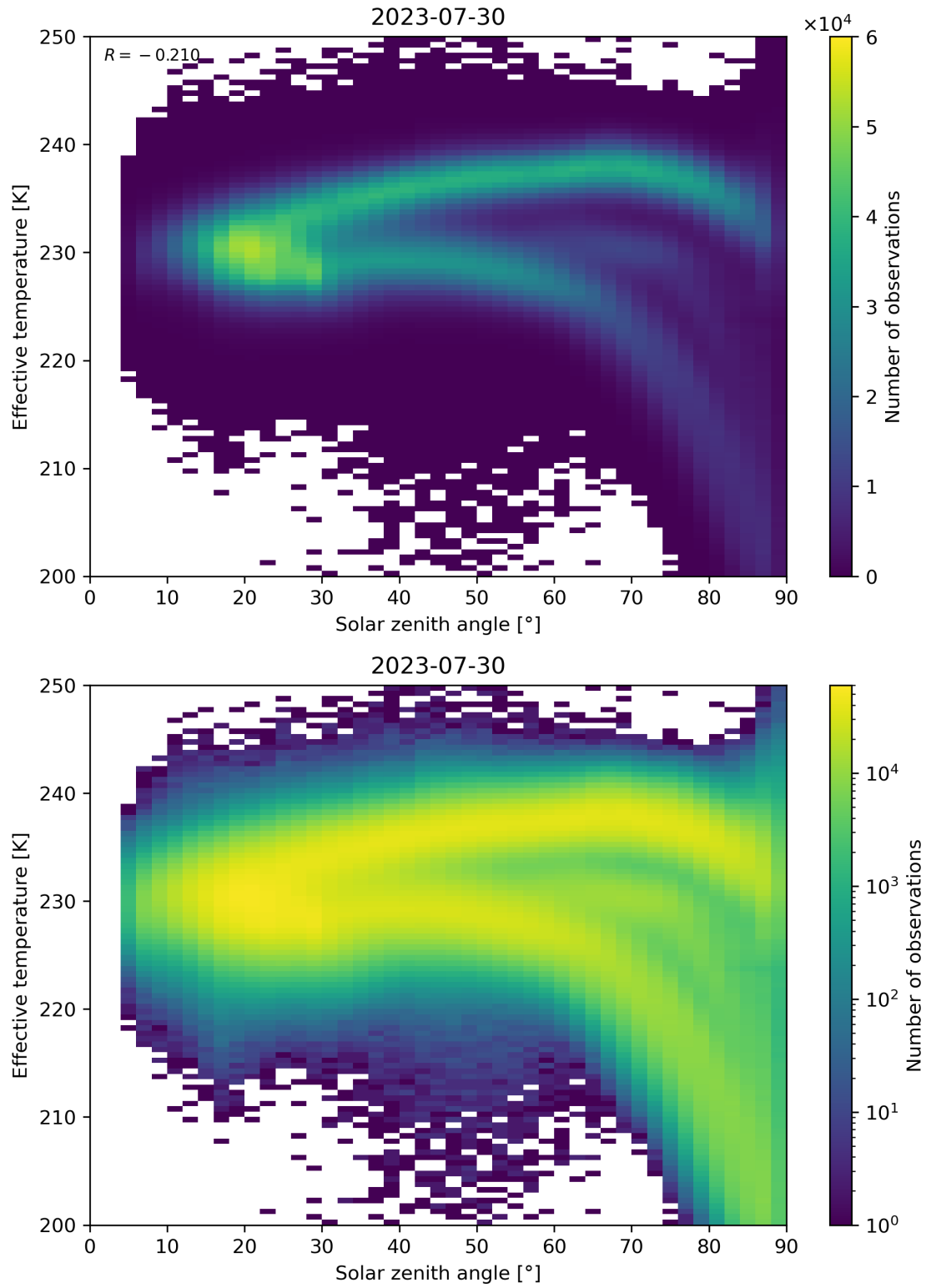
Figure 45: Scatter density plot of “Solar zenith angle” against “Effective temperature” for 2023-07-29 to 2023-07-31.
