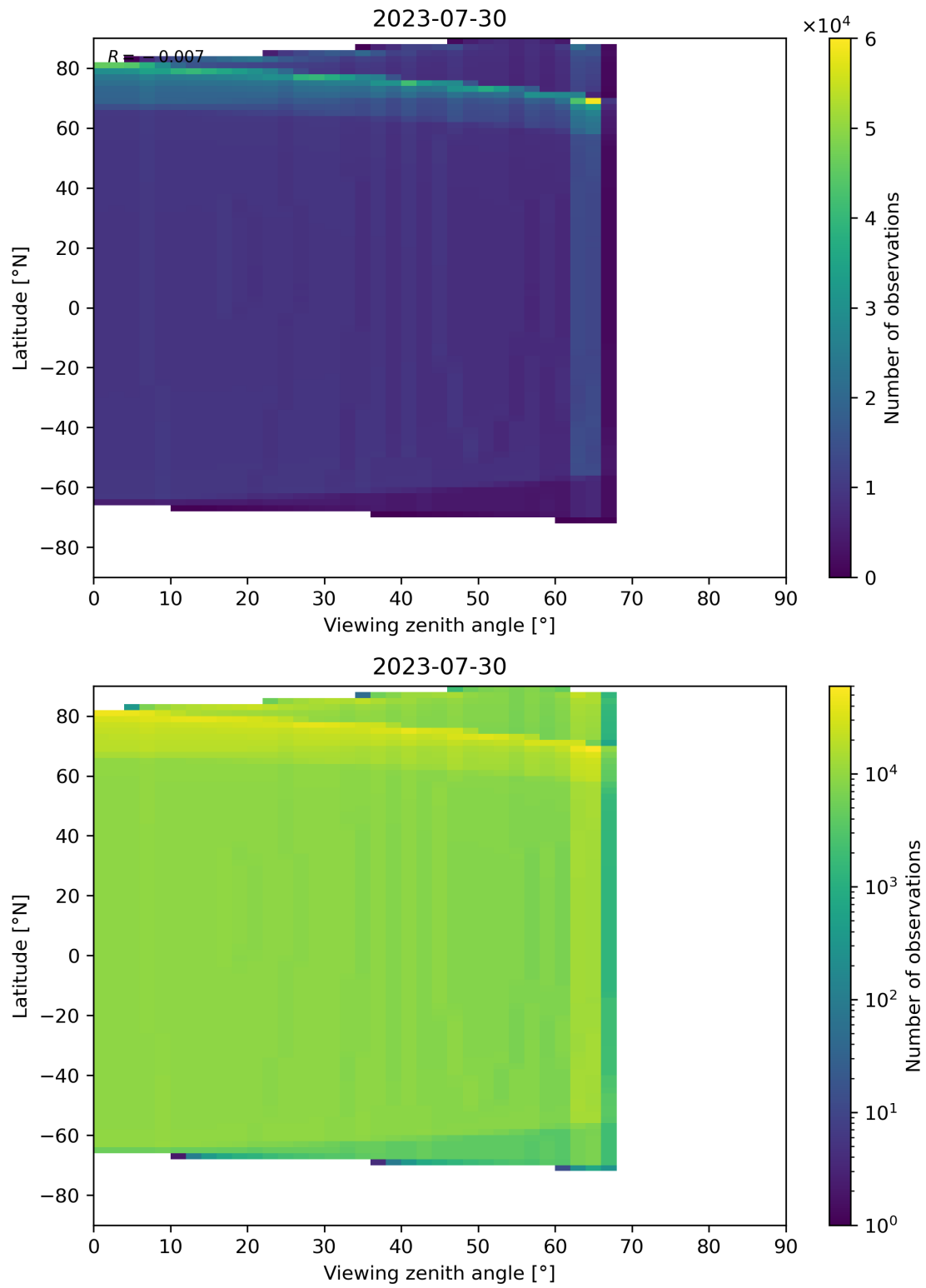
Figure 49: Scatter density plot of “Viewing zenith angle” against “Latitude” for 2023-07-29 to 2023-07-31.
