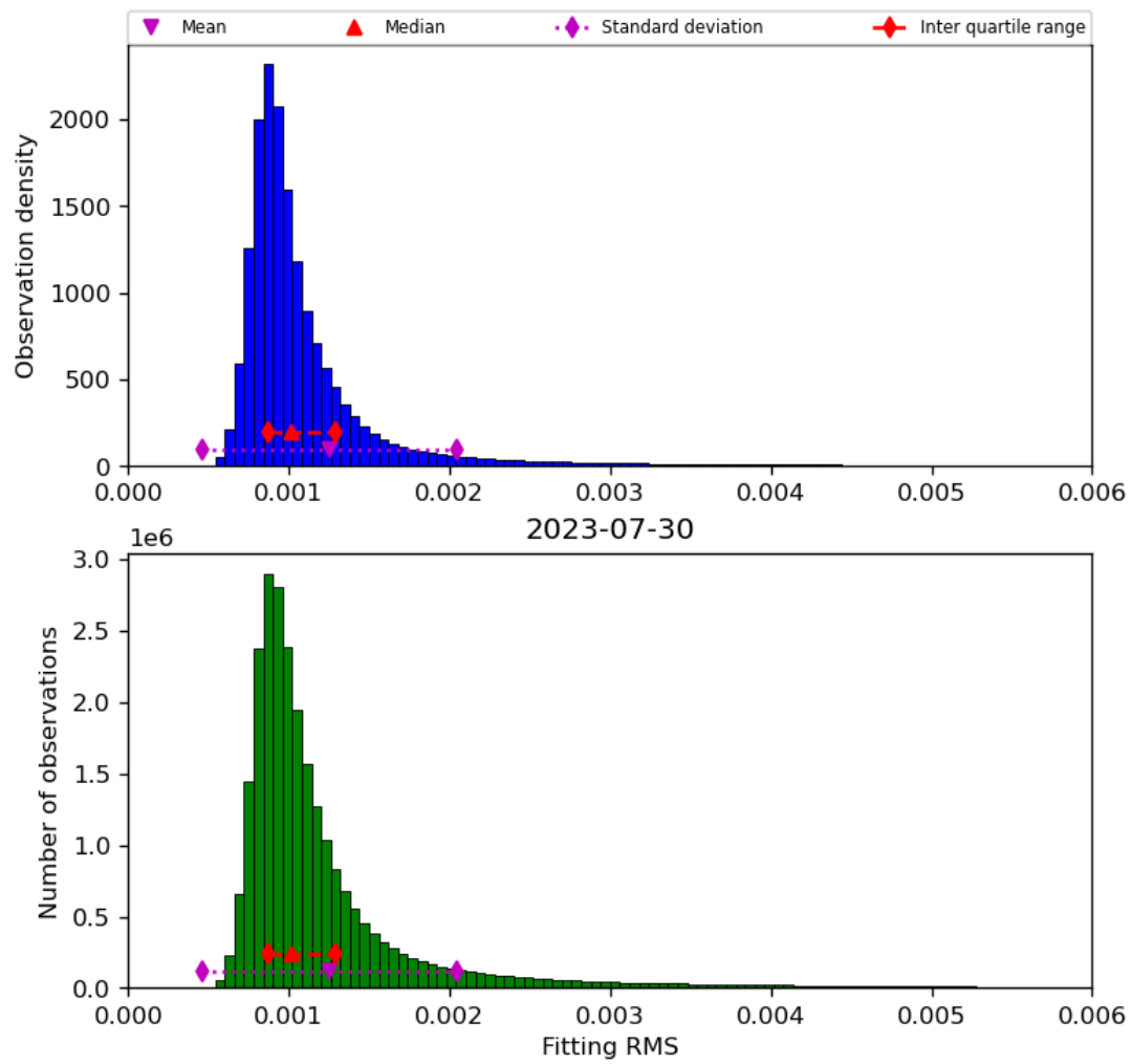
Figure 23: Histogram of “Fitting RMS” for 2023-07-29 to 2023-07-31
