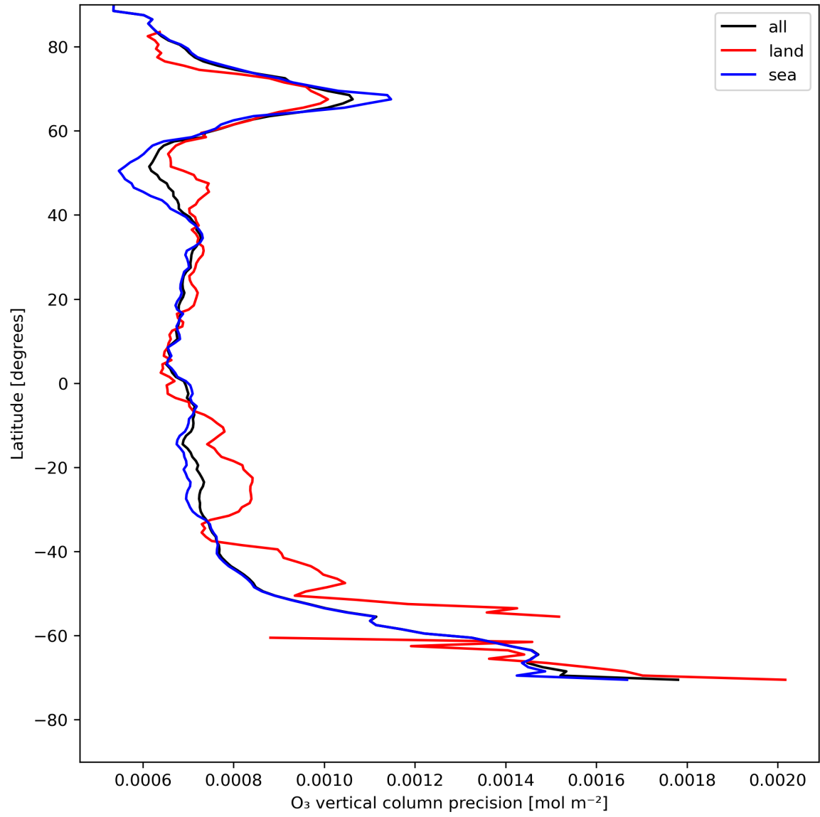
Figure 15: Zonal average of "O 3 vertical column precision" for 2023-07-29 to 2023-07-31.
