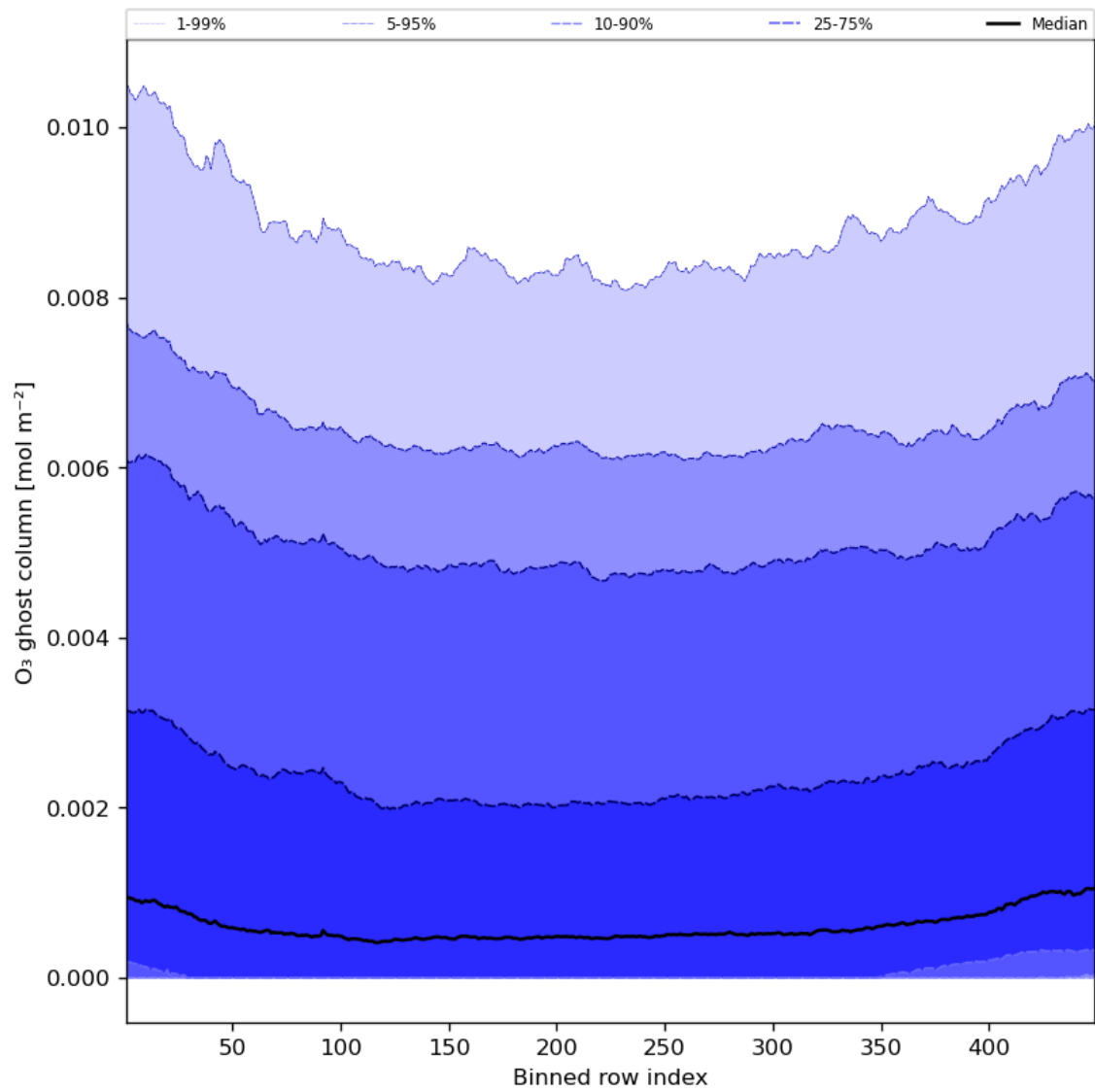
Figure 32: Along track statistics of “O 3 ghost column” for 2023-07-29 to 2023-07-31
