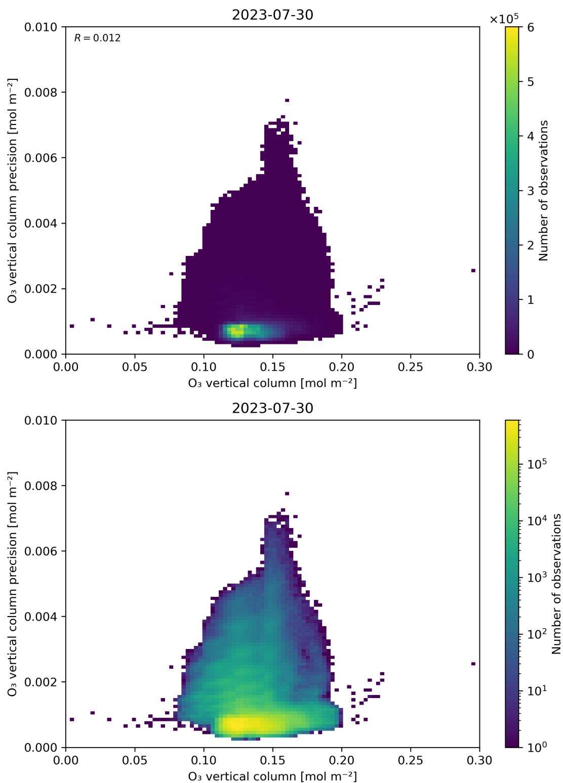
Figure 41: Scatter density plot of “O 3 vertical column” against “O 3 vertical column precision” for 2023-07-29 to 2023-07-31.
