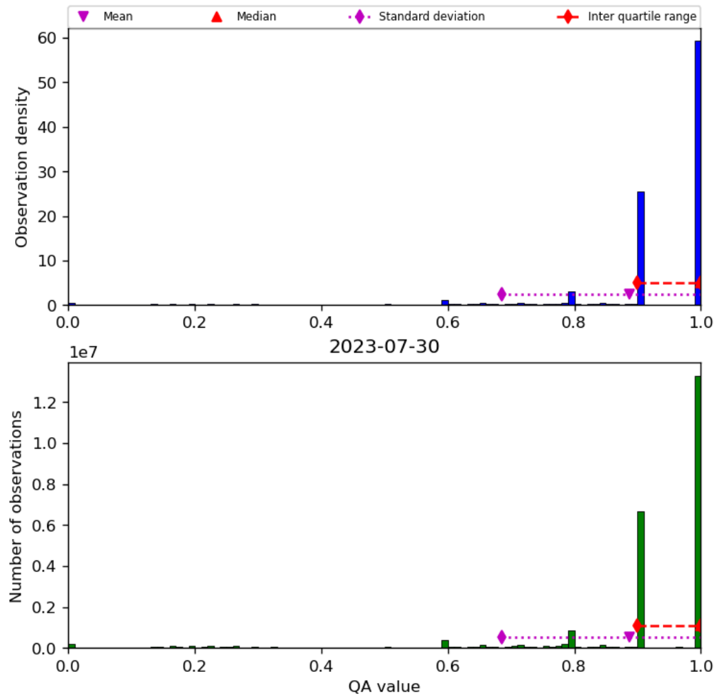
Figure 20: Histogram of “QA value” for 2023-07-29 to 2023-07-31
