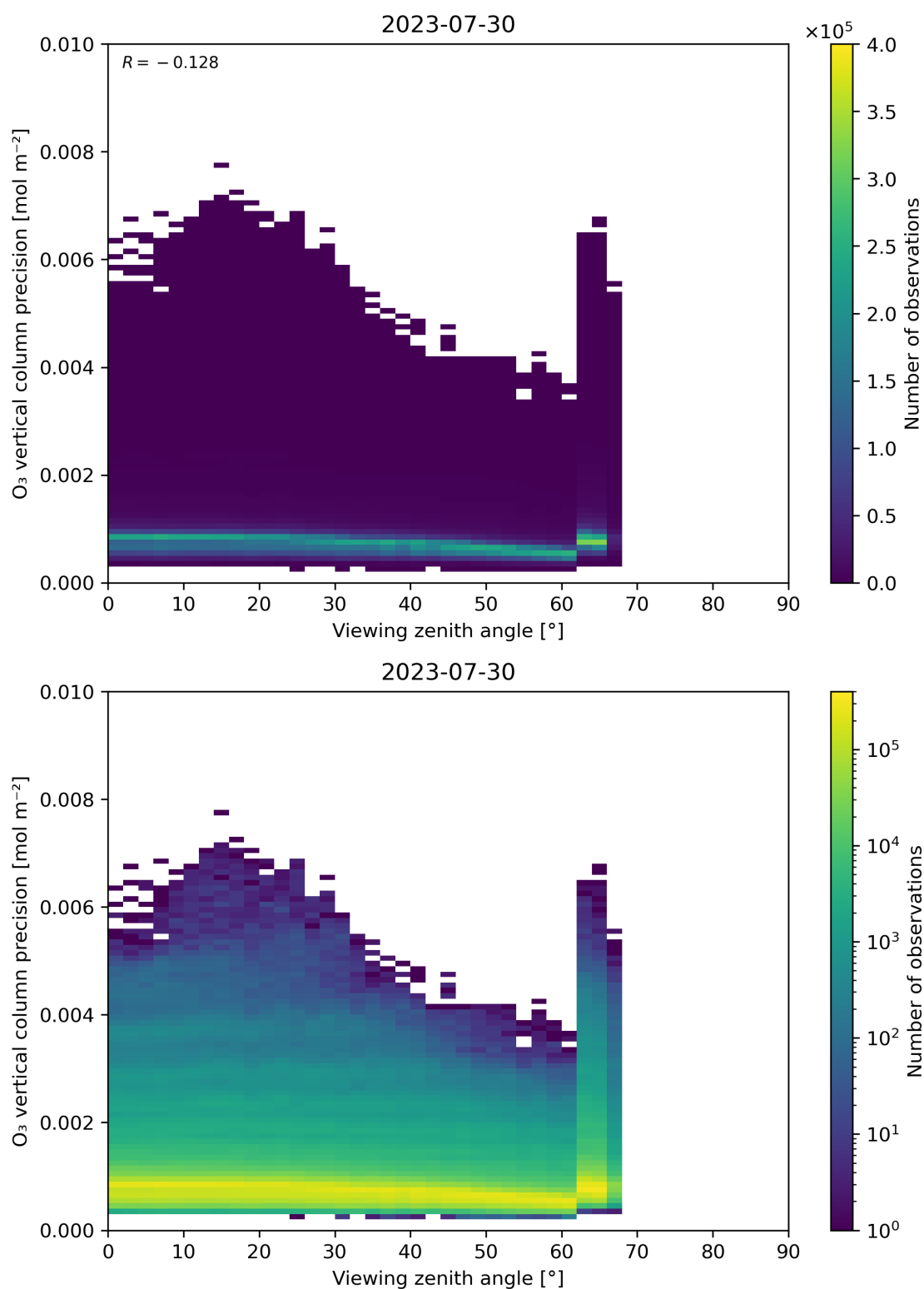
Figure 53: Scatter density plot of “Viewing zenith angle” against “O 3 vertical column precision” for 2023-07-29 to 2023-07-31.
