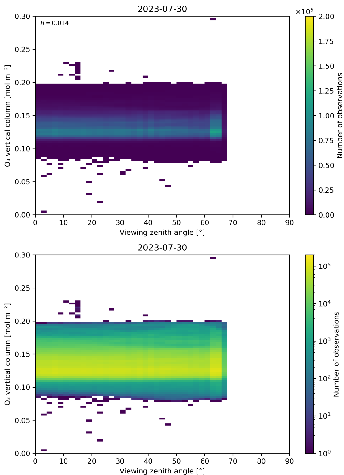
Figure 52: Scatter density plot of “Viewing zenith angle” against “O 3 vertical column” for 2023-07-29 to 2023-07-31.
