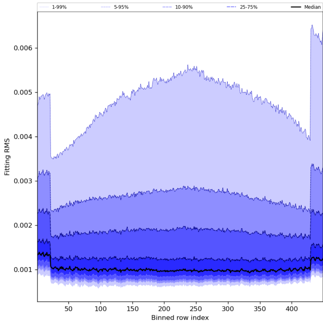
Figure 30: Along track statistics of “Fitting RMS” for 2023-07-29 to 2023-07-31
