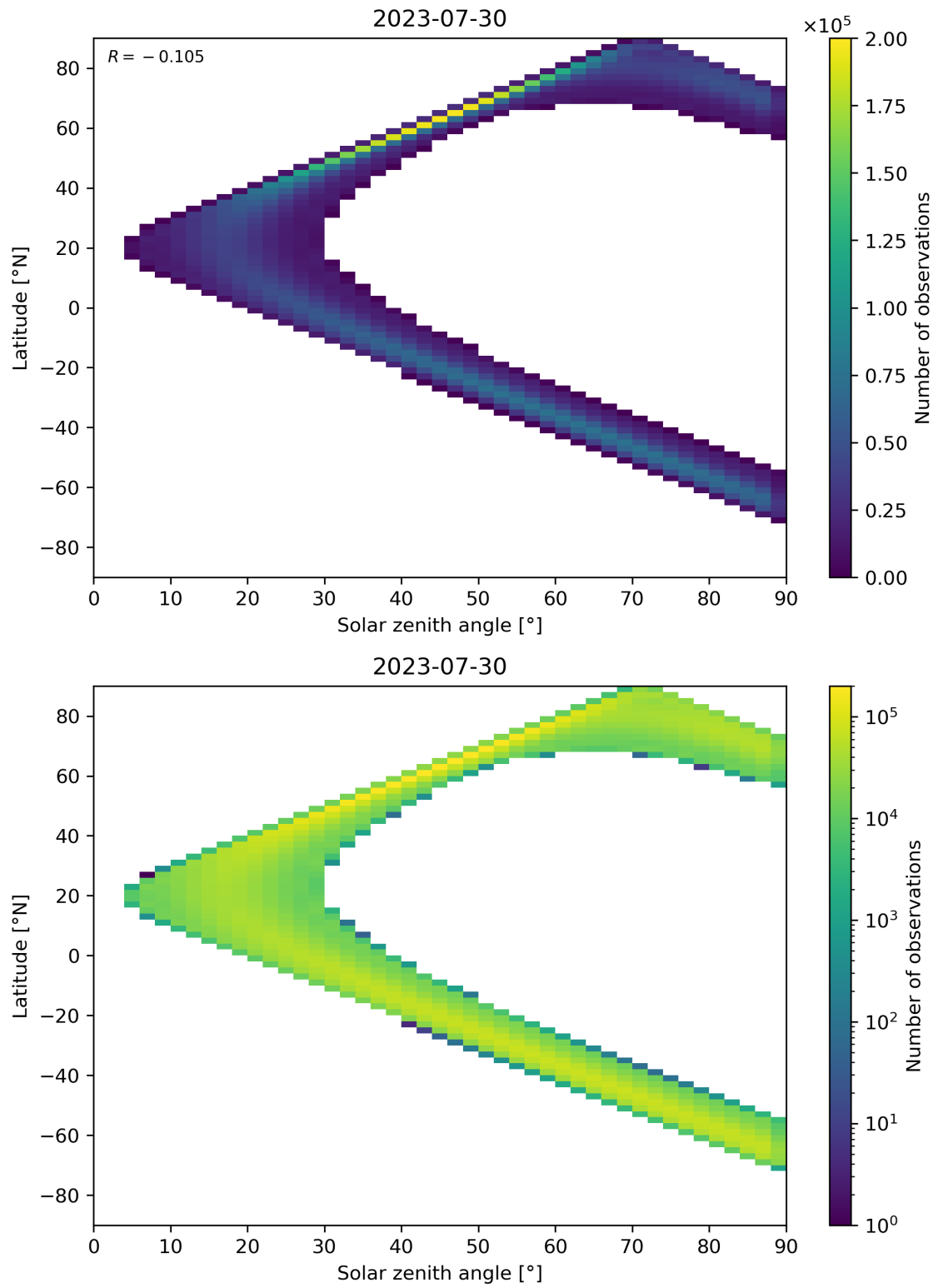
Figure 44: Scatter density plot of “Solar zenith angle” against “Latitude” for 2023-07-29 to 2023-07-31.
