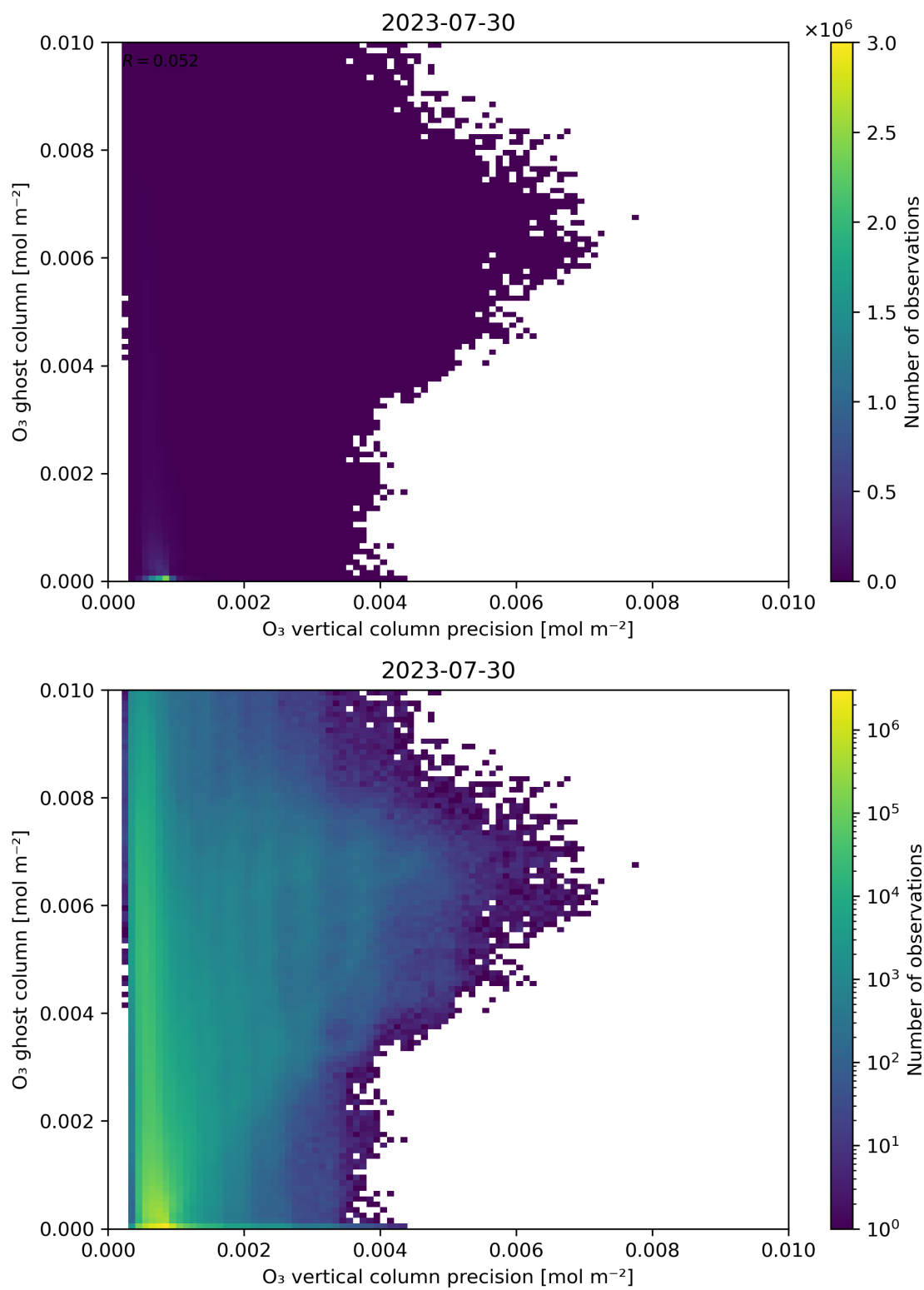
Figure 43: Scatter density plot of “ O_3 vertical column precision” against “ O_3 ghost column” for 2023-07-29 to 2023-07-31.
