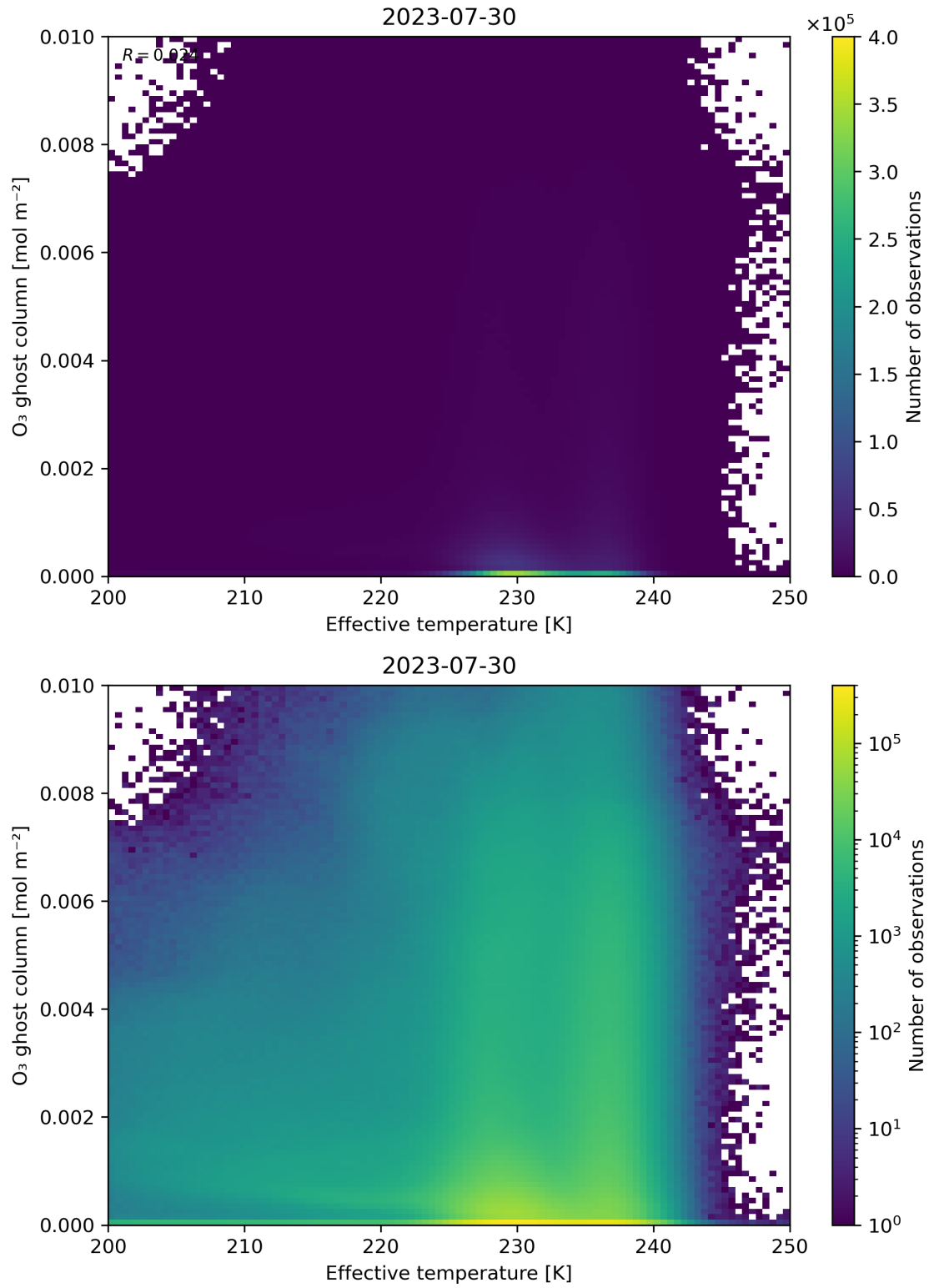
Figure 38: Scatter density plot of “Effective temperature” against “O 3 ghost column” for 2023-07-29 to 2023-07-31.
