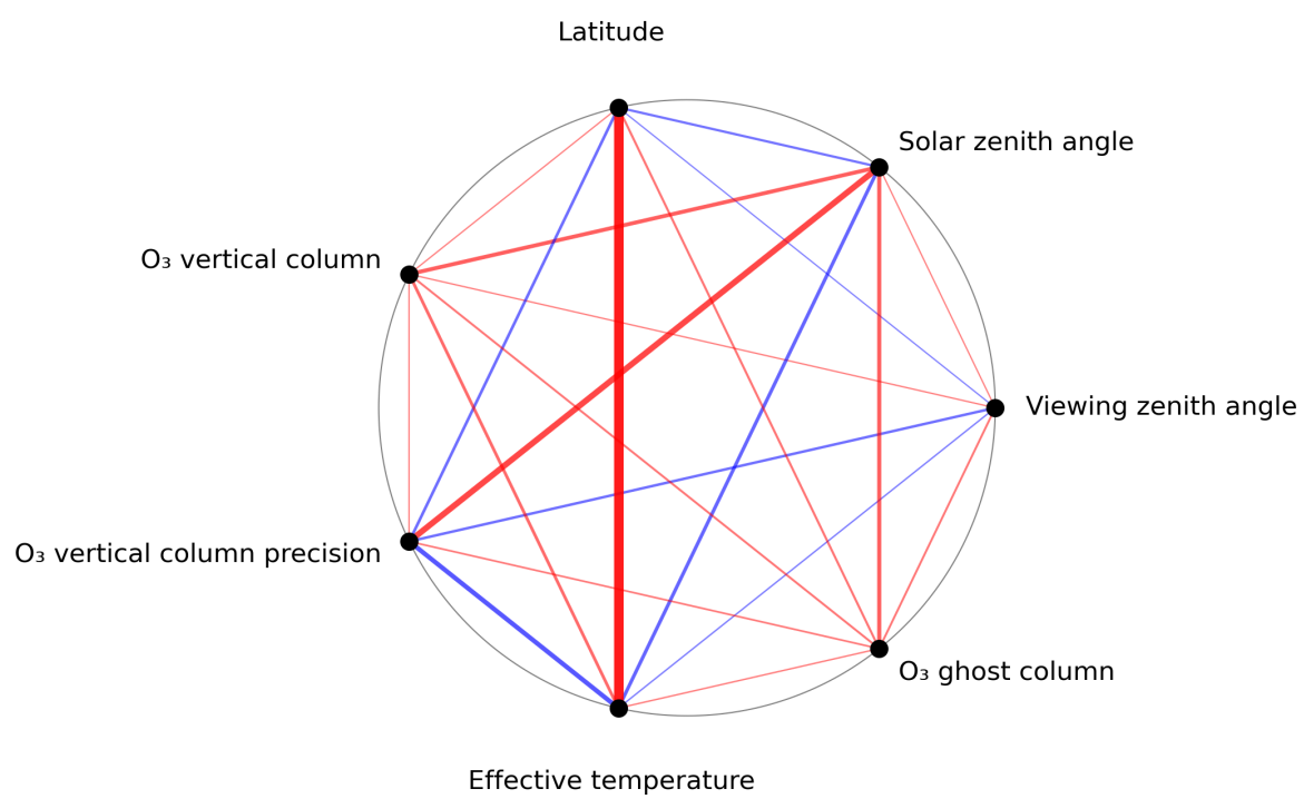
Figure 1: Map of correlation graph for 2023-07-29 to 2023-07-31.
