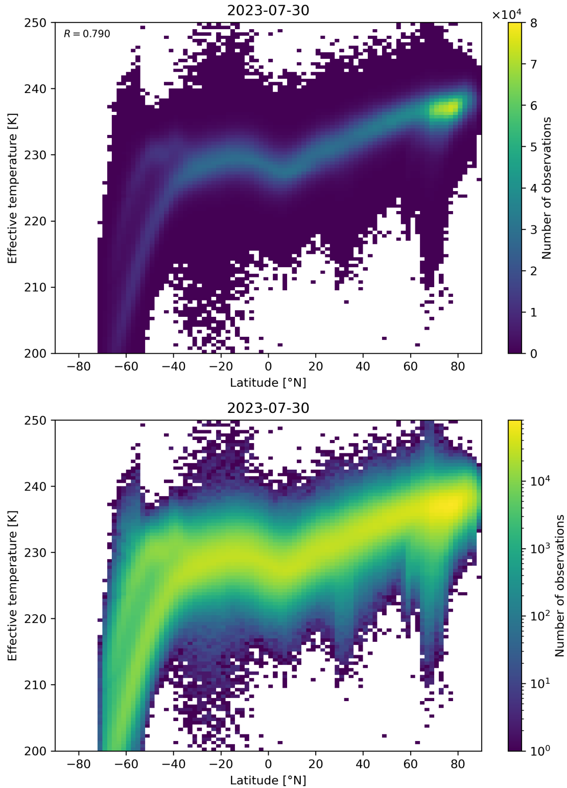
Figure 34: Scatter density plot of “Latitude” against “Effective temperature” for 2023-07-29 to 2023-07-31.
