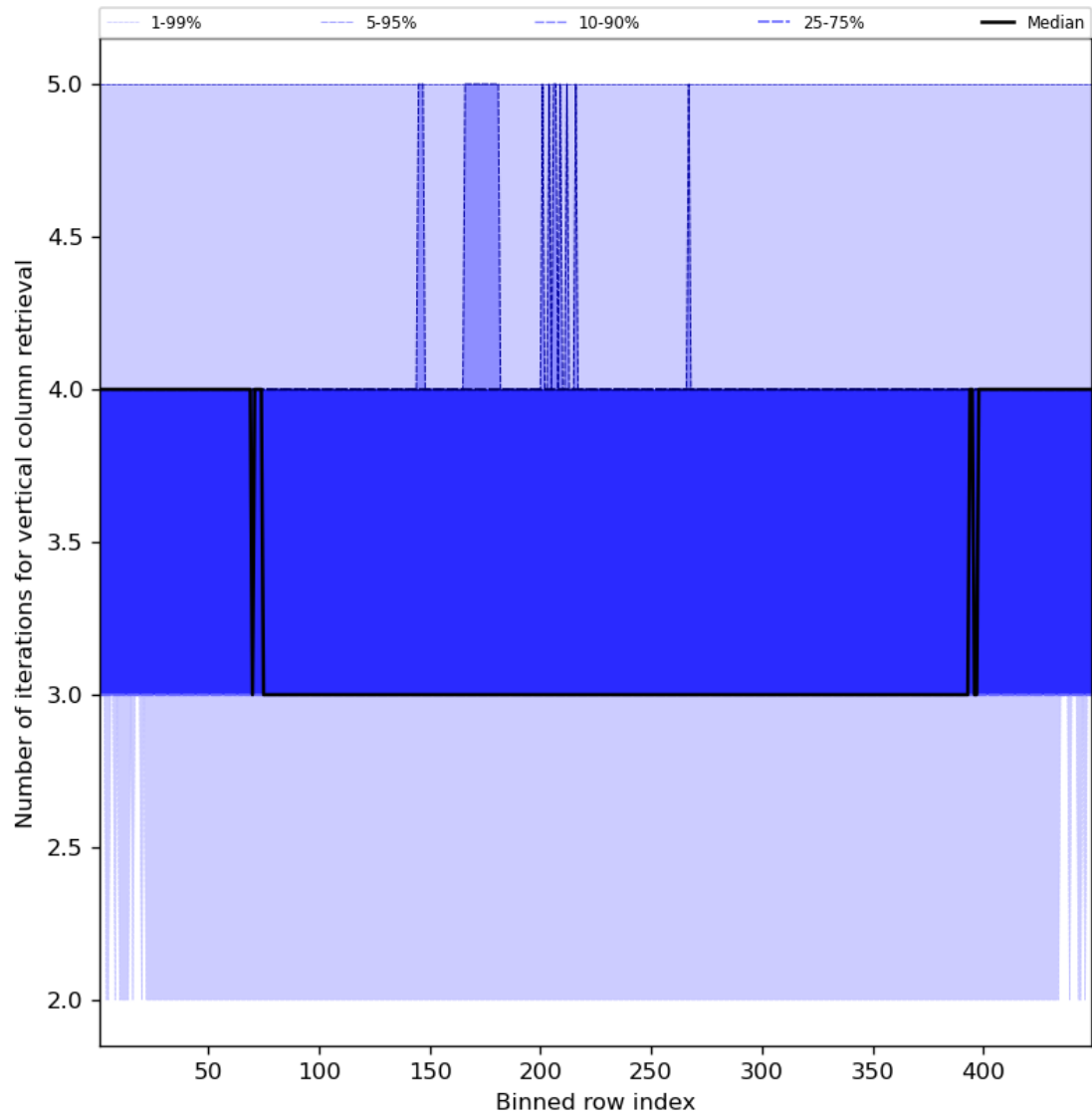
Figure 33: Along track statistics of “Number of iterations for vertical column retrieval” for 2023-07-29 to 2023-07-31
