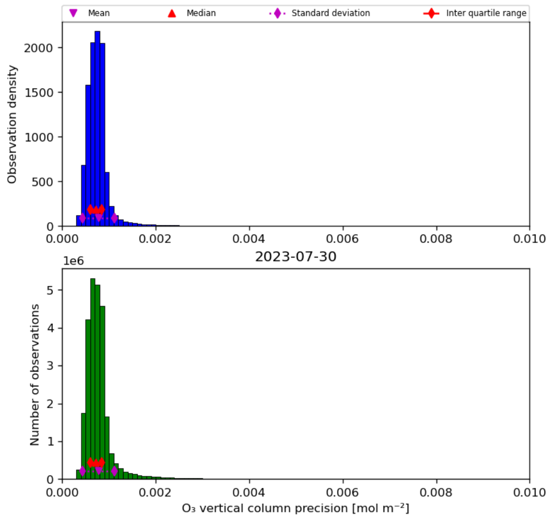
Figure 22: Histogram of “O 3 vertical column precision” for 2023-07-29 to 2023-07-31
