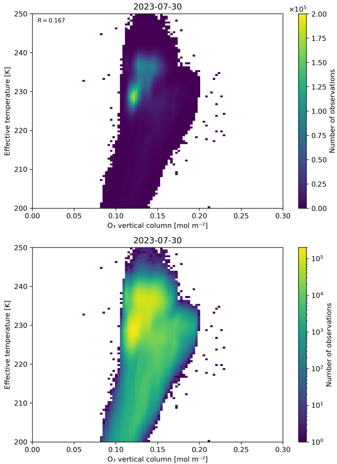
Figure 39: Scatter density plot of “O 3 vertical column” against “Effective temperature” for 2023-07-29 to 2023-07-31.
