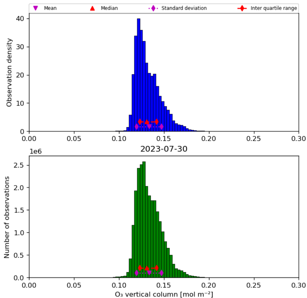
Figure 21: Histogram of “O 3 vertical column” for 2023-07-29 to 2023-07-31
