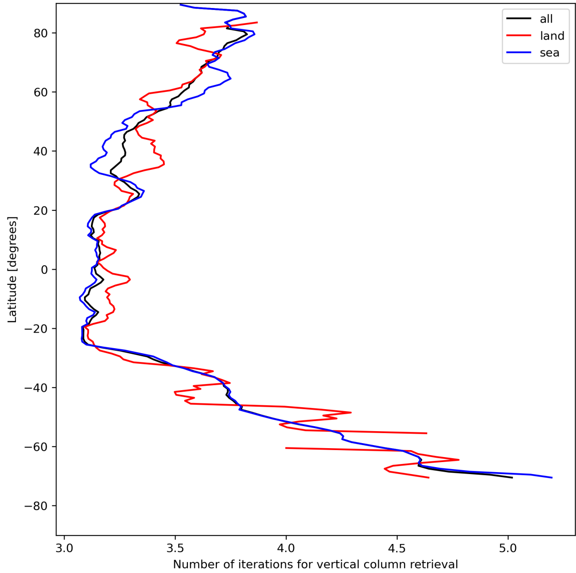
Figure 19: Zonal average of “Number of iterations for vertical column retrieval” for 2023-07-29 to 2023-07-31.
