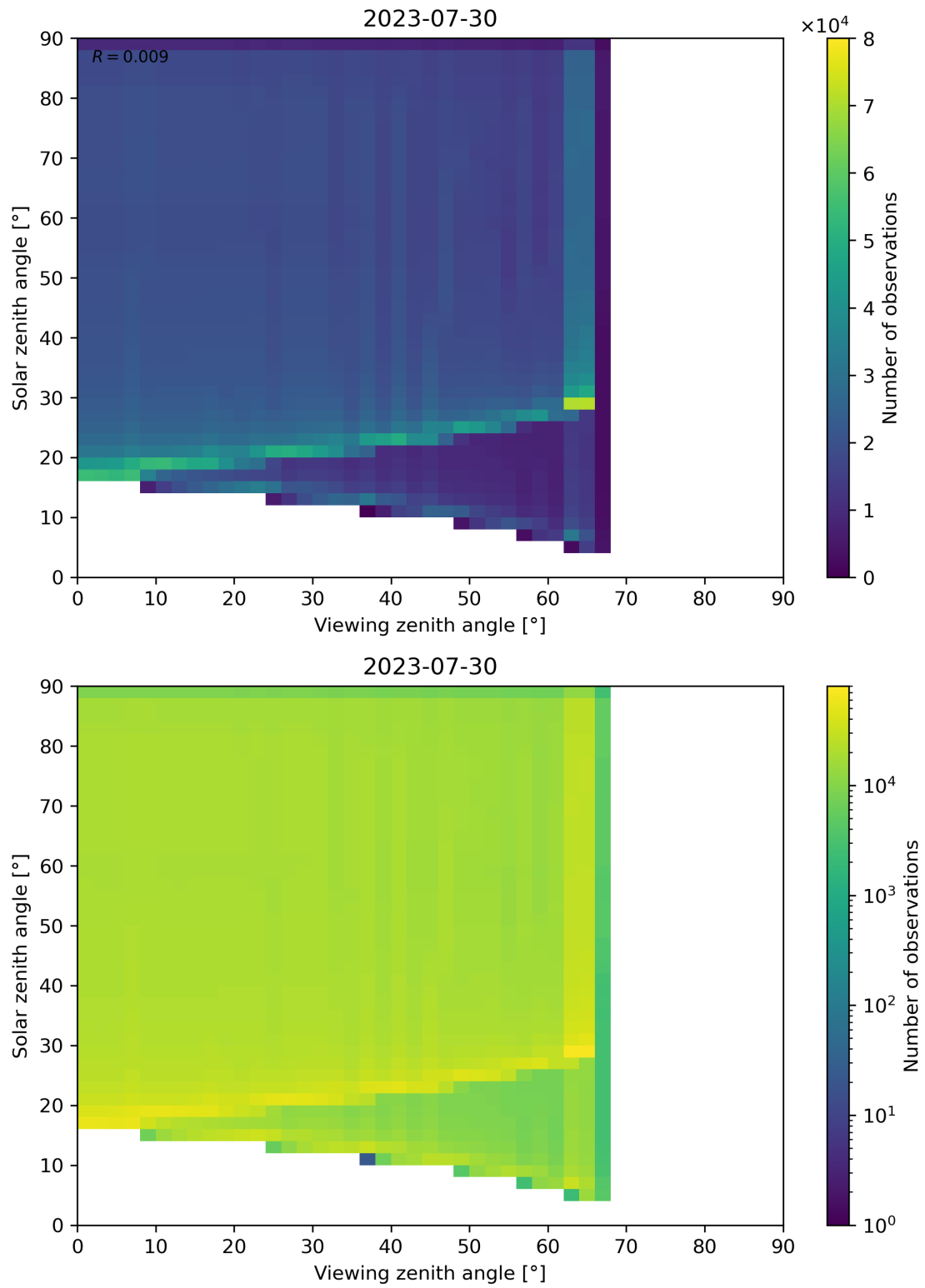
Figure 54: Scatter density plot of “Viewing zenith angle” against “Solar zenith angle” for 2023-07-29 to 2023-07-31.
