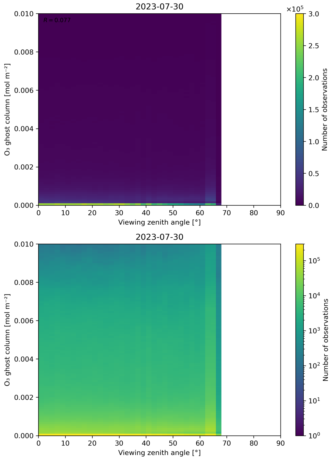
Figure 51: Scatter density plot of “Viewing zenith angle” against “O 3 ghost column” for 2023-07-29 to 2023-07-31.
