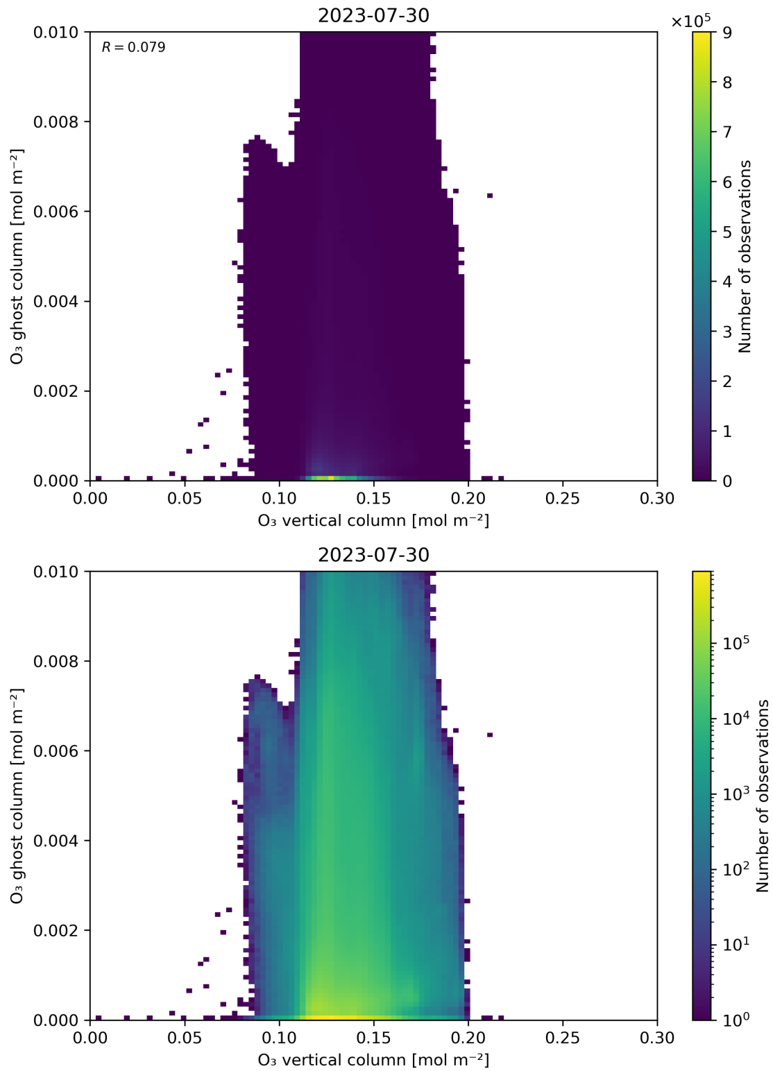
Figure 40: Scatter density plot of “O 3 vertical column” against “O 3 ghost column” for 2023-07-29 to 2023-07-31.
