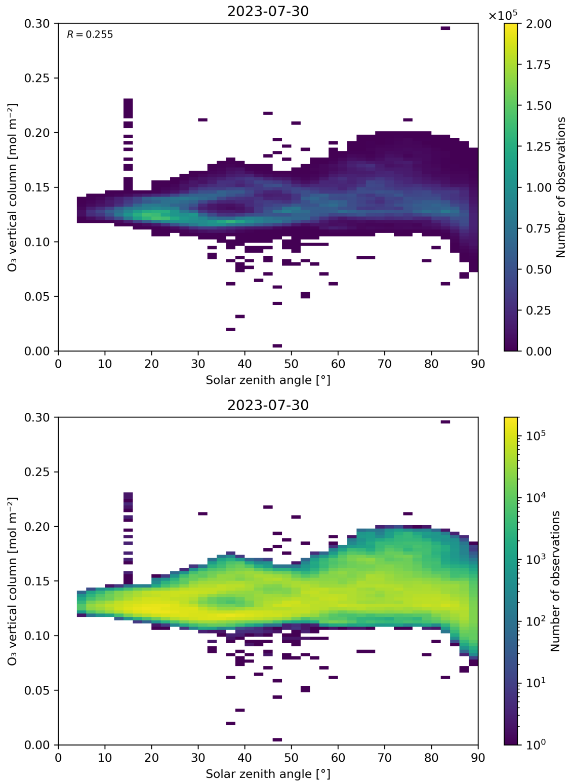
Figure 47: Scatter density plot of “Solar zenith angle” against “O 3 vertical column” for 2023-07-29 to 2023-07-31.
