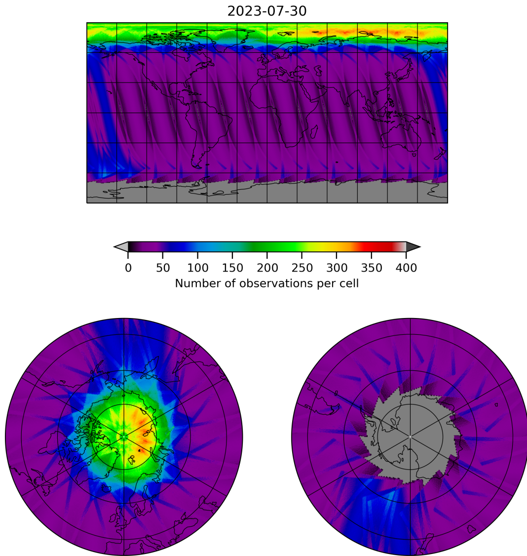
Figure 12: Map of the number of observations for 2023-07-29 to 2023-07-31
