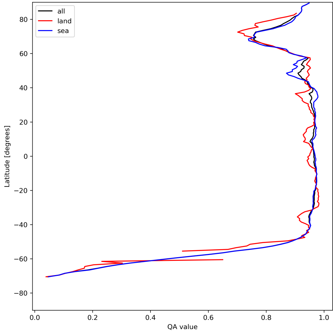
Figure 13: Zonal average of “QA value” for 2023-07-29 to 2023-07-31.
