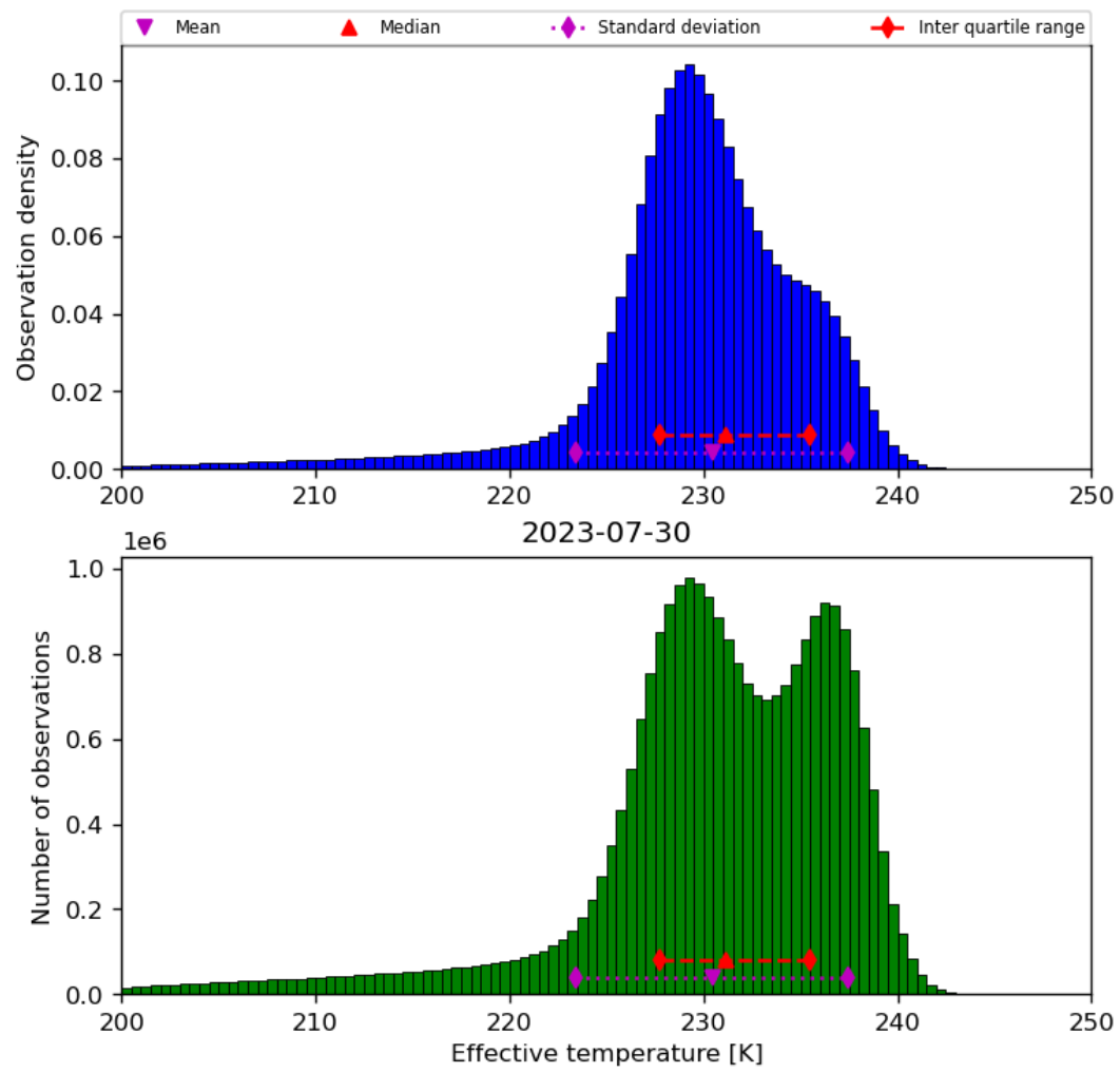
Figure 24: Histogram of “Effective temperature” for 2023-07-29 to 2023-07-31
