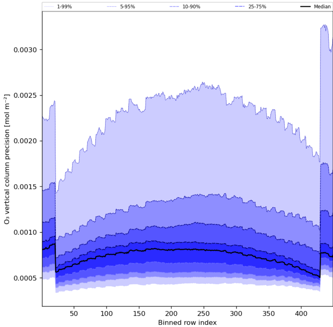
Figure 29: Along track statistics of “O 3 vertical column precision” for 2023-07-29 to 2023-07-31
