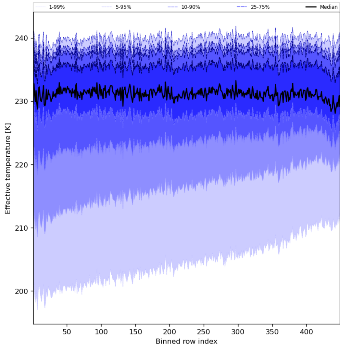
Figure 31: Along track statistics of “Effective temperature” for 2023-07-29 to 2023-07-31
