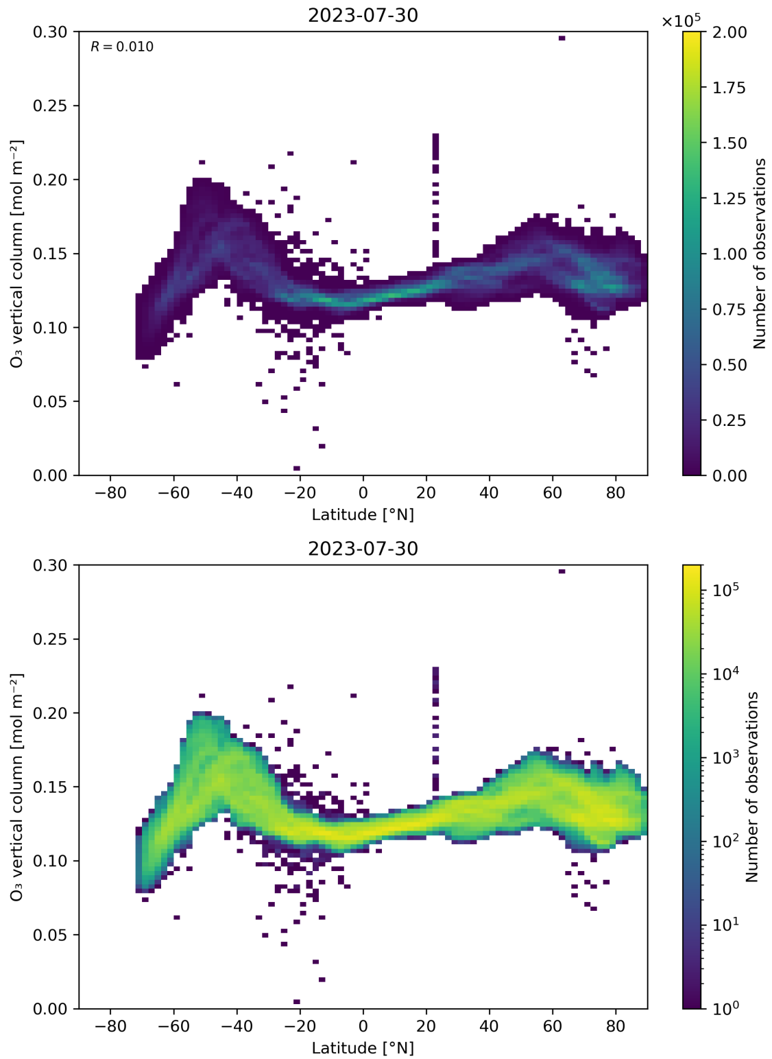
Figure 36: Scatter density plot of “Latitude” against “O 3 vertical column” for 2023-07-29 to 2023-07-31.
