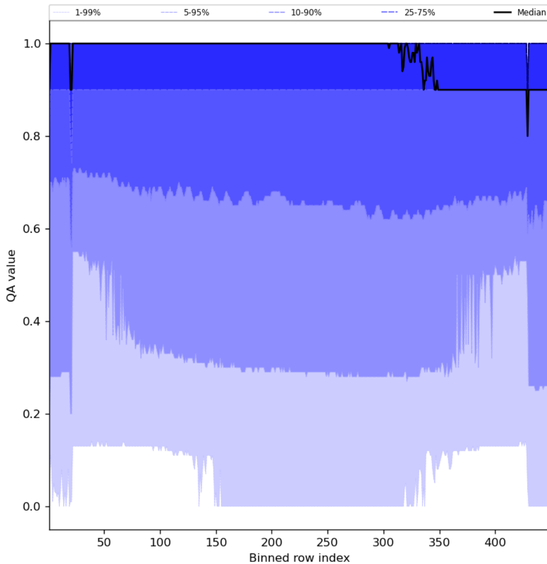
Figure 27: Along track statistics of “QA value” for 2023-07-29 to 2023-07-31
