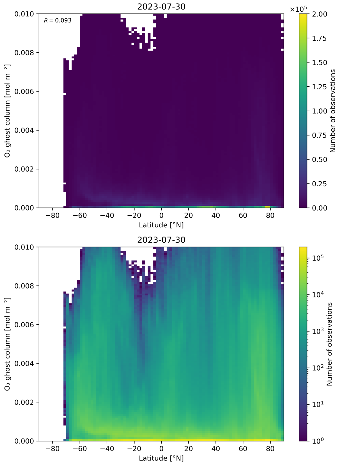
Figure 35: Scatter density plot of “Latitude” against “O 3 ghost column” for 2023-07-29 to 2023-07-31.
