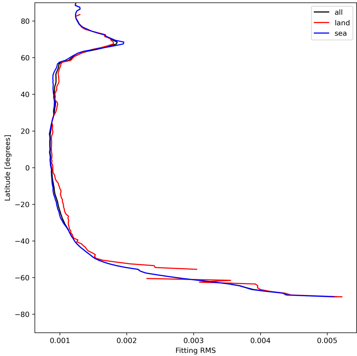
Figure 16: Zonal average of “Fitting RMS” for 2023-07-29 to 2023-07-31.
