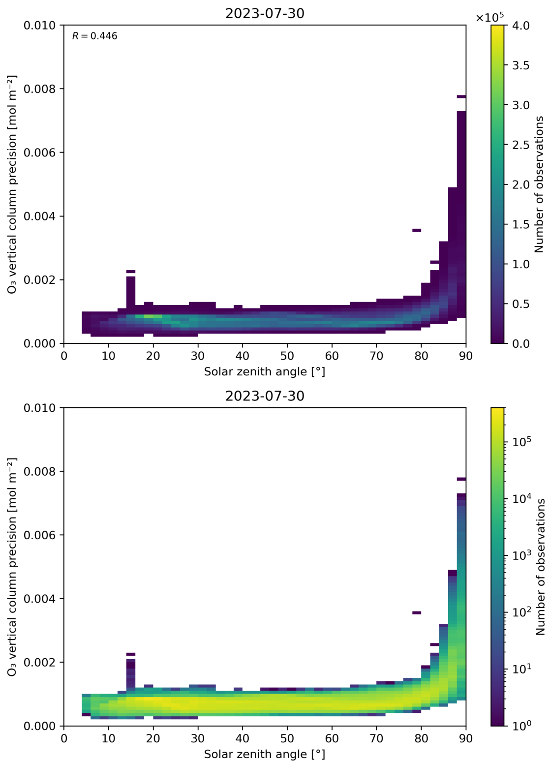
Figure 48: Scatter density plot of “Solar zenith angle” against “O 3 vertical column precision” for 2023-07-29 to 2023-07-31.
