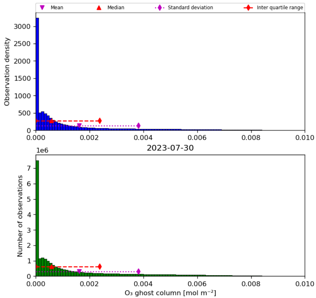
Figure 25: Histogram of "O 3 ghost column" for 2023-07-29 to 2023-07-31
