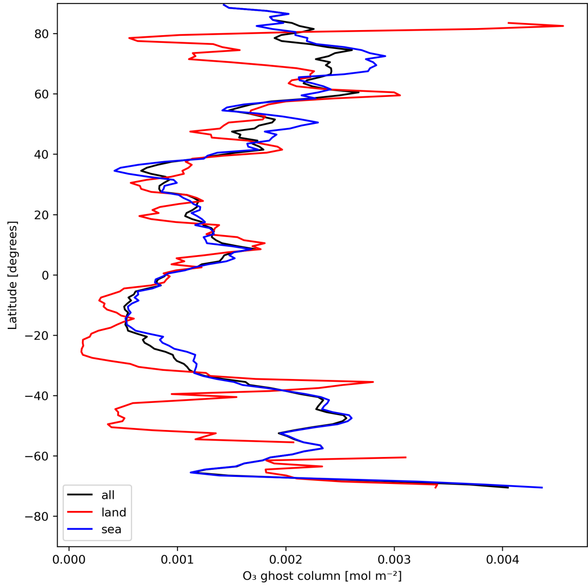
Figure 18: Zonal average of “O 3 ghost column” for 2023-07-29 to 2023-07-31.
