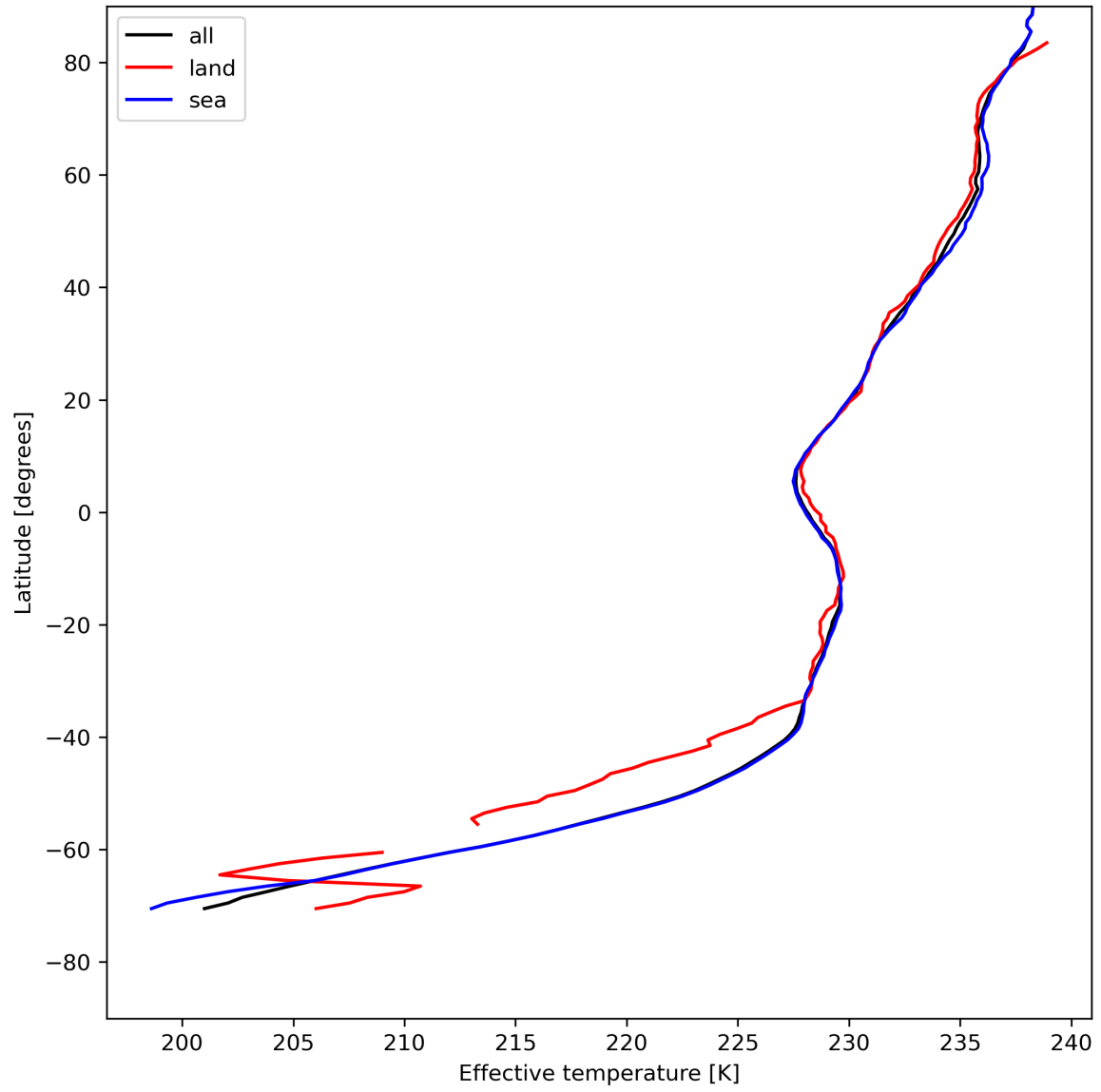
Figure 17: Zonal average of “Effective temperature” for 2023-07-29 to 2023-07-31.
