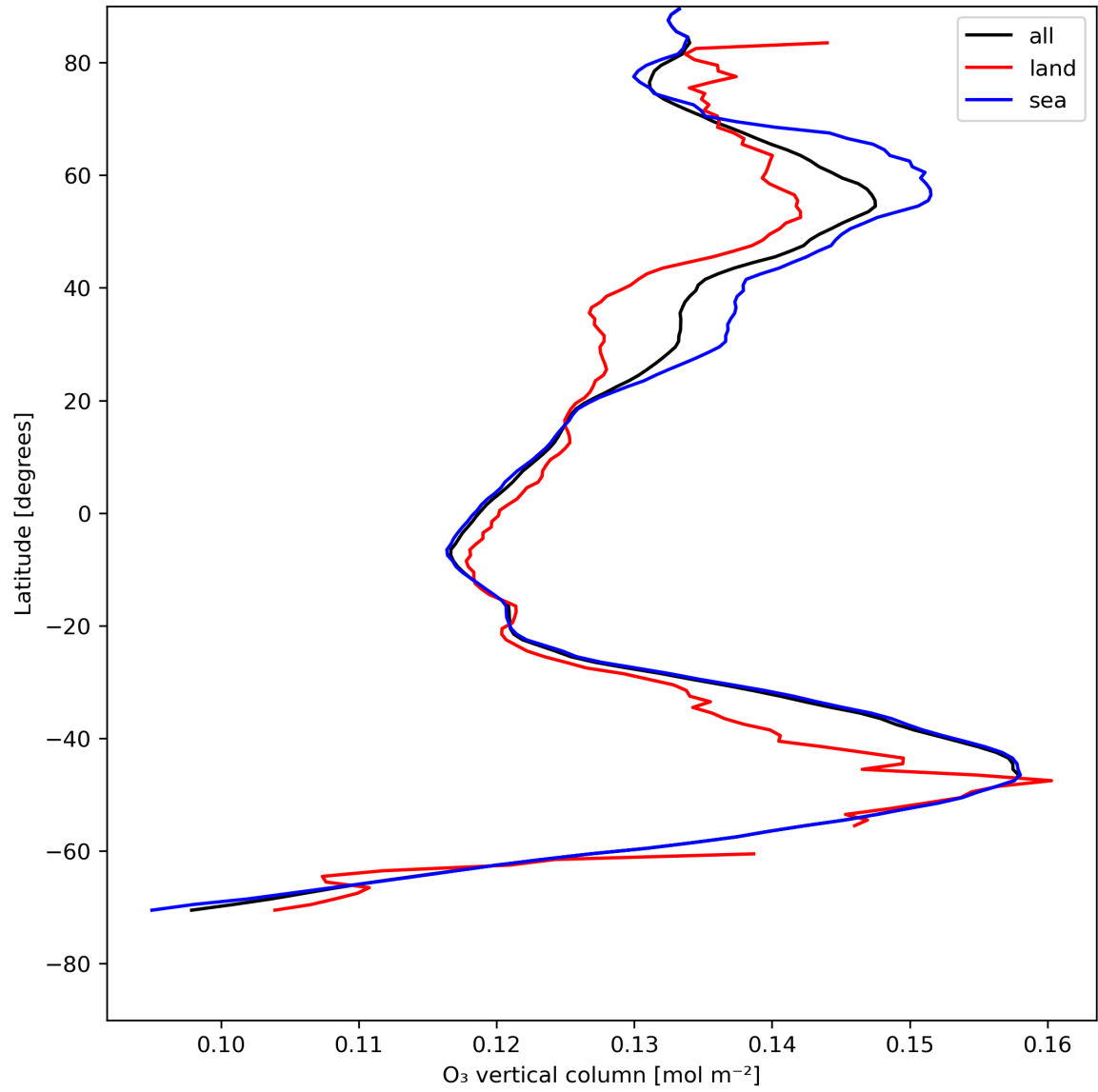
Figure 14: Zonal average of “O 3 vertical column” for 2023-07-29 to 2023-07-31.
