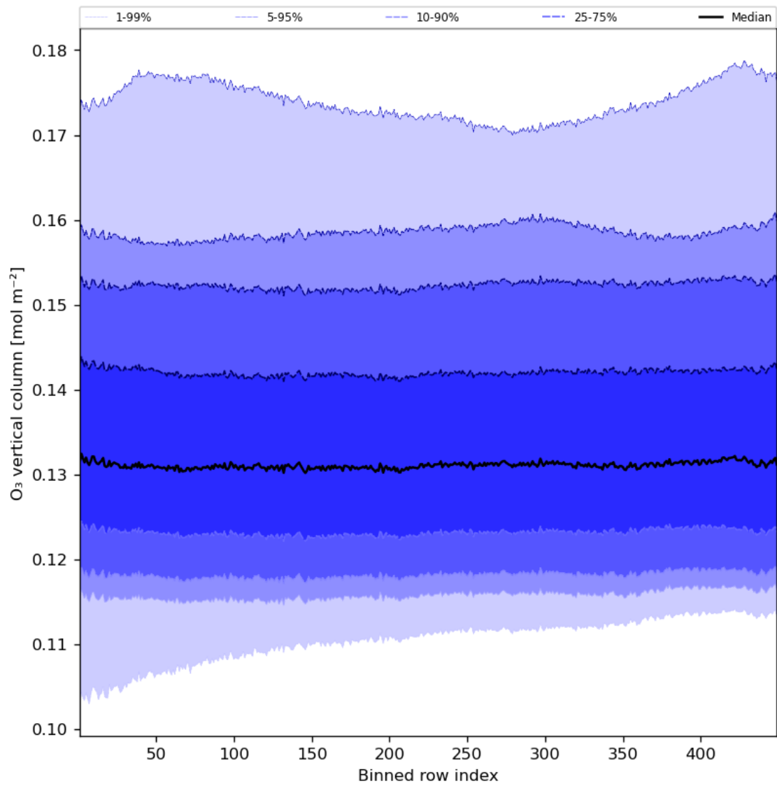
Figure 28: Along track statistics of “O 3 vertical column” for 2023-07-29 to 2023-07-31
