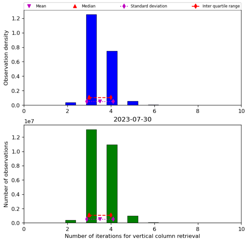
Figure 26: Histogram of “Number of iterations for vertical column retrieval” for 2023-07-29 to 2023-07-31
