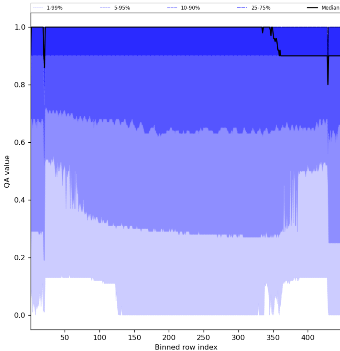
Figure 27: Along track statistics of “QA value” for 2023-07-30 to 2023-08-01
