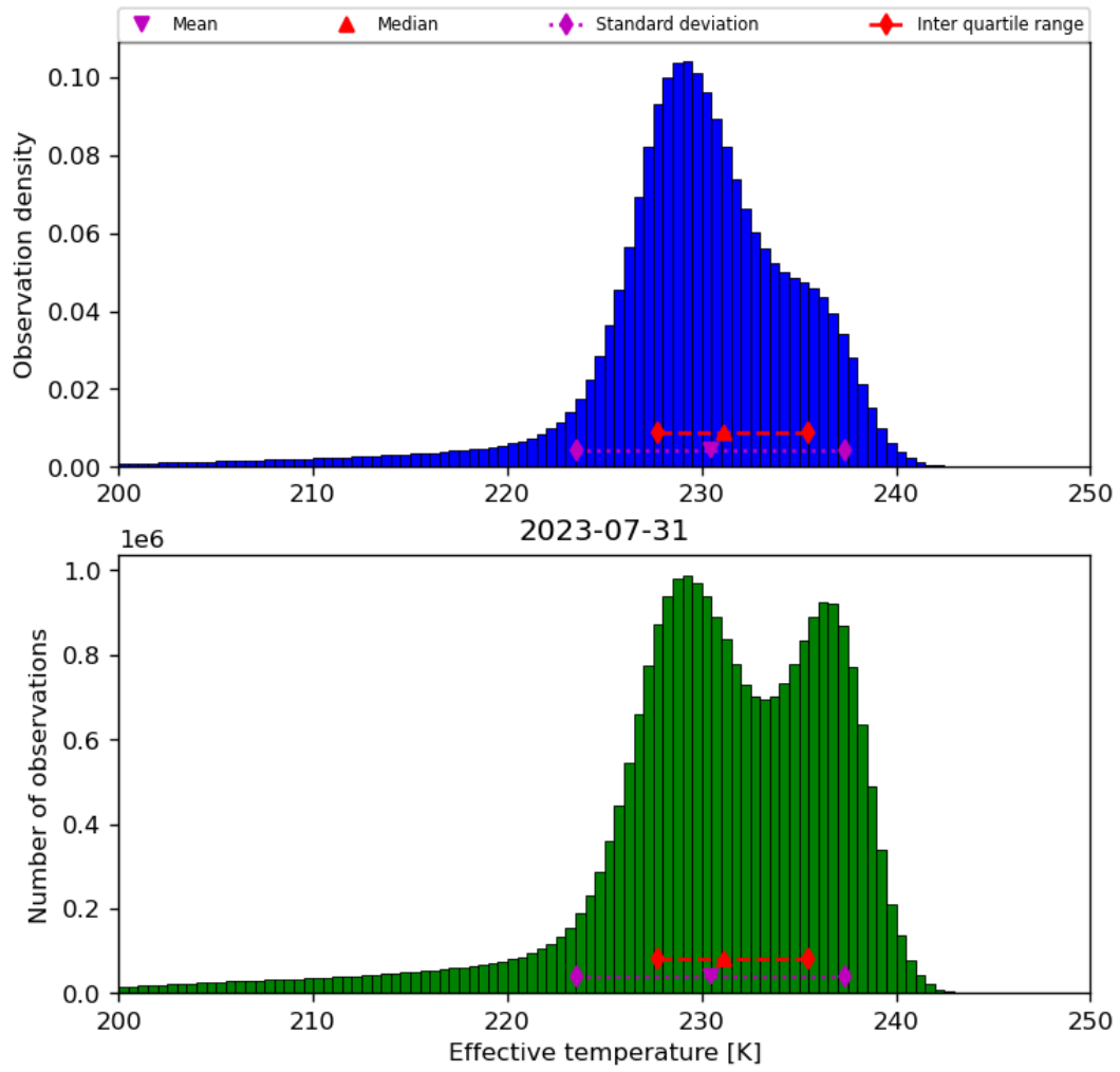
Figure 24: Histogram of “Effective temperature” for 2023-07-30 to 2023-08-01
