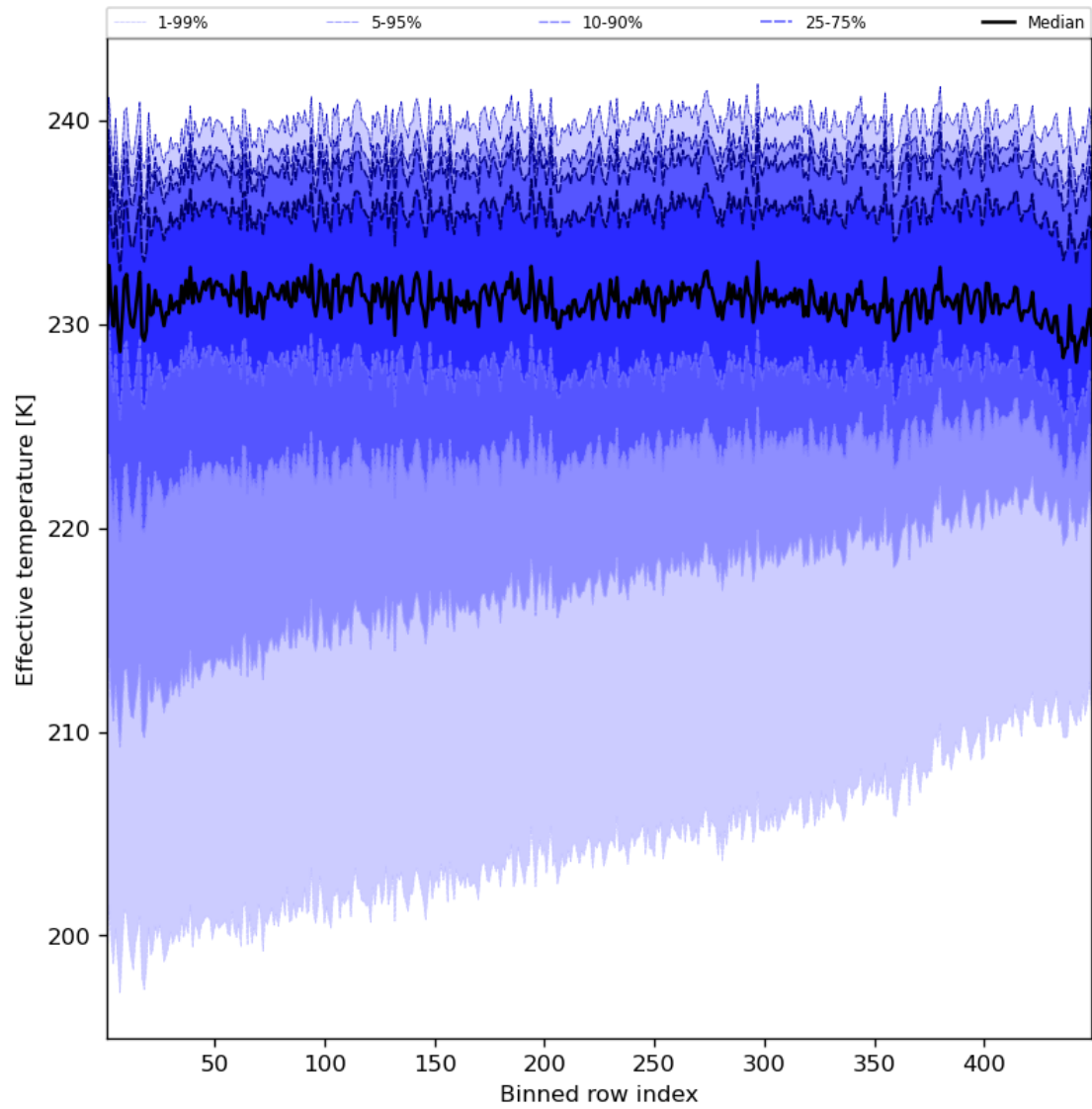
Figure 31: Along track statistics of “Effective temperature” for 2023-07-30 to 2023-08-01
