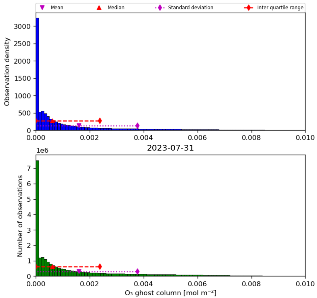
Figure 25: Histogram of "O 3 ghost column" for 2023-07-30 to 2023-08-01
