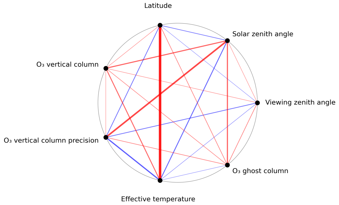
Figure 1: Map of correlation graph for 2023-07-30 to 2023-08-01.
