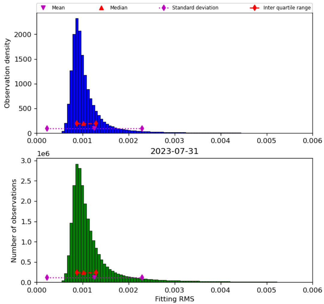
Figure 23: Histogram of “Fitting RMS” for 2023-07-30 to 2023-08-01
