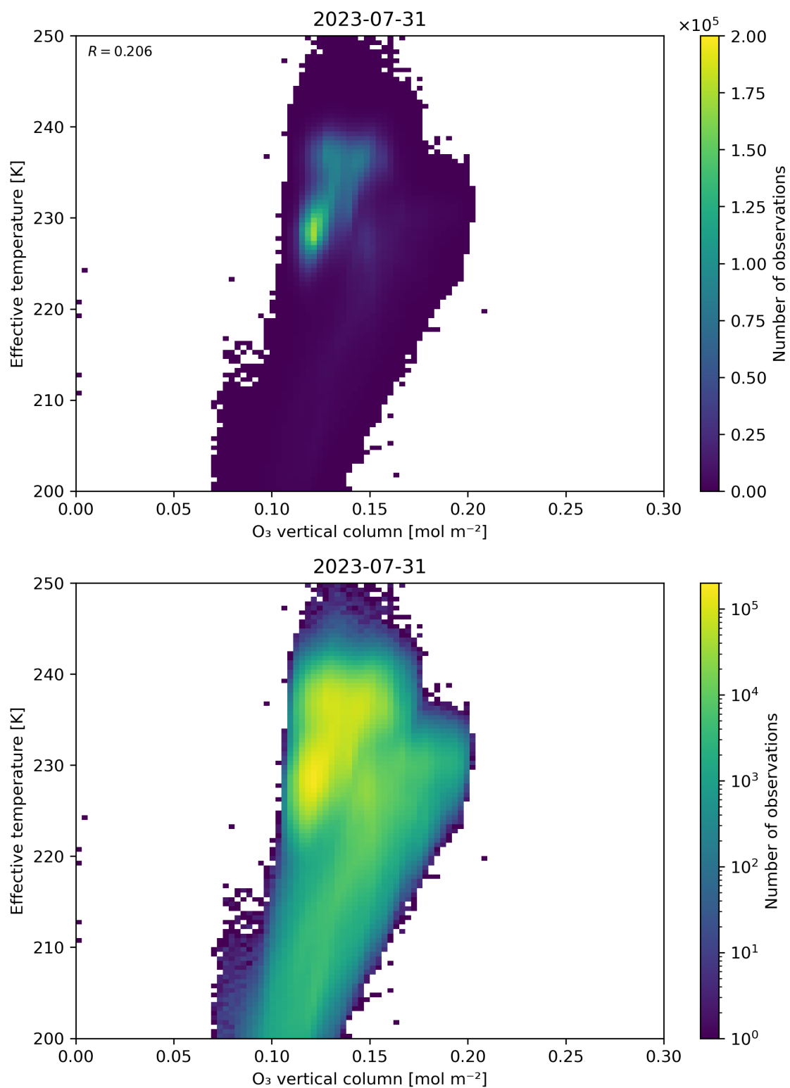
Figure 39: Scatter density plot of “O 3 vertical column” against “Effective temperature” for 2023-07-30 to 2023-08-01.
