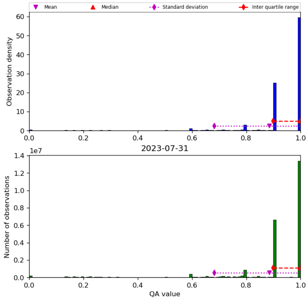
Figure 20: Histogram of “QA value” for 2023-07-30 to 2023-08-01
