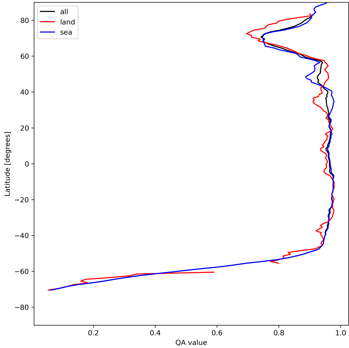
Figure 13: Zonal average of “QA value” for 2023-07-30 to 2023-08-01.
