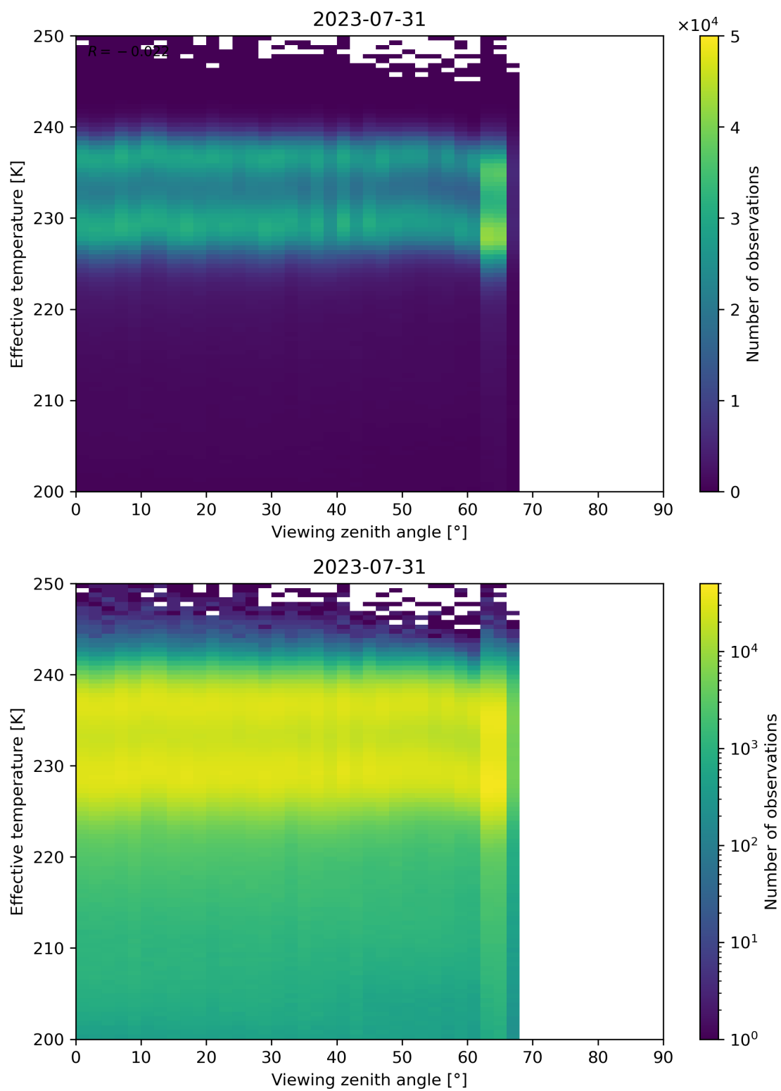
Figure 50: Scatter density plot of “Viewing zenith angle” against “Effective temperature” for 2023-07-30 to 2023-08-01.
