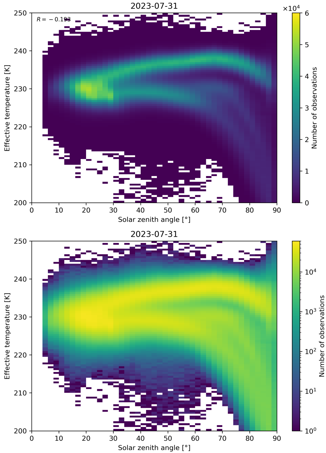
Figure 45: Scatter density plot of “Solar zenith angle” against “Effective temperature” for 2023-07-30 to 2023-08-01.
