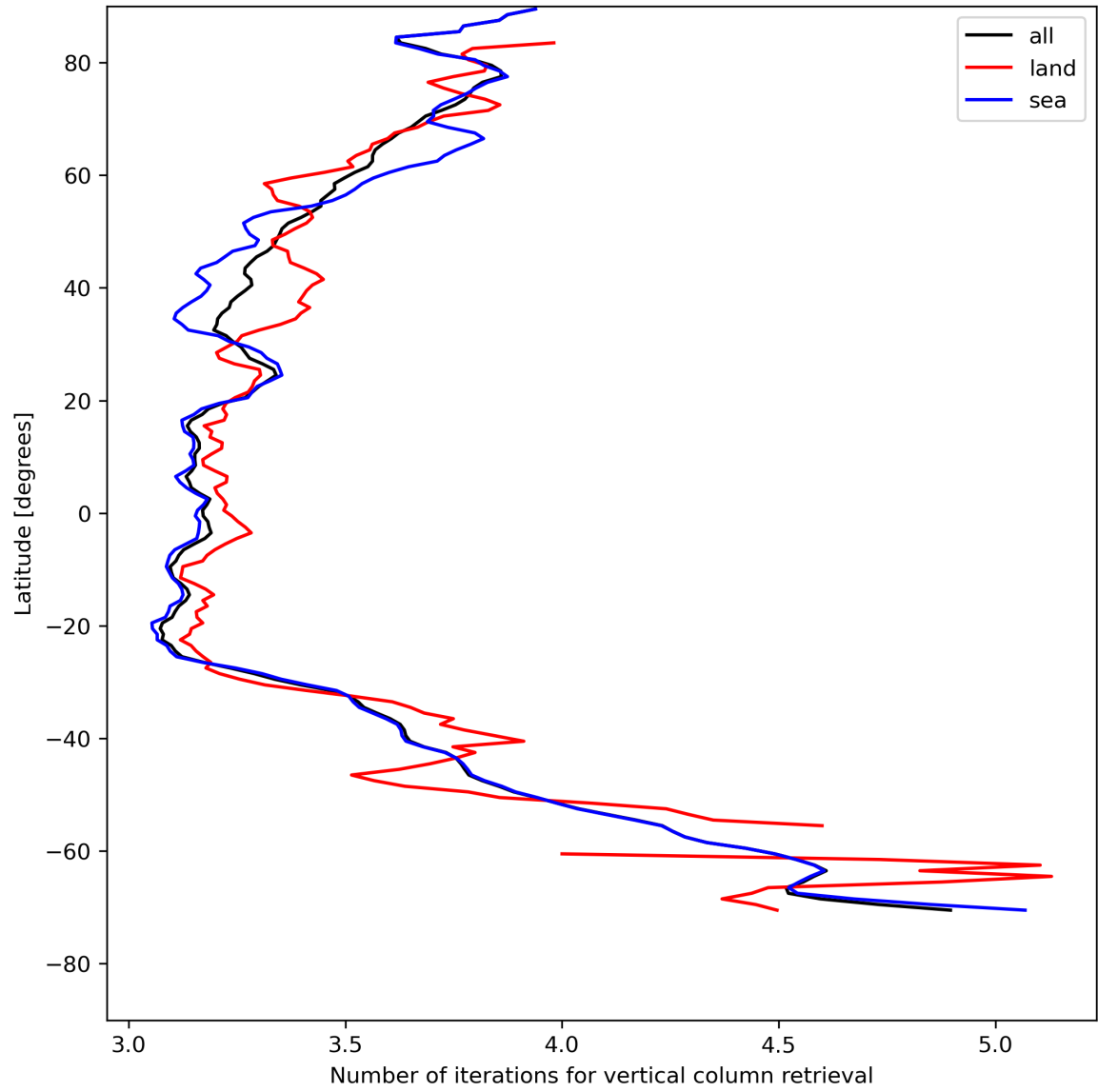
Figure 19: Zonal average of “Number of iterations for vertical column retrieval” for 2023-07-30 to 2023-08-01.
