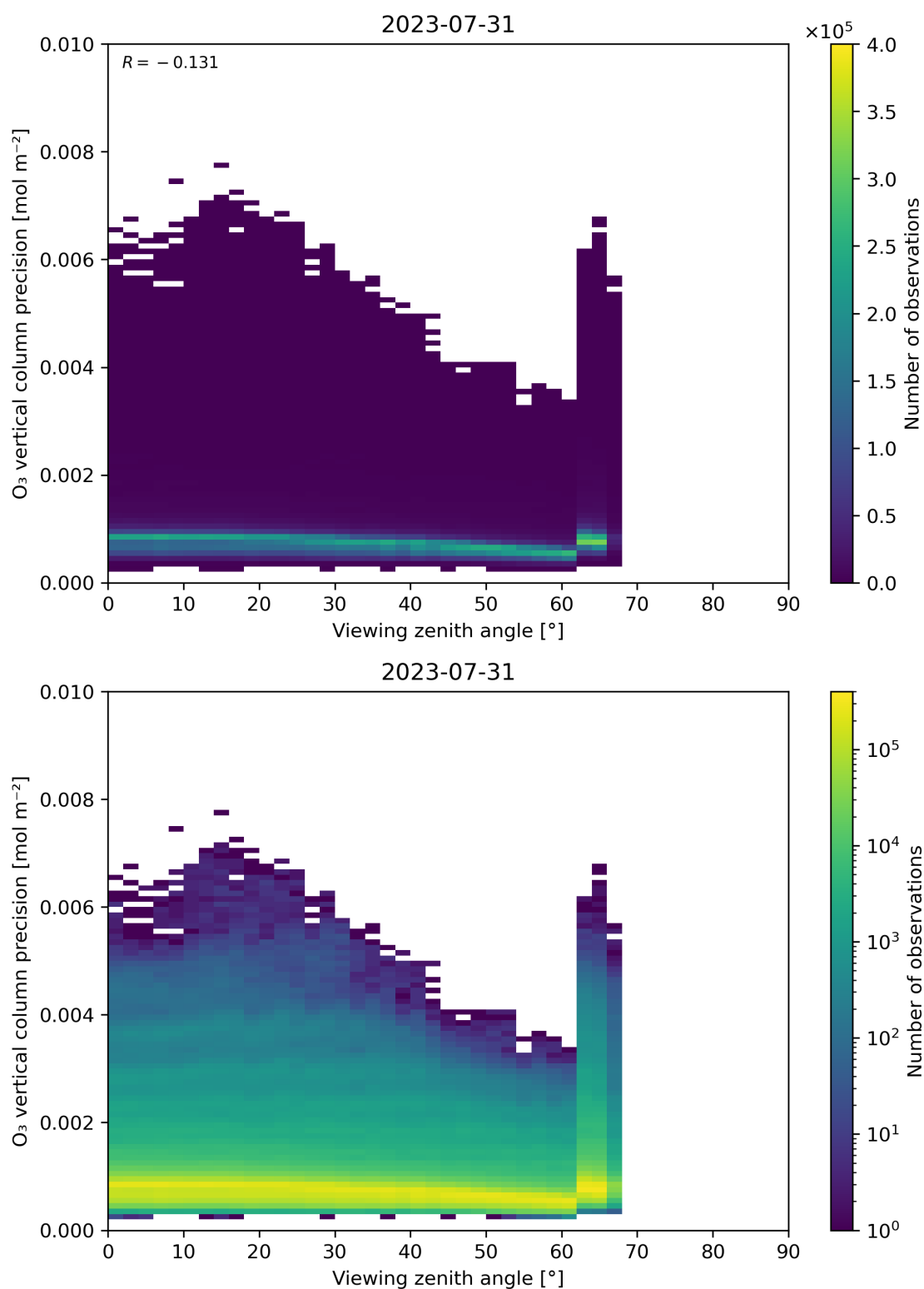
Figure 53: Scatter density plot of “Viewing zenith angle” against “O 3 vertical column precision” for 2023-07-30 to 2023-08-01.
