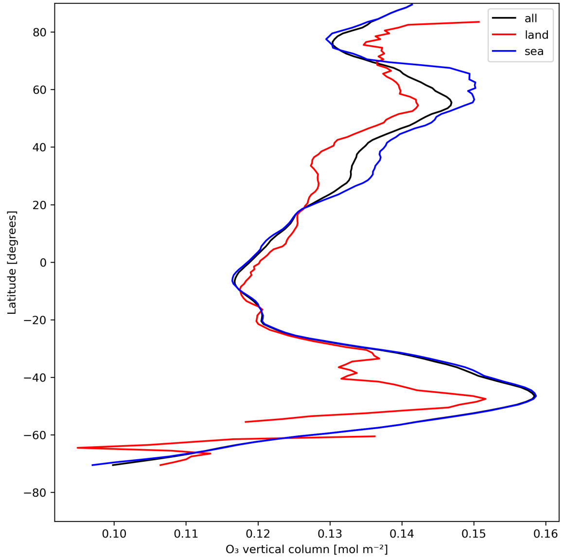
Figure 14: Zonal average of “O 3 vertical column” for 2023-07-30 to 2023-08-01.
