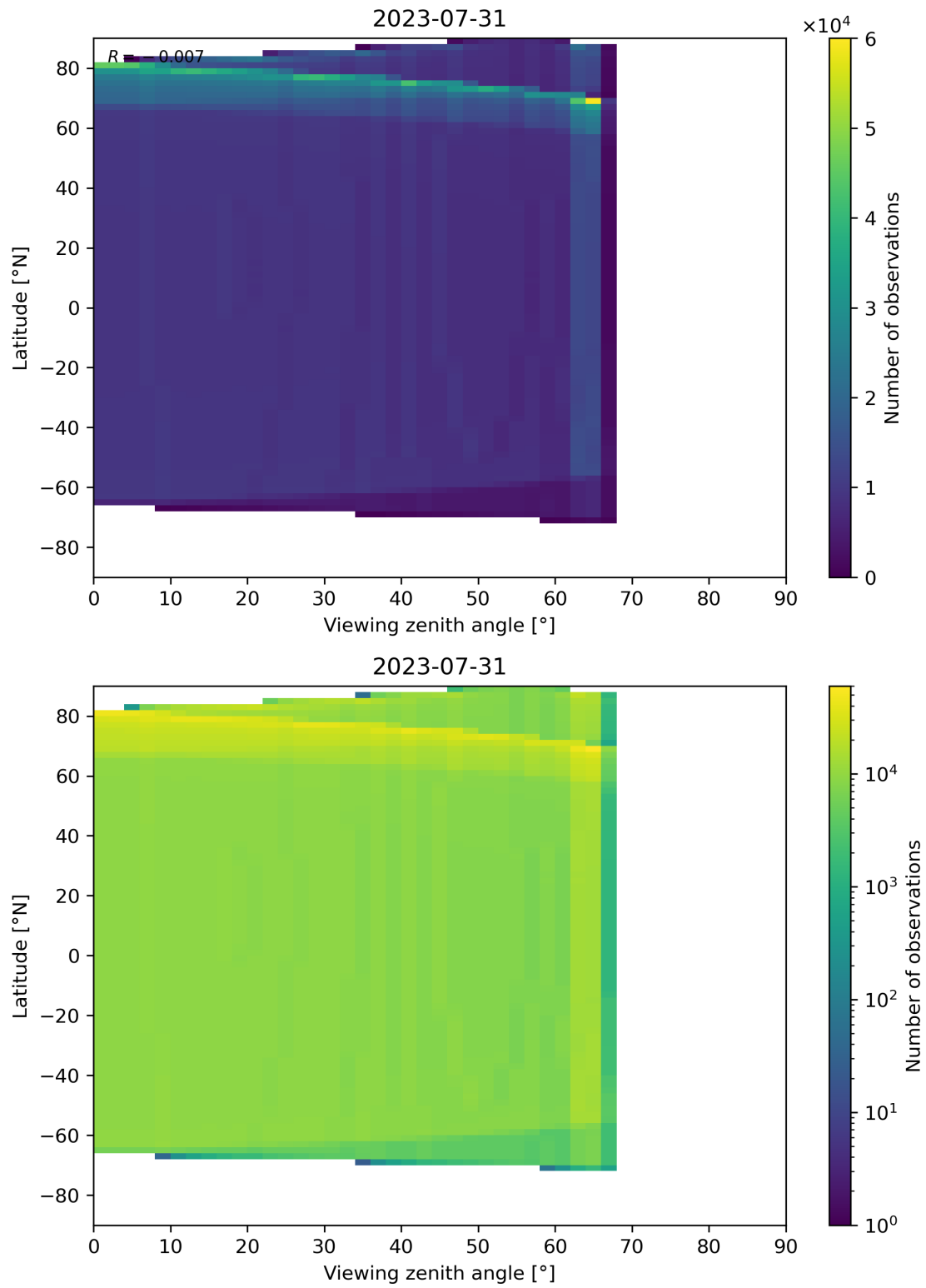
Figure 49: Scatter density plot of “Viewing zenith angle” against “Latitude” for 2023-07-30 to 2023-08-01.
