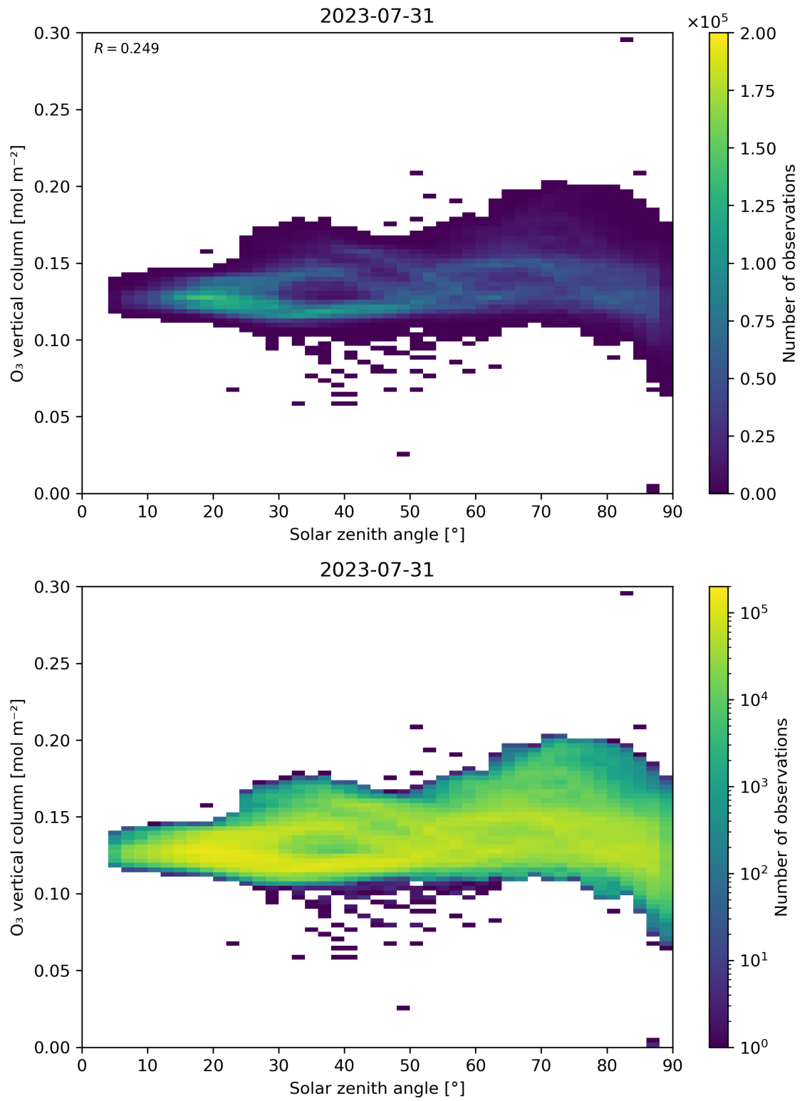
Figure 47: Scatter density plot of “Solar zenith angle” against “O 3 vertical column” for 2023-07-30 to 2023-08-01.
