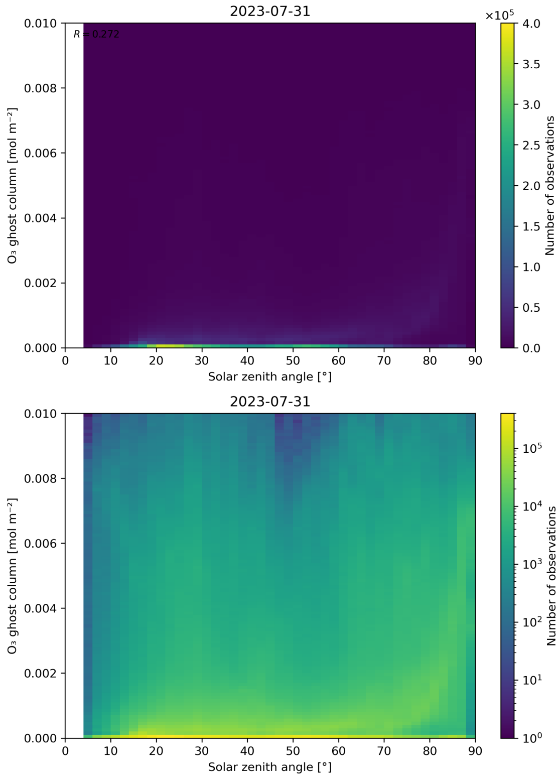
Figure 46: Scatter density plot of “Solar zenith angle” against “O 3 ghost column” for 2023-07-30 to 2023-08-01.
