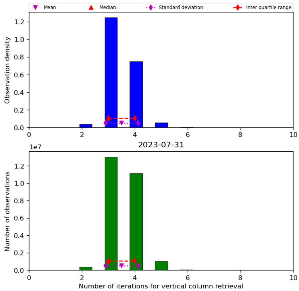
Figure 26: Histogram of “Number of iterations for vertical column retrieval” for 2023-07-30 to 2023-08-01
