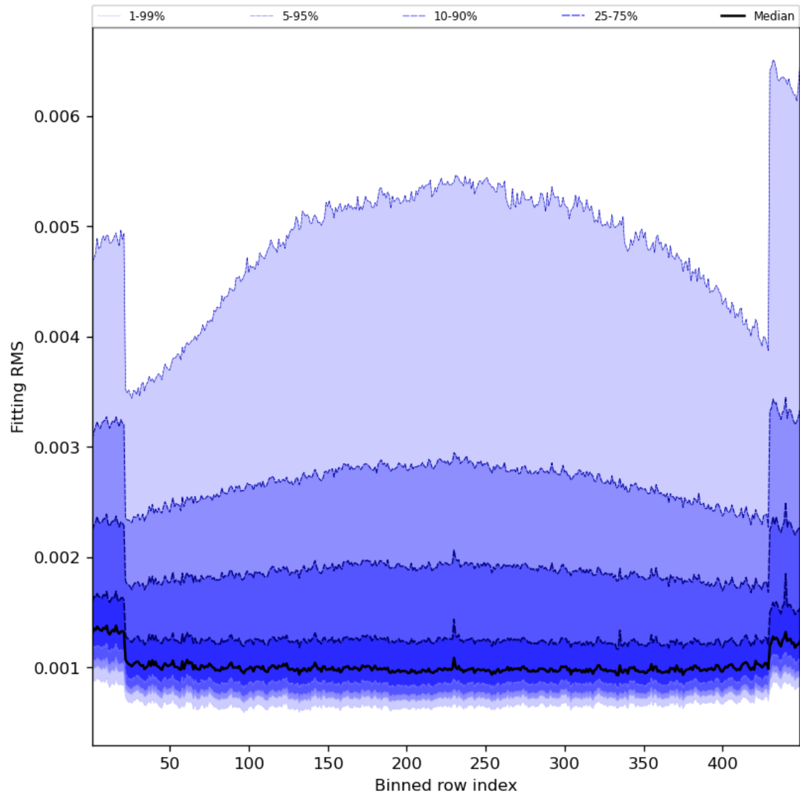
Figure 30: Along track statistics of “Fitting RMS” for 2023-07-30 to 2023-08-01
