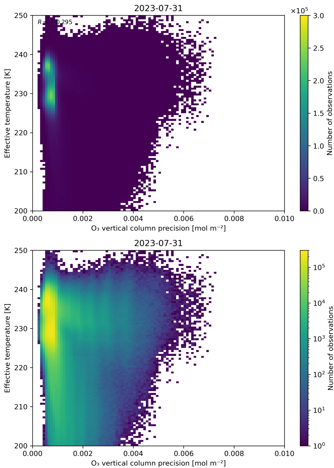
Figure 42: Scatter density plot of “O 3 vertical column precision” against “Effective temperature” for 2023-07-30 to 2023-08-01.
