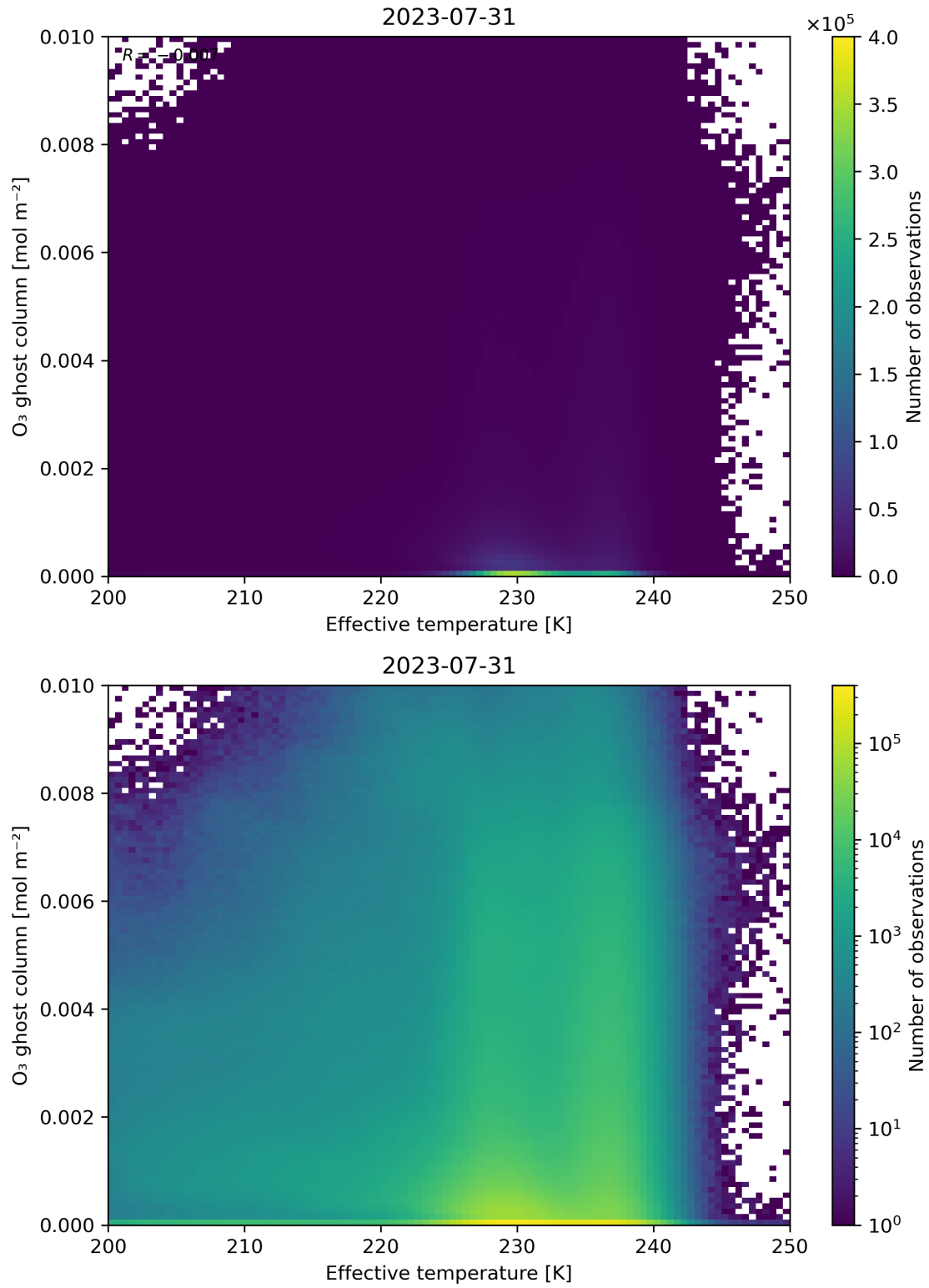
Figure 38: Scatter density plot of “Effective temperature” against “O 3 ghost column” for 2023-07-30 to 2023-08-01.
