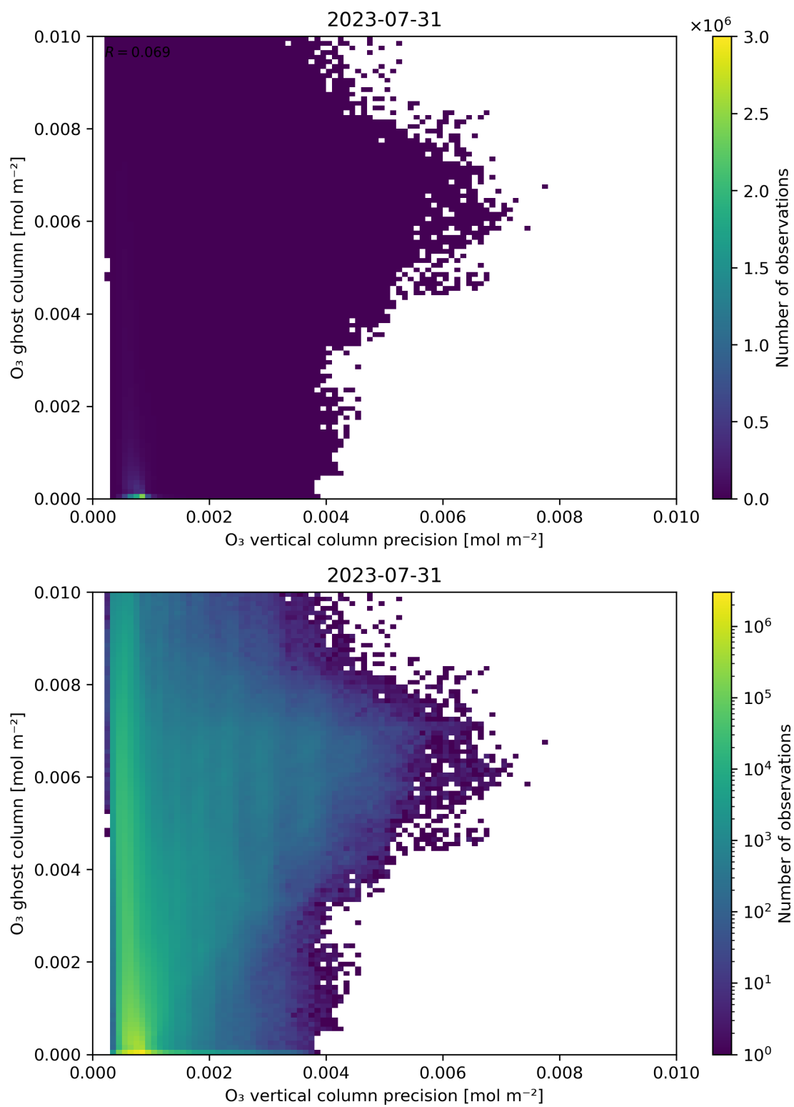
Figure 43: Scatter density plot of “ \text{O}_3 vertical column precision” against “ \text{O}_3 ghost column” for 2023-07-30 to 2023-08-01.
