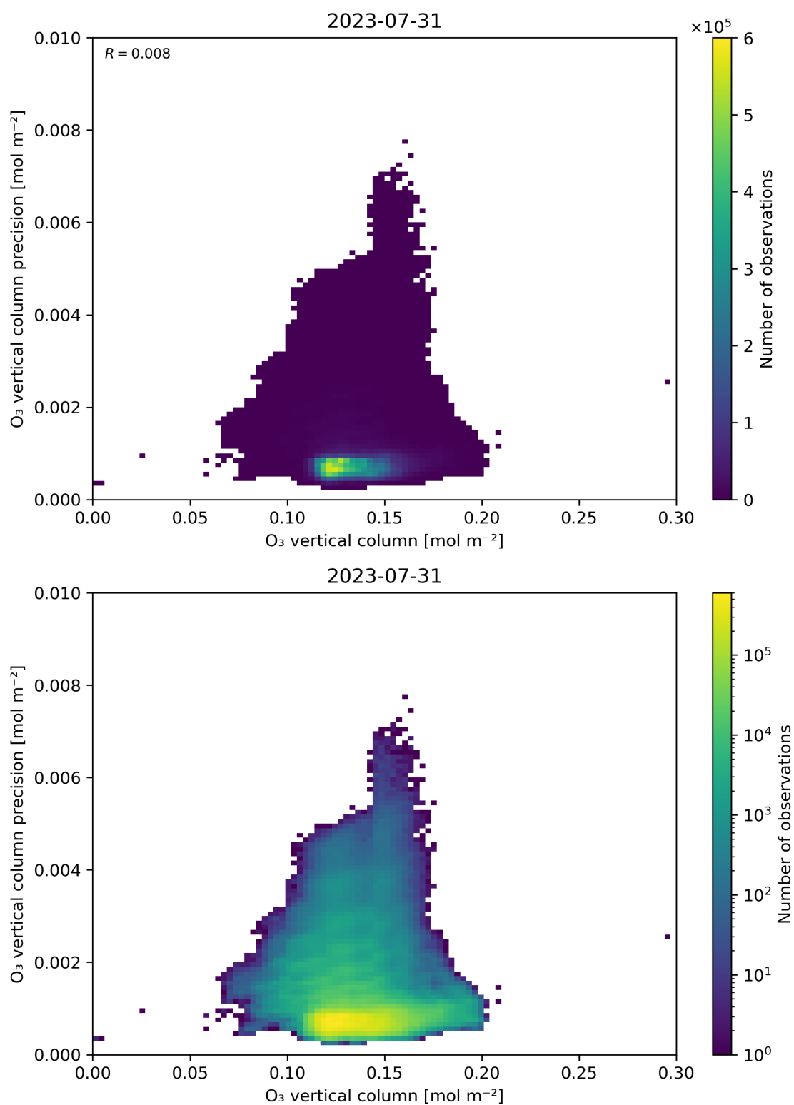
Figure 41: Scatter density plot of “O 3 vertical column” against “O 3 vertical column precision” for 2023-07-30 to 2023-08-01.
