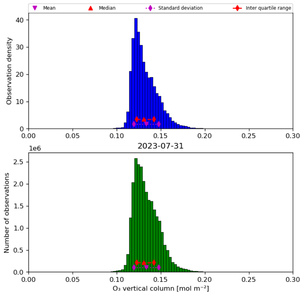
Figure 21: Histogram of “O 3 vertical column” for 2023-07-30 to 2023-08-01
