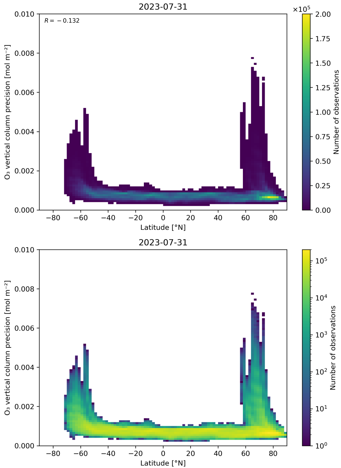
Figure 37: Scatter density plot of “Latitude” against “O 3 vertical column precision” for 2023-07-30 to 2023-08-01.
