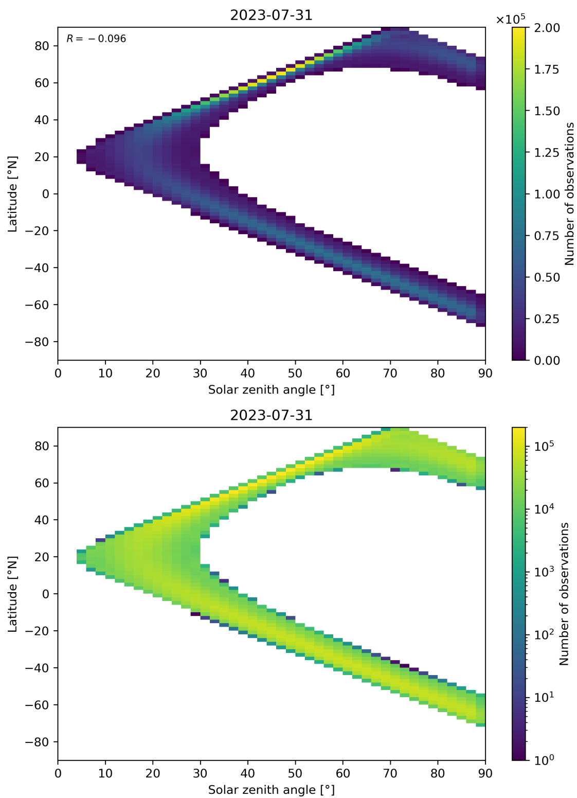
Figure 44: Scatter density plot of “Solar zenith angle” against “Latitude” for 2023-07-30 to 2023-08-01.
