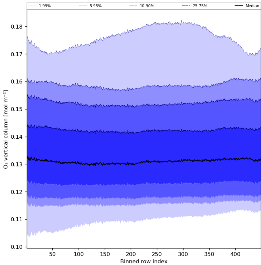
Figure 28: Along track statistics of “O 3 vertical column” for 2023-07-30 to 2023-08-01
