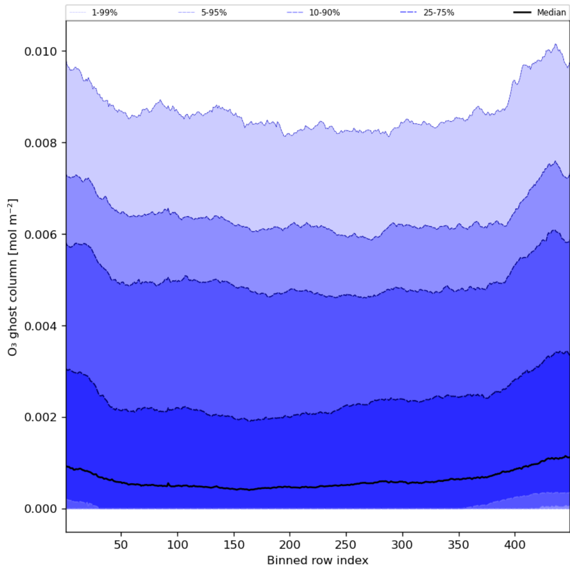
Figure 32: Along track statistics of “O 3 ghost column” for 2023-07-30 to 2023-08-01
