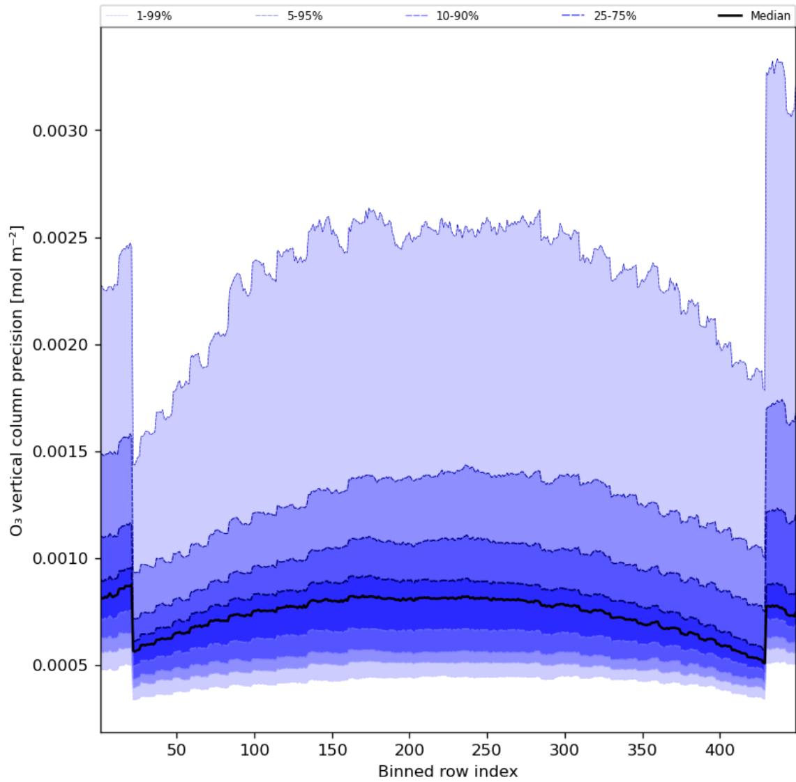
Figure 29: Along track statistics of “O 3 vertical column precision” for 2023-07-30 to 2023-08-01
