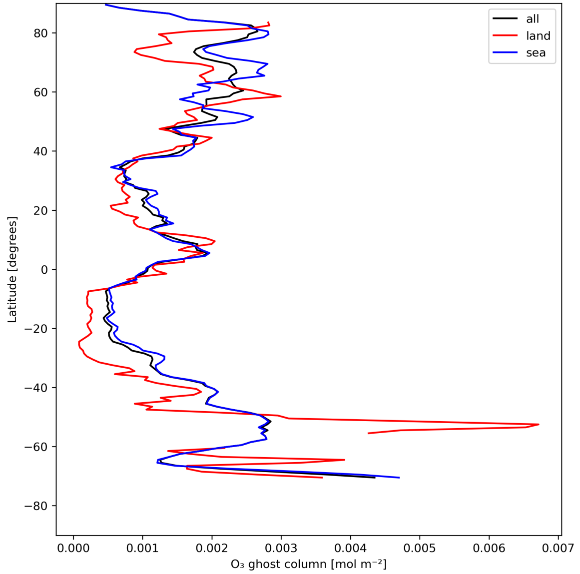
Figure 18: Zonal average of "O 3 ghost column" for 2023-07-30 to 2023-08-01.
