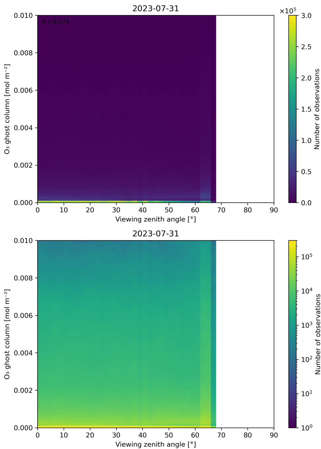
Figure 51: Scatter density plot of “Viewing zenith angle” against “O 3 ghost column” for 2023-07-30 to 2023-08-01.
