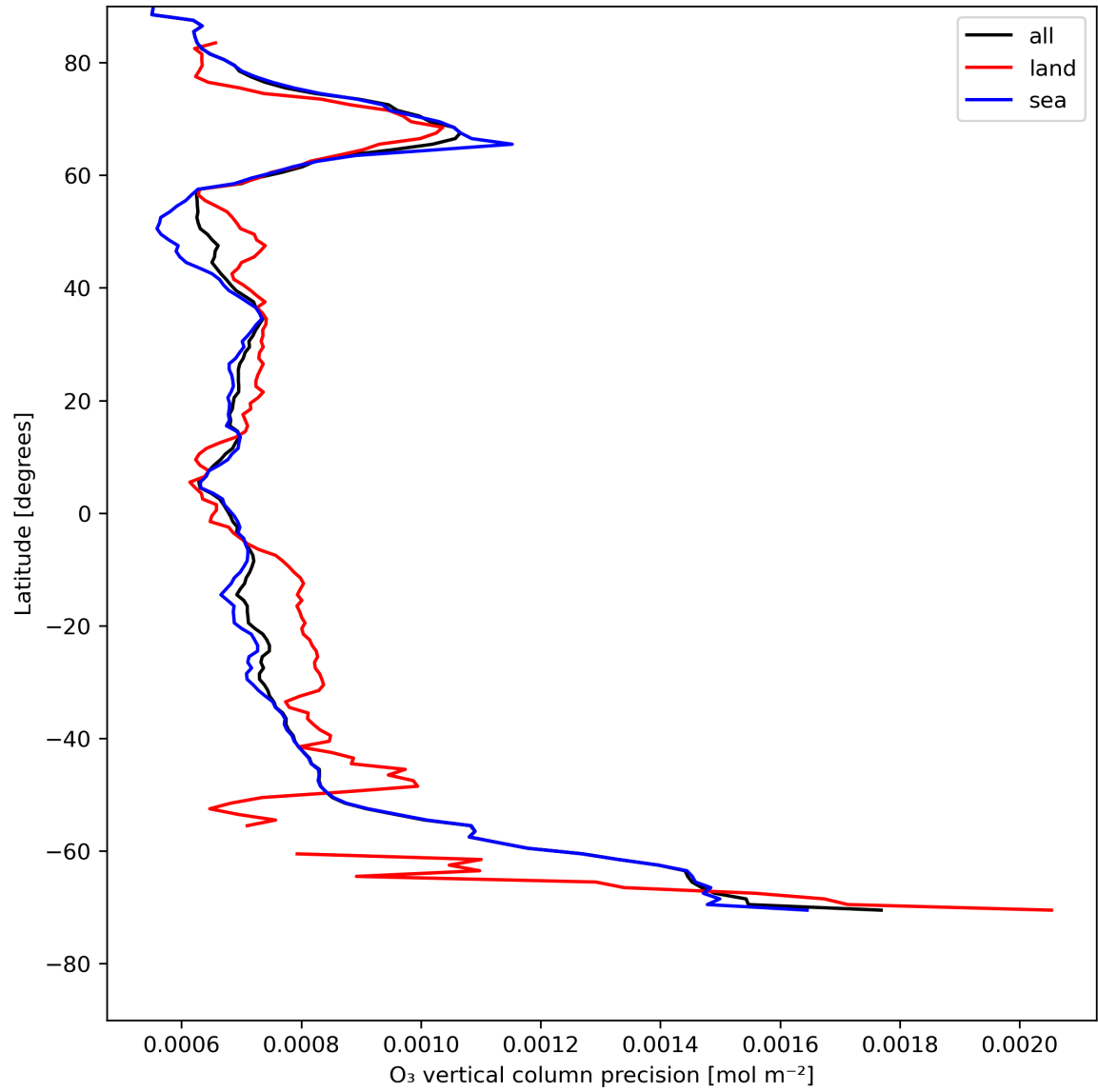
Figure 15: Zonal average of "O 3 vertical column precision" for 2023-07-30 to 2023-08-01.
