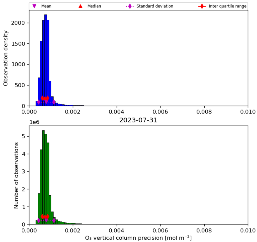
Figure 22: Histogram of “O 3 vertical column precision” for 2023-07-30 to 2023-08-01
