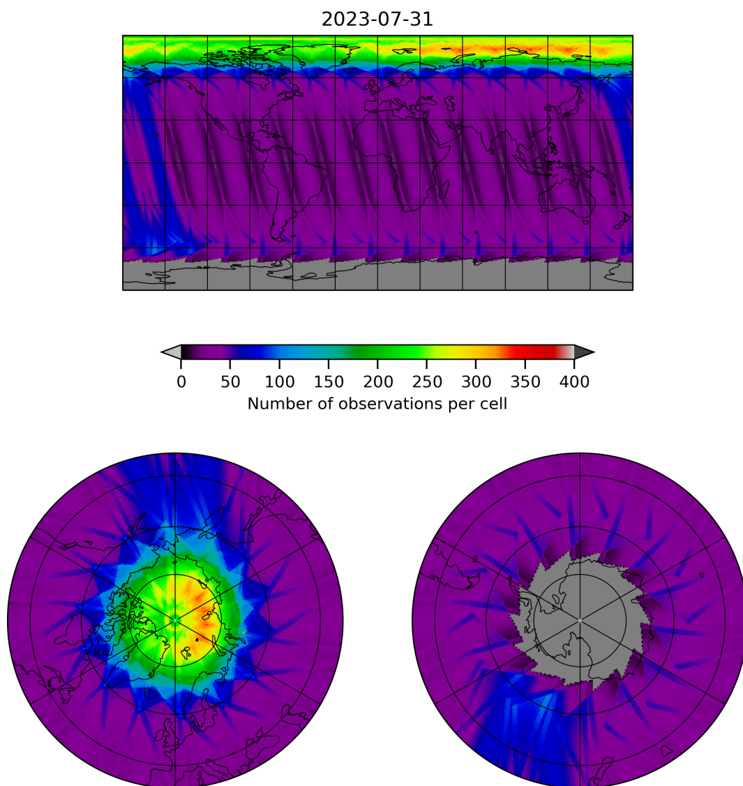
Figure 12: Map of the number of observations for 2023-07-30 to 2023-08-01
