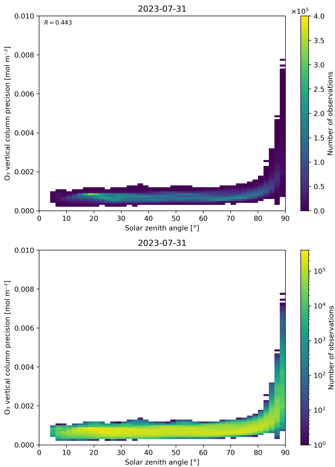
Figure 48: Scatter density plot of “Solar zenith angle” against “O 3 vertical column precision” for 2023-07-30 to 2023-08-01.
