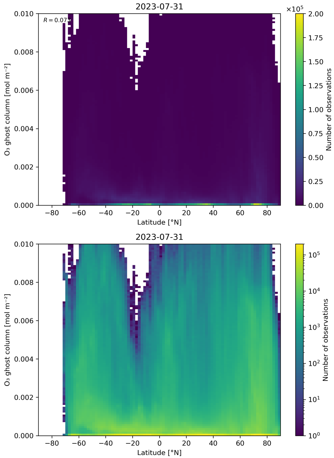
Figure 35: Scatter density plot of “Latitude” against “O 3 ghost column” for 2023-07-30 to 2023-08-01.
