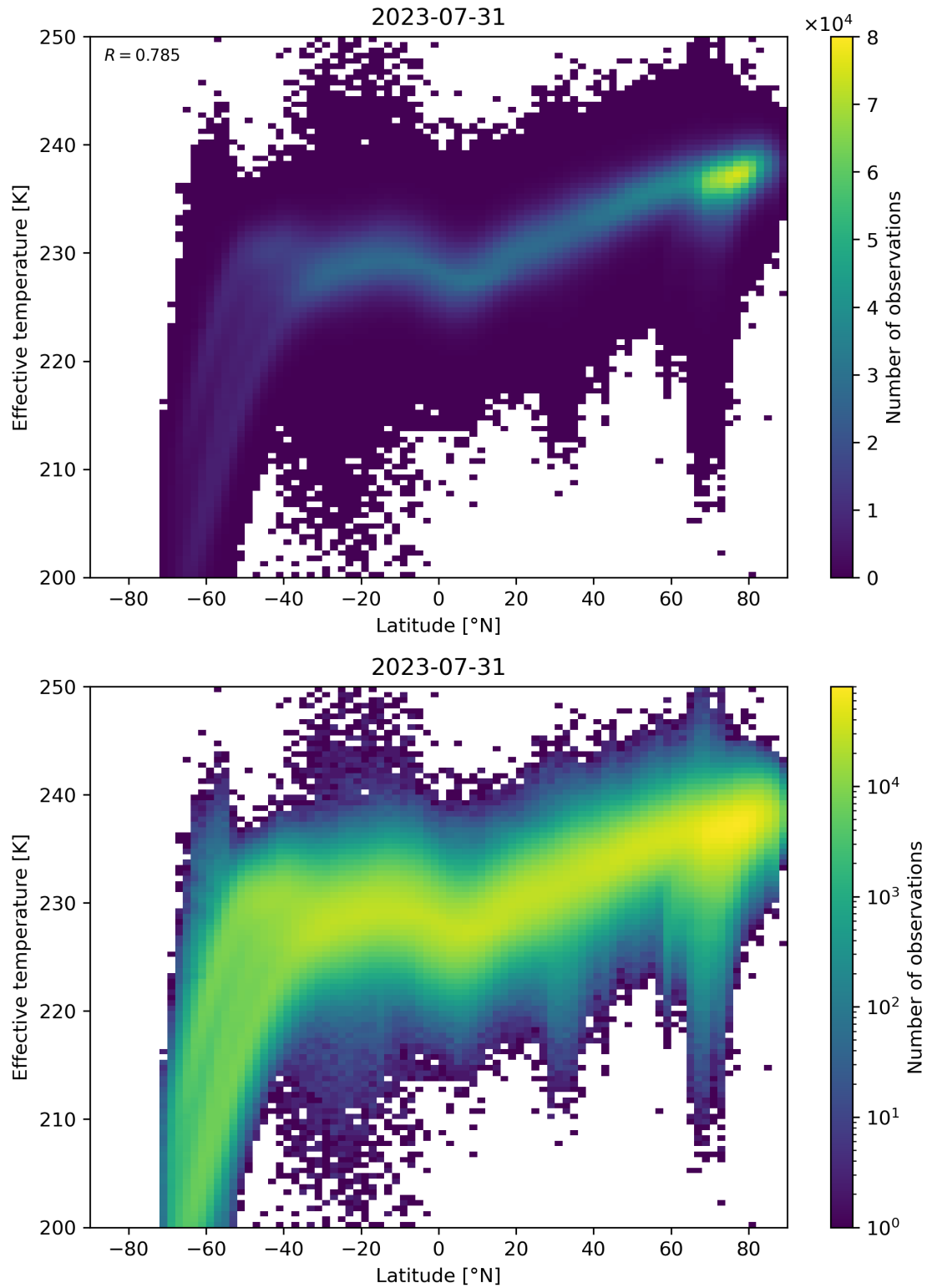
Figure 34: Scatter density plot of “Latitude” against “Effective temperature” for 2023-07-30 to 2023-08-01.
