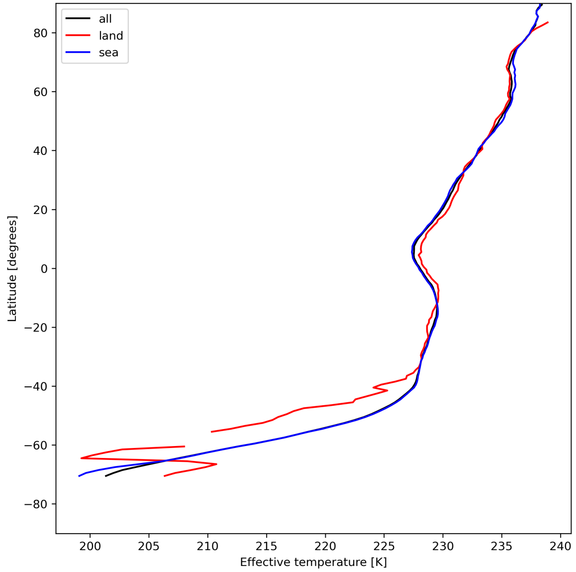
Figure 17: Zonal average of “Effective temperature” for 2023-07-30 to 2023-08-01.
