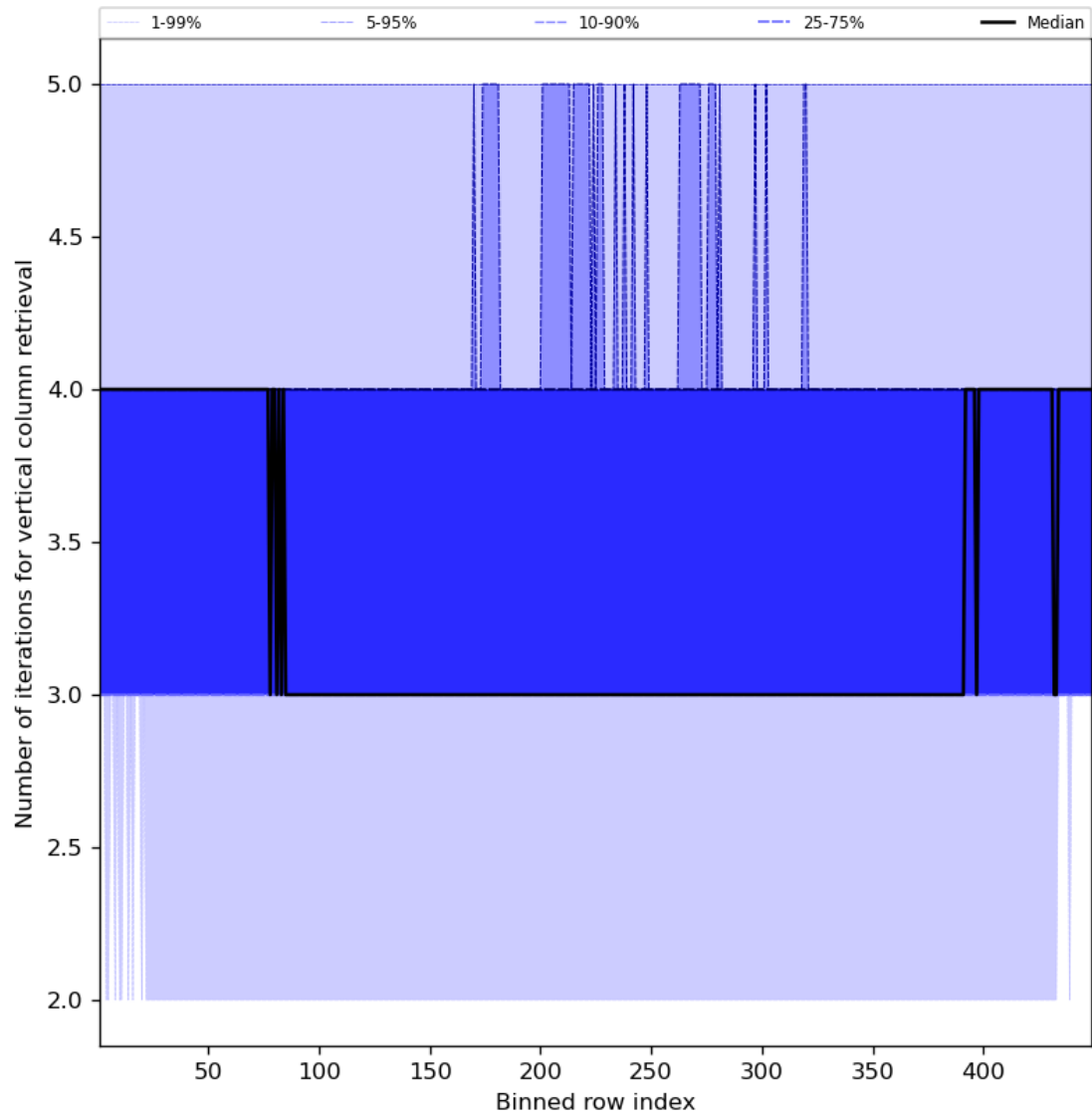
Figure 33: Along track statistics of “Number of iterations for vertical column retrieval” for 2023-07-30 to 2023-08-01
