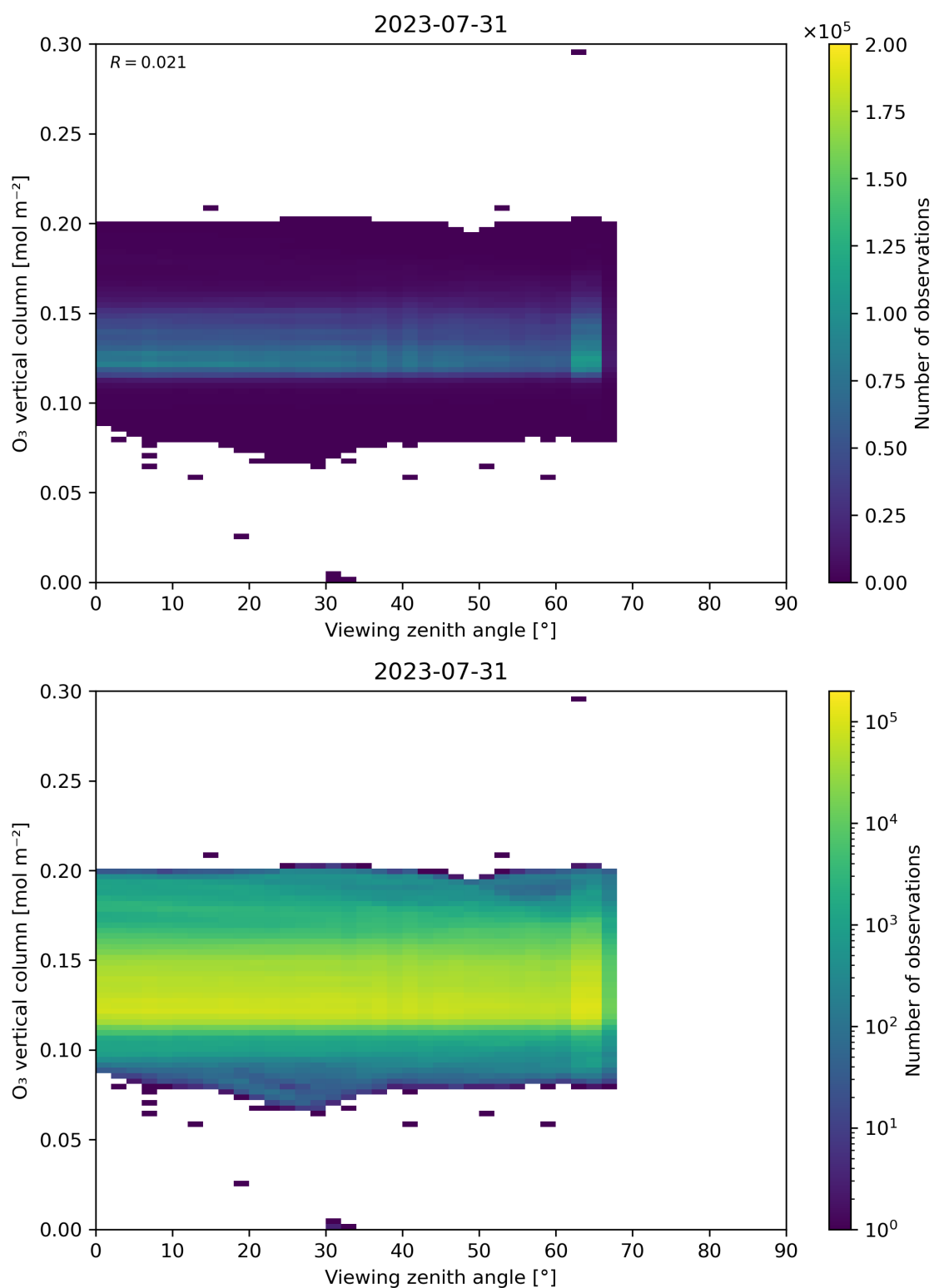
Figure 52: Scatter density plot of “Viewing zenith angle” against “O 3 vertical column” for 2023-07-30 to 2023-08-01.
