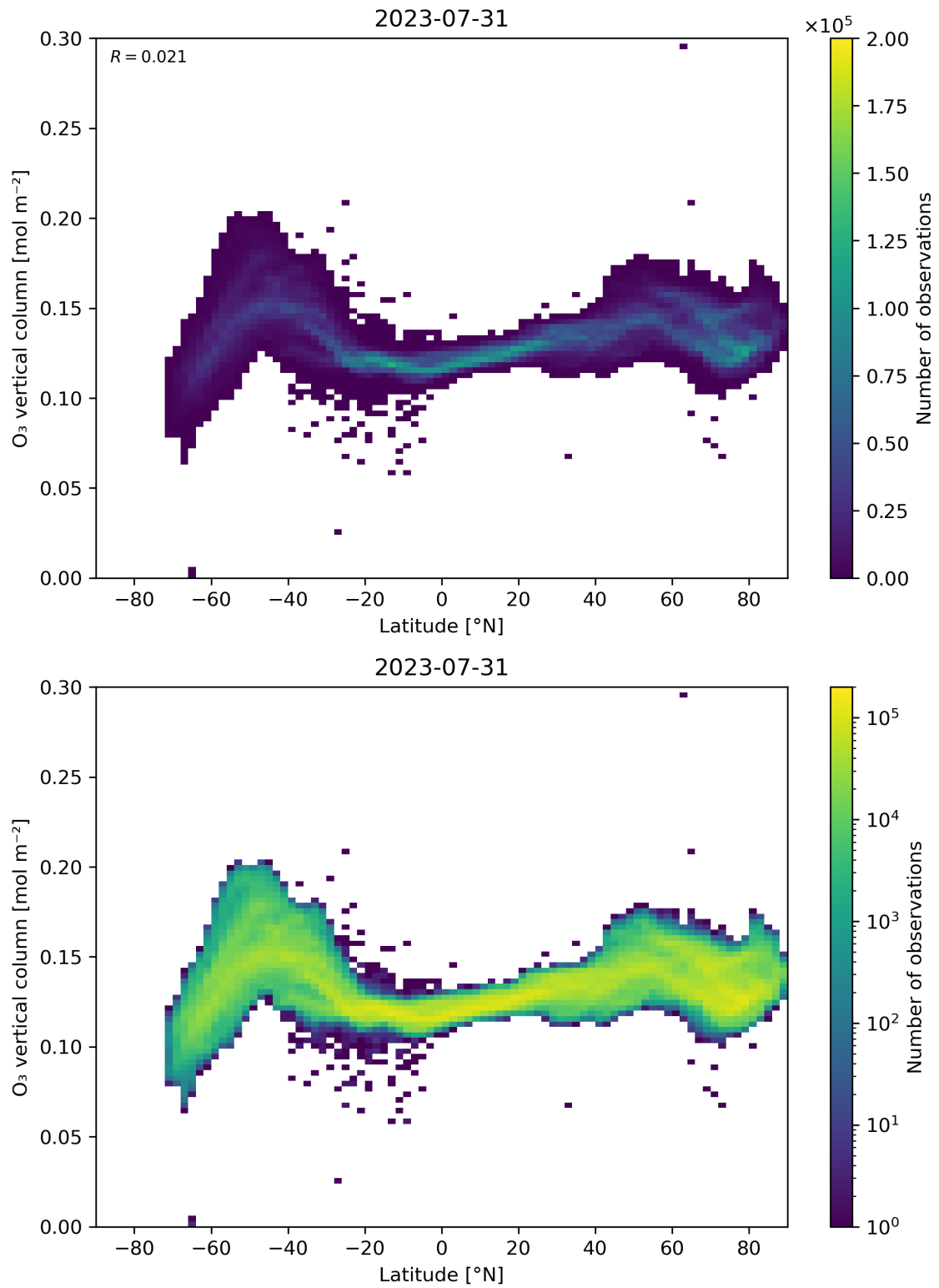
Figure 36: Scatter density plot of “Latitude” against “O 3 vertical column” for 2023-07-30 to 2023-08-01.
