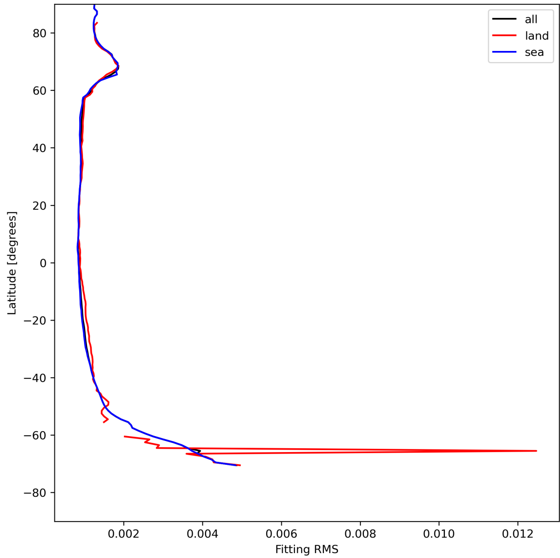
Figure 16: Zonal average of “Fitting RMS” for 2023-07-30 to 2023-08-01.
