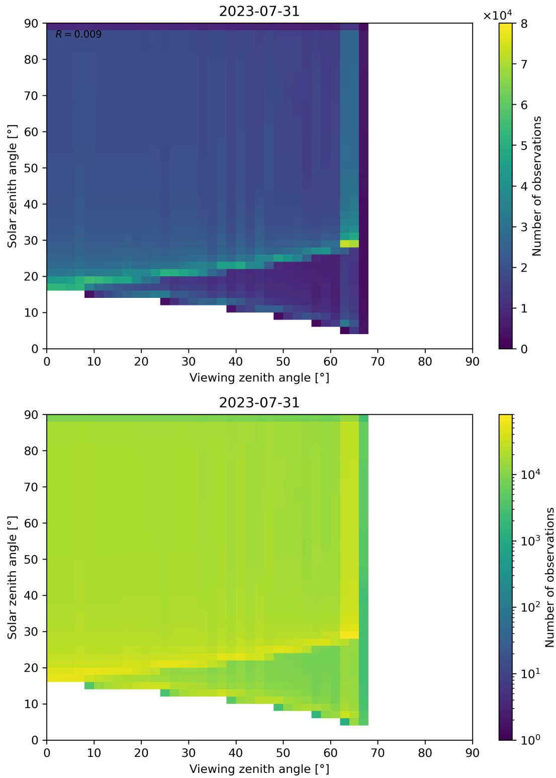
Figure 54: Scatter density plot of “Viewing zenith angle” against “Solar zenith angle” for 2023-07-30 to 2023-08-01.
