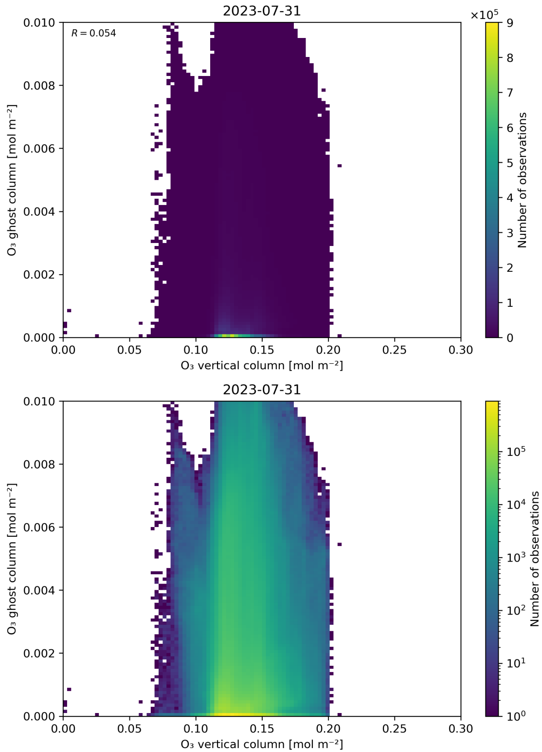
Figure 40: Scatter density plot of “O 3 vertical column” against “O 3 ghost column” for 2023-07-30 to 2023-08-01.
