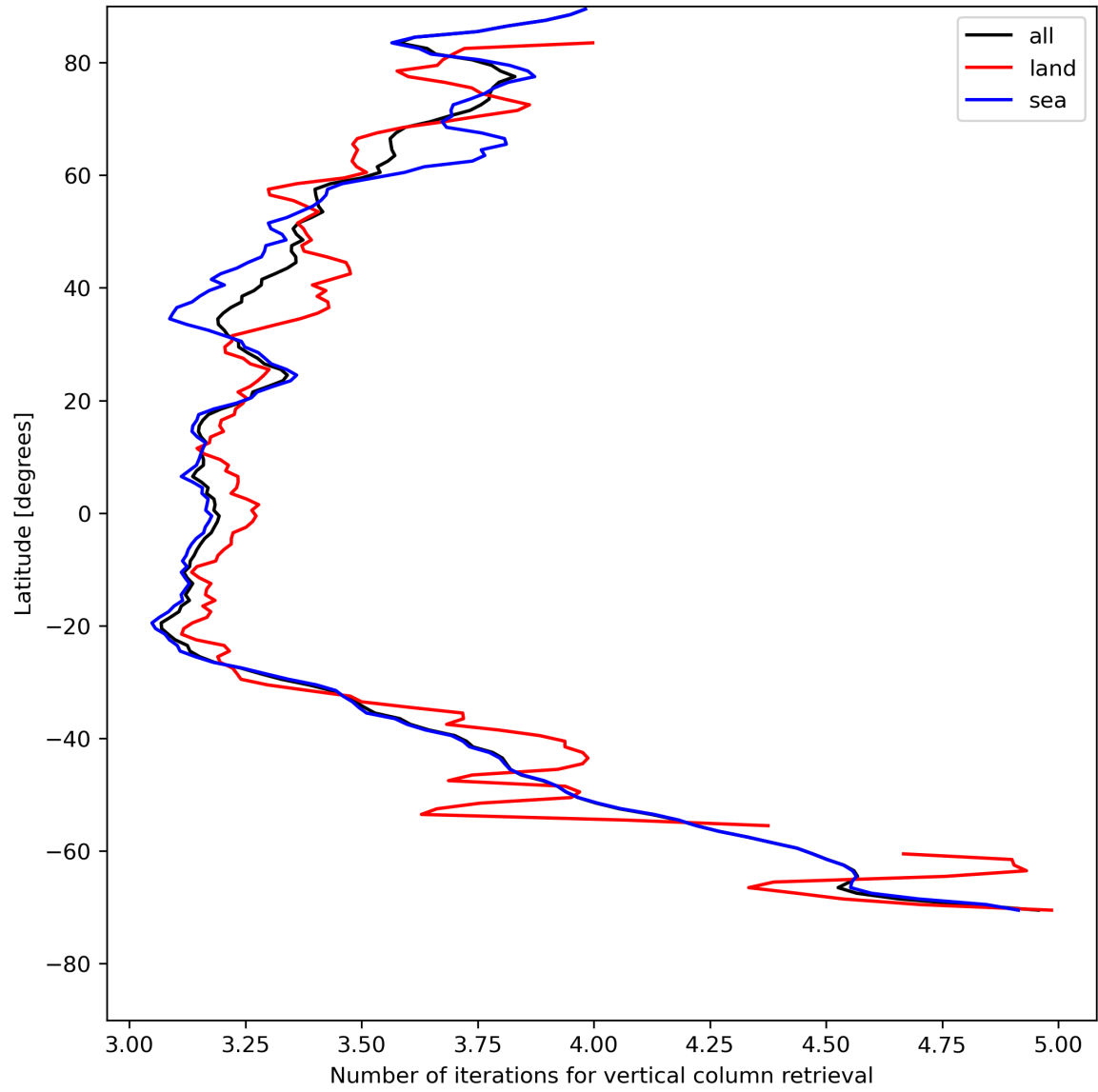
Figure 19: Zonal average of “Number of iterations for vertical column retrieval” for 2023-07-31 to 2023-08-02.
