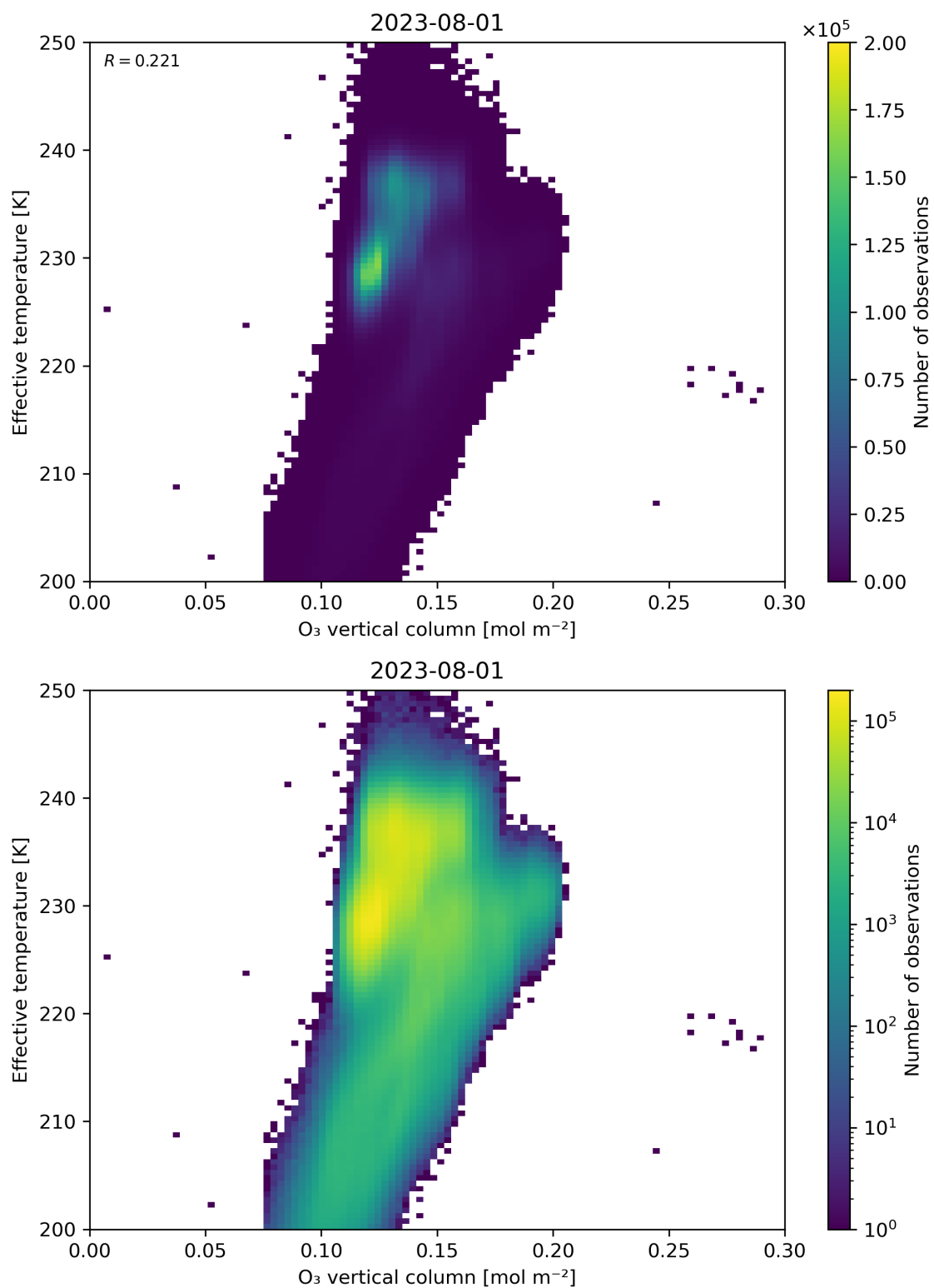
Figure 39: Scatter density plot of “O 3 vertical column” against “Effective temperature” for 2023-07-31 to 2023-08-02.
