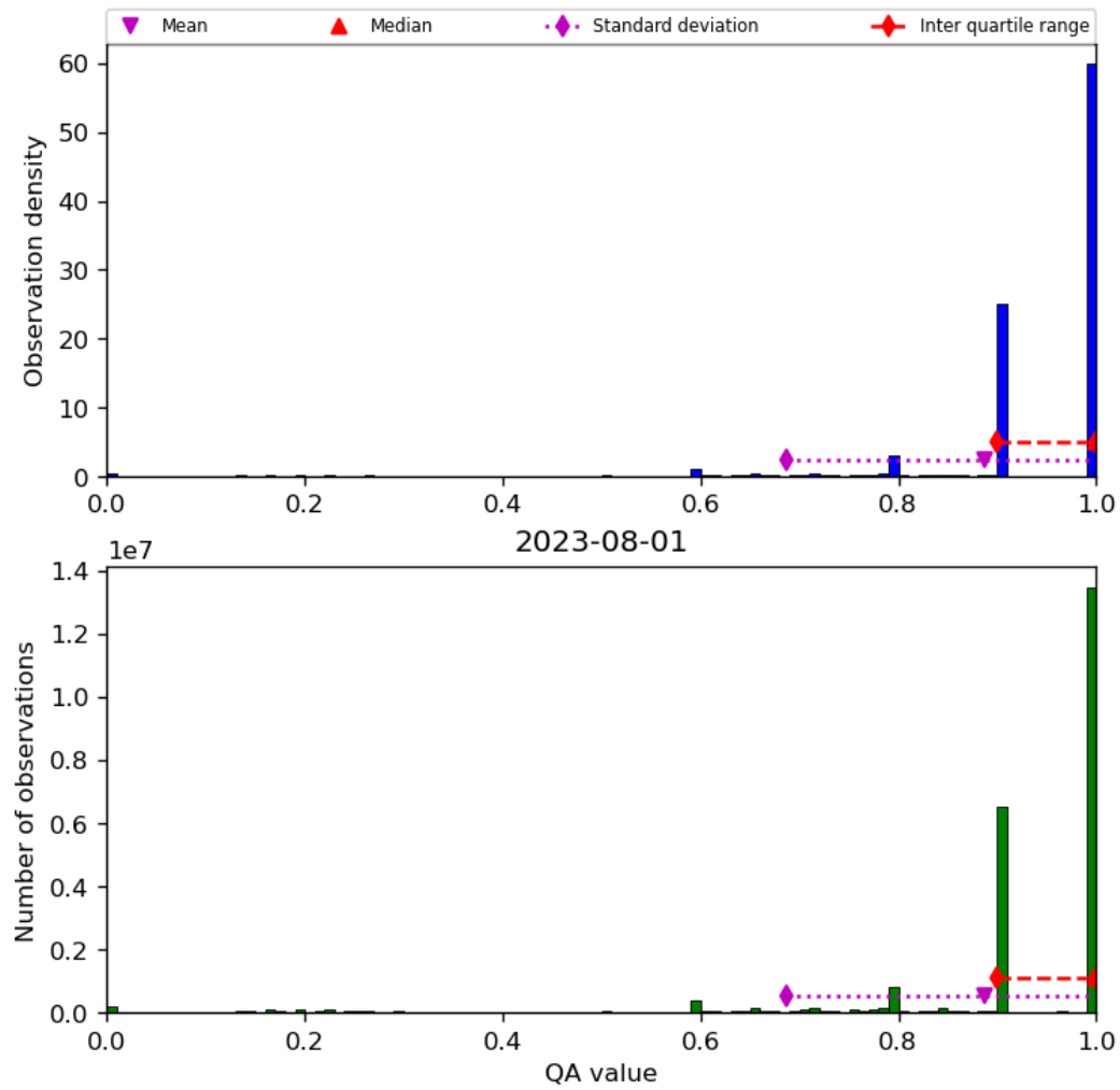
Figure 20: Histogram of “QA value” for 2023-07-31 to 2023-08-02
