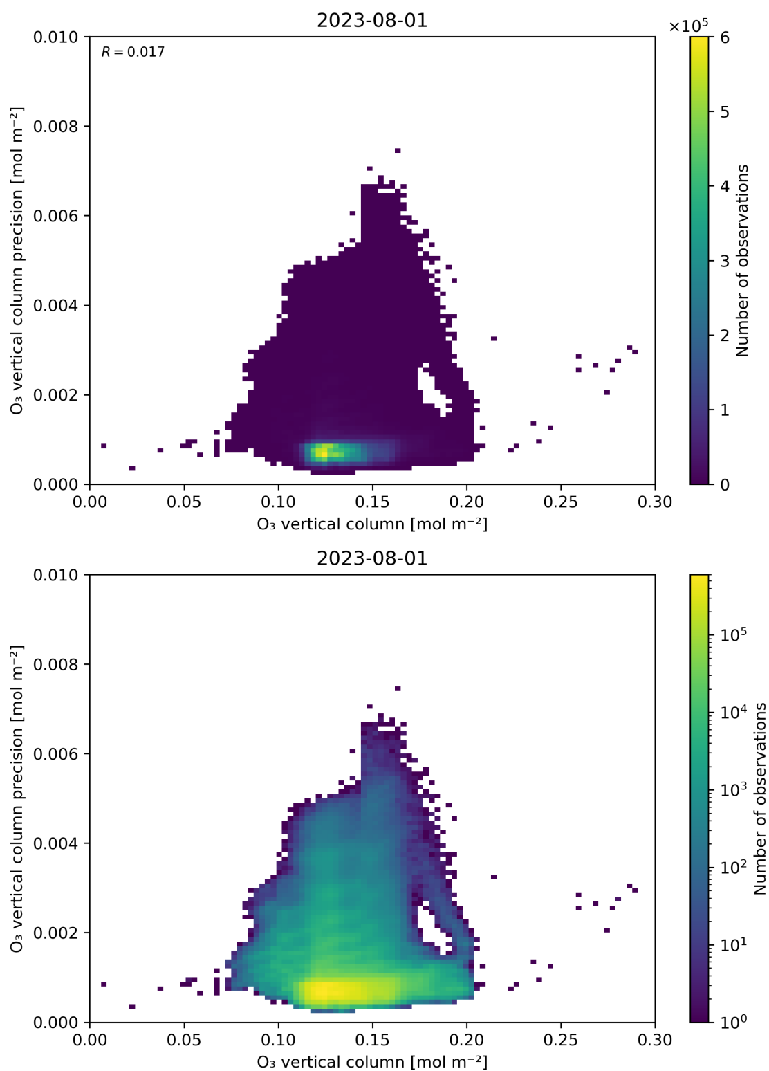
Figure 41: Scatter density plot of “O 3 vertical column” against “O 3 vertical column precision” for 2023-07-31 to 2023-08-02.
