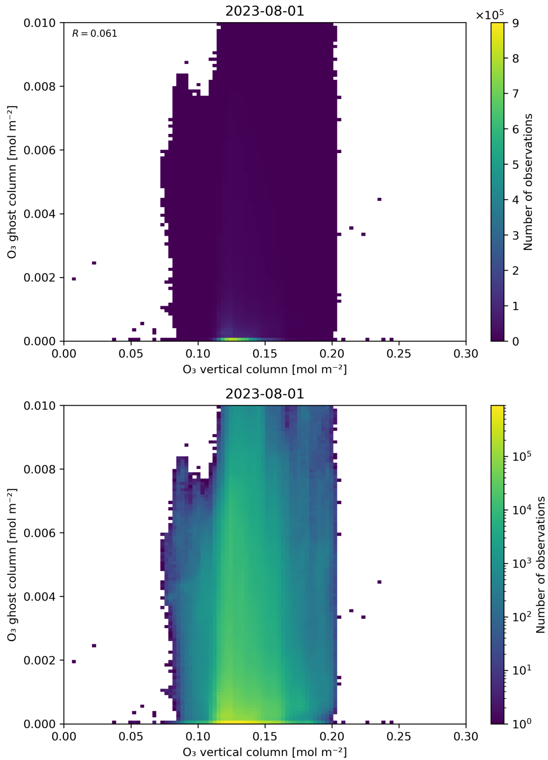
Figure 40: Scatter density plot of “O 3 vertical column” against “O 3 ghost column” for 2023-07-31 to 2023-08-02.
