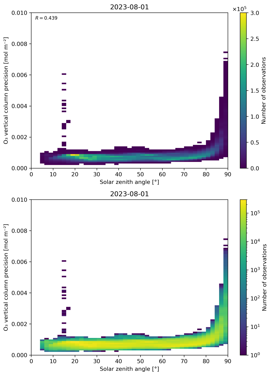
Figure 48: Scatter density plot of “Solar zenith angle” against “O 3 vertical column precision” for 2023-07-31 to 2023-08-02.
