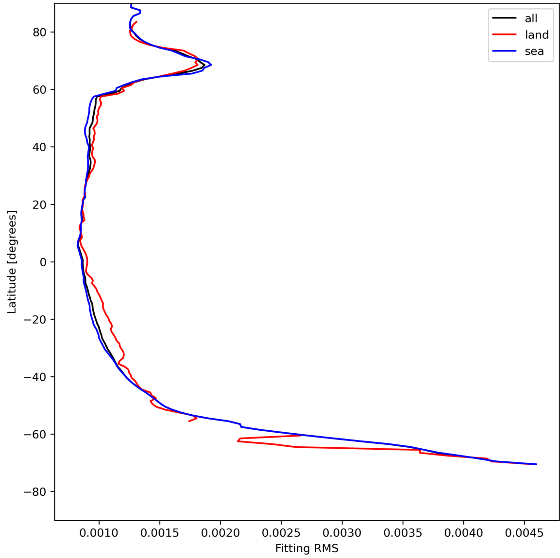
Figure 16: Zonal average of “Fitting RMS” for 2023-07-31 to 2023-08-02.
