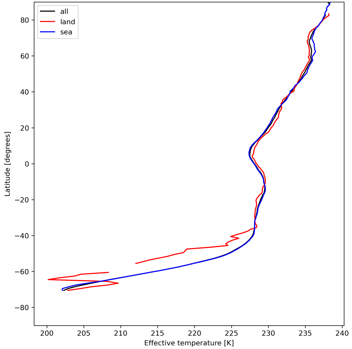
Figure 17: Zonal average of "Effective temperature" for 2023-07-31 to 2023-08-02.
