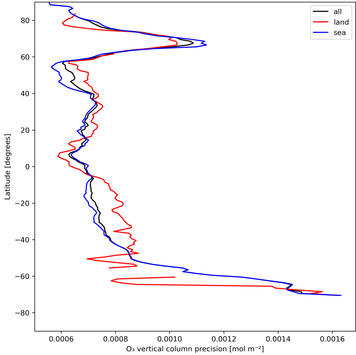
Figure 15: Zonal average of “O 3 vertical column precision” for 2023-07-31 to 2023-08-02.
