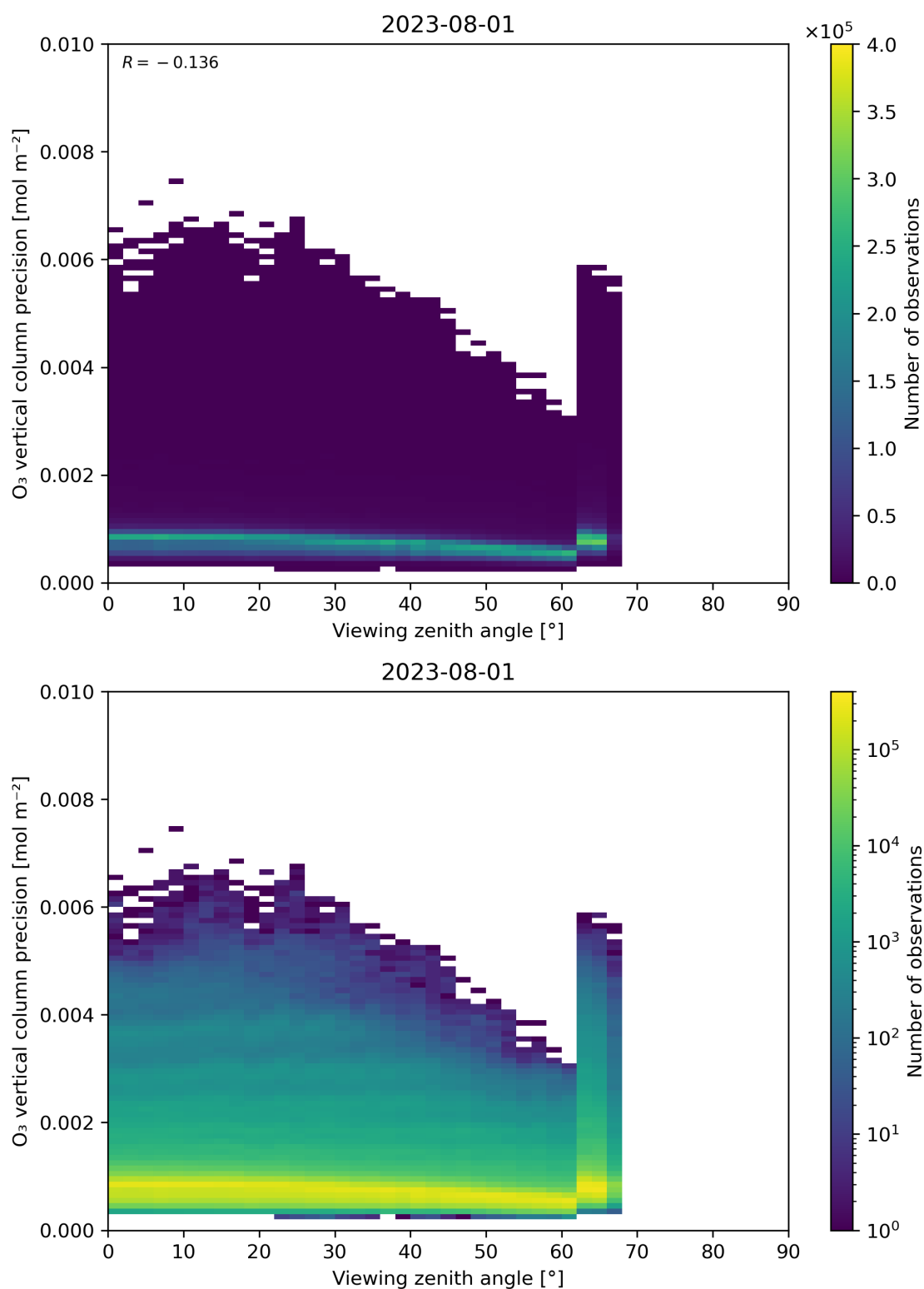
Figure 53: Scatter density plot of “Viewing zenith angle” against “O 3 vertical column precision” for 2023-07-31 to 2023-08-02.
