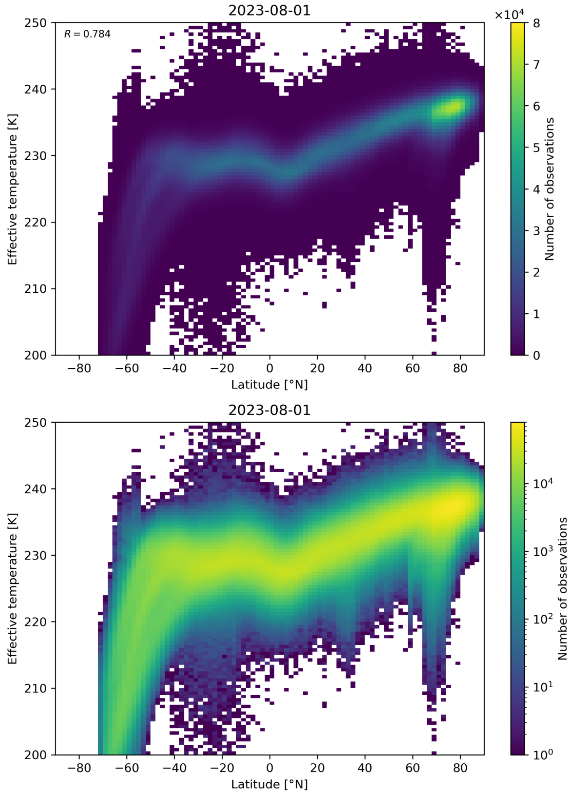
Figure 34: Scatter density plot of “Latitude” against “Effective temperature” for 2023-07-31 to 2023-08-02.
