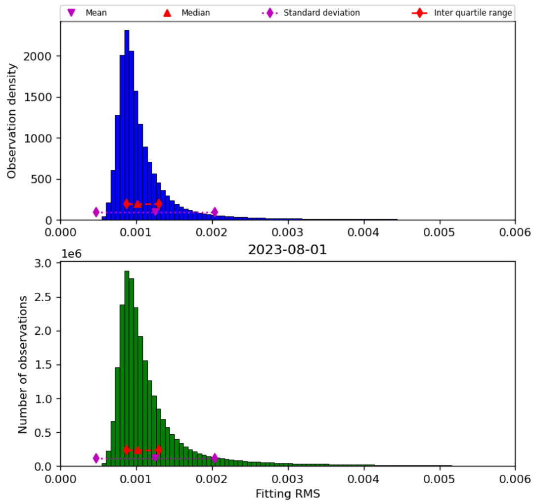
Figure 23: Histogram of “Fitting RMS” for 2023-07-31 to 2023-08-02
