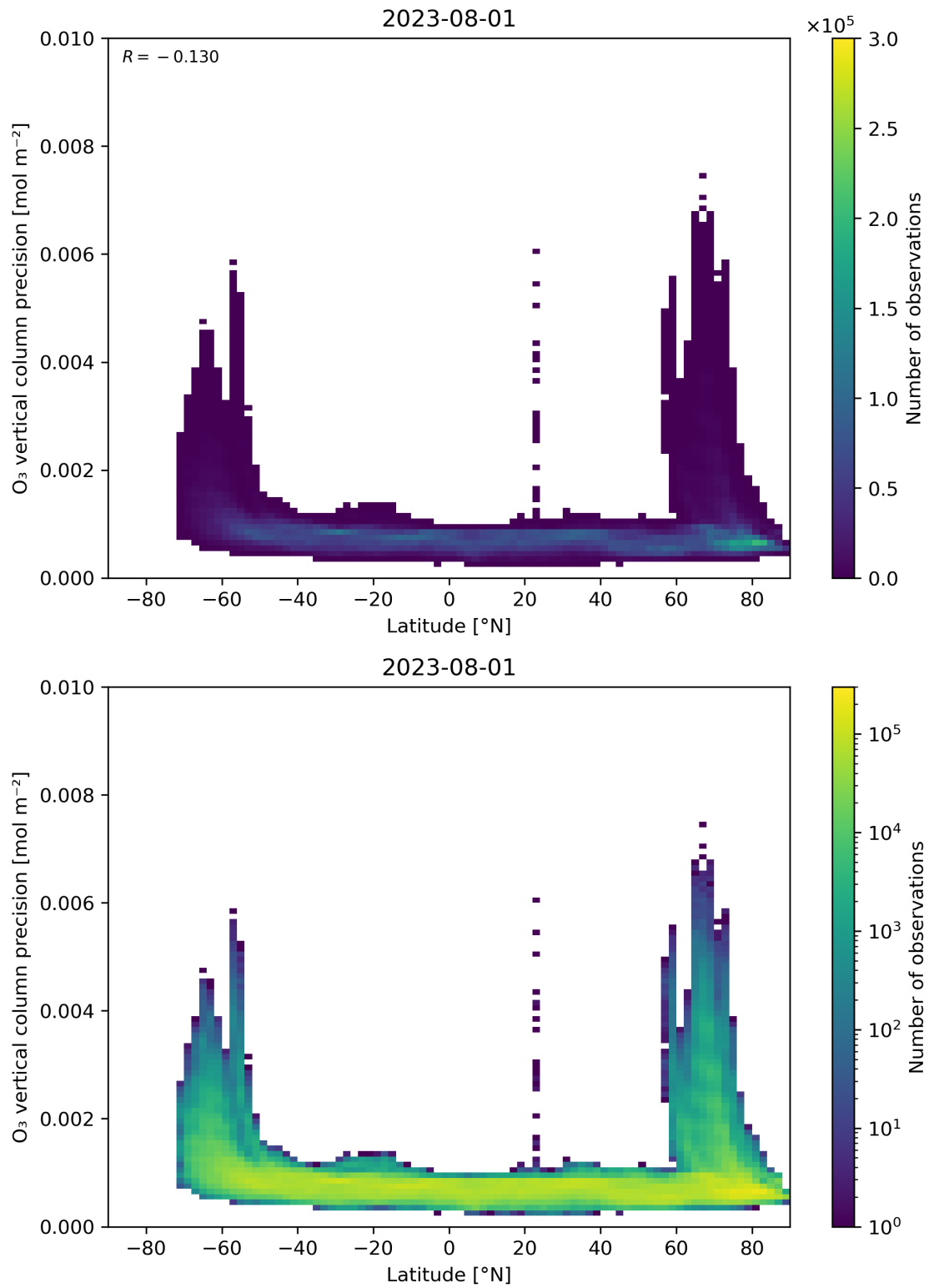
Figure 37: Scatter density plot of “Latitude” against “O 3 vertical column precision” for 2023-07-31 to 2023-08-02.
