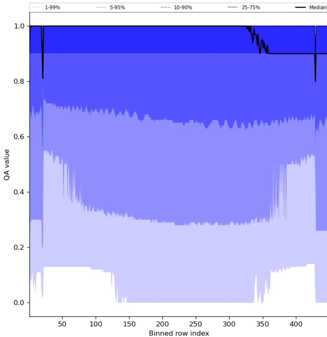
Figure 27: Along track statistics of “QA value” for 2023-07-31 to 2023-08-02
