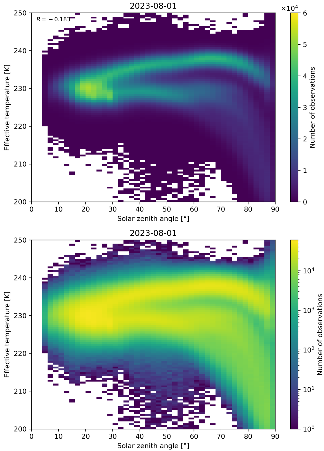
Figure 45: Scatter density plot of “Solar zenith angle” against “Effective temperature” for 2023-07-31 to 2023-08-02.
