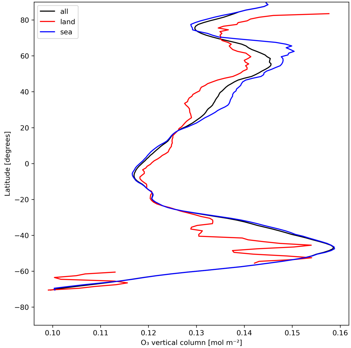
Figure 14: Zonal average of “O 3 vertical column” for 2023-07-31 to 2023-08-02.
