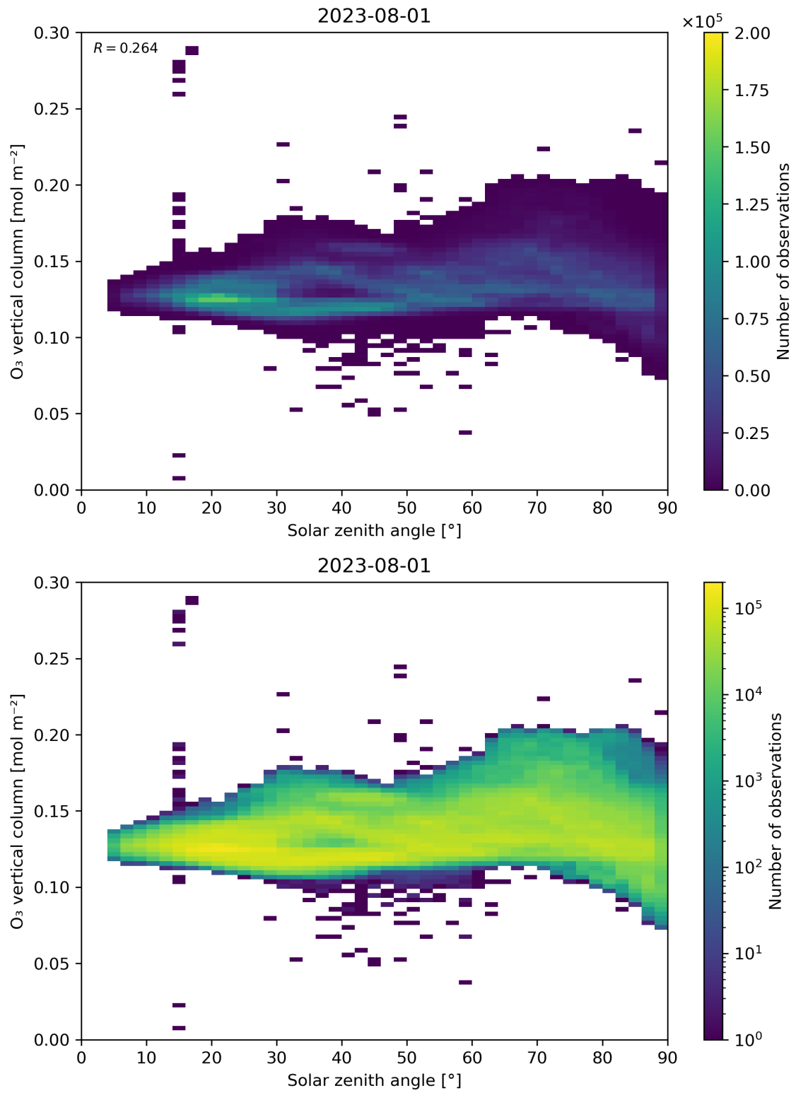
Figure 47: Scatter density plot of “Solar zenith angle” against “O 3 vertical column” for 2023-07-31 to 2023-08-02.
