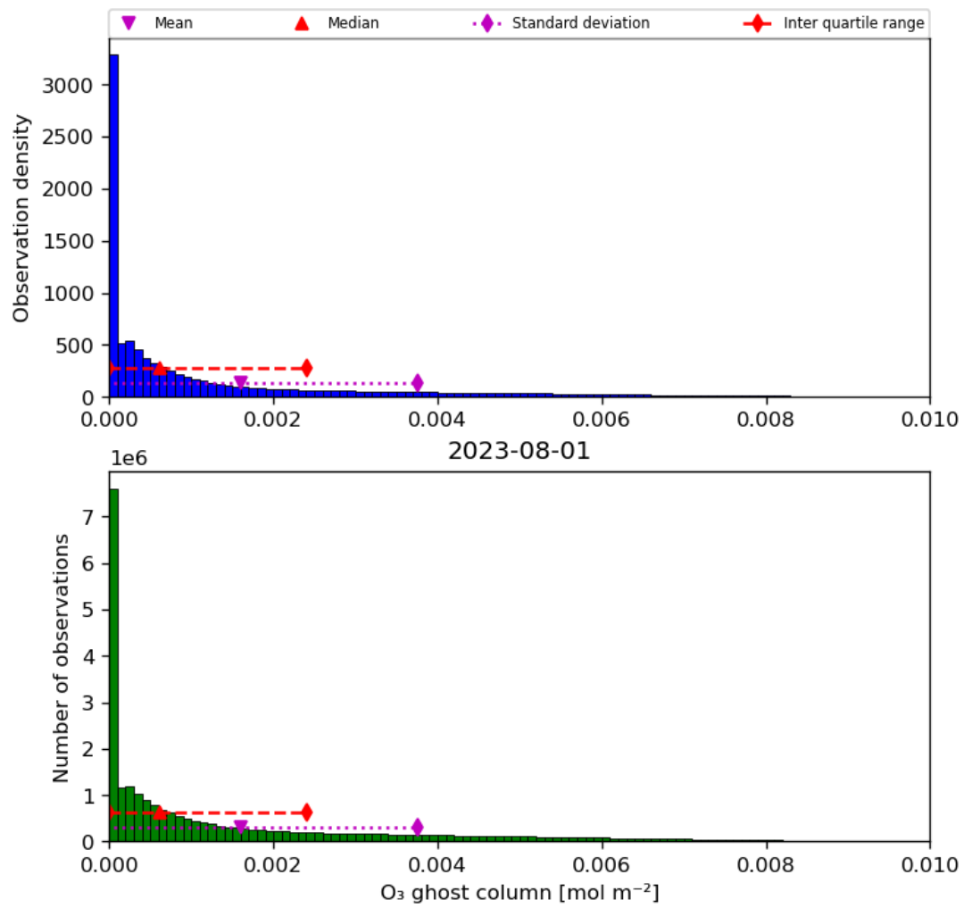
Figure 25: Histogram of “O 3 ghost column” for 2023-07-31 to 2023-08-02
