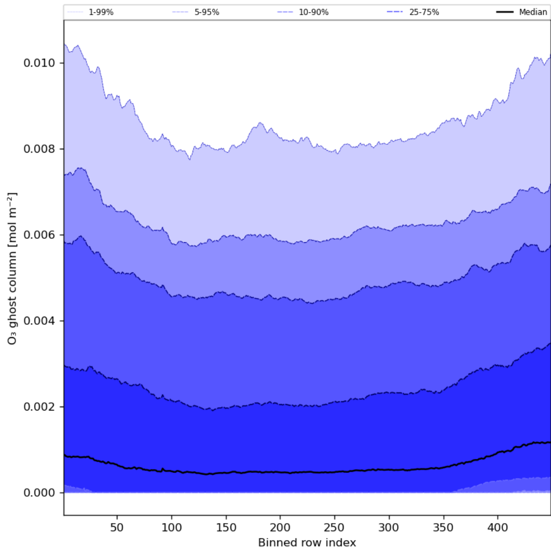
Figure 32: Along track statistics of “O 3 ghost column” for 2023-07-31 to 2023-08-02
