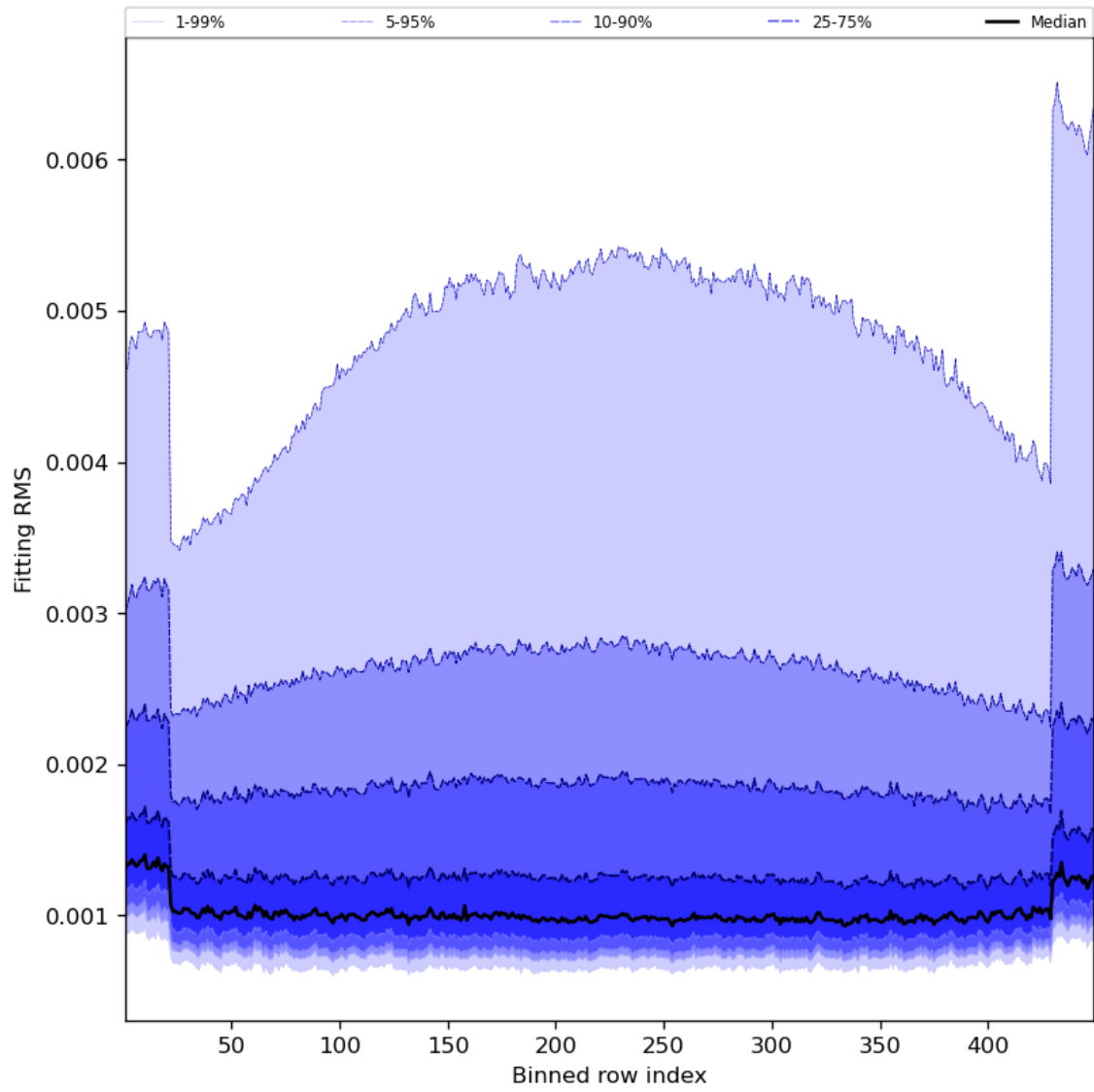
Figure 30: Along track statistics of “Fitting RMS” for 2023-07-31 to 2023-08-02
