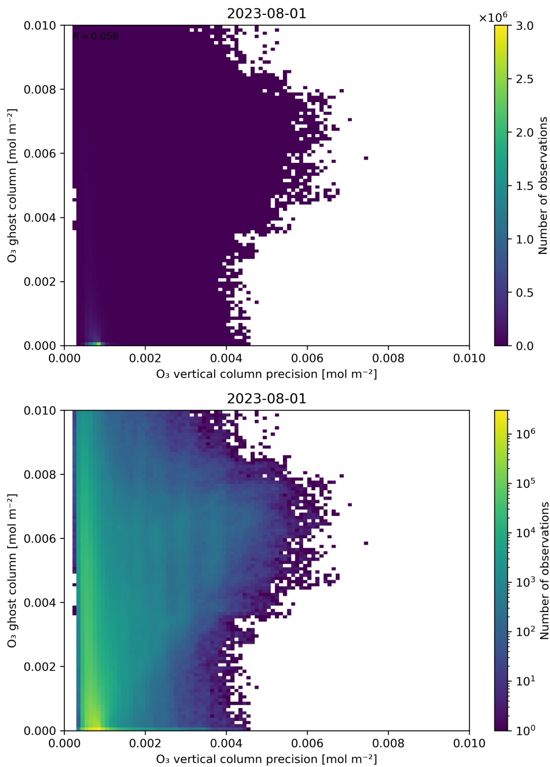
Figure 43: Scatter density plot of “O 3 vertical column precision” against “O 3 ghost column” for 2023-07-31 to 2023-08-02.
