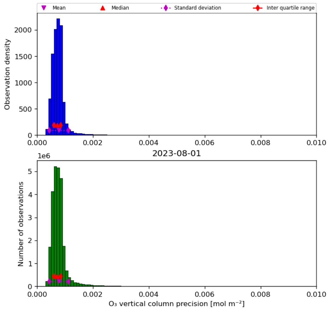
Figure 22: Histogram of “O 3 vertical column precision” for 2023-07-31 to 2023-08-02
