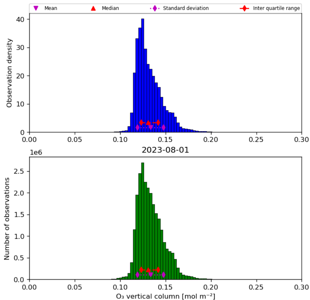
Figure 21: Histogram of “O 3 vertical column” for 2023-07-31 to 2023-08-02
