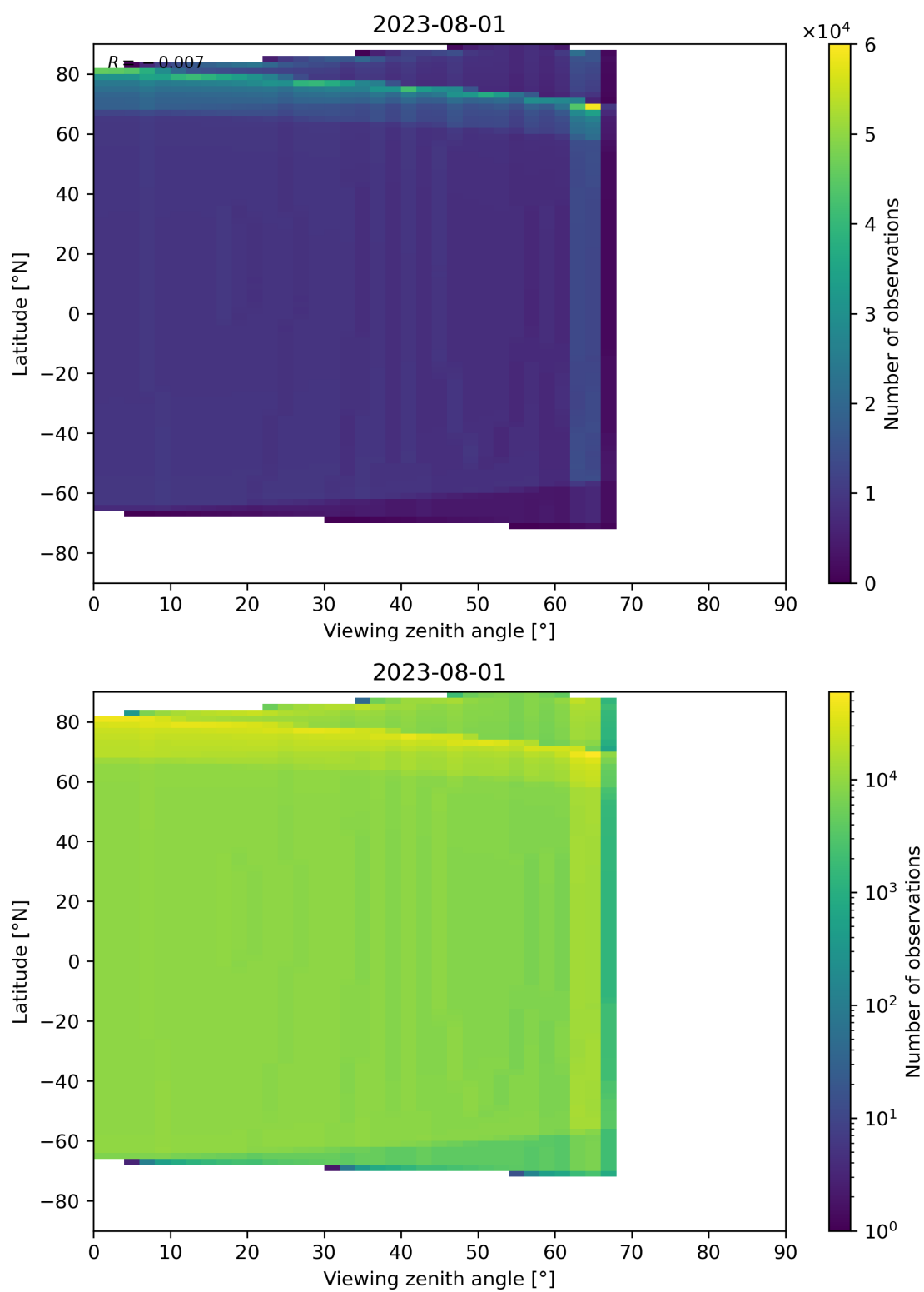
Figure 49: Scatter density plot of “Viewing zenith angle” against “Latitude” for 2023-07-31 to 2023-08-02.
