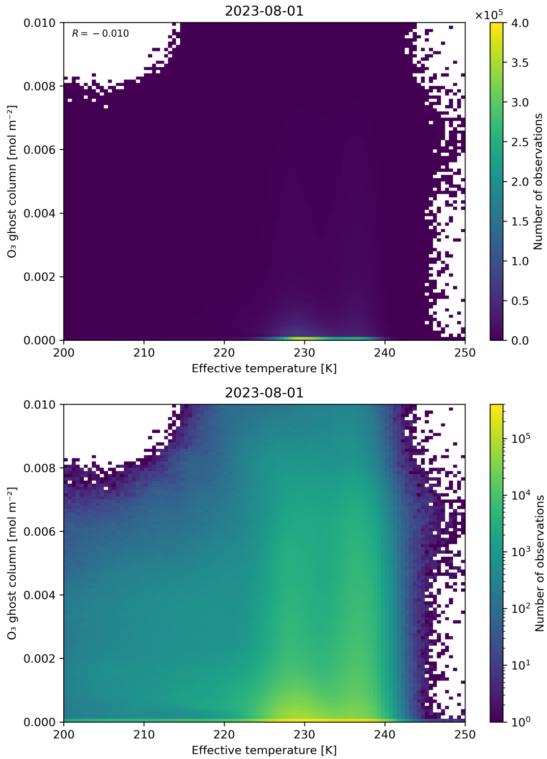
Figure 38: Scatter density plot of “Effective temperature” against “O 3 ghost column” for 2023-07-31 to 2023-08-02.
