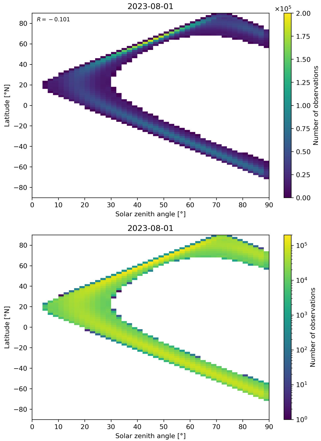
Figure 44: Scatter density plot of “Solar zenith angle” against “Latitude” for 2023-07-31 to 2023-08-02.
