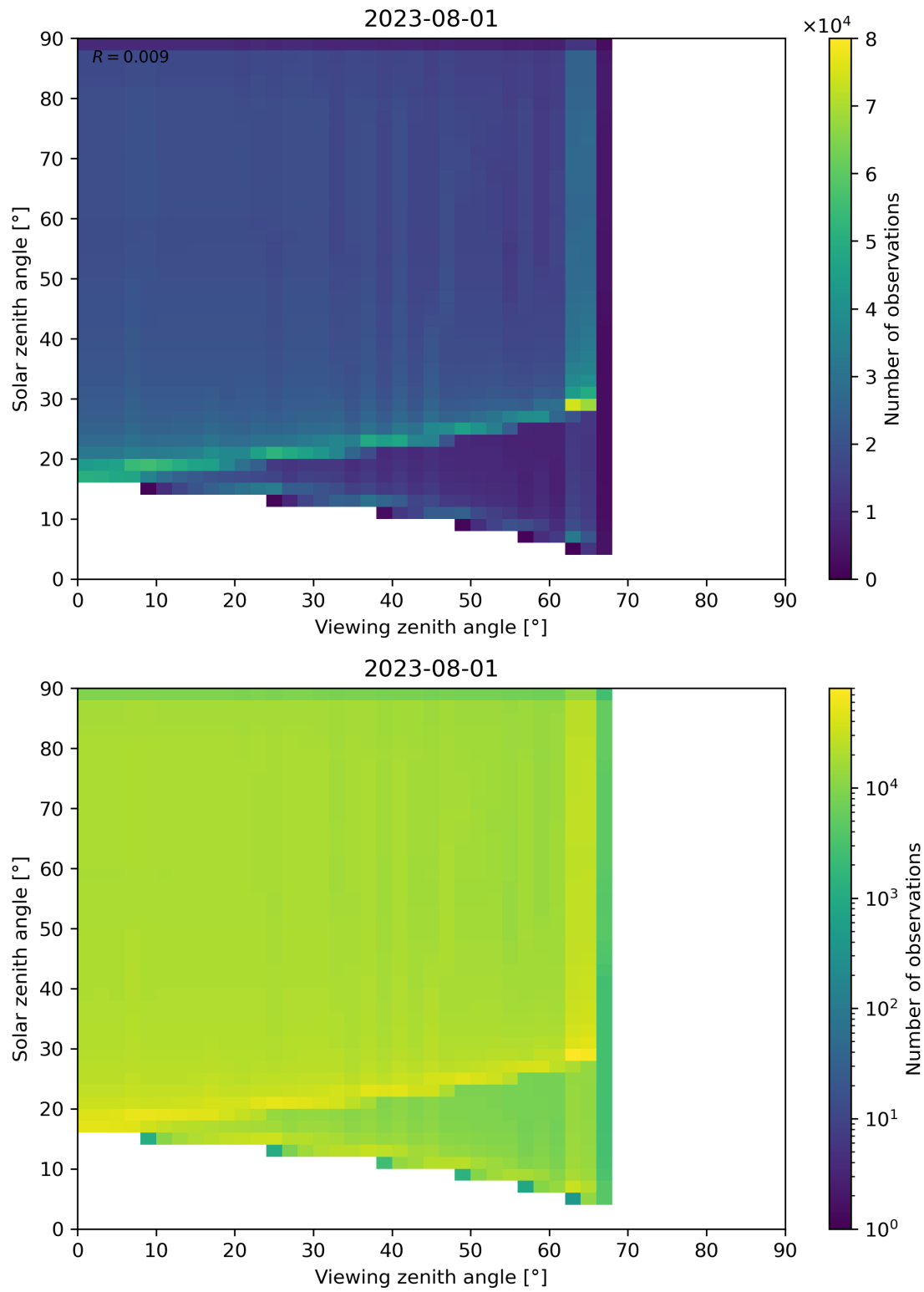
Figure 54: Scatter density plot of “Viewing zenith angle” against “Solar zenith angle” for 2023-07-31 to 2023-08-02.
