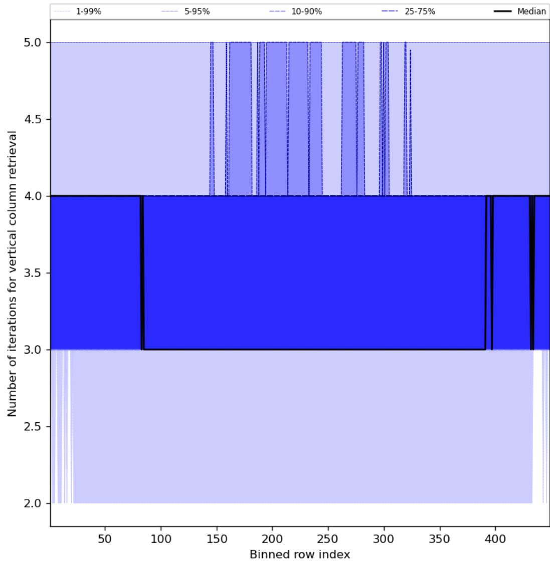
Figure 33: Along track statistics of “Number of iterations for vertical column retrieval” for 2023-07-31 to 2023-08-02
