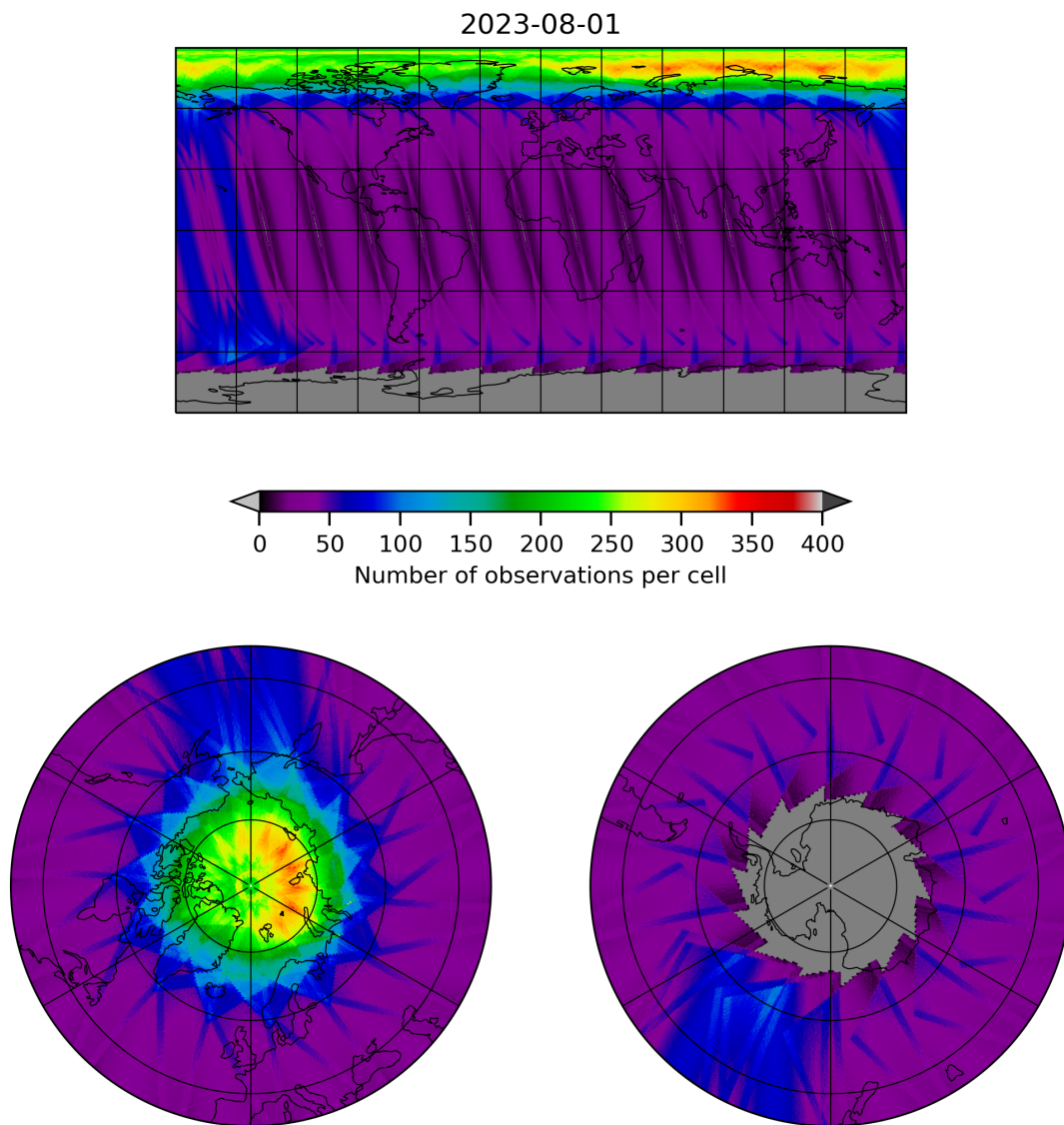
Figure 12: Map of the number of observations for 2023-07-31 to 2023-08-02
