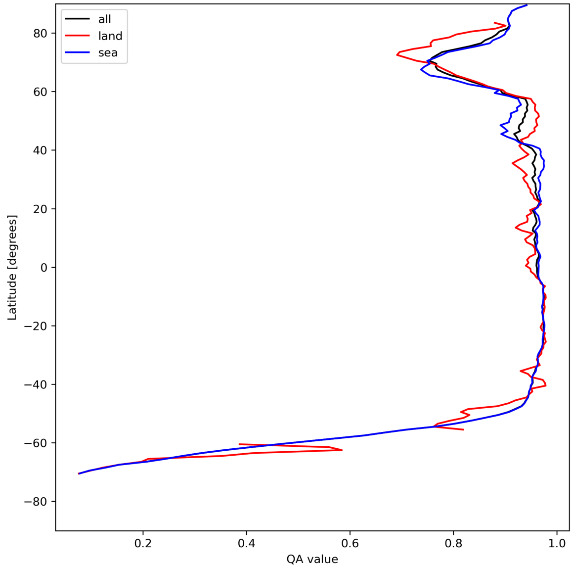
Figure 13: Zonal average of “QA value” for 2023-07-31 to 2023-08-02.
