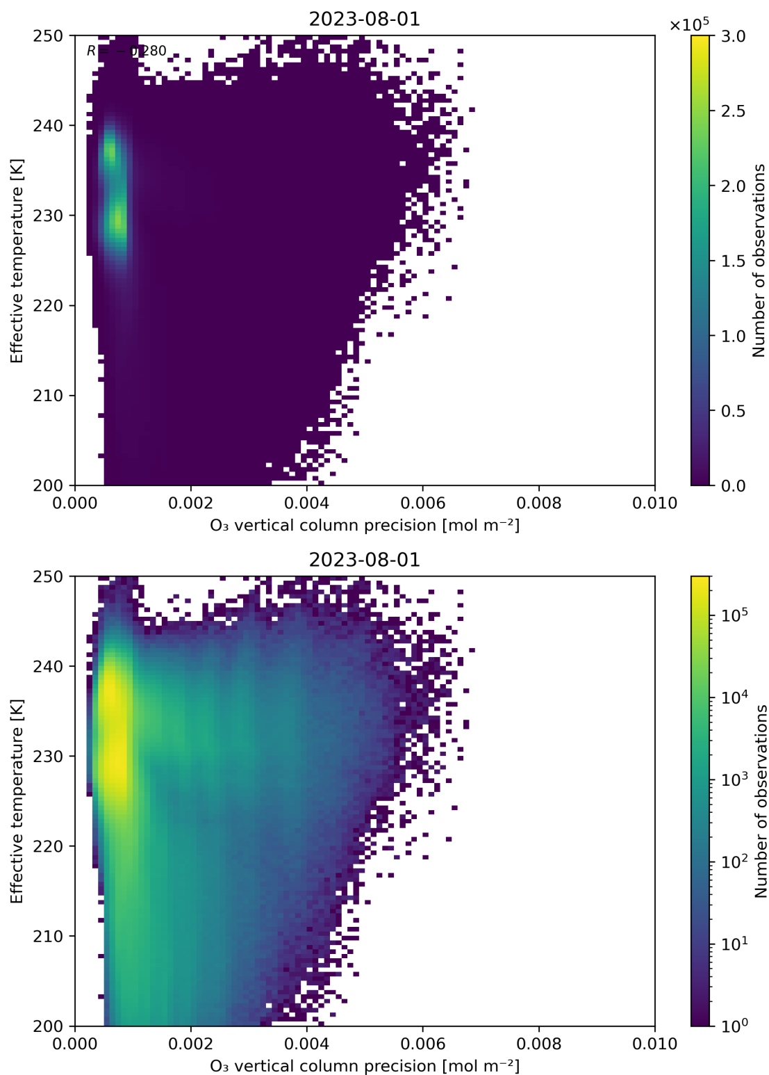
Figure 42: Scatter density plot of “O 3 vertical column precision” against “Effective temperature” for 2023-07-31 to 2023-08-02.
