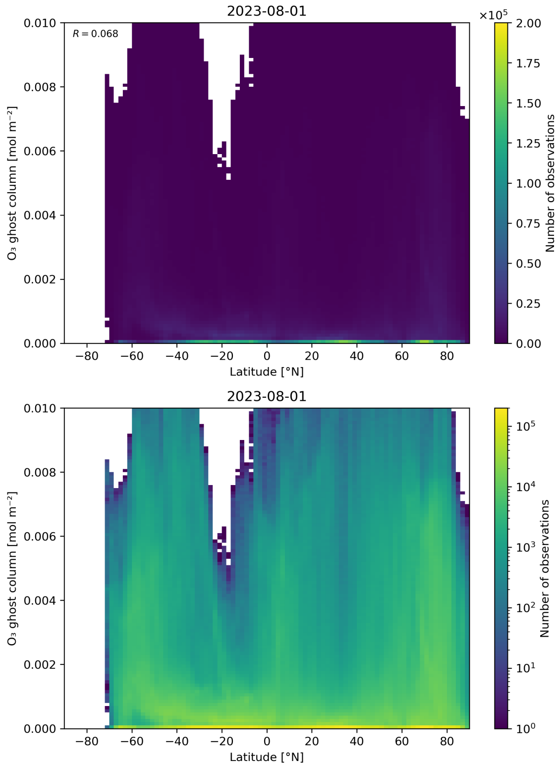
Figure 35: Scatter density plot of “Latitude” against “O 3 ghost column” for 2023-07-31 to 2023-08-02.
