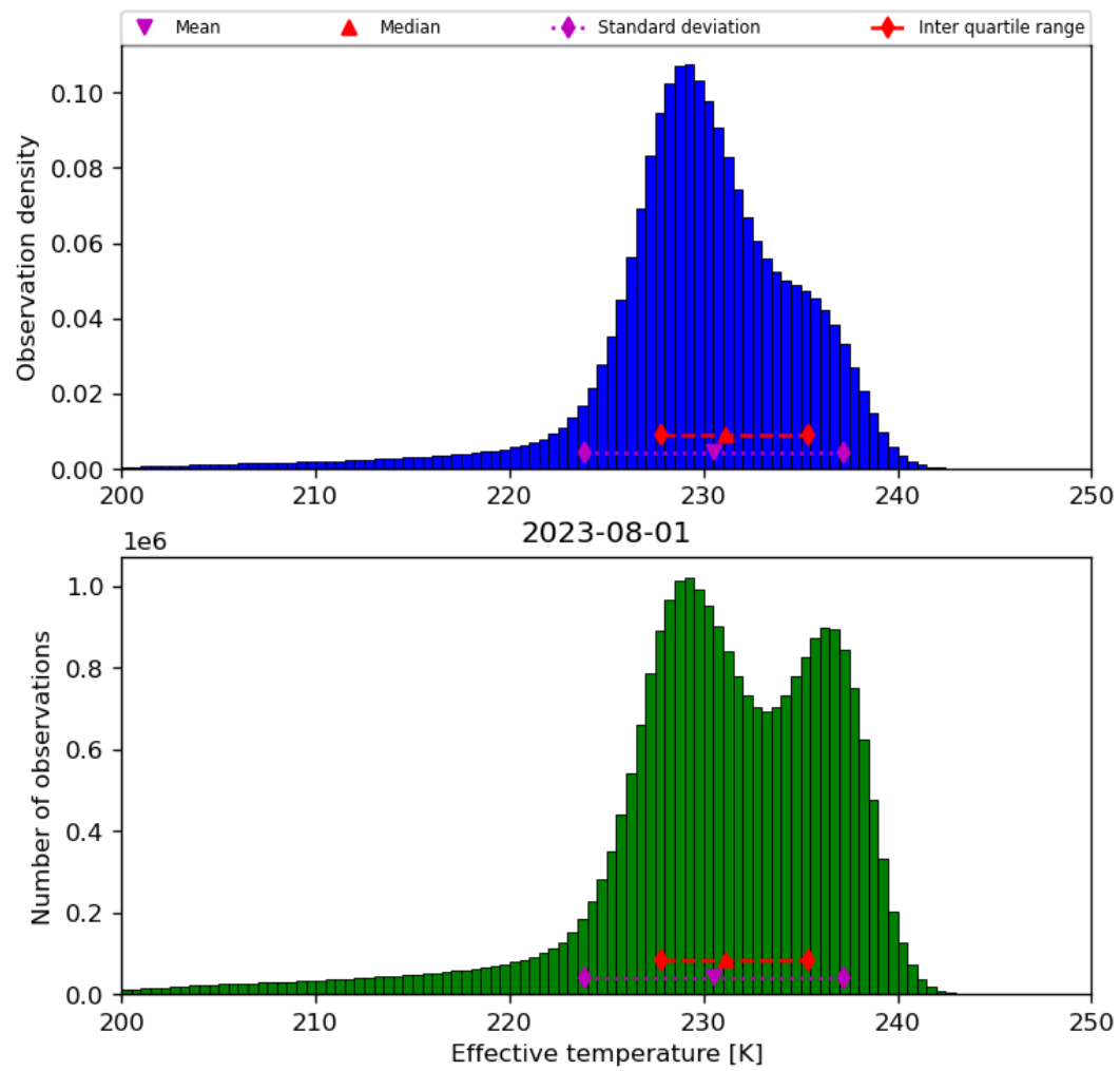
Figure 24: Histogram of “Effective temperature” for 2023-07-31 to 2023-08-02
