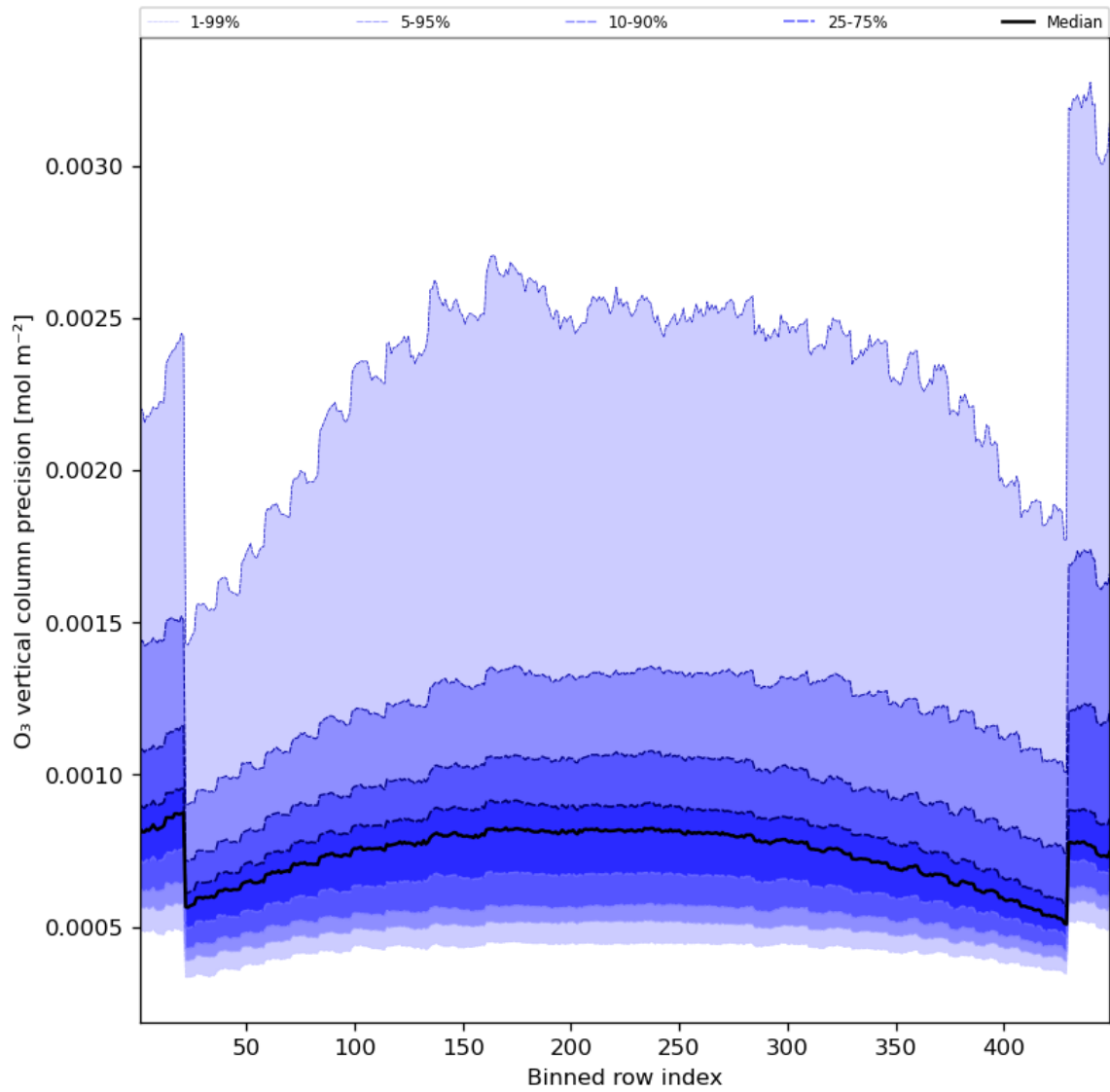
Figure 29: Along track statistics of “O 3 vertical column precision” for 2023-07-31 to 2023-08-02
