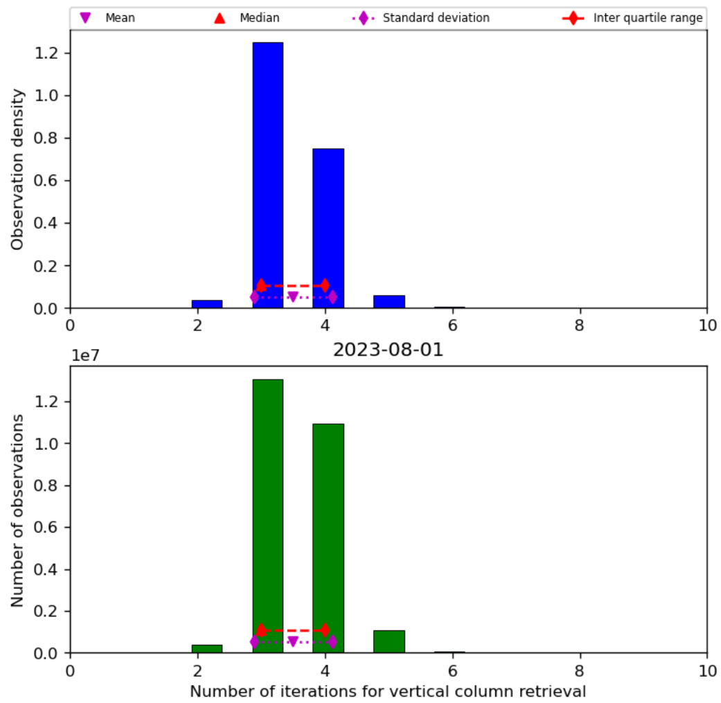
Figure 26: Histogram of “Number of iterations for vertical column retrieval” for 2023-07-31 to 2023-08-02
