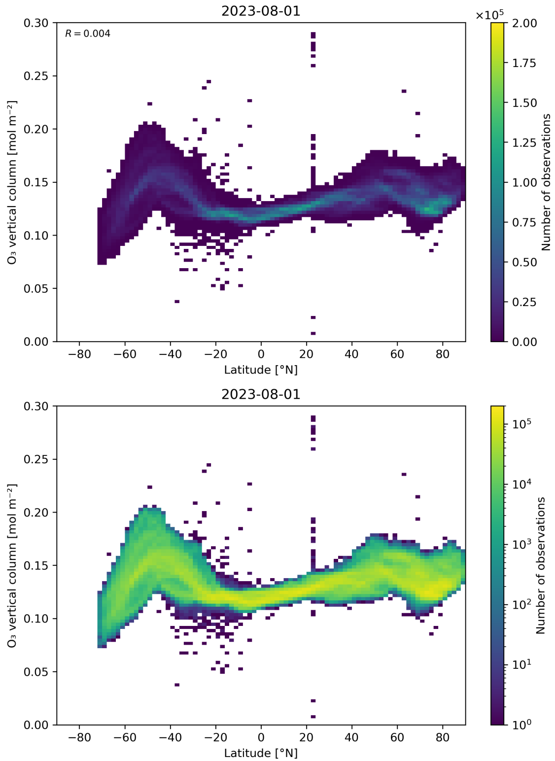
Figure 36: Scatter density plot of “Latitude” against “O 3 vertical column” for 2023-07-31 to 2023-08-02.
