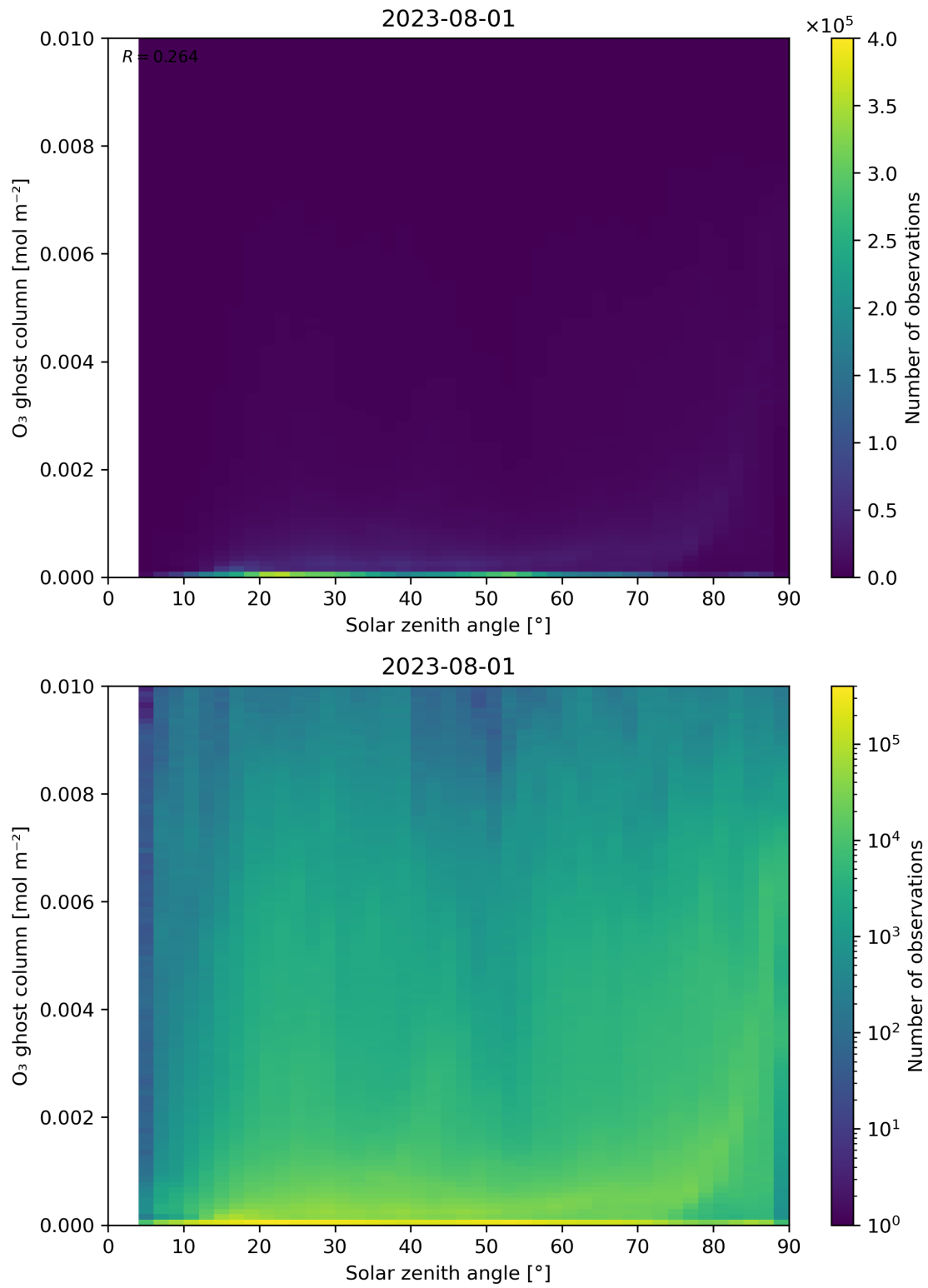
Figure 46: Scatter density plot of “Solar zenith angle” against “O 3 ghost column” for 2023-07-31 to 2023-08-02.
