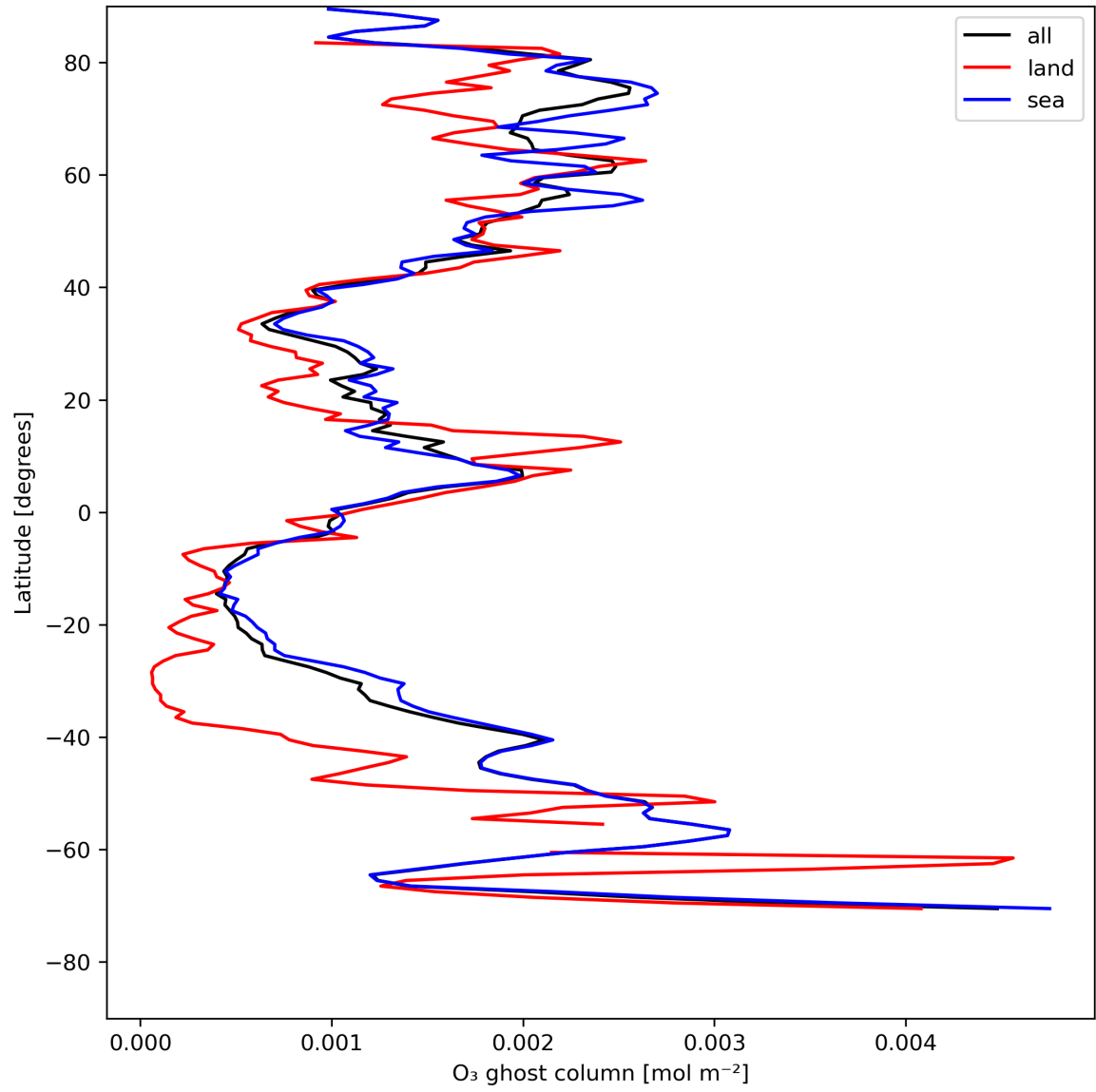
Figure 18: Zonal average of “O 3 ghost column” for 2023-07-31 to 2023-08-02.
