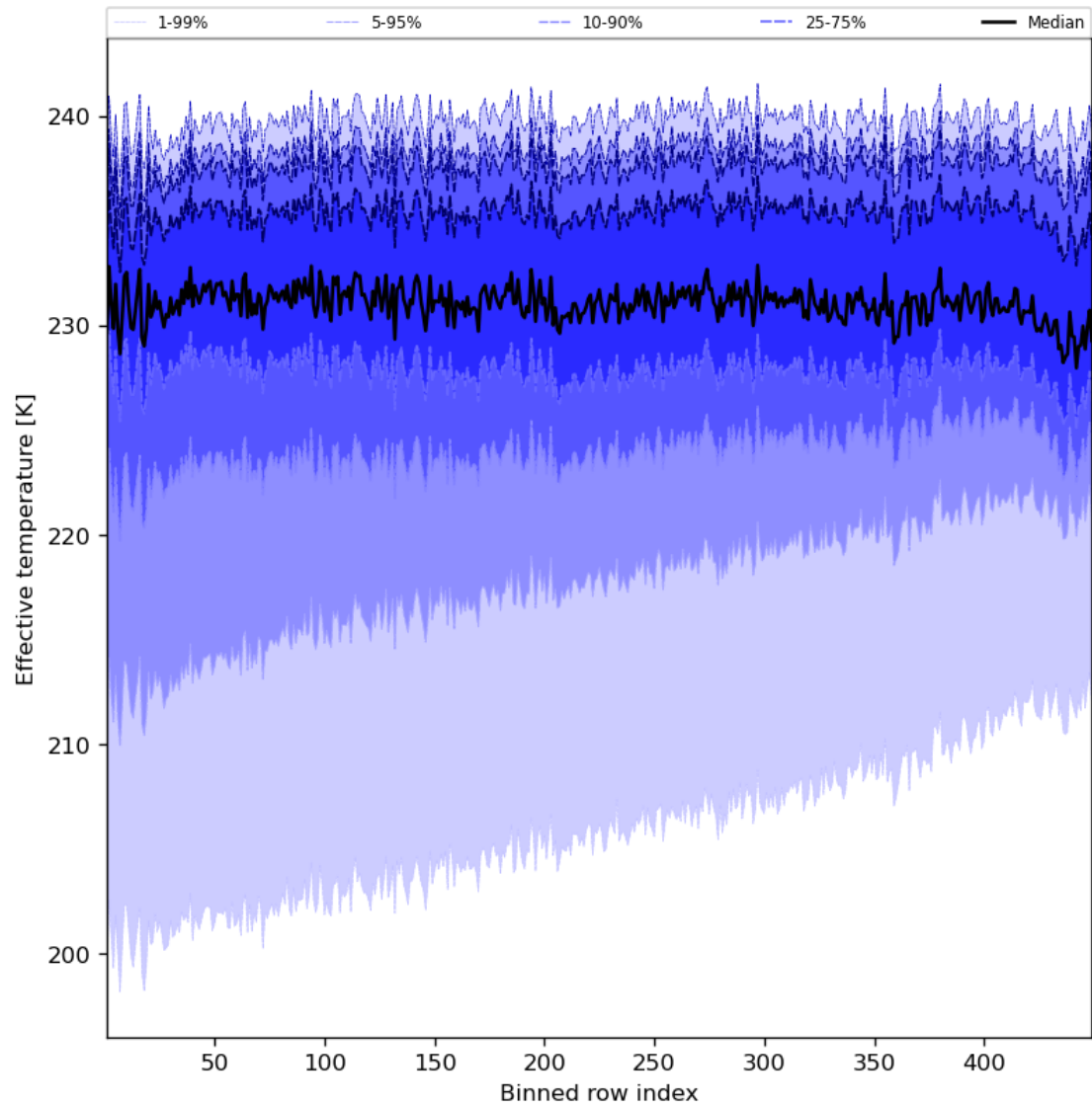
Figure 31: Along track statistics of “Effective temperature” for 2023-07-31 to 2023-08-02
