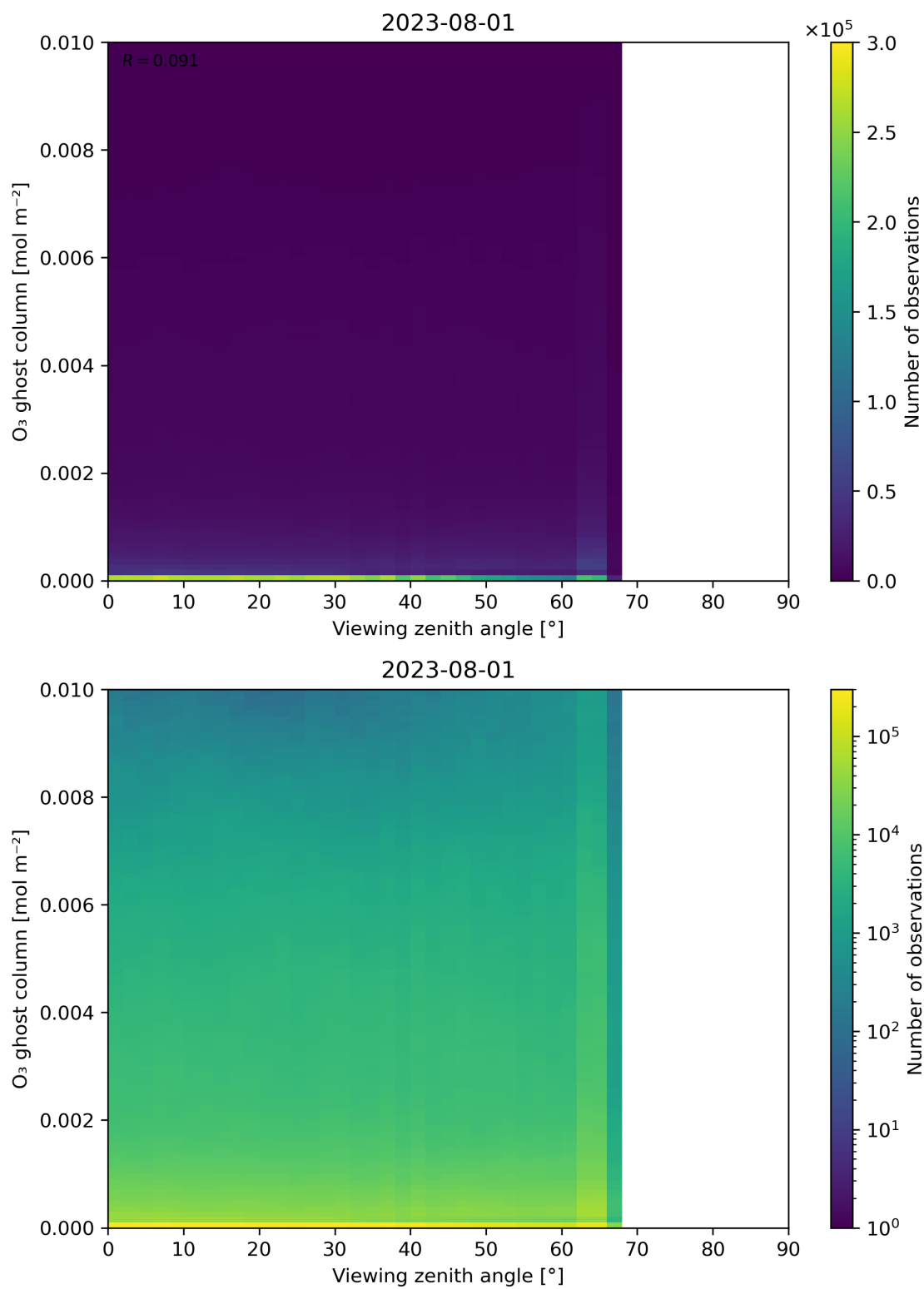
Figure 51: Scatter density plot of “Viewing zenith angle” against “O 3 ghost column” for 2023-07-31 to 2023-08-02.
