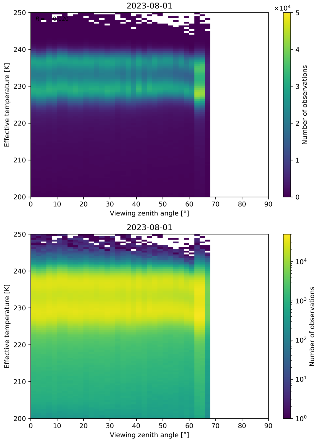
Figure 50: Scatter density plot of “Viewing zenith angle” against “Effective temperature” for 2023-07-31 to 2023-08-02.
