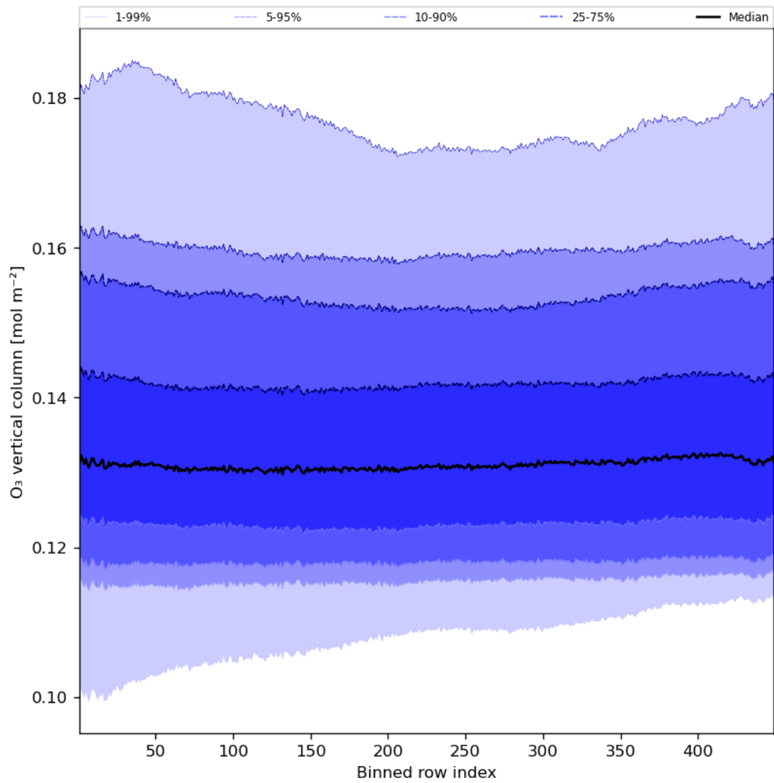
Figure 28: Along track statistics of “O 3 vertical column” for 2023-07-31 to 2023-08-02
